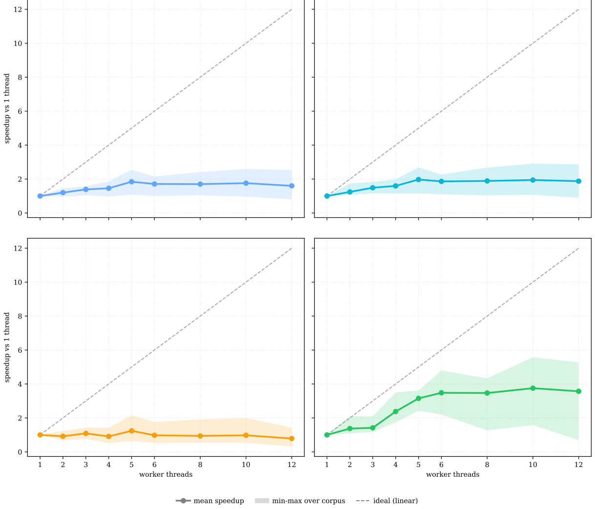
Figure 3: Thread scaling per solver, 1–12 workers, mean with min–max band over the corpus.
