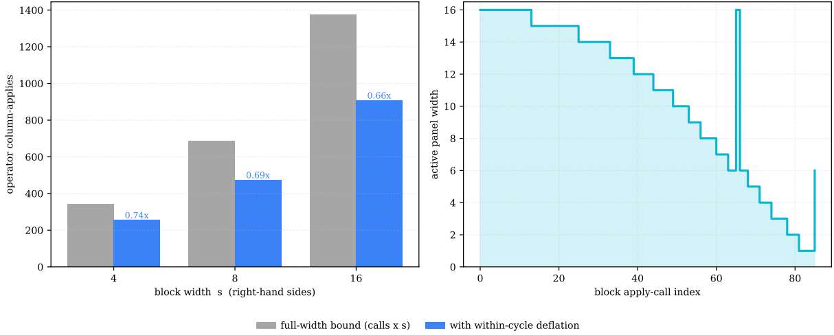
Figure 6: Block-GMRES within-cycle deflation. Left: total operator column-applies with mid-cycle compaction vs. the full-width bound ( \text{calls} \times s ), per block width. Right: the active-panel width per batched apply for s = 16 — the panel drains as columns converge, then refills briefly at the once-per-cycle full-width residual check. Multi-rate diagonal testbed, n = 20\,000 .
