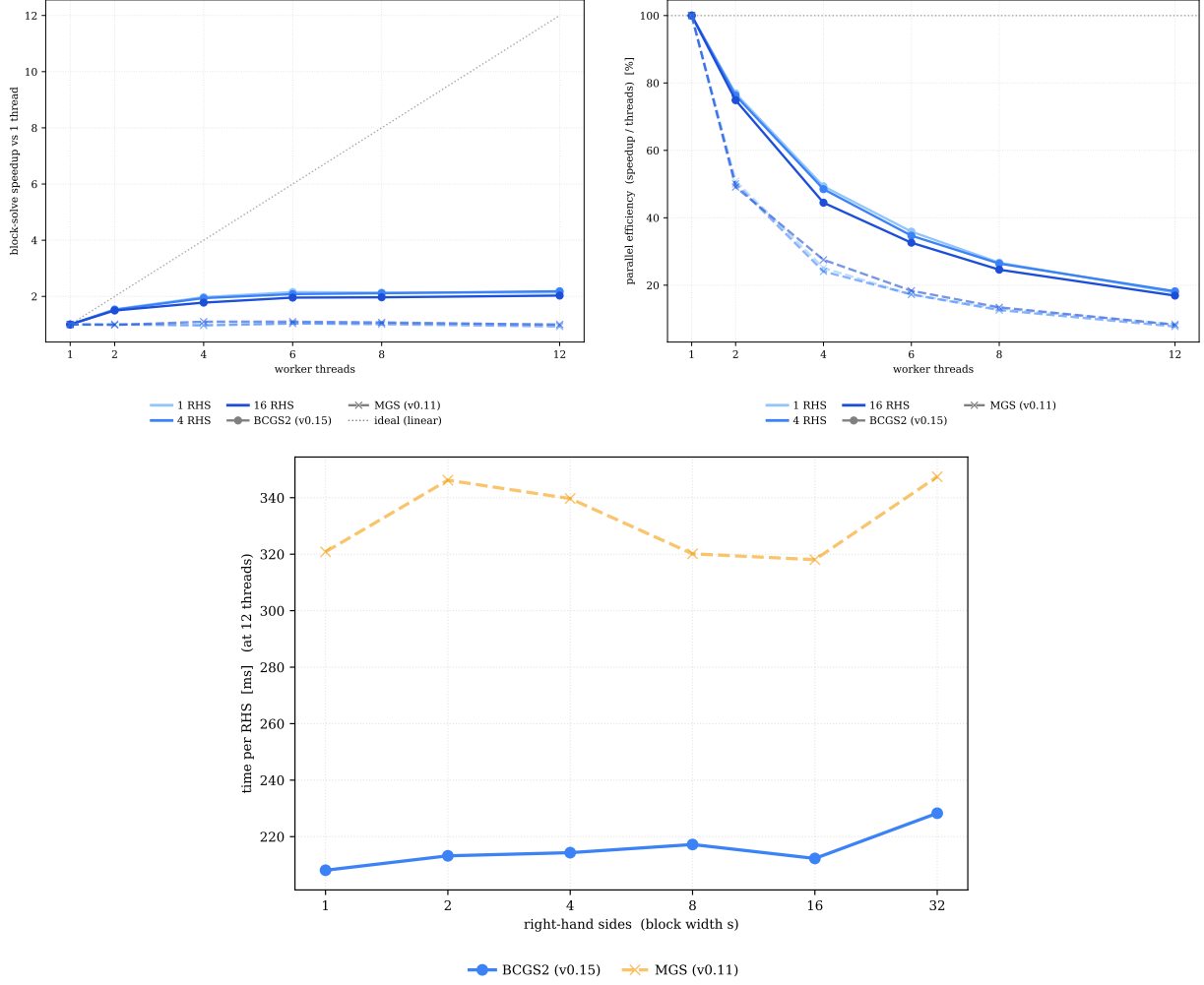
Figure 5: Multi-RHS block GMRES, BCGS2 (v0.15, solid) vs. the pre-BCGS2 per-RHS MGS (v0.11, dashed). Left: strong-scaling speedup vs. threads per block width. Right: parallel efficiency. Bottom: per-RHS cost vs. block width at 12 threads. Preconditioned convection–diffusion, n = 40\,000 , complex \mathbf{f64} .
