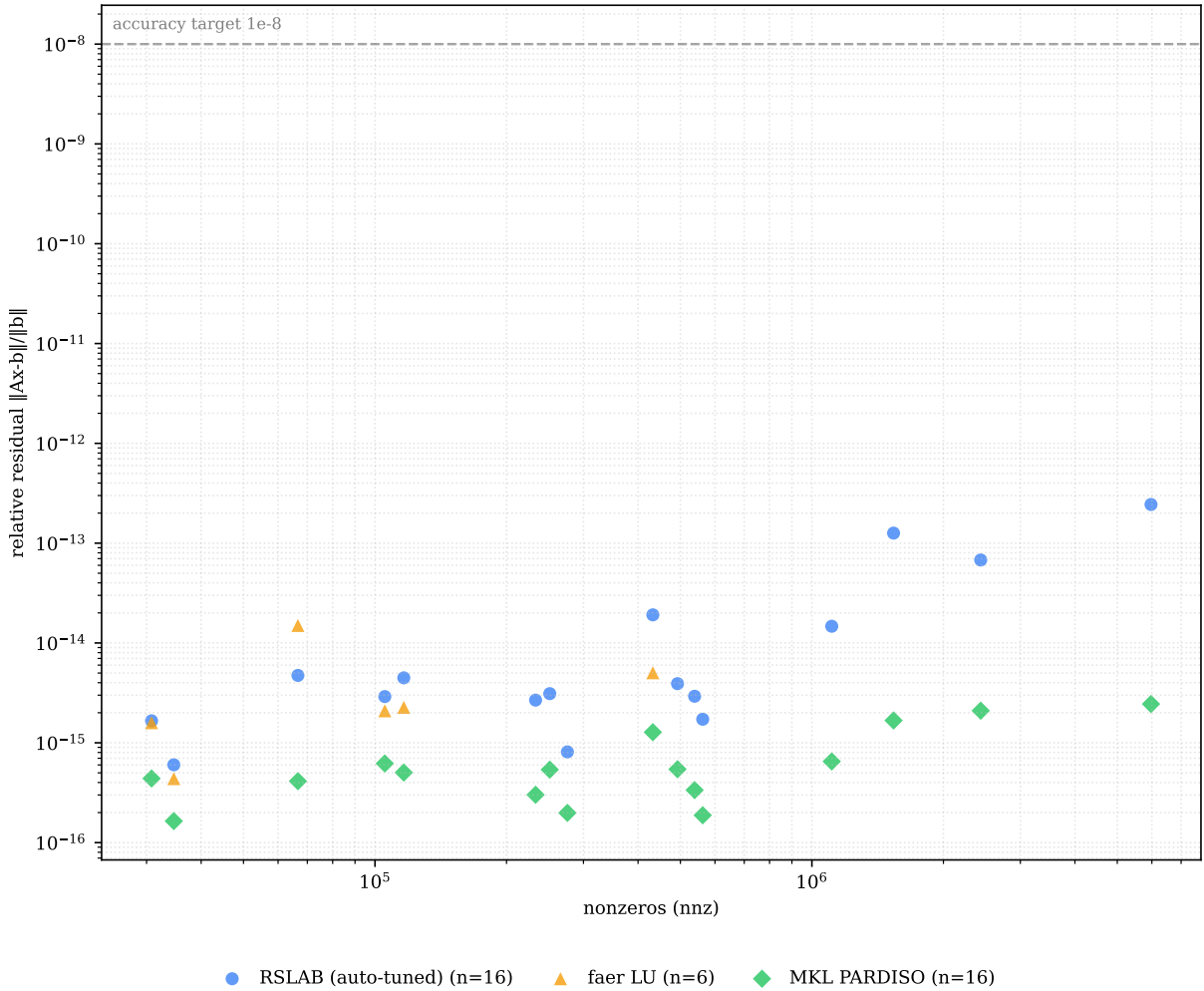
Figure 11: Relative residual across the corpus, per solver.
