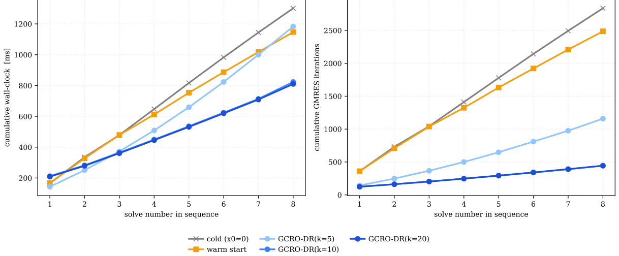
Figure 12: GCRO-DR subspace recycling over a sequence of 8 related solves (stagnation spectrum, n = 20\,000 ). Left: cumulative wall-clock; right: cumulative GMRES iterations, for cold, warm, and GCRO-DR( k ). Recycling cuts the cross-solve iteration total 6.4\times versus cold ( k=20 overlaps k=10 , the m/2 cap).
