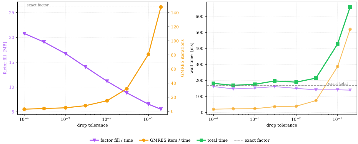
Figure 8: Incomplete-factor preconditioner + GMRES. Left: factor fill (memory) and GMRES iterations vs. drop_tol , with the exact factor as reference. Right: factor / GMRES / total wall time, exposing the sweet spot. Convection–diffusion, n = 32\,400 , complex f64 .
