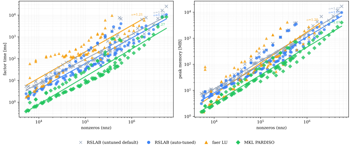
Figure 9: LU path (unsymmetric, PARDISO mtype 13): (left) factor wall-clock time and (right) peak memory vs. problem size. Each panel carries the untuned-default RSLAB curve (gray) beside the auto-tuned one (blue); the tuner closes part of the default→PARDISO distance. On time RSLAB scales slightly flatter than PARDISO ( \alpha \approx 1.18 vs. 1.27).
