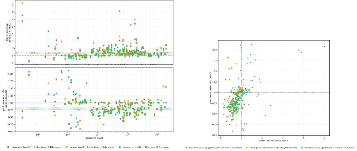
Figure 4: \text{LDL}^\top tuner vs. untuned default over 167 matrices: speedup and memory ratio by problem size (left), and the three Pareto modes as a time–memory cloud (right).
