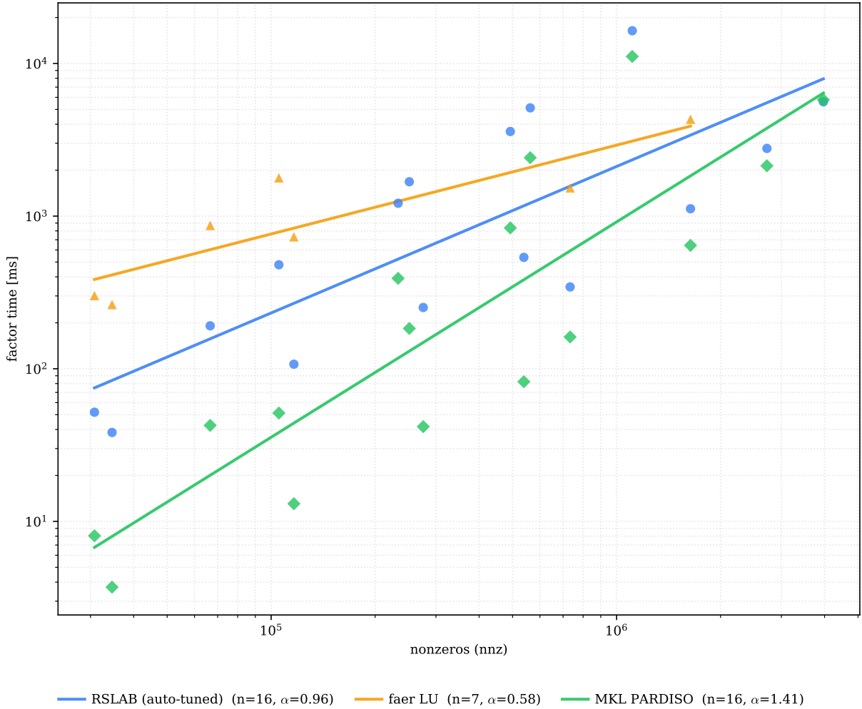
Figure 6: Corpus scaling of factor time vs. problem size, with power-law fits.
