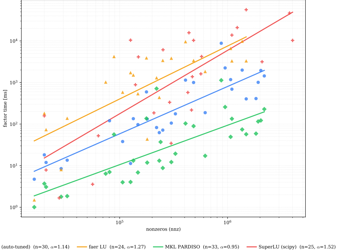
Figure 6: Corpus scaling of factor time vs. problem size, with power-law fits.
