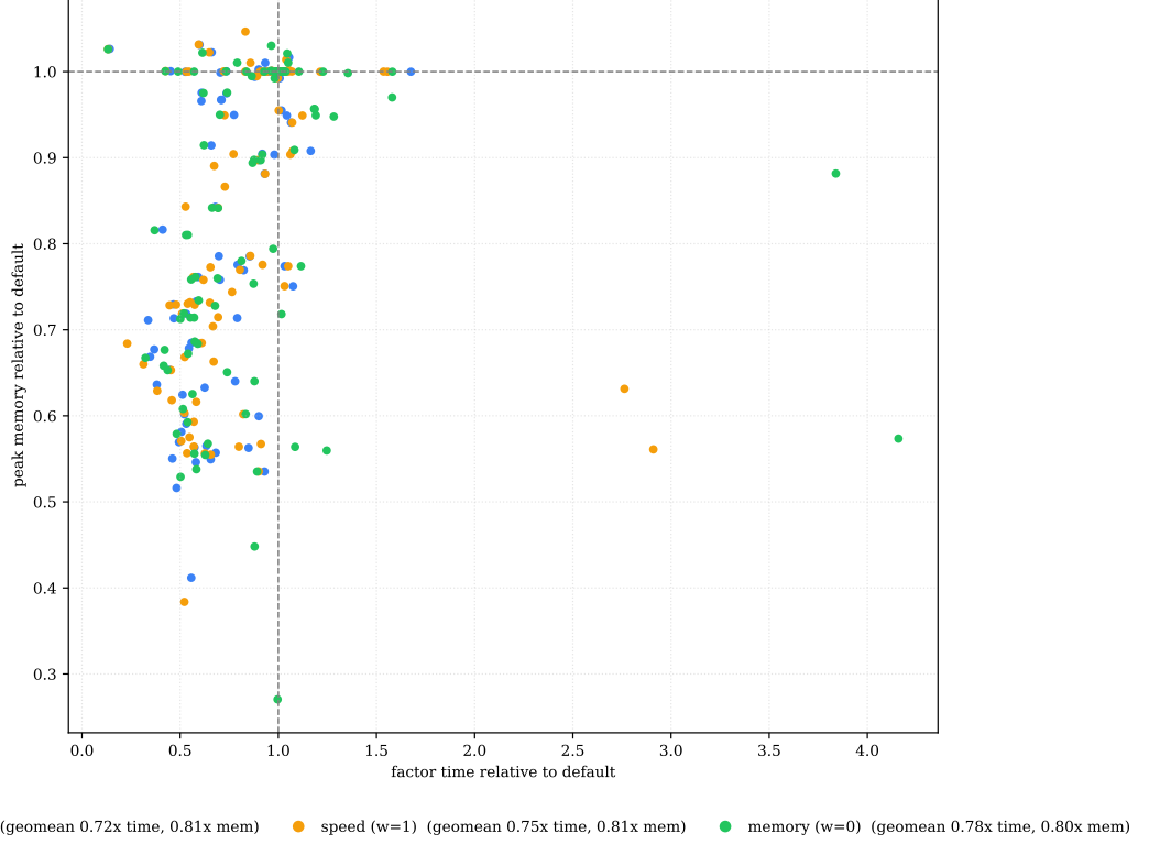
Figure 5: The tuner’s three Pareto modes as a time–memory cloud relative to the untuned default.
