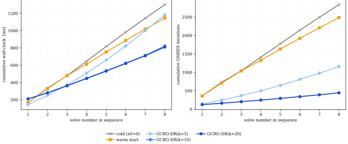
Figure 9: A sequence of eight related solves: cumulative wall-clock (left) and cumulative GMRES iterations (right), cold start vs. warm start vs. GCRO-DR recycling at three subspace sizes.
