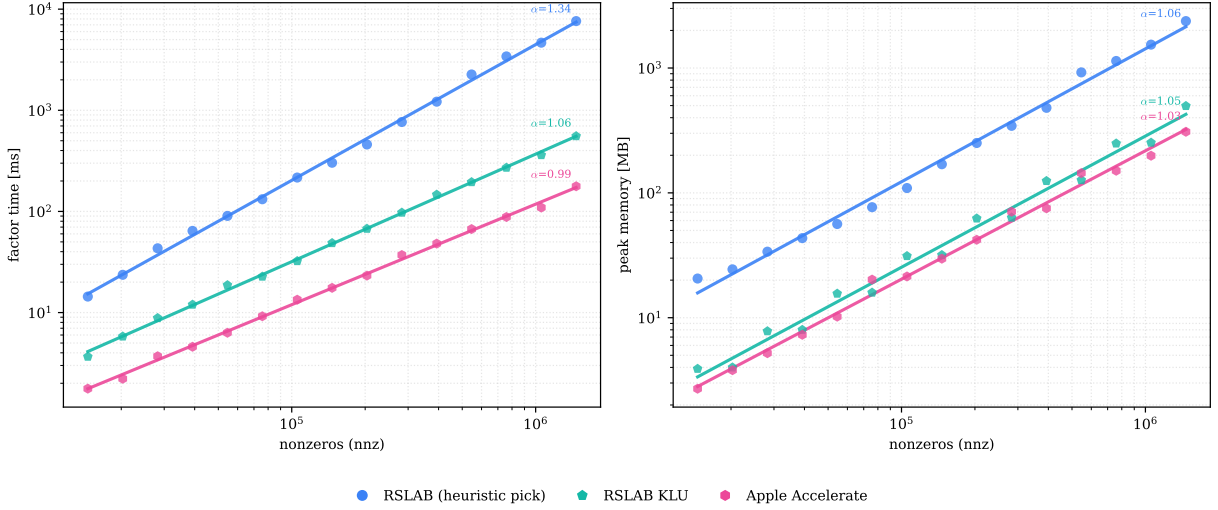
Figure 7: Apple M3: circuit-shaped matrices (complex MNA, G + j\omega C ). RSLAB KLU vs. the multifrontal LU default vs. Accelerate LU; one-shot factor — KLU’s refactor-driven sweep niche is not exercised here.
