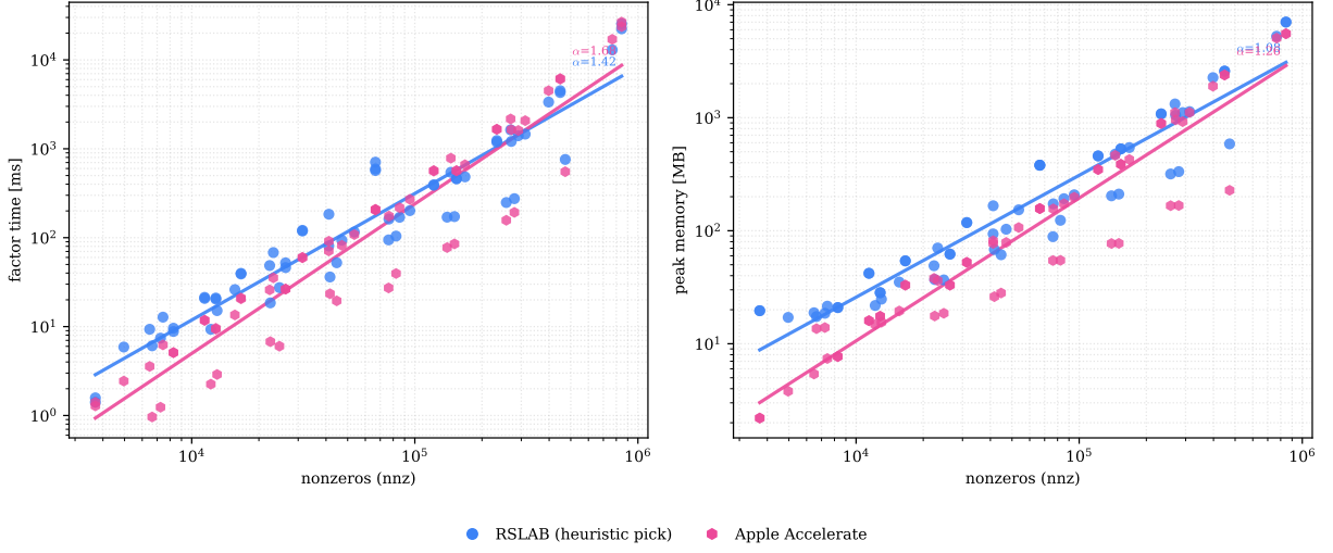
Figure 5: Apple M3: \text{LDL}^\top path (complex-symmetric + real-symmetric families) — factor wall-clock (left) and live-bytes peak (right) vs. problem size, RSLAB shipped pick vs. Apple Accelerate (vendor-best configuration), with power-law fits.
