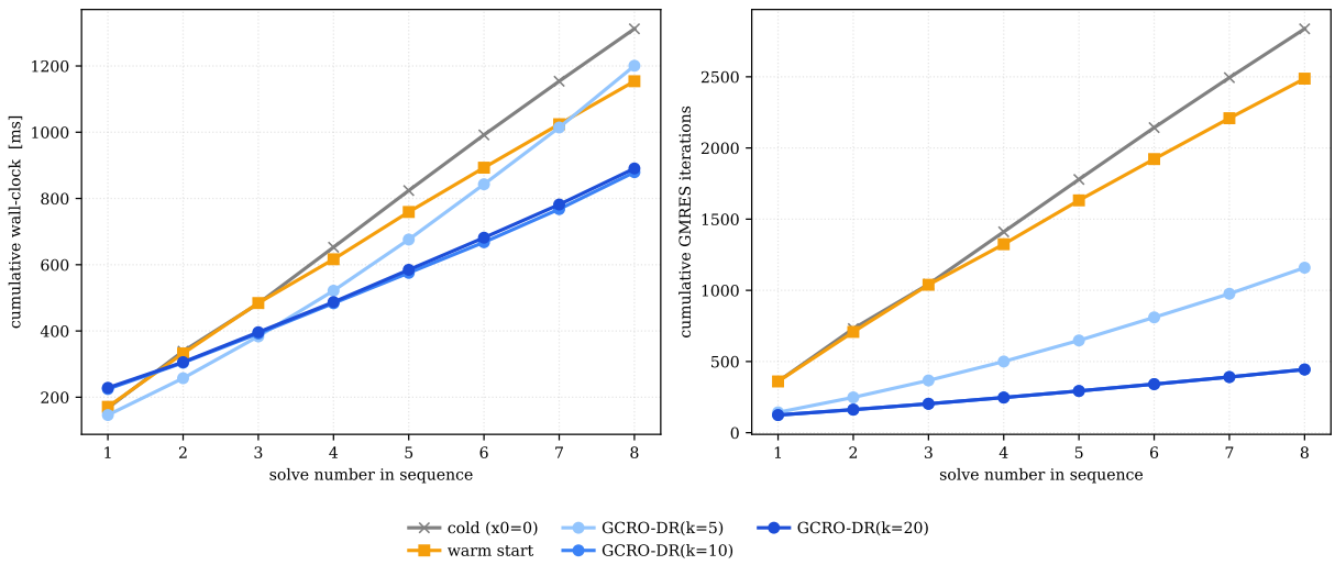
Figure 13: GCRO-DR subspace recycling over a sequence of 8 related solves (stagnation spectrum, n = 20000 ). Left: cumulative wall-clock; right: cumulative GMRES iterations, for cold, warm, and GCRO-DR( k ). Recycling cuts the cross-solve iteration total 6.4\times versus cold ( k=20 overlaps k=10 , the m/2 cap).
