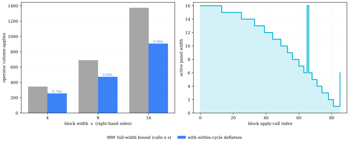
Figure 7: Block-GMRES within-cycle deflation. Left: total operator column-applies with mid-cycle compaction vs. the full-width bound ( \text{calls} \times s ), per block width. Right: the active-panel width per batched apply for s = 16 — the panel drains as columns converge, then refills briefly at the once-per-cycle full-width residual check. Multi-rate diagonal testbed, n = 20\,000 .
