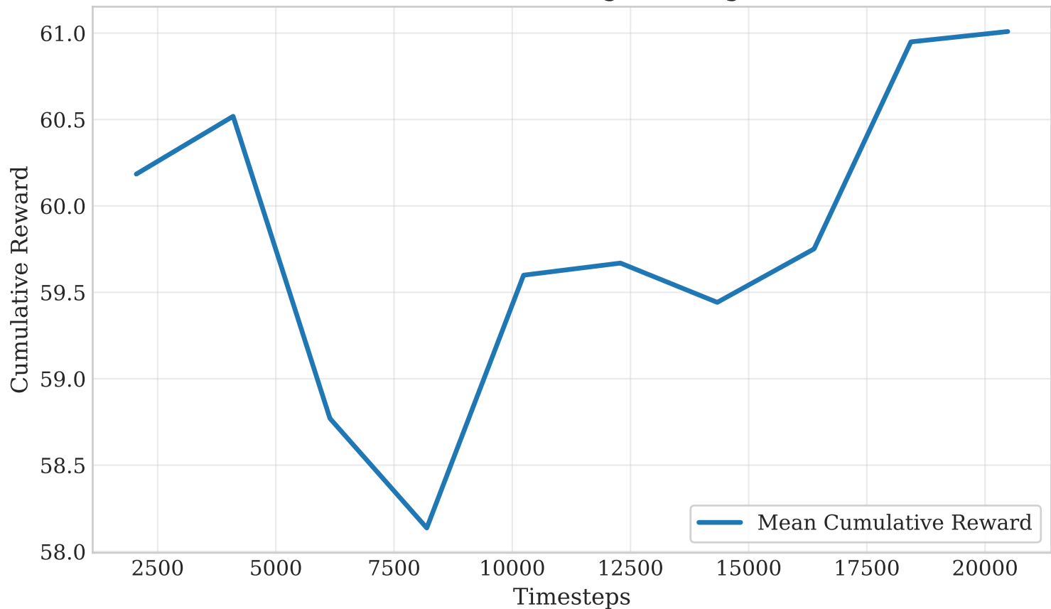
PPO Offline Training Convergence
