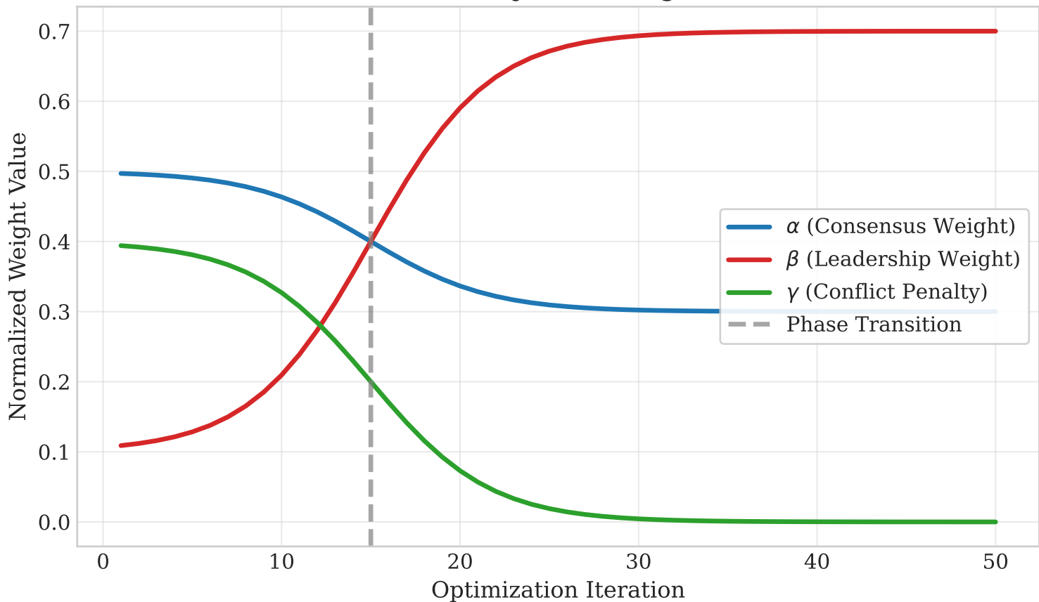
RL Controller: Objective Weight Evolution
