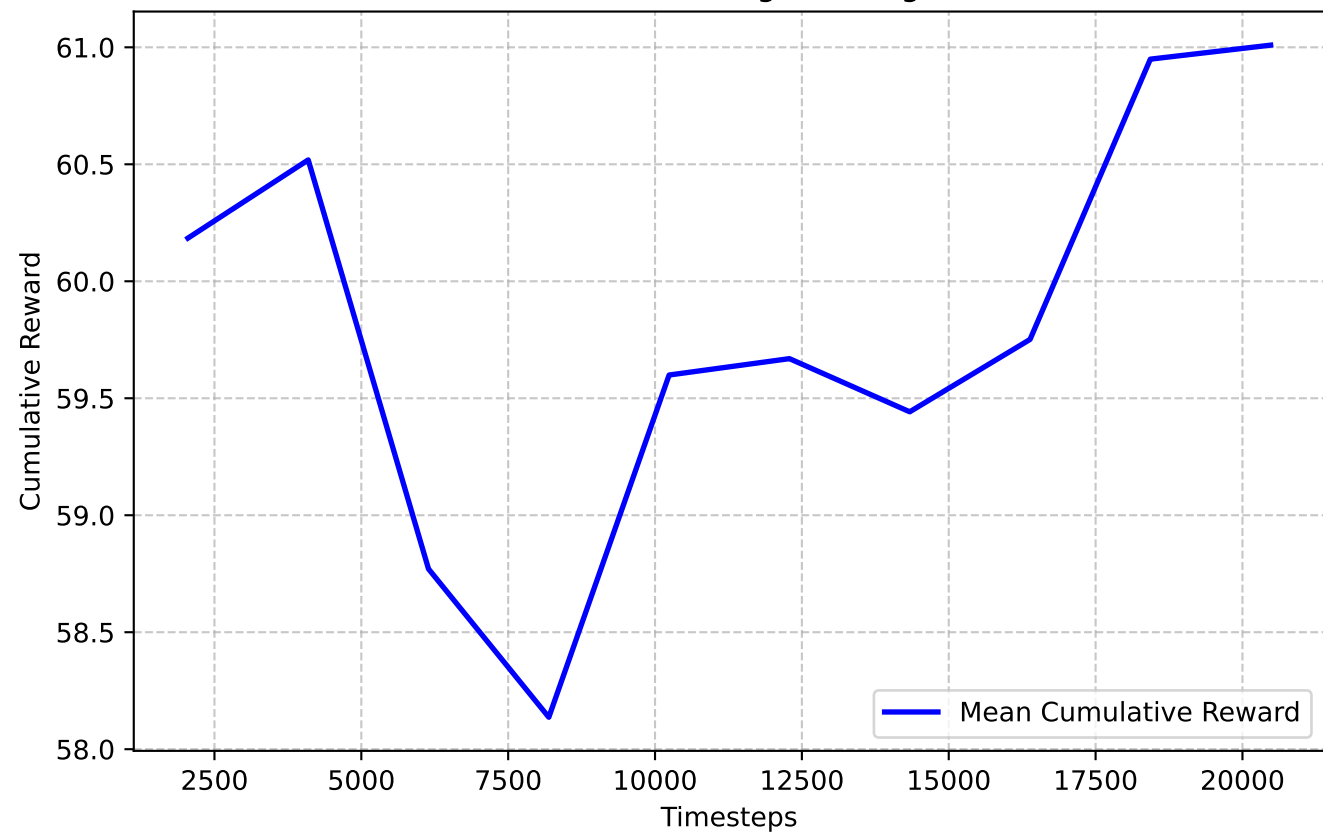
PPO Offline Training Convergence
