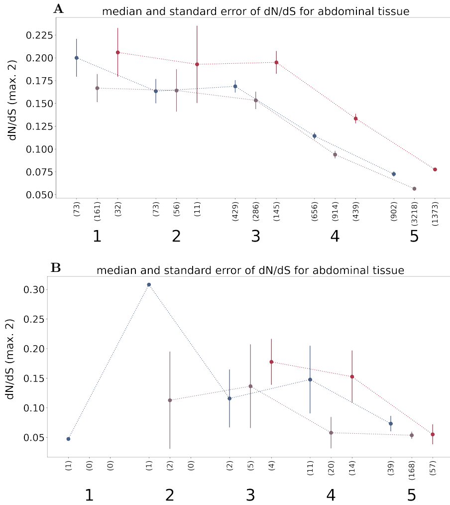
Figure 4: Impact of gene age and sex-bias on dN/dS and positively selected genes: X-axes ticks show sample size in parentheses, as well as gene age from less conserved orthologs (age 1) to highly conserved orthologs (age 5), or autosomal or X-linkage of orthologs (A or X). ( A,B ): median dN/dS and standard error of autosomal orthologs, split by gene age as well as sex-bias category according to abdominal tissues with male-bias being blue, unbiased being grey and female-bias being red. ( A ): autosomal, ( B ): X-linked.
