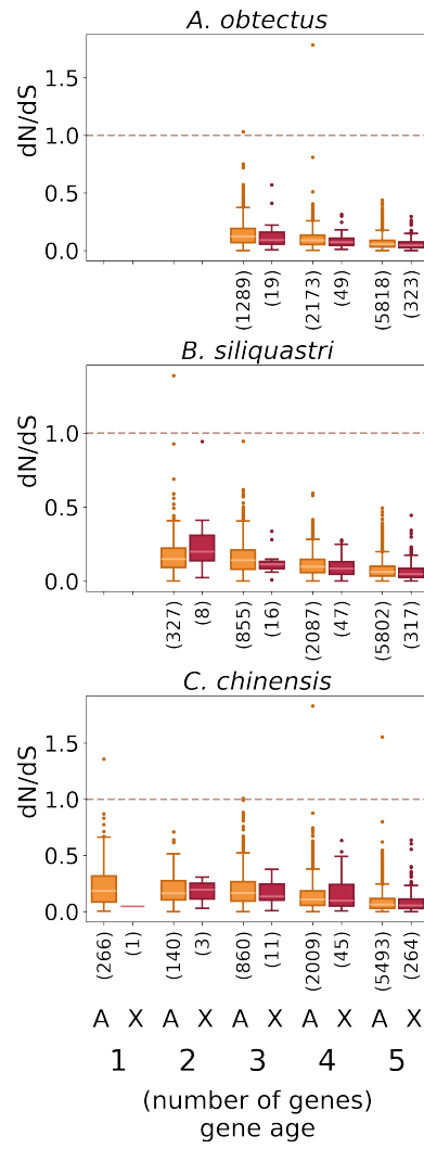
Figure 2: Gene age: Pairwise comparisons of C. maculatus with A. obtectus , B. siliquastri and C. chinensis respectively. The X-axis shows sample size in parentheses, as well as gene age (less conserved orthologs of age 1 to most conserved orthologs of age 5), and autosomal or X-linkage of orthologs (A or X). The box plots show dN/dS for autosomal (yellow) or X-linked (red) orthologs by gene age for C. maculatus compared to three other Bruchini species.
