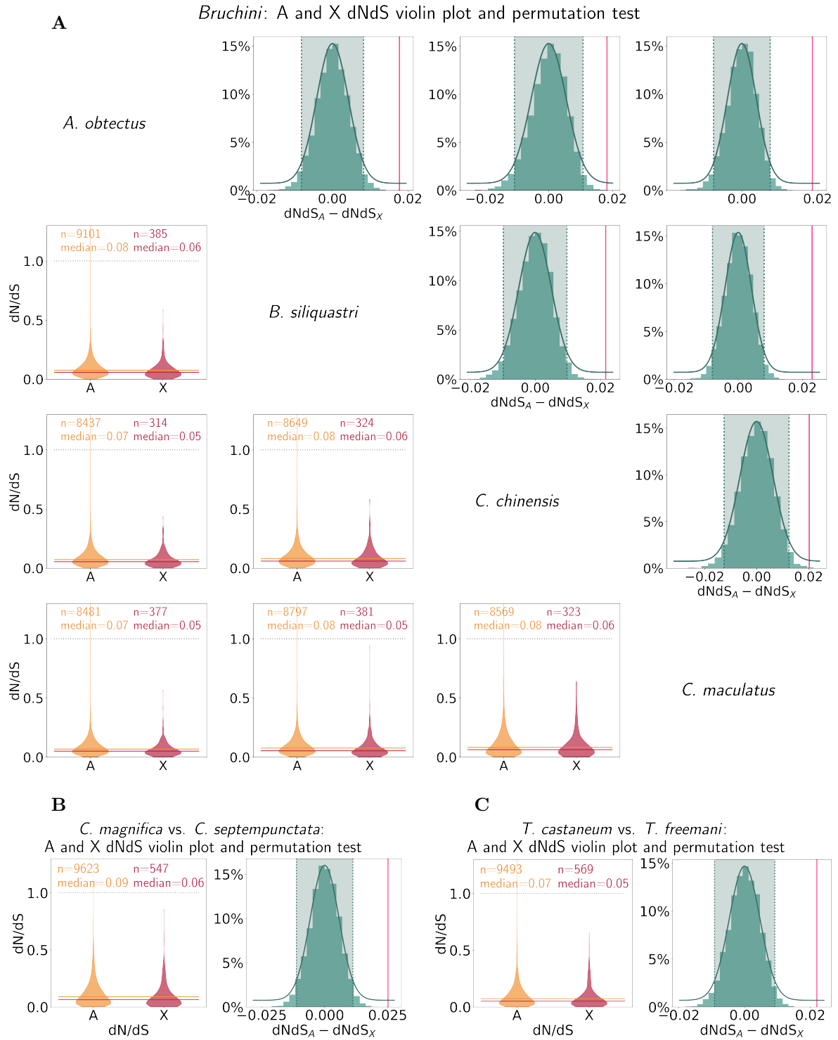
Figure 1: dN/dS of autosomal (A) and X-linked (X) genes Pairwise comparisons between members of three species lineages with violin plots of dN/dS values for X-linked and autosomal 1-to-1 orthologs. Permutation tests ( n=10000 , visualized with histograms, pink line shows measured median difference) show that dN/dS is significantly lower for X-linked orthologs in all comparisons within Bruchini (A), Coccinella (B), and Tribolium (C).
