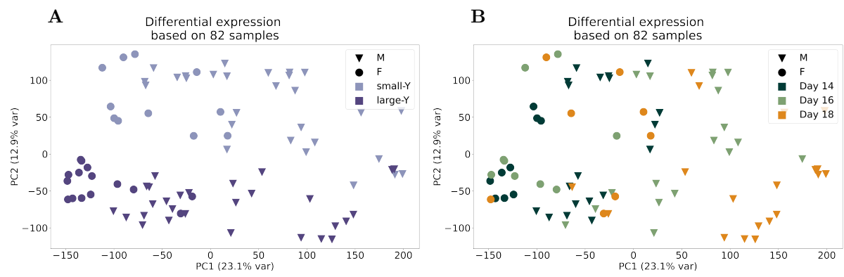
Figure S1: Line-biased genes in males. (A, B) PCA of all samples, highlighted by Y-haplotype (A) or time point (B).
