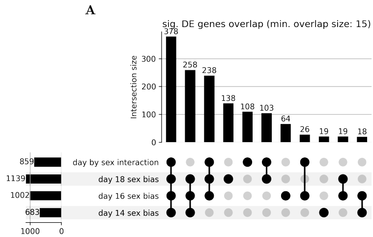
Figure 2: Sex bias across developmental stages. (A): UpSet plot showing the overlap of significantly sex-biased genes during different time points with each other and the genes that are significant in the day-by-sex interaction.
