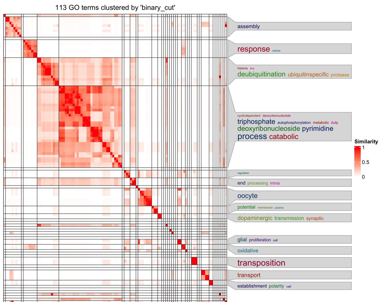
Figure S6: GO-term enrichment and semantic clustering of male line-biased samples on day 14.
