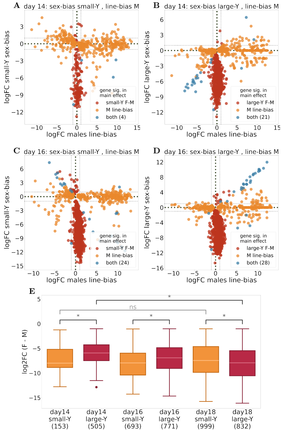
Figure 4: Intersection of sex bias and line bias across developmental stages. Log2FC of sex-bias (females - males contrast) and line-bias (large-Y - small-Y) of day 14 (A,B) and day 16 (C,D). Day 18 is not shown, there are very few line-biased genes (see Fig. 1) with one of them being sex-biased in the small-Y line and none in the large-Y line. (E) Magnitude of male-biased genes in all time points and both selection lines. Significance is tested via Mann-Whitney-U.
