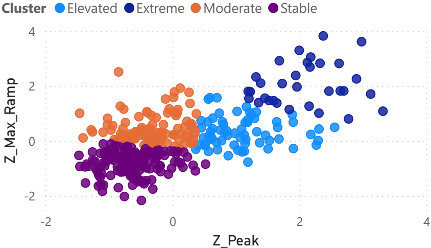
Z-Score Clustering
