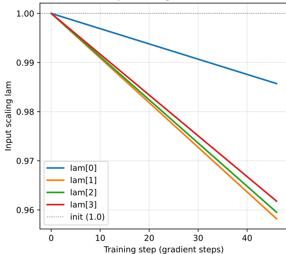
Input scaling evolution
