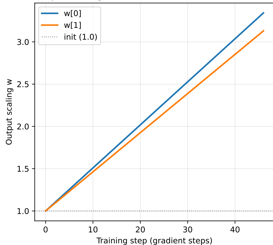
Output scaling evolution (Failure Mode 1 evidence)
