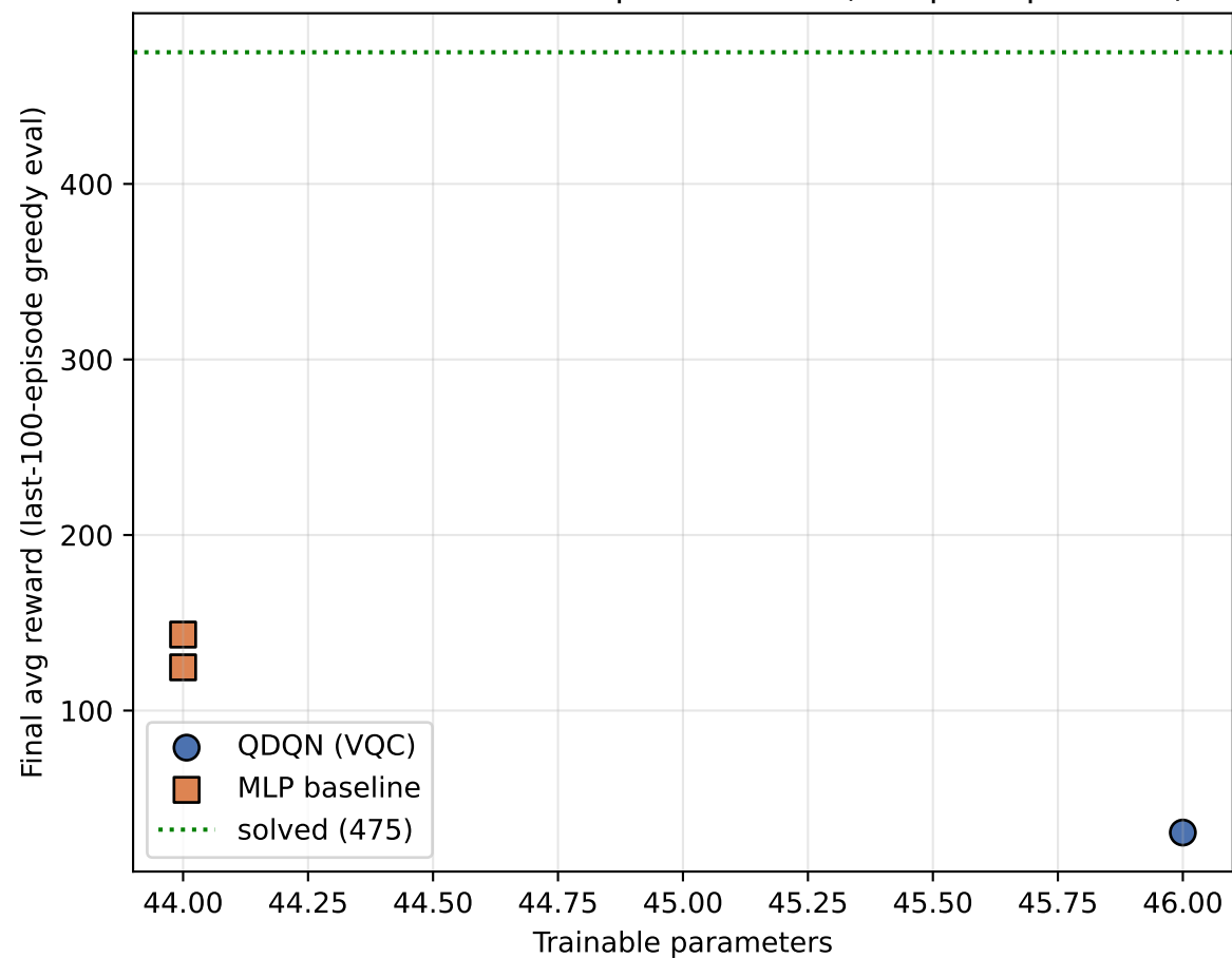
Parameter count vs. final performance (one point per seed)
