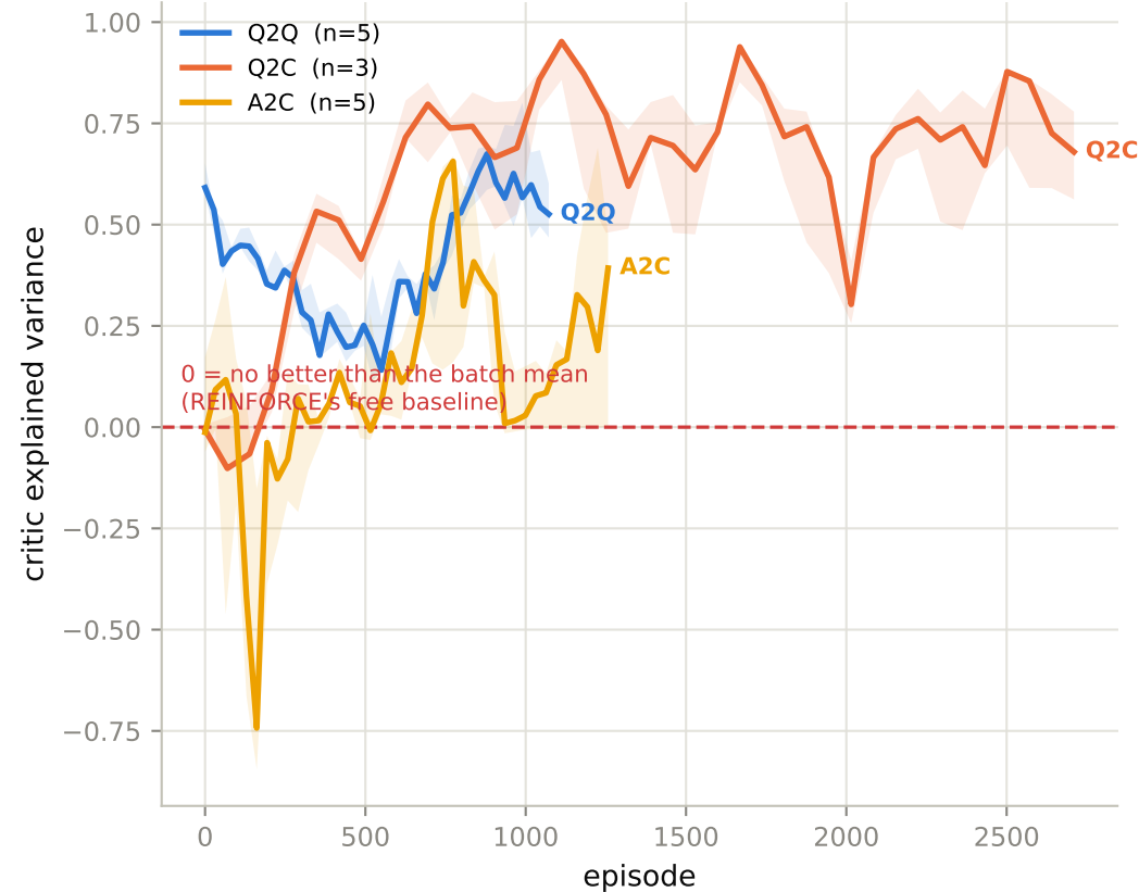
Critic quality
