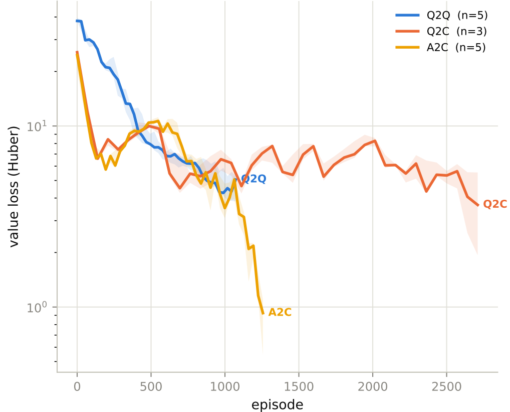
Value loss
