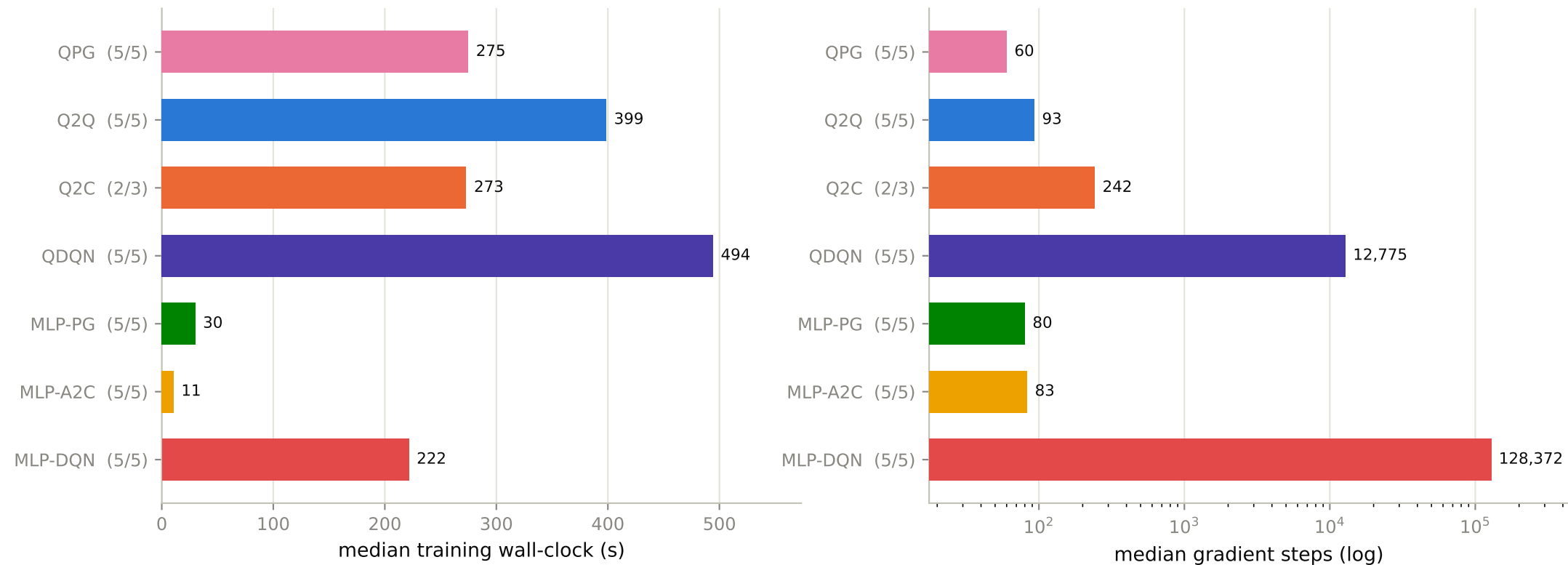
Cost: policy gradient takes far fewer, far more expensive steps
