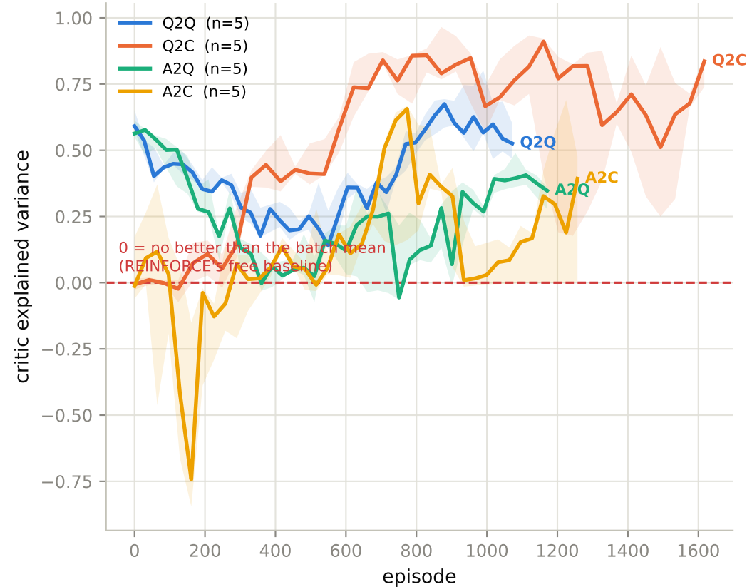
Critic quality
