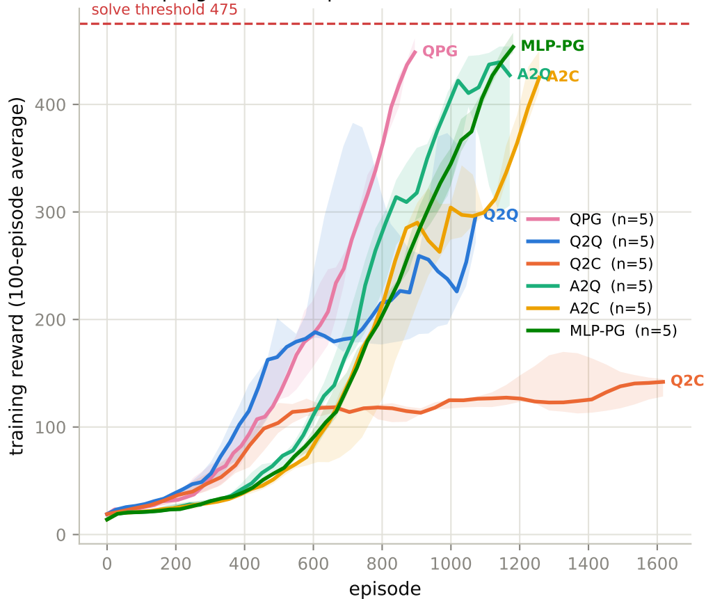
Reward progress — comparable across arms
