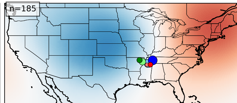
Cluster 7
