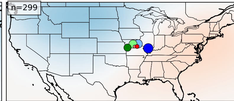
Cluster 2
