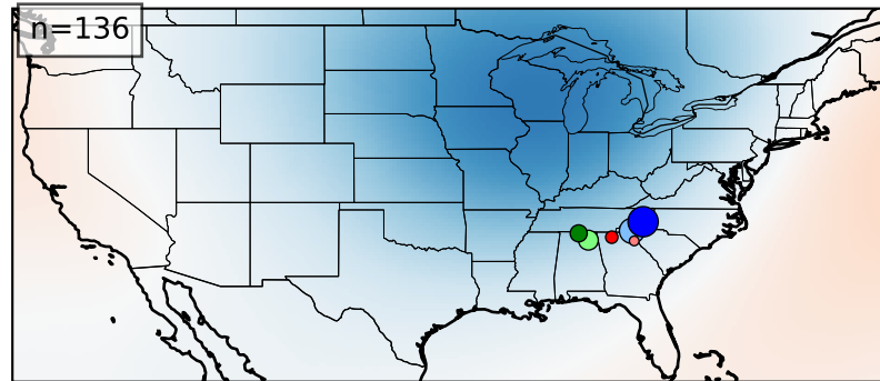
Cluster 0
