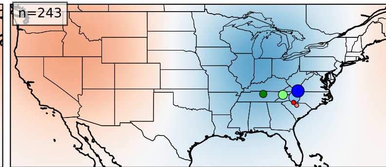
Cluster 5
