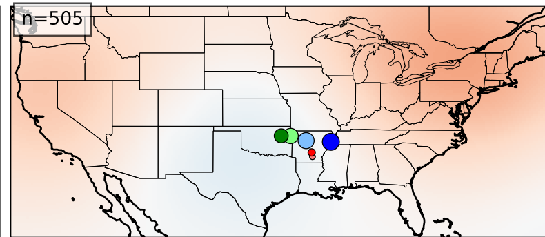
Cluster 4
