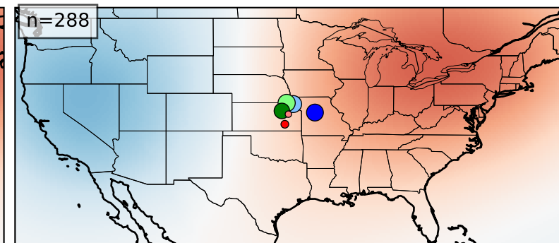
Cluster 8
