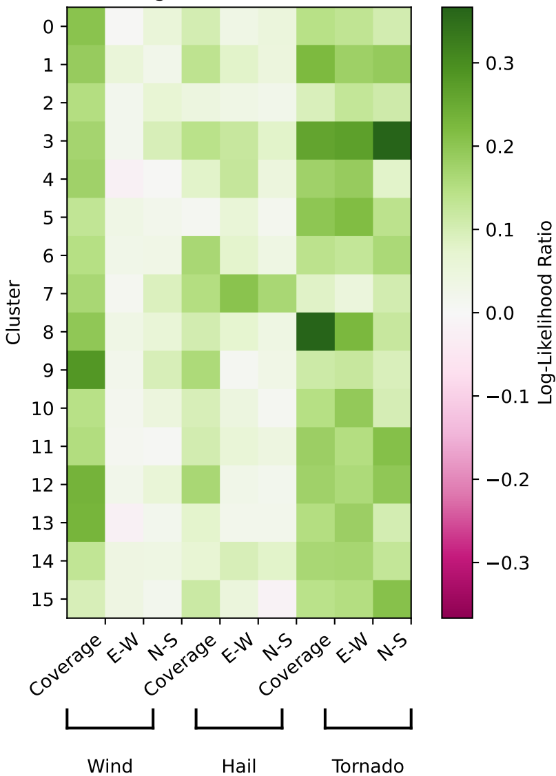
Log-Likelihood Ratio
