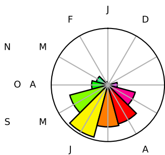
Cluster 6
