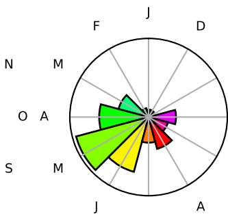
Cluster 9
