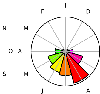
Cluster 10
