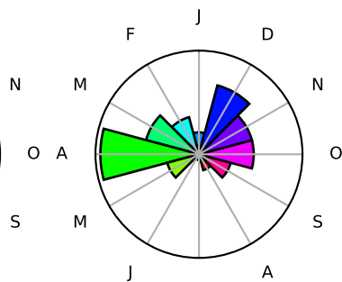
Cluster 11
