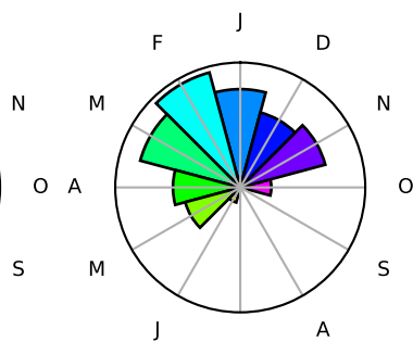
Cluster 7
