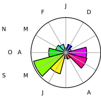
Cluster 5
