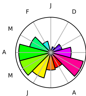
Cluster 8
