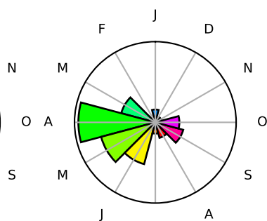
Cluster 15
