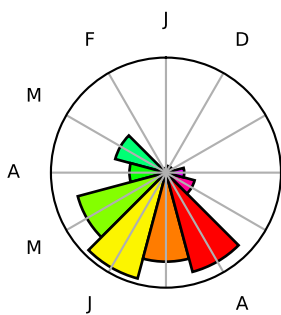
Cluster 4
