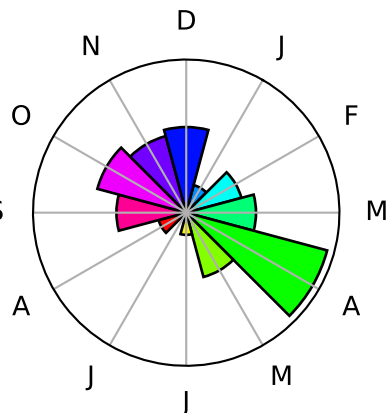
Cluster 1
