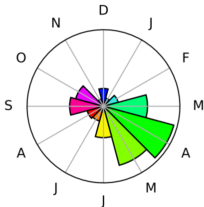
Cluster 8
