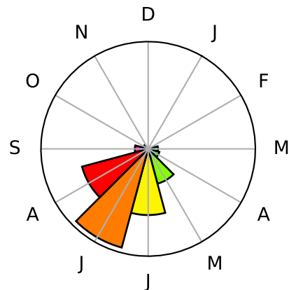
Cluster 9
