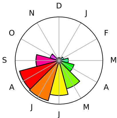
Cluster 7
