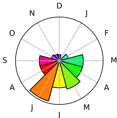
Cluster 2
