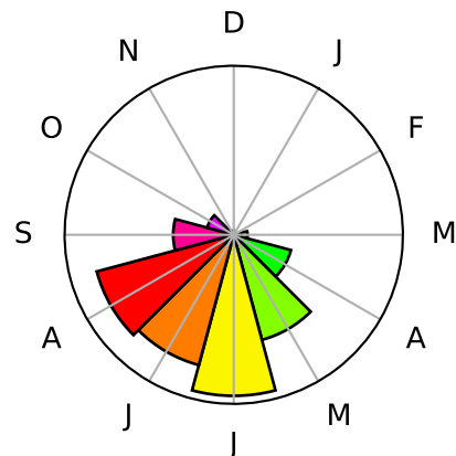
Cluster 3
