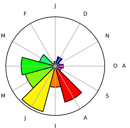
Cluster 7
