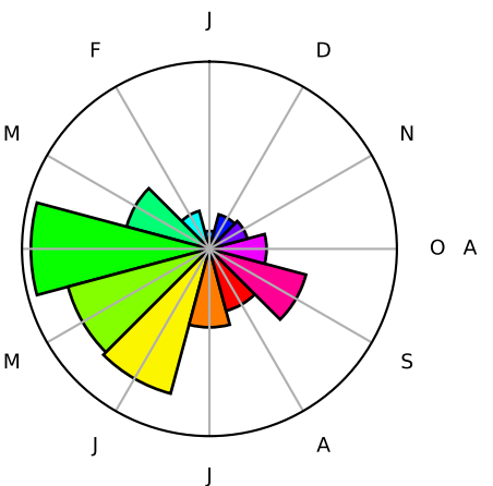
Cluster 4
