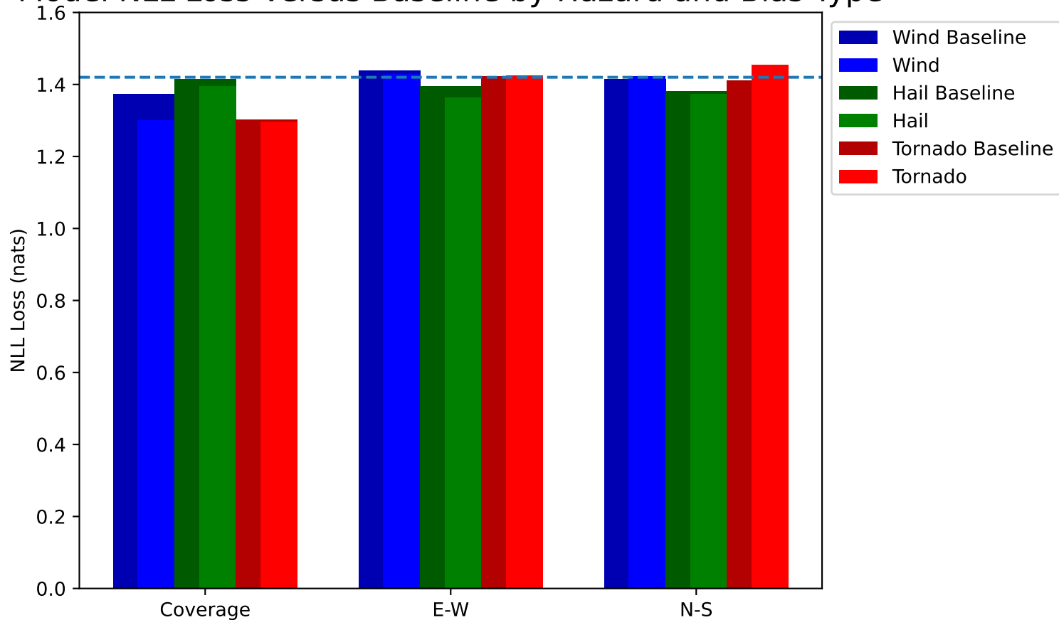
Model NLL Loss Versus Baseline by Hazard and Bias Type
