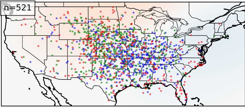
Cluster 3
