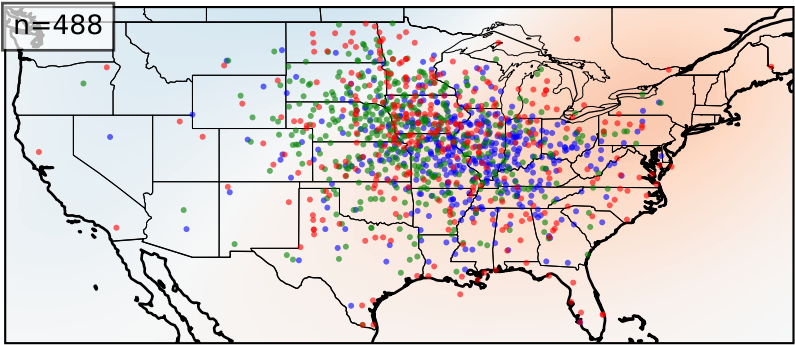
Cluster 7
