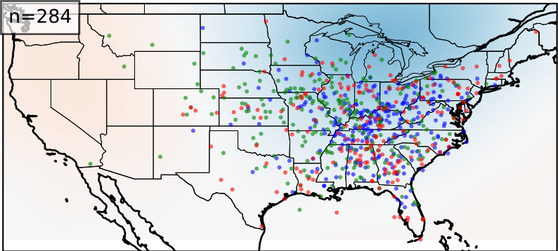
Cluster 2
