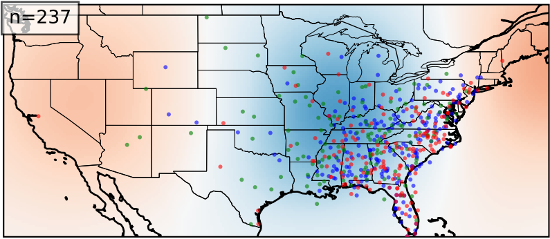
Cluster 1
