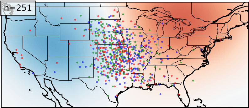
Cluster 8
