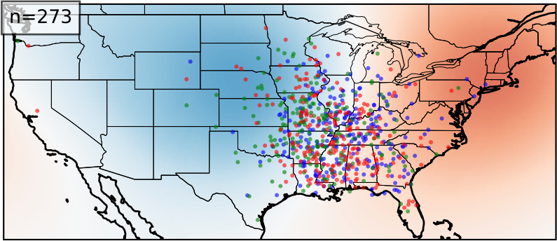
Cluster 4
