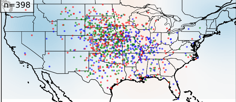
Cluster 9
