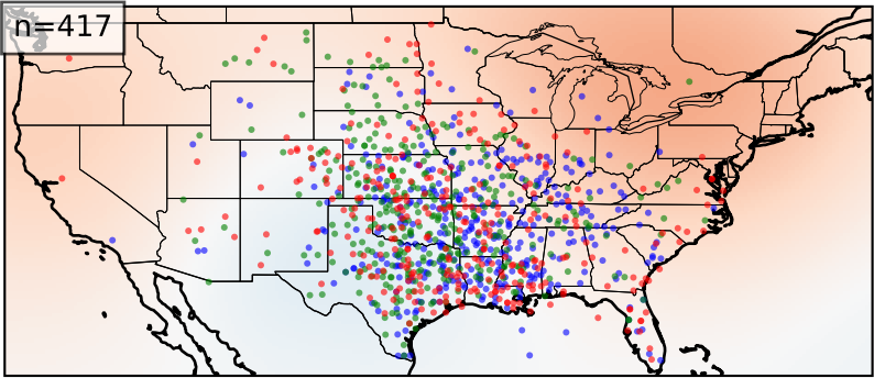
Cluster 5
