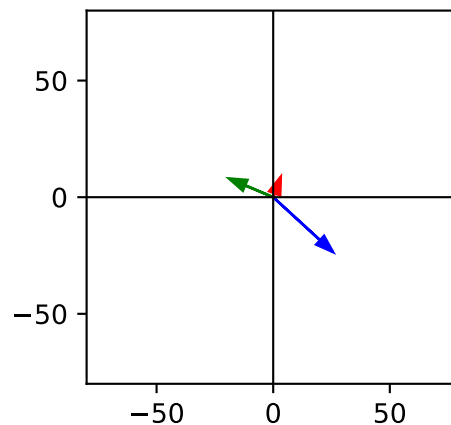
Cluster 8
