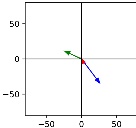
Cluster 4
