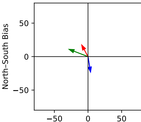
Cluster 6
