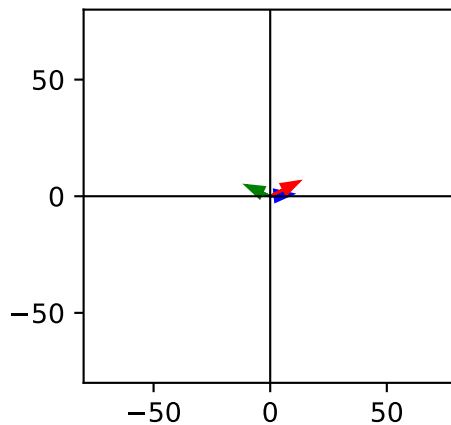
Cluster 7
