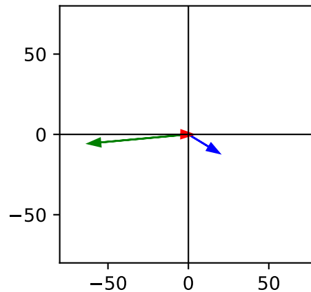
Cluster 5
