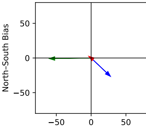
Cluster 3
