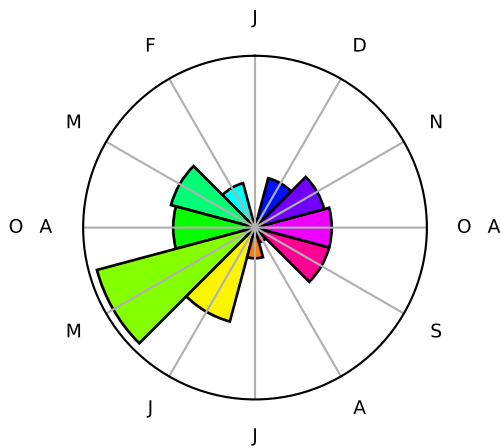
Cluster 7
