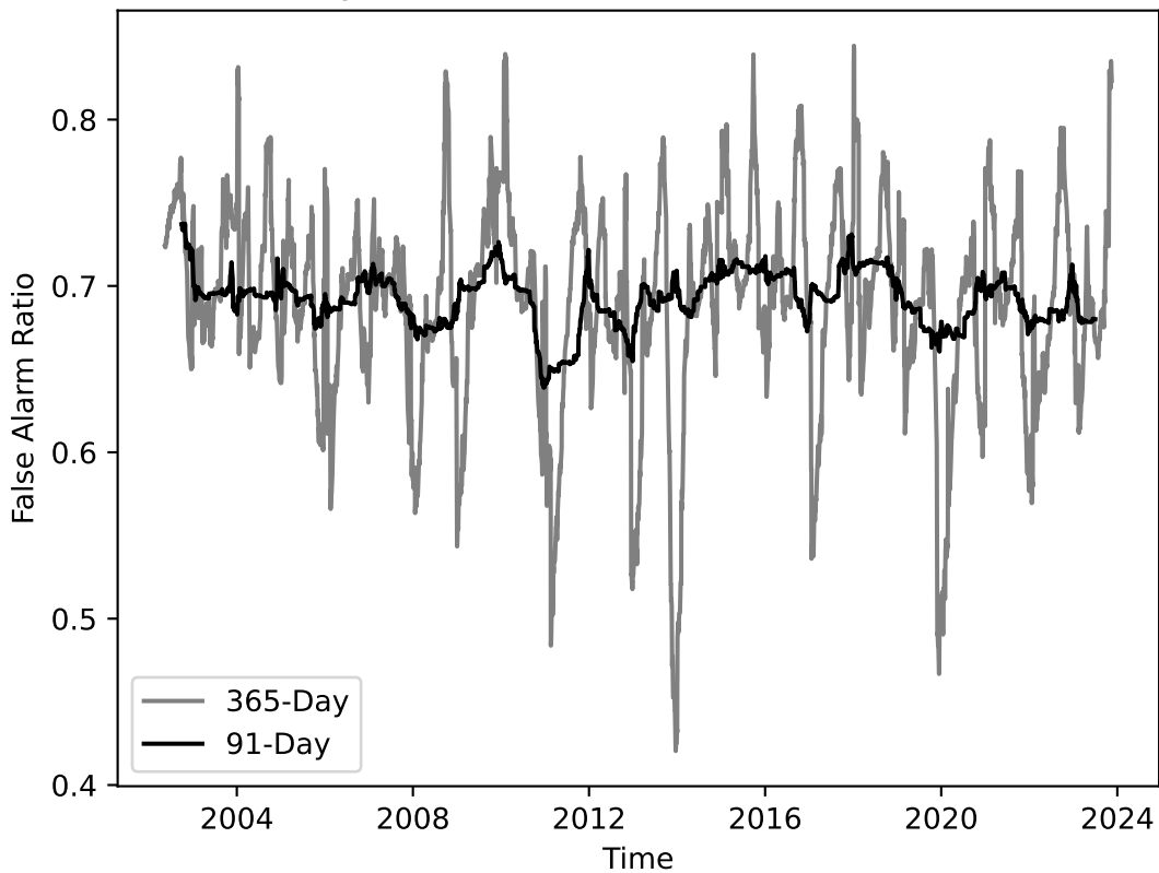
Yearly and Seasonal Wind False Alarm Ratio
