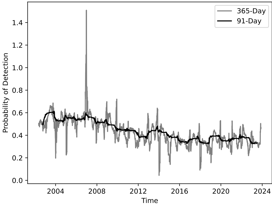
Yearly and Seasonal Hail Probability of Detection
