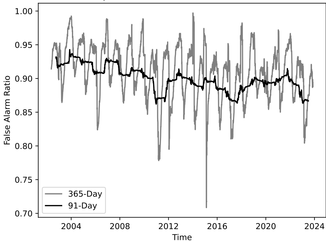
Yearly and Seasonal Hail False Alarm Ratio
