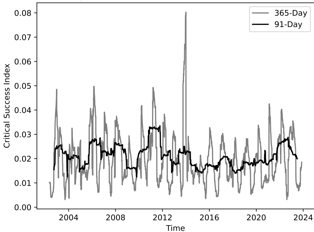
Yearly and Seasonal Tornado Critical Success Index
