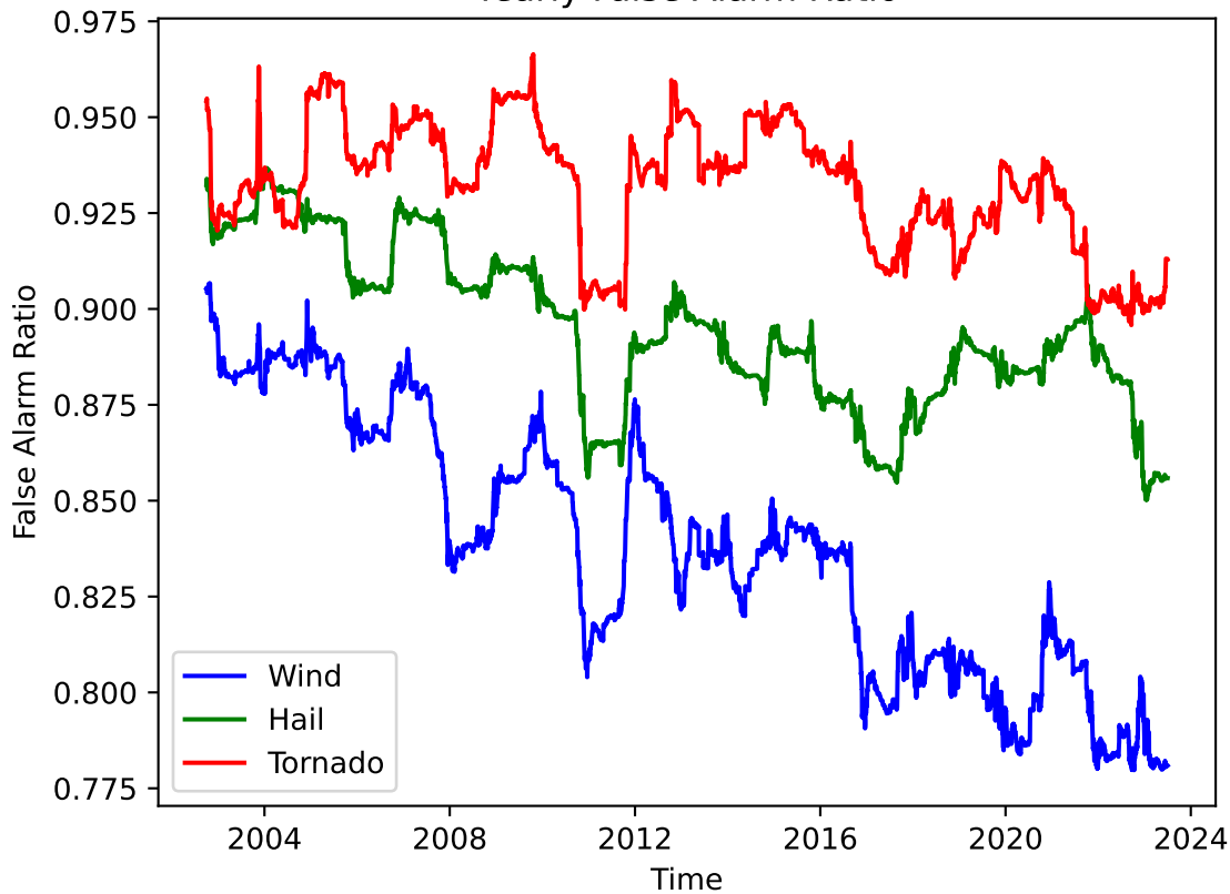
Yearly False Alarm Ratio
