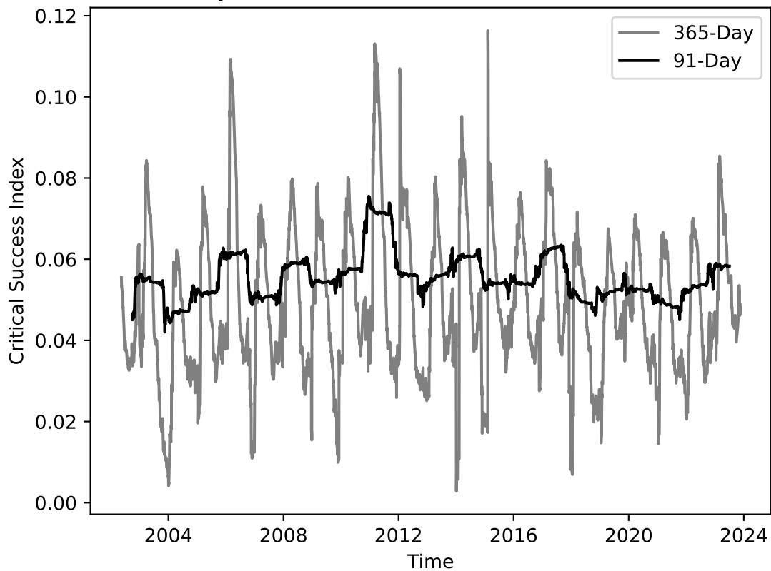
Yearly and Seasonal Hail Critical Success Index
