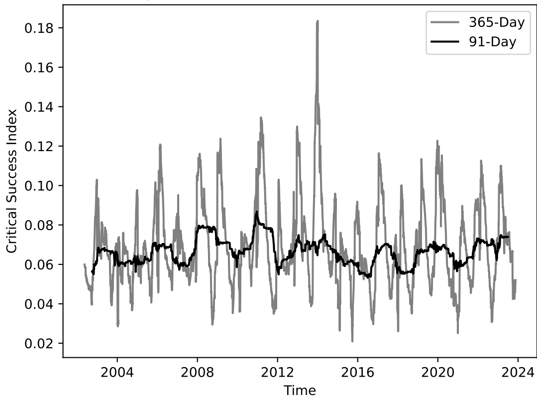
Yearly and Seasonal Wind Critical Success Index
