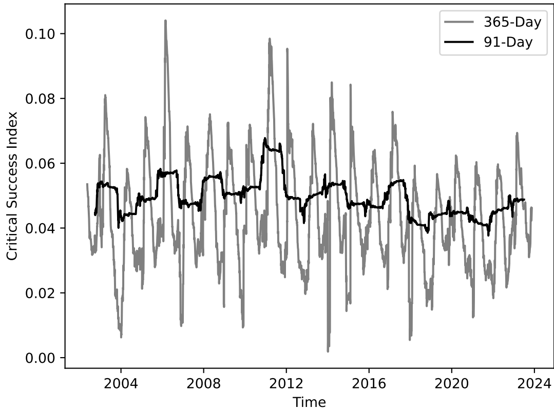
Yearly and Seasonal Hail Critical Success Index
