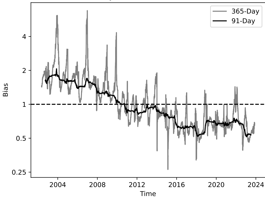
Yearly and Seasonal Hail Bias
