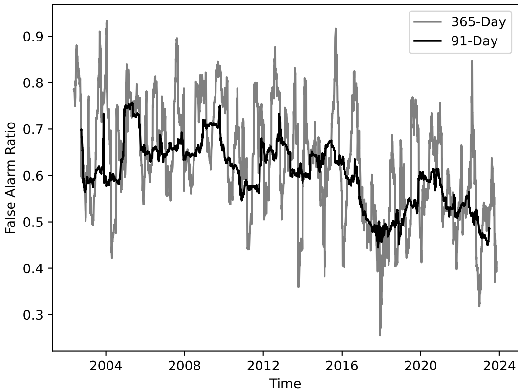
Yearly and Seasonal Tornado False Alarm Ratio
