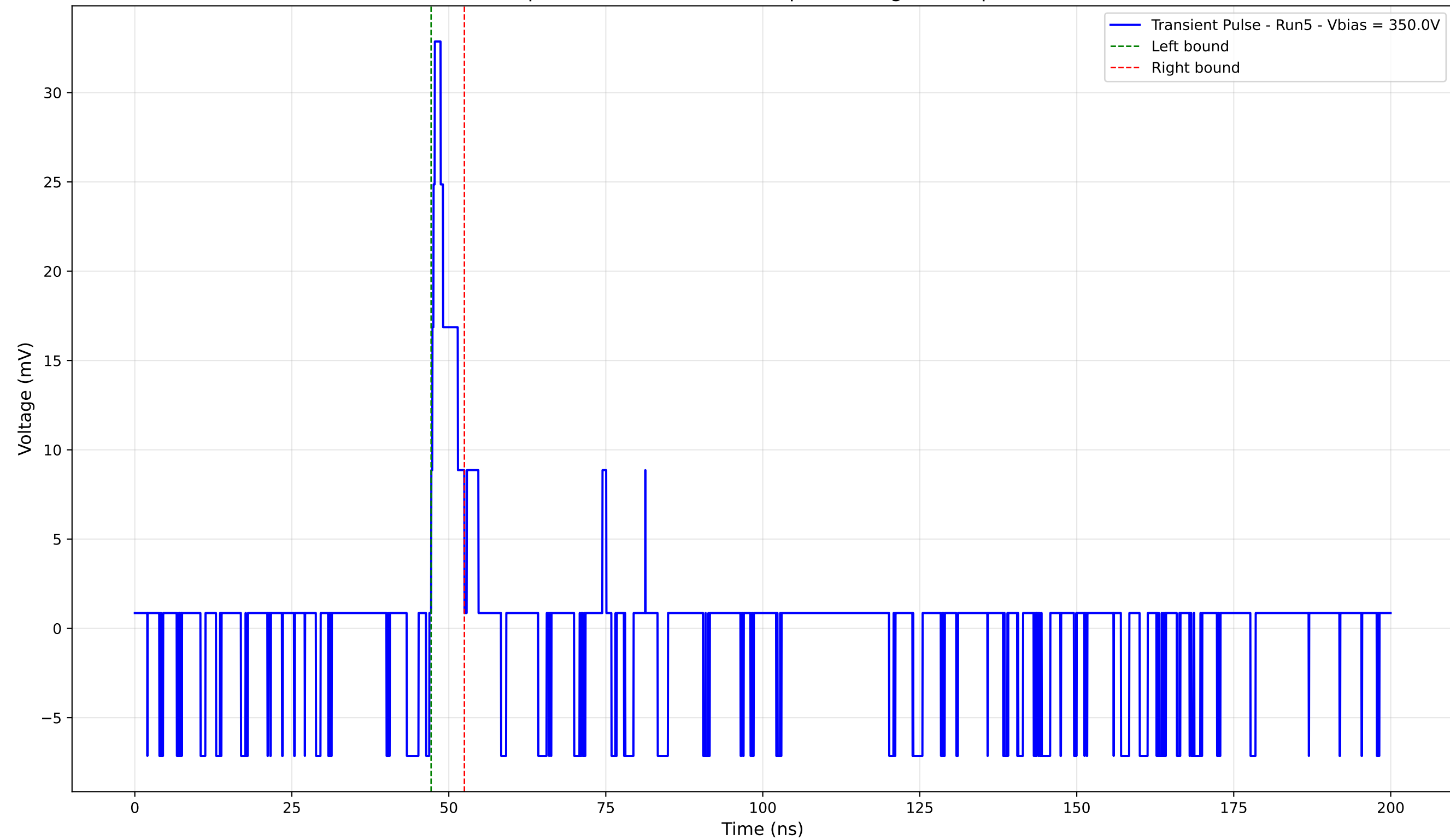
Transient Pulse - Sample: 4003 - Position: 50.0 \mu\text{m} - Charge: 1.98 pC - Rise Time: 0.57 ns
