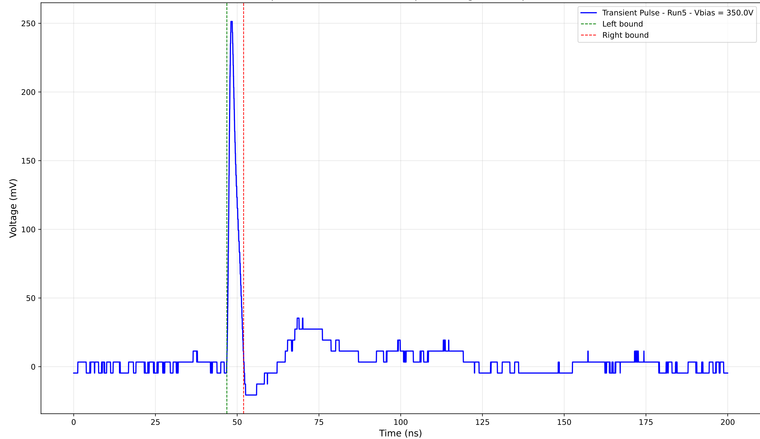
Transient Pulse - Sample: 4003 - Position: 460.0 \mu\text{m} - Charge: 13.09 pC - Rise Time: 0.91 ns
