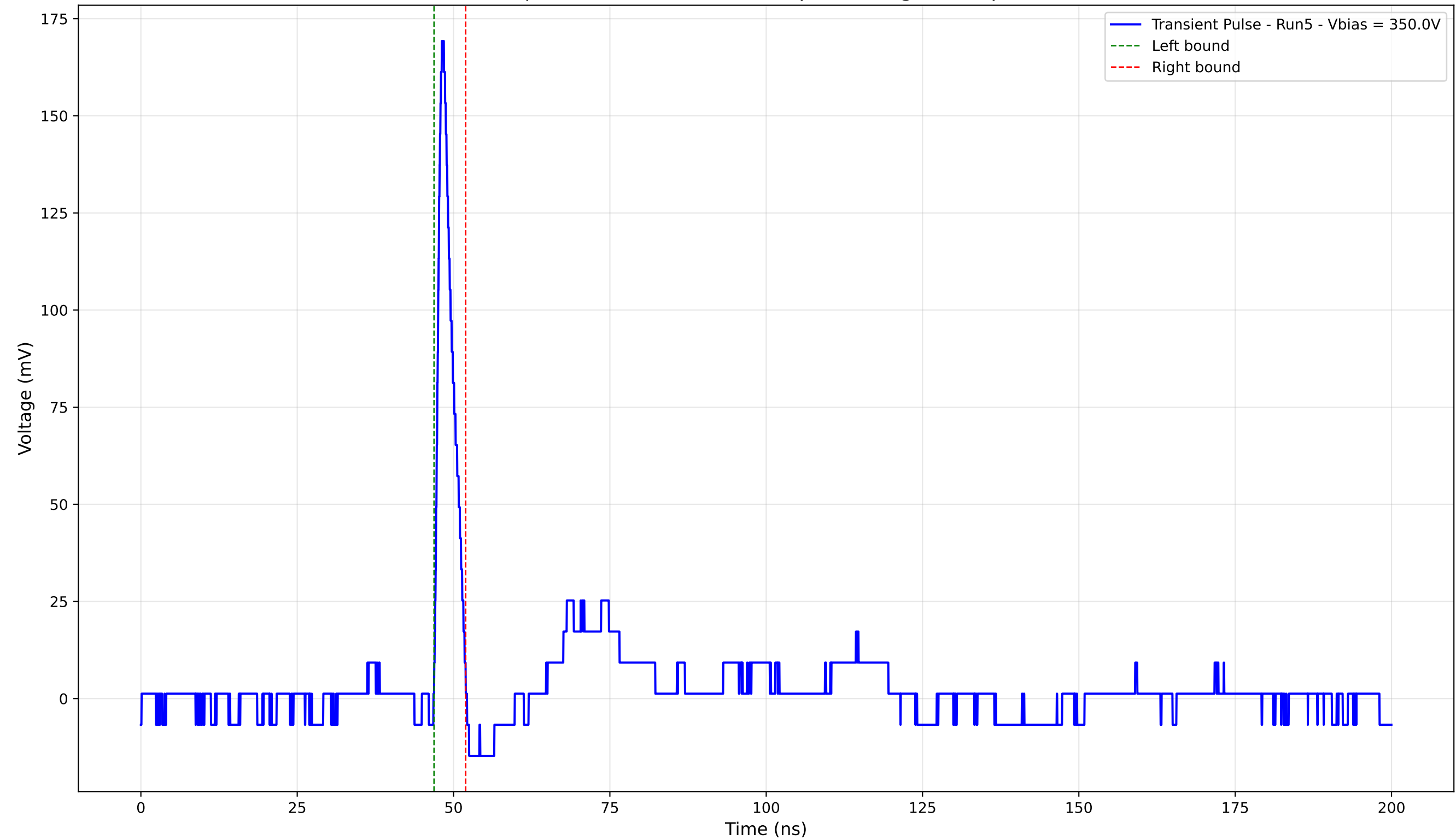
Transient Pulse - Sample: 4003 - Position: 575.0 \mu\text{m} - Charge: 8.82 pC - Rise Time: 0.92 ns
