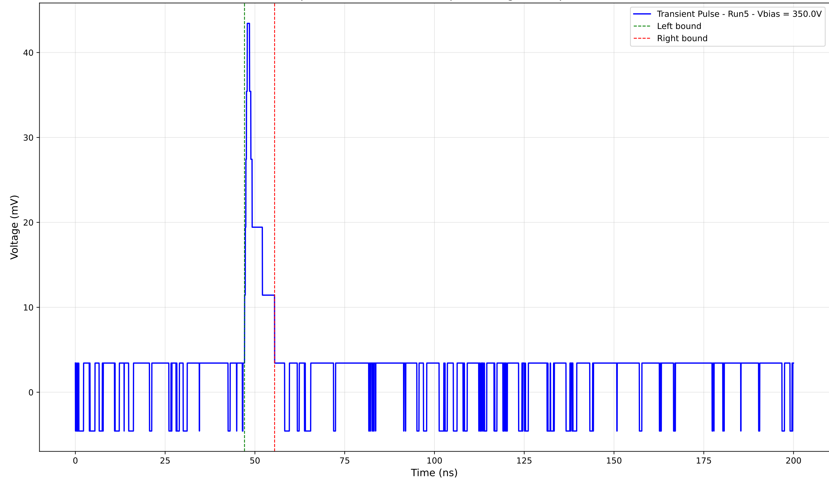
Transient Pulse - Sample: 4003 - Position: 55.0 \mu\text{m} - Charge: 3.25 pC - Rise Time: 0.76 ns
