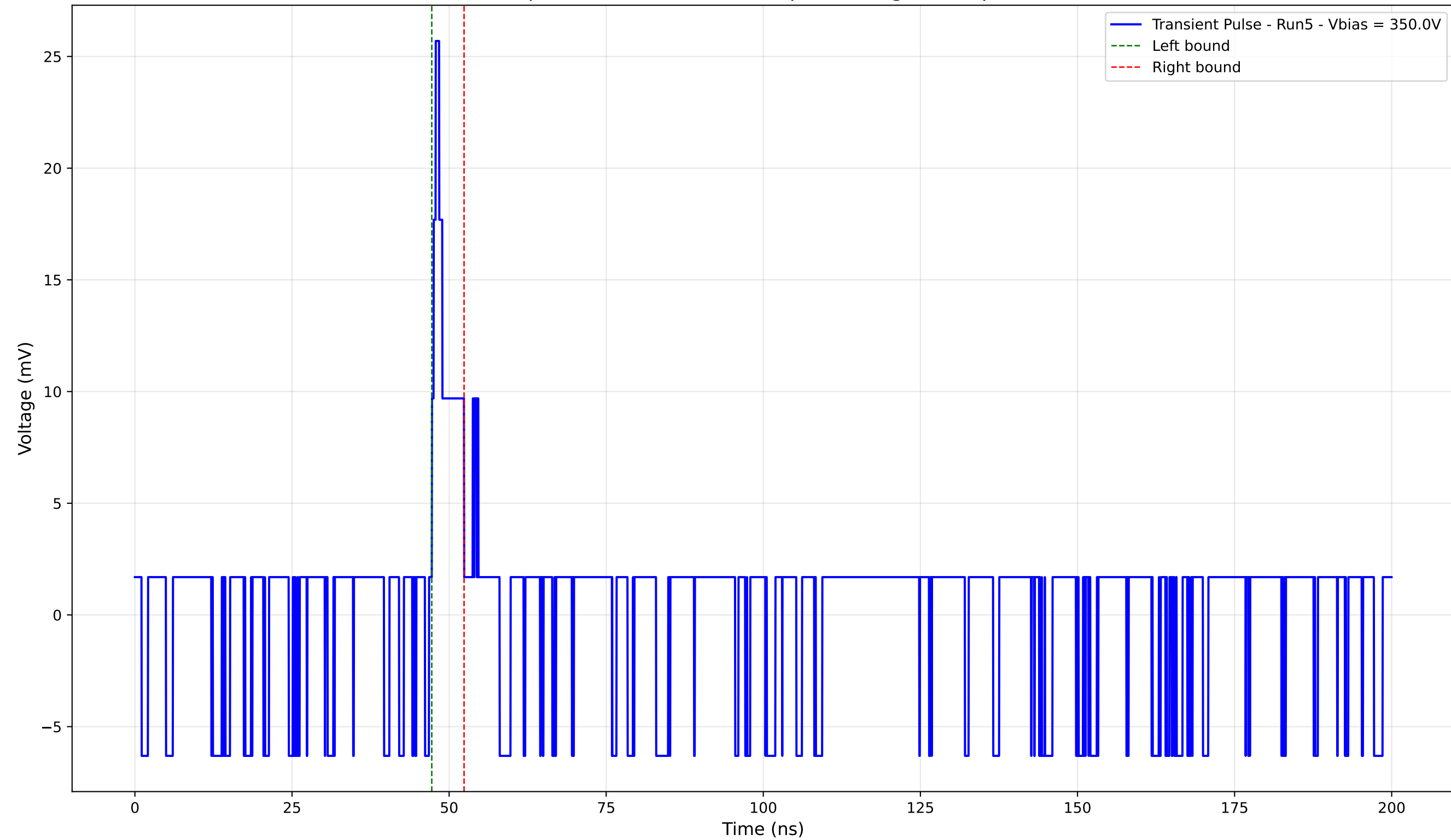
Transient Pulse - Sample: 4003 - Position: 35.0 \mu\text{m} - Charge: 1.30 pC - Rise Time: 0.62 ns
