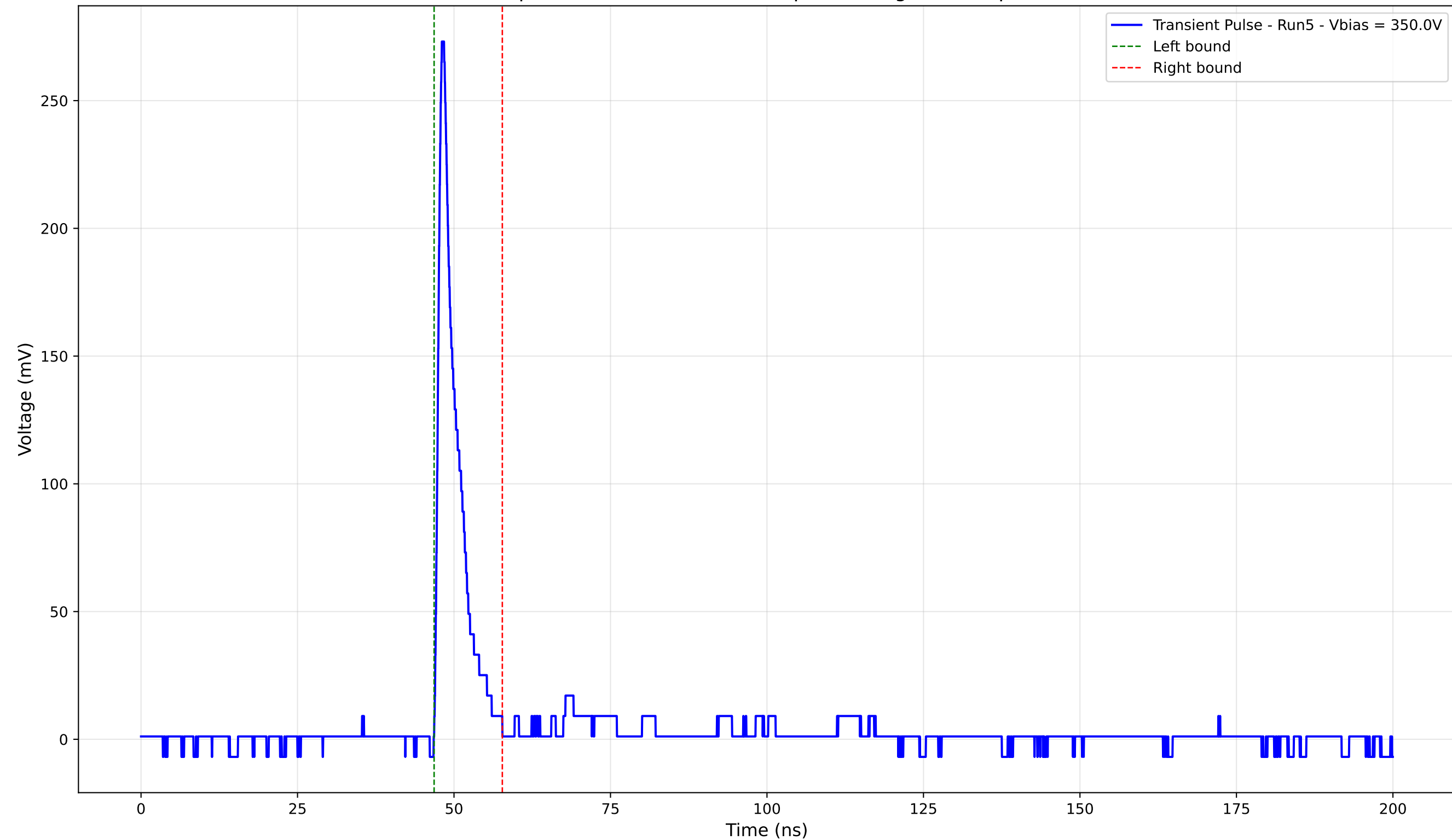
Transient Pulse - Sample: 4003 - Position: 260.0 \mu\text{m} - Charge: 18.37 pC - Rise Time: 0.87 ns
