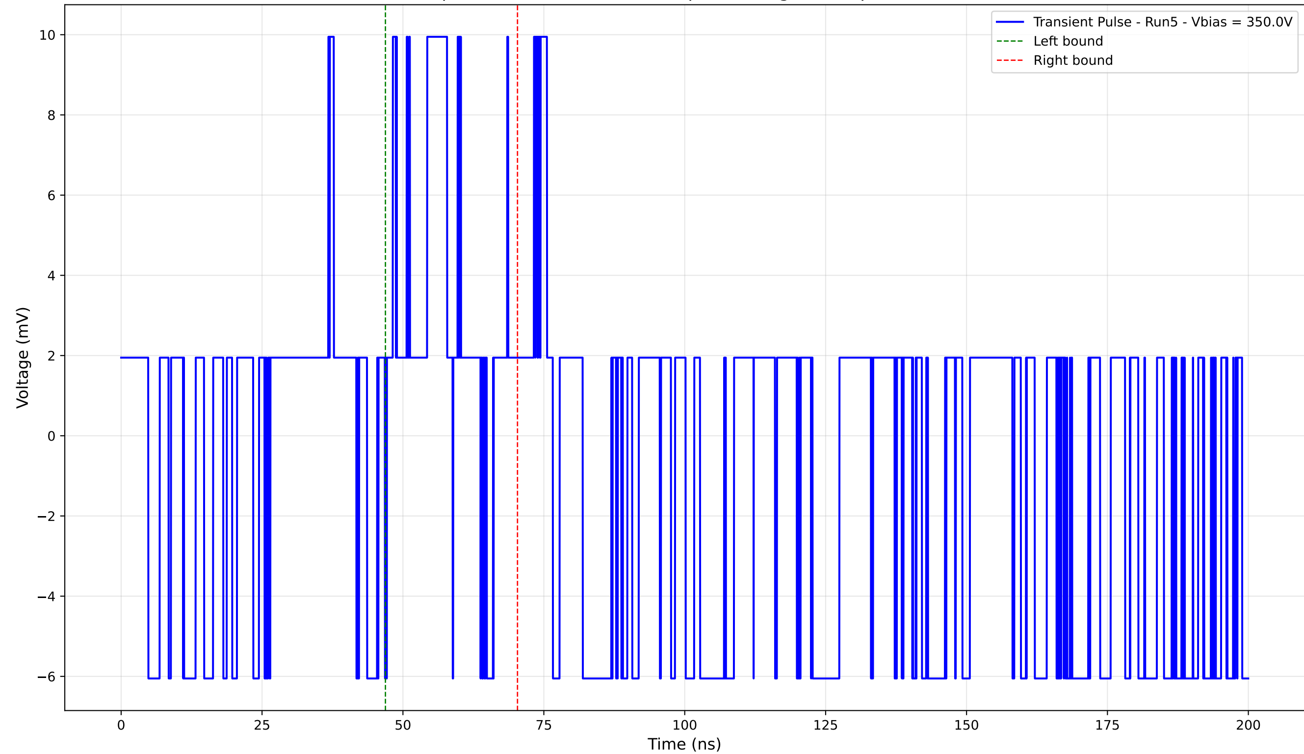
Transient Pulse - Sample: 4003 - Position: 640.0 \mu\text{m} - Charge: 1.45 pC - Rise Time: 0.00 ns (N/A)
