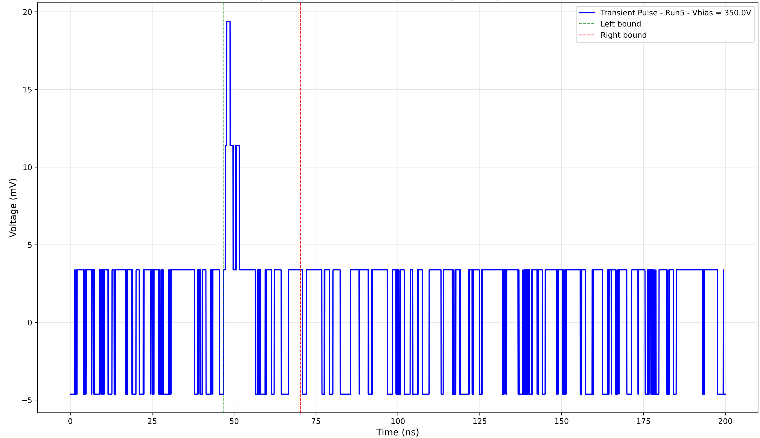
Transient Pulse - Sample: 4003 - Position: 20.0 \mu\text{m} - Charge: 1.41 pC - Rise Time: 0.00 ns (N/A)
