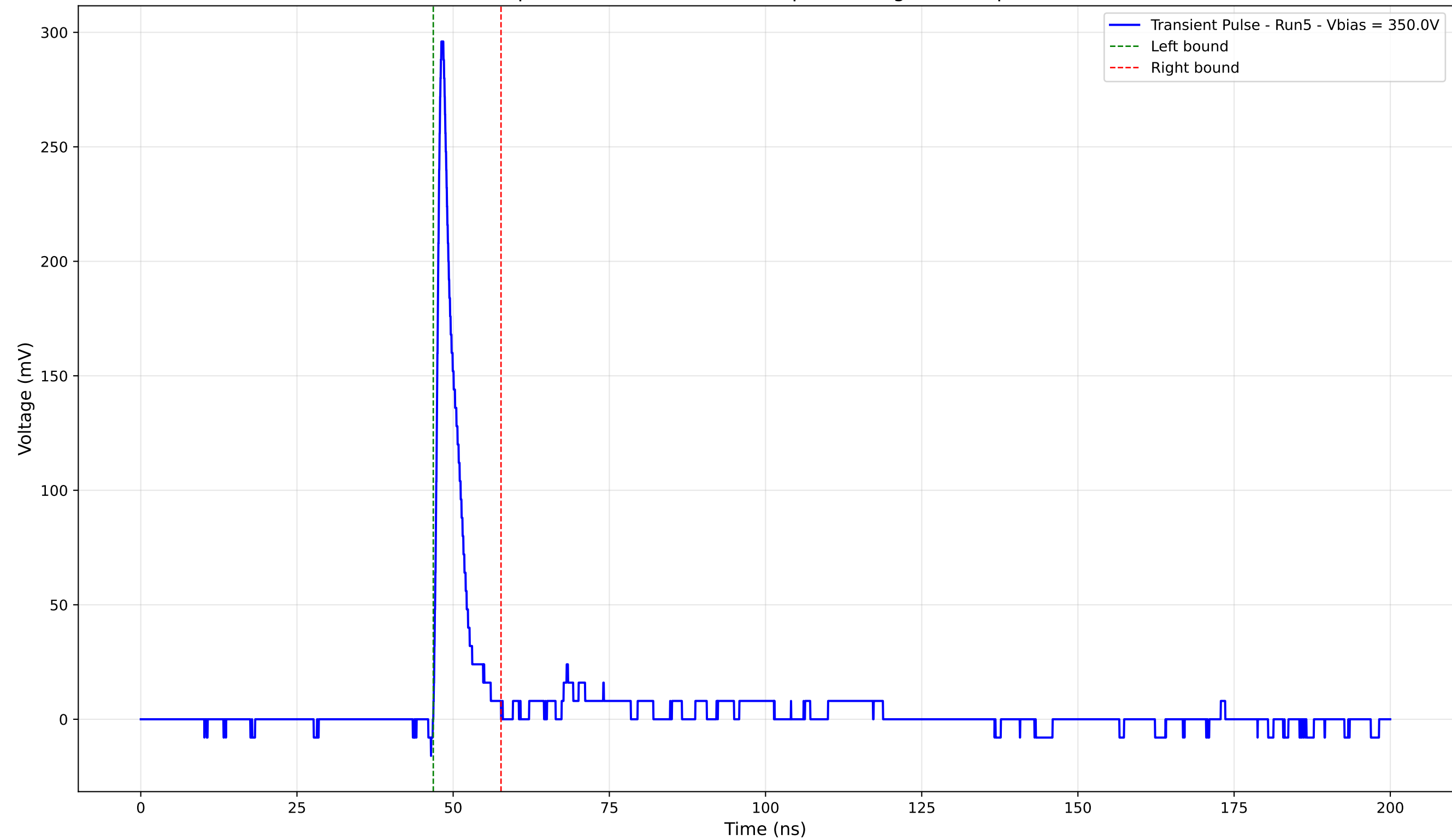
Transient Pulse - Sample: 4003 - Position: 310.0 \mu\text{m} - Charge: 19.08 pC - Rise Time: 0.93 ns
