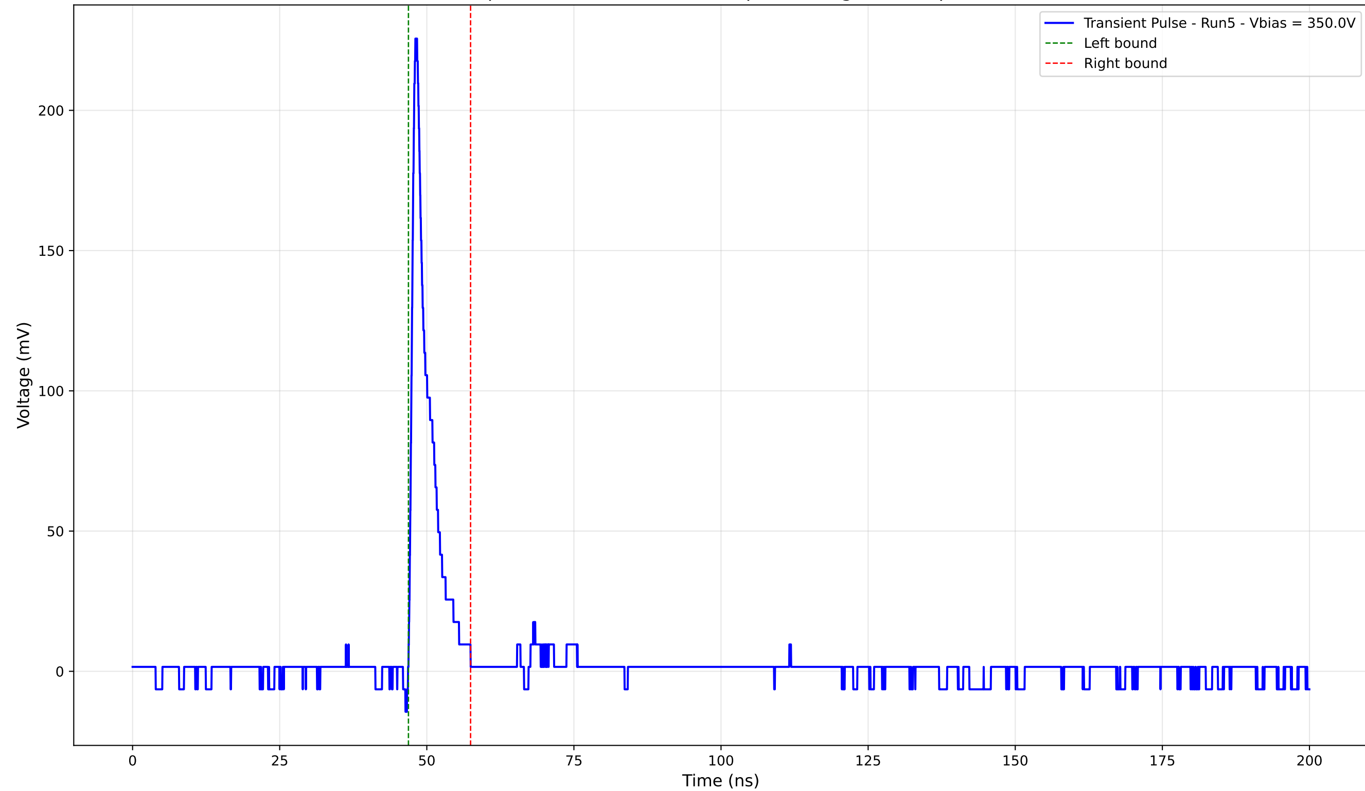
Transient Pulse - Sample: 4003 - Position: 215.0 \mu\text{m} - Charge: 14.60 pC - Rise Time: 0.87 ns
