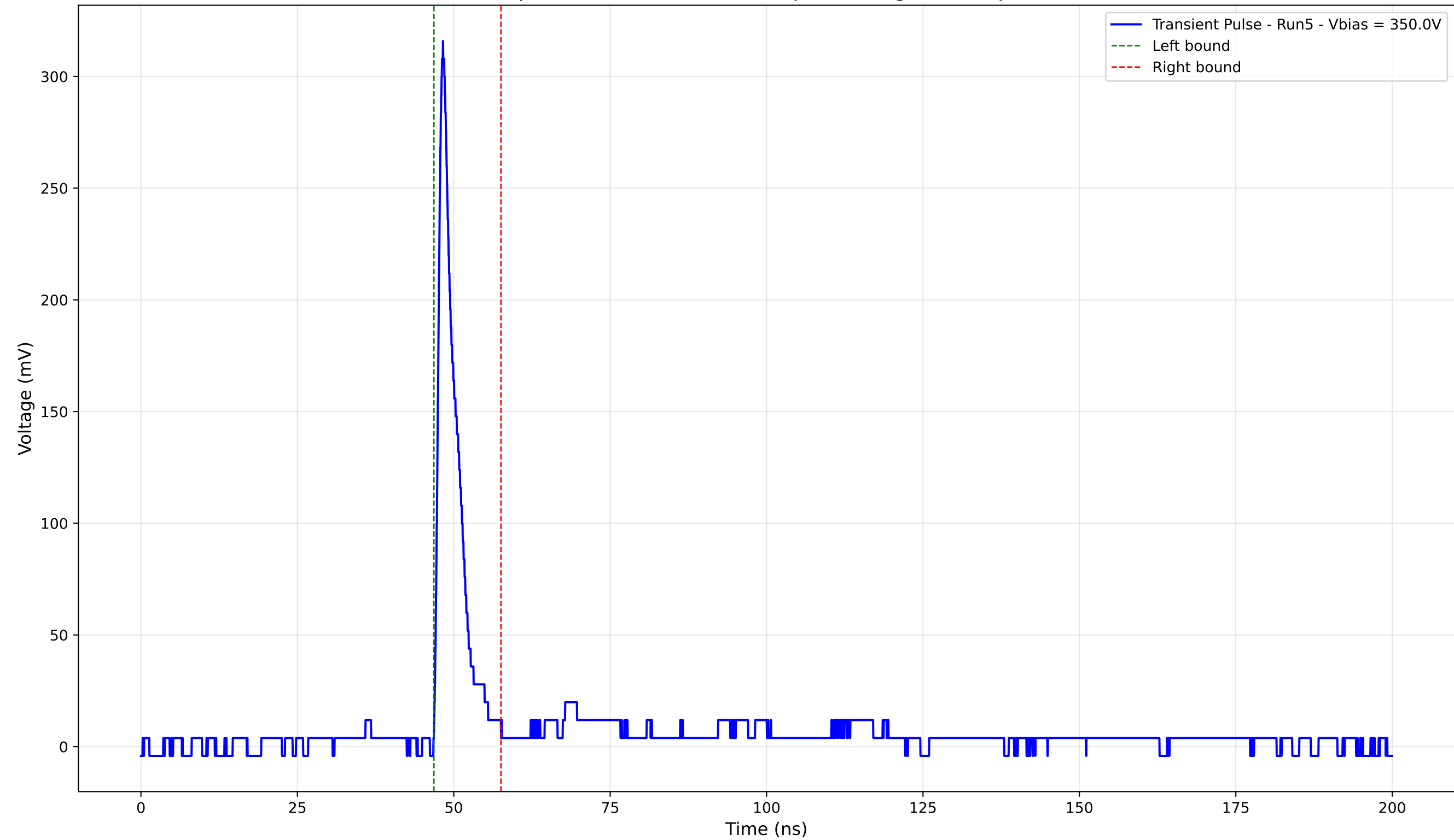
Transient Pulse - Sample: 4003 - Position: 340.0 \mu\text{m} - Charge: 20.44 pC - Rise Time: 0.97 ns
