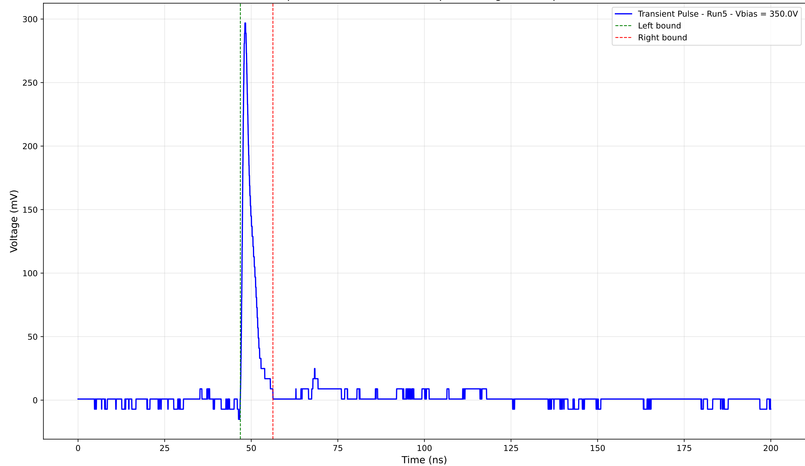
Transient Pulse - Sample: 4003 - Position: 300.0 \mu\text{m} - Charge: 18.02 pC - Rise Time: 0.91 ns
