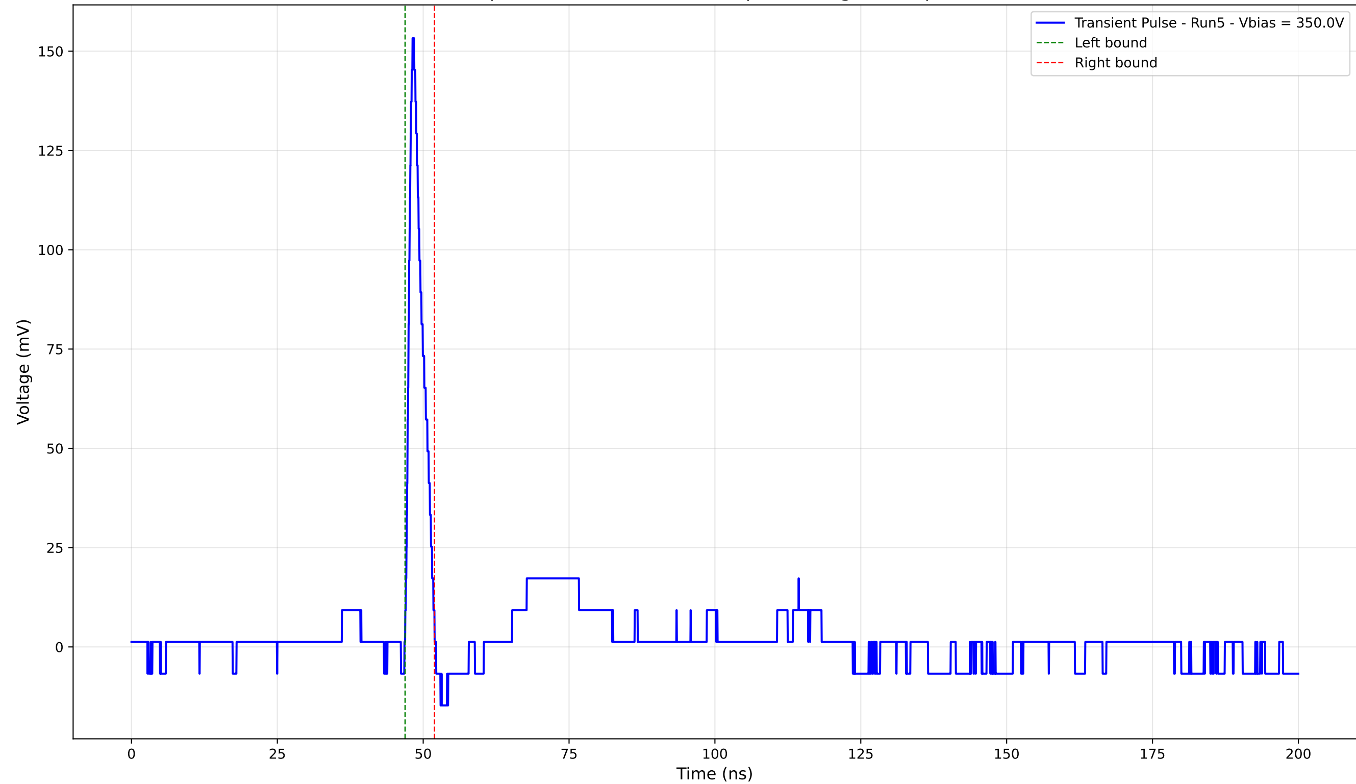
Transient Pulse - Sample: 4003 - Position: 555.0 \mu\text{m} - Charge: 7.94 pC - Rise Time: 1.00 ns
