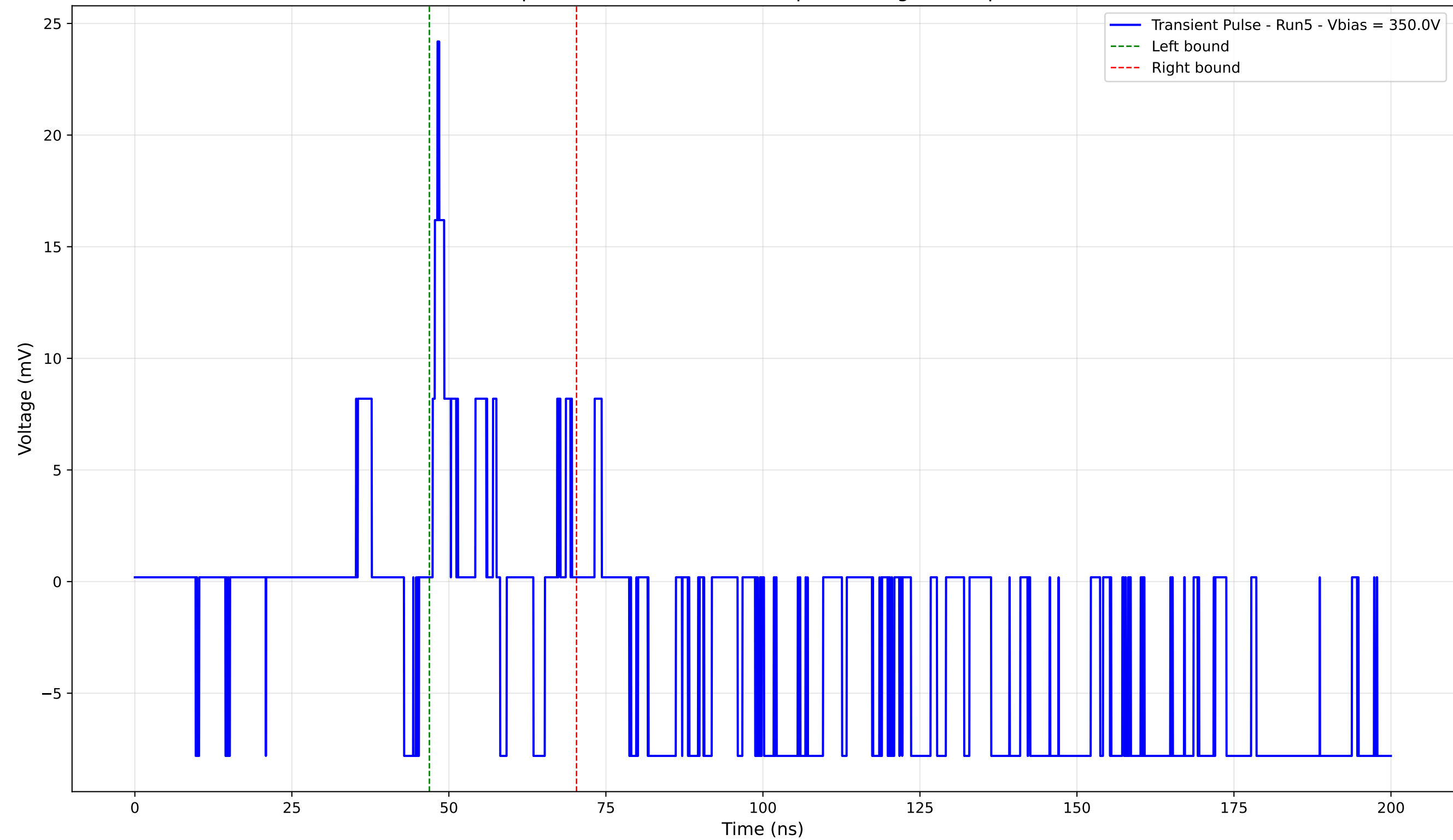
Transient Pulse - Sample: 4003 - Position: 620.0 \mu\text{m} - Charge: 1.10 pC - Rise Time: 0.77 ns
