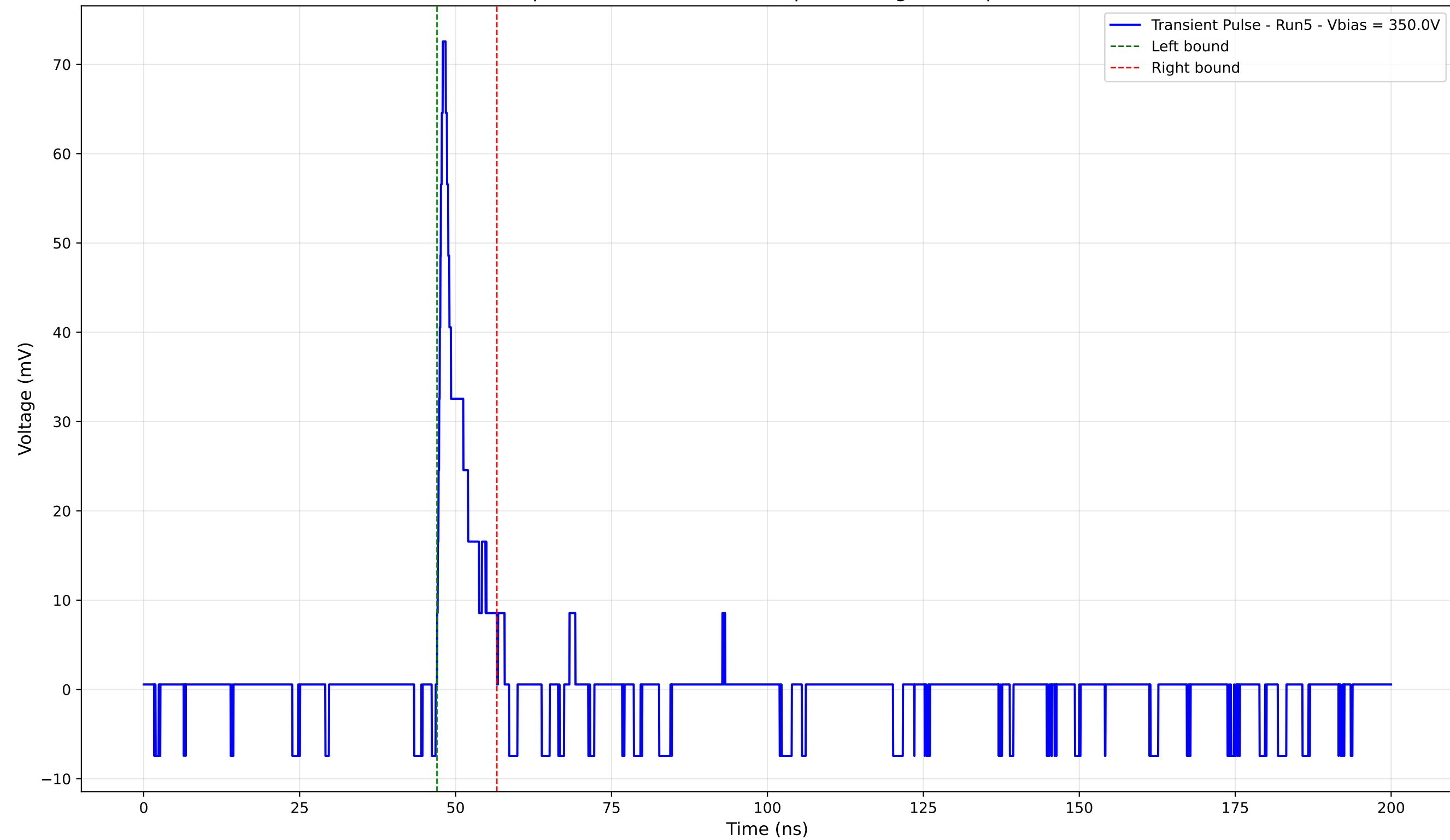
Transient Pulse - Sample: 4003 - Position: 85.0 \mu\text{m} - Charge: 5.10 pC - Rise Time: 0.90 ns
