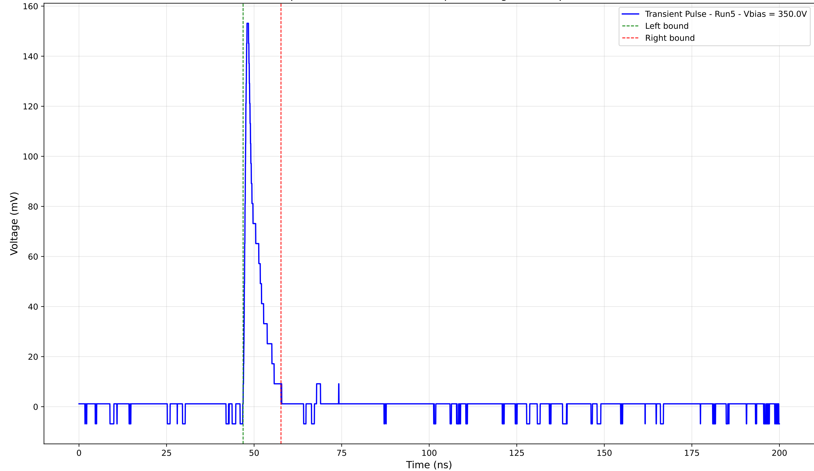
Transient Pulse - Sample: 4003 - Position: 155.0 \mu\text{m} - Charge: 11.29 pC - Rise Time: 0.88 ns
