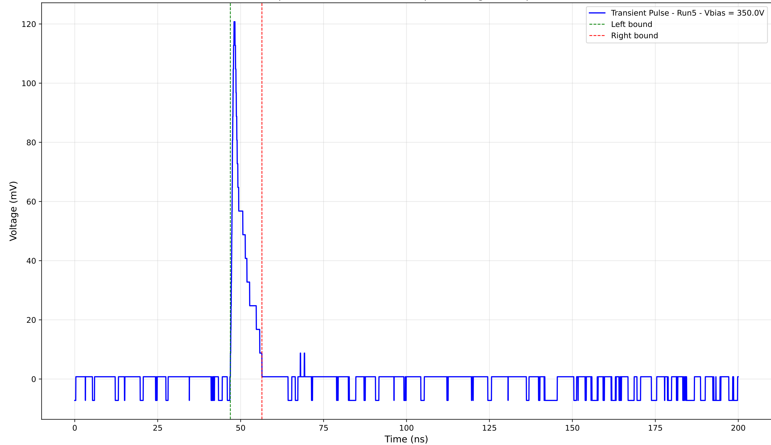
Transient Pulse - Sample: 4003 - Position: 125.0 \mu\text{m} - Charge: 8.53 pC - Rise Time: 0.85 ns
