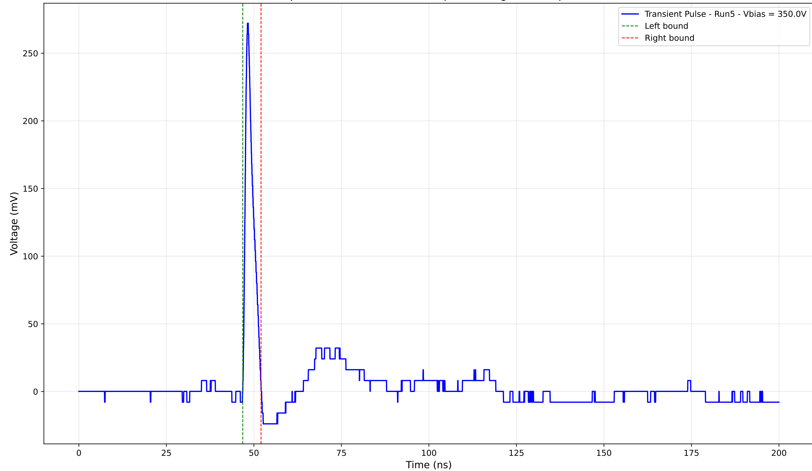
Transient Pulse - Sample: 4003 - Position: 445.0 \mu\text{m} - Charge: 13.90 pC - Rise Time: 0.91 ns
