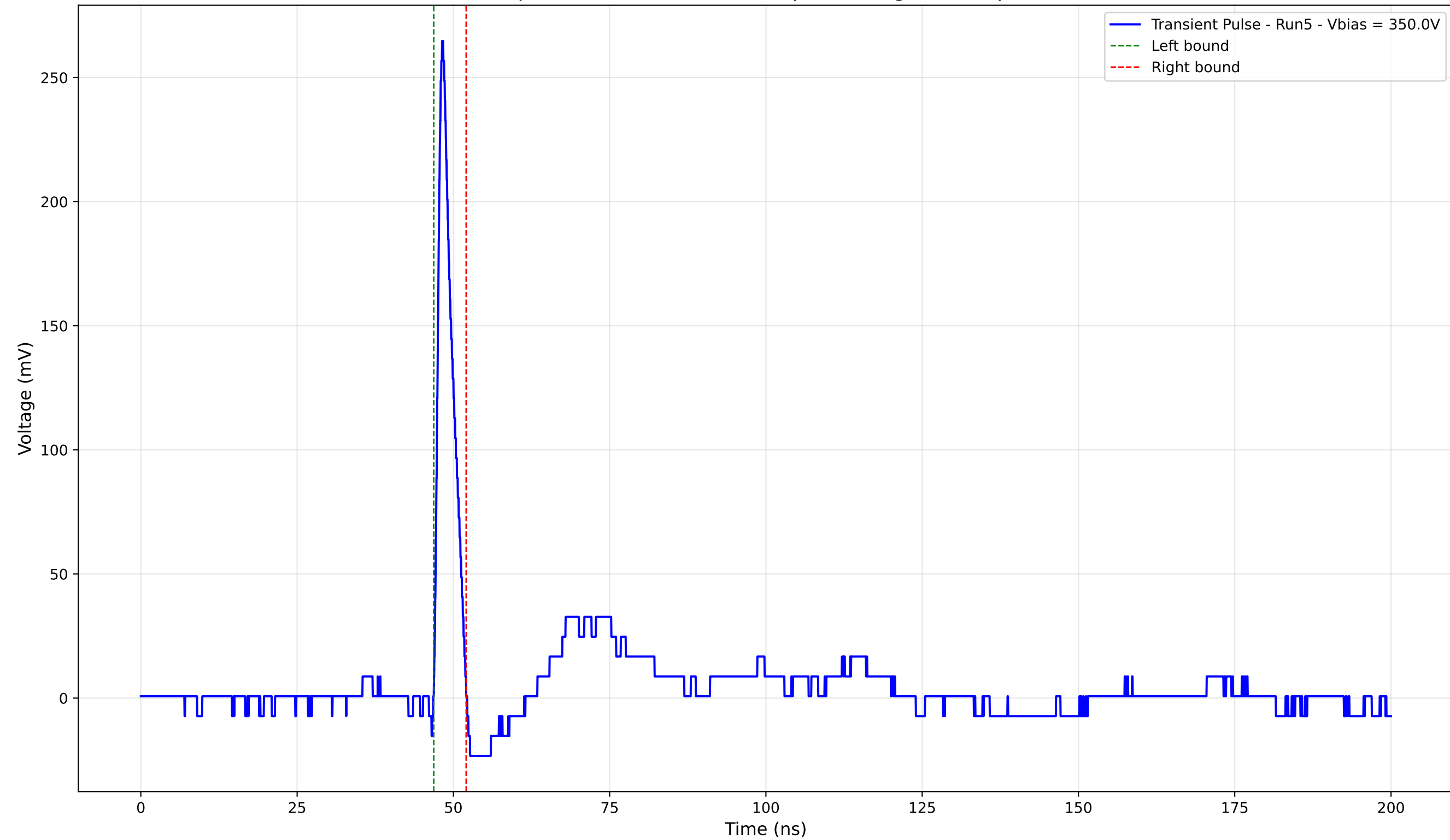
Transient Pulse - Sample: 4003 - Position: 450.0 \mu\text{m} - Charge: 13.53 pC - Rise Time: 0.90 ns
