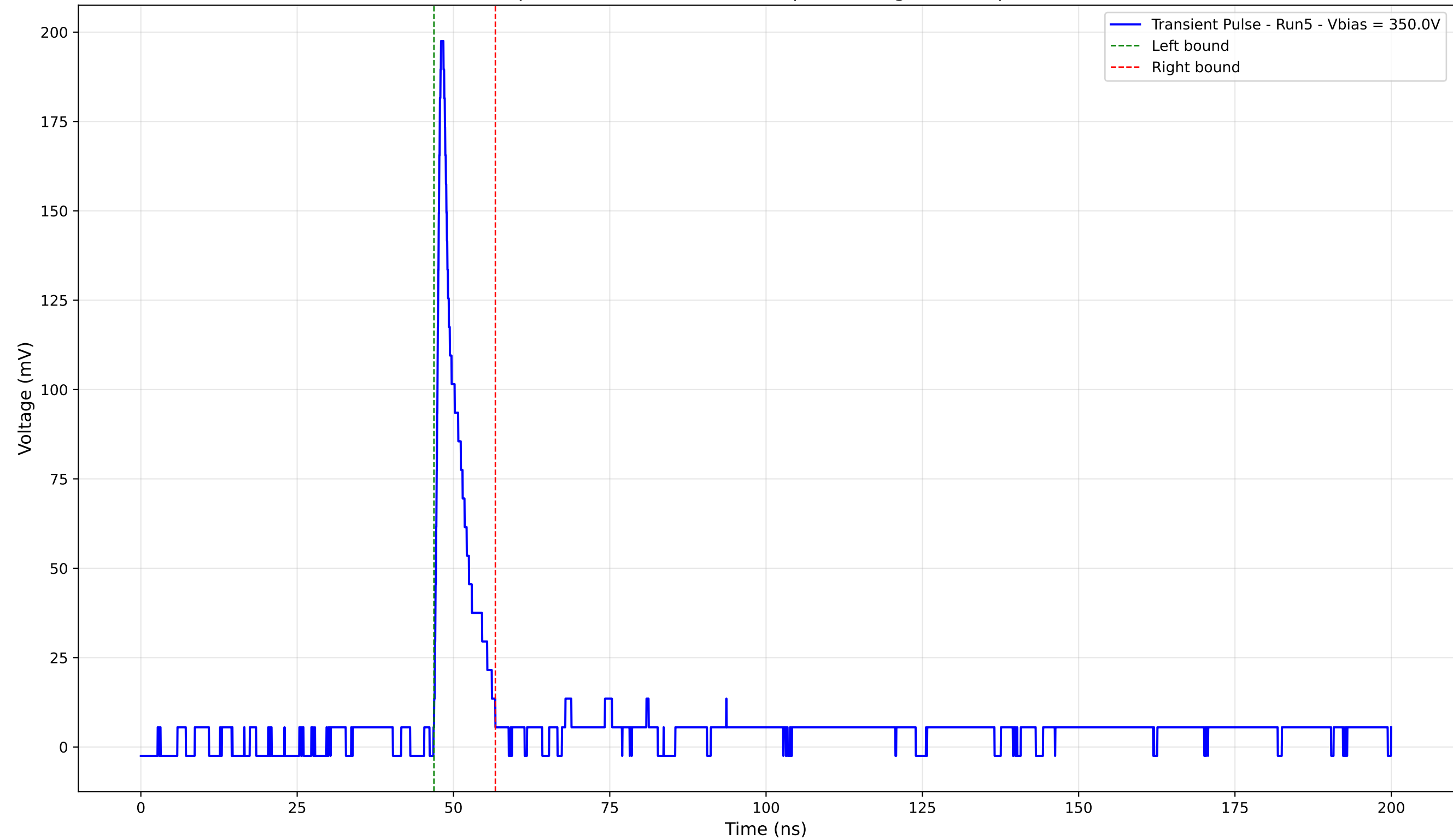
Transient Pulse - Sample: 4003 - Position: 185.0 \mu\text{m} - Charge: 14.57 pC - Rise Time: 0.84 ns
