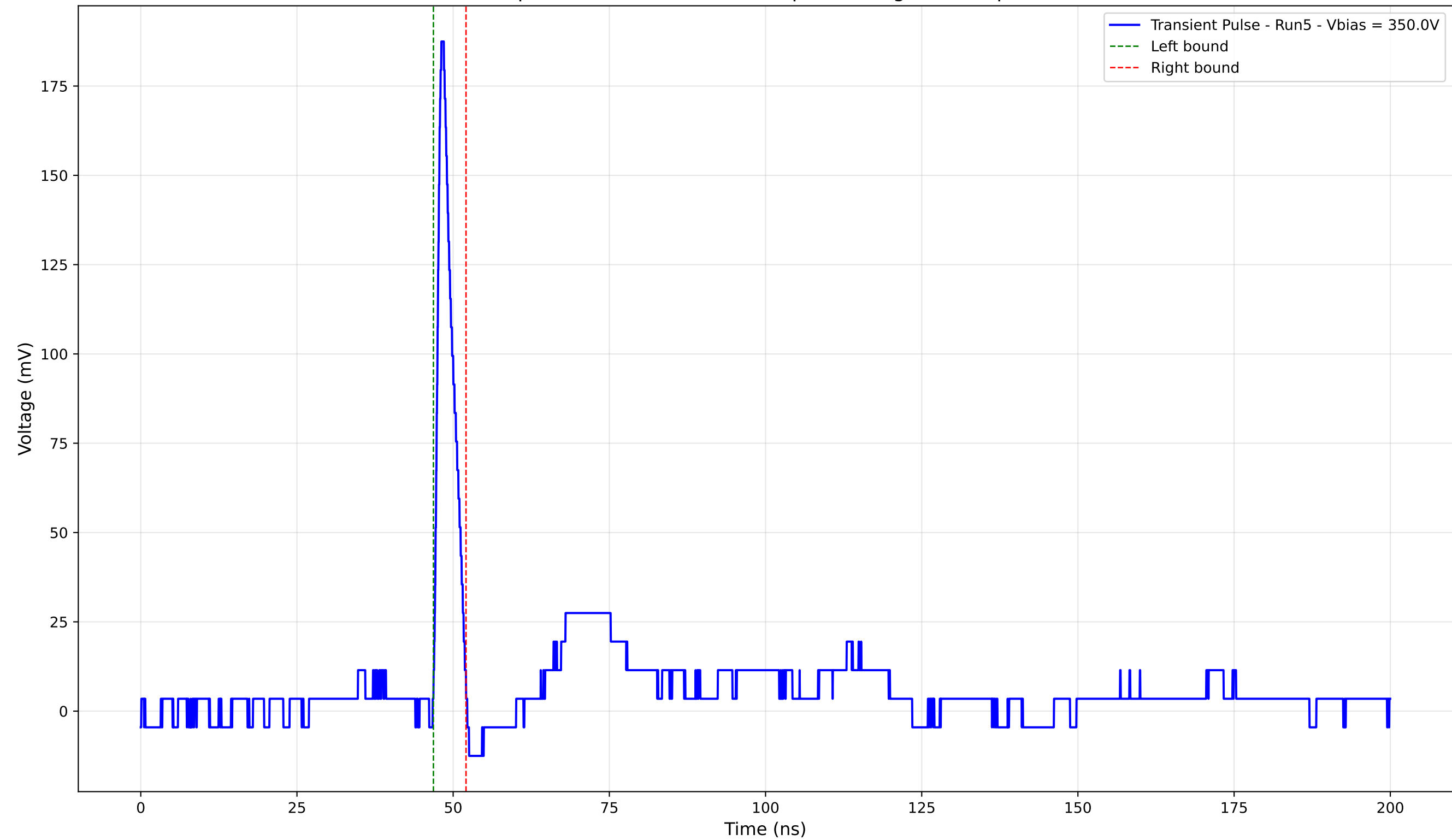
Transient Pulse - Sample: 4003 - Position: 510.0 \mu\text{m} - Charge: 10.20 pC - Rise Time: 0.94 ns
