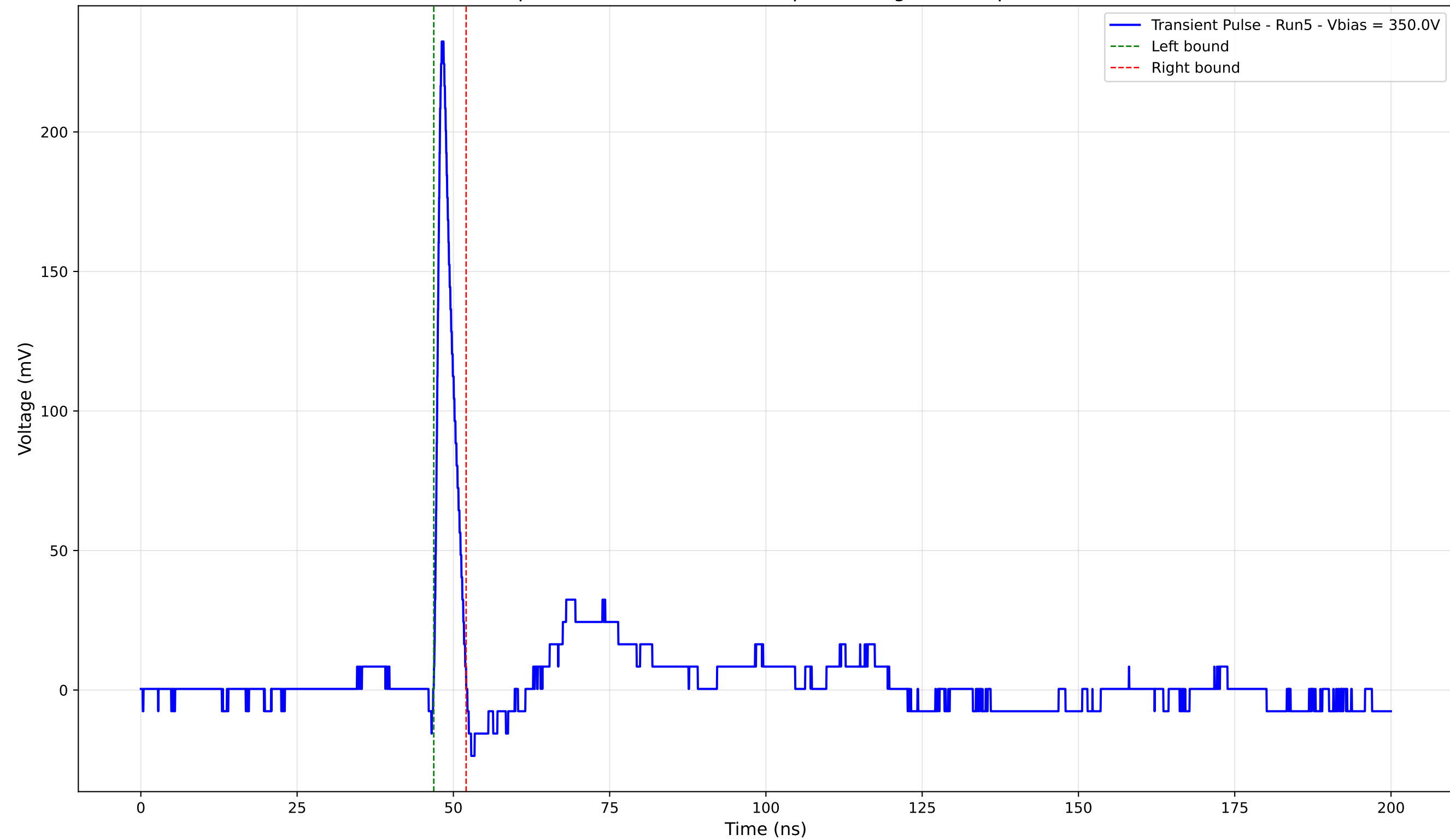
Transient Pulse - Sample: 4003 - Position: 475.0 \mu\text{m} - Charge: 11.99 pC - Rise Time: 0.92 ns
