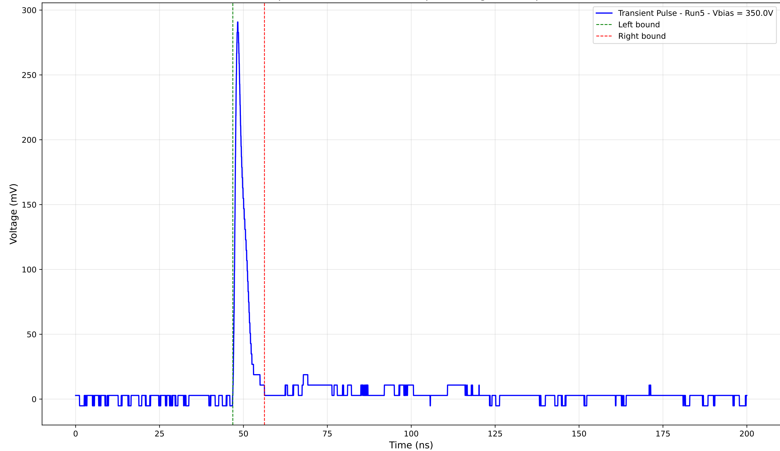
Transient Pulse - Sample: 4003 - Position: 390.0 \mu\text{m} - Charge: 17.97 pC - Rise Time: 0.95 ns
