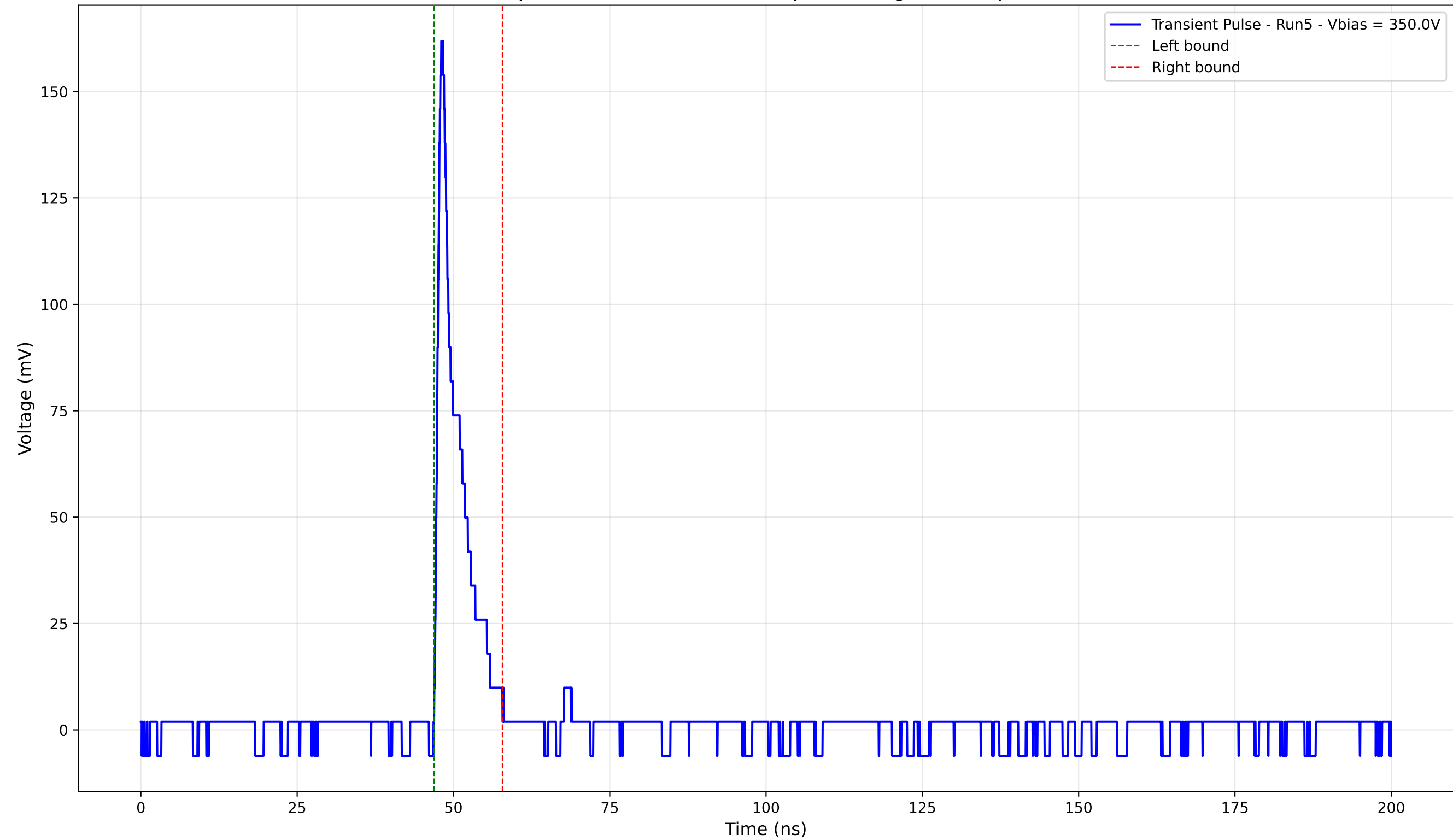
Transient Pulse - Sample: 4003 - Position: 160.0 \mu\text{m} - Charge: 11.90 pC - Rise Time: 0.82 ns
