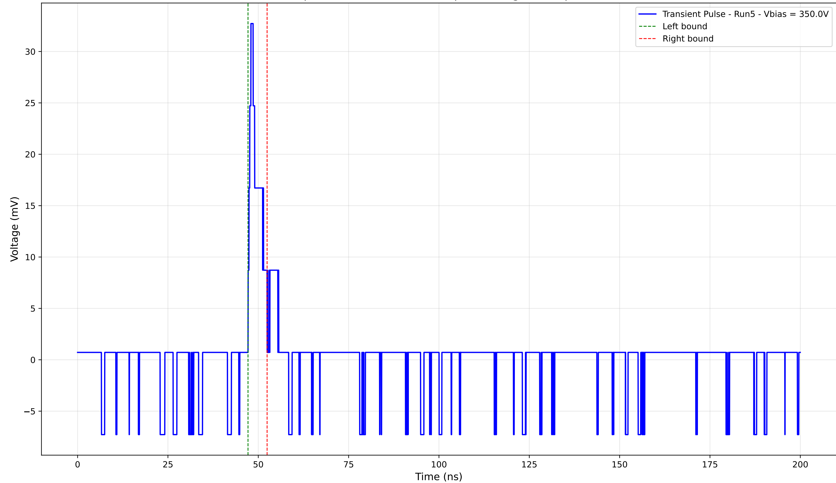
Transient Pulse - Sample: 4003 - Position: 45.0 \mu\text{m} - Charge: 1.88 pC - Rise Time: 0.79 ns
