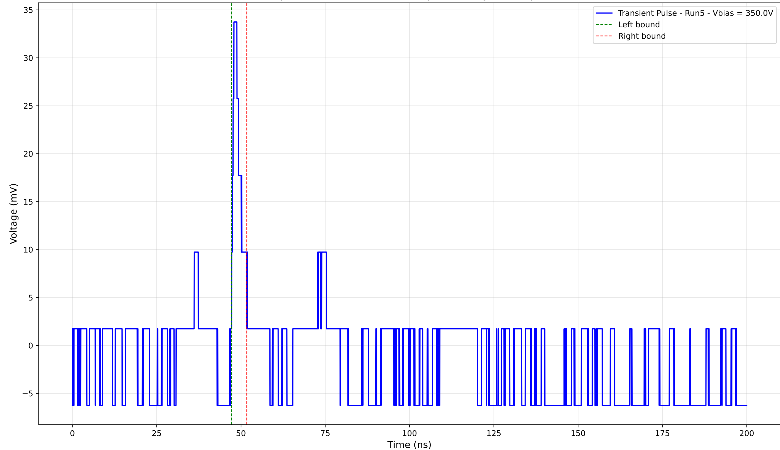
Transient Pulse - Sample: 4003 - Position: 615.0 \mu\text{m} - Charge: 1.71 pC - Rise Time: 0.68 ns
