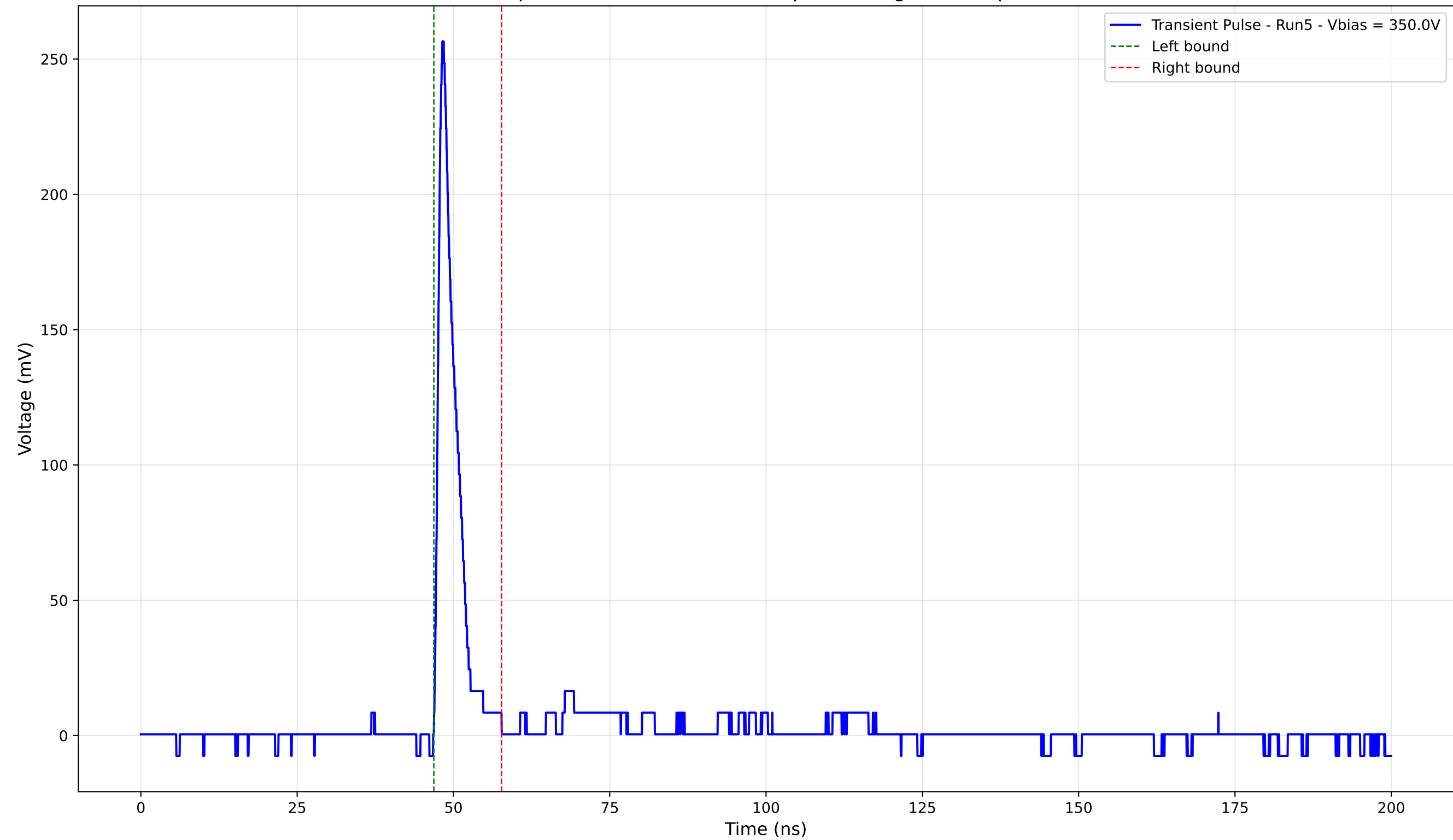
Transient Pulse - Sample: 4003 - Position: 430.0 \mu\text{m} - Charge: 16.08 pC - Rise Time: 0.90 ns
