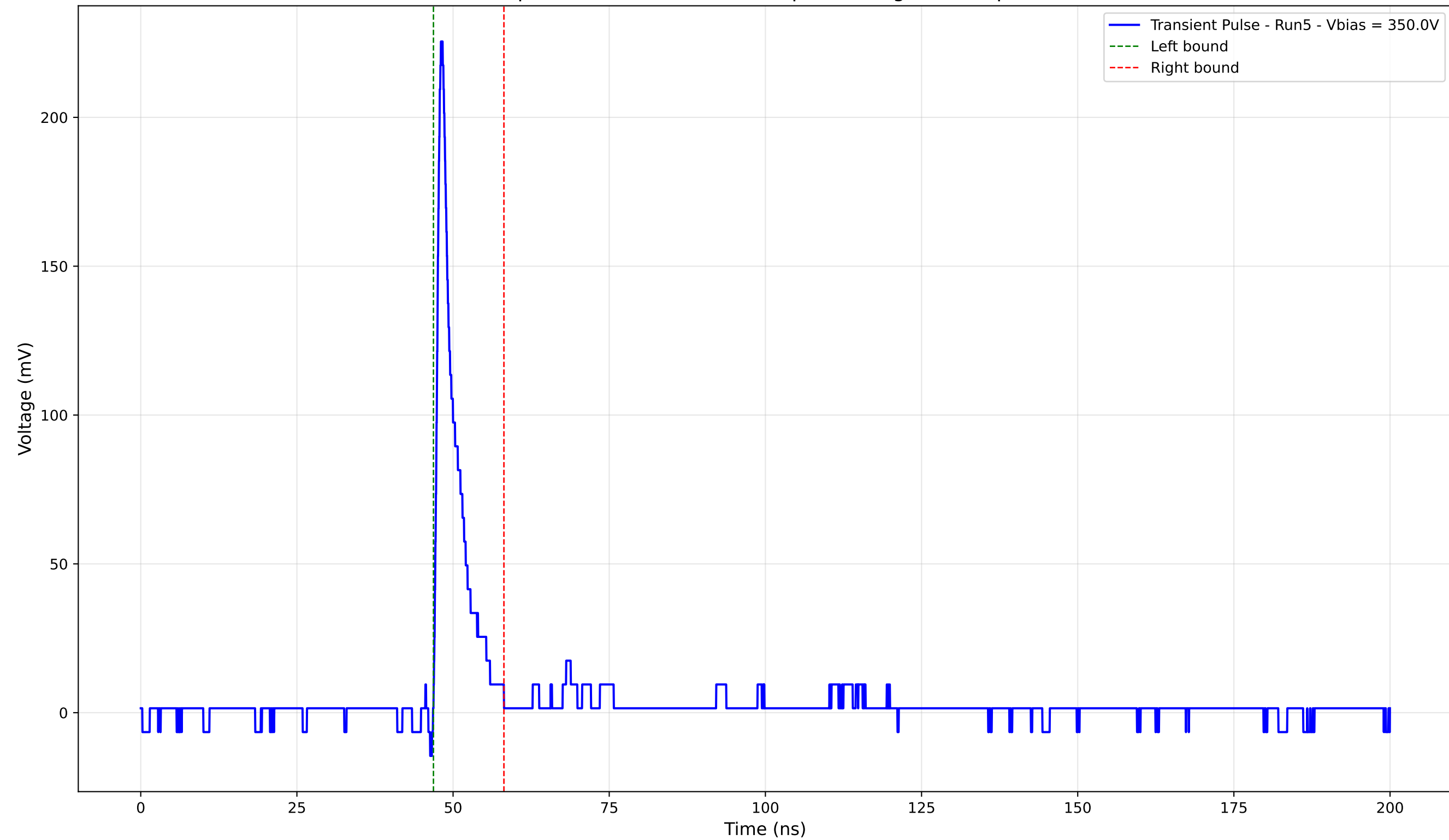
Transient Pulse - Sample: 4003 - Position: 210.0 \mu\text{m} - Charge: 15.02 pC - Rise Time: 0.89 ns
