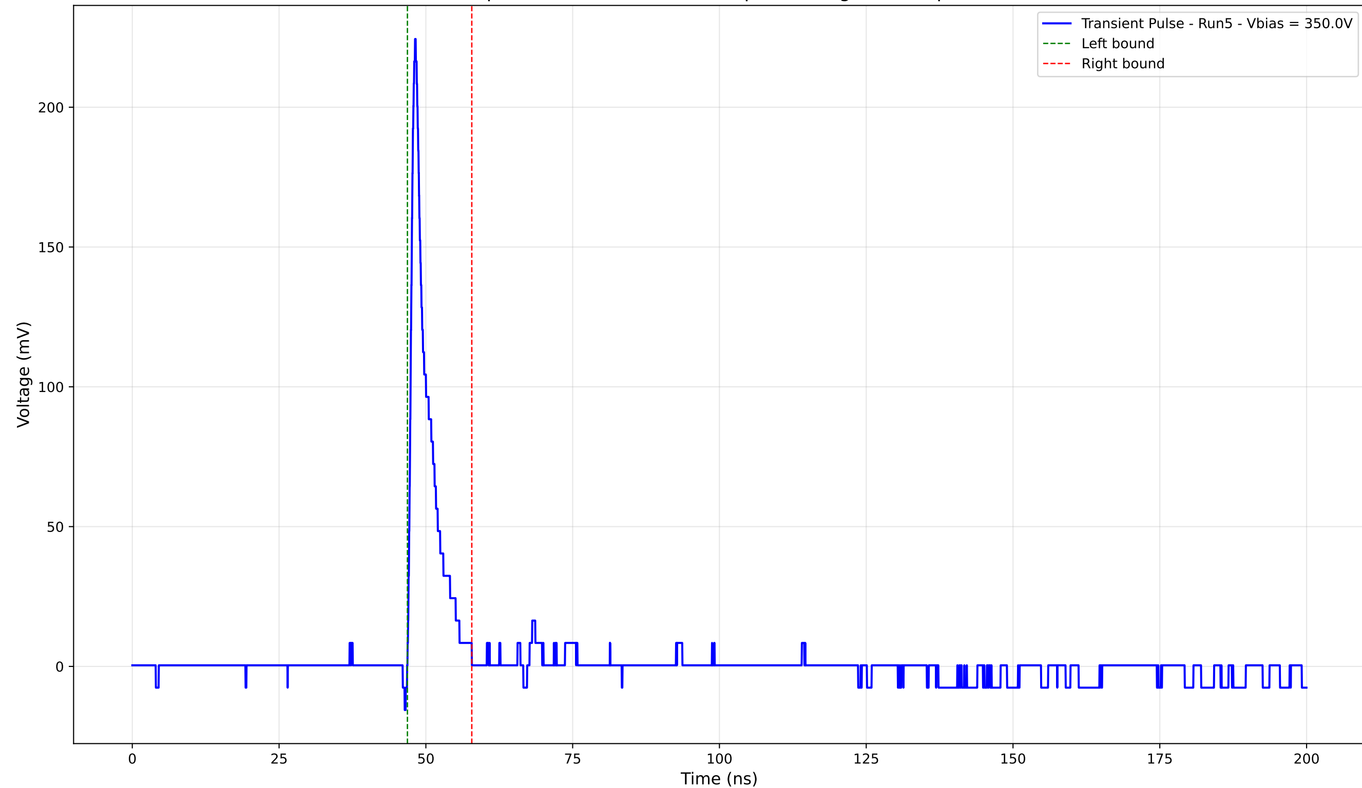
Transient Pulse - Sample: 4003 - Position: 205.0 \mu\text{m} - Charge: 14.64 pC - Rise Time: 0.90 ns
