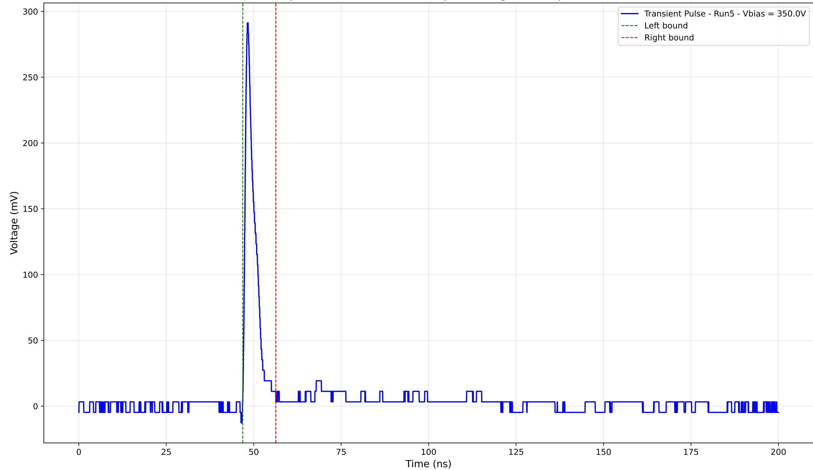
Transient Pulse - Sample: 4003 - Position: 385.0 \mu\text{m} - Charge: 18.27 pC - Rise Time: 0.94 ns
