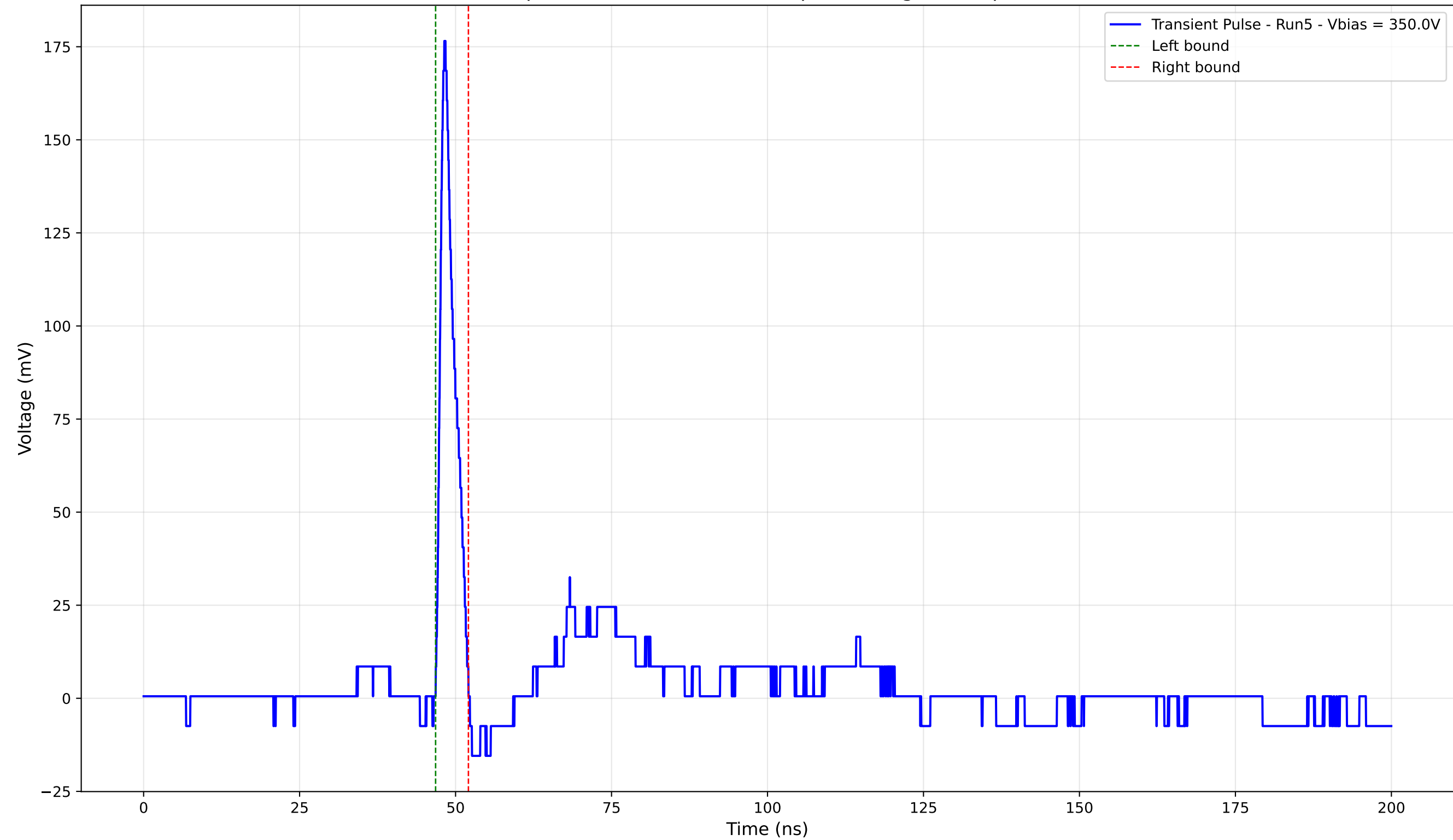
Transient Pulse - Sample: 4003 - Position: 535.0 \mu\text{m} - Charge: 9.15 pC - Rise Time: 0.94 ns
