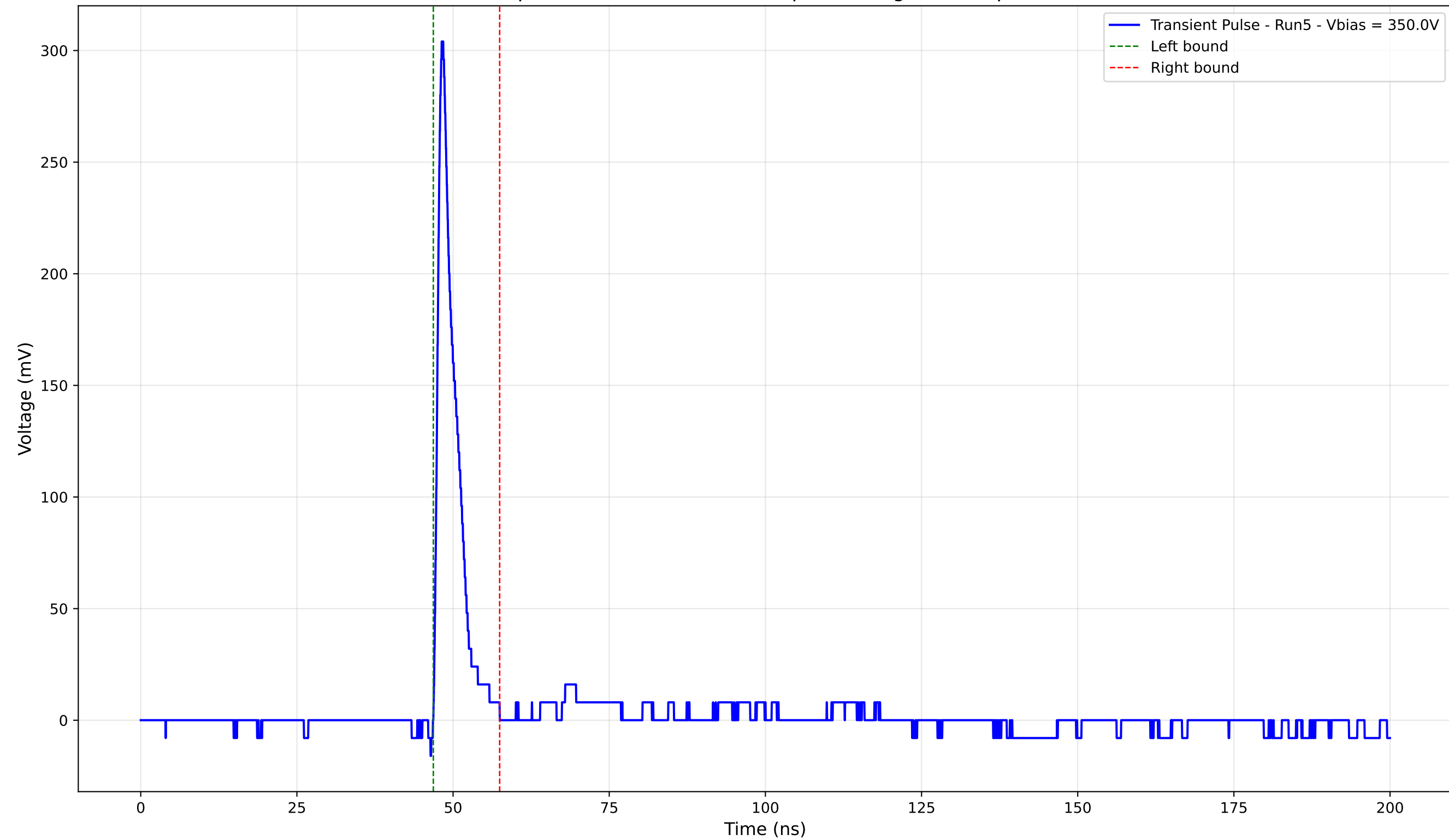
Transient Pulse - Sample: 4003 - Position: 350.0 \mu\text{m} - Charge: 19.39 pC - Rise Time: 0.94 ns
