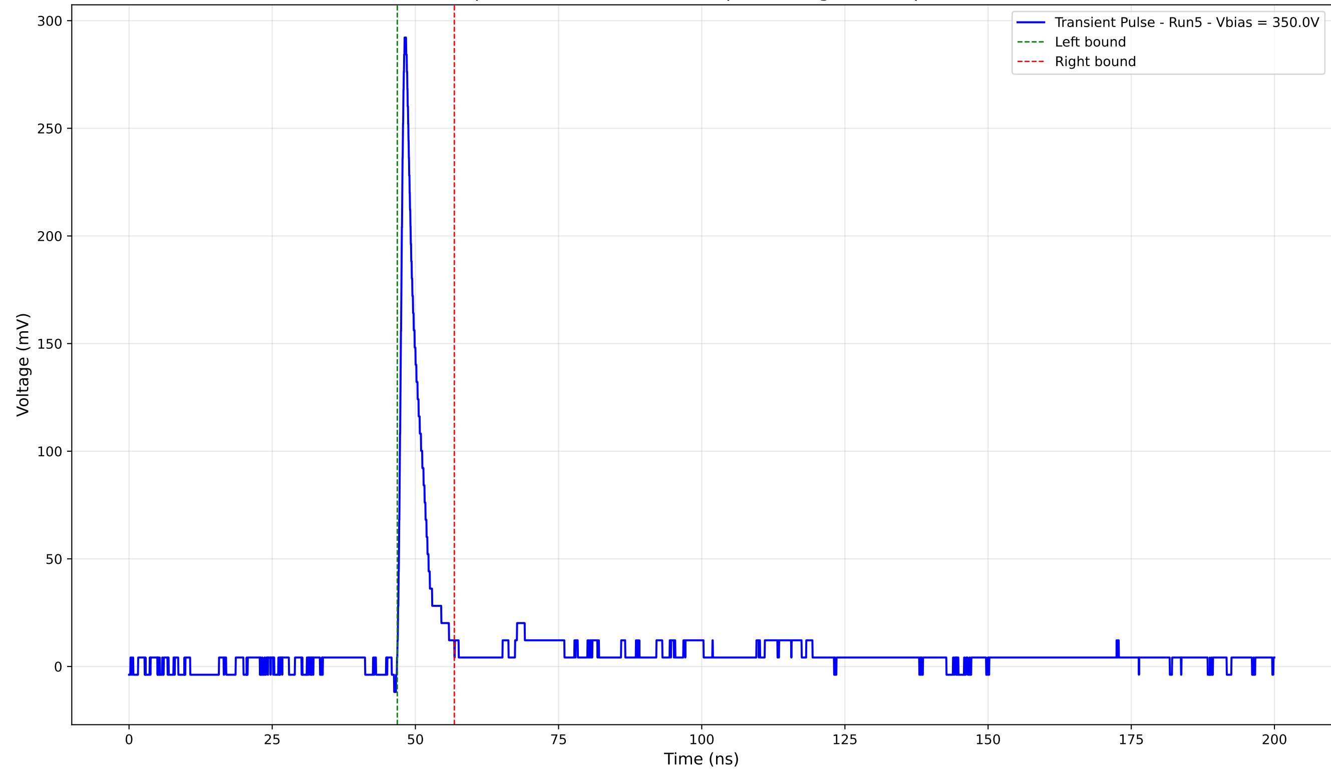
Transient Pulse - Sample: 4003 - Position: 285.0 \mu\text{m} - Charge: 18.70 pC - Rise Time: 0.90 ns
