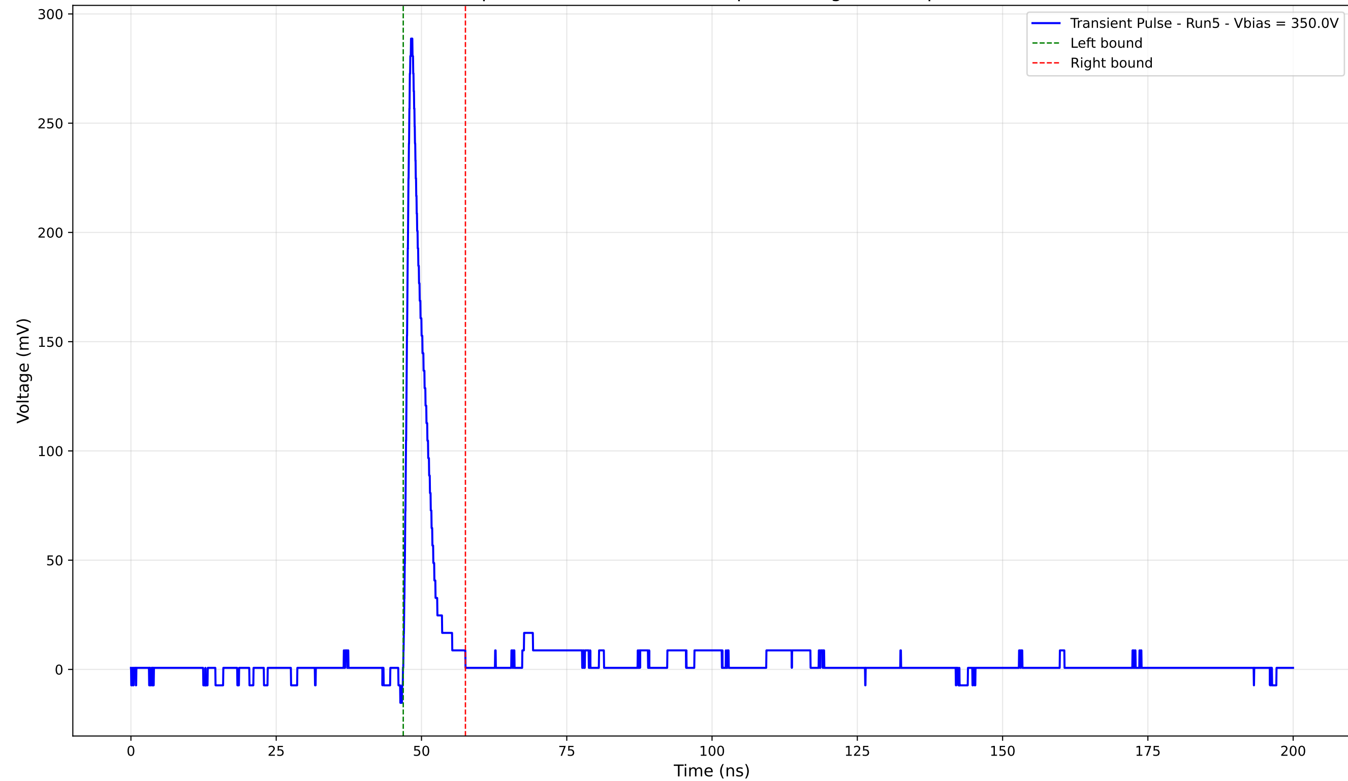
Transient Pulse - Sample: 4003 - Position: 375.0 \mu\text{m} - Charge: 18.33 pC - Rise Time: 0.93 ns
