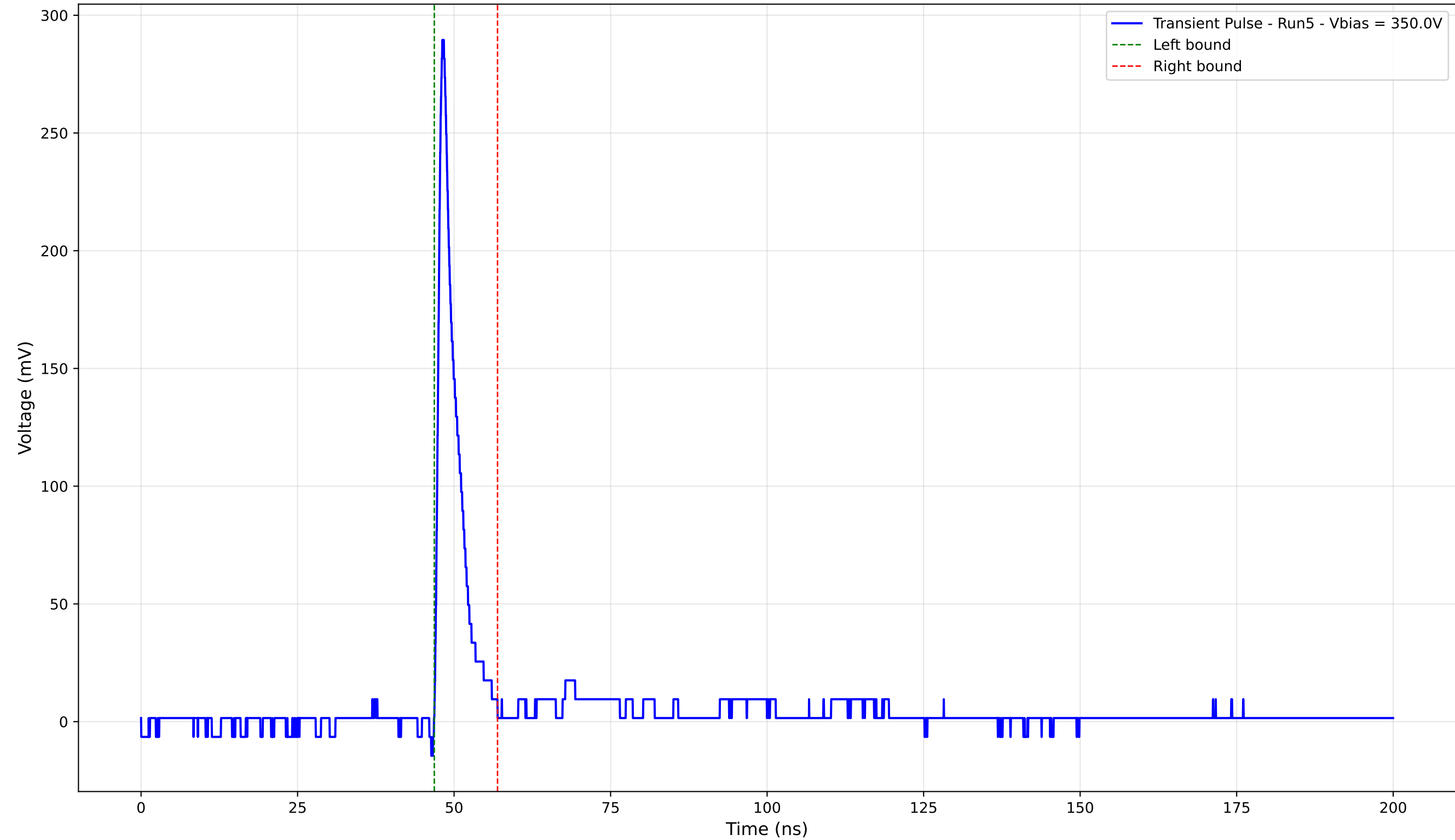
Transient Pulse - Sample: 4003 - Position: 290.0 \mu\text{m} - Charge: 18.74 pC - Rise Time: 0.89 ns
