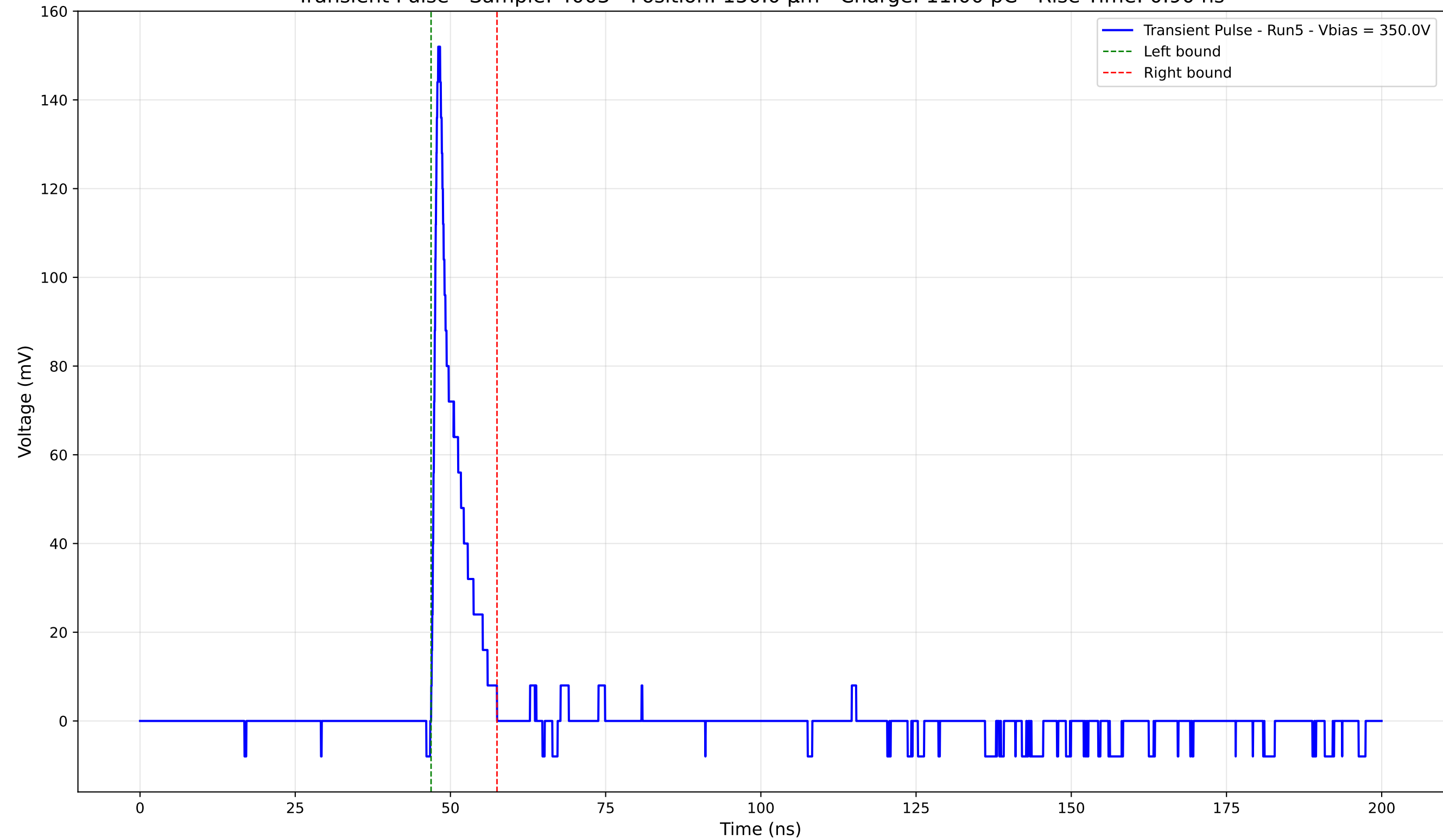
Transient Pulse - Sample: 4003 - Position: 150.0 \mu\text{m} - Charge: 11.00 pC - Rise Time: 0.90 ns
