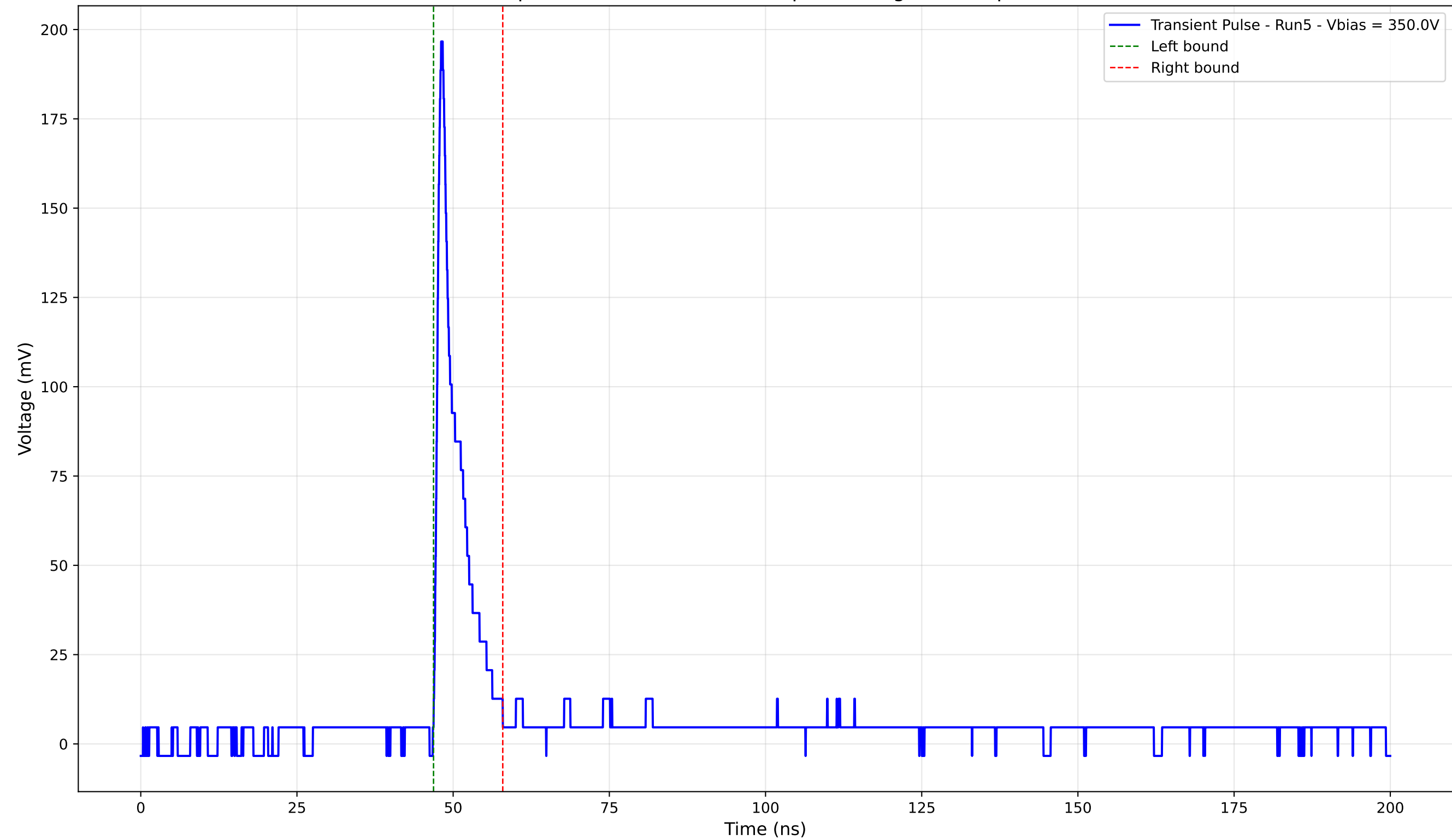
Transient Pulse - Sample: 4003 - Position: 180.0 \mu\text{m} - Charge: 14.50 pC - Rise Time: 0.92 ns
