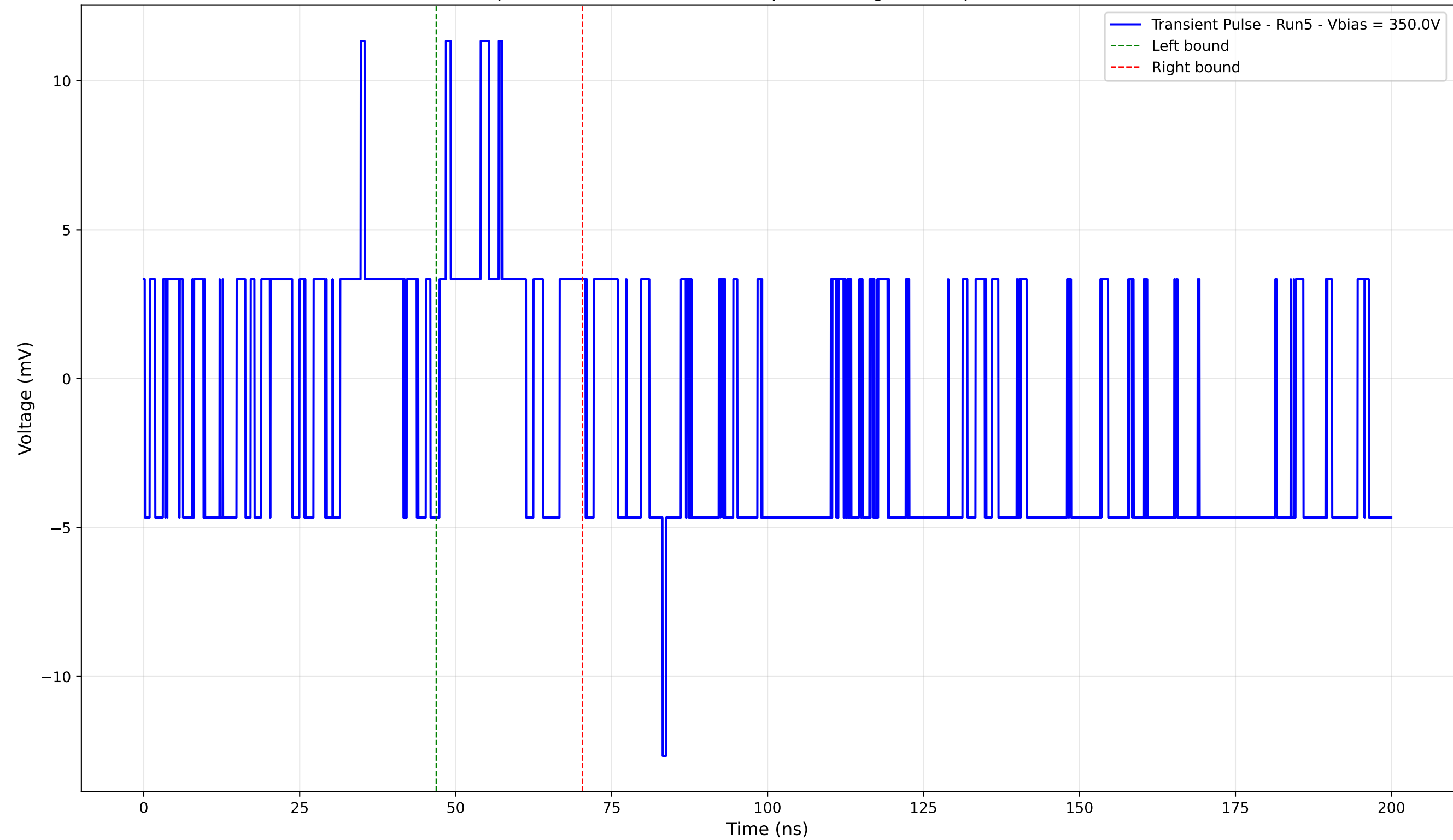
Transient Pulse - Sample: 4003 - Position: 645.0 \mu\text{m} - Charge: 1.29 pC - Rise Time: 0.00 ns (N/A)
