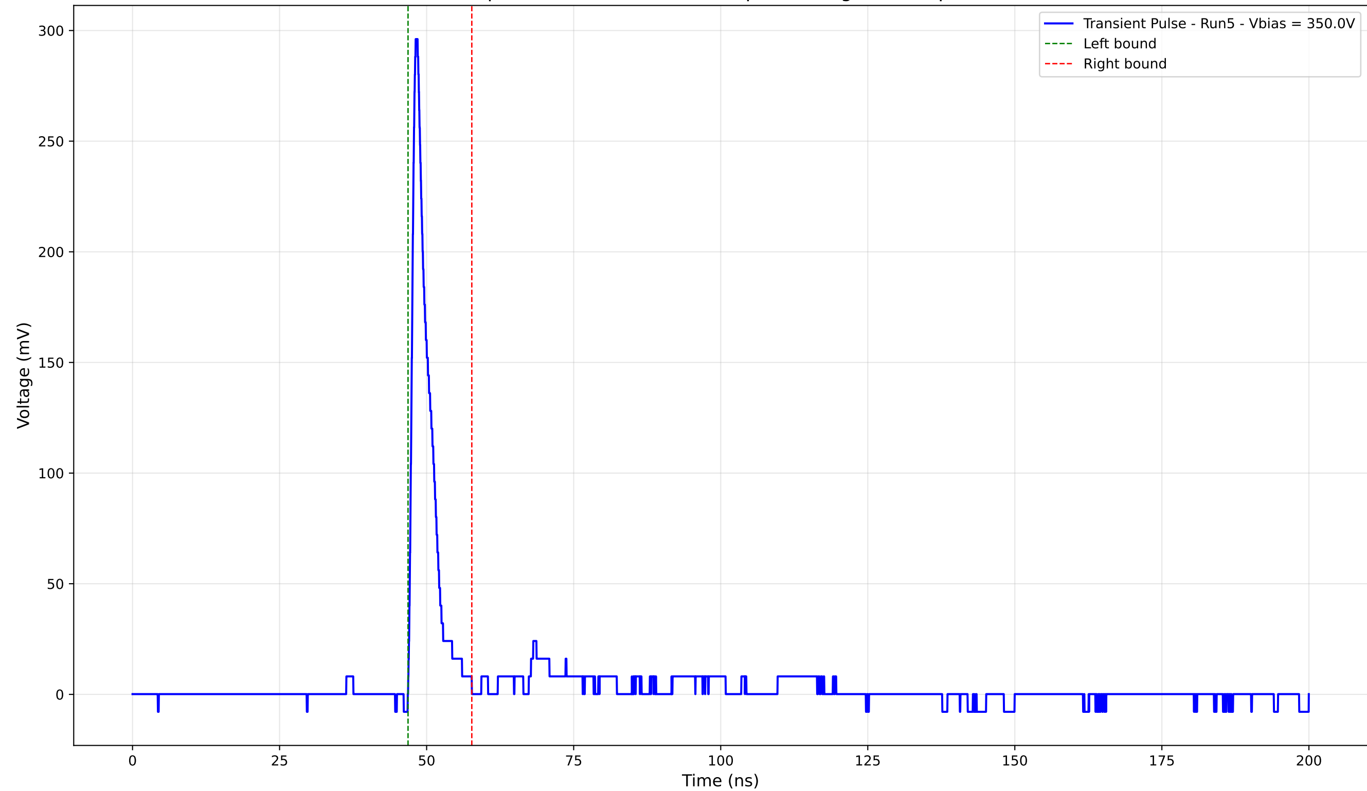
Transient Pulse - Sample: 4003 - Position: 365.0 \mu\text{m} - Charge: 19.14 pC - Rise Time: 0.91 ns
