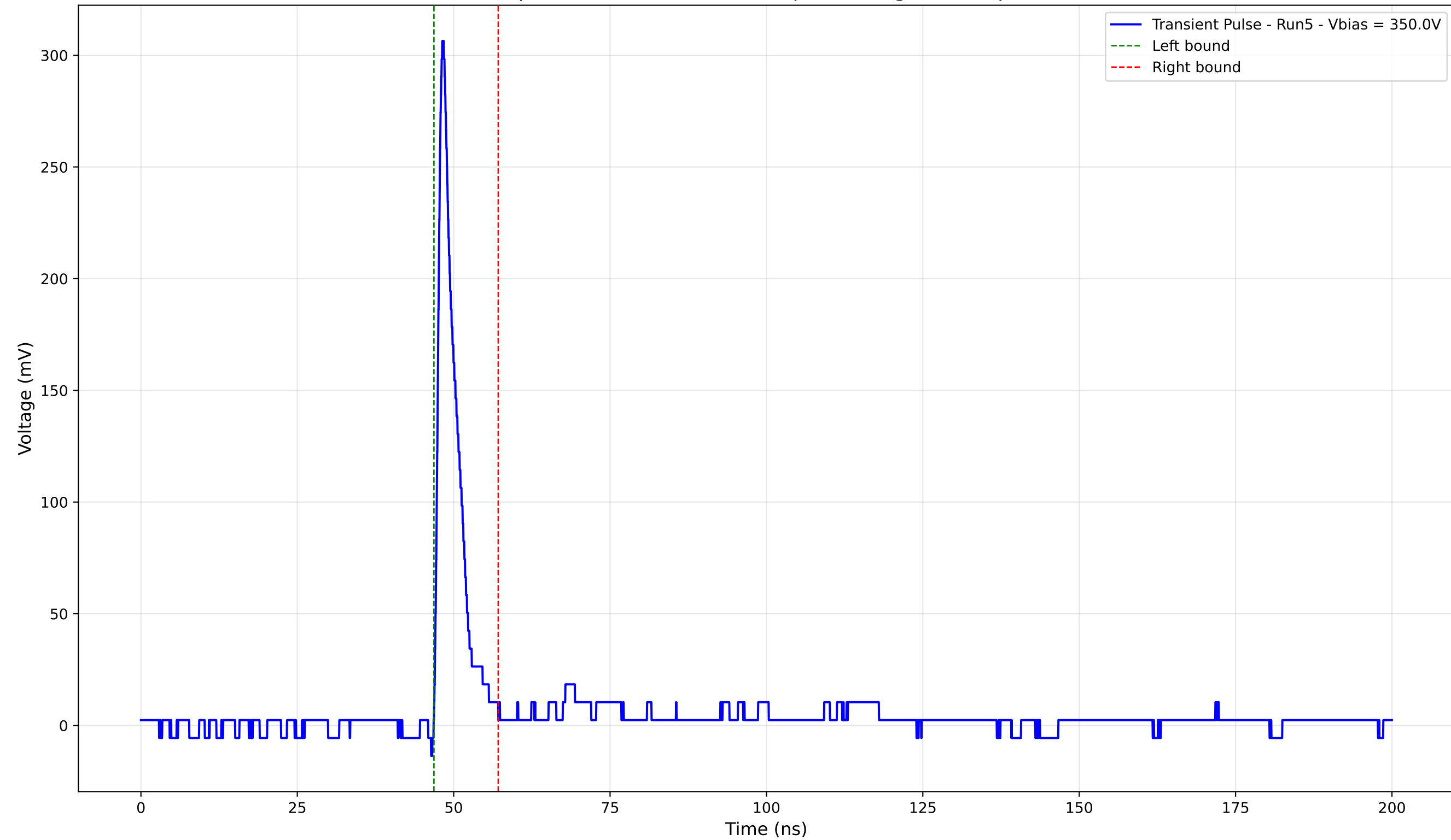
Transient Pulse - Sample: 4003 - Position: 345.0 \mu\text{m} - Charge: 19.79 pC - Rise Time: 0.93 ns
