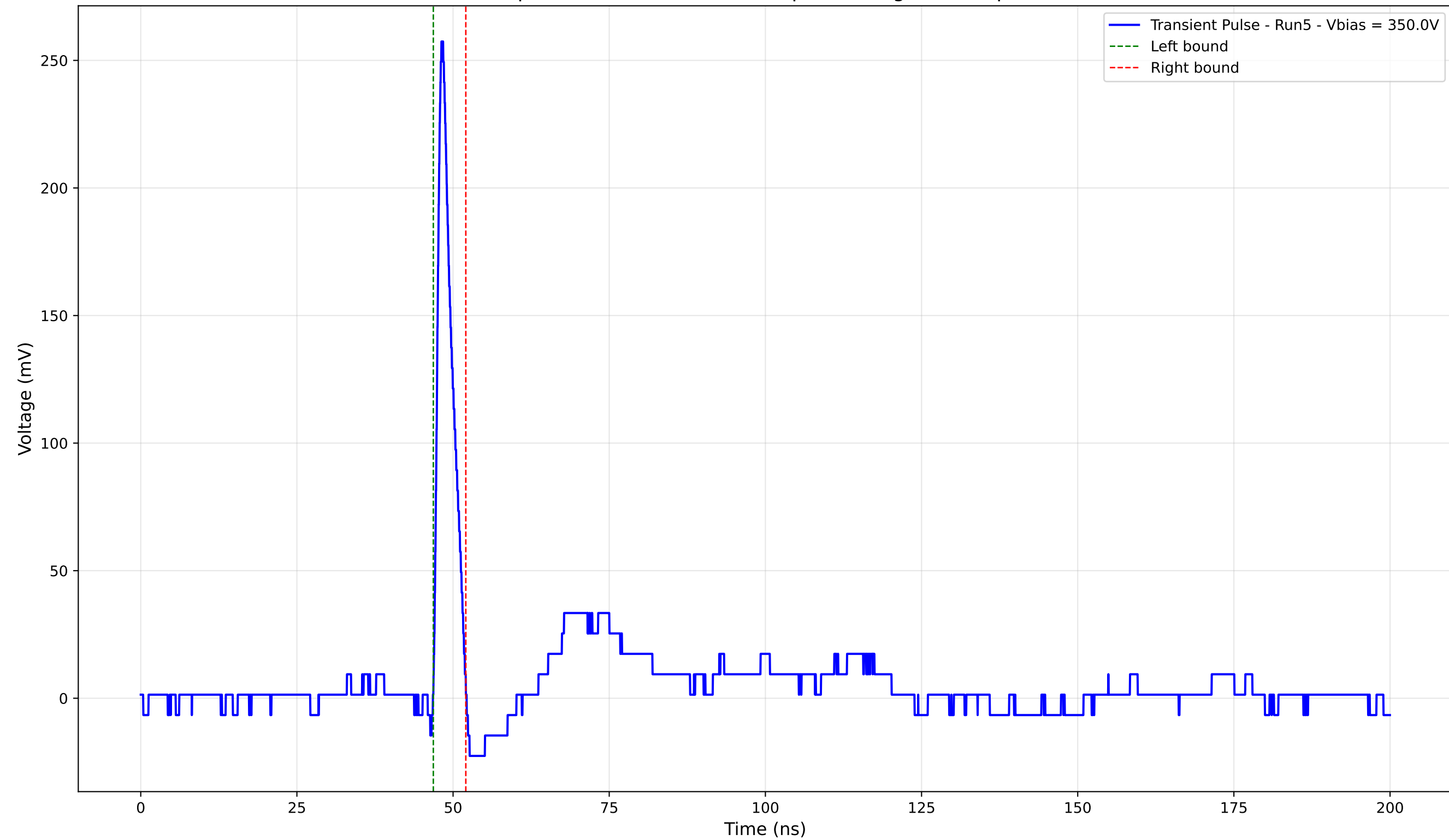
Transient Pulse - Sample: 4003 - Position: 455.0 \mu\text{m} - Charge: 13.34 pC - Rise Time: 0.88 ns
