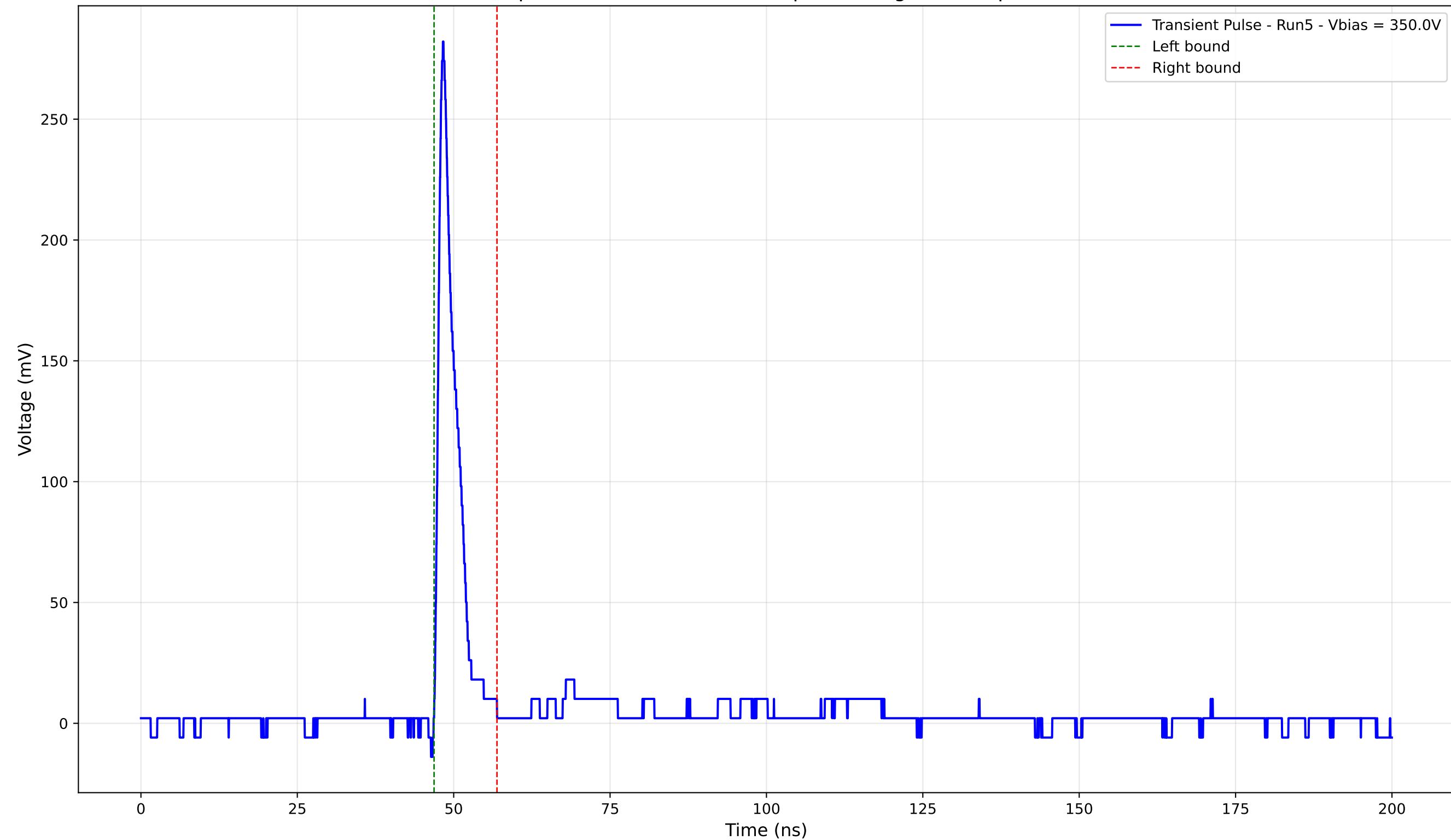
Transient Pulse - Sample: 4003 - Position: 400.0 \mu\text{m} - Charge: 17.55 pC - Rise Time: 0.93 ns
