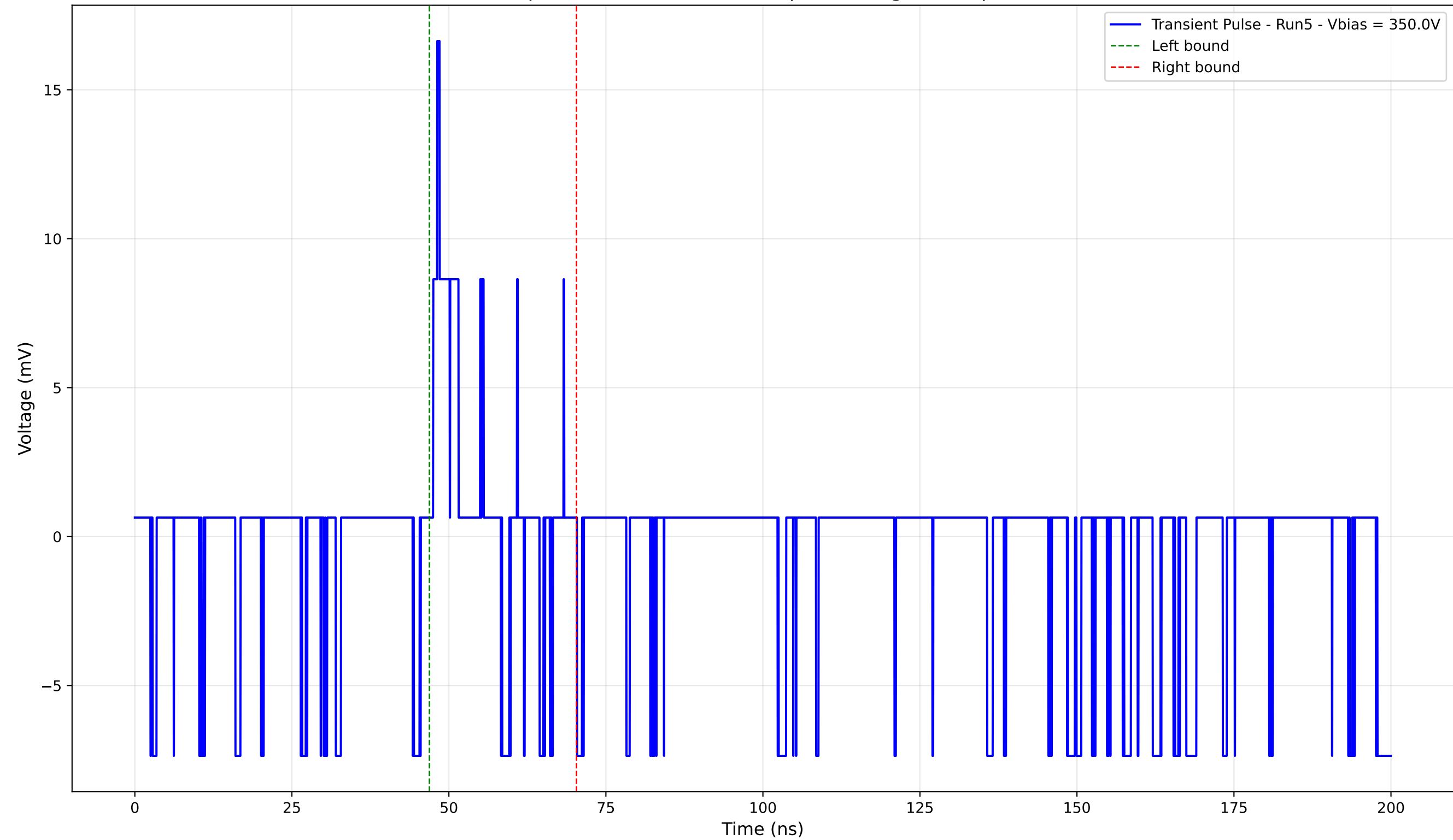
Transient Pulse - Sample: 4003 - Position: 15.0 \mu\text{m} - Charge: 0.70 pC - Rise Time: 0.66 ns
