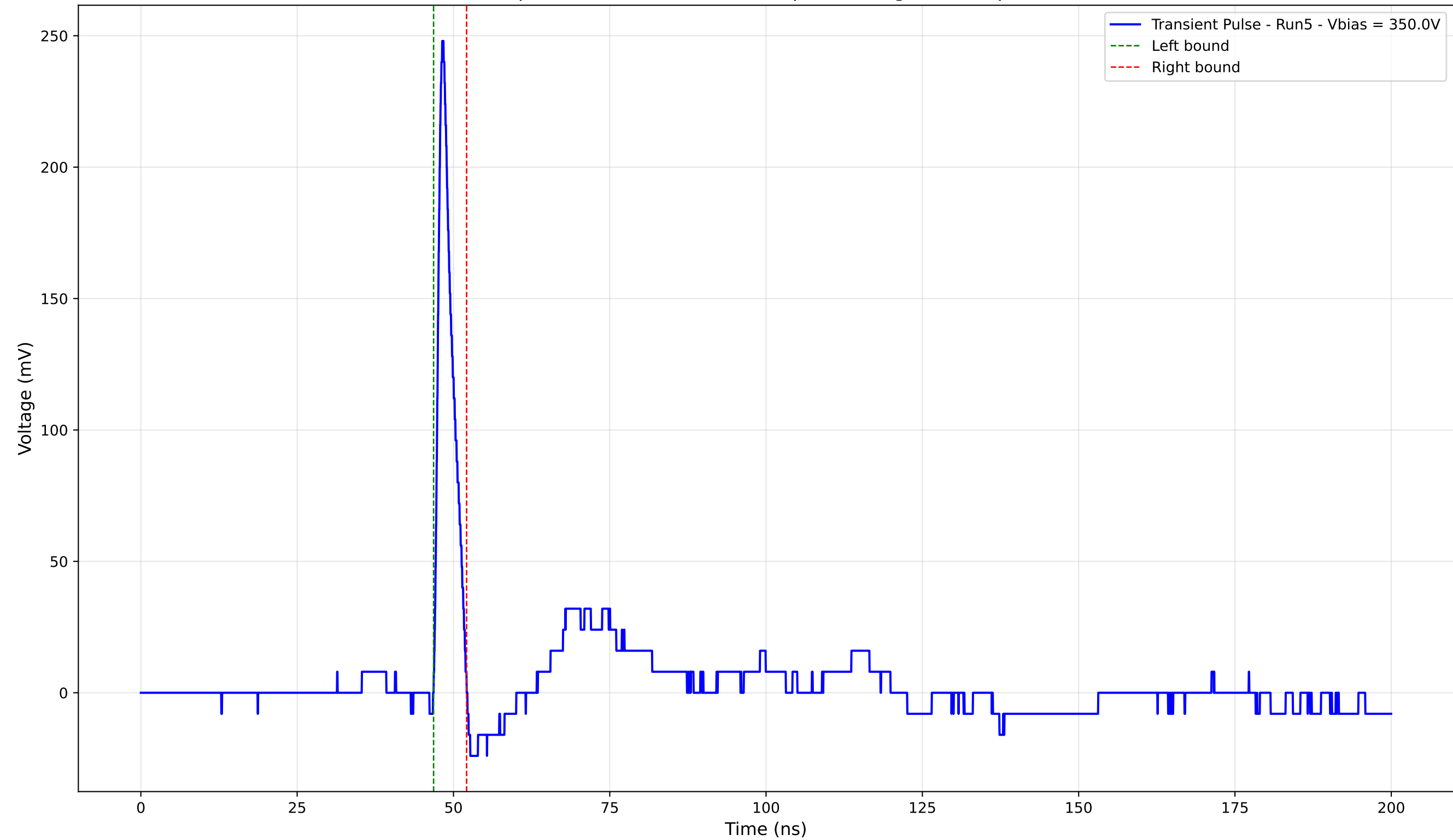
Transient Pulse - Sample: 4003 - Position: 465.0 \mu\text{m} - Charge: 12.84 pC - Rise Time: 0.90 ns
