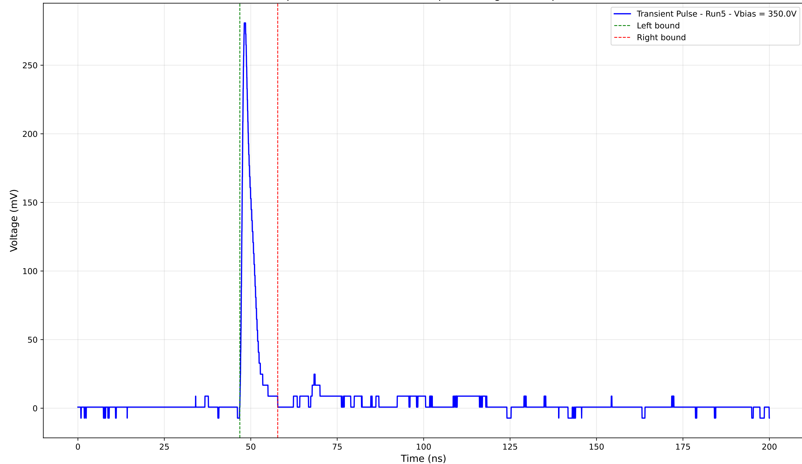
Transient Pulse - Sample: 4003 - Position: 395.0 \mu\text{m} - Charge: 18.07 pC - Rise Time: 0.89 ns
