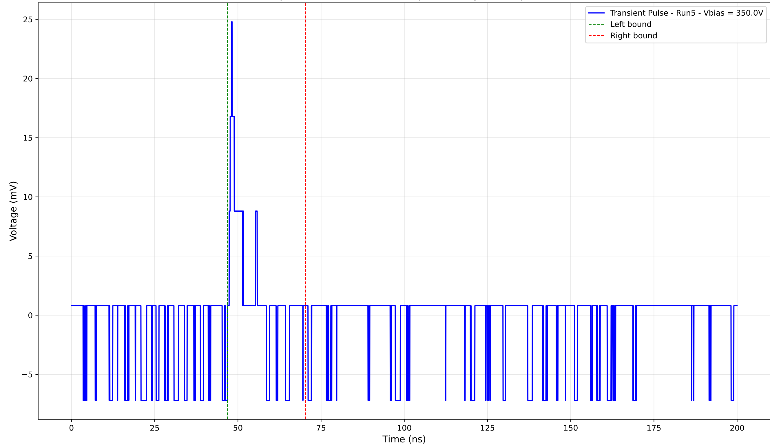
Transient Pulse - Sample: 4003 - Position: 30.0 \mu\text{m} - Charge: 0.91 pC - Rise Time: 0.78 ns
