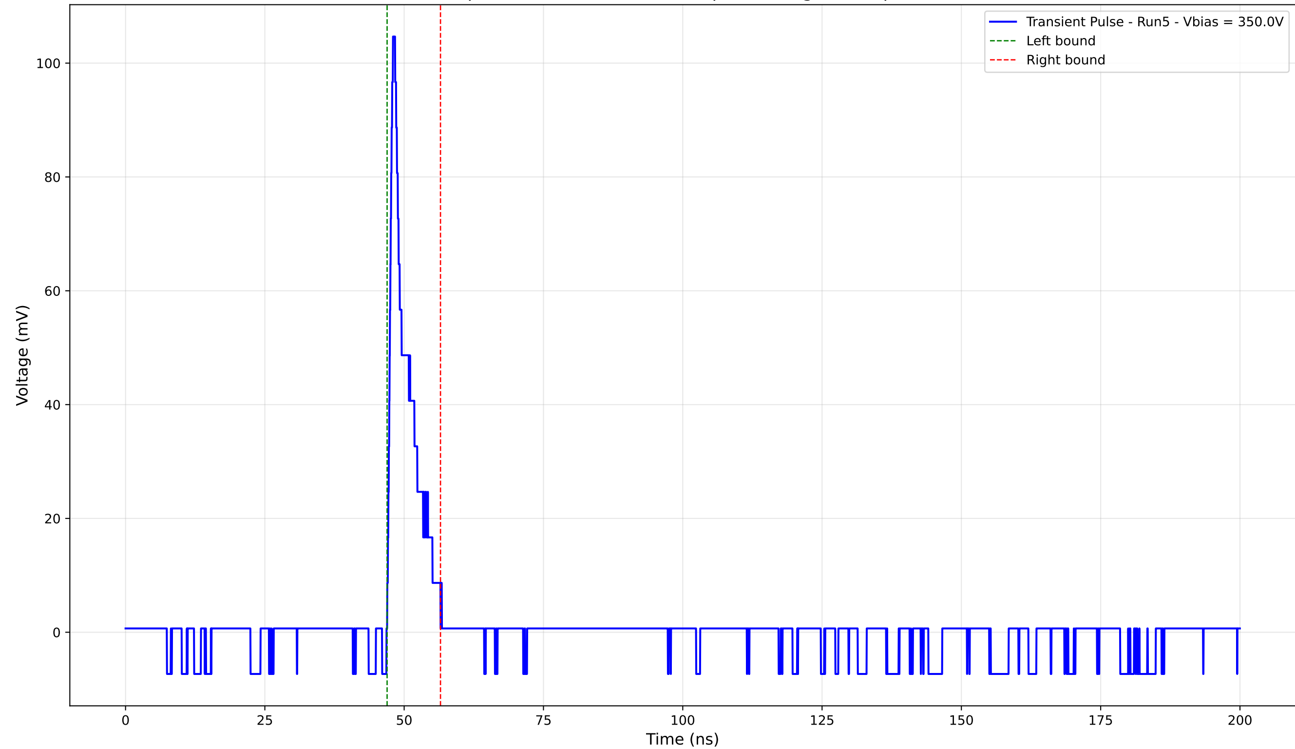
Transient Pulse - Sample: 4003 - Position: 115.0 \mu\text{m} - Charge: 7.44 pC - Rise Time: 0.78 ns
