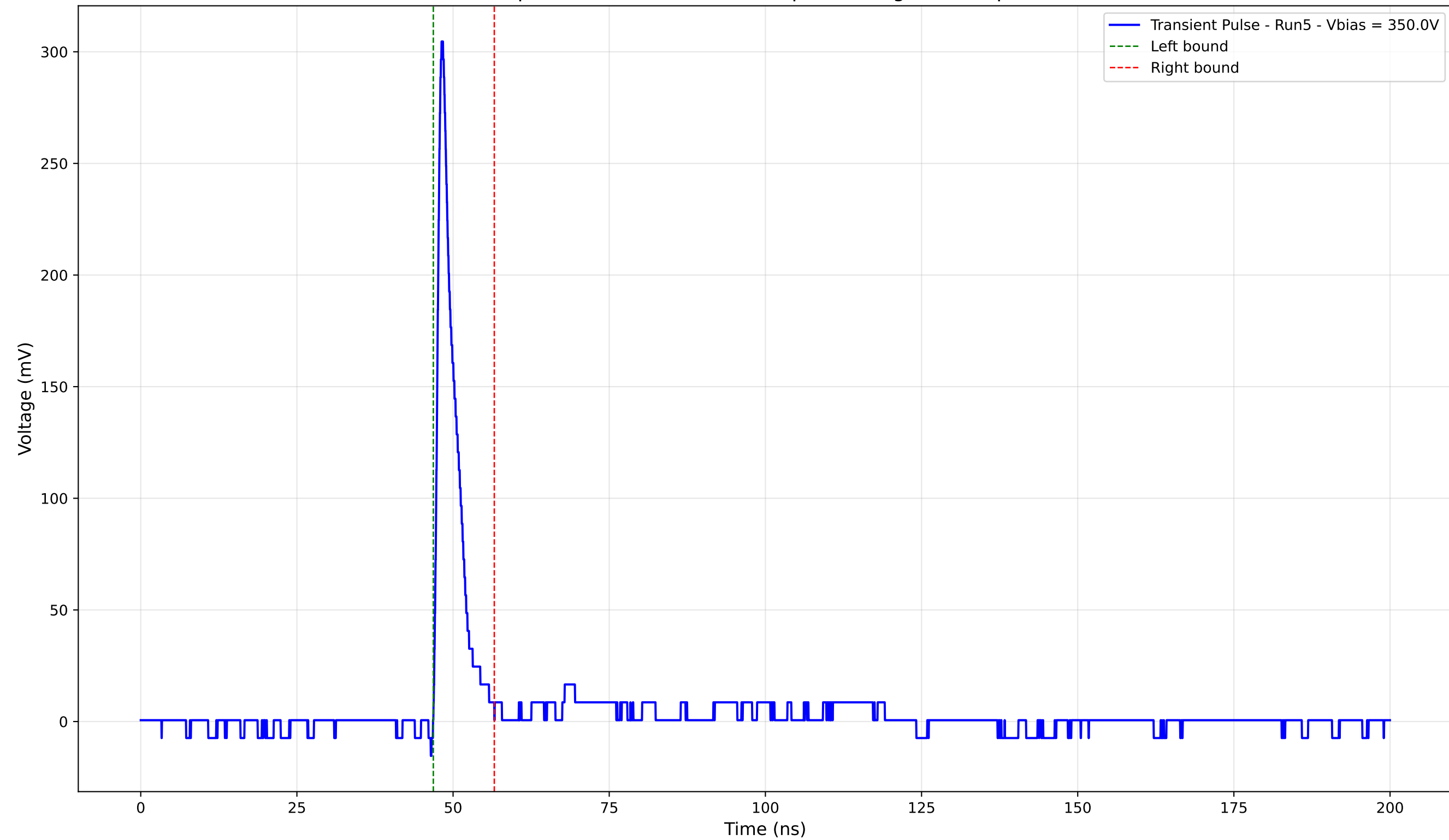
Transient Pulse - Sample: 4003 - Position: 325.0 \mu\text{m} - Charge: 19.18 pC - Rise Time: 0.93 ns
