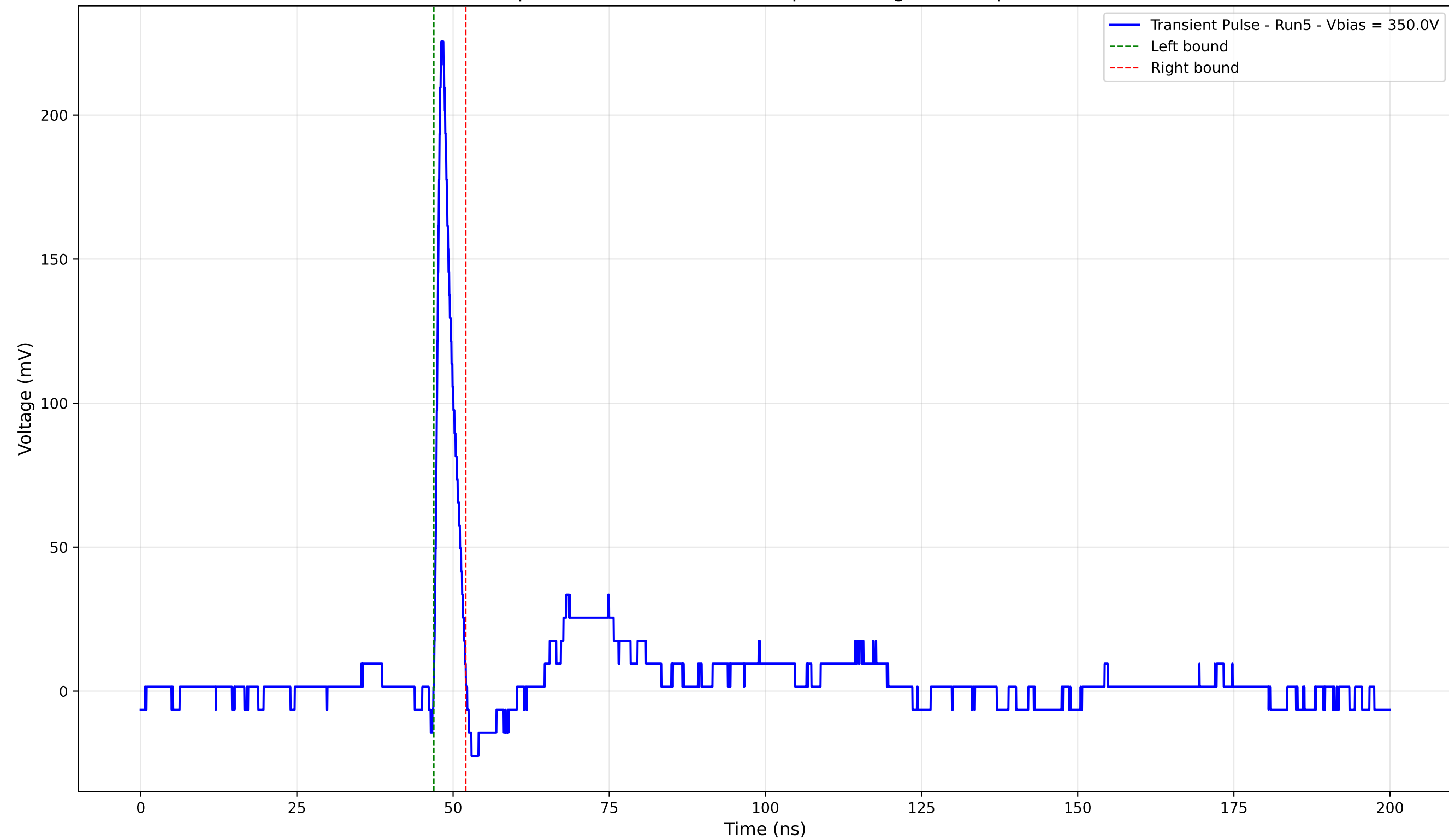
Transient Pulse - Sample: 4003 - Position: 485.0 \mu\text{m} - Charge: 11.49 pC - Rise Time: 0.89 ns
