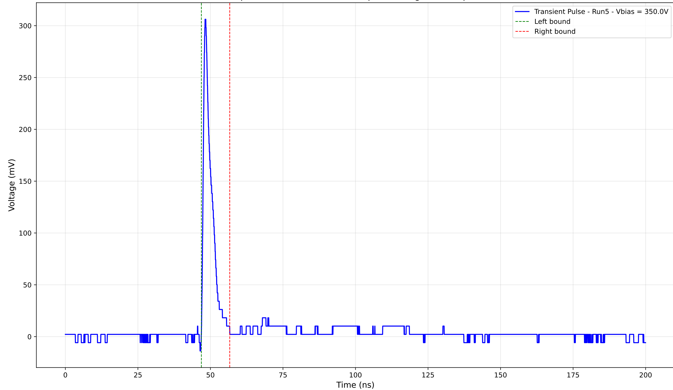
Transient Pulse - Sample: 4003 - Position: 335.0 \mu\text{m} - Charge: 19.50 pC - Rise Time: 0.93 ns
