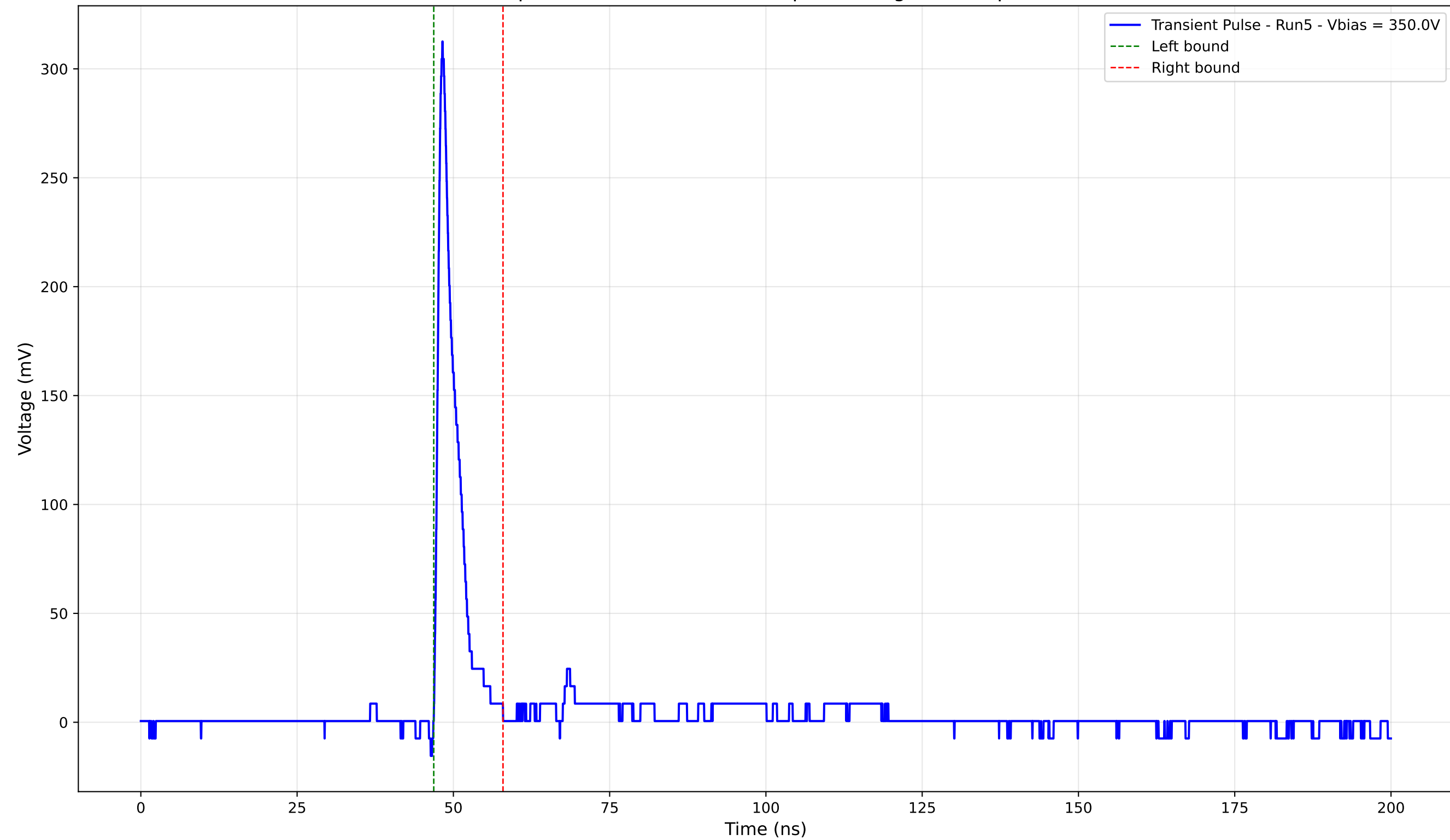
Transient Pulse - Sample: 4003 - Position: 330.0 \mu\text{m} - Charge: 19.85 pC - Rise Time: 0.94 ns
