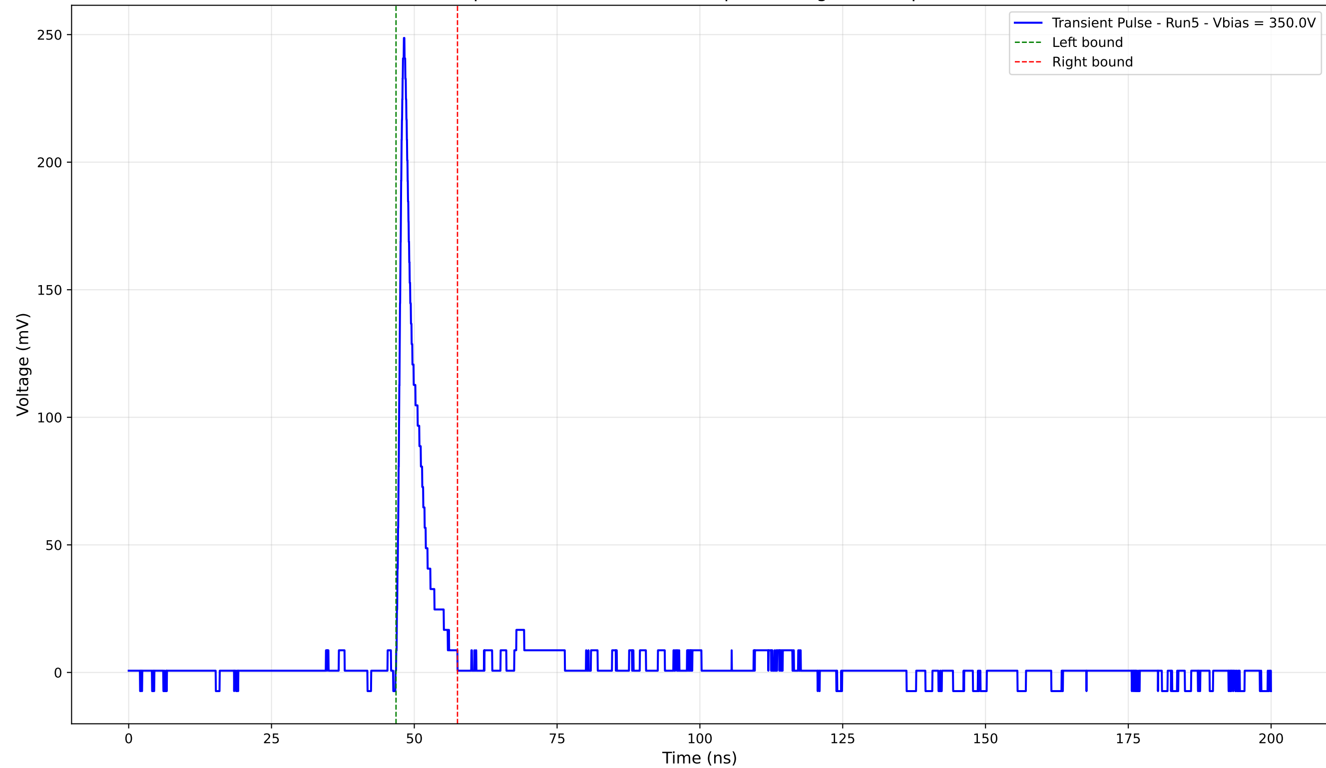
Transient Pulse - Sample: 4003 - Position: 230.0 \mu\text{m} - Charge: 15.96 pC - Rise Time: 0.88 ns
