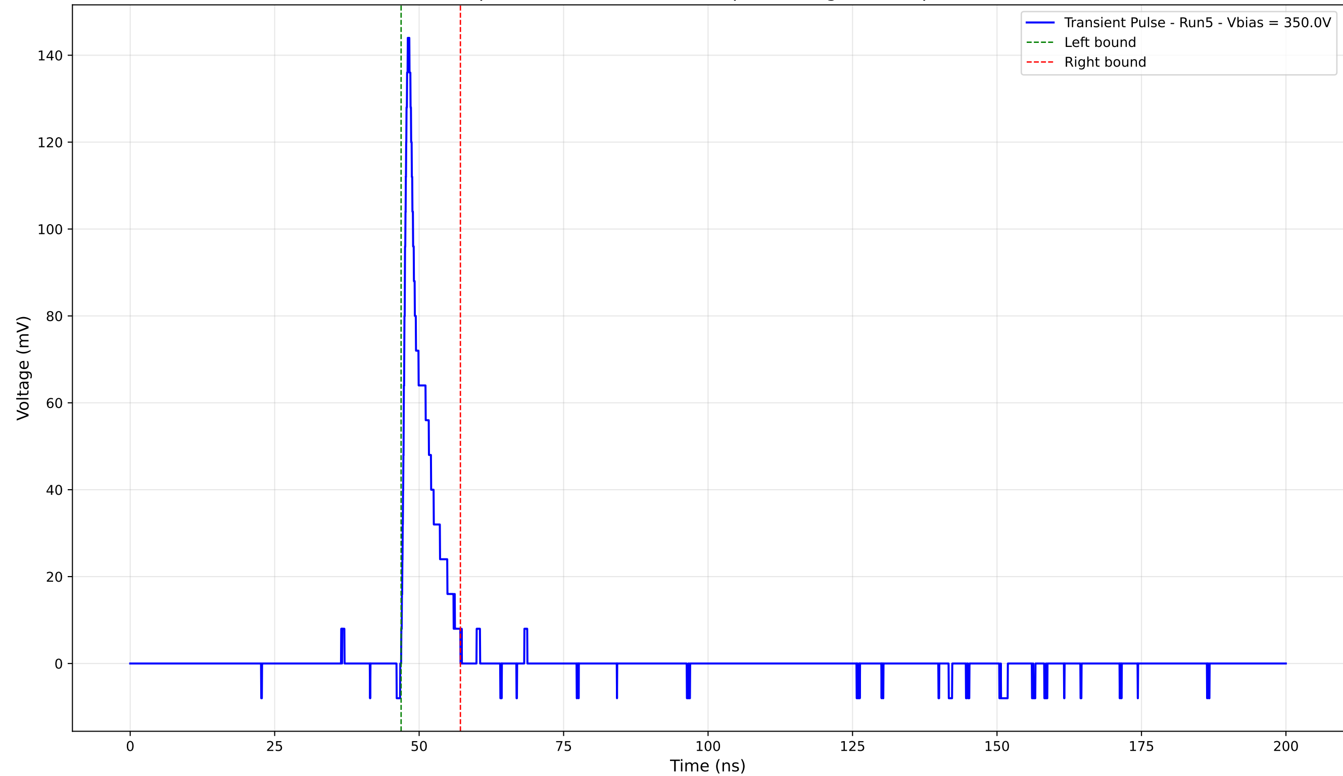
Transient Pulse - Sample: 4003 - Position: 145.0 \mu\text{m} - Charge: 10.34 pC - Rise Time: 0.90 ns
