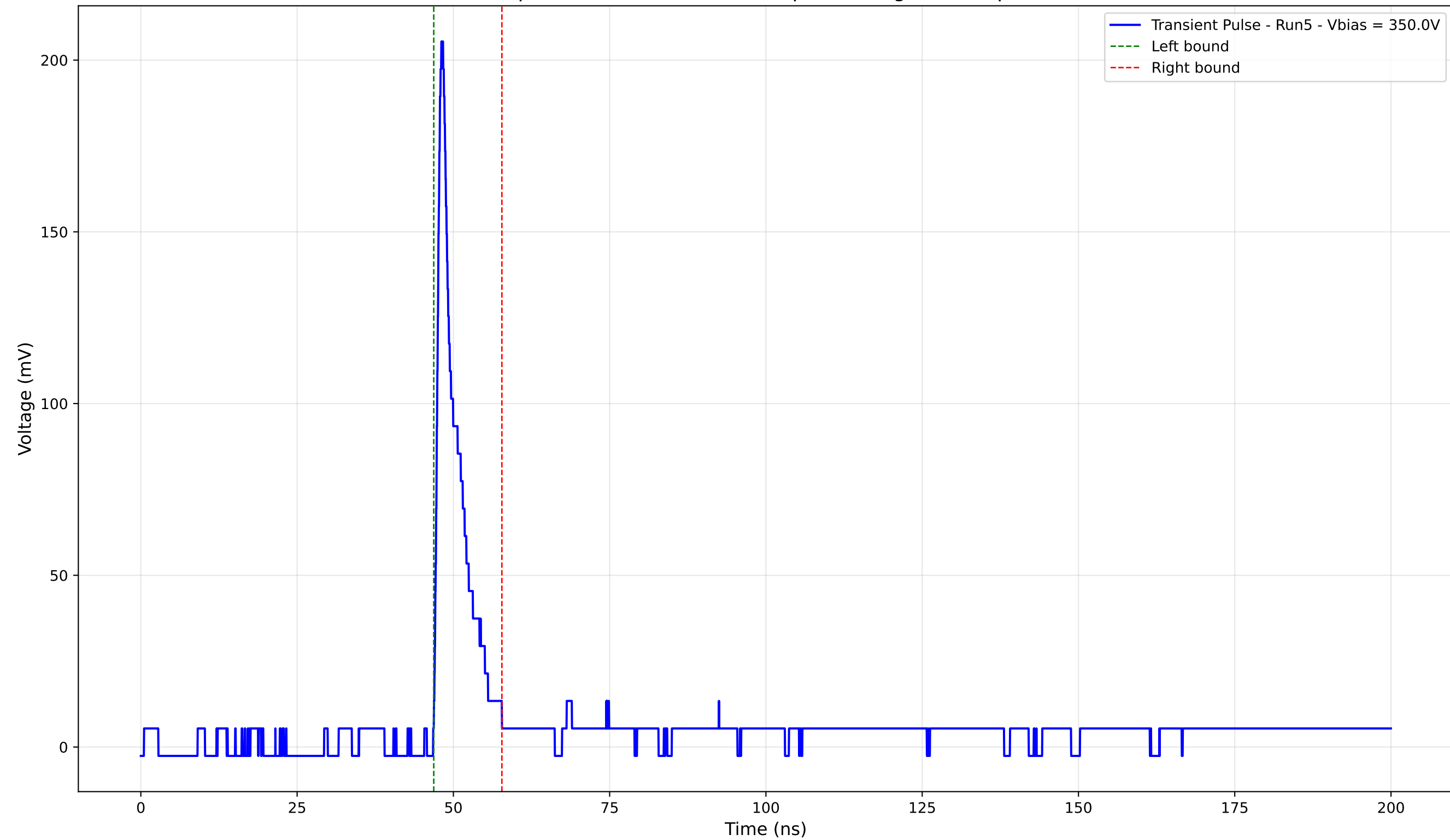
Transient Pulse - Sample: 4003 - Position: 190.0 \mu\text{m} - Charge: 14.82 pC - Rise Time: 0.90 ns
