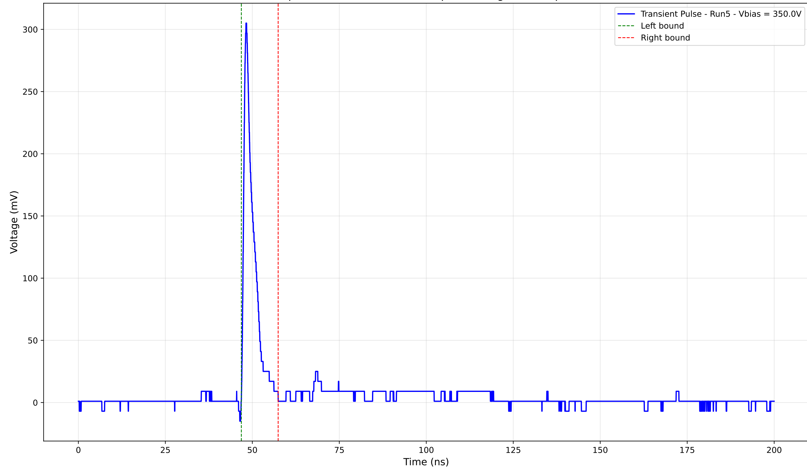
Transient Pulse - Sample: 4003 - Position: 315.0 \mu\text{m} - Charge: 19.44 pC - Rise Time: 0.93 ns
