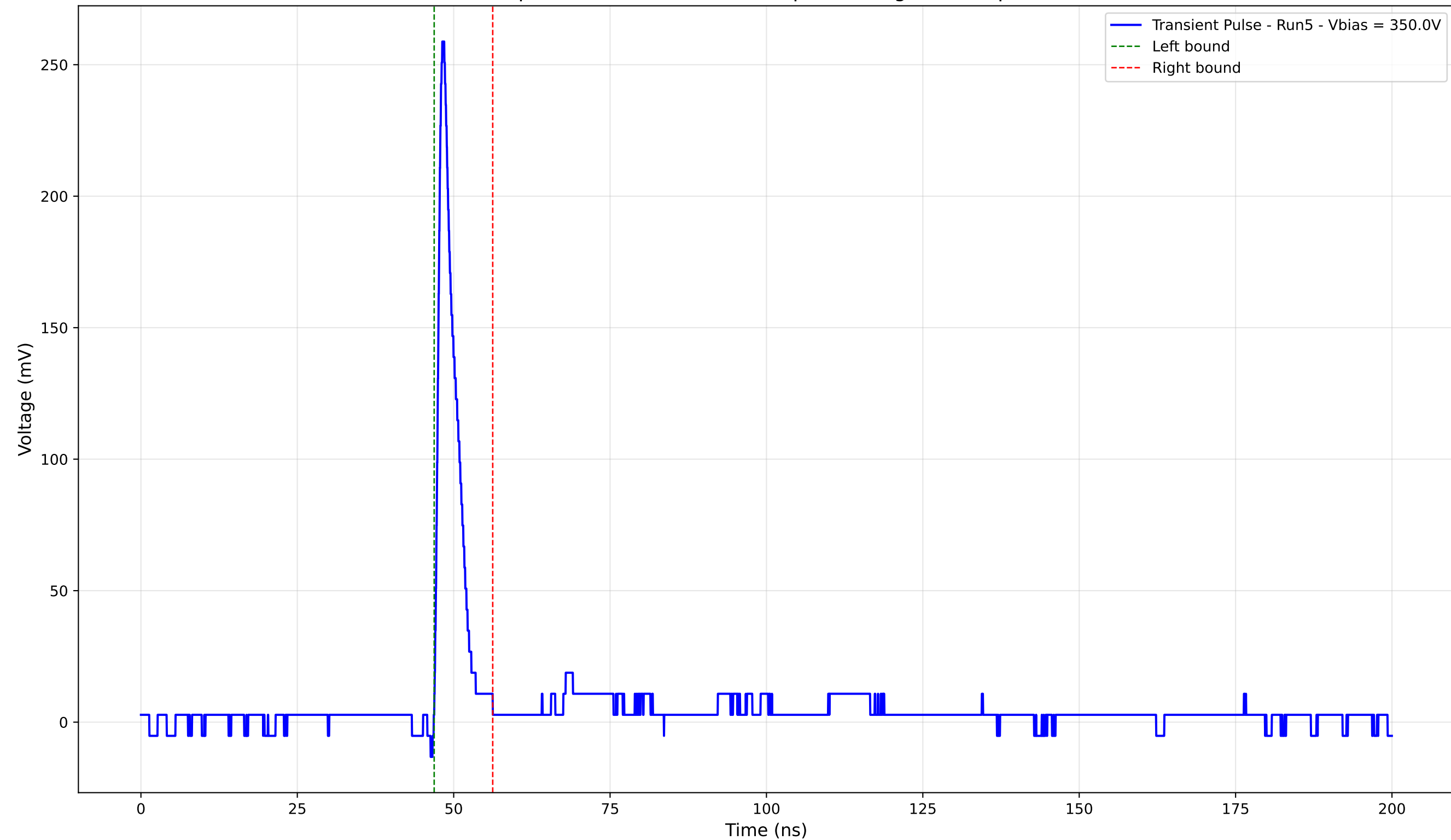
Transient Pulse - Sample: 4003 - Position: 425.0 \mu\text{m} - Charge: 16.19 pC - Rise Time: 0.92 ns
