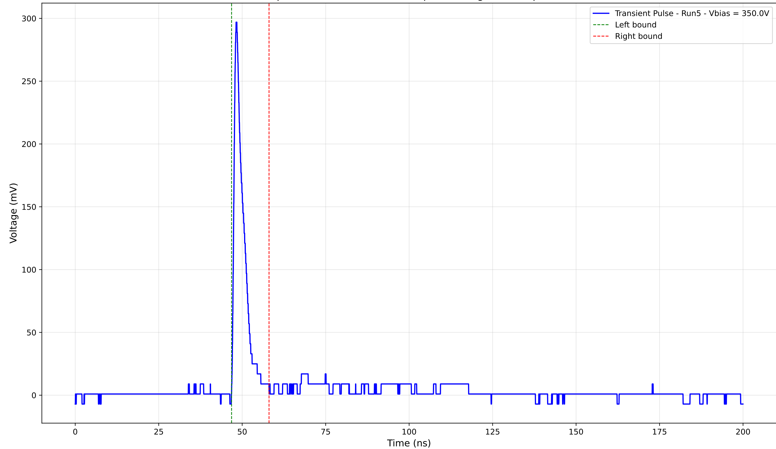
Transient Pulse - Sample: 4003 - Position: 370.0 \mu\text{m} - Charge: 19.27 pC - Rise Time: 0.93 ns
