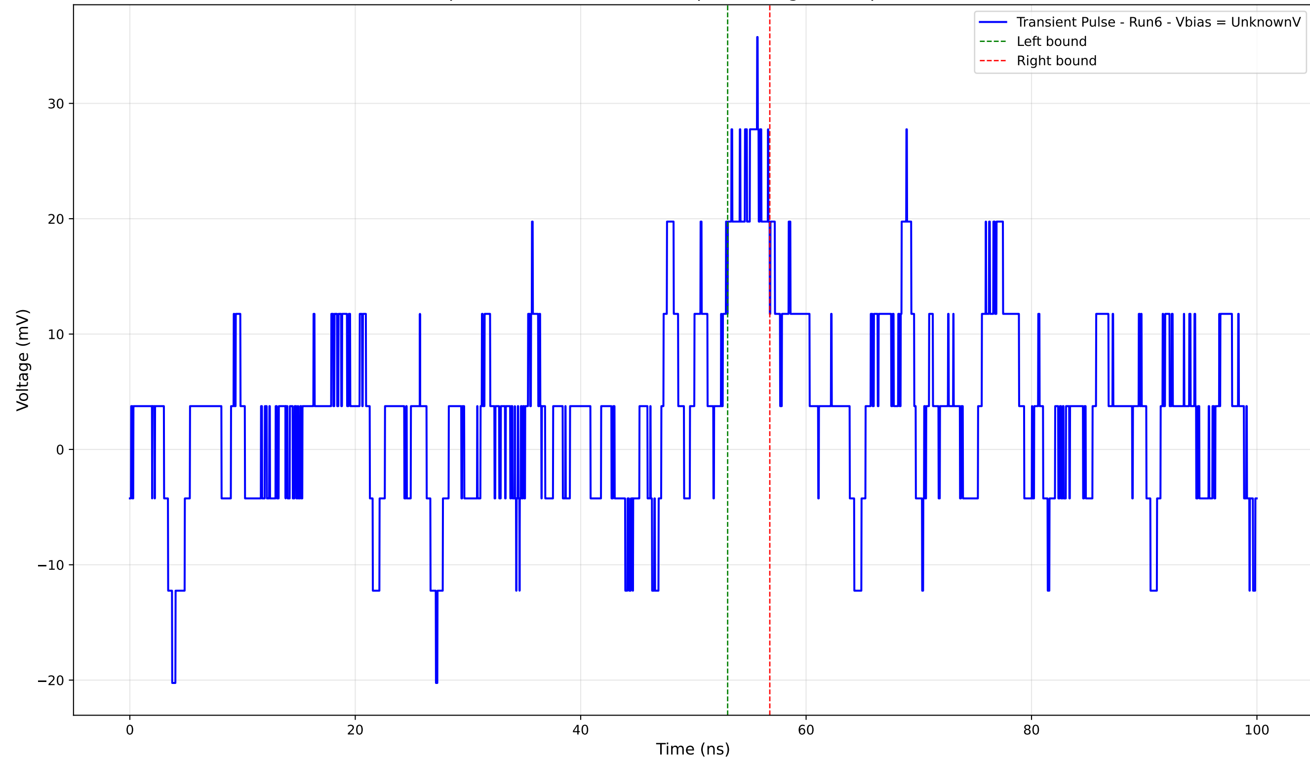
Transient Pulse - Sample: 4004 - Position: 470.0 \mu\text{m} - Charge: 1.69 pC - Rise Time: 0.00 ns (N/A)
