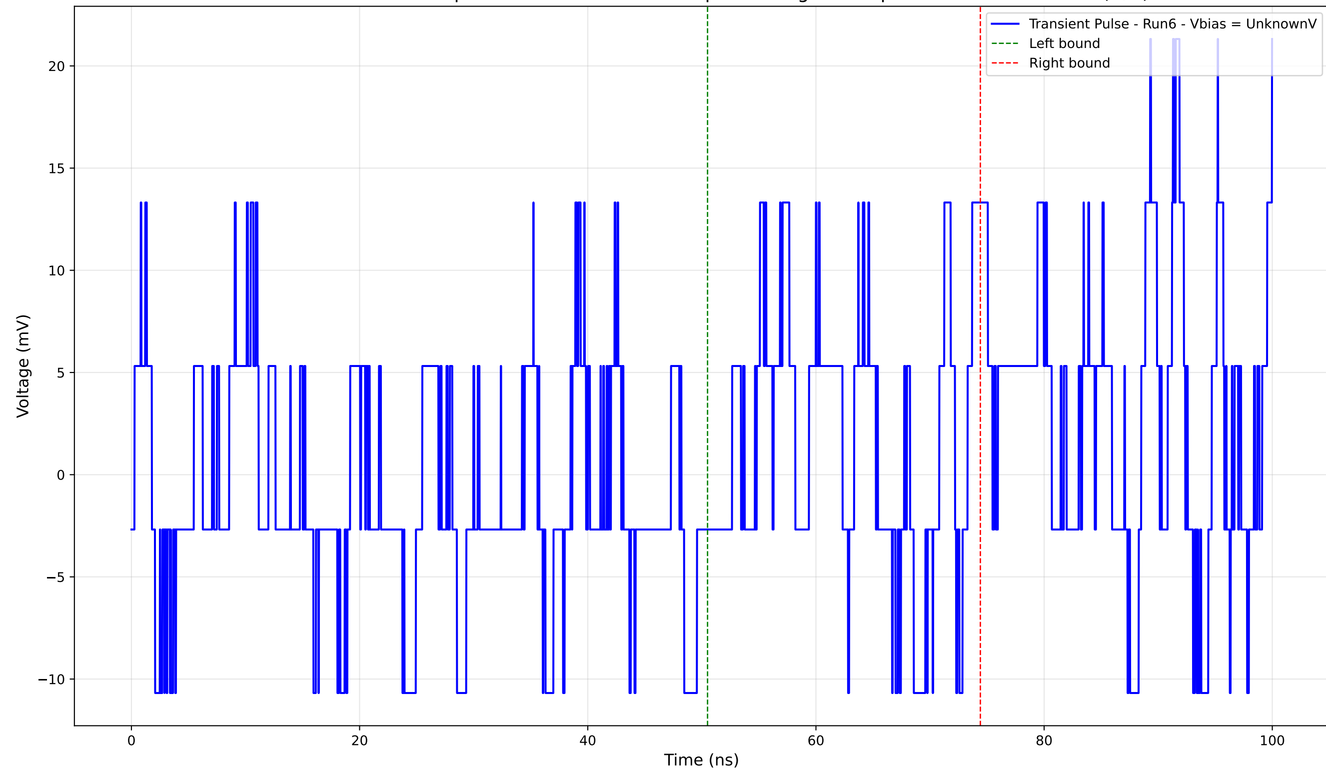
Transient Pulse - Sample: 4004 - Position: 235.0 \mu\text{m} - Charge: 0.78 pC - Rise Time: 0.00 ns (N/A)
