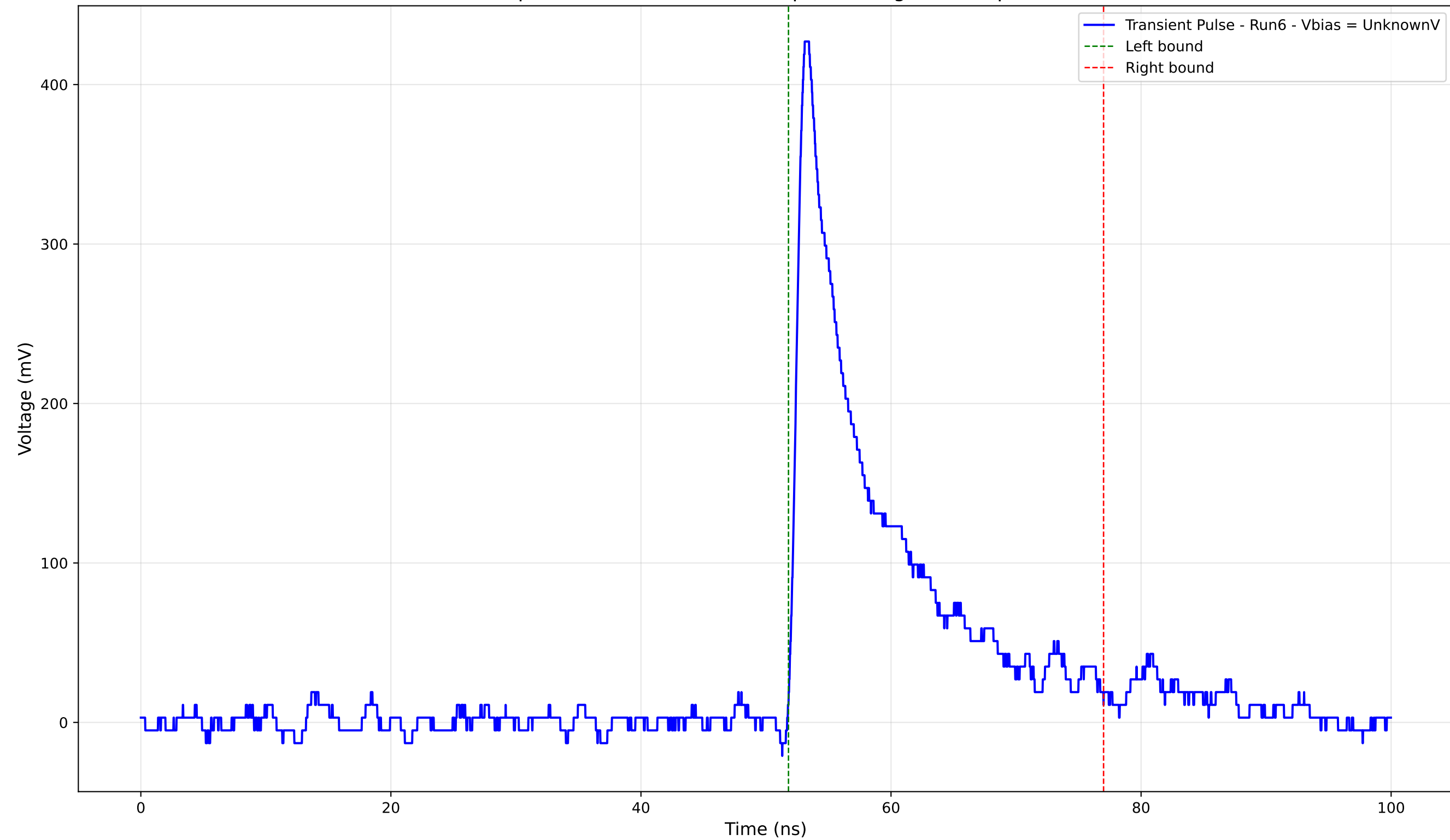
Transient Pulse - Sample: 4004 - Position: 605.0 \mu\text{m} - Charge: 56.21 pC - Rise Time: 0.96 ns
