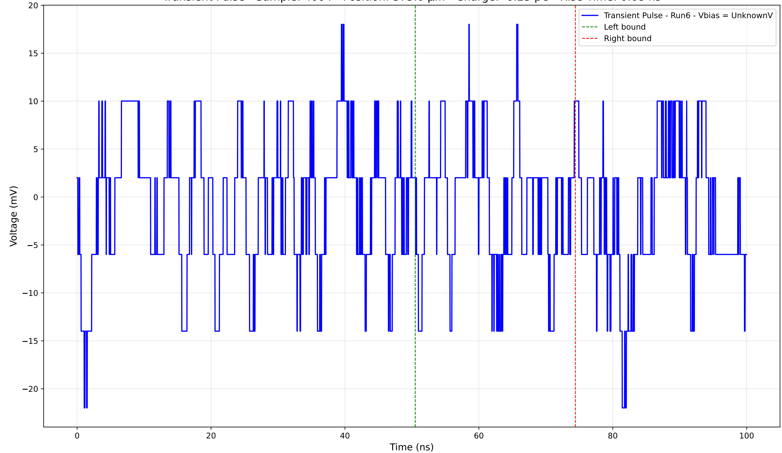
Transient Pulse - Sample: 4004 - Position: 375.0 \mu\text{m} - Charge: -0.23 pC - Rise Time: 0.68 ns
