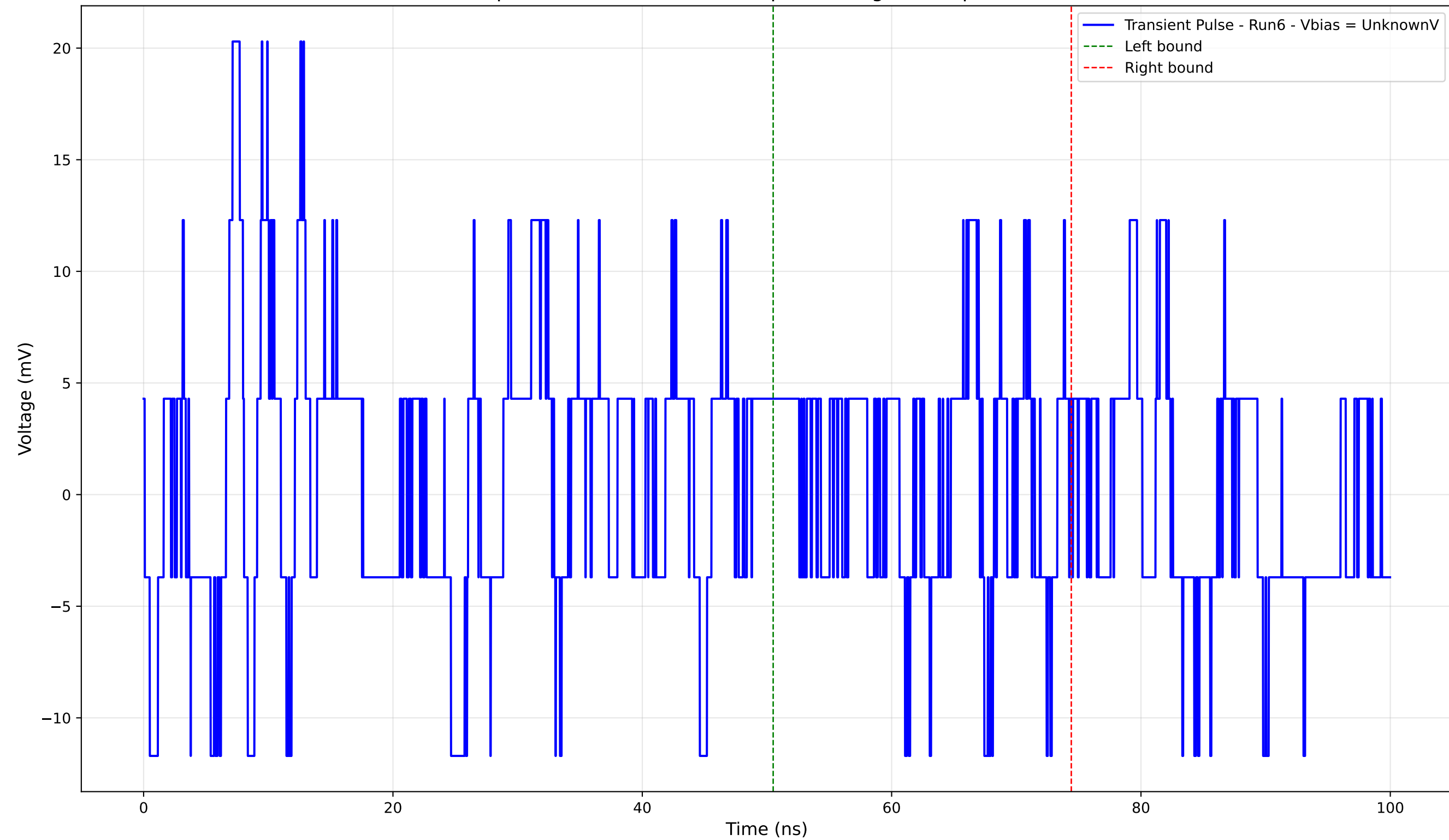
Transient Pulse - Sample: 4004 - Position: 260.0 \mu\text{m} - Charge: 0.50 pC - Rise Time: 0.00 ns (N/A)
