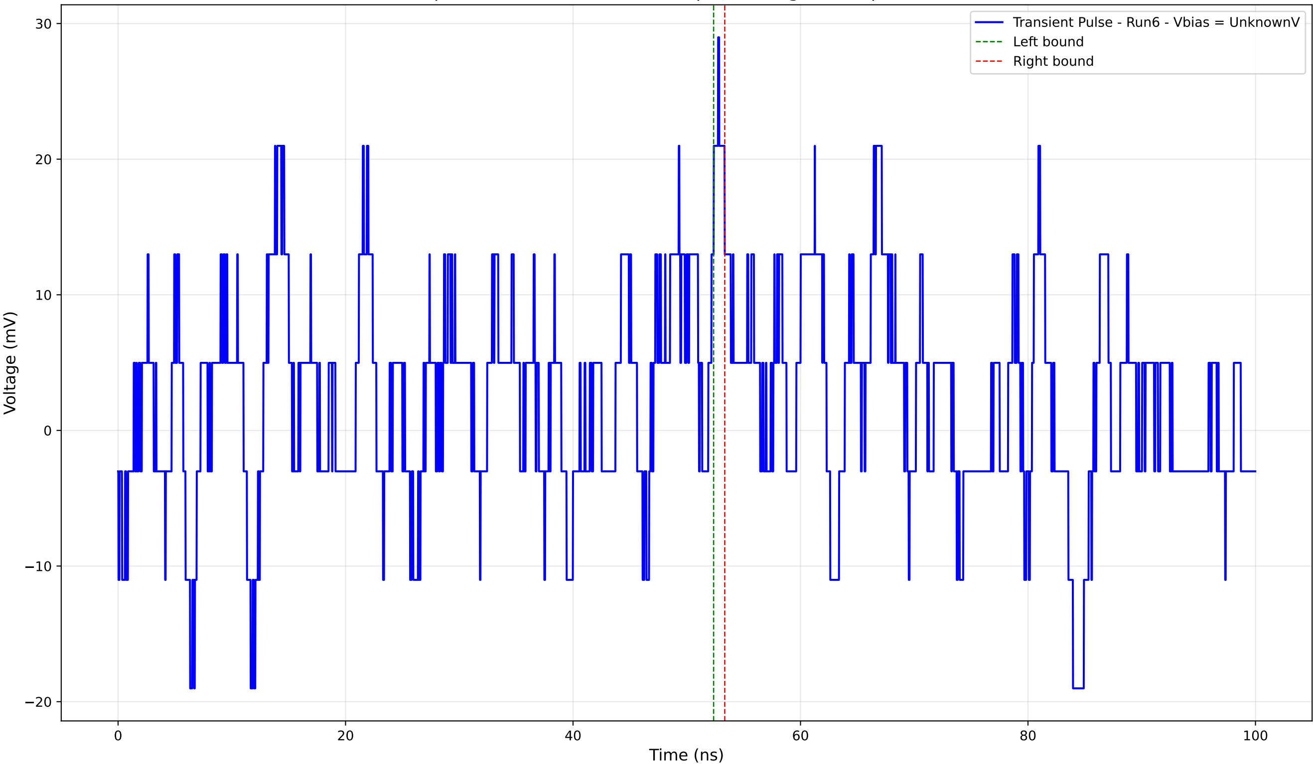
Transient Pulse - Sample: 4004 - Position: 1180.0 \mu\text{m} - Charge: 0.42 pC - Rise Time: 0.00 ns (N/A)
