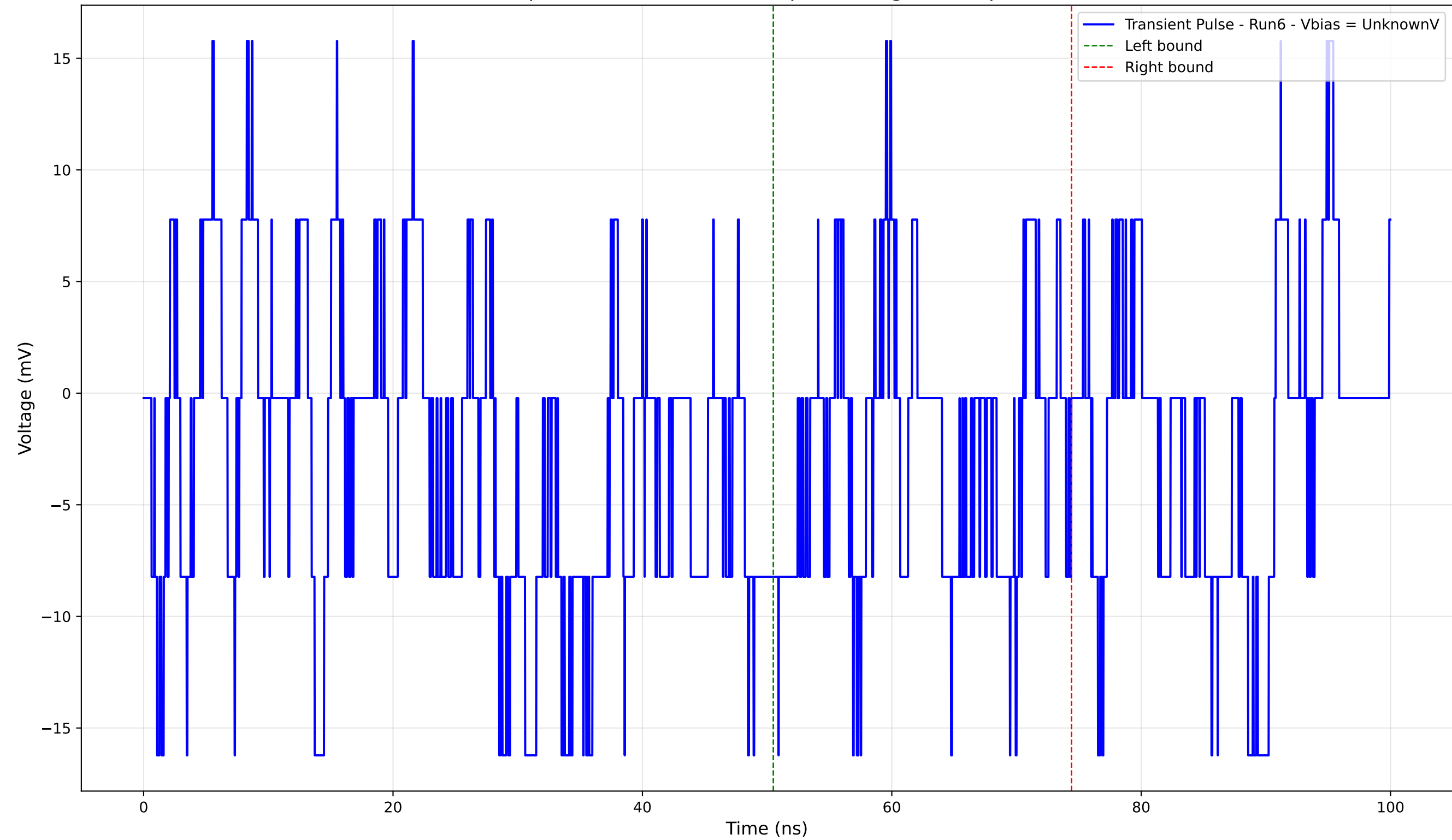
Transient Pulse - Sample: 4004 - Position: 15.0 \mu\text{m} - Charge: -1.17 pC - Rise Time: 0.20 ns
