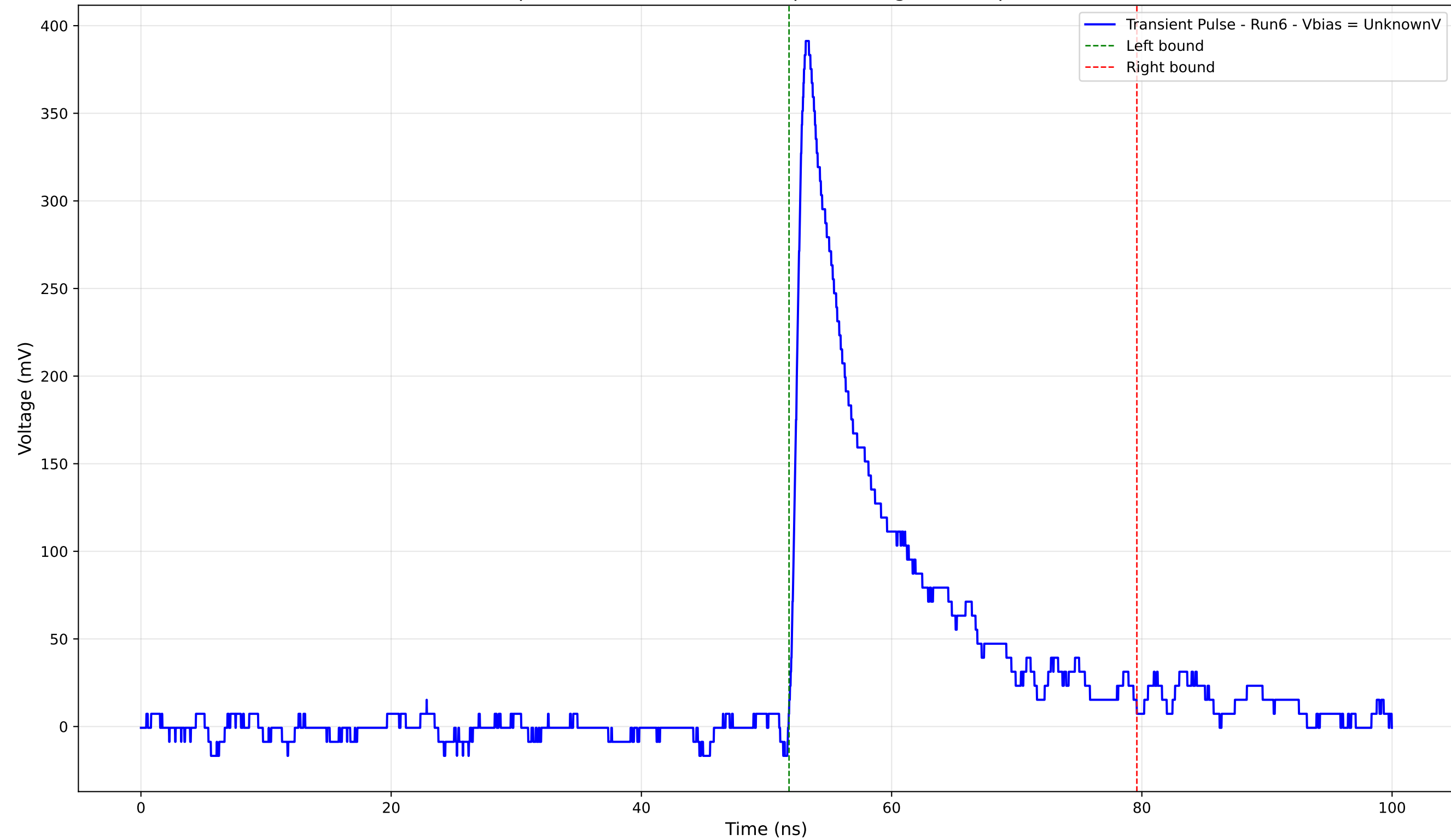
Transient Pulse - Sample: 4004 - Position: 635.0 \mu\text{m} - Charge: 53.73 pC - Rise Time: 0.94 ns
