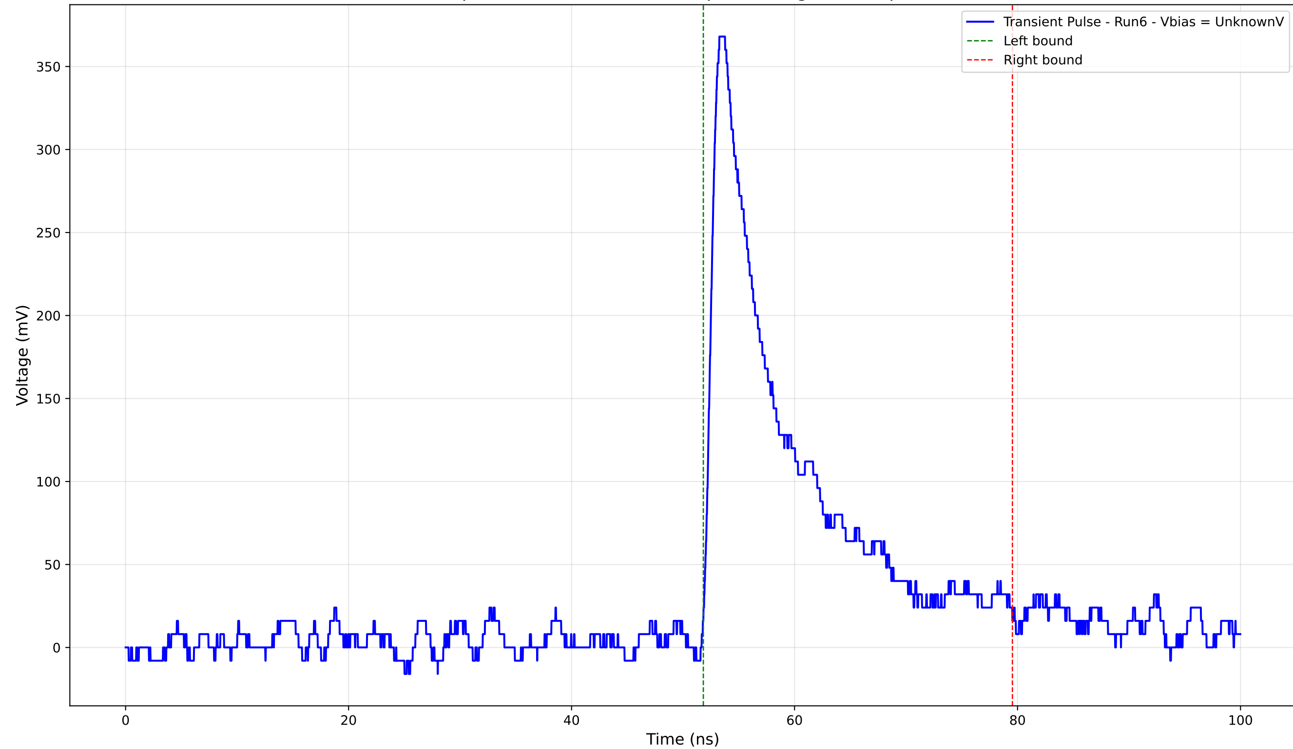
Transient Pulse - Sample: 4004 - Position: 575.0 \mu\text{m} - Charge: 55.58 pC - Rise Time: 1.07 ns
