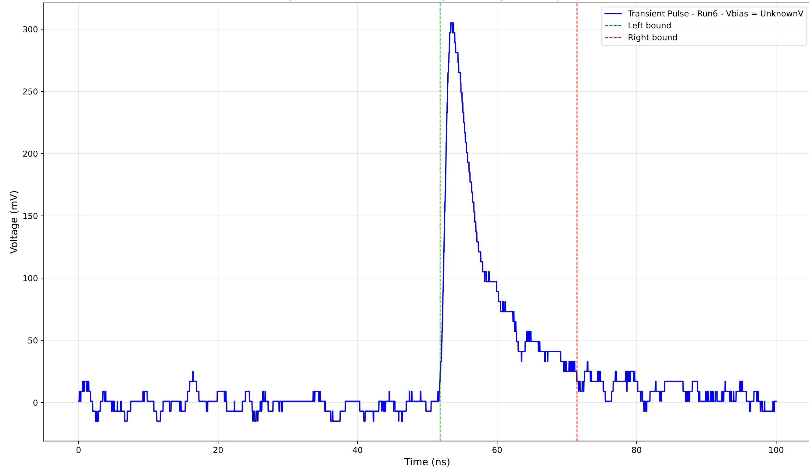
Transient Pulse - Sample: 4004 - Position: 700.0 \mu\text{m} - Charge: 39.33 pC - Rise Time: 1.19 ns
