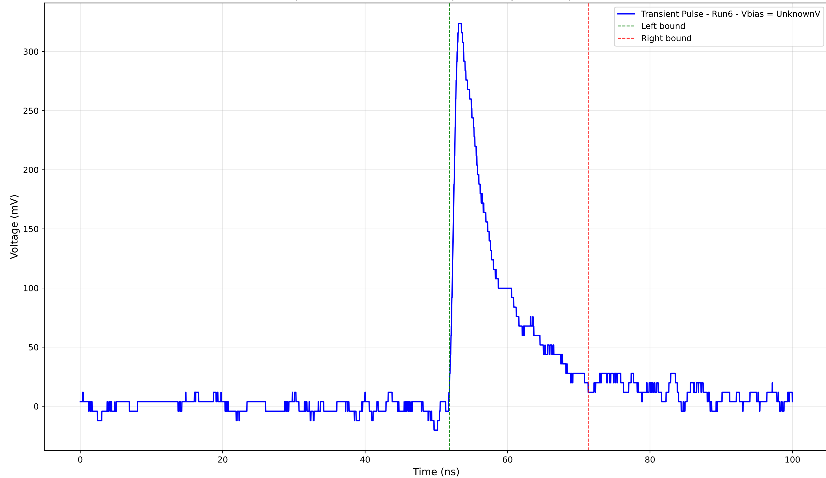
Transient Pulse - Sample: 4004 - Position: 670.0 \mu\text{m} - Charge: 41.85 pC - Rise Time: 0.95 ns
