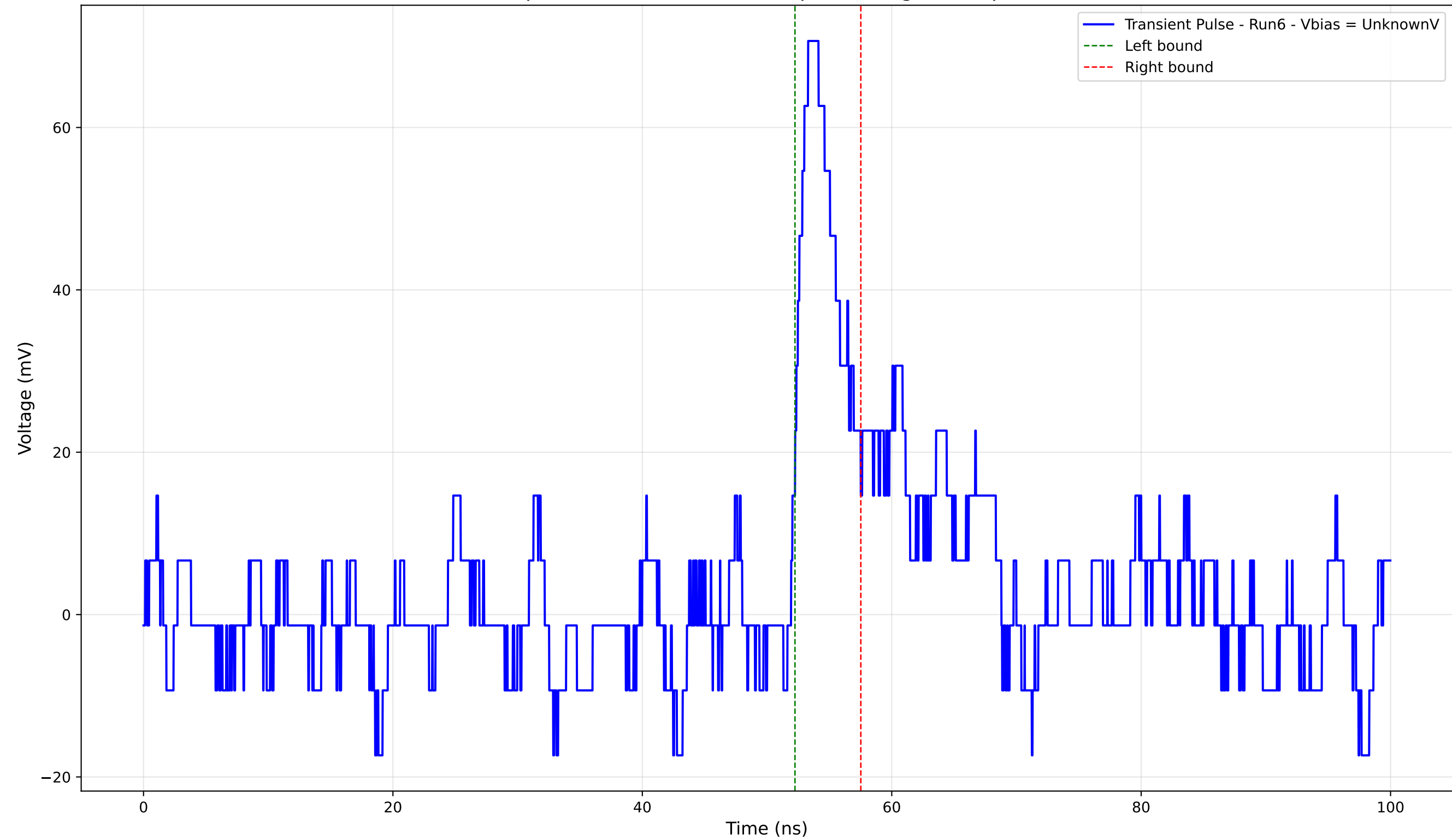
Transient Pulse - Sample: 4004 - Position: 980.0 \mu\text{m} - Charge: 4.87 pC - Rise Time: 1.28 ns
