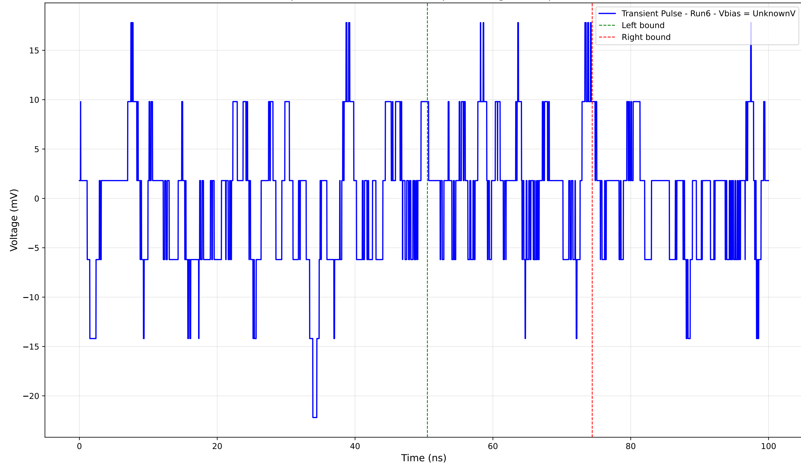
Transient Pulse - Sample: 4004 - Position: 370.0 \mu\text{m} - Charge: 0.96 pC - Rise Time: 0.98 ns
