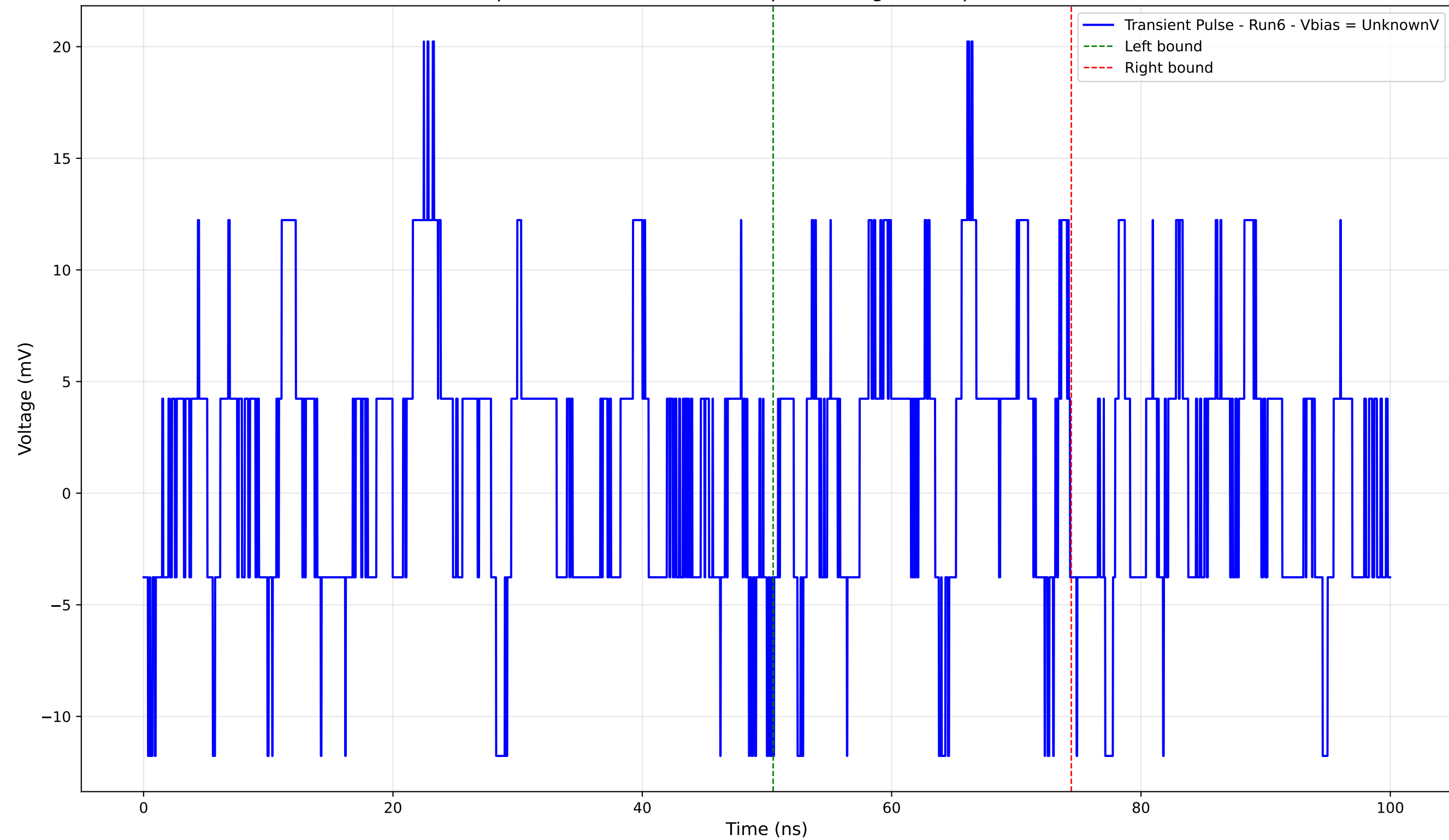
Transient Pulse - Sample: 4004 - Position: 255.0 \mu\text{m} - Charge: 1.29 pC - Rise Time: 0.00 ns (N/A)
