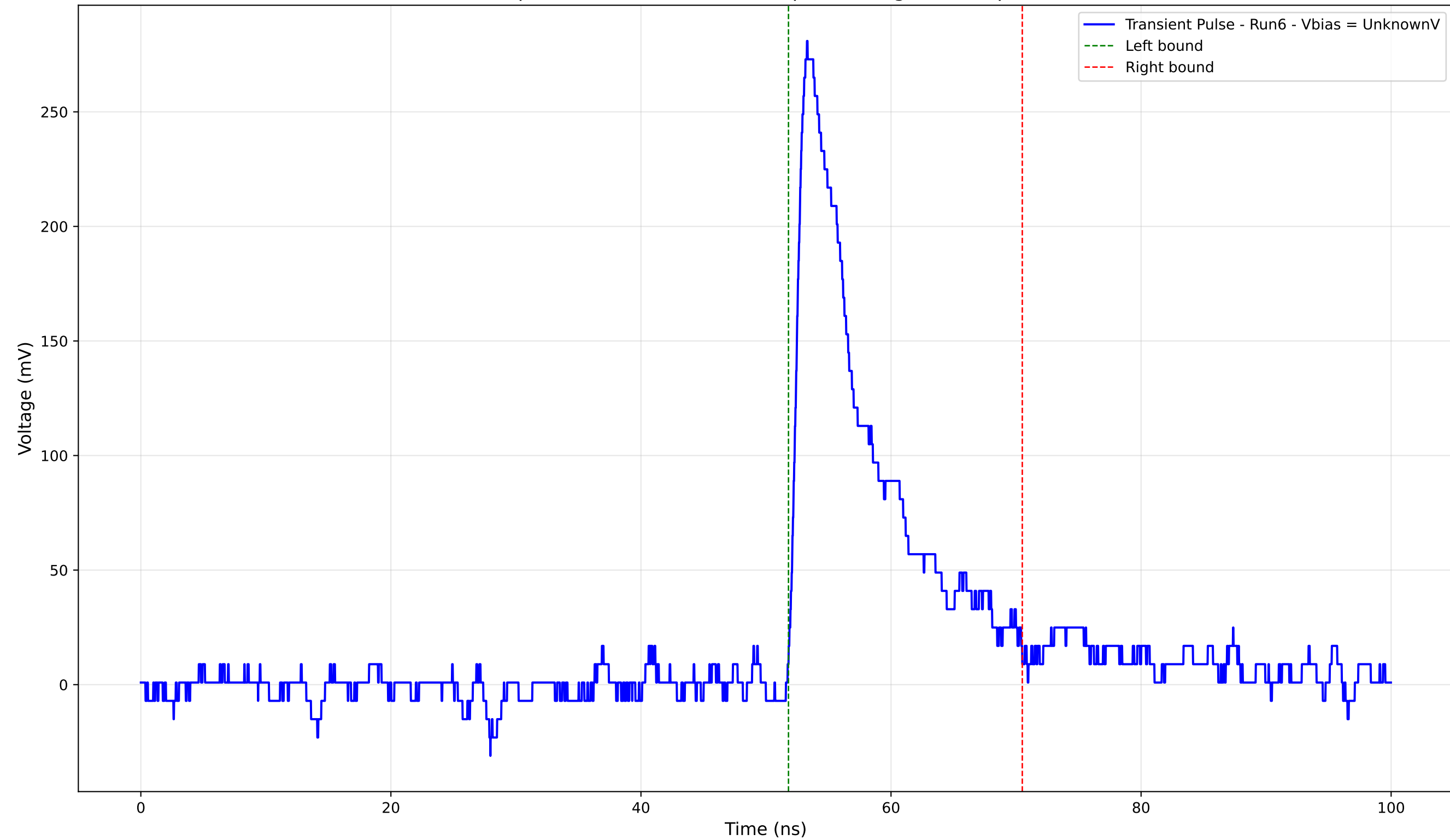
Transient Pulse - Sample: 4004 - Position: 680.0 \mu\text{m} - Charge: 36.10 pC - Rise Time: 1.05 ns
