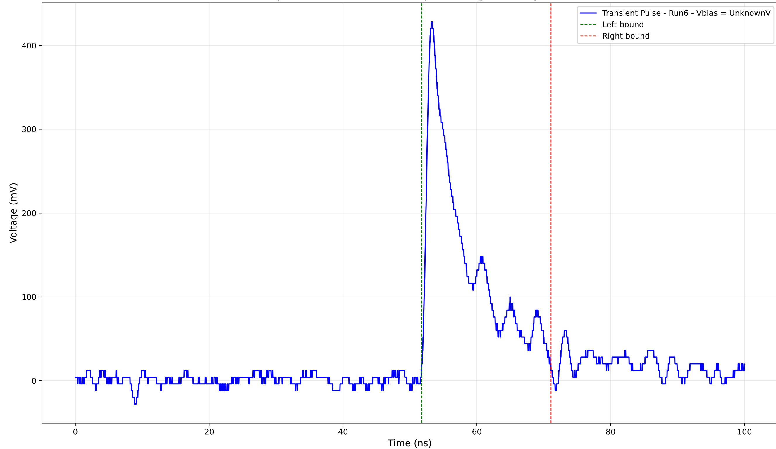
Transient Pulse - Sample: 4004 - Position: 590.0 \mu\text{m} - Charge: 54.36 pC - Rise Time: 0.96 ns
