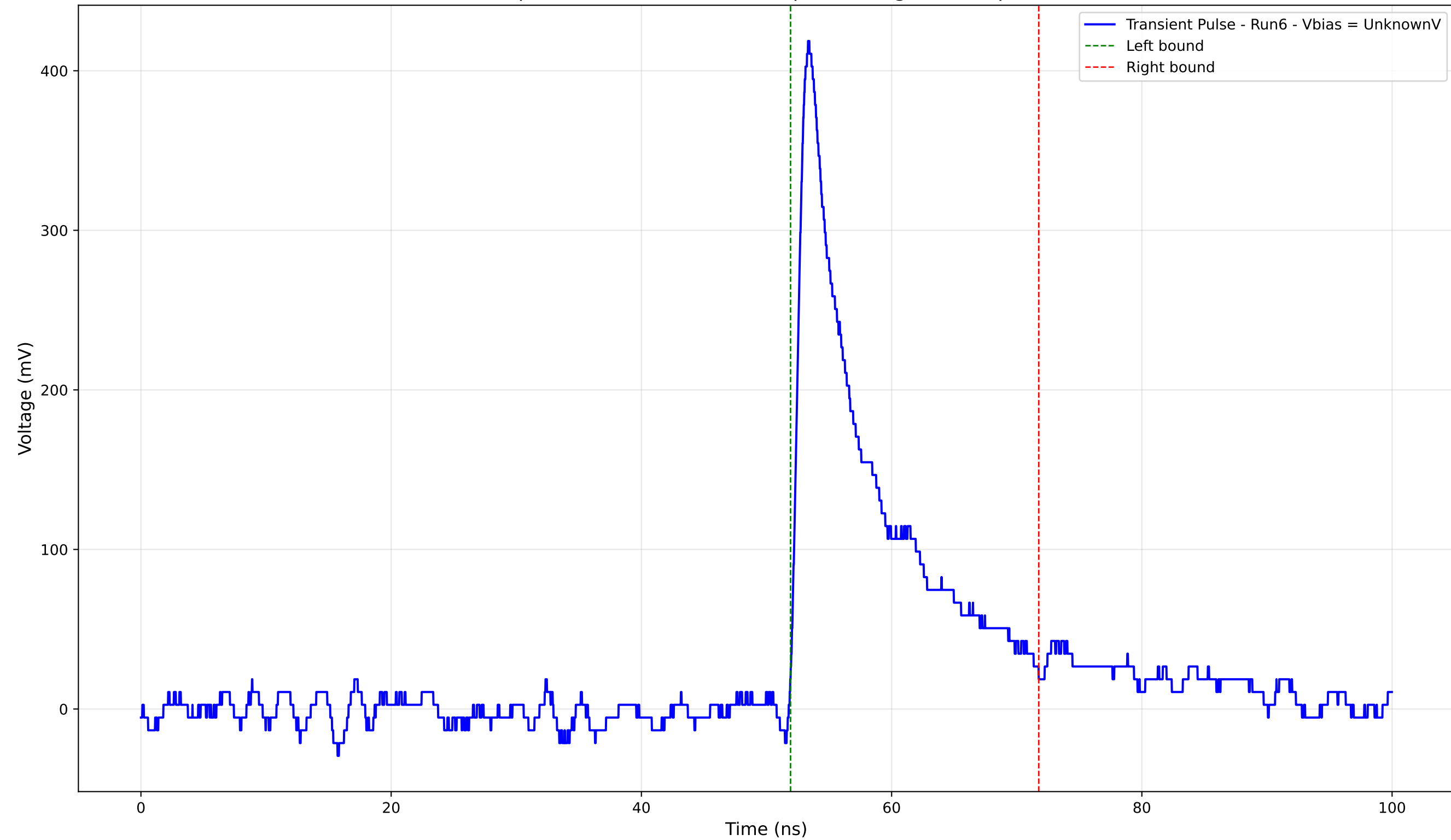
Transient Pulse - Sample: 4004 - Position: 585.0 \mu\text{m} - Charge: 52.10 pC - Rise Time: 0.96 ns
