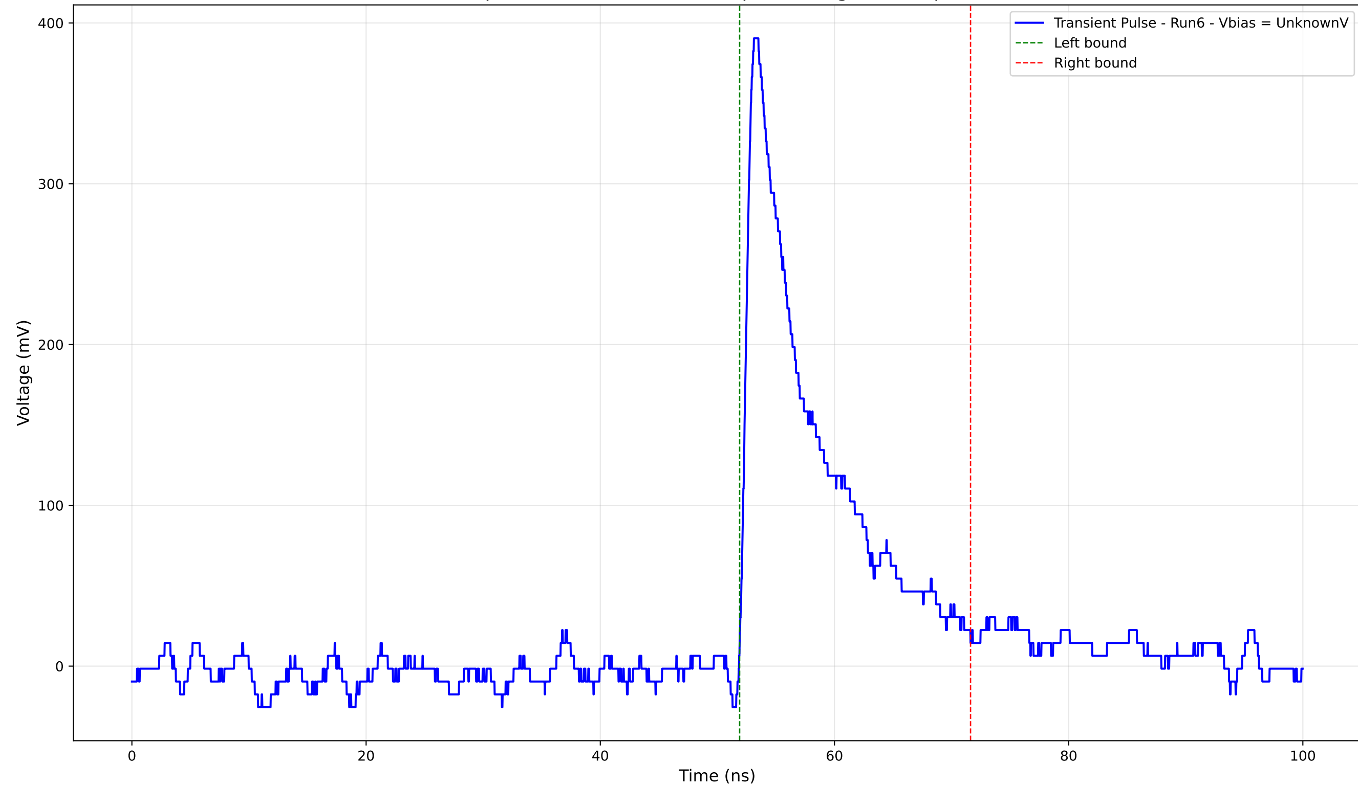
Transient Pulse - Sample: 4004 - Position: 650.0 \mu\text{m} - Charge: 49.74 pC - Rise Time: 0.88 ns
