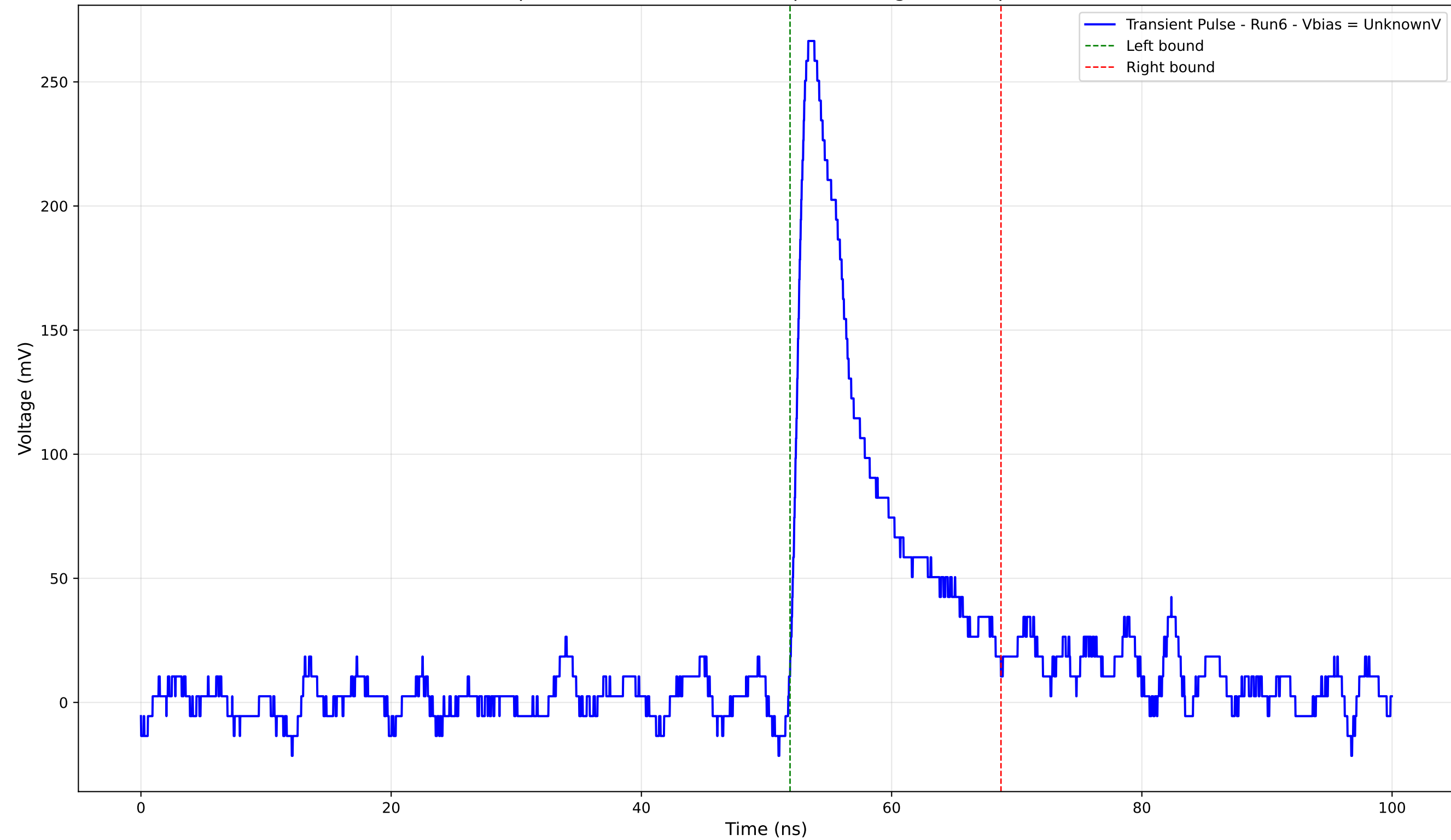
Transient Pulse - Sample: 4004 - Position: 740.0 \mu\text{m} - Charge: 32.95 pC - Rise Time: 1.02 ns
