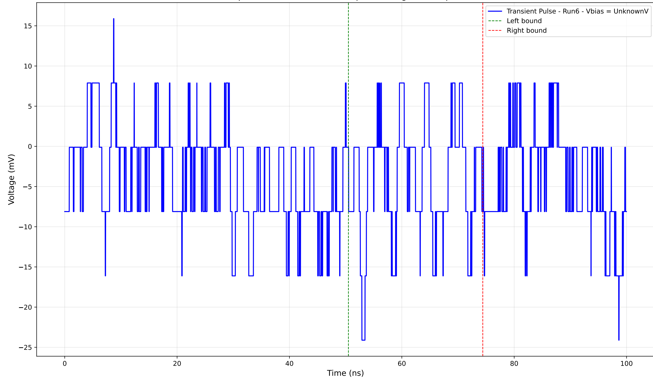
Transient Pulse - Sample: 4004 - Position: 55.0 \mu\text{m} - Charge: -1.88 pC - Rise Time: 0.49 ns
