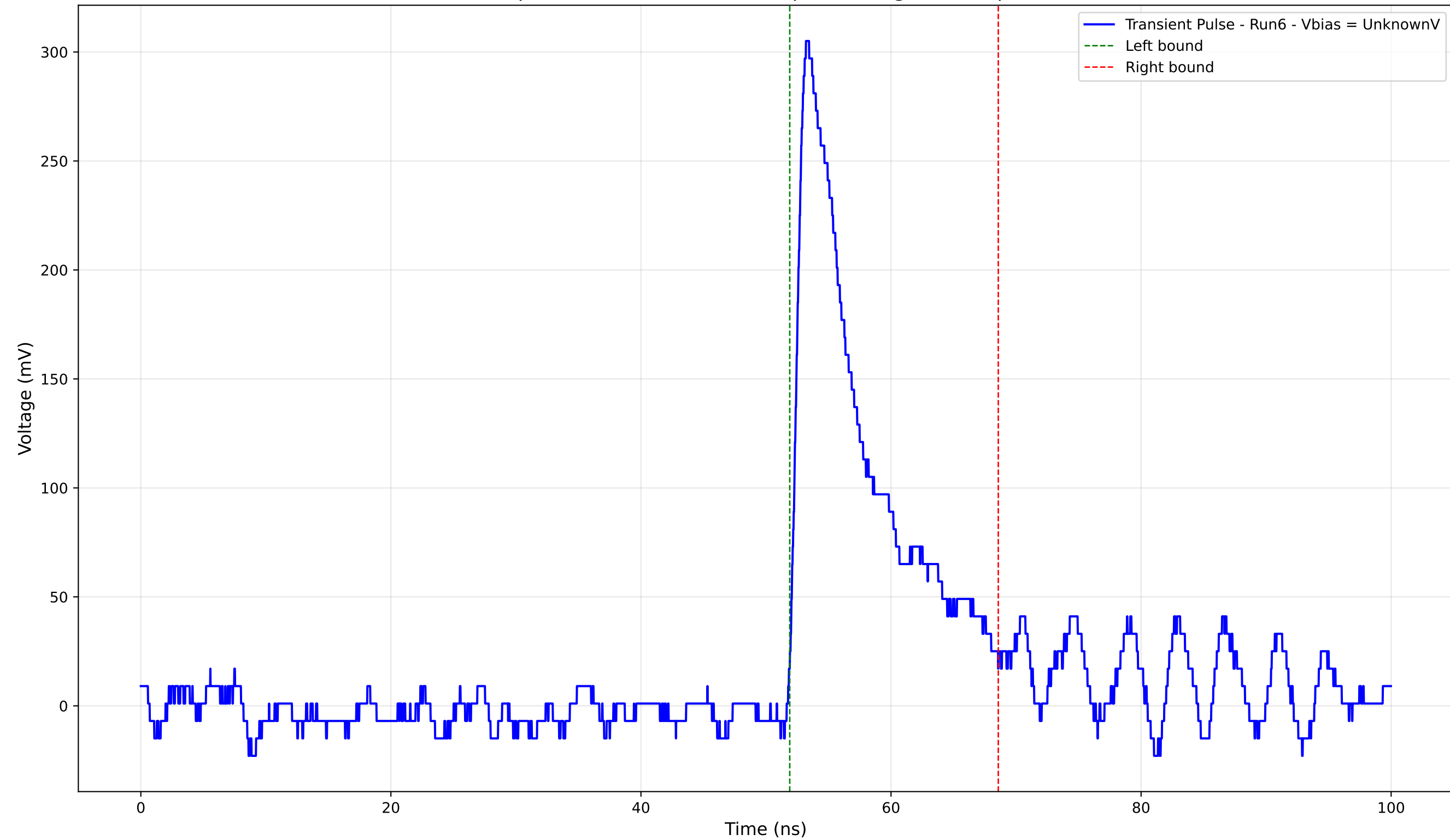
Transient Pulse - Sample: 4004 - Position: 695.0 \mu\text{m} - Charge: 37.76 pC - Rise Time: 0.99 ns
