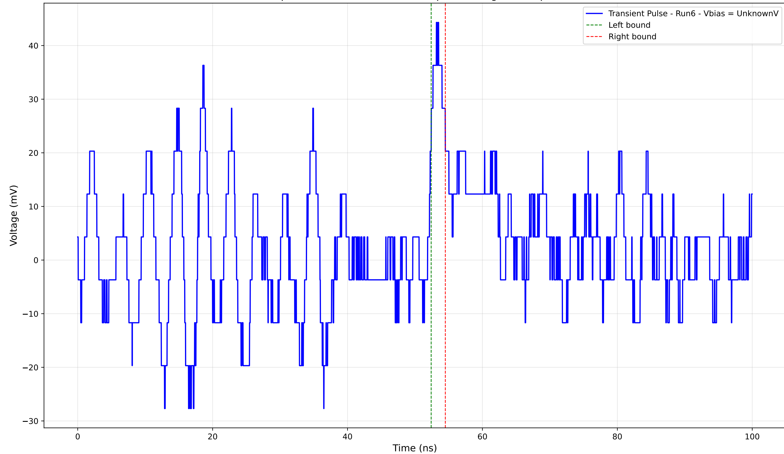
Transient Pulse - Sample: 4004 - Position: 1085.0 \mu\text{m} - Charge: 1.43 pC - Rise Time: 1.04 ns
