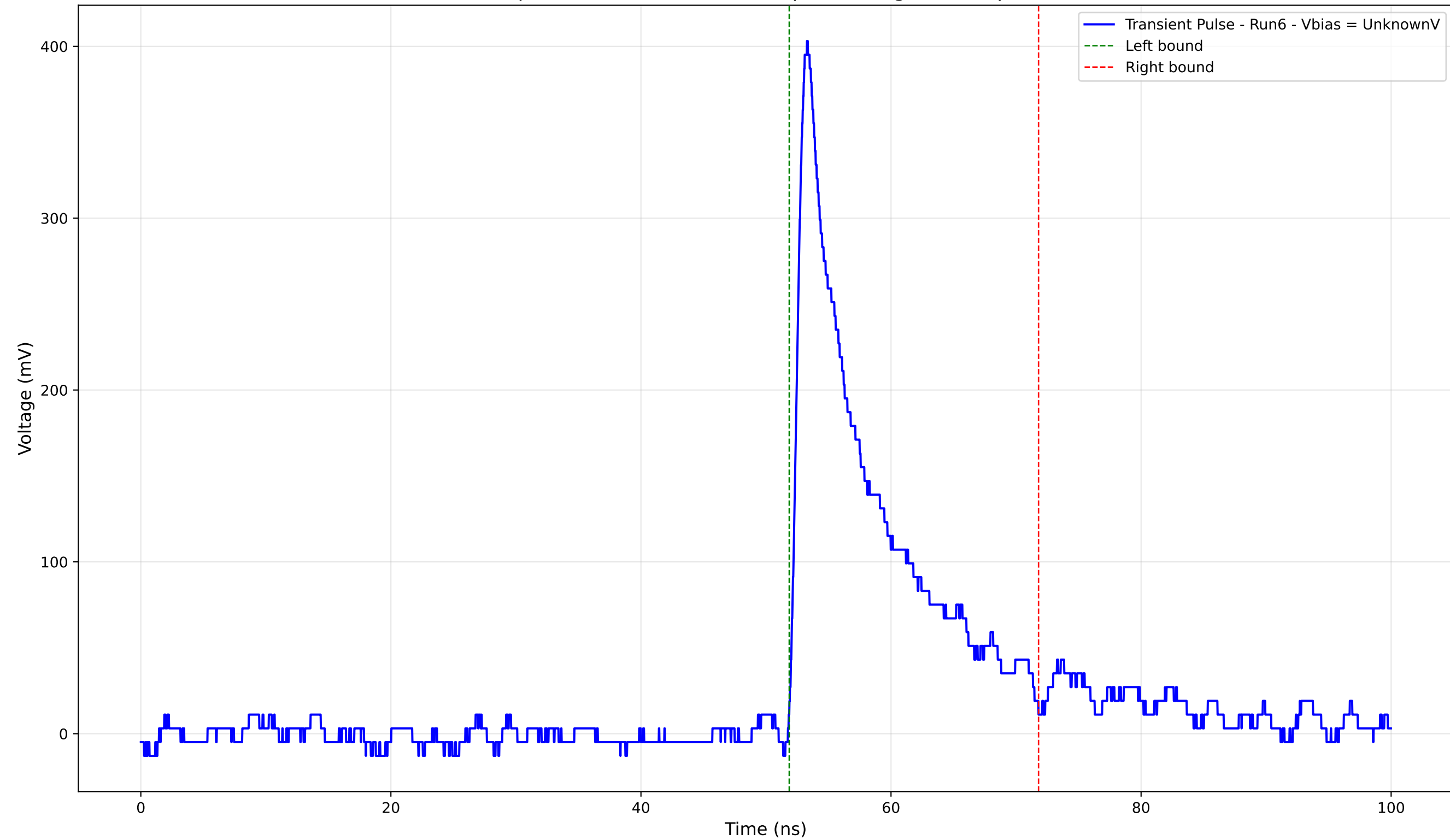
Transient Pulse - Sample: 4004 - Position: 615.0 \mu\text{m} - Charge: 50.22 pC - Rise Time: 0.95 ns
