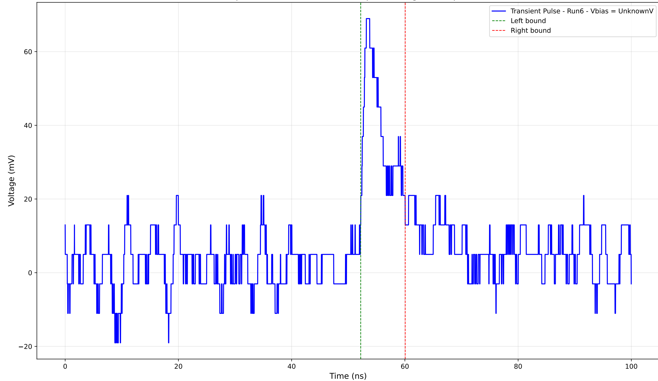
Transient Pulse - Sample: 4004 - Position: 1020.0 \mu\text{m} - Charge: 6.12 pC - Rise Time: 1.08 ns
