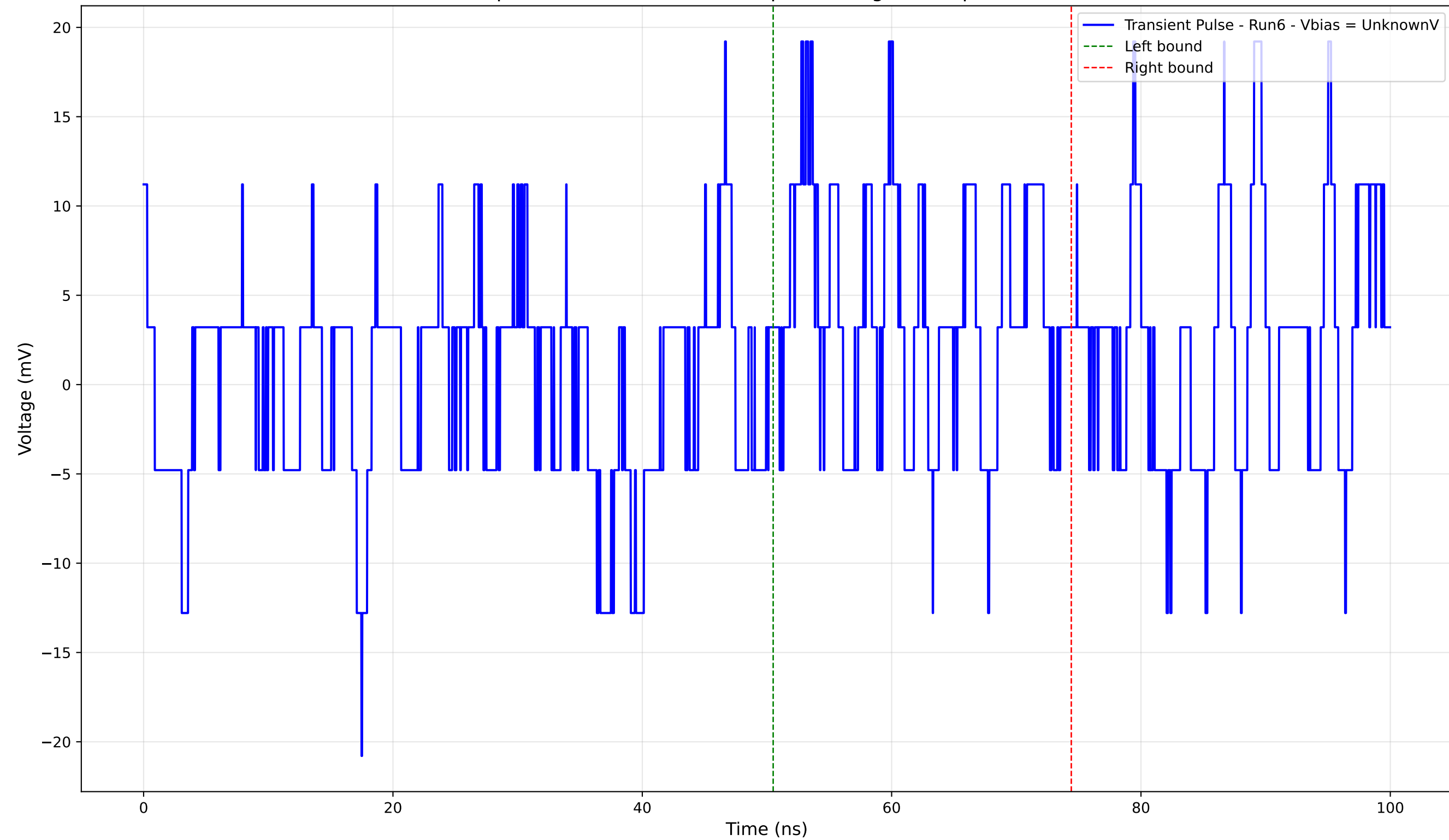
Transient Pulse - Sample: 4004 - Position: 440.0 \mu\text{m} - Charge: 2.02 pC - Rise Time: 0.00 ns (N/A)
