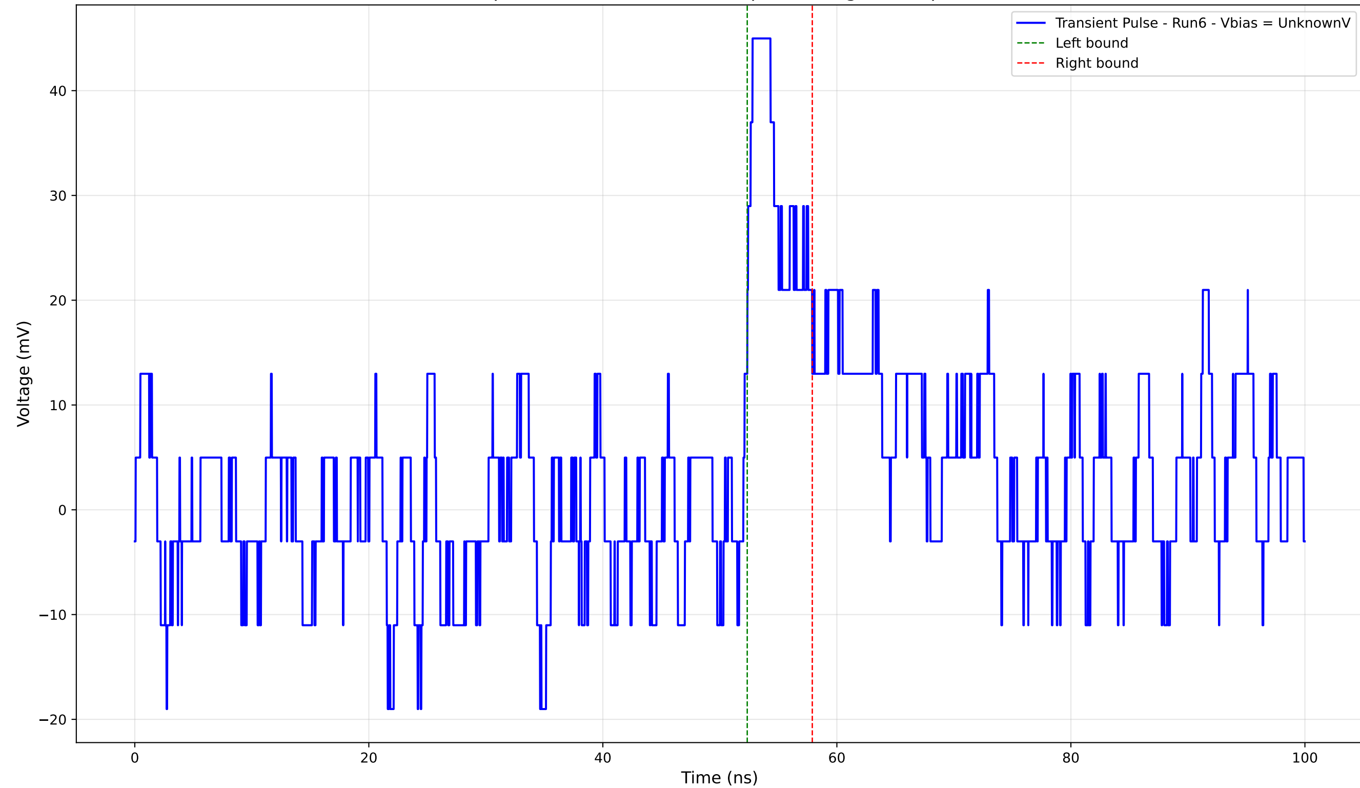
Transient Pulse - Sample: 4004 - Position: 910.0 \mu\text{m} - Charge: 3.44 pC - Rise Time: 0.78 ns
