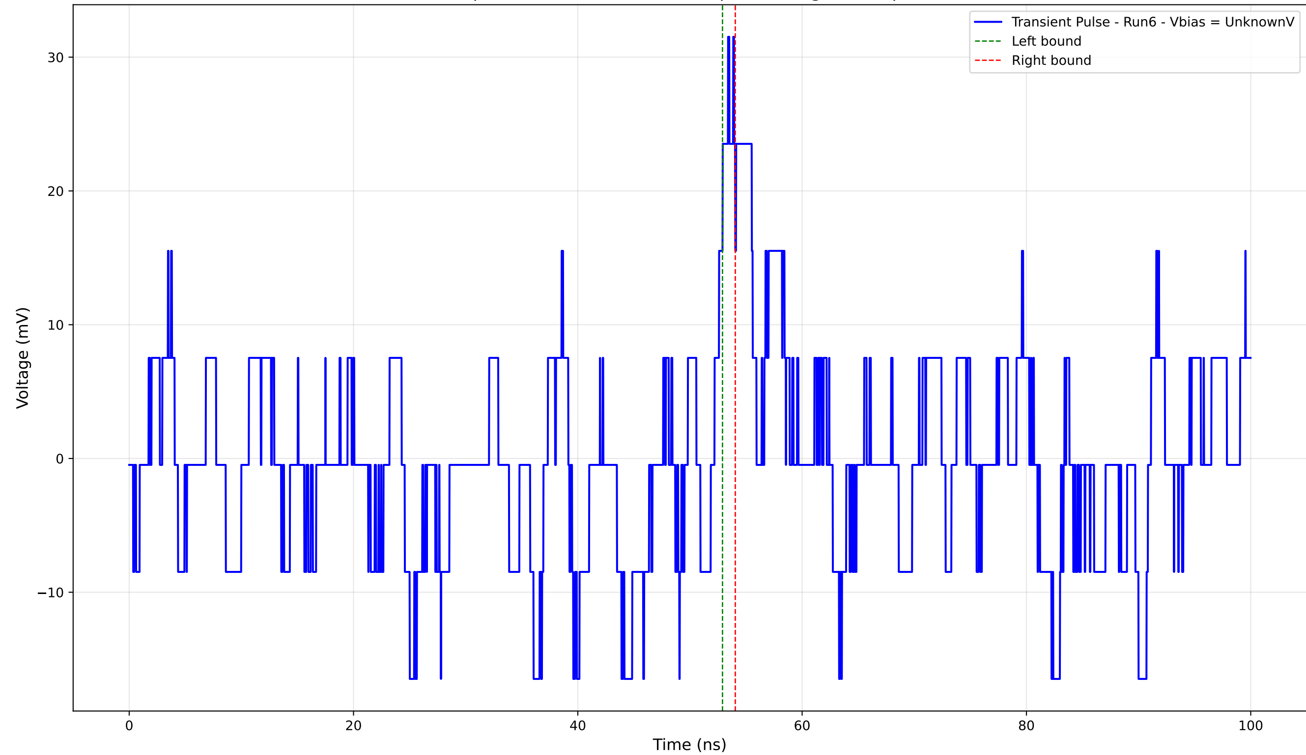
Transient Pulse - Sample: 4004 - Position: 480.0 \mu\text{m} - Charge: 0.57 pC - Rise Time: 1.21 ns
