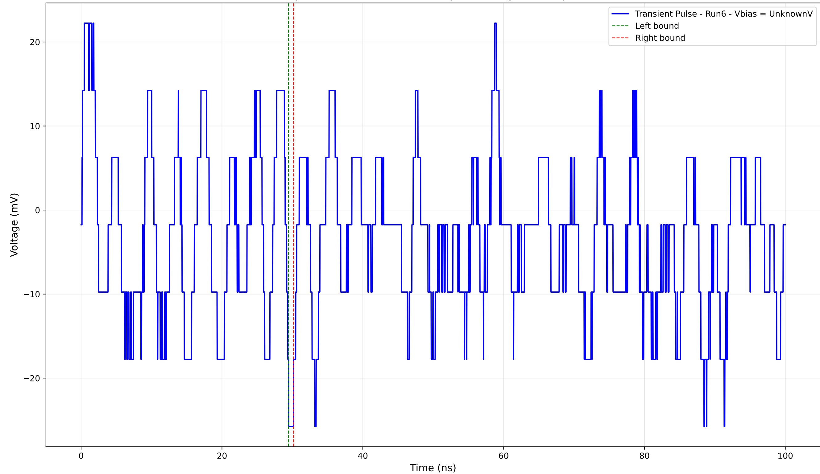
Transient Pulse - Sample: 4004 - Position: 295.0 \mu\text{m} - Charge: -0.37 pC - Rise Time: 0.30 ns
