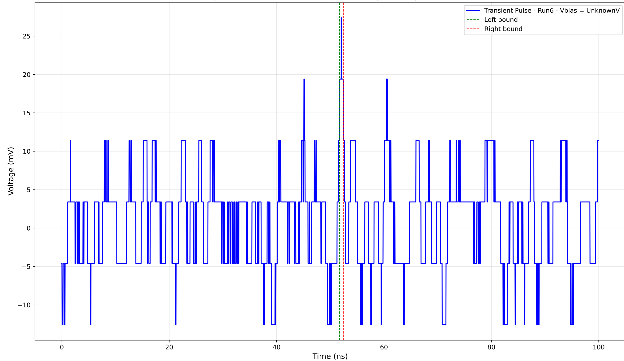
Transient Pulse - Sample: 4004 - Position: 360.0 \mu\text{m} - Charge: 0.27 pC - Rise Time: 0.00 ns (N/A)
