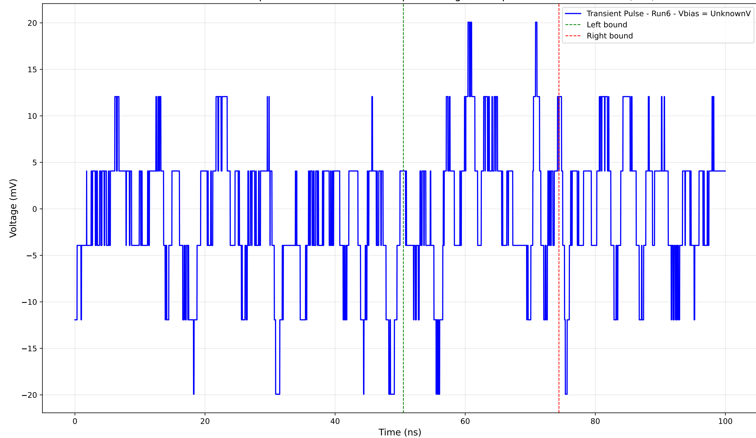
Transient Pulse - Sample: 4004 - Position: 265.0 \mu\text{m} - Charge: 0.33 pC - Rise Time: 0.00 ns (N/A)
