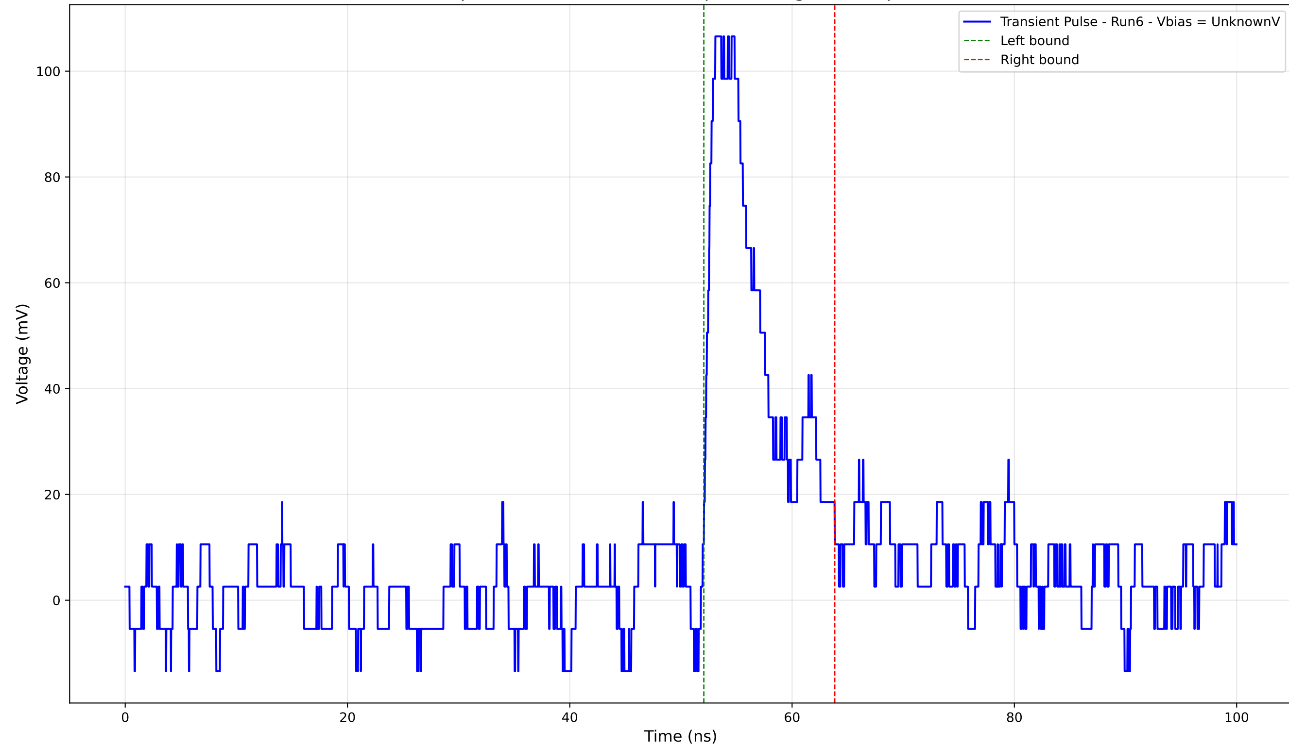
Transient Pulse - Sample: 4004 - Position: 815.0 \mu\text{m} - Charge: 12.23 pC - Rise Time: 0.82 ns
