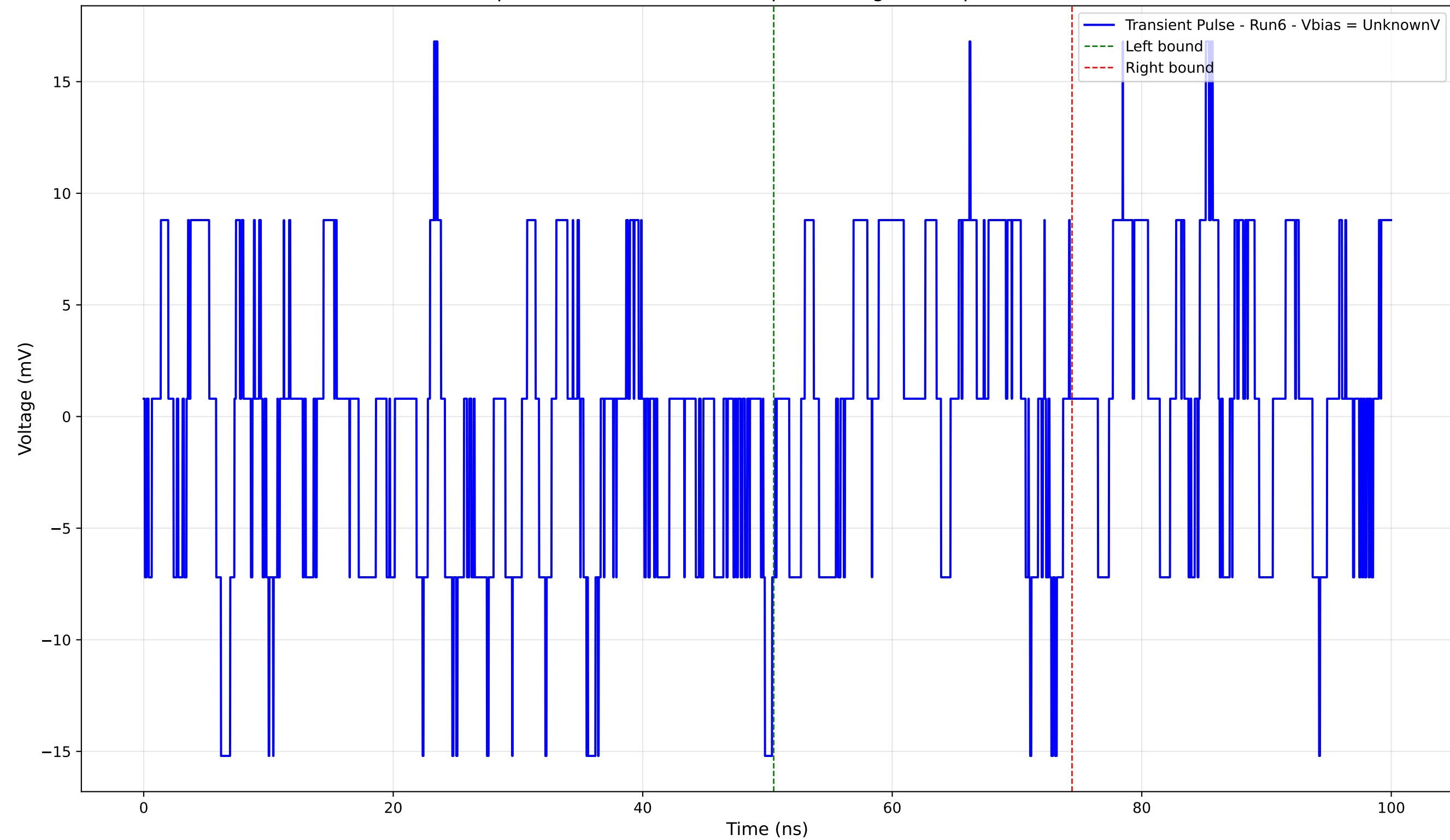
Transient Pulse - Sample: 4004 - Position: 405.0 \mu\text{m} - Charge: 0.79 pC - Rise Time: 0.00 ns (N/A)
