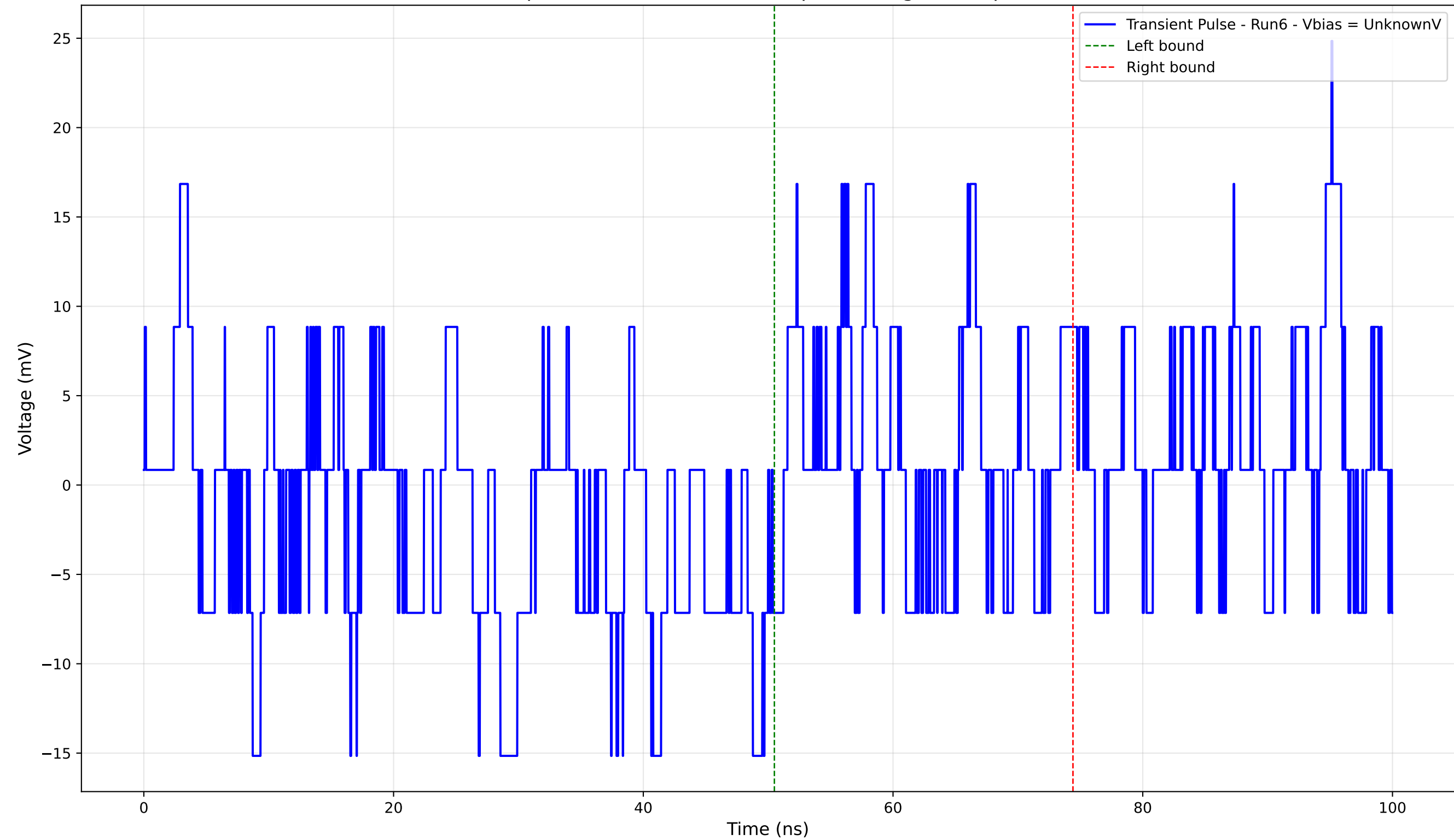
Transient Pulse - Sample: 4004 - Position: 240.0 \mu\text{m} - Charge: 1.04 pC - Rise Time: 0.88 ns
