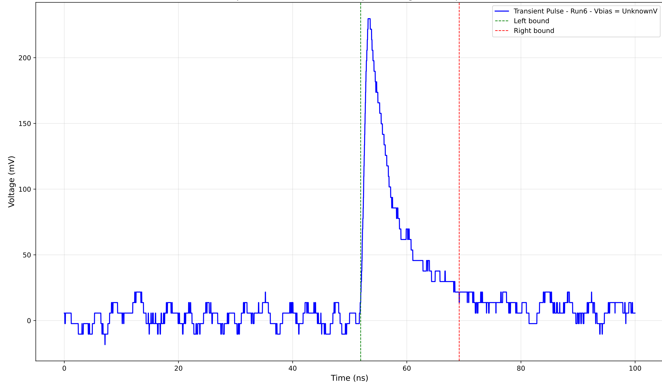
Transient Pulse - Sample: 4004 - Position: 755.0 \mu\text{m} - Charge: 27.58 pC - Rise Time: 1.10 ns
