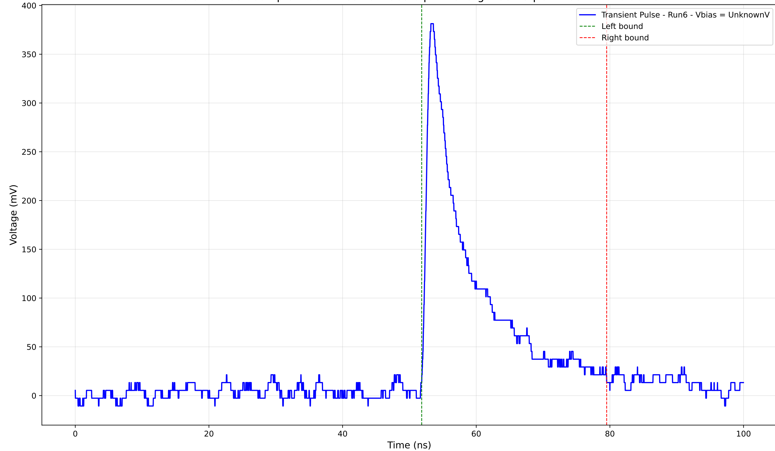
Transient Pulse - Sample: 4004 - Position: 565.0 \mu\text{m} - Charge: 55.75 pC - Rise Time: 0.98 ns
