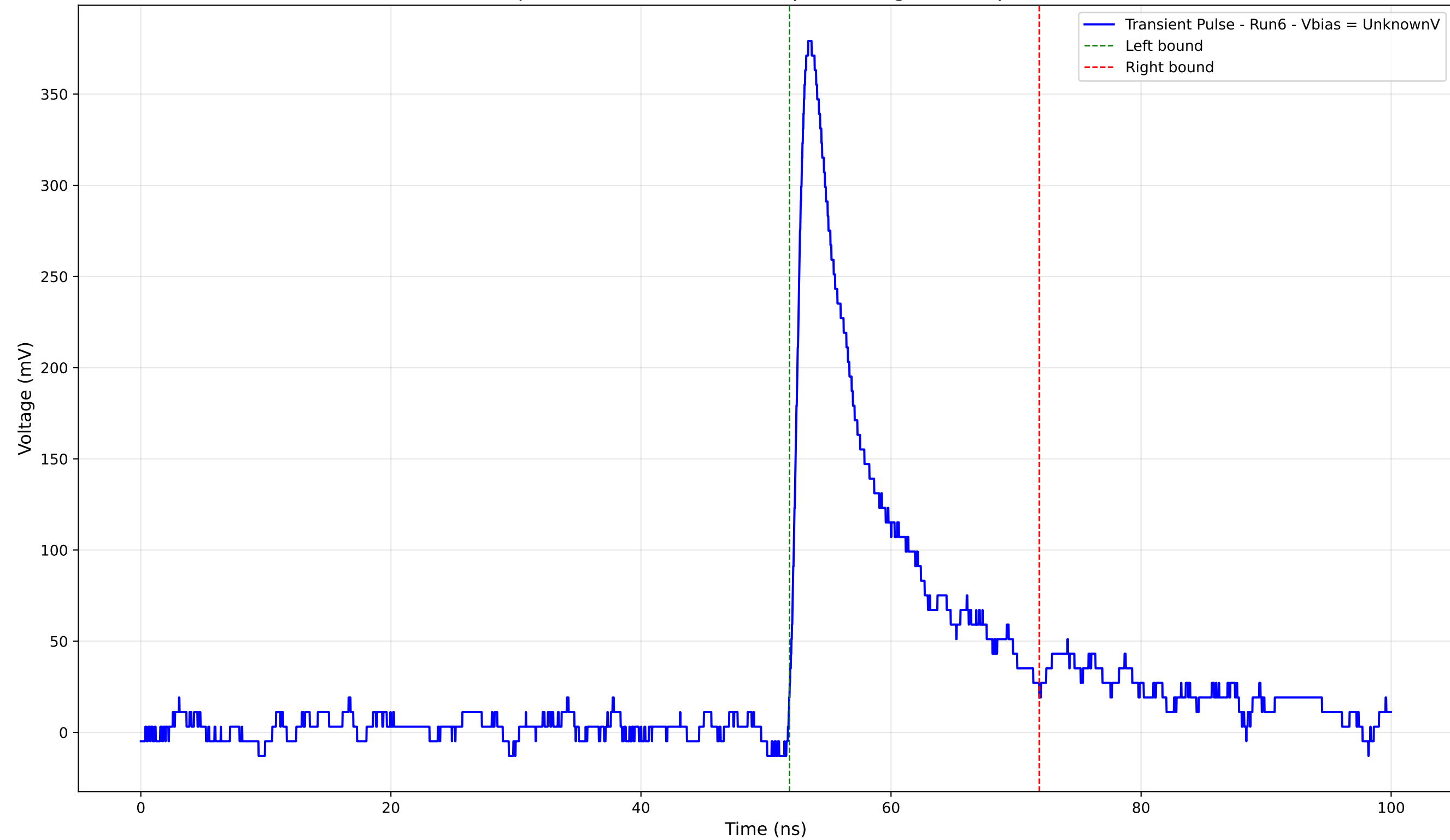
Transient Pulse - Sample: 4004 - Position: 540.0 \mu\text{m} - Charge: 50.90 pC - Rise Time: 1.05 ns
