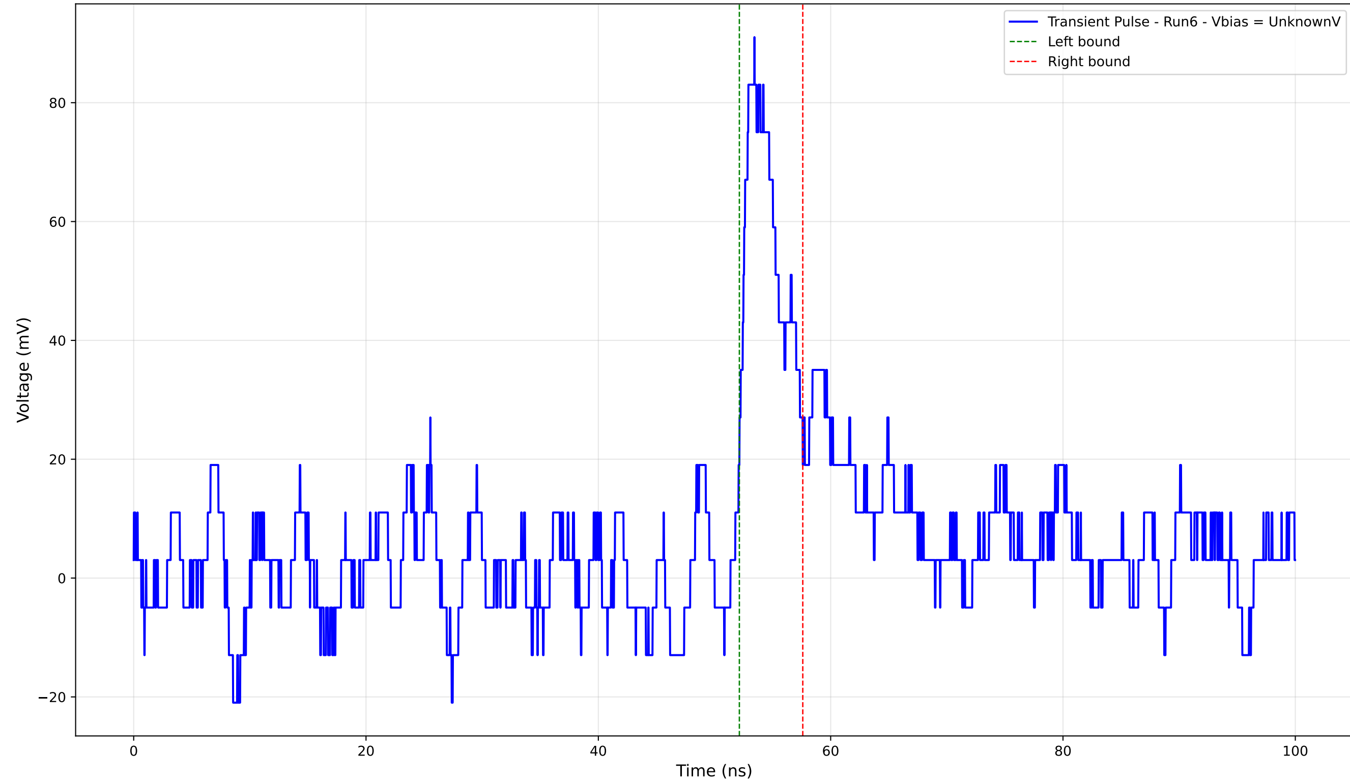
Transient Pulse - Sample: 4004 - Position: 975.0 \mu\text{m} - Charge: 6.25 pC - Rise Time: 1.12 ns
