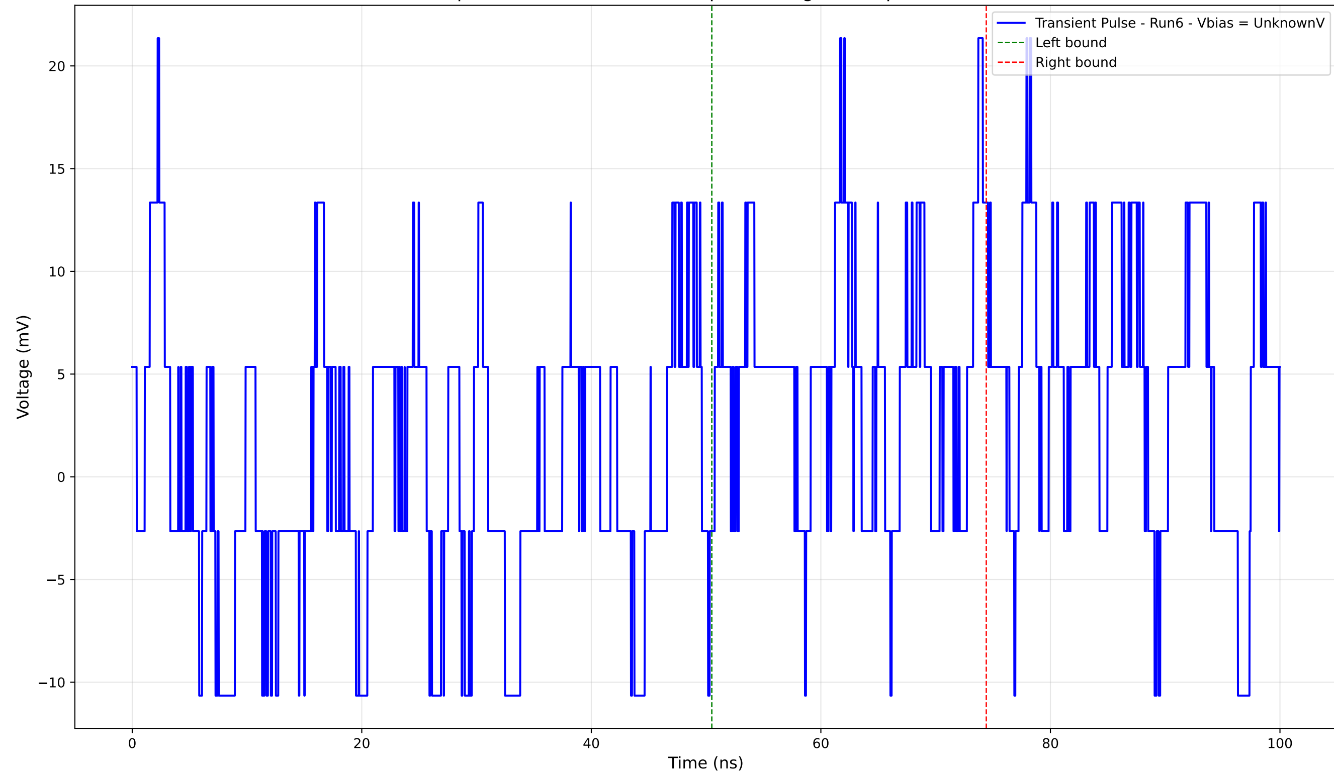
Transient Pulse - Sample: 4004 - Position: 130.0 \mu\text{m} - Charge: 2.30 pC - Rise Time: 0.00 ns (N/A)
