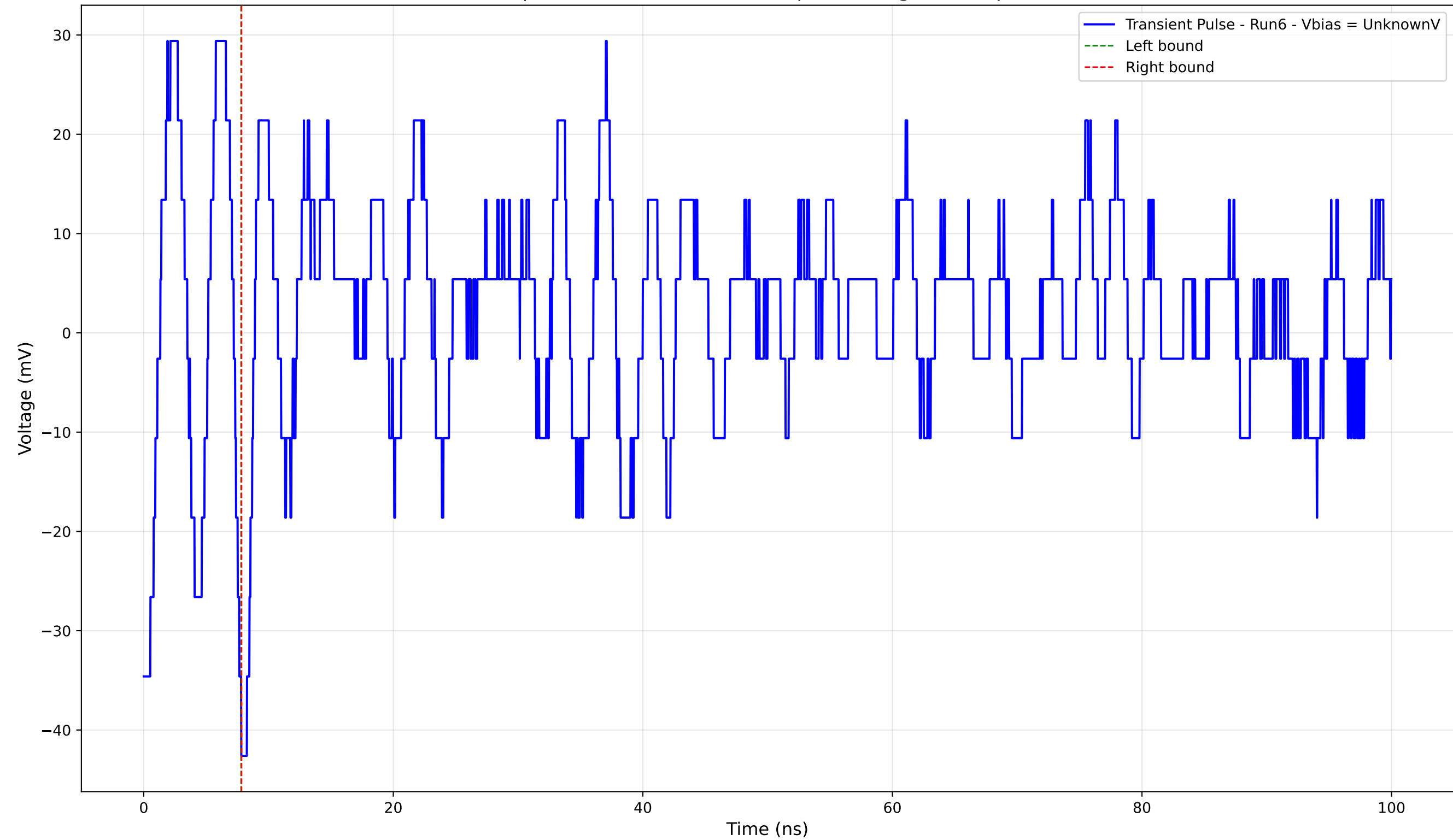
Transient Pulse - Sample: 4004 - Position: 410.0 \mu\text{m} - Charge: -0.03 pC - Rise Time: 0.50 ns
