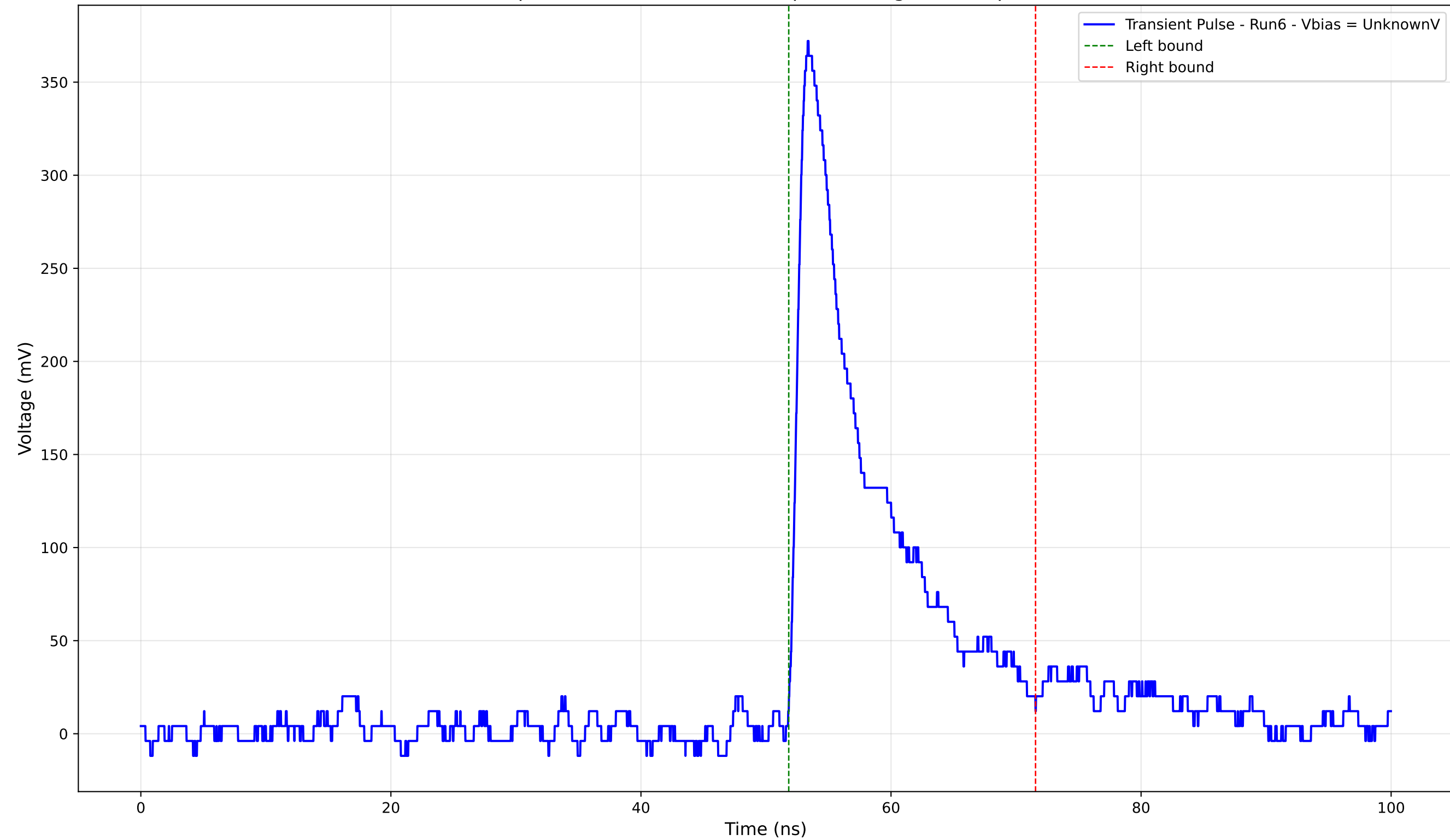
Transient Pulse - Sample: 4004 - Position: 580.0 \mu\text{m} - Charge: 48.24 pC - Rise Time: 1.04 ns
