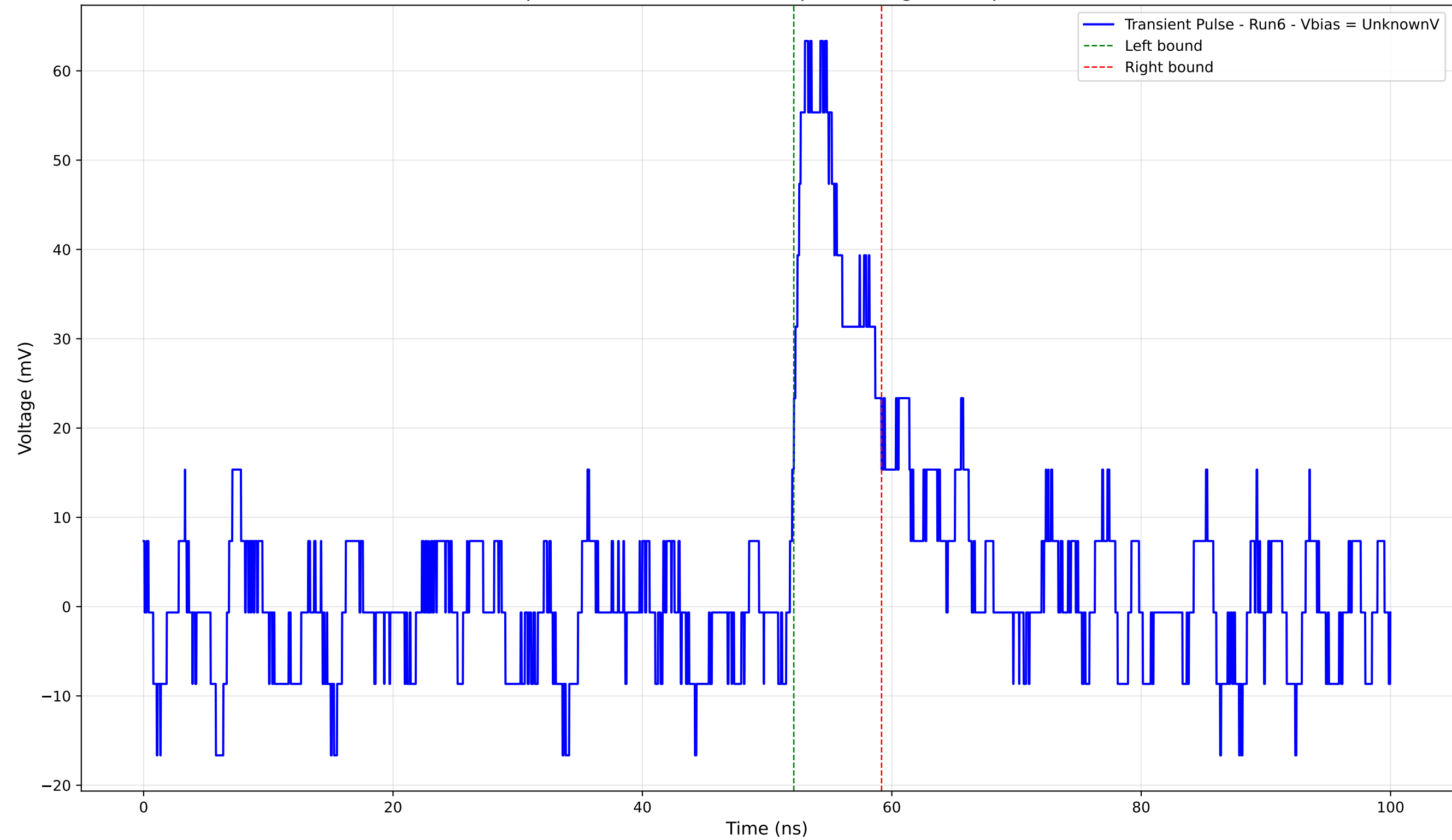
Transient Pulse - Sample: 4004 - Position: 885.0 \mu\text{m} - Charge: 5.92 pC - Rise Time: 1.20 ns
