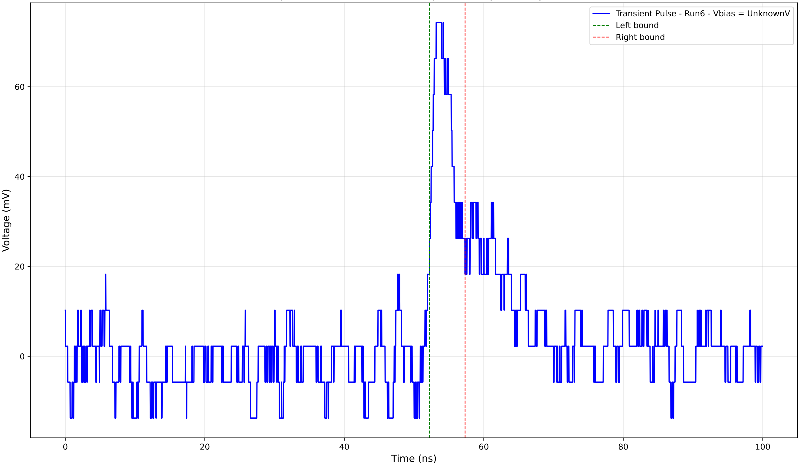
Transient Pulse - Sample: 4004 - Position: 970.0 \mu\text{m} - Charge: 5.14 pC - Rise Time: 1.41 ns
