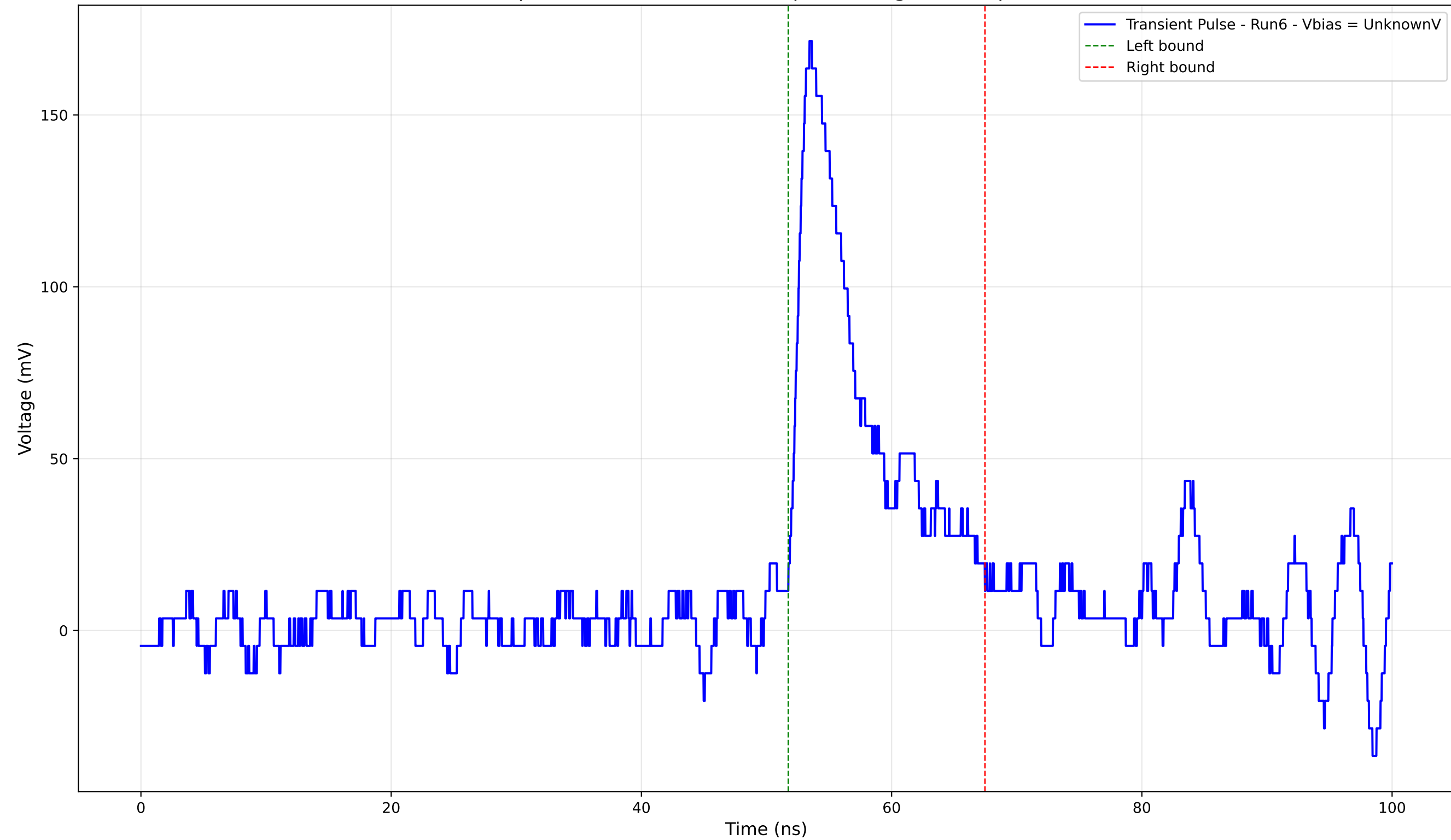
Transient Pulse - Sample: 4004 - Position: 790.0 \mu\text{m} - Charge: 20.95 pC - Rise Time: 1.31 ns
