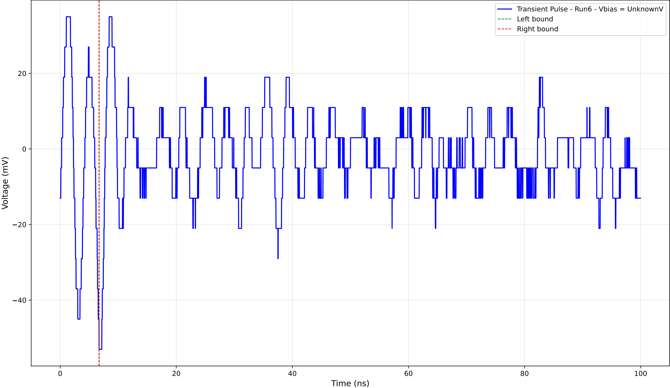
Transient Pulse - Sample: 4004 - Position: 0.0 \mu\text{m} - Charge: -0.04 pC - Rise Time: 0.60 ns
