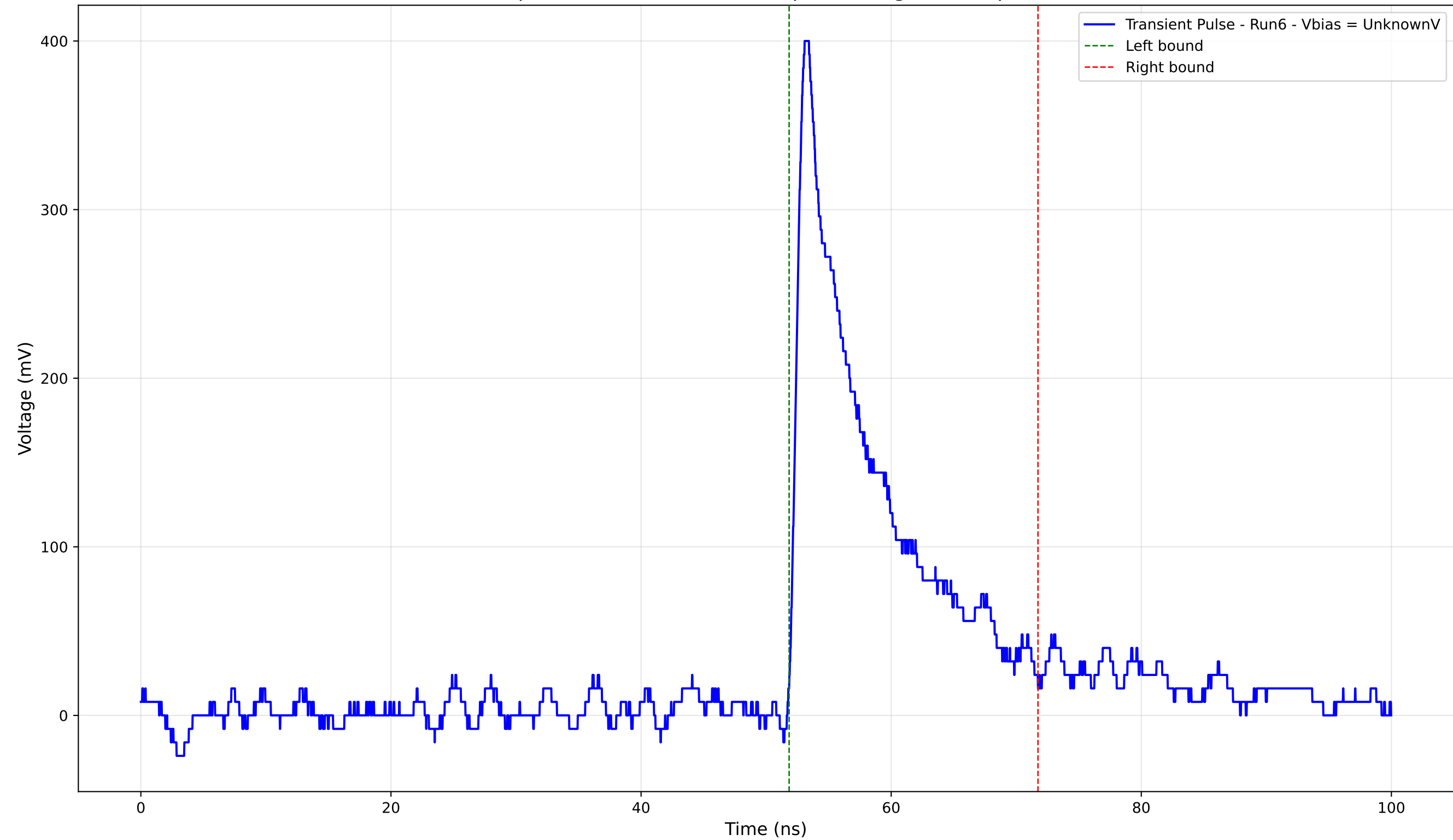
Transient Pulse - Sample: 4004 - Position: 620.0 \mu\text{m} - Charge: 51.97 pC - Rise Time: 0.92 ns
