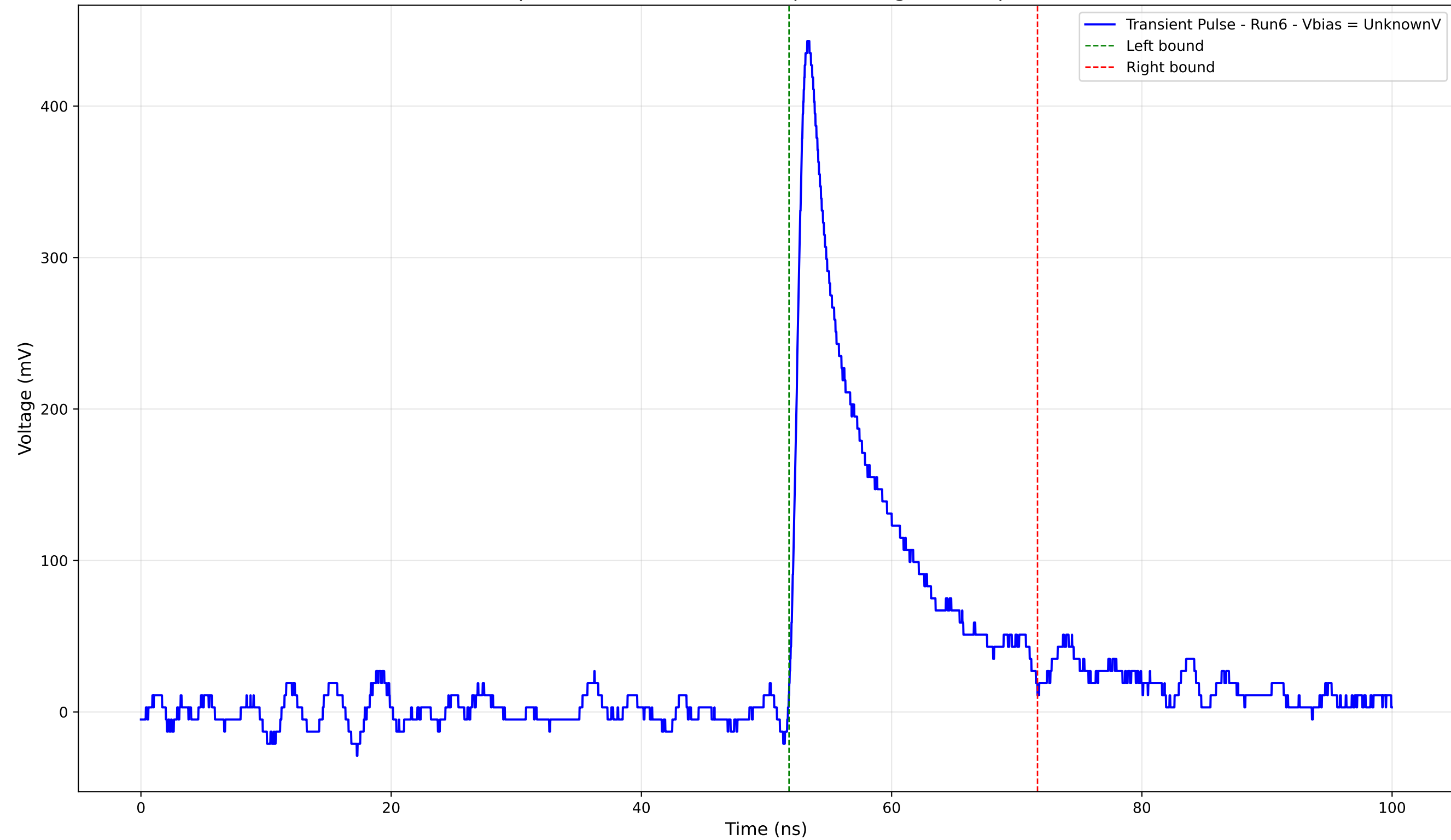
Transient Pulse - Sample: 4004 - Position: 600.0 \mu\text{m} - Charge: 54.33 pC - Rise Time: 0.98 ns
