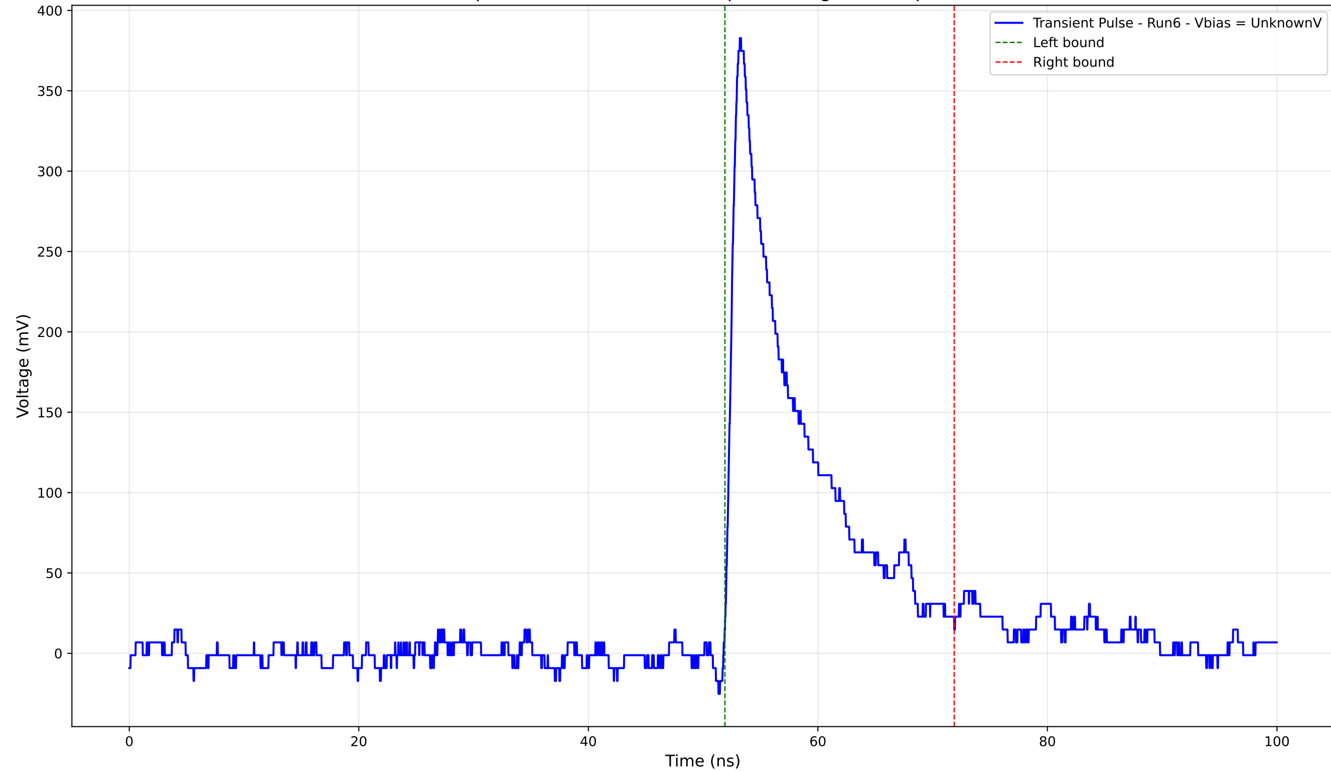
Transient Pulse - Sample: 4004 - Position: 630.0 \mu\text{m} - Charge: 48.72 pC - Rise Time: 0.93 ns
