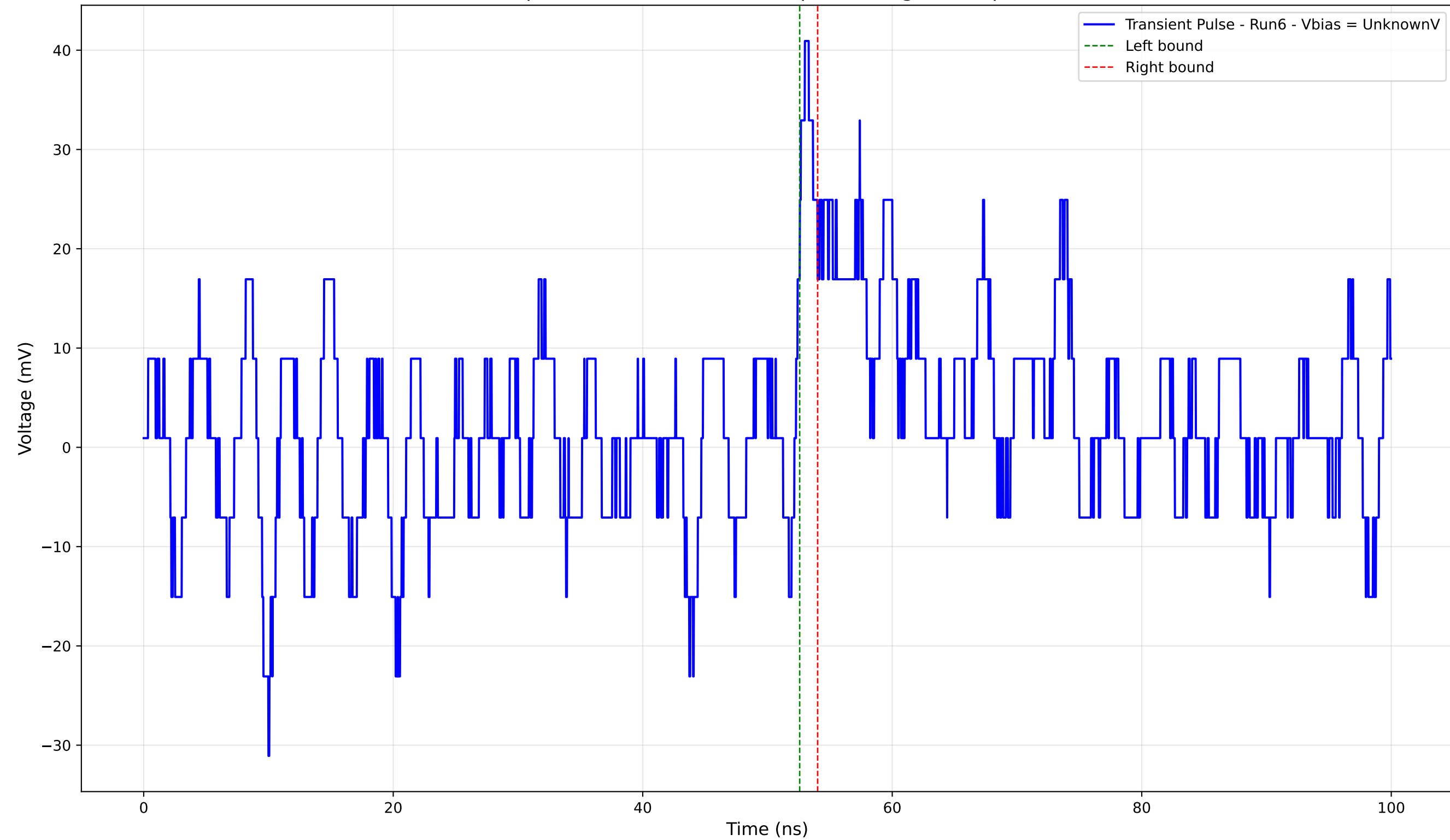
Transient Pulse - Sample: 4004 - Position: 860.0 \mu\text{m} - Charge: 0.92 pC - Rise Time: 0.71 ns
