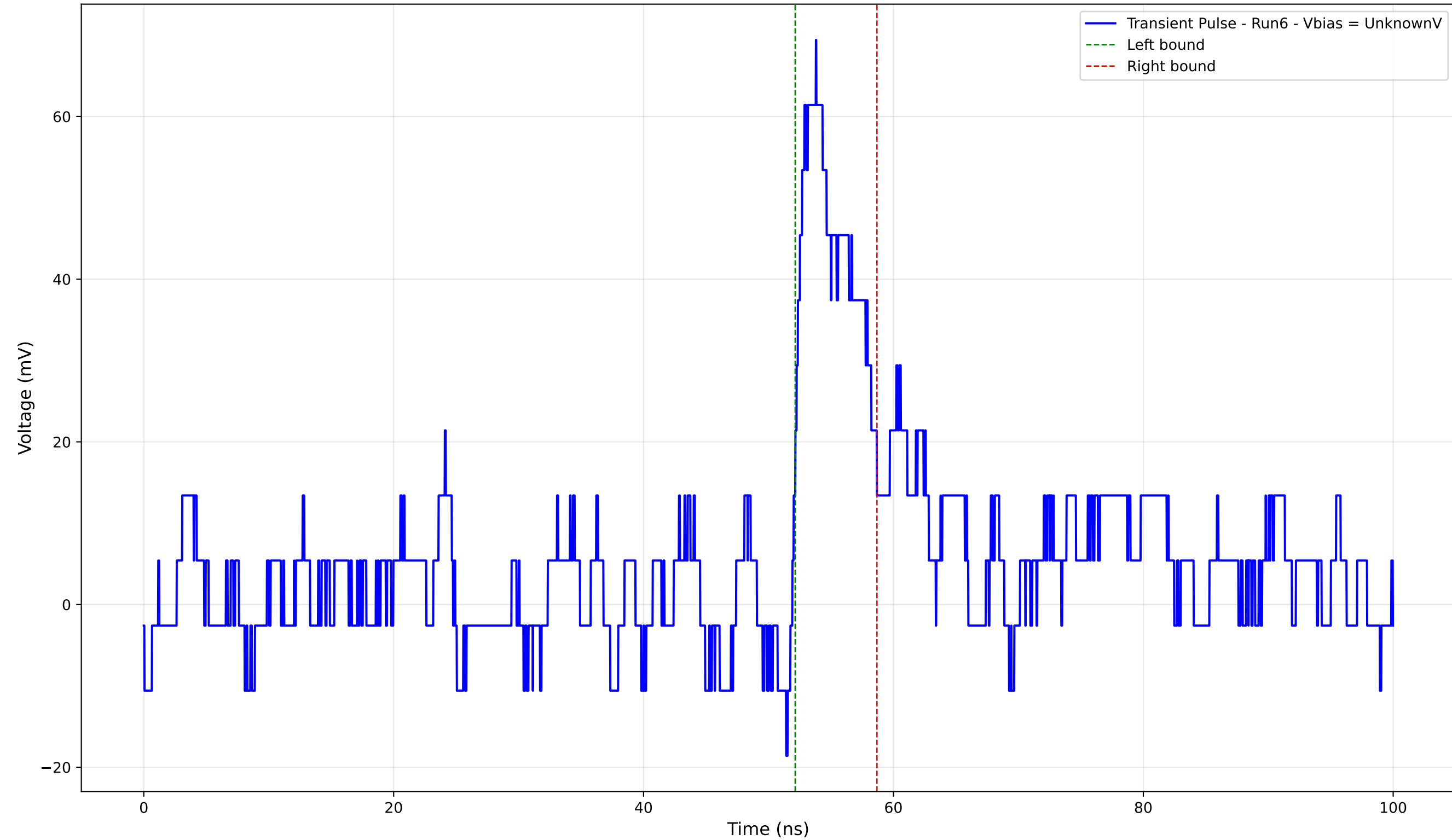
Transient Pulse - Sample: 4004 - Position: 940.0 \mu\text{m} - Charge: 5.78 pC - Rise Time: 1.80 ns
