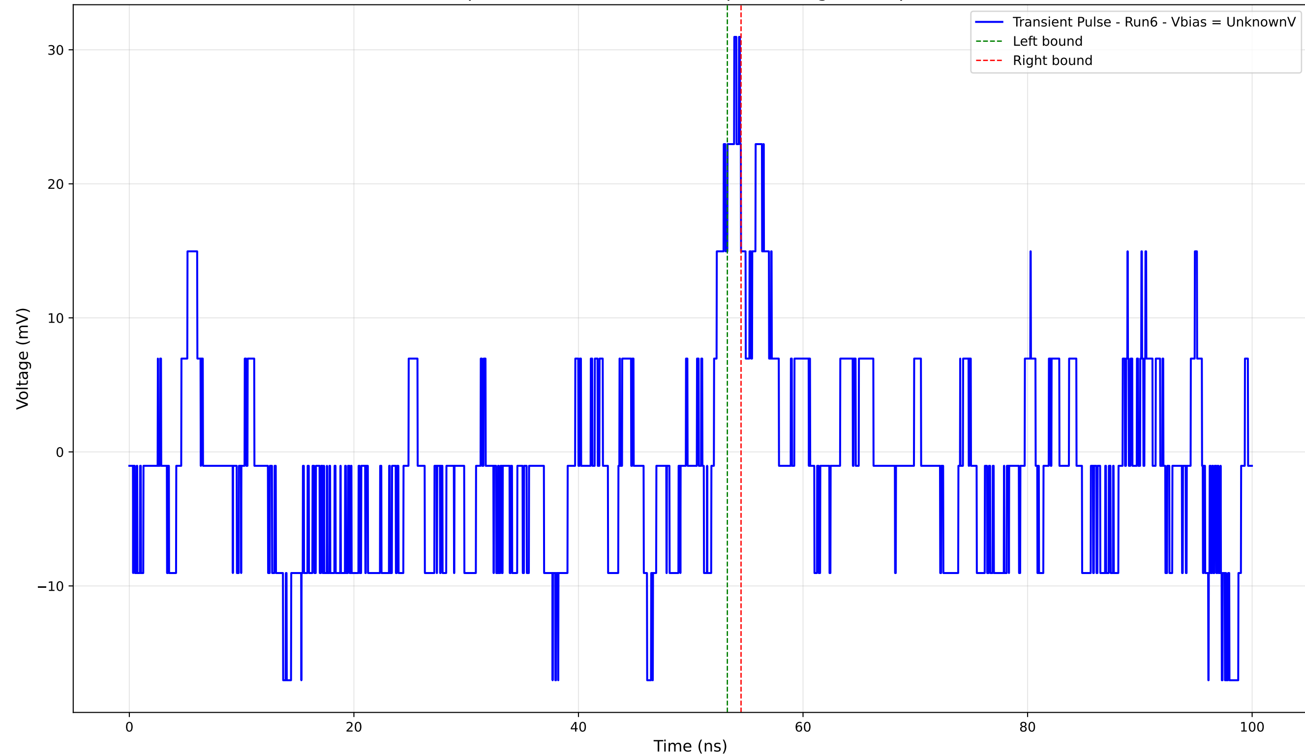
Transient Pulse - Sample: 4004 - Position: 1150.0 \mu\text{m} - Charge: 0.61 pC - Rise Time: 1.81 ns
