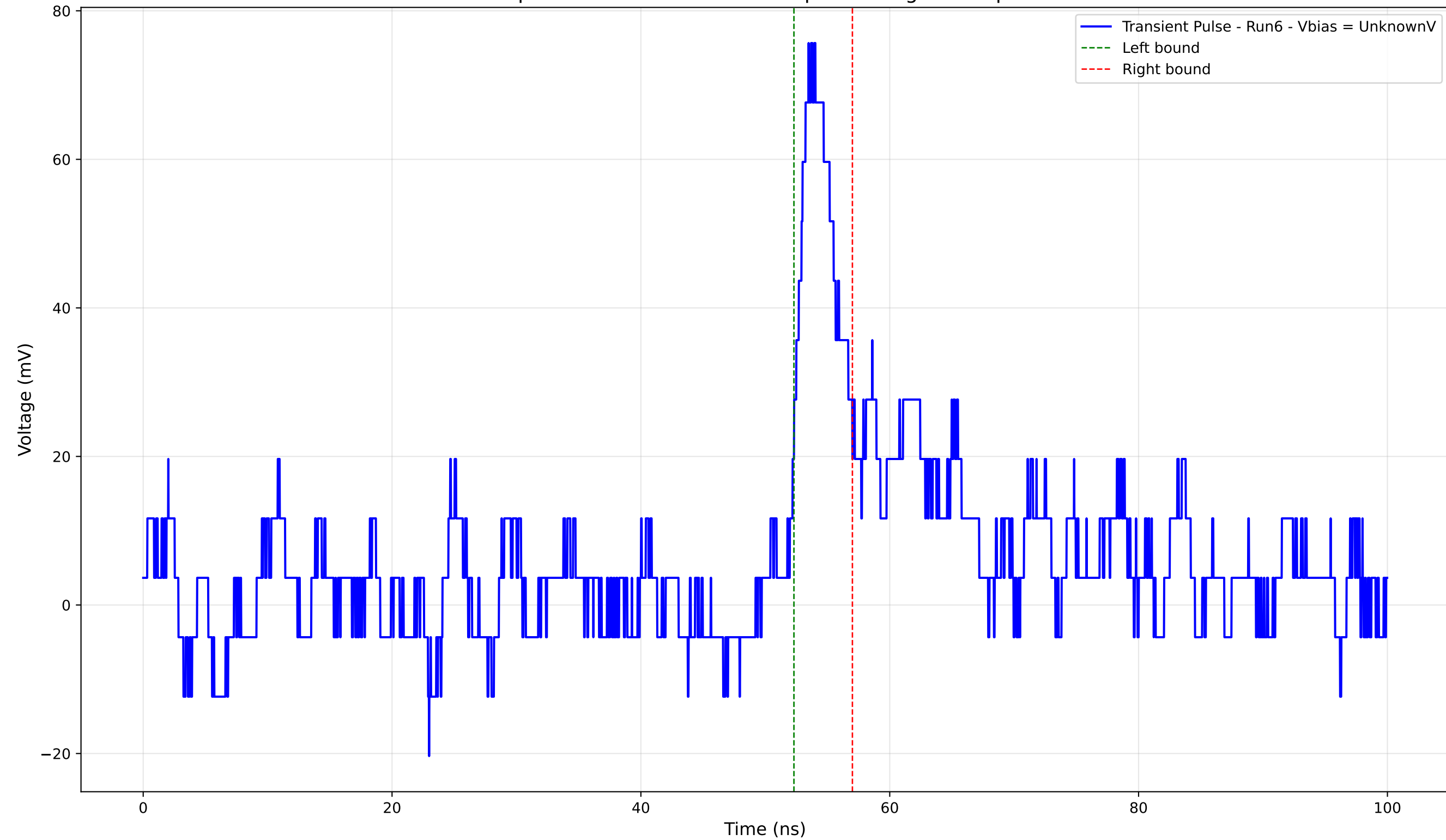
Transient Pulse - Sample: 4004 - Position: 1015.0 \mu\text{m} - Charge: 4.79 pC - Rise Time: 1.51 ns
