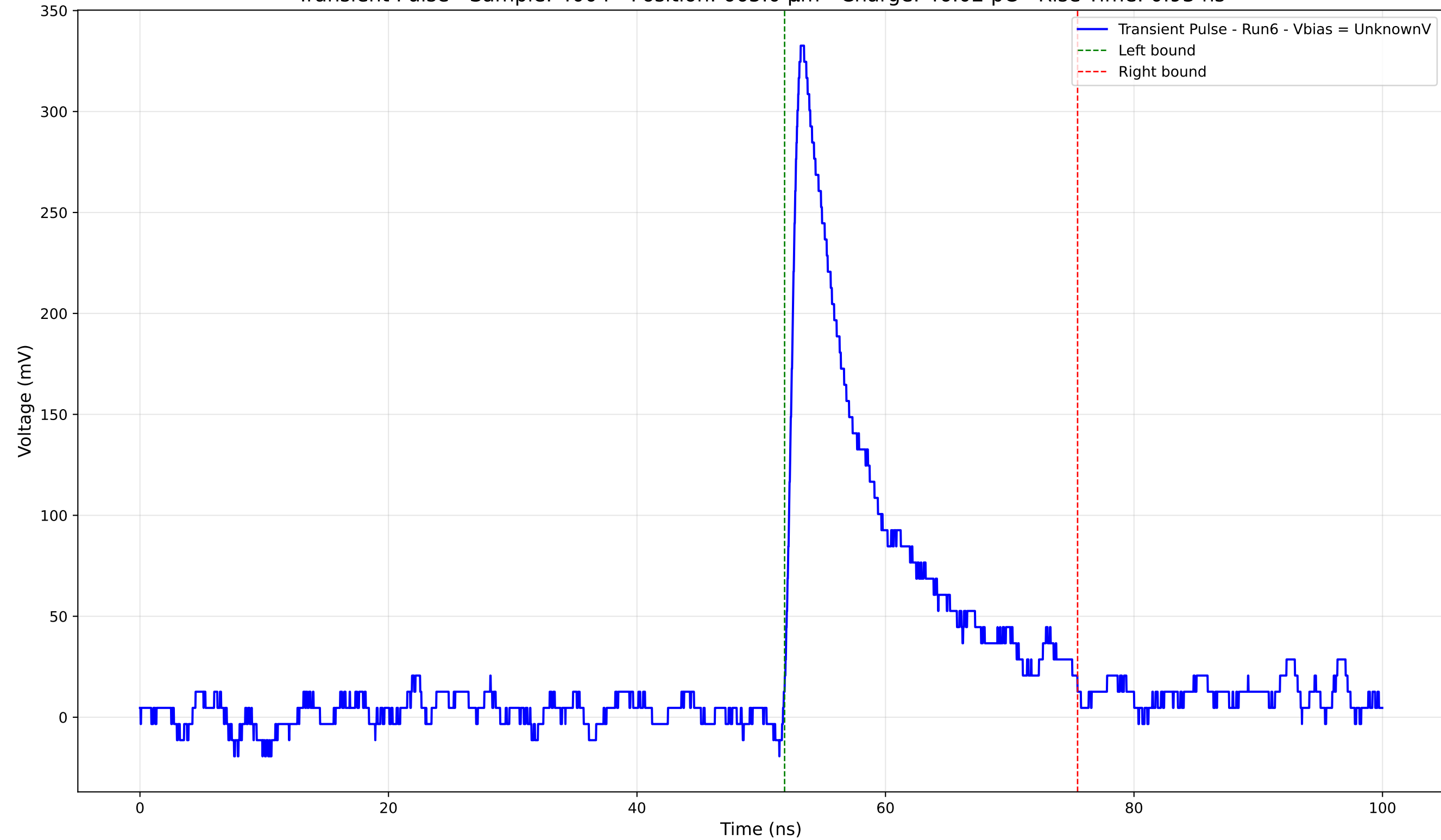
Transient Pulse - Sample: 4004 - Position: 665.0 \mu\text{m} - Charge: 46.02 pC - Rise Time: 0.93 ns
