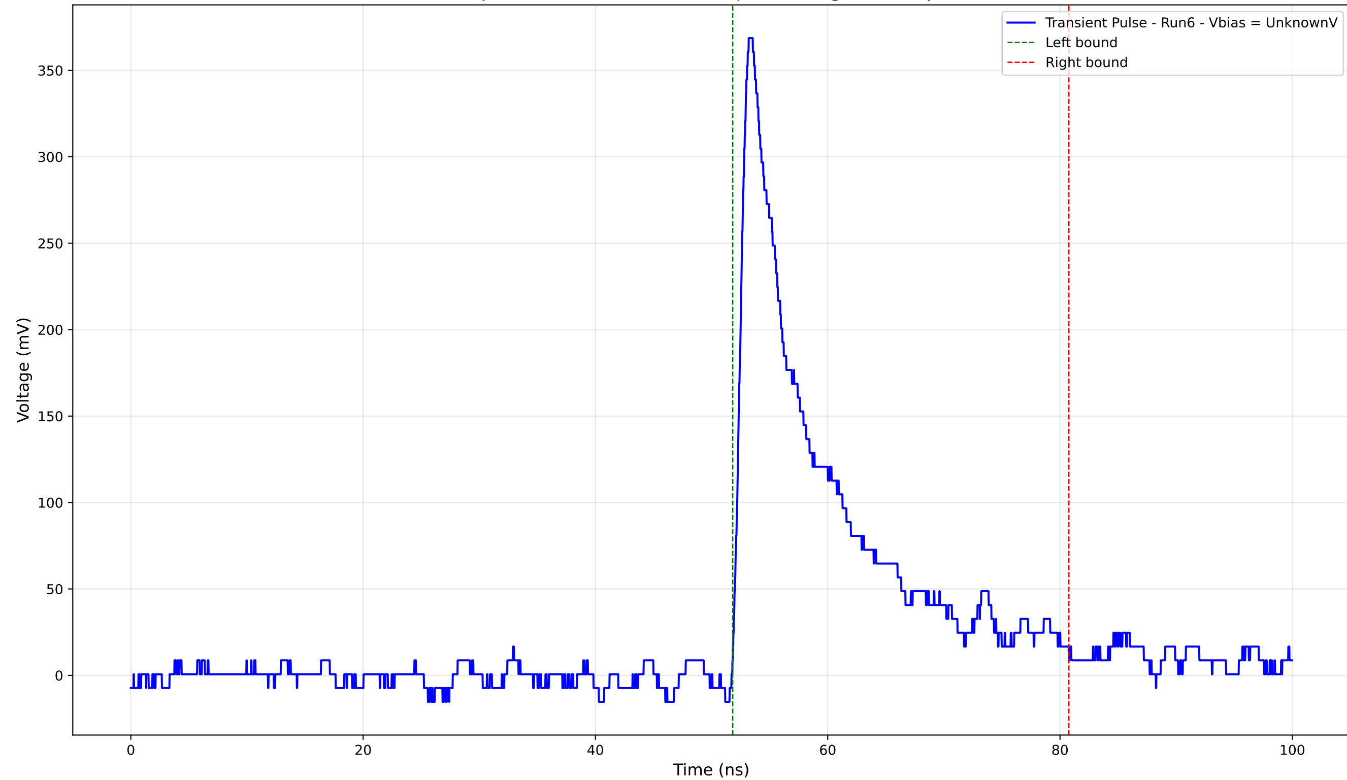
Transient Pulse - Sample: 4004 - Position: 535.0 \mu\text{m} - Charge: 53.24 pC - Rise Time: 1.01 ns
