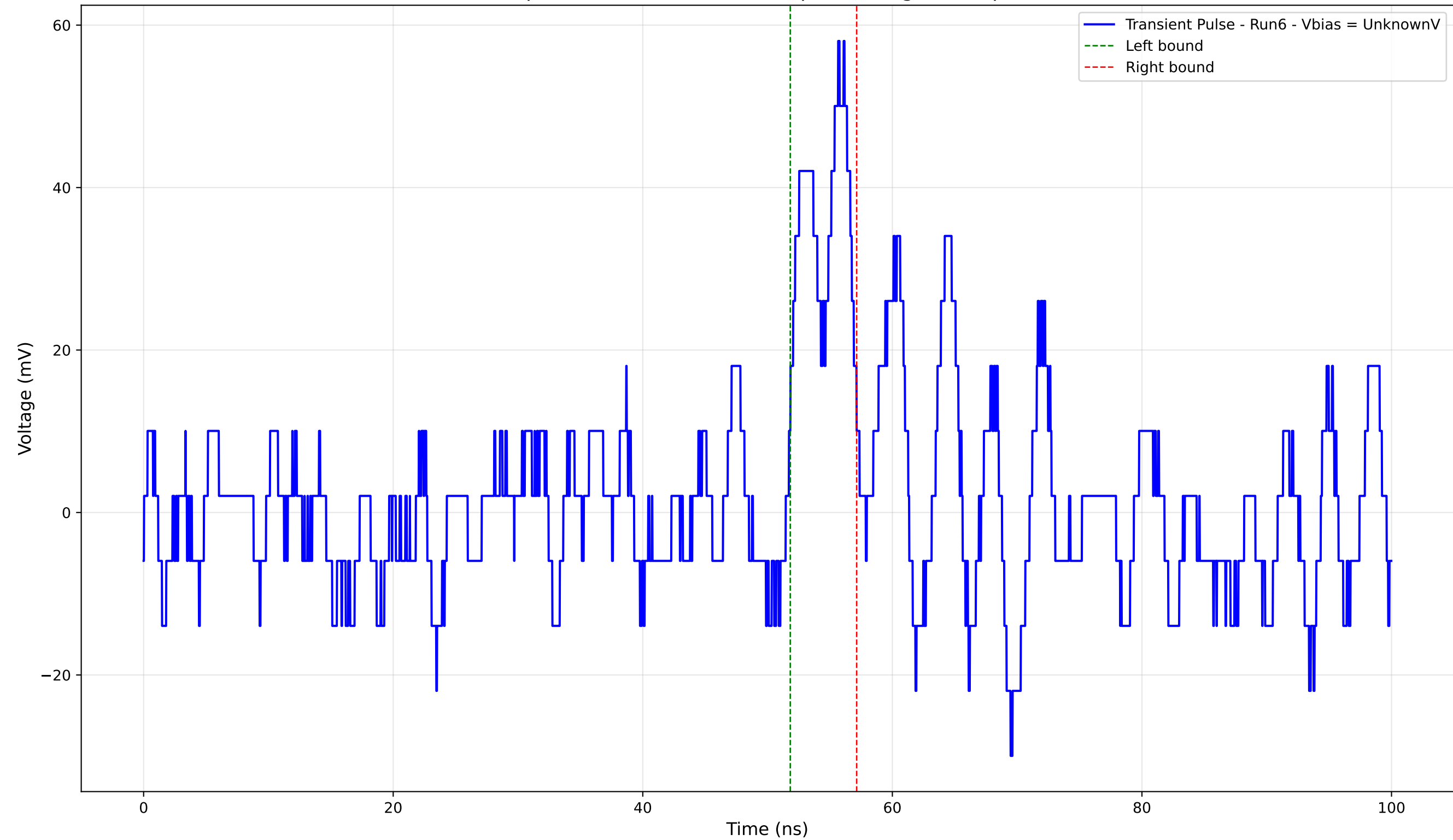
Transient Pulse - Sample: 4004 - Position: 500.0 \mu\text{m} - Charge: 3.86 pC - Rise Time: 3.95 ns
