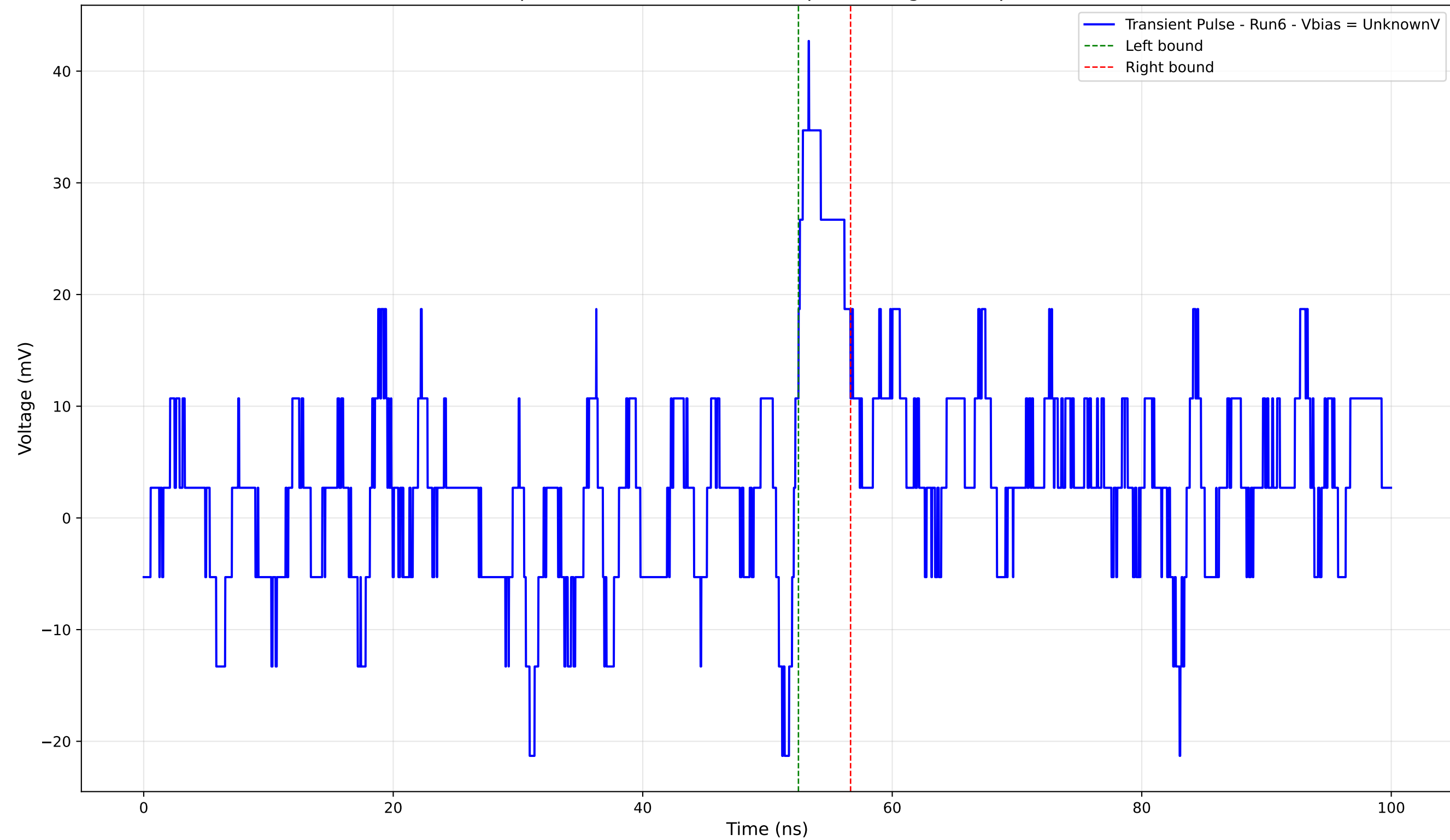
Transient Pulse - Sample: 4004 - Position: 1100.0 \mu\text{m} - Charge: 2.37 pC - Rise Time: 1.08 ns
