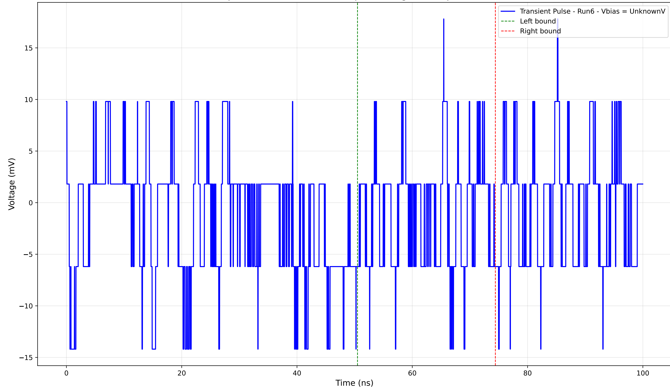
Transient Pulse - Sample: 4004 - Position: 180.0 \mu\text{m} - Charge: -0.43 pC - Rise Time: 0.00 ns (N/A)
