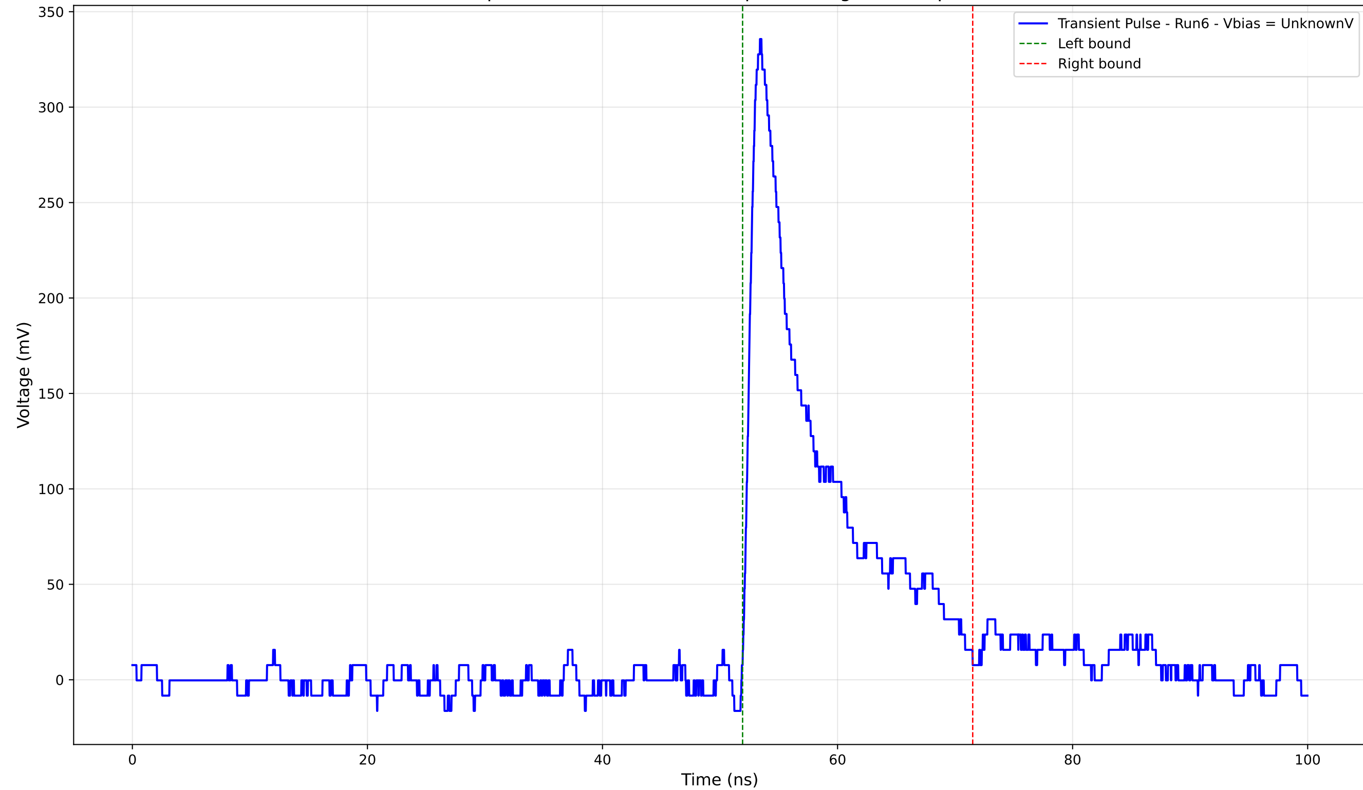
Transient Pulse - Sample: 4004 - Position: 530.0 \mu\text{m} - Charge: 42.21 pC - Rise Time: 0.94 ns
