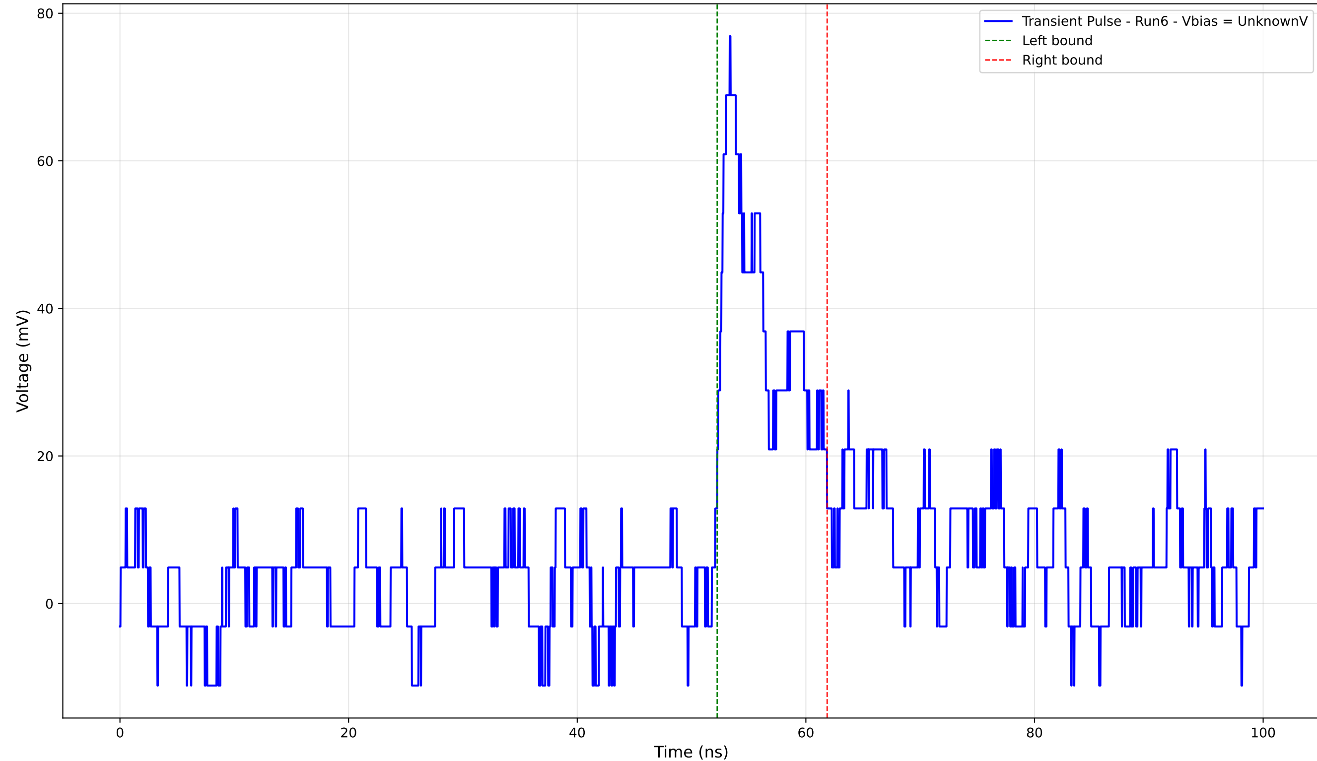
Transient Pulse - Sample: 4004 - Position: 1010.0 \mu\text{m} - Charge: 7.44 pC - Rise Time: 1.27 ns
