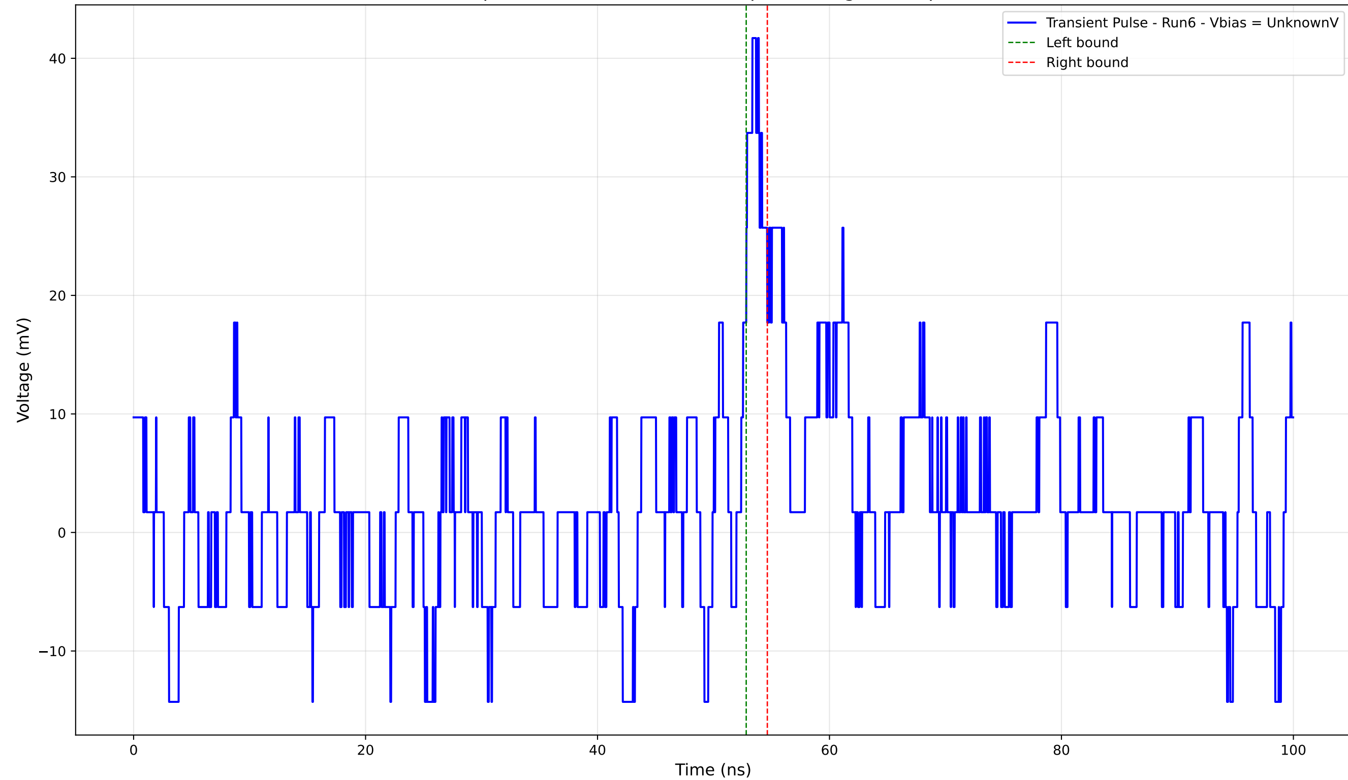
Transient Pulse - Sample: 4004 - Position: 1140.0 \mu\text{m} - Charge: 1.19 pC - Rise Time: 0.97 ns
