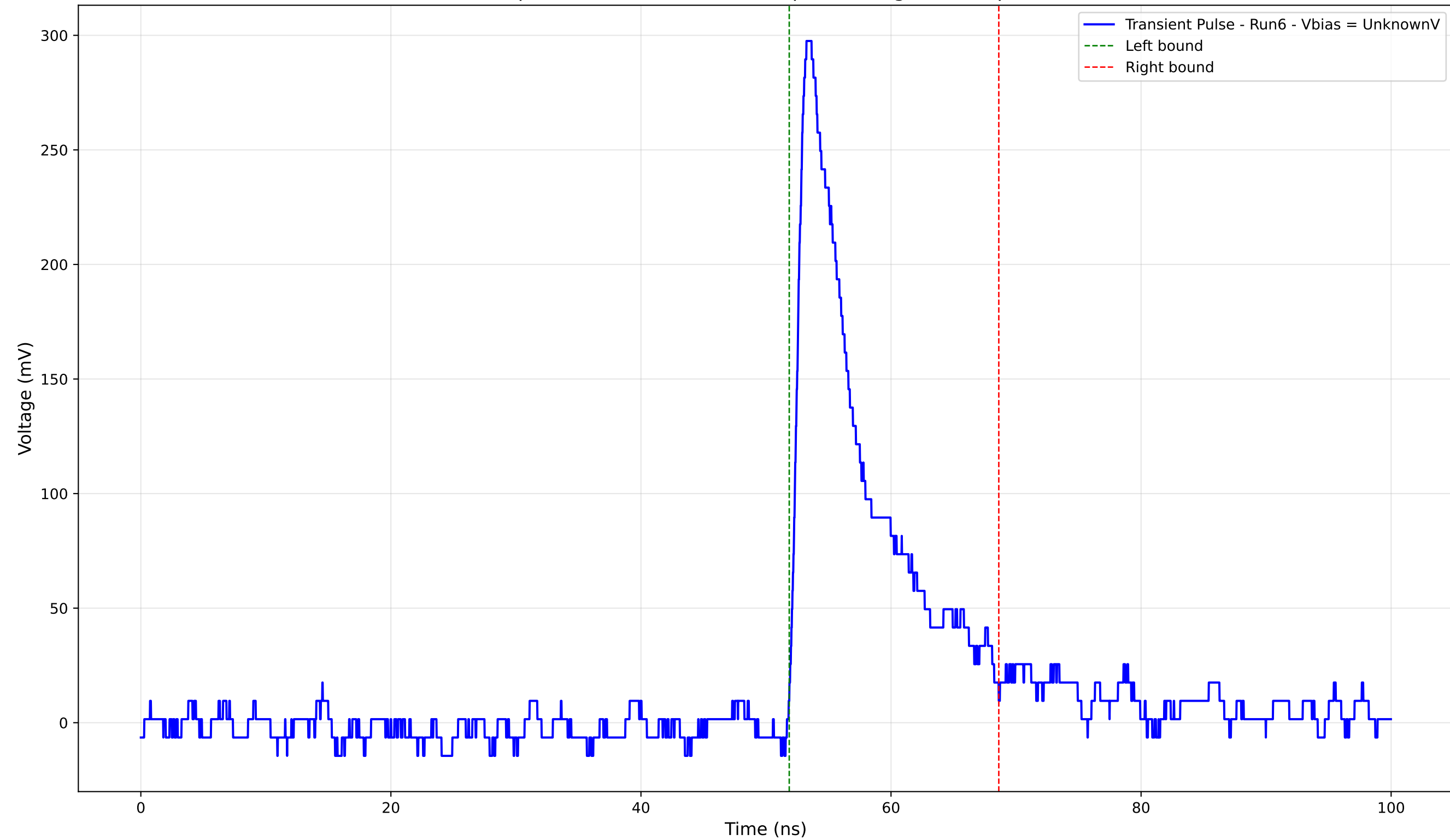
Transient Pulse - Sample: 4004 - Position: 725.0 \mu\text{m} - Charge: 35.38 pC - Rise Time: 1.01 ns
