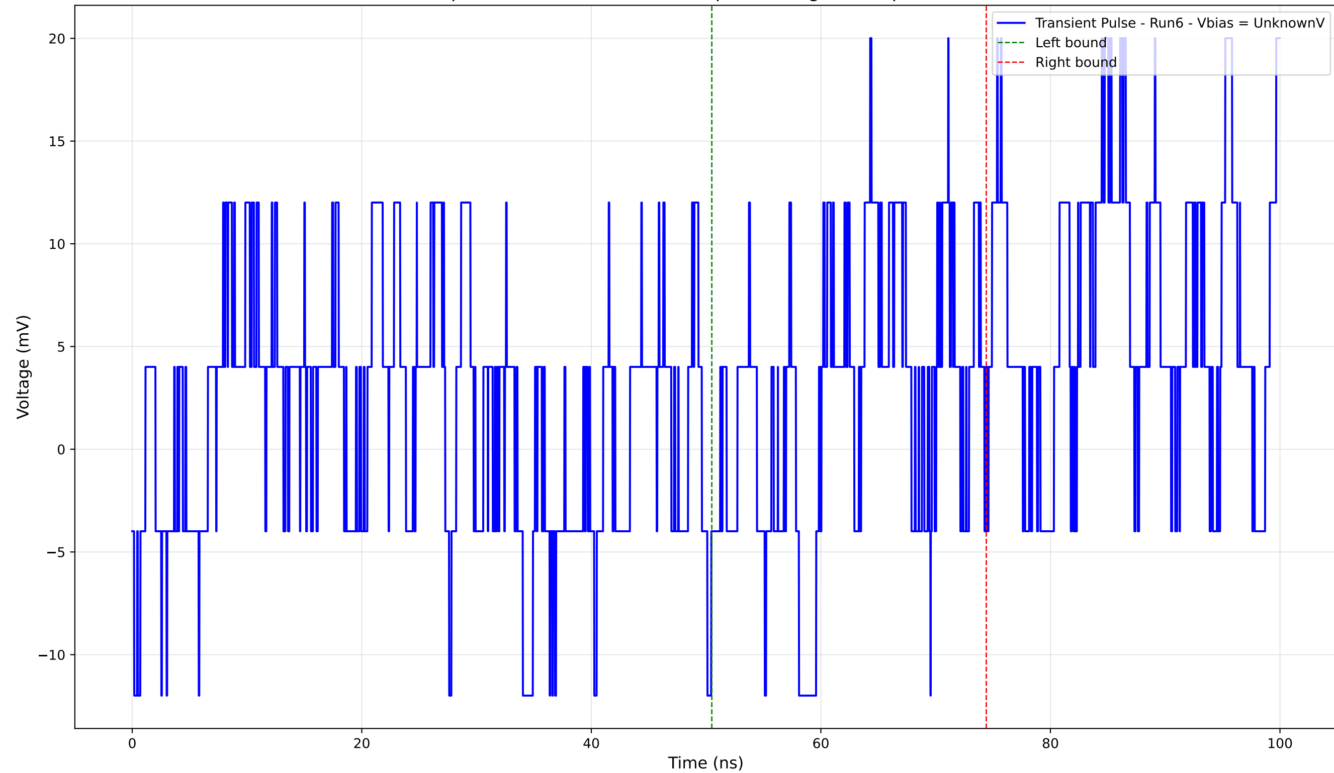
Transient Pulse - Sample: 4004 - Position: 1200.0 \mu\text{m} - Charge: 1.12 pC - Rise Time: 0.00 ns (N/A)
