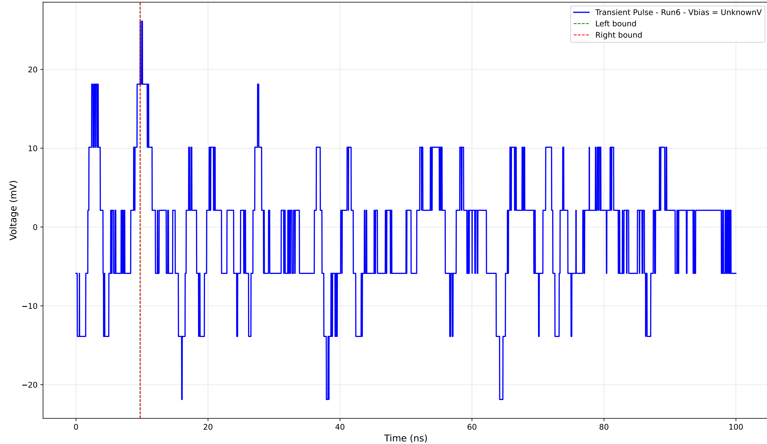
Transient Pulse - Sample: 4004 - Position: 380.0 \mu\text{m} - Charge: 0.02 pC - Rise Time: 0.80 ns
