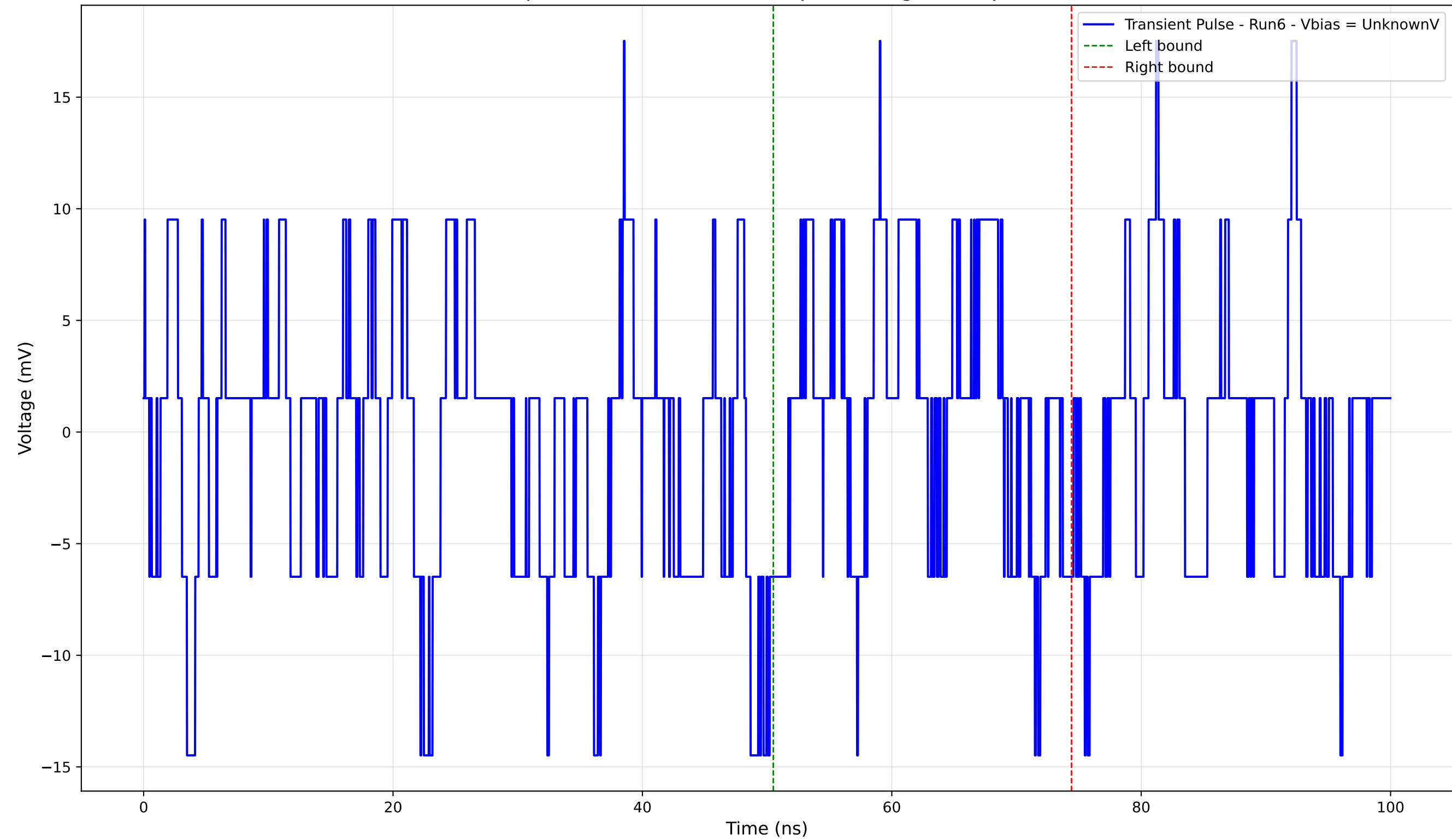
Transient Pulse - Sample: 4004 - Position: 415.0 \mu\text{m} - Charge: 0.70 pC - Rise Time: 0.12 ns
