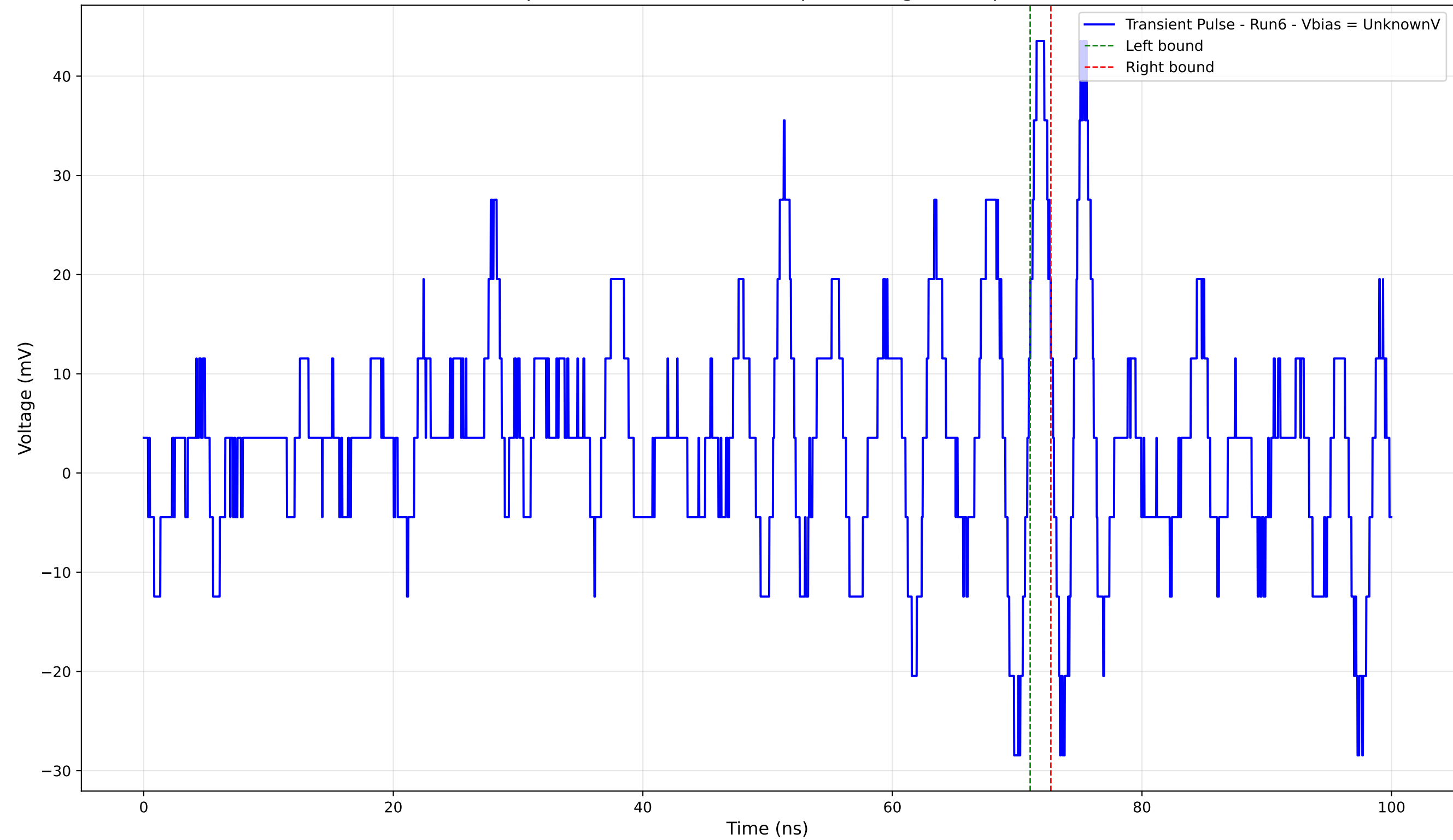
Transient Pulse - Sample: 4004 - Position: 220.0 \mu\text{m} - Charge: 1.13 pC - Rise Time: 0.64 ns
