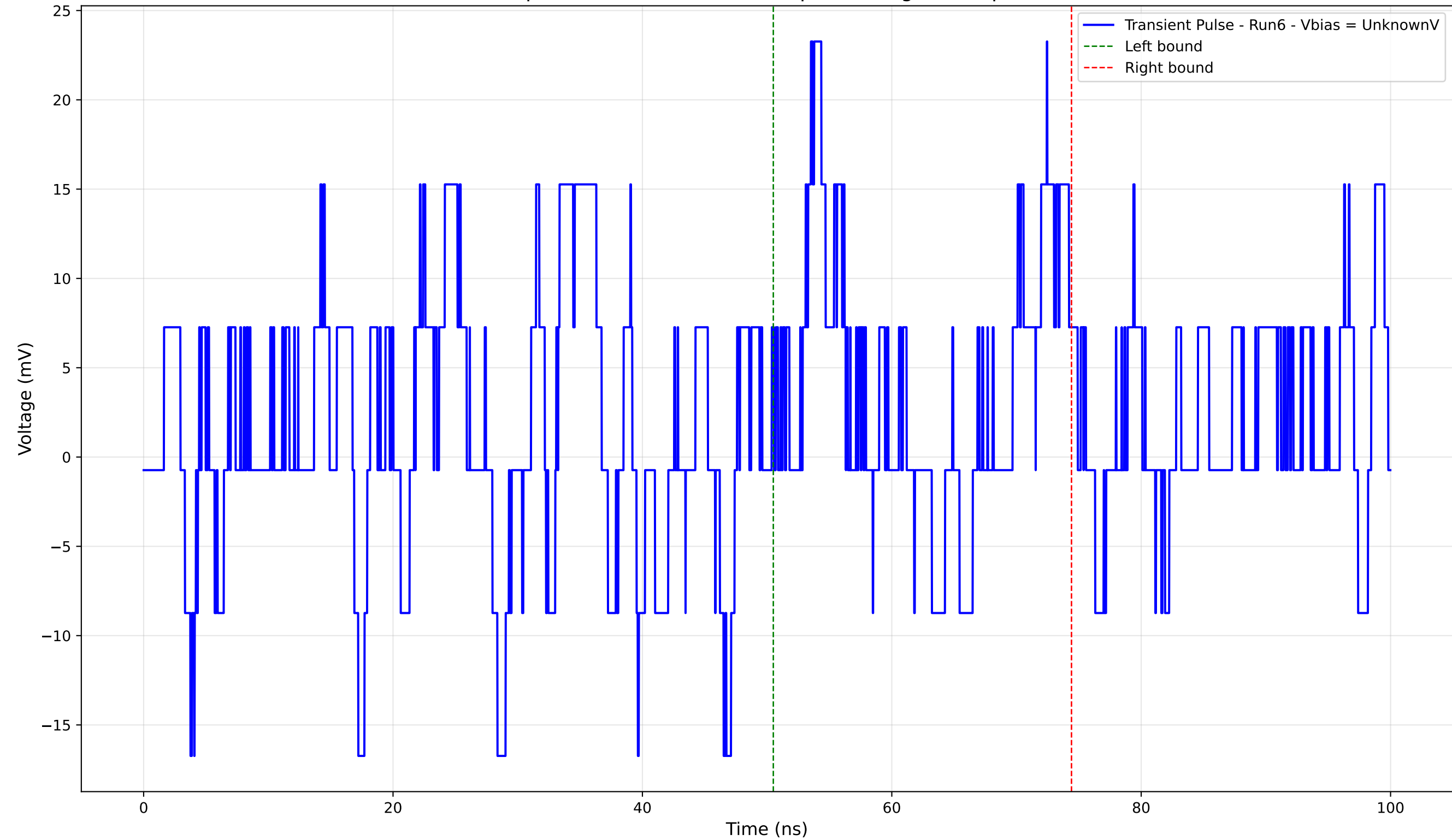
Transient Pulse - Sample: 4004 - Position: 105.0 \mu\text{m} - Charge: 1.92 pC - Rise Time: 0.68 ns
