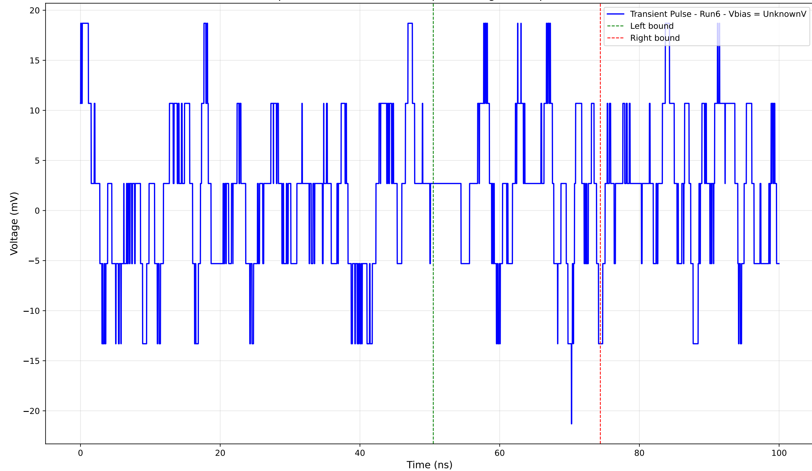
Transient Pulse - Sample: 4004 - Position: 165.0 \mu\text{m} - Charge: 1.01 pC - Rise Time: 0.00 ns (N/A)
