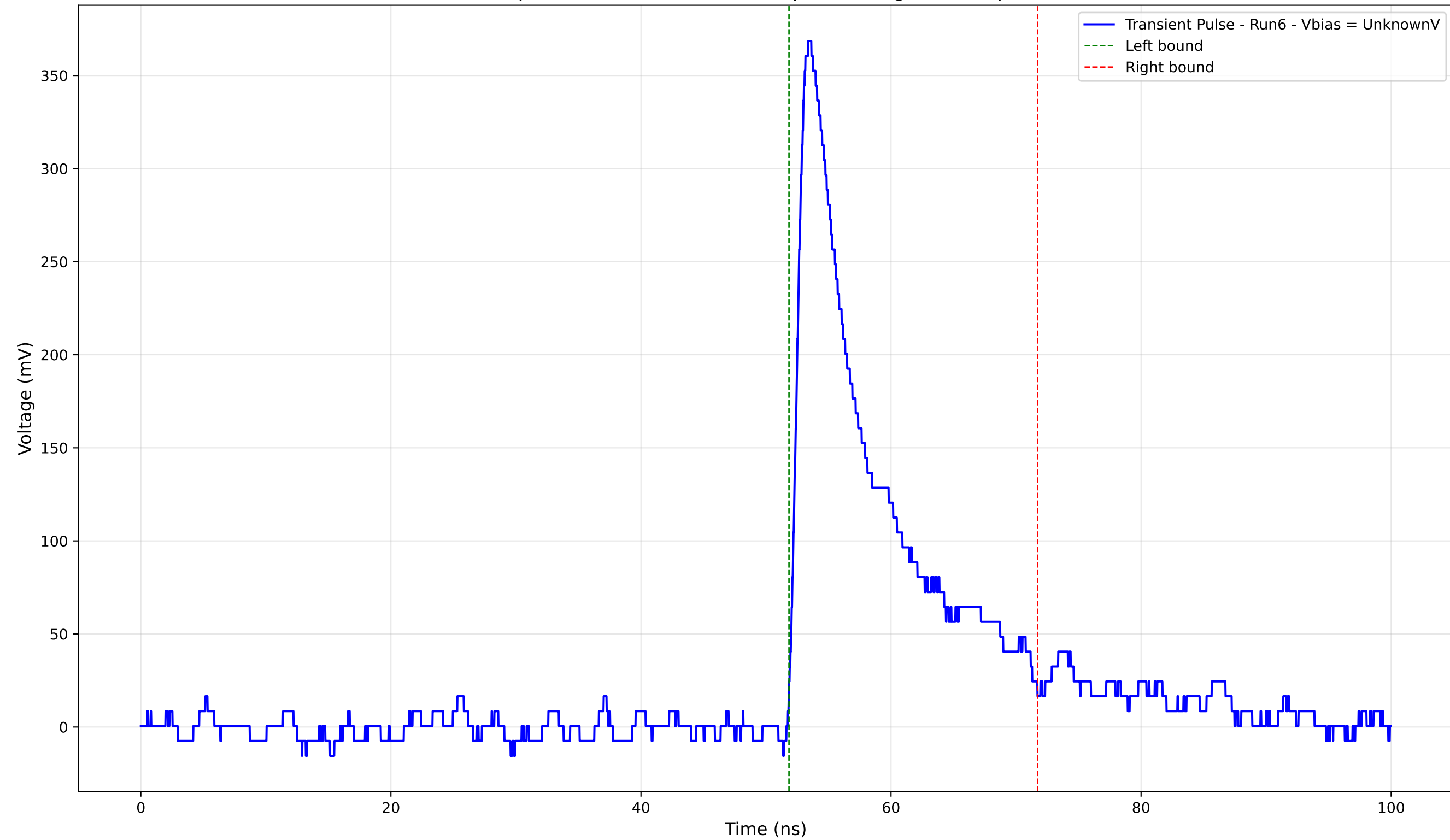
Transient Pulse - Sample: 4004 - Position: 560.0 \mu\text{m} - Charge: 50.24 pC - Rise Time: 1.05 ns
