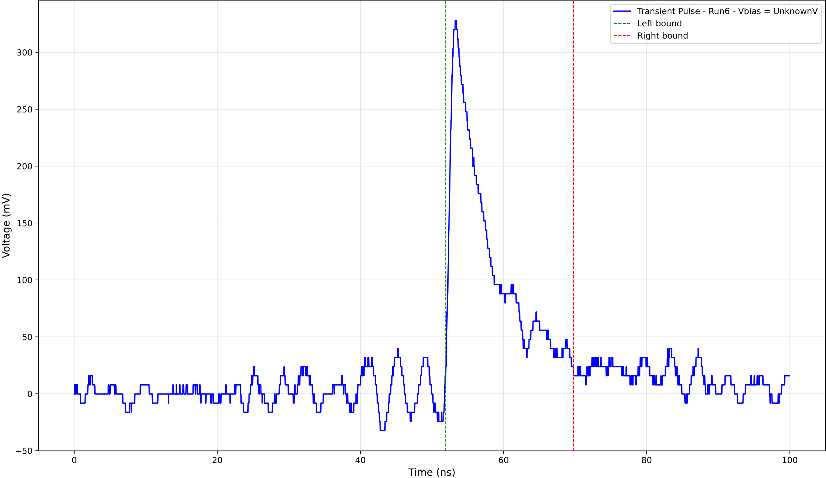
Transient Pulse - Sample: 4004 - Position: 710.0 \mu\text{m} - Charge: 40.74 pC - Rise Time: 0.90 ns
