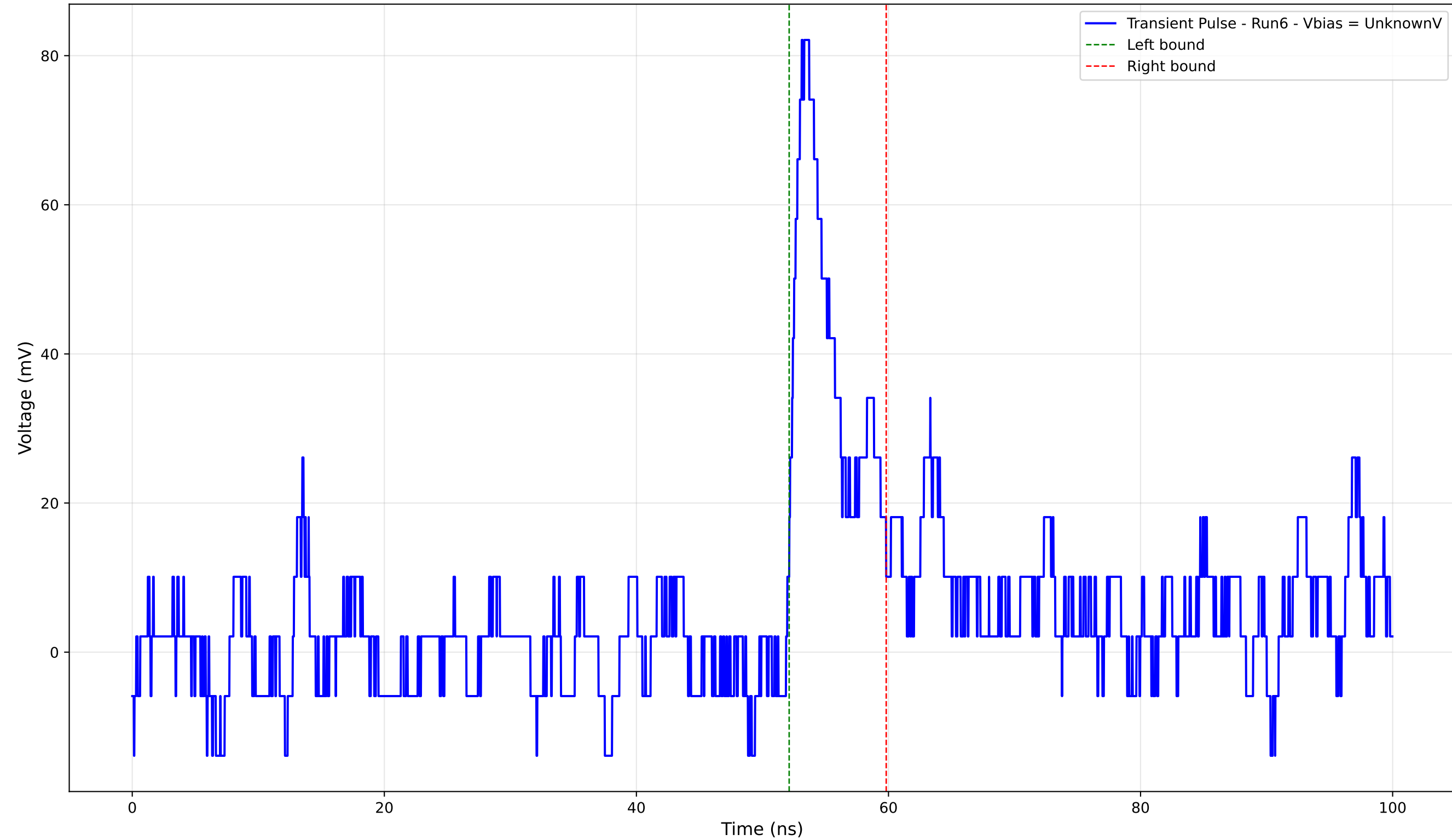
Transient Pulse - Sample: 4004 - Position: 1000.0 \mu\text{m} - Charge: 6.31 pC - Rise Time: 1.00 ns
