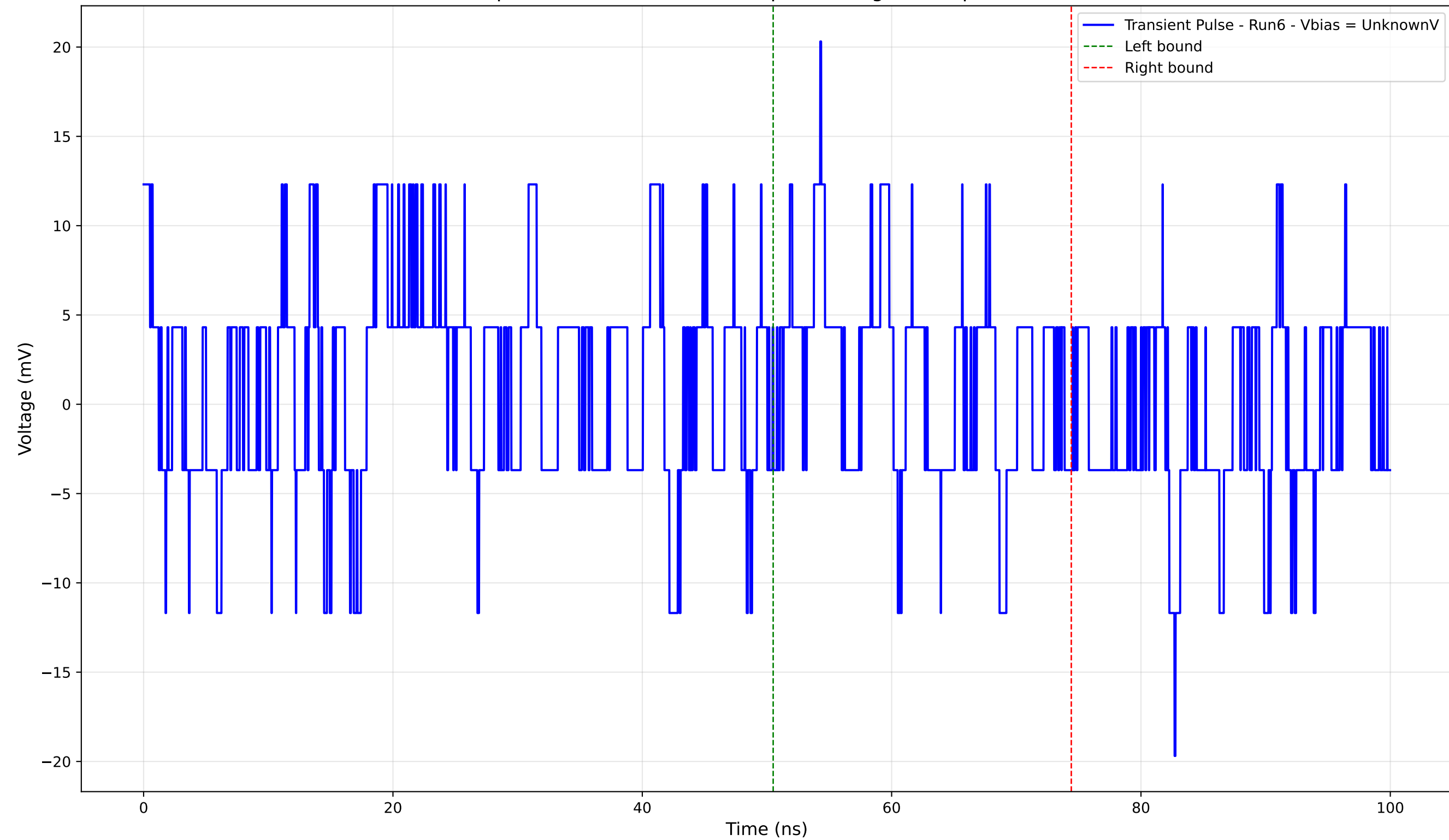
Transient Pulse - Sample: 4004 - Position: 120.0 \mu\text{m} - Charge: 0.74 pC - Rise Time: 0.00 ns (N/A)
