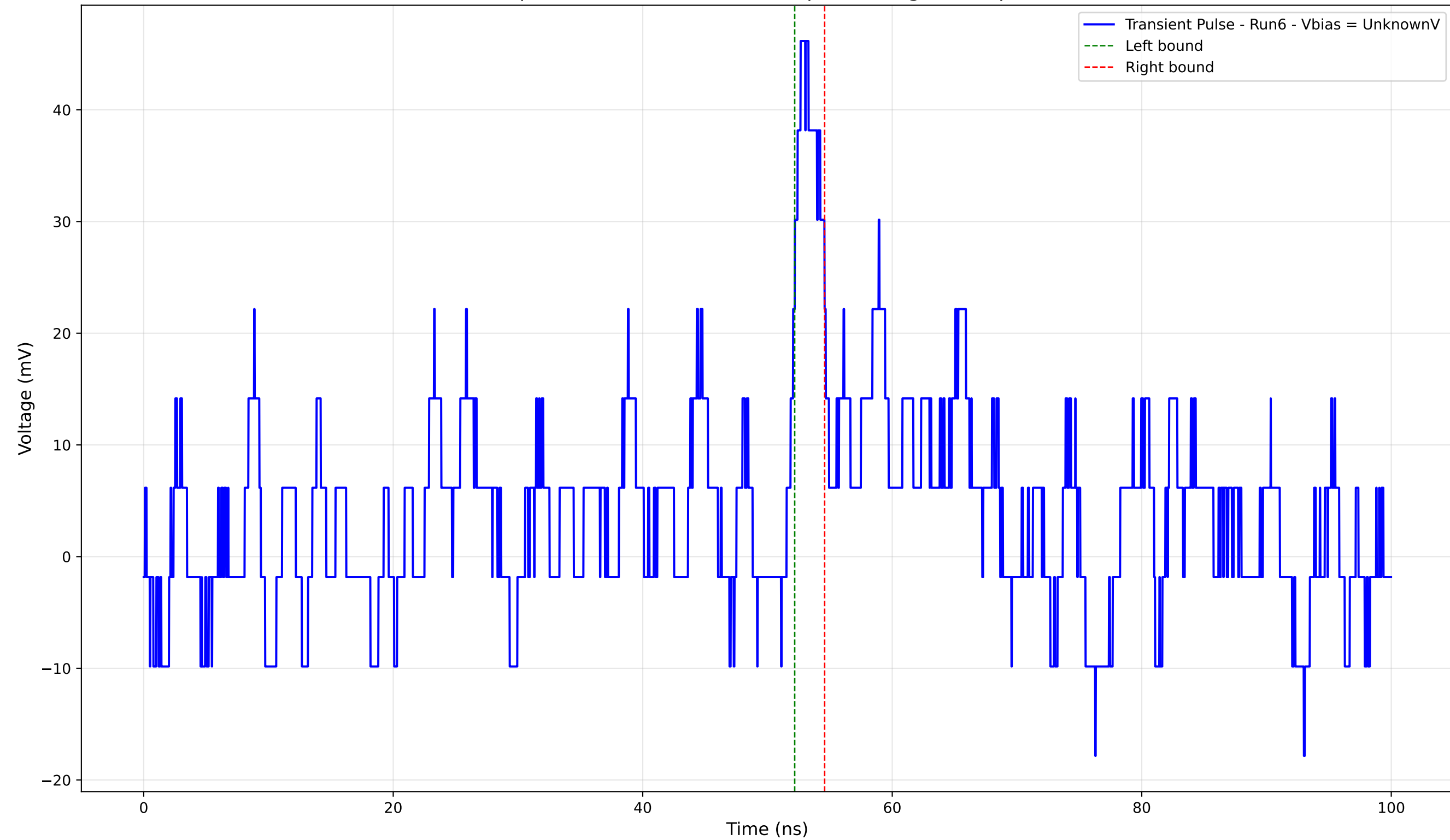
Transient Pulse - Sample: 4004 - Position: 1125.0 \mu\text{m} - Charge: 1.83 pC - Rise Time: 1.13 ns
