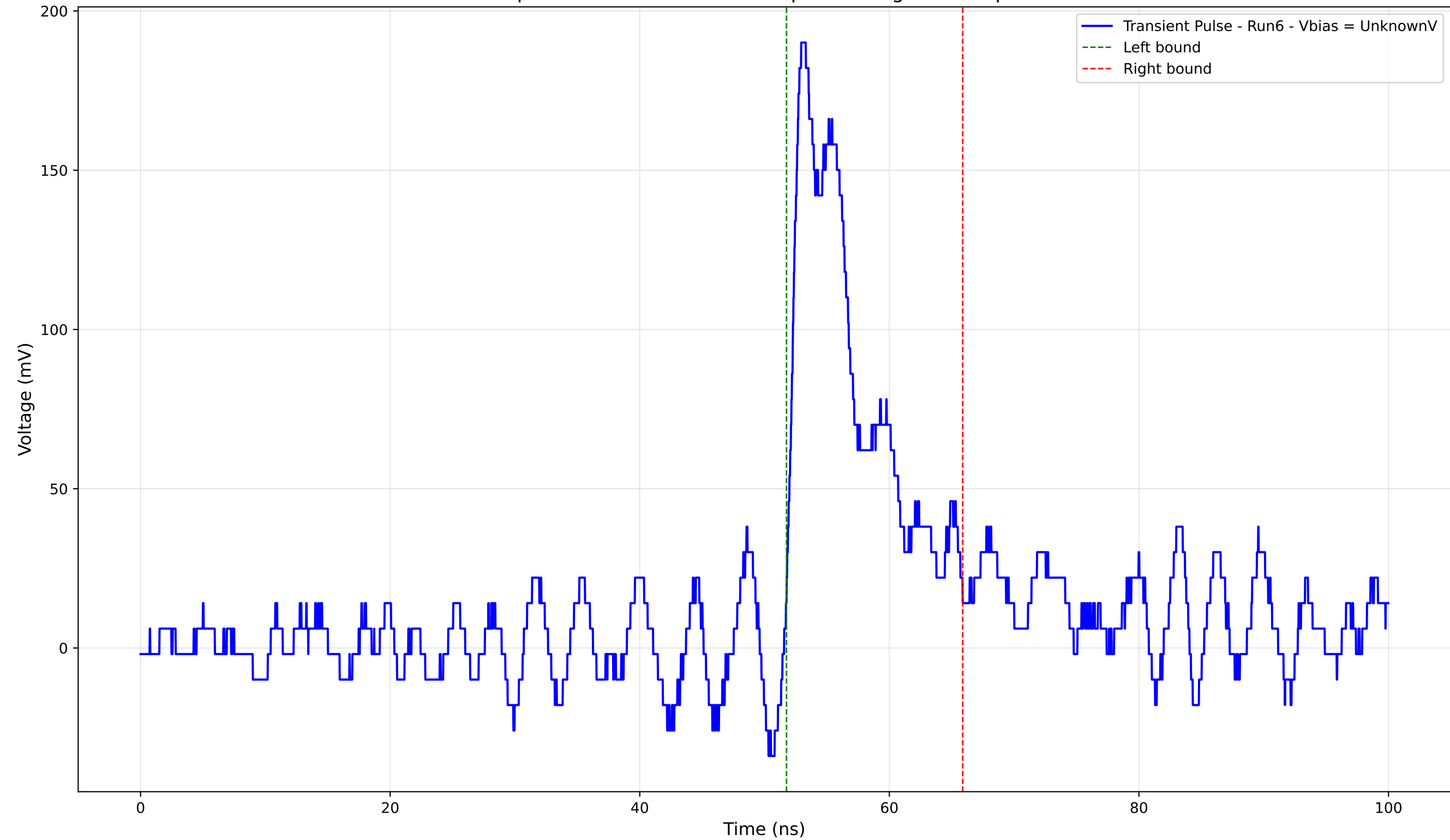
Transient Pulse - Sample: 4004 - Position: 765.0 \mu\text{m} - Charge: 23.25 pC - Rise Time: 0.95 ns
