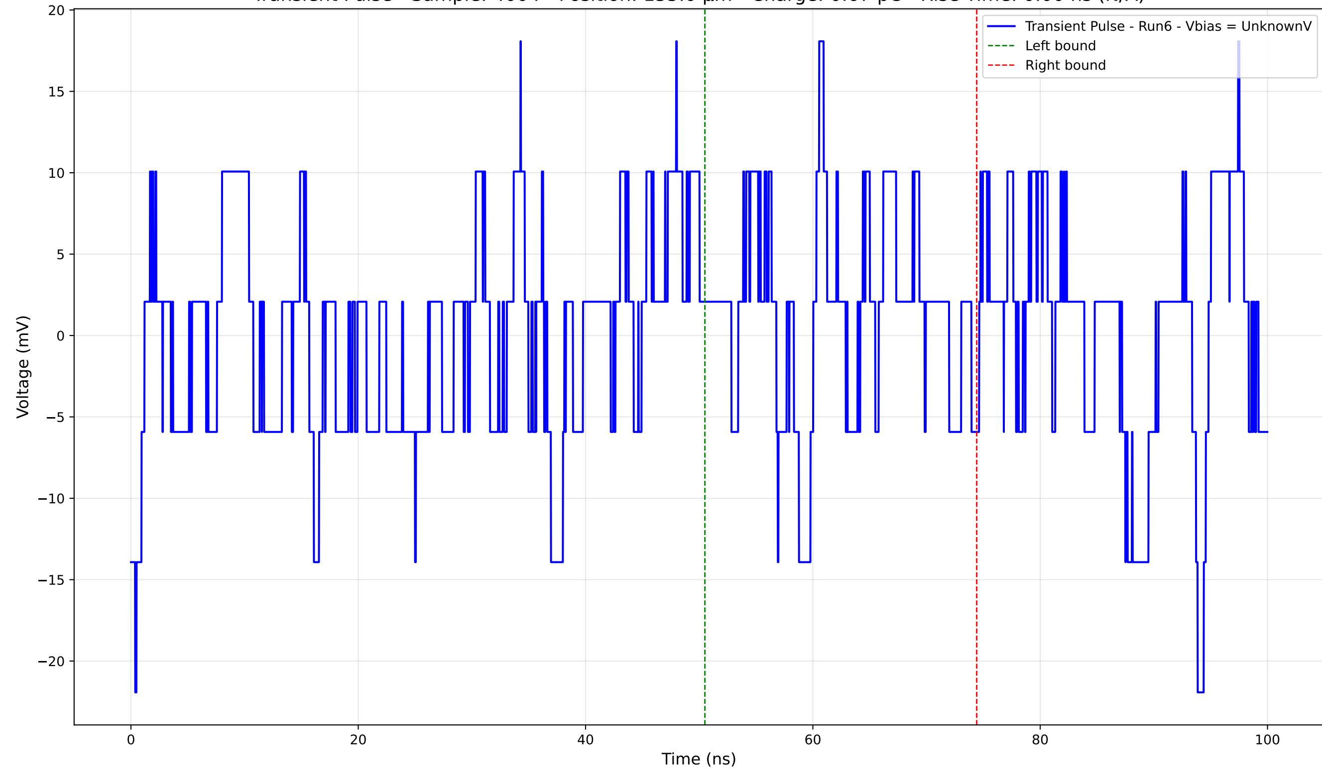
Transient Pulse - Sample: 4004 - Position: 155.0 \mu\text{m} - Charge: 0.67 pC - Rise Time: 0.00 ns (N/A)
