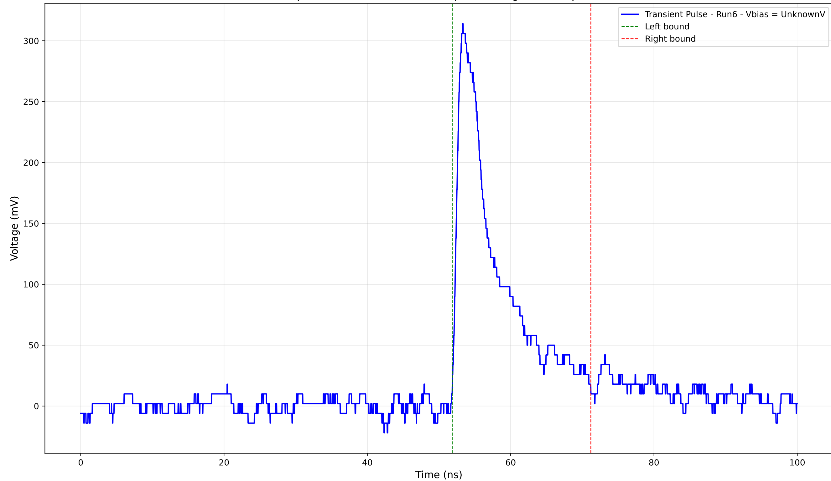
Transient Pulse - Sample: 4004 - Position: 720.0 \mu\text{m} - Charge: 39.39 pC - Rise Time: 1.09 ns
