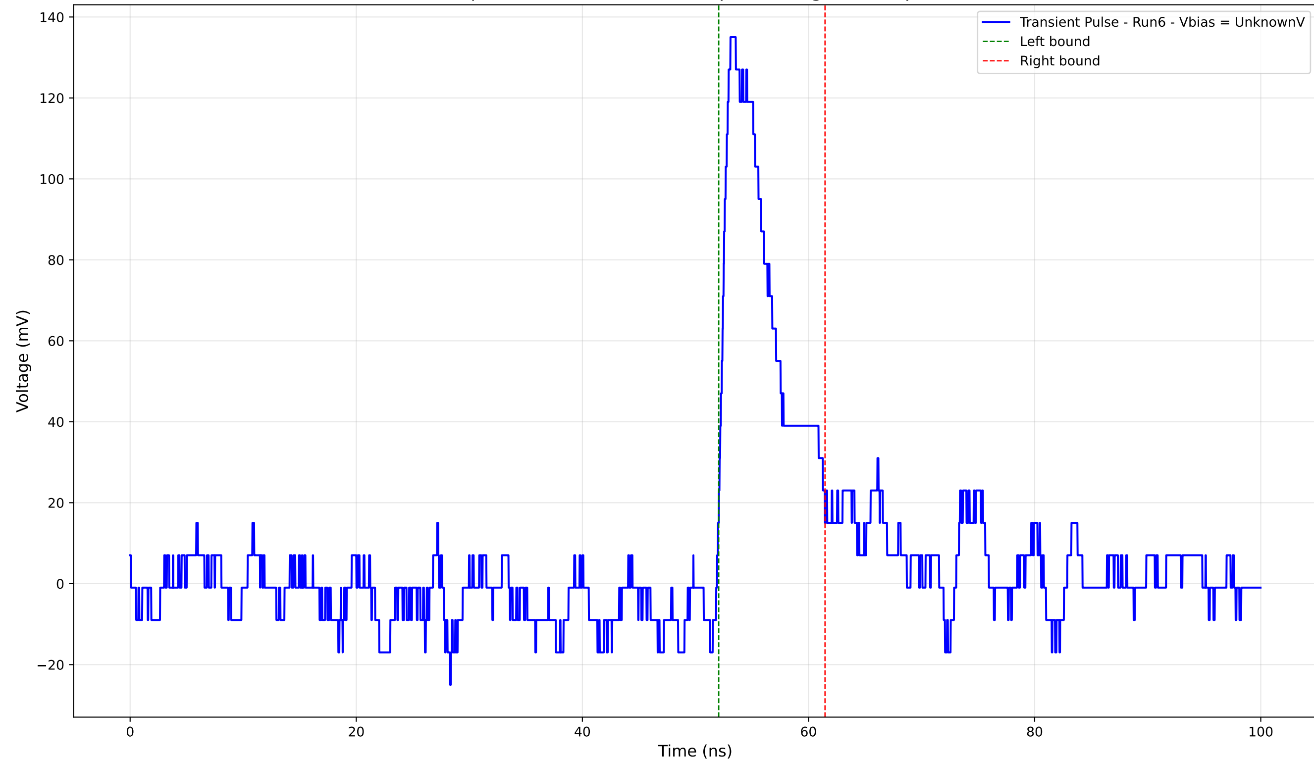
Transient Pulse - Sample: 4004 - Position: 800.0 \mu\text{m} - Charge: 13.56 pC - Rise Time: 0.94 ns
