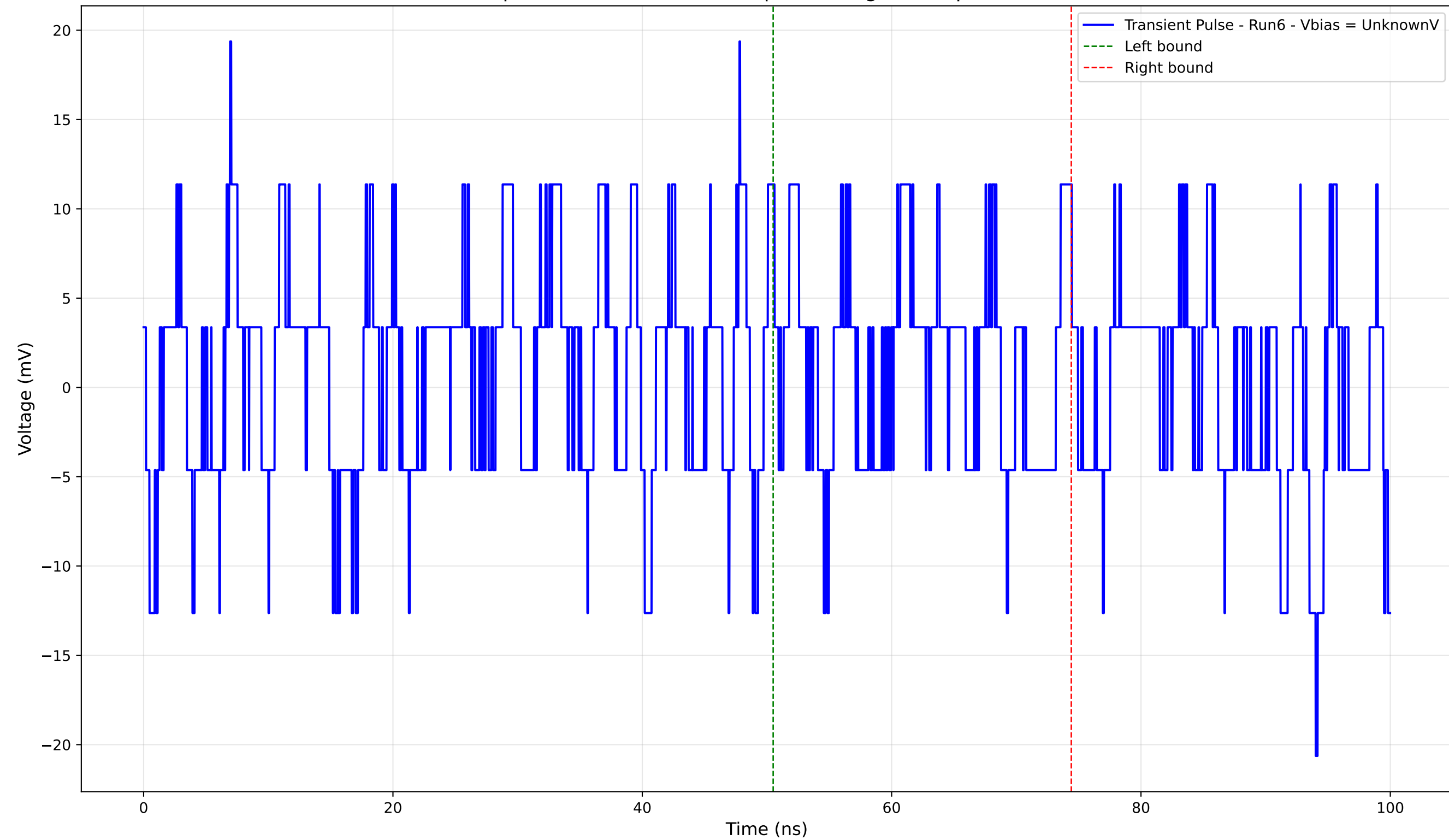
Transient Pulse - Sample: 4004 - Position: 40.0 \mu\text{m} - Charge: 0.73 pC - Rise Time: 0.00 ns (N/A)
