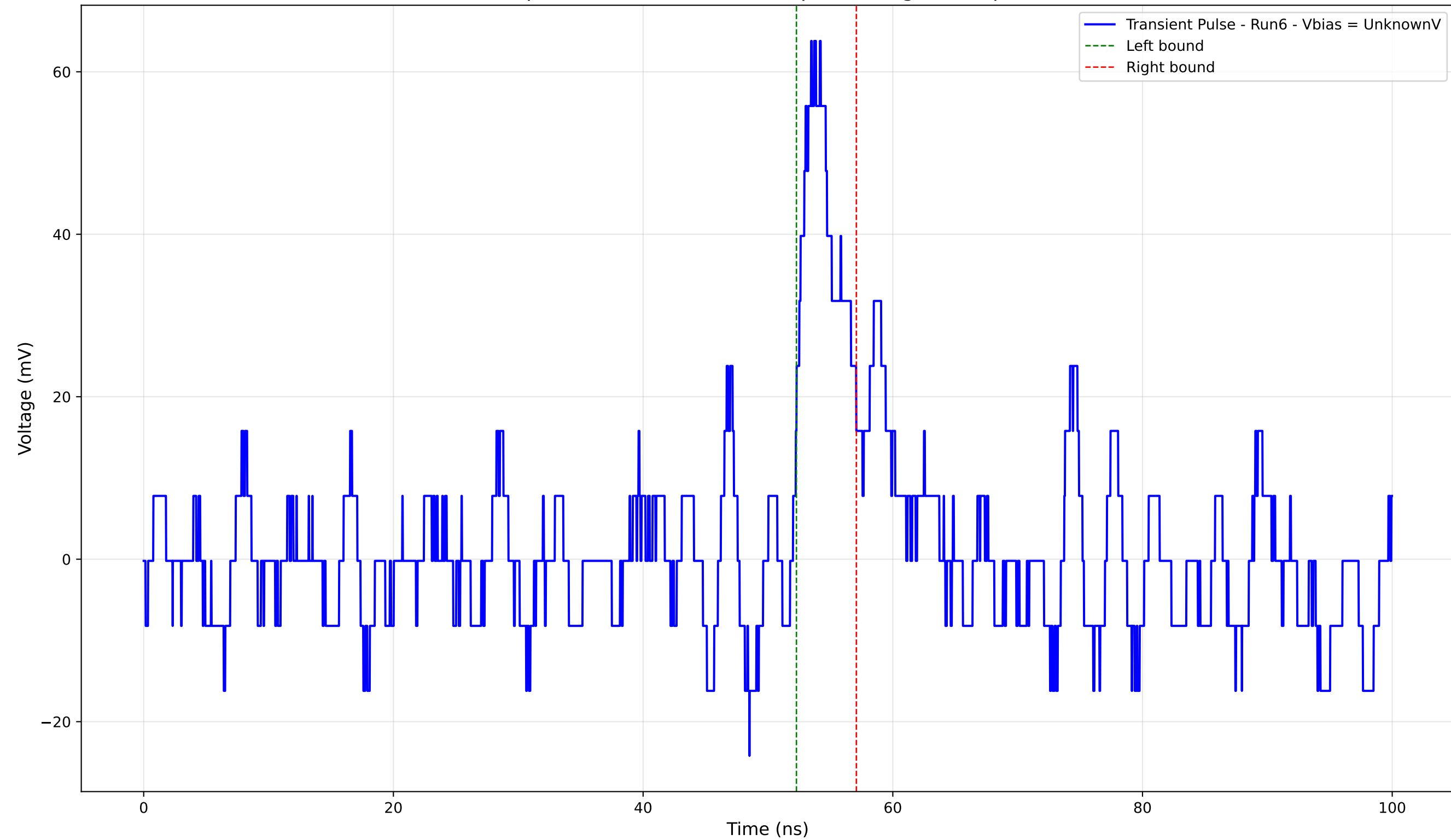
Transient Pulse - Sample: 4004 - Position: 880.0 \mu\text{m} - Charge: 3.93 pC - Rise Time: 1.44 ns
