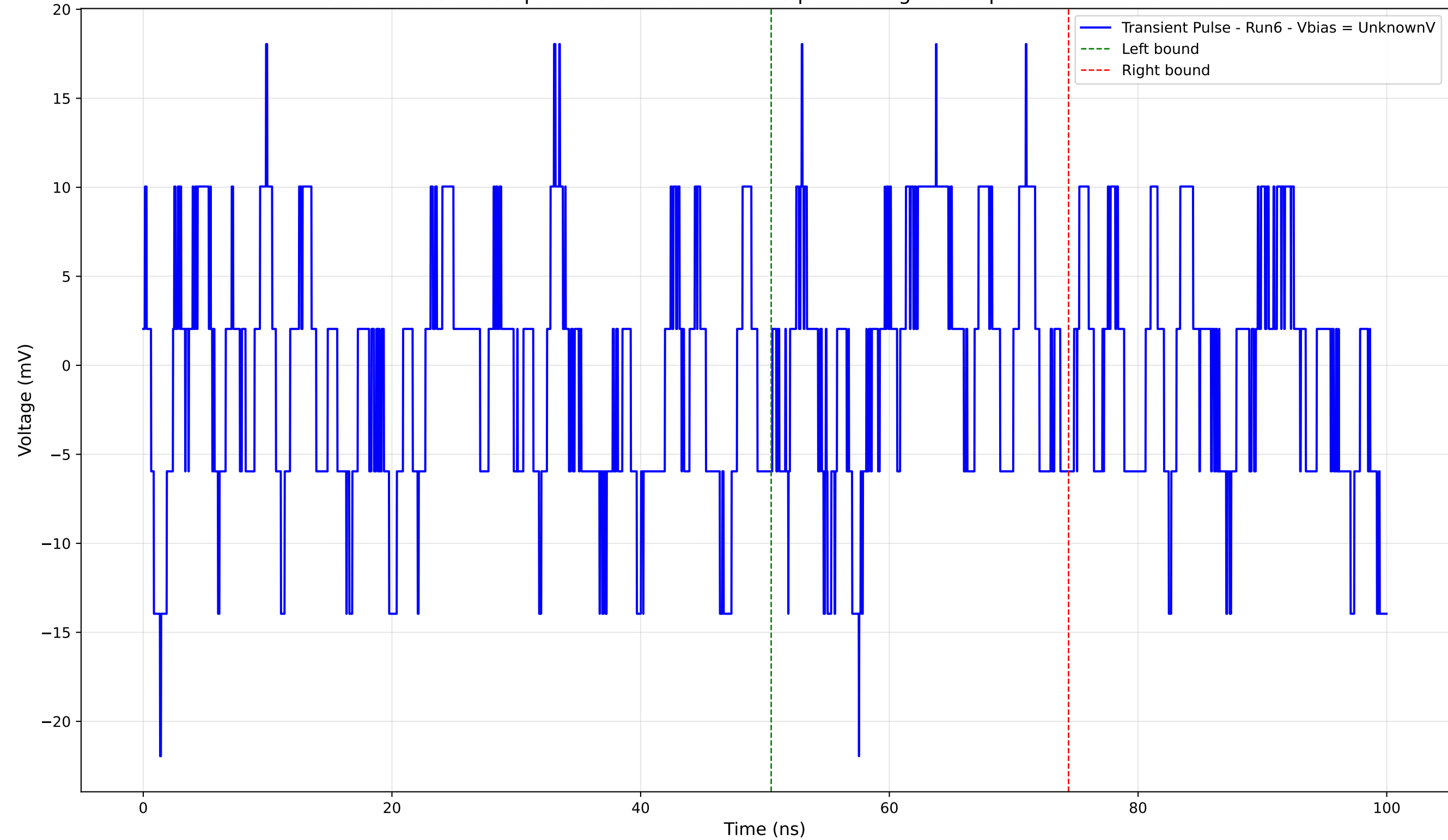
Transient Pulse - Sample: 4004 - Position: 345.0 \mu\text{m} - Charge: 0.56 pC - Rise Time: 0.74 ns
