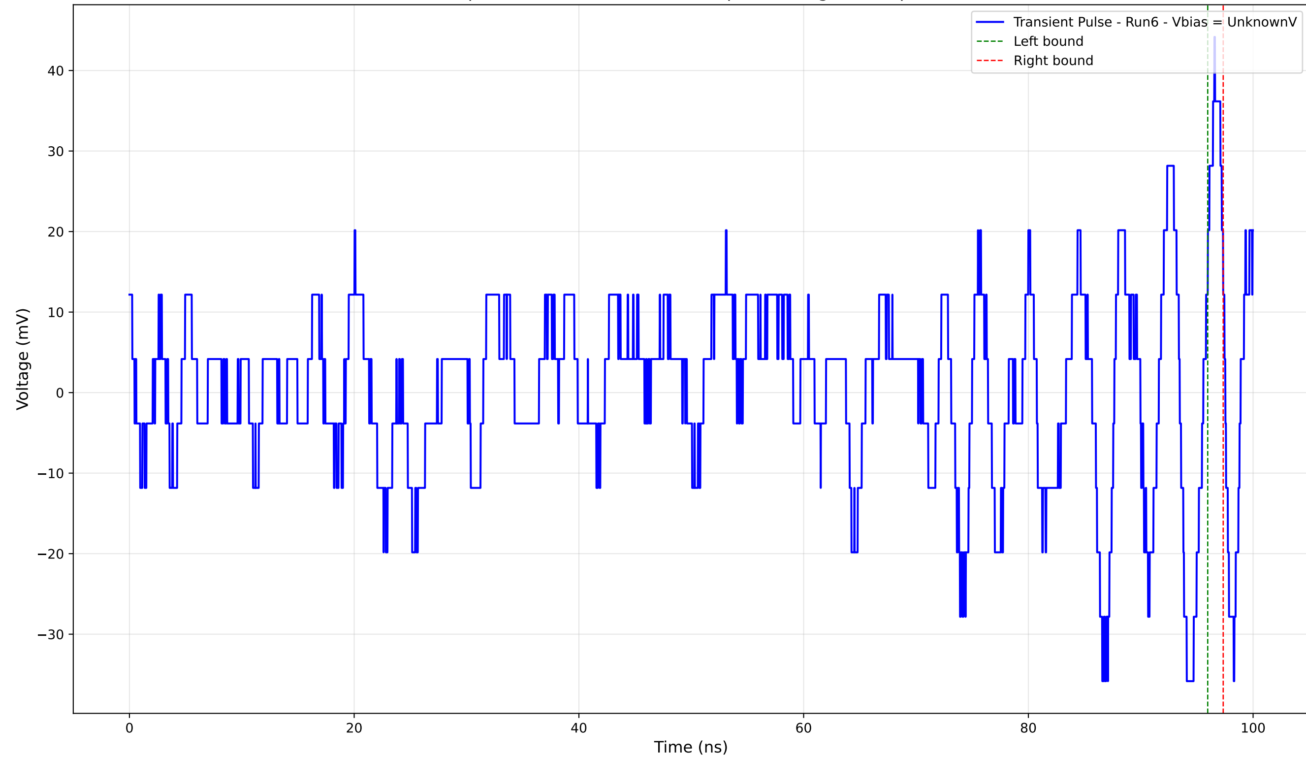
Transient Pulse - Sample: 4004 - Position: 1185.0 \mu\text{m} - Charge: 0.84 pC - Rise Time: 0.76 ns
