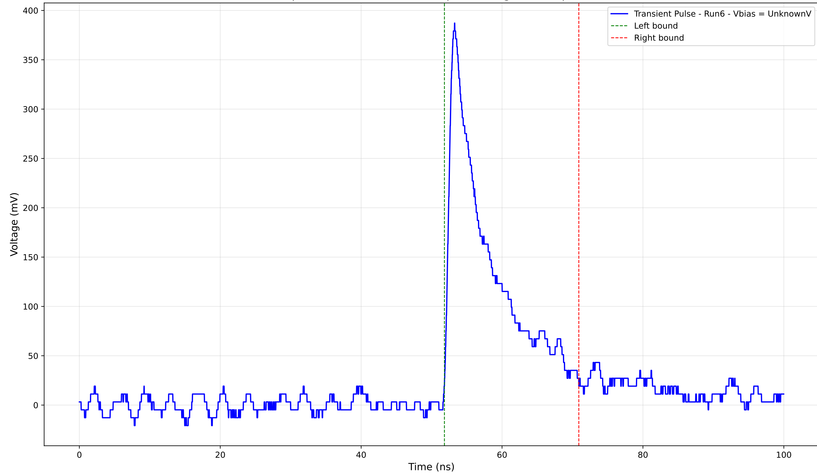
Transient Pulse - Sample: 4004 - Position: 625.0 \mu\text{m} - Charge: 49.84 pC - Rise Time: 1.03 ns
