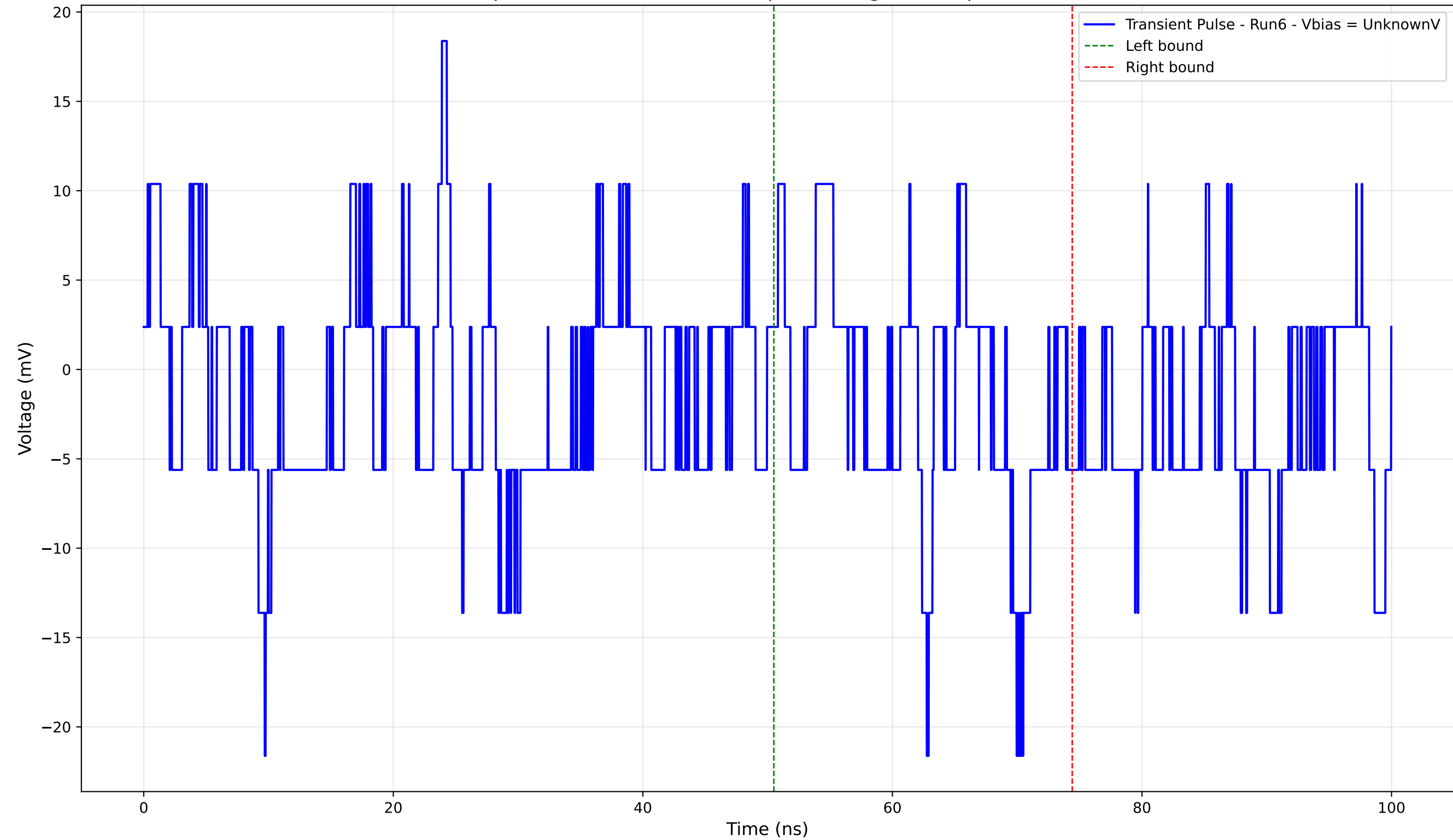
Transient Pulse - Sample: 4004 - Position: 150.0 \mu\text{m} - Charge: -0.67 pC - Rise Time: 0.00 ns (N/A)
