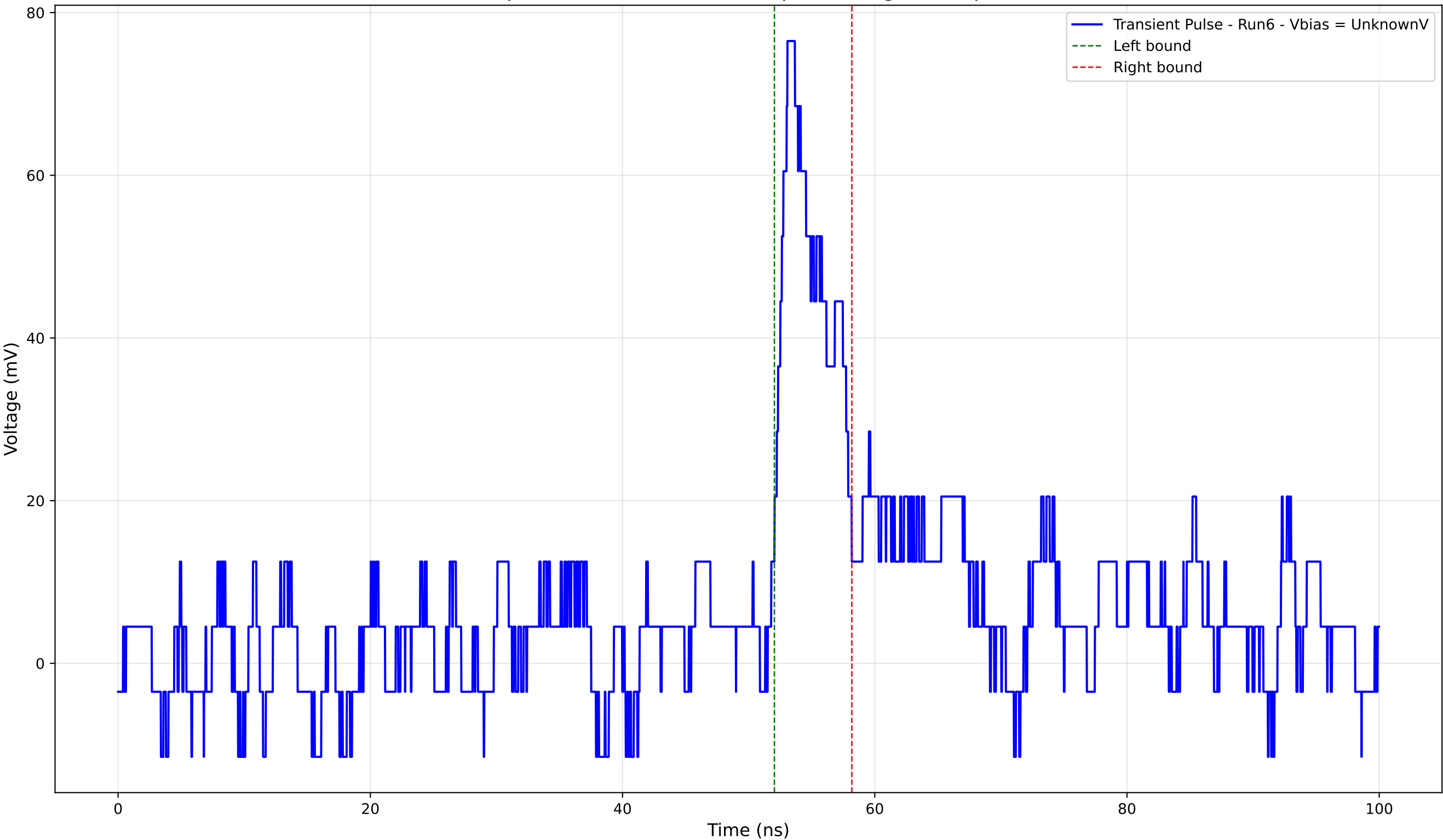
Transient Pulse - Sample: 4004 - Position: 890.0 \mu\text{m} - Charge: 5.98 pC - Rise Time: 1.29 ns
