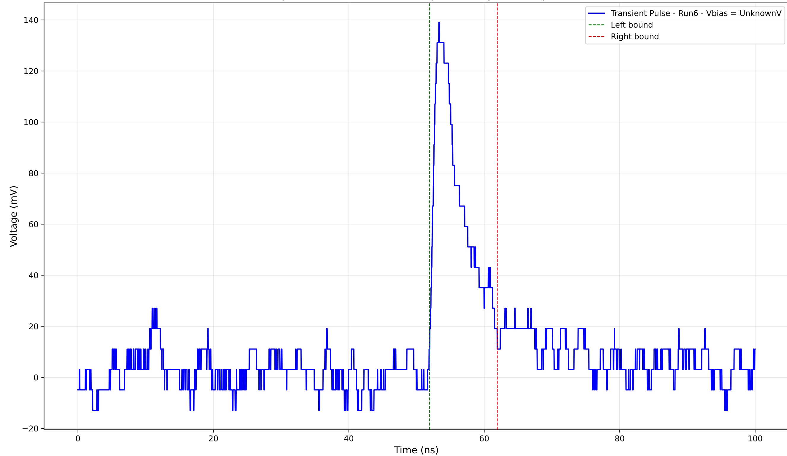
Transient Pulse - Sample: 4004 - Position: 805.0 \mu\text{m} - Charge: 13.66 pC - Rise Time: 1.09 ns
