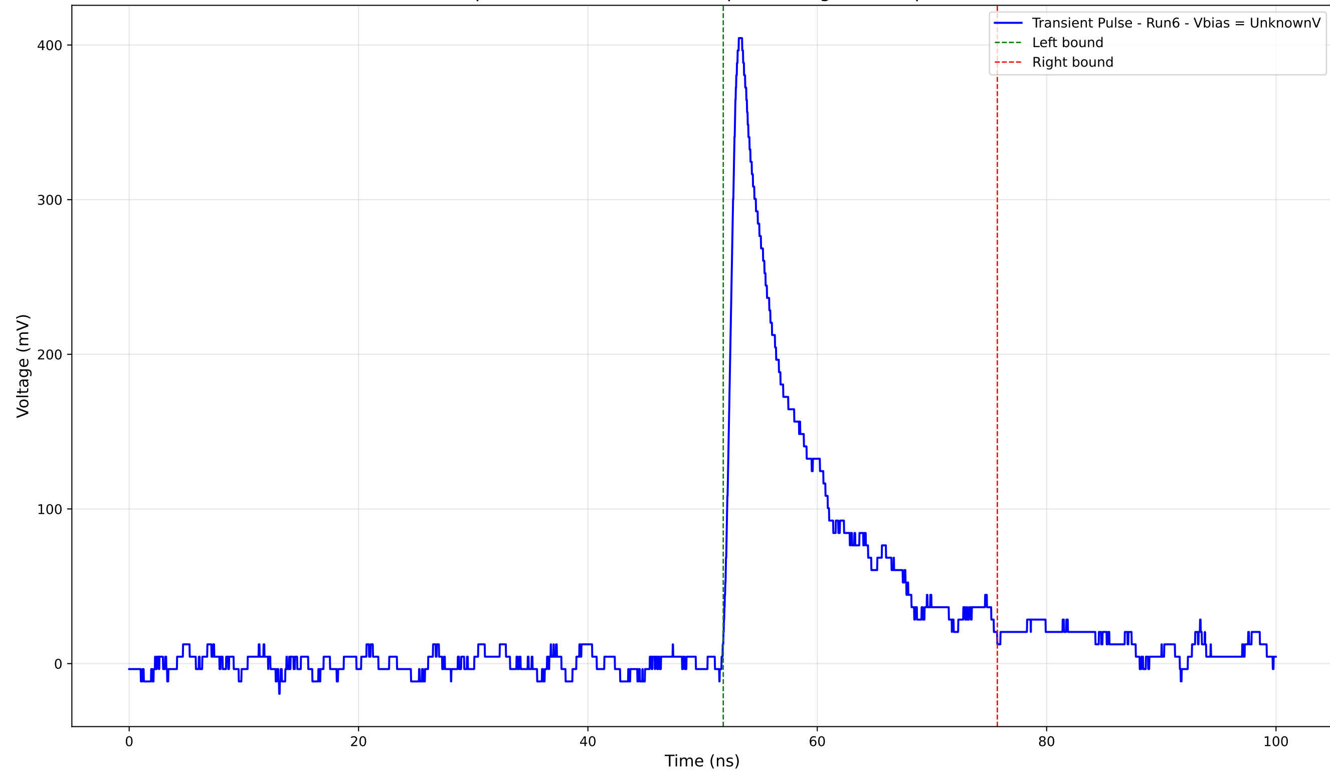
Transient Pulse - Sample: 4004 - Position: 640.0 \mu\text{m} - Charge: 54.48 pC - Rise Time: 0.93 ns
