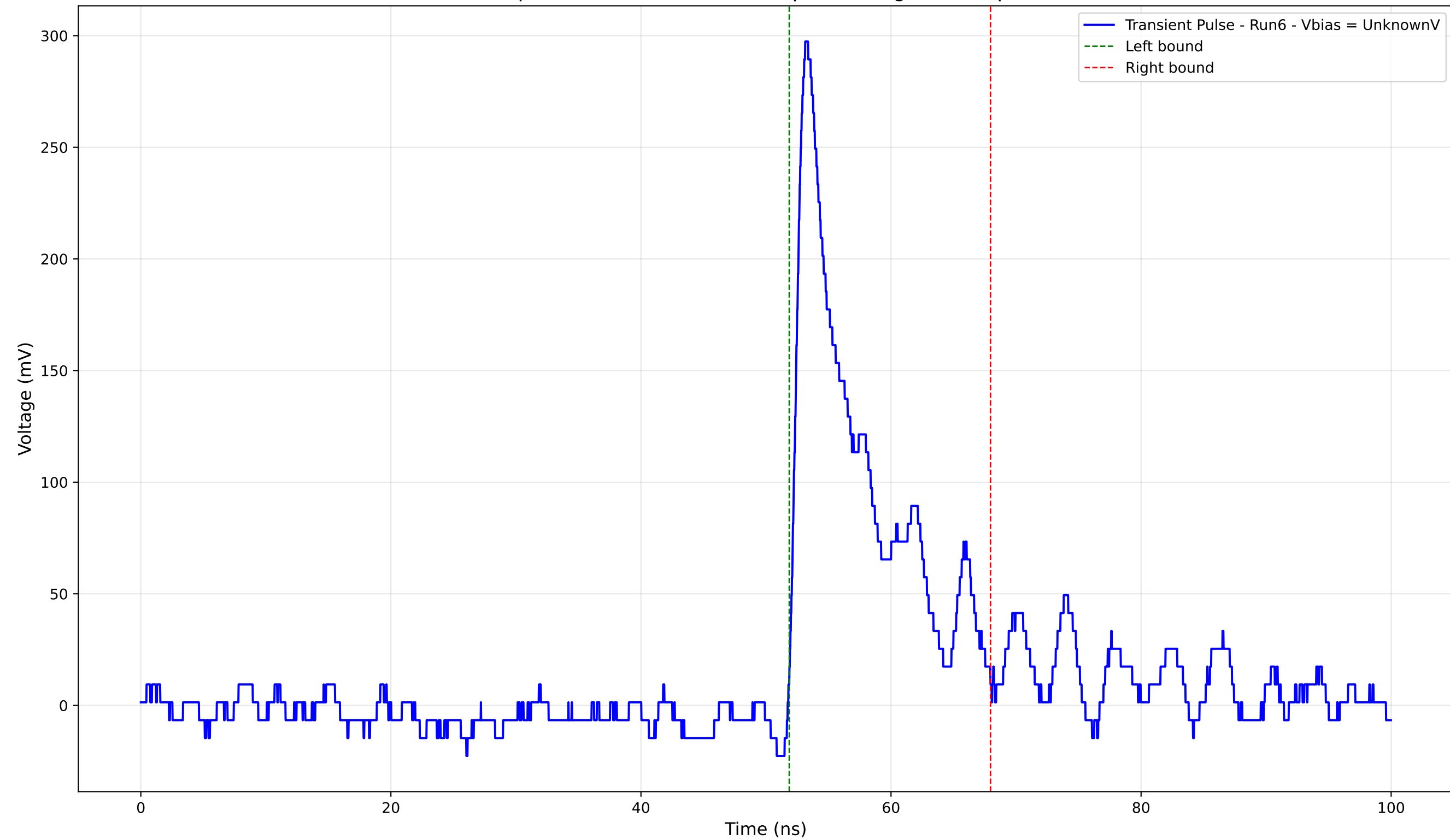
Transient Pulse - Sample: 4004 - Position: 525.0 \mu\text{m} - Charge: 32.86 pC - Rise Time: 0.97 ns
