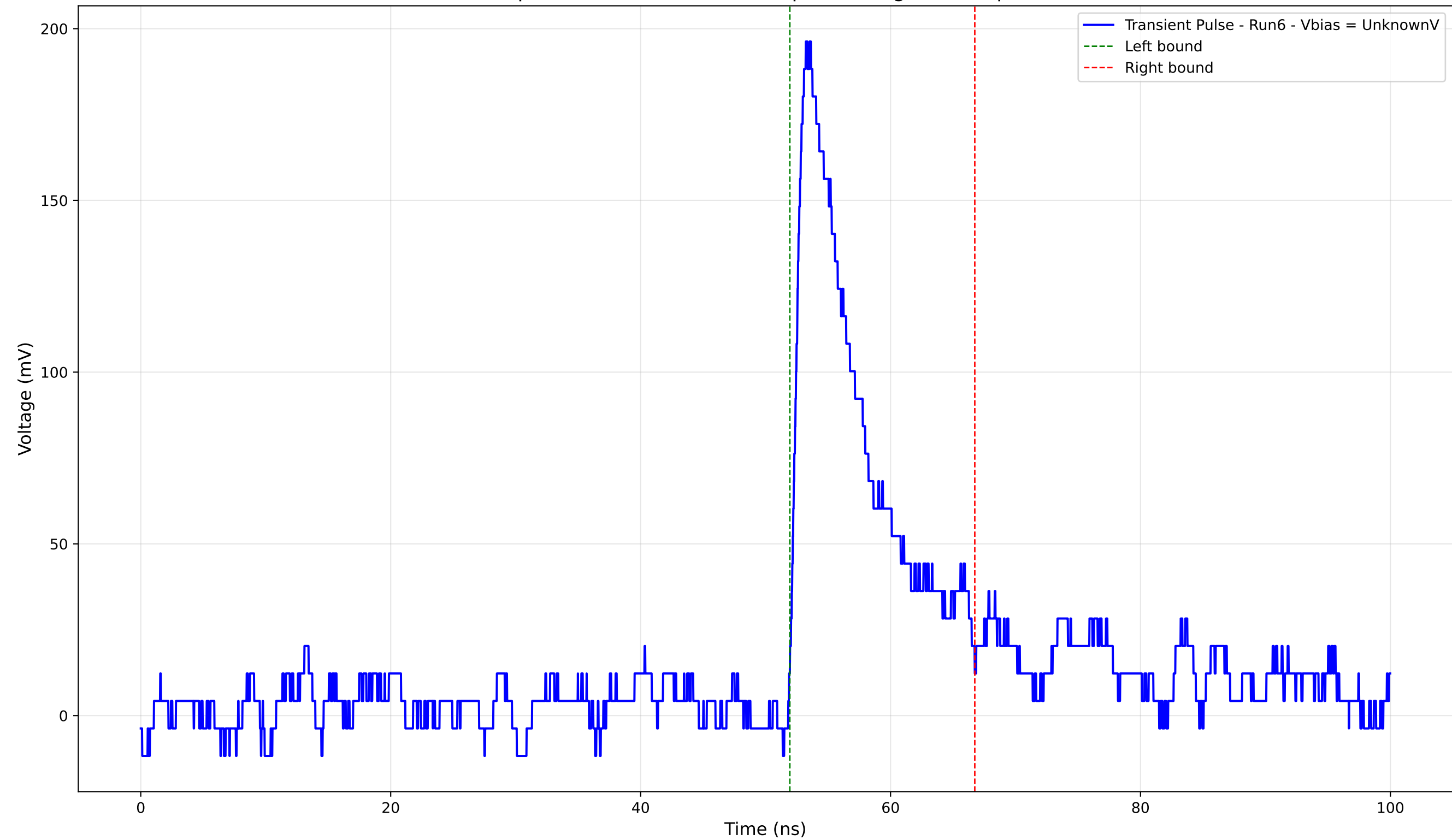
Transient Pulse - Sample: 4004 - Position: 770.0 \mu\text{m} - Charge: 23.78 pC - Rise Time: 1.02 ns
