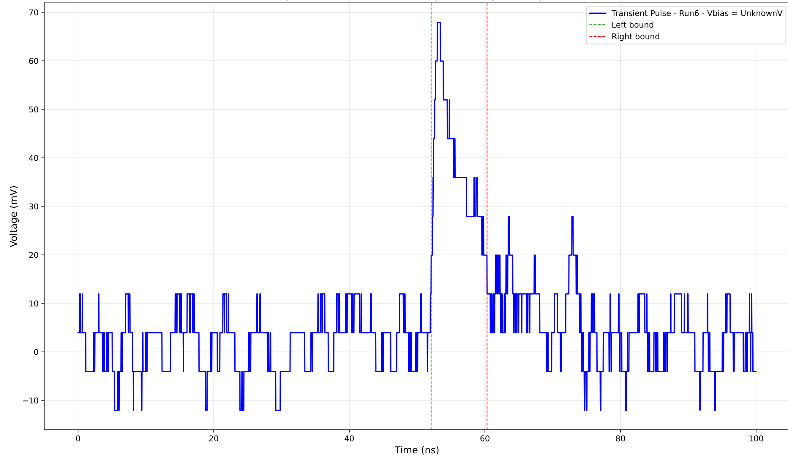
Transient Pulse - Sample: 4004 - Position: 945.0 \mu\text{m} - Charge: 6.38 pC - Rise Time: 1.03 ns
