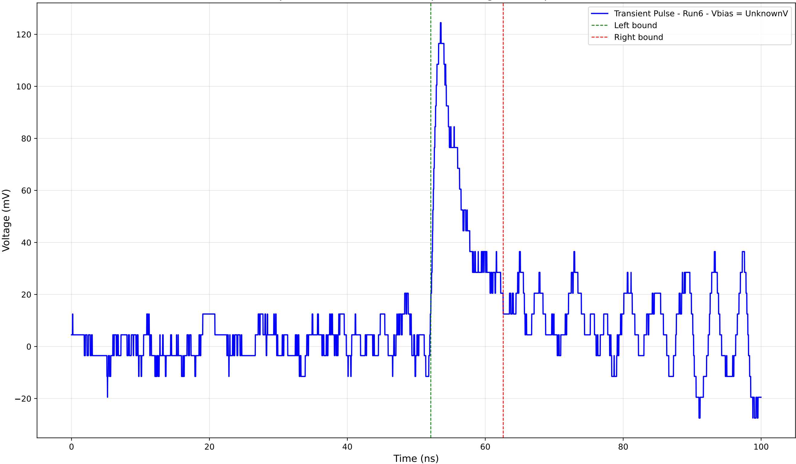
Transient Pulse - Sample: 4004 - Position: 820.0 \mu\text{m} - Charge: 11.53 pC - Rise Time: 1.20 ns
