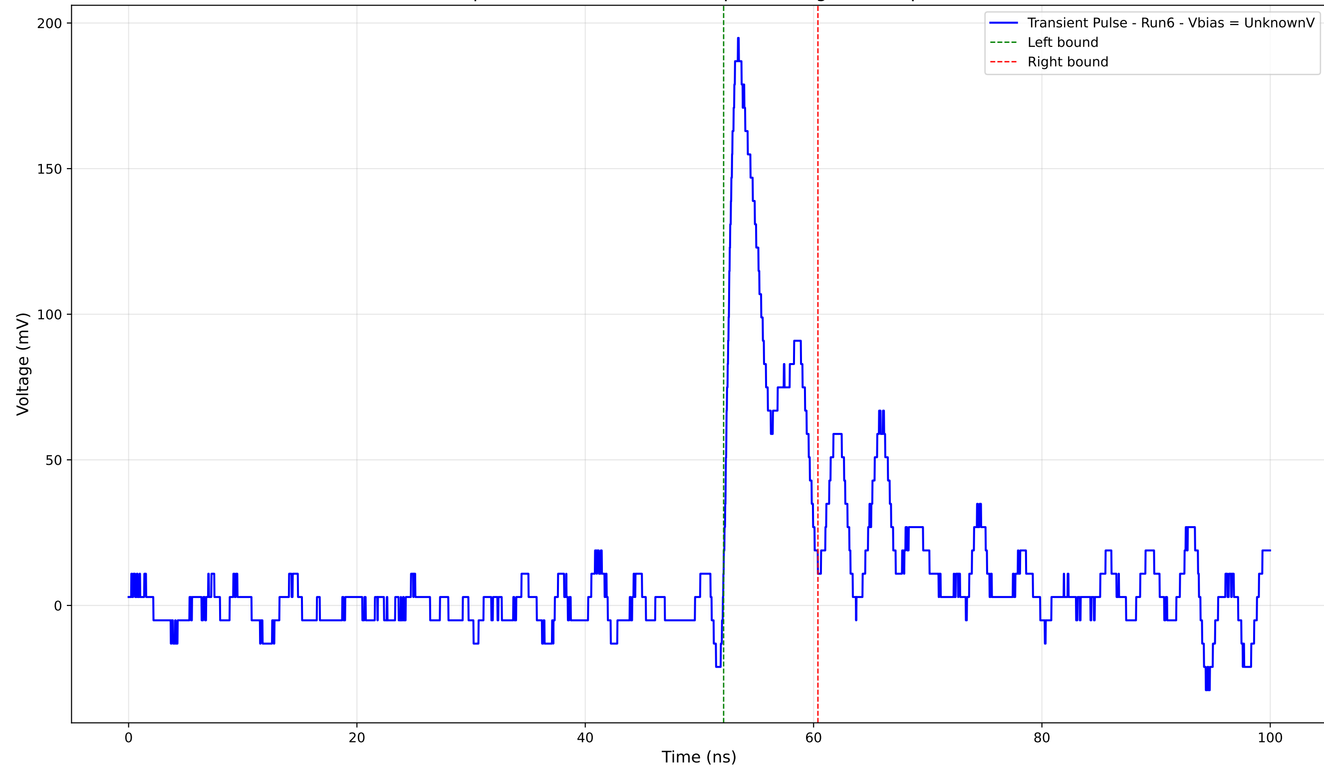
Transient Pulse - Sample: 4004 - Position: 515.0 \mu\text{m} - Charge: 16.16 pC - Rise Time: 0.88 ns
