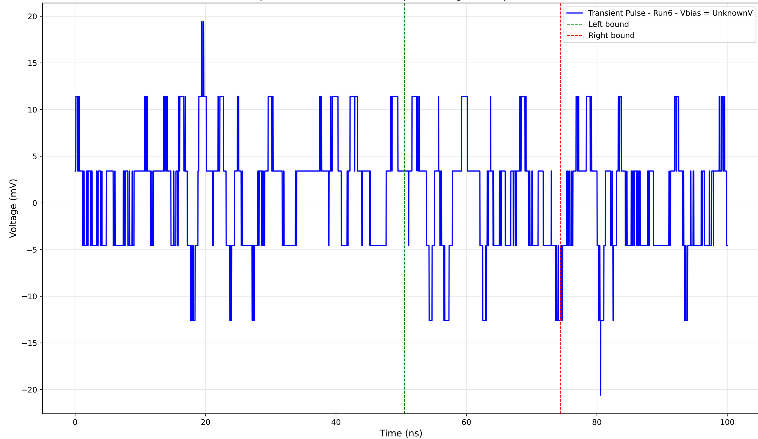
Transient Pulse - Sample: 4004 - Position: 350.0 \mu\text{m} - Charge: 0.08 pC - Rise Time: 0.00 ns (N/A)
