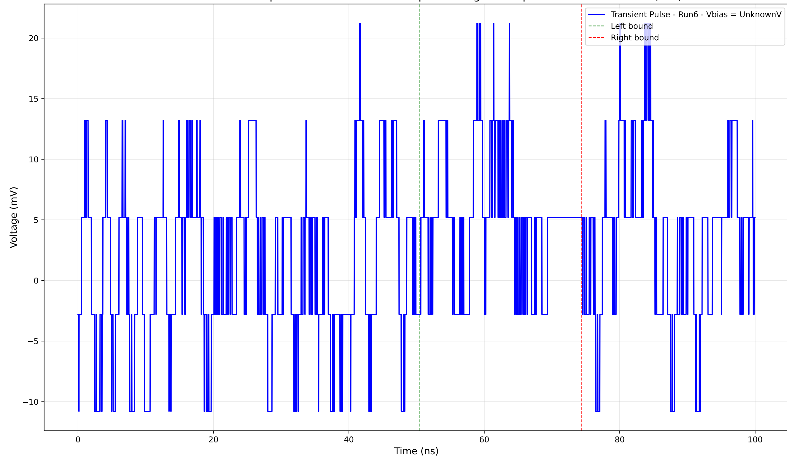
Transient Pulse - Sample: 4004 - Position: 300.0 \mu\text{m} - Charge: 2.55 pC - Rise Time: 0.00 ns (N/A)
