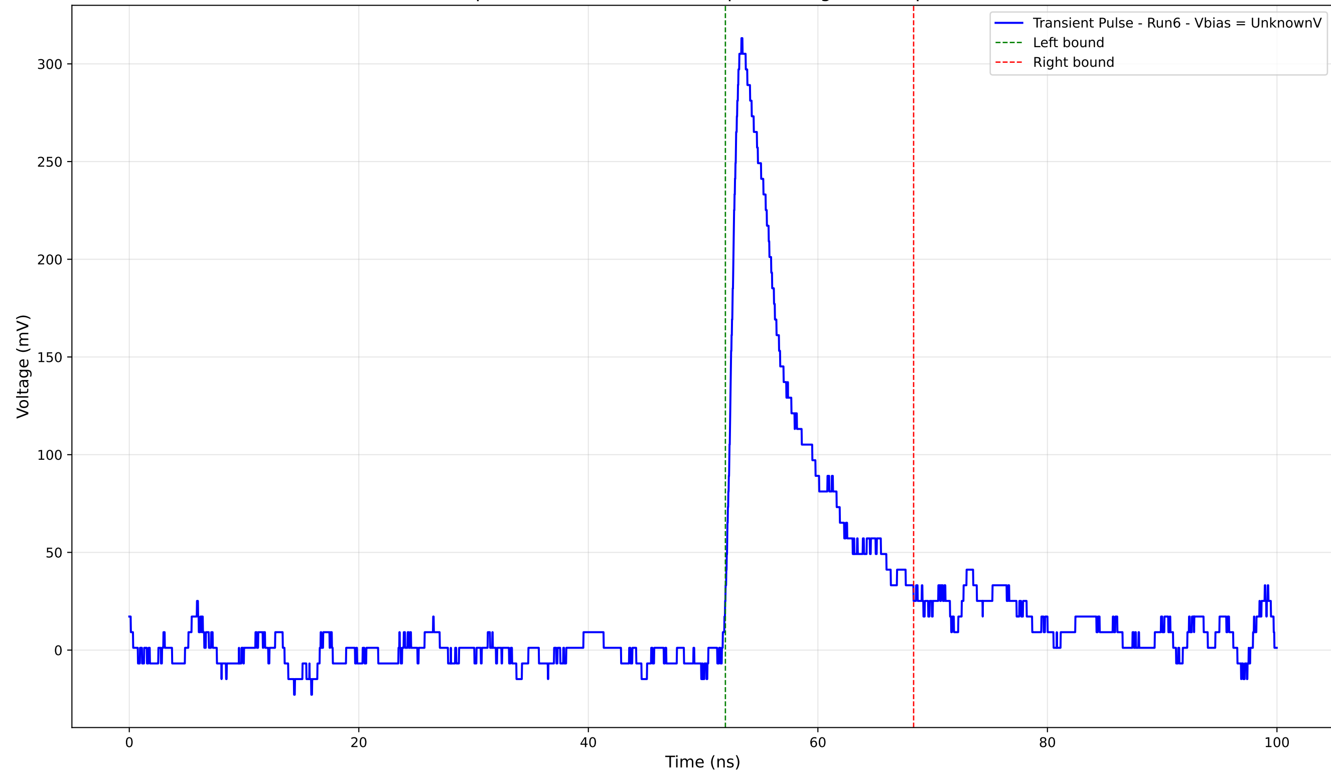
Transient Pulse - Sample: 4004 - Position: 685.0 \mu\text{m} - Charge: 38.42 pC - Rise Time: 1.08 ns
