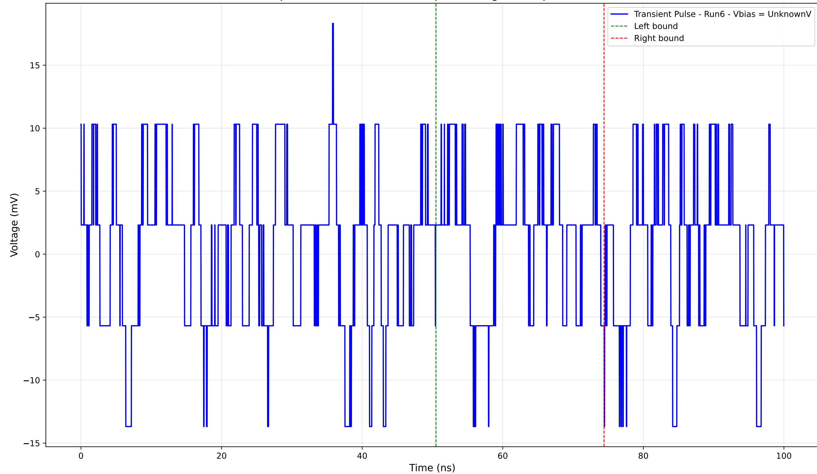
Transient Pulse - Sample: 4004 - Position: 100.0 \mu\text{m} - Charge: 0.92 pC - Rise Time: 0.00 ns (N/A)
