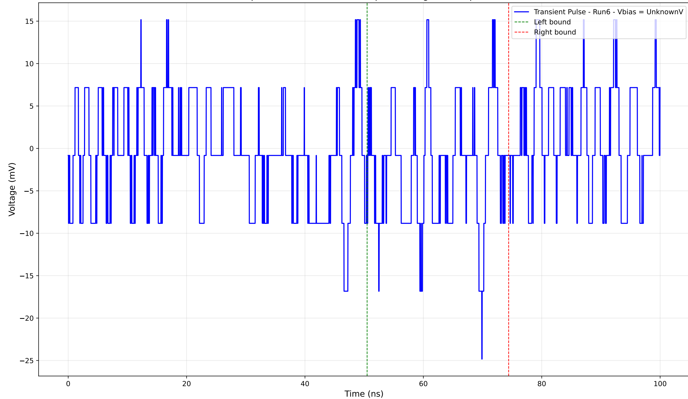
Transient Pulse - Sample: 4004 - Position: 70.0 \mu\text{m} - Charge: -1.08 pC - Rise Time: 0.82 ns
