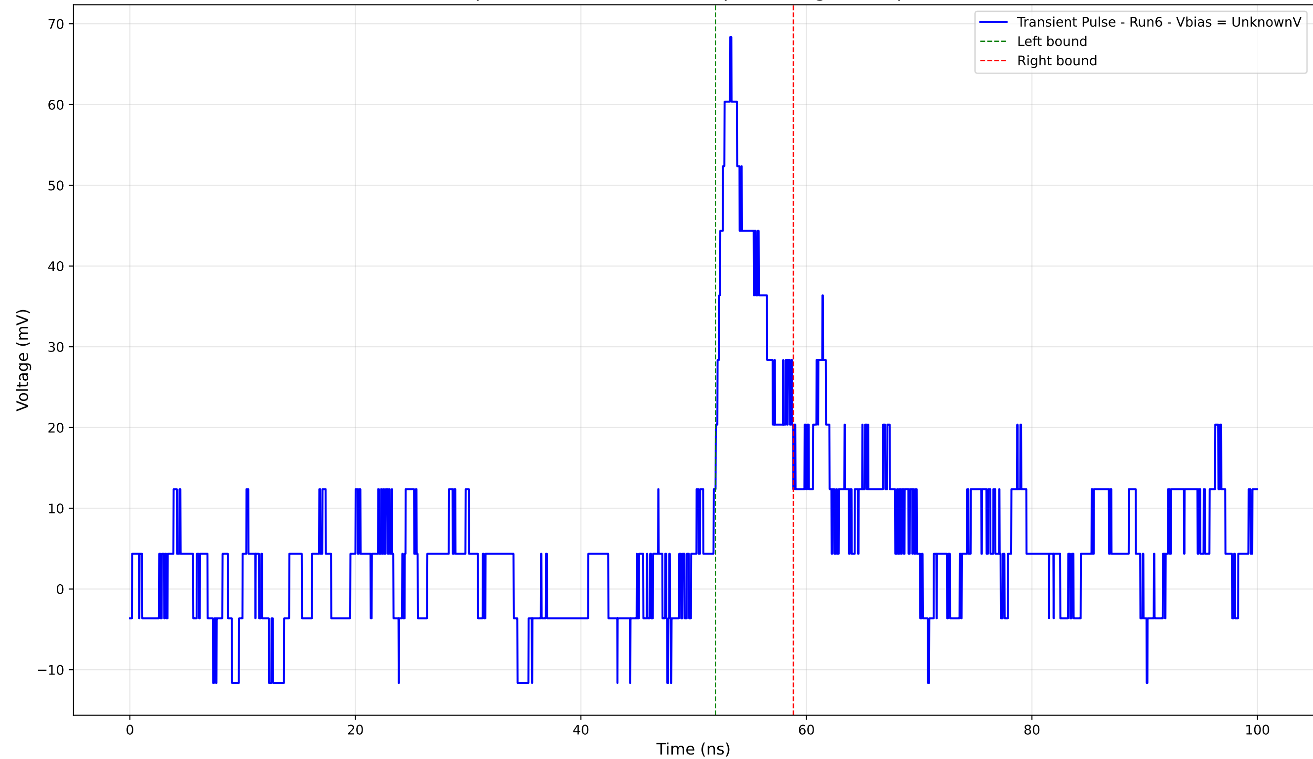
Transient Pulse - Sample: 4004 - Position: 895.0 \mu\text{m} - Charge: 5.30 pC - Rise Time: 1.47 ns
