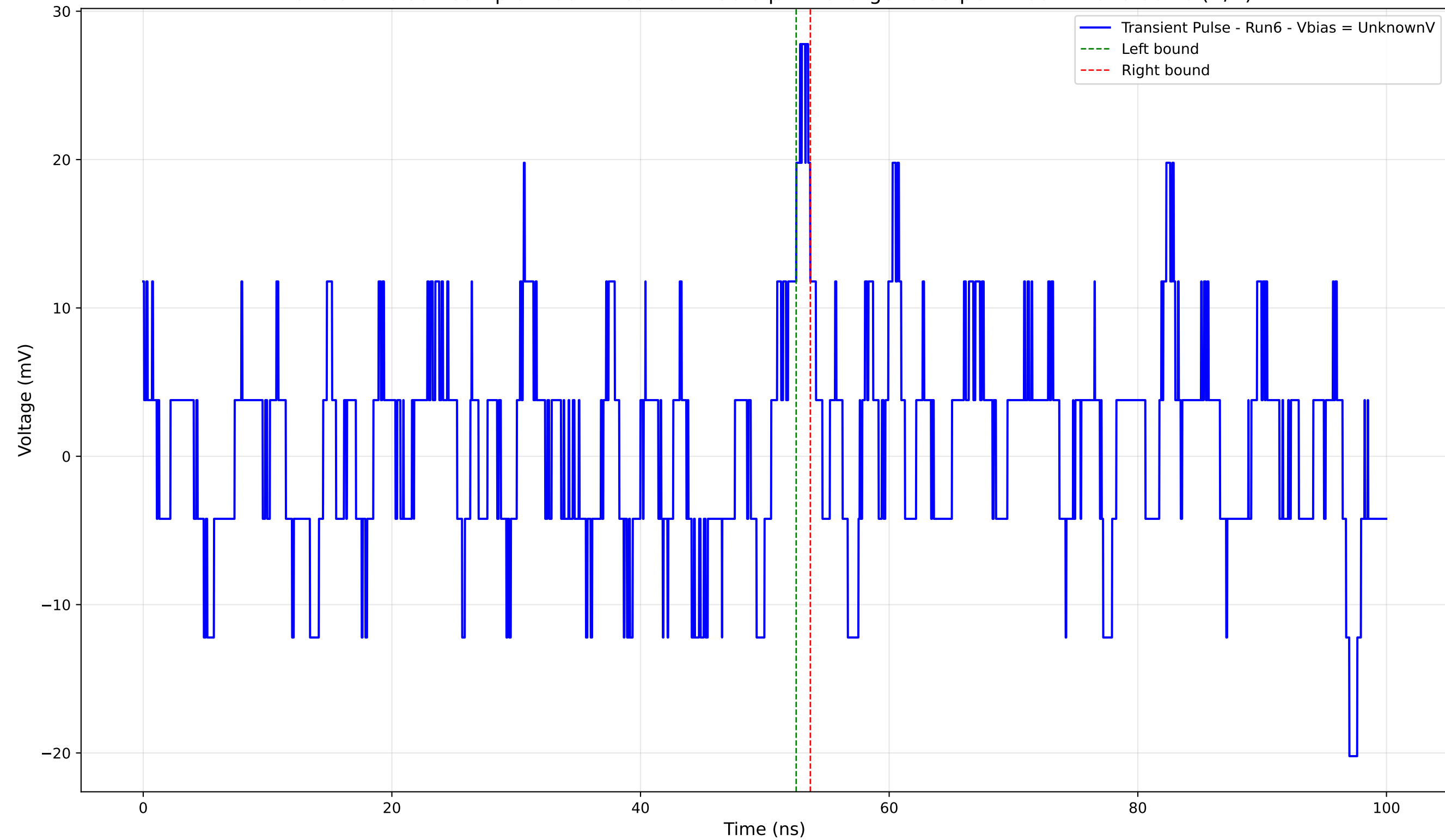
Transient Pulse - Sample: 4004 - Position: 430.0 \mu\text{m} - Charge: 0.53 pC - Rise Time: 0.00 ns (N/A)
