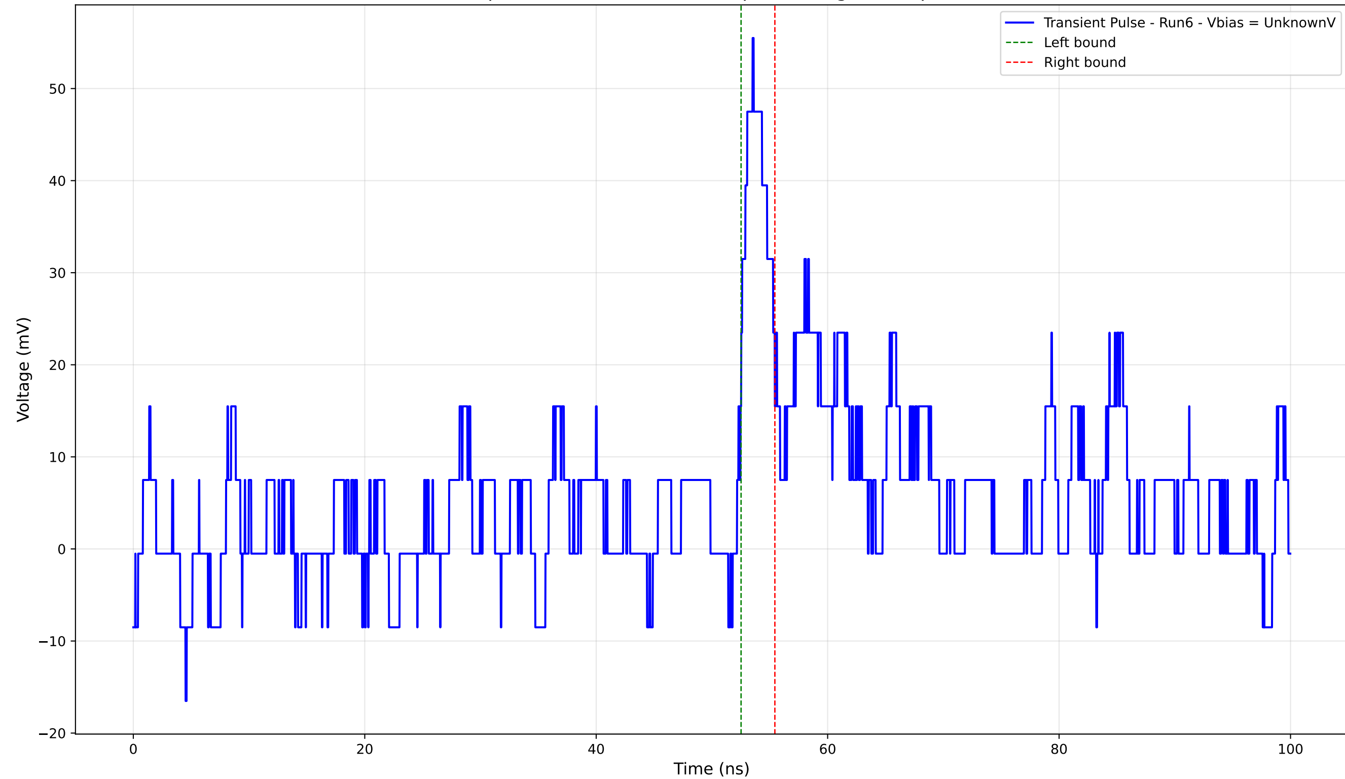
Transient Pulse - Sample: 4004 - Position: 870.0 \mu\text{m} - Charge: 2.32 pC - Rise Time: 1.35 ns
