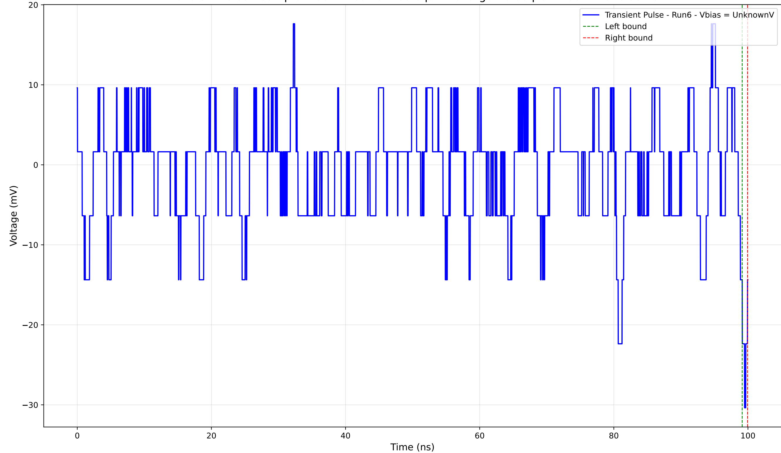
Transient Pulse - Sample: 4004 - Position: 60.0 \mu\text{m} - Charge: -0.38 pC - Rise Time: 0.95 ns
