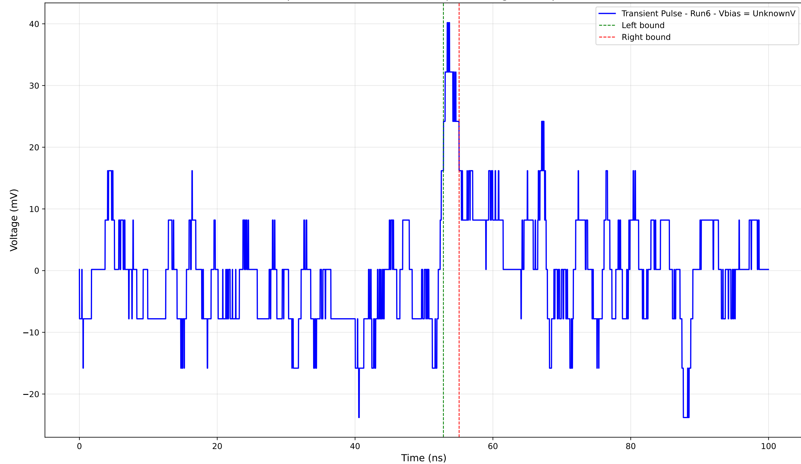
Transient Pulse - Sample: 4004 - Position: 1135.0 \mu\text{m} - Charge: 1.34 pC - Rise Time: 1.03 ns
