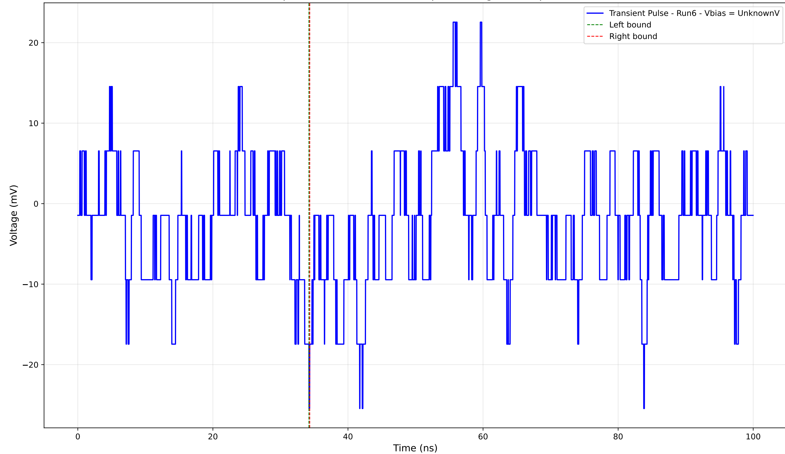
Transient Pulse - Sample: 4004 - Position: 465.0 \mu\text{m} - Charge: -0.06 pC - Rise Time: 1.44 ns
