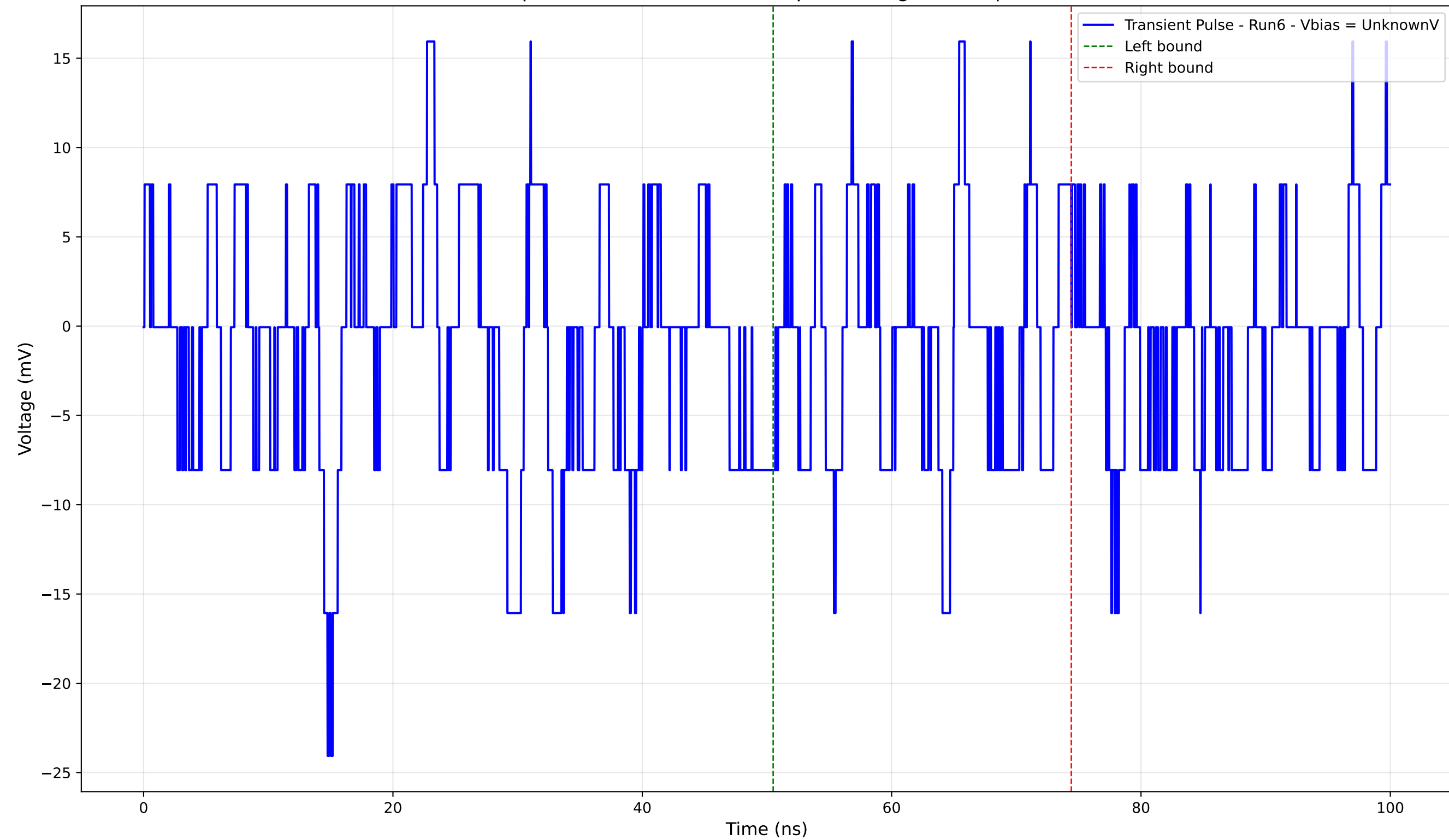
Transient Pulse - Sample: 4004 - Position: 185.0 \mu\text{m} - Charge: -0.46 pC - Rise Time: 0.67 ns
