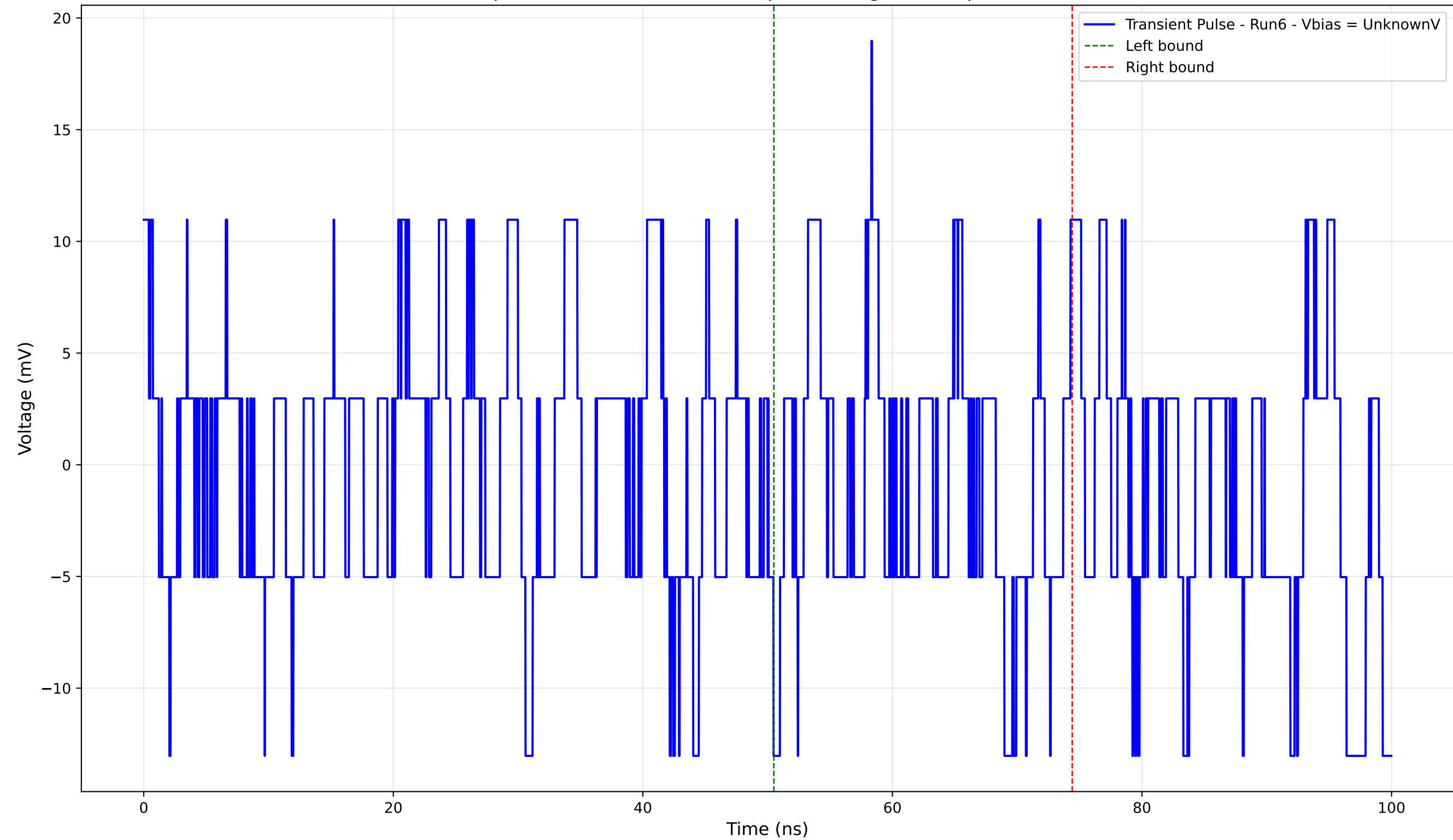
Transient Pulse - Sample: 4004 - Position: 335.0 \mu\text{m} - Charge: -0.34 pC - Rise Time: 0.00 ns (N/A)
