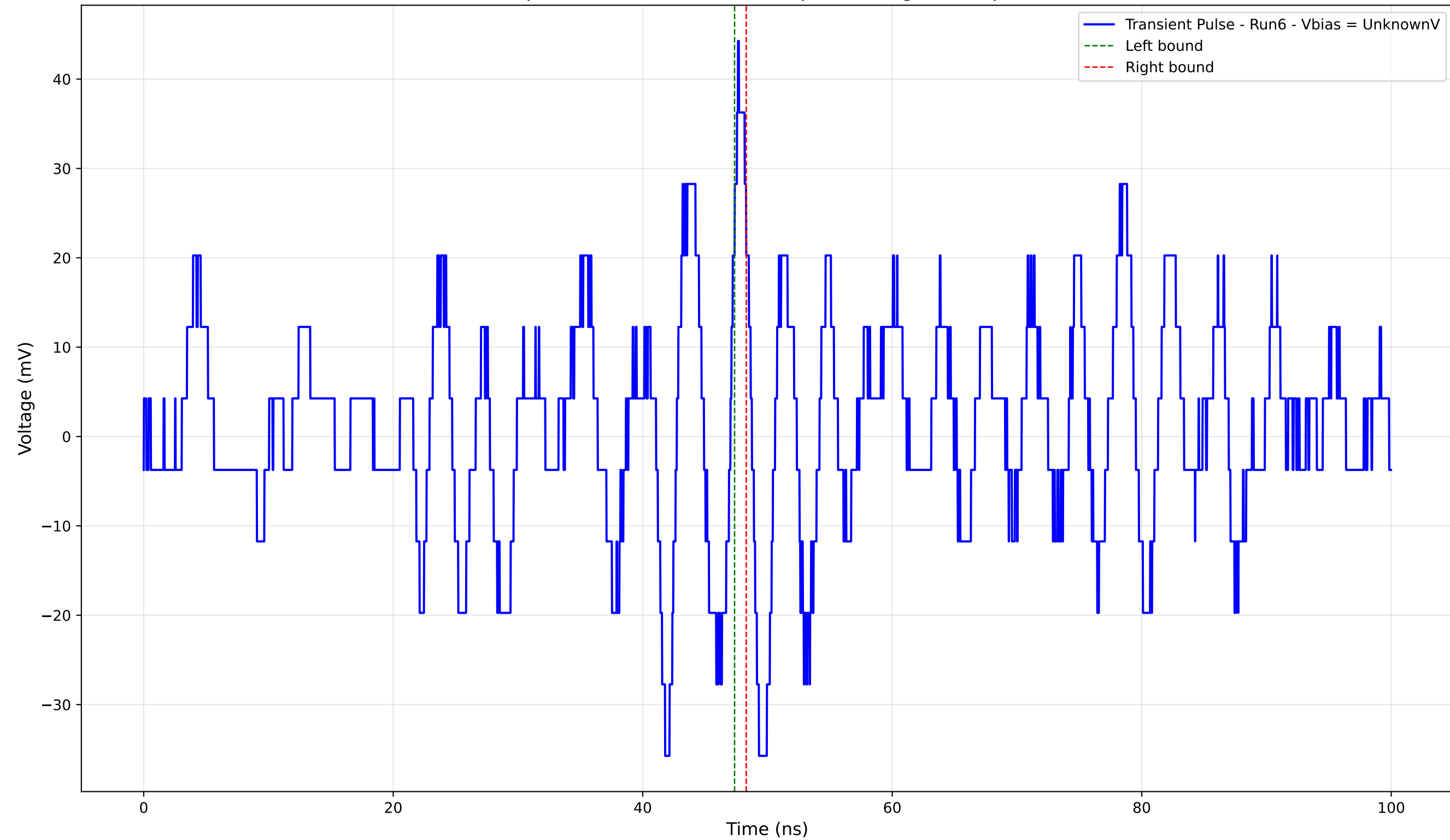
Transient Pulse - Sample: 4004 - Position: 135.0 \mu\text{m} - Charge: 0.64 pC - Rise Time: 0.54 ns
