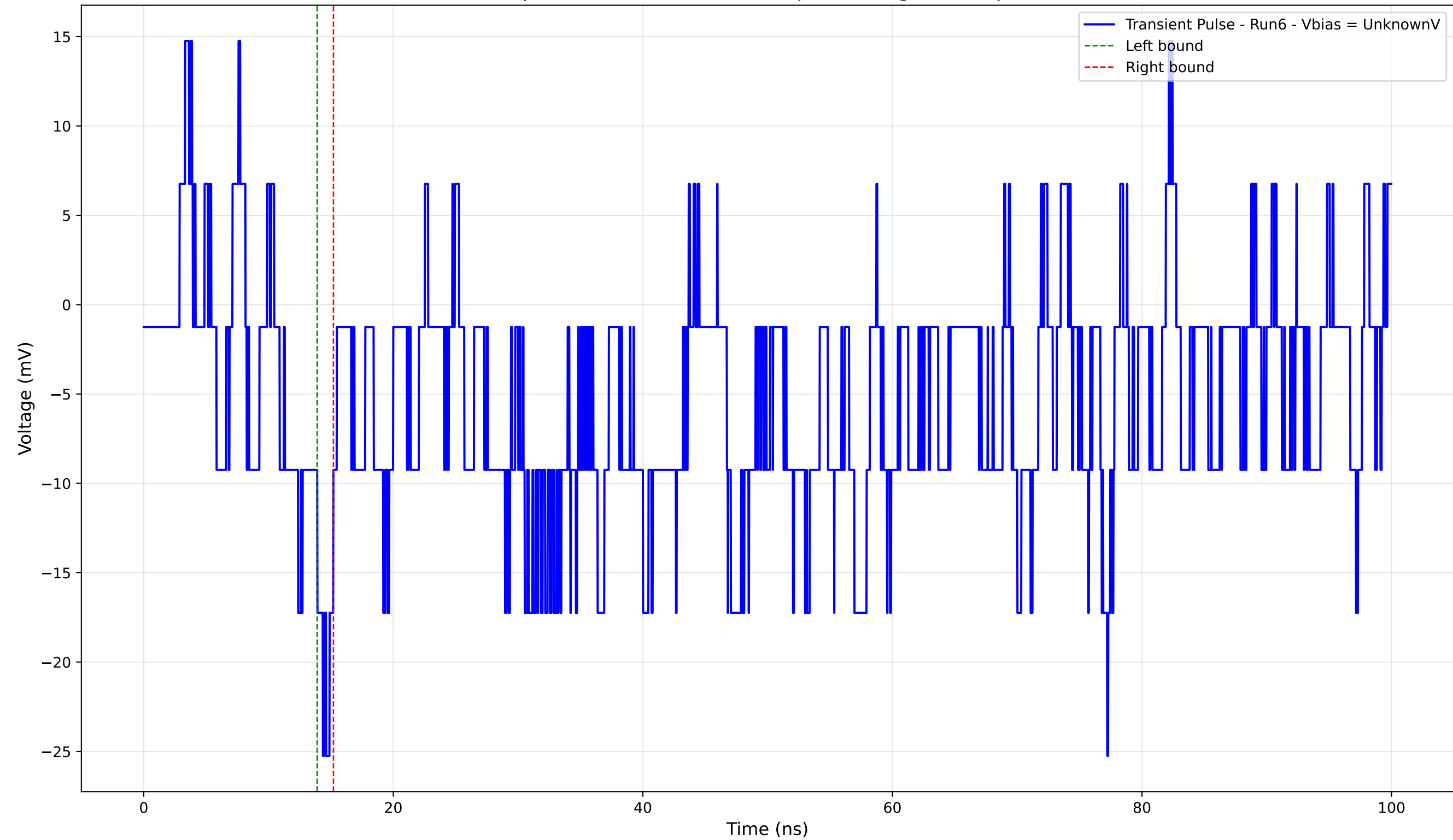
Transient Pulse - Sample: 4004 - Position: 110.0 \mu\text{m} - Charge: -0.51 pC - Rise Time: 3.06 ns
