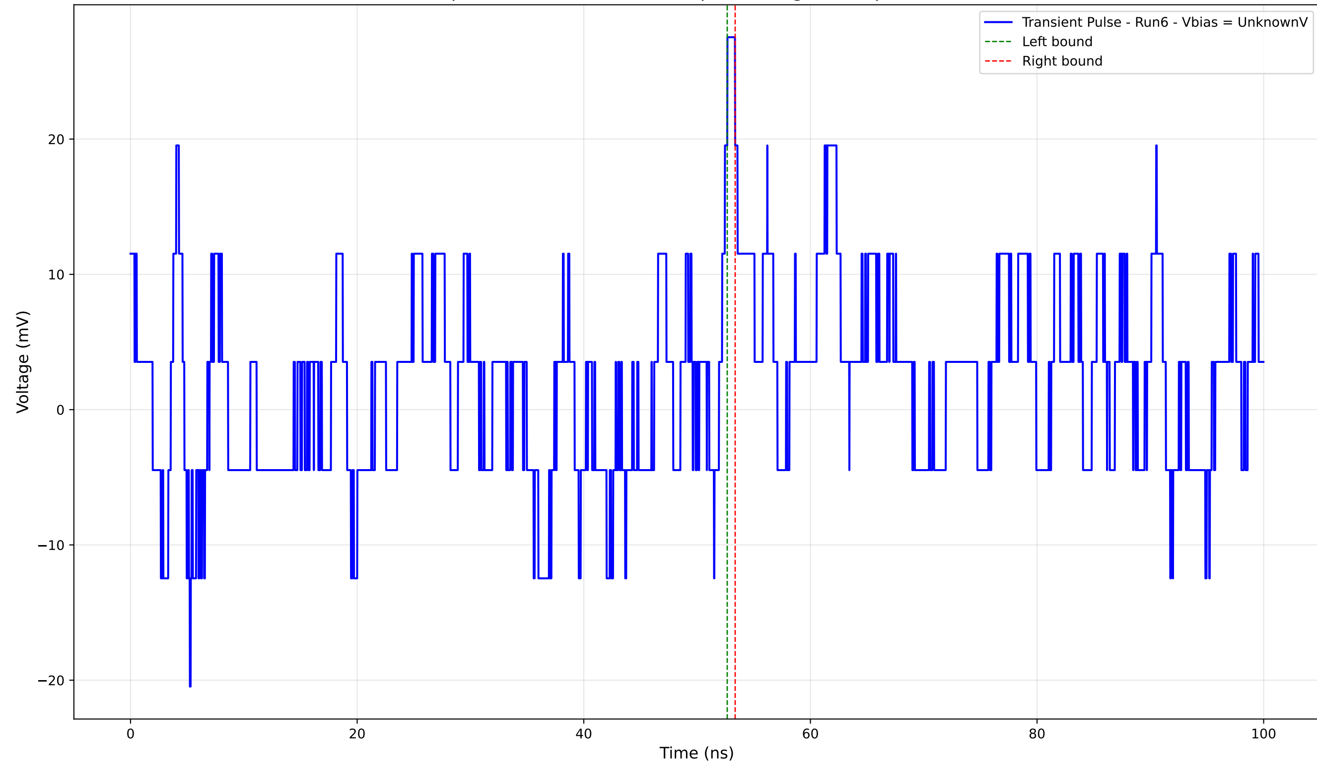
Transient Pulse - Sample: 4004 - Position: 450.0 \mu\text{m} - Charge: 0.38 pC - Rise Time: 0.00 ns (N/A)
