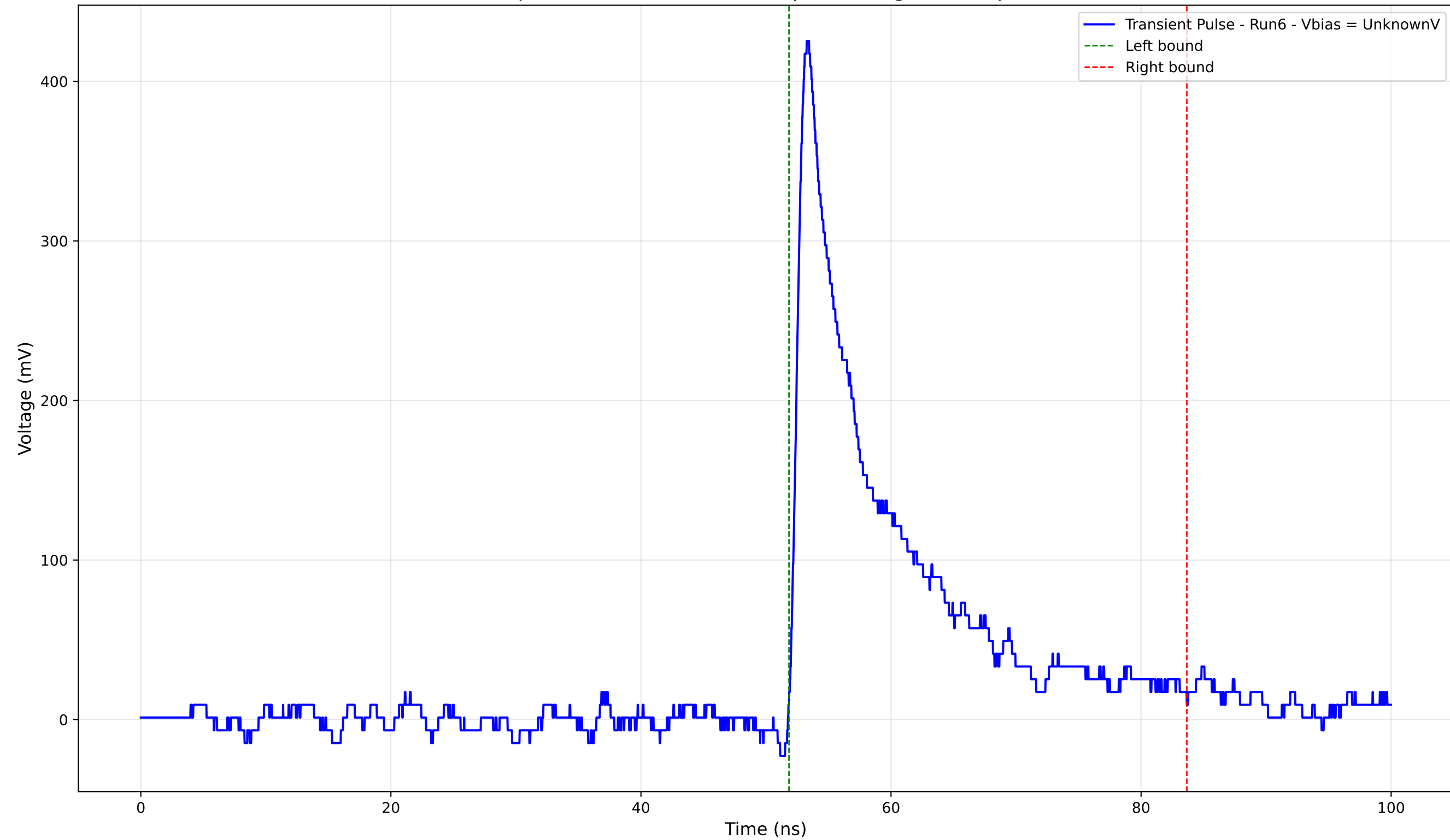
Transient Pulse - Sample: 4004 - Position: 595.0 \mu\text{m} - Charge: 59.84 pC - Rise Time: 0.94 ns
