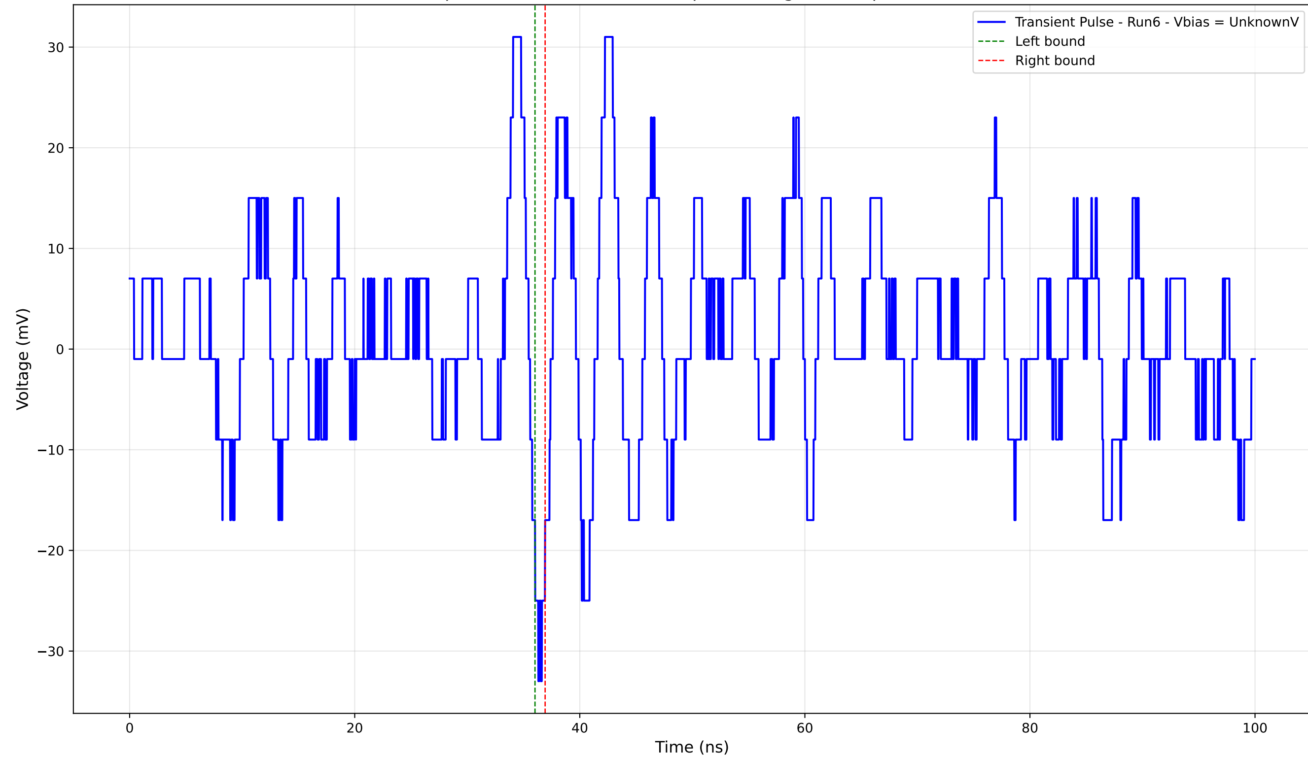
Transient Pulse - Sample: 4004 - Position: 280.0 \mu\text{m} - Charge: -0.48 pC - Rise Time: 0.00 ns (N/A)
