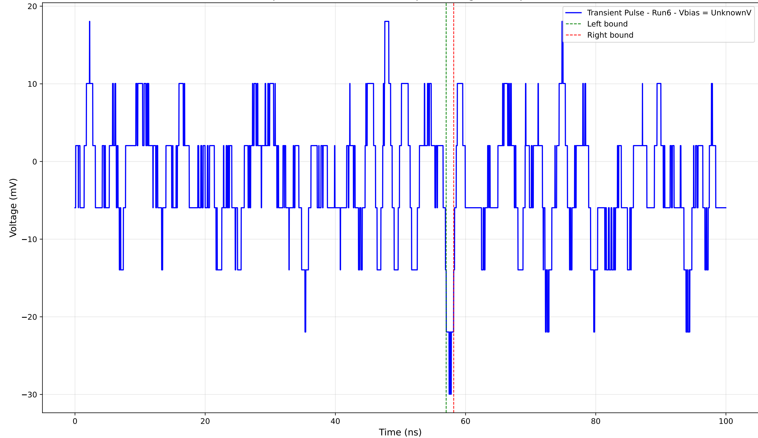
Transient Pulse - Sample: 4004 - Position: 170.0 \mu\text{m} - Charge: -0.55 pC - Rise Time: 0.94 ns
