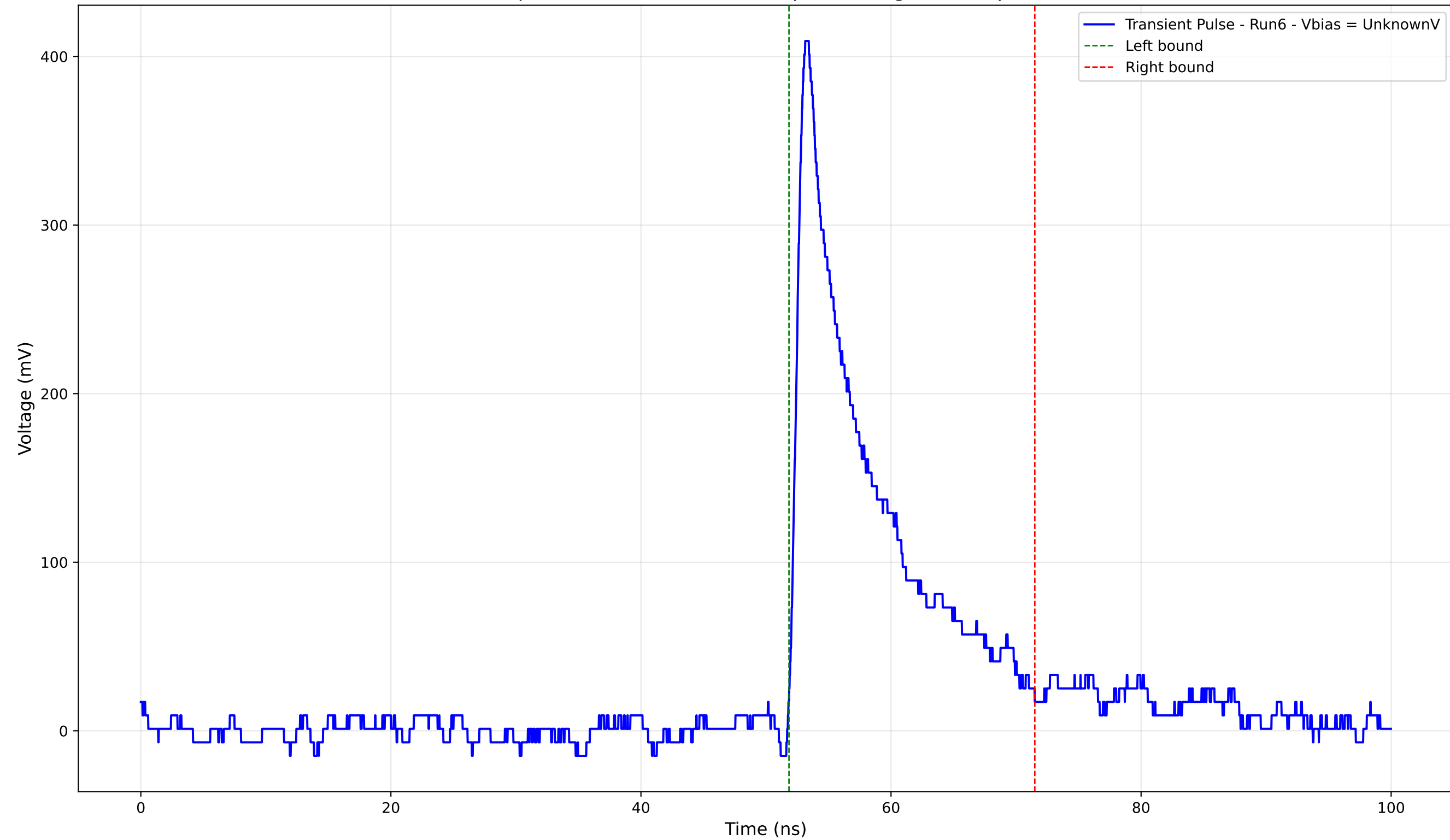
Transient Pulse - Sample: 4004 - Position: 610.0 \mu\text{m} - Charge: 51.71 pC - Rise Time: 0.94 ns
