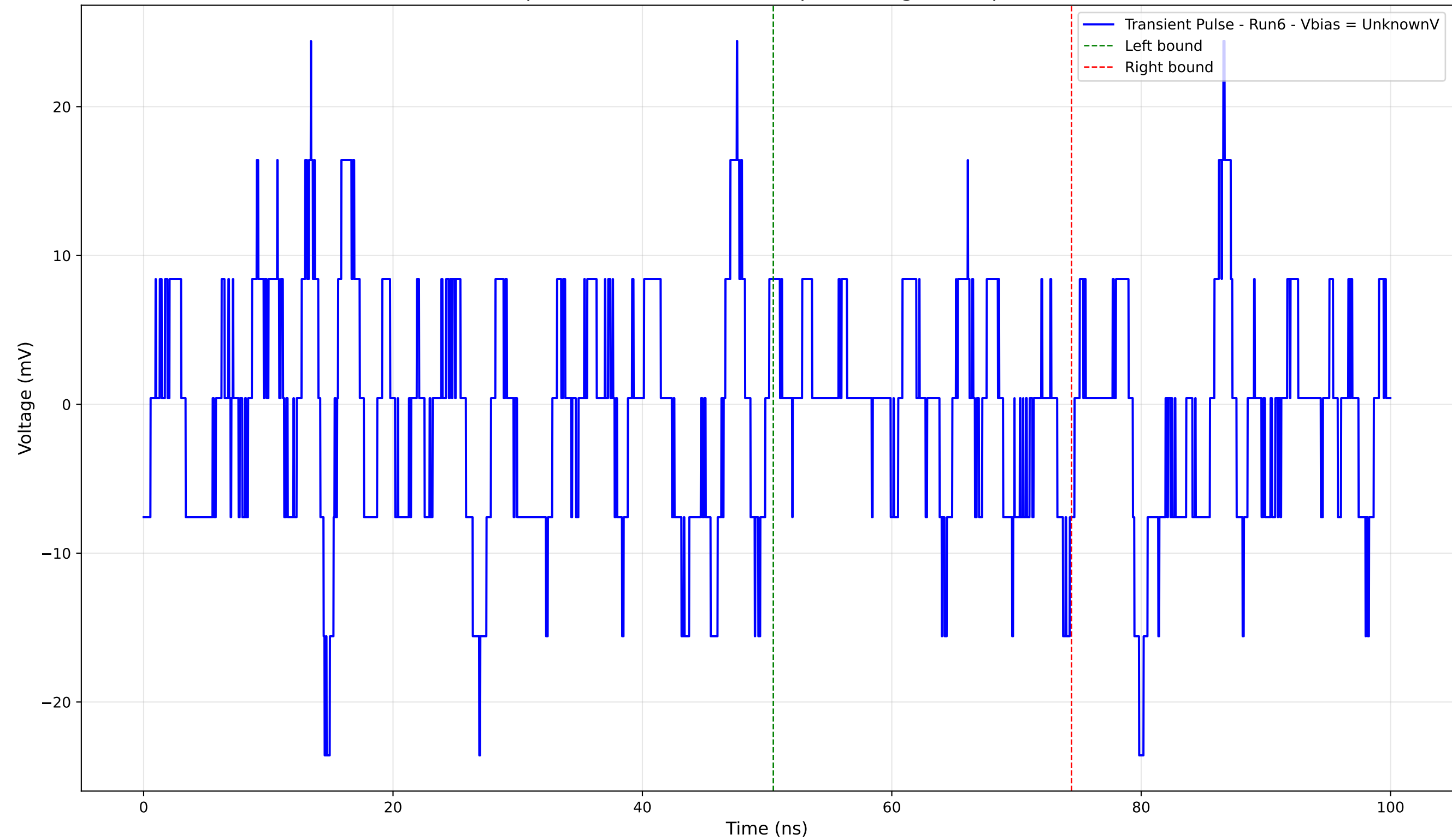
Transient Pulse - Sample: 4004 - Position: 315.0 \mu\text{m} - Charge: 0.06 pC - Rise Time: 0.75 ns
