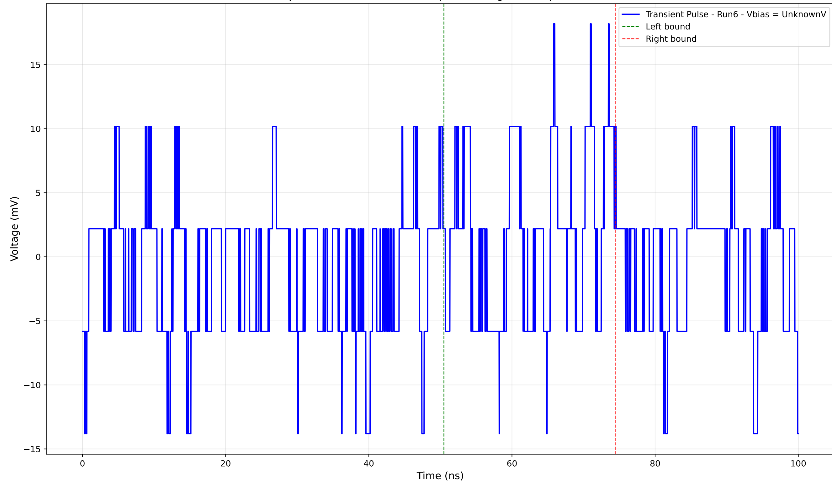
Transient Pulse - Sample: 4004 - Position: 80.0 \mu\text{m} - Charge: 0.81 pC - Rise Time: 0.00 ns (N/A)
