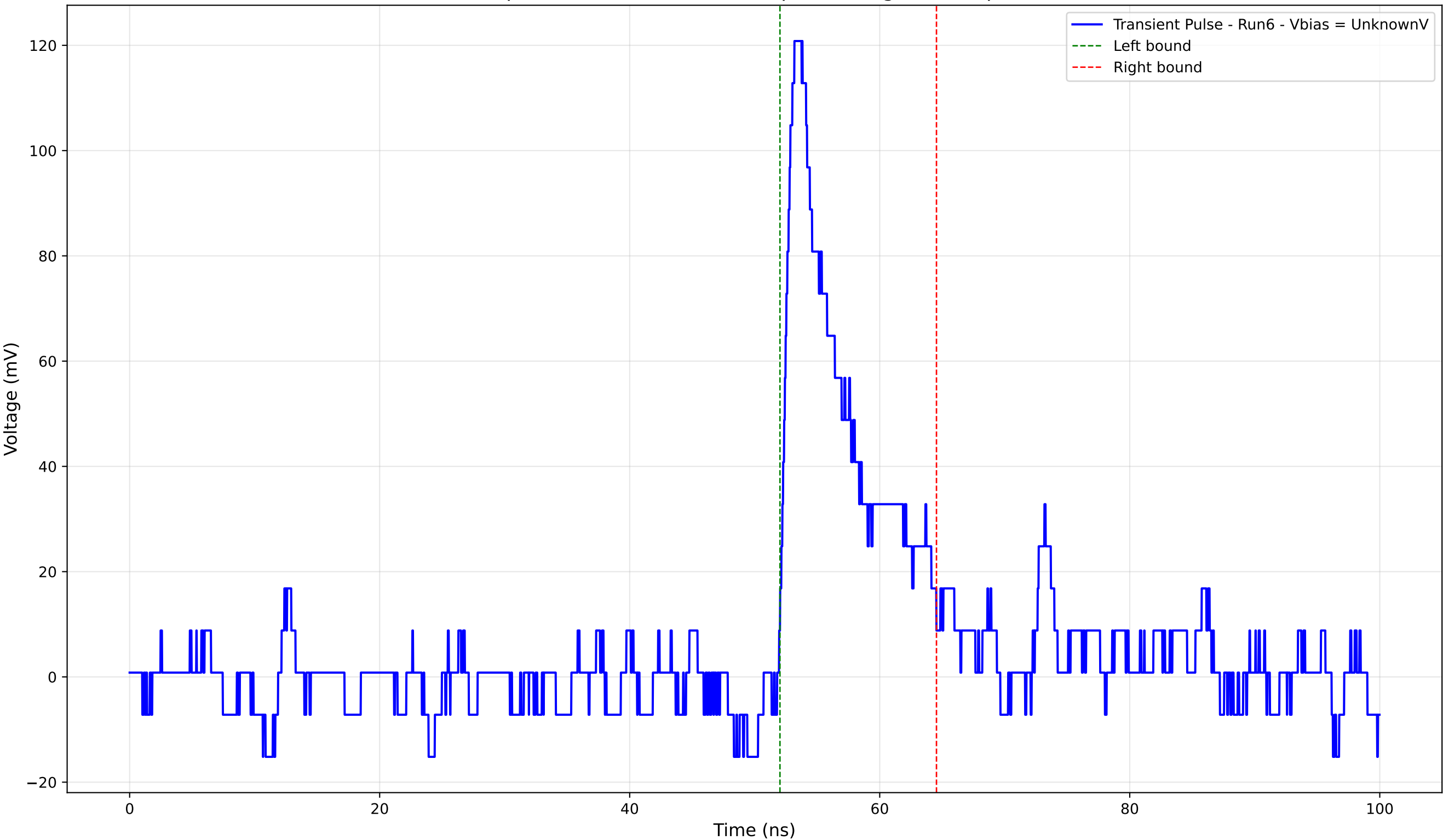
Transient Pulse - Sample: 4004 - Position: 810.0 \mu\text{m} - Charge: 12.91 pC - Rise Time: 0.99 ns
