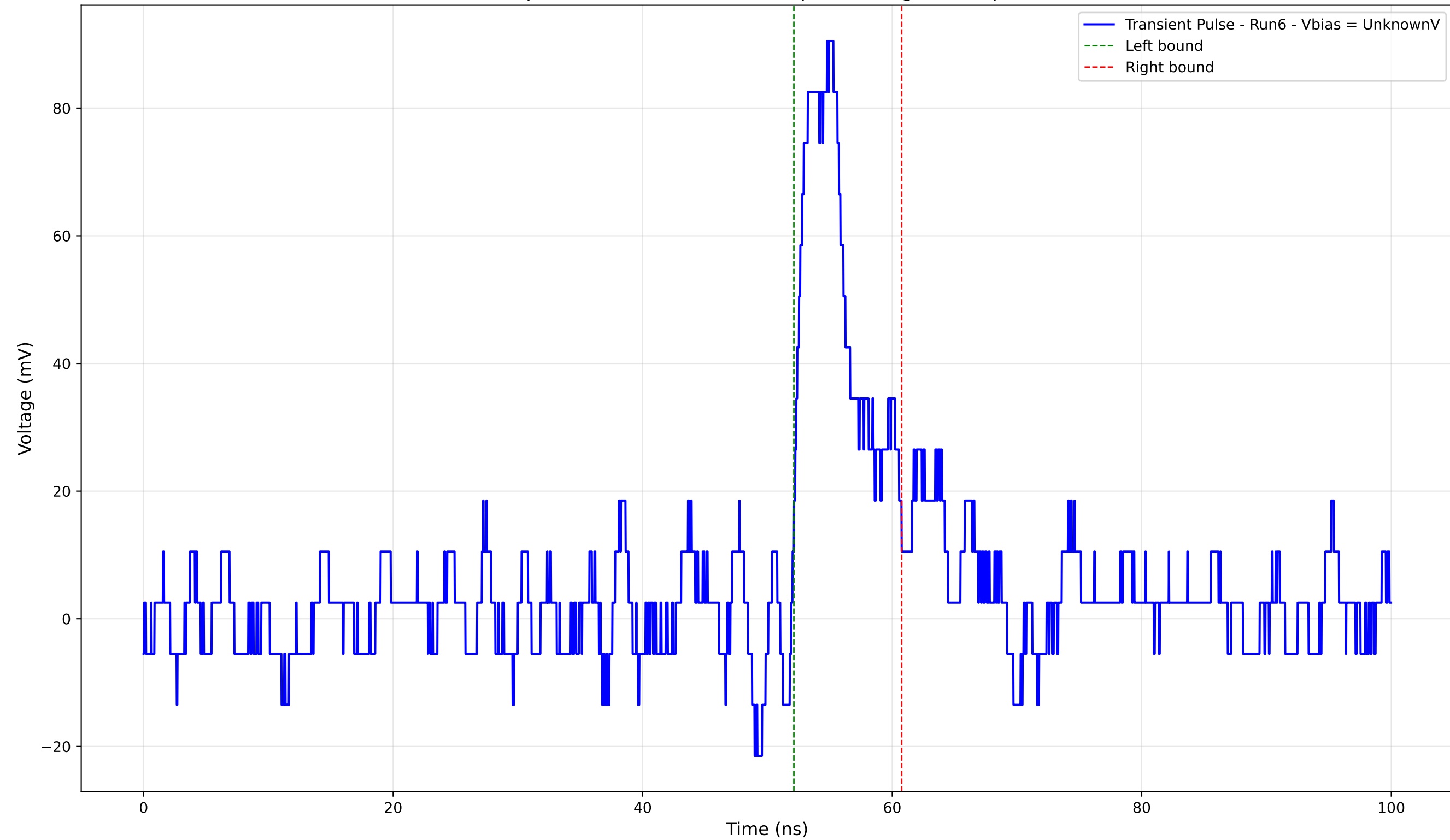
Transient Pulse - Sample: 4004 - Position: 825.0 \mu\text{m} - Charge: 8.70 pC - Rise Time: 1.22 ns
