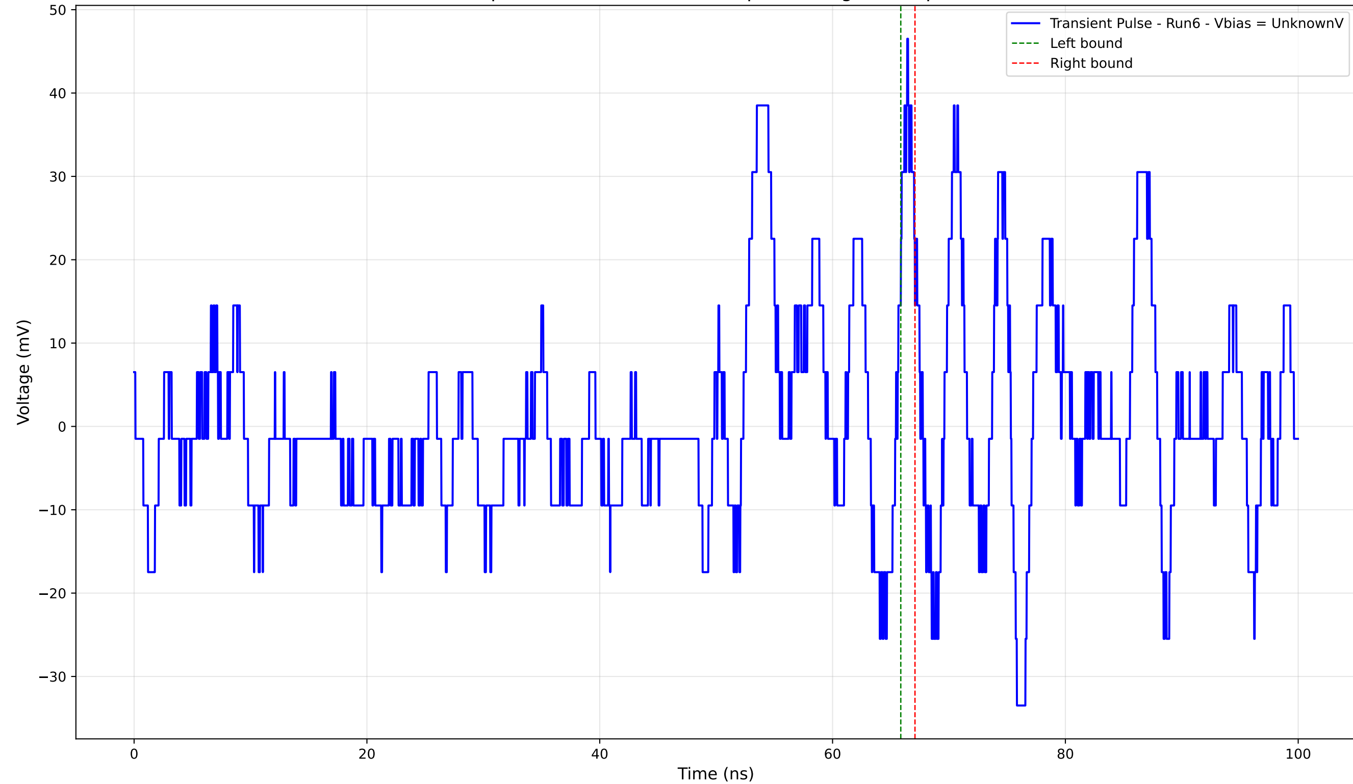
Transient Pulse - Sample: 4004 - Position: 455.0 \mu\text{m} - Charge: 0.81 pC - Rise Time: 0.83 ns
