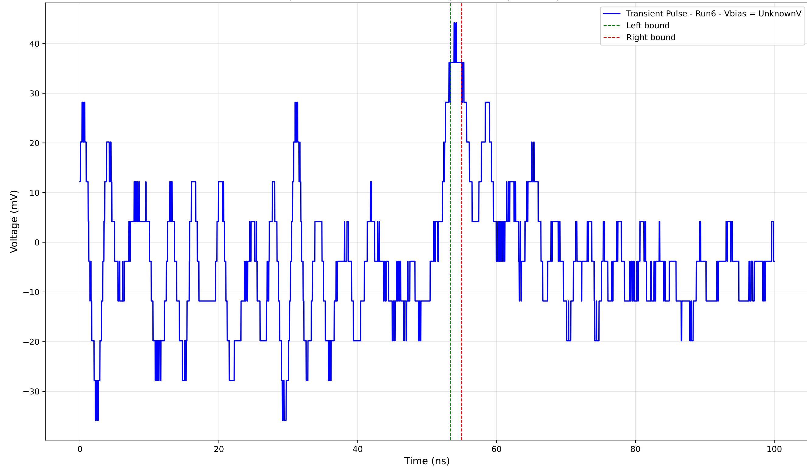
Transient Pulse - Sample: 4004 - Position: 1055.0 \mu\text{m} - Charge: 1.20 pC - Rise Time: 1.70 ns
