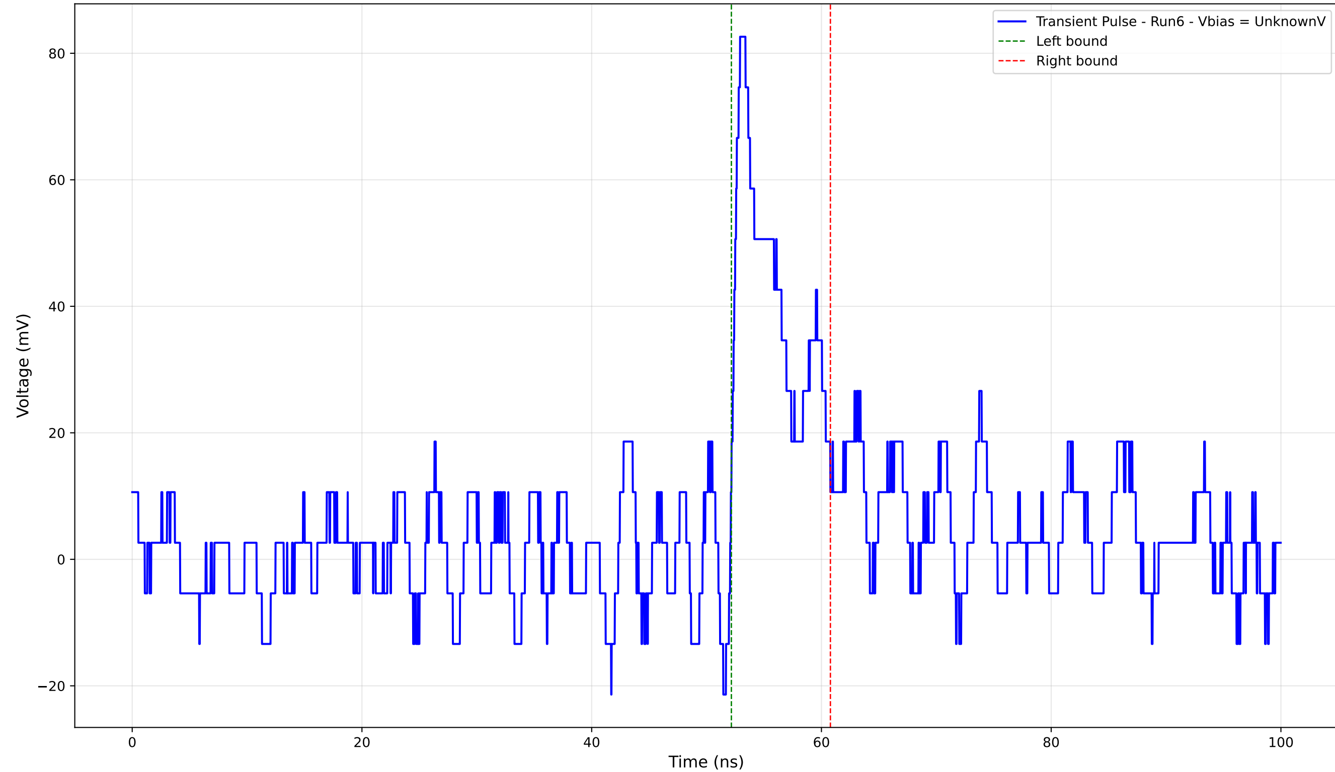
Transient Pulse - Sample: 4004 - Position: 505.0 \mu\text{m} - Charge: 7.14 pC - Rise Time: 0.69 ns
