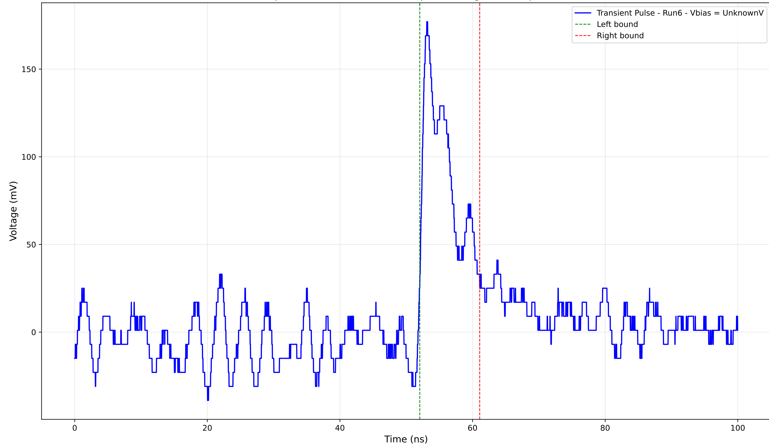
Transient Pulse - Sample: 4004 - Position: 785.0 \mu\text{m} - Charge: 16.42 pC - Rise Time: 0.90 ns
