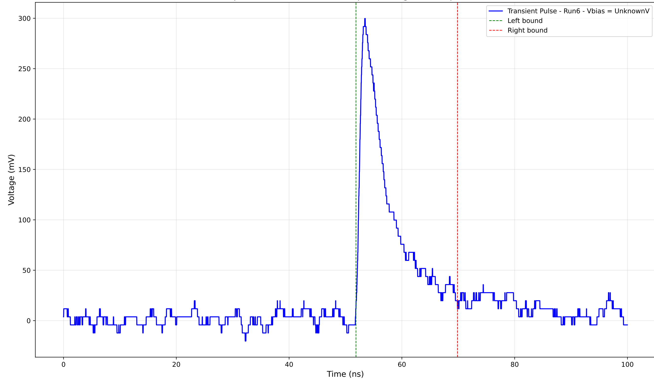
Transient Pulse - Sample: 4004 - Position: 730.0 \mu\text{m} - Charge: 36.28 pC - Rise Time: 1.01 ns
