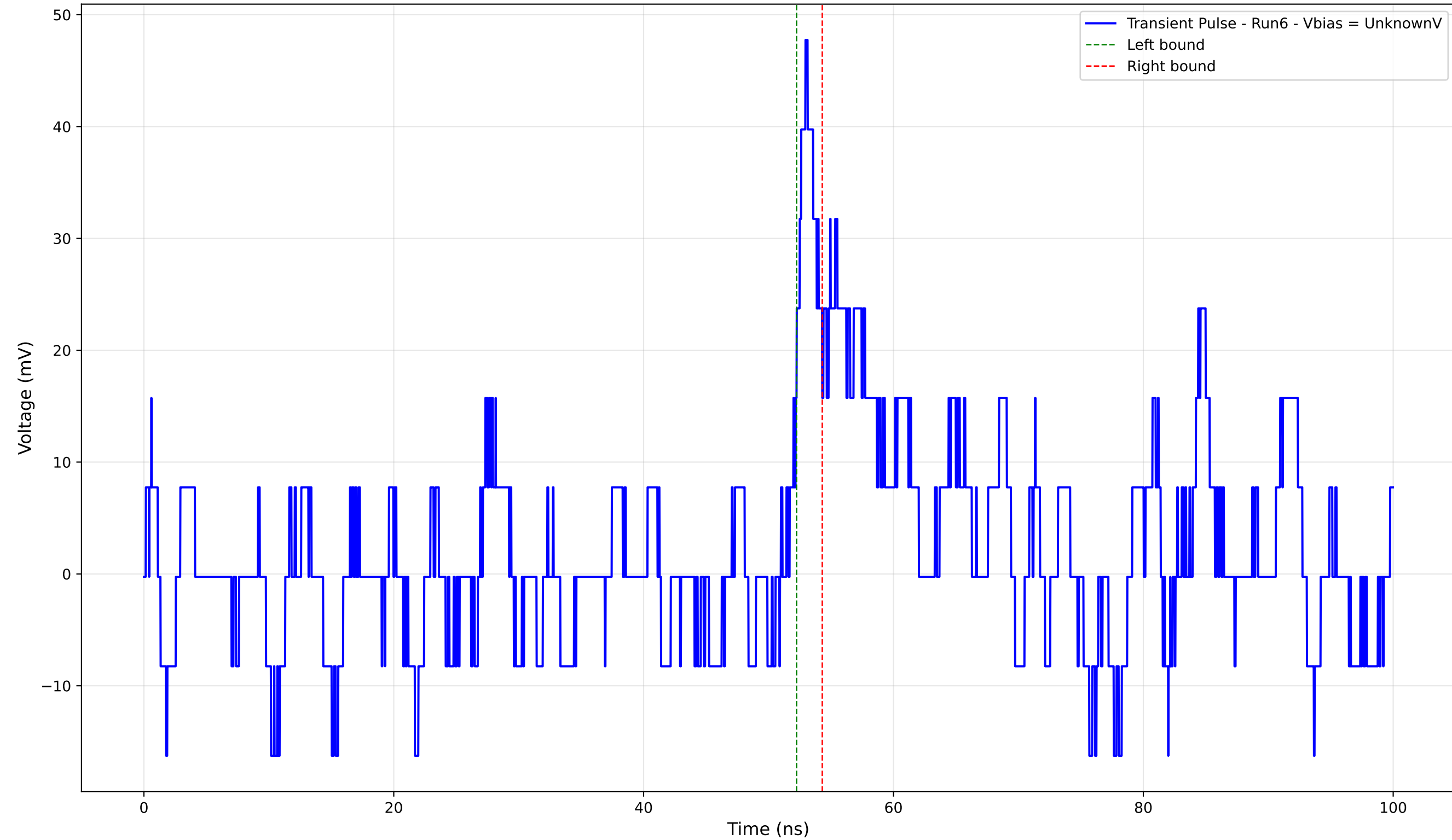
Transient Pulse - Sample: 4004 - Position: 1045.0 \mu\text{m} - Charge: 1.38 pC - Rise Time: 1.27 ns
