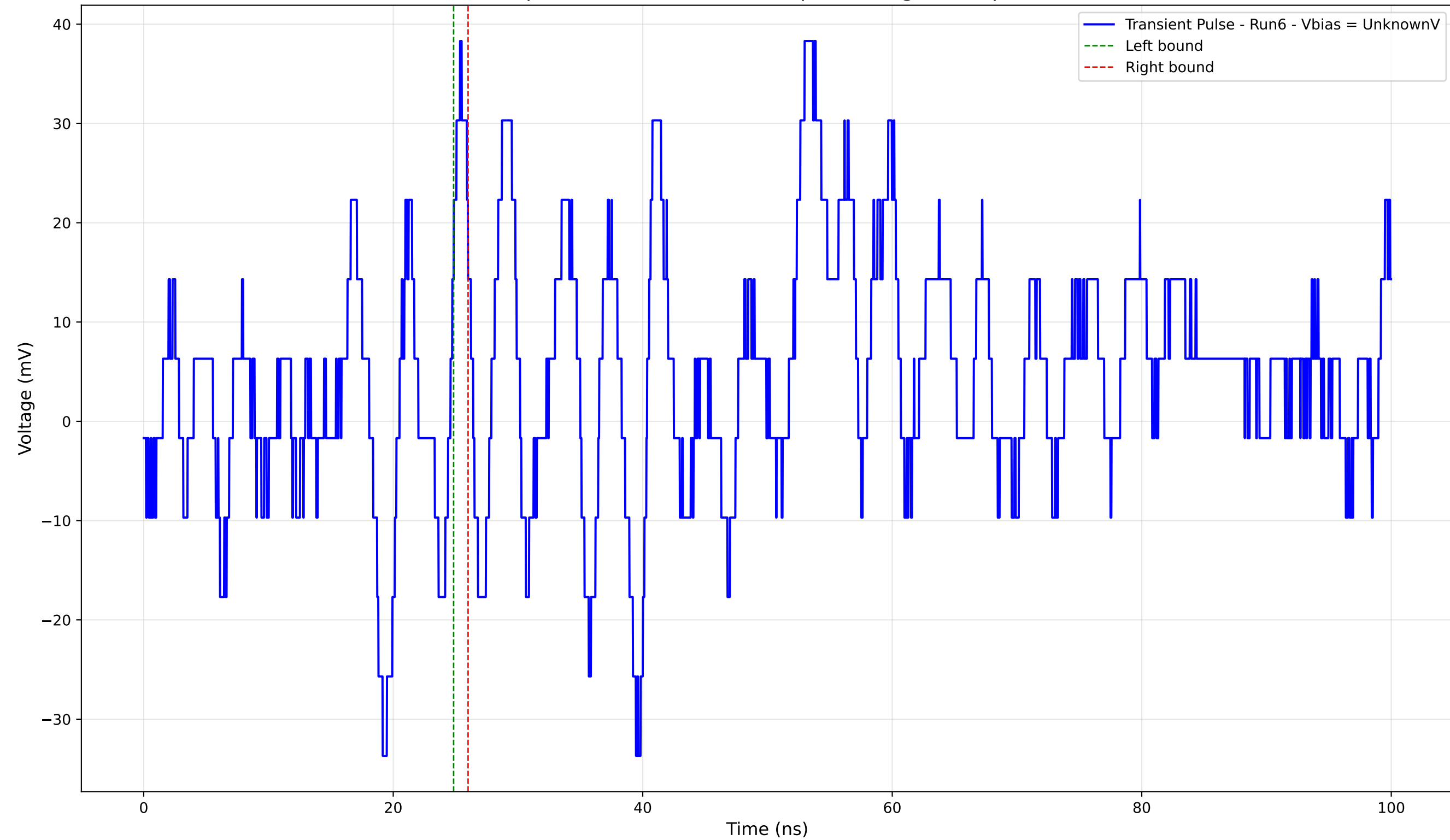
Transient Pulse - Sample: 4004 - Position: 850.0 \mu\text{m} - Charge: 0.67 pC - Rise Time: 0.77 ns
