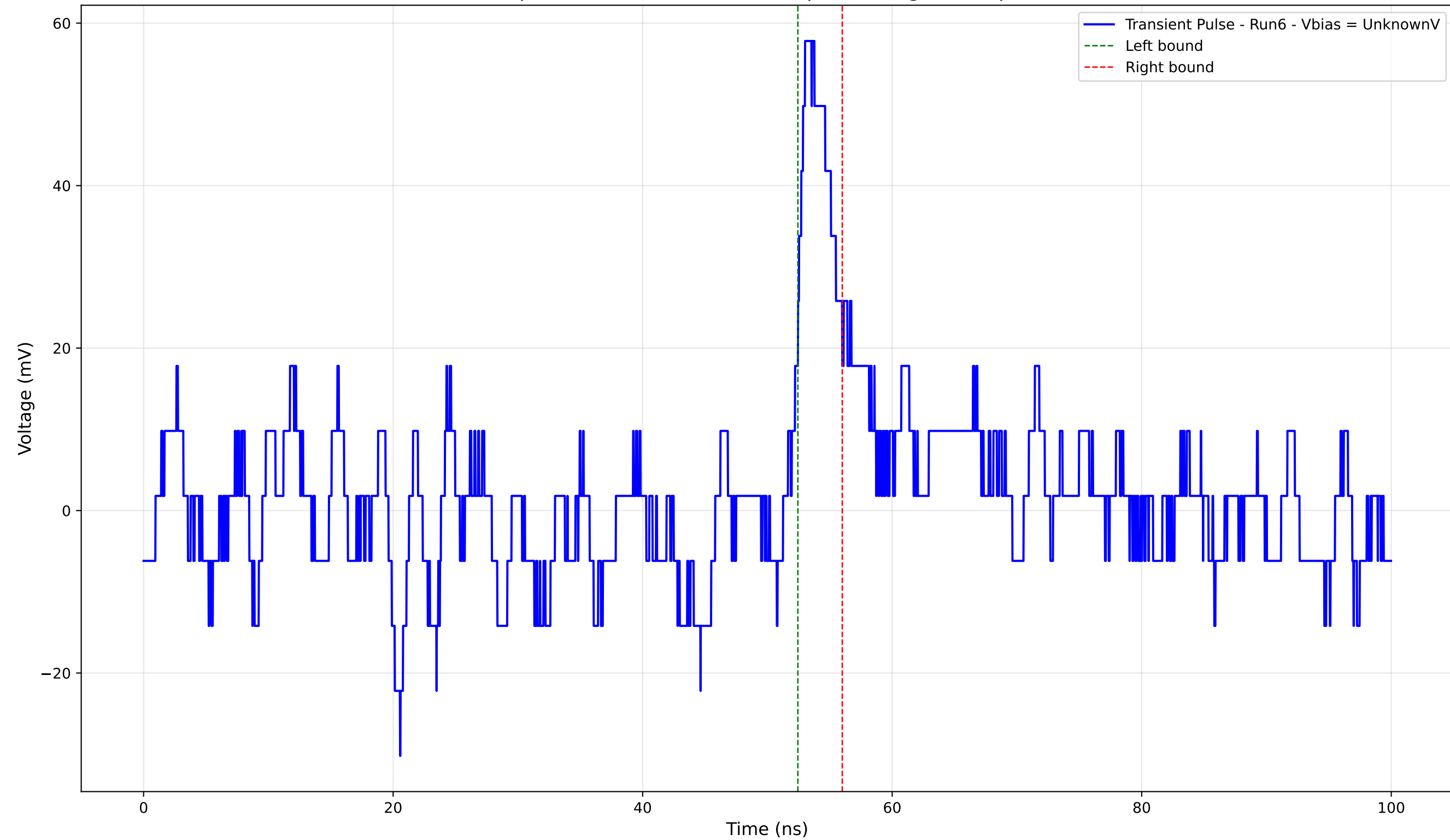
Transient Pulse - Sample: 4004 - Position: 1075.0 \mu\text{m} - Charge: 3.09 pC - Rise Time: 1.07 ns
