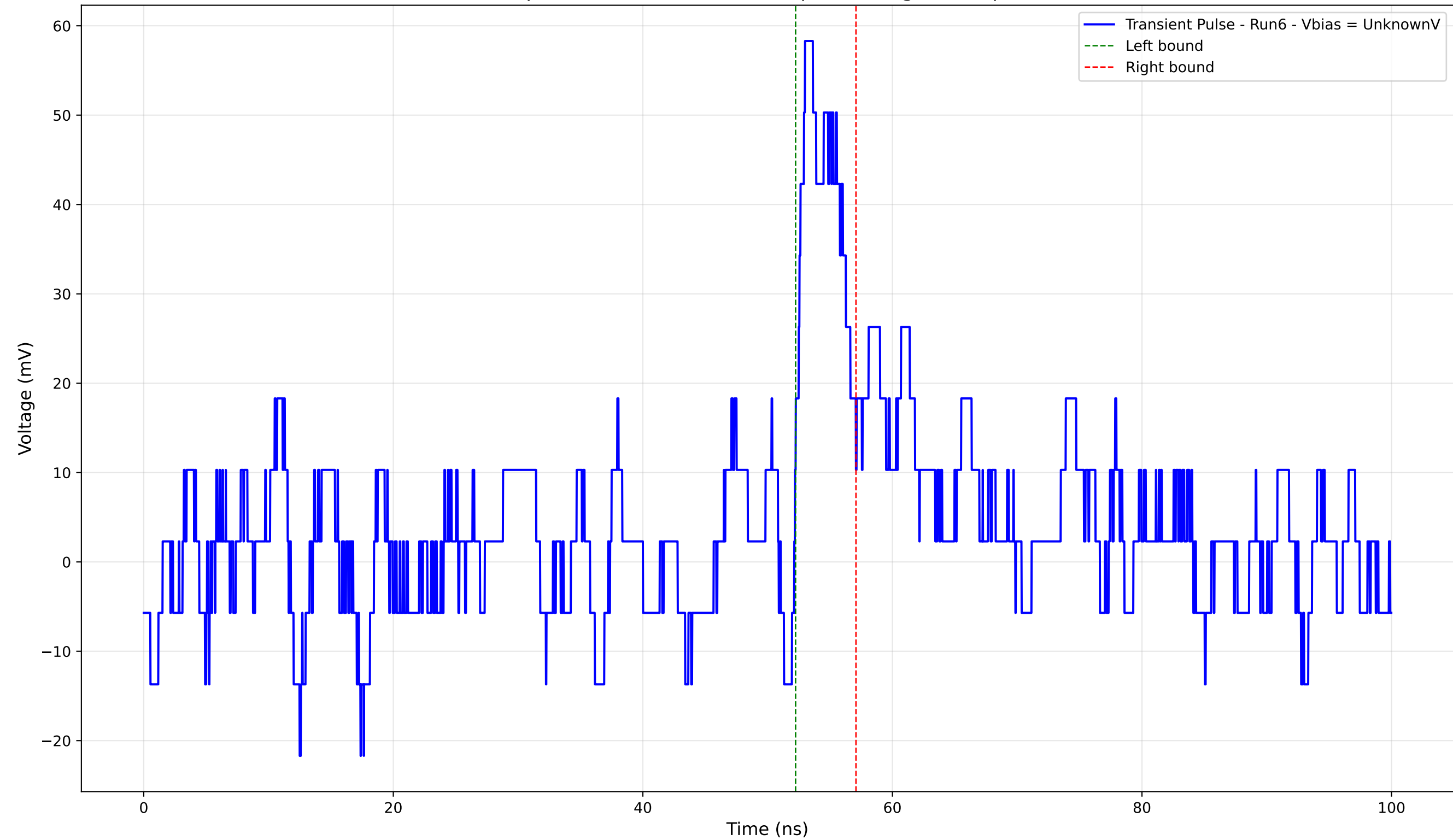
Transient Pulse - Sample: 4004 - Position: 915.0 \mu\text{m} - Charge: 3.93 pC - Rise Time: 0.81 ns
