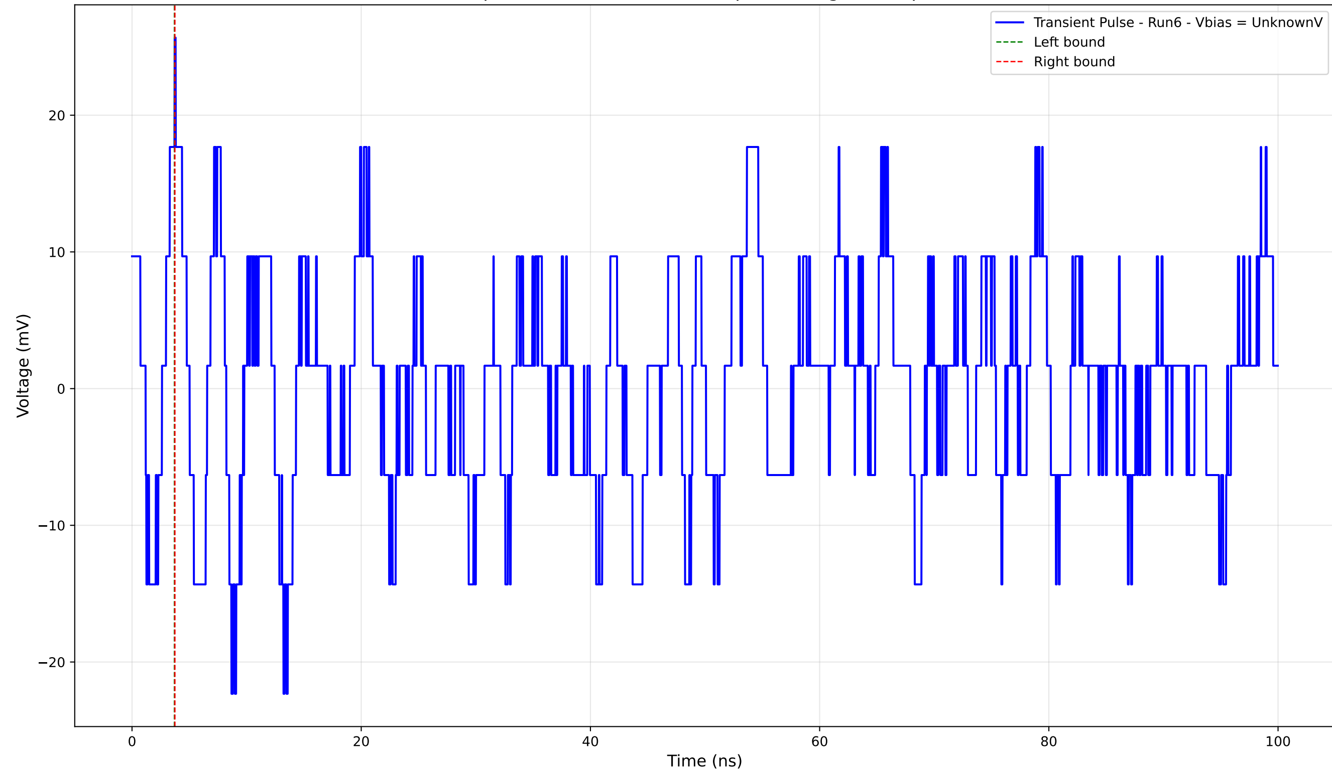
Transient Pulse - Sample: 4004 - Position: 425.0 \mu\text{m} - Charge: 0.02 pC - Rise Time: 0.76 ns
