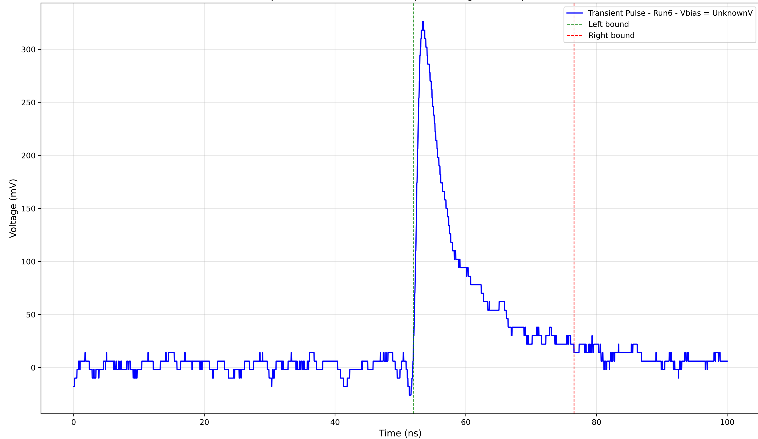
Transient Pulse - Sample: 4004 - Position: 705.0 \mu\text{m} - Charge: 43.84 pC - Rise Time: 0.91 ns
