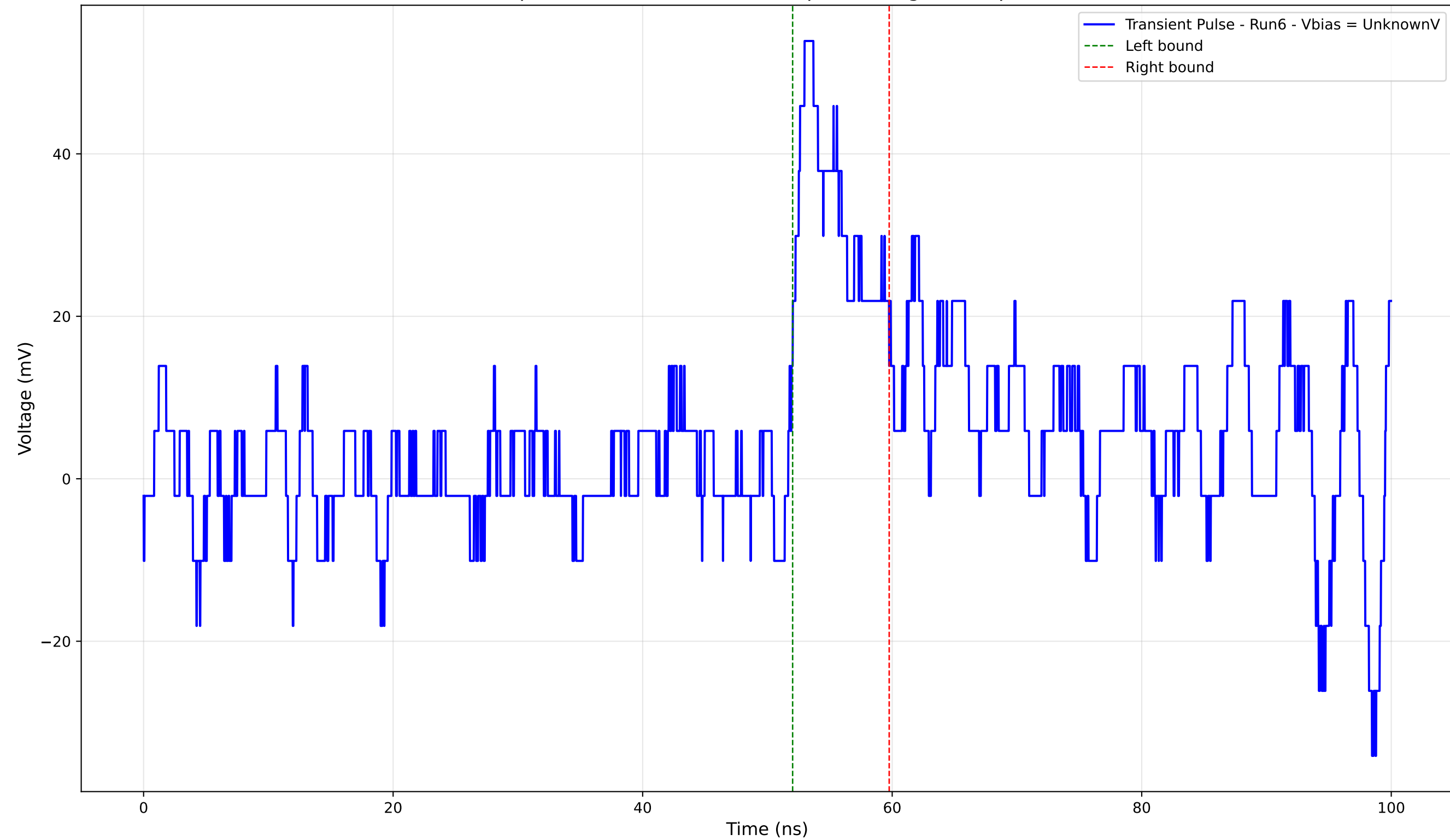
Transient Pulse - Sample: 4004 - Position: 1040.0 \mu\text{m} - Charge: 5.05 pC - Rise Time: 1.30 ns
