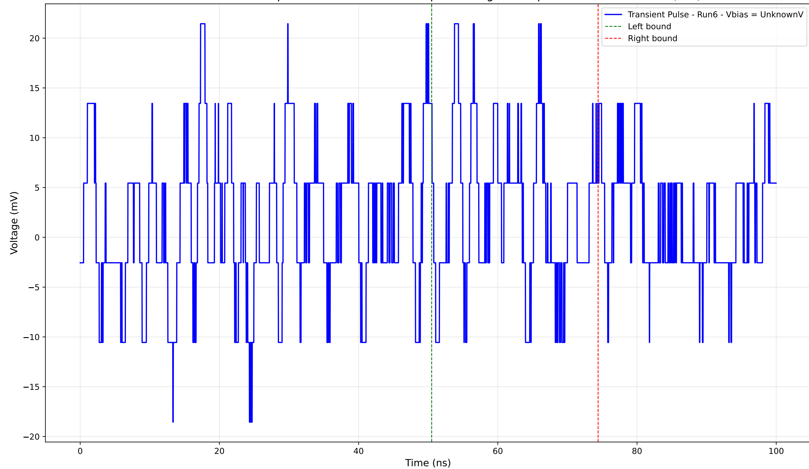
Transient Pulse - Sample: 4004 - Position: 310.0 \mu\text{m} - Charge: 1.32 pC - Rise Time: 0.00 ns (N/A)
