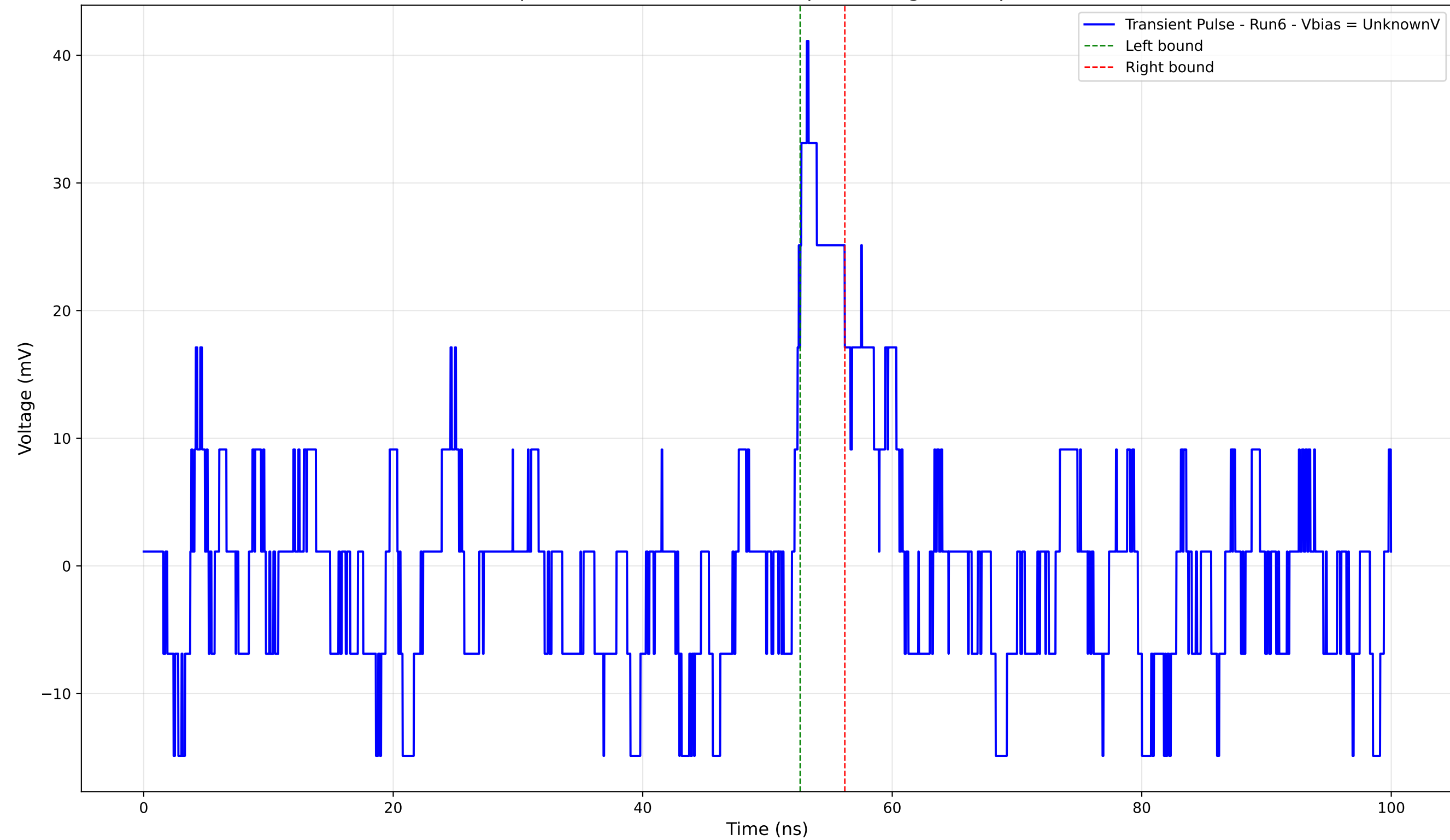
Transient Pulse - Sample: 4004 - Position: 1110.0 \mu\text{m} - Charge: 2.02 pC - Rise Time: 0.99 ns
