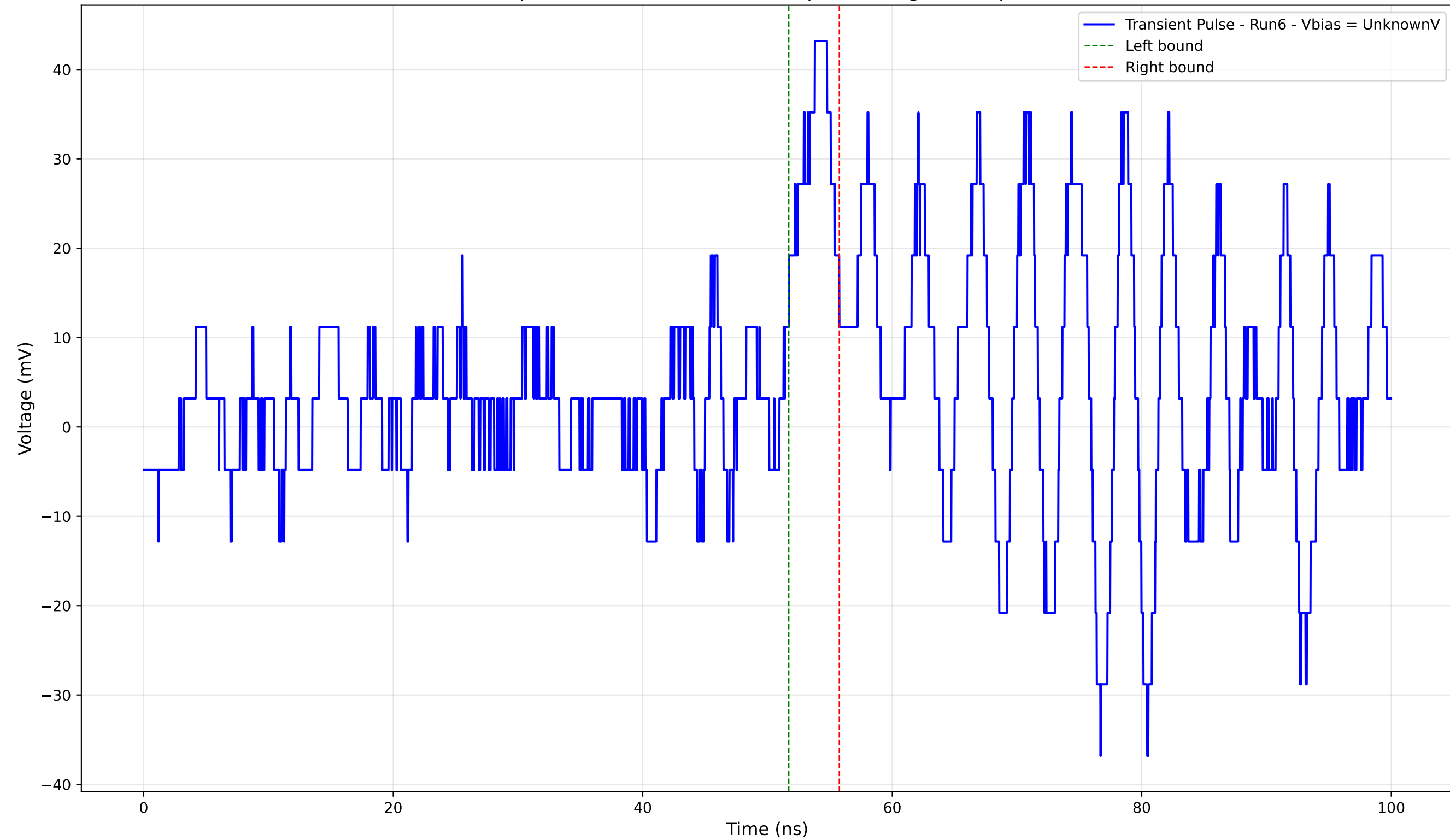
Transient Pulse - Sample: 4004 - Position: 1115.0 \mu\text{m} - Charge: 2.49 pC - Rise Time: 2.40 ns
