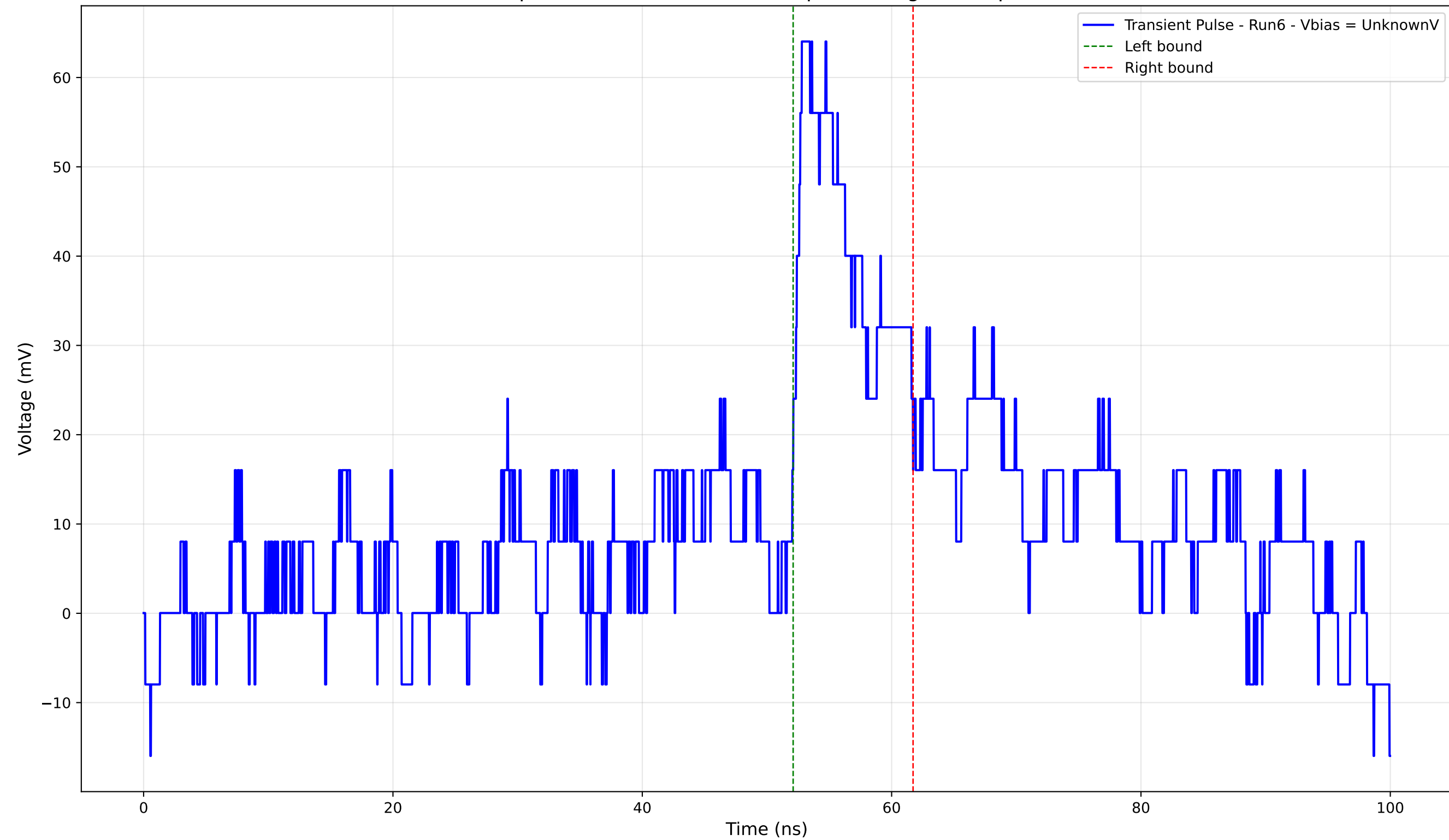
Transient Pulse - Sample: 4004 - Position: 1030.0 \mu\text{m} - Charge: 7.93 pC - Rise Time: 1.20 ns
