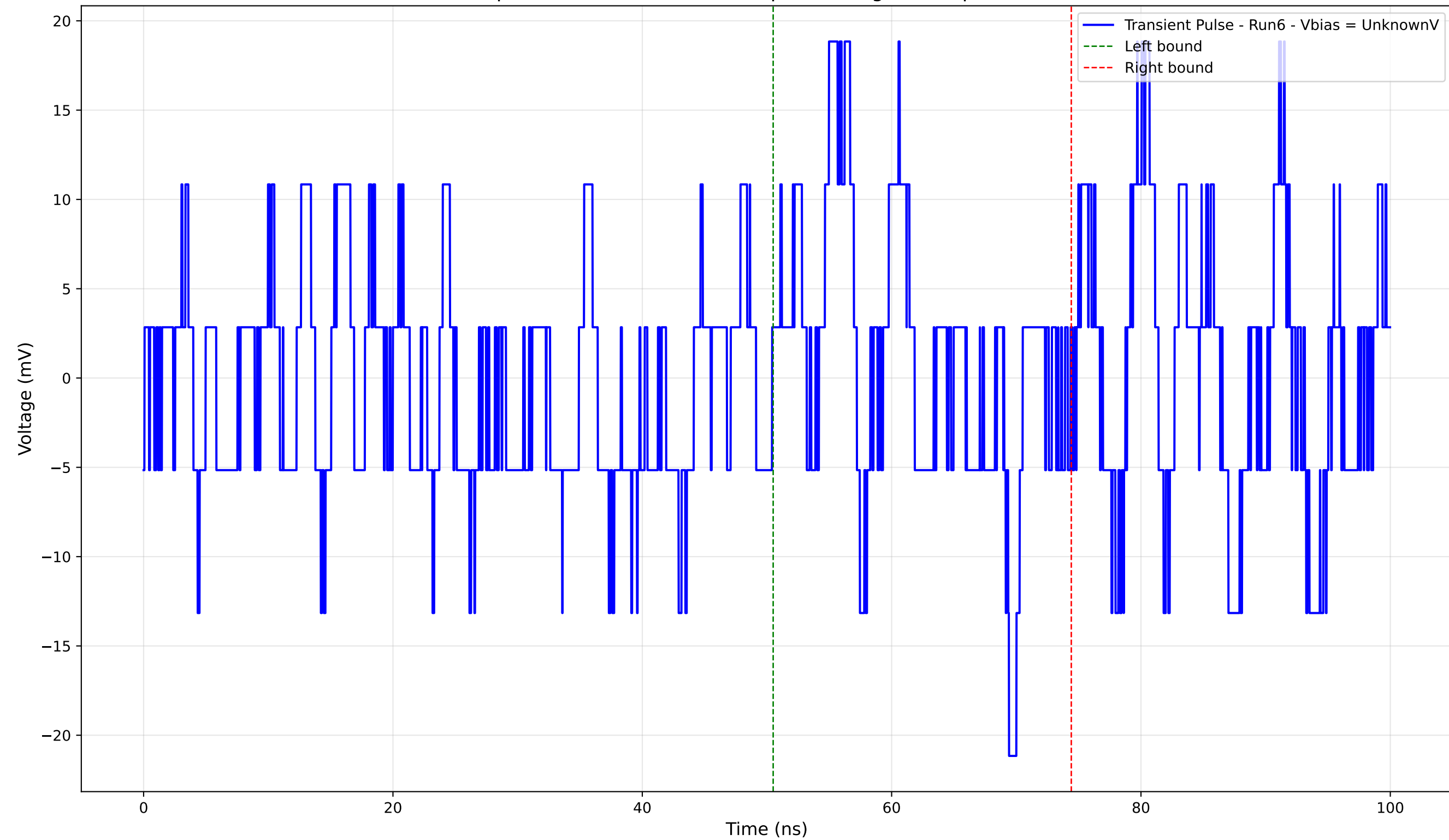
Transient Pulse - Sample: 4004 - Position: 115.0 \mu\text{m} - Charge: 0.55 pC - Rise Time: 0.00 ns (N/A)
