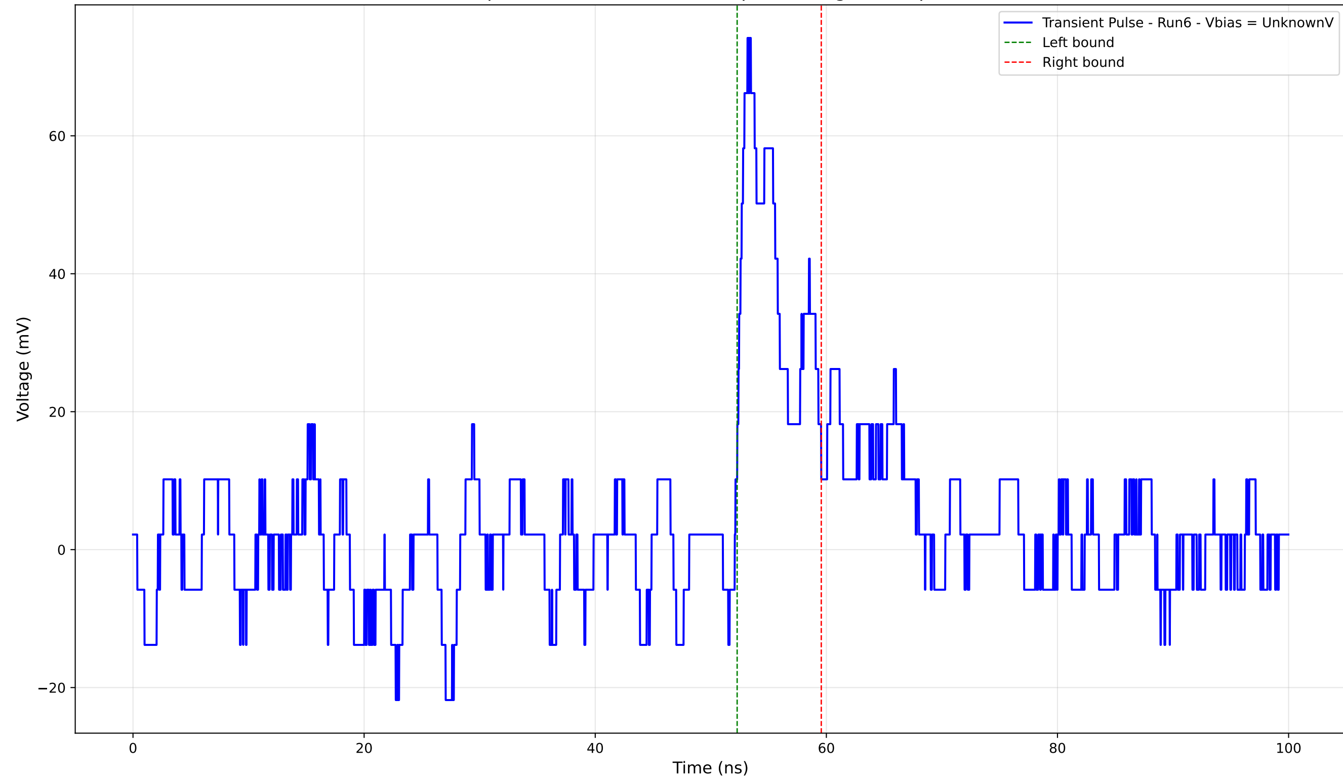
Transient Pulse - Sample: 4004 - Position: 935.0 \mu\text{m} - Charge: 5.79 pC - Rise Time: 1.05 ns
