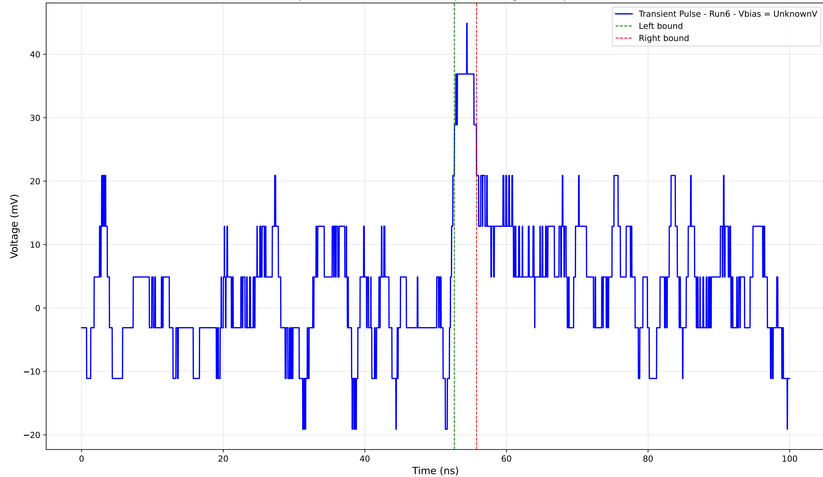
Transient Pulse - Sample: 4004 - Position: 865.0 \mu\text{m} - Charge: 2.21 pC - Rise Time: 2.30 ns
