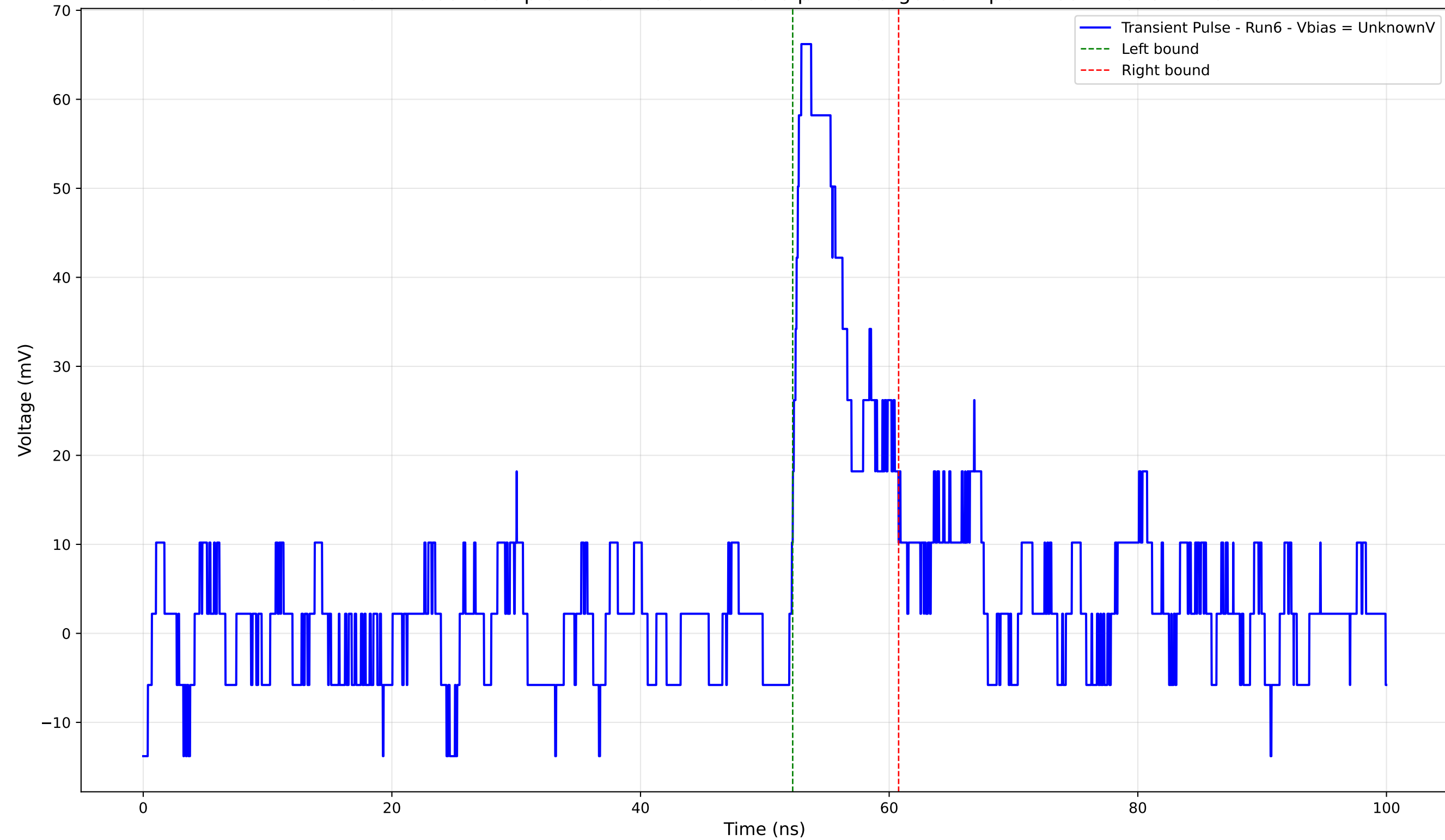
Transient Pulse - Sample: 4004 - Position: 950.0 \mu\text{m} - Charge: 6.42 pC - Rise Time: 0.77 ns
