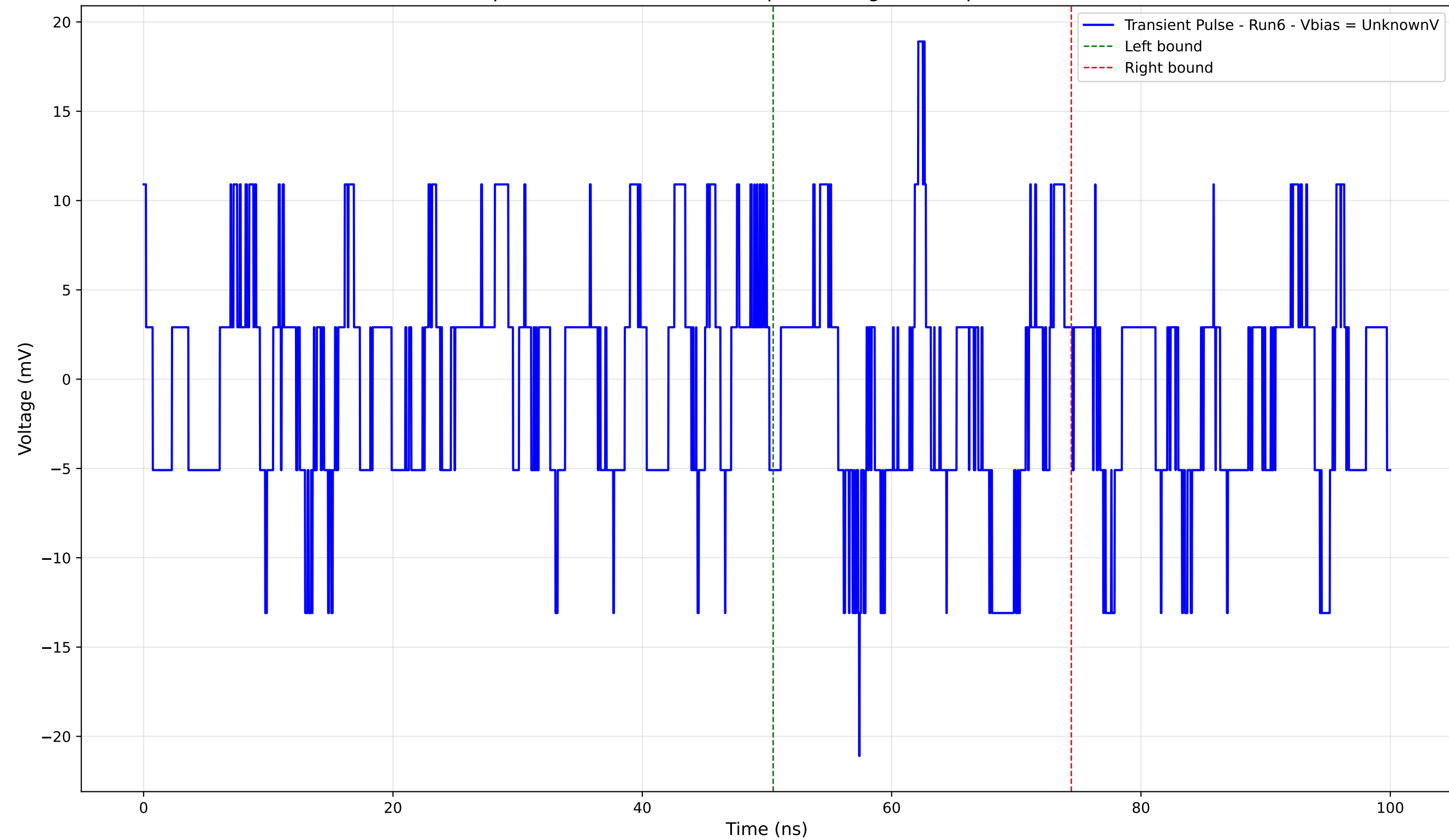
Transient Pulse - Sample: 4004 - Position: 140.0 \mu\text{m} - Charge: -0.57 pC - Rise Time: 0.00 ns (N/A)
