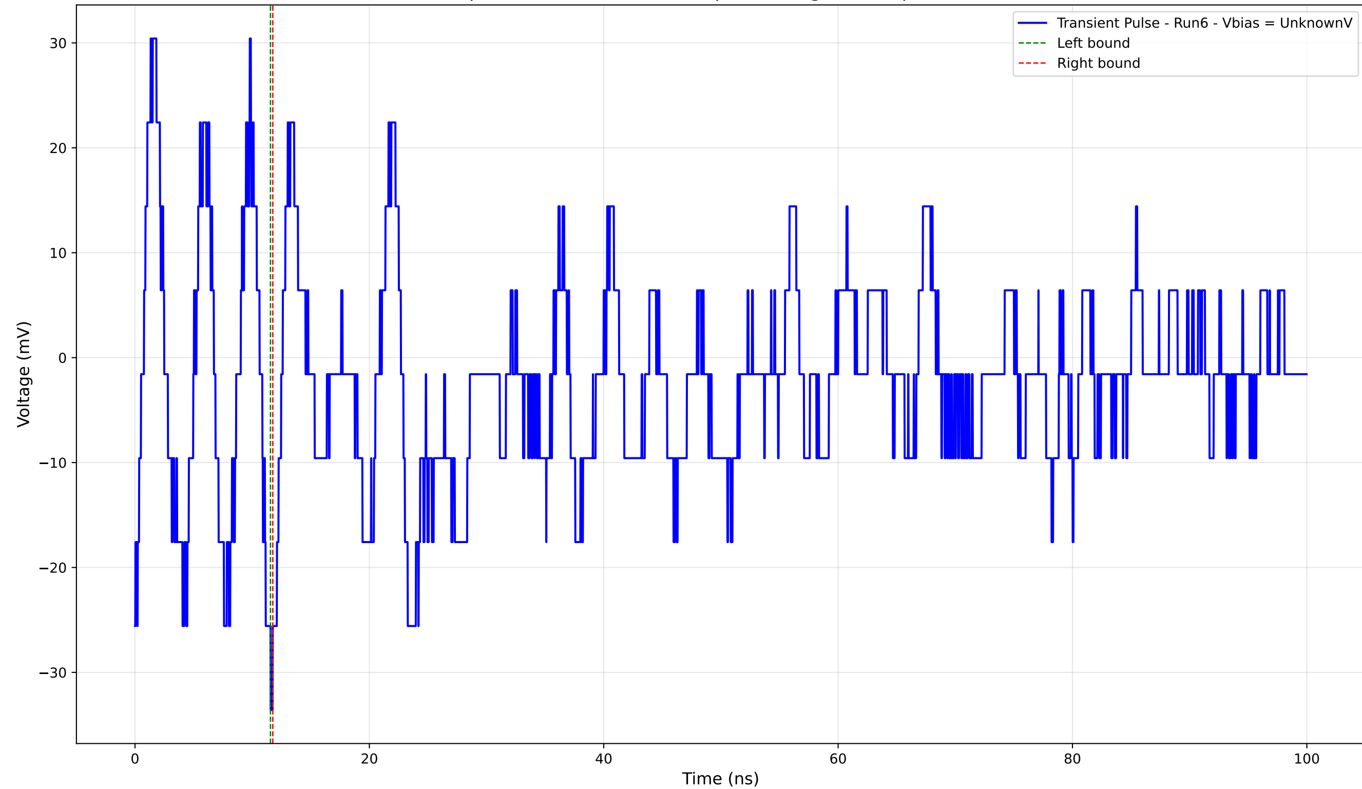
Transient Pulse - Sample: 4004 - Position: 45.0 \mu\text{m} - Charge: -0.13 pC - Rise Time: 0.00 ns (N/A)
