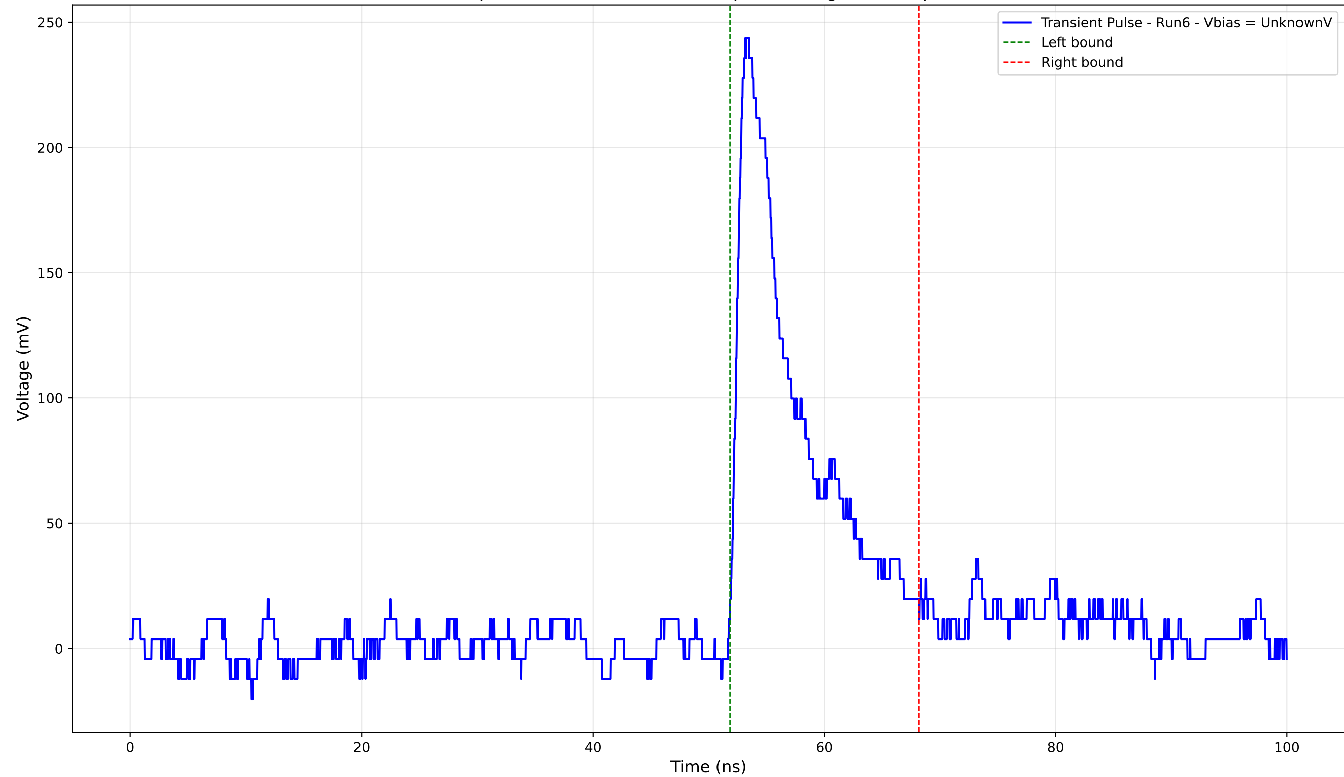
Transient Pulse - Sample: 4004 - Position: 745.0 \mu\text{m} - Charge: 28.96 pC - Rise Time: 0.97 ns
