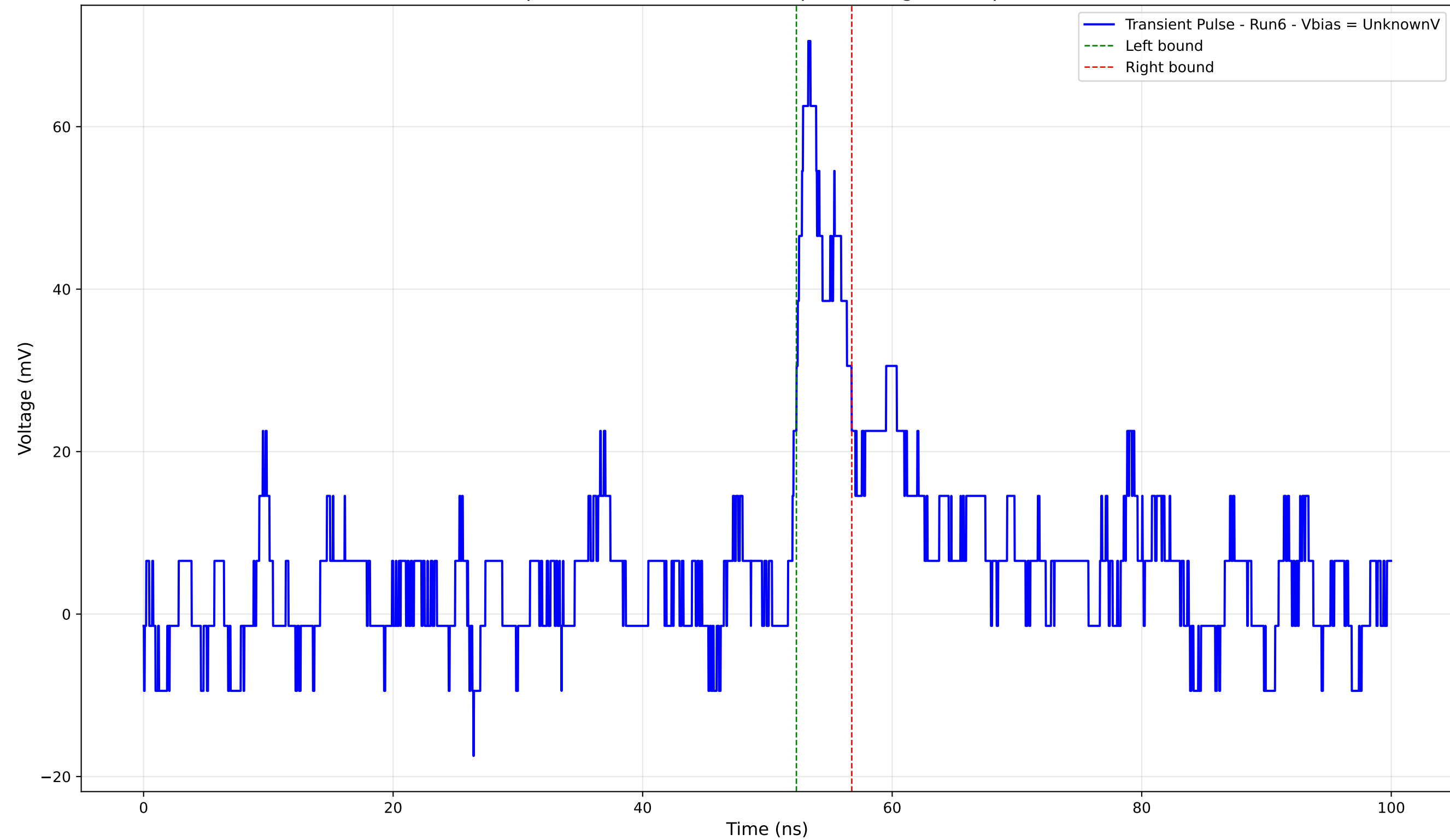
Transient Pulse - Sample: 4004 - Position: 920.0 \mu\text{m} - Charge: 4.17 pC - Rise Time: 1.28 ns
