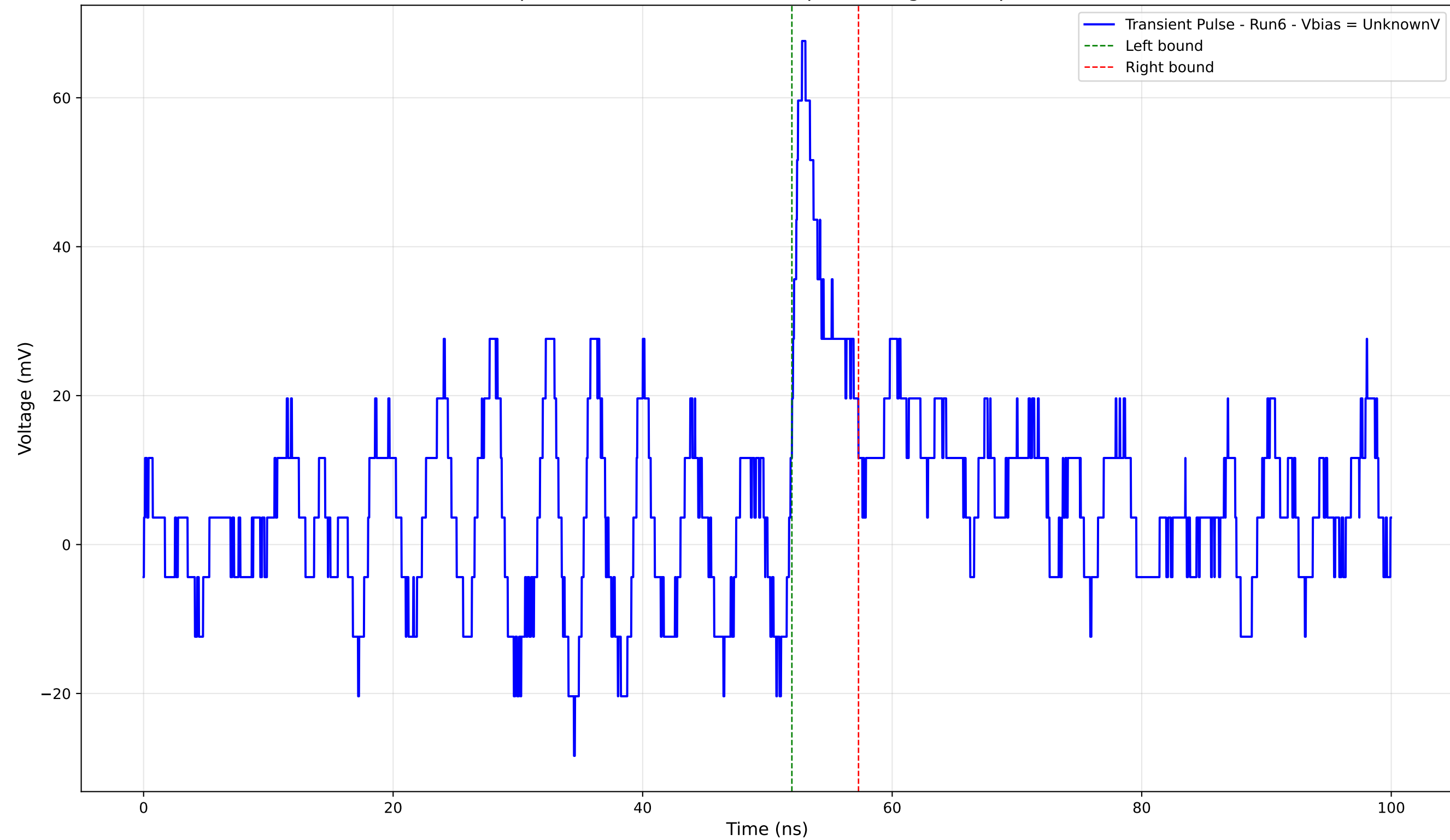
Transient Pulse - Sample: 4004 - Position: 1070.0 \mu\text{m} - Charge: 3.91 pC - Rise Time: 0.93 ns
