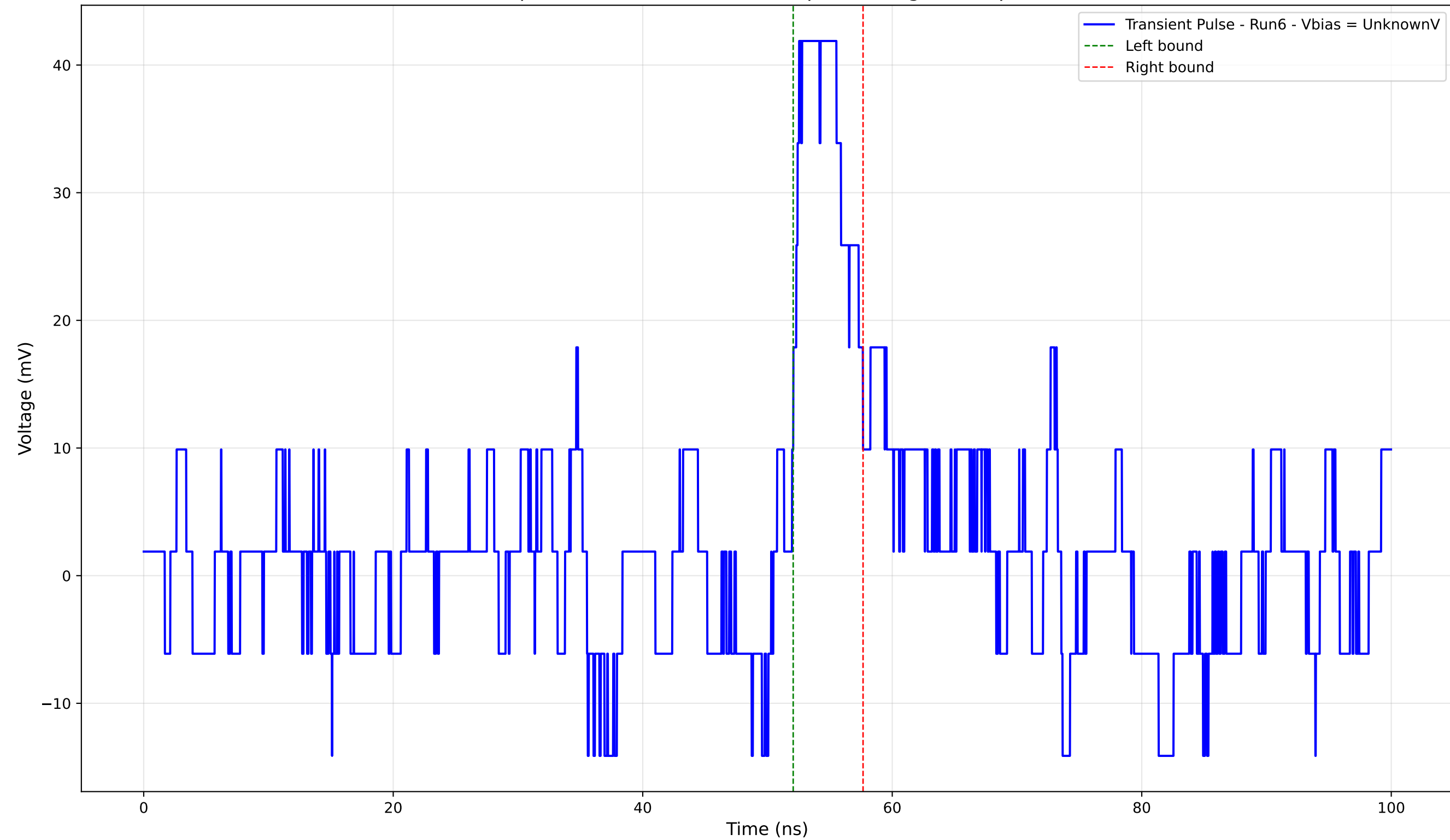
Transient Pulse - Sample: 4004 - Position: 1035.0 \mu\text{m} - Charge: 3.80 pC - Rise Time: 0.57 ns
