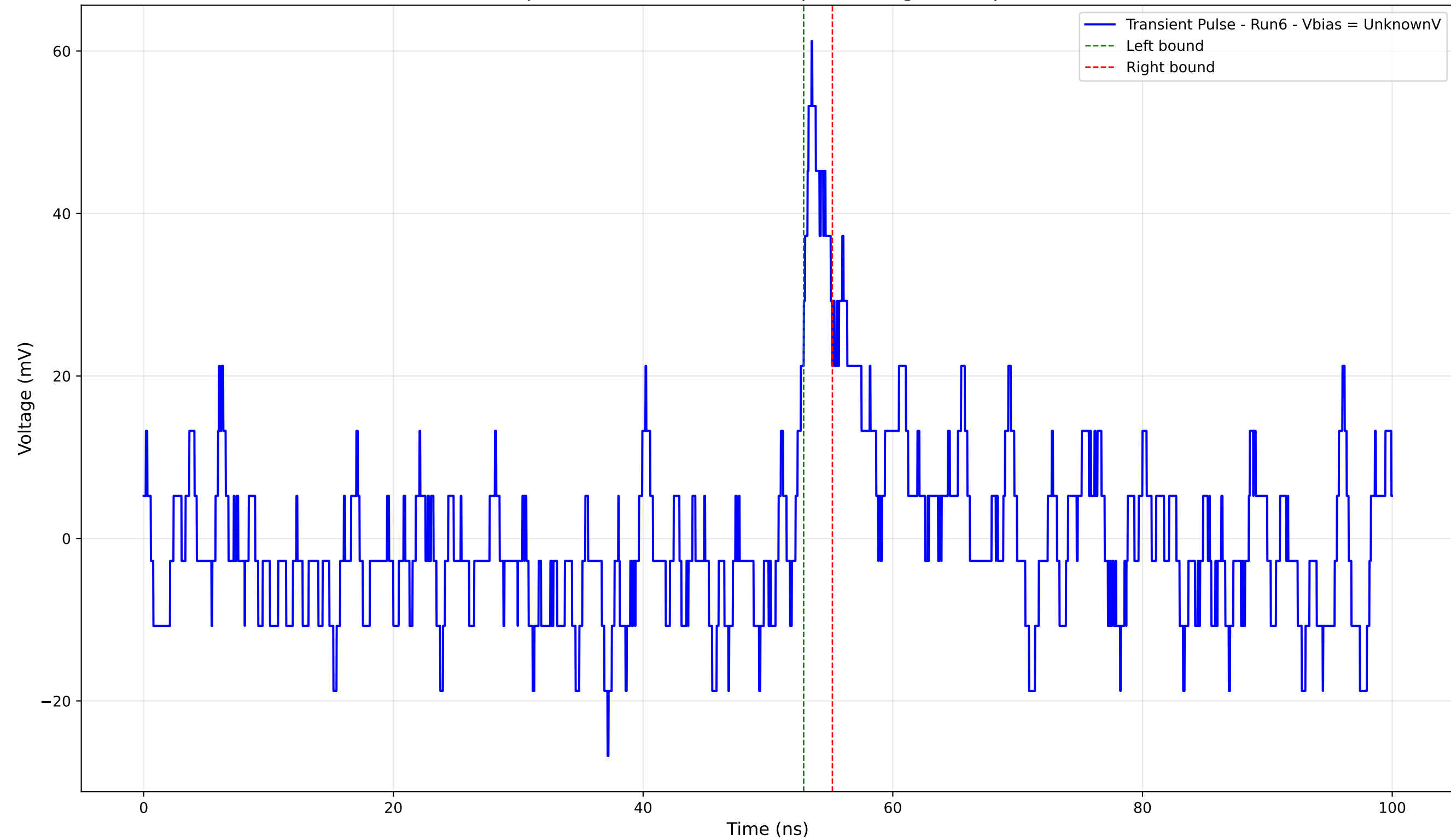
Transient Pulse - Sample: 4004 - Position: 840.0 \mu\text{m} - Charge: 1.98 pC - Rise Time: 1.14 ns
