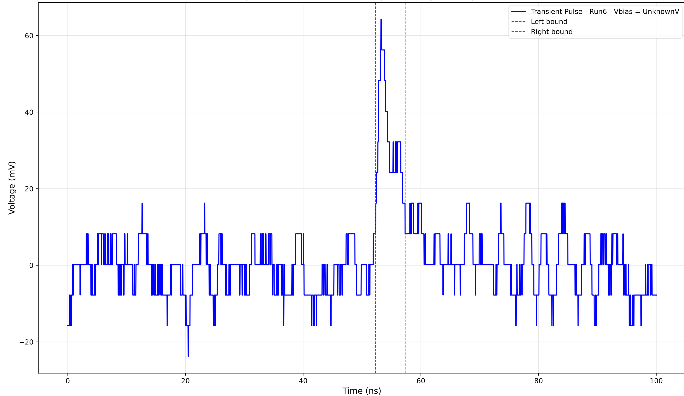
Transient Pulse - Sample: 4004 - Position: 1060.0 \mu\text{m} - Charge: 3.35 pC - Rise Time: 1.30 ns
