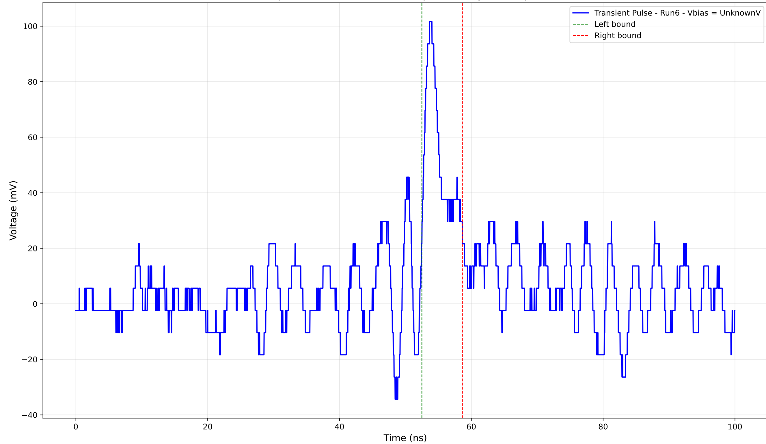
Transient Pulse - Sample: 4004 - Position: 965.0 \mu\text{m} - Charge: 6.61 pC - Rise Time: 1.03 ns
