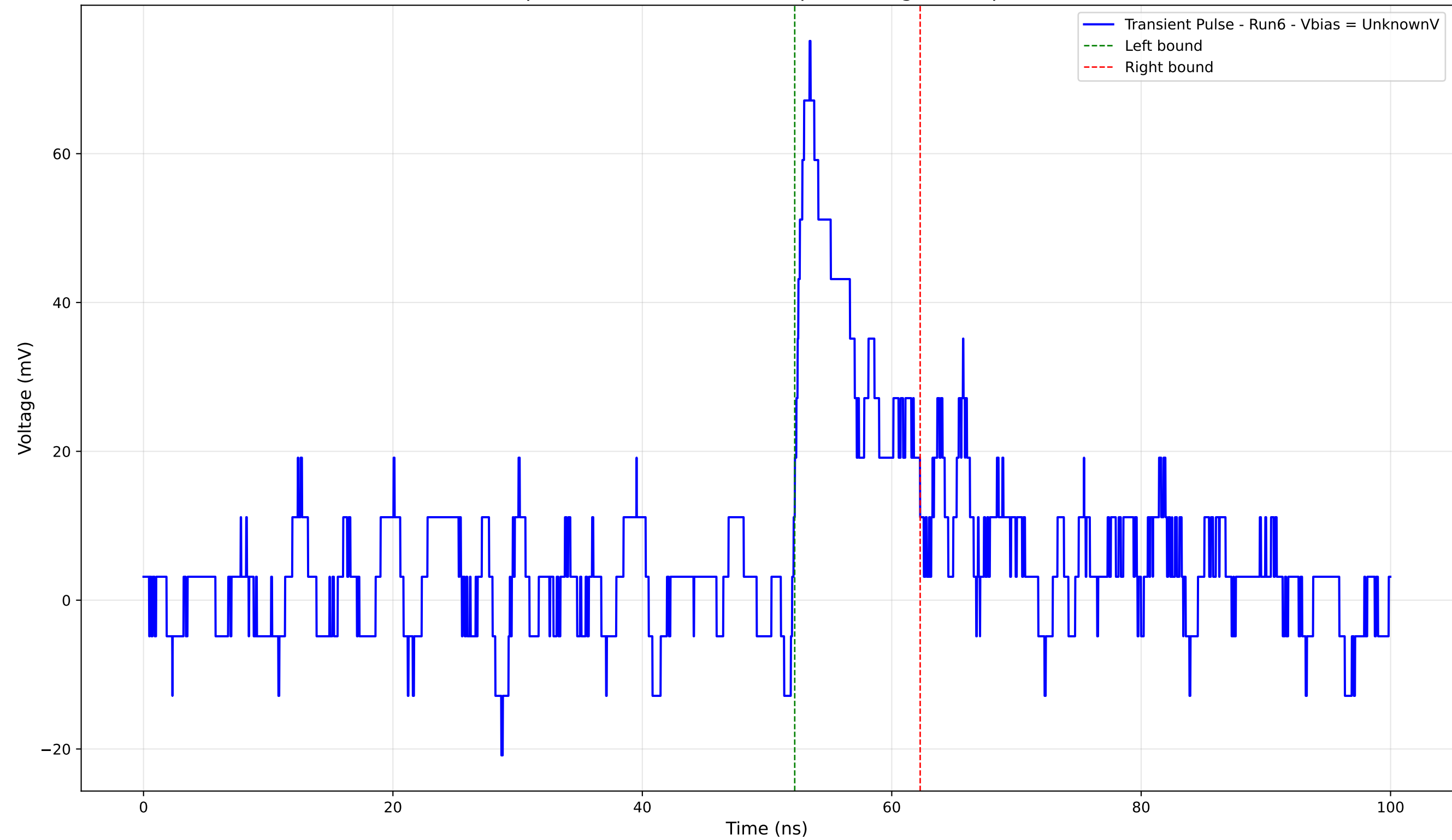
Transient Pulse - Sample: 4004 - Position: 985.0 \mu\text{m} - Charge: 7.23 pC - Rise Time: 1.29 ns
