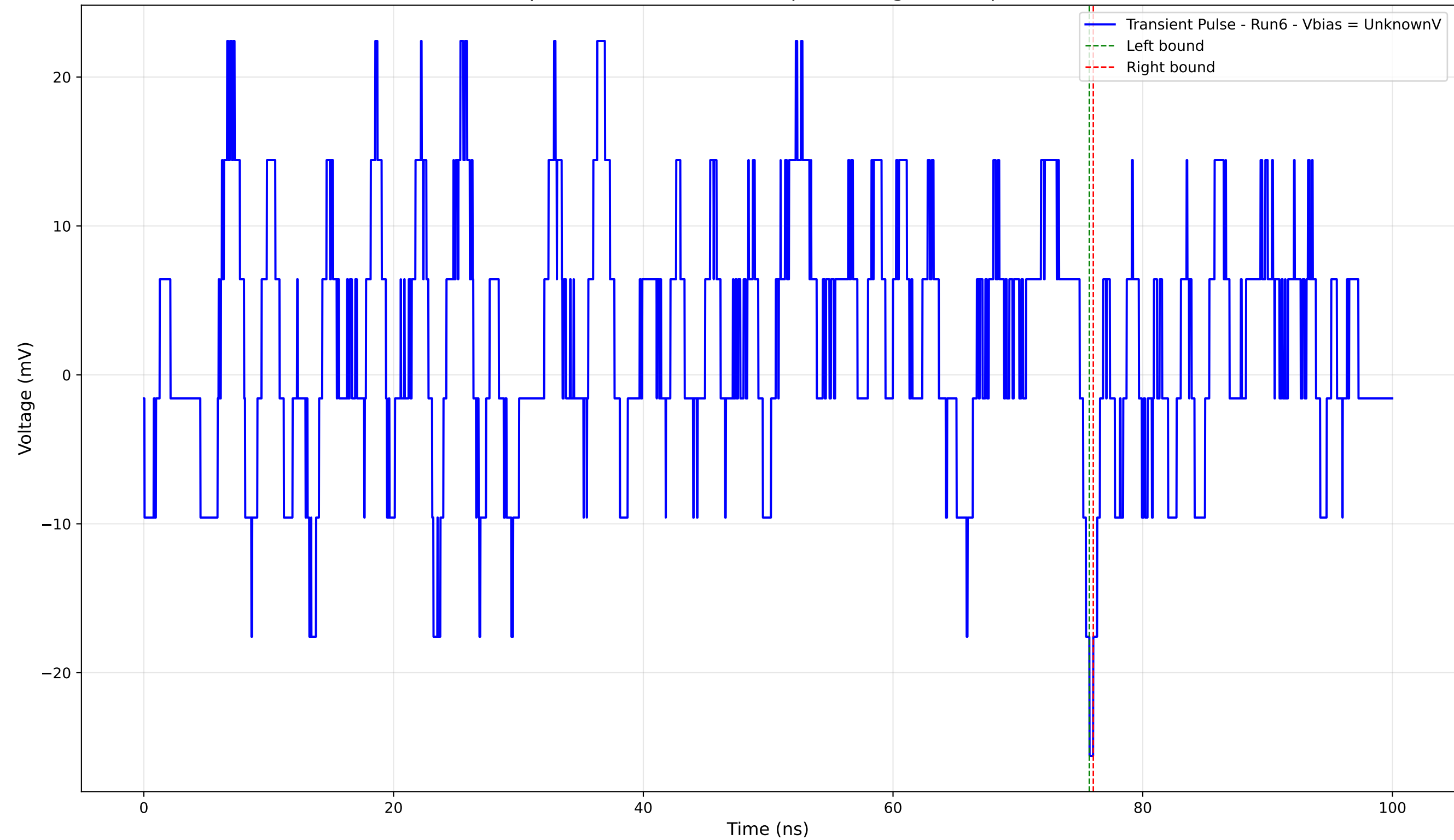
Transient Pulse - Sample: 4004 - Position: 65.0 \mu\text{m} - Charge: -0.16 pC - Rise Time: 0.52 ns
