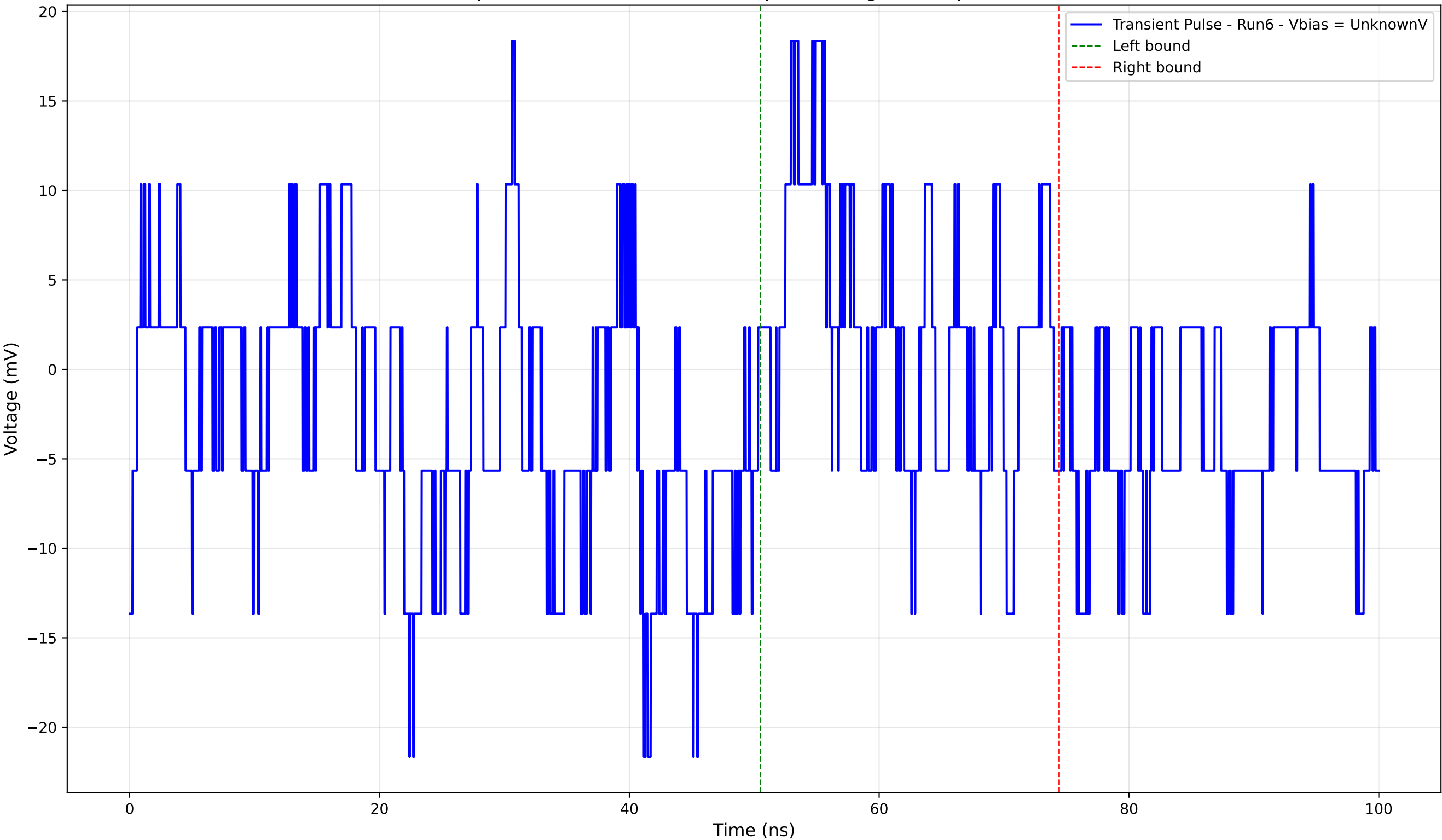
Transient Pulse - Sample: 4004 - Position: 1165.0 \mu\text{m} - Charge: 1.13 pC - Rise Time: 0.00 ns (N/A)
