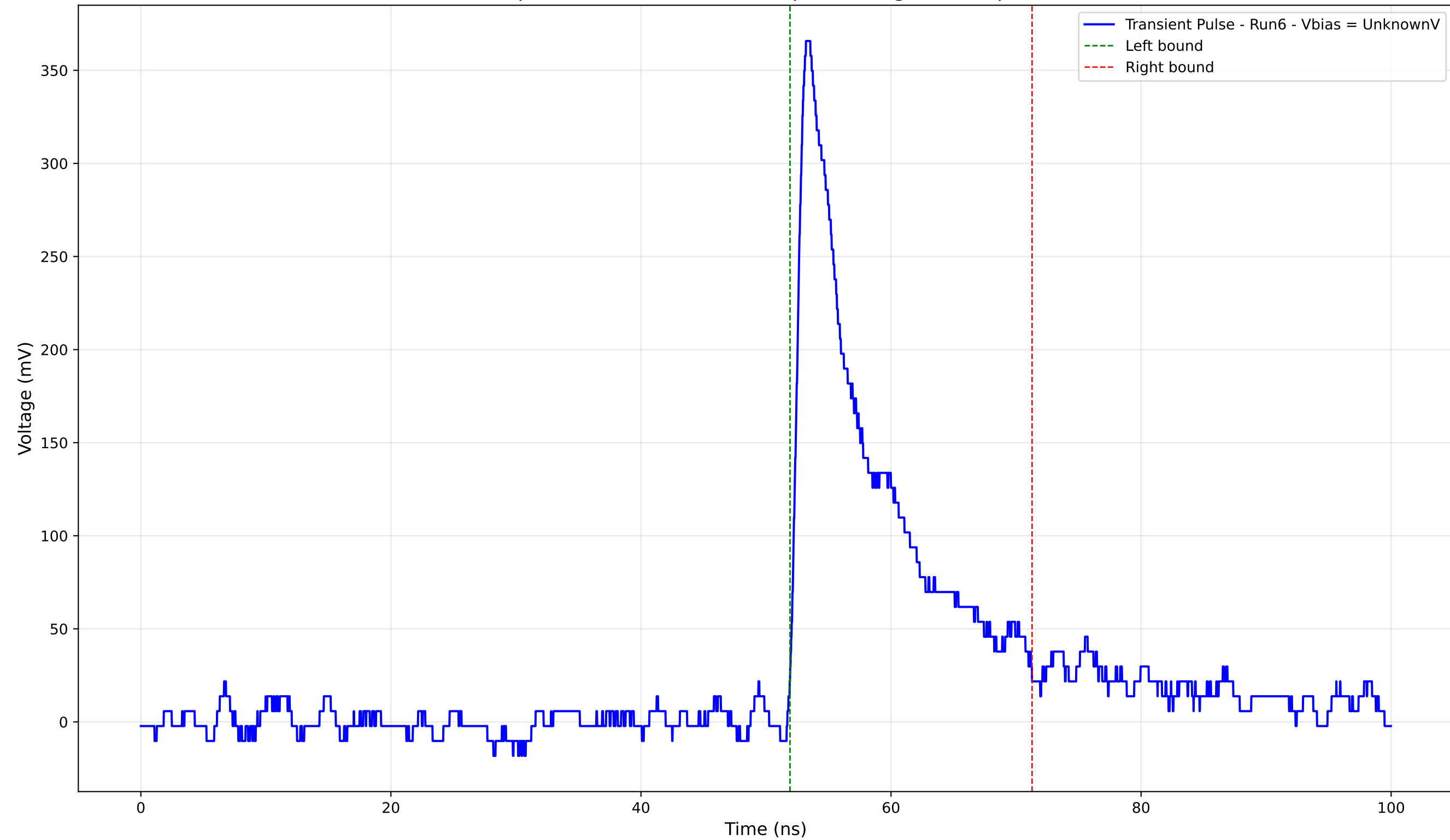
Transient Pulse - Sample: 4004 - Position: 570.0 \mu\text{m} - Charge: 49.06 pC - Rise Time: 0.98 ns
