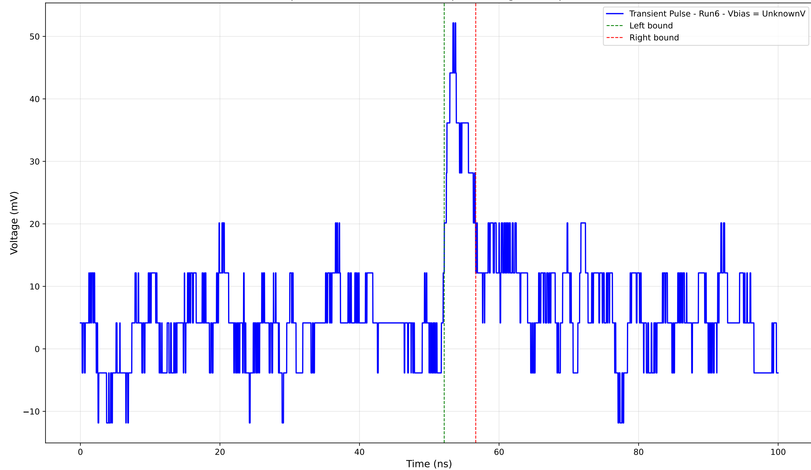
Transient Pulse - Sample: 4004 - Position: 1120.0 \mu\text{m} - Charge: 3.09 pC - Rise Time: 1.42 ns
