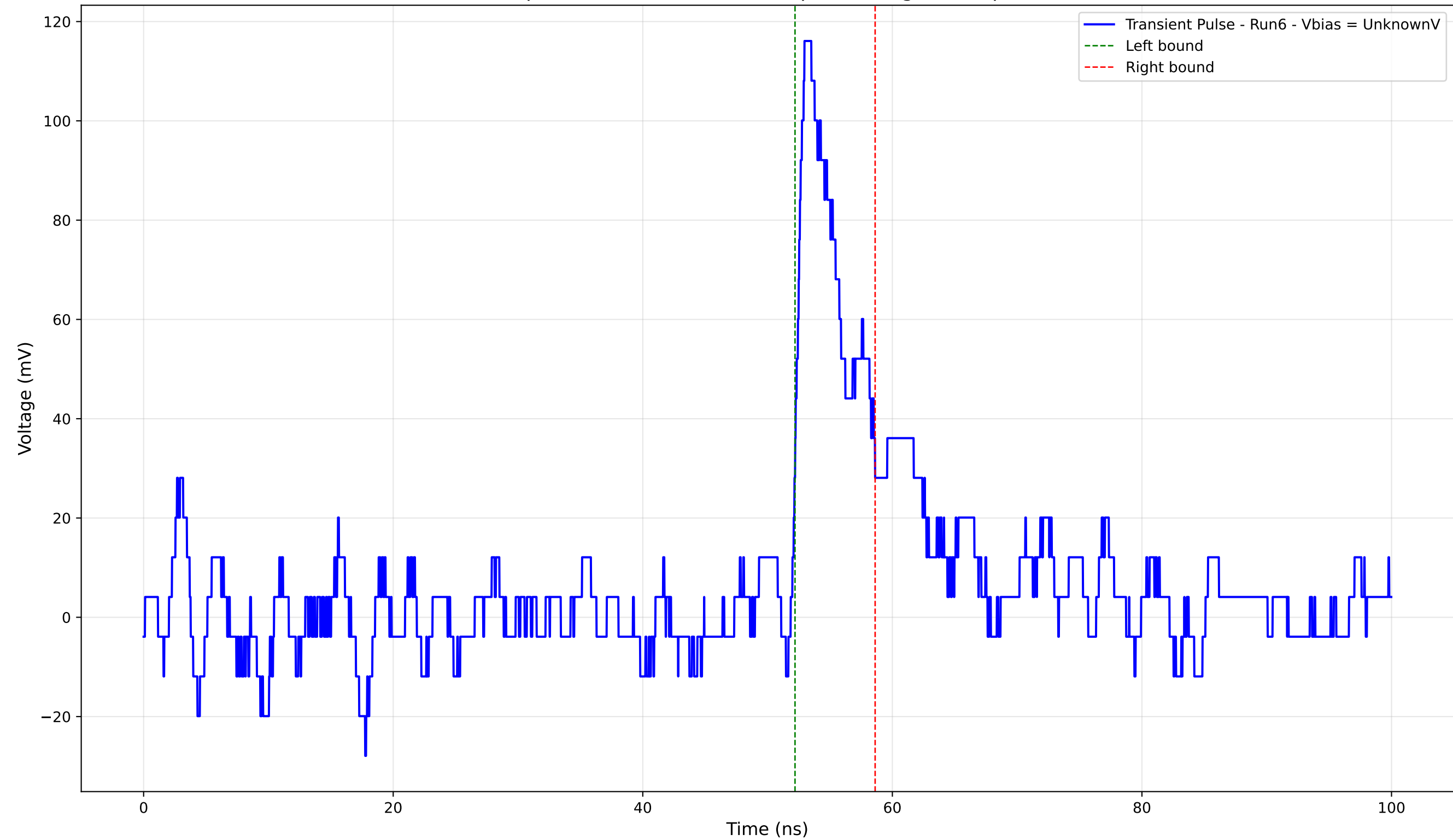
Transient Pulse - Sample: 4004 - Position: 510.0 \mu\text{m} - Charge: 9.20 pC - Rise Time: 0.90 ns
