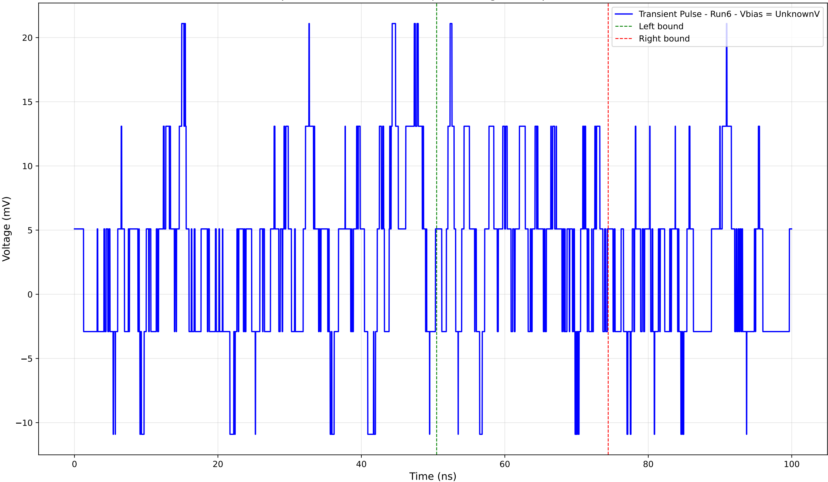
Transient Pulse - Sample: 4004 - Position: 10.0 \mu\text{m} - Charge: 2.13 pC - Rise Time: 0.00 ns (N/A)
