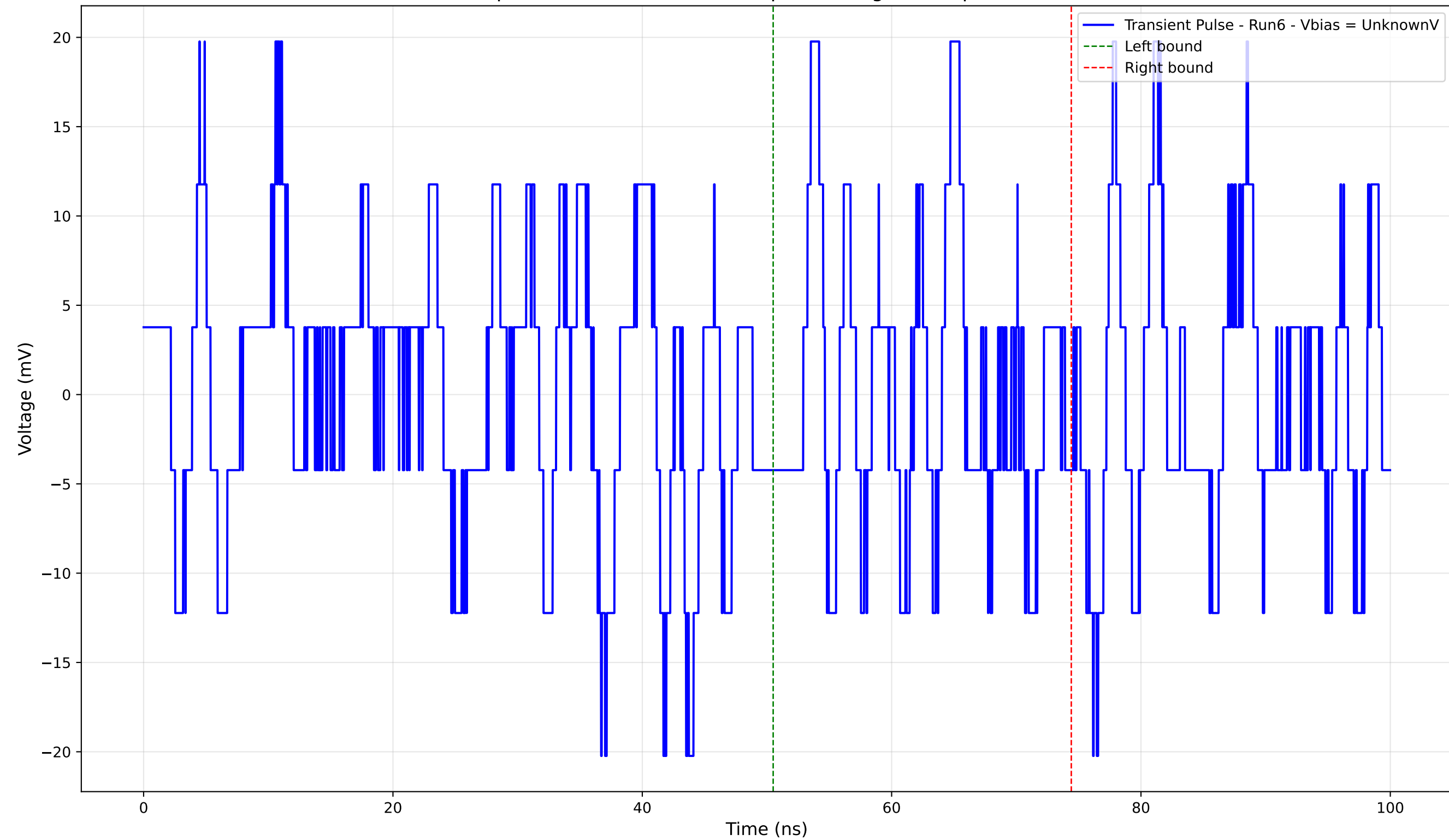
Transient Pulse - Sample: 4004 - Position: 400.0 \mu\text{m} - Charge: 0.09 pC - Rise Time: 0.00 ns (N/A)
