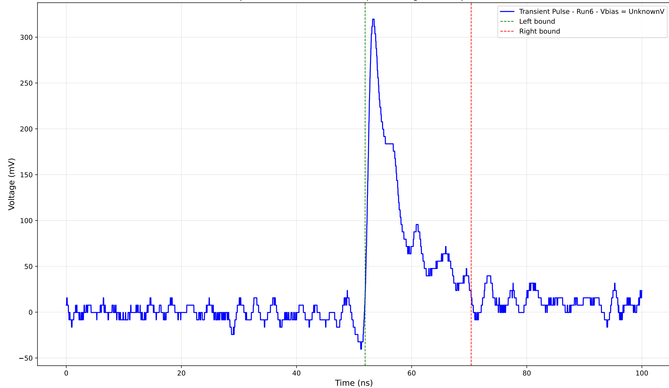
Transient Pulse - Sample: 4004 - Position: 675.0 \mu\text{m} - Charge: 38.38 pC - Rise Time: 0.96 ns
