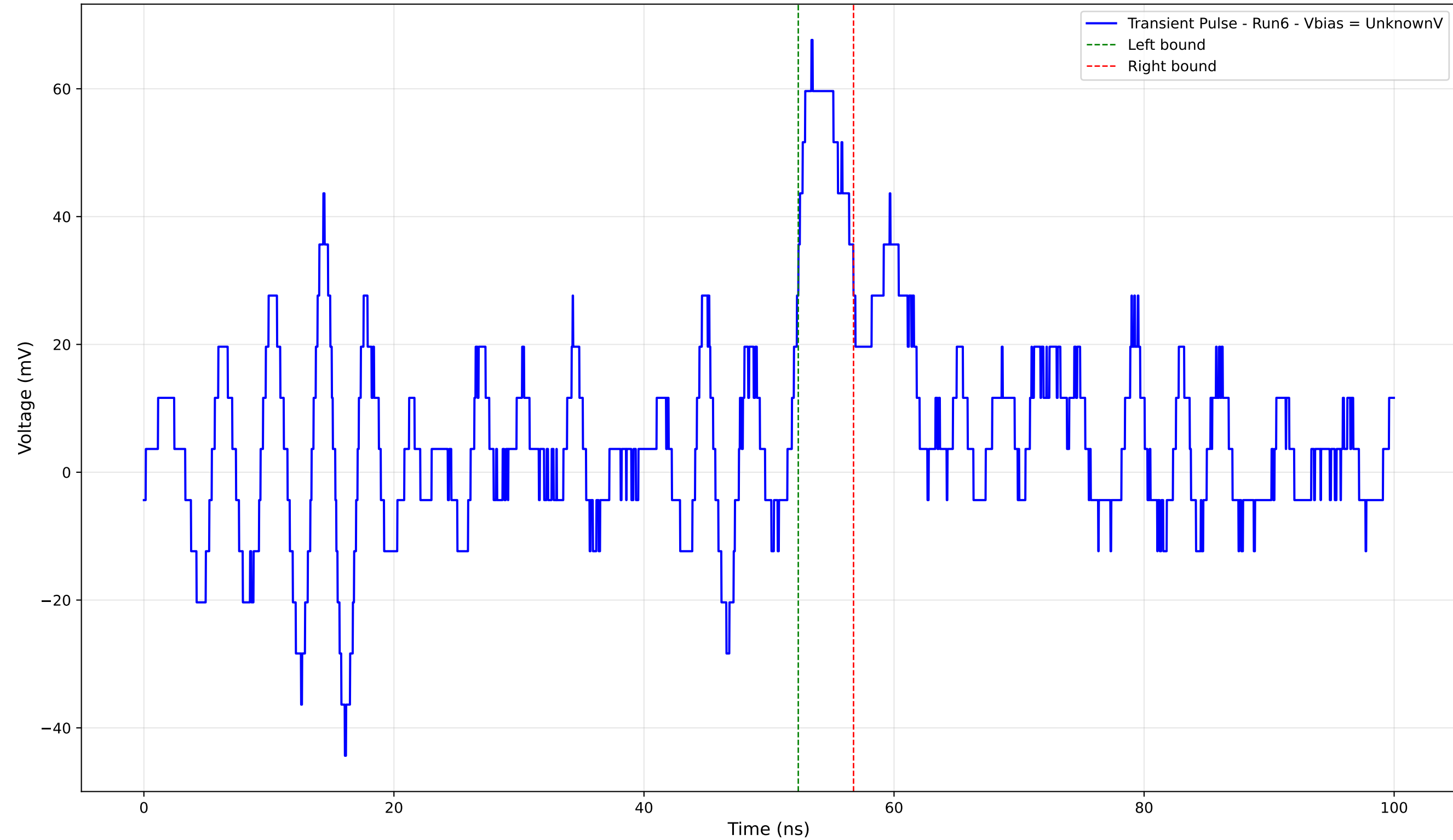
Transient Pulse - Sample: 4004 - Position: 835.0 \mu\text{m} - Charge: 4.62 pC - Rise Time: 1.57 ns
