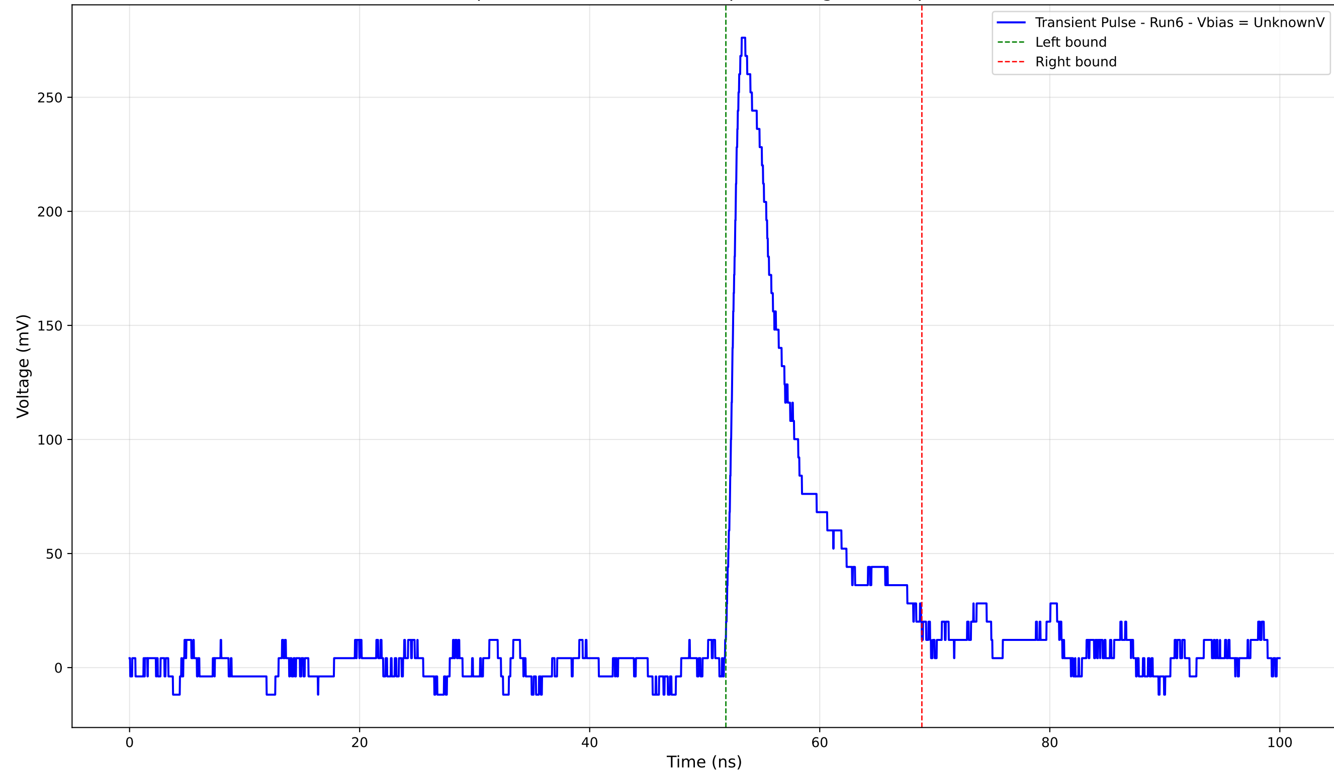
Transient Pulse - Sample: 4004 - Position: 735.0 \mu\text{m} - Charge: 32.82 pC - Rise Time: 1.02 ns
