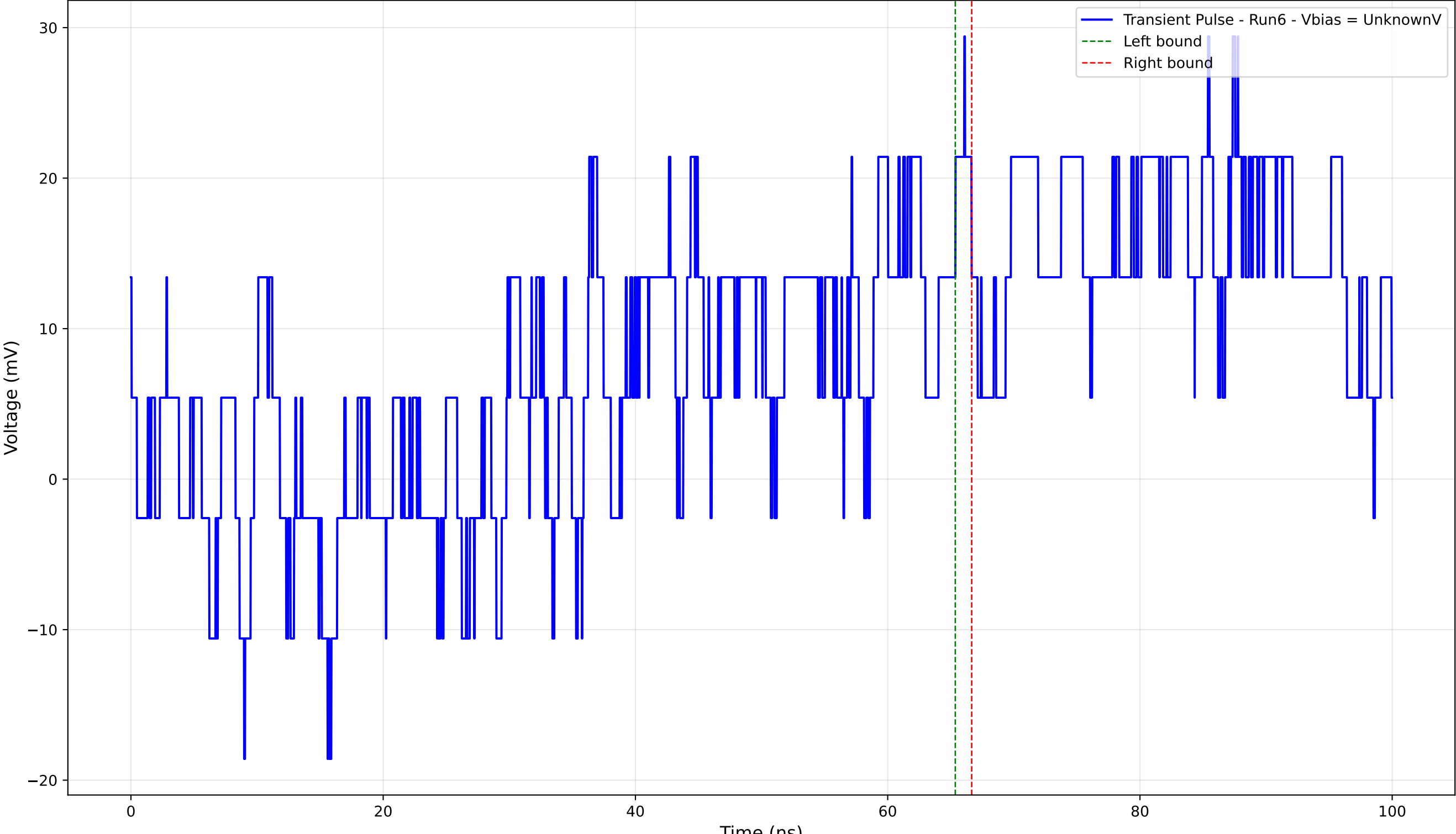
Transient Pulse - Sample: 4004 - Position: 230.0 \mu\text{m} - Charge: 0.56 pC - Rise Time: 7.50 ns
