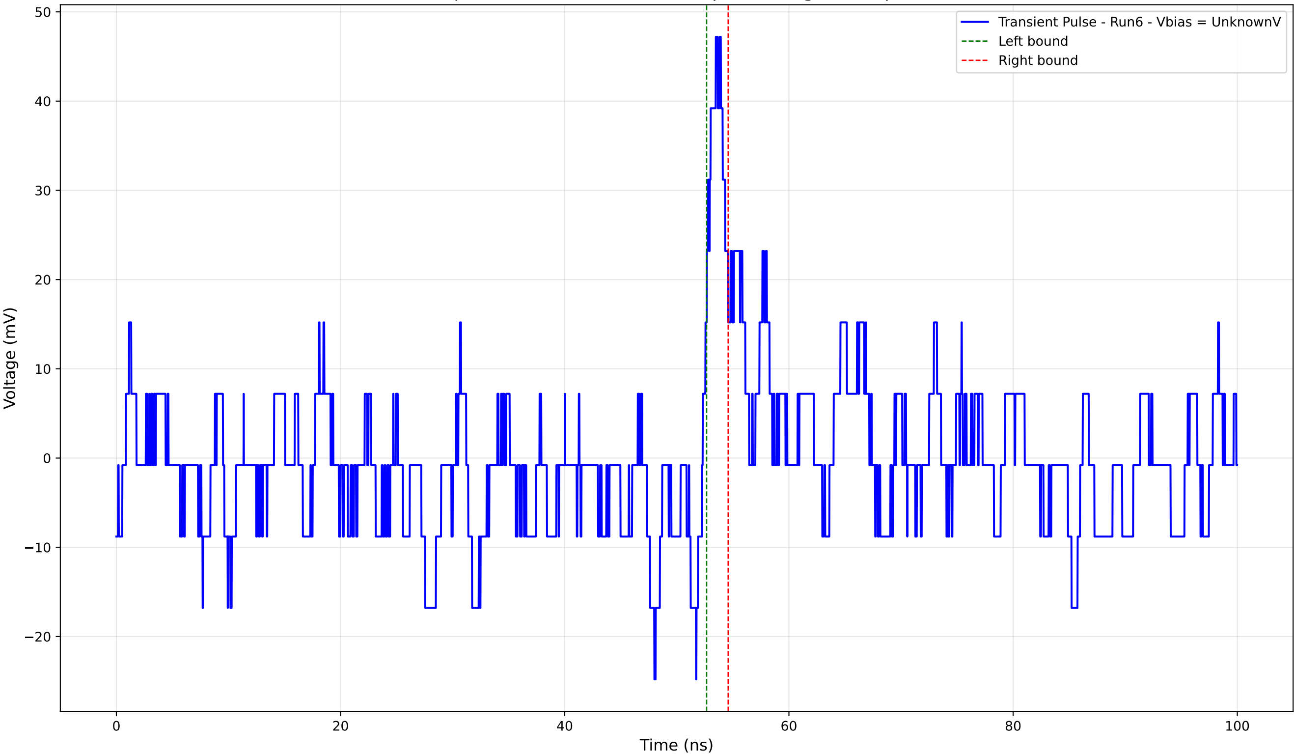
Transient Pulse - Sample: 4004 - Position: 1105.0 \mu\text{m} - Charge: 1.35 pC - Rise Time: 1.17 ns
