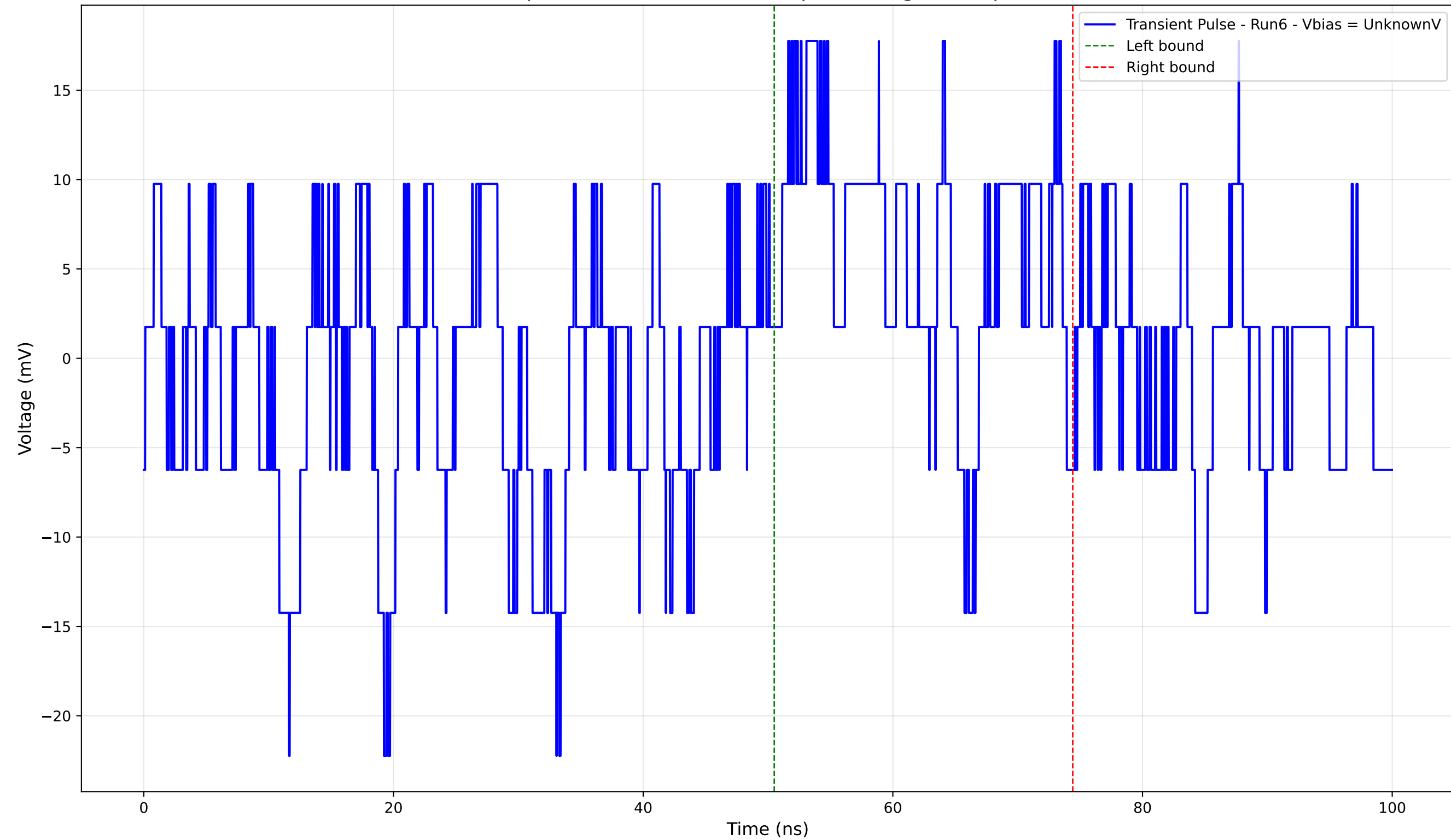
Transient Pulse - Sample: 4004 - Position: 445.0 \mu\text{m} - Charge: 2.95 pC - Rise Time: 1.14 ns
