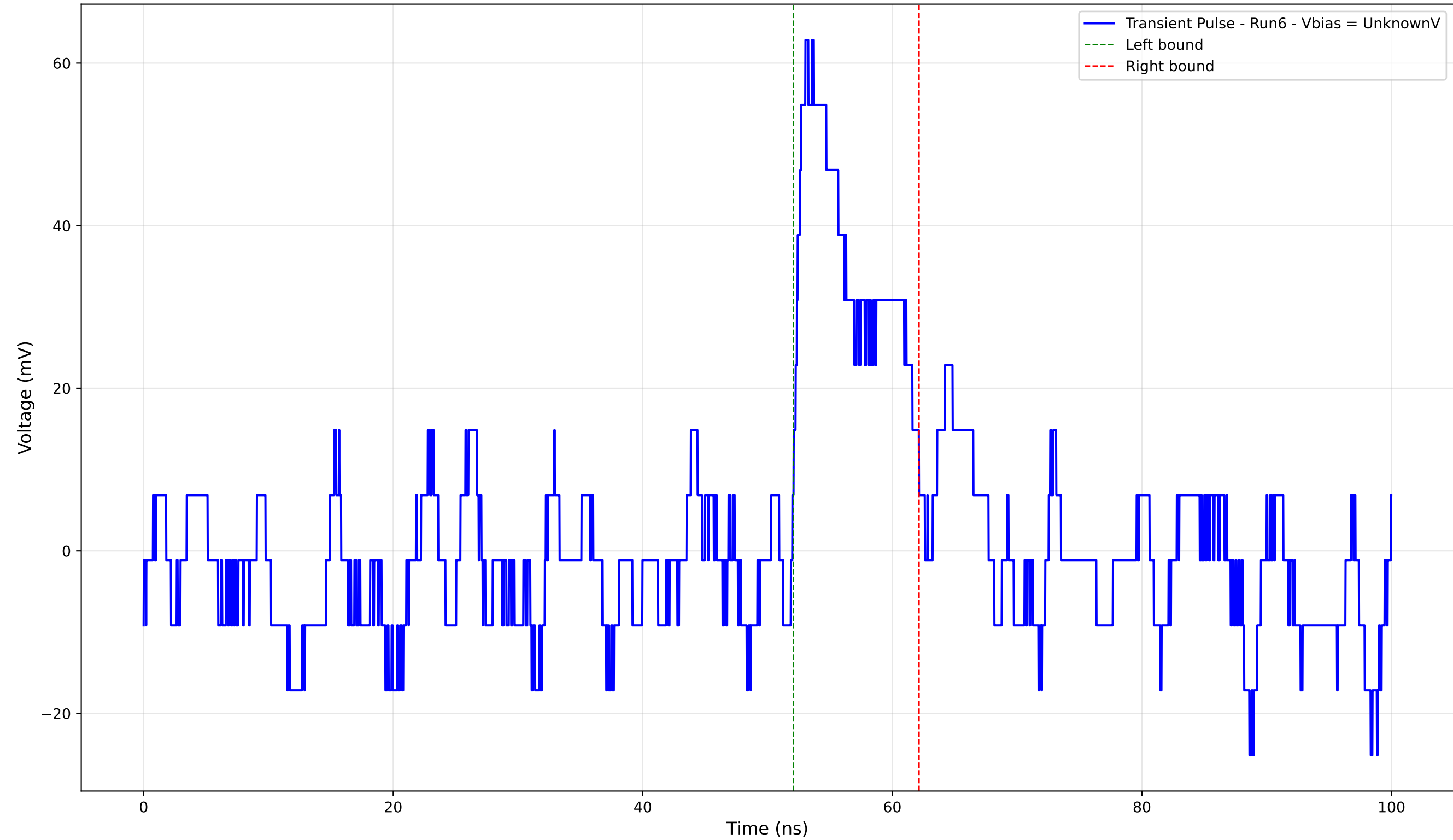
Transient Pulse - Sample: 4004 - Position: 960.0 \mu\text{m} - Charge: 7.24 pC - Rise Time: 1.04 ns
