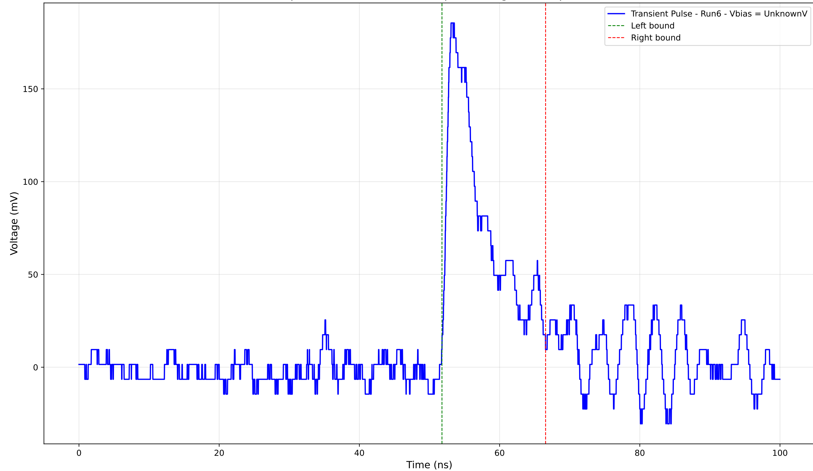
Transient Pulse - Sample: 4004 - Position: 780.0 \mu\text{m} - Charge: 23.07 pC - Rise Time: 1.02 ns
