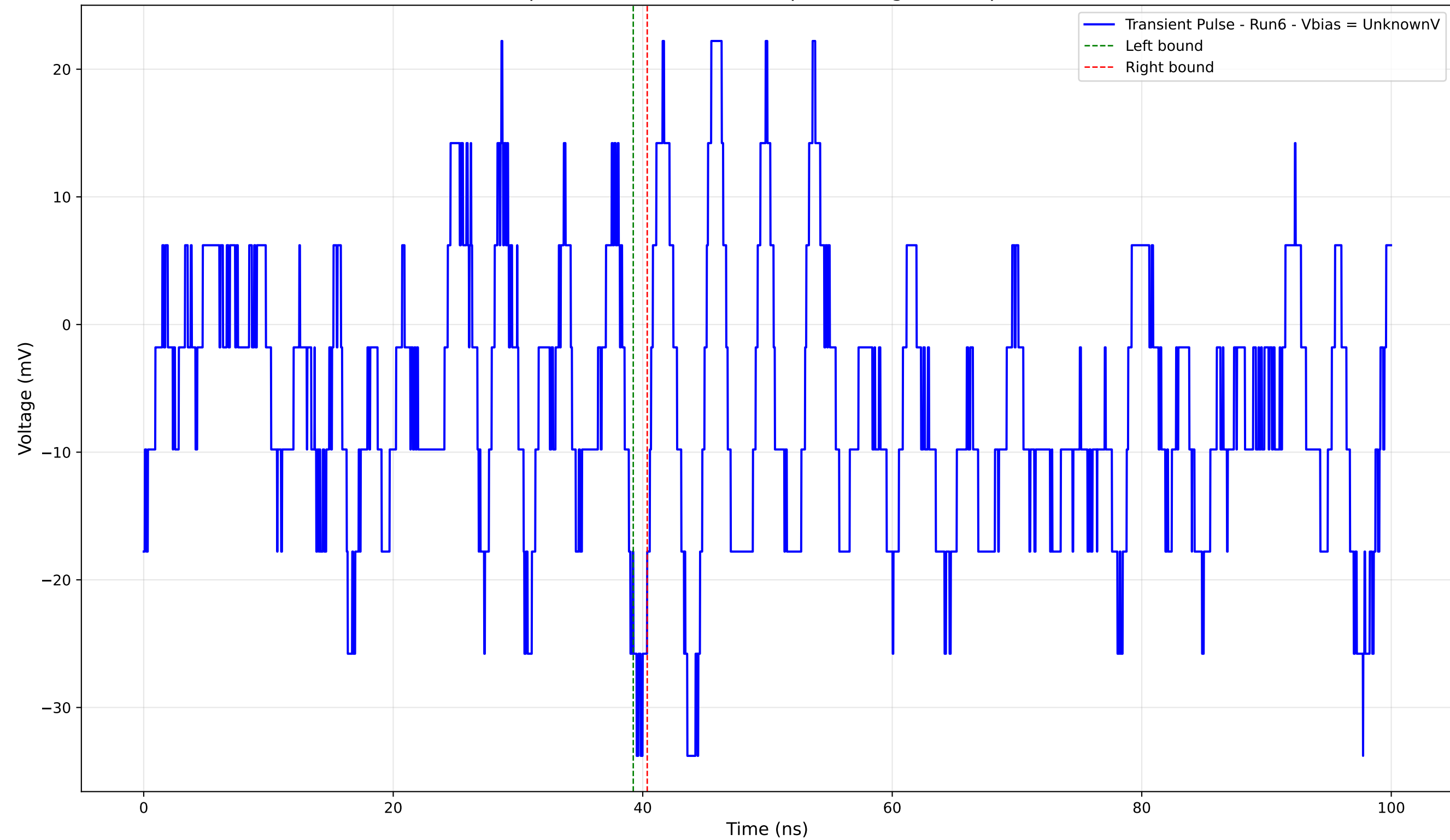
Transient Pulse - Sample: 4004 - Position: 20.0 \mu\text{m} - Charge: -0.62 pC - Rise Time: 0.98 ns
