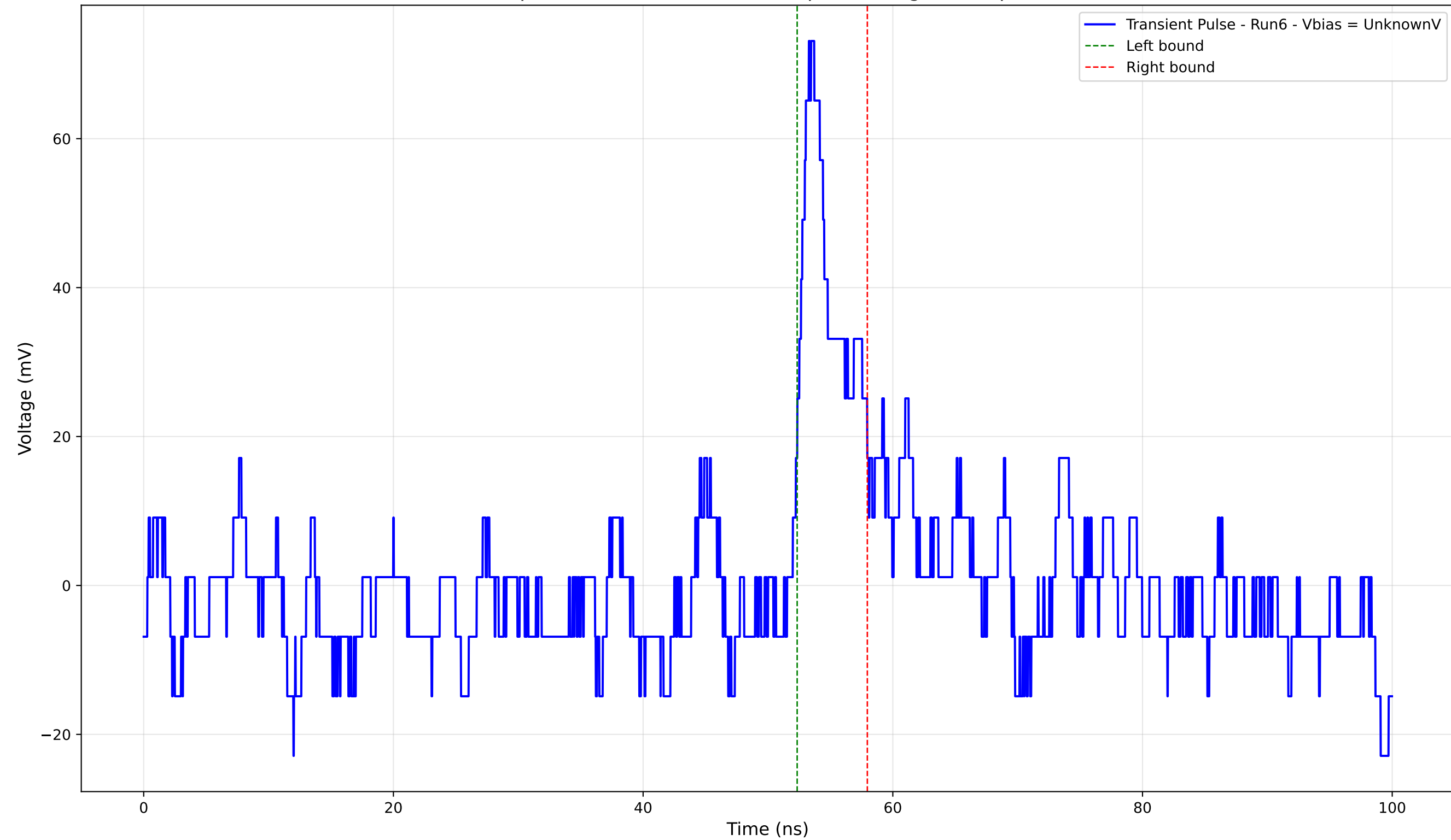
Transient Pulse - Sample: 4004 - Position: 1025.0 \mu\text{m} - Charge: 4.62 pC - Rise Time: 1.28 ns
