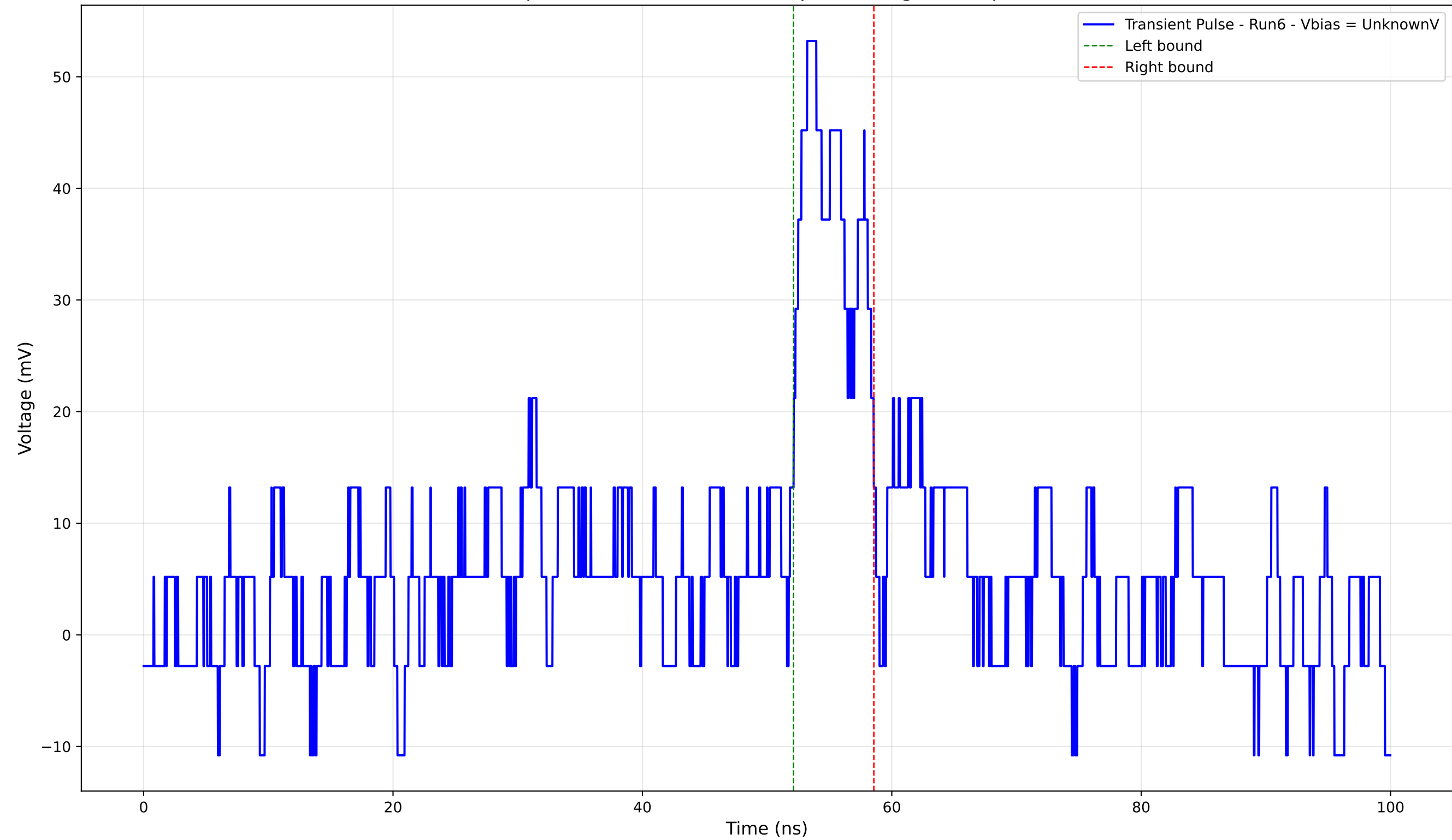
Transient Pulse - Sample: 4004 - Position: 845.0 \mu\text{m} - Charge: 4.91 pC - Rise Time: 1.40 ns
