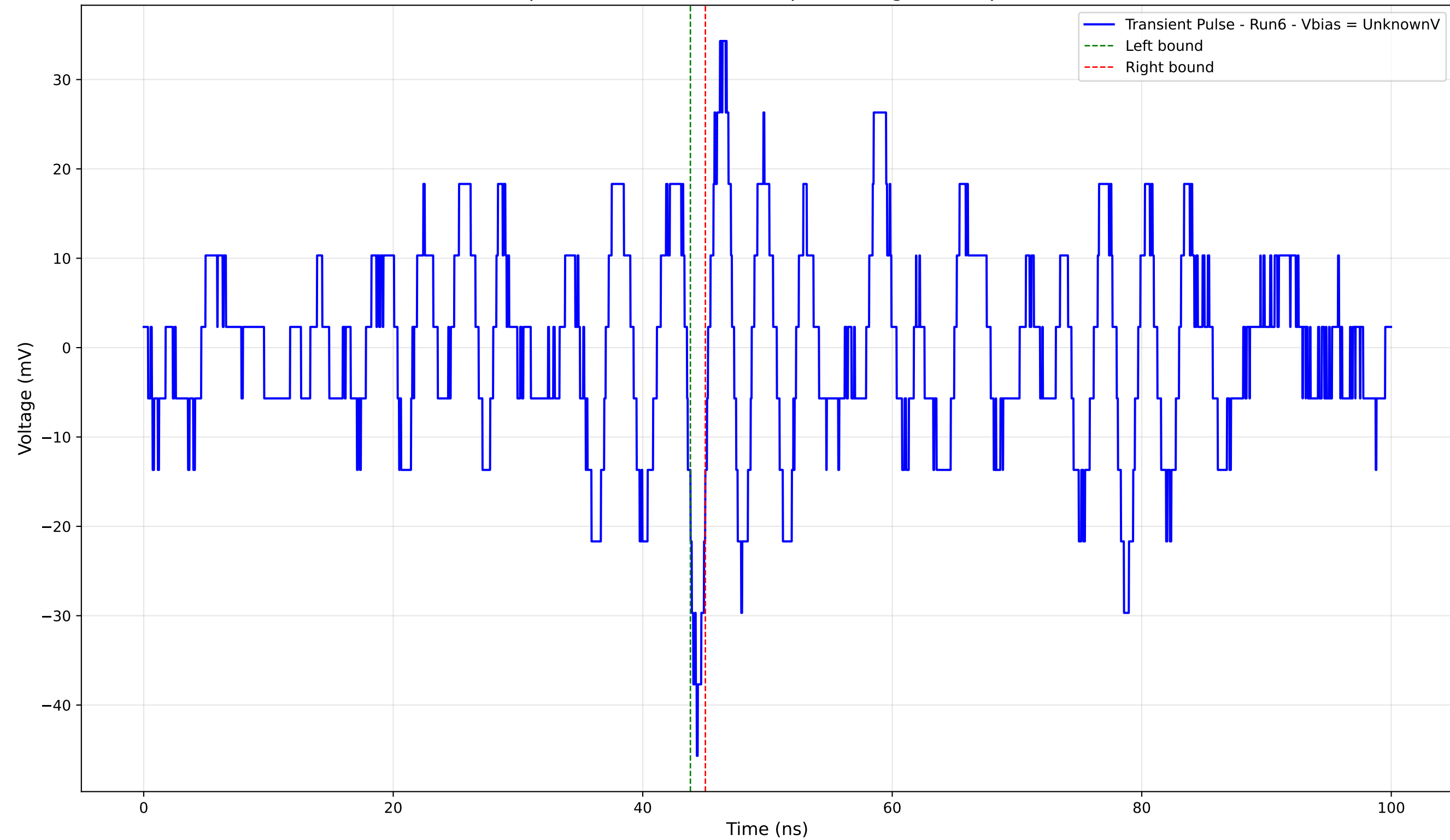
Transient Pulse - Sample: 4004 - Position: 50.0 \mu\text{m} - Charge: -0.78 pC - Rise Time: 0.79 ns
