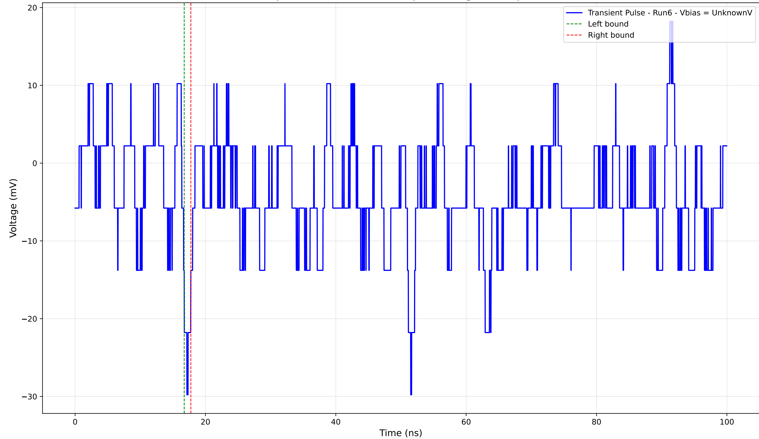
Transient Pulse - Sample: 4004 - Position: 30.0 \mu\text{m} - Charge: -0.47 pC - Rise Time: 0.80 ns
