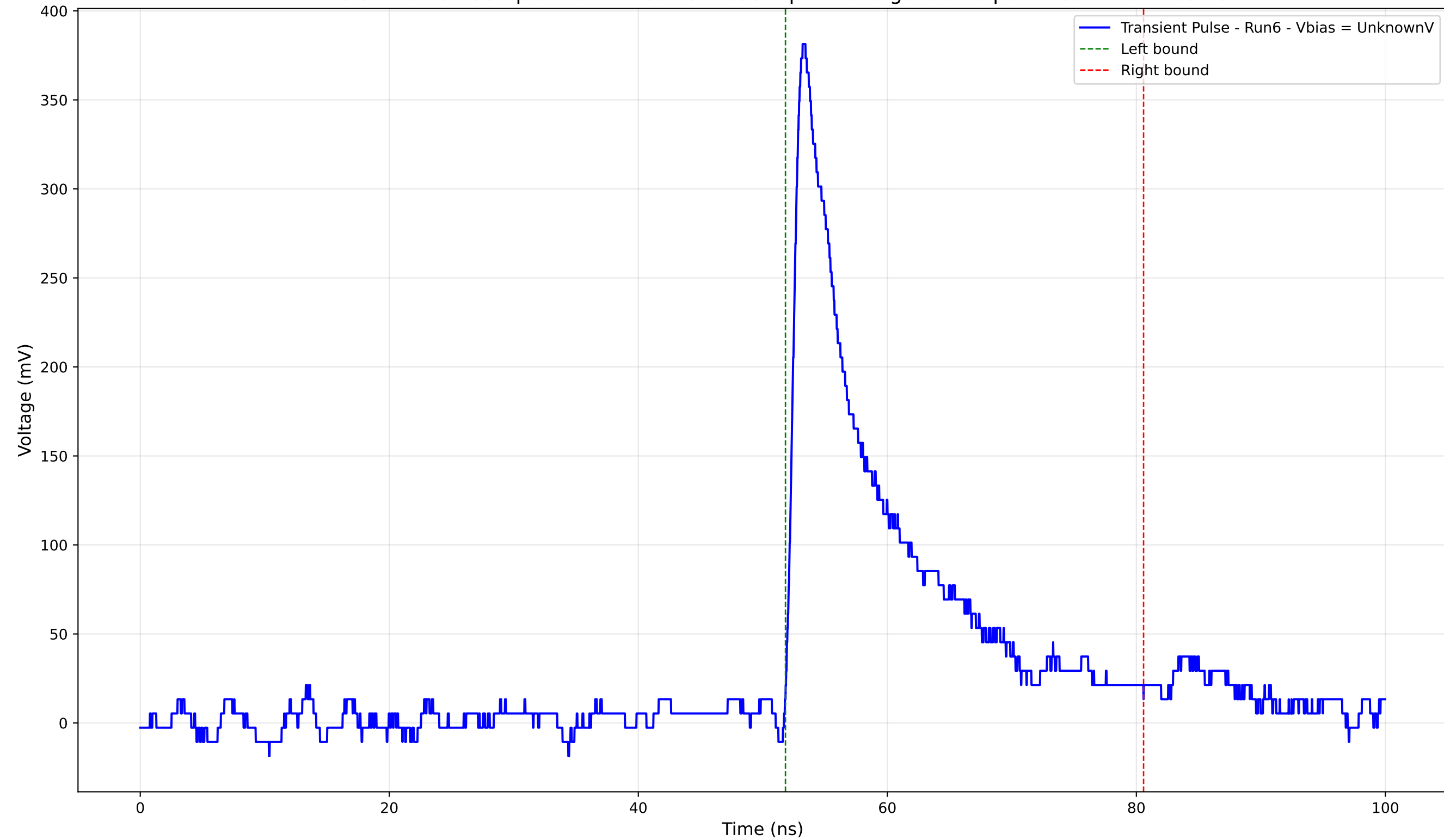
Transient Pulse - Sample: 4004 - Position: 655.0 \mu\text{m} - Charge: 56.16 pC - Rise Time: 1.00 ns
