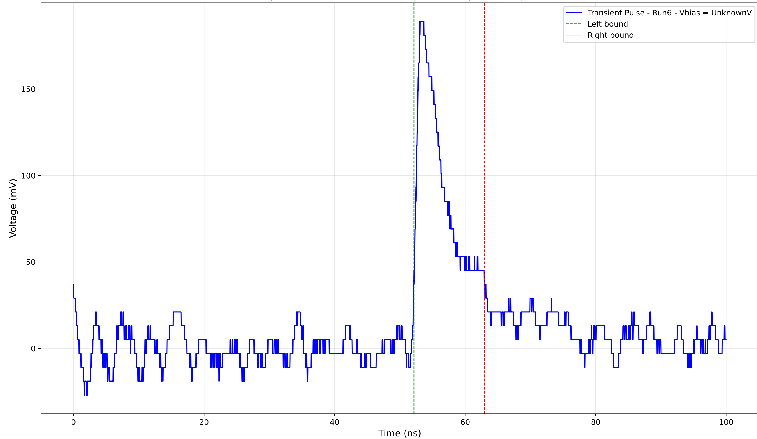
Transient Pulse - Sample: 4004 - Position: 775.0 \mu\text{m} - Charge: 19.92 pC - Rise Time: 0.97 ns
