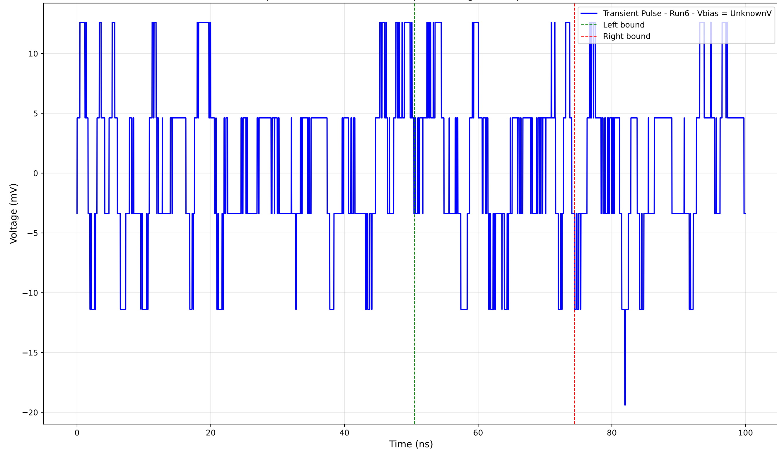
Transient Pulse - Sample: 4004 - Position: 320.0 \mu\text{m} - Charge: 0.46 pC - Rise Time: 0.00 ns (N/A)
