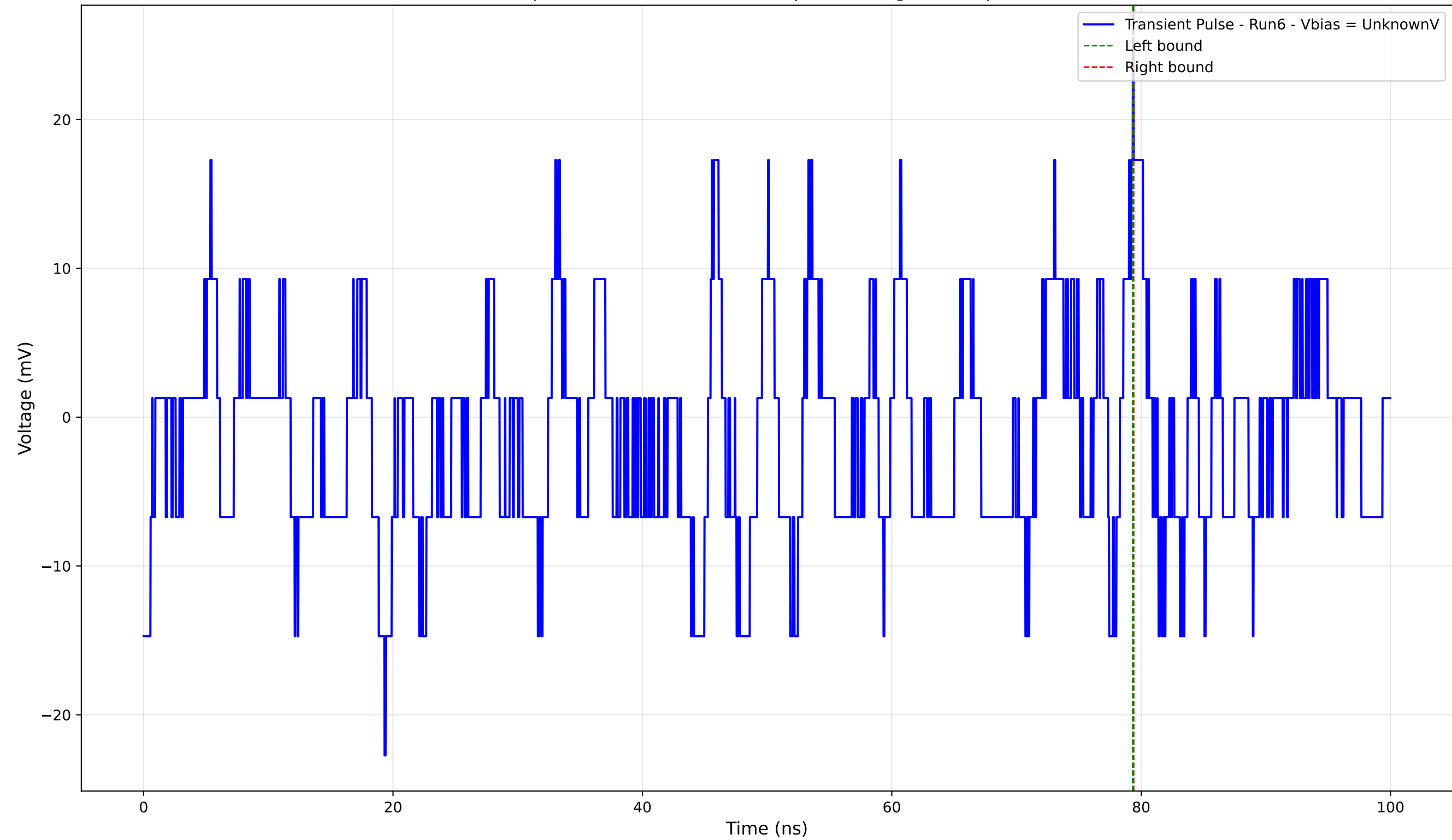
Transient Pulse - Sample: 4004 - Position: 90.0 \mu\text{m} - Charge: 0.04 pC - Rise Time: 0.78 ns
