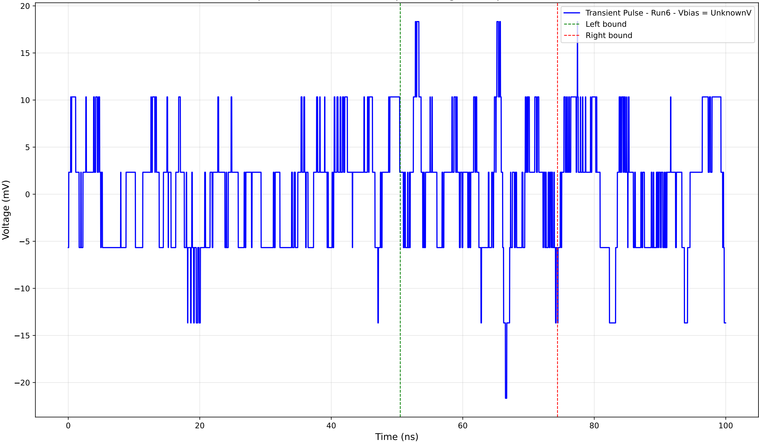
Transient Pulse - Sample: 4004 - Position: 35.0 \mu\text{m} - Charge: 0.31 pC - Rise Time: 0.00 ns (N/A)
