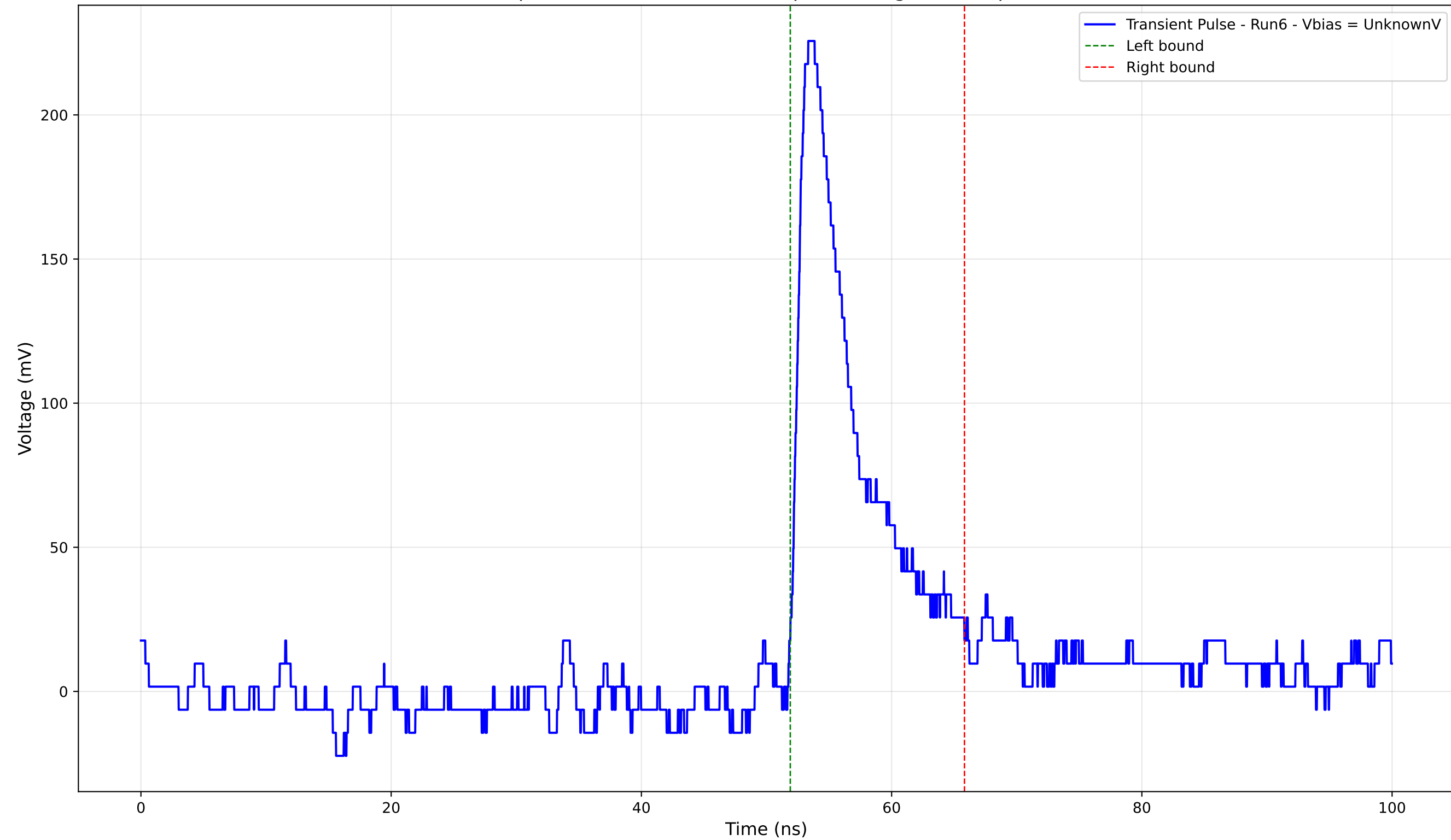
Transient Pulse - Sample: 4004 - Position: 750.0 \mu\text{m} - Charge: 24.54 pC - Rise Time: 1.11 ns
