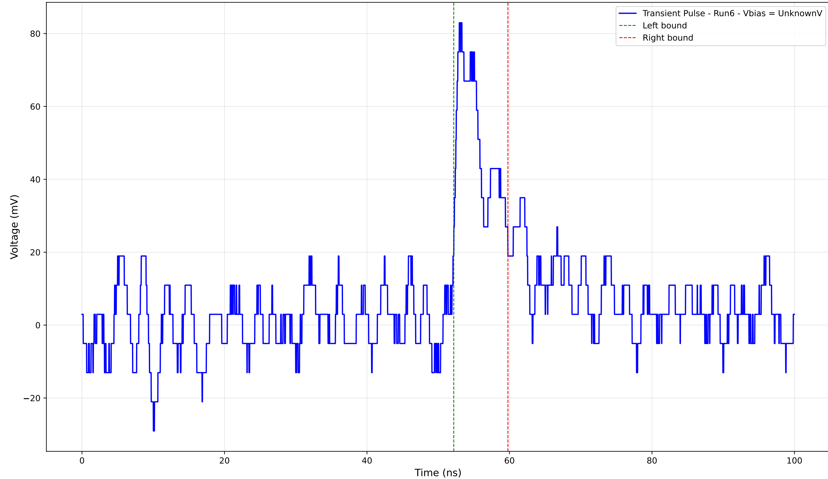
Transient Pulse - Sample: 4004 - Position: 830.0 \mu\text{m} - Charge: 7.67 pC - Rise Time: 0.83 ns
