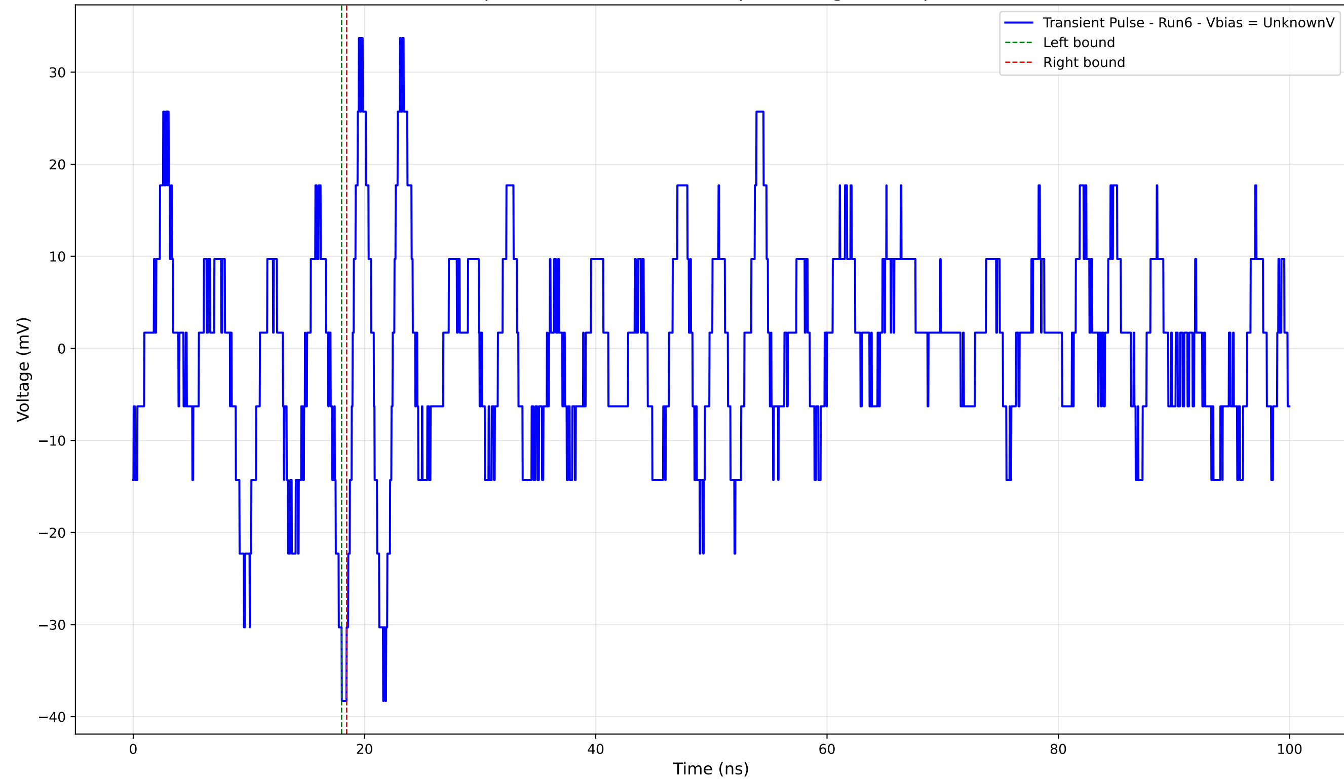
Transient Pulse - Sample: 4004 - Position: 420.0 \mu\text{m} - Charge: -0.33 pC - Rise Time: 0.97 ns
