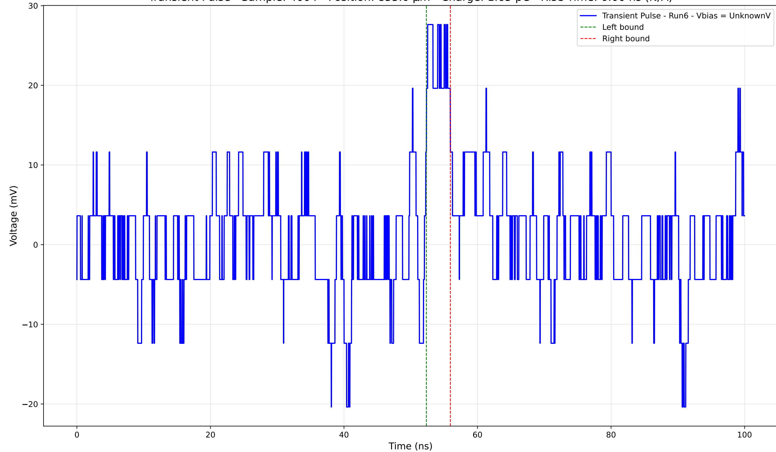
Transient Pulse - Sample: 4004 - Position: 855.0 \mu\text{m} - Charge: 1.65 pC - Rise Time: 0.00 ns (N/A)
