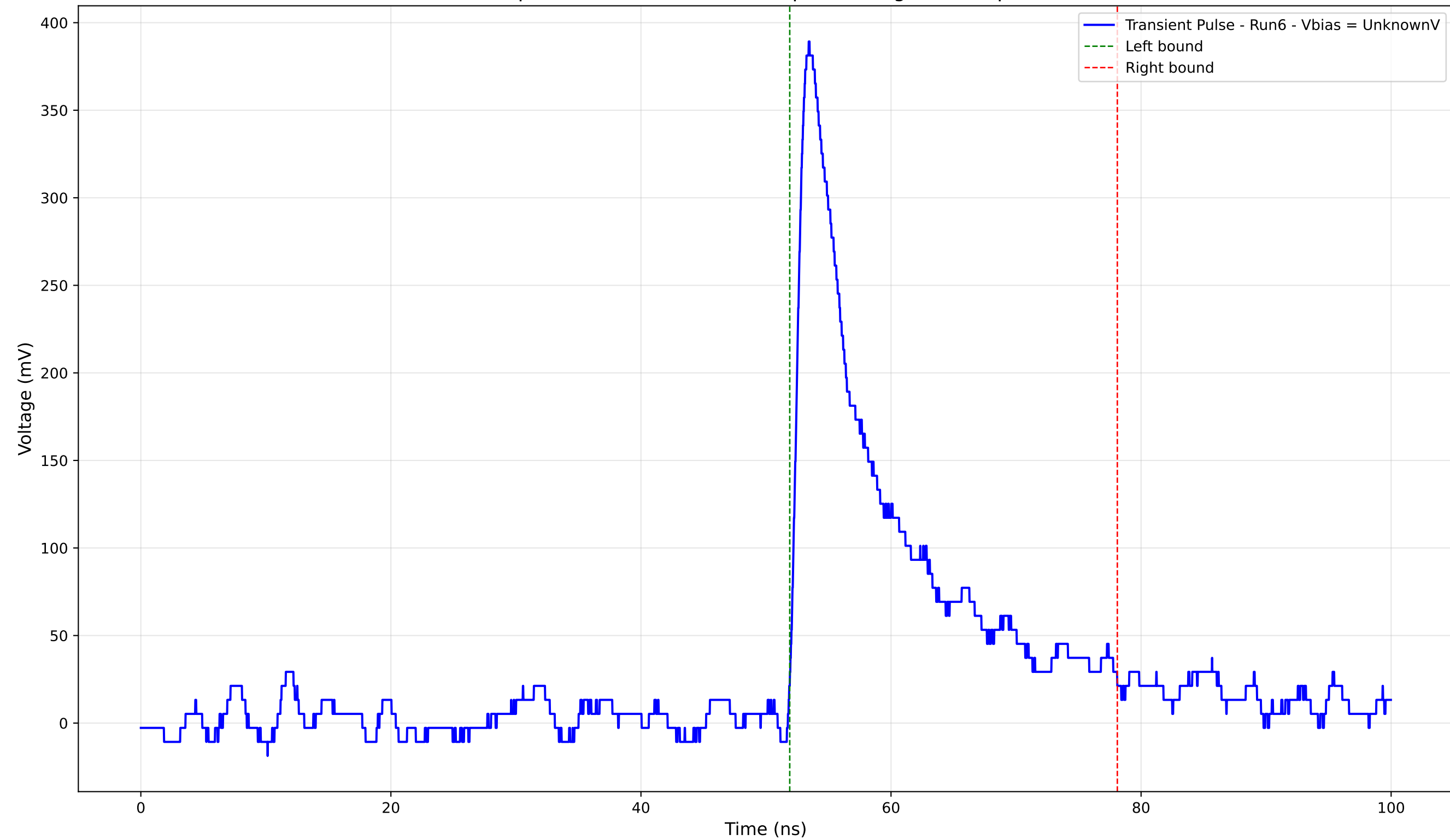
Transient Pulse - Sample: 4004 - Position: 545.0 \mu\text{m} - Charge: 57.27 pC - Rise Time: 1.06 ns
