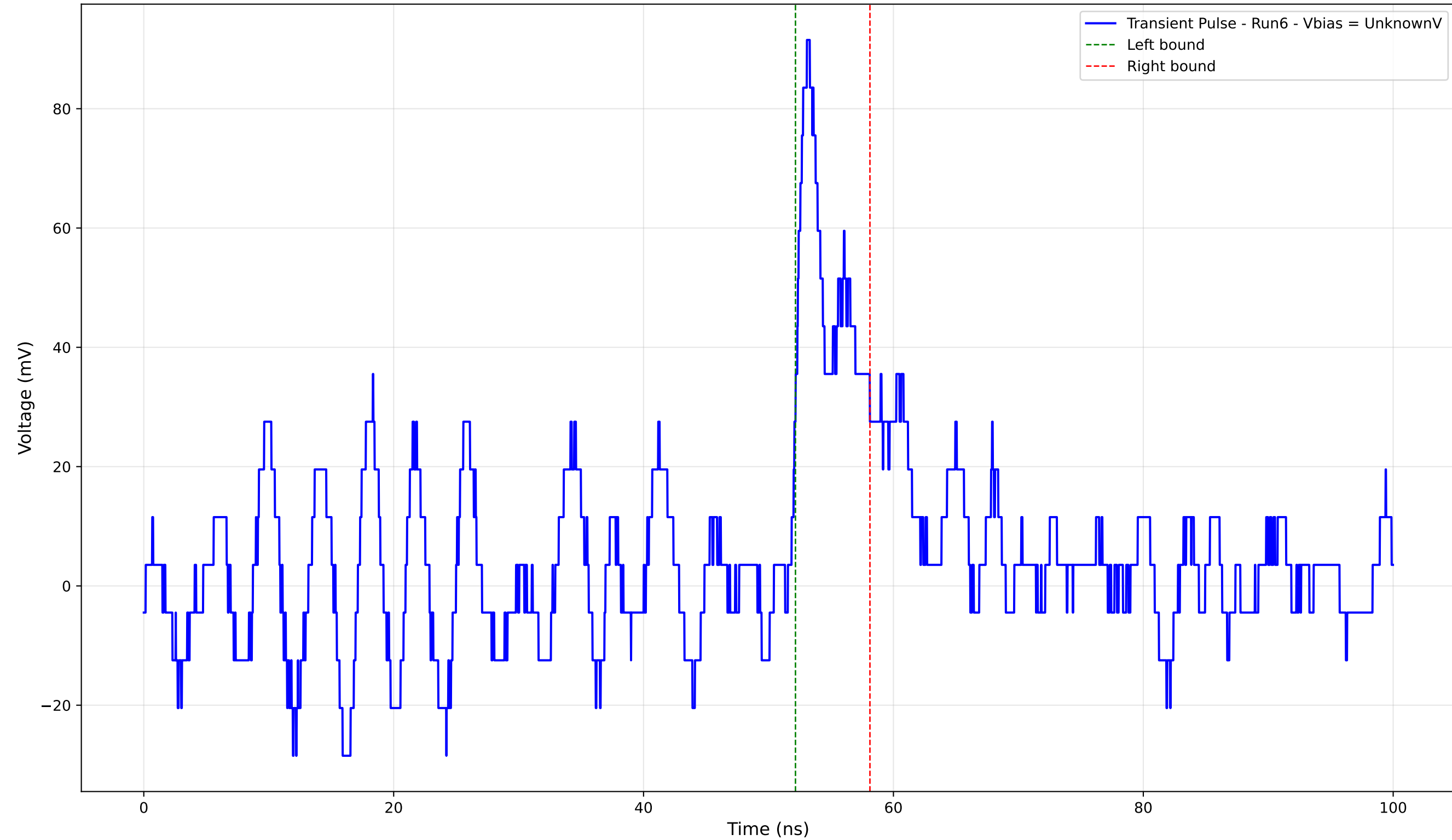
Transient Pulse - Sample: 4004 - Position: 995.0 \mu\text{m} - Charge: 6.14 pC - Rise Time: 0.93 ns
