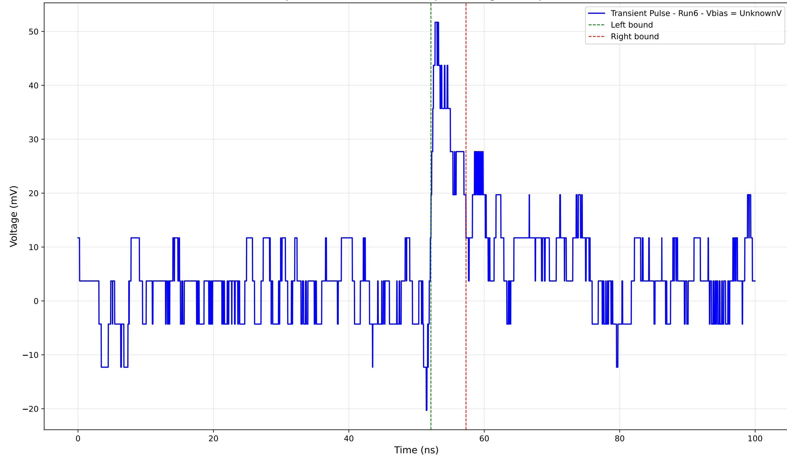
Transient Pulse - Sample: 4004 - Position: 495.0 \mu\text{m} - Charge: 3.42 pC - Rise Time: 0.72 ns
