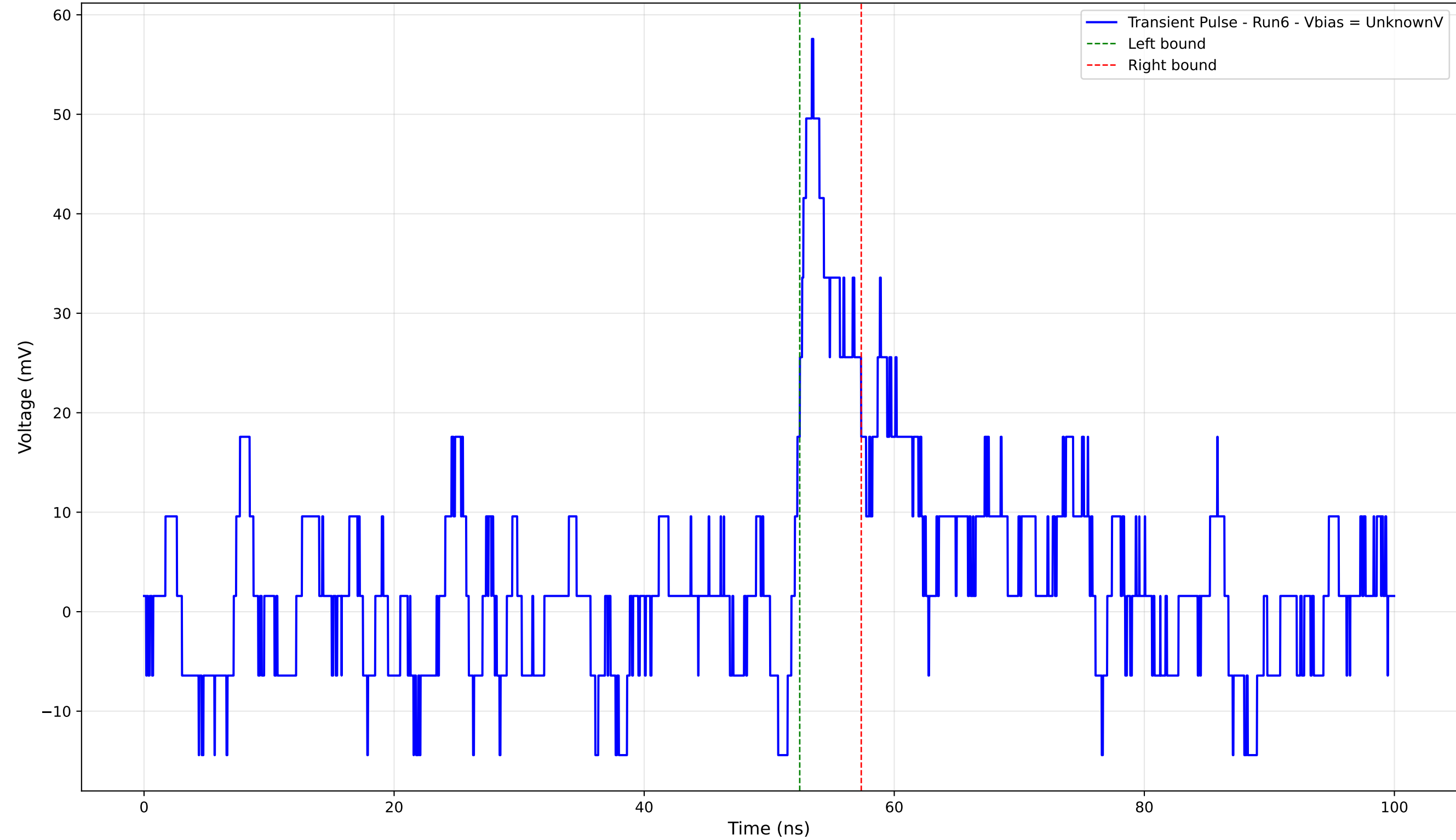
Transient Pulse - Sample: 4004 - Position: 875.0 \mu\text{m} - Charge: 3.48 pC - Rise Time: 1.37 ns
