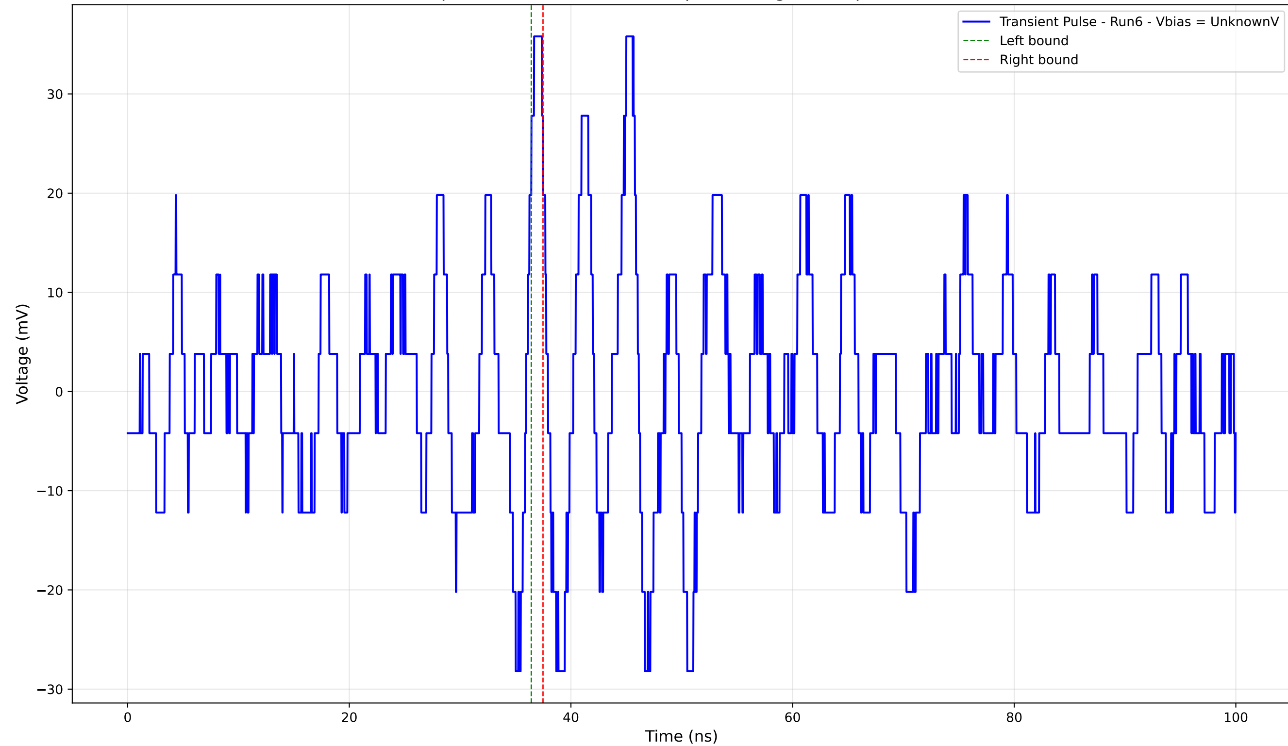
Transient Pulse - Sample: 4004 - Position: 270.0 \mu\text{m} - Charge: 0.70 pC - Rise Time: 0.00 ns (N/A)
