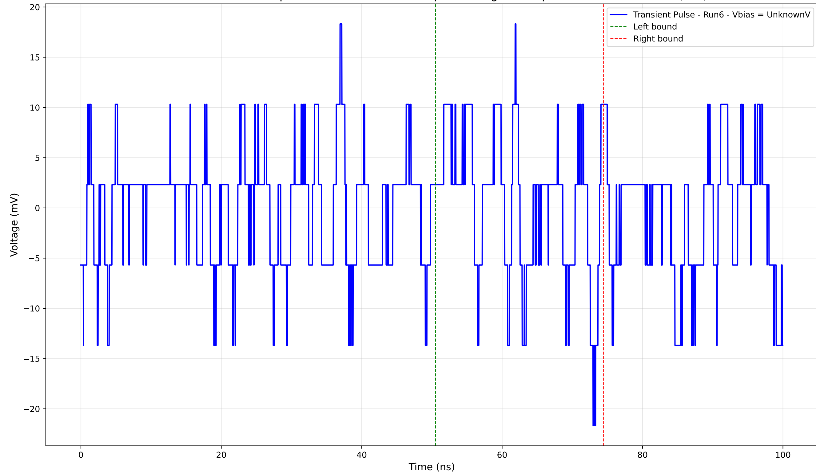
Transient Pulse - Sample: 4004 - Position: 210.0 \mu\text{m} - Charge: 0.30 pC - Rise Time: 0.00 ns (N/A)
