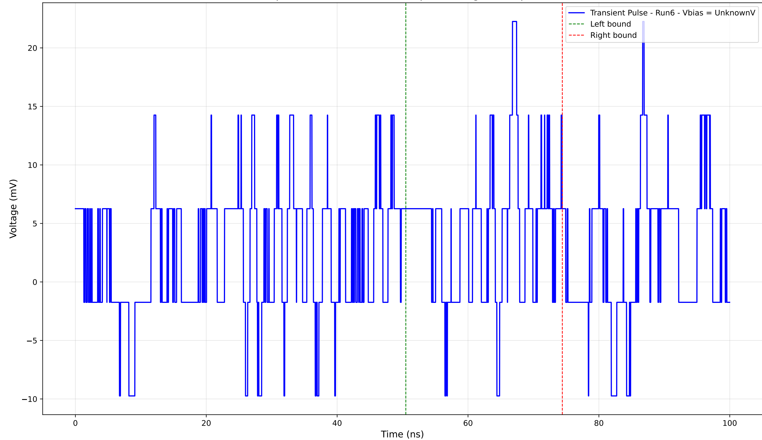
Transient Pulse - Sample: 4004 - Position: 395.0 \mu\text{m} - Charge: 2.14 pC - Rise Time: 0.76 ns
