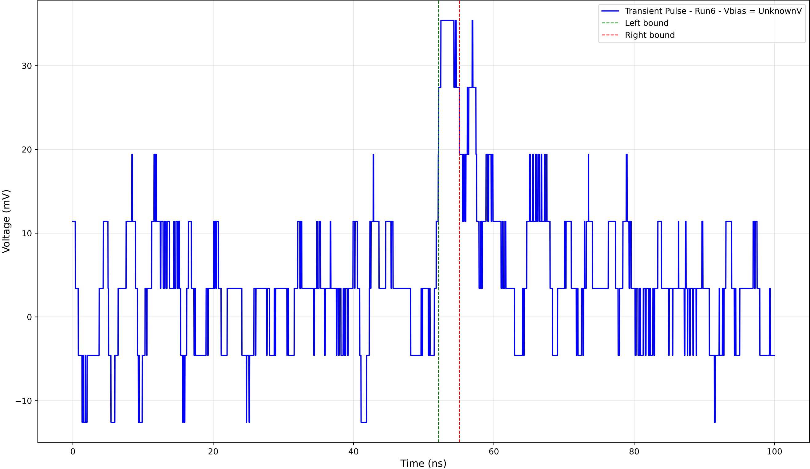
Transient Pulse - Sample: 4004 - Position: 1095.0 \mu\text{m} - Charge: 1.95 pC - Rise Time: 0.68 ns
