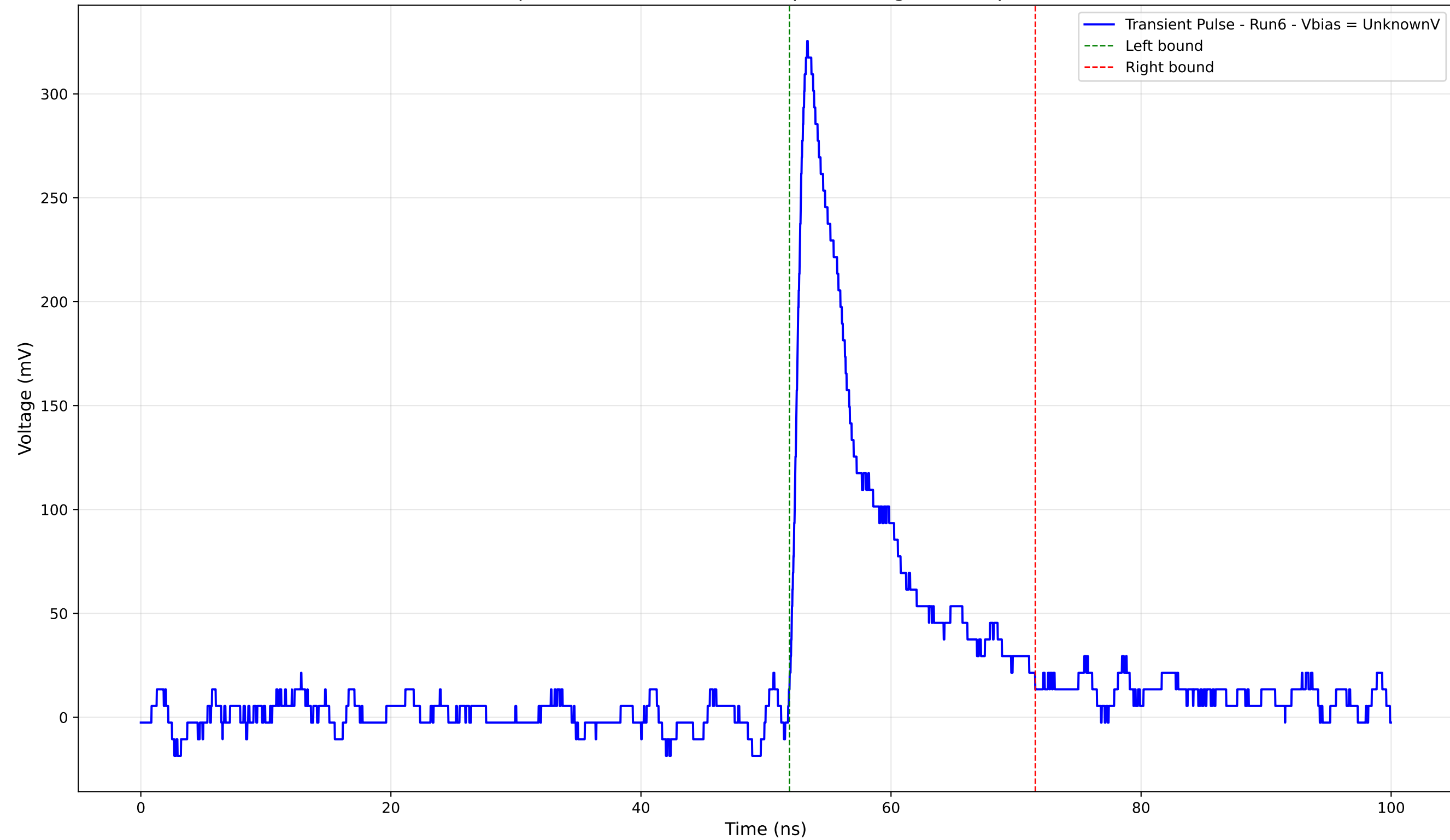
Transient Pulse - Sample: 4004 - Position: 715.0 \mu\text{m} - Charge: 39.46 pC - Rise Time: 0.99 ns
