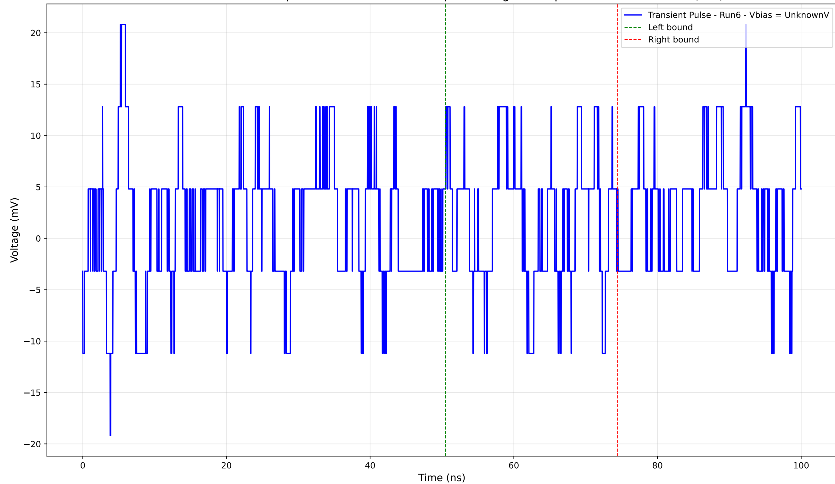
Transient Pulse - Sample: 4004 - Position: 125.0 \mu\text{m} - Charge: 0.98 pC - Rise Time: 0.00 ns (N/A)
