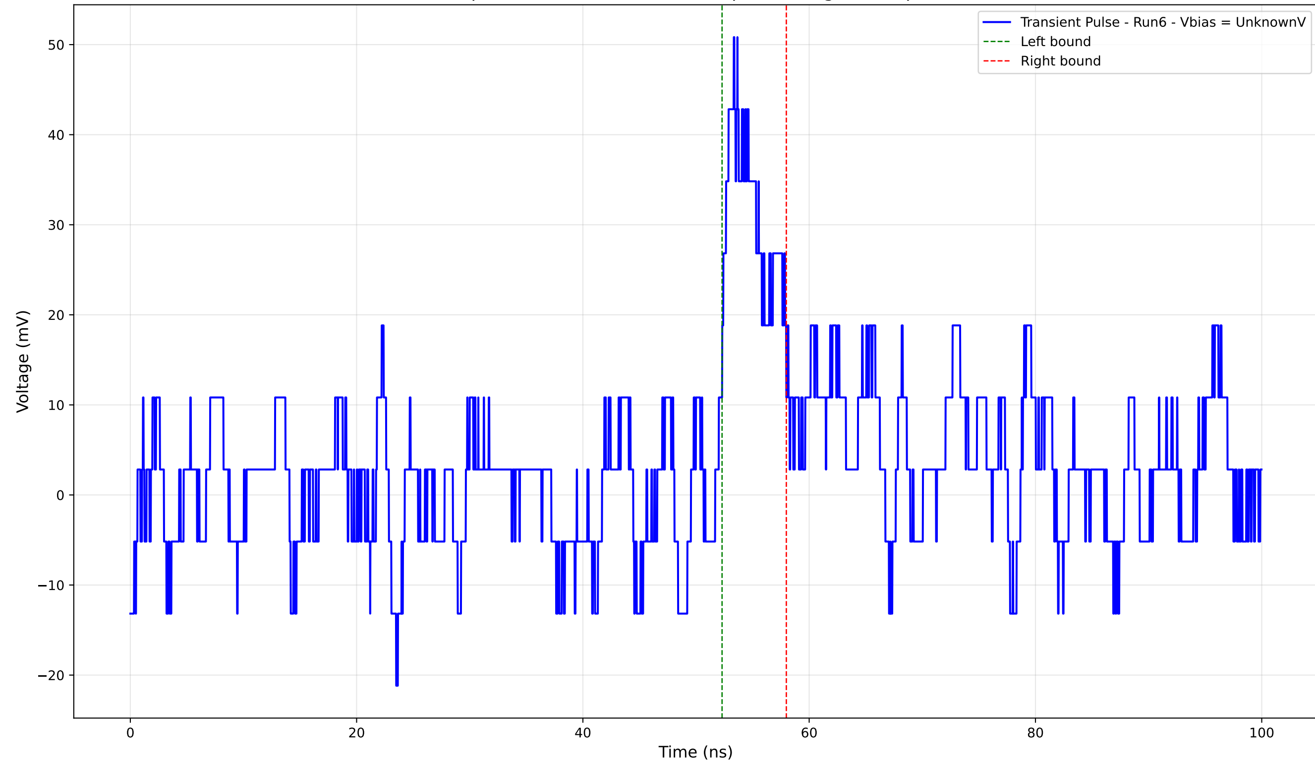
Transient Pulse - Sample: 4004 - Position: 1050.0 \mu\text{m} - Charge: 3.49 pC - Rise Time: 1.33 ns
