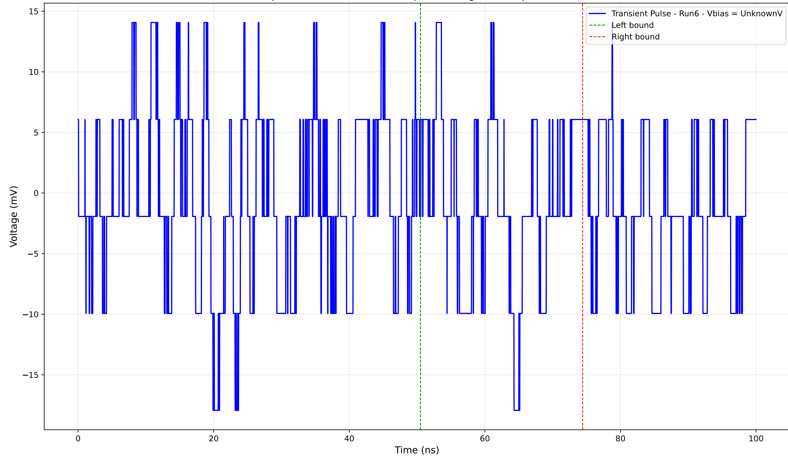
Transient Pulse - Sample: 4004 - Position: 75.0 \mu\text{m} - Charge: -0.32 pC - Rise Time: 0.00 ns (N/A)
