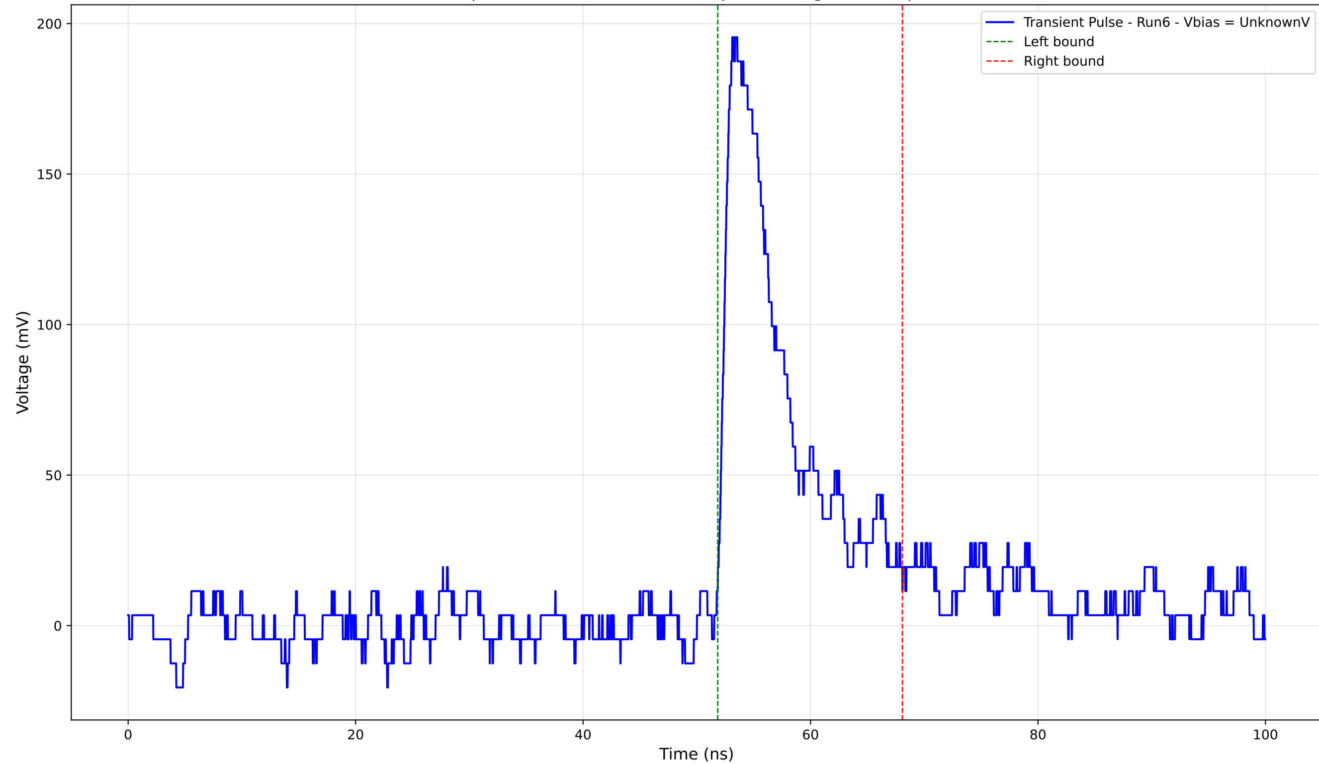
Transient Pulse - Sample: 4004 - Position: 760.0 \mu\text{m} - Charge: 24.29 pC - Rise Time: 0.98 ns
