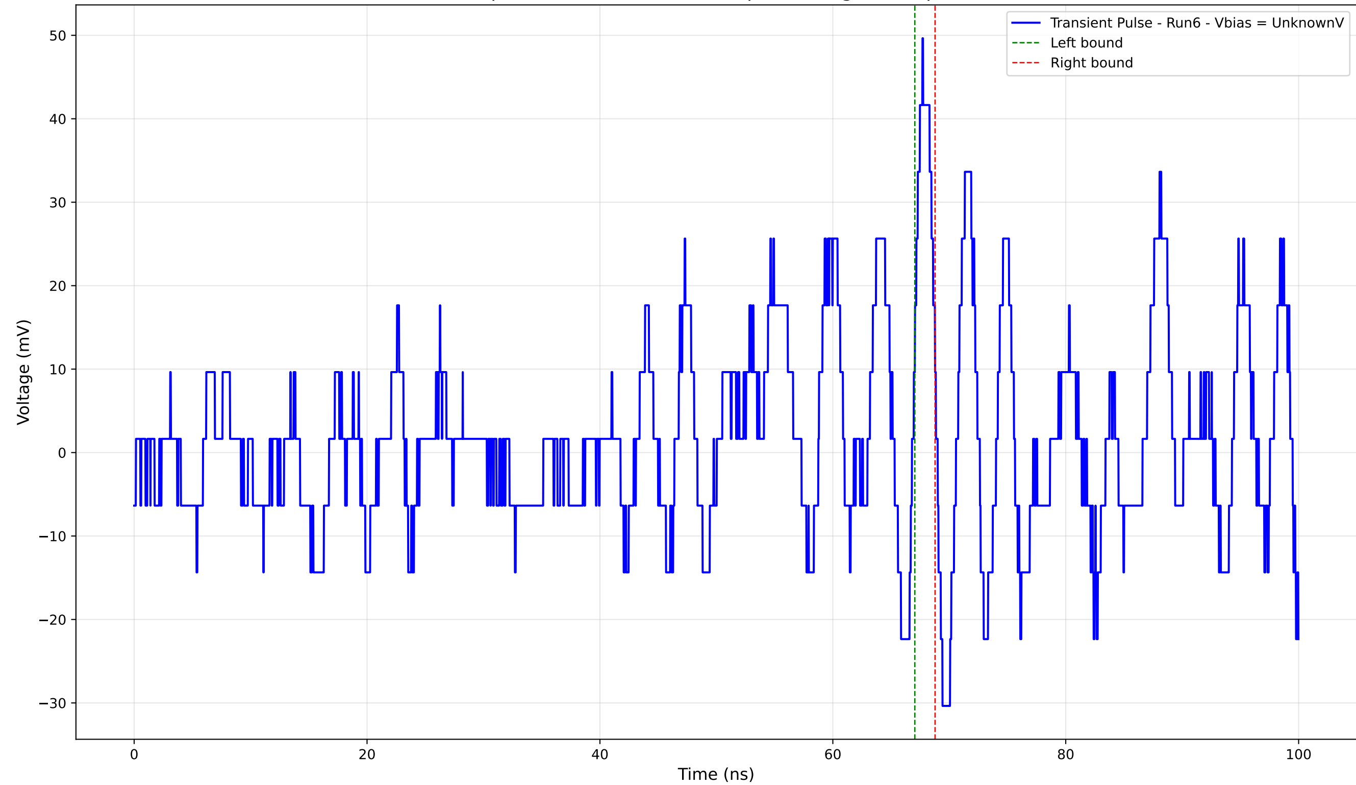
Transient Pulse - Sample: 4004 - Position: 475.0 \mu\text{m} - Charge: 1.17 pC - Rise Time: 0.75 ns
