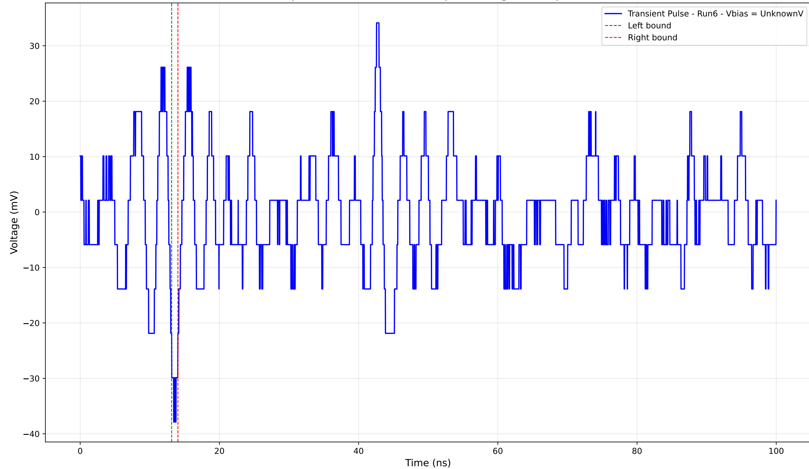
Transient Pulse - Sample: 4004 - Position: 275.0 \mu\text{m} - Charge: -0.58 pC - Rise Time: 0.71 ns
