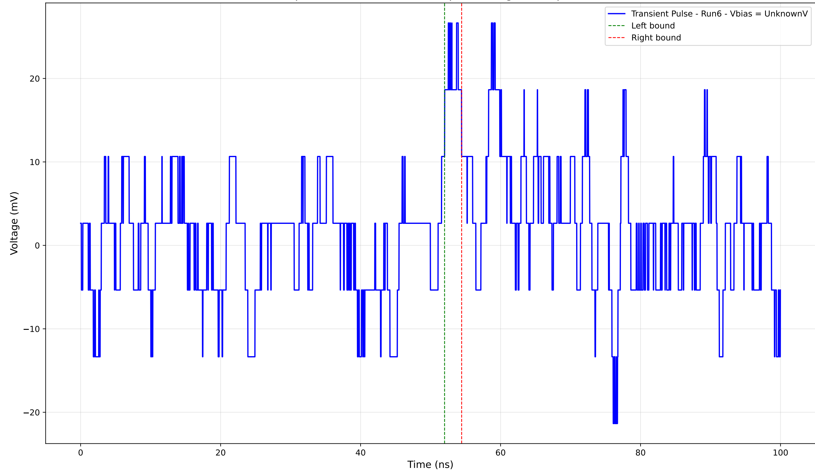
Transient Pulse - Sample: 4004 - Position: 485.0 \mu\text{m} - Charge: 0.98 pC - Rise Time: 0.98 ns
