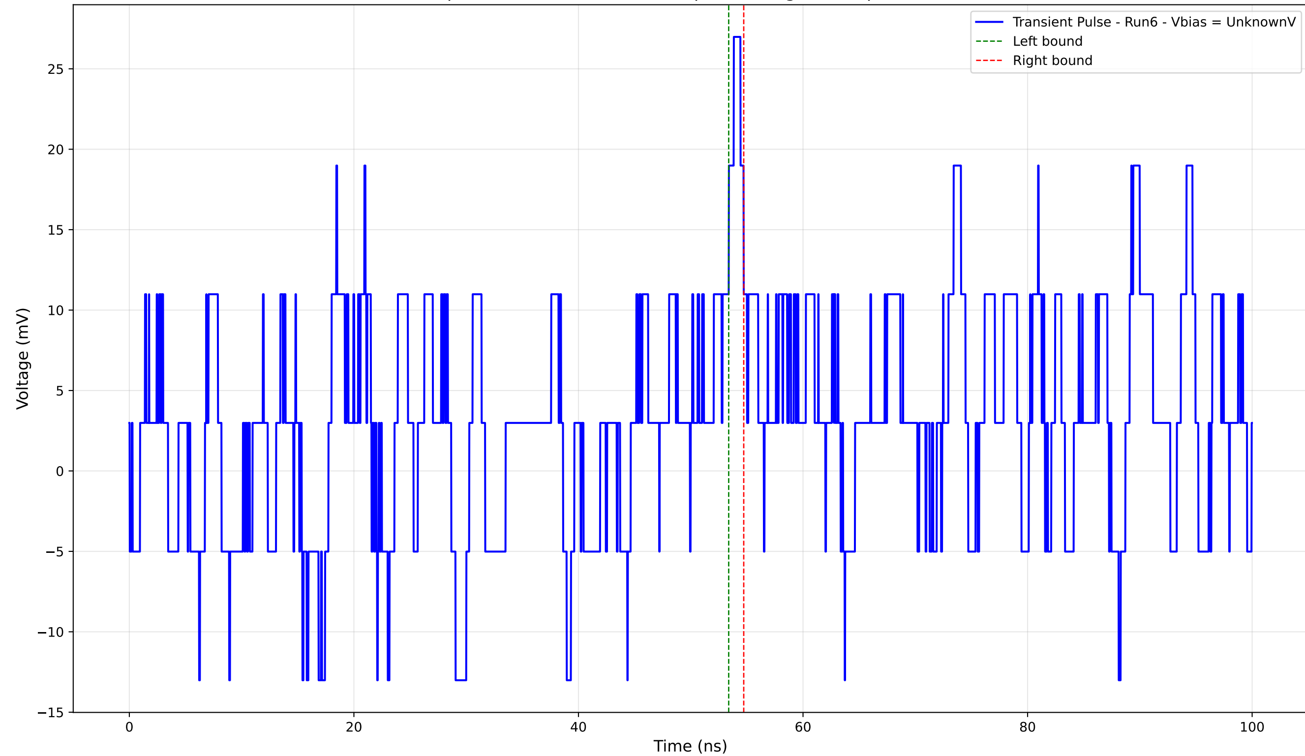
Transient Pulse - Sample: 4004 - Position: 435.0 \mu\text{m} - Charge: 0.60 pC - Rise Time: 0.00 ns (N/A)
