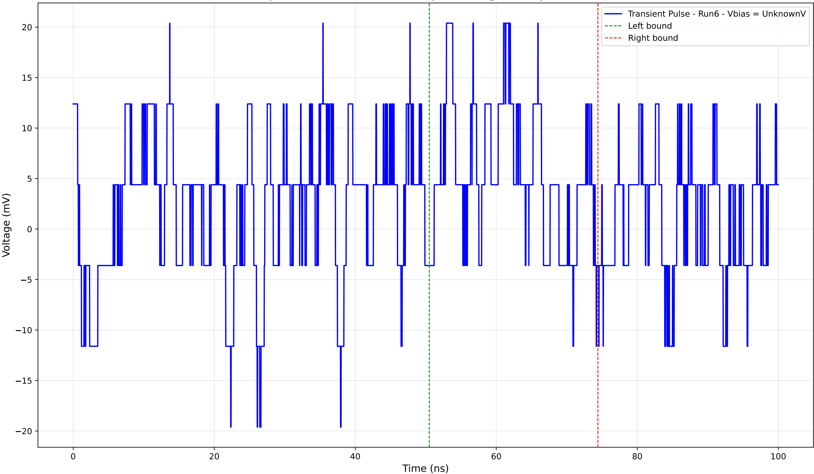
Transient Pulse - Sample: 4004 - Position: 1175.0 \mu\text{m} - Charge: 2.73 pC - Rise Time: 0.00 ns (N/A)
