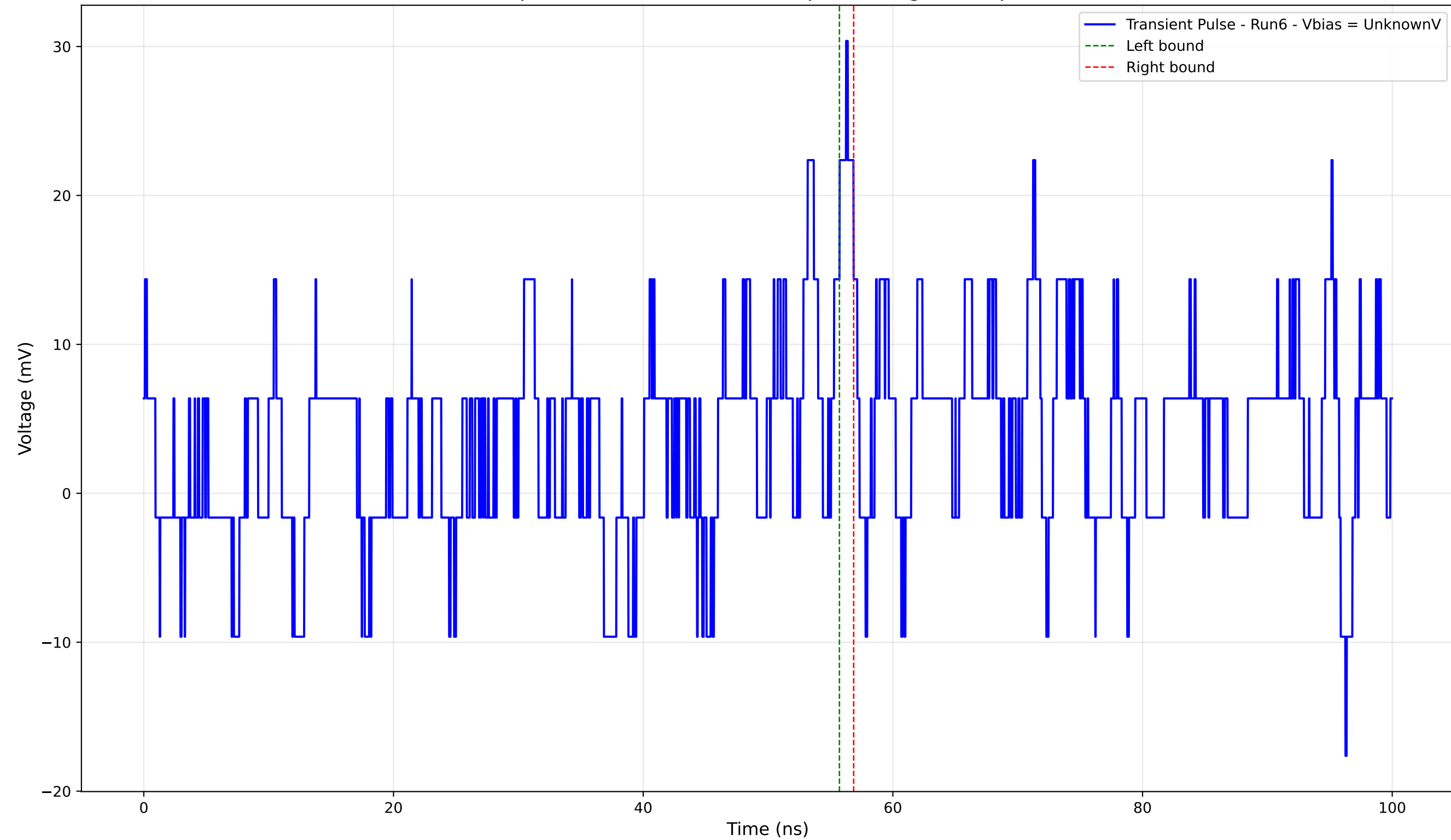
Transient Pulse - Sample: 4004 - Position: 1190.0 \mu\text{m} - Charge: 0.53 pC - Rise Time: 1.21 ns
