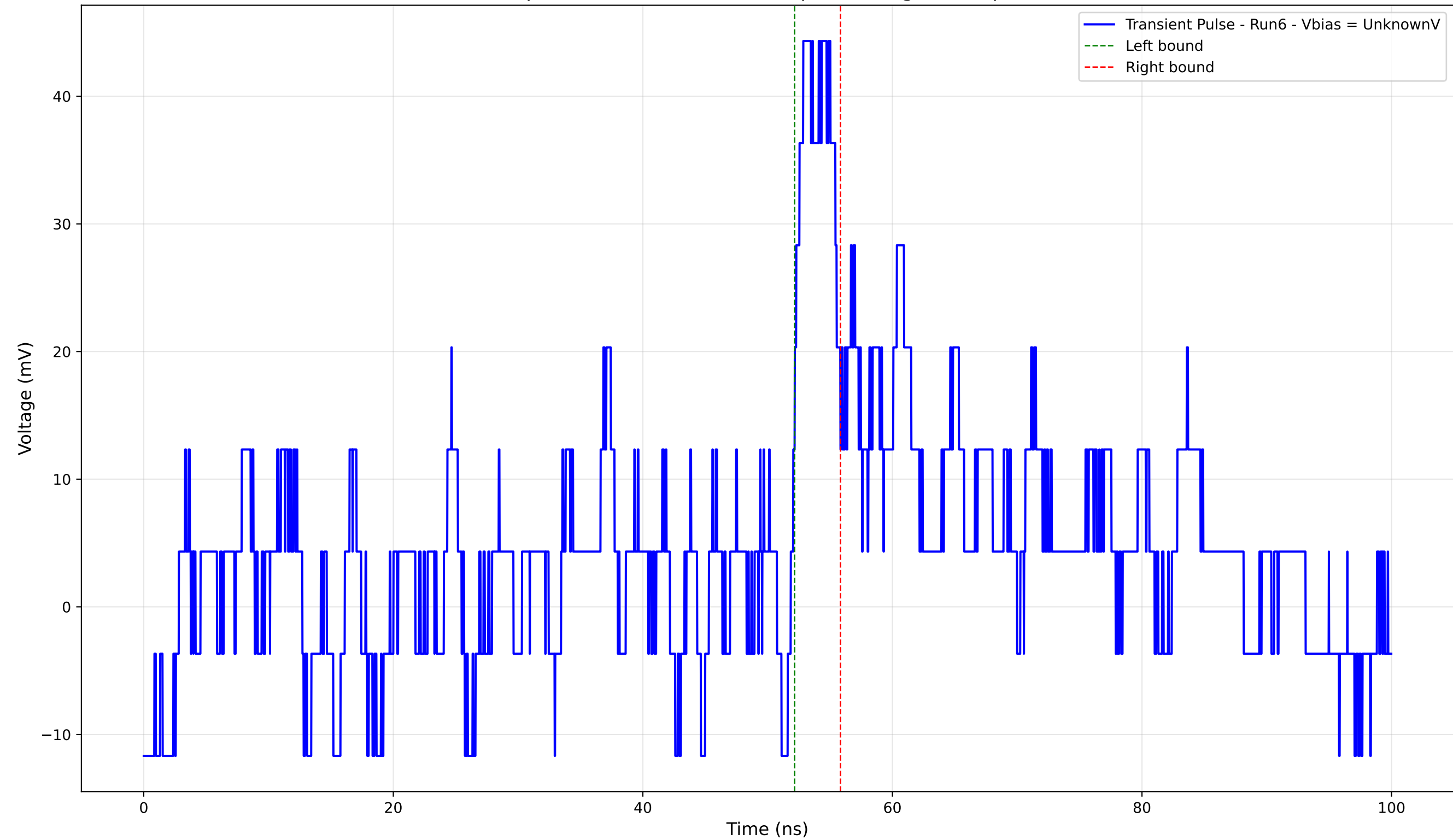
Transient Pulse - Sample: 4004 - Position: 905.0 \mu\text{m} - Charge: 2.69 pC - Rise Time: 0.82 ns
