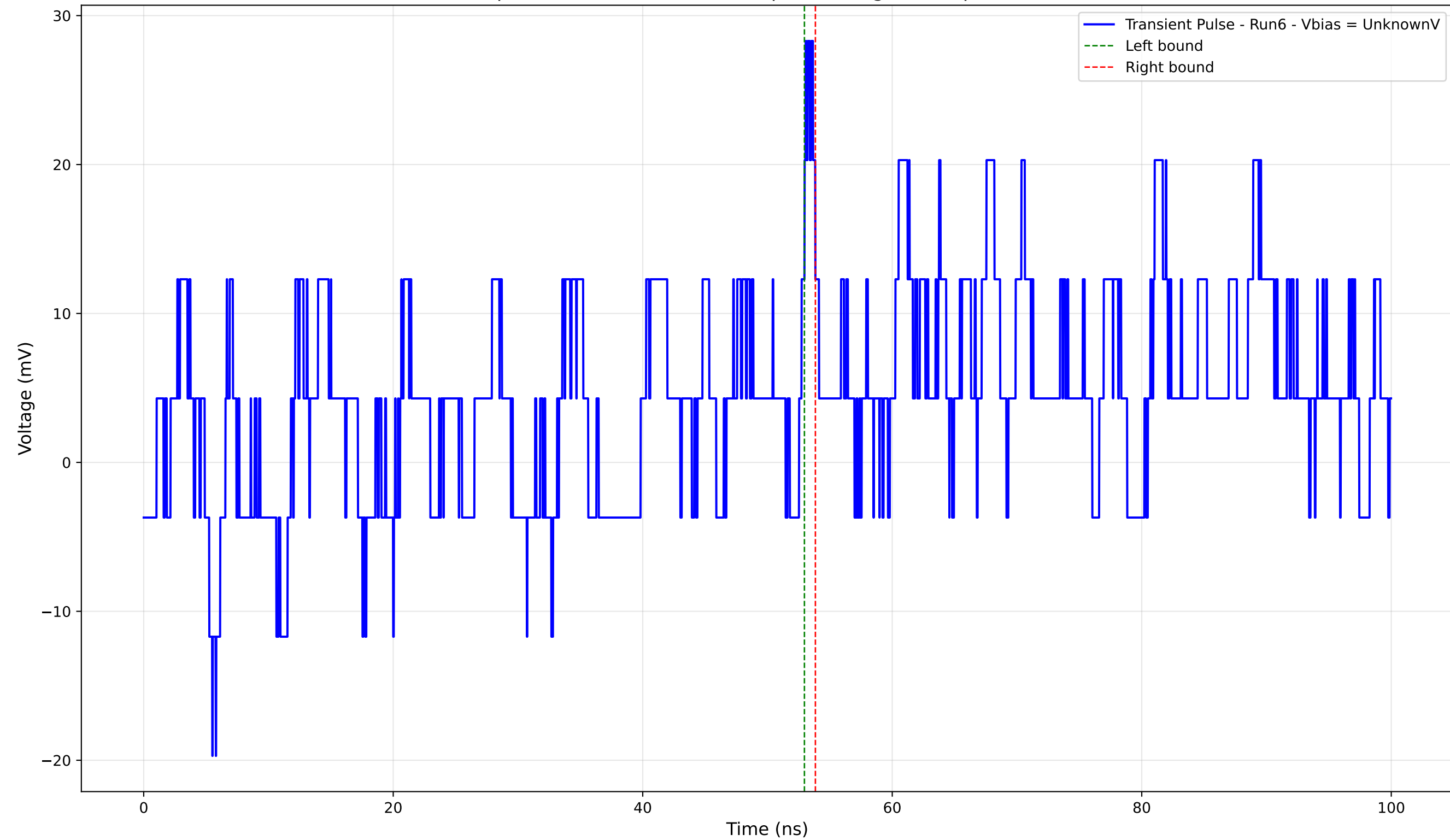
Transient Pulse - Sample: 4004 - Position: 340.0 \mu\text{m} - Charge: 0.42 pC - Rise Time: 0.00 ns (N/A)
