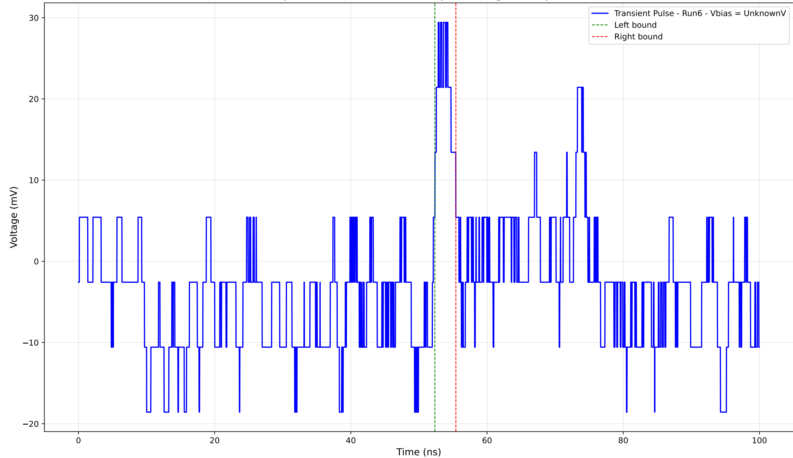
Transient Pulse - Sample: 4004 - Position: 1145.0 \mu\text{m} - Charge: 1.30 pC - Rise Time: 0.74 ns
