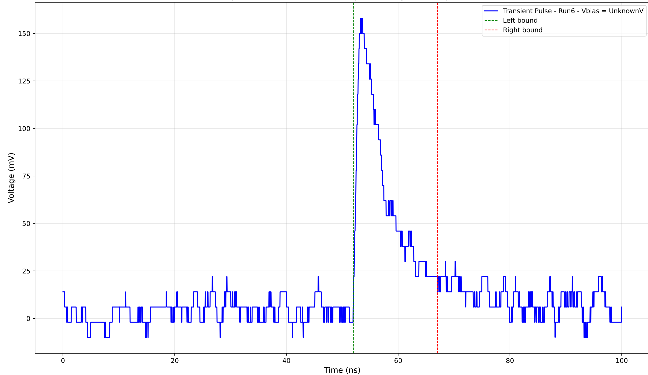
Transient Pulse - Sample: 4004 - Position: 795.0 \mu\text{m} - Charge: 19.43 pC - Rise Time: 1.02 ns
