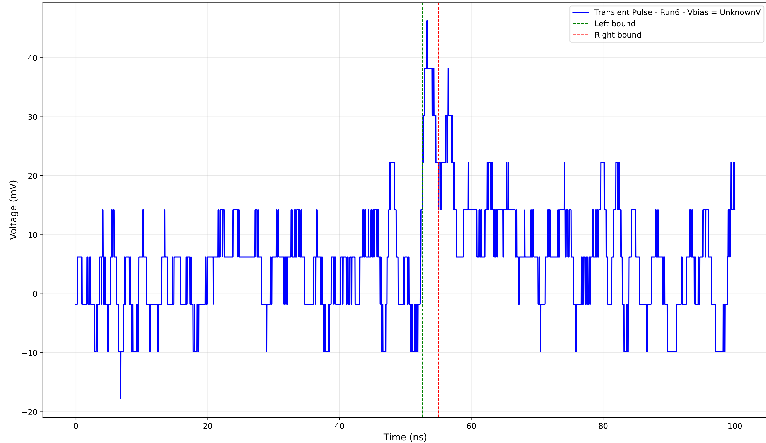
Transient Pulse - Sample: 4004 - Position: 490.0 \mu\text{m} - Charge: 1.62 pC - Rise Time: 1.03 ns
