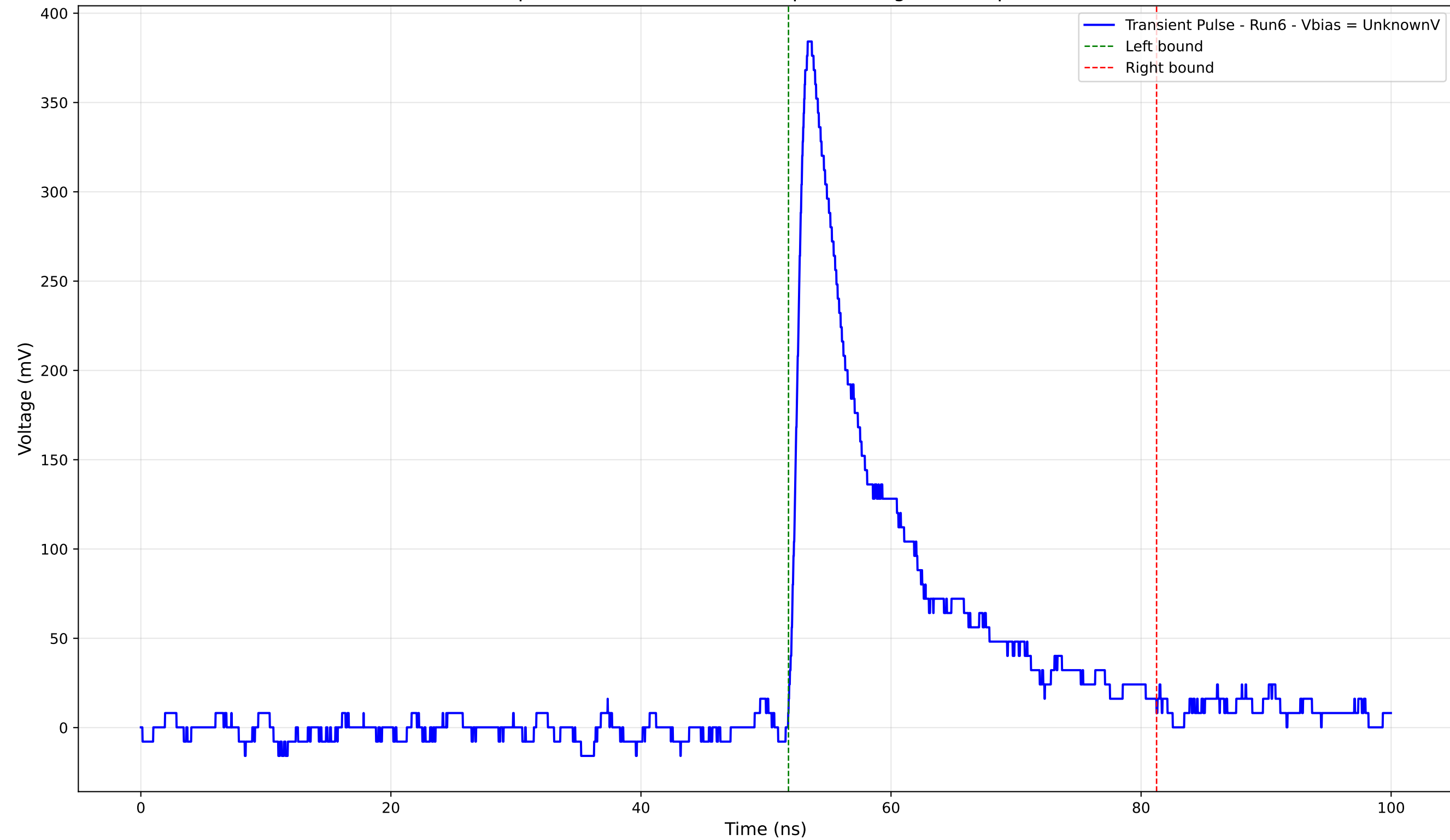
Transient Pulse - Sample: 4004 - Position: 550.0 \mu\text{m} - Charge: 56.51 pC - Rise Time: 1.08 ns
