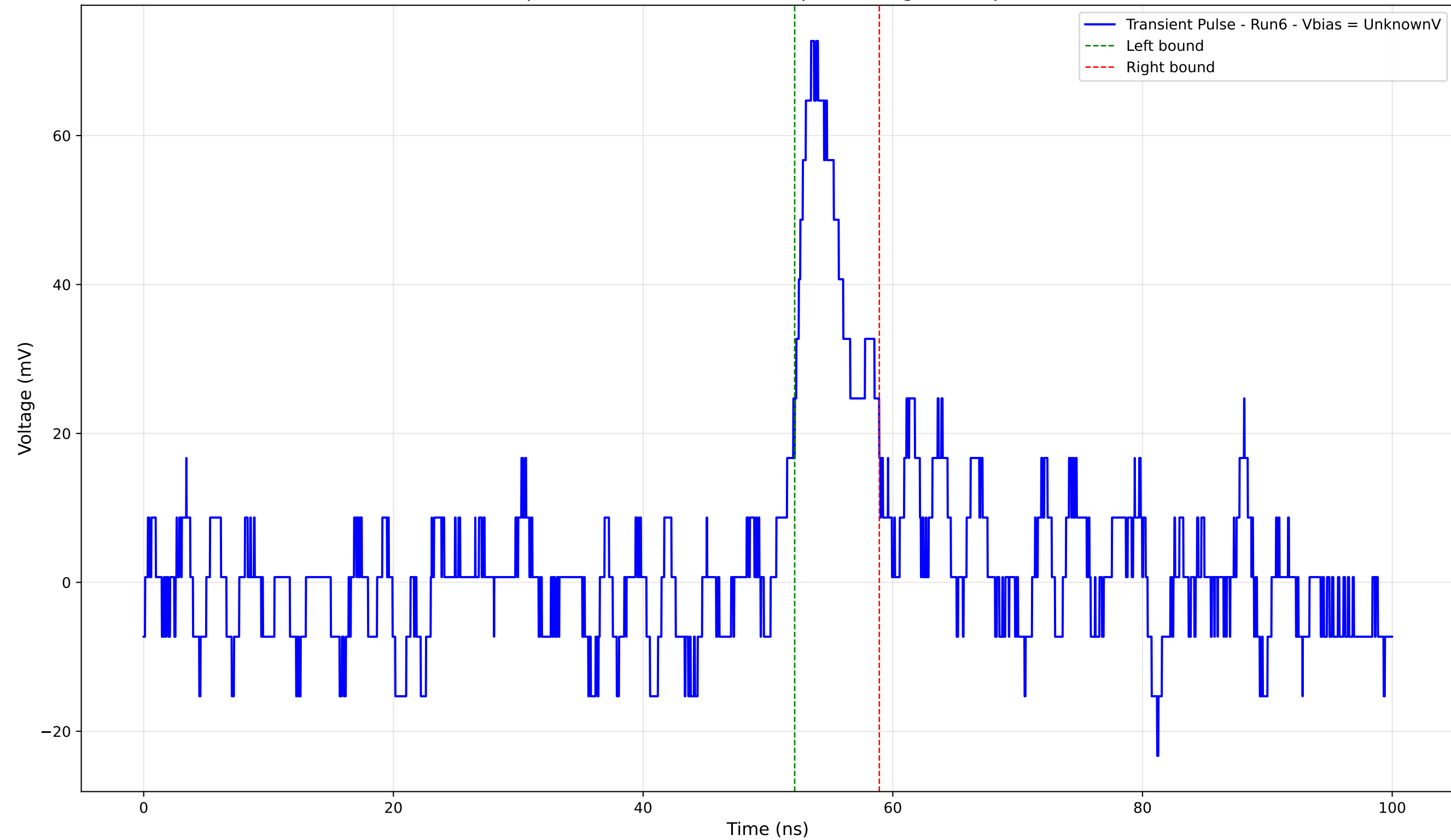
Transient Pulse - Sample: 4004 - Position: 930.0 \mu\text{m} - Charge: 5.94 pC - Rise Time: 2.78 ns
