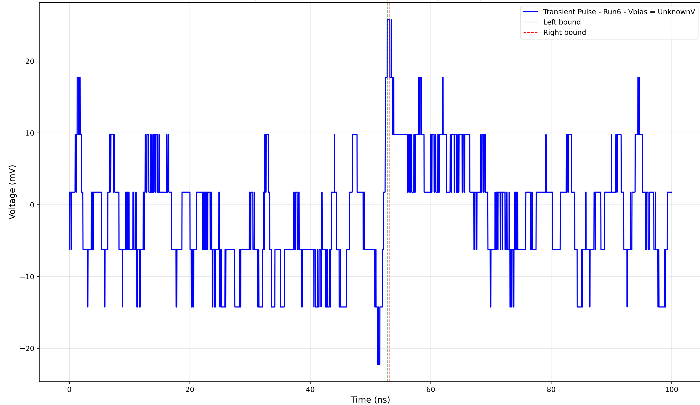
Transient Pulse - Sample: 4004 - Position: 460.0 \mu\text{m} - Charge: 0.23 pC - Rise Time: 0.36 ns
