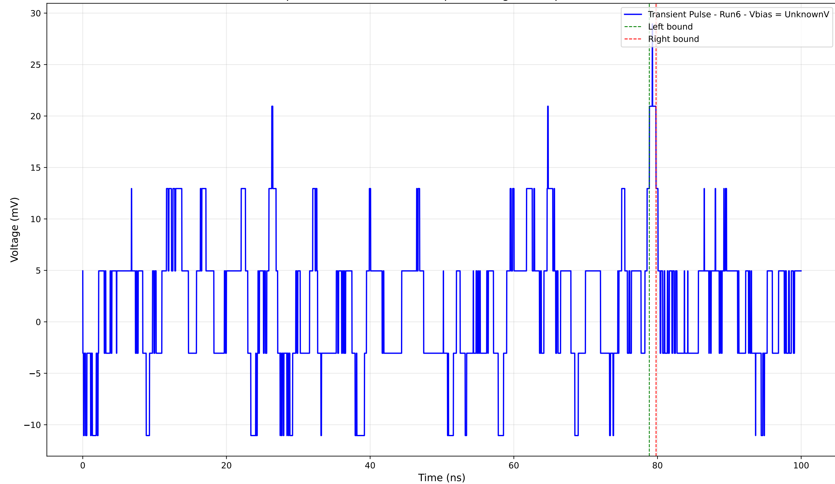
Transient Pulse - Sample: 4004 - Position: 245.0 \mu\text{m} - Charge: 0.40 pC - Rise Time: 0.00 ns (N/A)
