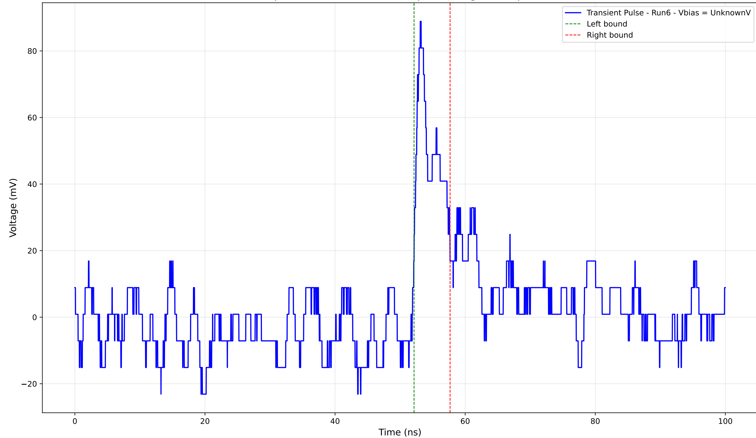
Transient Pulse - Sample: 4004 - Position: 925.0 \mu\text{m} - Charge: 5.63 pC - Rise Time: 0.84 ns
