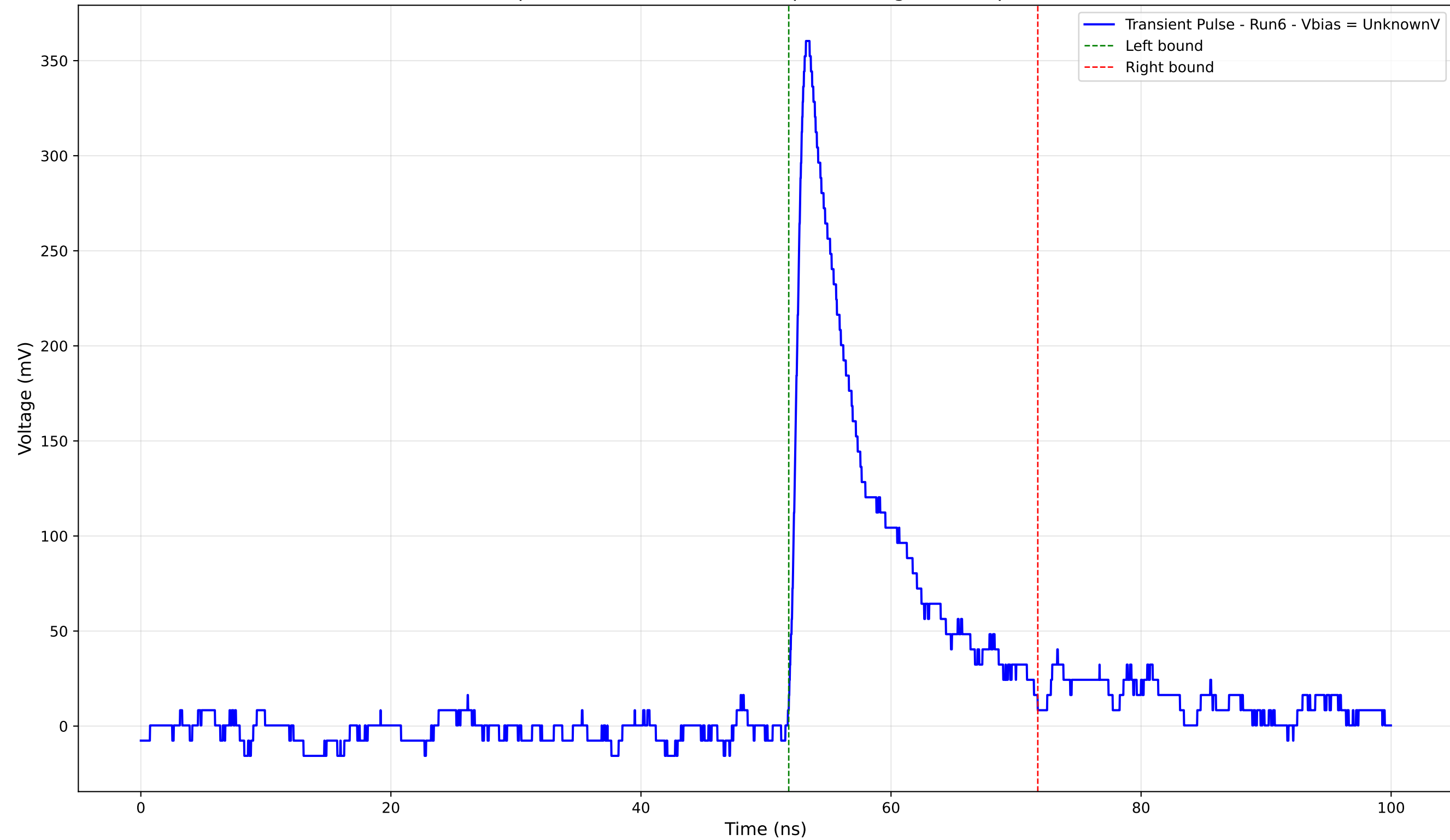
Transient Pulse - Sample: 4004 - Position: 660.0 \mu\text{m} - Charge: 44.62 pC - Rise Time: 0.99 ns
