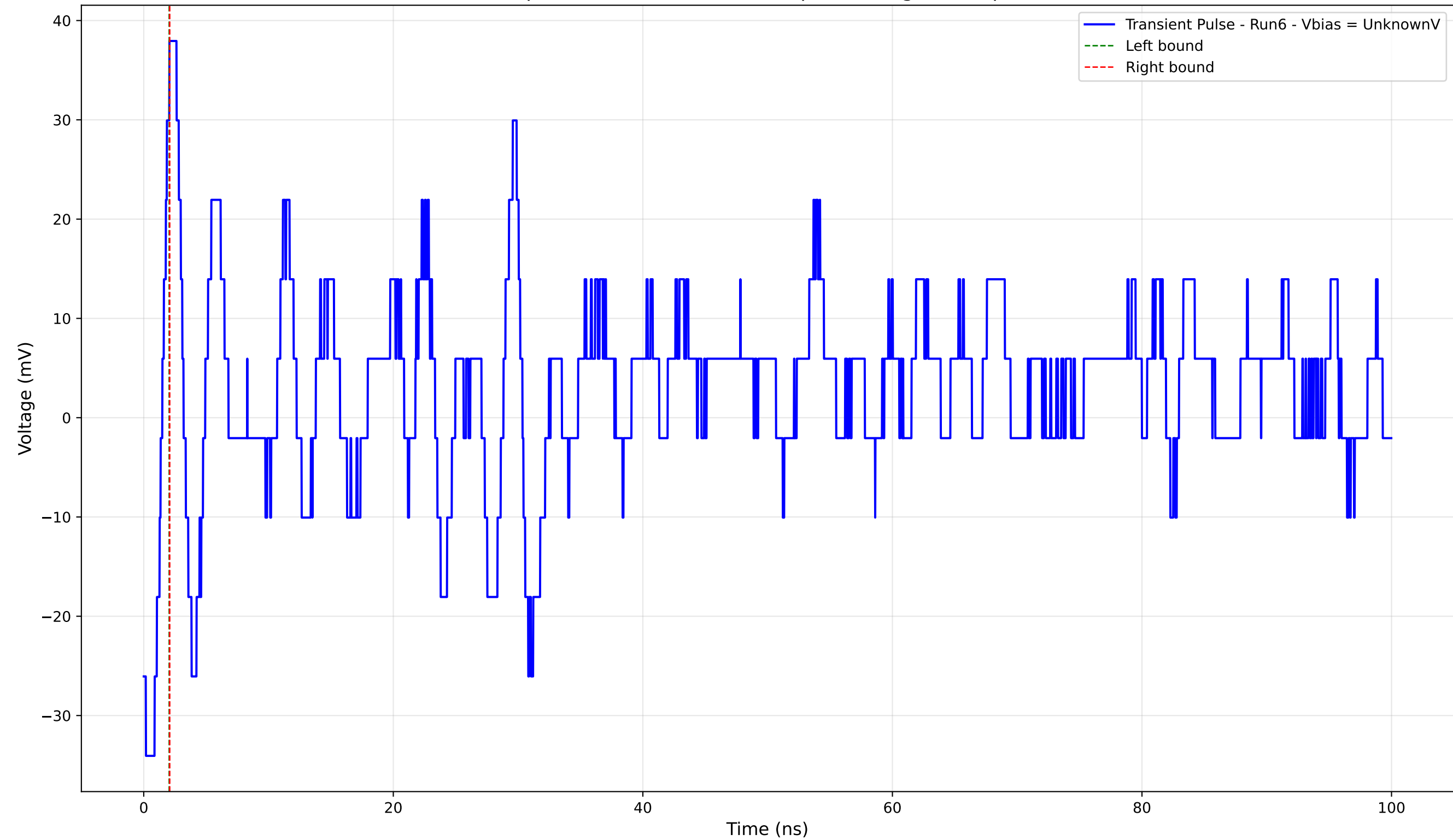
Transient Pulse - Sample: 4004 - Position: 225.0 \mu\text{m} - Charge: 0.03 pC - Rise Time: 0.57 ns
