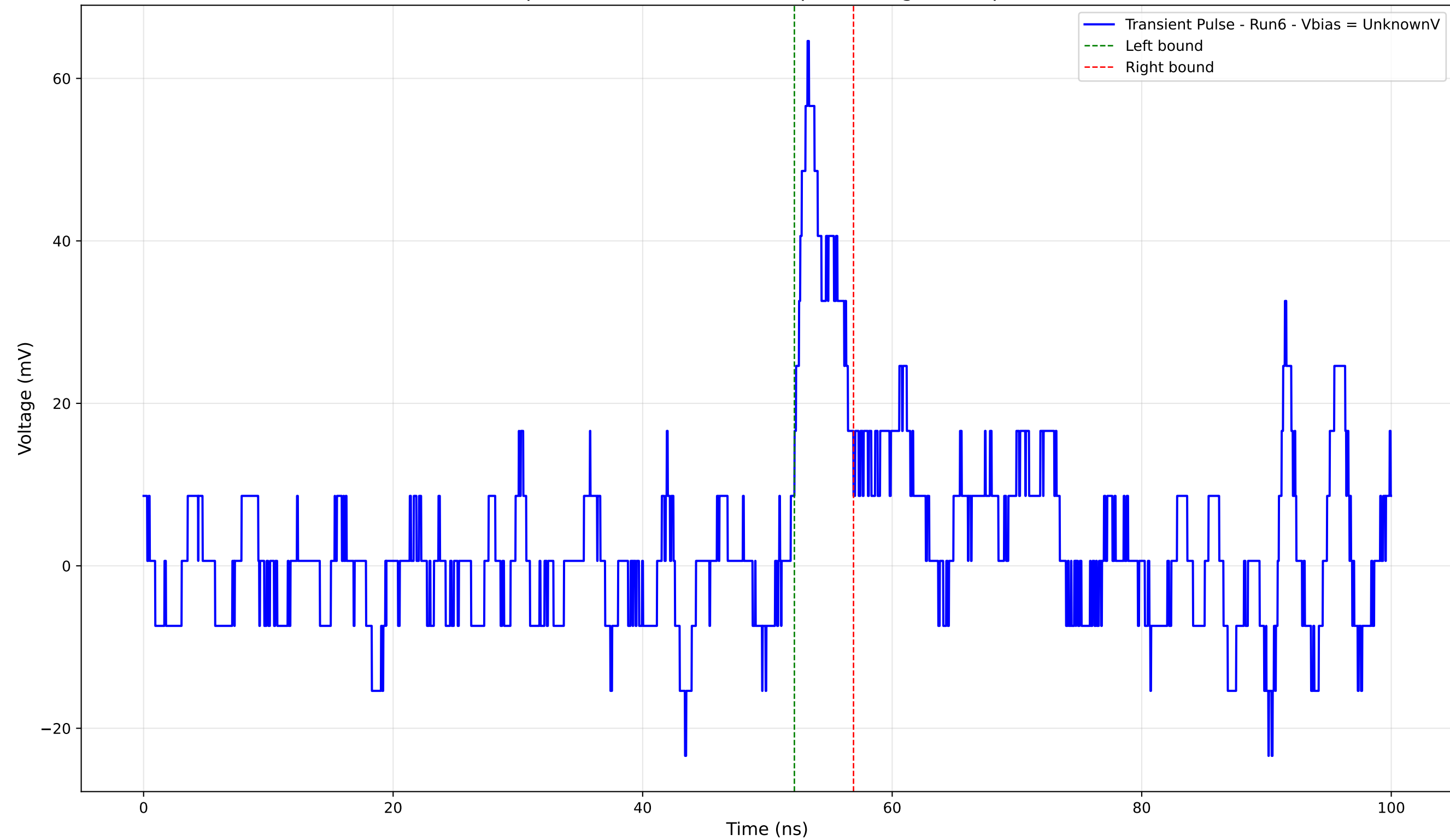
Transient Pulse - Sample: 4004 - Position: 900.0 \mu\text{m} - Charge: 3.56 pC - Rise Time: 1.35 ns
