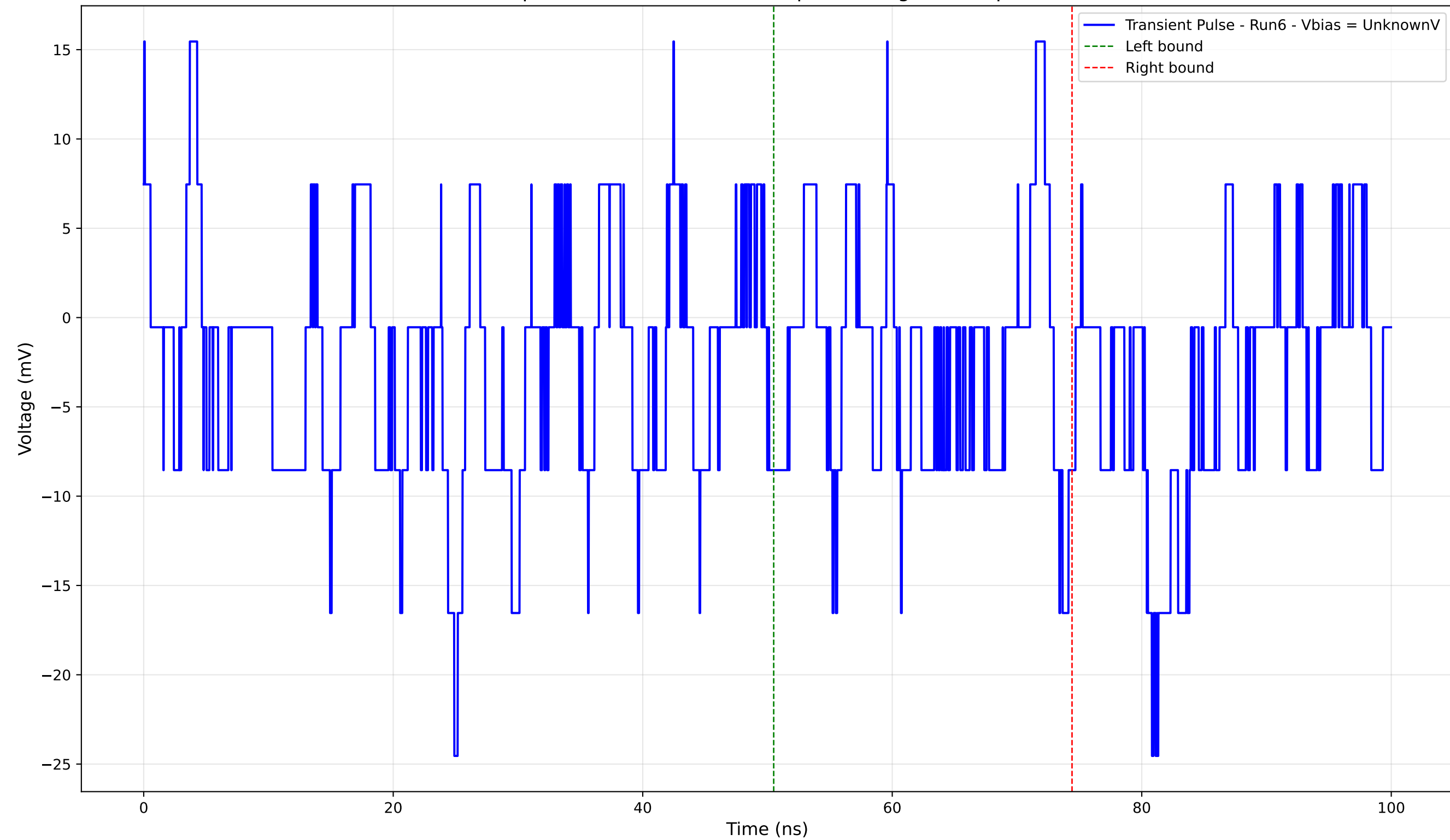
Transient Pulse - Sample: 4004 - Position: 190.0 \mu\text{m} - Charge: -1.13 pC - Rise Time: 0.96 ns
