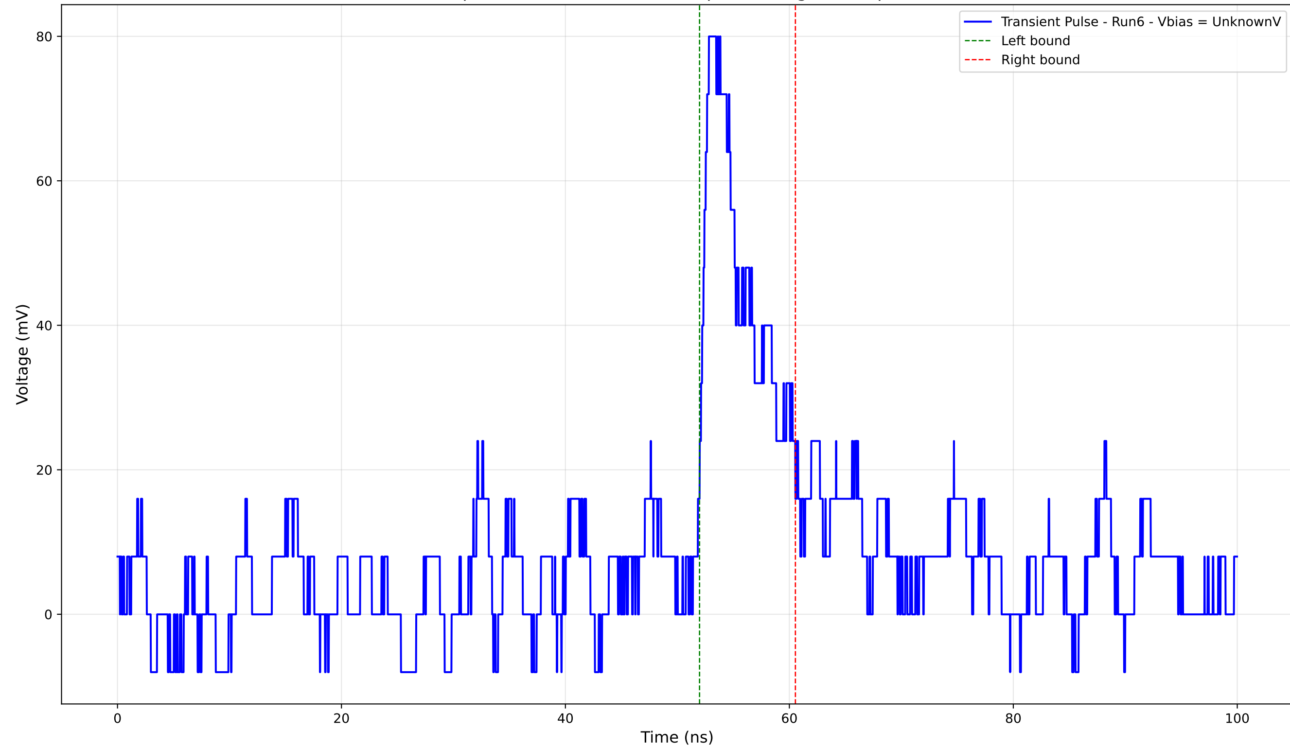
Transient Pulse - Sample: 4004 - Position: 990.0 \mu\text{m} - Charge: 7.91 pC - Rise Time: 1.00 ns
