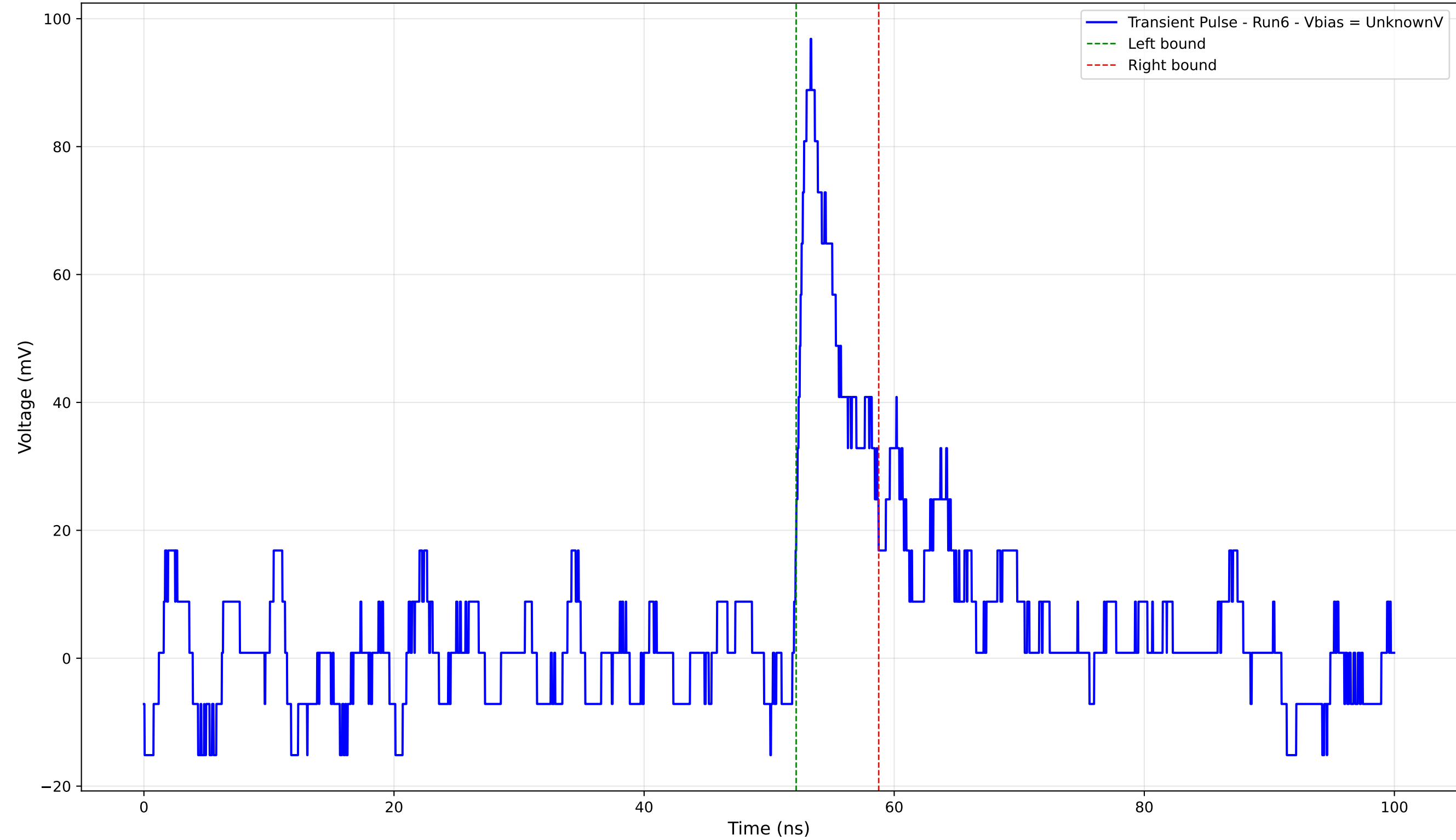
Transient Pulse - Sample: 4004 - Position: 955.0 \mu\text{m} - Charge: 6.99 pC - Rise Time: 0.90 ns
