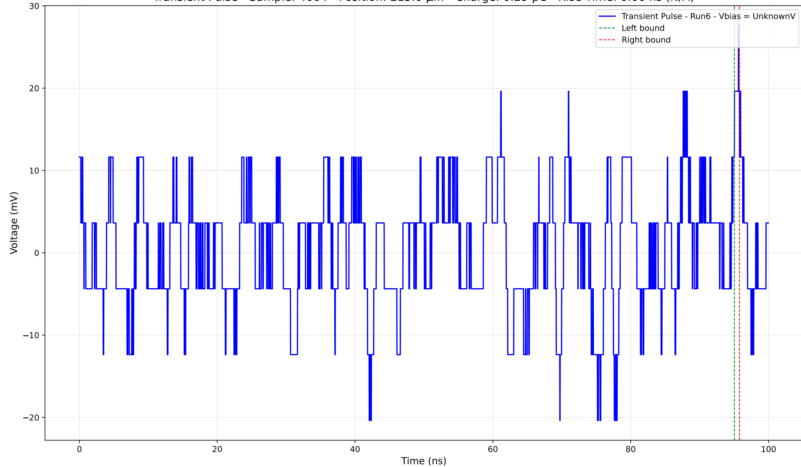
Transient Pulse - Sample: 4004 - Position: 215.0 \mu\text{m} - Charge: 0.29 pC - Rise Time: 0.00 ns (N/A)
