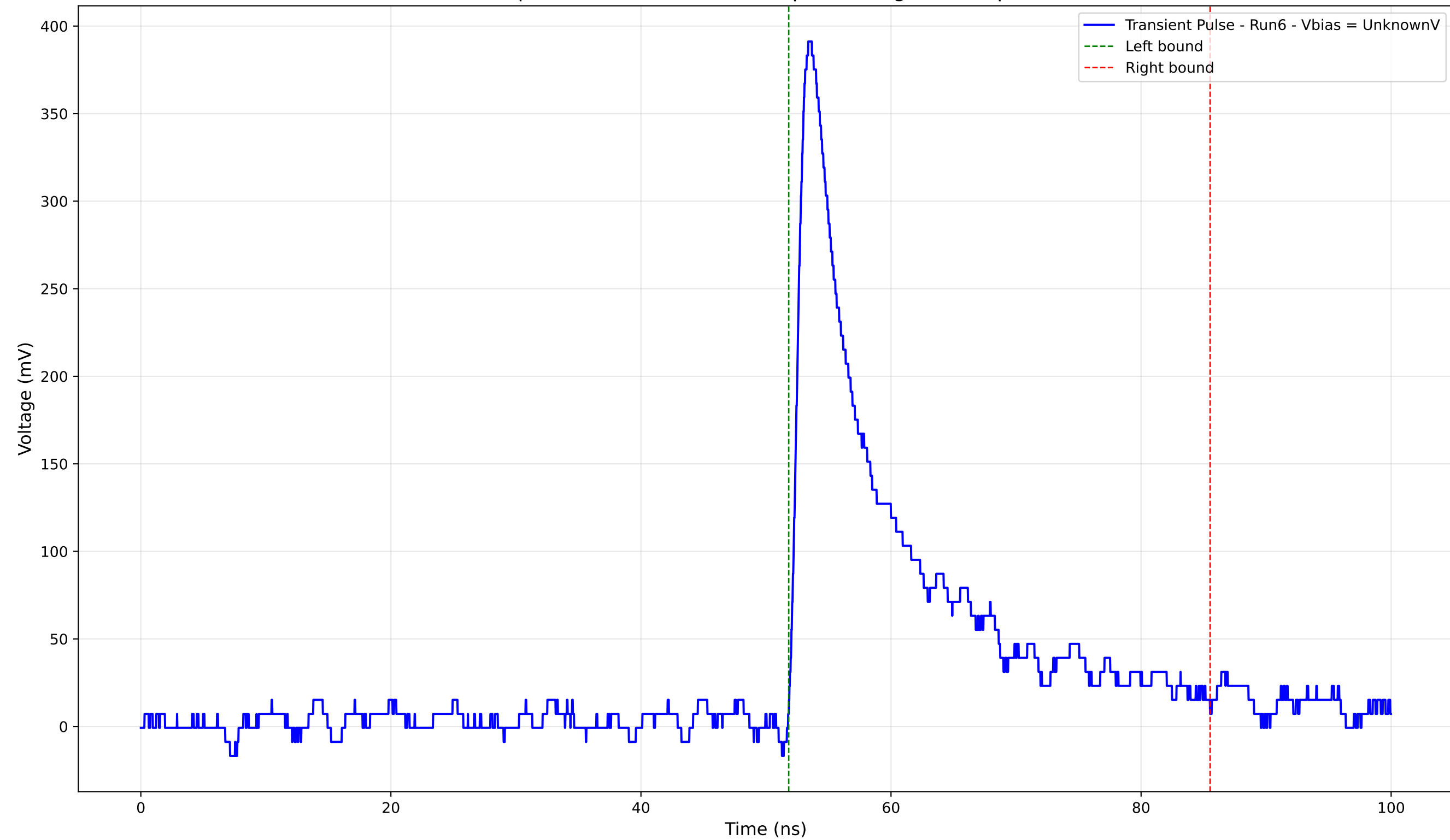
Transient Pulse - Sample: 4004 - Position: 555.0 \mu\text{m} - Charge: 60.62 pC - Rise Time: 1.06 ns
