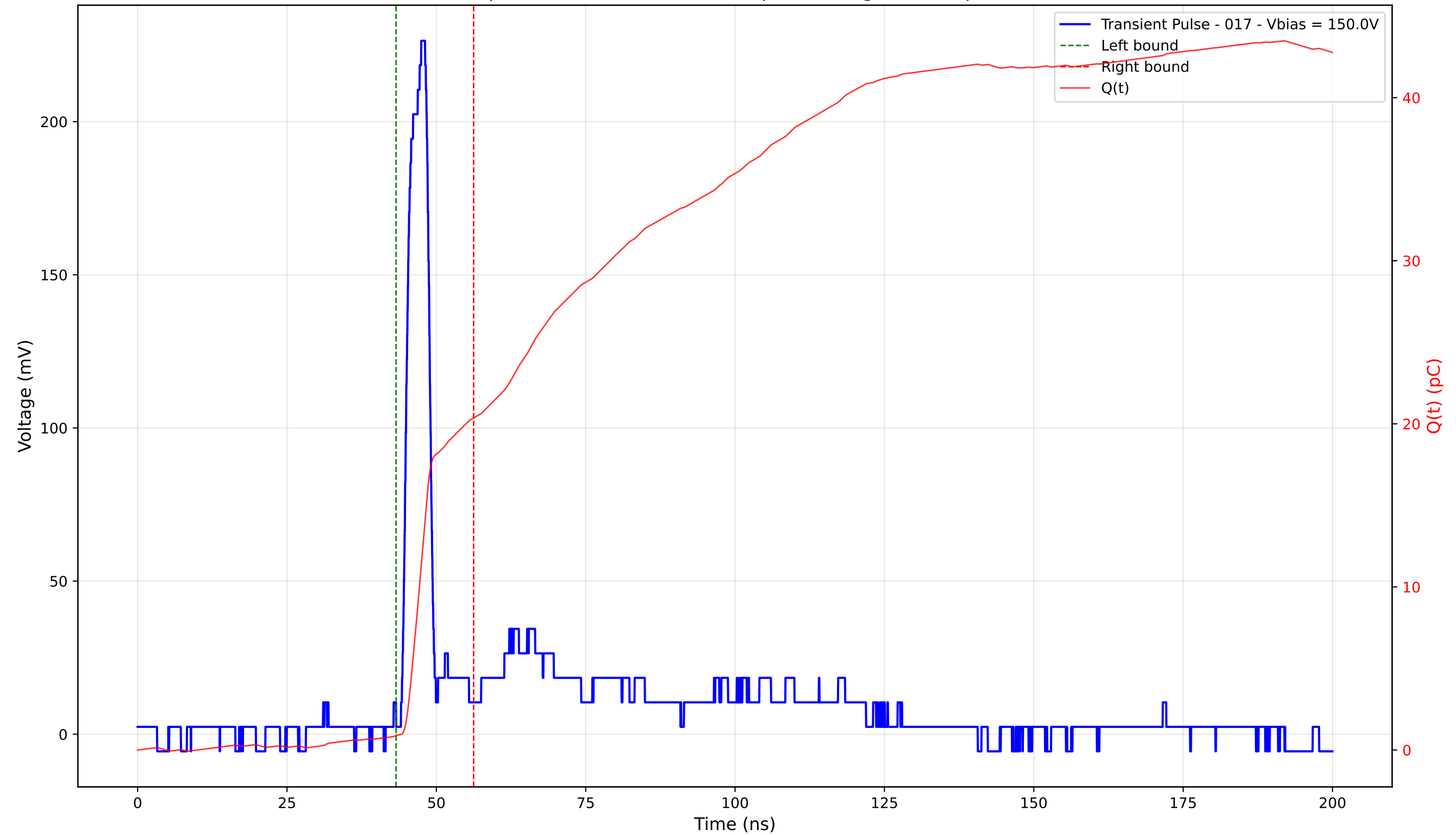
Transient Pulse - Sample: 4003 - Position: 275.0 \mu\text{m} - Charge: 19.45 pC - Rise Time: 2.55 ns
