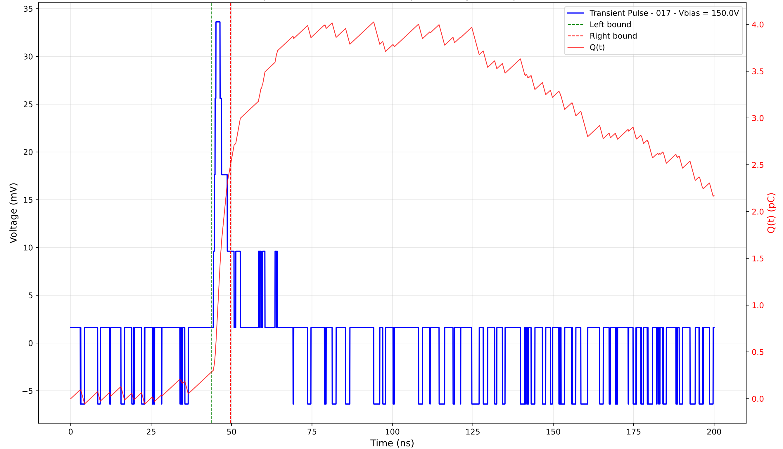
Transient Pulse - Sample: 4003 - Position: 380.0 \mu\text{m} - Charge: 2.21 pC - Rise Time: 0.82 ns
