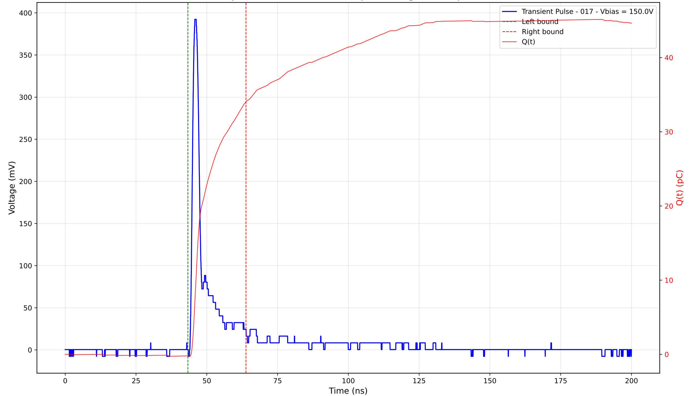
Transient Pulse - Sample: 4003 - Position: 220.0 \mu\text{m} - Charge: 34.26 pC - Rise Time: 1.18 ns
