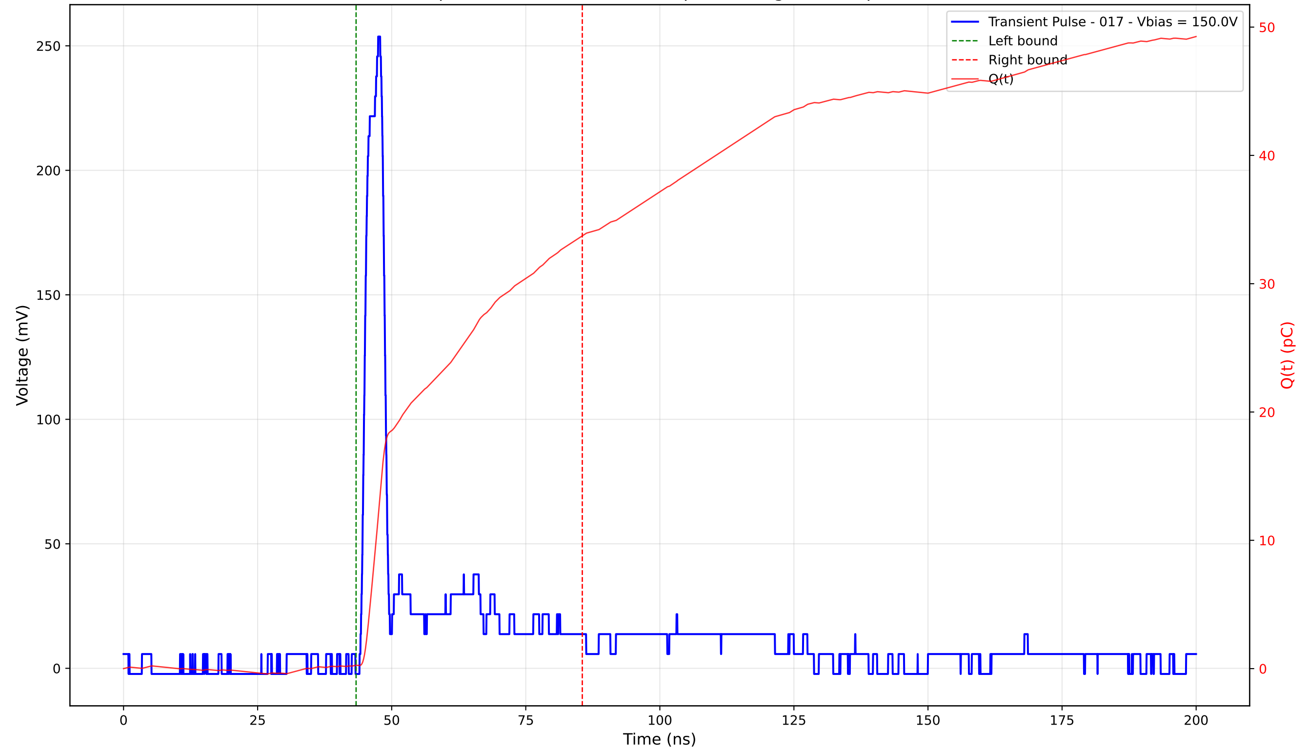
Transient Pulse - Sample: 4003 - Position: 270.0 \mu\text{m} - Charge: 33.48 pC - Rise Time: 2.53 ns
