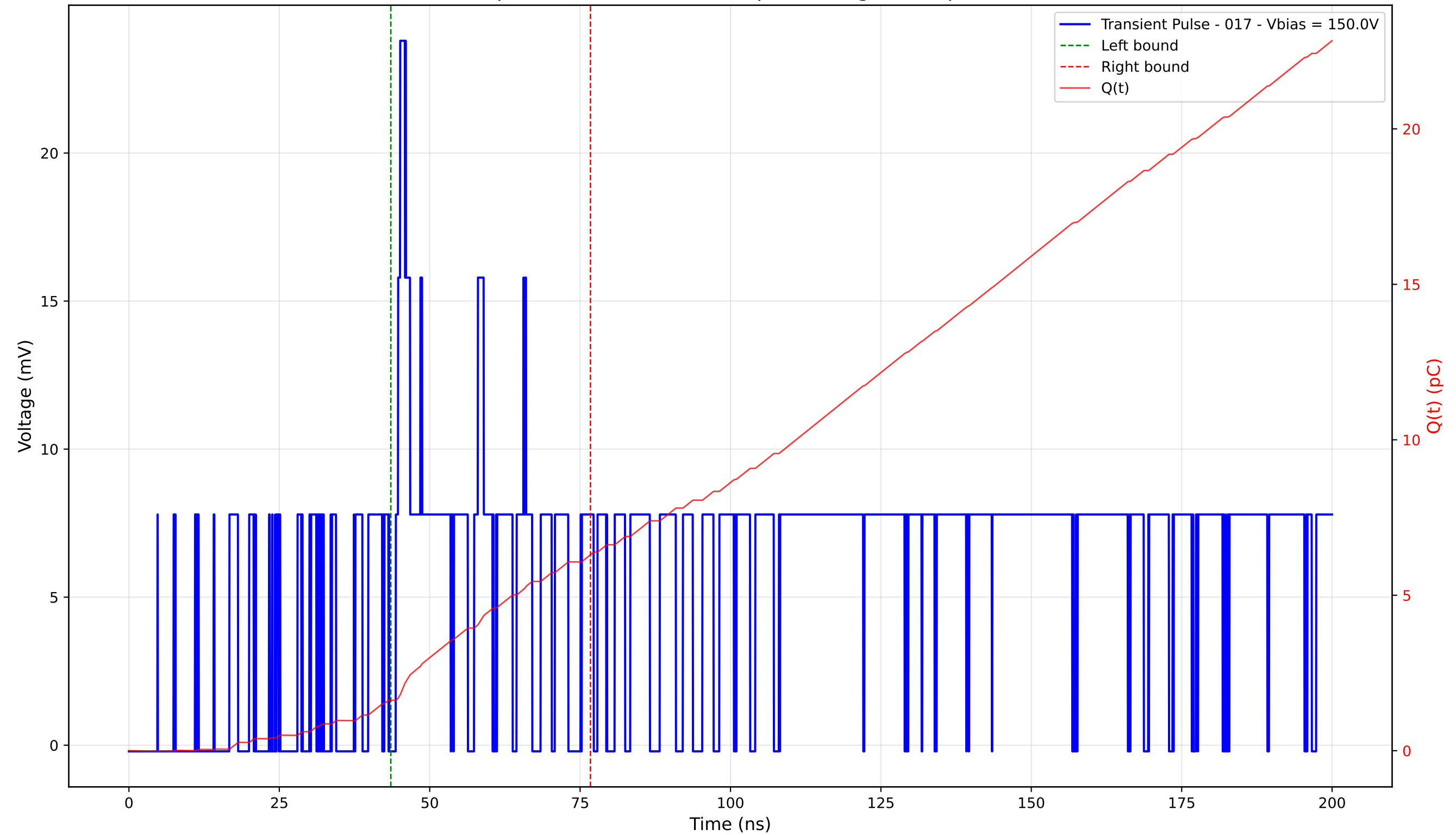
Transient Pulse - Sample: 4003 - Position: 75.0 \mu\text{m} - Charge: 4.68 pC - Rise Time: 0.73 ns
