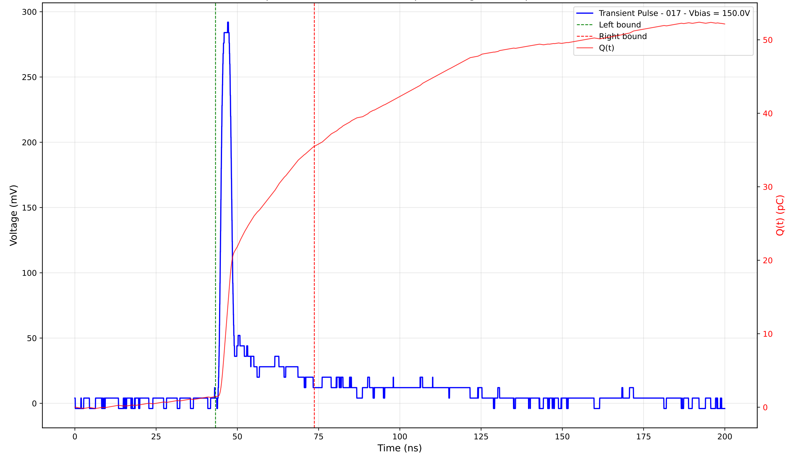
Transient Pulse - Sample: 4003 - Position: 255.0 \mu\text{m} - Charge: 34.04 pC - Rise Time: 1.28 ns
