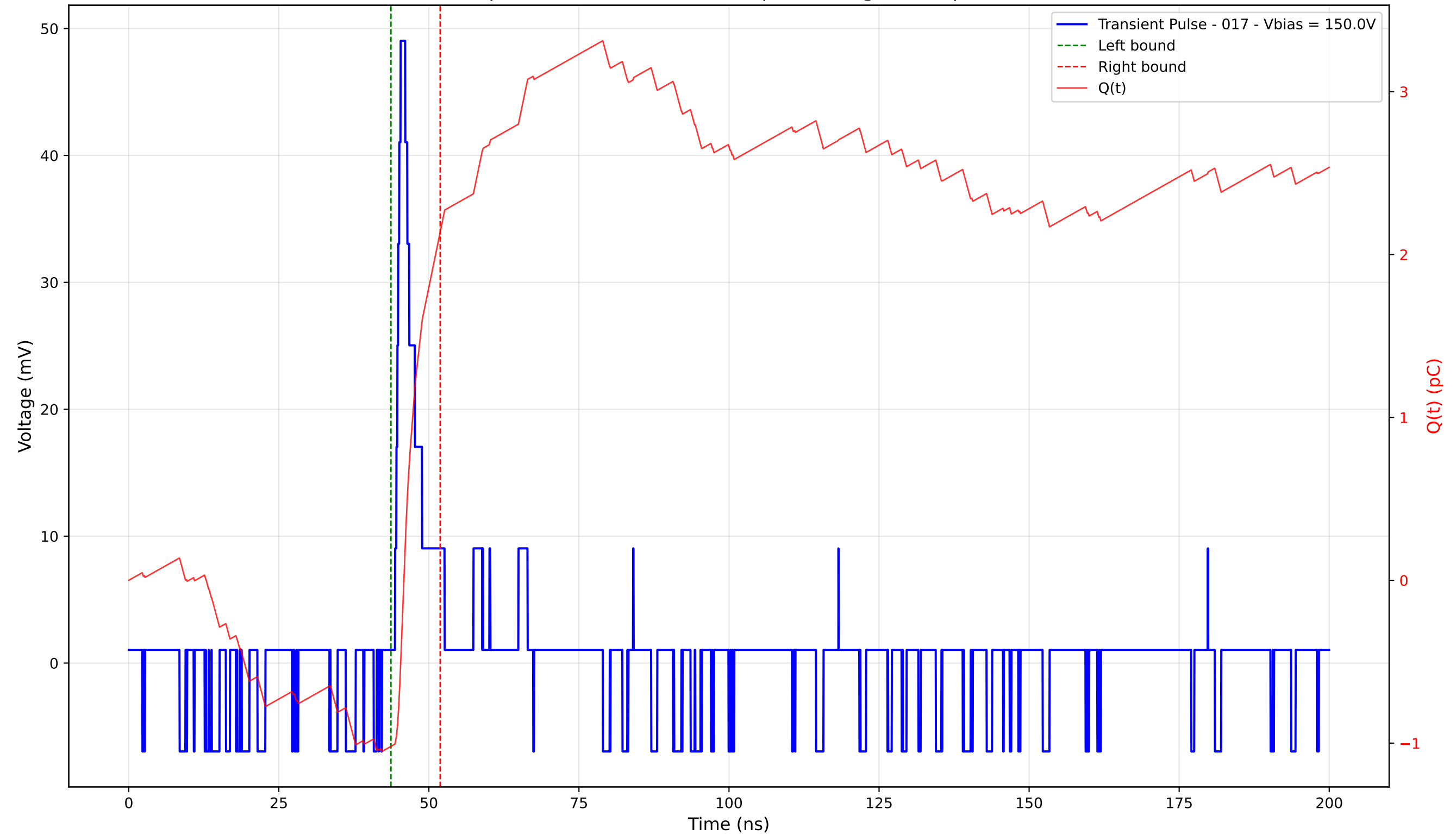
Transient Pulse - Sample: 4003 - Position: 385.0 \mu\text{m} - Charge: 3.16 pC - Rise Time: 0.93 ns
