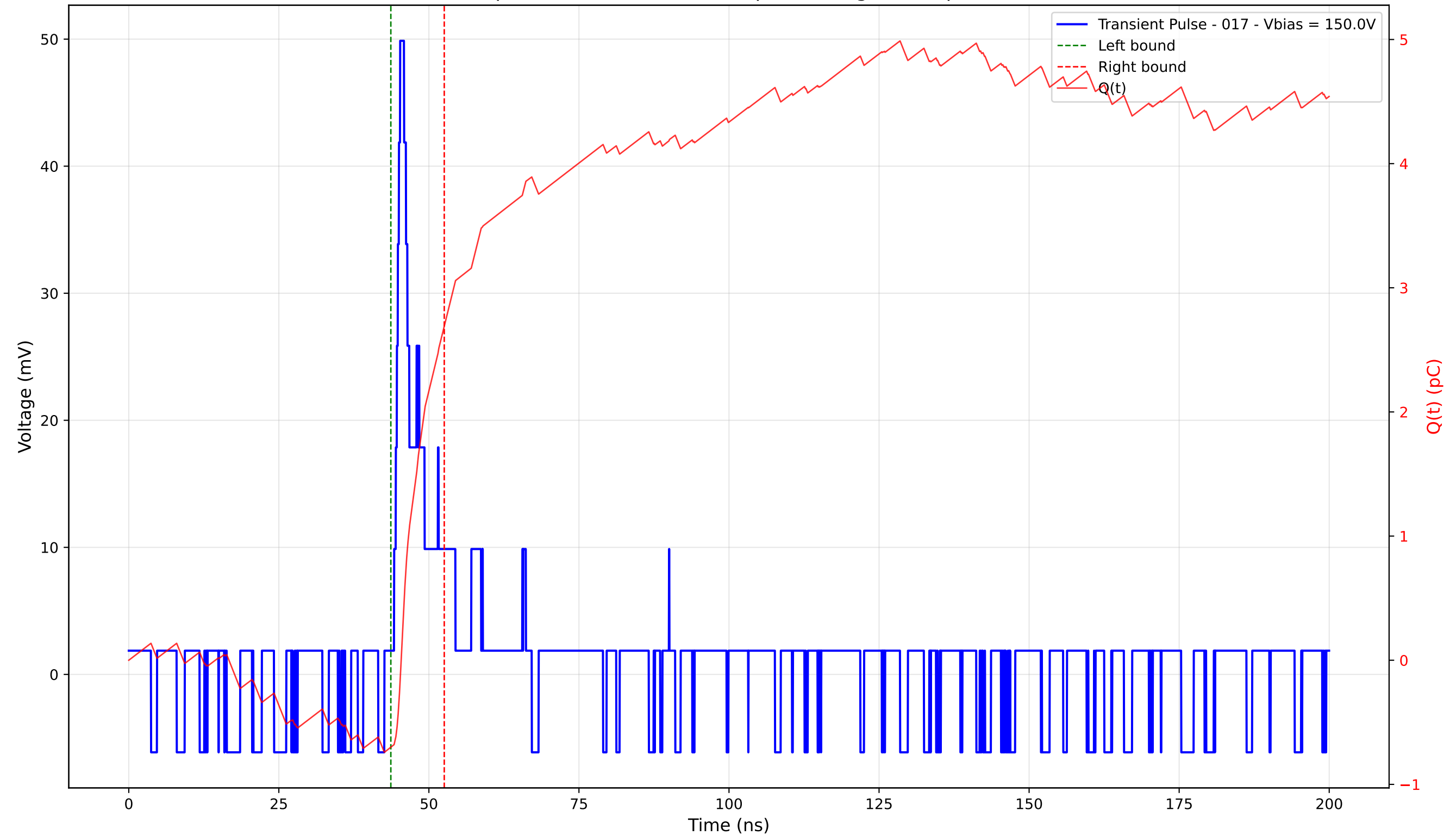
Transient Pulse - Sample: 4003 - Position: 85.0 \mu\text{m} - Charge: 3.39 pC - Rise Time: 1.01 ns
