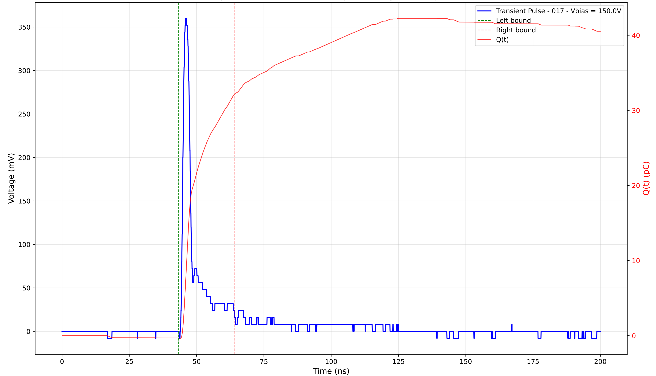
Transient Pulse - Sample: 4003 - Position: 230.0 \mu\text{m} - Charge: 32.52 pC - Rise Time: 1.19 ns
