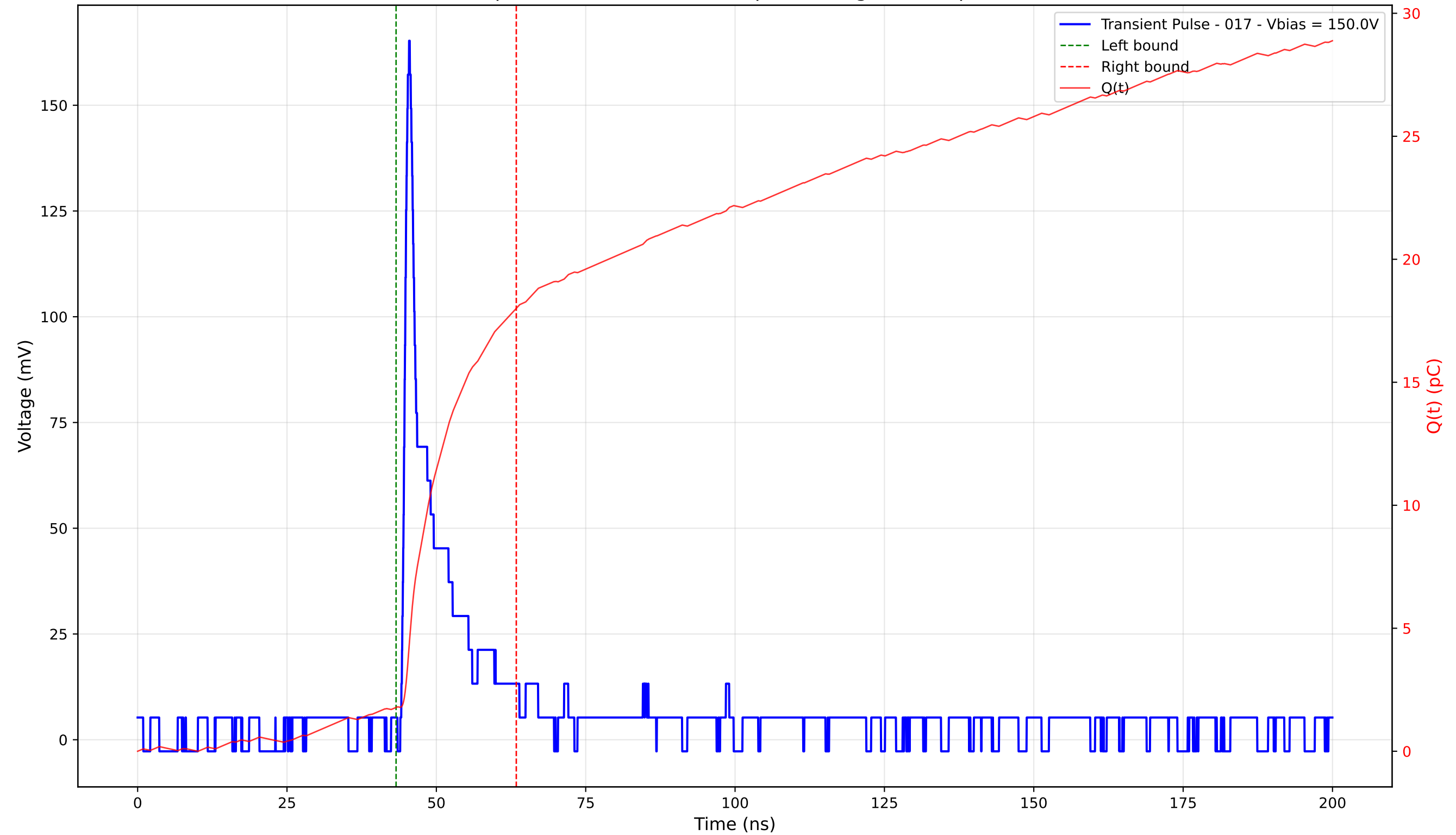
Transient Pulse - Sample: 4003 - Position: 95.0 \mu\text{m} - Charge: 16.23 pC - Rise Time: 0.91 ns
