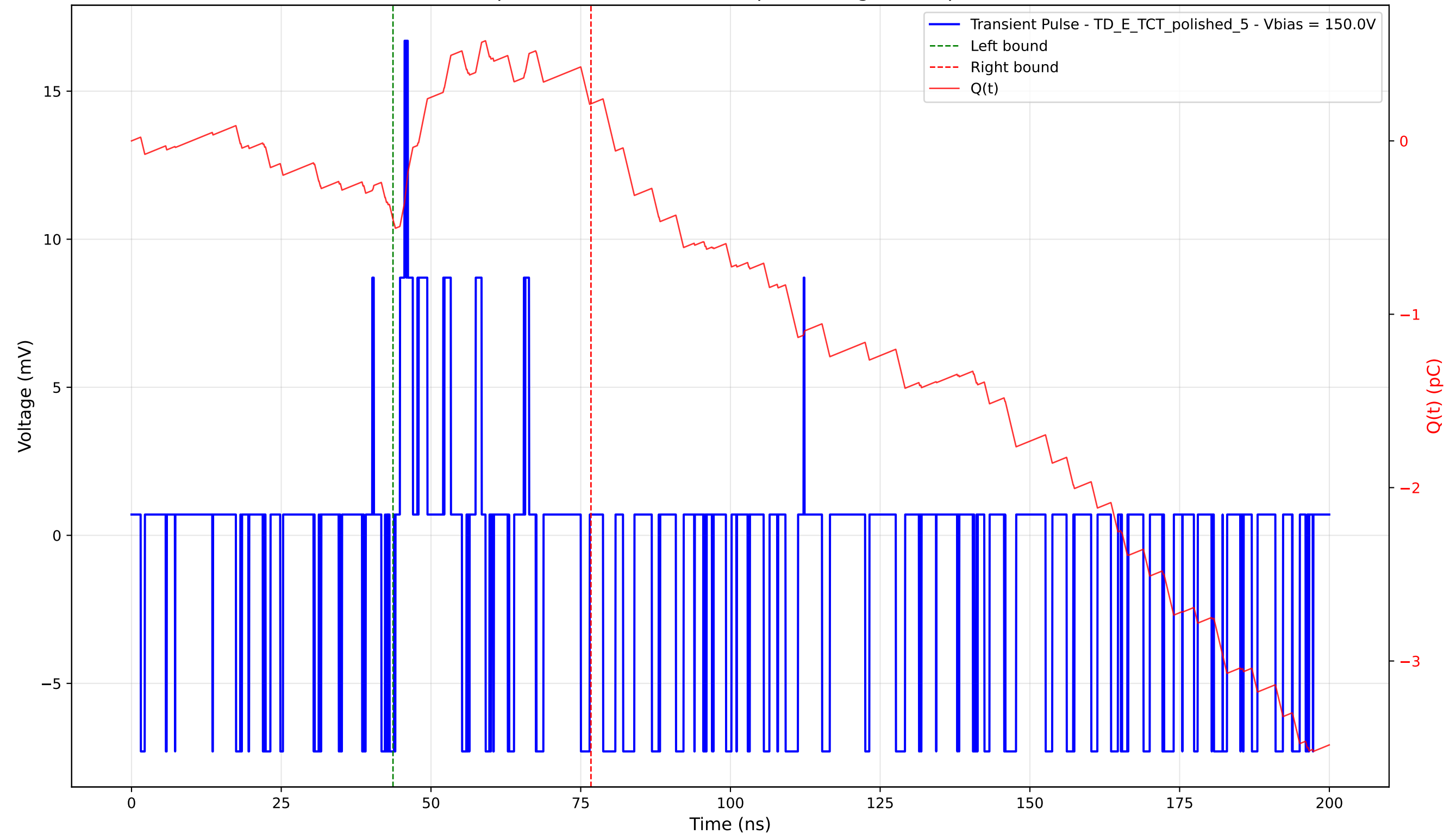
Transient Pulse - Sample: 4003 - Position: 15.0 \mu\text{m} - Charge: 0.67 pC - Rise Time: 0.78 ns
