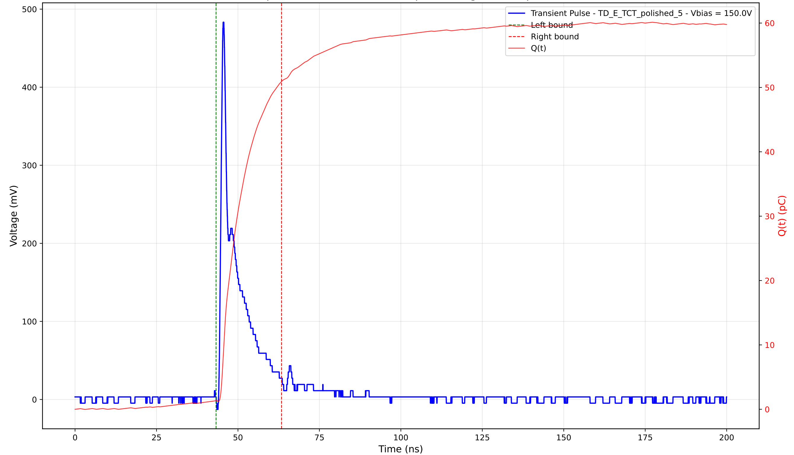
Transient Pulse - Sample: 4003 - Position: 125.0 \mu\text{m} - Charge: 49.58 pC - Rise Time: 0.95 ns
