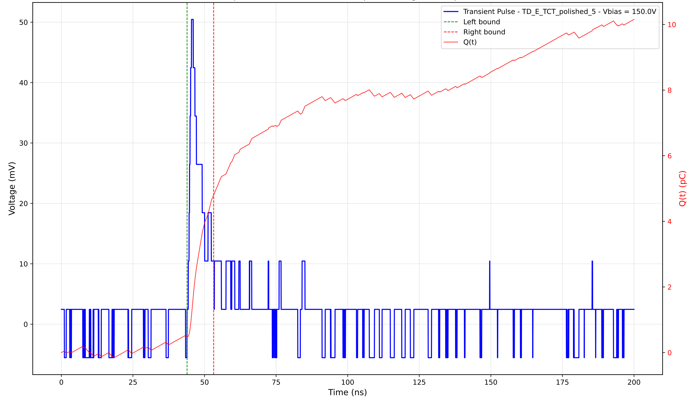
Transient Pulse - Sample: 4003 - Position: 390.0 \mu\text{m} - Charge: 4.33 pC - Rise Time: 1.13 ns
