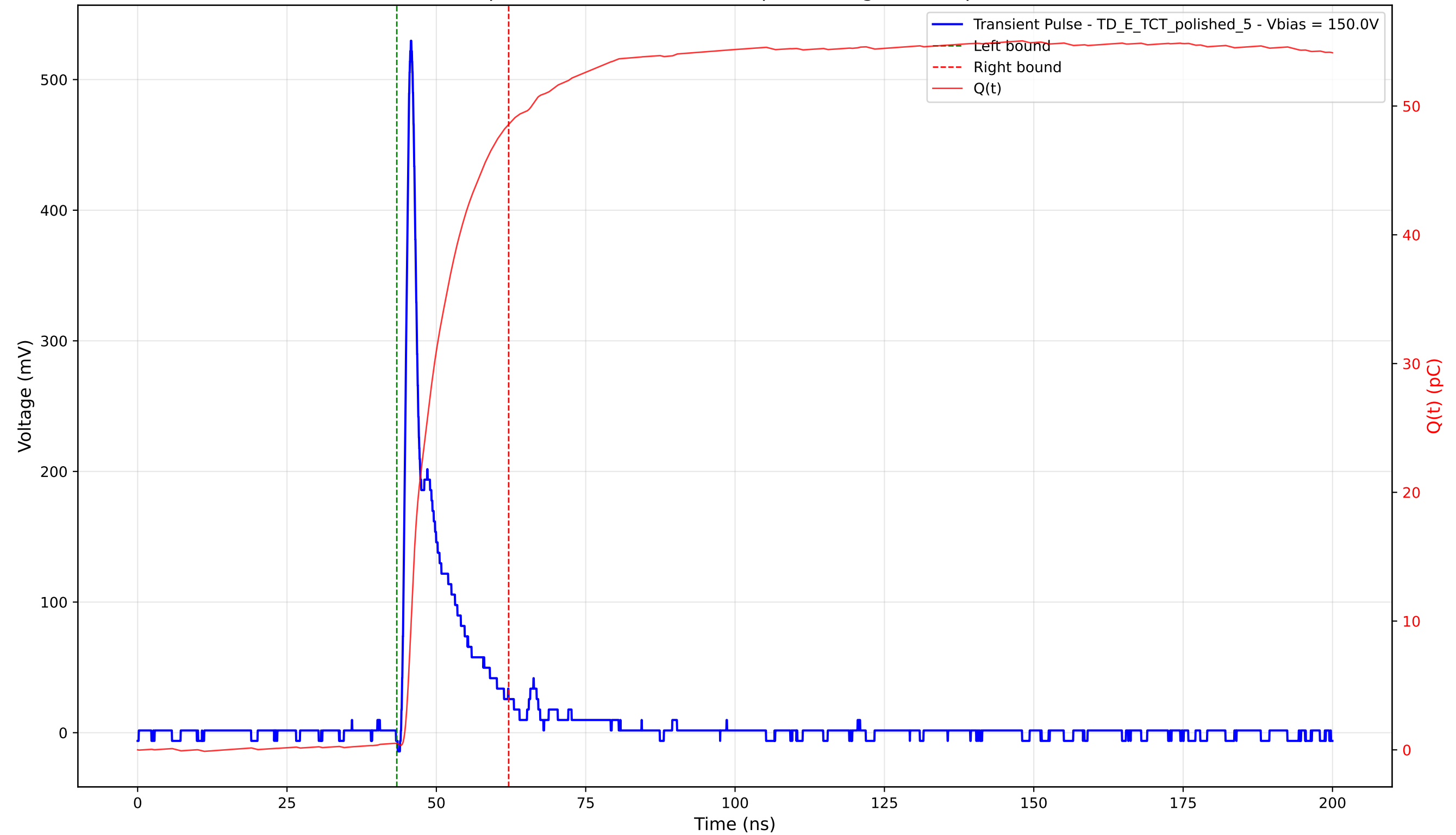
Transient Pulse - Sample: 4003 - Position: 170.0 \mu\text{m} - Charge: 48.09 pC - Rise Time: 1.05 ns
