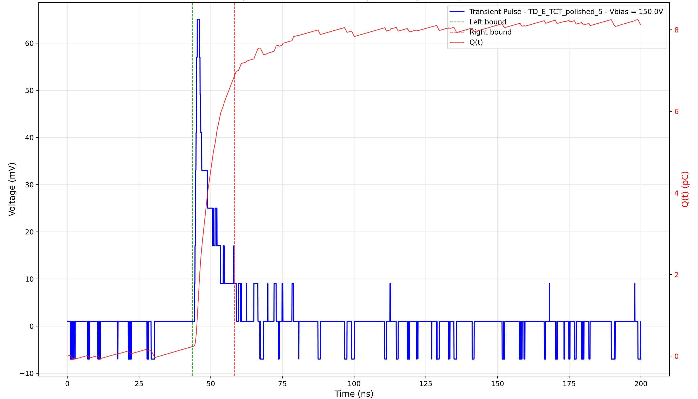
Transient Pulse - Sample: 4003 - Position: 85.0 \mu\text{m} - Charge: 6.63 pC - Rise Time: 0.99 ns
