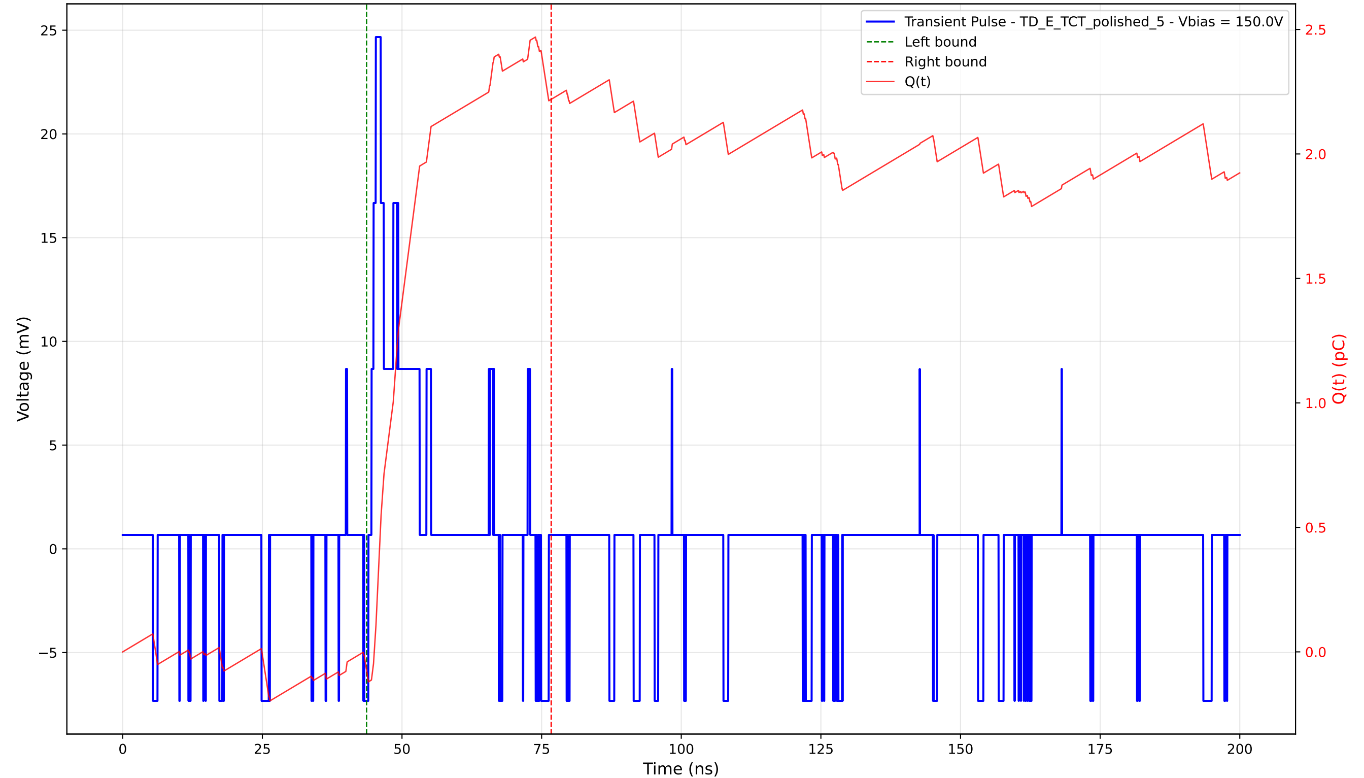
Transient Pulse - Sample: 4003 - Position: 35.0 \mu\text{m} - Charge: 2.29 pC - Rise Time: 0.78 ns
