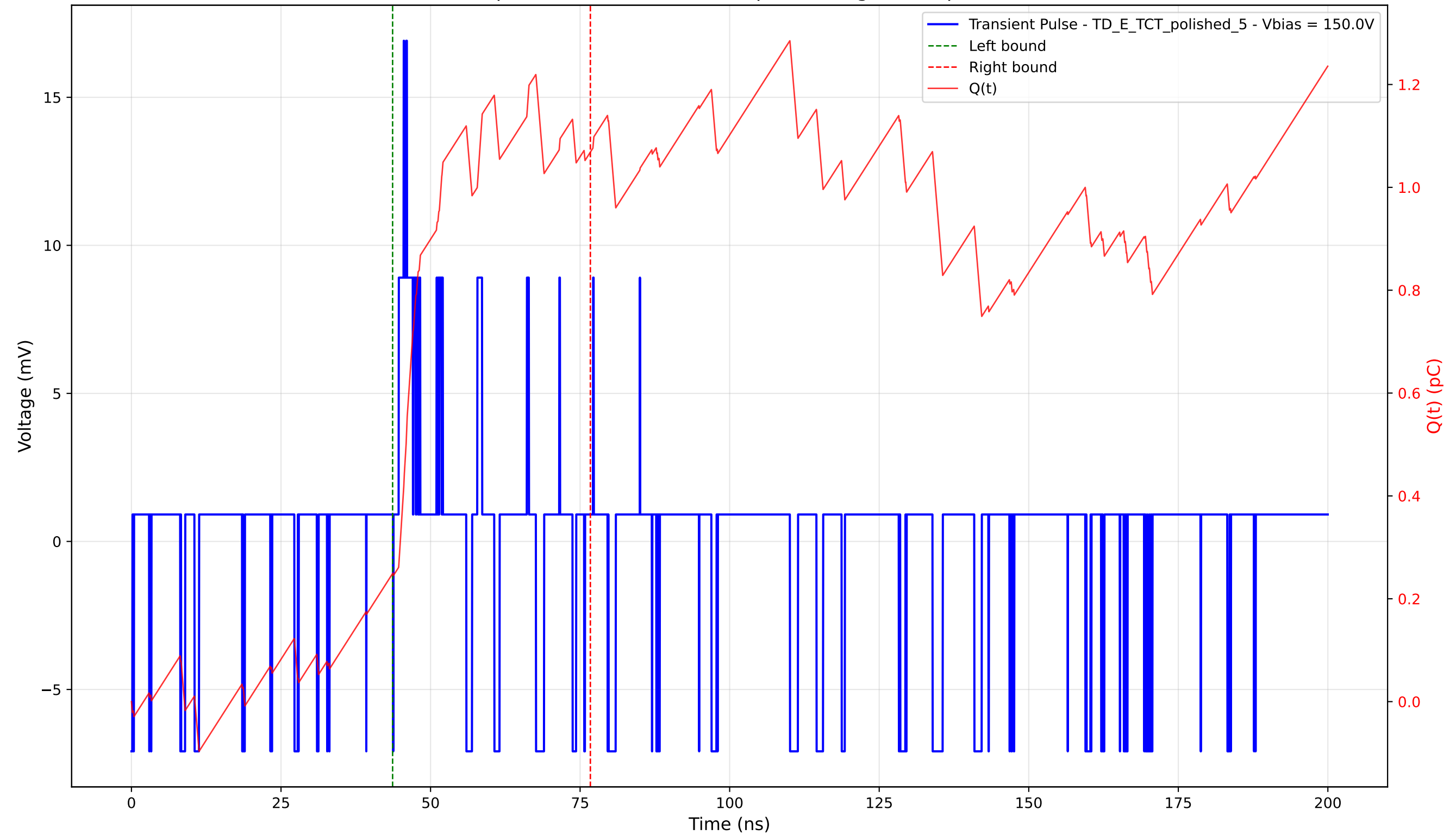
Transient Pulse - Sample: 4003 - Position: 10.0 \mu\text{m} - Charge: 0.82 pC - Rise Time: 0.84 ns
