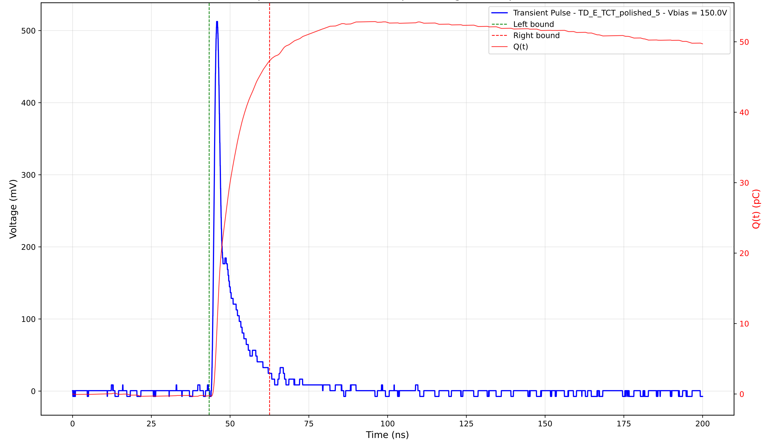
Transient Pulse - Sample: 4003 - Position: 185.0 \mu\text{m} - Charge: 47.53 pC - Rise Time: 1.11 ns
