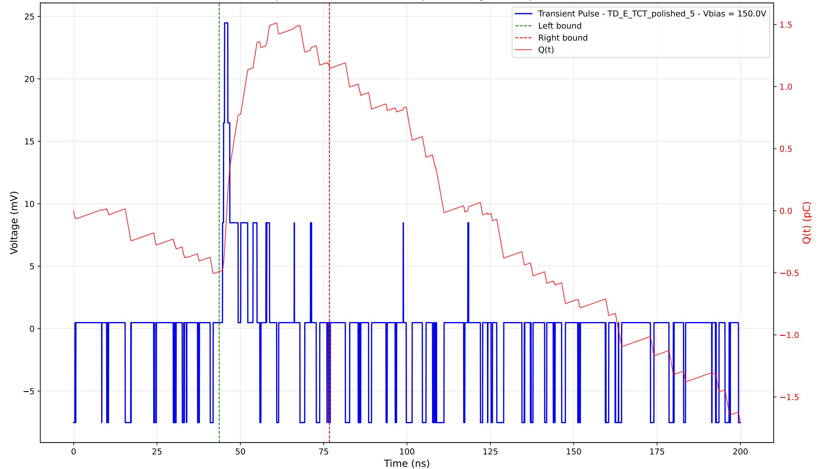
Transient Pulse - Sample: 4003 - Position: 25.0 \mu\text{m} - Charge: 1.65 pC - Rise Time: 0.62 ns
