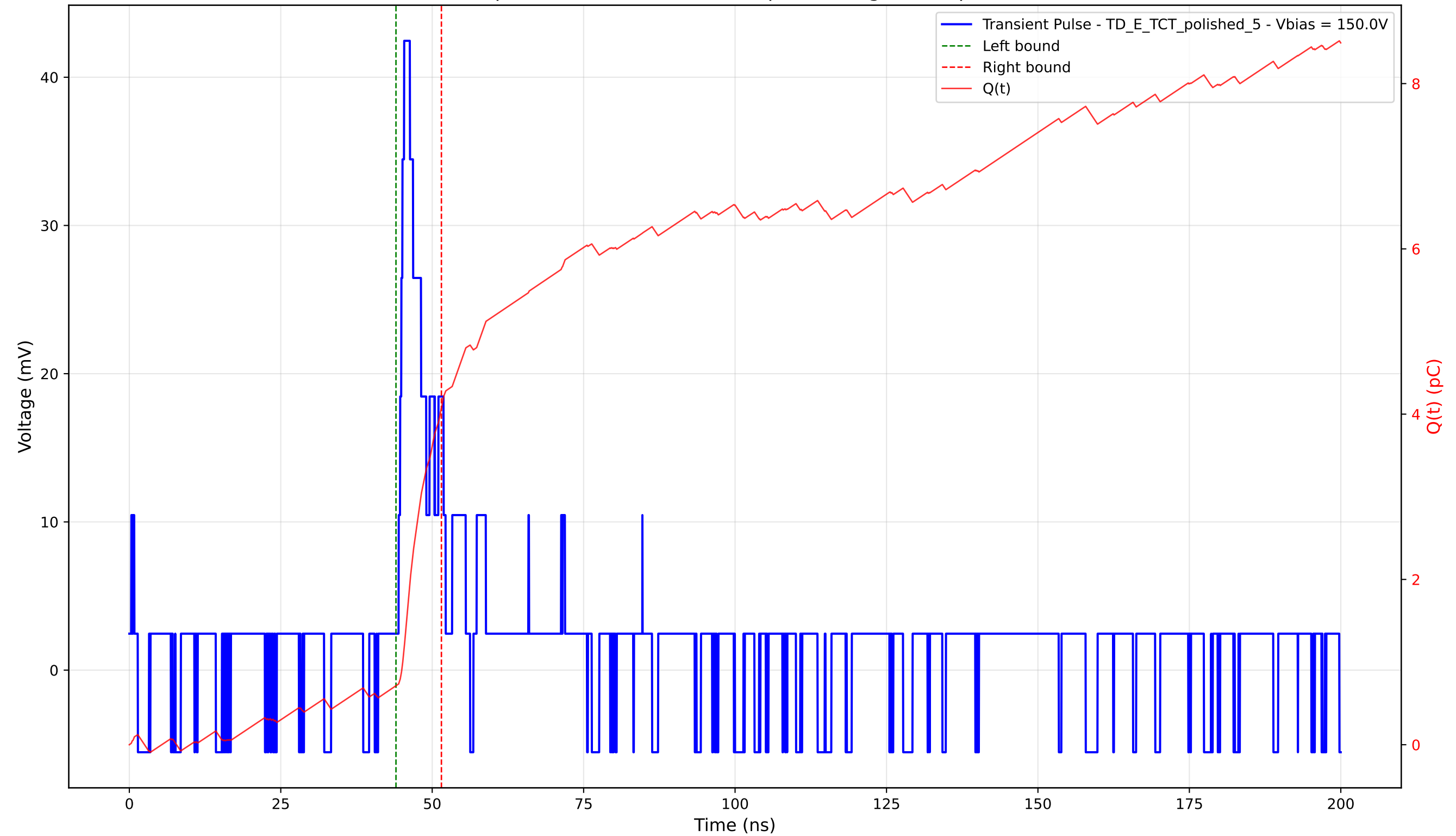
Transient Pulse - Sample: 4003 - Position: 400.0 \mu\text{m} - Charge: 3.37 pC - Rise Time: 0.92 ns
