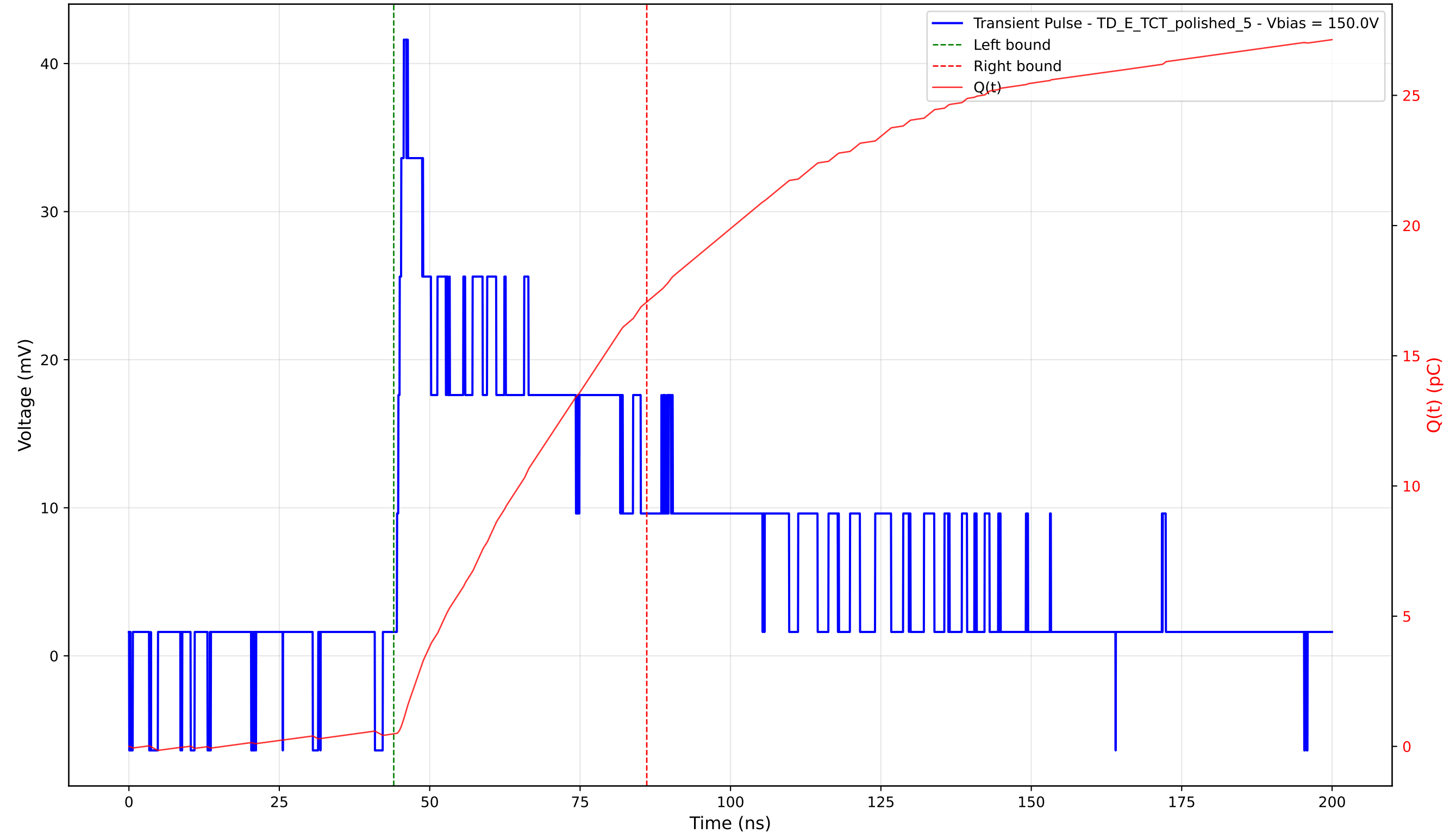
Transient Pulse - Sample: 4003 - Position: 315.0 \mu\text{m} - Charge: 16.58 pC - Rise Time: 1.13 ns
