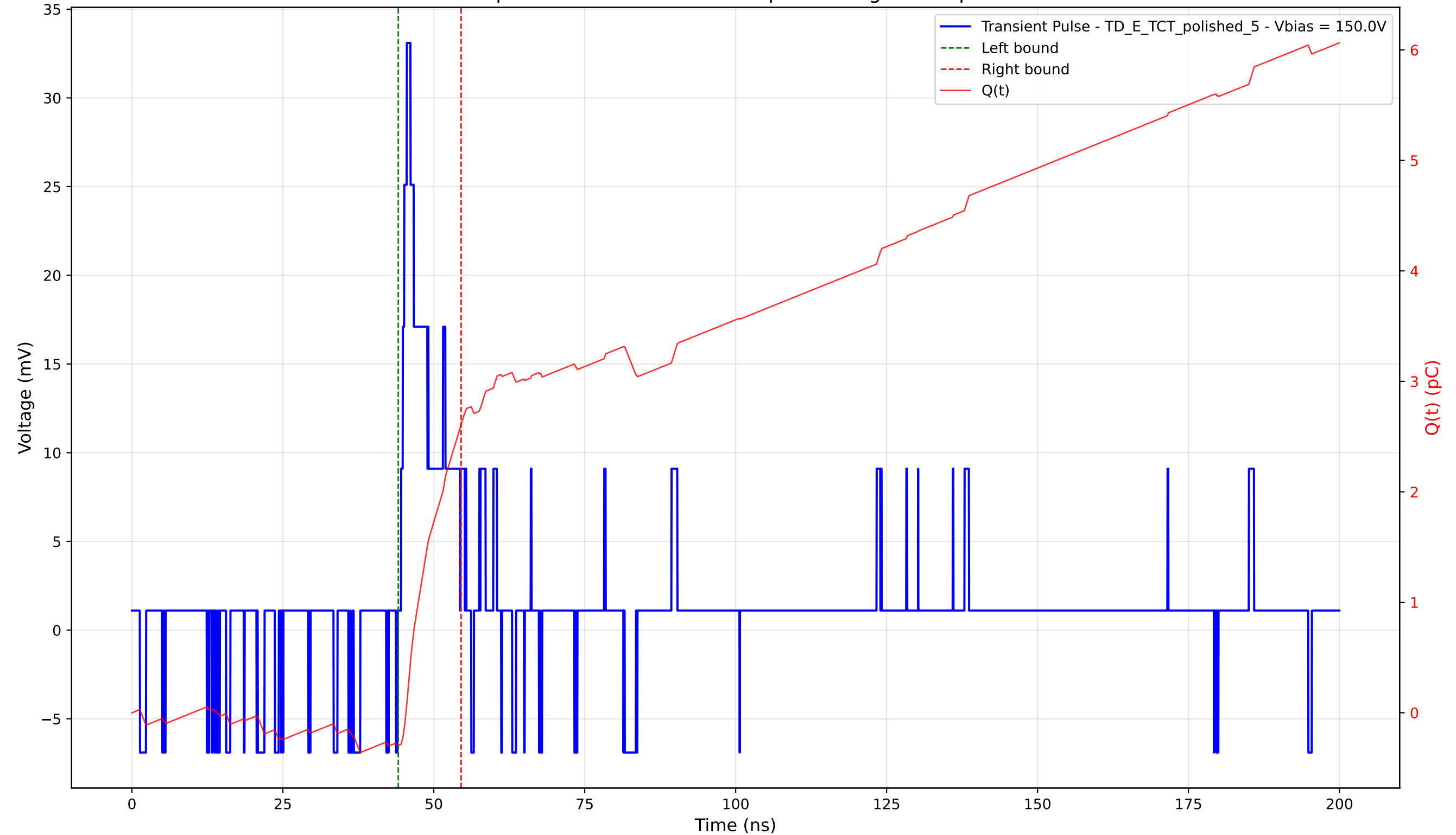
Transient Pulse - Sample: 4003 - Position: 350.0 \mu\text{m} - Charge: 2.90 pC - Rise Time: 0.95 ns
