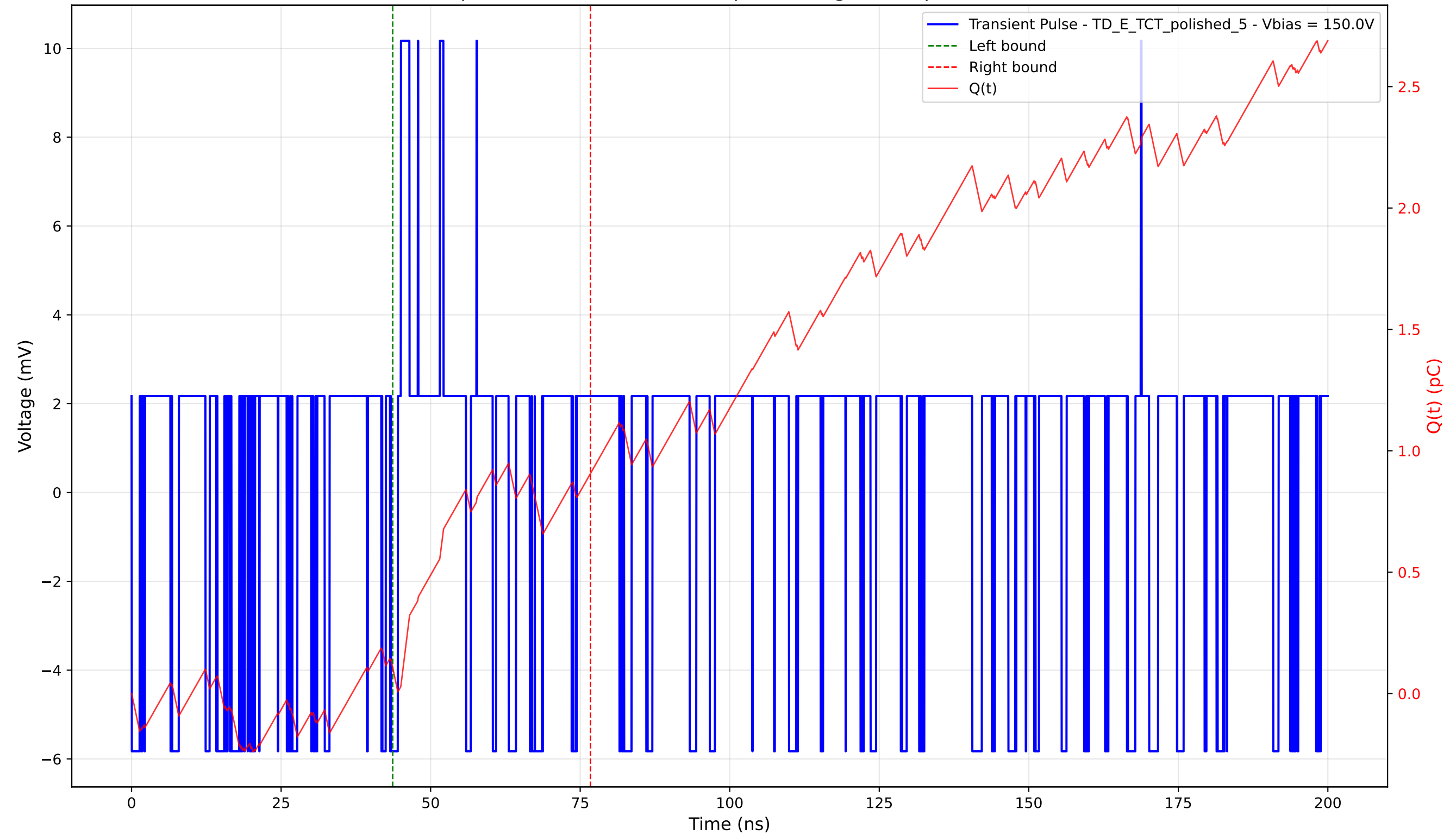
Transient Pulse - Sample: 4003 - Position: 425.0 \mu\text{m} - Charge: 0.80 pC - Rise Time: 0.00 ns (N/A)
