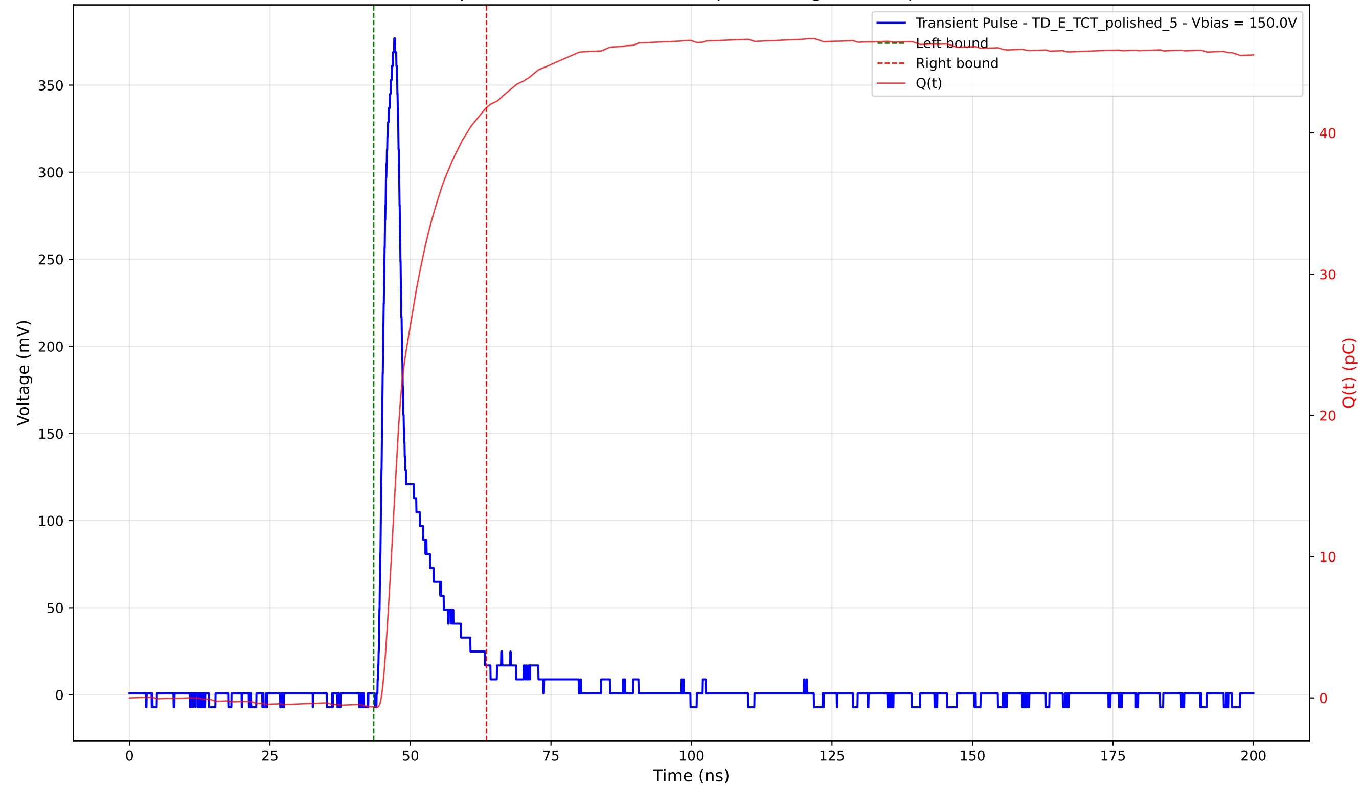
Transient Pulse - Sample: 4003 - Position: 250.0 \mu\text{m} - Charge: 42.41 pC - Rise Time: 1.89 ns
