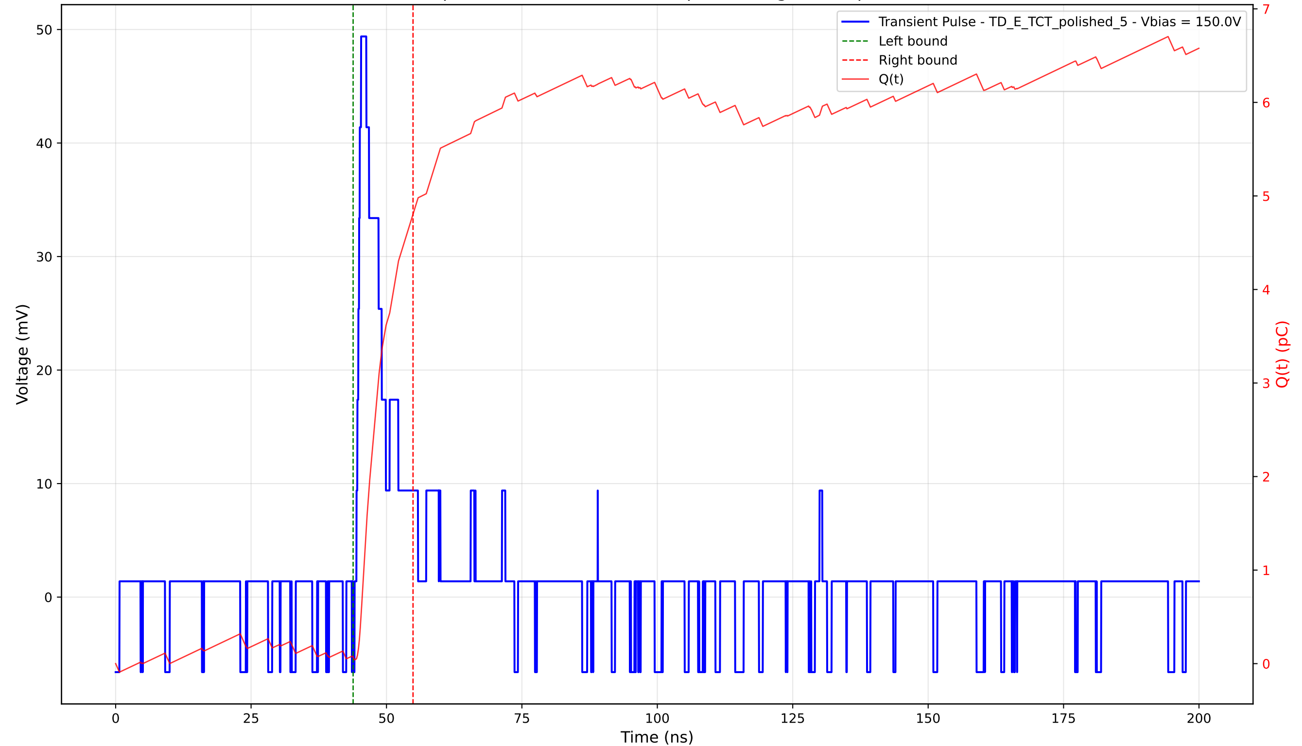
Transient Pulse - Sample: 4003 - Position: 385.0 \mu\text{m} - Charge: 4.74 pC - Rise Time: 0.85 ns
