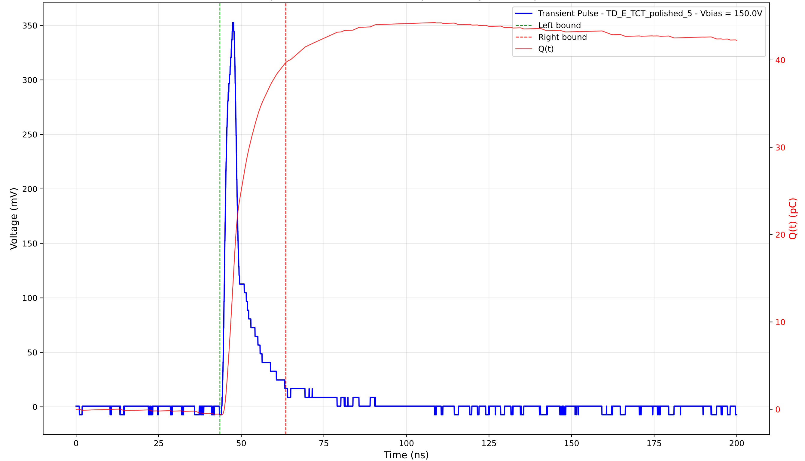
Transient Pulse - Sample: 4003 - Position: 260.0 \mu\text{m} - Charge: 40.27 pC - Rise Time: 2.35 ns
