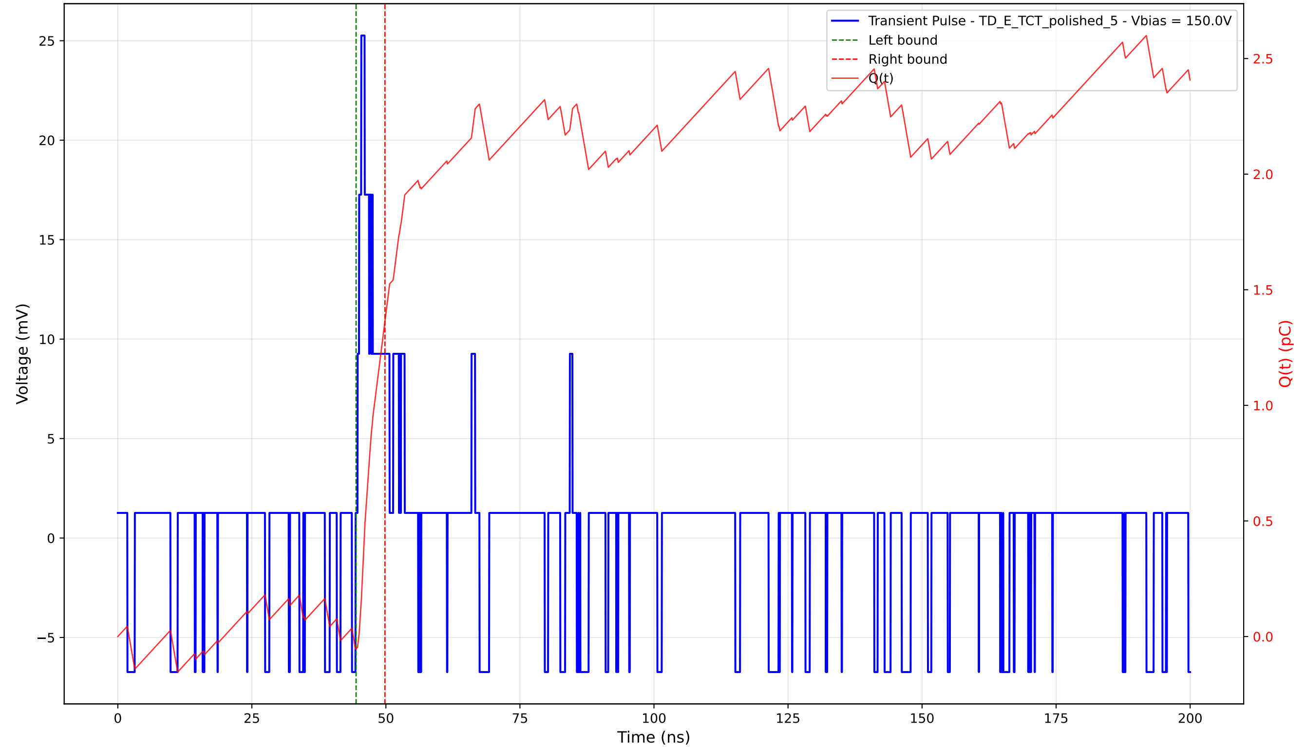
Transient Pulse - Sample: 4003 - Position: 30.0 \mu\text{m} - Charge: 1.42 pC - Rise Time: 0.70 ns
