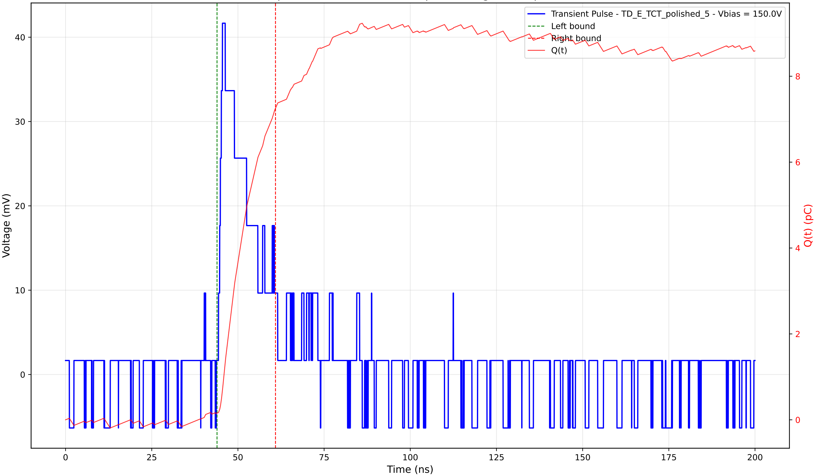
Transient Pulse - Sample: 4003 - Position: 50.0 \mu\text{m} - Charge: 7.10 pC - Rise Time: 1.15 ns
