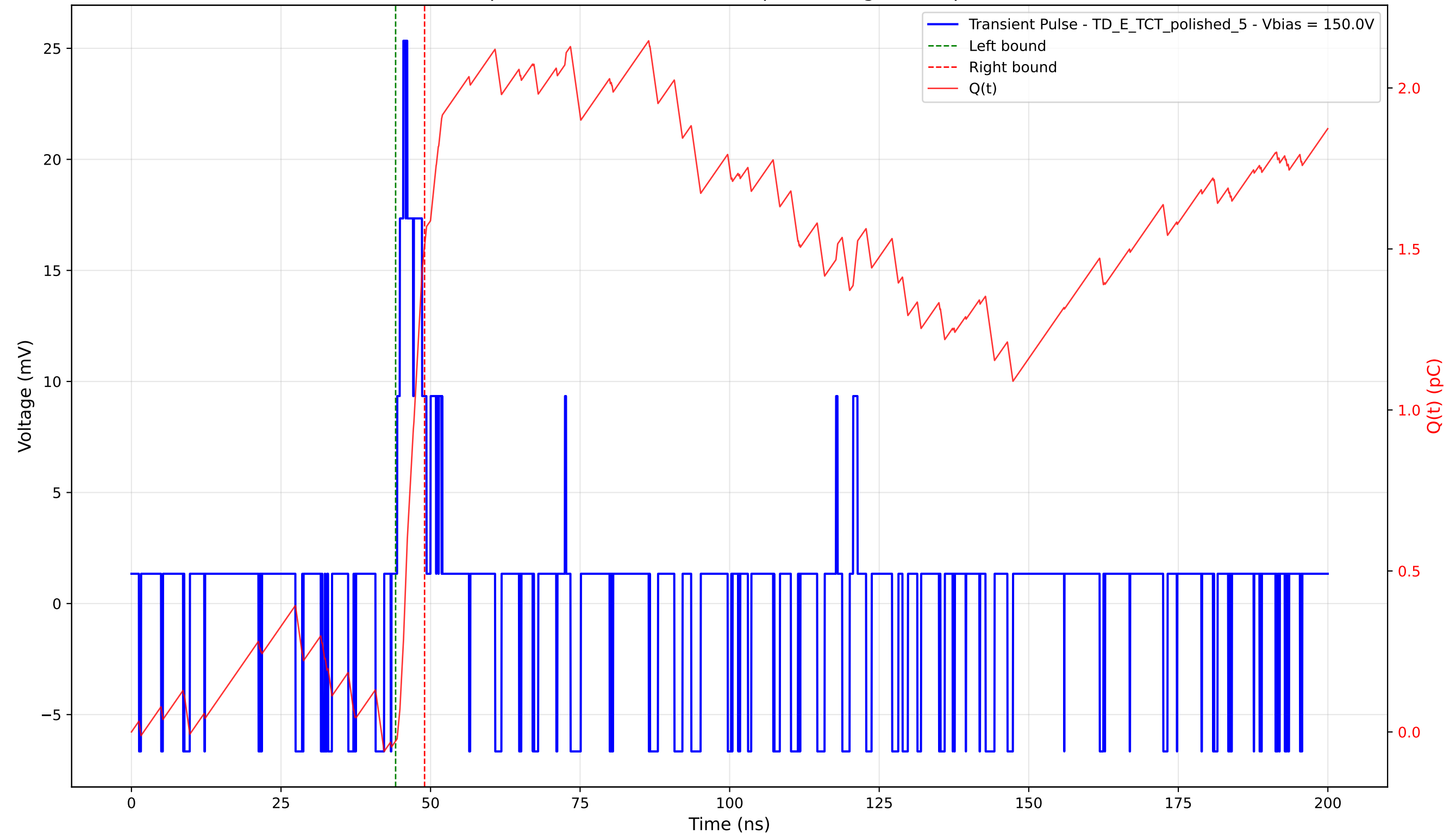
Transient Pulse - Sample: 4003 - Position: 410.0 \mu\text{m} - Charge: 1.54 pC - Rise Time: 1.04 ns
