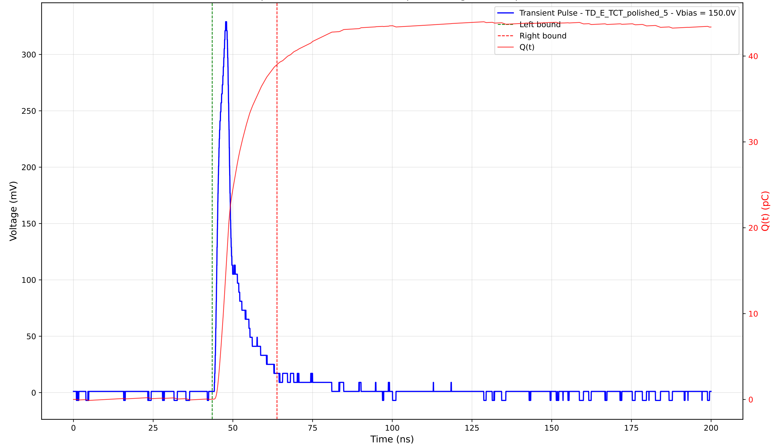
Transient Pulse - Sample: 4003 - Position: 270.0 \mu\text{m} - Charge: 38.98 pC - Rise Time: 2.68 ns
