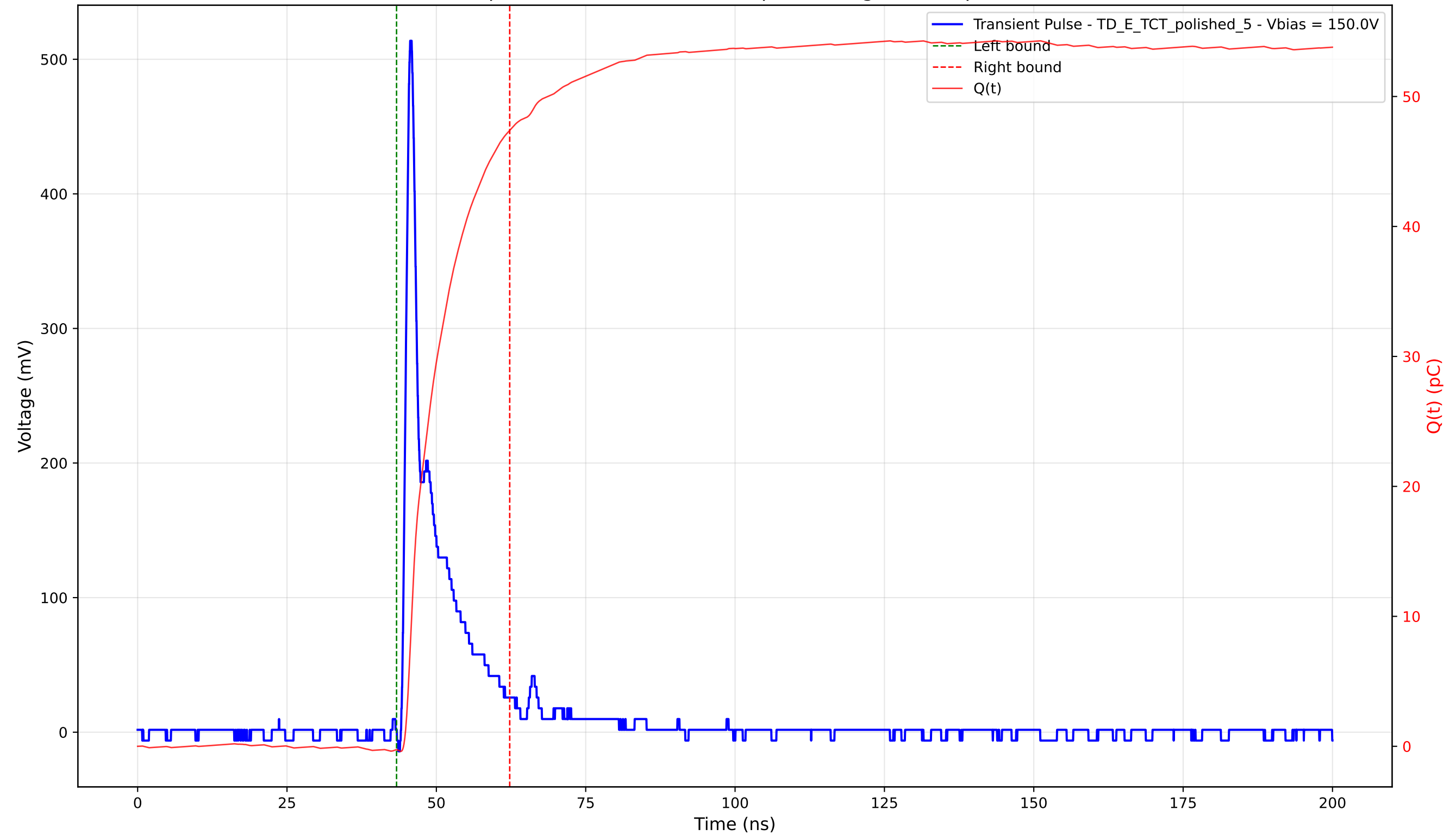
Transient Pulse - Sample: 4003 - Position: 165.0 \mu\text{m} - Charge: 47.66 pC - Rise Time: 1.01 ns
