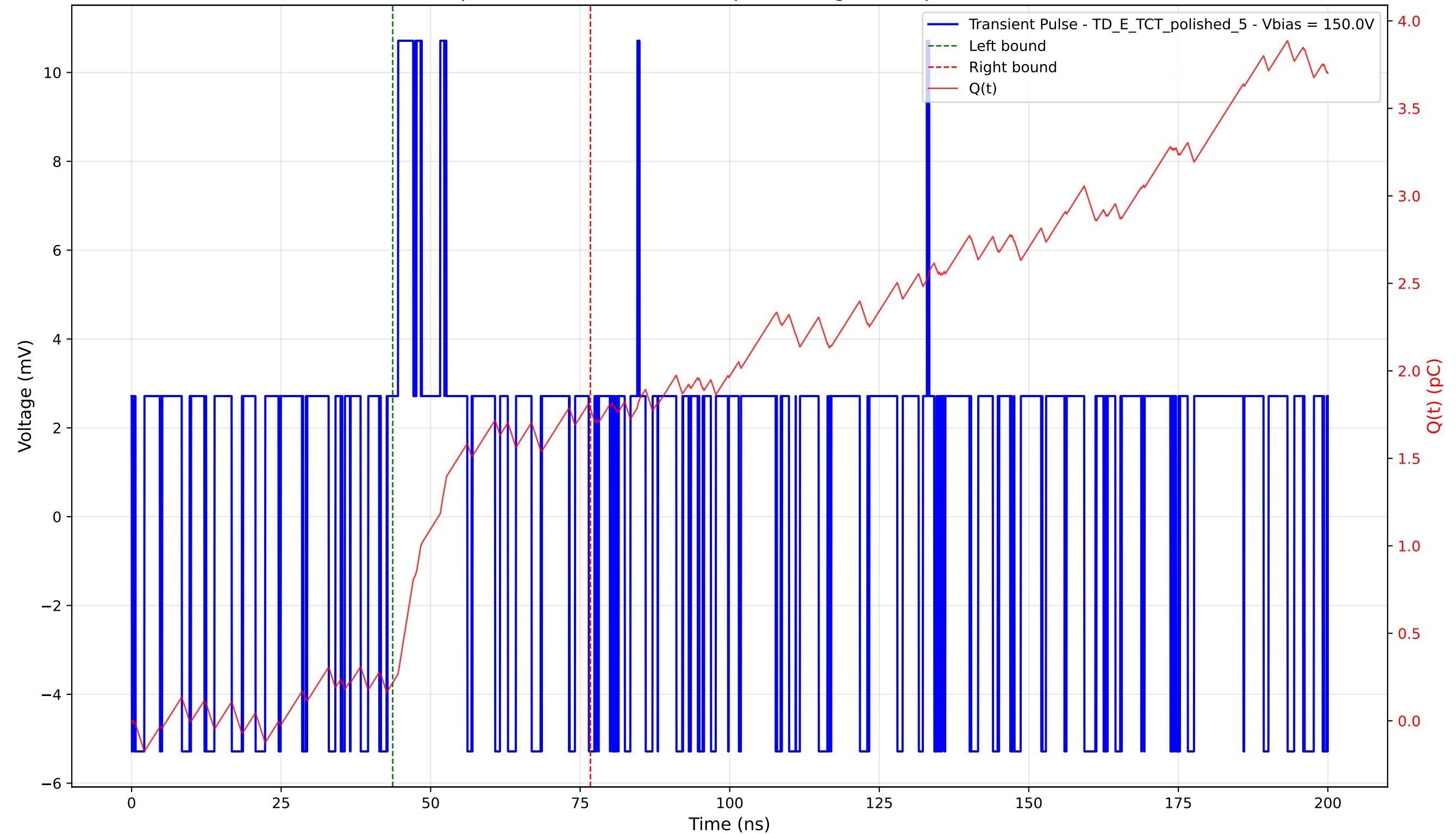
Transient Pulse - Sample: 4003 - Position: 420.0 \mu\text{m} - Charge: 1.57 pC - Rise Time: 0.00 ns (N/A)
