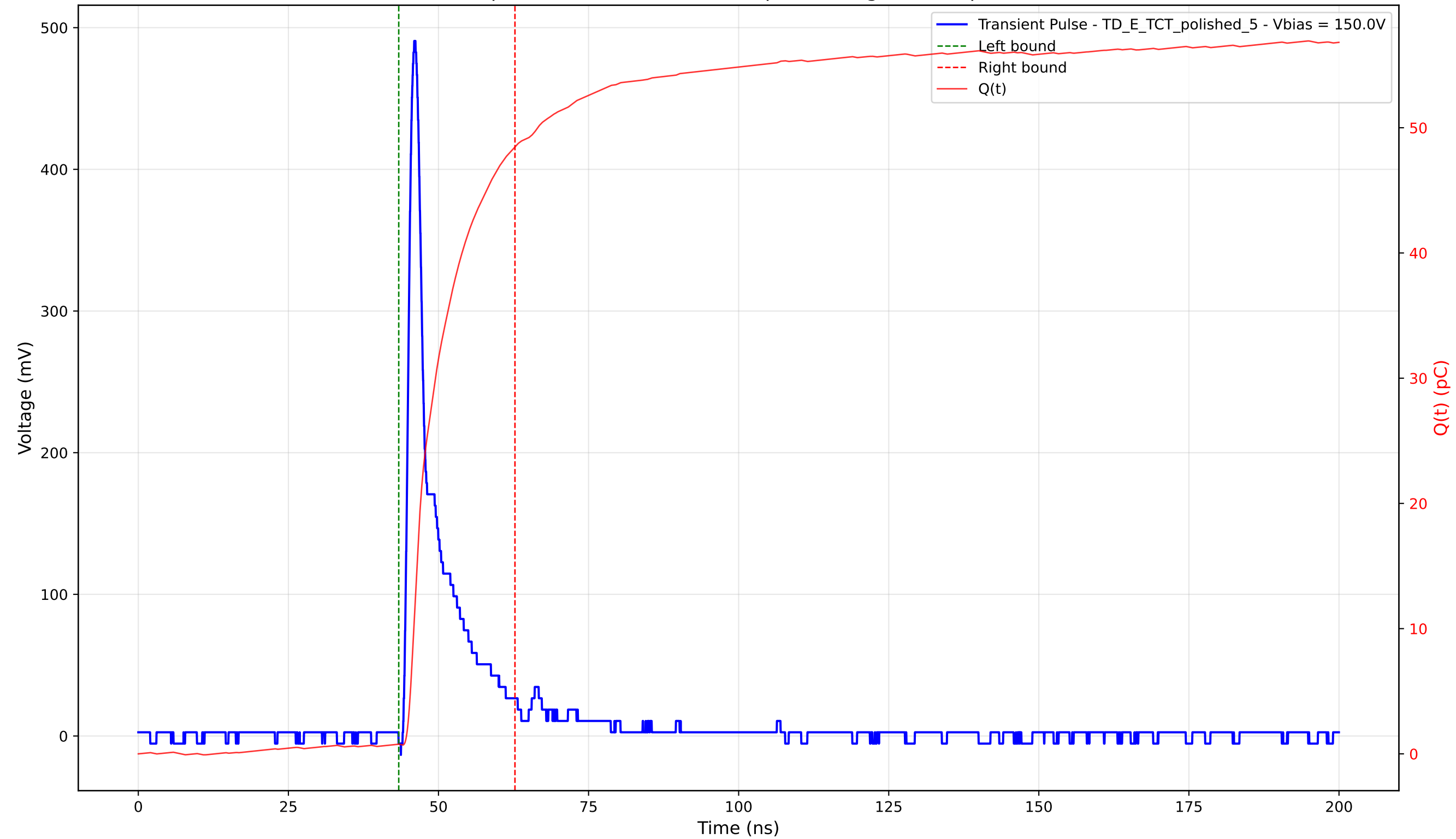
Transient Pulse - Sample: 4003 - Position: 205.0 \mu\text{m} - Charge: 47.70 pC - Rise Time: 1.18 ns
