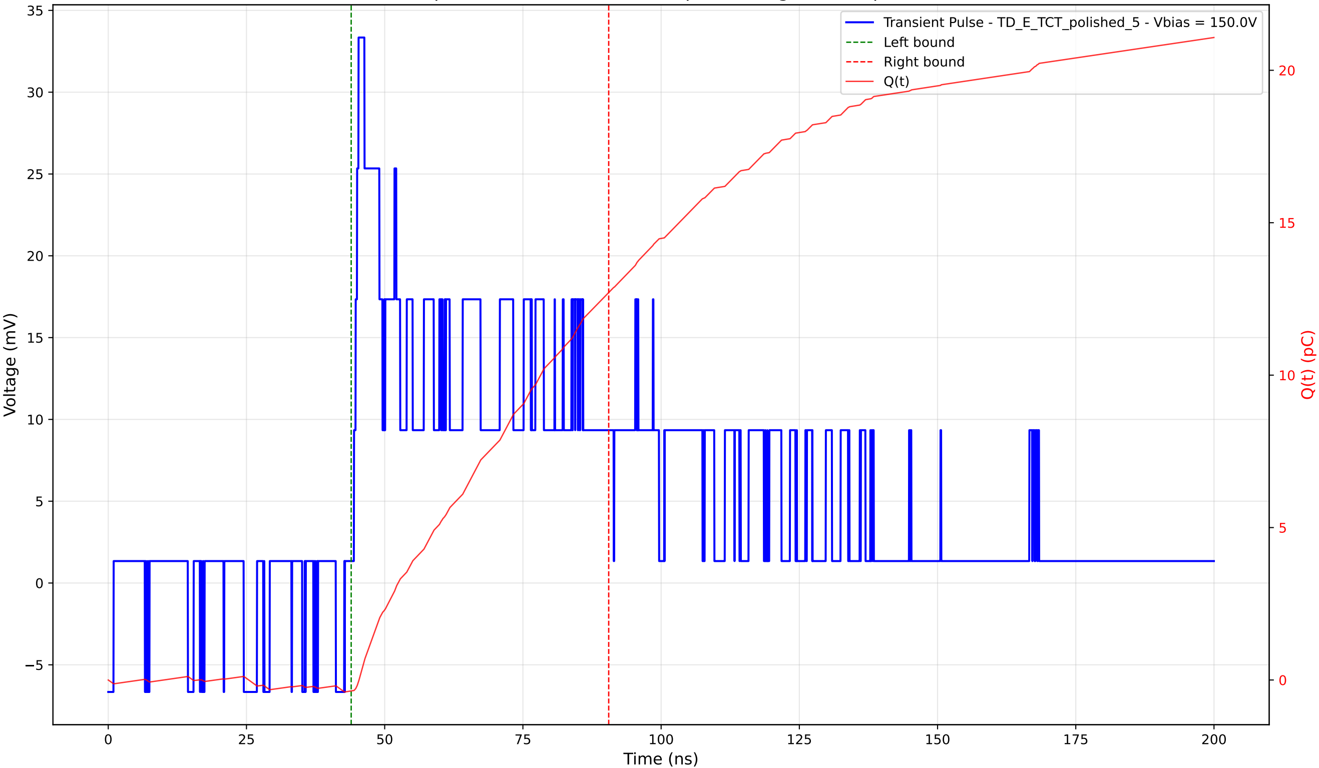
Transient Pulse - Sample: 4003 - Position: 320.0 \mu\text{m} - Charge: 13.08 pC - Rise Time: 0.84 ns
