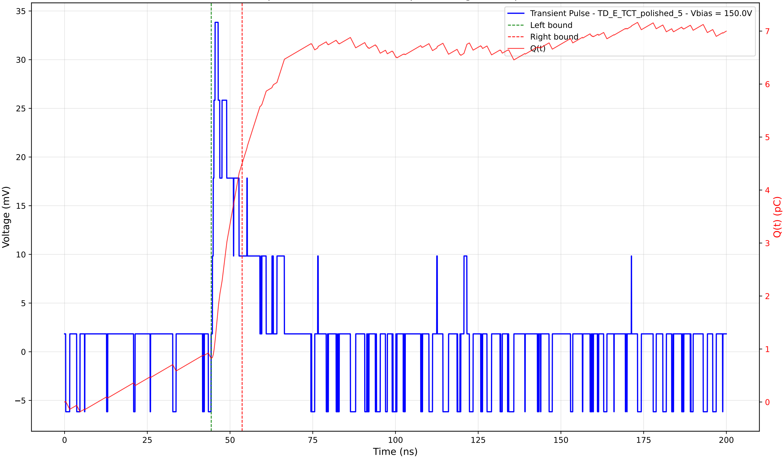
Transient Pulse - Sample: 4003 - Position: 45.0 \mu\text{m} - Charge: 3.68 pC - Rise Time: 0.82 ns
