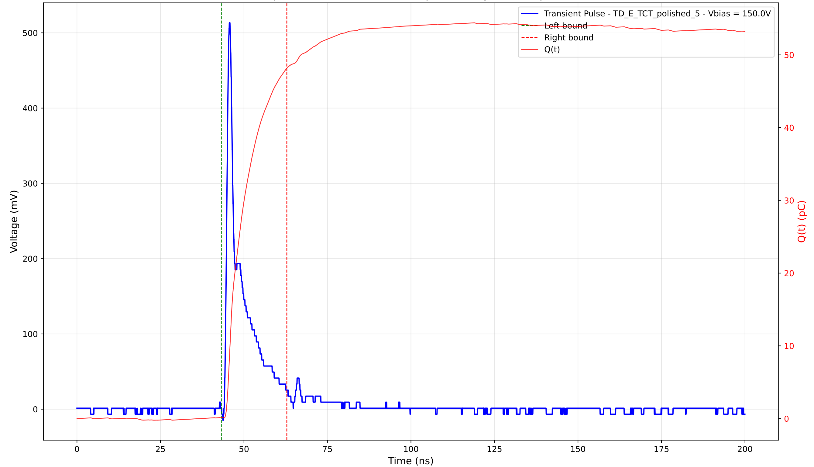
Transient Pulse - Sample: 4003 - Position: 160.0 \mu\text{m} - Charge: 47.97 pC - Rise Time: 1.02 ns
