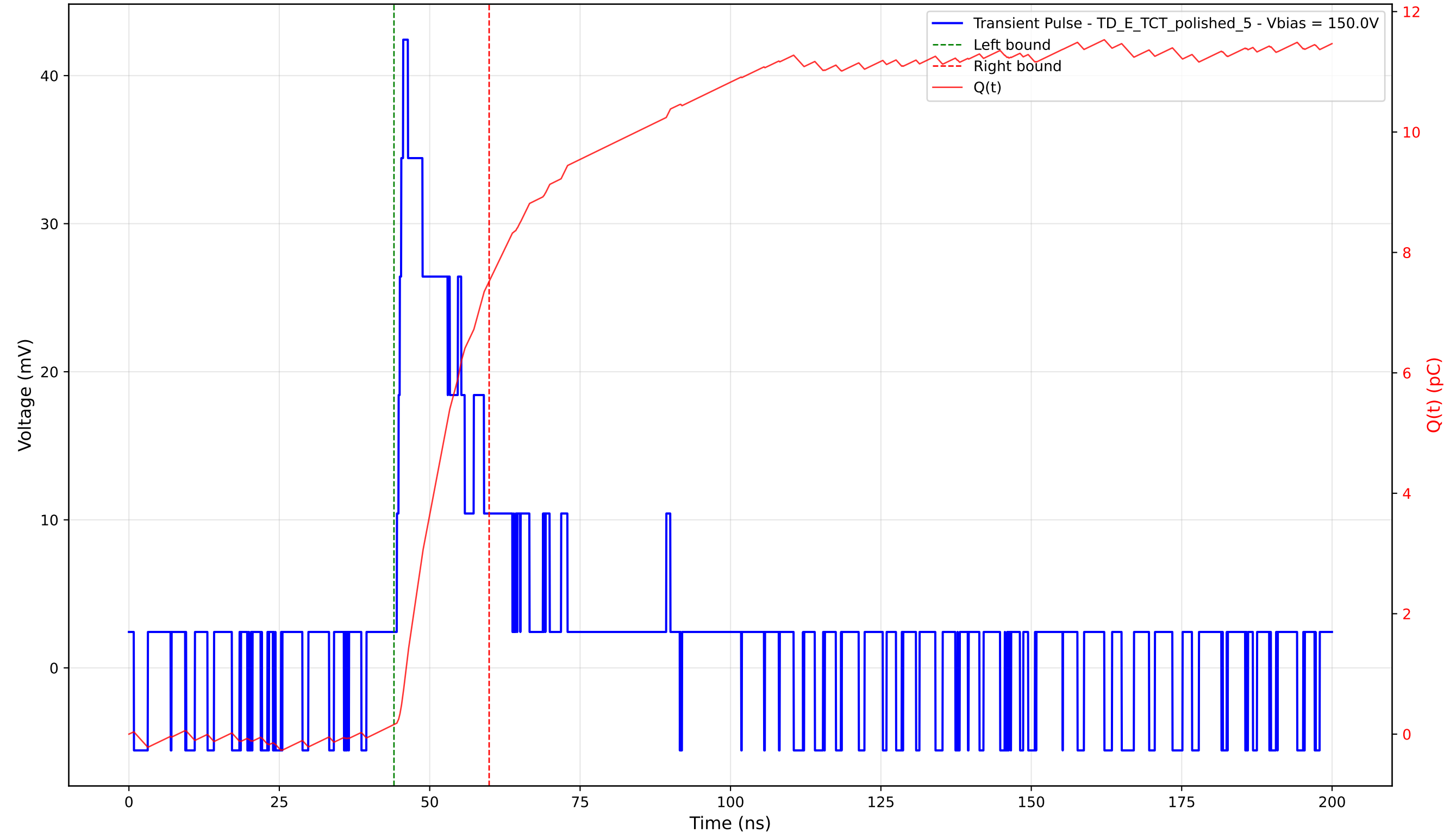
Transient Pulse - Sample: 4003 - Position: 55.0 \mu\text{m} - Charge: 7.36 pC - Rise Time: 1.06 ns
