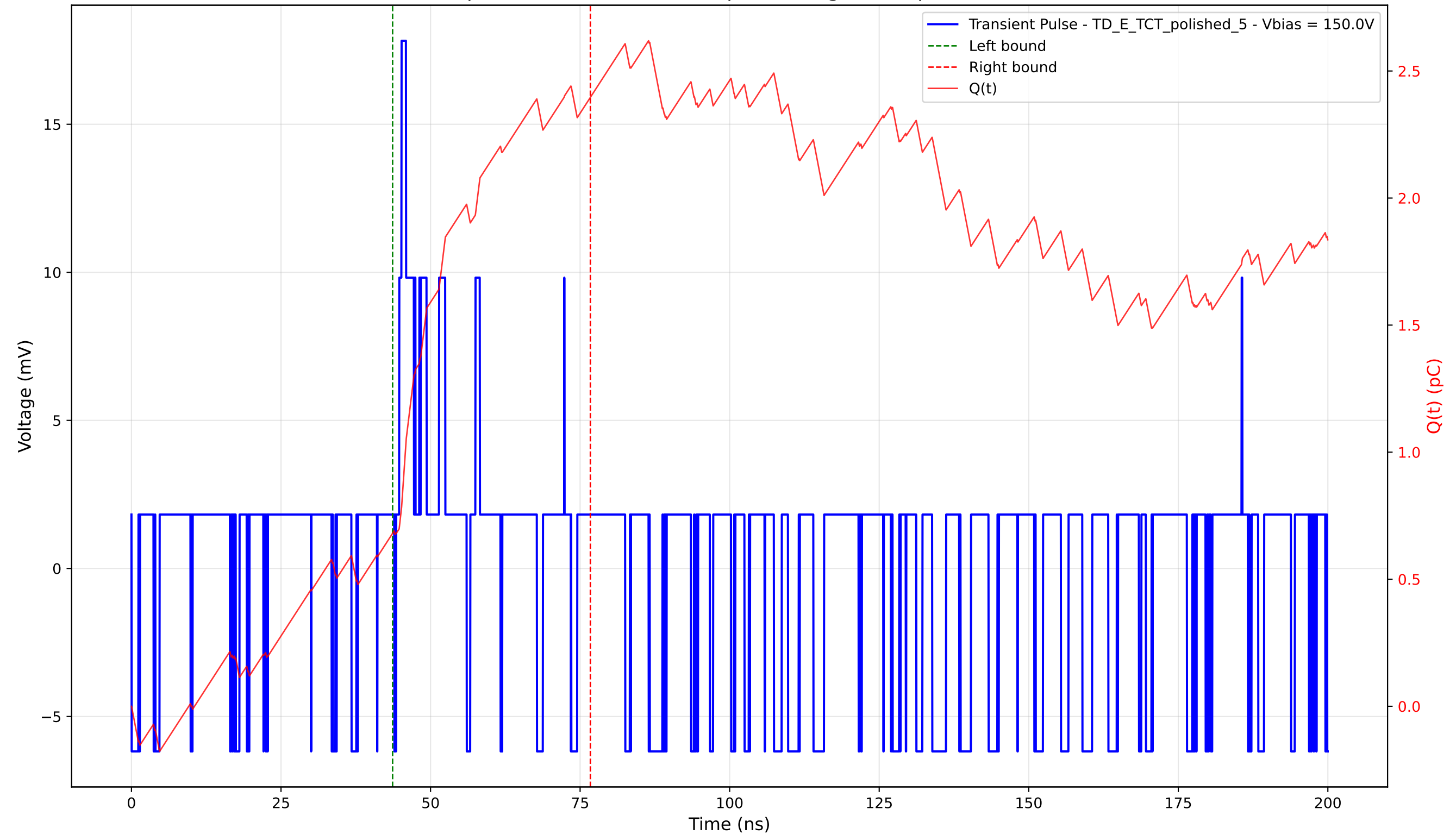
Transient Pulse - Sample: 4003 - Position: 70.0 \mu\text{m} - Charge: 1.71 pC - Rise Time: 0.00 ns (N/A)
