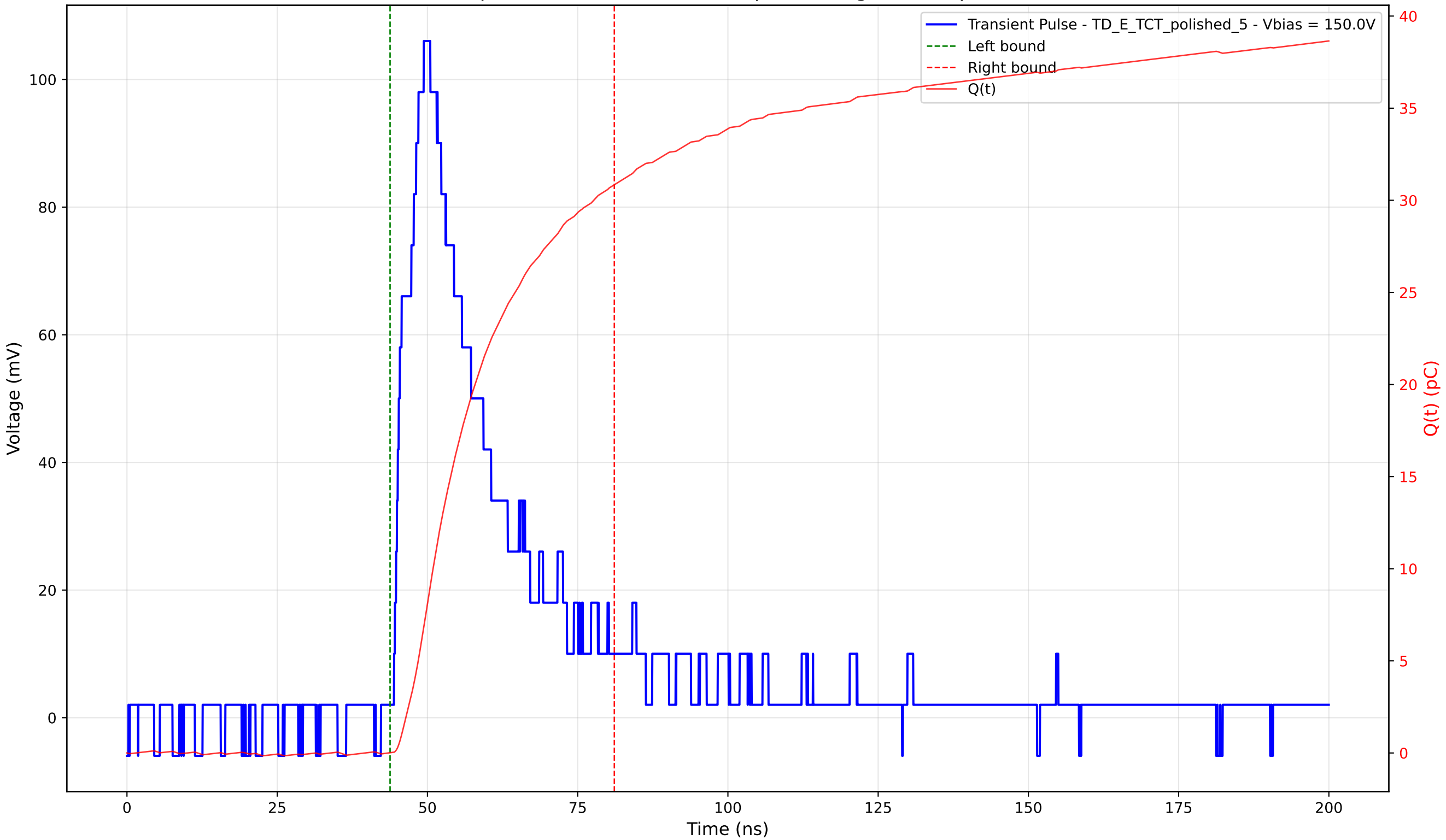
Transient Pulse - Sample: 4003 - Position: 300.0 \mu\text{m} - Charge: 30.83 pC - Rise Time: 3.94 ns
