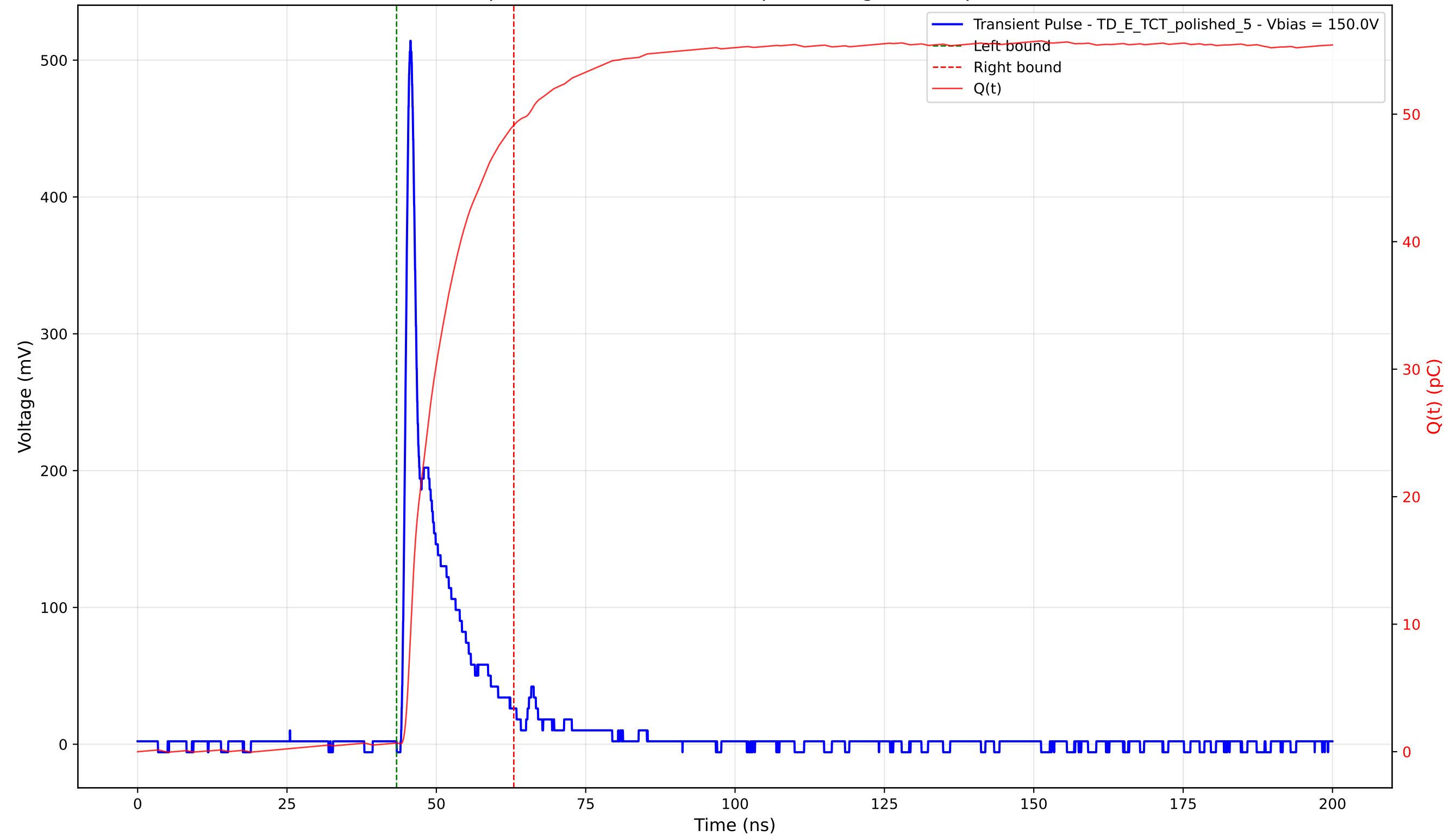
Transient Pulse - Sample: 4003 - Position: 155.0 \mu\text{m} - Charge: 48.44 pC - Rise Time: 1.02 ns
