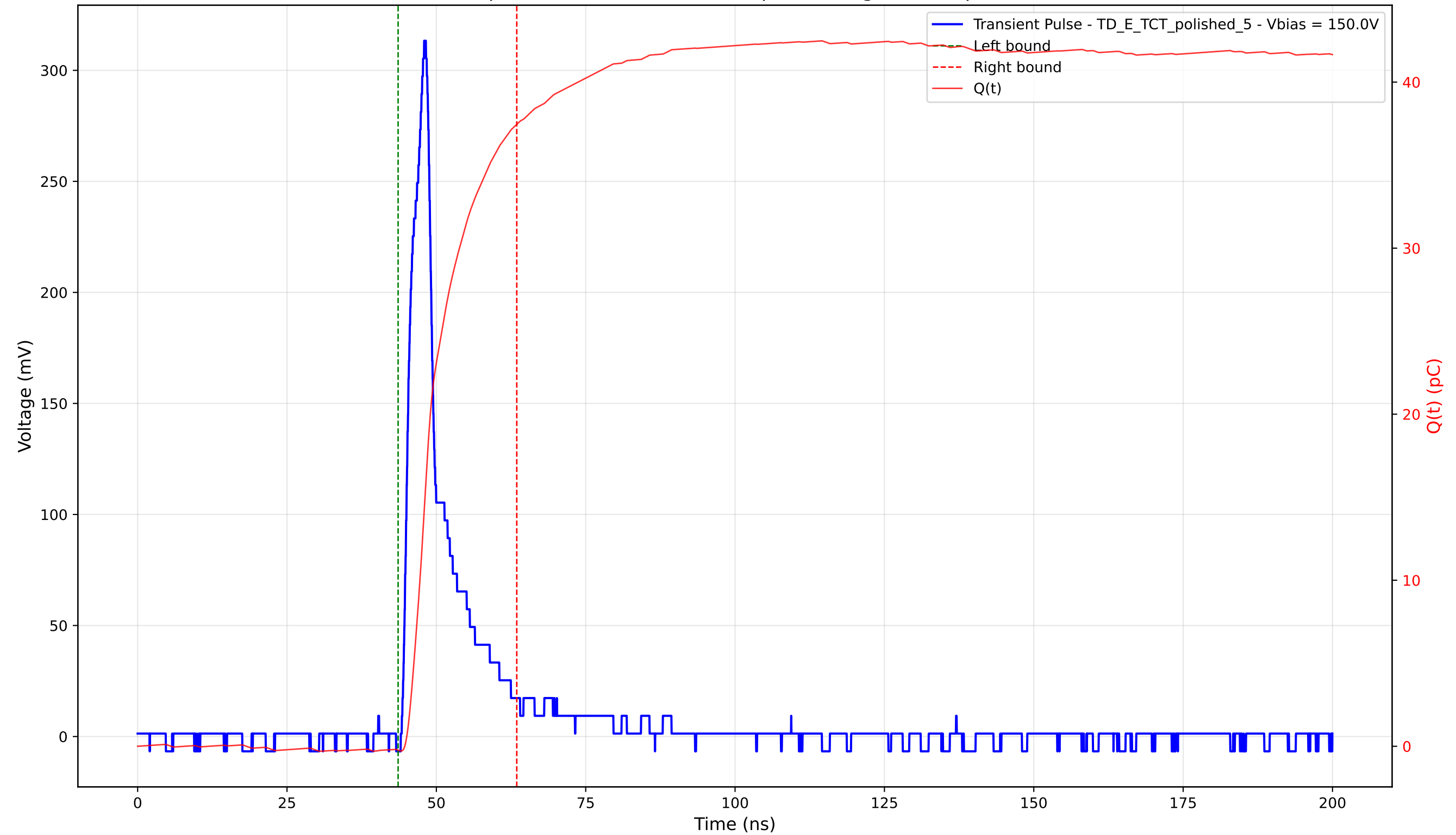
Transient Pulse - Sample: 4003 - Position: 275.0 \mu\text{m} - Charge: 37.69 pC - Rise Time: 3.00 ns
