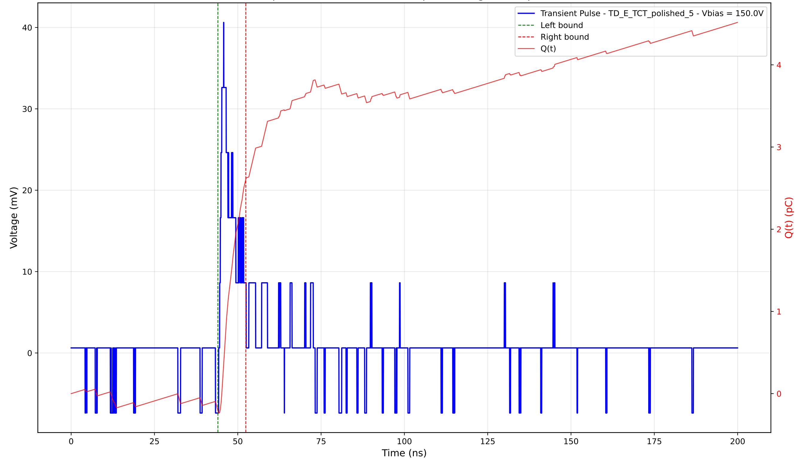
Transient Pulse - Sample: 4003 - Position: 375.0 \mu\text{m} - Charge: 2.81 pC - Rise Time: 1.21 ns
