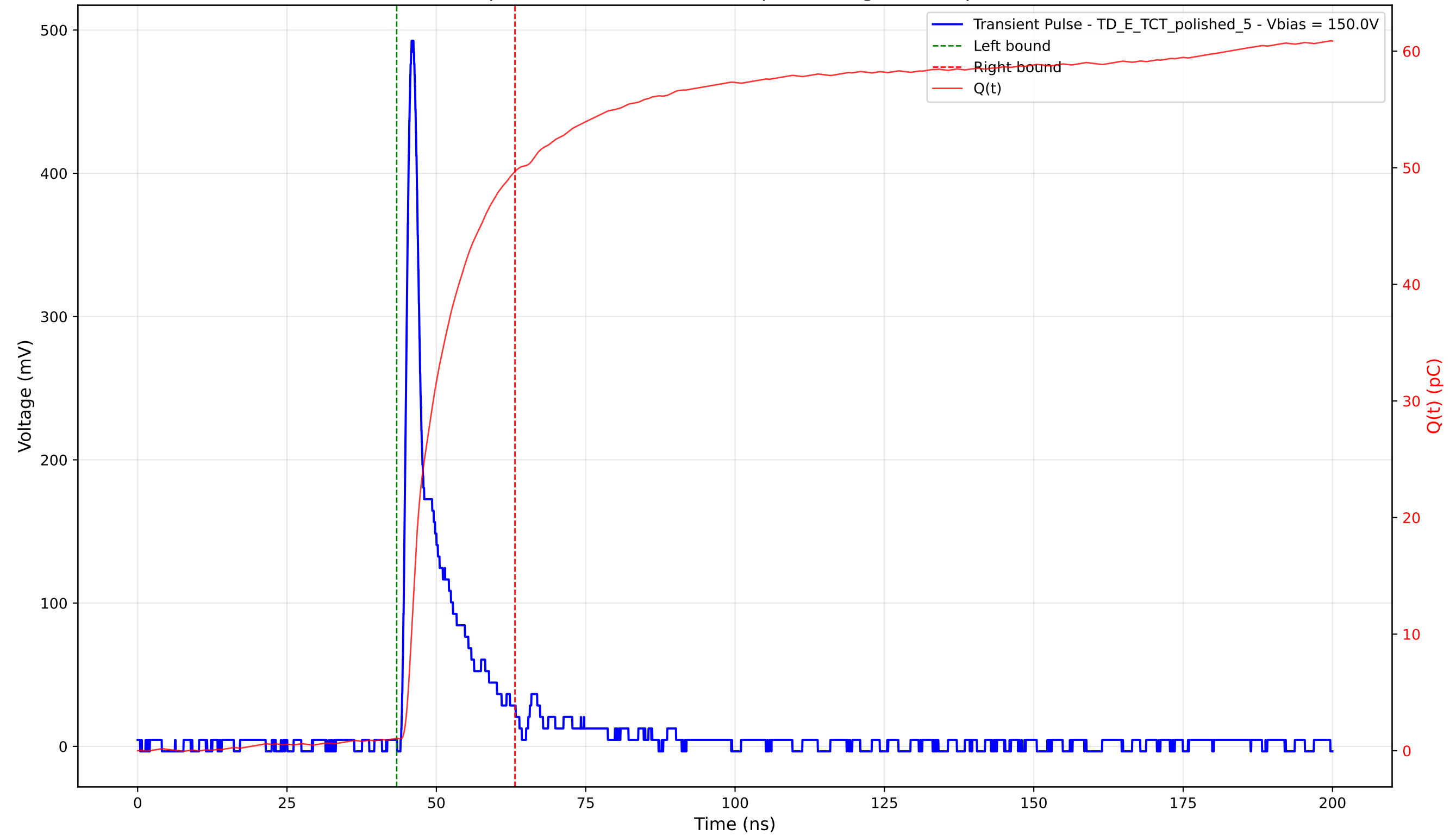
Transient Pulse - Sample: 4003 - Position: 200.0 \mu\text{m} - Charge: 48.63 pC - Rise Time: 1.17 ns
