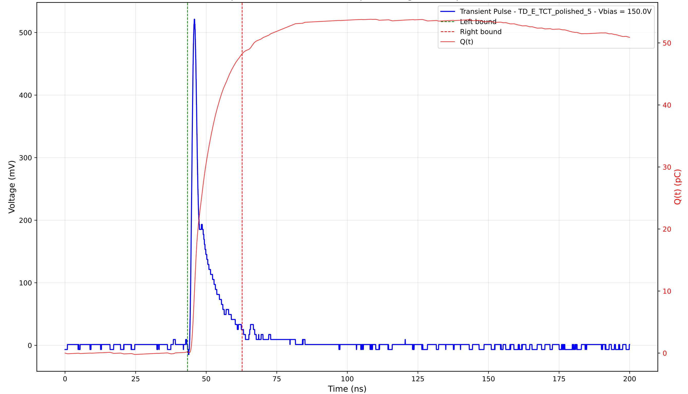
Transient Pulse - Sample: 4003 - Position: 180.0 \mu\text{m} - Charge: 48.06 pC - Rise Time: 1.10 ns
