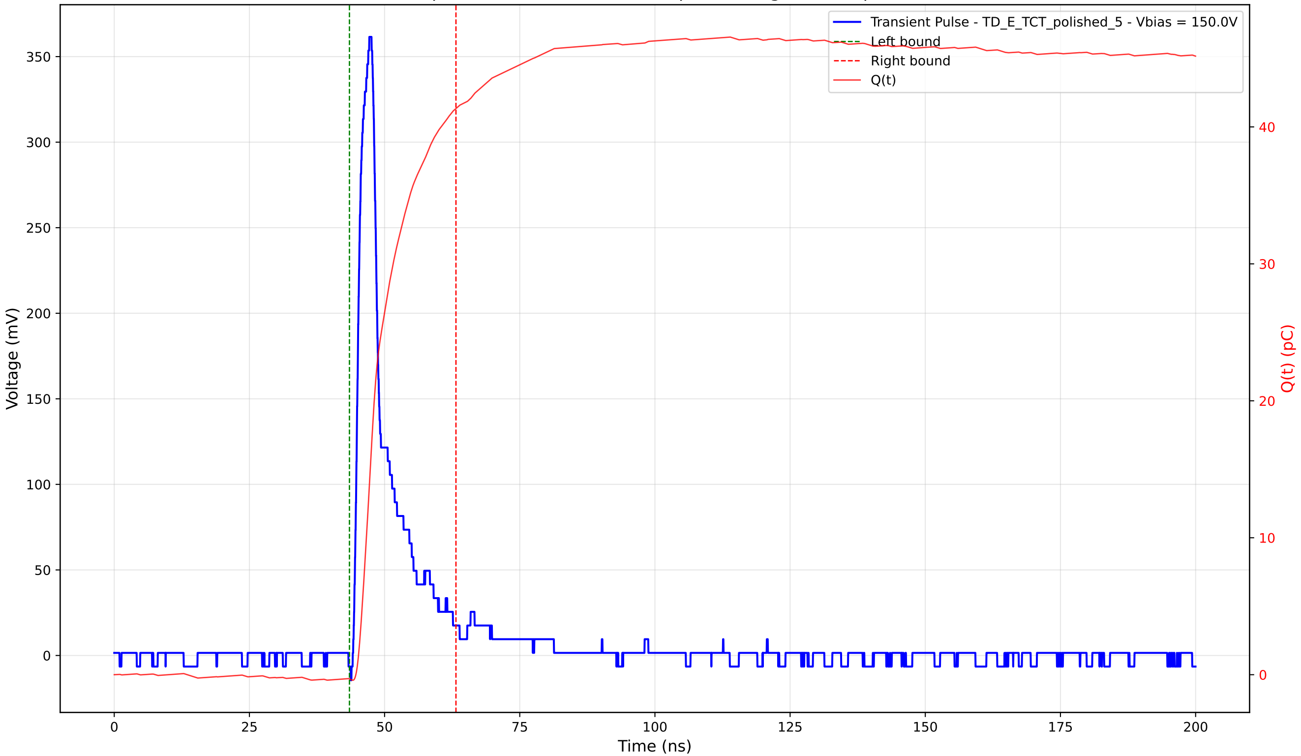
Transient Pulse - Sample: 4003 - Position: 255.0 \mu\text{m} - Charge: 41.65 pC - Rise Time: 1.91 ns
