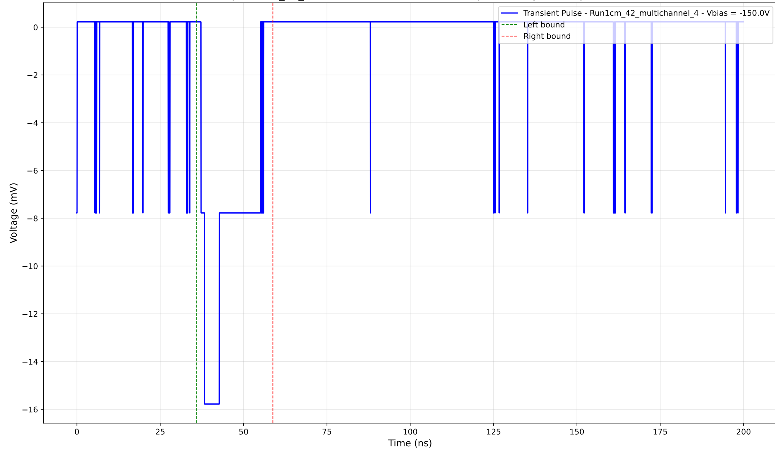
Transient Pulse - Sample: 1cm_42_multichannel - Position: 4140.0 \mu\text{m} - Charge: 3.51 pC - Rise Time: 1.08 ns
