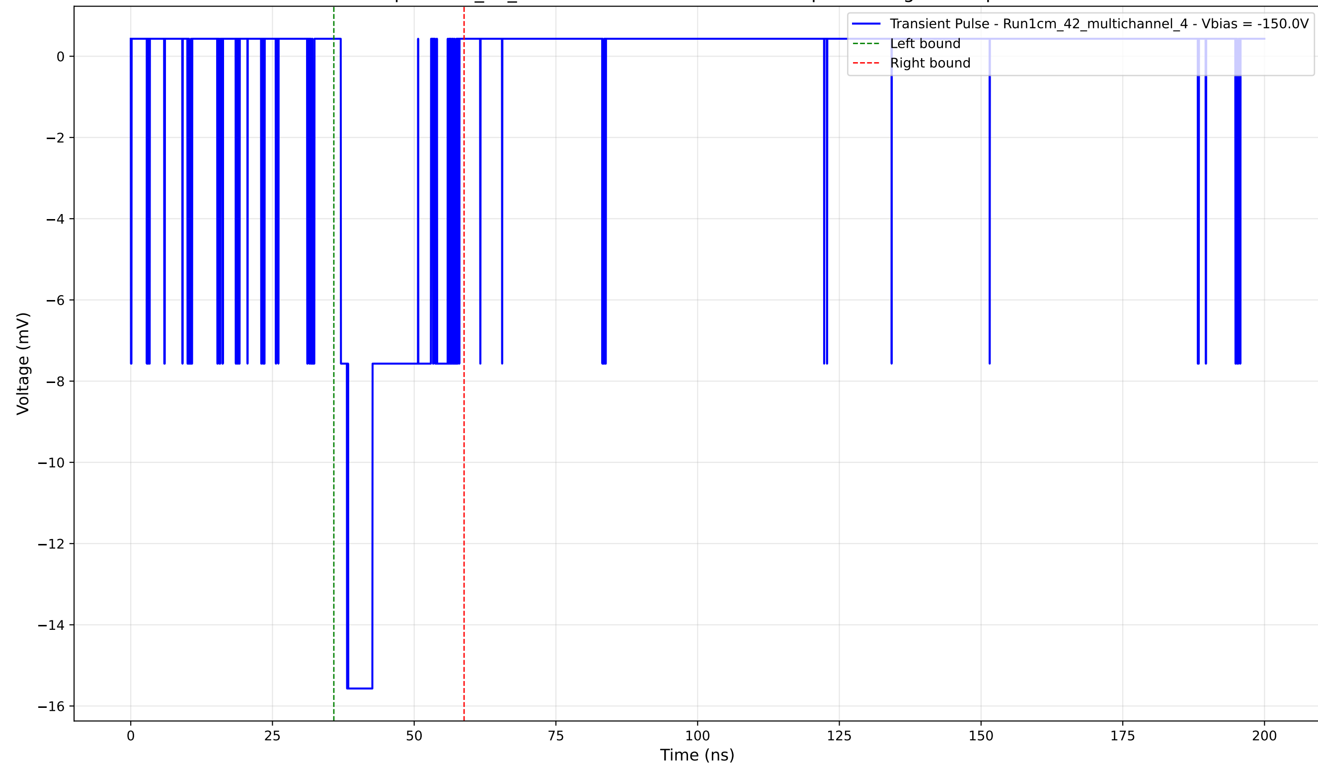
Transient Pulse - Sample: 1cm_42_multichannel - Position: 4265.0 \mu\text{m} - Charge: 3.61 pC - Rise Time: 1.10 ns
