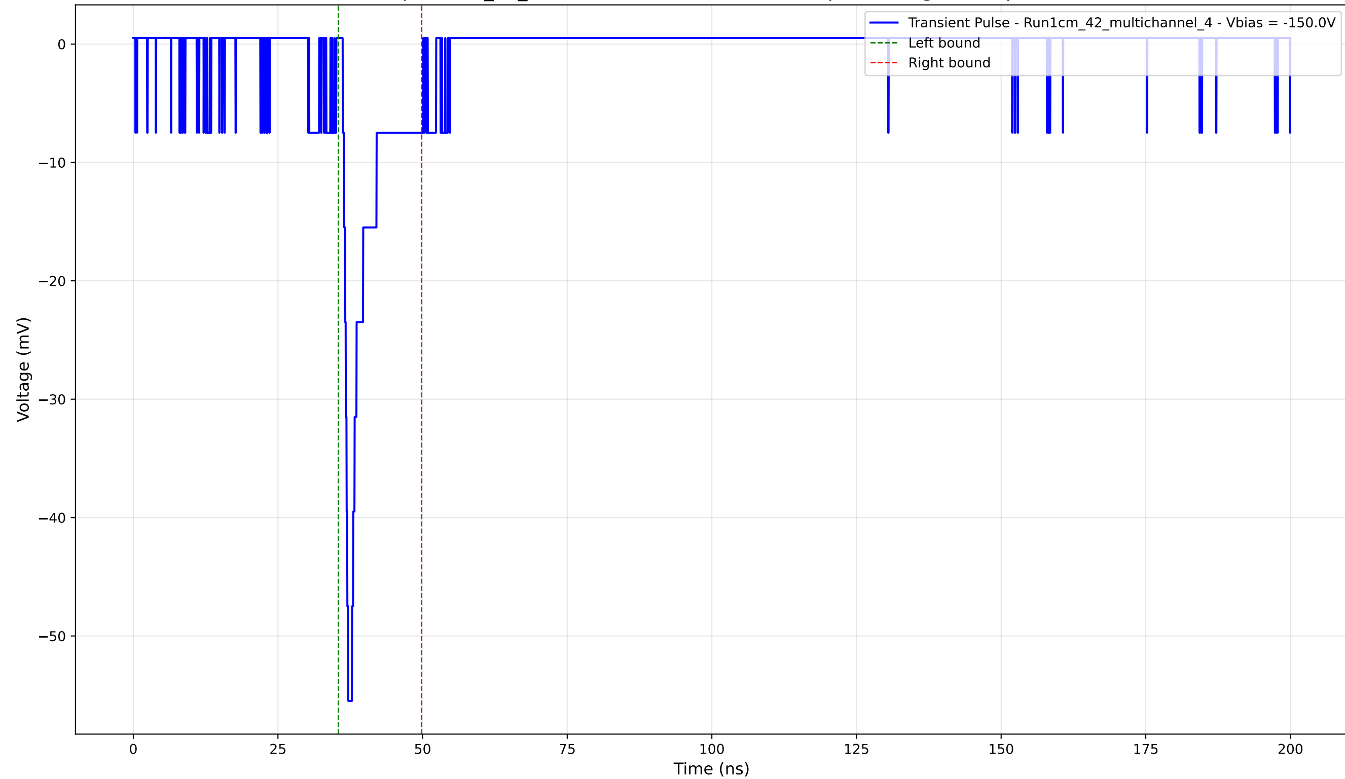
Transient Pulse - Sample: 1cm_42_multichannel - Position: 2055.0 \mu\text{m} - Charge: 4.21 pC - Rise Time: 0.95 ns
