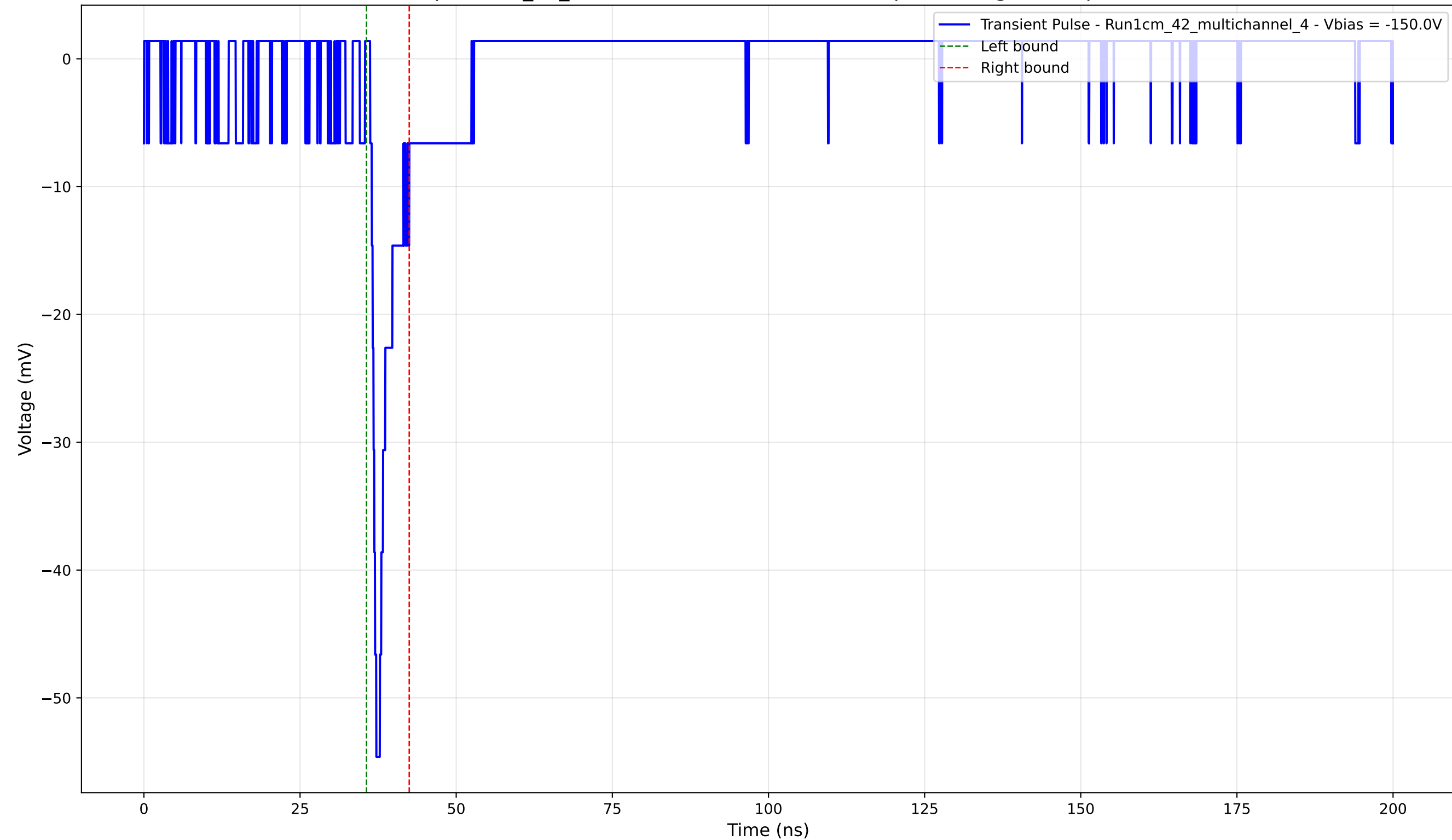
Transient Pulse - Sample: 1cm_42_multichannel - Position: 2740.0 \mu\text{m} - Charge: 3.00 pC - Rise Time: 0.98 ns
