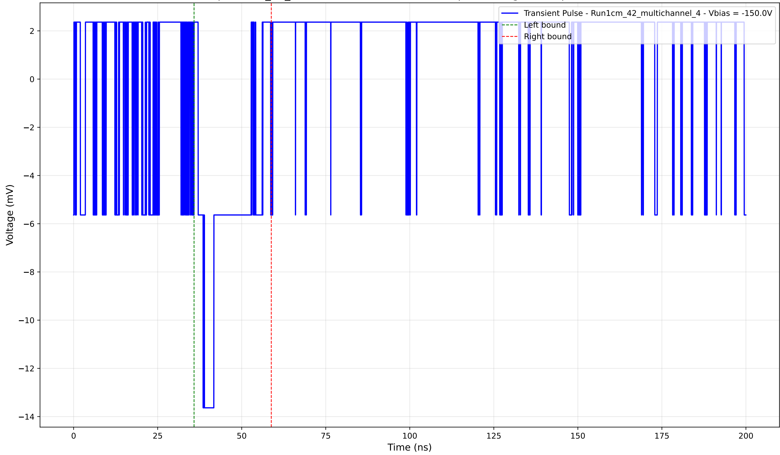
Transient Pulse - Sample: 1cm_42_multichannel - Position: 195.0 \mu\text{m} - Charge: 2.36 pC - Rise Time: 0.00 ns (N/A)
