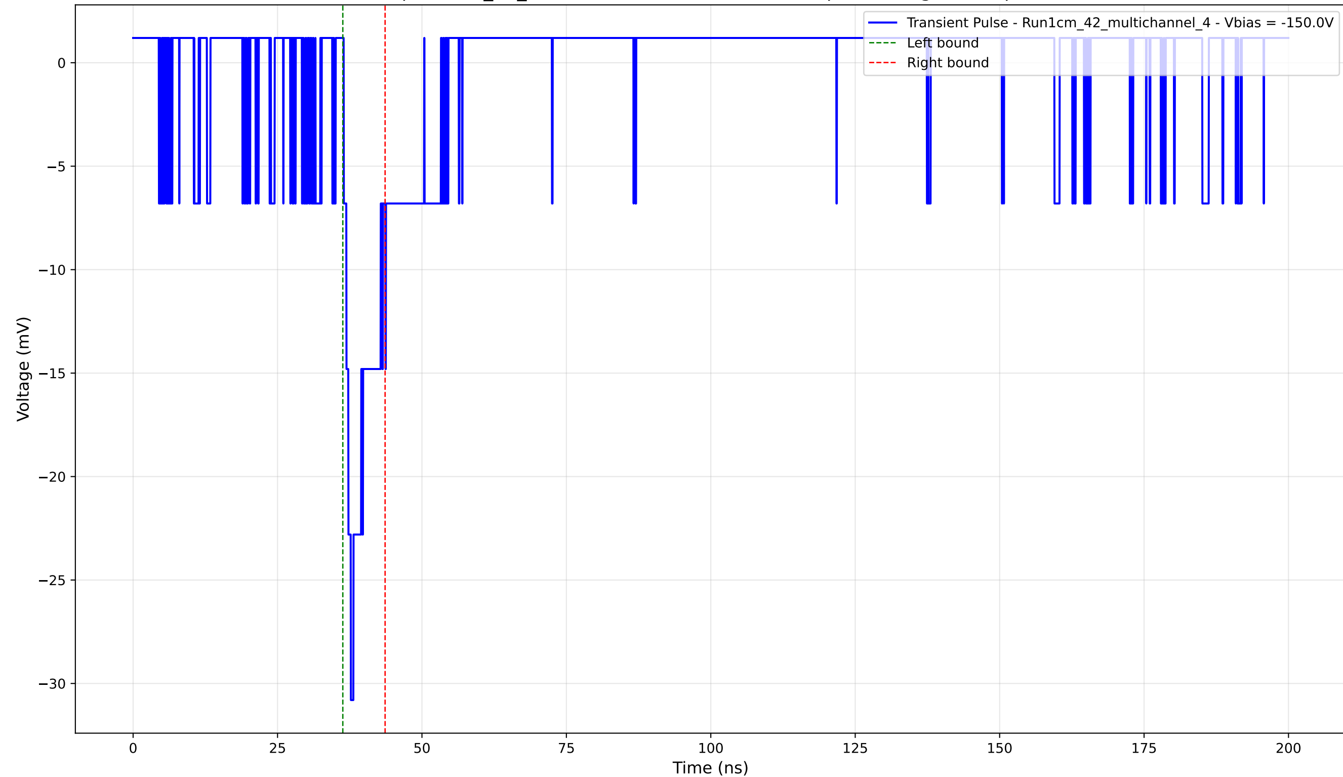
Transient Pulse - Sample: 1cm_42_multichannel - Position: 3265.0 \mu\text{m} - Charge: 2.39 pC - Rise Time: 1.23 ns
