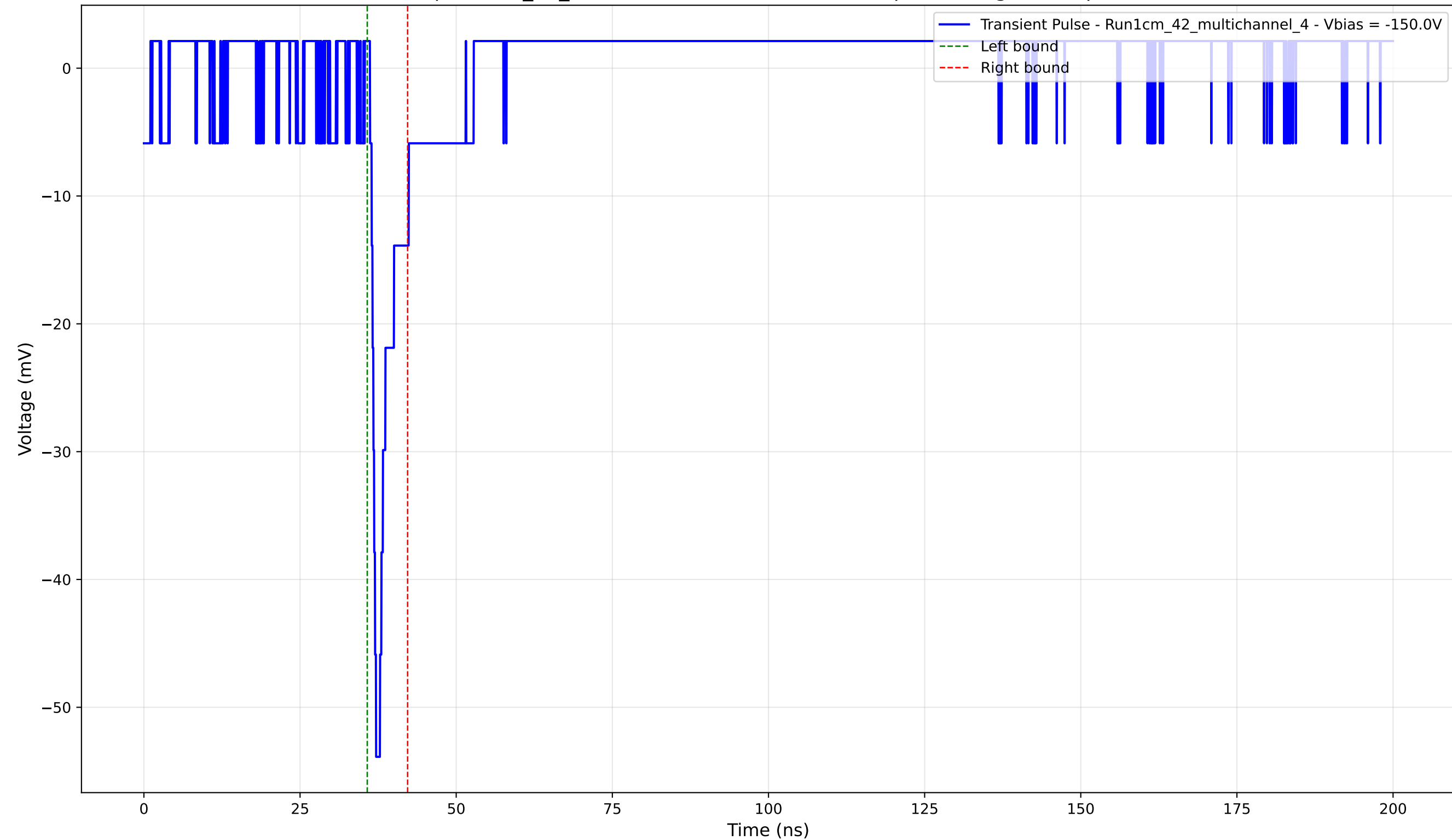
Transient Pulse - Sample: 1cm_42_multichannel - Position: 2030.0 \mu\text{m} - Charge: 2.96 pC - Rise Time: 0.96 ns
