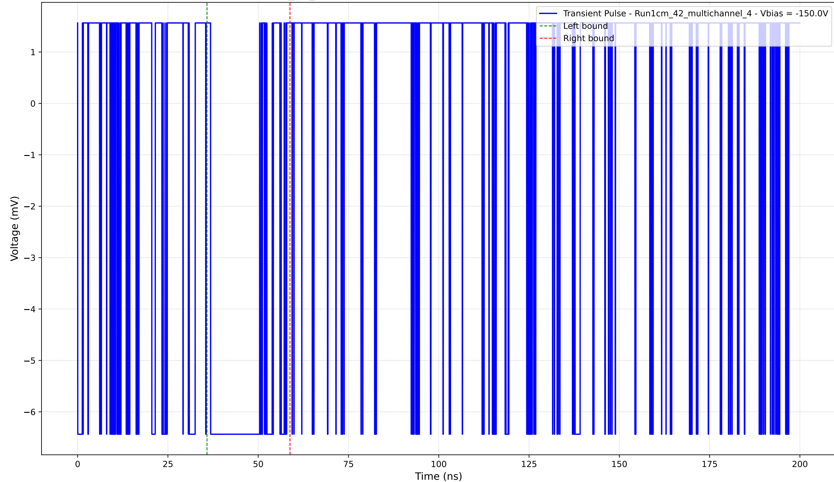
Transient Pulse - Sample: 1cm_42_multichannel - Position: 90.0 \mu\text{m} - Charge: 2.14 pC - Rise Time: 0.00 ns (N/A)
