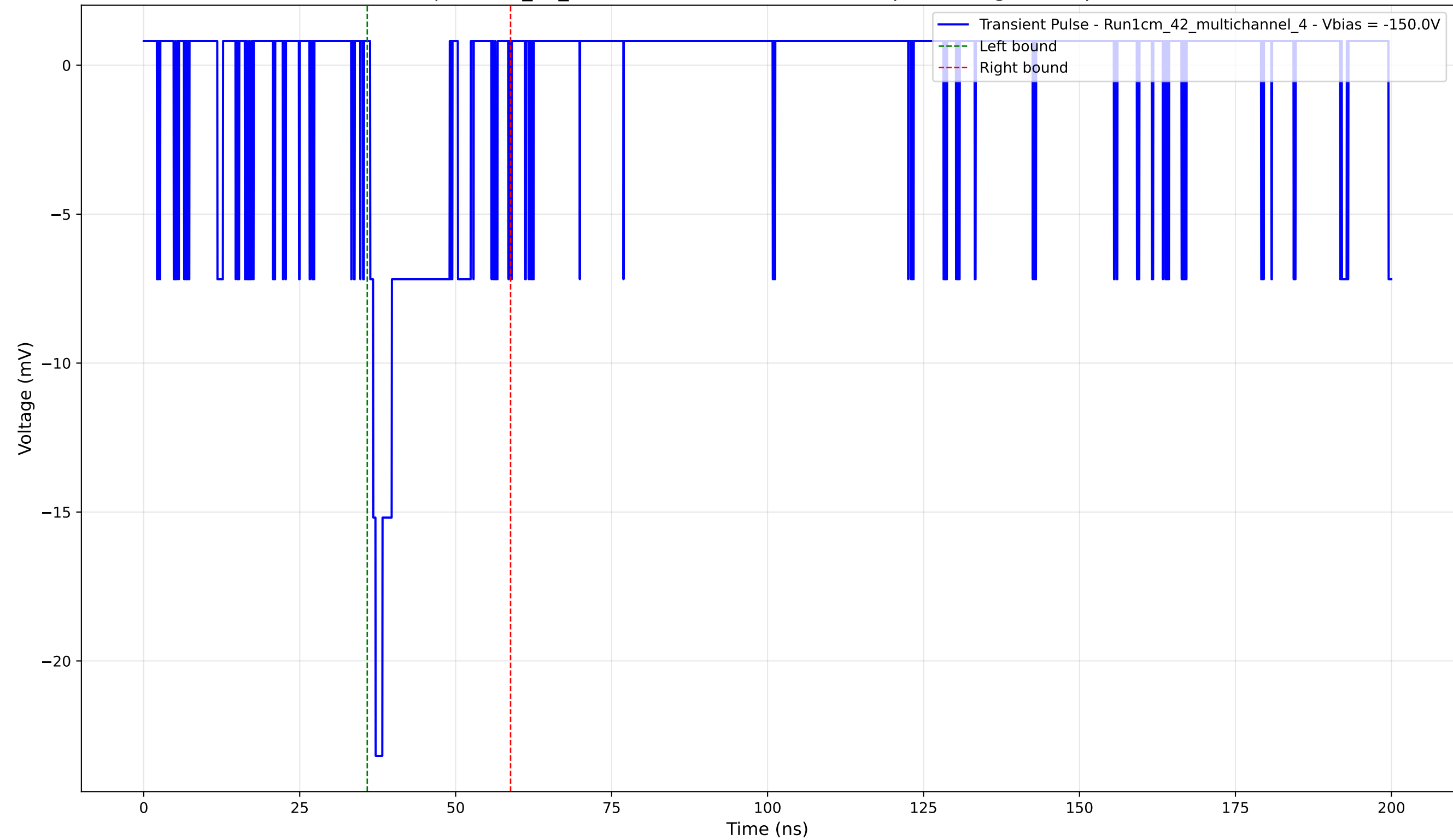
Transient Pulse - Sample: 1cm_42_multichannel - Position: 1830.0 \mu\text{m} - Charge: 2.78 pC - Rise Time: 0.88 ns
