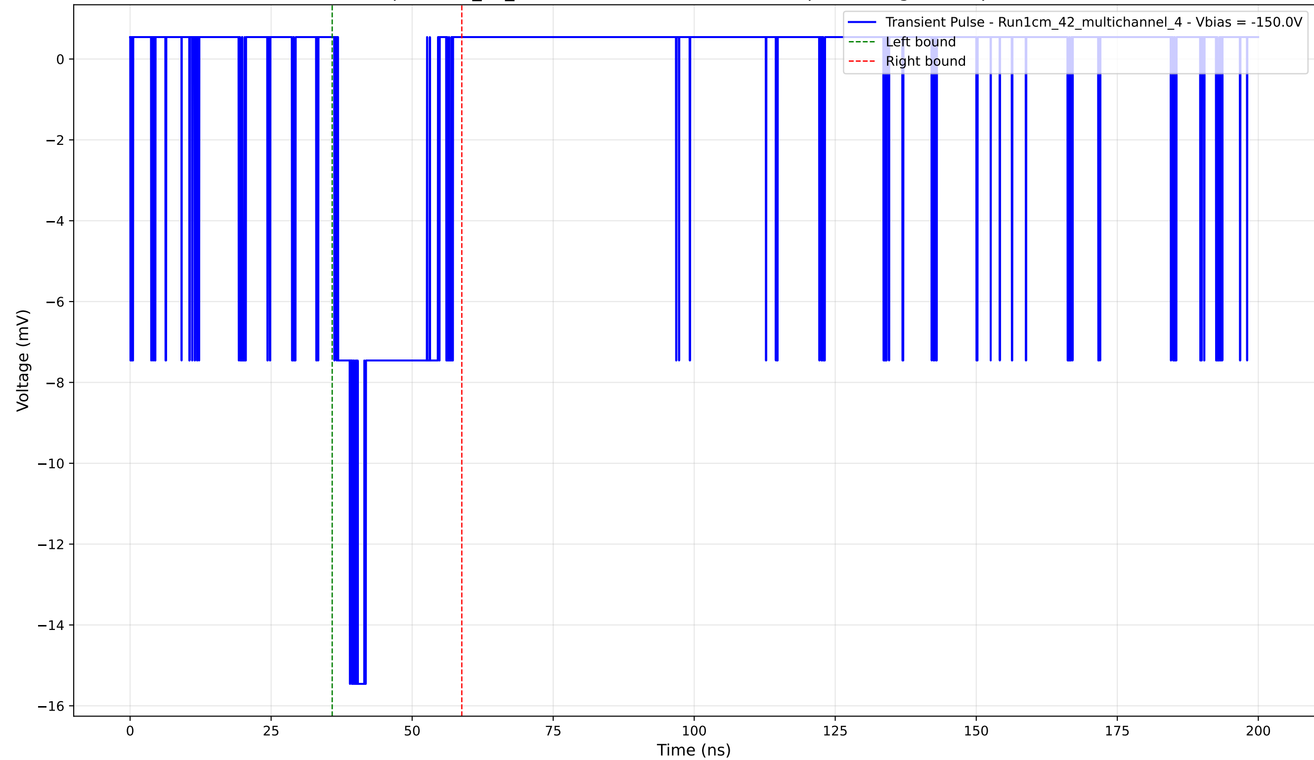
Transient Pulse - Sample: 1cm_42_multichannel - Position: 4465.0 \mu\text{m} - Charge: 3.10 pC - Rise Time: 2.08 ns
