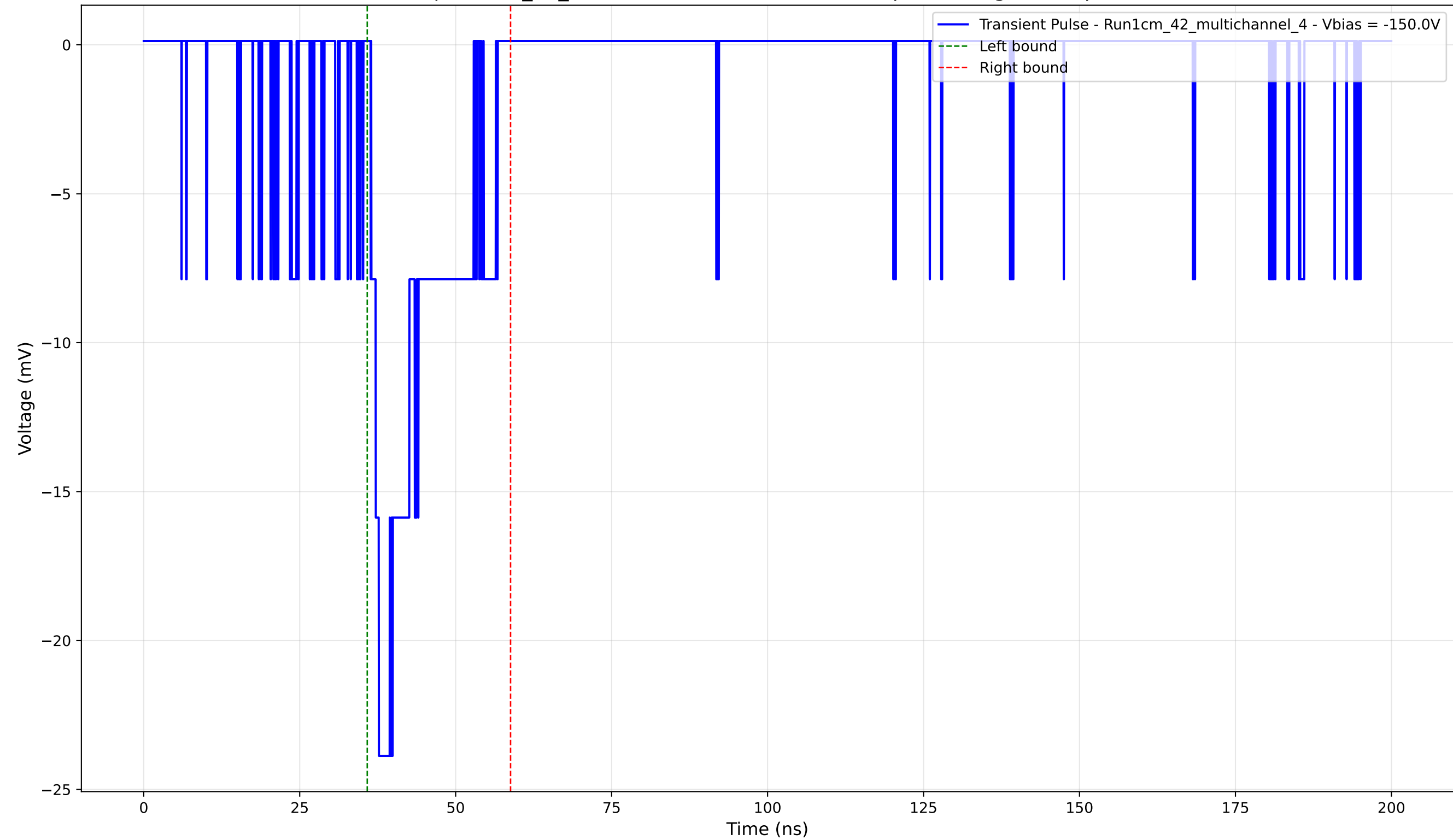
Transient Pulse - Sample: 1cm_42_multichannel - Position: 3490.0 \mu\text{m} - Charge: 4.25 pC - Rise Time: 1.21 ns
