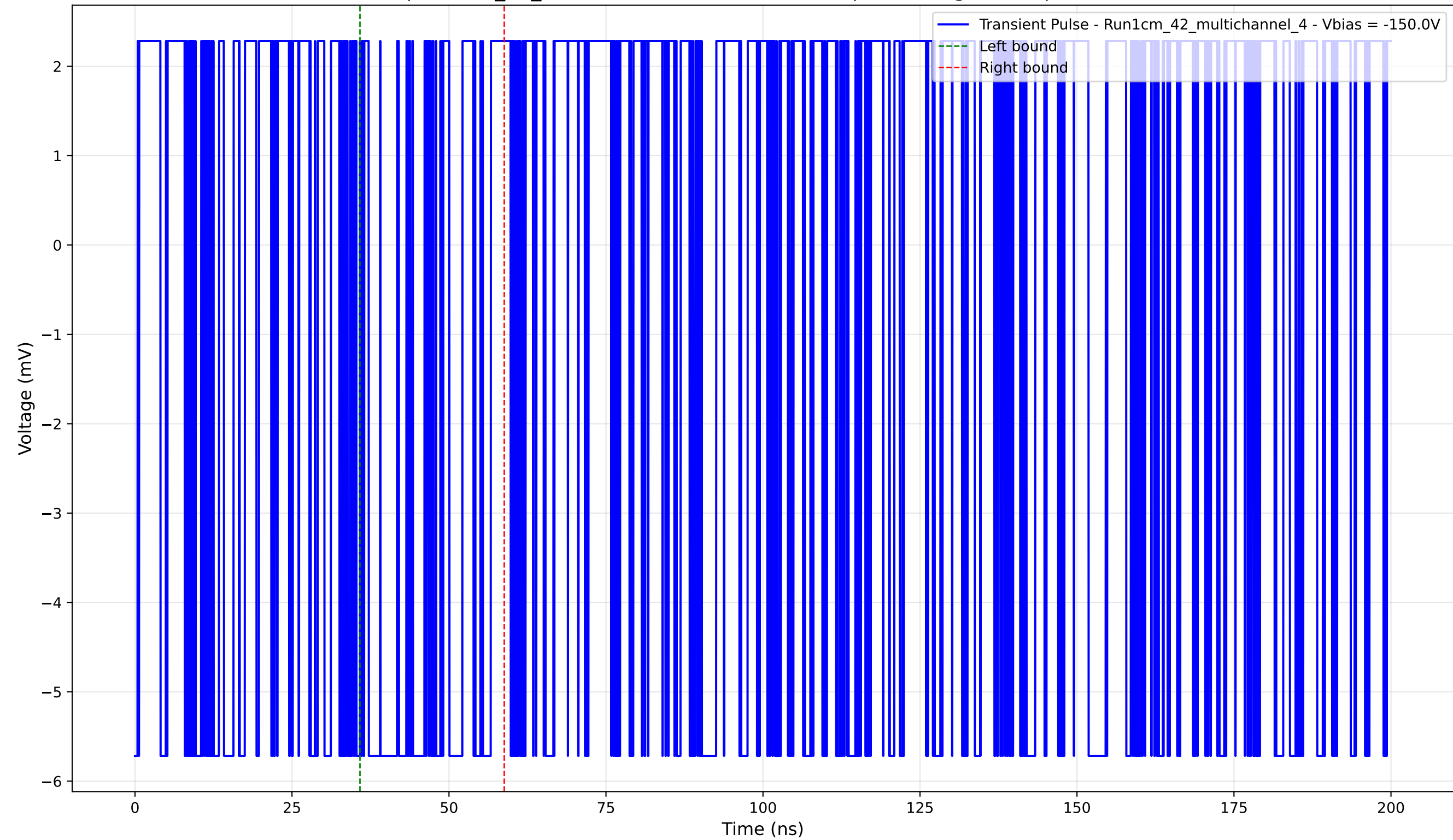
Transient Pulse - Sample: 1cm_42_multichannel - Position: 840.0 \mu\text{m} - Charge: 1.34 pC - Rise Time: 0.00 ns (N/A)
