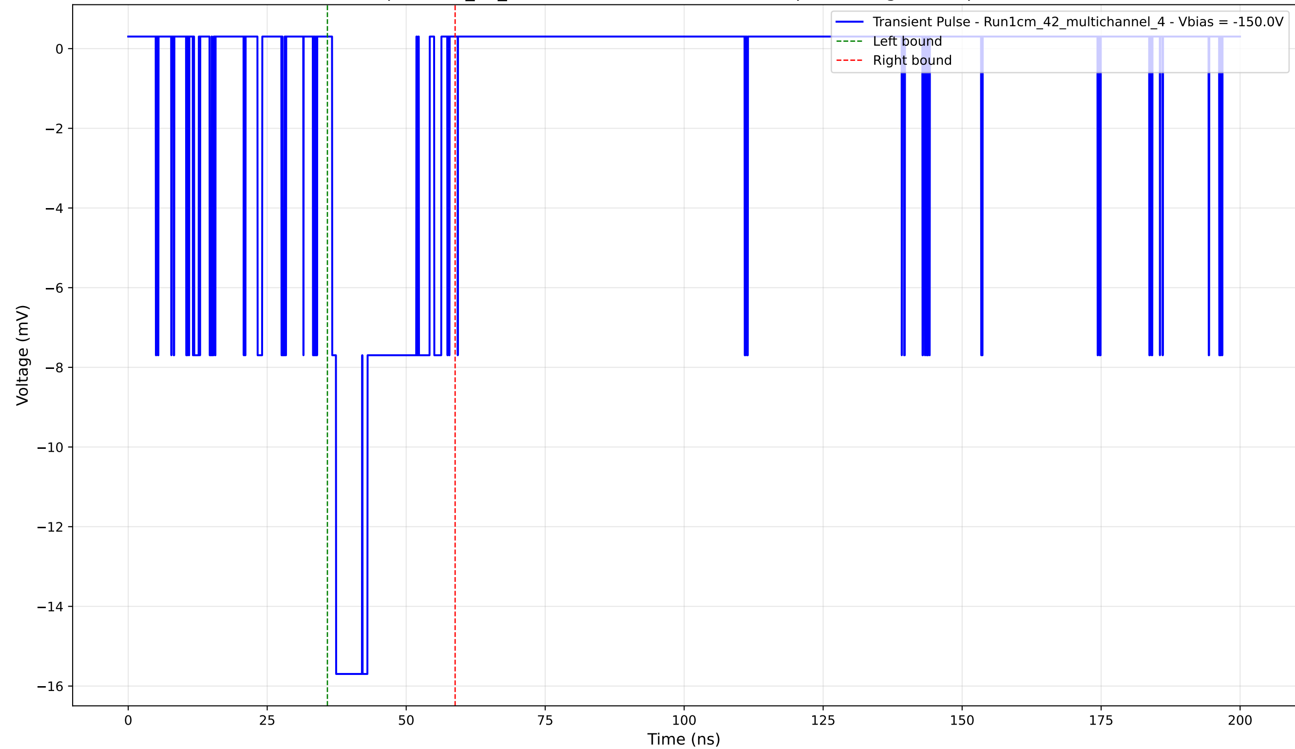
Transient Pulse - Sample: 1cm_42_multichannel - Position: 3600.0 \mu\text{m} - Charge: 3.75 pC - Rise Time: 0.72 ns
