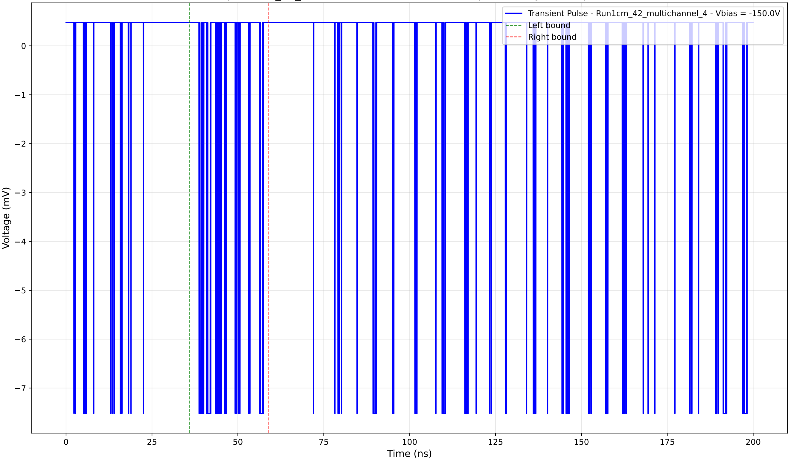
Transient Pulse - Sample: 1cm_42_multichannel - Position: 3880.0 \mu\text{m} - Charge: 0.48 pC - Rise Time: 0.02 ns
