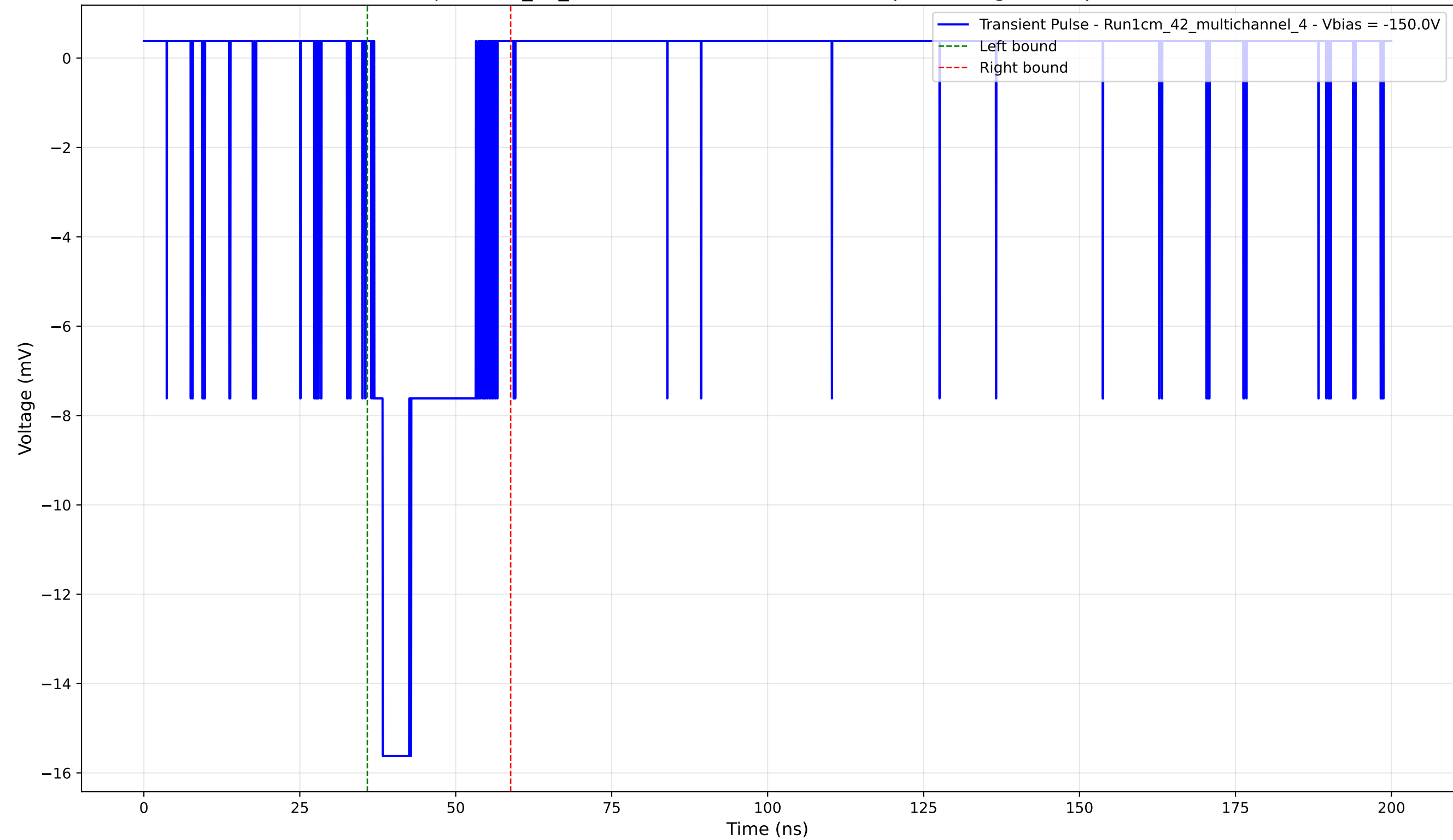
Transient Pulse - Sample: 1cm_42_multichannel - Position: 4275.0 \mu\text{m} - Charge: 3.41 pC - Rise Time: 1.36 ns
