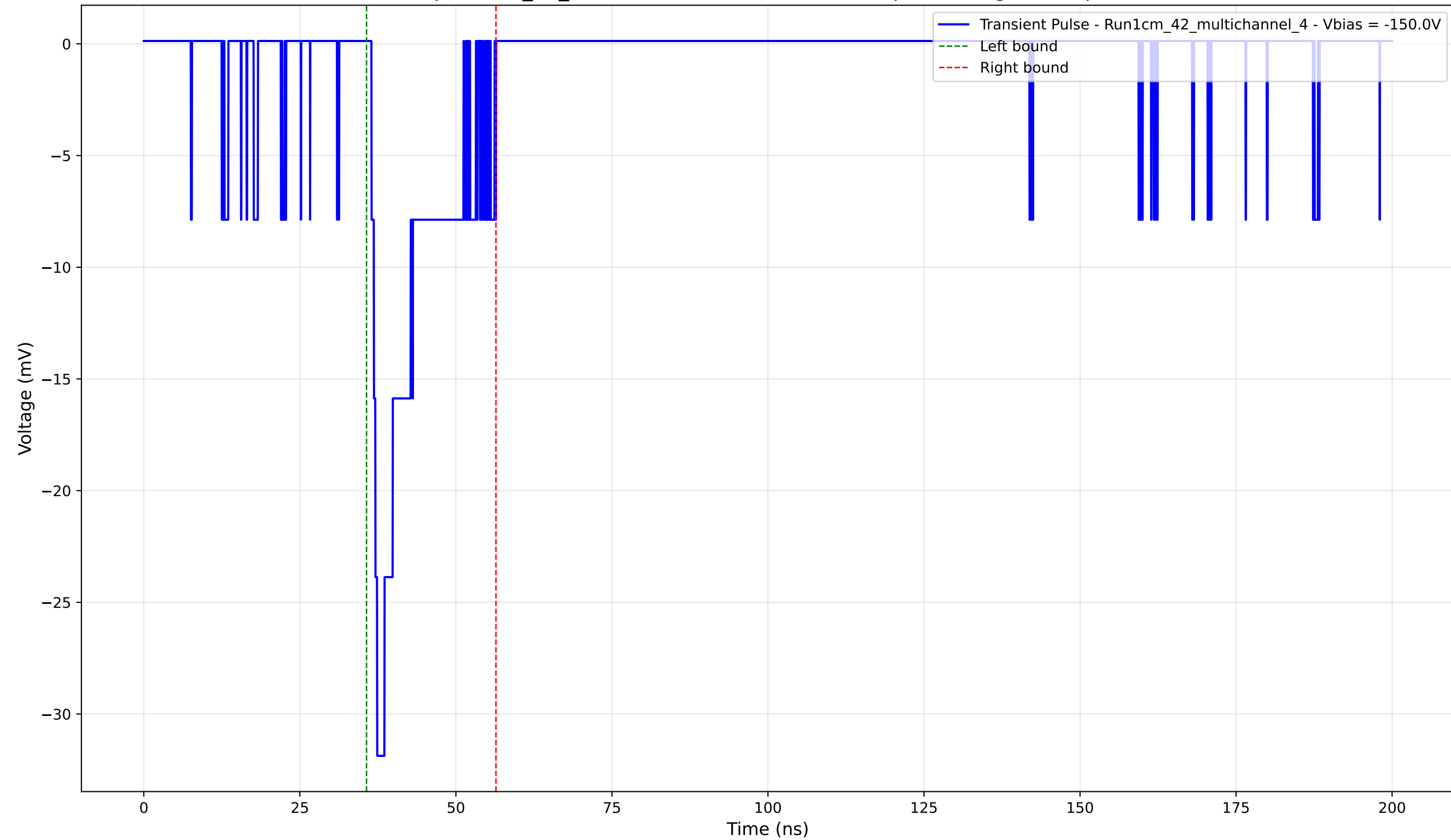
Transient Pulse - Sample: 1cm_42_multichannel - Position: 1610.0 \mu\text{m} - Charge: 4.44 pC - Rise Time: 0.91 ns
