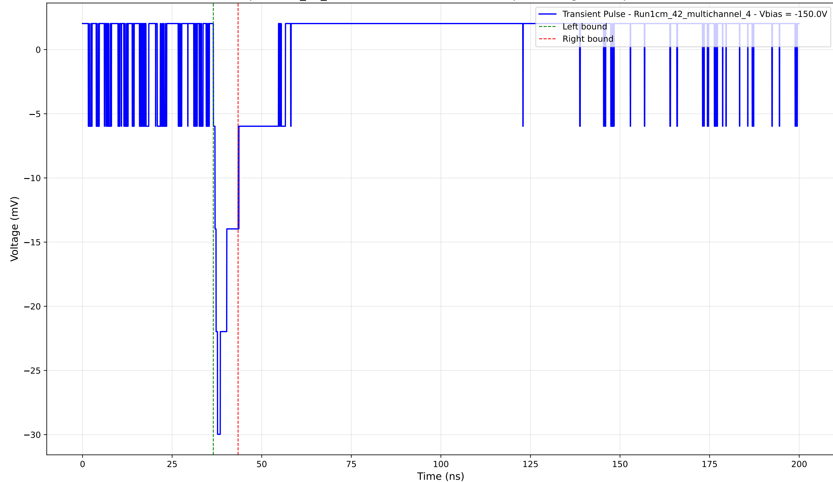
Transient Pulse - Sample: 1cm_42_multichannel - Position: 1475.0 \mu\text{m} - Charge: 2.46 pC - Rise Time: 1.18 ns
