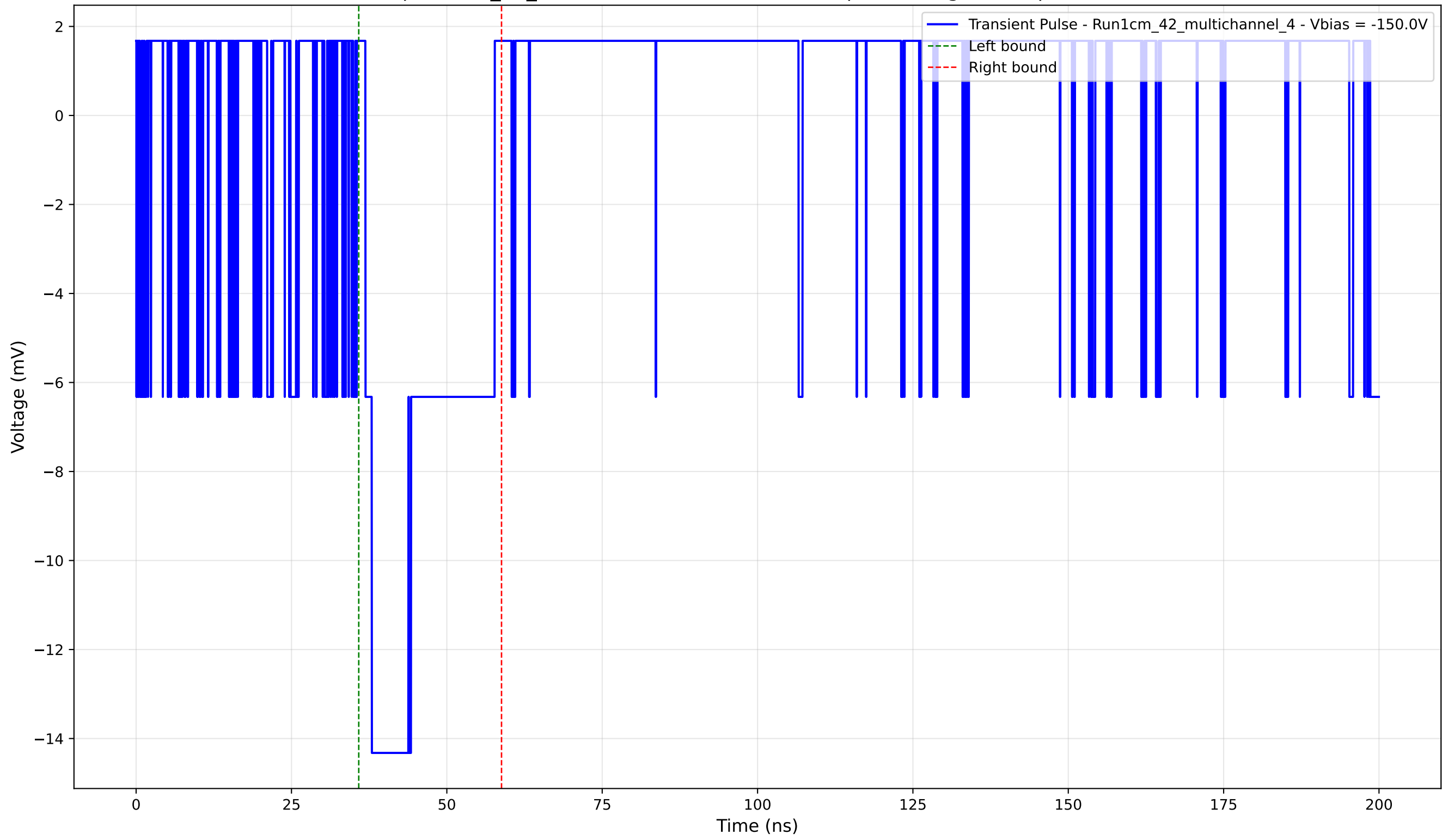
Transient Pulse - Sample: 1cm_42_multichannel - Position: 660.0 \mu\text{m} - Charge: 3.56 pC - Rise Time: 0.00 ns (N/A)
