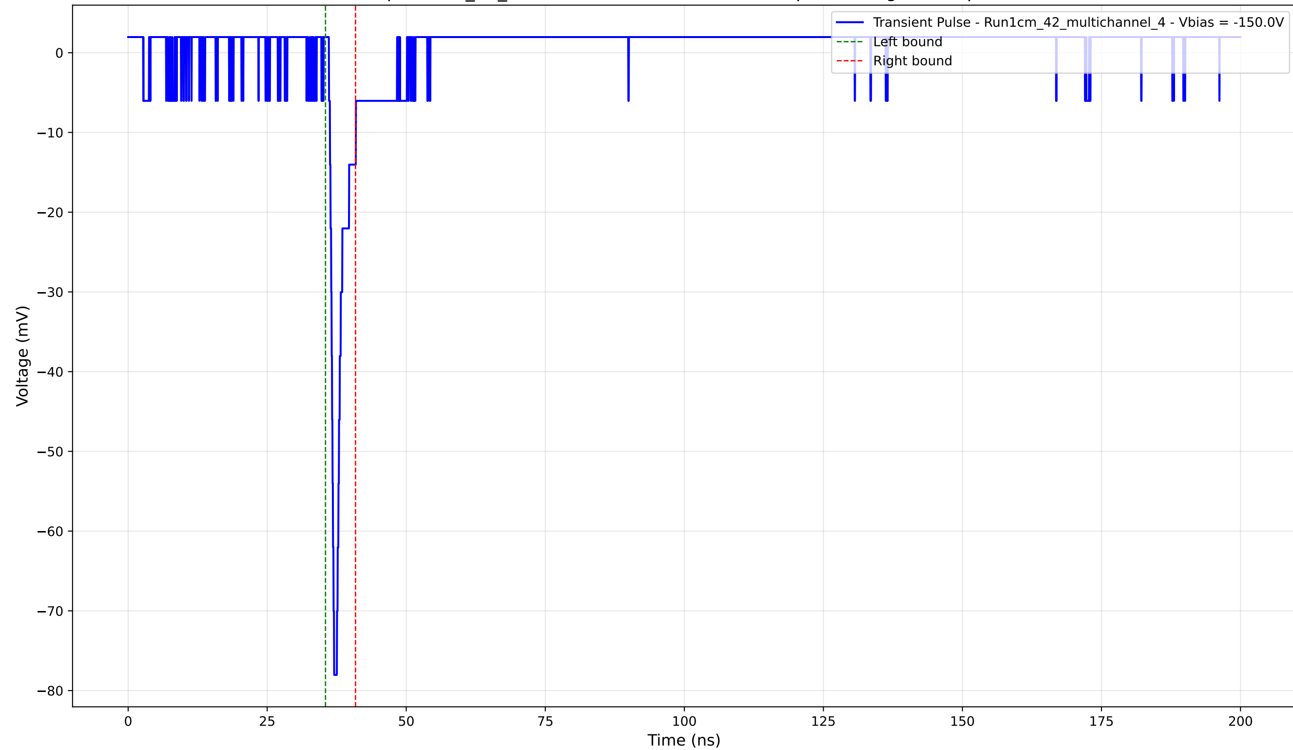
Transient Pulse - Sample: 1cm_42_multichannel - Position: 2265.0 \mu\text{m} - Charge: 3.17 pC - Rise Time: 0.76 ns
