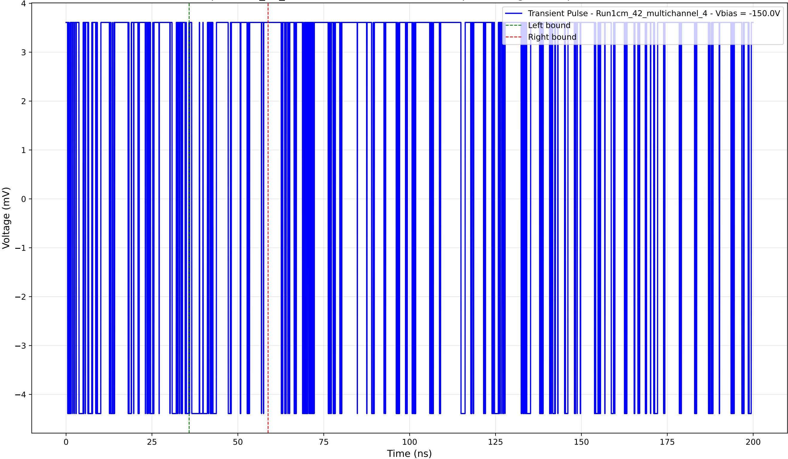
Transient Pulse - Sample: 1cm_42_multichannel - Position: 1900.0 \mu\text{m} - Charge: 0.47 pC - Rise Time: 0.00 ns (N/A)
