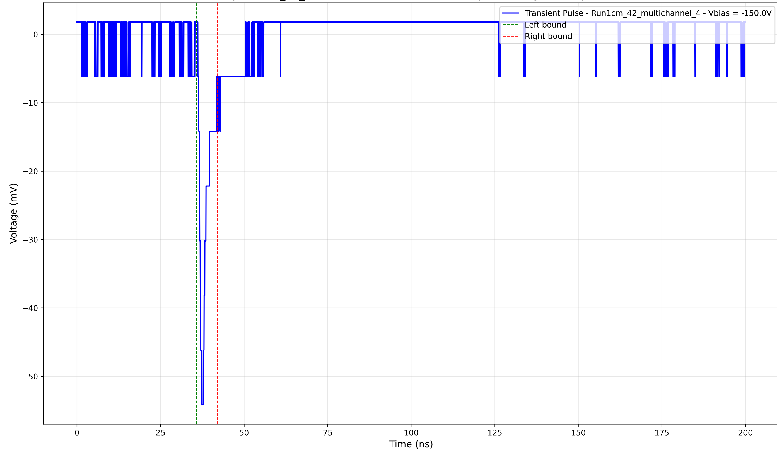
Transient Pulse - Sample: 1cm_42_multichannel - Position: 2750.0 \mu\text{m} - Charge: 2.84 pC - Rise Time: 1.02 ns
