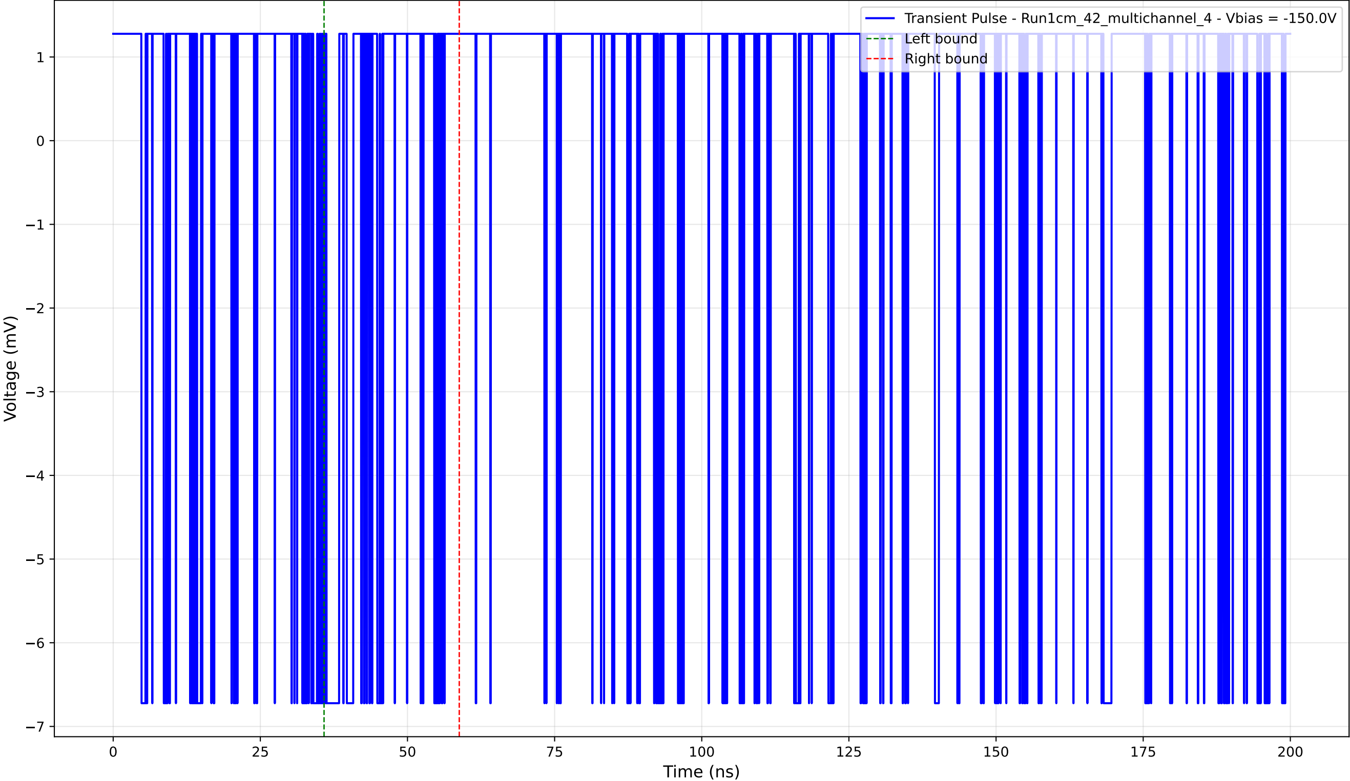
Transient Pulse - Sample: 1cm_42_multichannel - Position: 2400.0 \mu\text{m} - Charge: 0.39 pC - Rise Time: 0.00 ns (N/A)
