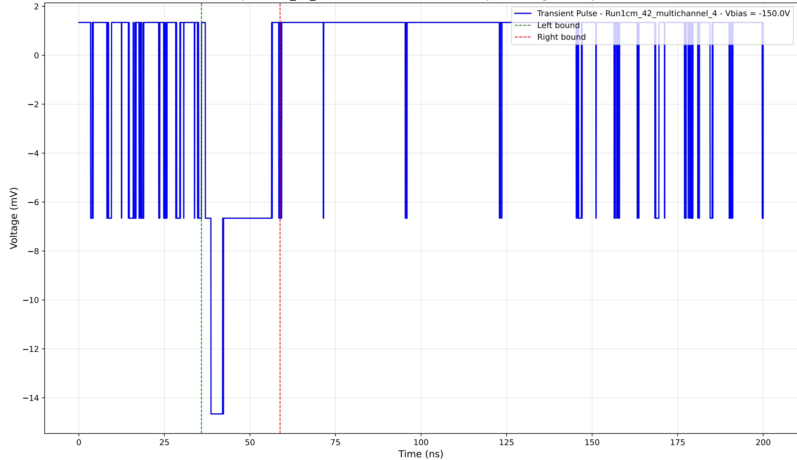
Transient Pulse - Sample: 1cm_42_multichannel - Position: 165.0 \mu\text{m} - Charge: 3.11 pC - Rise Time: 1.66 ns
