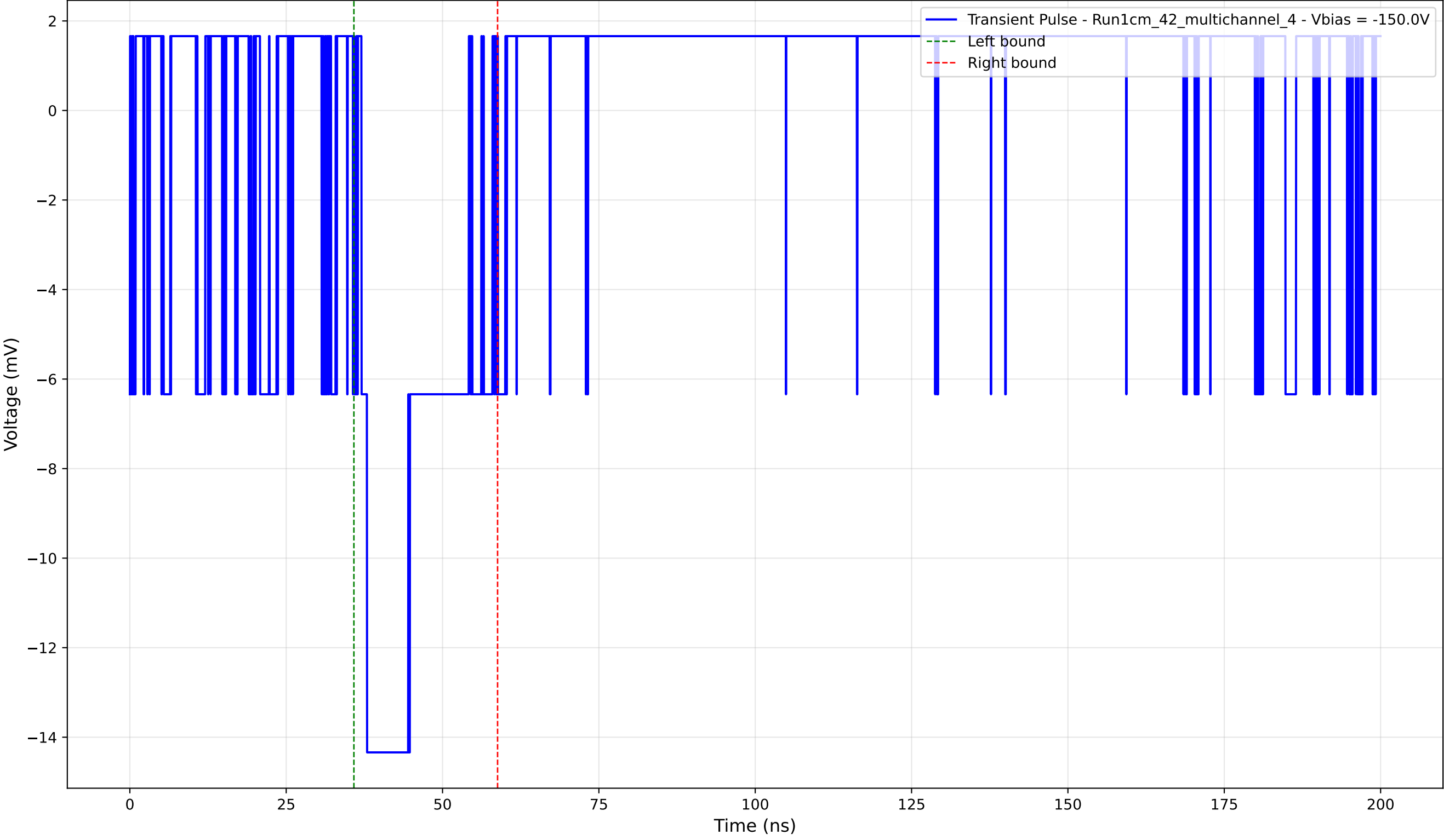
Transient Pulse - Sample: 1cm_42_multichannel - Position: 625.0 \mu\text{m} - Charge: 3.70 pC - Rise Time: 0.00 ns (N/A)
