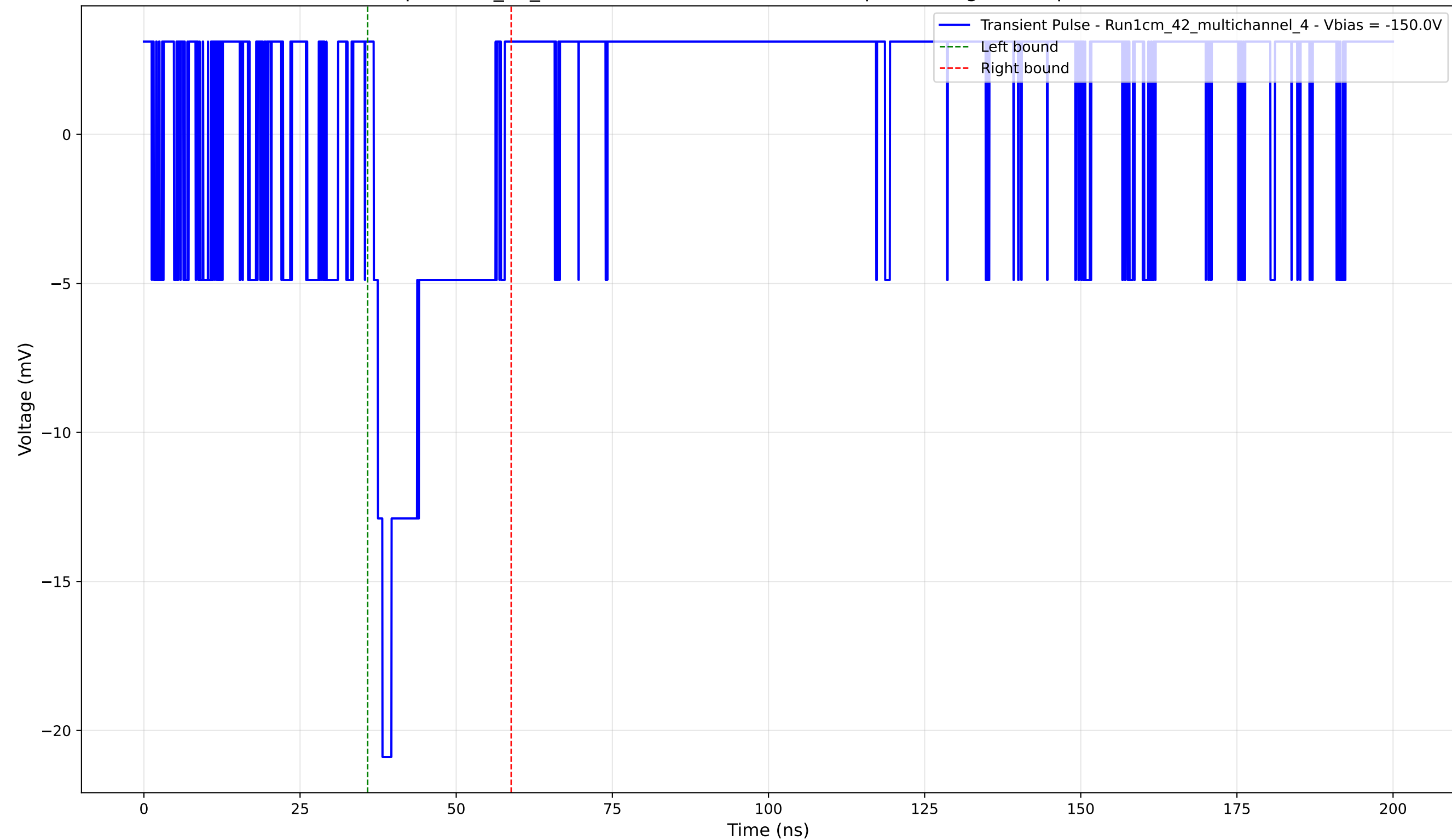
Transient Pulse - Sample: 1cm_42_multichannel - Position: 1050.0 \mu\text{m} - Charge: 3.09 pC - Rise Time: 0.00 ns (N/A)
