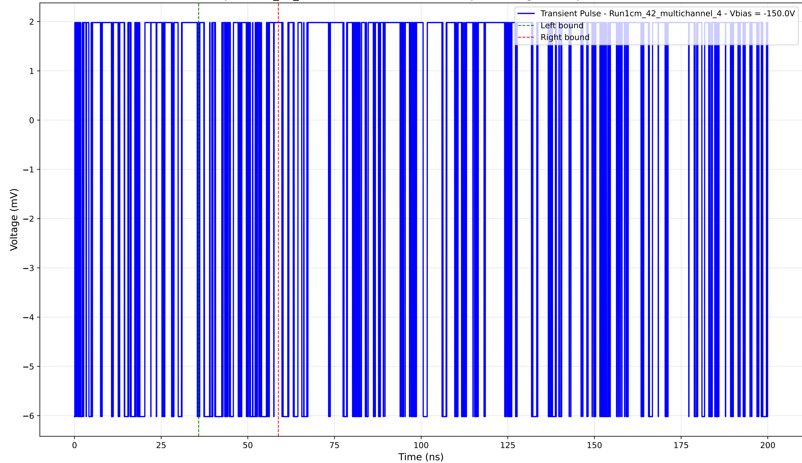
Transient Pulse - Sample: 1cm_42_multichannel - Position: 360.0 \mu\text{m} - Charge: 0.89 pC - Rise Time: 0.00 ns (N/A)
