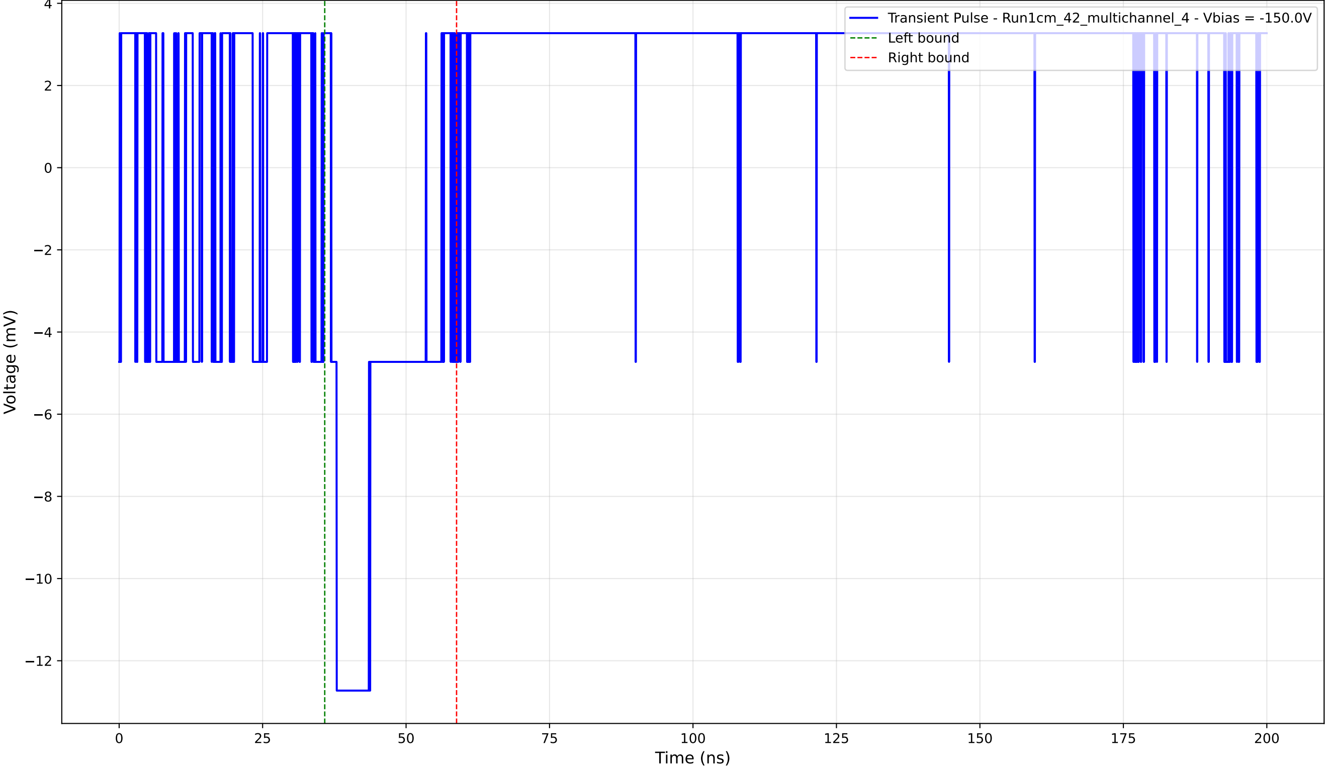
Transient Pulse - Sample: 1cm_42_multichannel - Position: 655.0 \mu\text{m} - Charge: 2.57 pC - Rise Time: 0.00 ns (N/A)
