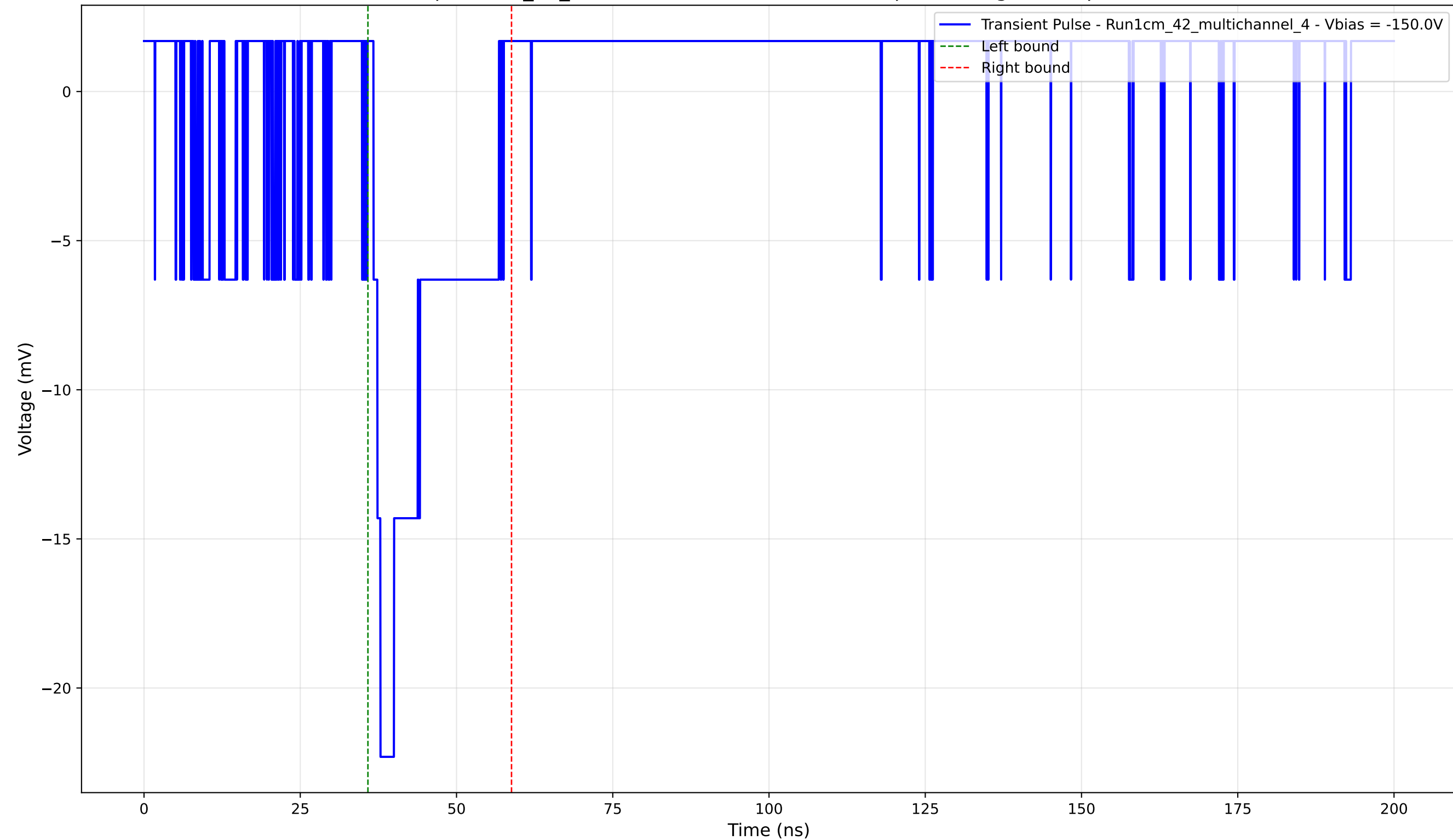
Transient Pulse - Sample: 1cm_42_multichannel - Position: 1155.0 \mu\text{m} - Charge: 3.89 pC - Rise Time: 1.12 ns
