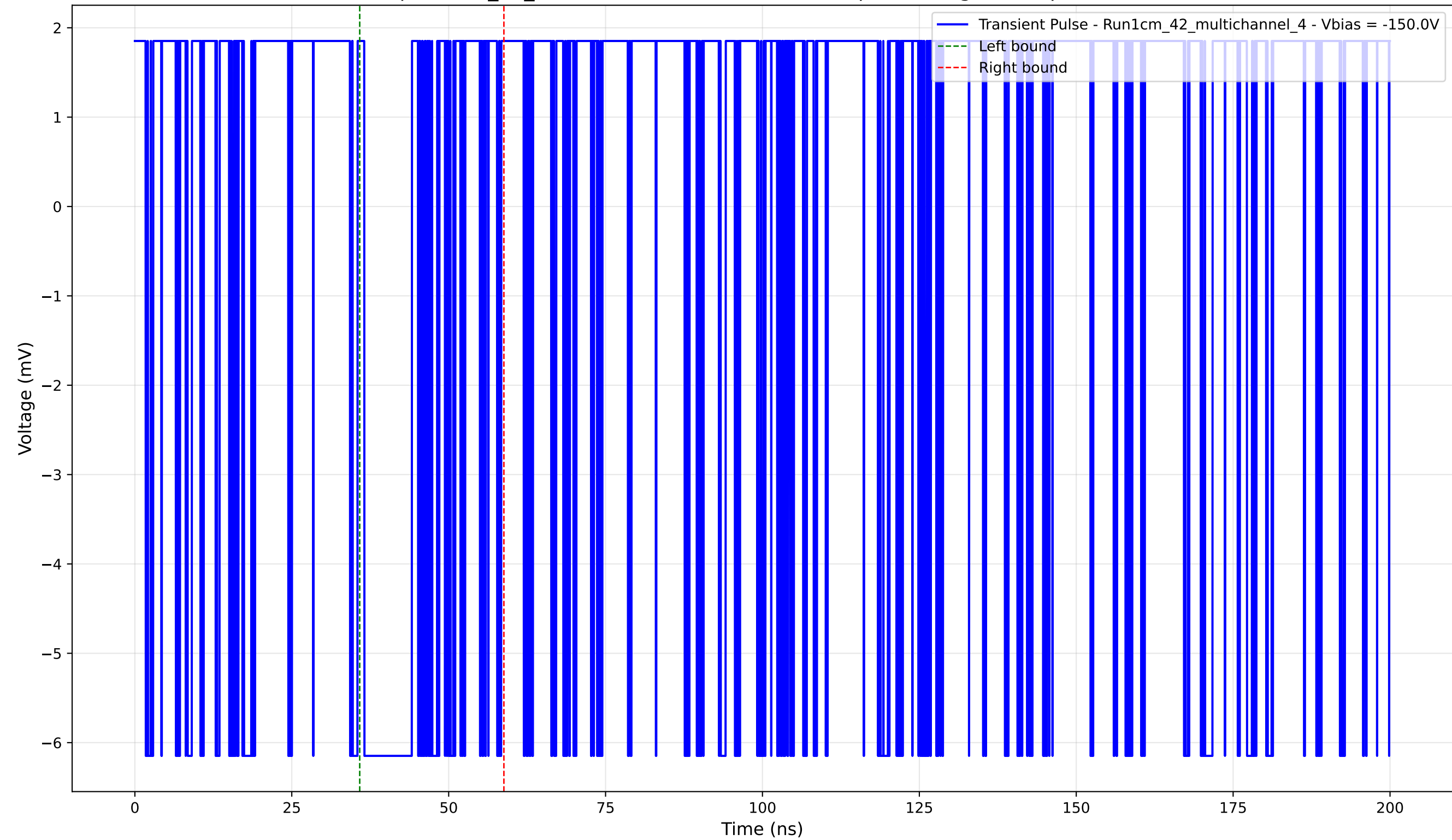
Transient Pulse - Sample: 1cm_42_multichannel - Position: 1850.0 \mu\text{m} - Charge: 1.15 pC - Rise Time: 0.00 ns (N/A)
