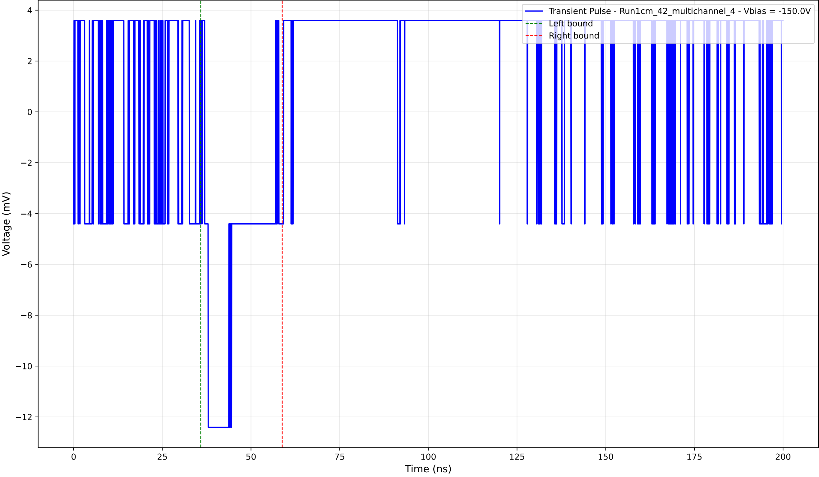
Transient Pulse - Sample: 1cm_42_multichannel - Position: 560.0 \mu\text{m} - Charge: 2.74 pC - Rise Time: 0.00 ns (N/A)
