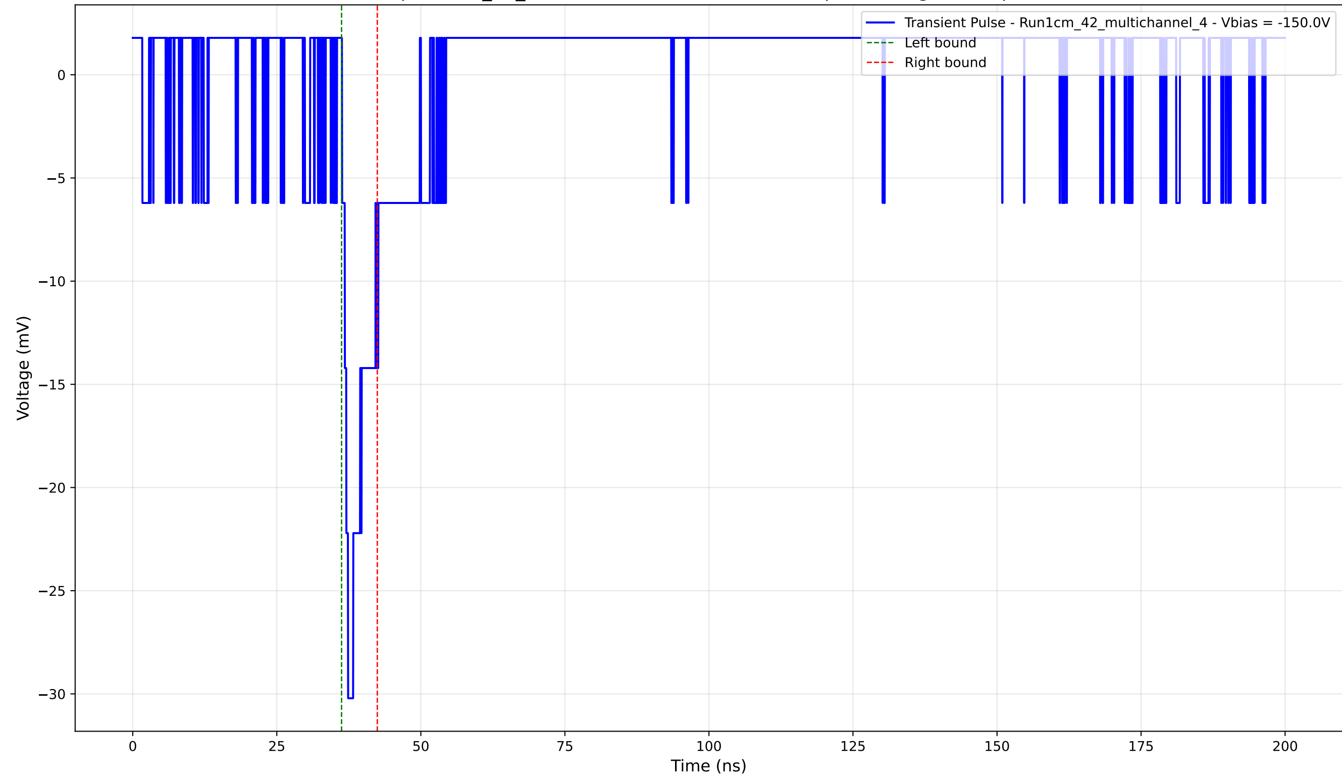
Transient Pulse - Sample: 1cm_42_multichannel - Position: 3090.0 \mu\text{m} - Charge: 2.17 pC - Rise Time: 1.05 ns
