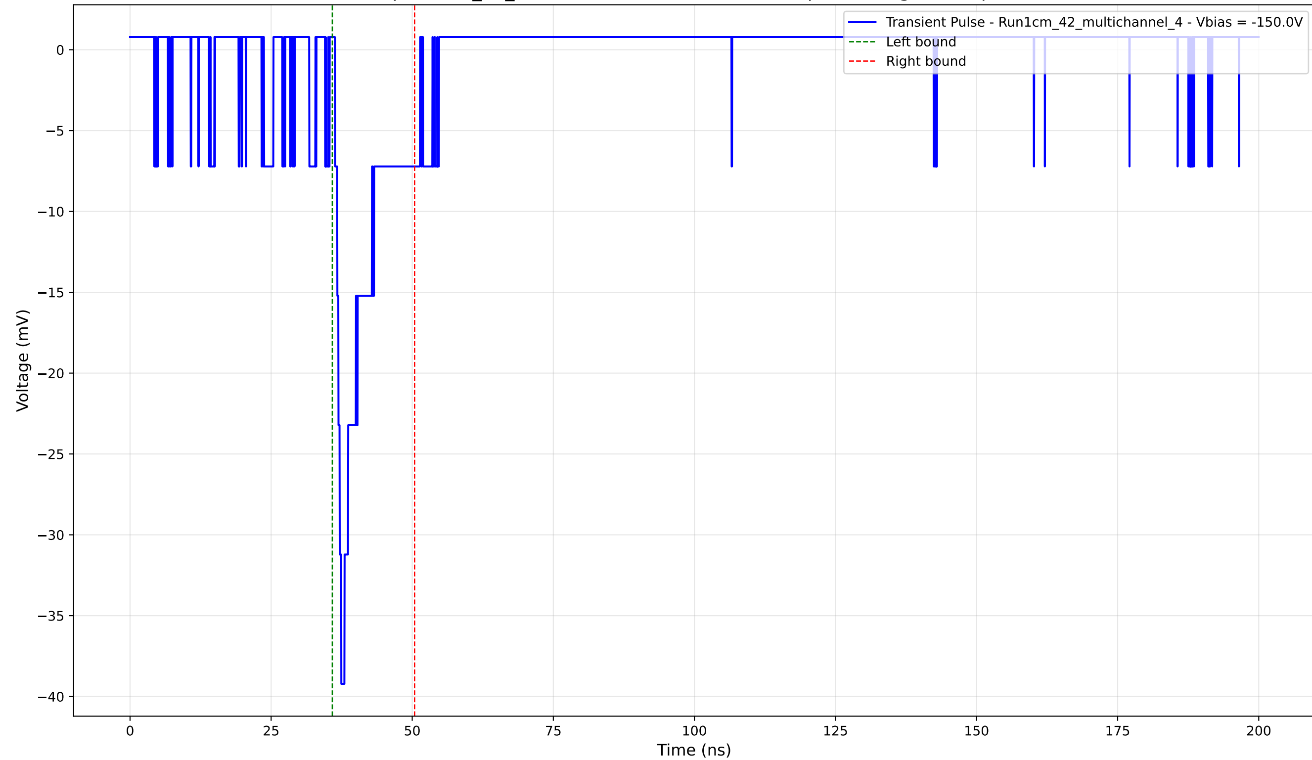
Transient Pulse - Sample: 1cm_42_multichannel - Position: 1700.0 \mu\text{m} - Charge: 3.90 pC - Rise Time: 1.11 ns
