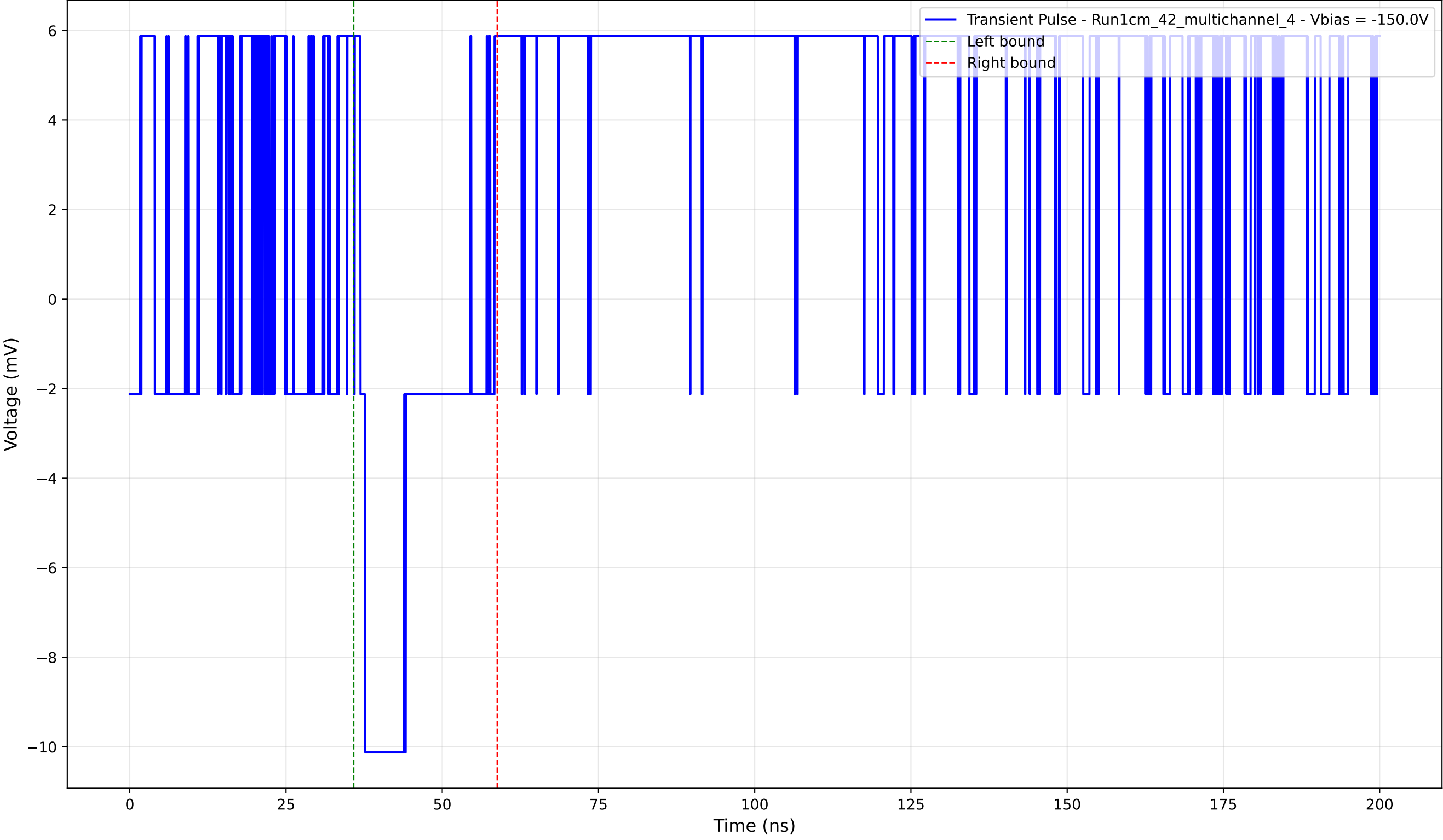
Transient Pulse - Sample: 1cm_42_multichannel - Position: 755.0 \mu\text{m} - Charge: 1.70 pC - Rise Time: 0.00 ns (N/A)
