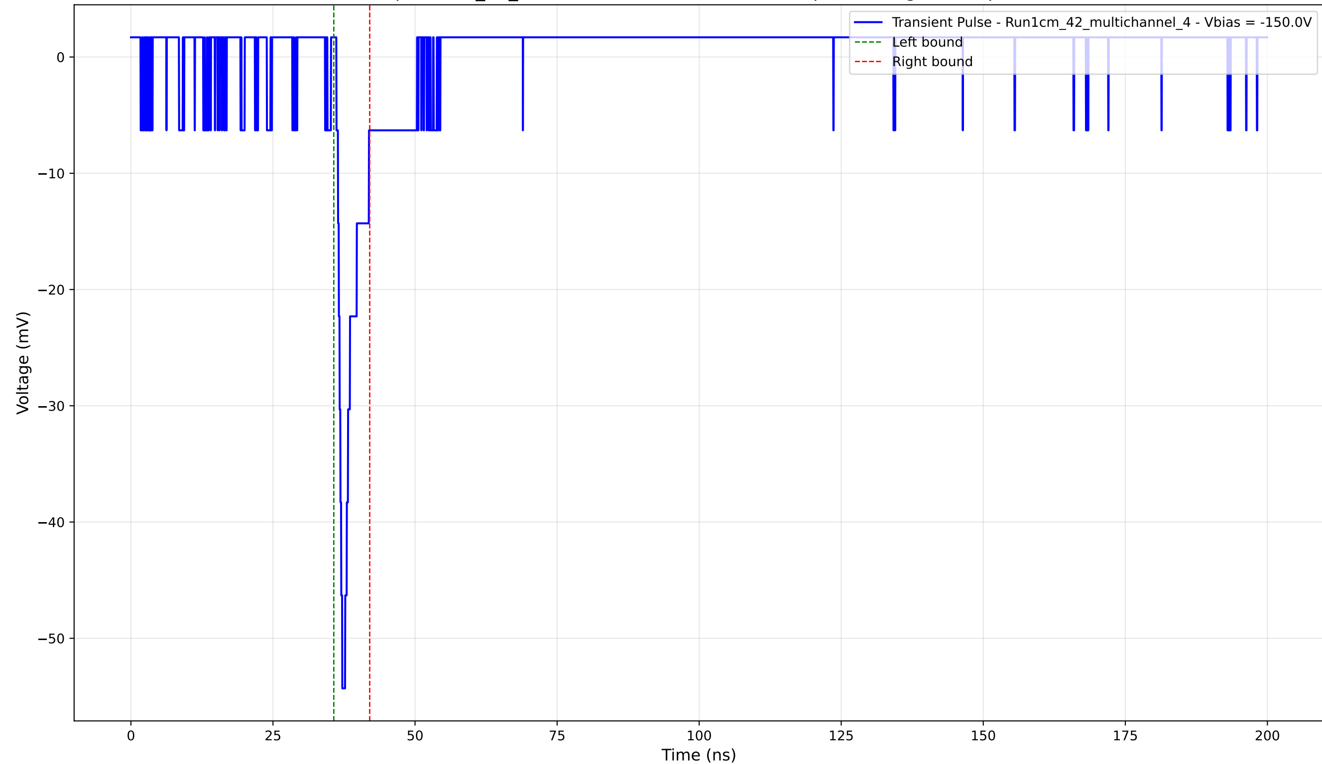
Transient Pulse - Sample: 1cm_42_multichannel - Position: 2720.0 \mu\text{m} - Charge: 2.85 pC - Rise Time: 1.02 ns
