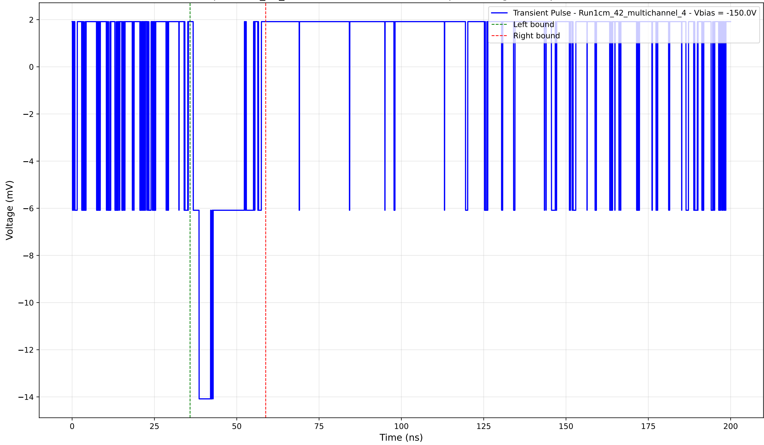
Transient Pulse - Sample: 1cm_42_multichannel - Position: 190.0 \mu\text{m} - Charge: 2.80 pC - Rise Time: 0.00 ns (N/A)
