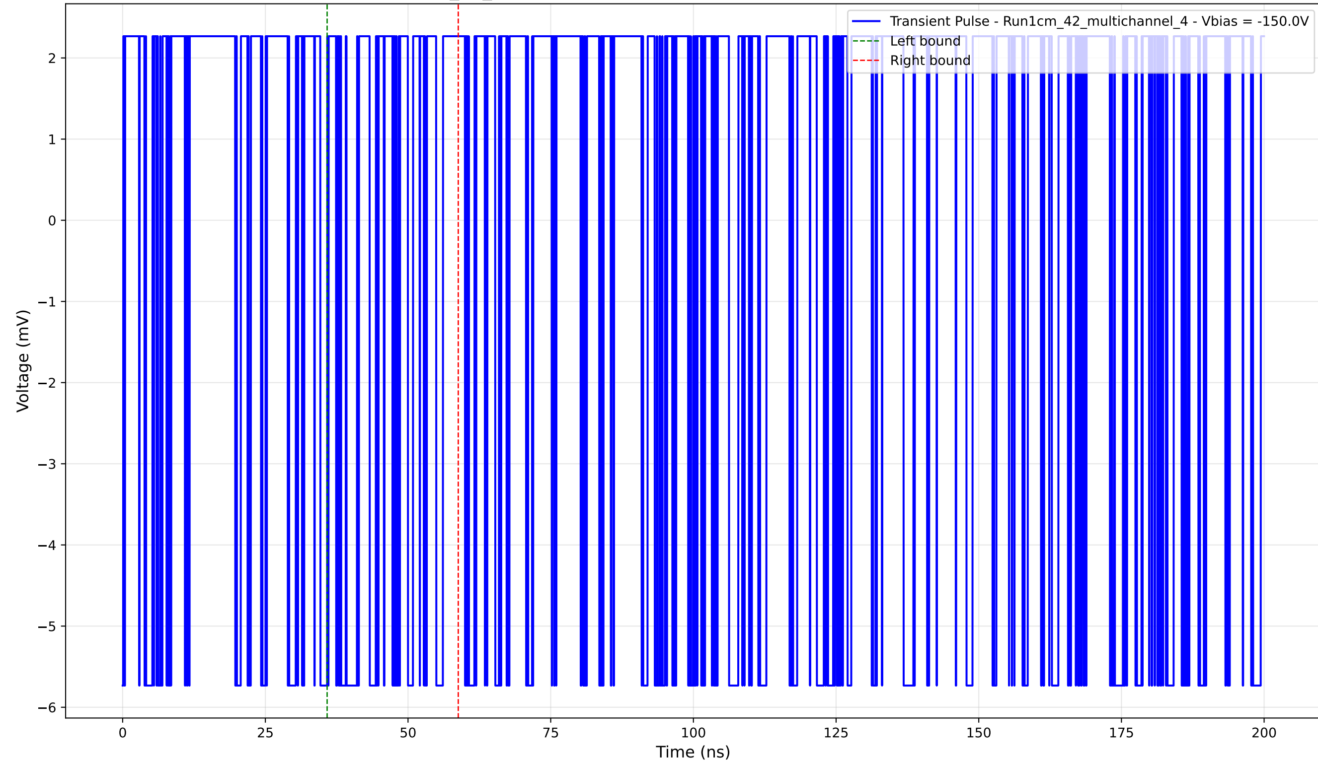
Transient Pulse - Sample: 1cm_42_multichannel - Position: 885.0 \mu\text{m} - Charge: 0.27 pC - Rise Time: 0.00 ns (N/A)
