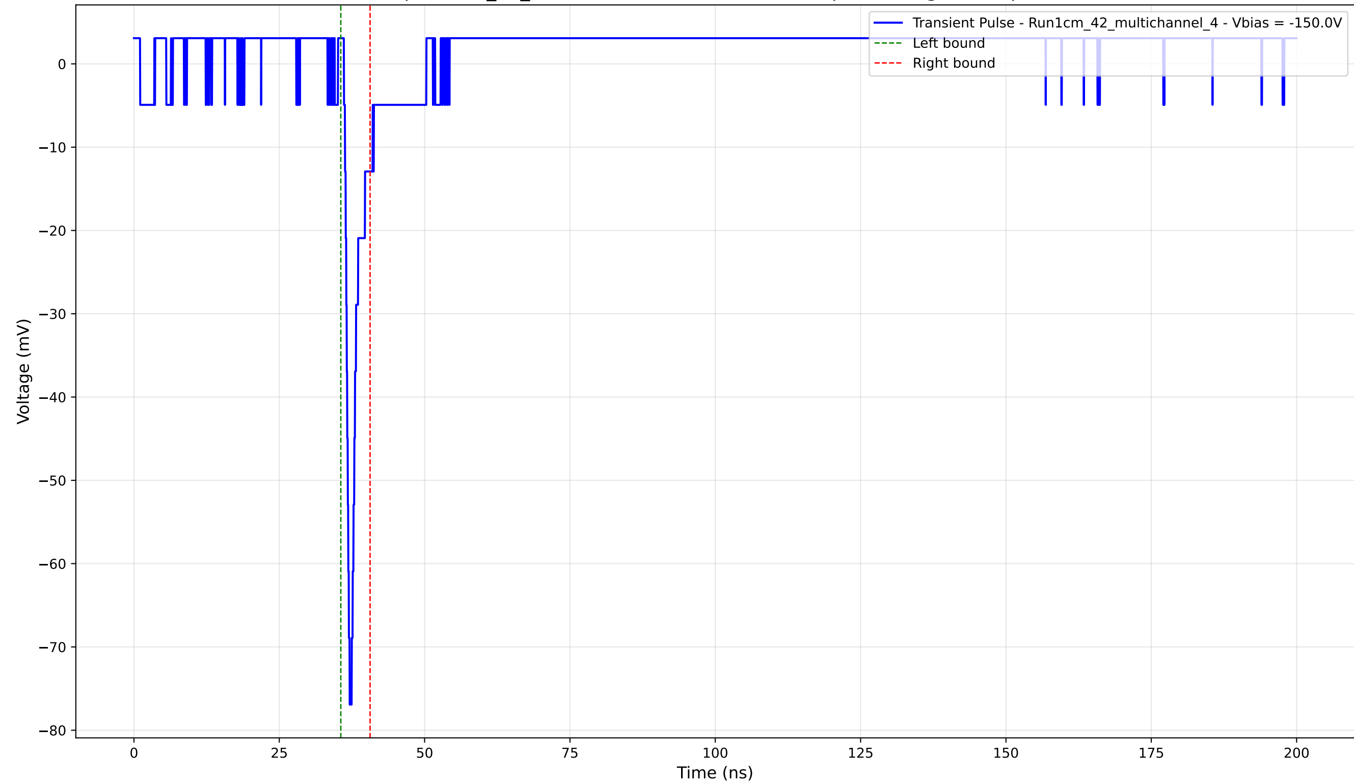
Transient Pulse - Sample: 1cm_42_multichannel - Position: 2235.0 \mu\text{m} - Charge: 2.92 pC - Rise Time: 0.81 ns
