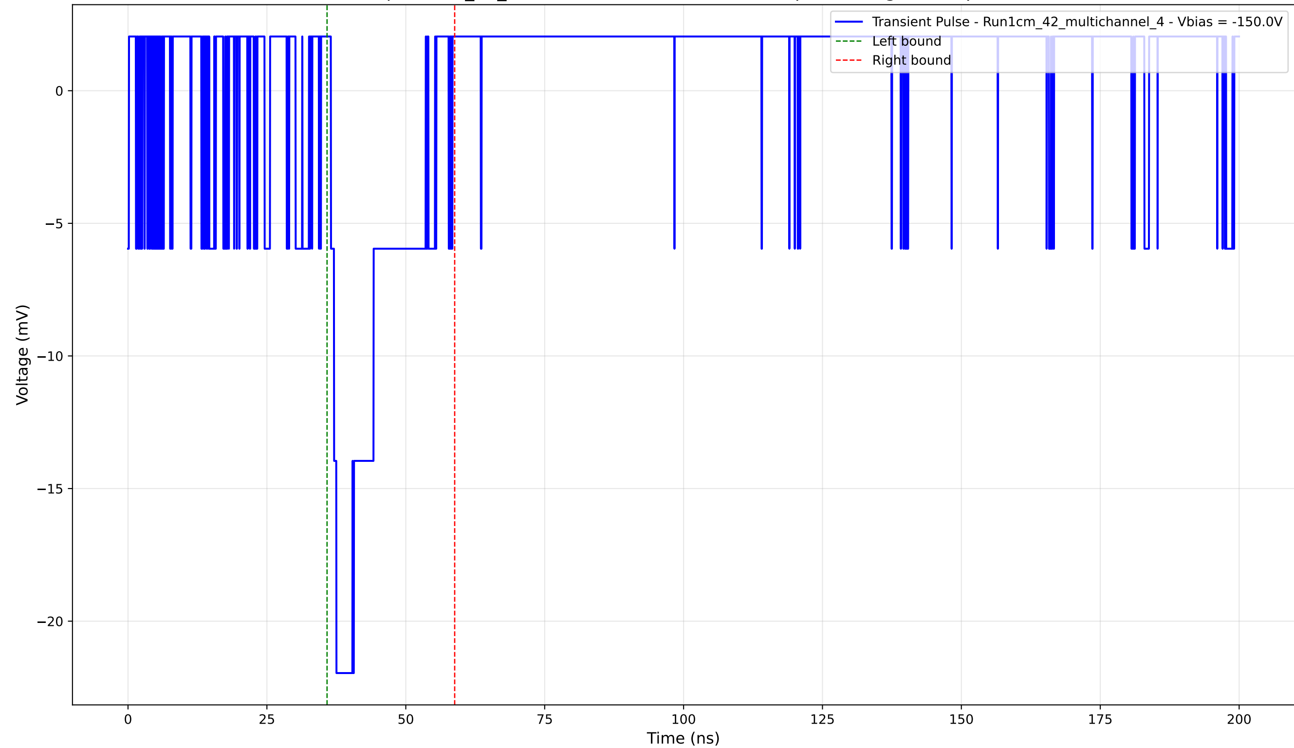
Transient Pulse - Sample: 1cm_42_multichannel - Position: 1285.0 \mu\text{m} - Charge: 3.76 pC - Rise Time: 1.00 ns
