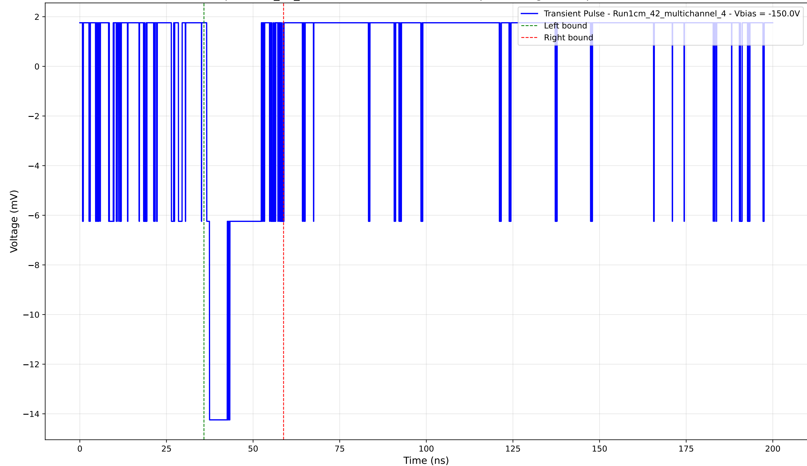
Transient Pulse - Sample: 1cm_42_multichannel - Position: 3645.0 \mu\text{m} - Charge: 2.97 pC - Rise Time: 0.00 ns (N/A)
