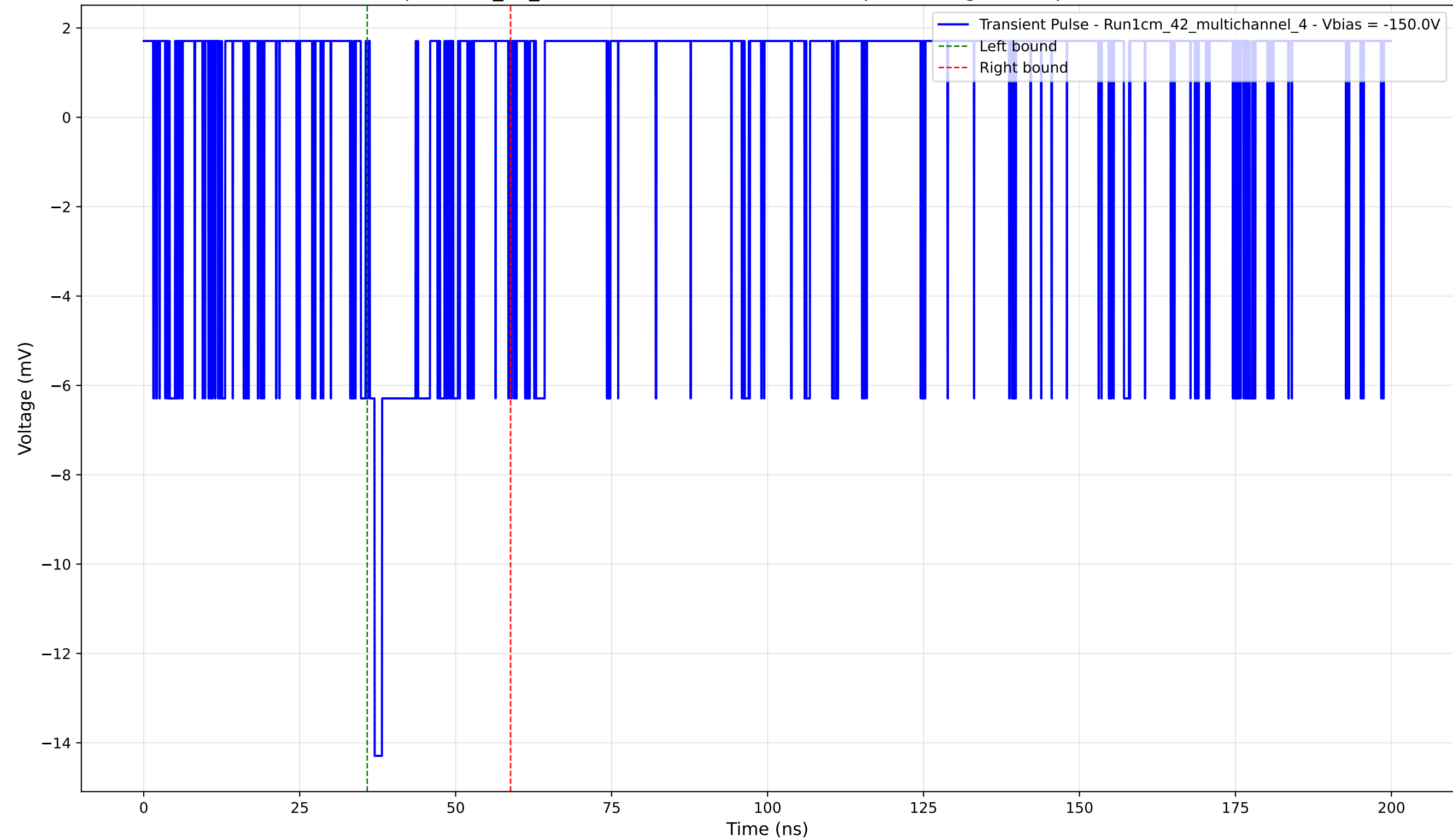
Transient Pulse - Sample: 1cm_42_multichannel - Position: 2850.0 \mu\text{m} - Charge: 1.46 pC - Rise Time: 0.00 ns (N/A)
