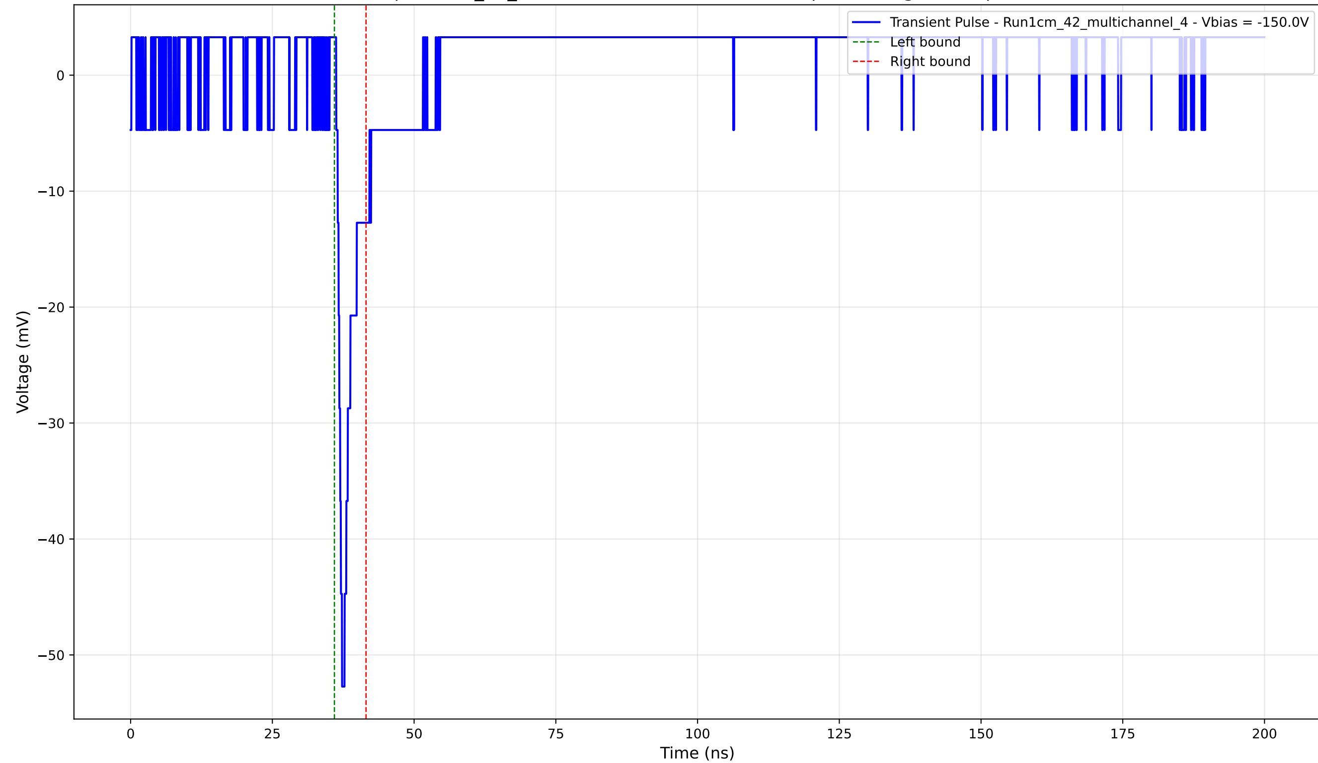
Transient Pulse - Sample: 1cm_42_multichannel - Position: 1970.0 \mu\text{m} - Charge: 2.55 pC - Rise Time: 0.78 ns
