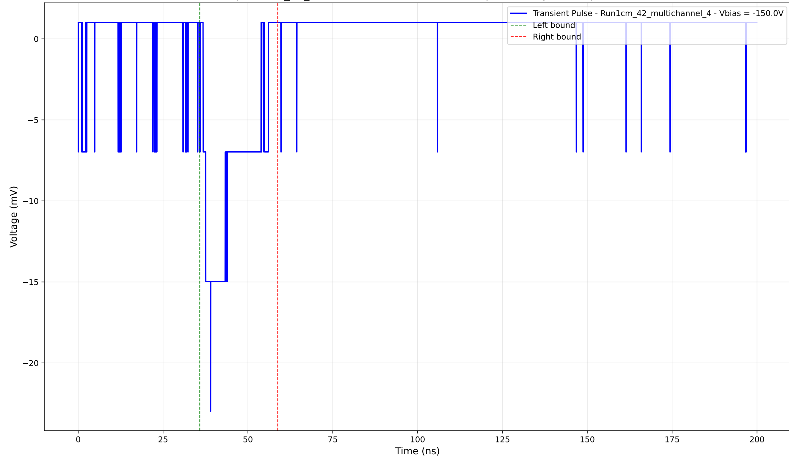
Transient Pulse - Sample: 1cm_42_multichannel - Position: 3790.0 \mu\text{m} - Charge: 3.45 pC - Rise Time: 2.18 ns
