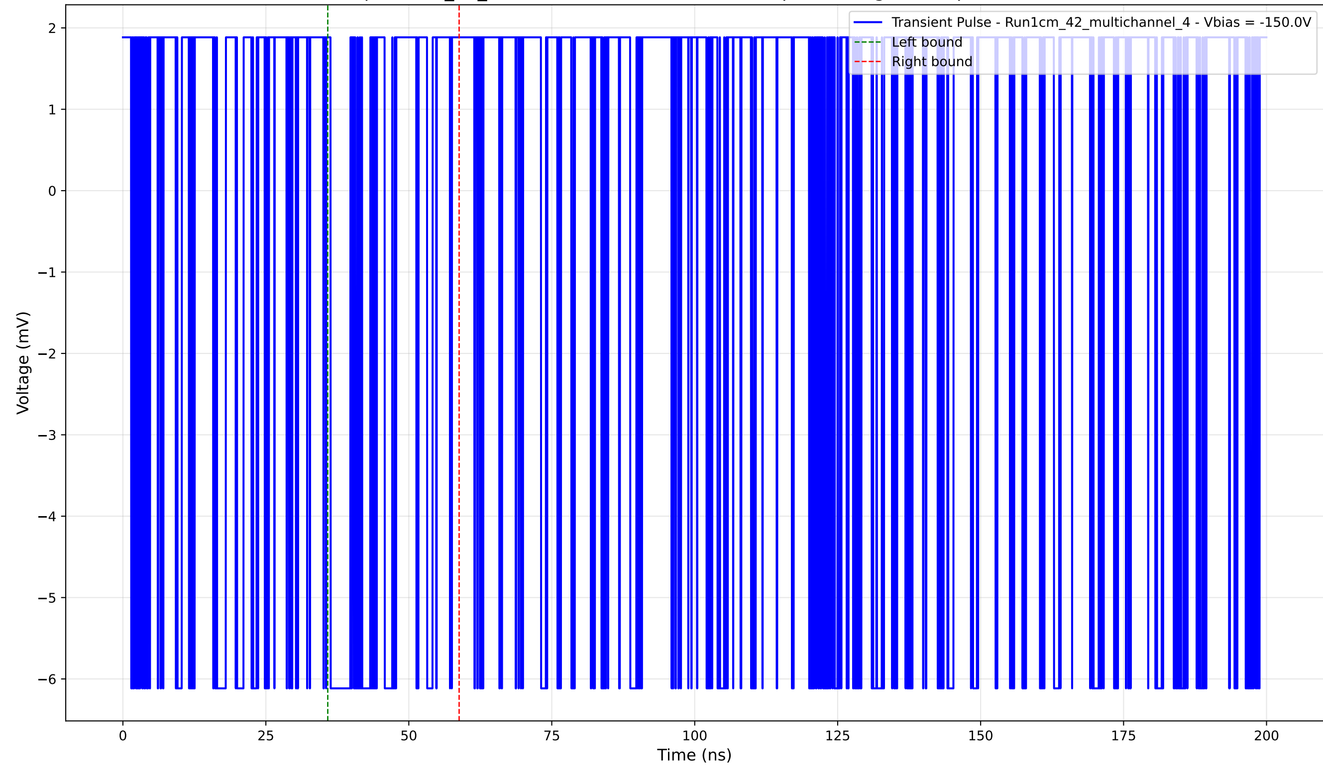
Transient Pulse - Sample: 1cm_42_multichannel - Position: 2405.0 \mu\text{m} - Charge: 0.71 pC - Rise Time: 0.00 ns (N/A)
