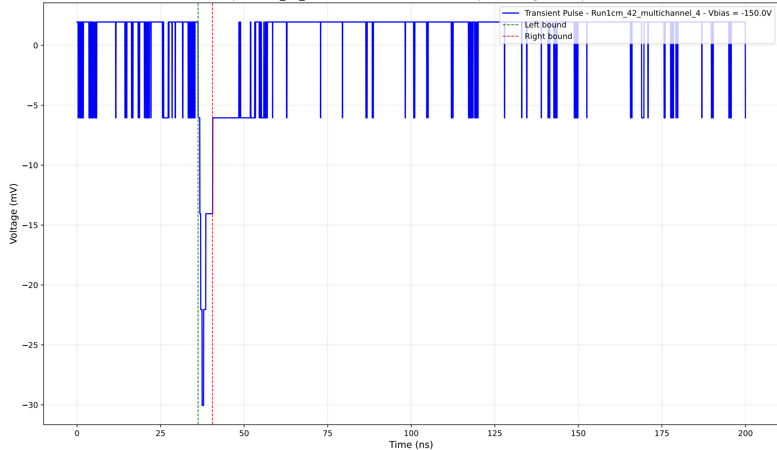
Transient Pulse - Sample: 1cm_42_multichannel - Position: 1825.0 \mu\text{m} - Charge: 1.45 pC - Rise Time: 1.21 ns
