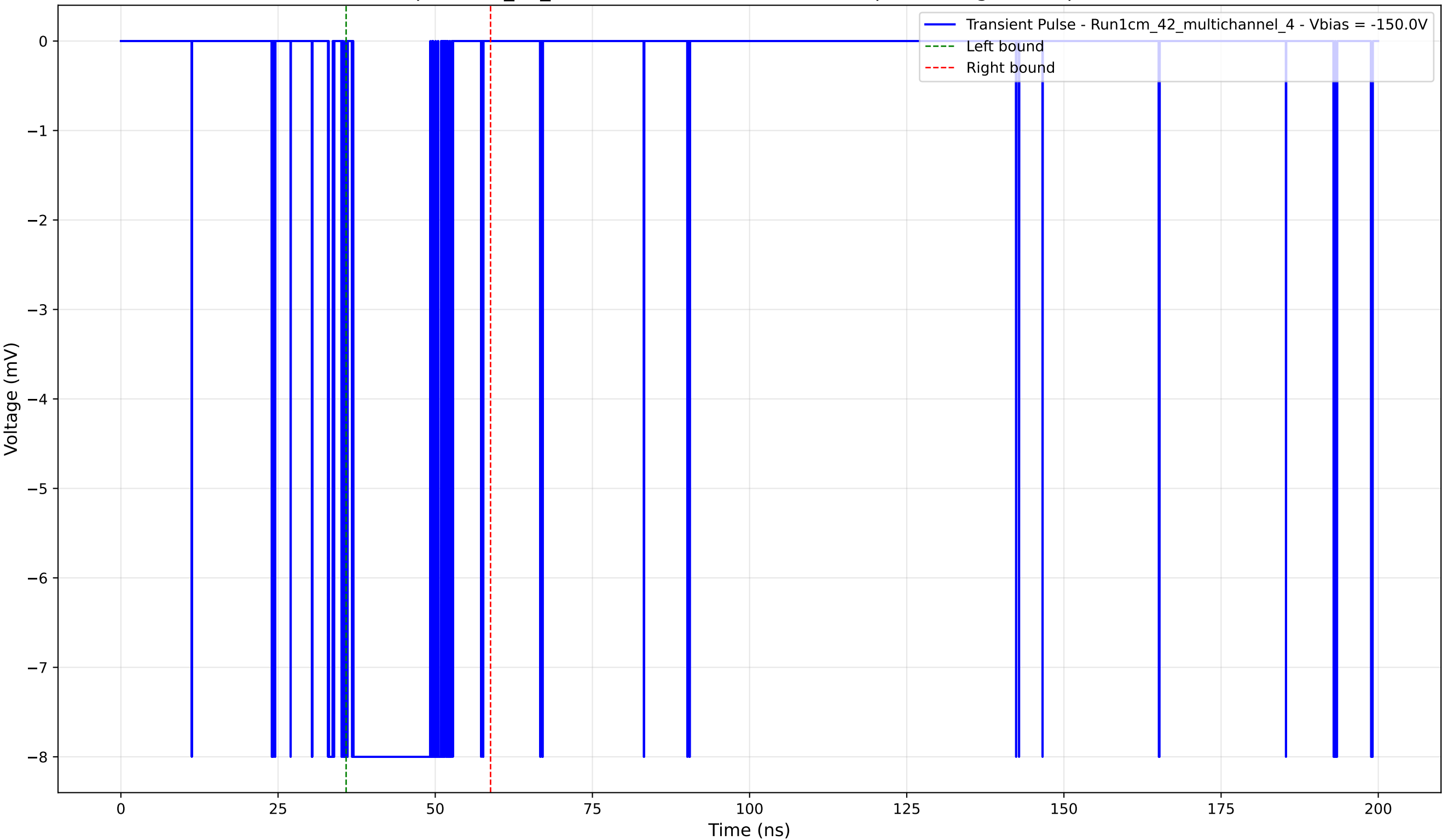
Transient Pulse - Sample: 1cm_42_multichannel - Position: 3955.0 \mu\text{m} - Charge: 2.37 pC - Rise Time: 0.02 ns
