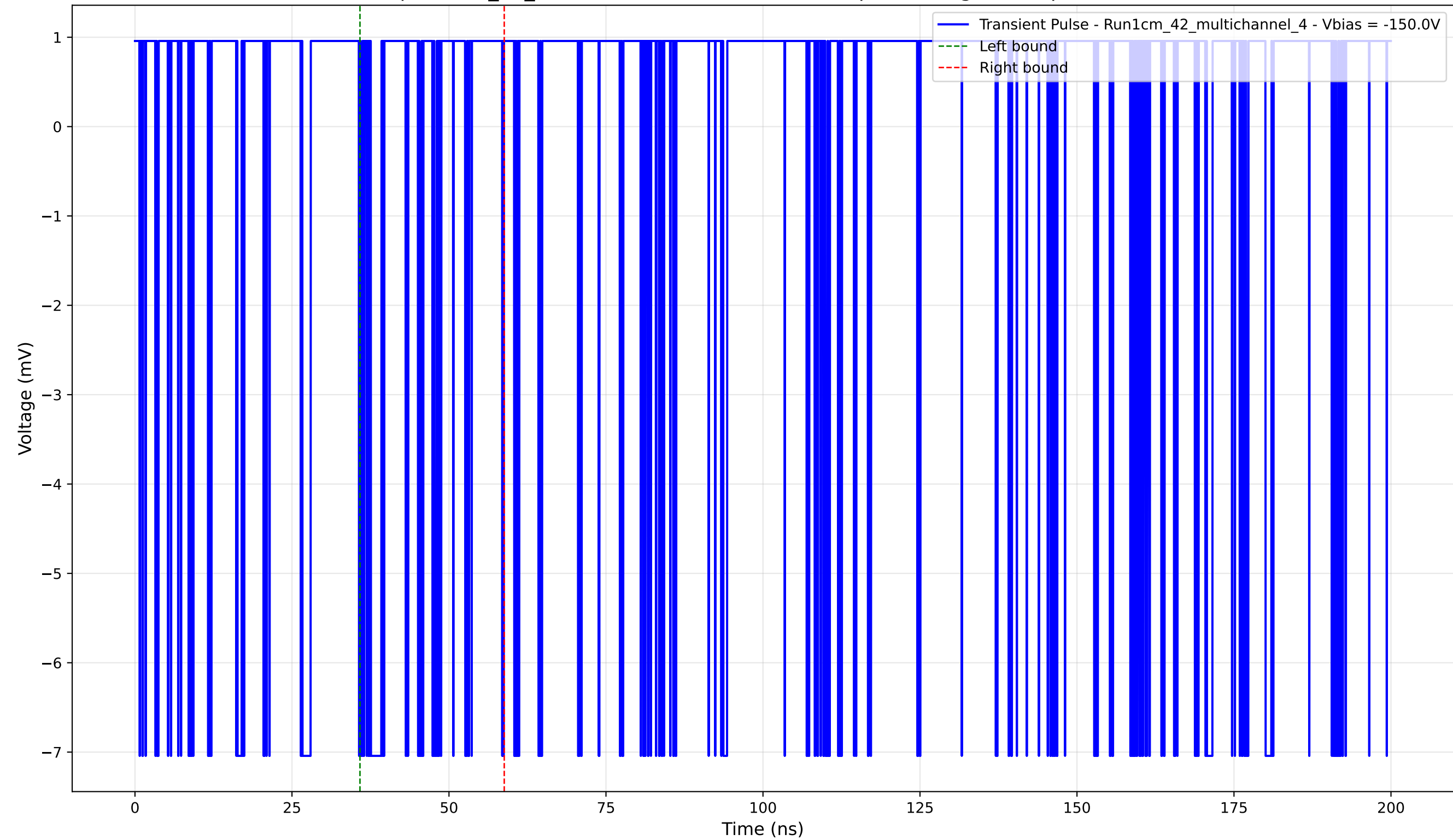
Transient Pulse - Sample: 1cm_42_multichannel - Position: 3395.0 \mu\text{m} - Charge: 0.35 pC - Rise Time: 0.00 ns (N/A)
