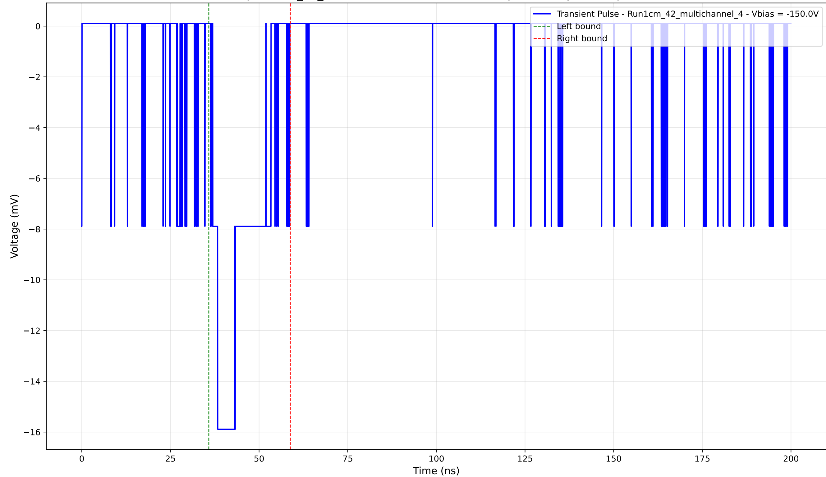
Transient Pulse - Sample: 1cm_42_multichannel - Position: 4490.0 \mu\text{m} - Charge: 3.49 pC - Rise Time: 1.40 ns
