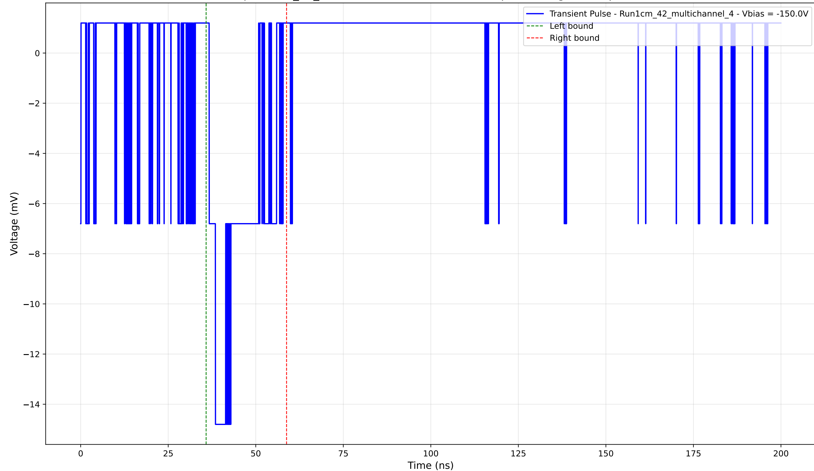
Transient Pulse - Sample: 1cm_42_multichannel - Position: 4735.0 \mu\text{m} - Charge: 2.89 pC - Rise Time: 1.80 ns
