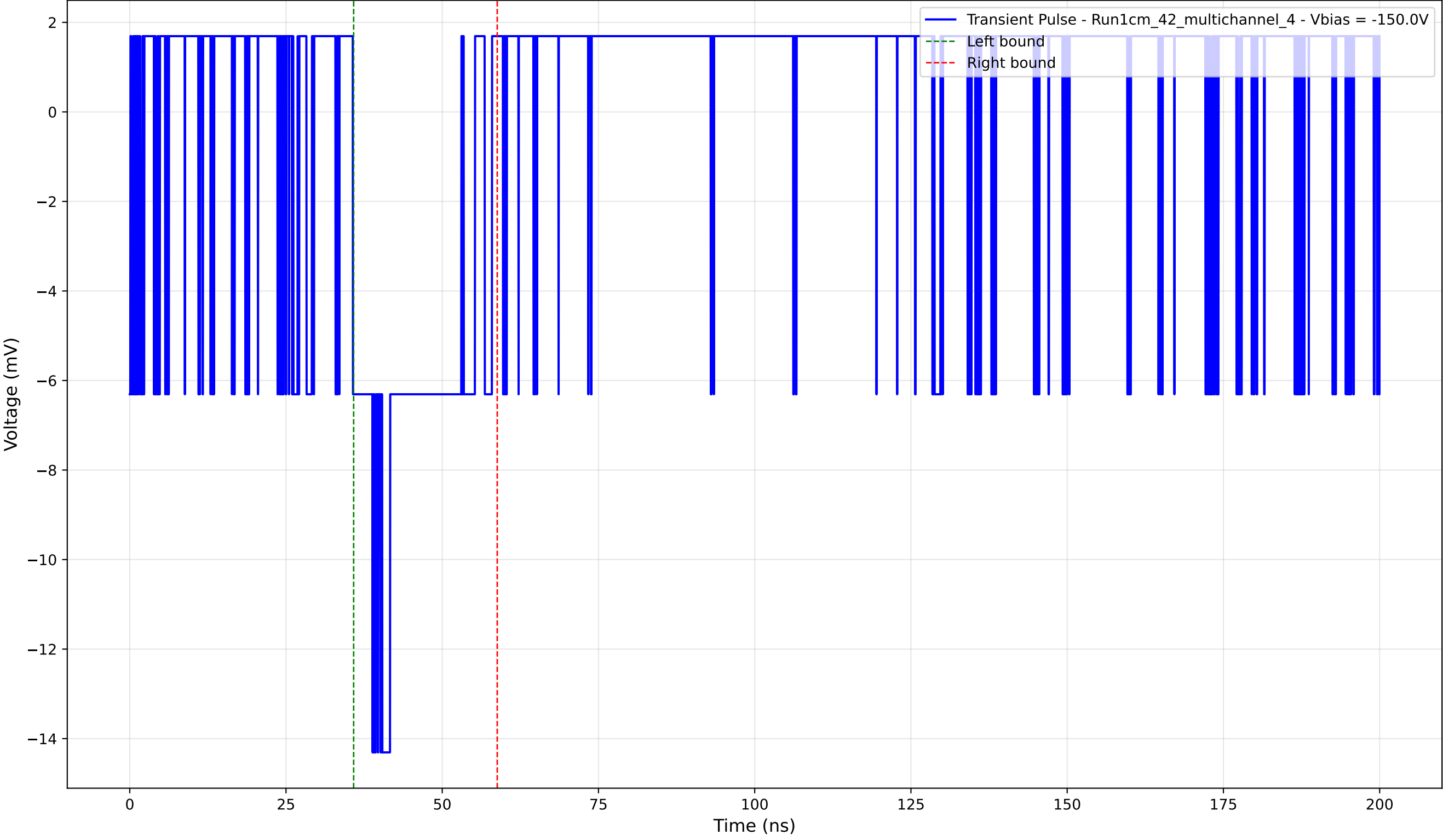
Transient Pulse - Sample: 1cm_42_multichannel - Position: 420.0 \mu\text{m} - Charge: 2.76 pC - Rise Time: 0.00 ns (N/A)
