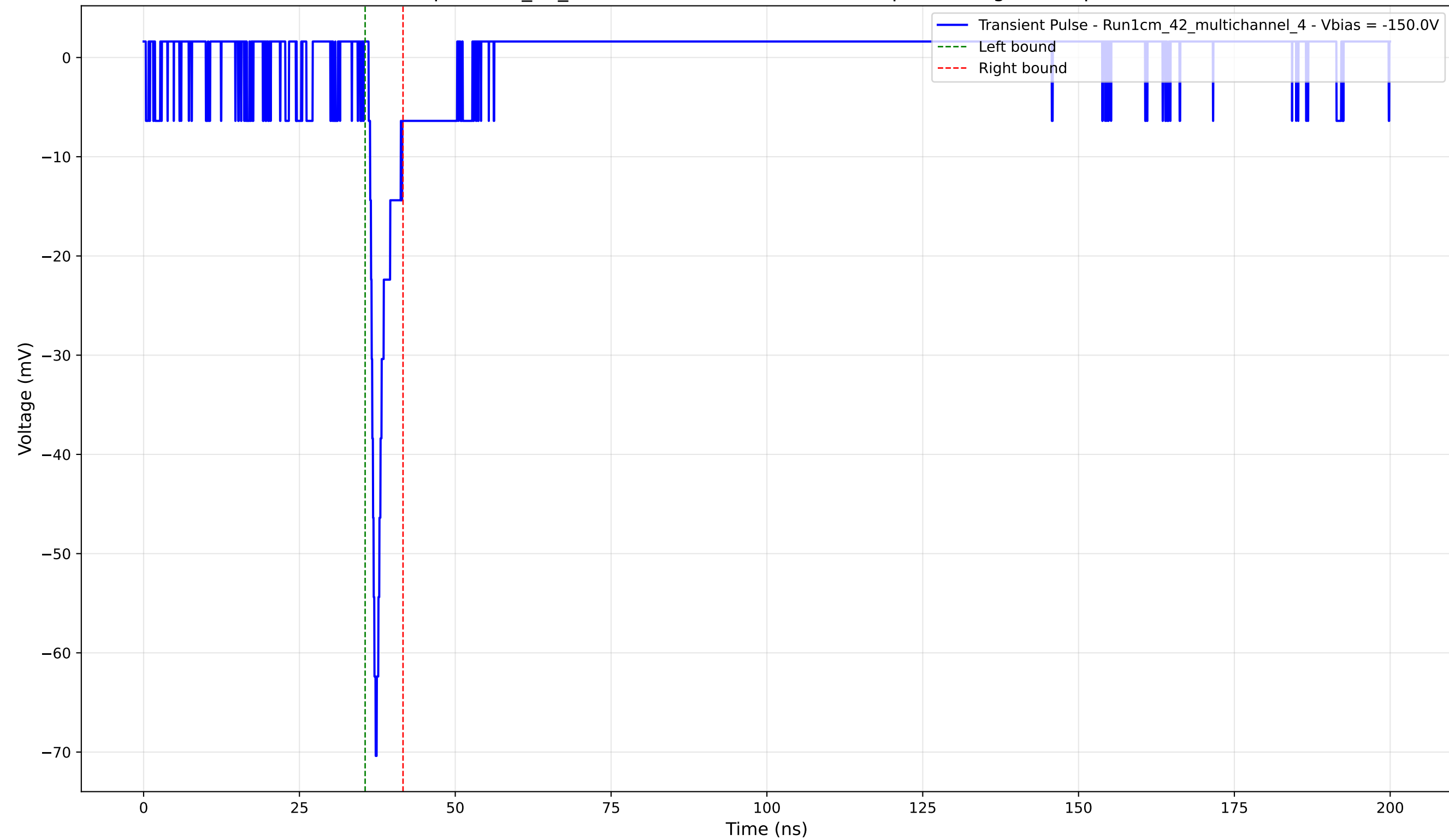
Transient Pulse - Sample: 1cm_42_multichannel - Position: 2575.0 \mu\text{m} - Charge: 3.02 pC - Rise Time: 0.90 ns
