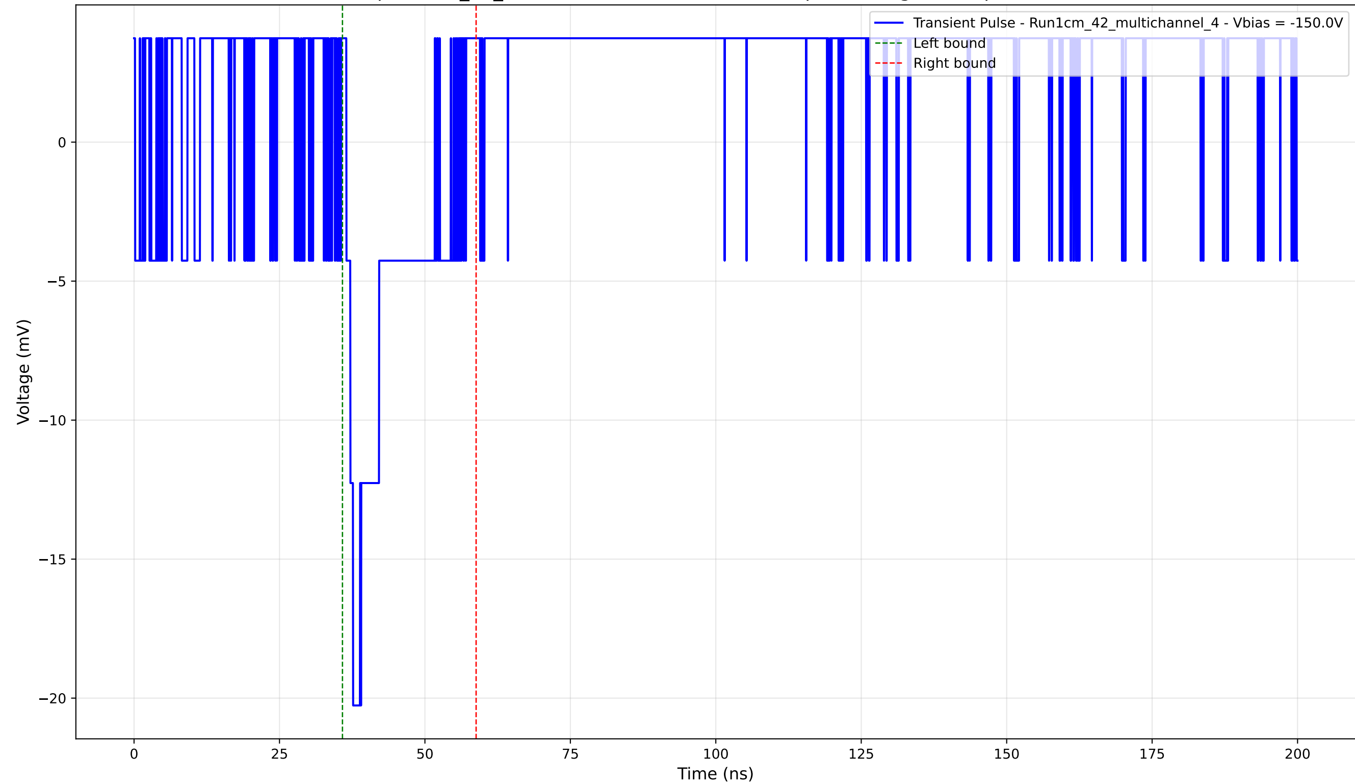
Transient Pulse - Sample: 1cm_42_multichannel - Position: 1435.0 \mu\text{m} - Charge: 2.34 pC - Rise Time: 0.00 ns (N/A)
