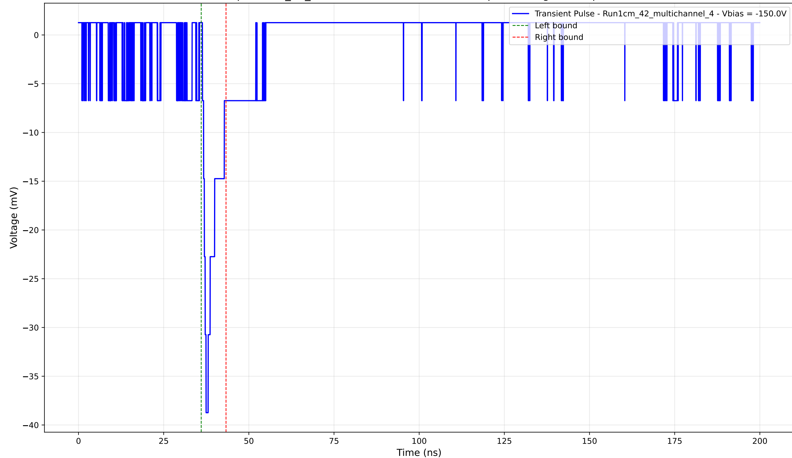
Transient Pulse - Sample: 1cm_42_multichannel - Position: 1695.0 \mu\text{m} - Charge: 2.71 pC - Rise Time: 1.07 ns
