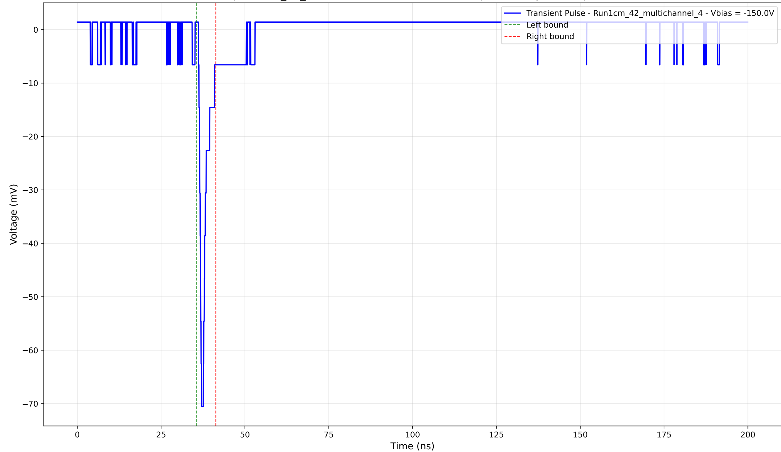
Transient Pulse - Sample: 1cm_42_multichannel - Position: 2545.0 \mu\text{m} - Charge: 3.05 pC - Rise Time: 0.76 ns
