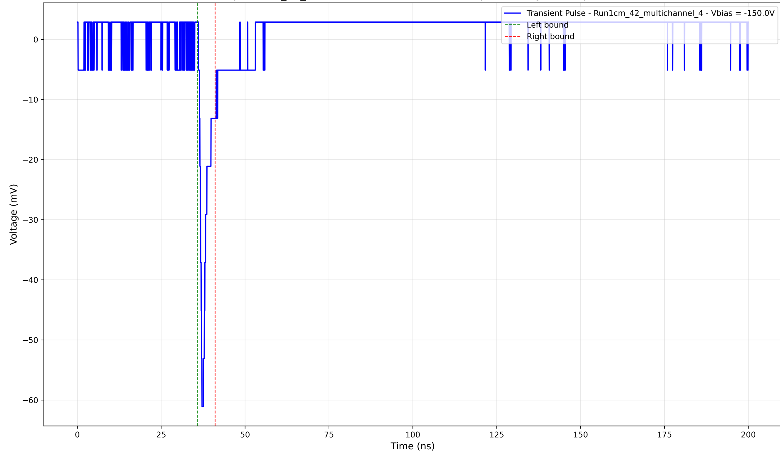
Transient Pulse - Sample: 1cm_42_multichannel - Position: 2110.0 \mu\text{m} - Charge: 2.70 pC - Rise Time: 0.78 ns
