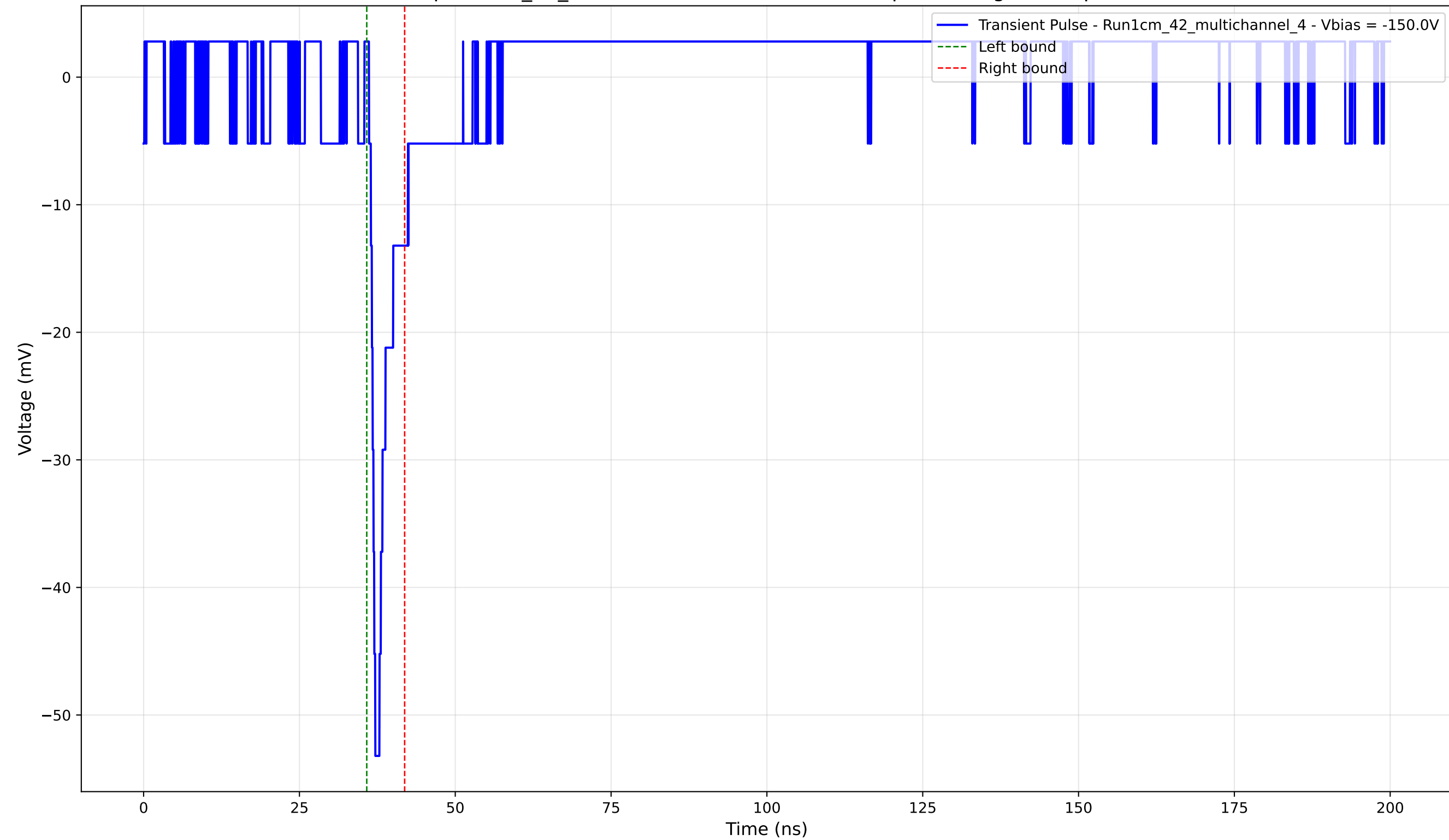
Transient Pulse - Sample: 1cm_42_multichannel - Position: 1995.0 \mu\text{m} - Charge: 2.83 pC - Rise Time: 0.72 ns
