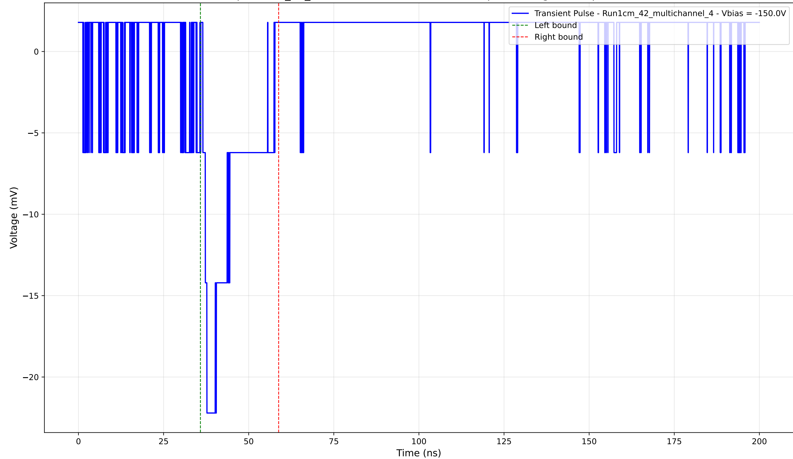
Transient Pulse - Sample: 1cm_42_multichannel - Position: 1220.0 \mu\text{m} - Charge: 4.05 pC - Rise Time: 1.20 ns
