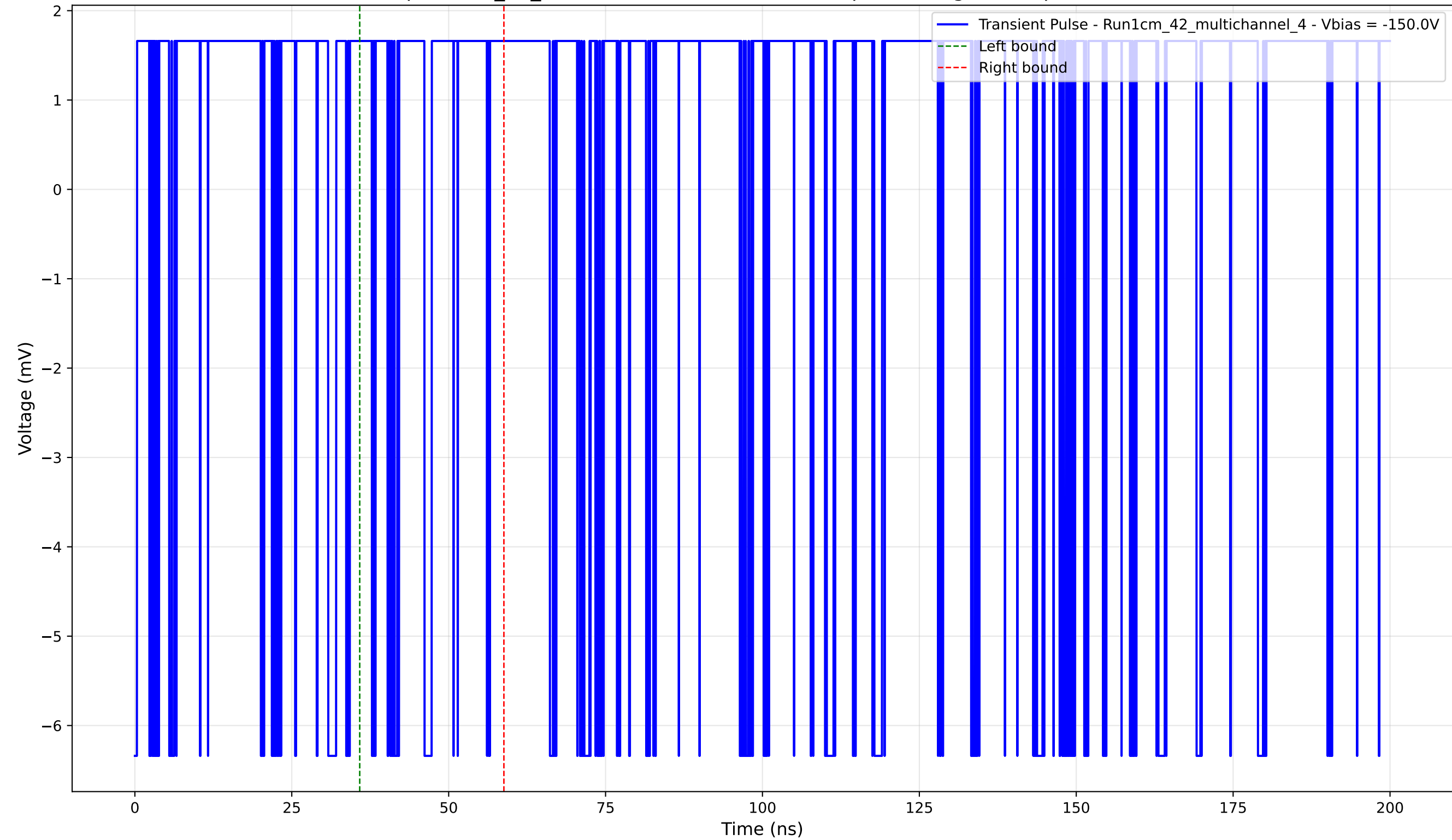
Transient Pulse - Sample: 1cm_42_multichannel - Position: 370.0 \mu\text{m} - Charge: 0.30 pC - Rise Time: 0.00 ns (N/A)
