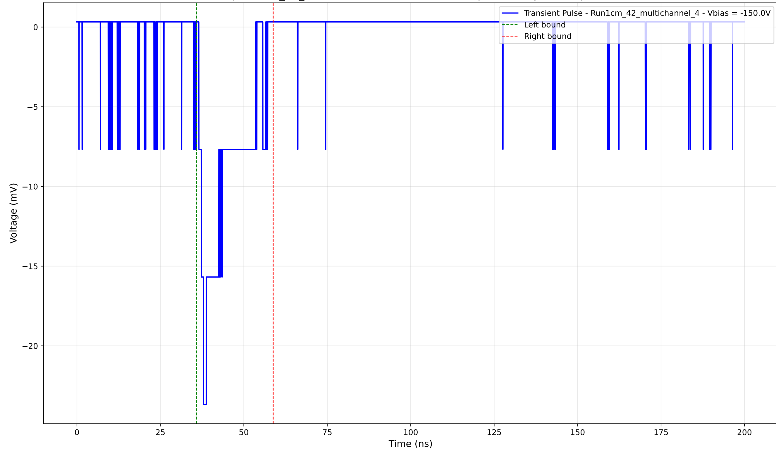
Transient Pulse - Sample: 1cm_42_multichannel - Position: 3560.0 \mu\text{m} - Charge: 3.81 pC - Rise Time: 1.39 ns
