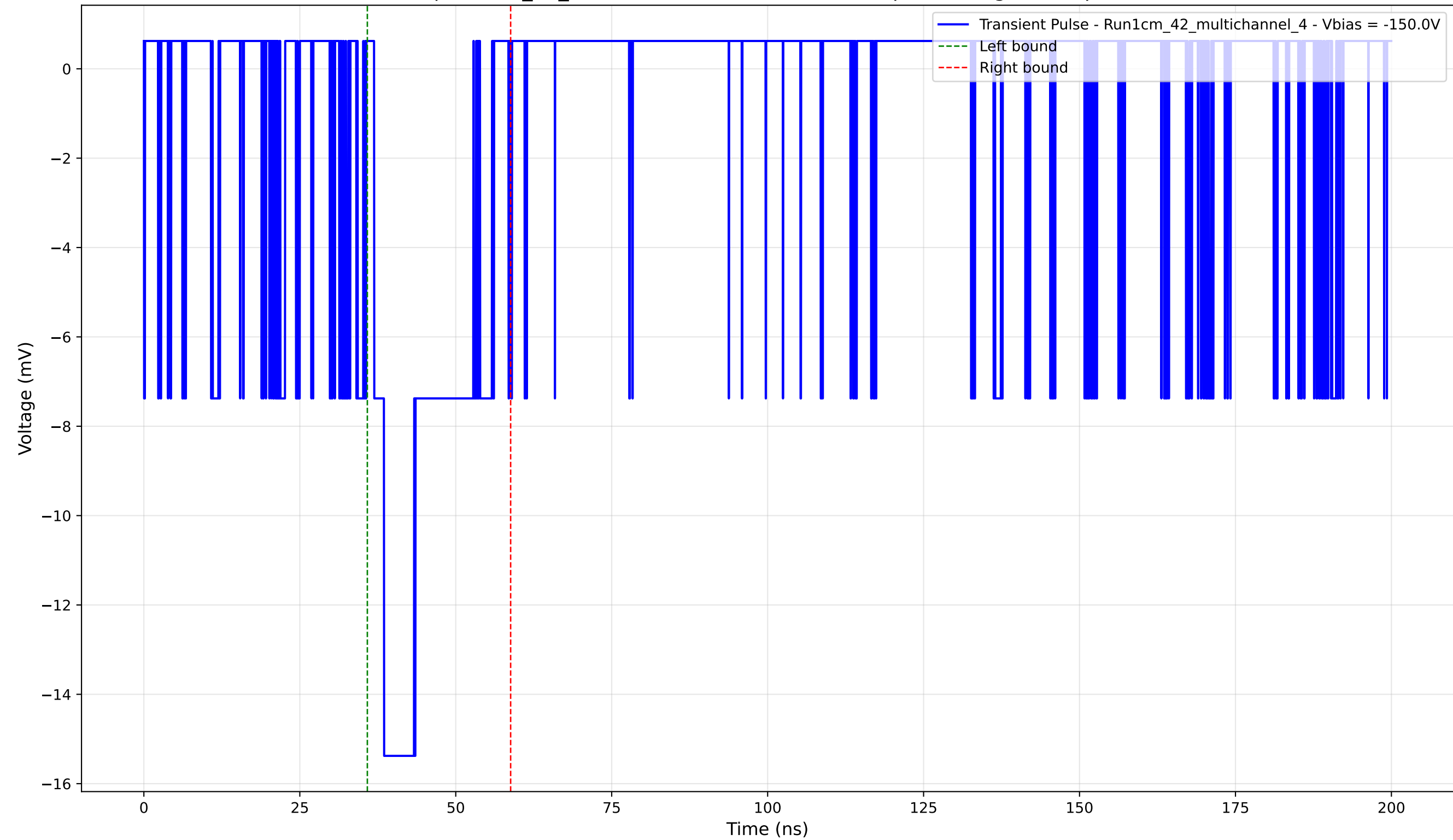
Transient Pulse - Sample: 1cm_42_multichannel - Position: 4555.0 \mu\text{m} - Charge: 3.49 pC - Rise Time: 1.60 ns
