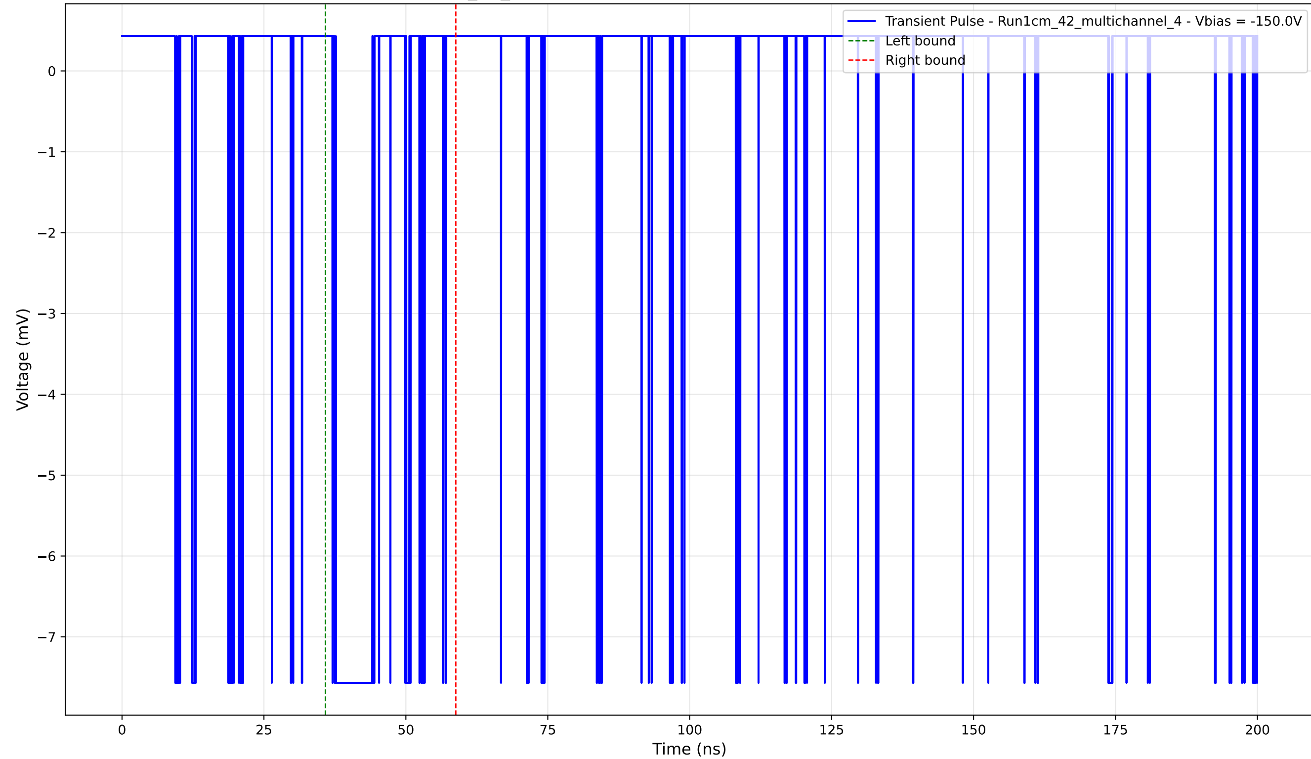
Transient Pulse - Sample: 1cm_42_multichannel - Position: 3940.0 \mu\text{m} - Charge: 1.13 pC - Rise Time: 0.02 ns
