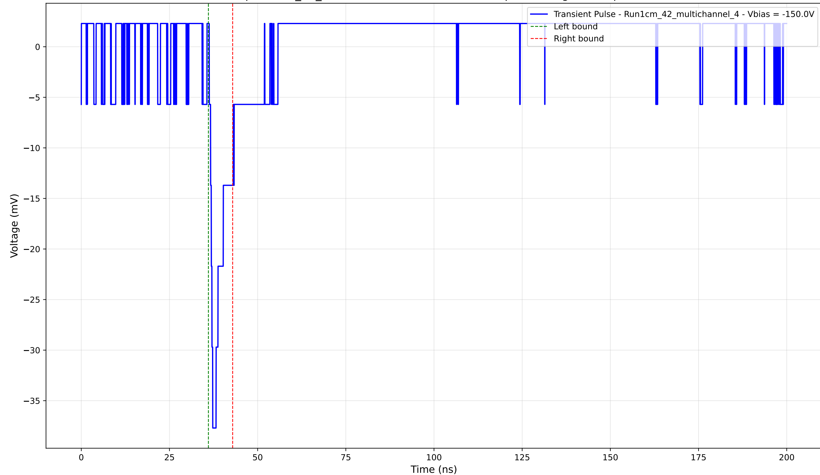
Transient Pulse - Sample: 1cm_42_multichannel - Position: 1750.0 \mu\text{m} - Charge: 2.72 pC - Rise Time: 0.99 ns
