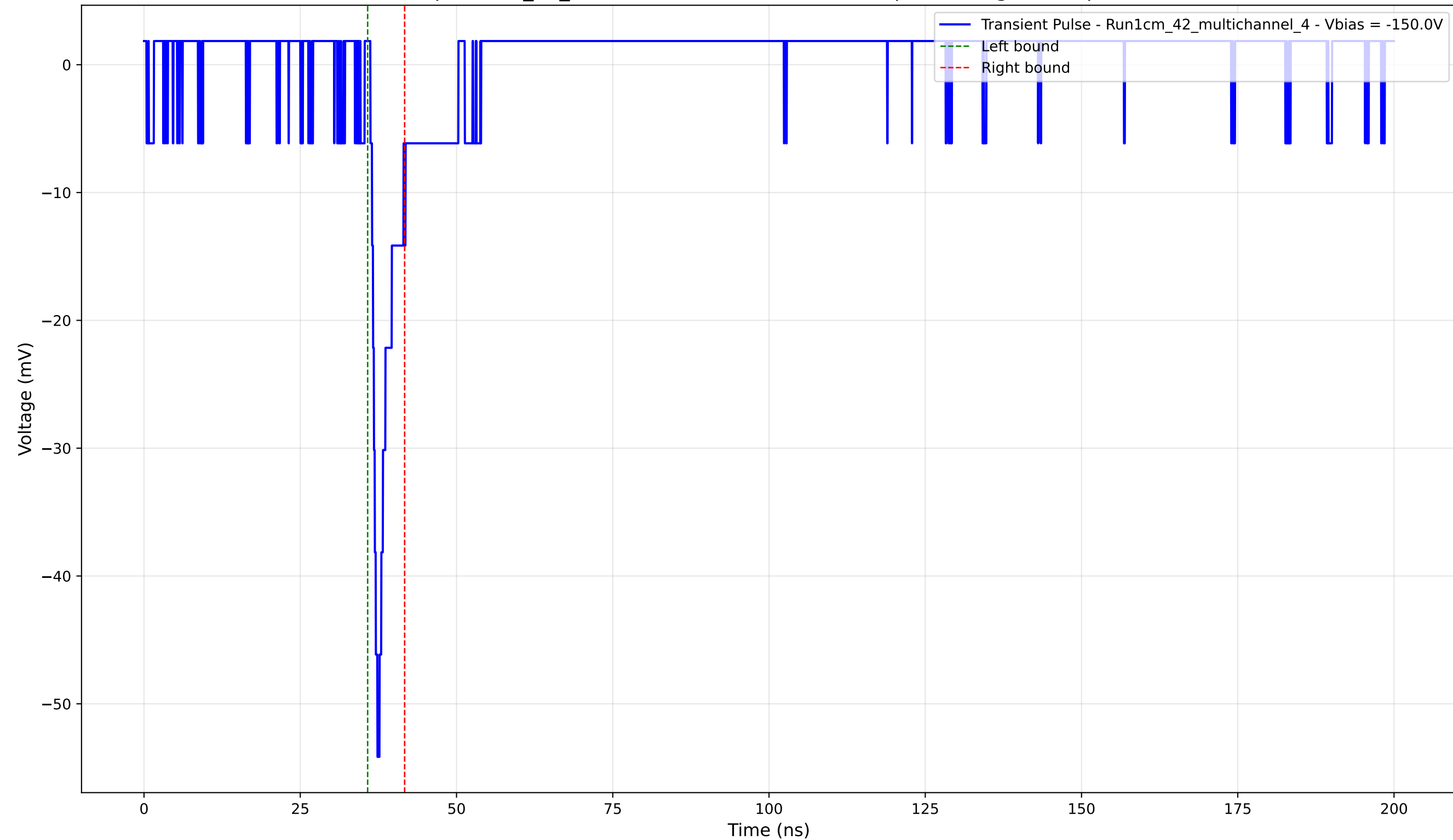
Transient Pulse - Sample: 1cm_42_multichannel - Position: 2770.0 \mu\text{m} - Charge: 2.65 pC - Rise Time: 1.12 ns
