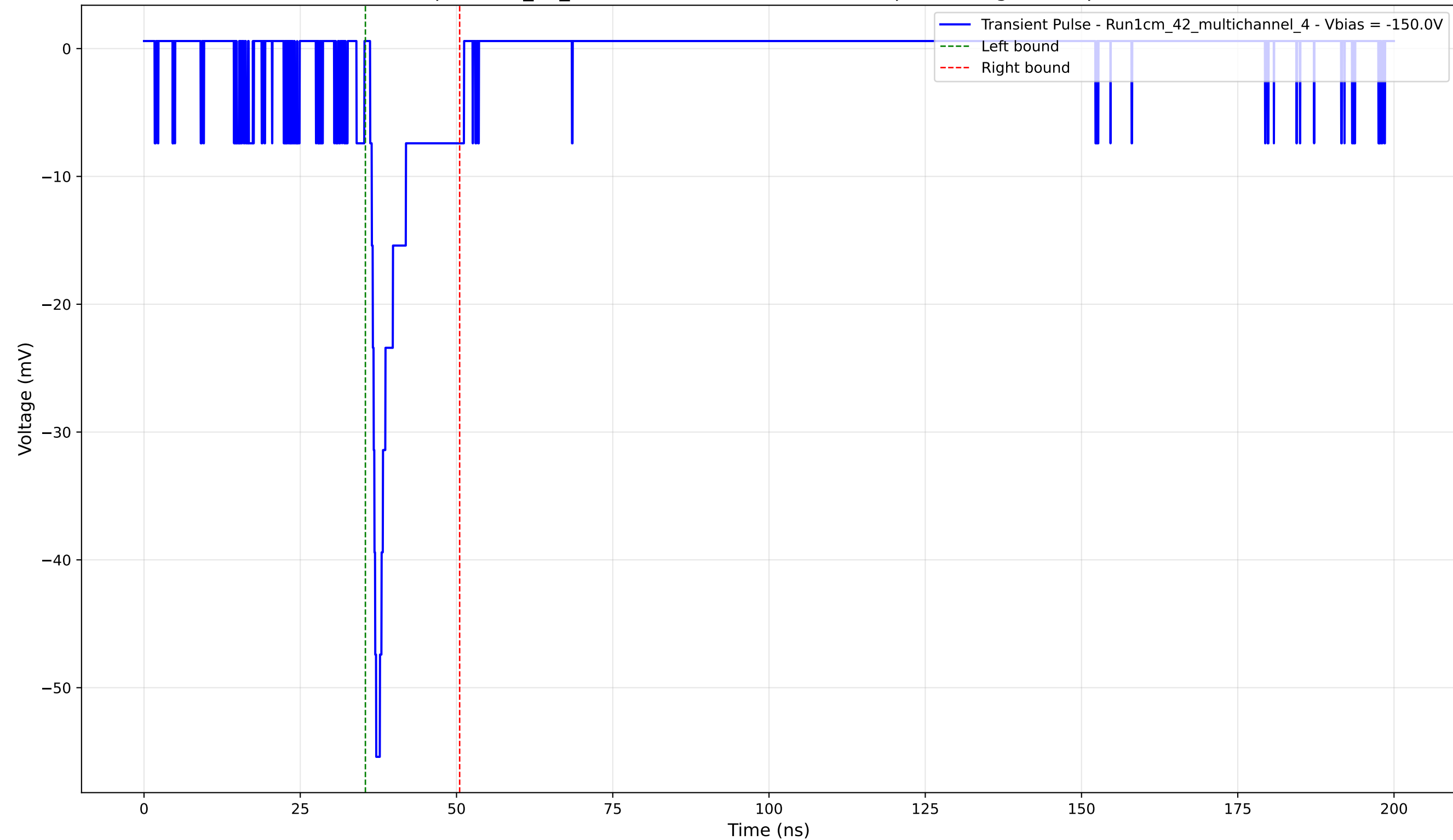
Transient Pulse - Sample: 1cm_42_multichannel - Position: 2050.0 \mu\text{m} - Charge: 4.28 pC - Rise Time: 0.97 ns
