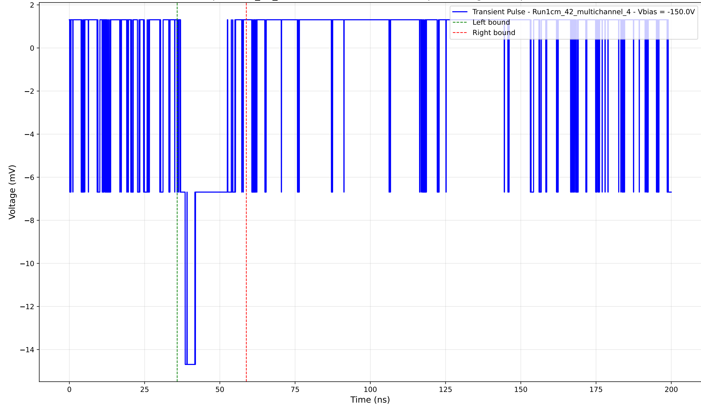
Transient Pulse - Sample: 1cm_42_multichannel - Position: 295.0 \mu\text{m} - Charge: 2.87 pC - Rise Time: 1.54 ns
