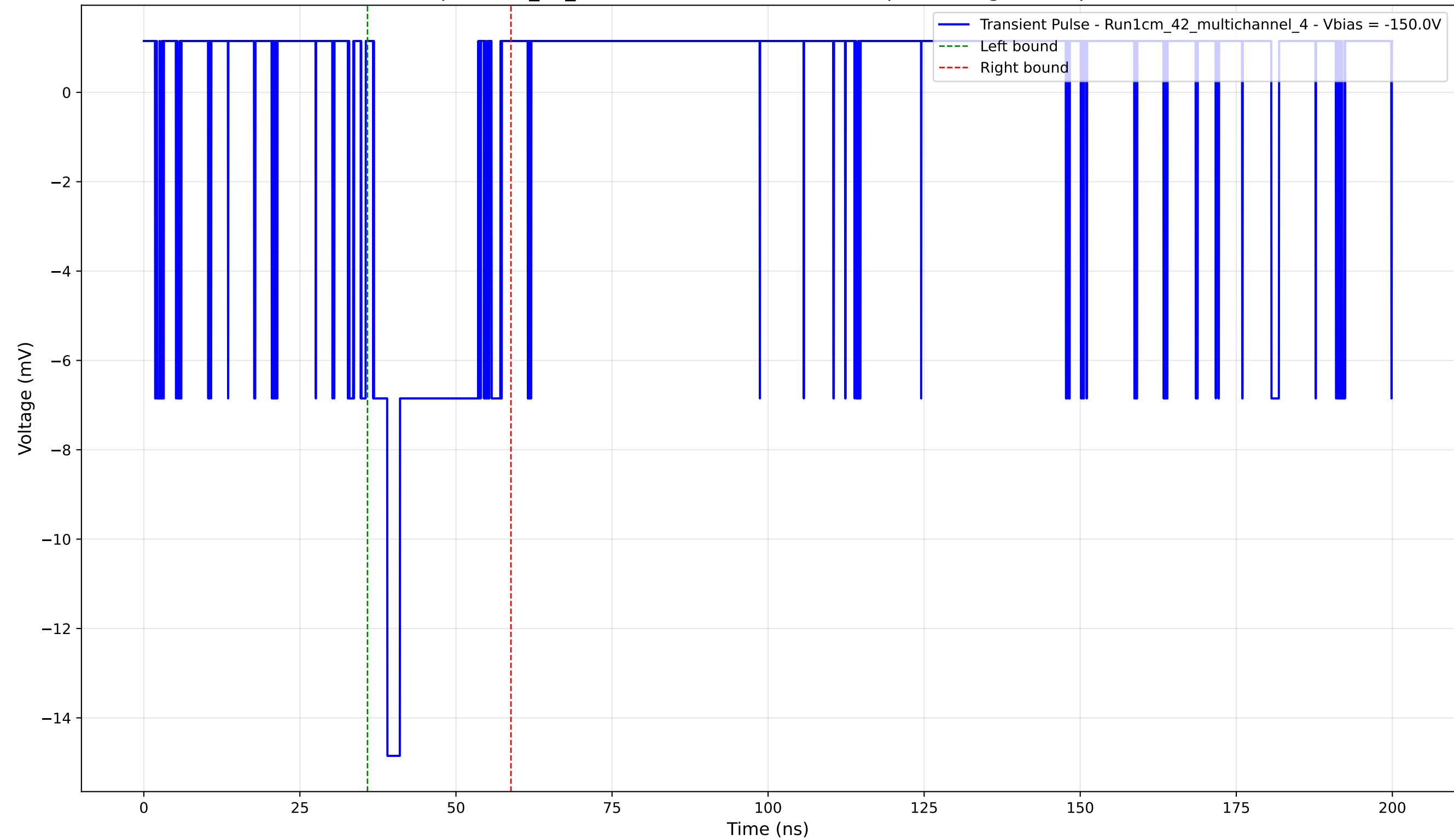
Transient Pulse - Sample: 1cm_42_multichannel - Position: 125.0 \mu\text{m} - Charge: 2.83 pC - Rise Time: 2.16 ns
