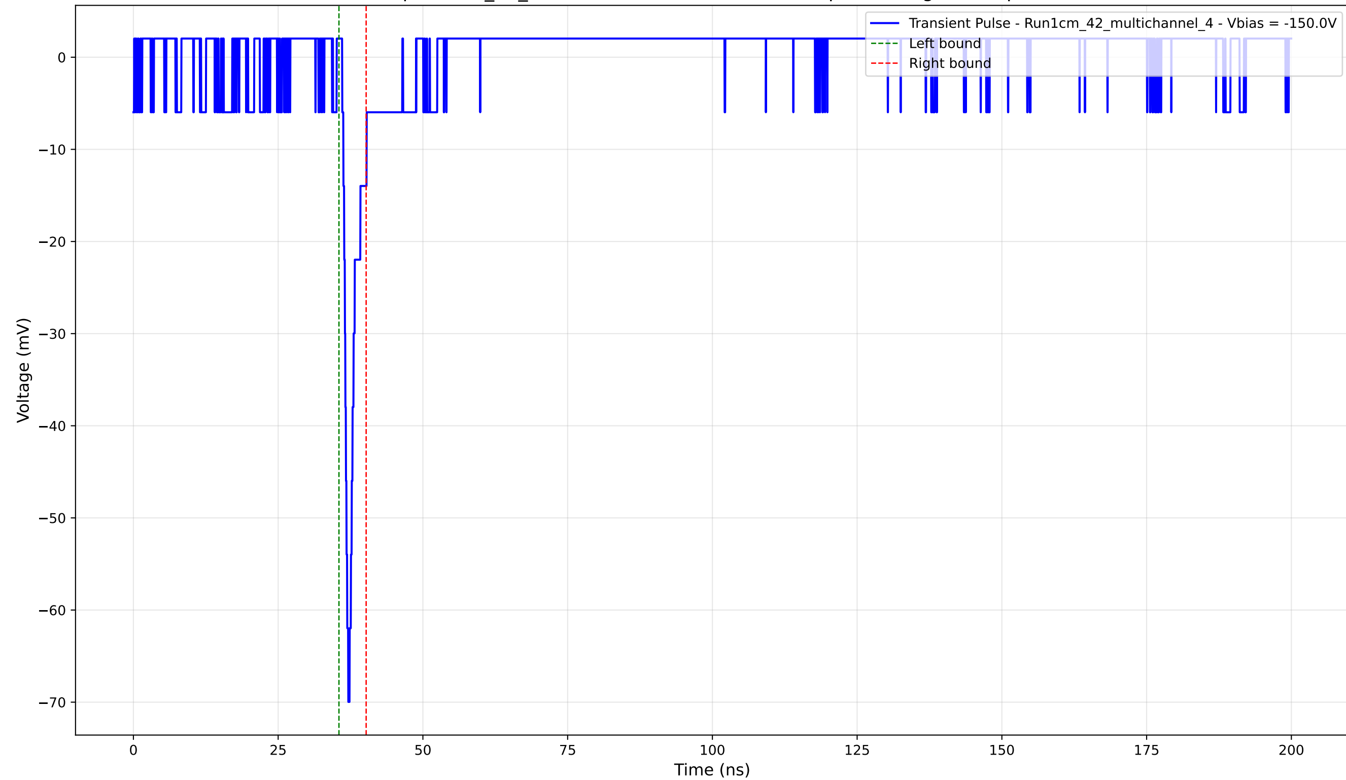
Transient Pulse - Sample: 1cm_42_multichannel - Position: 2450.0 \mu\text{m} - Charge: 2.52 pC - Rise Time: 0.86 ns
