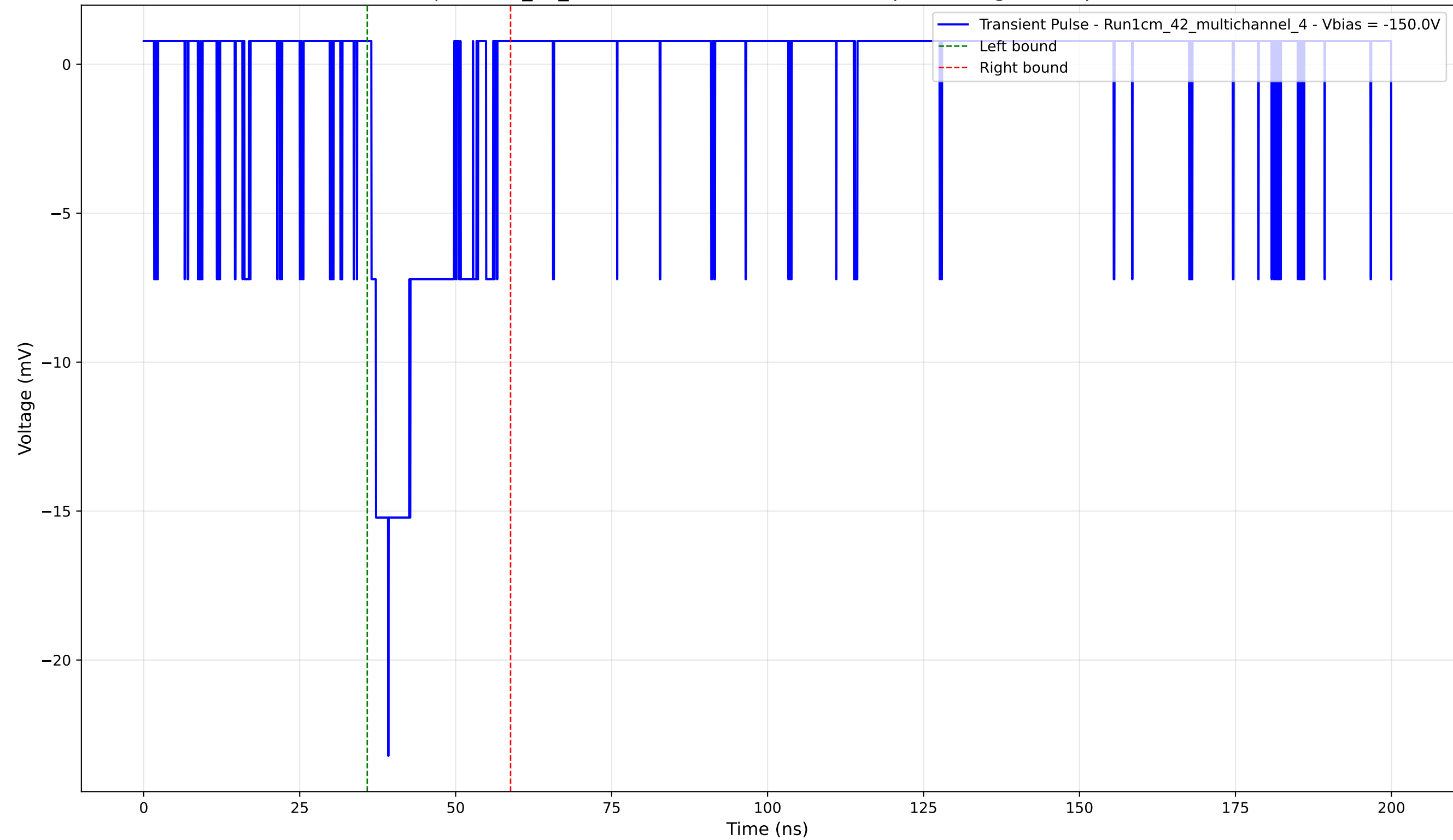
Transient Pulse - Sample: 1cm_42_multichannel - Position: 3470.0 \mu\text{m} - Charge: 3.33 pC - Rise Time: 2.70 ns
