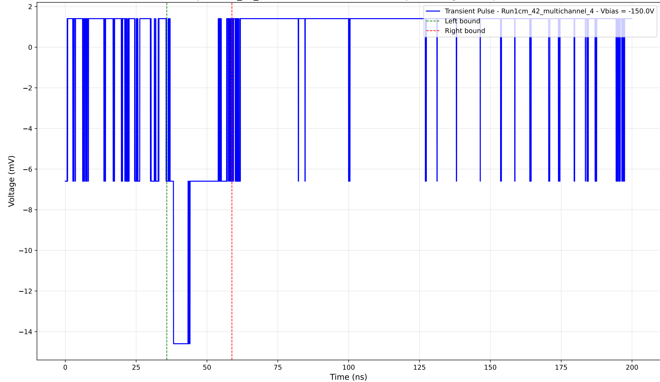
Transient Pulse - Sample: 1cm_42_multichannel - Position: 4300.0 \mu\text{m} - Charge: 3.56 pC - Rise Time: 1.24 ns
