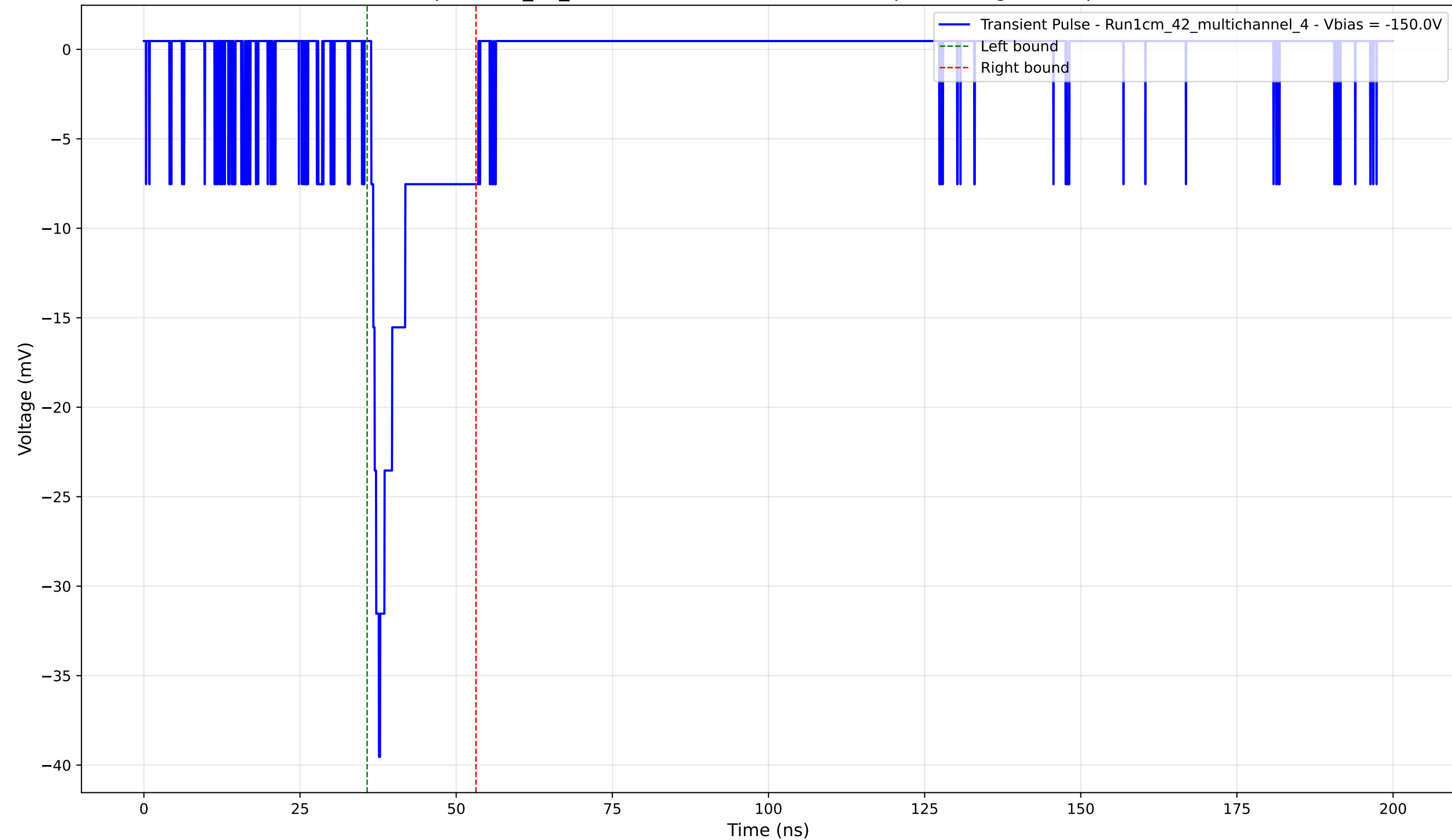
Transient Pulse - Sample: 1cm_42_multichannel - Position: 3035.0 \mu\text{m} - Charge: 4.04 pC - Rise Time: 1.23 ns
