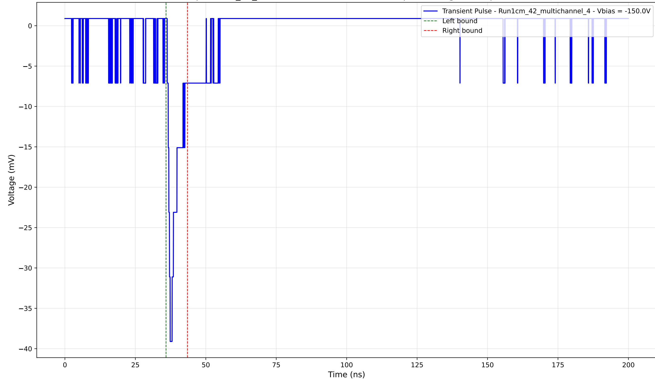
Transient Pulse - Sample: 1cm_42_multichannel - Position: 3010.0 \mu\text{m} - Charge: 2.70 pC - Rise Time: 1.03 ns
