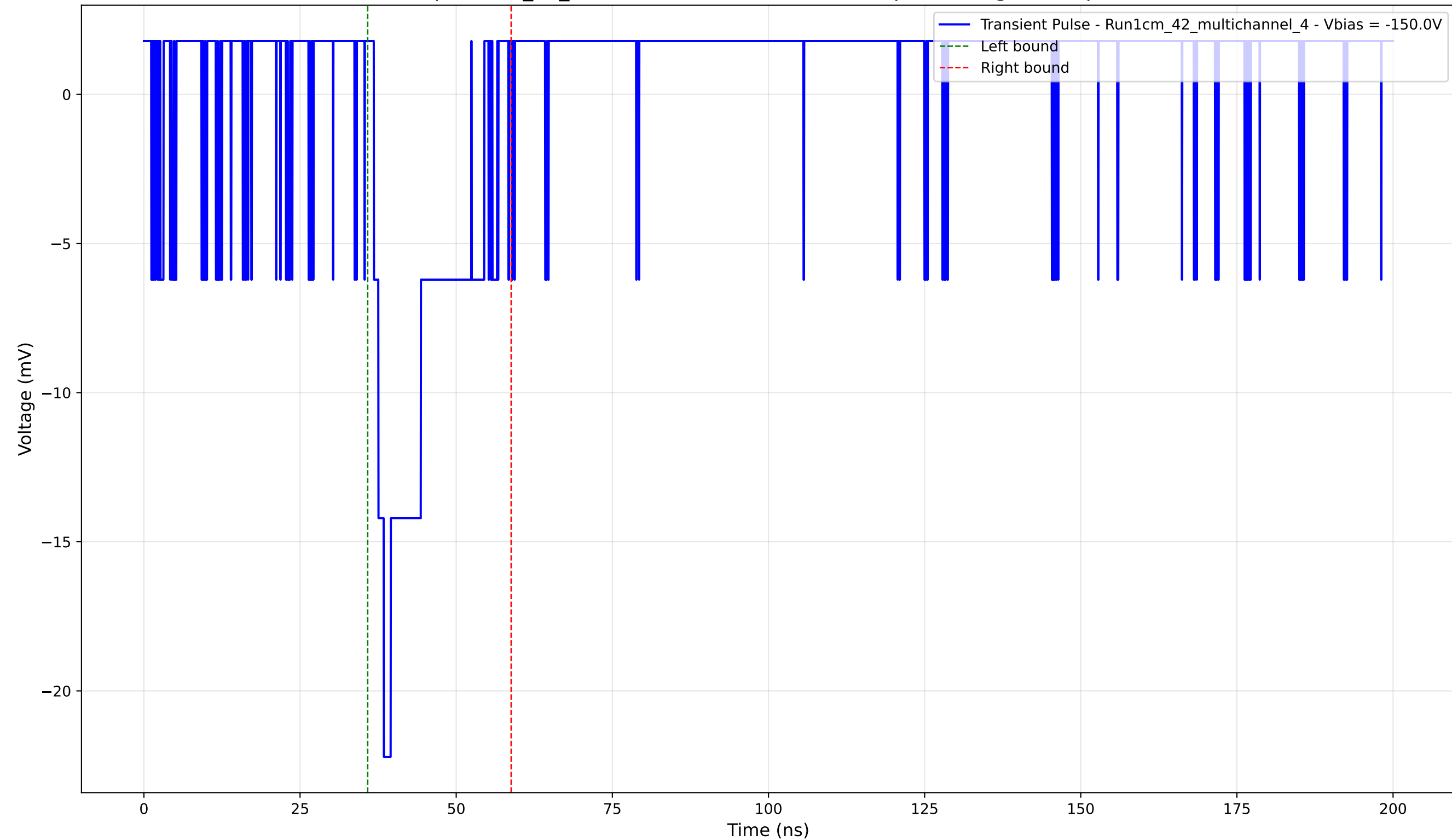
Transient Pulse - Sample: 1cm_42_multichannel - Position: 3680.0 \mu\text{m} - Charge: 3.47 pC - Rise Time: 1.60 ns
