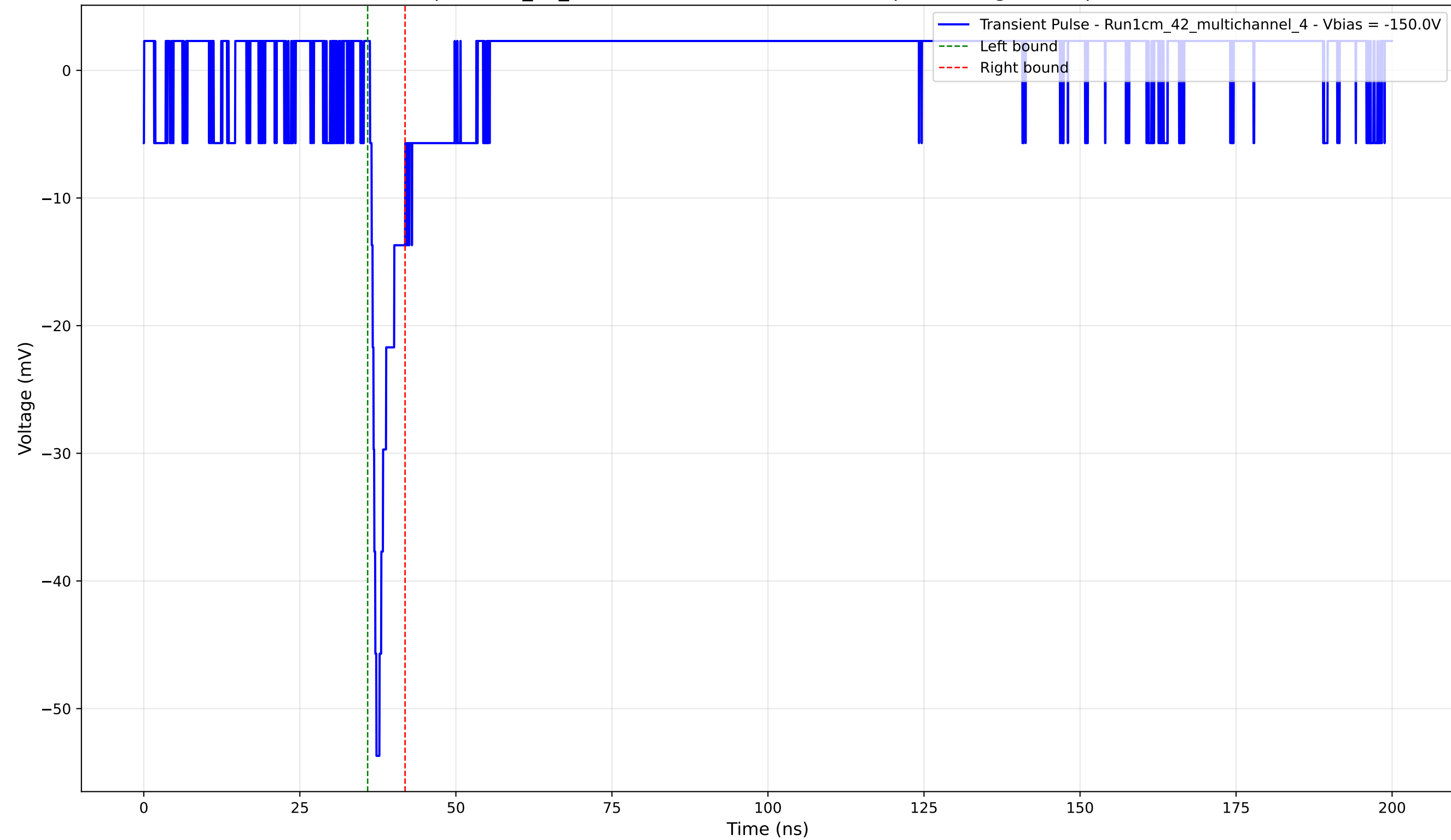
Transient Pulse - Sample: 1cm_42_multichannel - Position: 1975.0 \mu\text{m} - Charge: 2.82 pC - Rise Time: 1.02 ns
