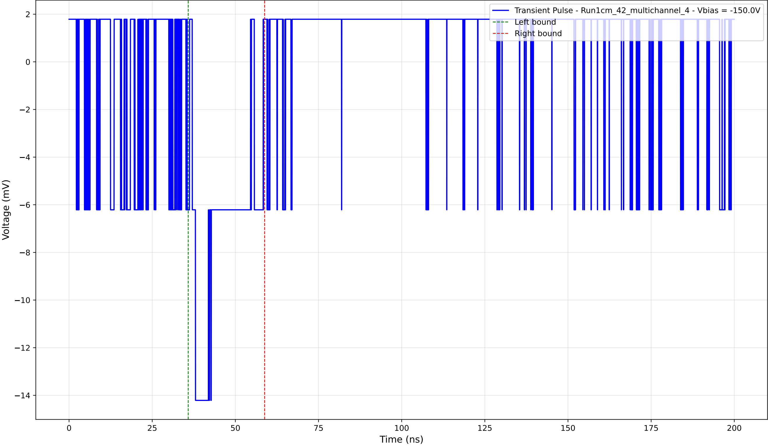
Transient Pulse - Sample: 1cm_42_multichannel - Position: 805.0 \mu\text{m} - Charge: 3.21 pC - Rise Time: 0.00 ns (N/A)
