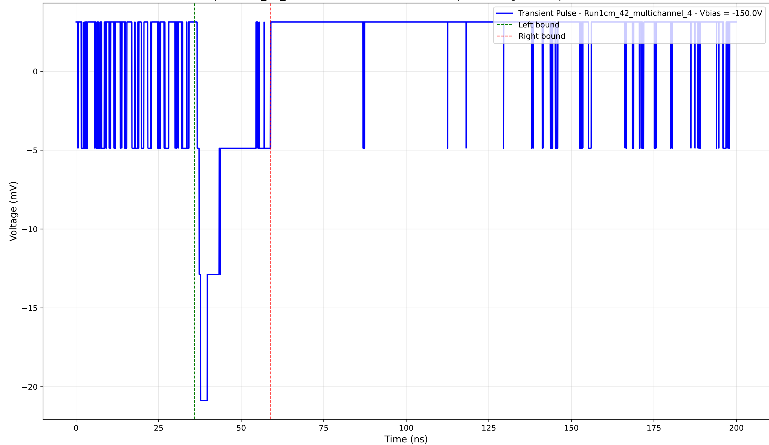
Transient Pulse - Sample: 1cm_42_multichannel - Position: 1180.0 \mu\text{m} - Charge: 3.33 pC - Rise Time: 0.00 ns (N/A)
