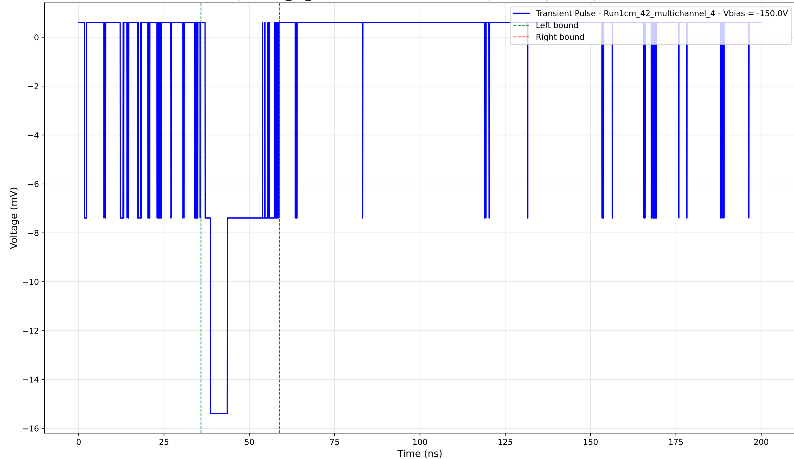
Transient Pulse - Sample: 1cm_42_multichannel - Position: 4710.0 \mu\text{m} - Charge: 3.80 pC - Rise Time: 1.56 ns
