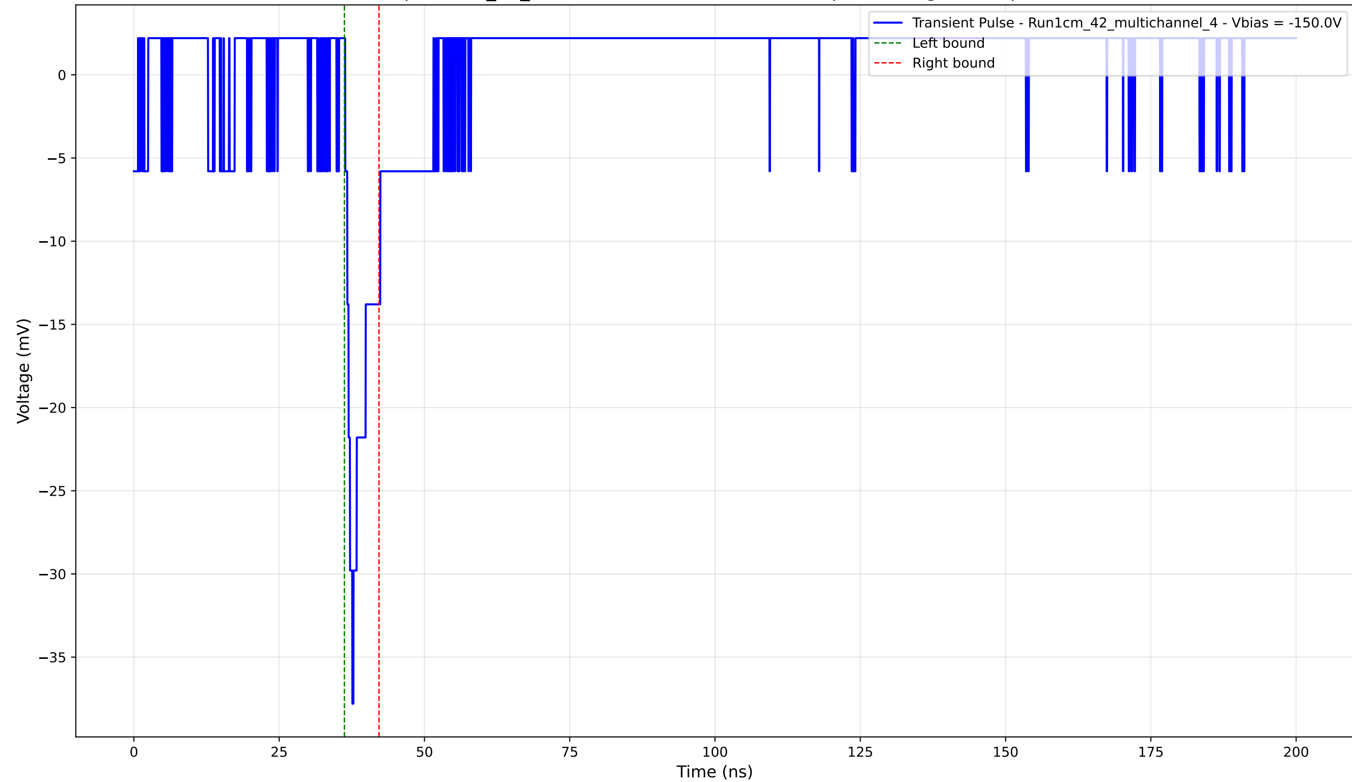
Transient Pulse - Sample: 1cm_42_multichannel - Position: 3040.0 \mu\text{m} - Charge: 2.23 pC - Rise Time: 1.23 ns
