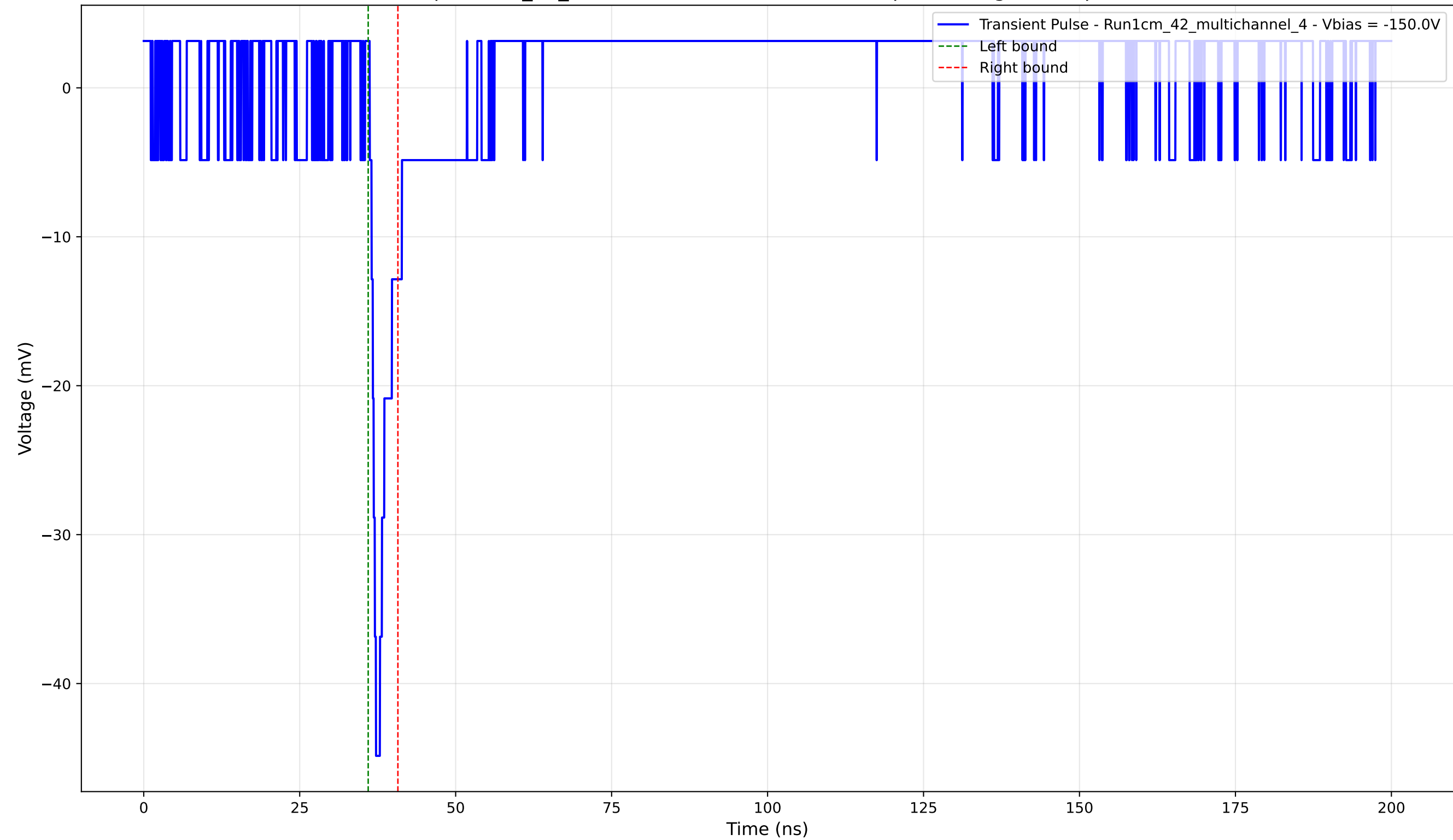
Transient Pulse - Sample: 1cm_42_multichannel - Position: 1950.0 \mu\text{m} - Charge: 2.15 pC - Rise Time: 1.00 ns
