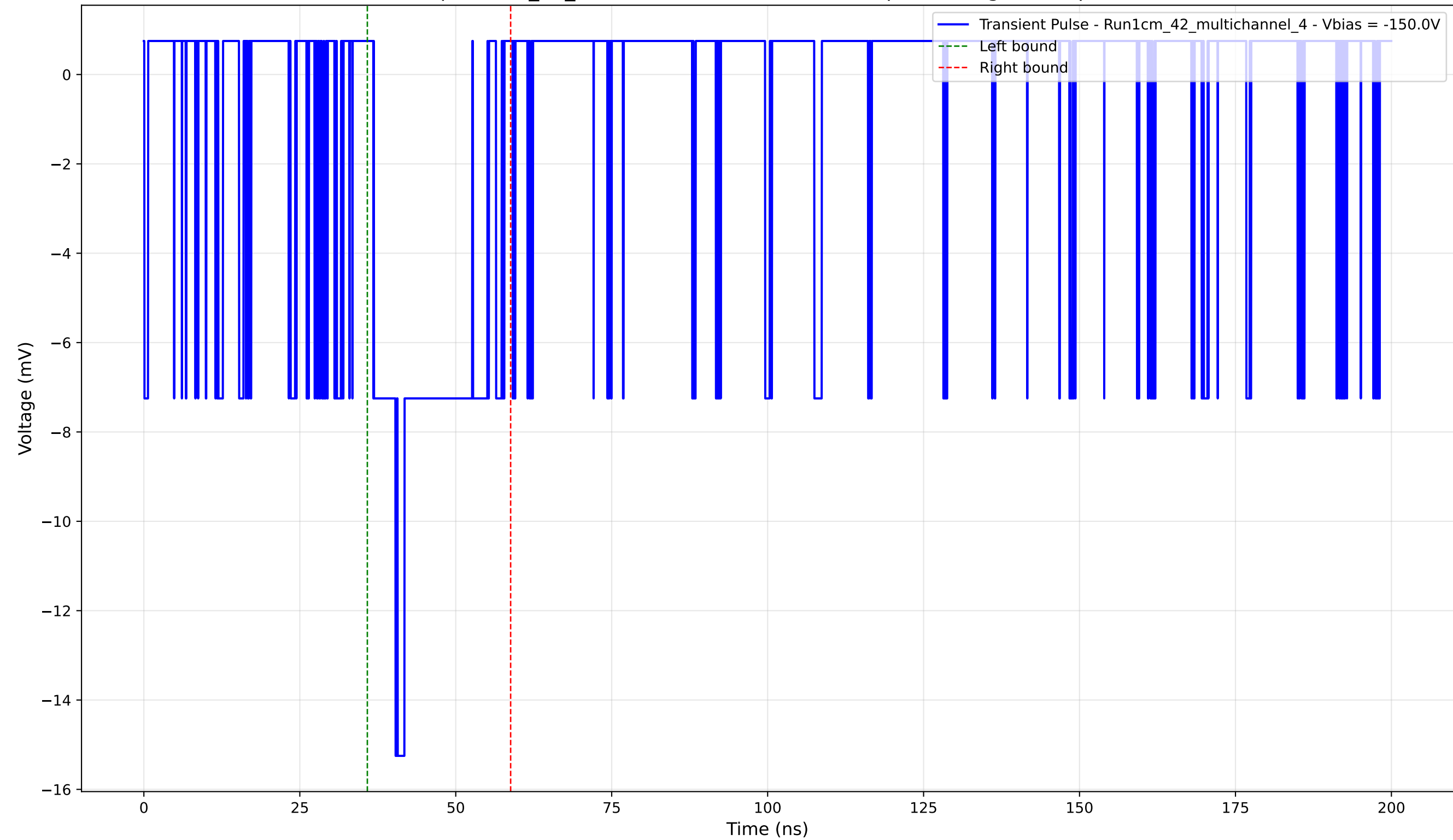
Transient Pulse - Sample: 1cm_42_multichannel - Position: 115.0 \mu\text{m} - Charge: 2.99 pC - Rise Time: 3.48 ns
