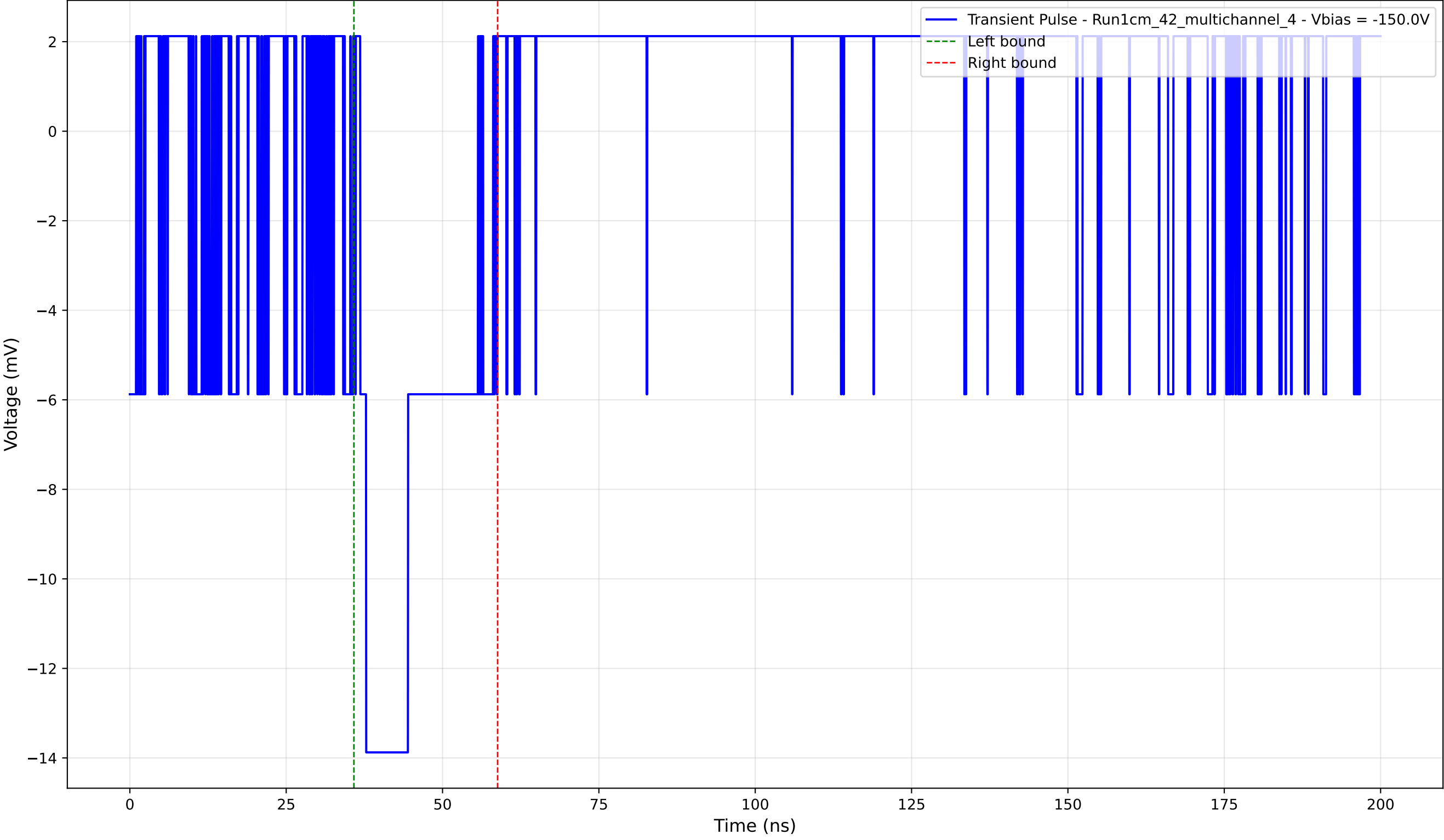
Transient Pulse - Sample: 1cm_42_multichannel - Position: 770.0 \mu\text{m} - Charge: 3.49 pC - Rise Time: 0.00 ns (N/A)
