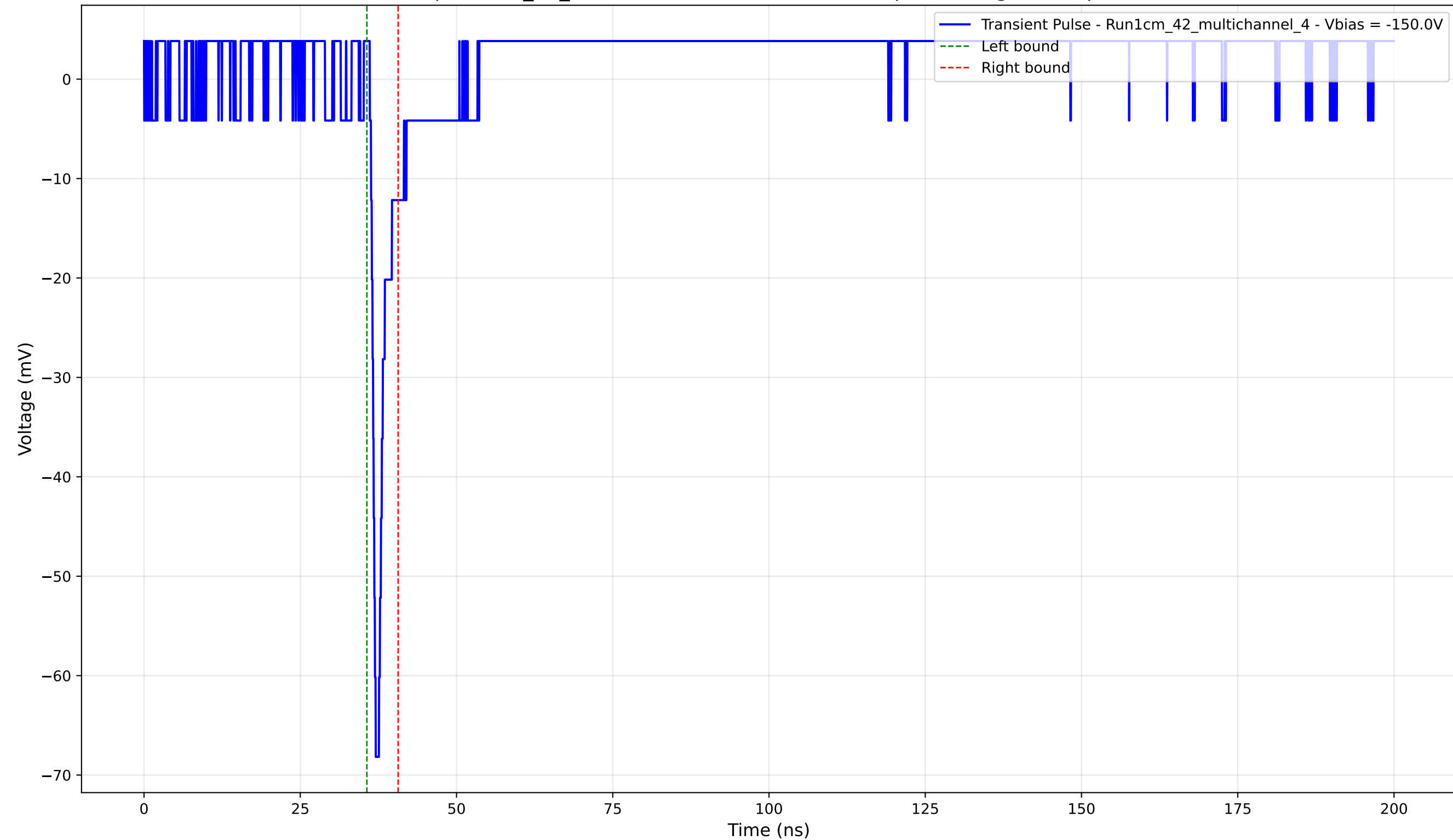
Transient Pulse - Sample: 1cm_42_multichannel - Position: 2200.0 \mu\text{m} - Charge: 2.71 pC - Rise Time: 0.75 ns
