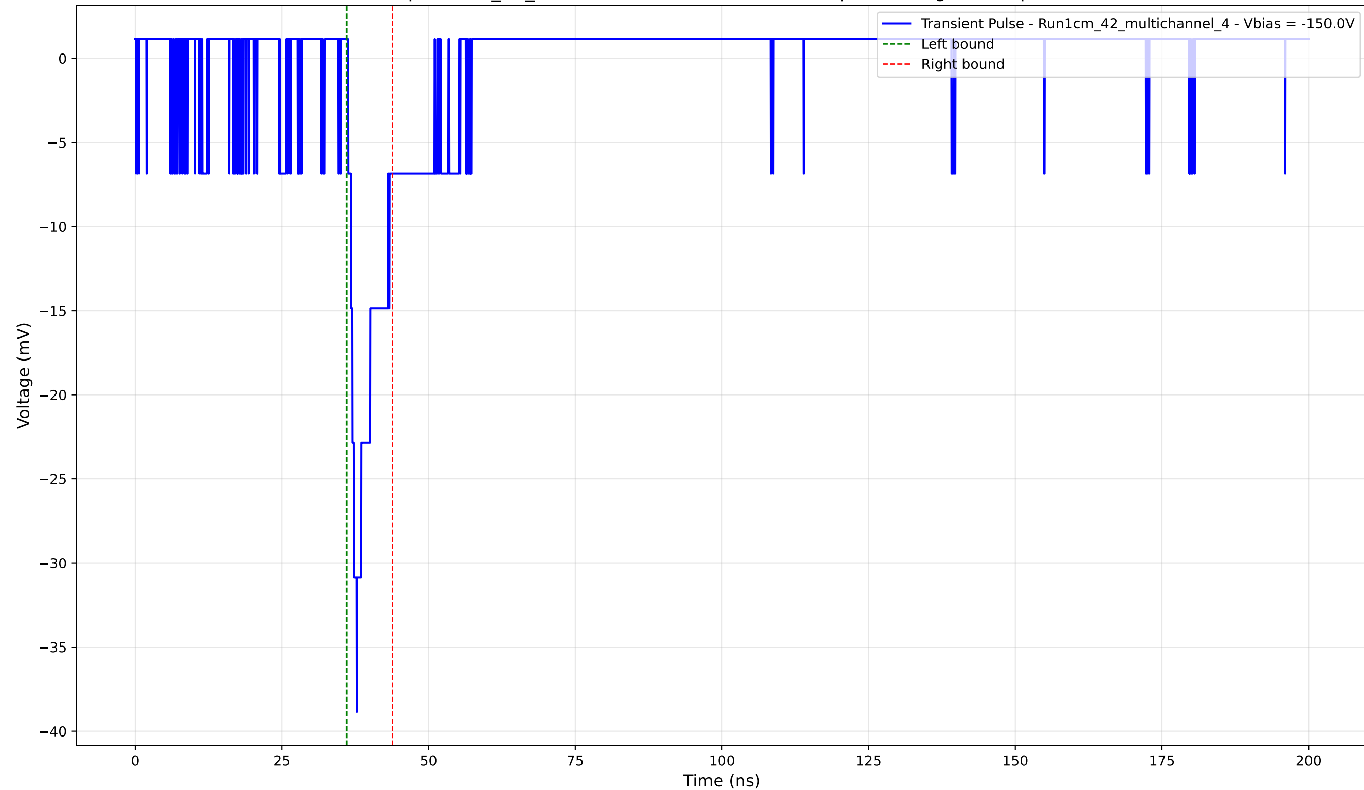
Transient Pulse - Sample: 1cm_42_multichannel - Position: 1650.0 \mu\text{m} - Charge: 2.78 pC - Rise Time: 1.49 ns
