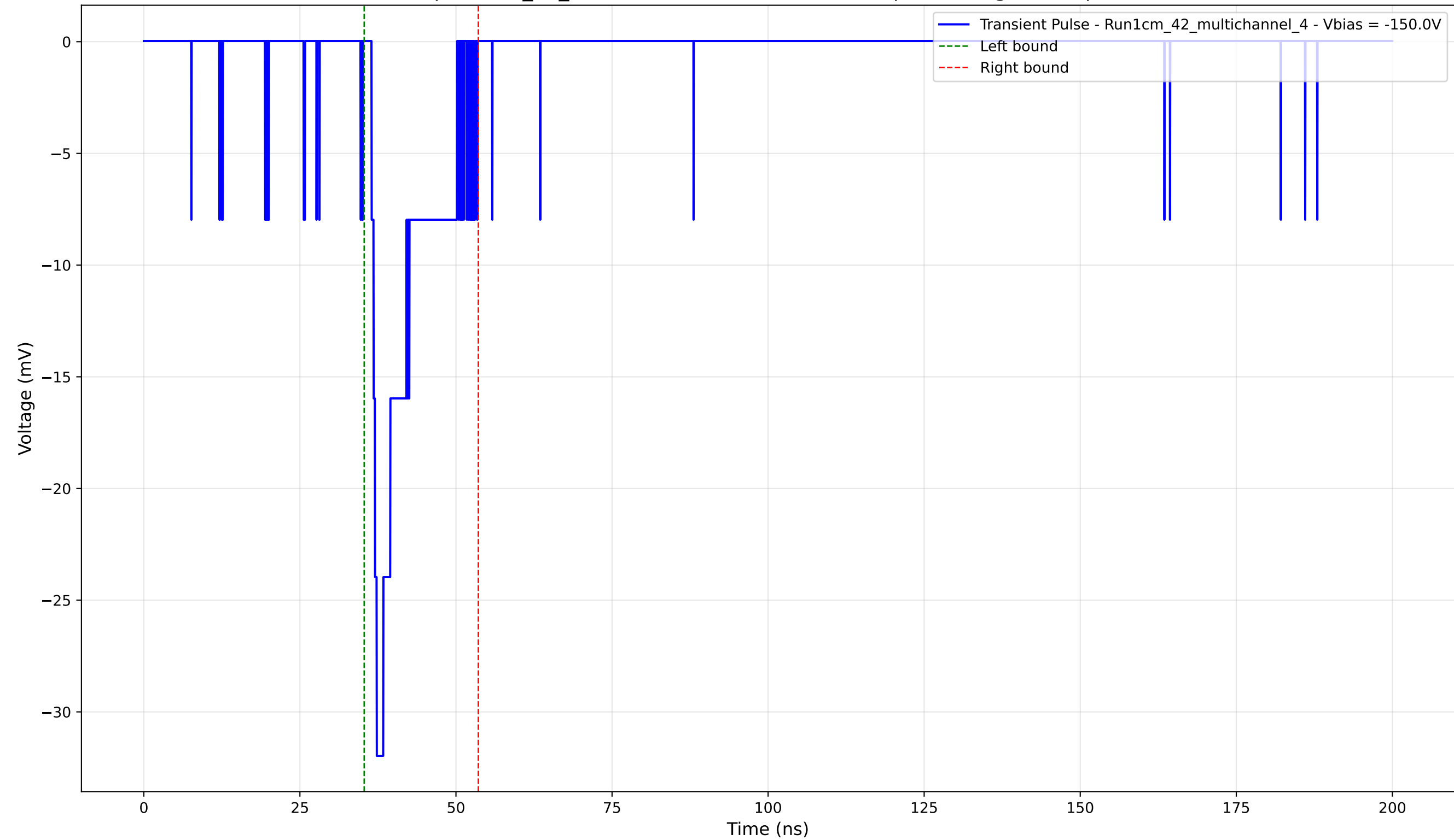
Transient Pulse - Sample: 1cm_42_multichannel - Position: 3085.0 \mu\text{m} - Charge: 3.79 pC - Rise Time: 0.83 ns
