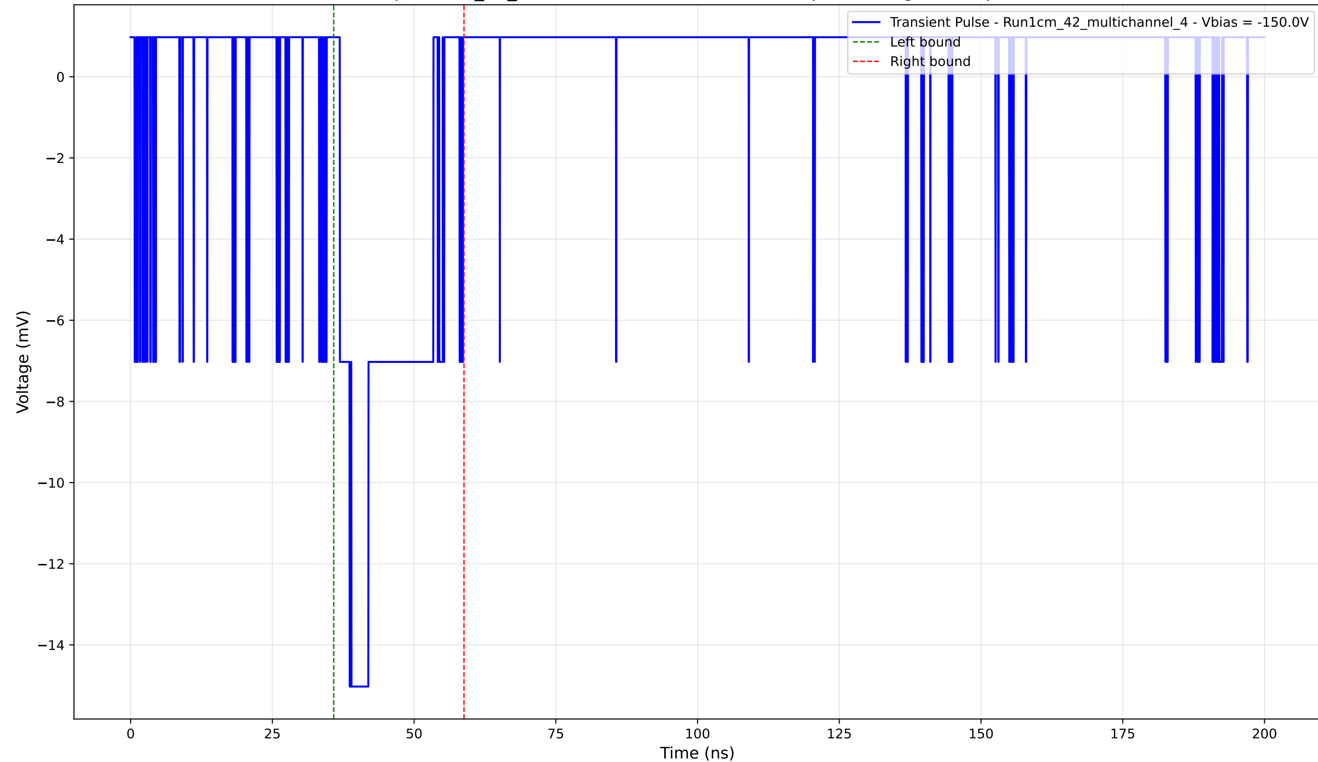
Transient Pulse - Sample: 1cm_42_multichannel - Position: 4765.0 \mu\text{m} - Charge: 2.95 pC - Rise Time: 1.74 ns
