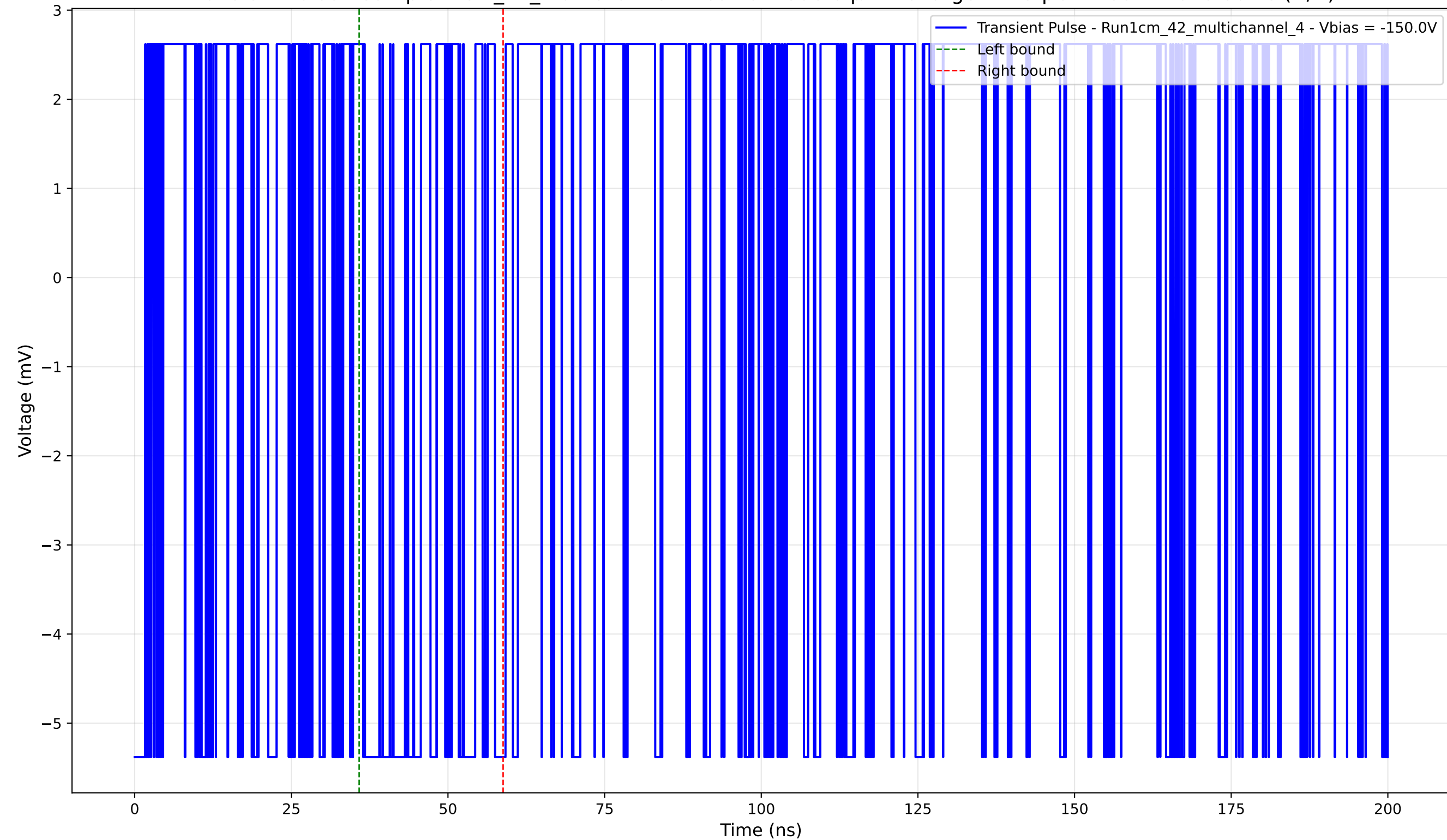
Transient Pulse - Sample: 1cm_42_multichannel - Position: 390.0 \mu\text{m} - Charge: 1.13 pC - Rise Time: 0.00 ns (N/A)
