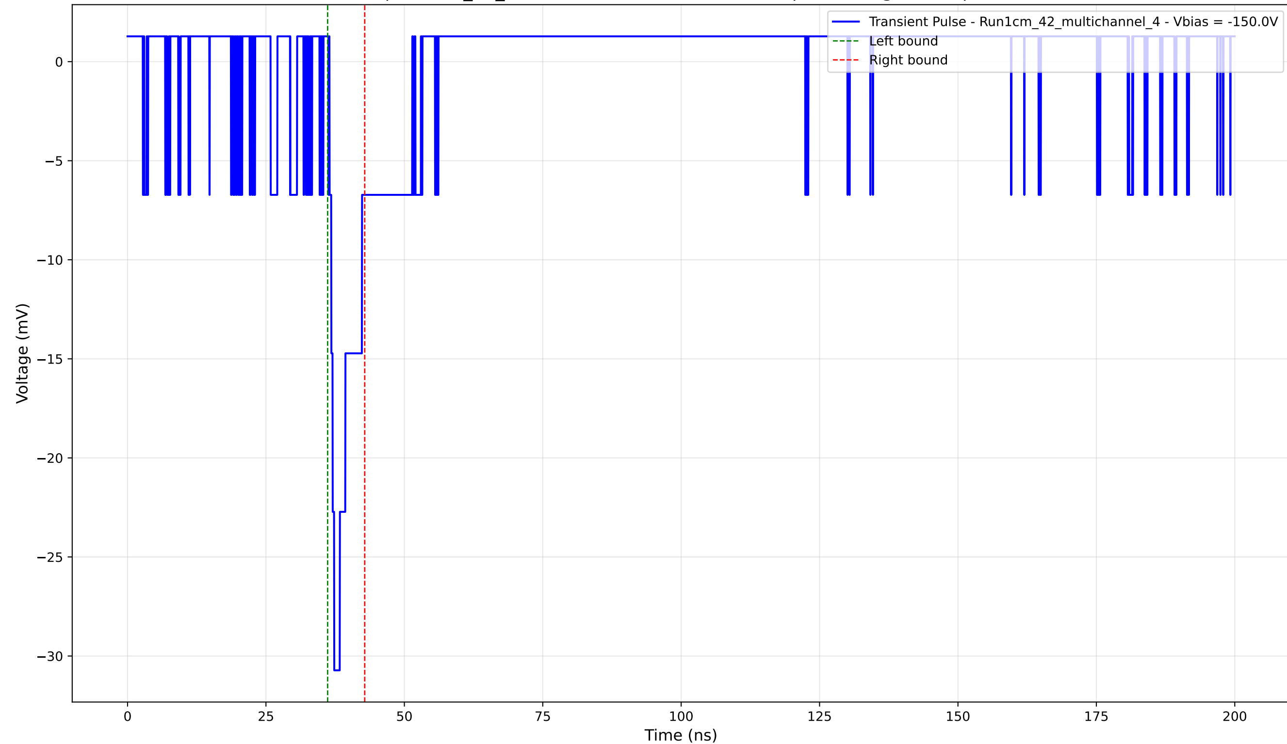
Transient Pulse - Sample: 1cm_42_multichannel - Position: 3110.0 \mu\text{m} - Charge: 2.28 pC - Rise Time: 0.85 ns
