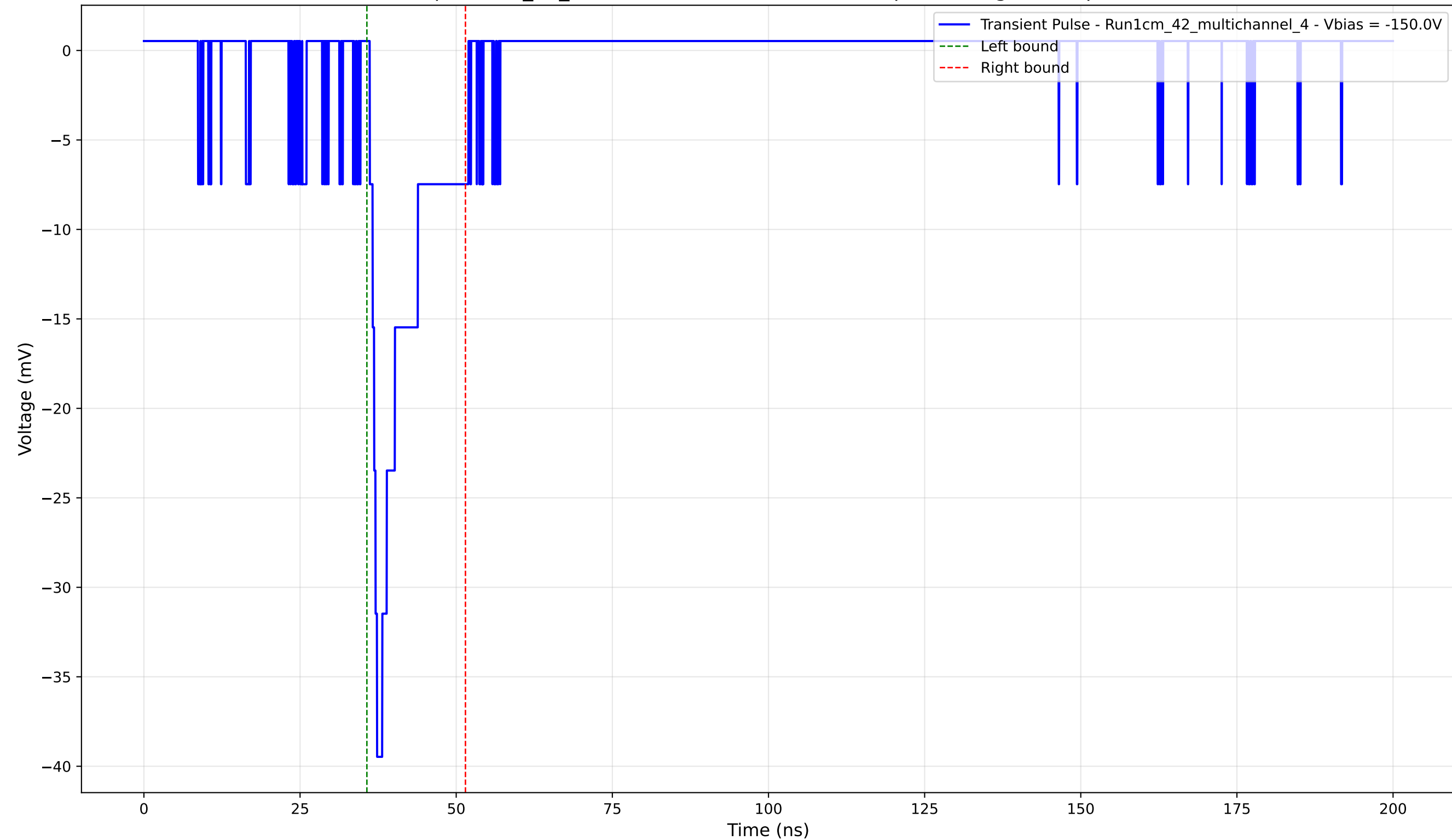
Transient Pulse - Sample: 1cm_42_multichannel - Position: 1730.0 \mu\text{m} - Charge: 4.40 pC - Rise Time: 1.17 ns
