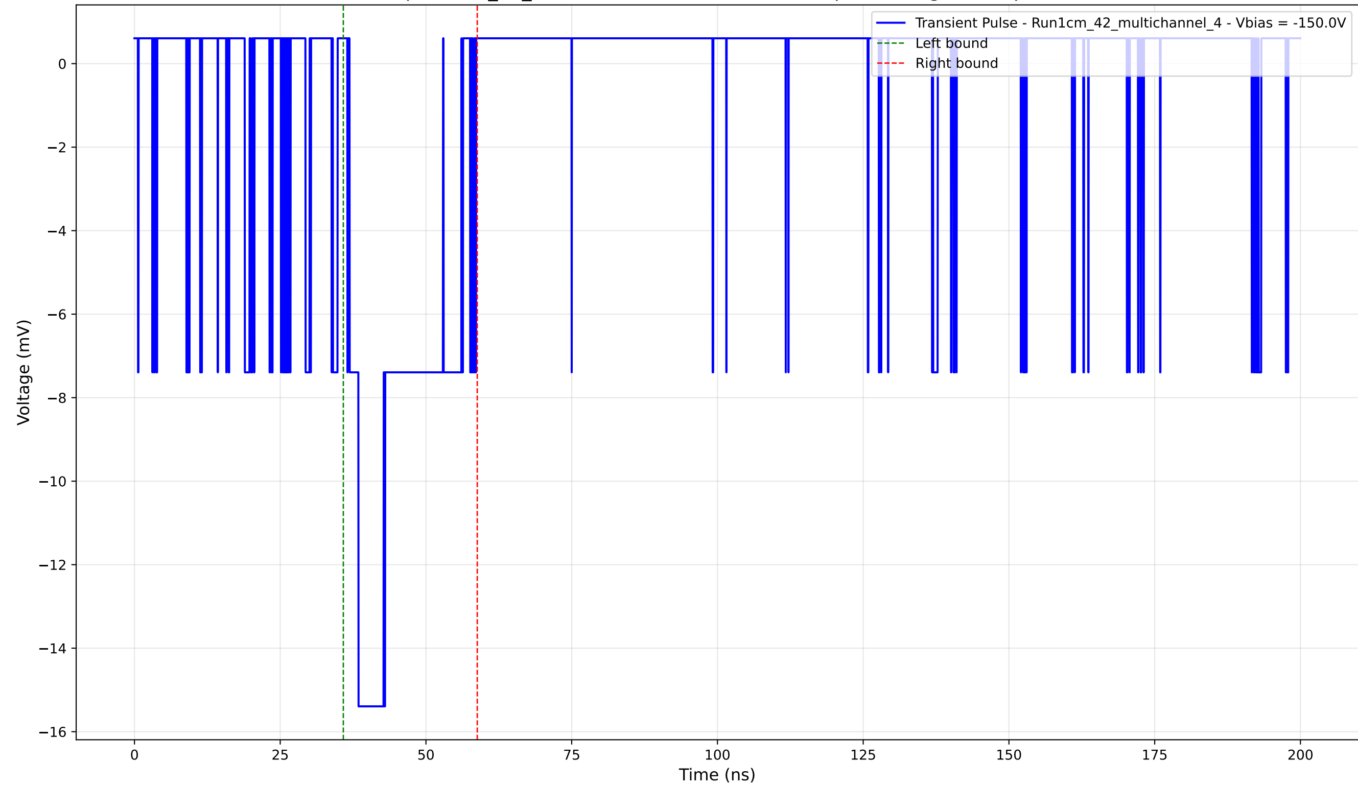
Transient Pulse - Sample: 1cm_42_multichannel - Position: 4270.0 \mu\text{m} - Charge: 3.63 pC - Rise Time: 1.54 ns
