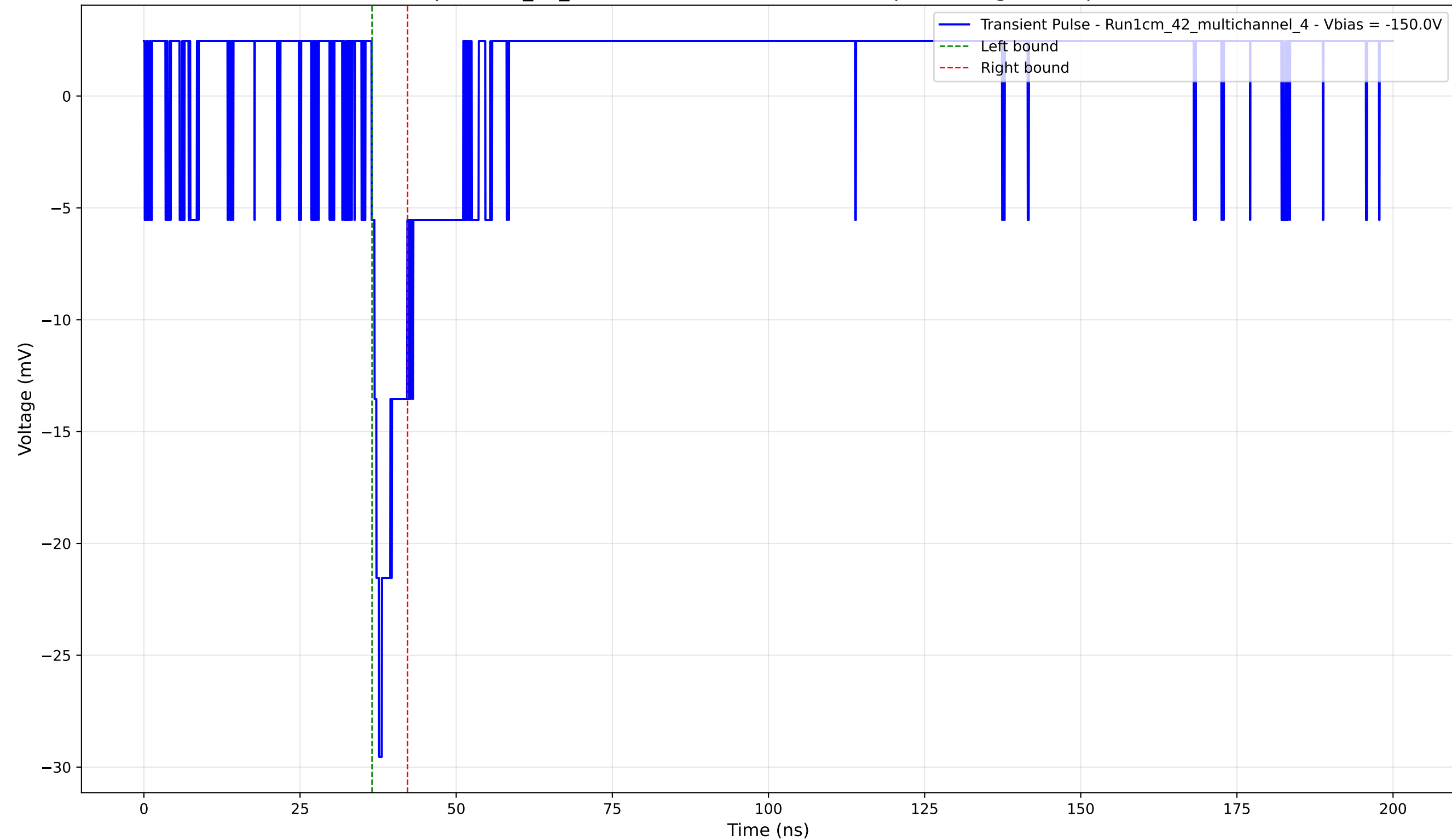
Transient Pulse - Sample: 1cm_42_multichannel - Position: 3235.0 \mu\text{m} - Charge: 1.93 pC - Rise Time: 1.20 ns
