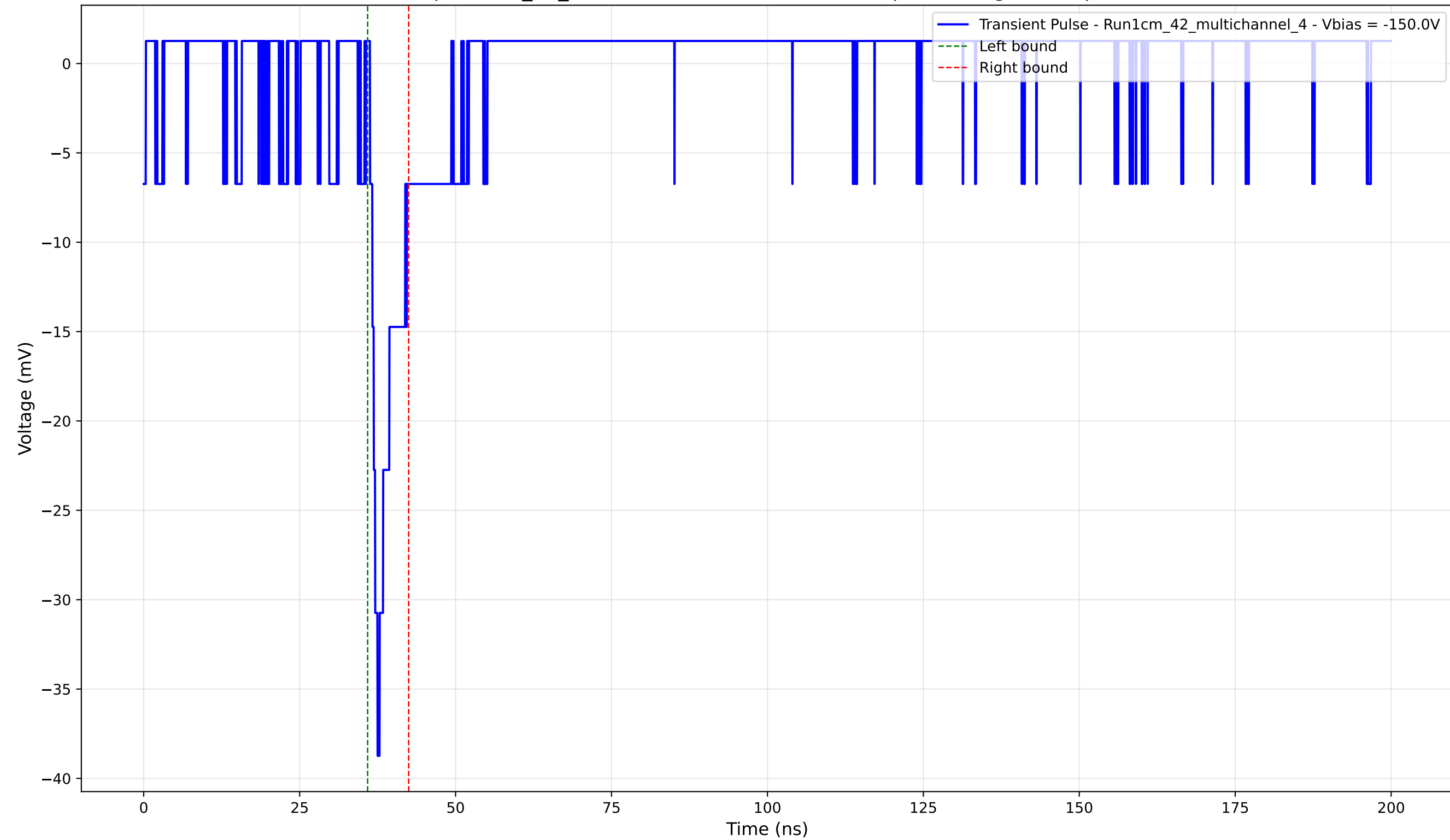
Transient Pulse - Sample: 1cm_42_multichannel - Position: 2965.0 \mu\text{m} - Charge: 2.34 pC - Rise Time: 1.21 ns
