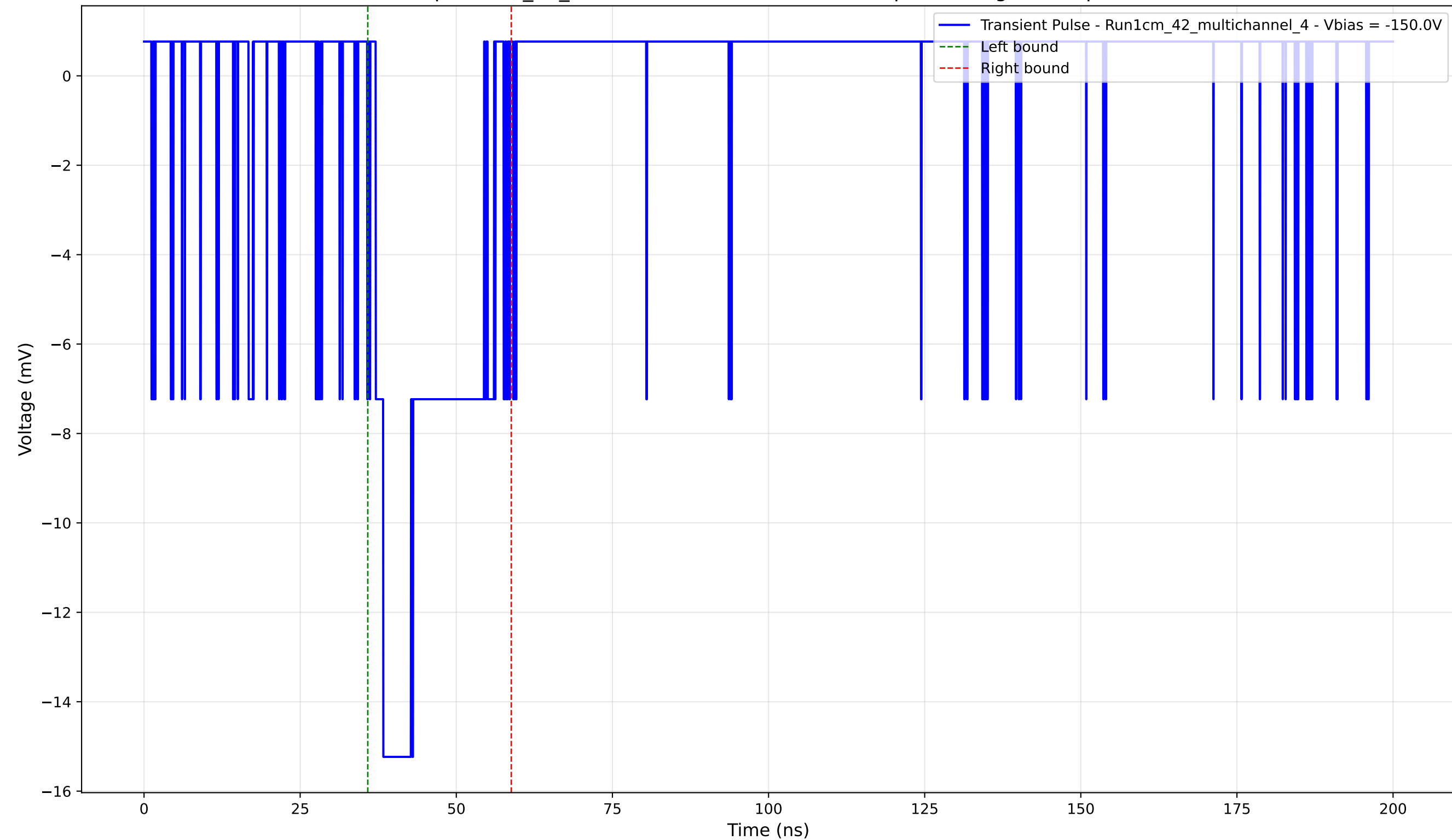
Transient Pulse - Sample: 1cm_42_multichannel - Position: 4630.0 \mu\text{m} - Charge: 3.48 pC - Rise Time: 1.22 ns
