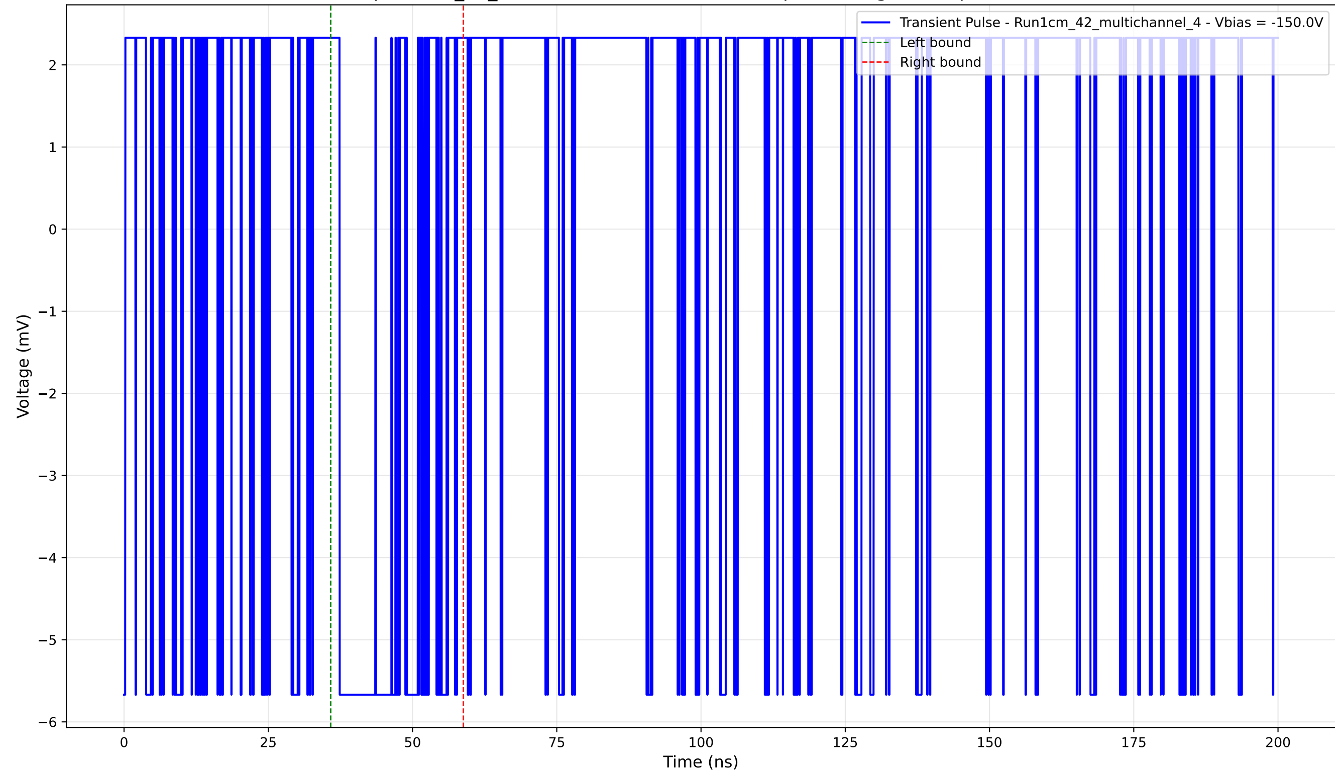
Transient Pulse - Sample: 1cm_42_multichannel - Position: 405.0 \mu\text{m} - Charge: 1.35 pC - Rise Time: 0.00 ns (N/A)
