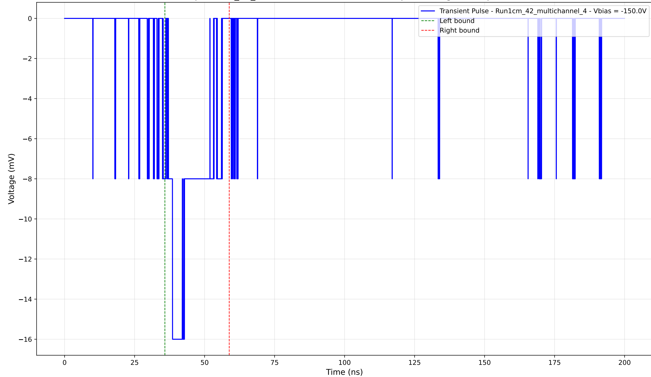
Transient Pulse - Sample: 1cm_42_multichannel - Position: 4770.0 \mu\text{m} - Charge: 3.61 pC - Rise Time: 1.46 ns
