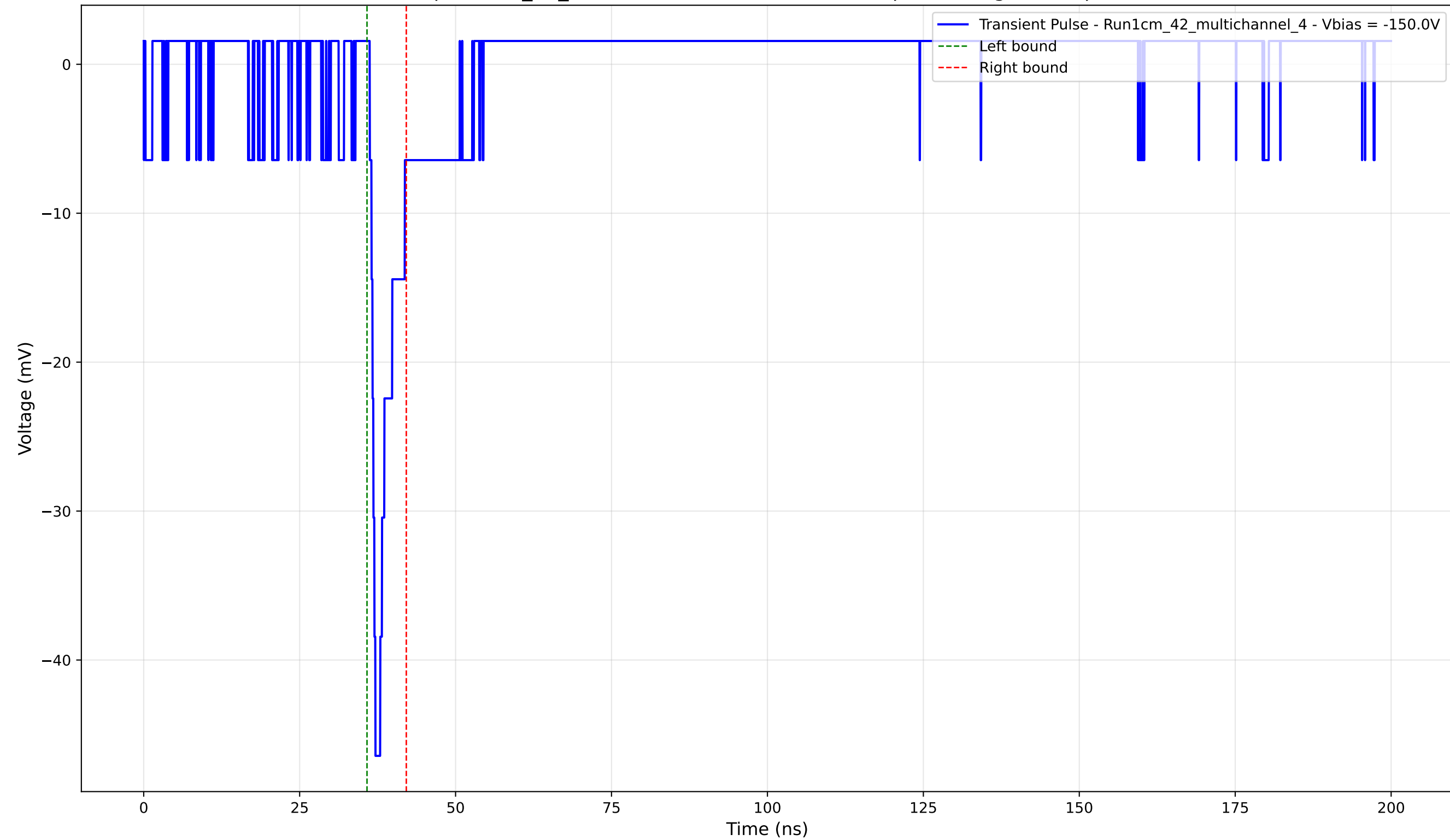
Transient Pulse - Sample: 1cm_42_multichannel - Position: 2805.0 \mu\text{m} - Charge: 2.70 pC - Rise Time: 0.91 ns
