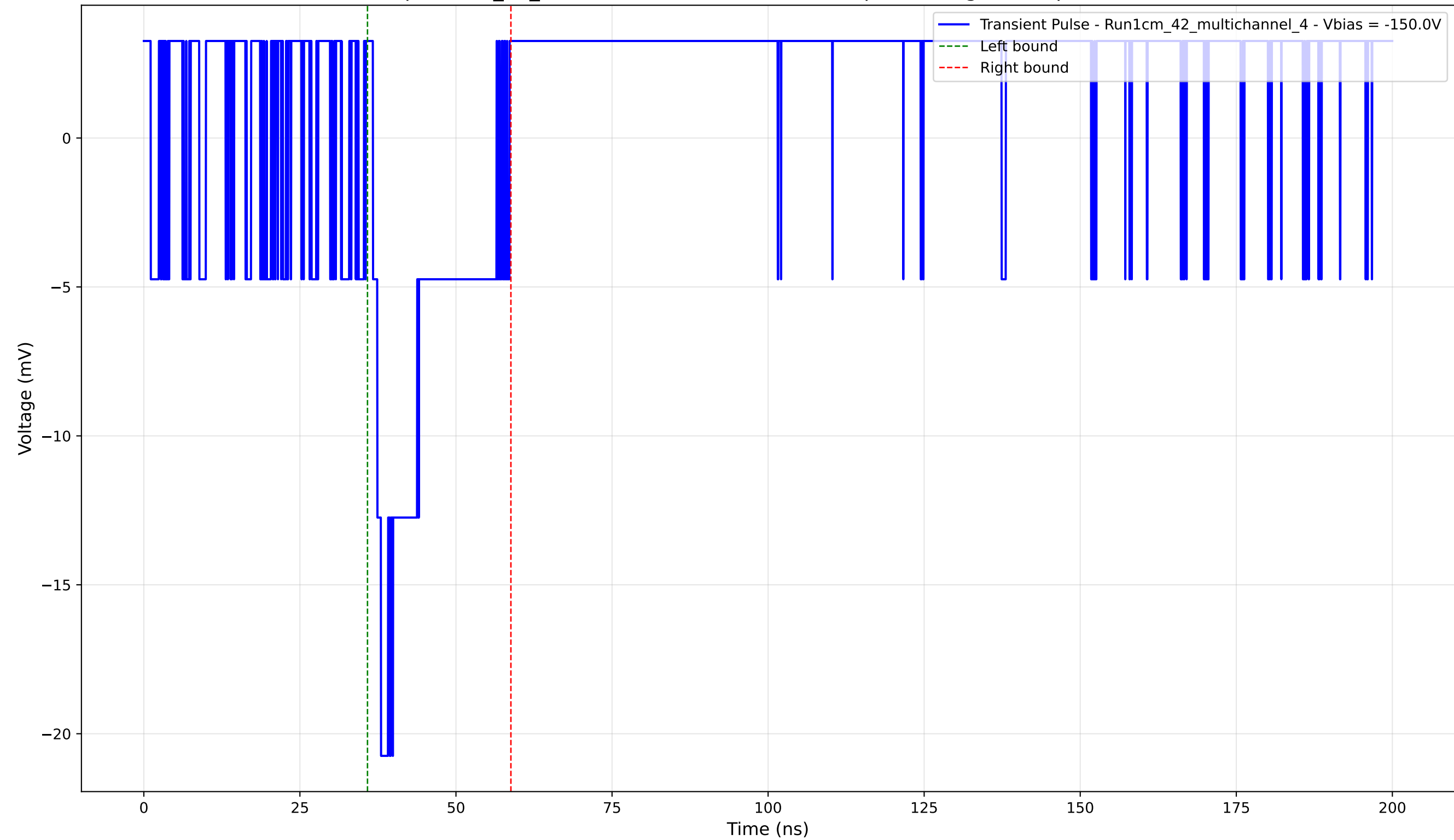
Transient Pulse - Sample: 1cm_42_multichannel - Position: 1080.0 \mu\text{m} - Charge: 3.15 pC - Rise Time: 0.00 ns (N/A)
