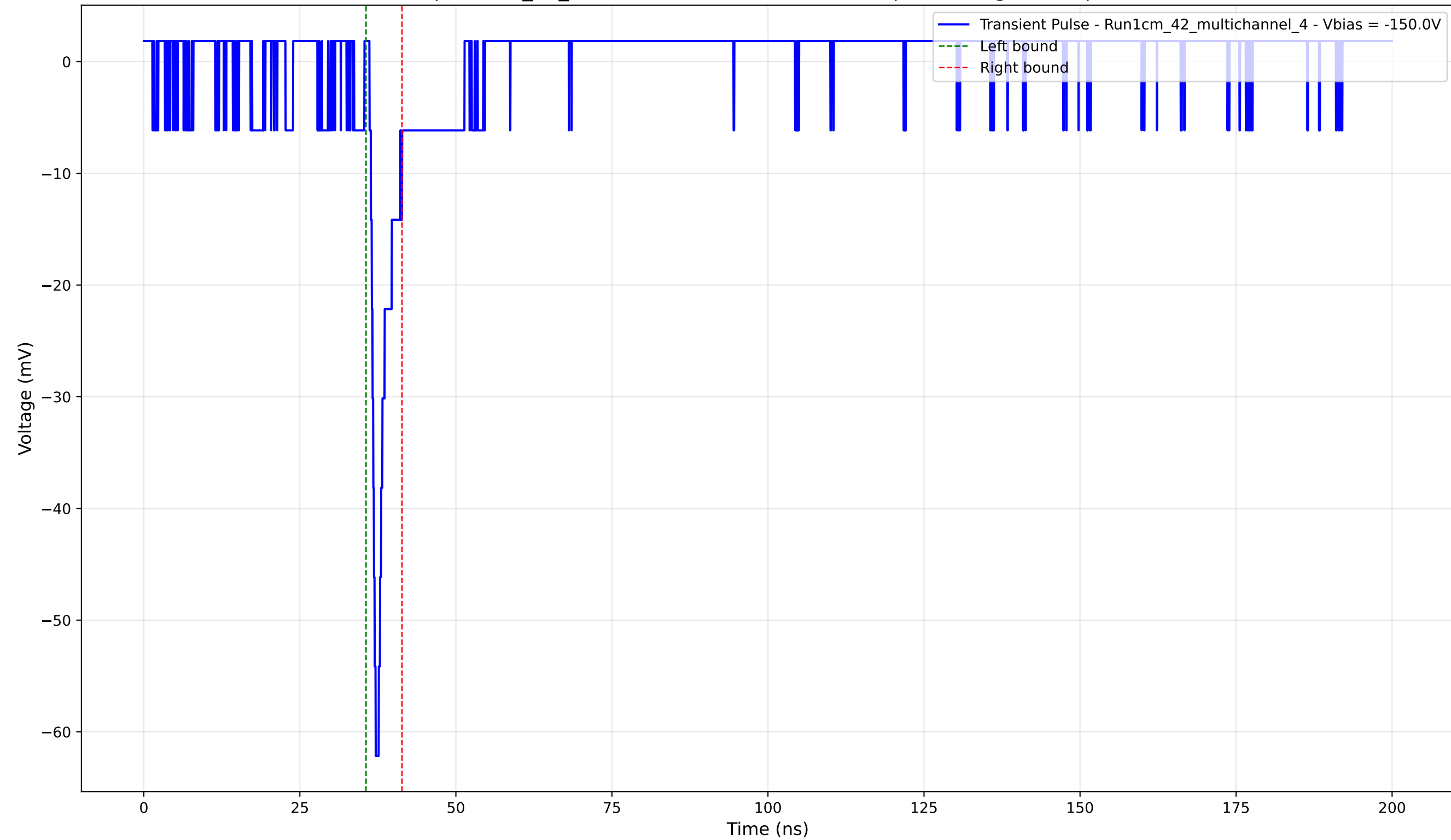
Transient Pulse - Sample: 1cm_42_multichannel - Position: 2140.0 \mu\text{m} - Charge: 2.87 pC - Rise Time: 0.78 ns
