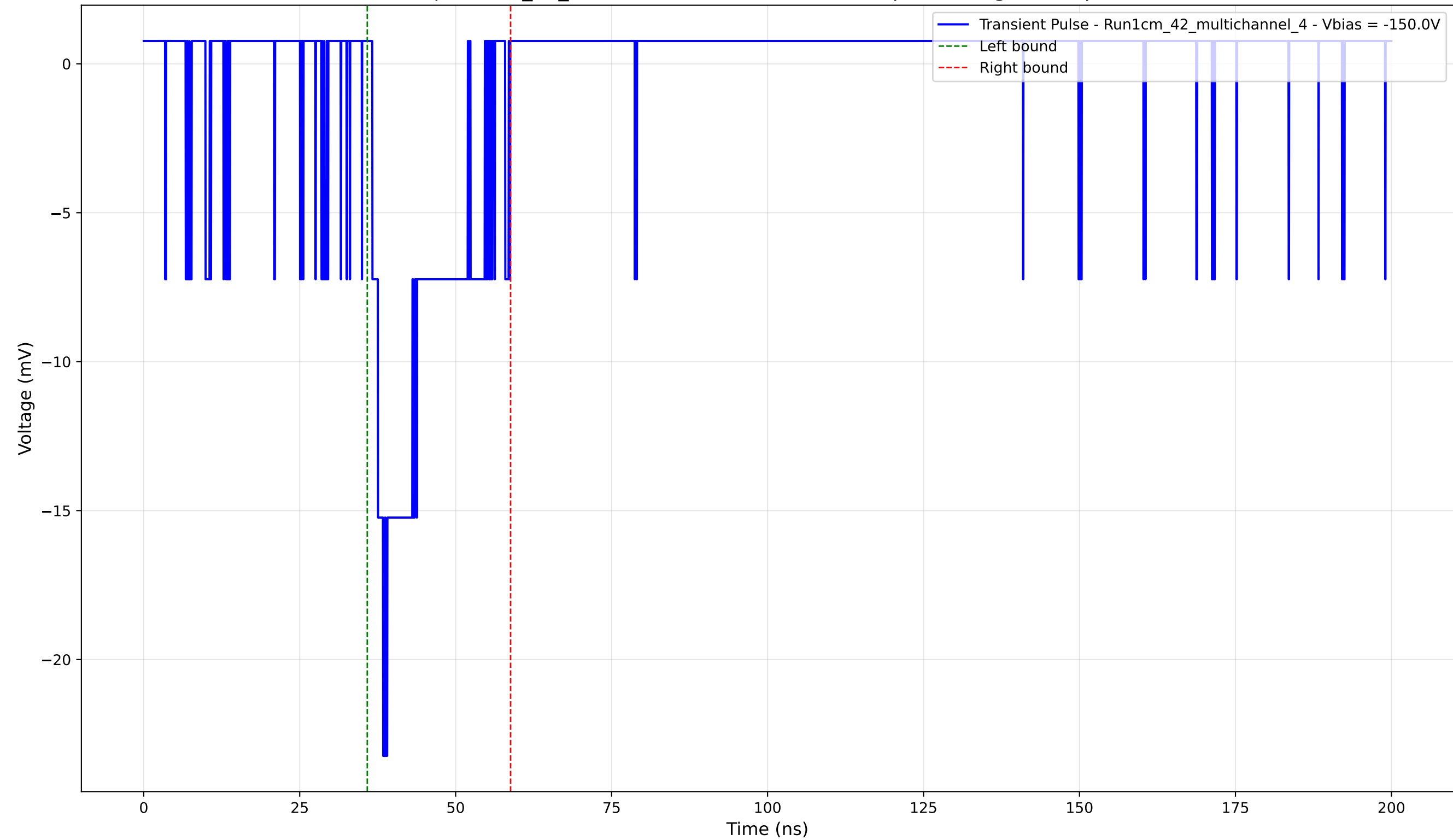
Transient Pulse - Sample: 1cm_42_multichannel - Position: 3670.0 \mu\text{m} - Charge: 3.74 pC - Rise Time: 1.74 ns
