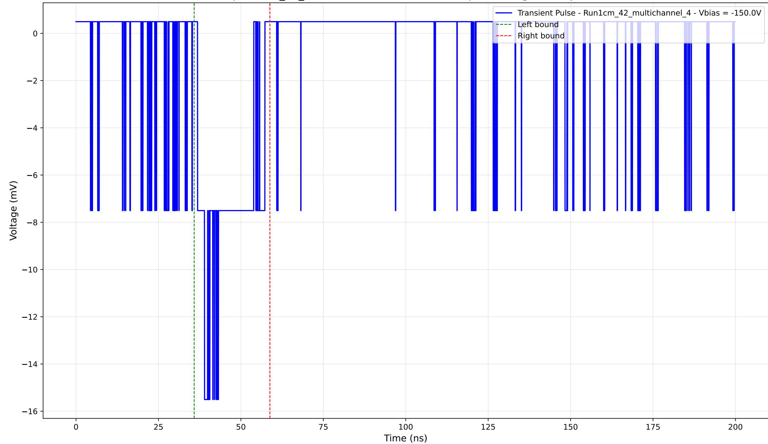
Transient Pulse - Sample: 1cm_42_multichannel - Position: 130.0 \mu\text{m} - Charge: 3.20 pC - Rise Time: 2.12 ns
