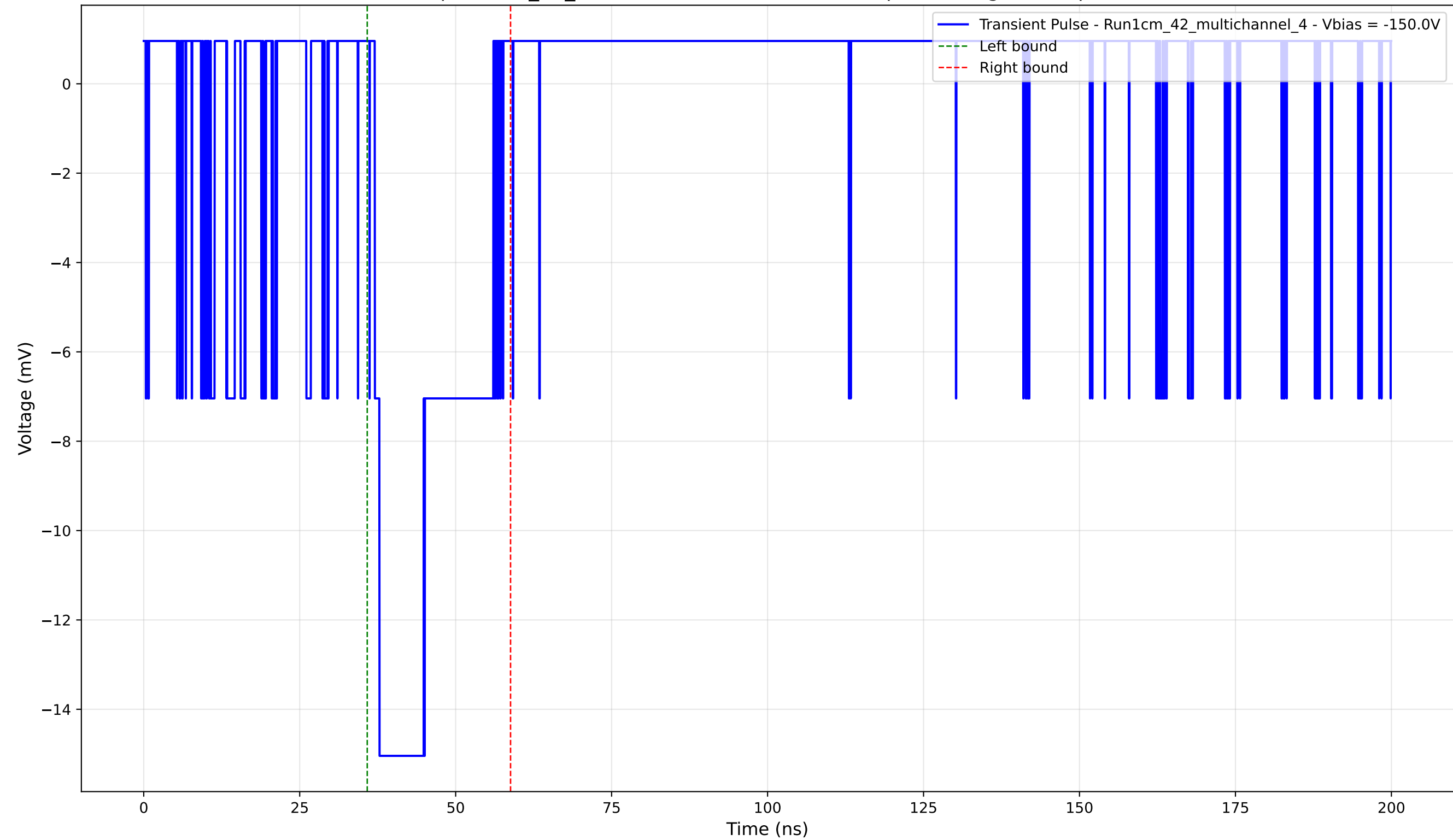
Transient Pulse - Sample: 1cm_42_multichannel - Position: 710.0 \mu\text{m} - Charge: 3.84 pC - Rise Time: 0.76 ns
