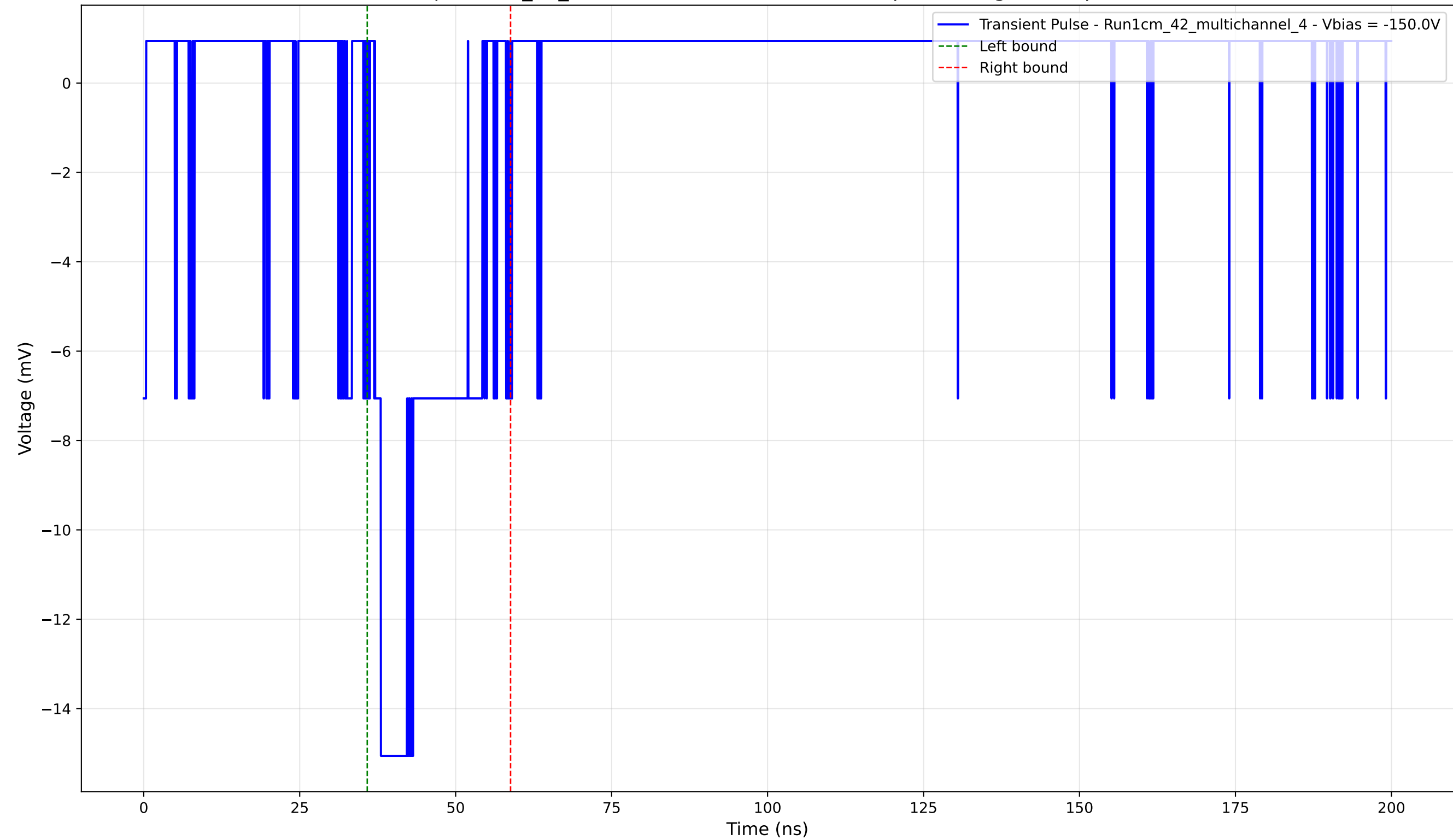
Transient Pulse - Sample: 1cm_42_multichannel - Position: 4085.0 \mu\text{m} - Charge: 3.27 pC - Rise Time: 0.94 ns
