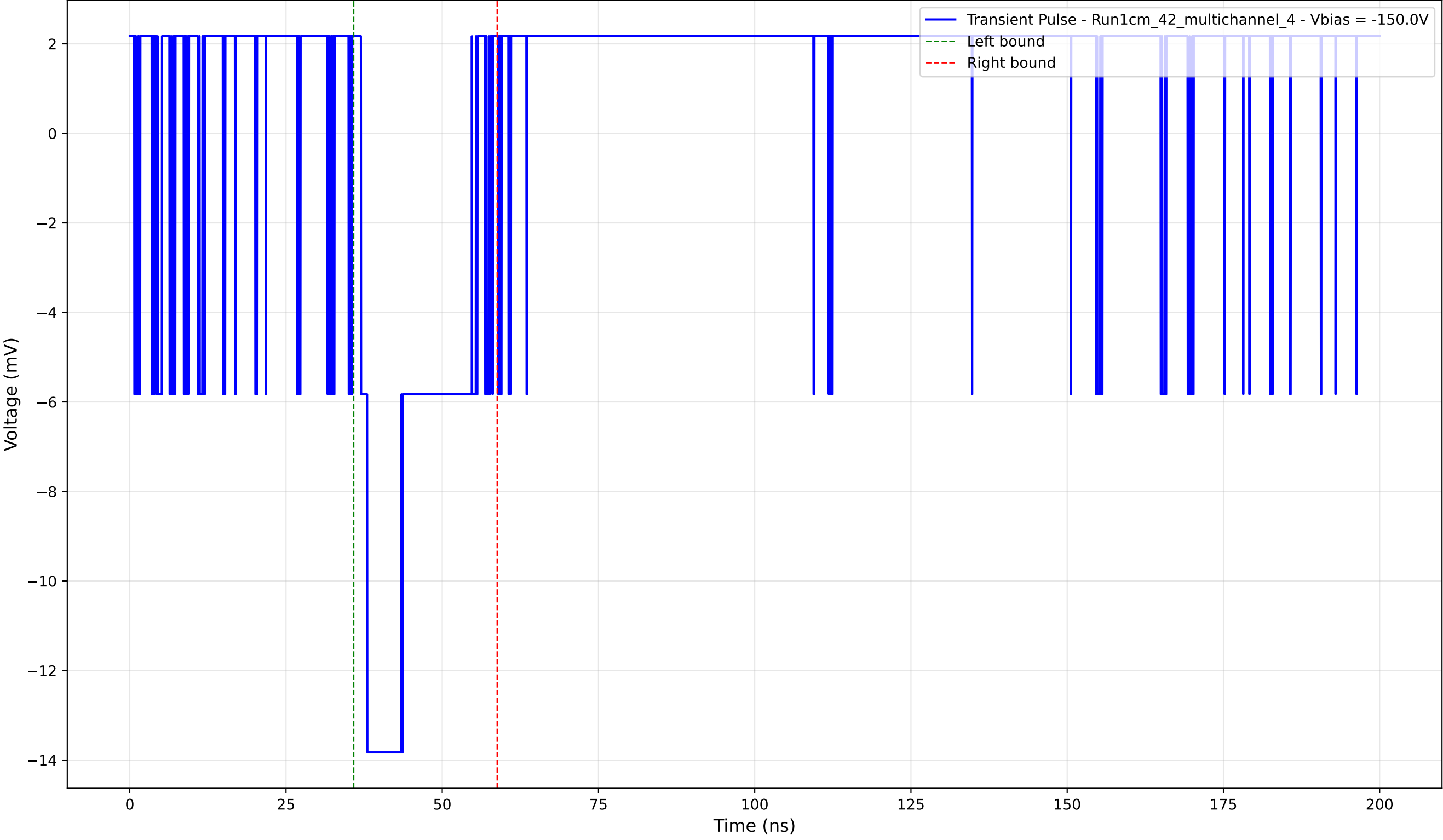
Transient Pulse - Sample: 1cm_42_multichannel - Position: 470.0 \mu\text{m} - Charge: 2.99 pC - Rise Time: 0.00 ns (N/A)
