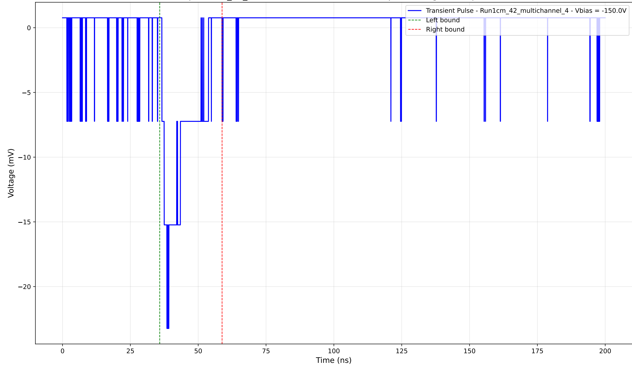
Transient Pulse - Sample: 1cm_42_multichannel - Position: 3615.0 \mu\text{m} - Charge: 3.40 pC - Rise Time: 1.86 ns
