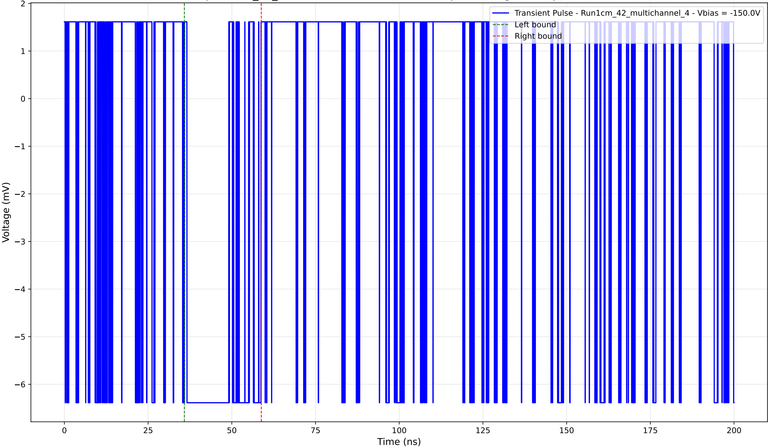
Transient Pulse - Sample: 1cm_42_multichannel - Position: 1335.0 \mu\text{m} - Charge: 2.32 pC - Rise Time: 0.00 ns (N/A)
