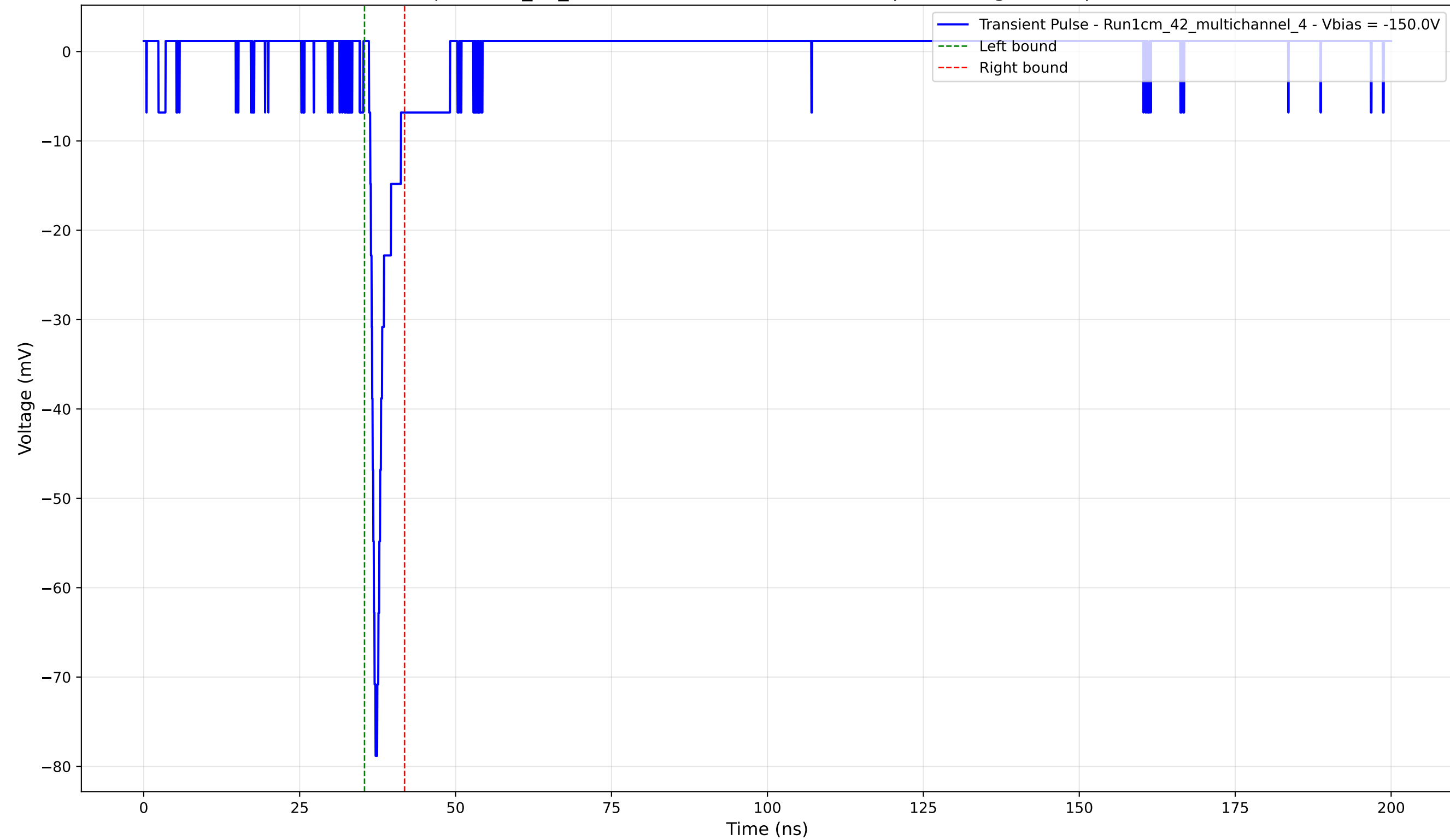
Transient Pulse - Sample: 1cm_42_multichannel - Position: 2225.0 \mu\text{m} - Charge: 3.31 pC - Rise Time: 0.86 ns
