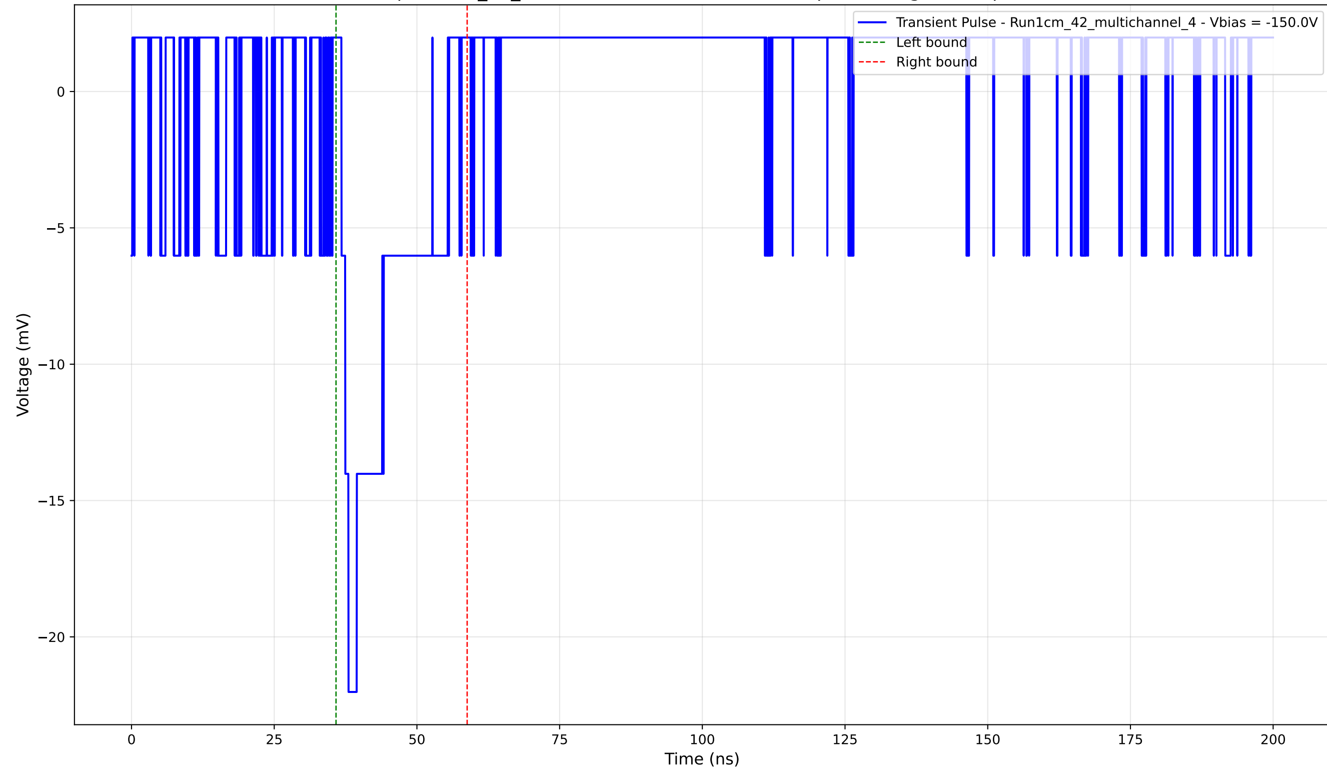
Transient Pulse - Sample: 1cm_42_multichannel - Position: 1100.0 \mu\text{m} - Charge: 3.39 pC - Rise Time: 1.24 ns
