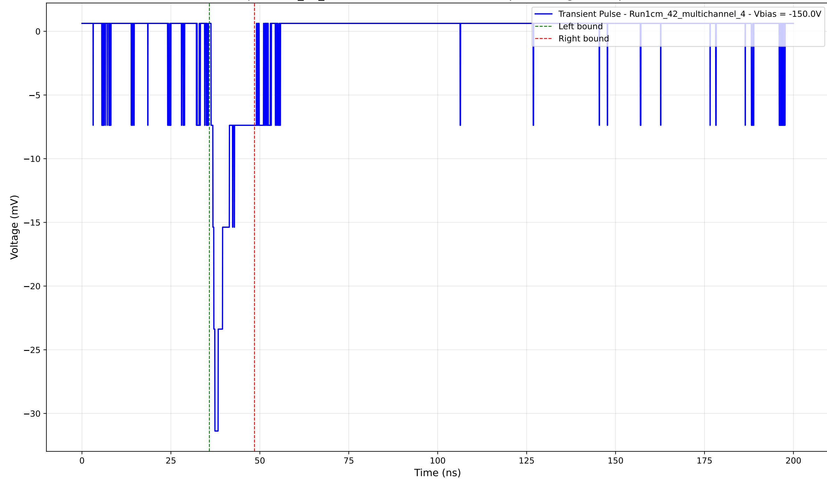
Transient Pulse - Sample: 1cm_42_multichannel - Position: 3095.0 \mu\text{m} - Charge: 3.11 pC - Rise Time: 1.09 ns
