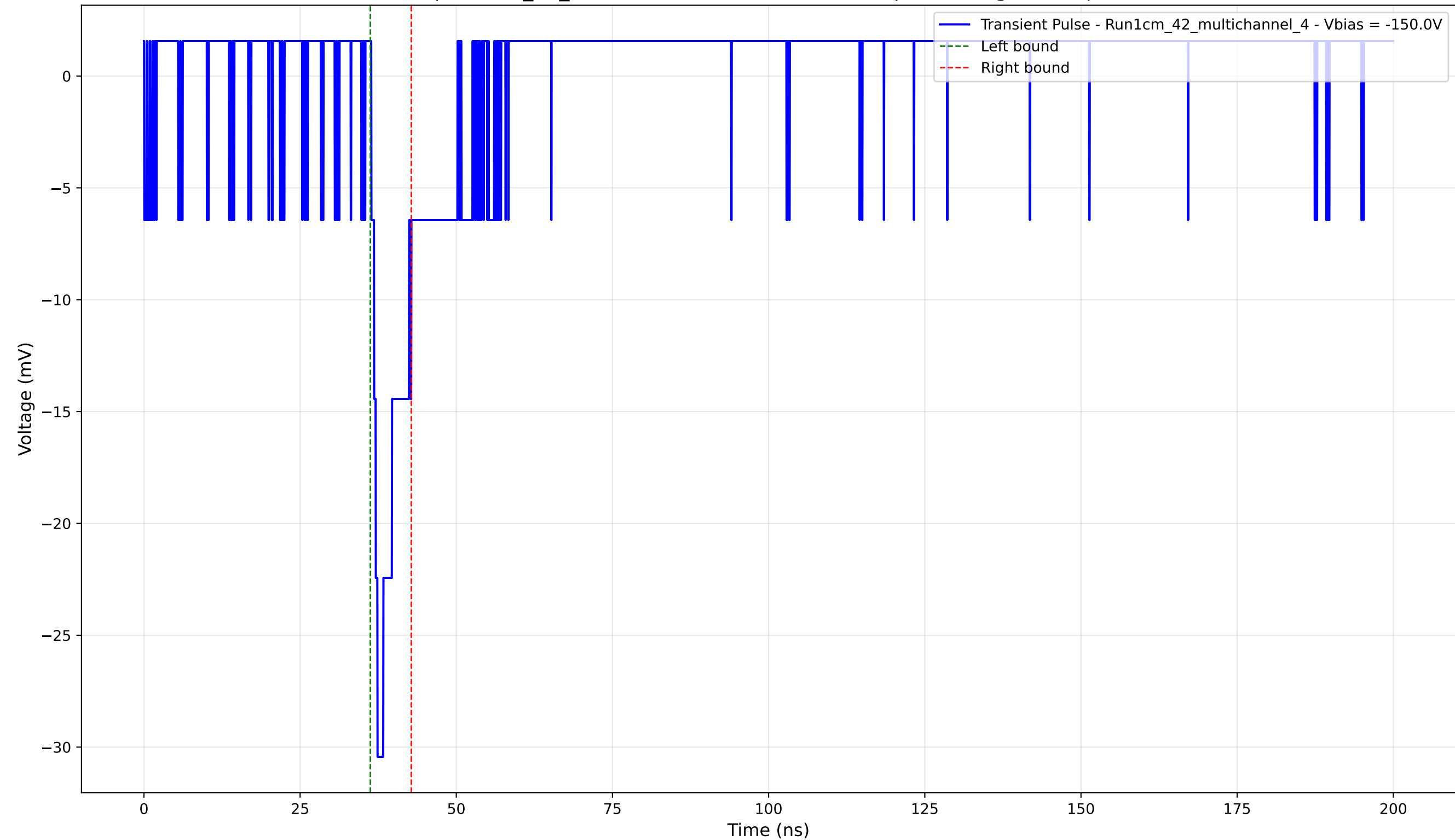
Transient Pulse - Sample: 1cm_42_multichannel - Position: 3130.0 \mu\text{m} - Charge: 2.30 pC - Rise Time: 0.99 ns
