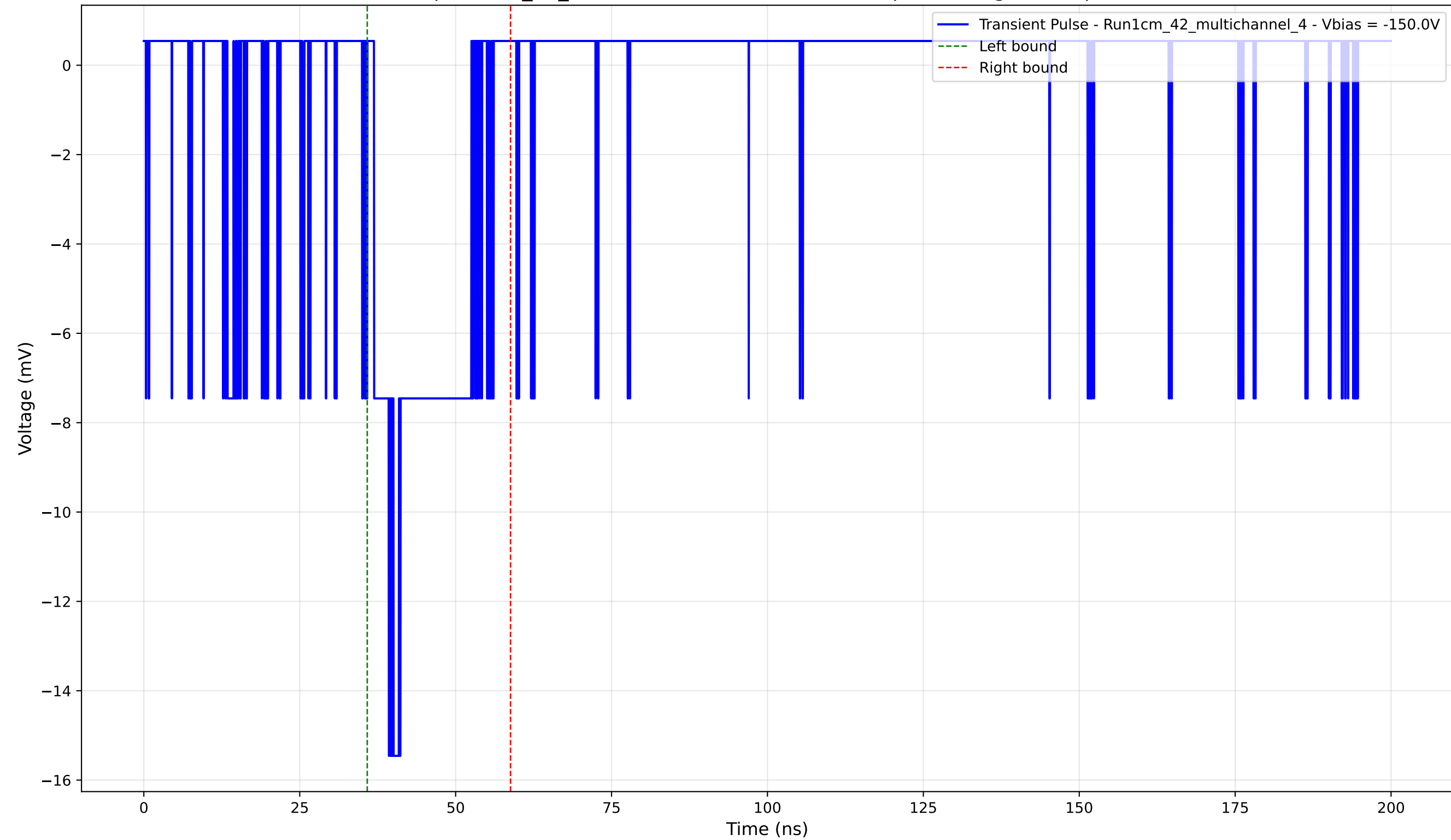
Transient Pulse - Sample: 1cm_42_multichannel - Position: 4810.0 \mu\text{m} - Charge: 2.64 pC - Rise Time: 2.38 ns
