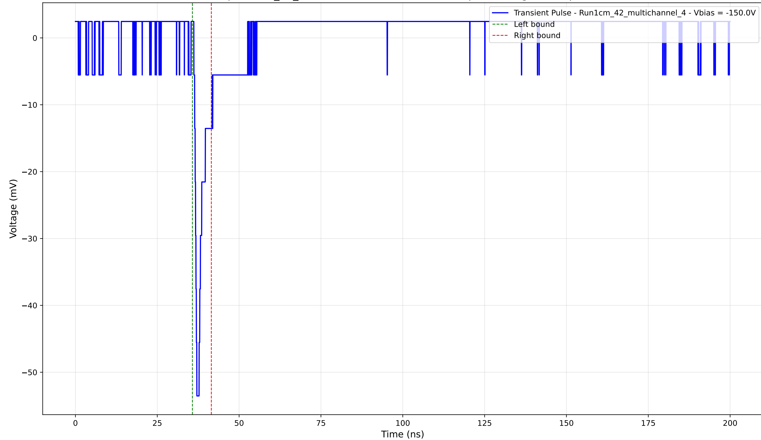
Transient Pulse - Sample: 1cm_42_multichannel - Position: 2685.0 \mu\text{m} - Charge: 2.68 pC - Rise Time: 0.90 ns
