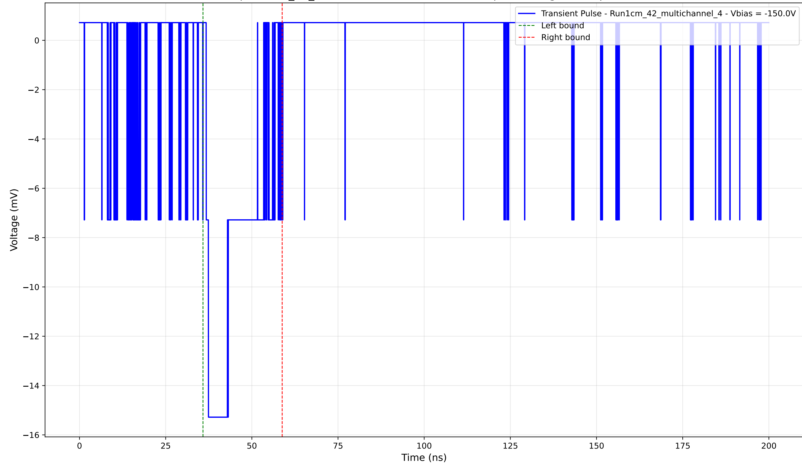
Transient Pulse - Sample: 1cm_42_multichannel - Position: 3610.0 \mu\text{m} - Charge: 3.59 pC - Rise Time: 0.66 ns
