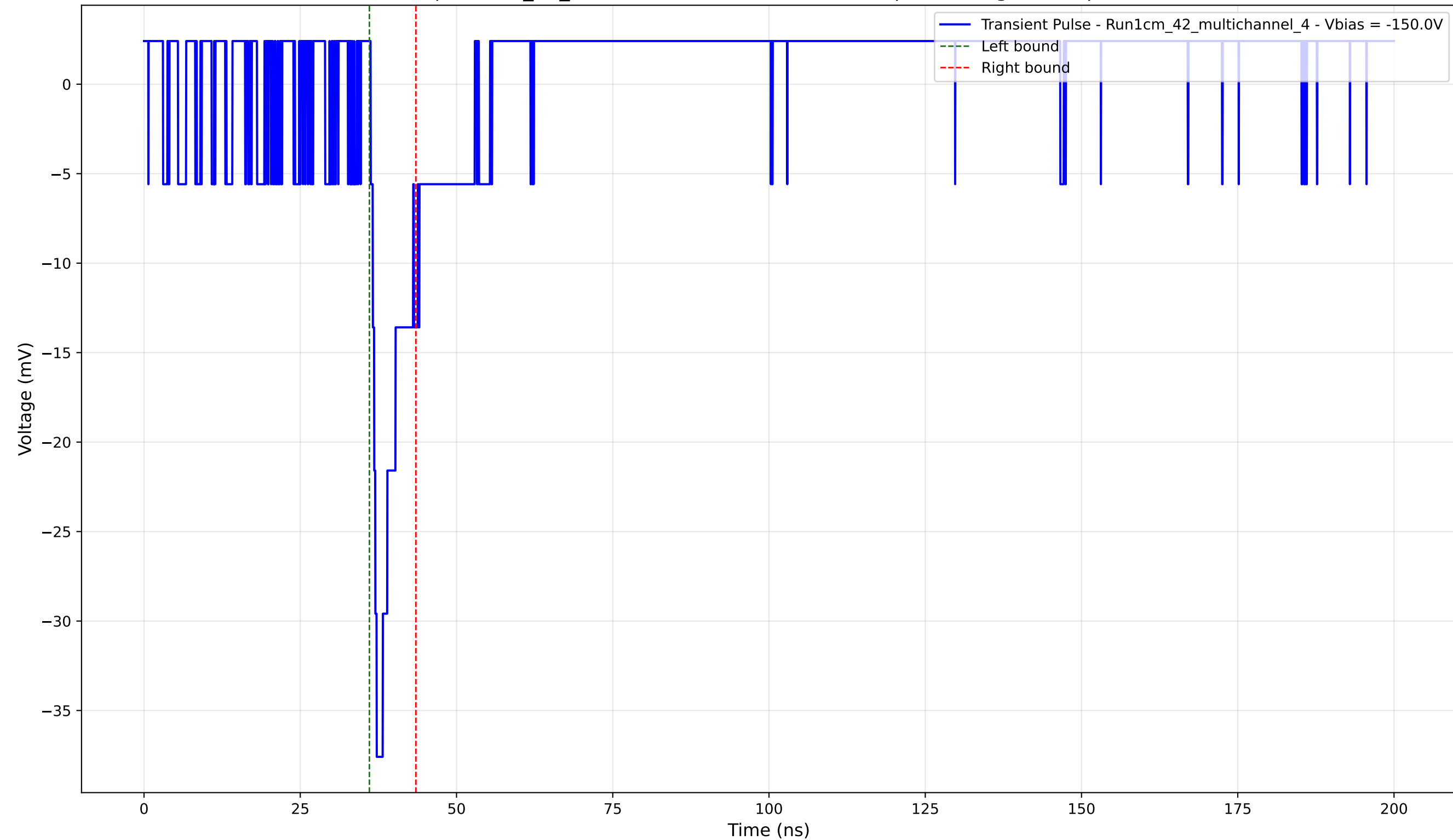
Transient Pulse - Sample: 1cm_42_multichannel - Position: 1765.0 \mu\text{m} - Charge: 2.90 pC - Rise Time: 0.97 ns
