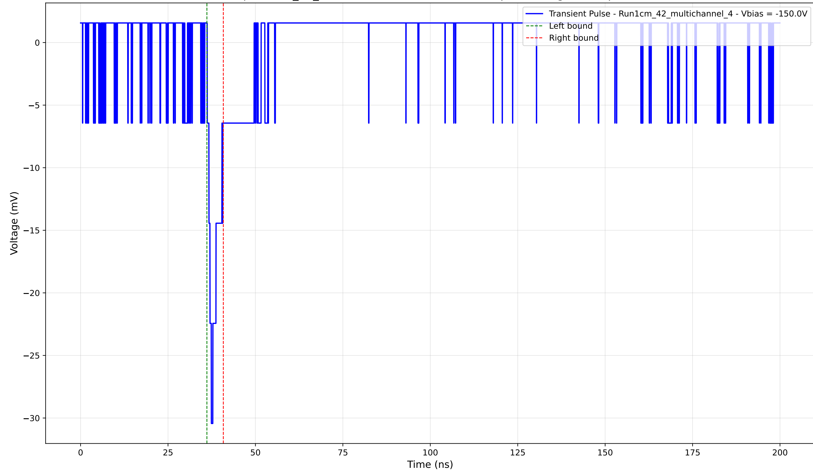
Transient Pulse - Sample: 1cm_42_multichannel - Position: 2950.0 \mu\text{m} - Charge: 1.56 pC - Rise Time: 1.19 ns
