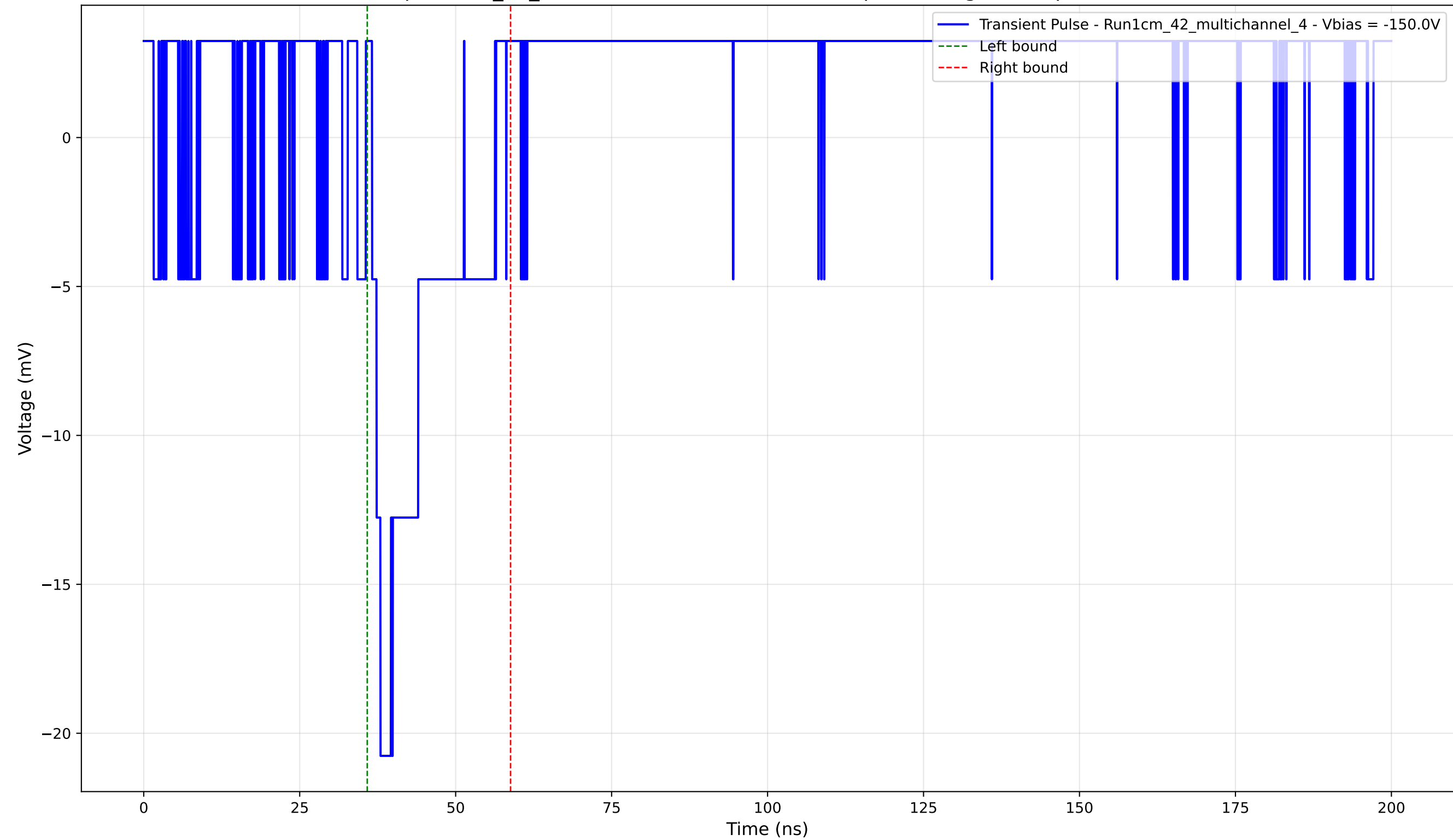
Transient Pulse - Sample: 1cm_42_multichannel - Position: 1095.0 \mu\text{m} - Charge: 3.03 pC - Rise Time: 0.00 ns (N/A)
