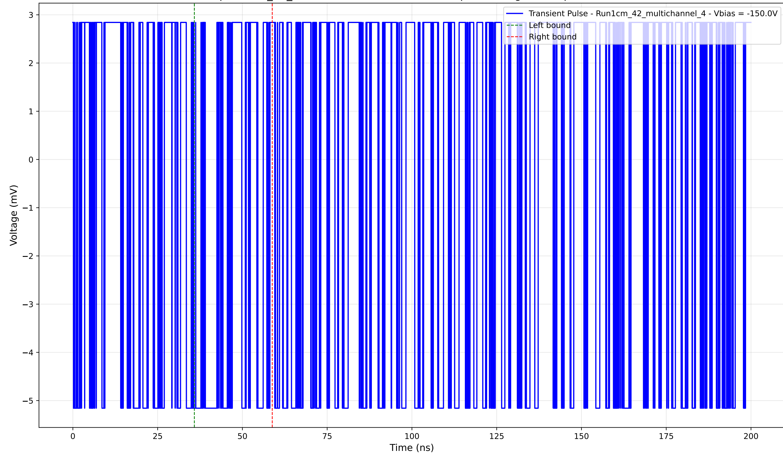
Transient Pulse - Sample: 1cm_42_multichannel - Position: 875.0 \mu\text{m} - Charge: 0.68 pC - Rise Time: 0.00 ns (N/A)
