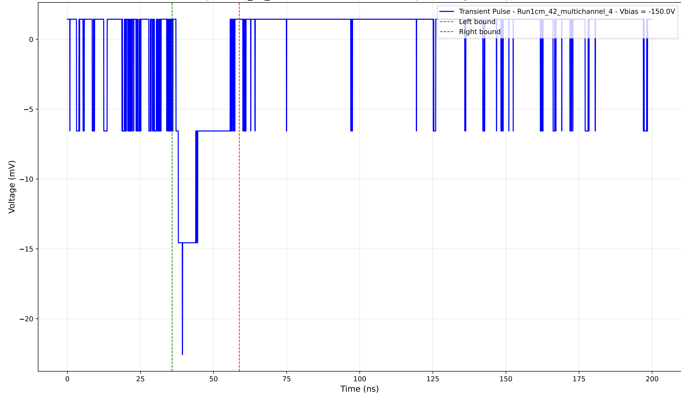
Transient Pulse - Sample: 1cm_42_multichannel - Position: 675.0 \mu\text{m} - Charge: 3.45 pC - Rise Time: 2.20 ns
