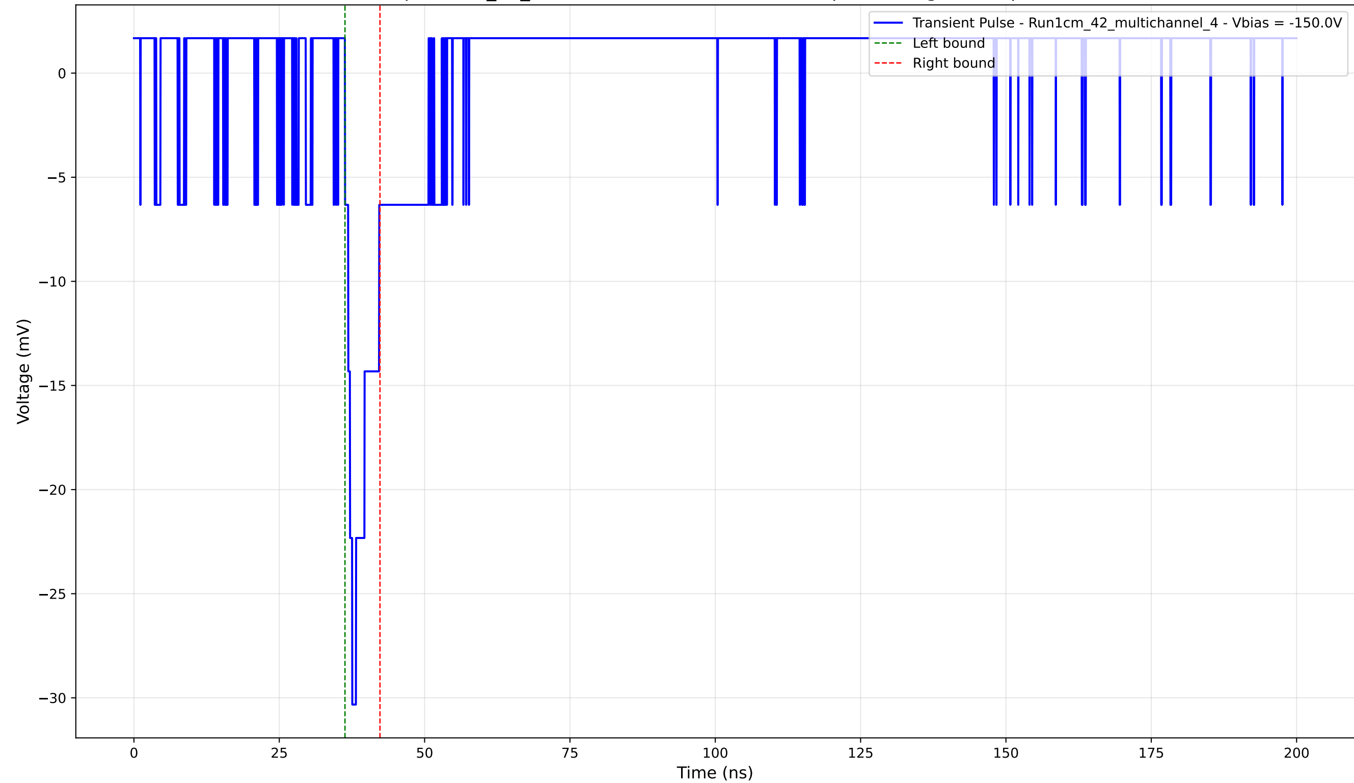
Transient Pulse - Sample: 1cm_42_multichannel - Position: 3170.0 \mu\text{m} - Charge: 2.12 pC - Rise Time: 1.25 ns
