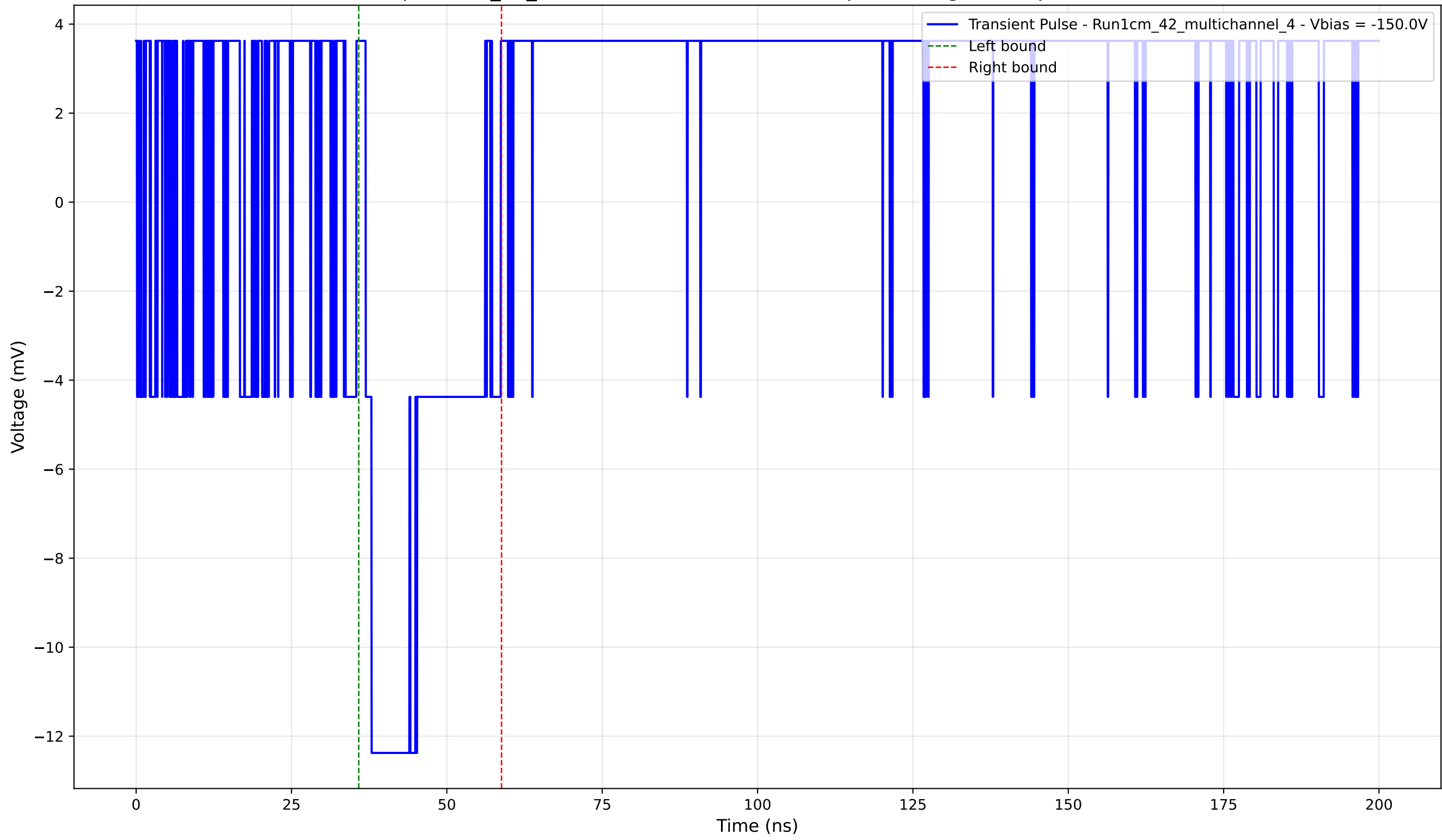
Transient Pulse - Sample: 1cm_42_multichannel - Position: 670.0 \mu\text{m} - Charge: 2.80 pC - Rise Time: 0.00 ns (N/A)
