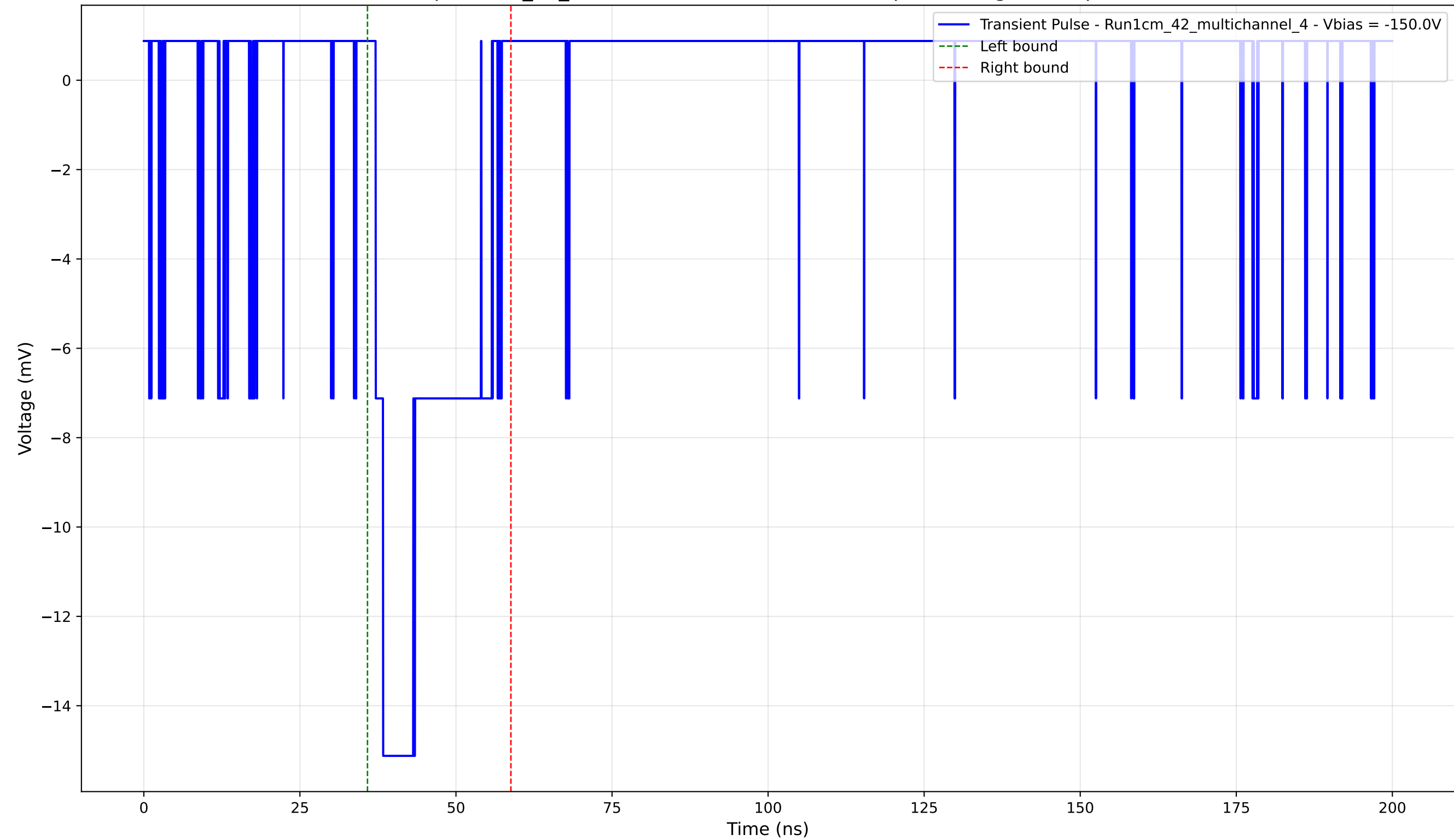
Transient Pulse - Sample: 1cm_42_multichannel - Position: 4145.0 \mu\text{m} - Charge: 3.42 pC - Rise Time: 1.20 ns
