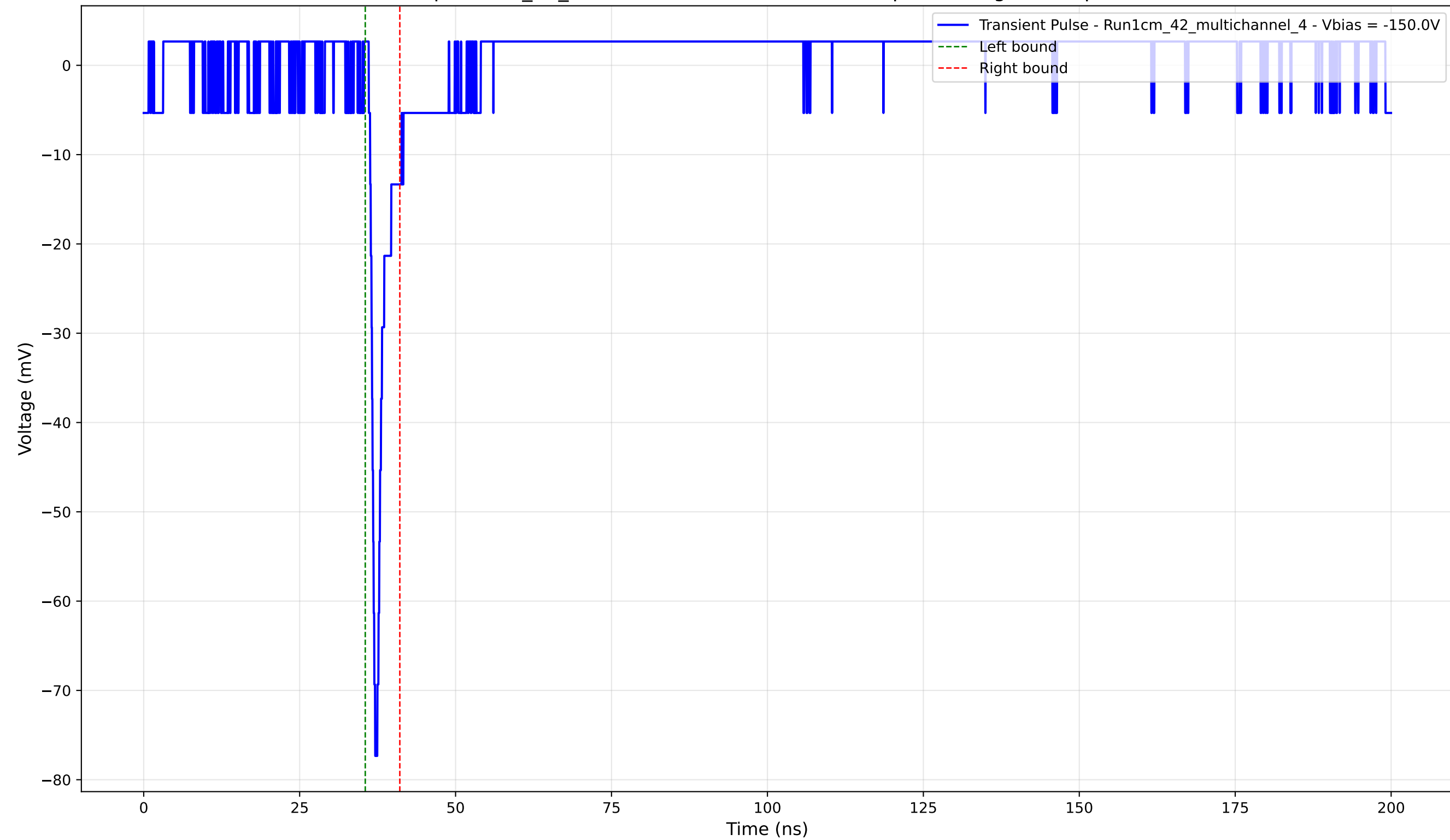
Transient Pulse - Sample: 1cm_42_multichannel - Position: 2525.0 \mu\text{m} - Charge: 3.08 pC - Rise Time: 0.81 ns
