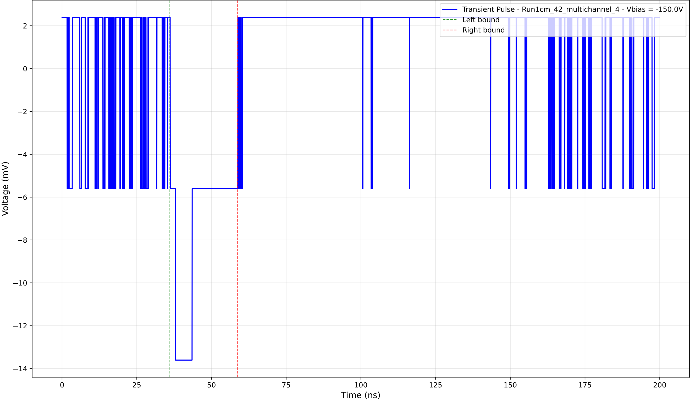
Transient Pulse - Sample: 1cm_42_multichannel - Position: 600.0 \mu\text{m} - Charge: 3.41 pC - Rise Time: 0.00 ns (N/A)
