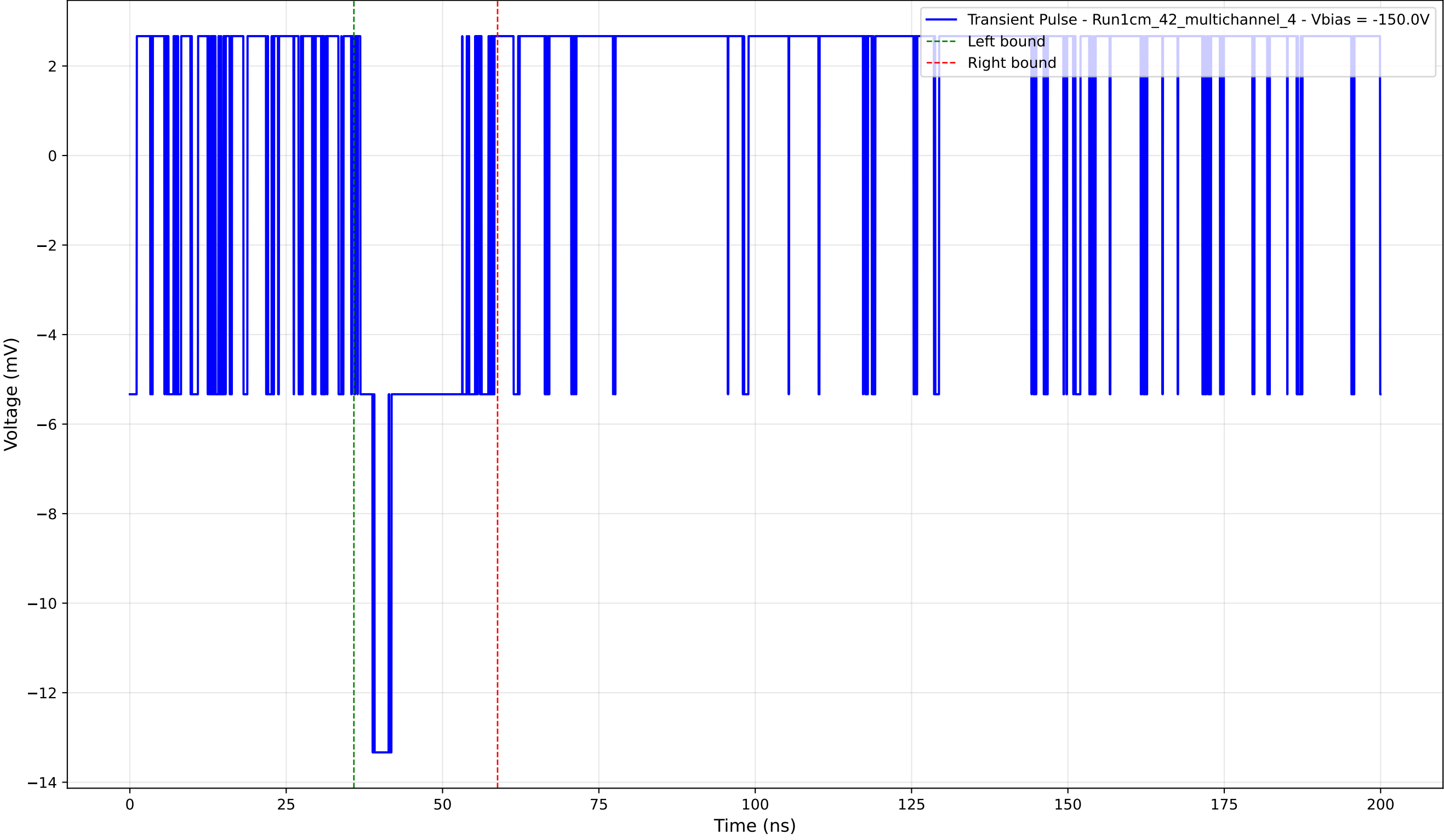
Transient Pulse - Sample: 1cm_42_multichannel - Position: 425.0 \mu\text{m} - Charge: 2.50 pC - Rise Time: 0.00 ns (N/A)
