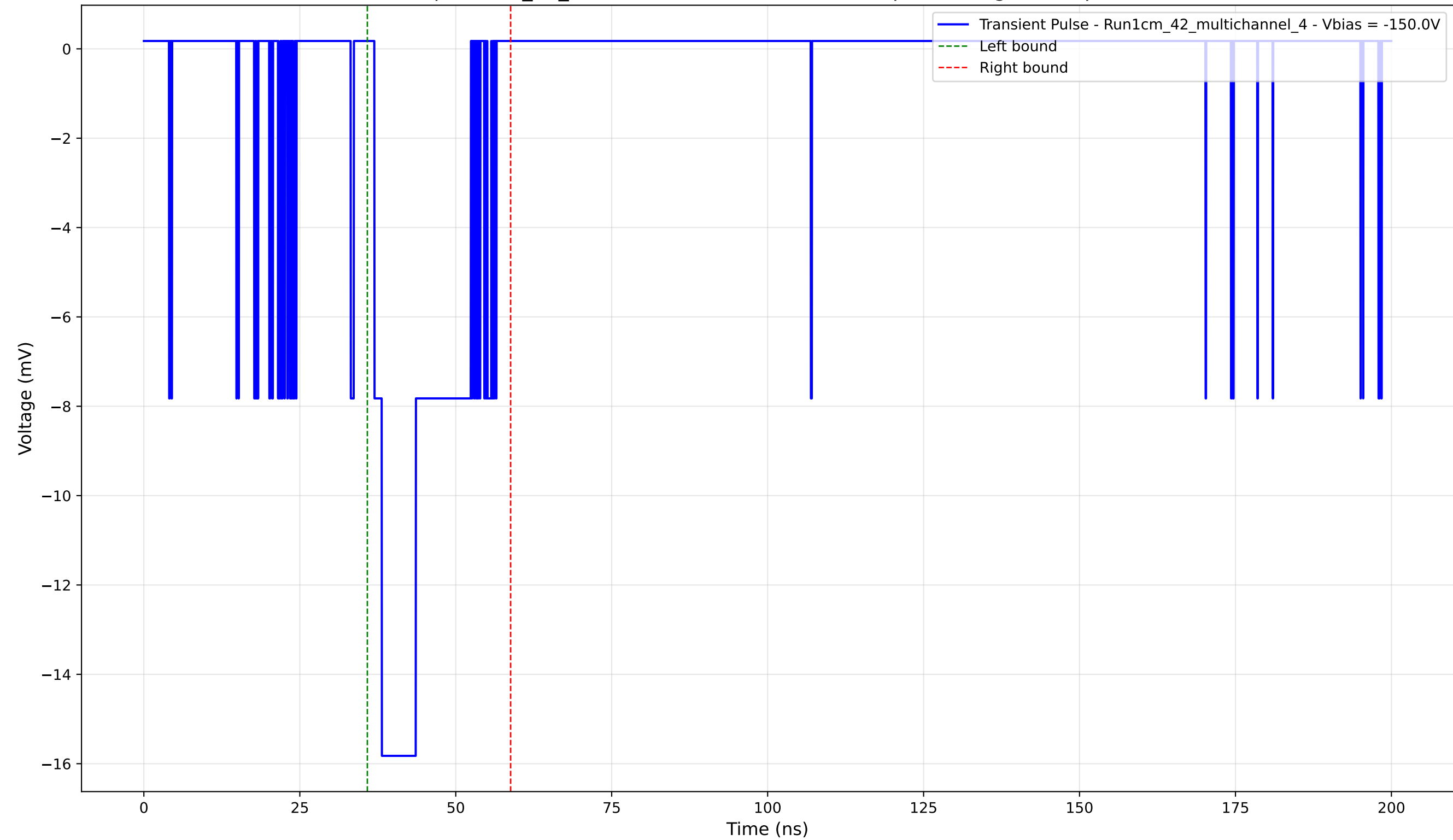
Transient Pulse - Sample: 1cm_42_multichannel - Position: 4045.0 \mu\text{m} - Charge: 3.57 pC - Rise Time: 1.20 ns
