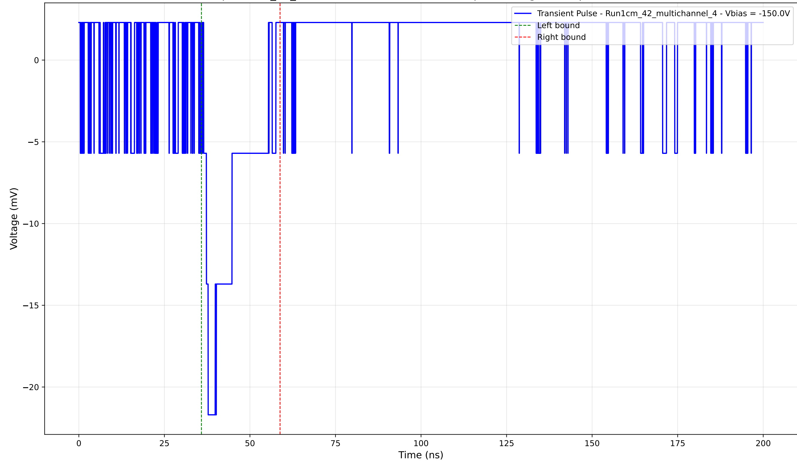
Transient Pulse - Sample: 1cm_42_multichannel - Position: 1160.0 \mu\text{m} - Charge: 3.75 pC - Rise Time: 0.00 ns (N/A)
