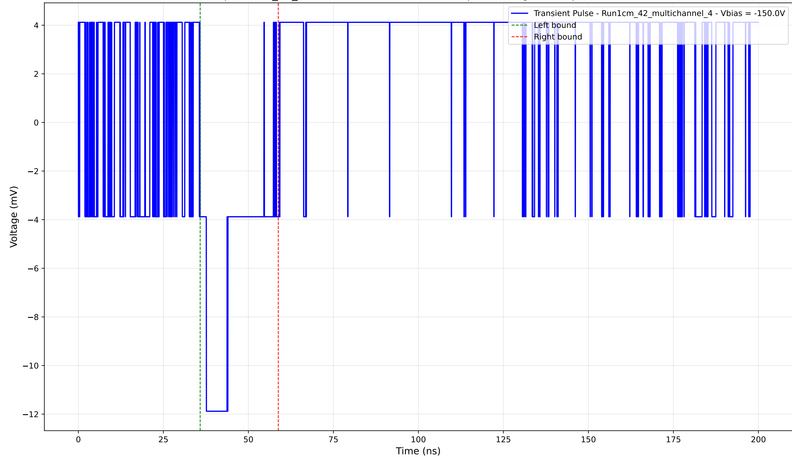
Transient Pulse - Sample: 1cm_42_multichannel - Position: 935.0 \mu\text{m} - Charge: 2.70 pC - Rise Time: 0.00 ns (N/A)
