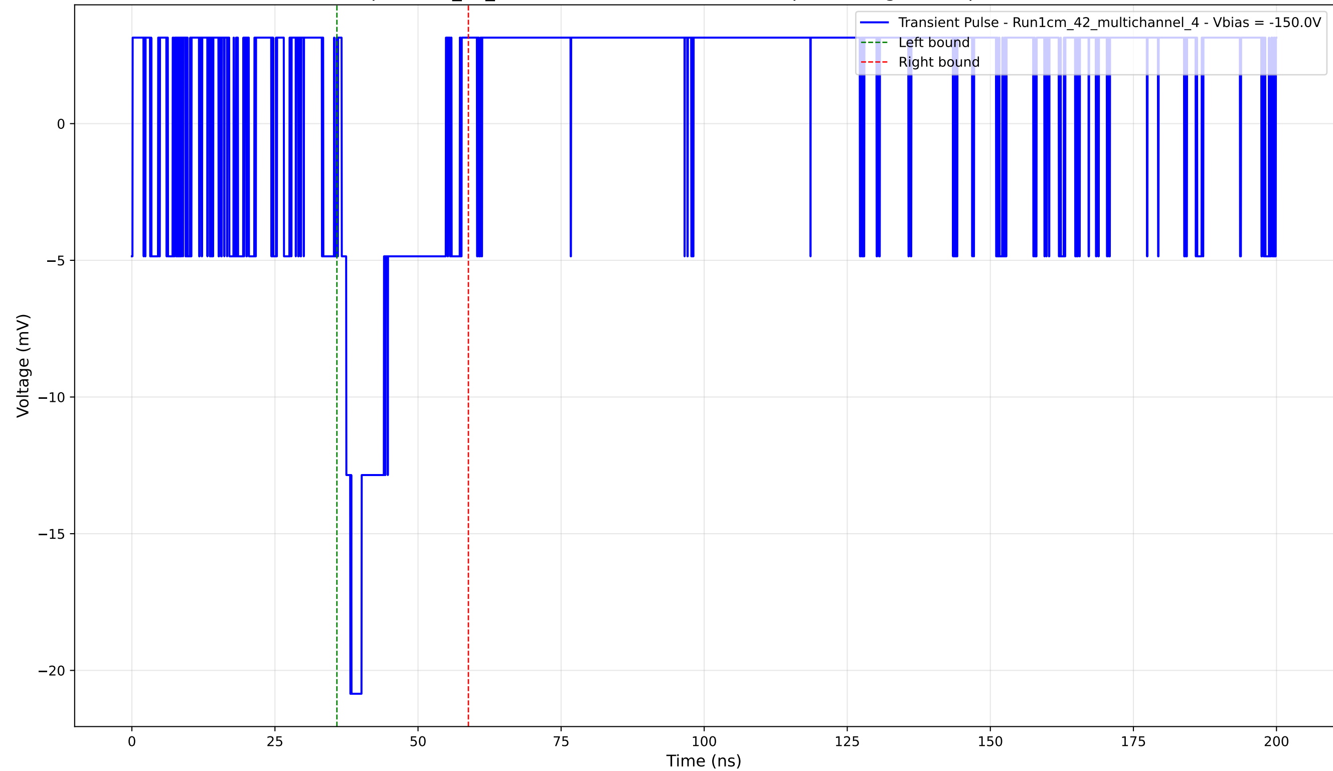
Transient Pulse - Sample: 1cm_42_multichannel - Position: 1055.0 \mu\text{m} - Charge: 3.19 pC - Rise Time: 0.00 ns (N/A)
