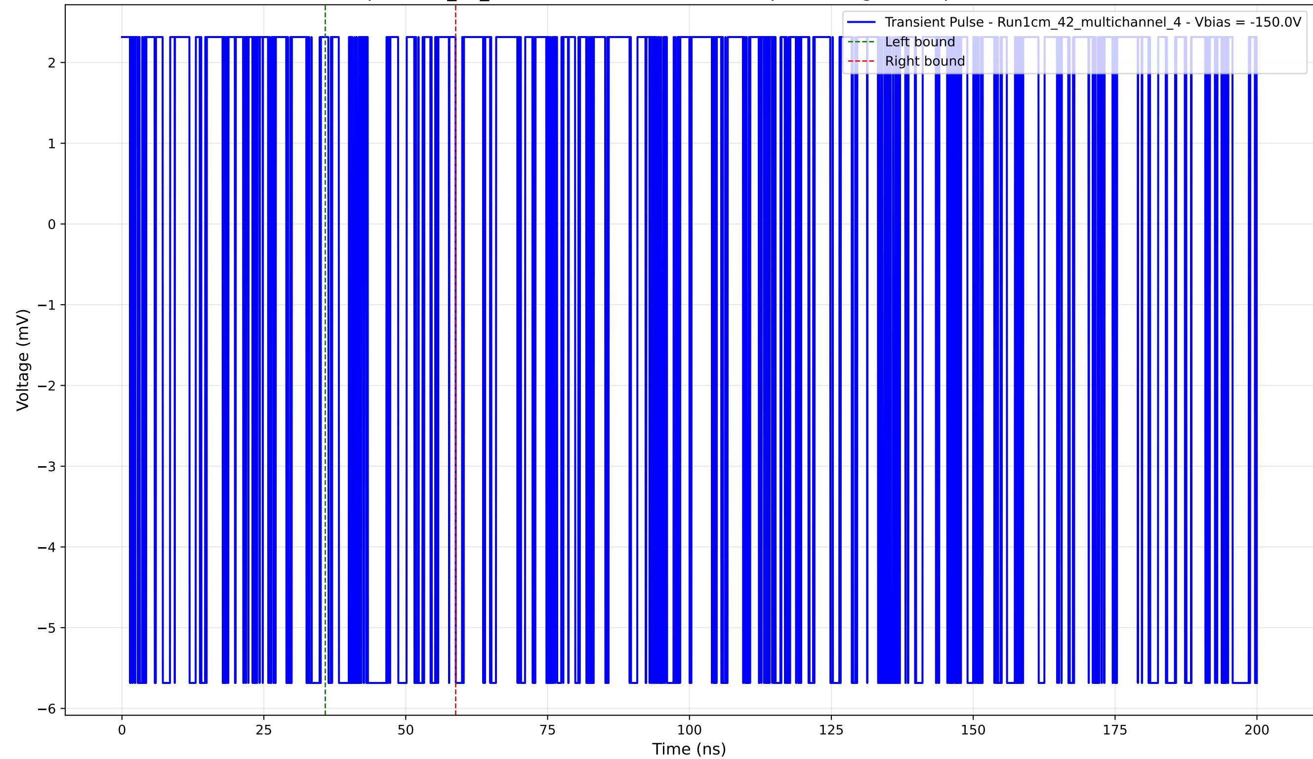
Transient Pulse - Sample: 1cm_42_multichannel - Position: 340.0 \mu\text{m} - Charge: 0.75 pC - Rise Time: 0.00 ns (N/A)
