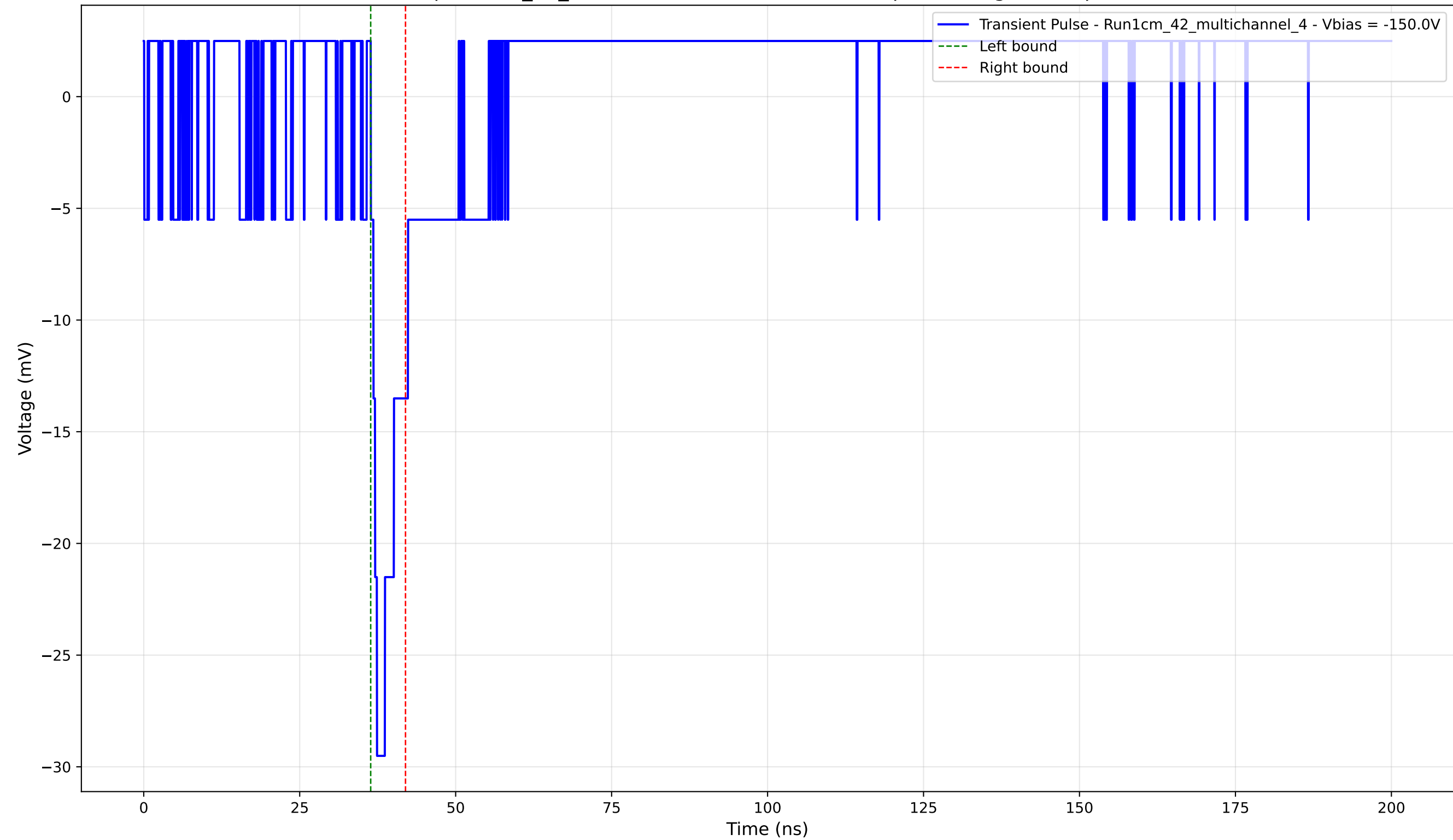
Transient Pulse - Sample: 1cm_42_multichannel - Position: 1585.0 \mu\text{m} - Charge: 2.13 pC - Rise Time: 1.00 ns
