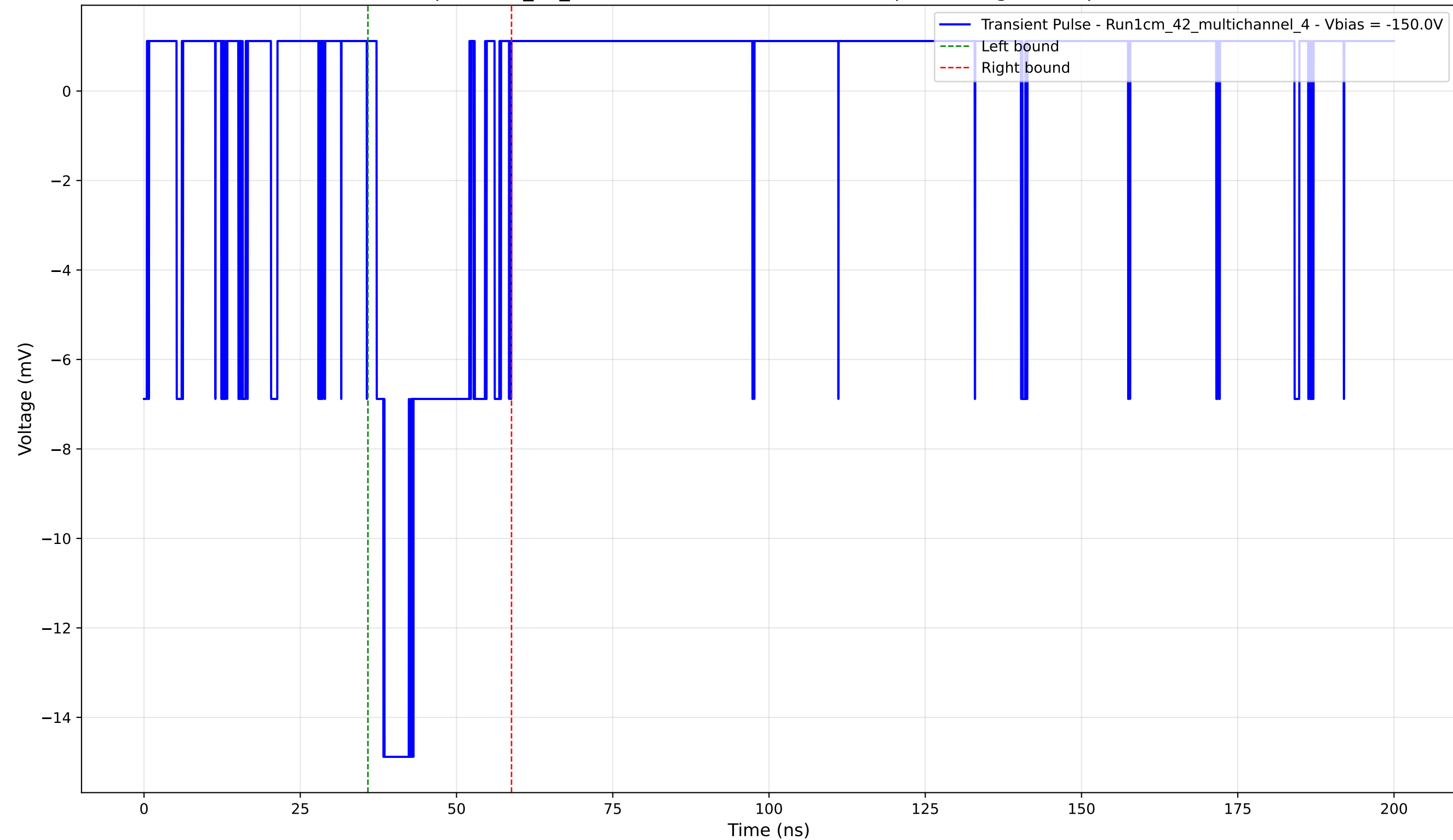
Transient Pulse - Sample: 1cm_42_multichannel - Position: 4235.0 \mu\text{m} - Charge: 3.05 pC - Rise Time: 1.10 ns
