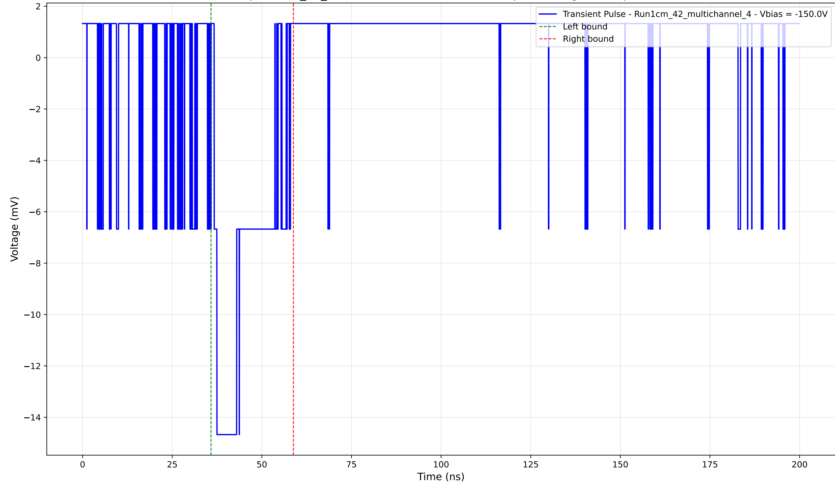
Transient Pulse - Sample: 1cm_42_multichannel - Position: 3665.0 \mu\text{m} - Charge: 3.36 pC - Rise Time: 0.78 ns
