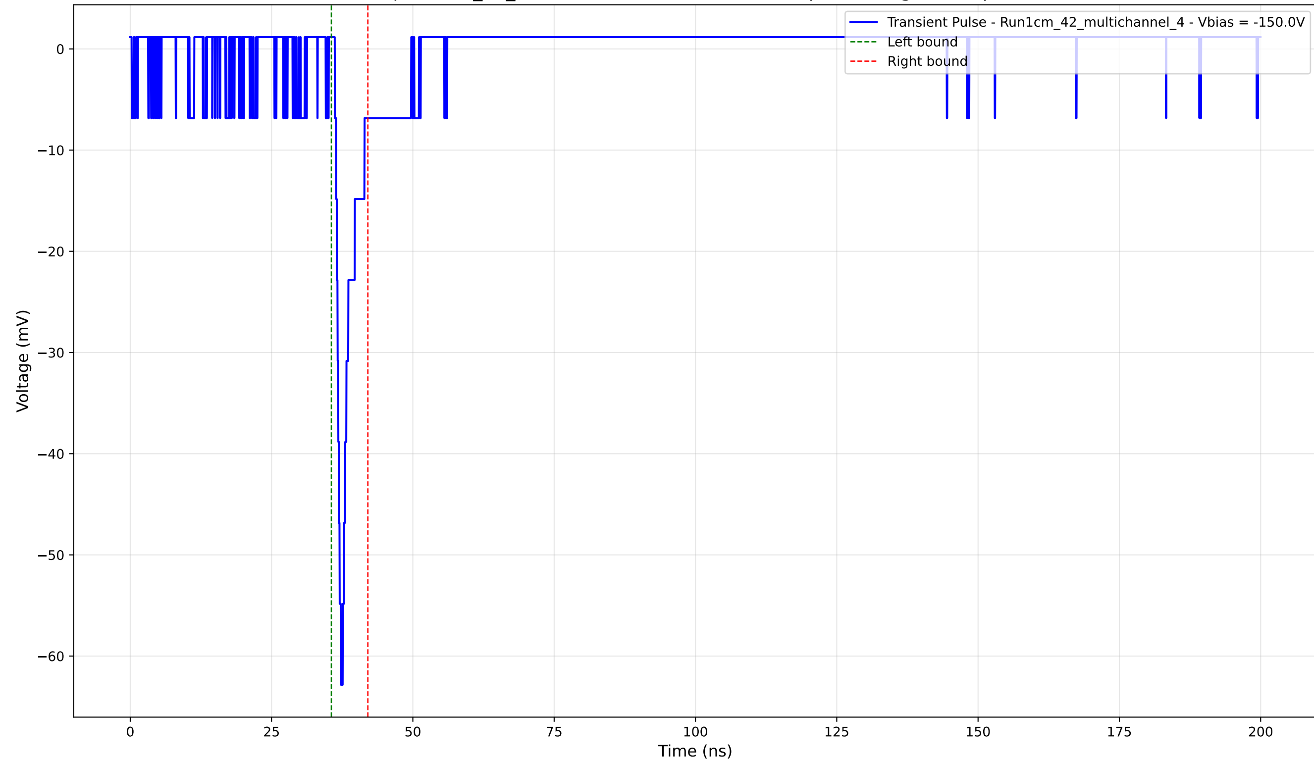
Transient Pulse - Sample: 1cm_42_multichannel - Position: 2090.0 \mu\text{m} - Charge: 2.98 pC - Rise Time: 1.06 ns
