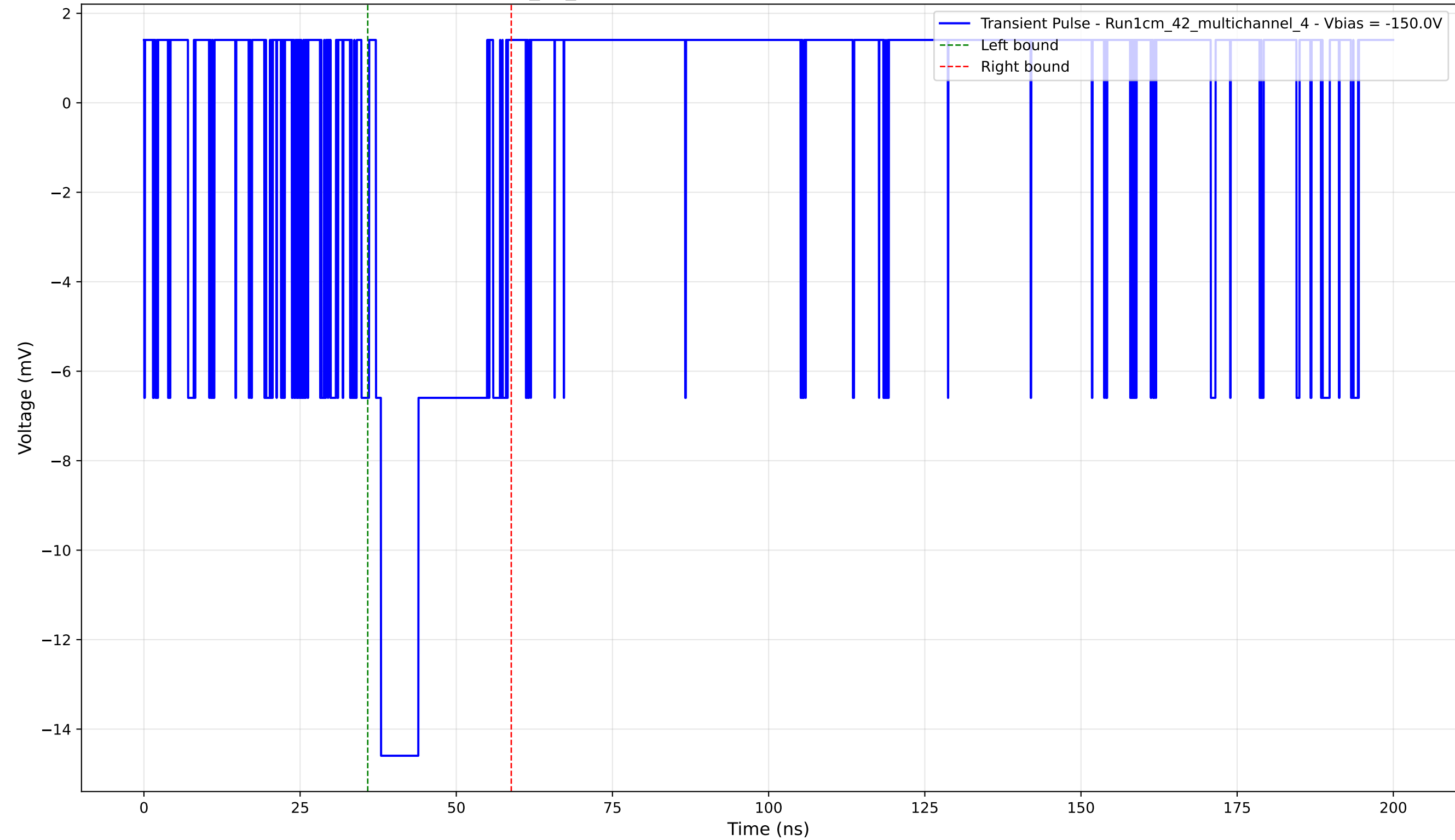
Transient Pulse - Sample: 1cm_42_multichannel - Position: 570.0 \mu\text{m} - Charge: 3.56 pC - Rise Time: 0.82 ns
