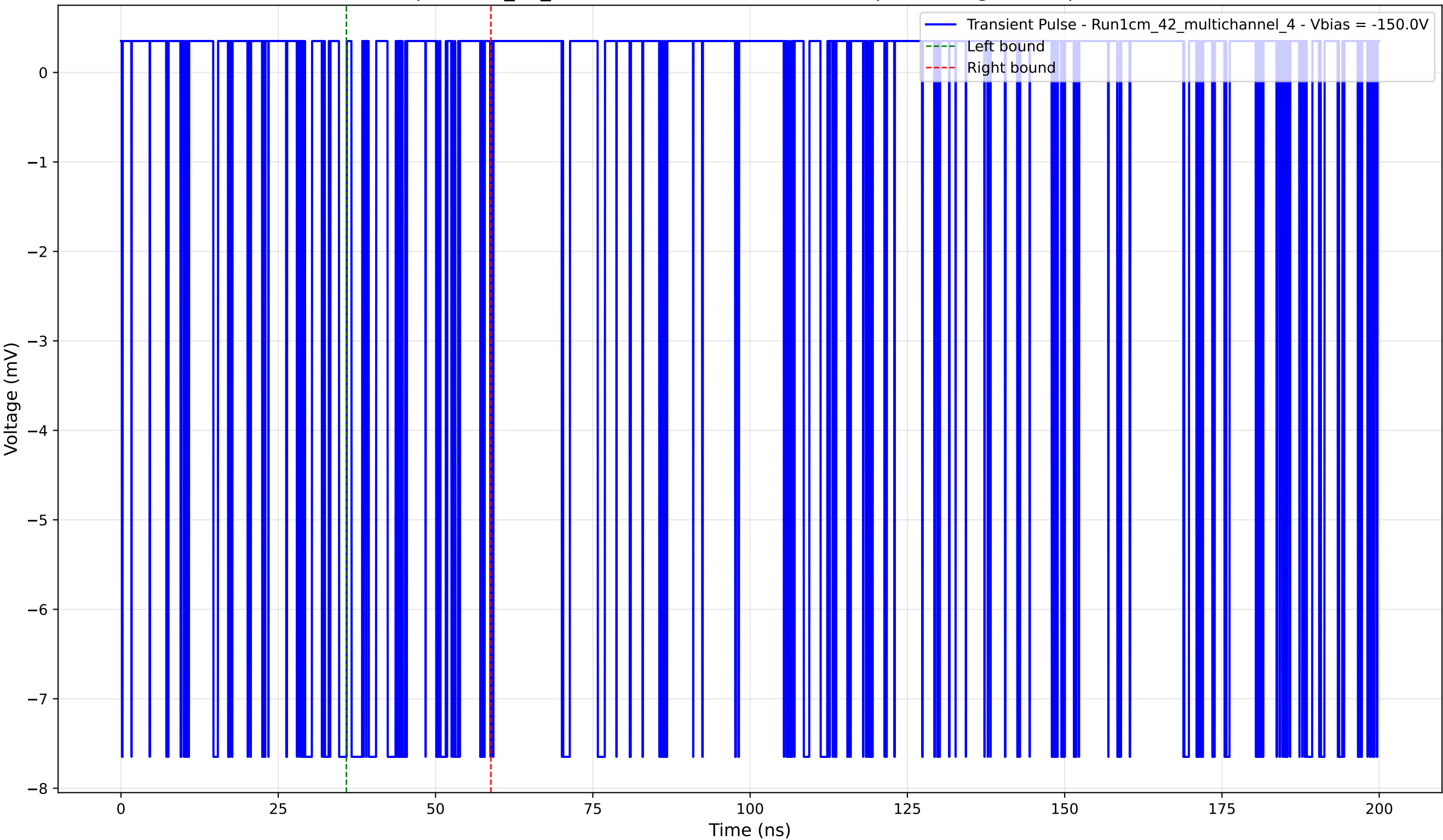
Transient Pulse - Sample: 1cm_42_multichannel - Position: 1885.0 \mu\text{m} - Charge: 1.17 pC - Rise Time: 0.02 ns
