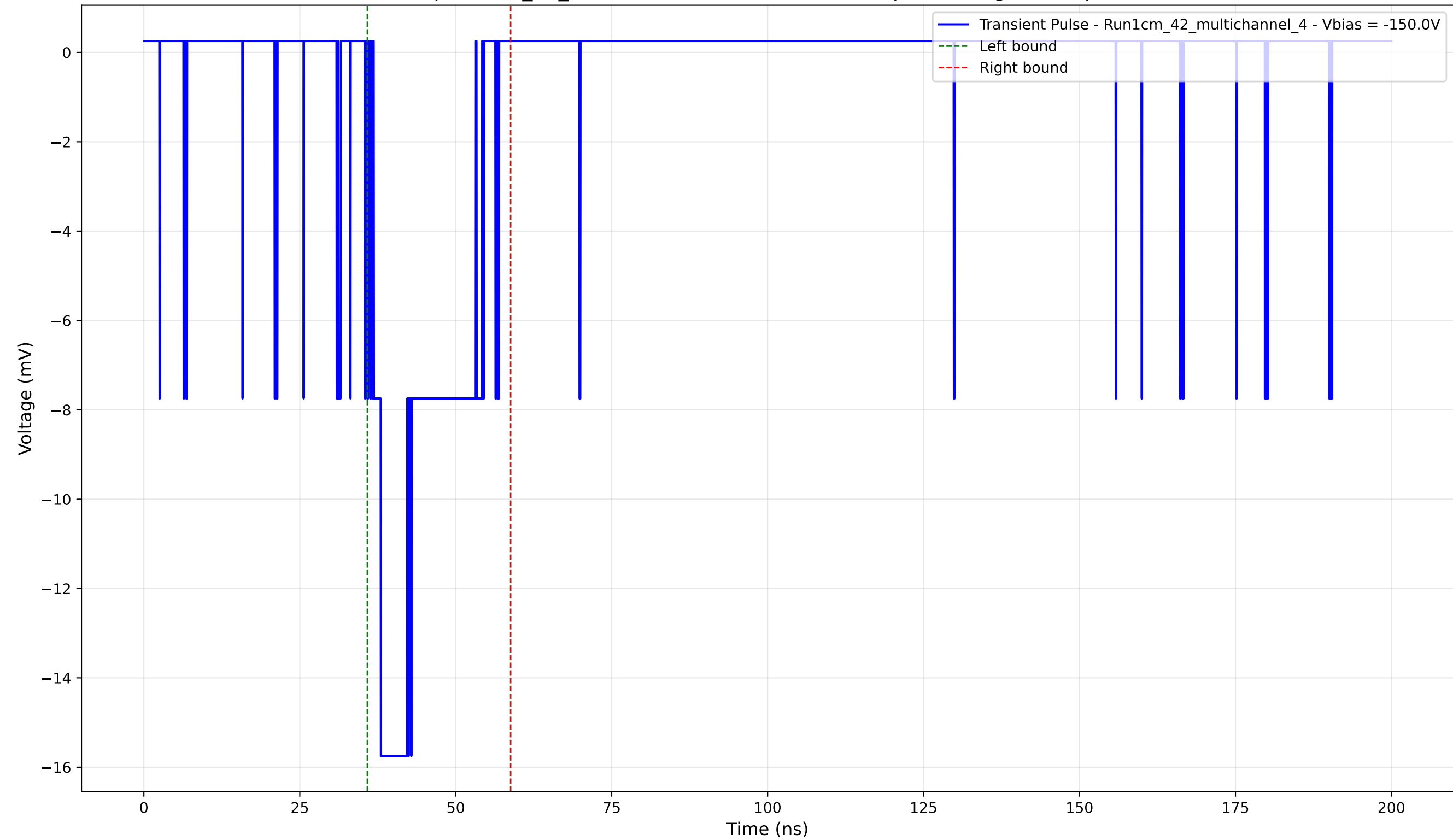
Transient Pulse - Sample: 1cm_42_multichannel - Position: 3830.0 \mu\text{m} - Charge: 3.48 pC - Rise Time: 1.14 ns
