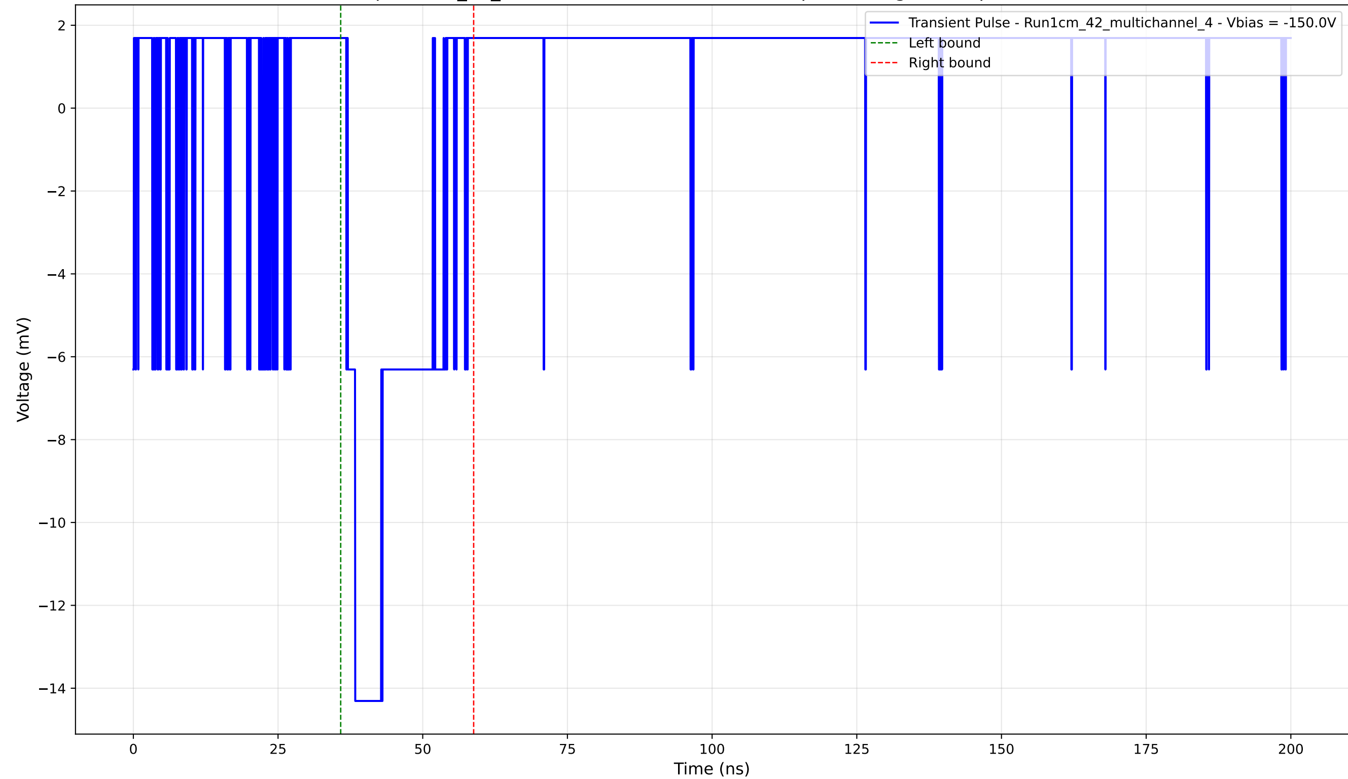
Transient Pulse - Sample: 1cm_42_multichannel - Position: 4170.0 \mu\text{m} - Charge: 2.72 pC - Rise Time: 0.00 ns (N/A)
