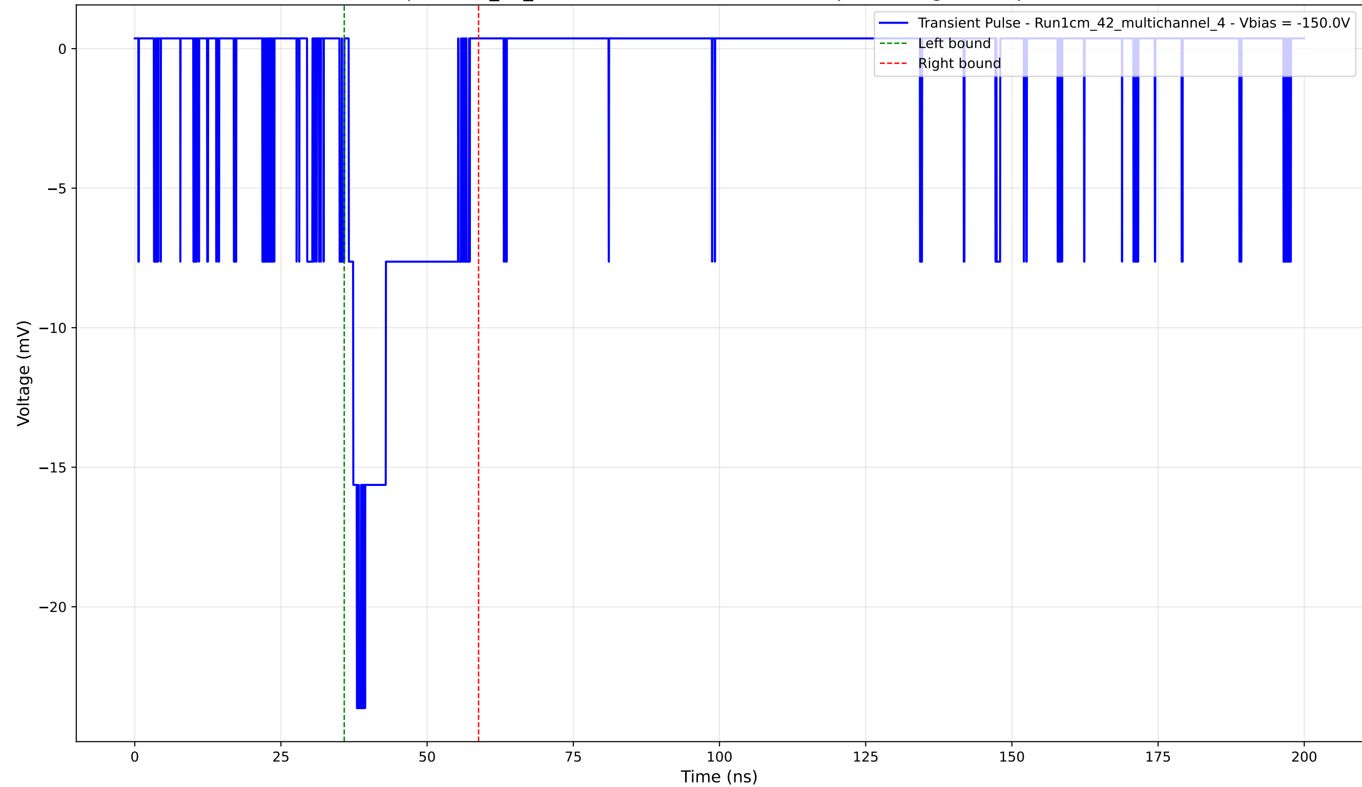
Transient Pulse - Sample: 1cm_42_multichannel - Position: 3545.0 \mu\text{m} - Charge: 4.09 pC - Rise Time: 1.39 ns
