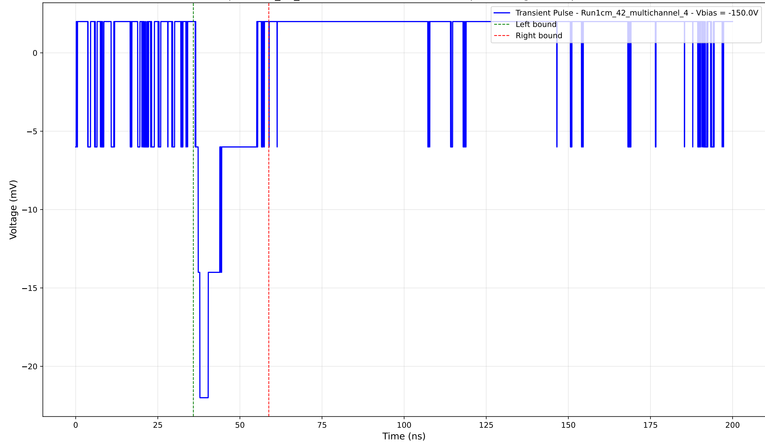
Transient Pulse - Sample: 1cm_42_multichannel - Position: 1175.0 \mu\text{m} - Charge: 3.62 pC - Rise Time: 1.26 ns
