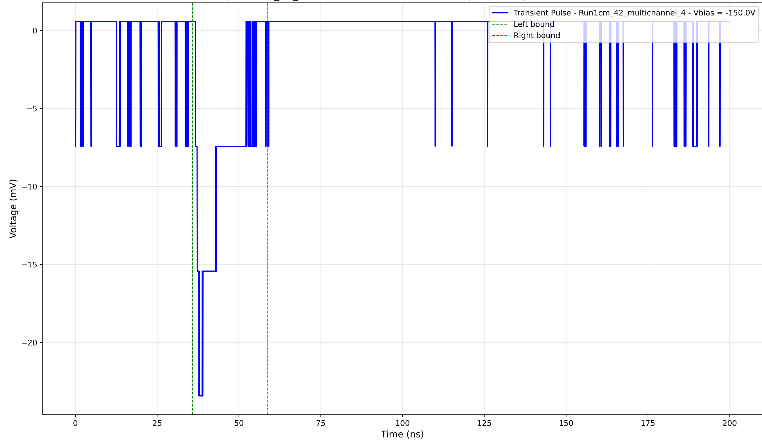
Transient Pulse - Sample: 1cm_42_multichannel - Position: 3485.0 \mu\text{m} - Charge: 3.65 pC - Rise Time: 1.05 ns
