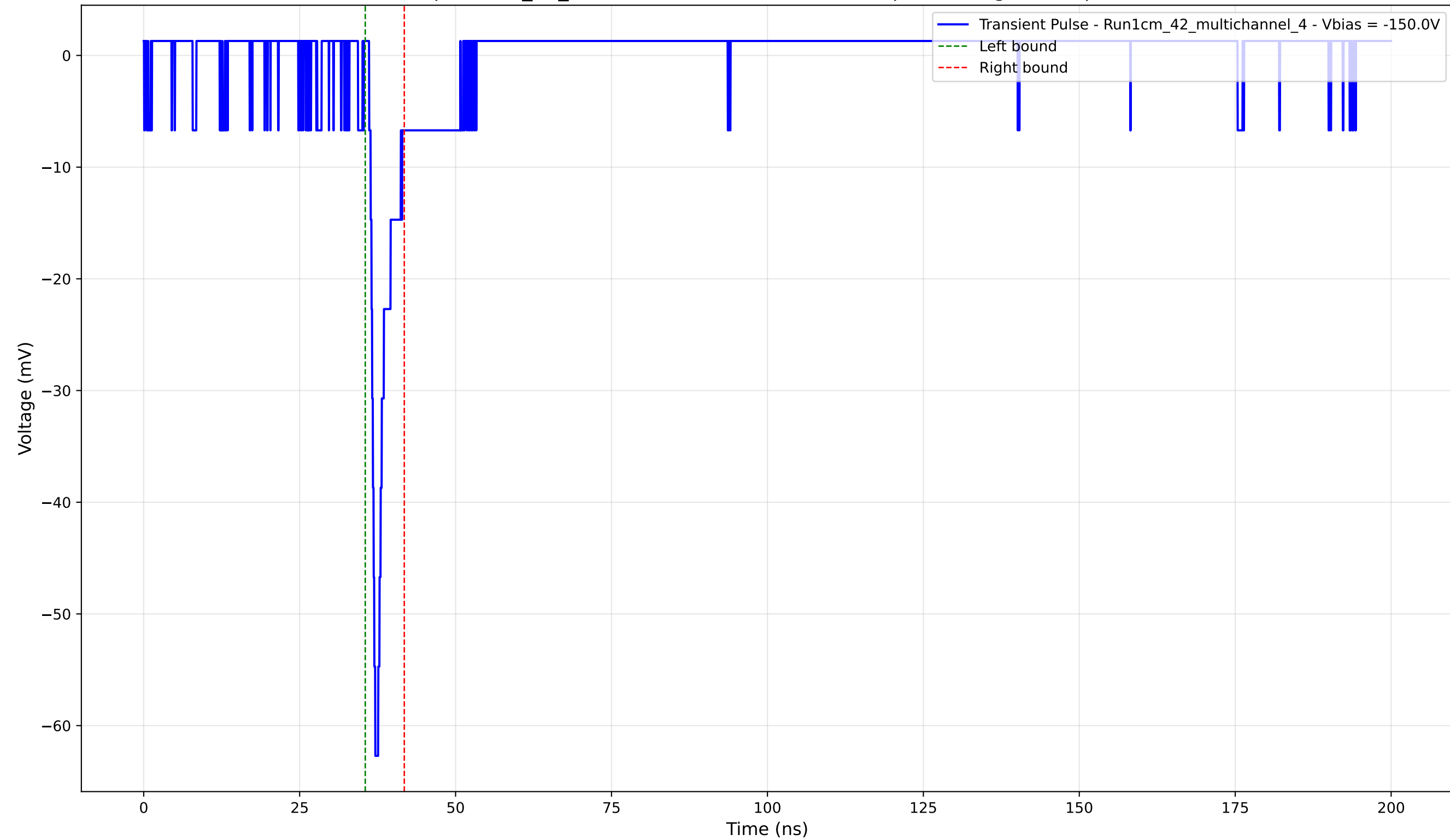
Transient Pulse - Sample: 1cm_42_multichannel - Position: 2610.0 \mu\text{m} - Charge: 2.94 pC - Rise Time: 0.98 ns
