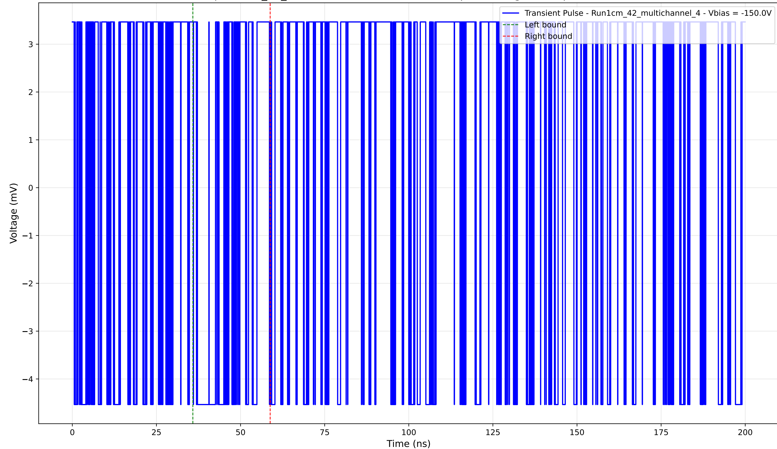
Transient Pulse - Sample: 1cm_42_multichannel - Position: 1345.0 \mu\text{m} - Charge: 0.15 pC - Rise Time: 0.00 ns (N/A)
