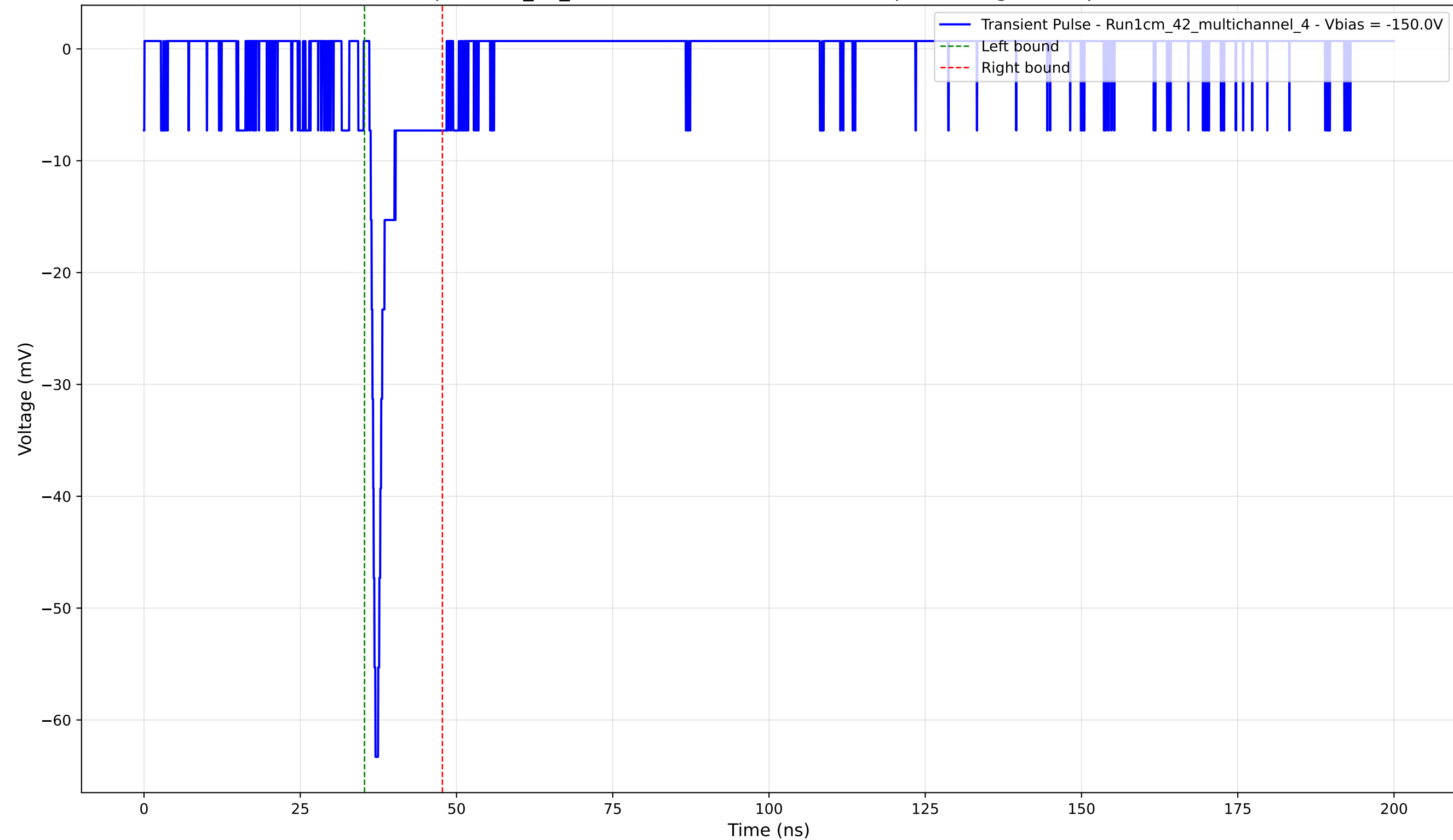
Transient Pulse - Sample: 1cm_42_multichannel - Position: 2325.0 \mu\text{m} - Charge: 3.47 pC - Rise Time: 0.96 ns
