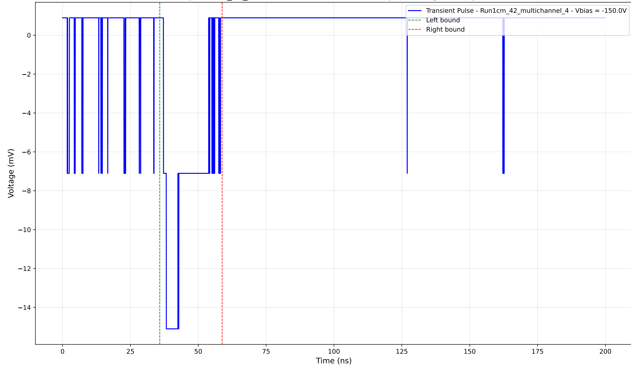
Transient Pulse - Sample: 1cm_42_multichannel - Position: 4180.0 \mu\text{m} - Charge: 3.18 pC - Rise Time: 1.06 ns
