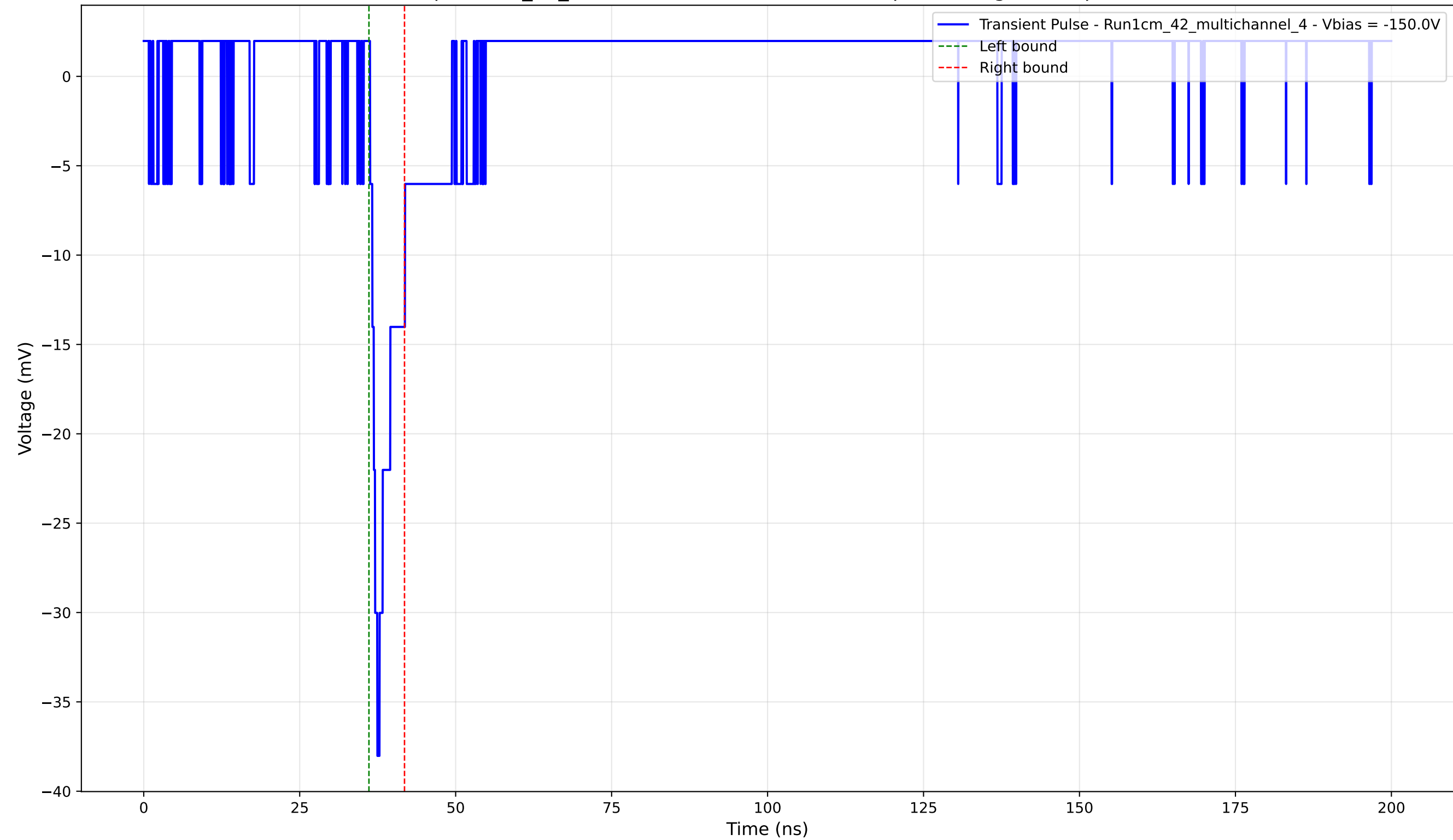
Transient Pulse - Sample: 1cm_42_multichannel - Position: 2960.0 \mu\text{m} - Charge: 2.16 pC - Rise Time: 1.17 ns
