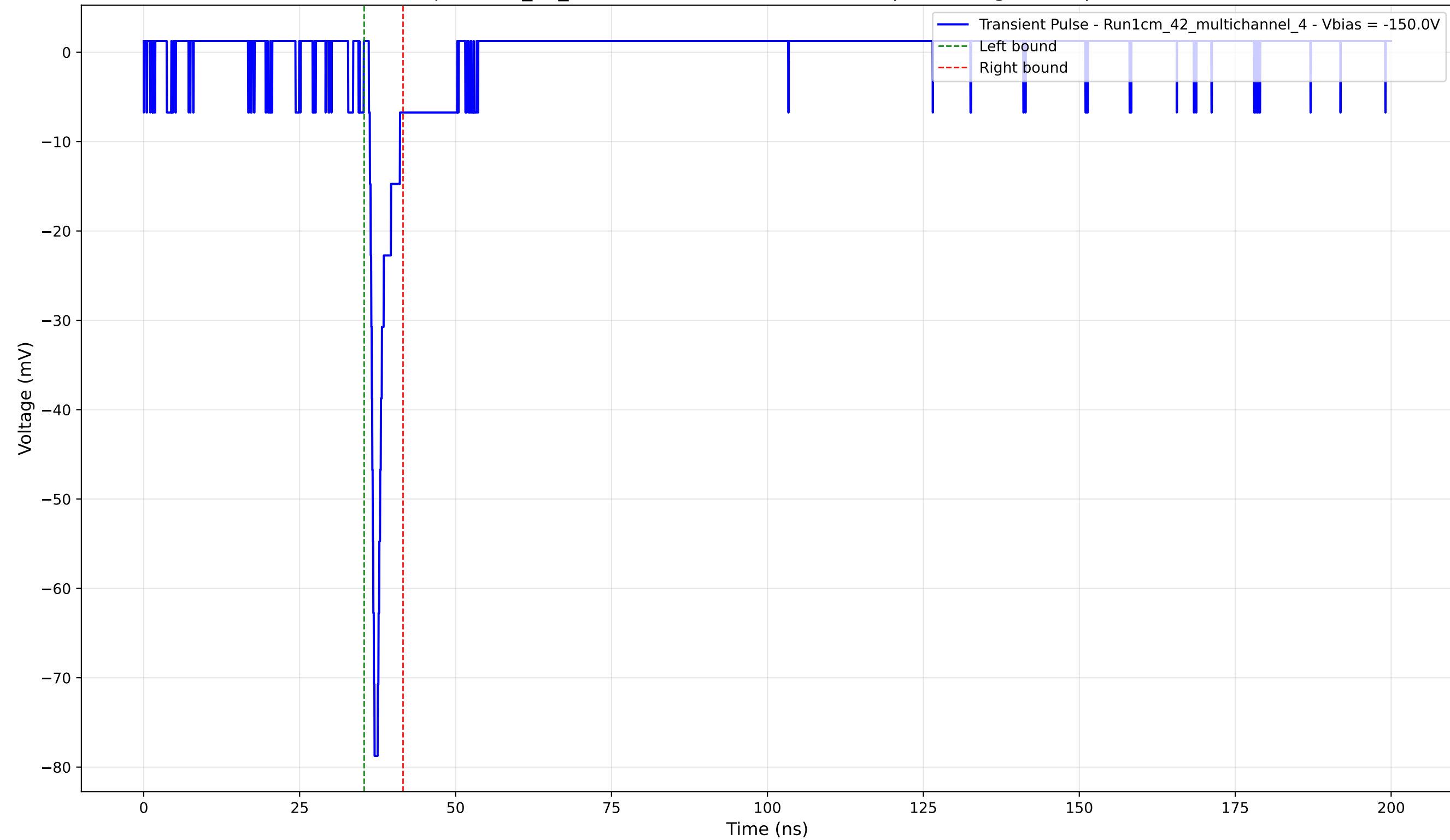
Transient Pulse - Sample: 1cm_42_multichannel - Position: 2485.0 \mu\text{m} - Charge: 3.36 pC - Rise Time: 0.76 ns
