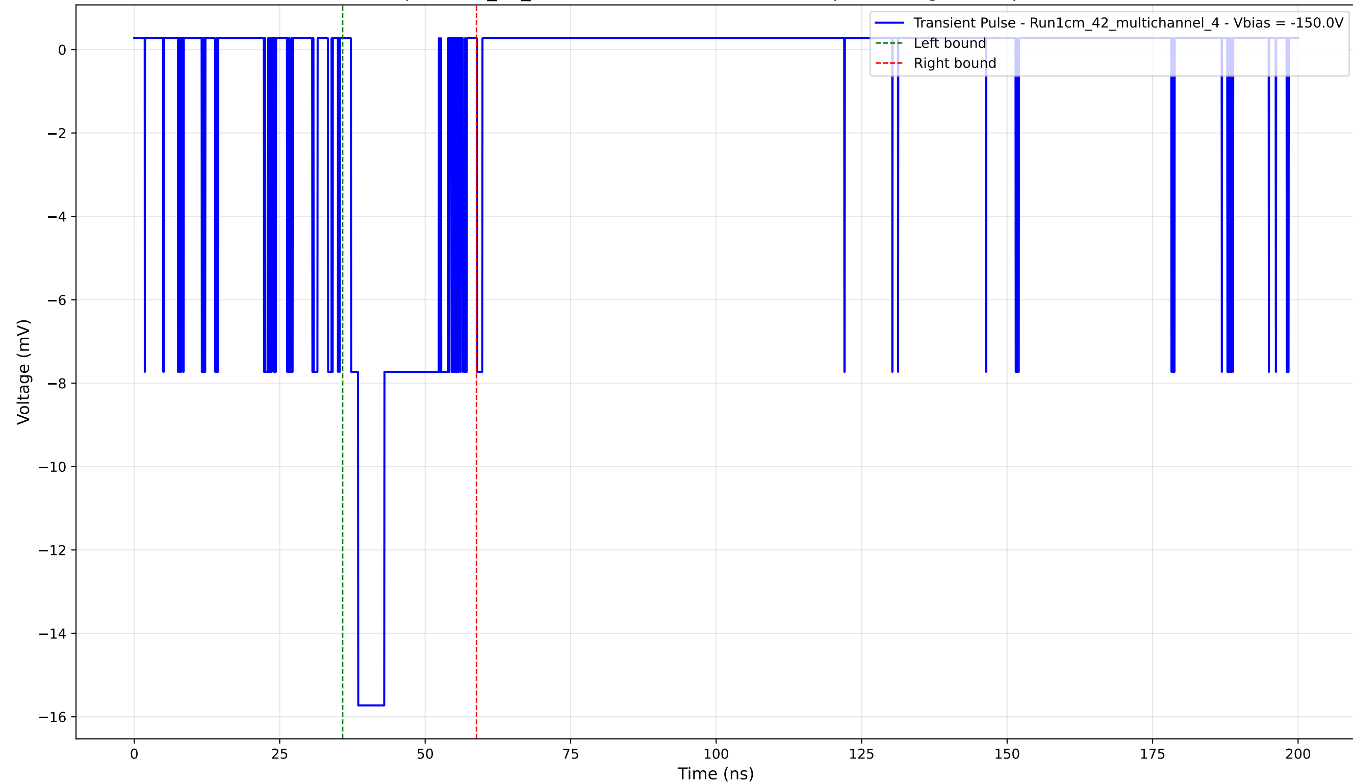
Transient Pulse - Sample: 1cm_42_multichannel - Position: 4280.0 \mu\text{m} - Charge: 3.46 pC - Rise Time: 1.24 ns
