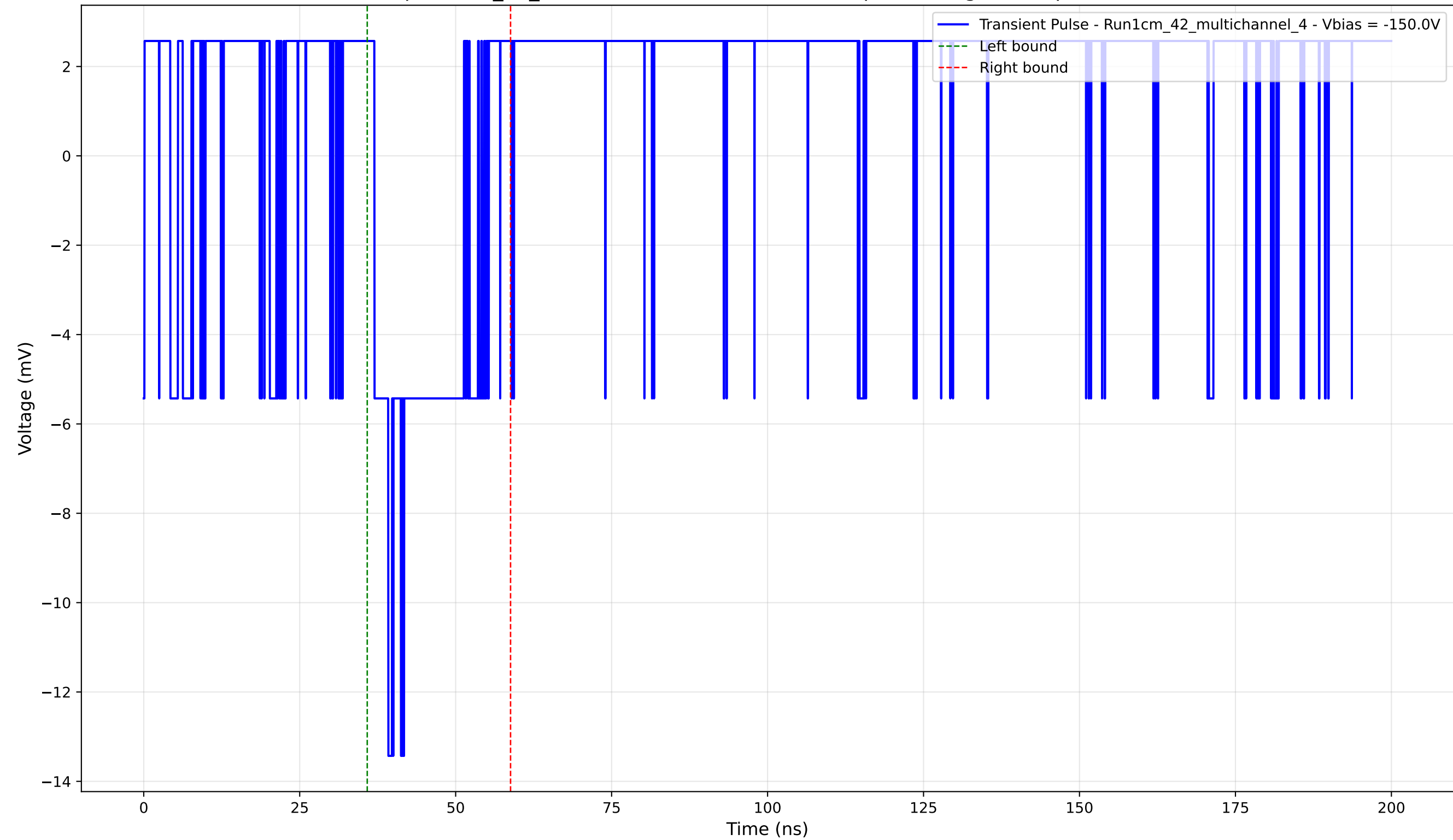
Transient Pulse - Sample: 1cm_42_multichannel - Position: 4835.0 \mu\text{m} - Charge: 1.70 pC - Rise Time: 0.00 ns (N/A)
