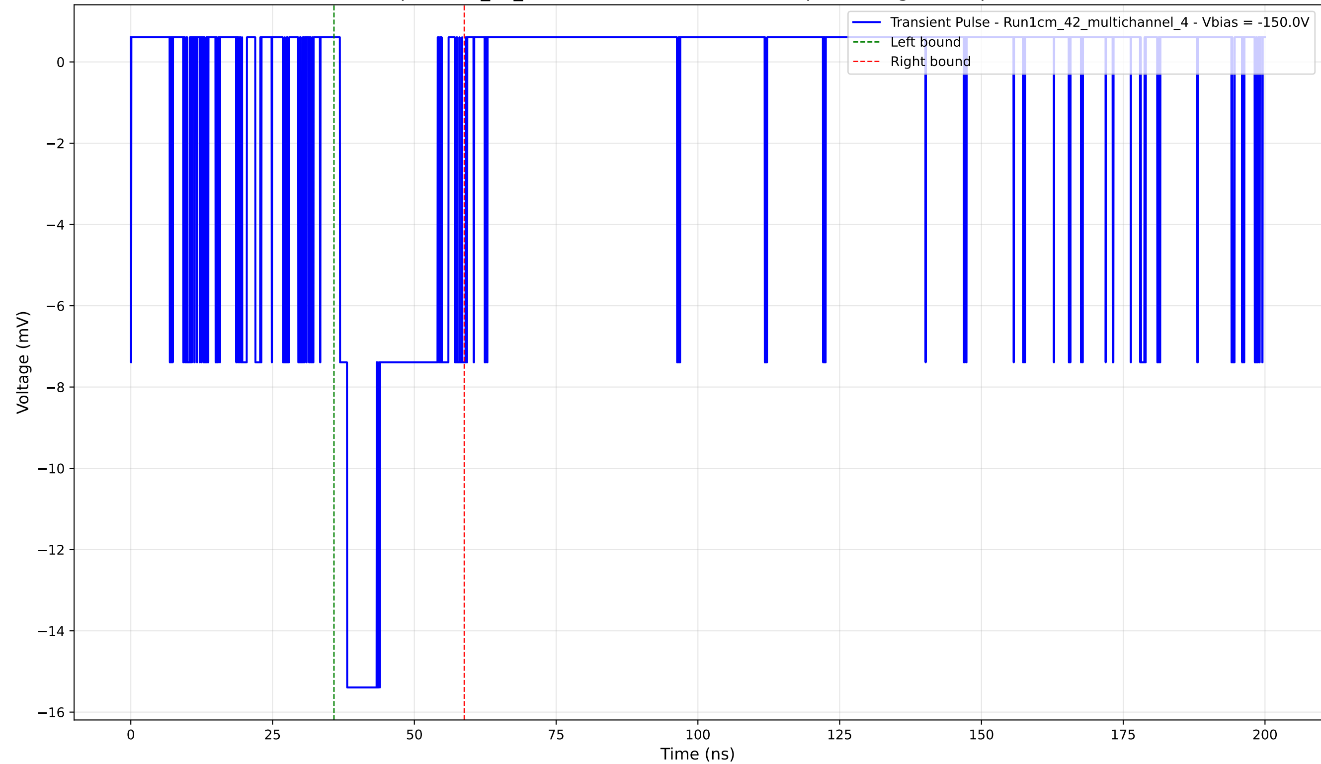
Transient Pulse - Sample: 1cm_42_multichannel - Position: 455.0 \mu\text{m} - Charge: 3.83 pC - Rise Time: 1.28 ns
