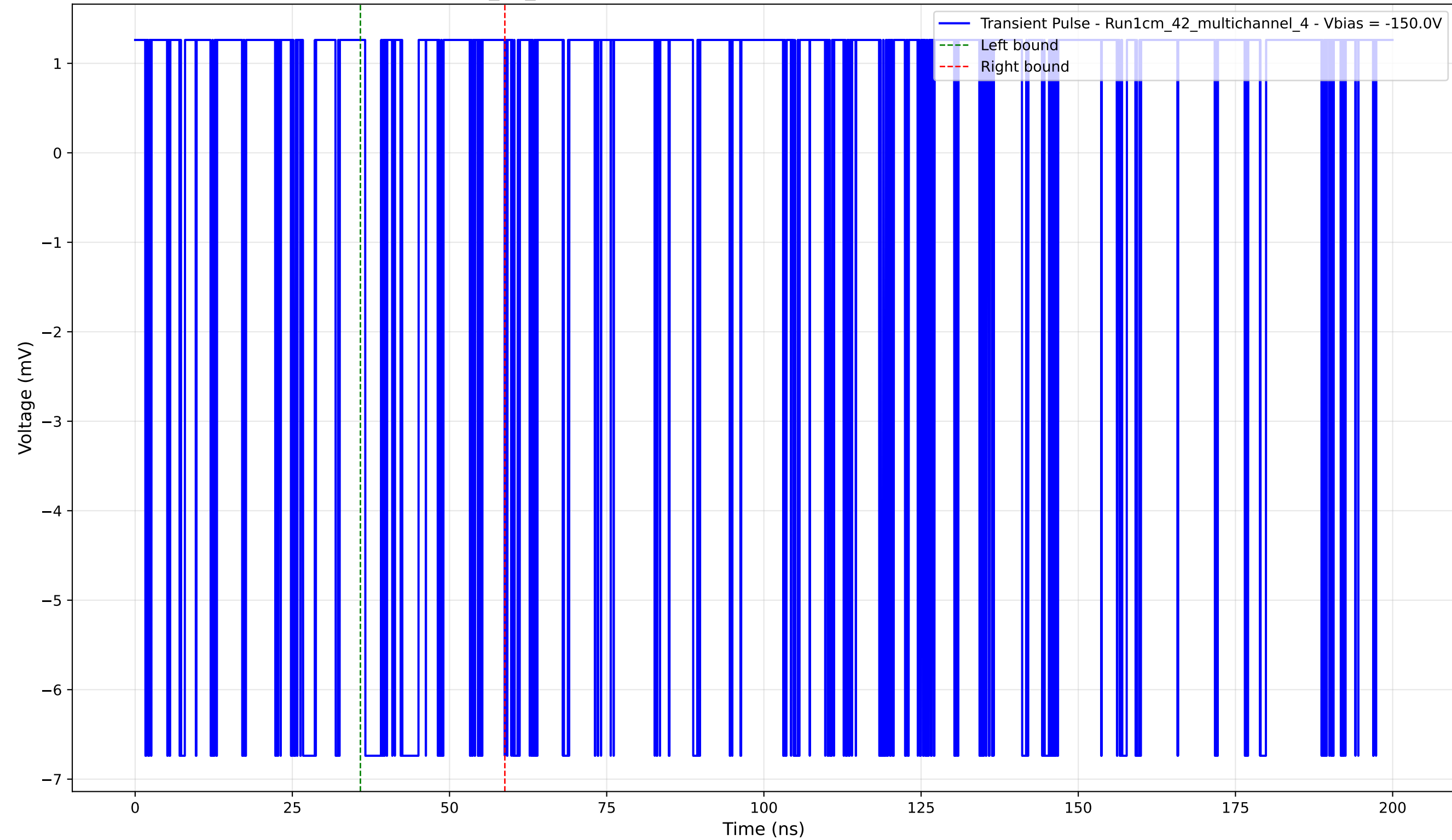
Transient Pulse - Sample: 1cm_42_multichannel - Position: 2390.0 \mu\text{m} - Charge: 0.58 pC - Rise Time: 0.00 ns (N/A)
