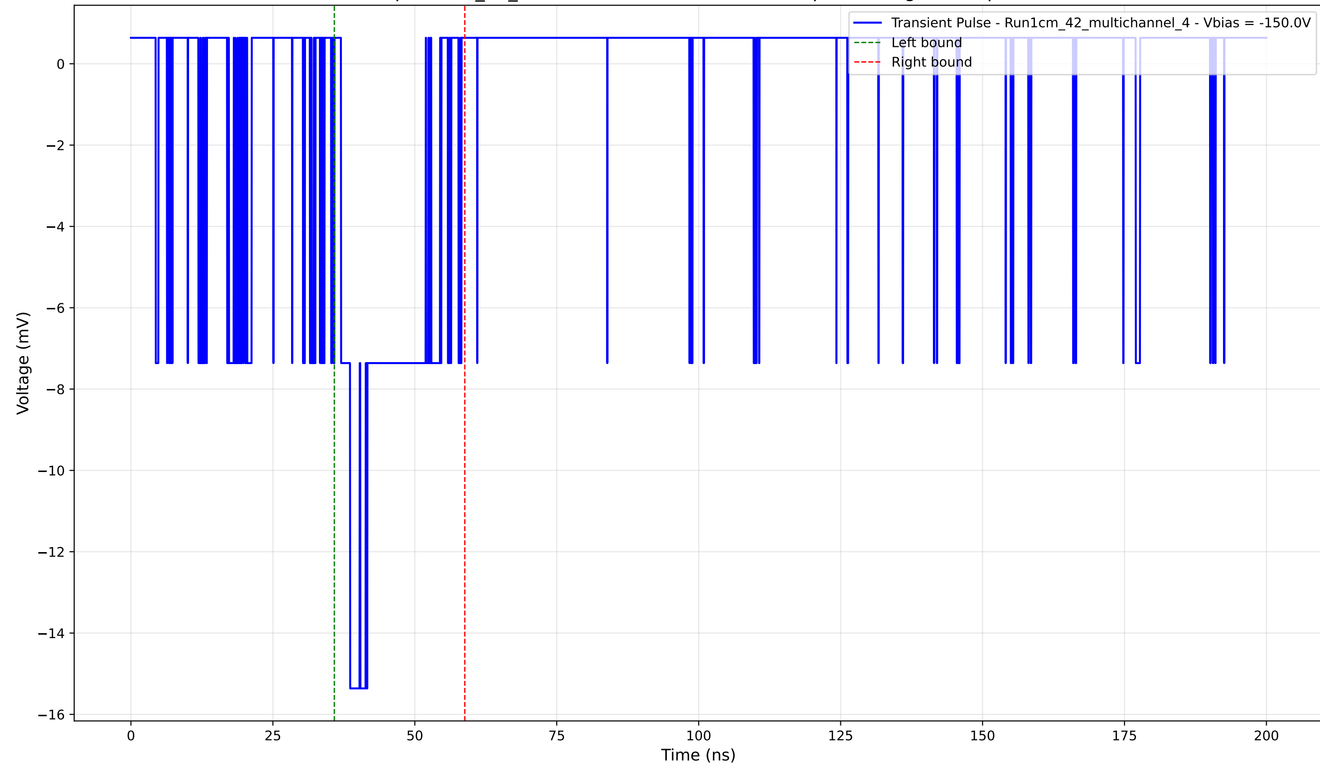
Transient Pulse - Sample: 1cm_42_multichannel - Position: 4780.0 \mu\text{m} - Charge: 3.03 pC - Rise Time: 1.62 ns
