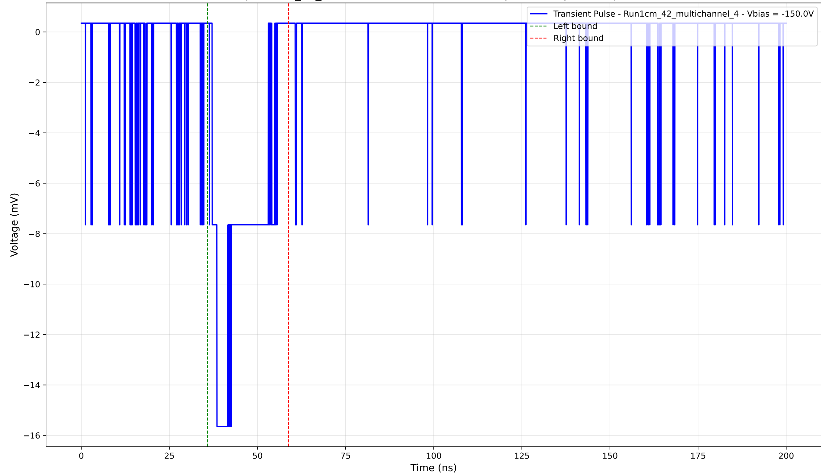
Transient Pulse - Sample: 1cm_42_multichannel - Position: 4665.0 \mu\text{m} - Charge: 3.26 pC - Rise Time: 1.38 ns
