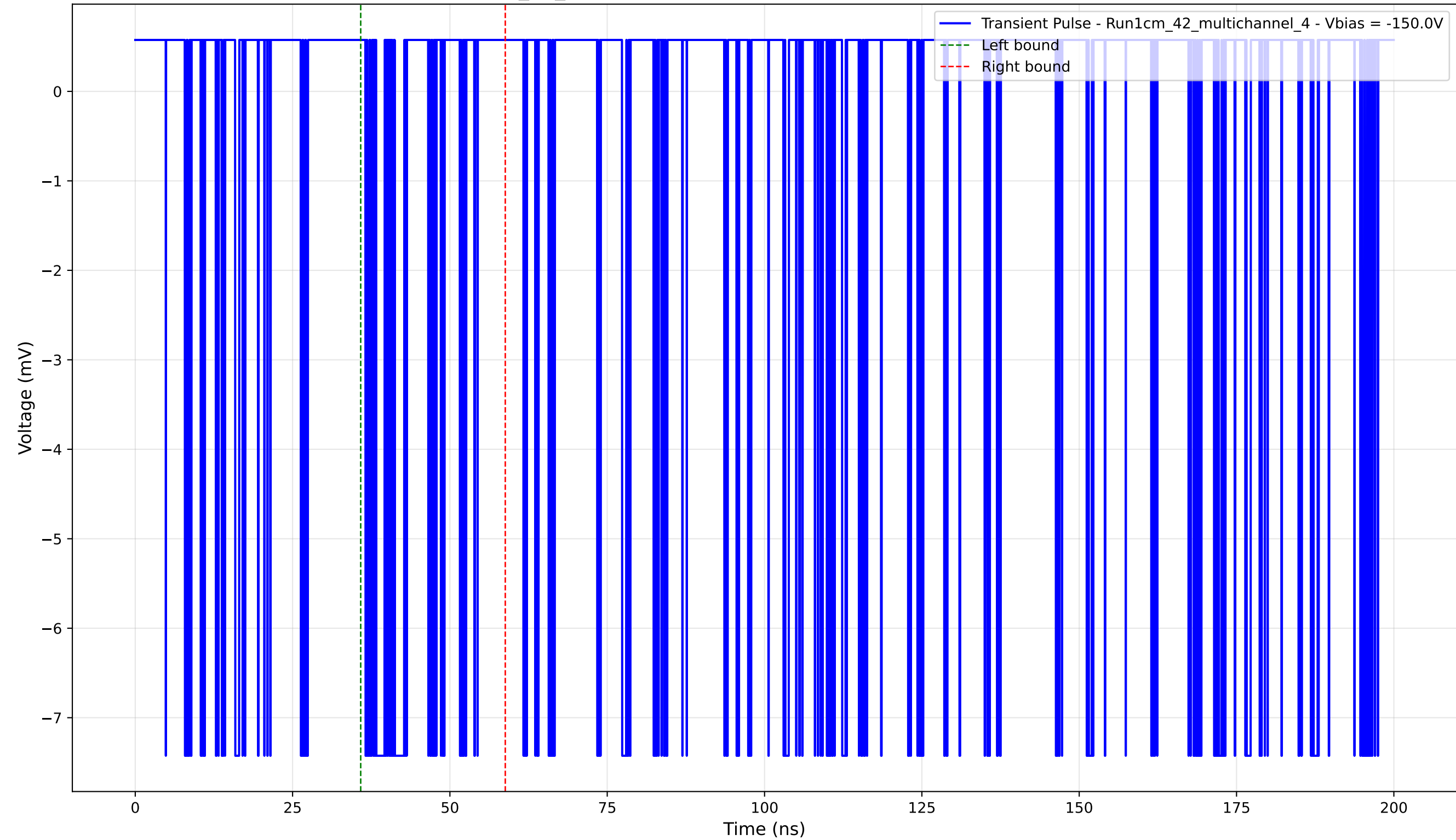
Transient Pulse - Sample: 1cm_42_multichannel - Position: 3390.0 \mu\text{m} - Charge: 0.74 pC - Rise Time: 0.02 ns
