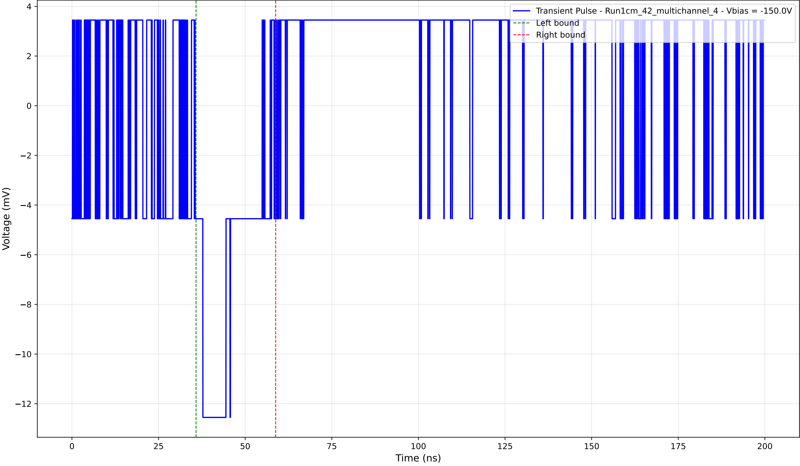
Transient Pulse - Sample: 1cm_42_multichannel - Position: 750.0 \mu\text{m} - Charge: 2.96 pC - Rise Time: 0.00 ns (N/A)
