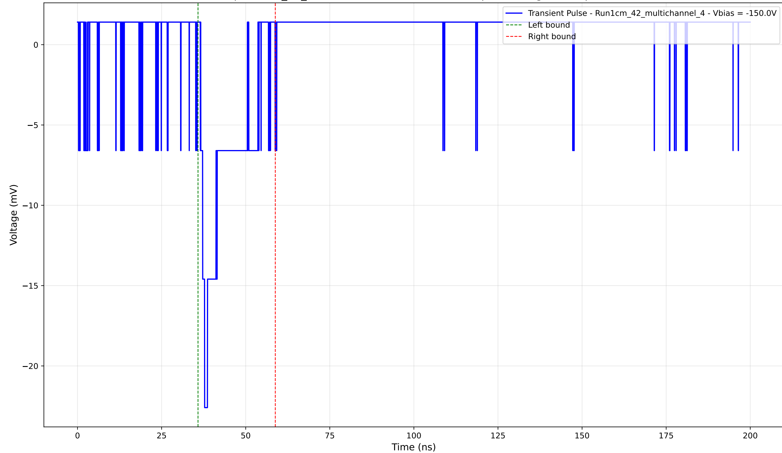
Transient Pulse - Sample: 1cm_42_multichannel - Position: 3335.0 \mu\text{m} - Charge: 2.93 pC - Rise Time: 1.16 ns
