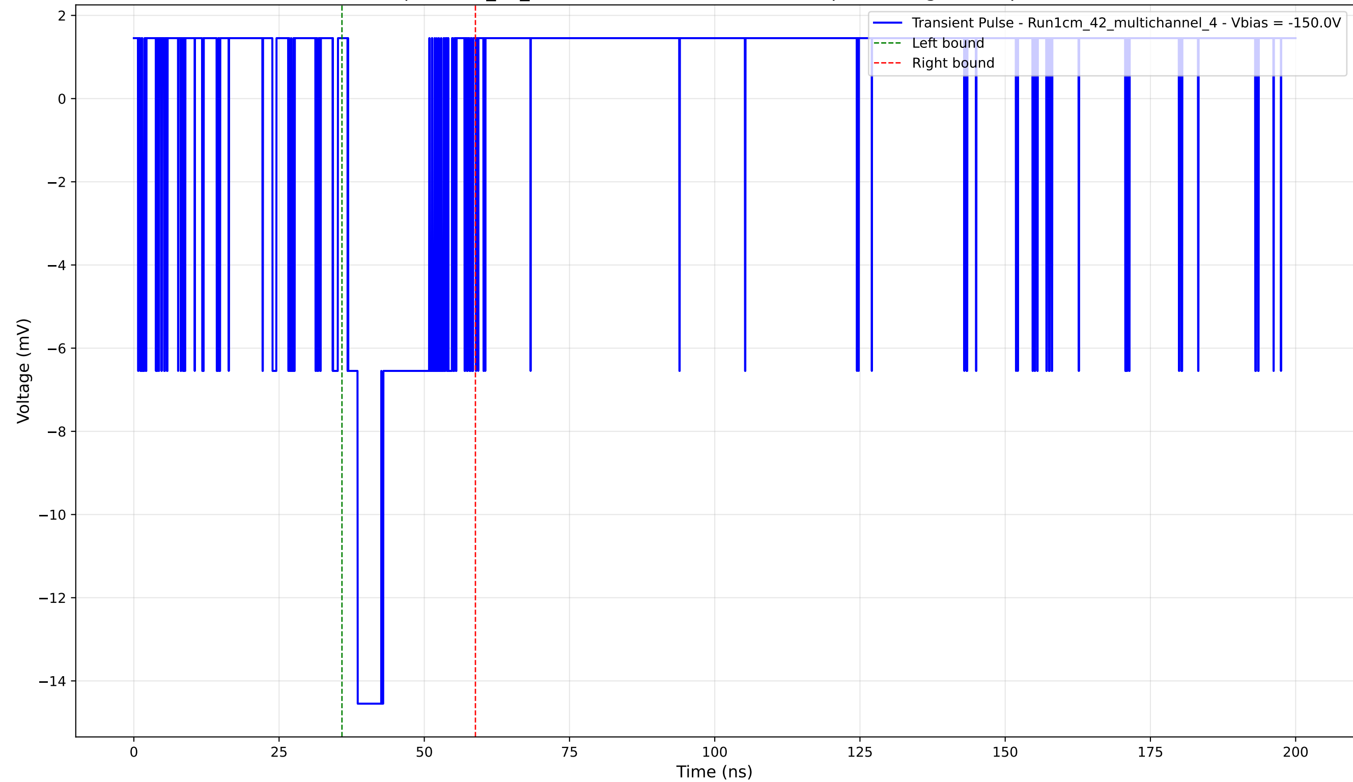
Transient Pulse - Sample: 1cm_42_multichannel - Position: 4655.0 \mu\text{m} - Charge: 2.92 pC - Rise Time: 1.64 ns
