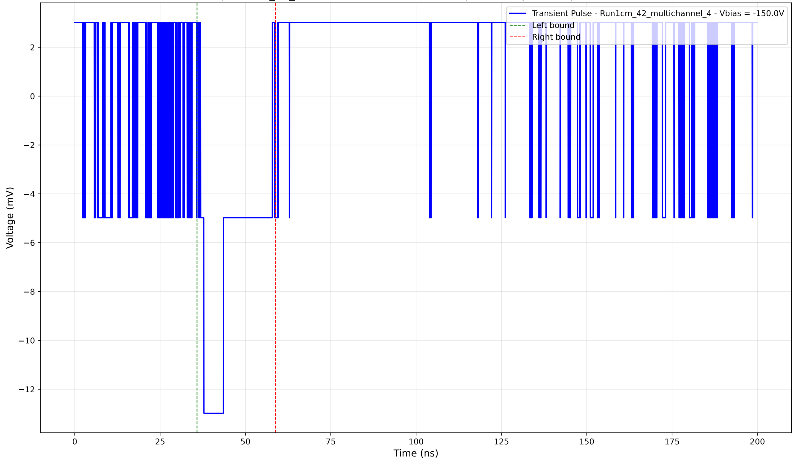
Transient Pulse - Sample: 1cm_42_multichannel - Position: 775.0 \mu\text{m} - Charge: 2.94 pC - Rise Time: 0.00 ns (N/A)
