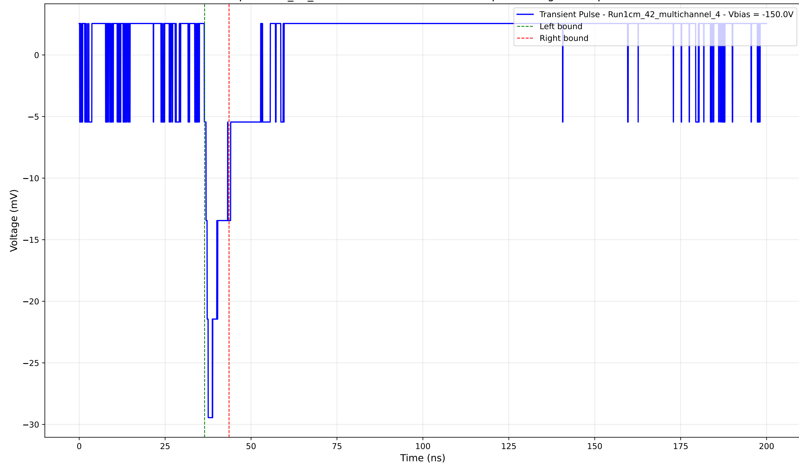
Transient Pulse - Sample: 1cm_42_multichannel - Position: 1500.0 \mu\text{m} - Charge: 2.53 pC - Rise Time: 1.14 ns
