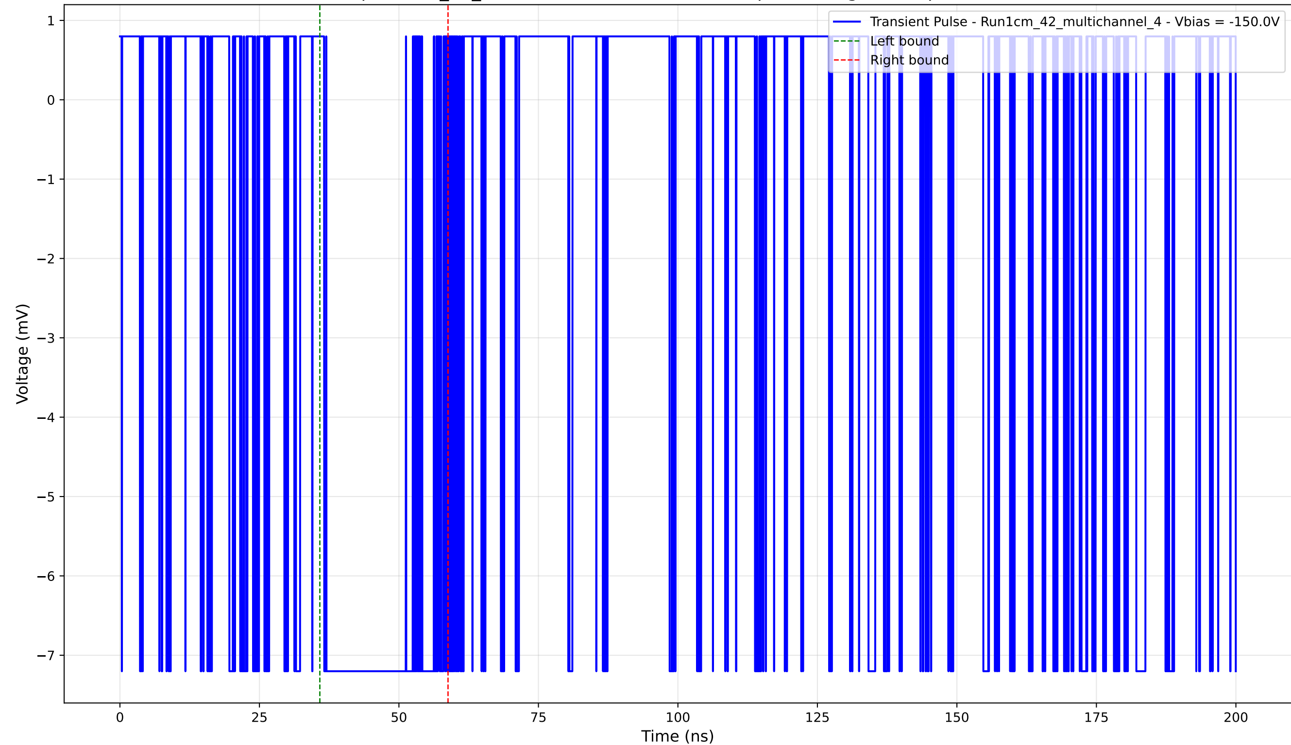
Transient Pulse - Sample: 1cm_42_multichannel - Position: 310.0 \mu\text{m} - Charge: 2.86 pC - Rise Time: 0.00 ns (N/A)
