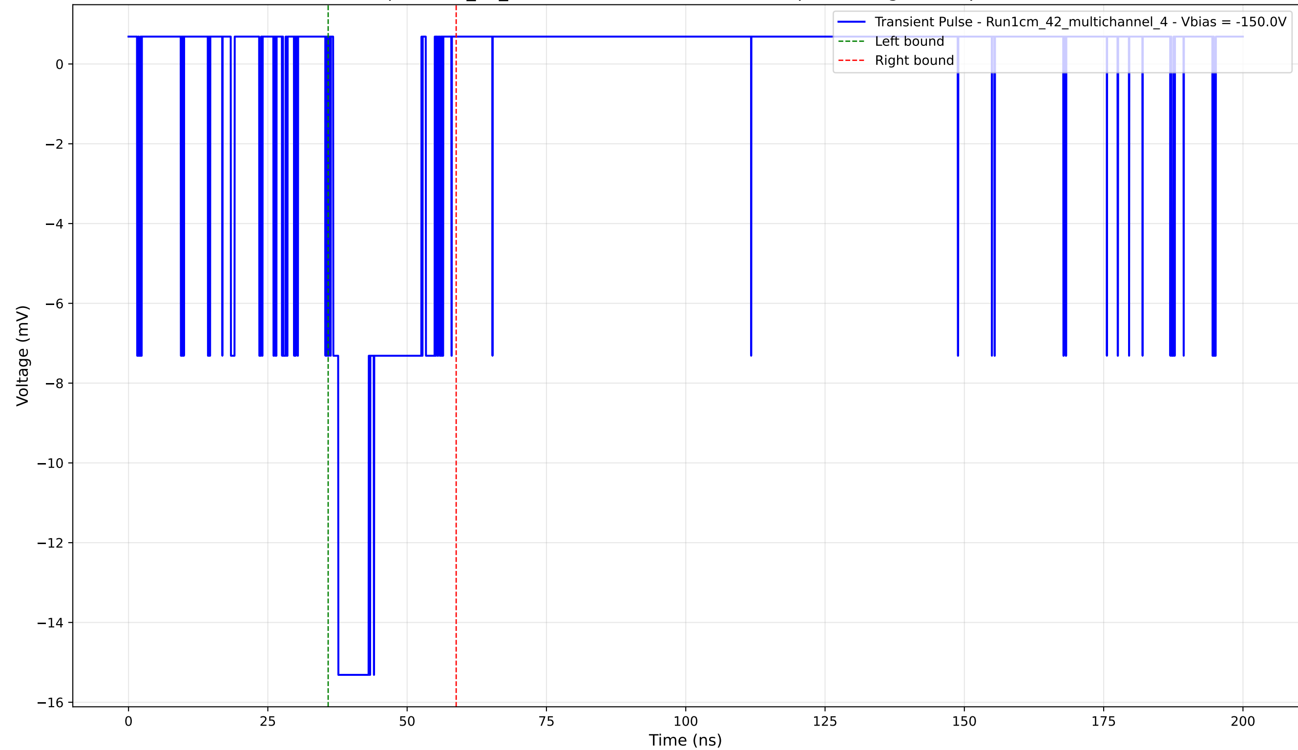
Transient Pulse - Sample: 1cm_42_multichannel - Position: 3765.0 \mu\text{m} - Charge: 3.57 pC - Rise Time: 0.92 ns
