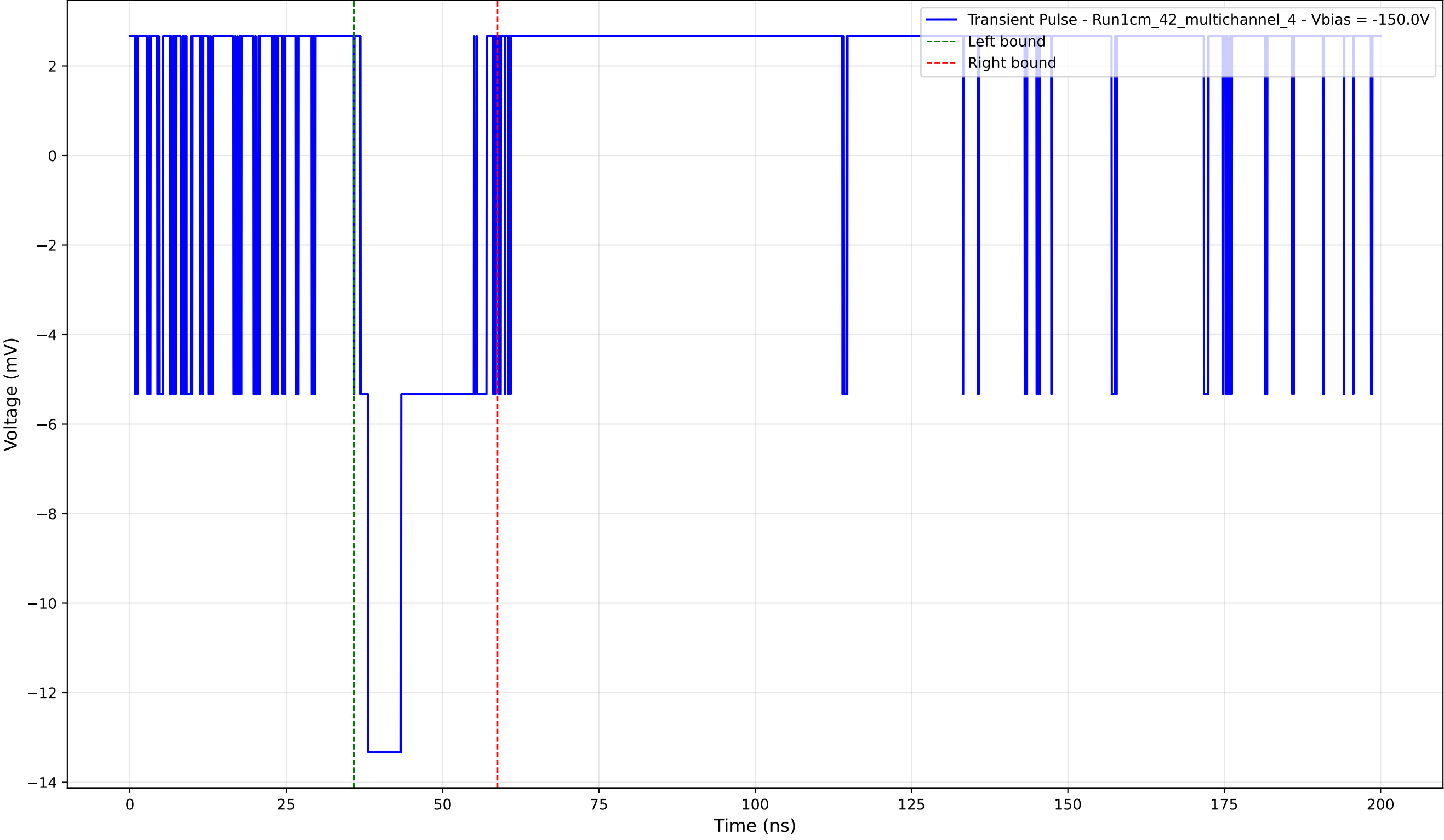
Transient Pulse - Sample: 1cm_42_multichannel - Position: 495.0 \mu\text{m} - Charge: 2.85 pC - Rise Time: 0.00 ns (N/A)
