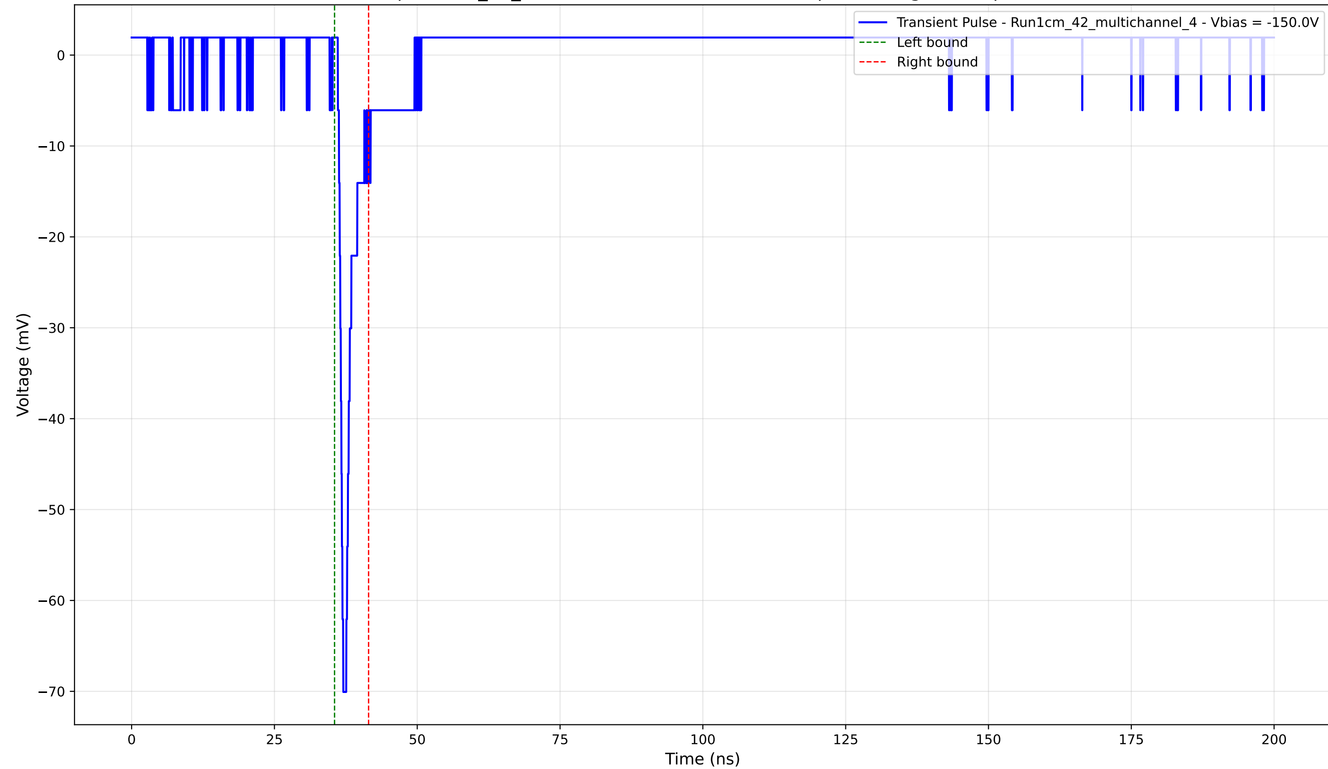
Transient Pulse - Sample: 1cm_42_multichannel - Position: 2540.0 \mu\text{m} - Charge: 3.09 pC - Rise Time: 0.76 ns
