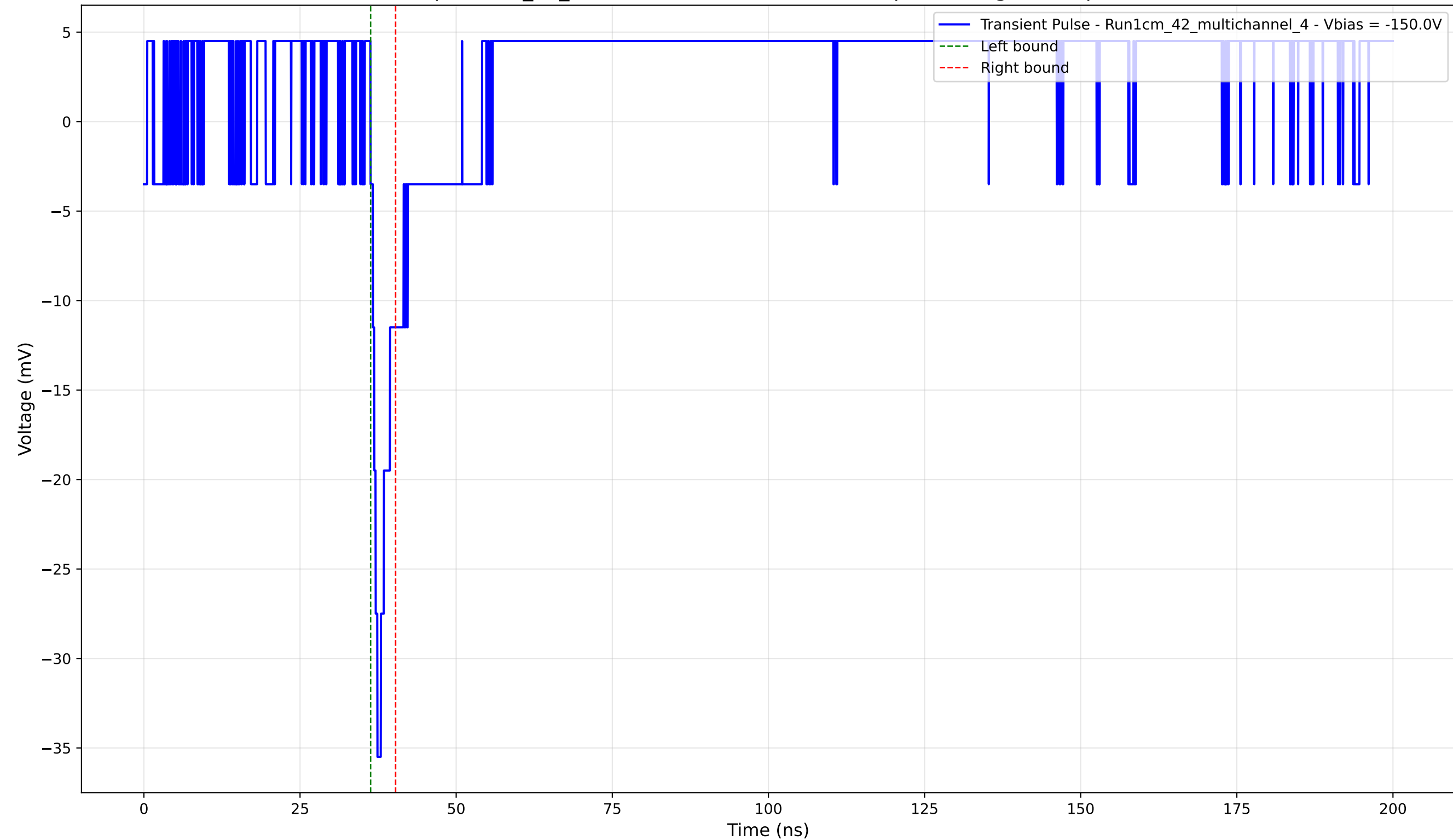
Transient Pulse - Sample: 1cm_42_multichannel - Position: 1810.0 \mu\text{m} - Charge: 1.57 pC - Rise Time: 0.74 ns
