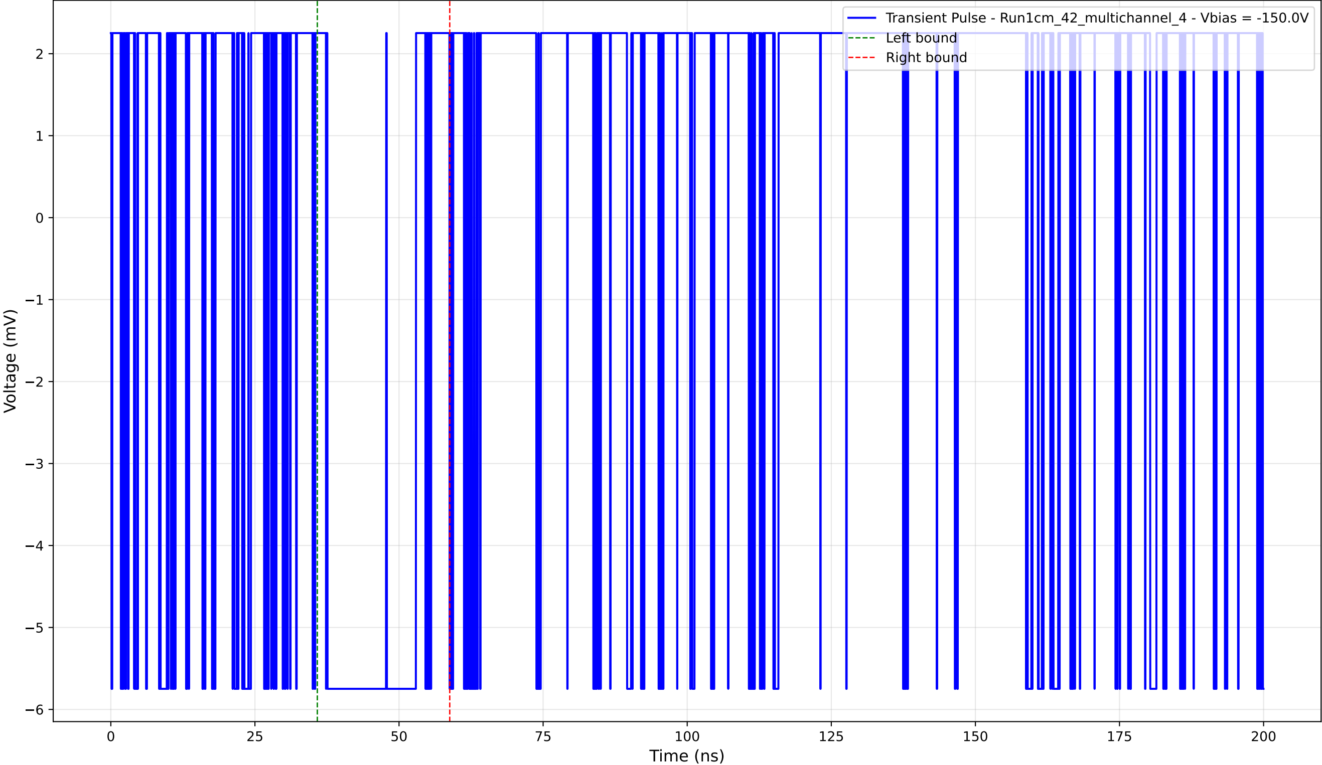
Transient Pulse - Sample: 1cm_42_multichannel - Position: 4360.0 \mu\text{m} - Charge: 1.49 pC - Rise Time: 0.00 ns (N/A)
