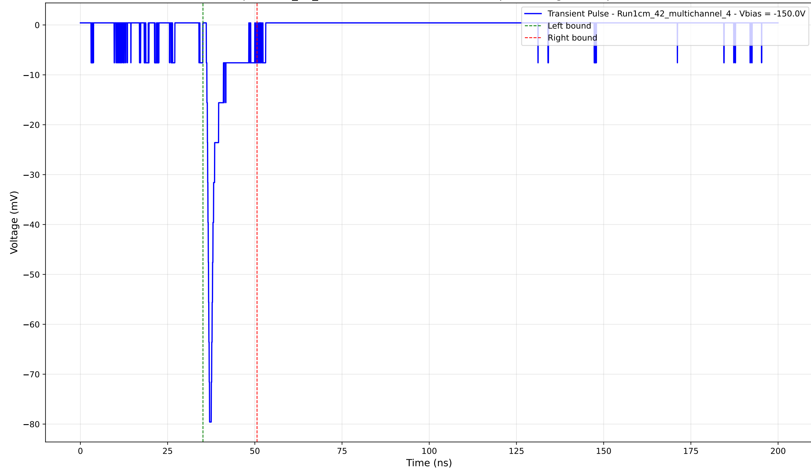
Transient Pulse - Sample: 1cm_42_multichannel - Position: 2280.0 \mu\text{m} - Charge: 4.73 pC - Rise Time: 0.78 ns
