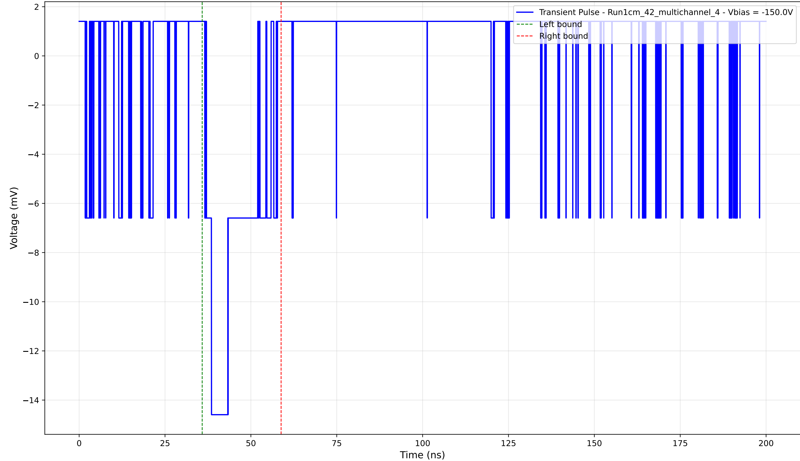
Transient Pulse - Sample: 1cm_42_multichannel - Position: 4625.0 \mu\text{m} - Charge: 3.21 pC - Rise Time: 1.48 ns
