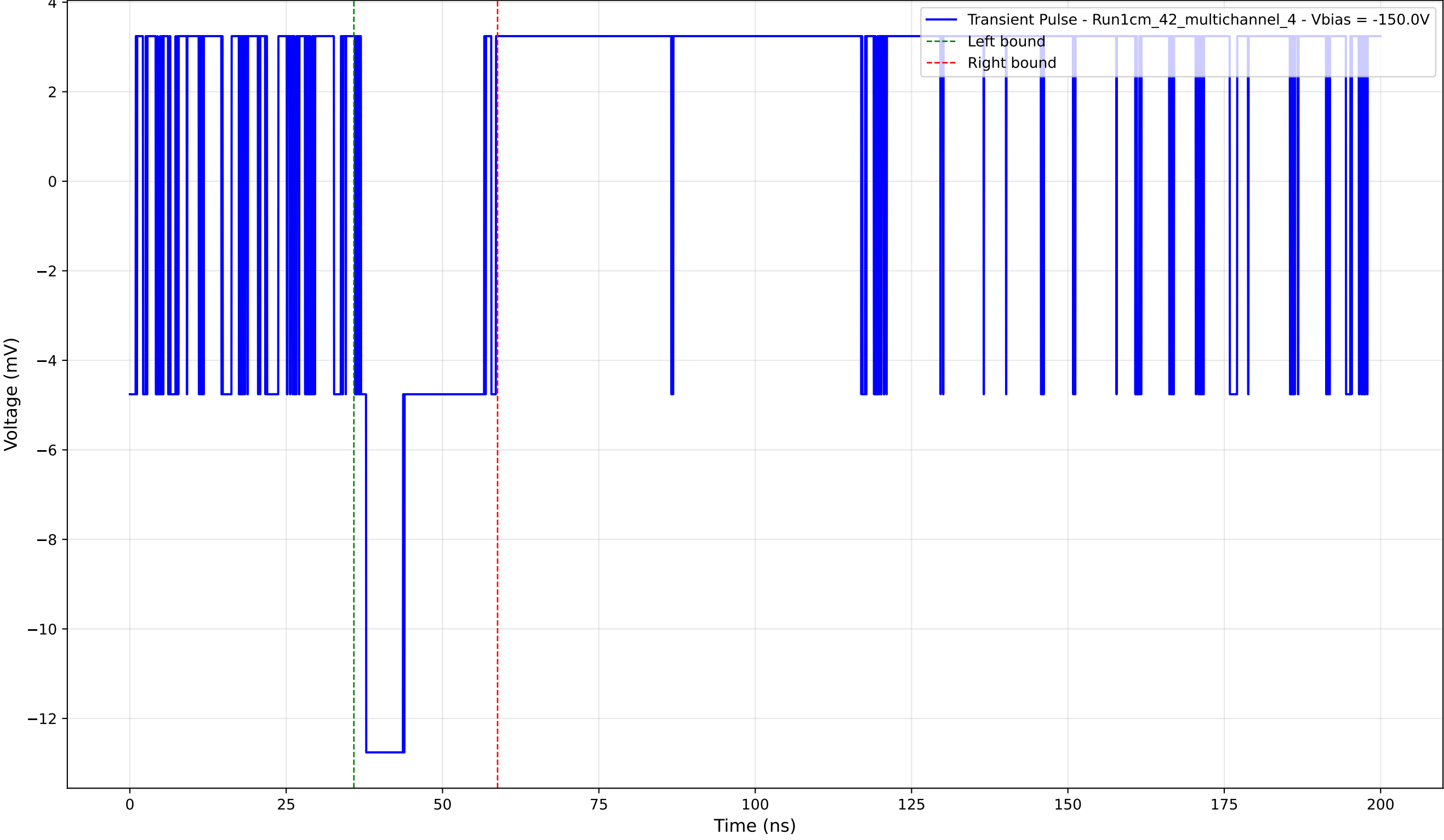
Transient Pulse - Sample: 1cm_42_multichannel - Position: 650.0 \mu\text{m} - Charge: 2.80 pC - Rise Time: 0.00 ns (N/A)
