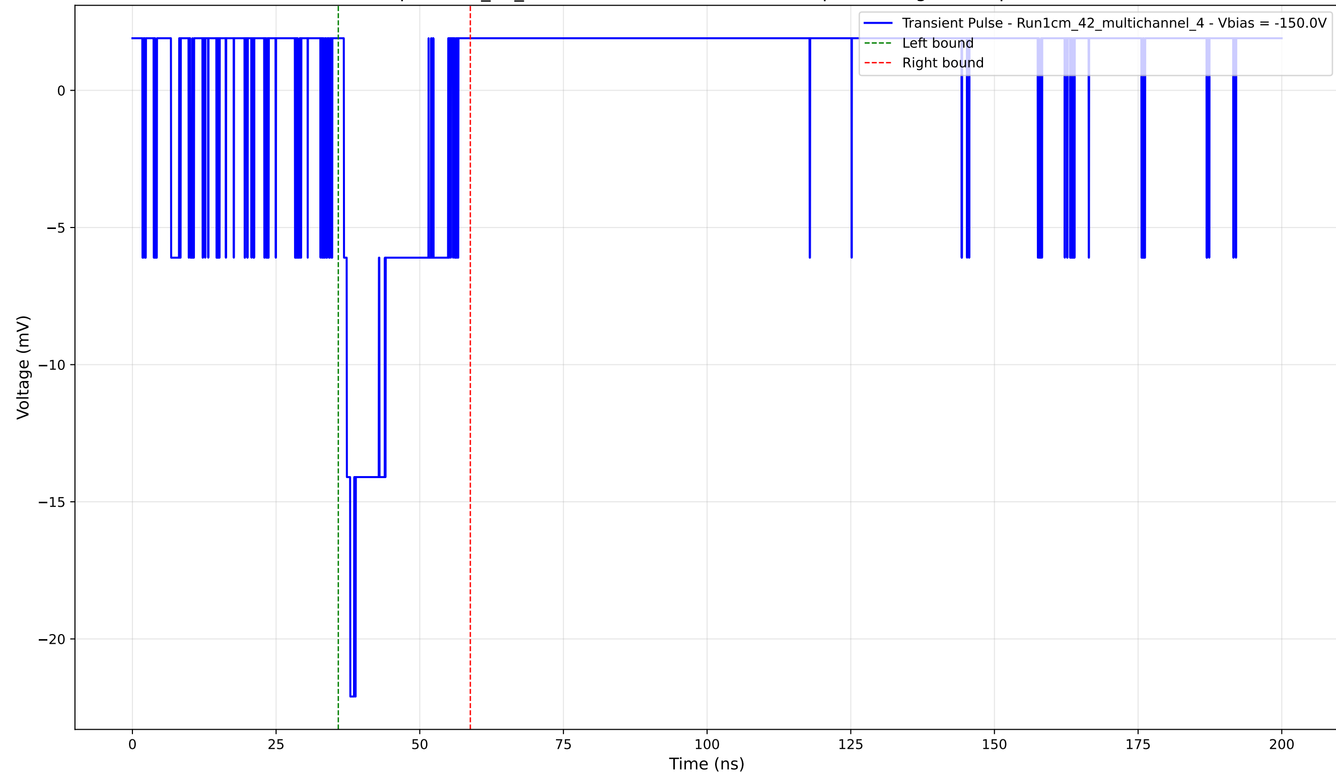
Transient Pulse - Sample: 1cm_42_multichannel - Position: 3575.0 \mu\text{m} - Charge: 3.27 pC - Rise Time: 1.12 ns
