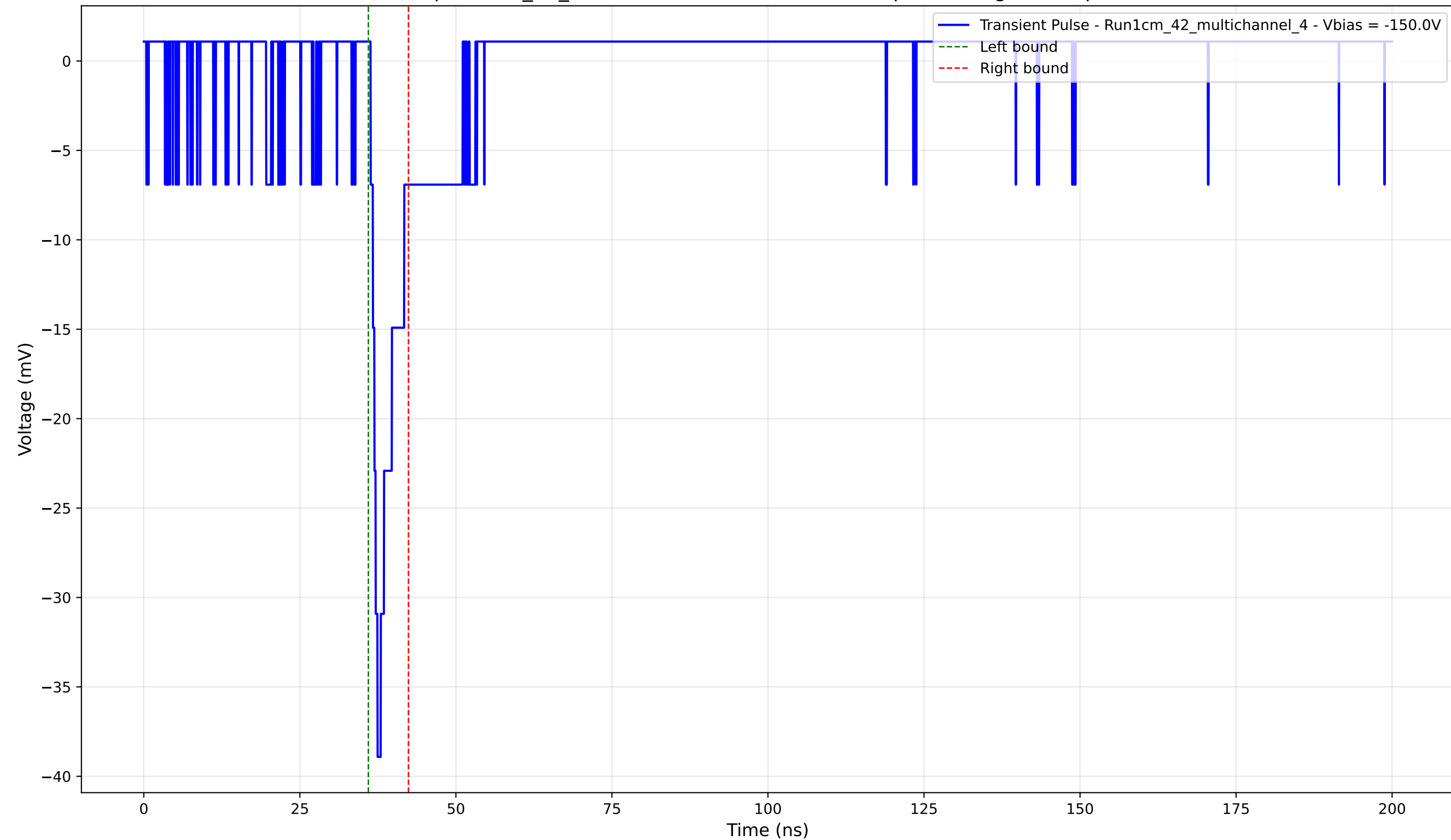
Transient Pulse - Sample: 1cm_42_multichannel - Position: 3015.0 \mu\text{m} - Charge: 2.38 pC - Rise Time: 1.11 ns
