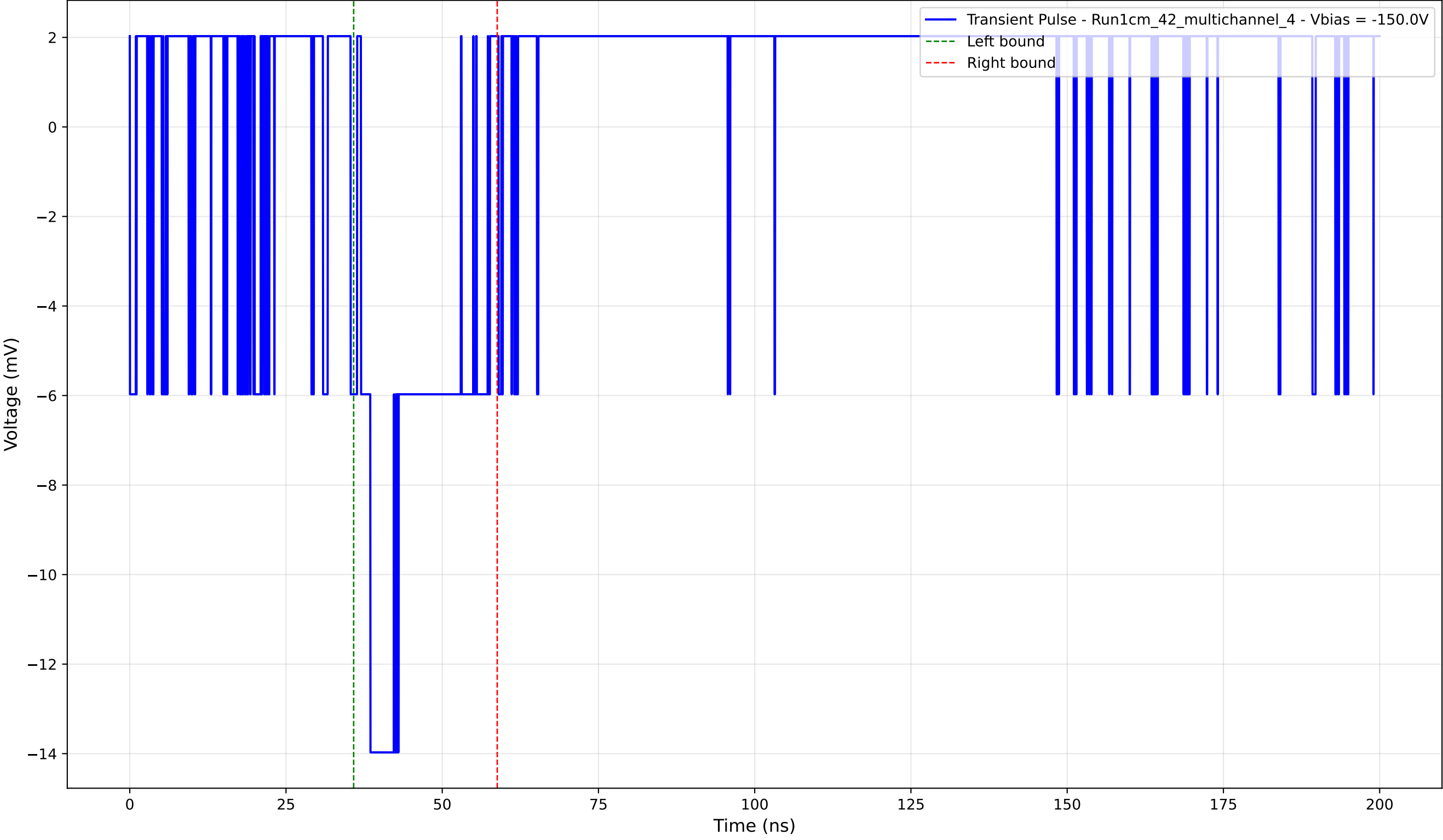
Transient Pulse - Sample: 1cm_42_multichannel - Position: 280.0 \mu\text{m} - Charge: 3.06 pC - Rise Time: 0.00 ns (N/A)
