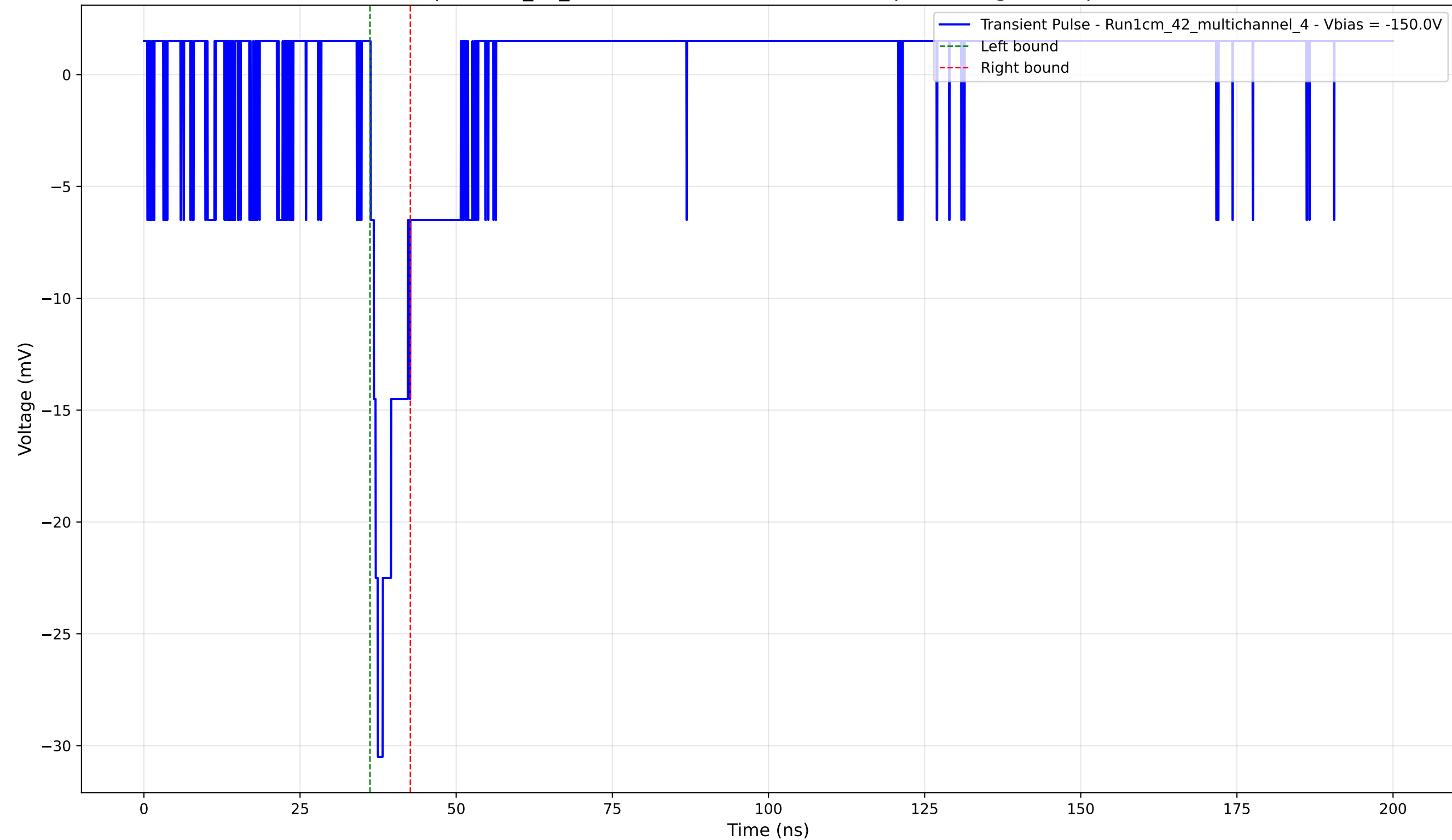
Transient Pulse - Sample: 1cm_42_multichannel - Position: 3145.0 \mu\text{m} - Charge: 2.24 pC - Rise Time: 1.15 ns
