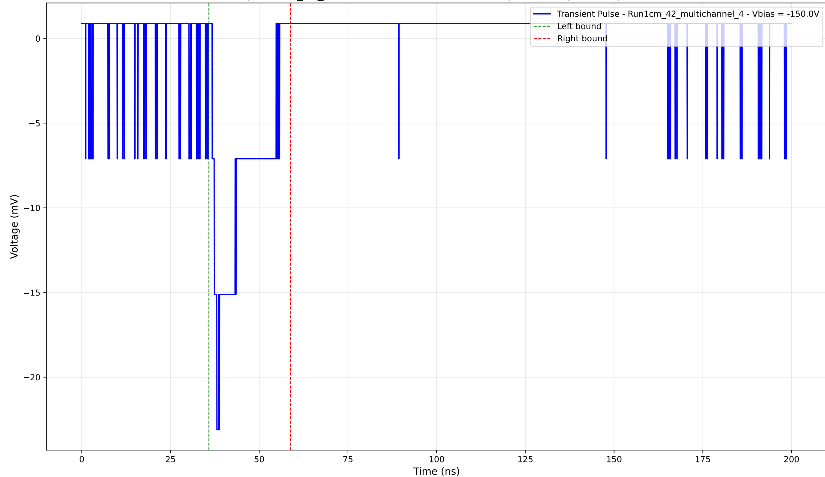
Transient Pulse - Sample: 1cm_42_multichannel - Position: 3635.0 \mu\text{m} - Charge: 3.60 pC - Rise Time: 1.34 ns
