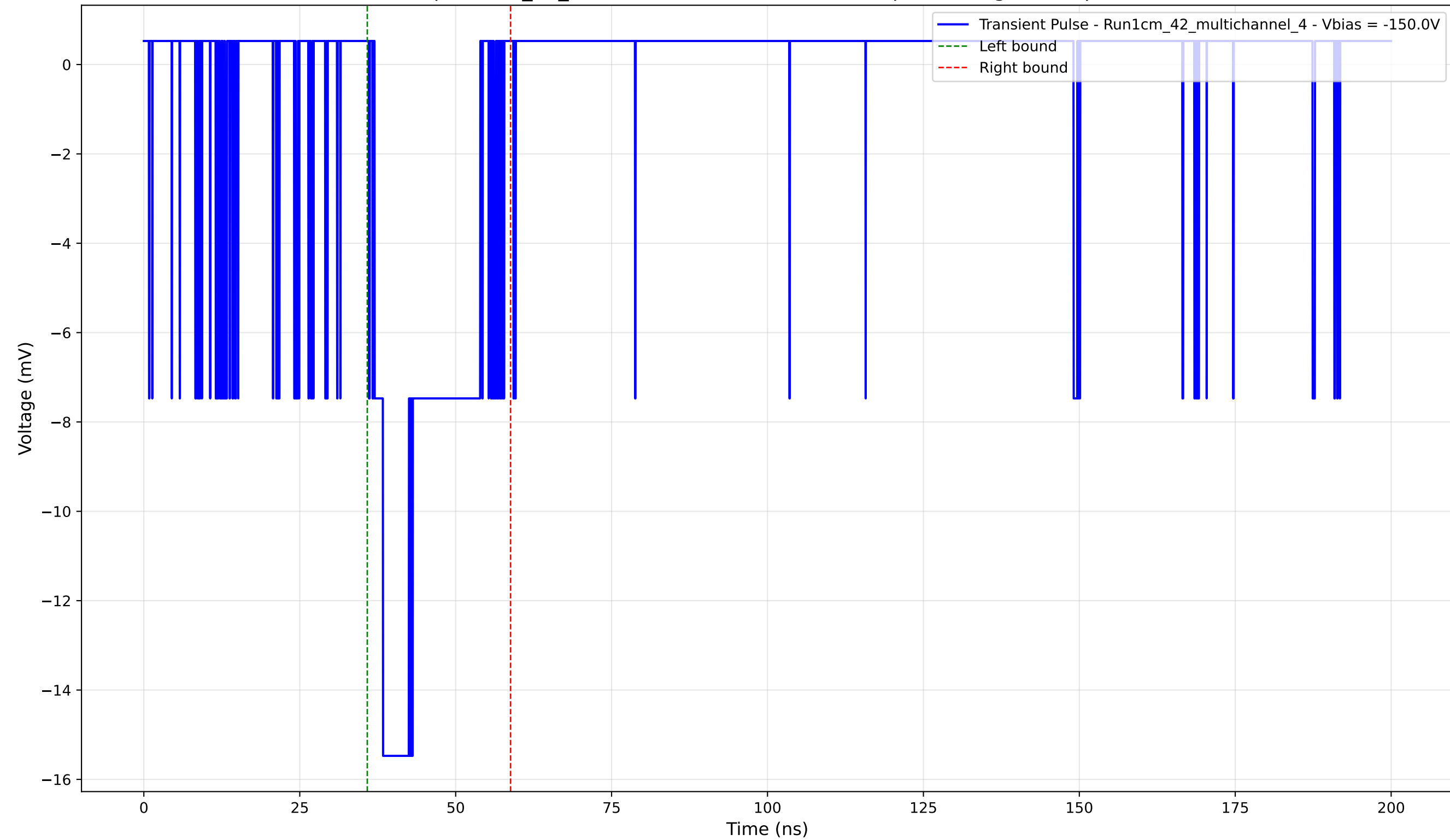
Transient Pulse - Sample: 1cm_42_multichannel - Position: 4200.0 \mu\text{m} - Charge: 3.41 pC - Rise Time: 1.36 ns
