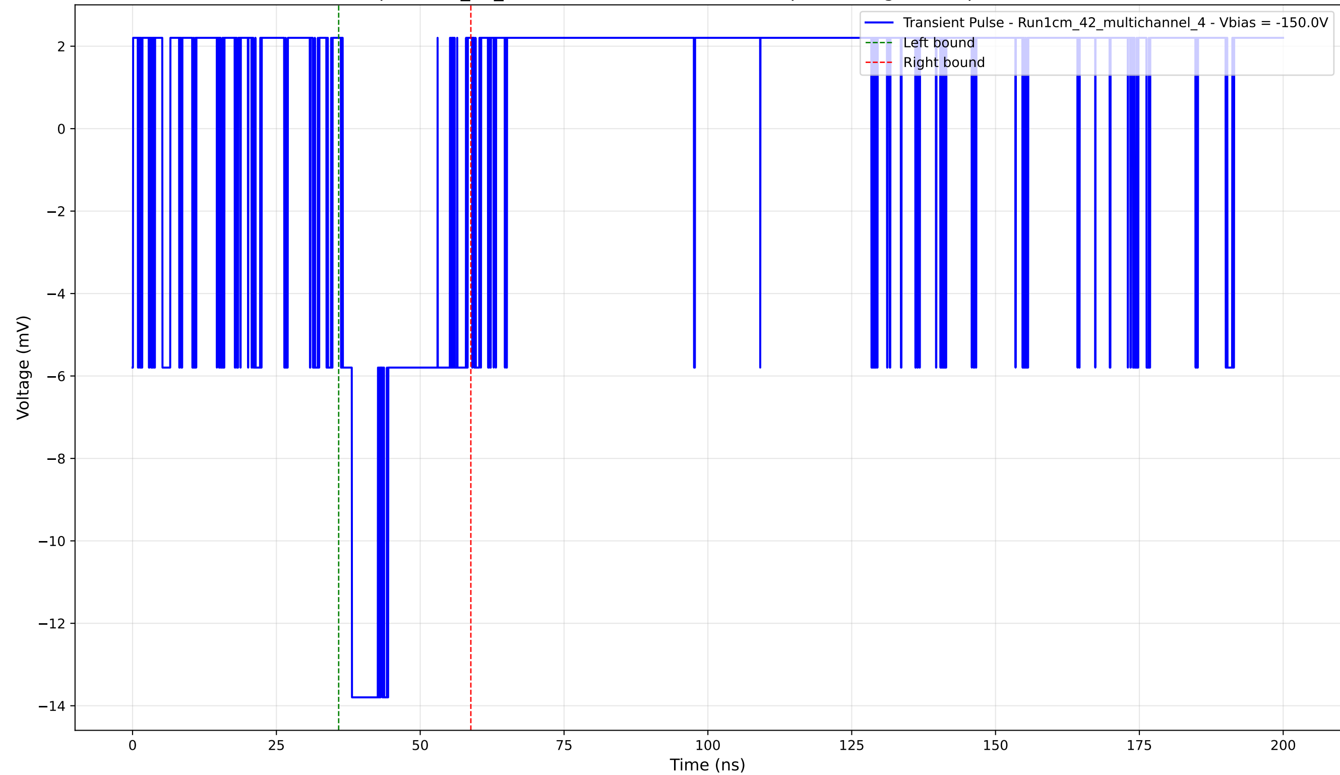
Transient Pulse - Sample: 1cm_42_multichannel - Position: 480.0 \mu\text{m} - Charge: 3.30 pC - Rise Time: 0.00 ns (N/A)
