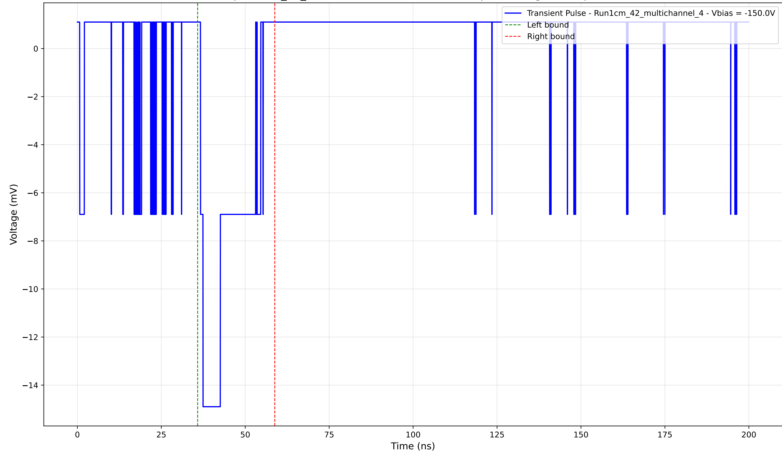
Transient Pulse - Sample: 1cm_42_multichannel - Position: 3630.0 \mu\text{m} - Charge: 3.18 pC - Rise Time: 0.76 ns
