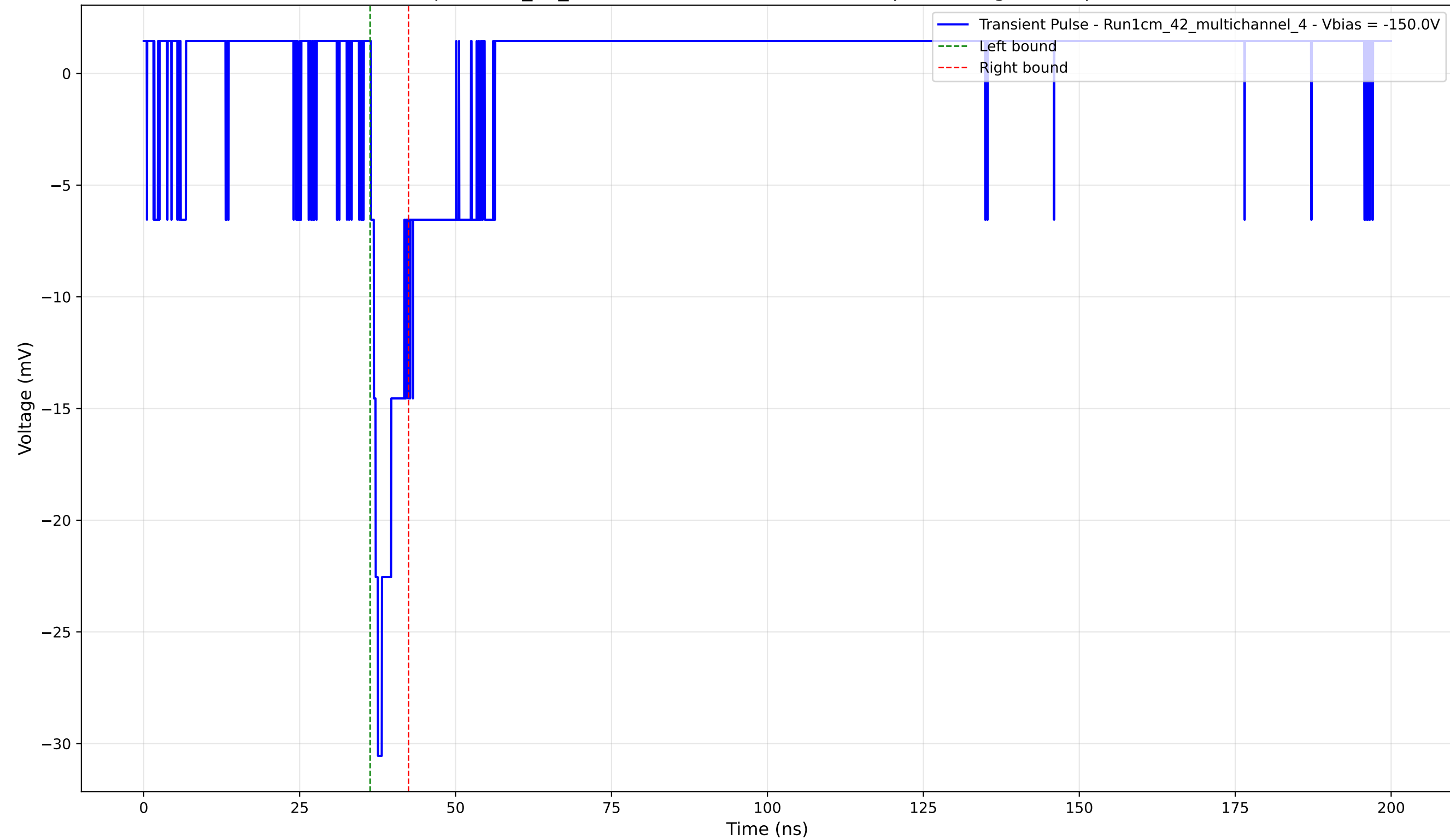
Transient Pulse - Sample: 1cm_42_multichannel - Position: 3195.0 \mu\text{m} - Charge: 2.11 pC - Rise Time: 1.11 ns
