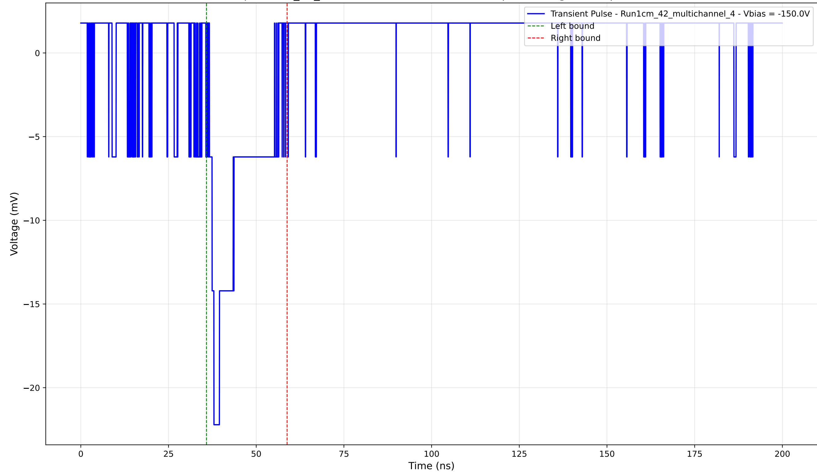
Transient Pulse - Sample: 1cm_42_multichannel - Position: 1145.0 \mu\text{m} - Charge: 3.64 pC - Rise Time: 1.30 ns
