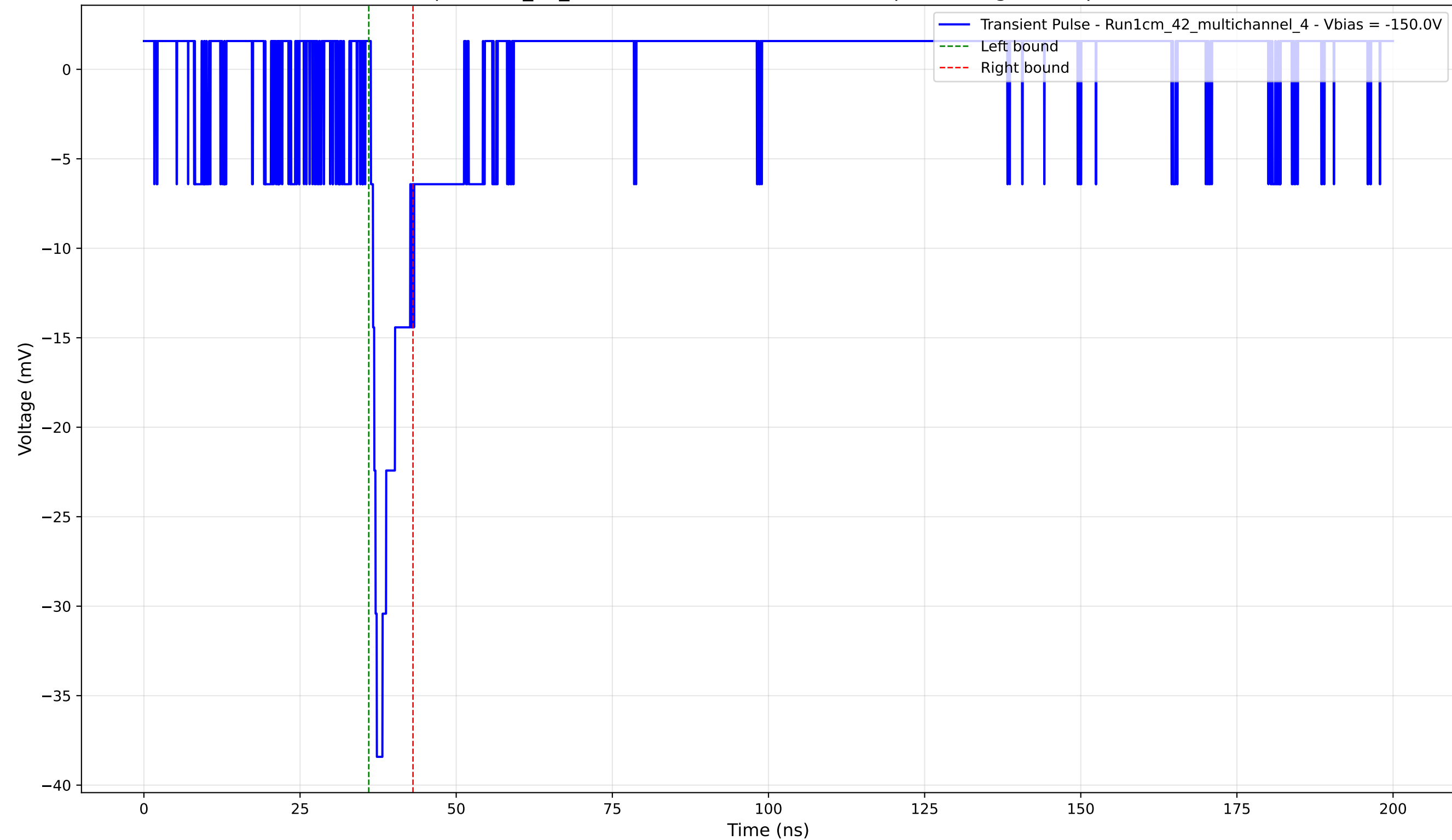
Transient Pulse - Sample: 1cm_42_multichannel - Position: 1745.0 \mu\text{m} - Charge: 2.79 pC - Rise Time: 0.95 ns
