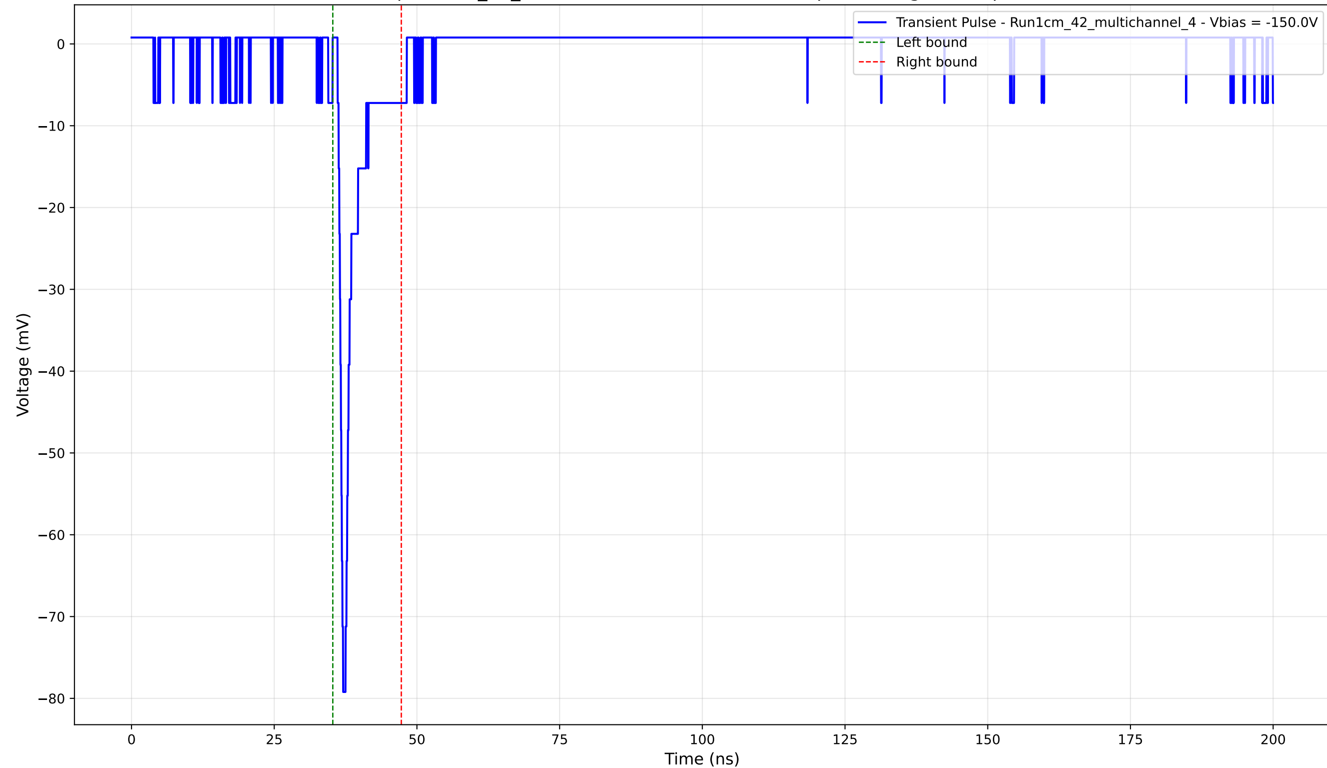
Transient Pulse - Sample: 1cm_42_multichannel - Position: 2515.0 \mu\text{m} - Charge: 4.21 pC - Rise Time: 0.80 ns
