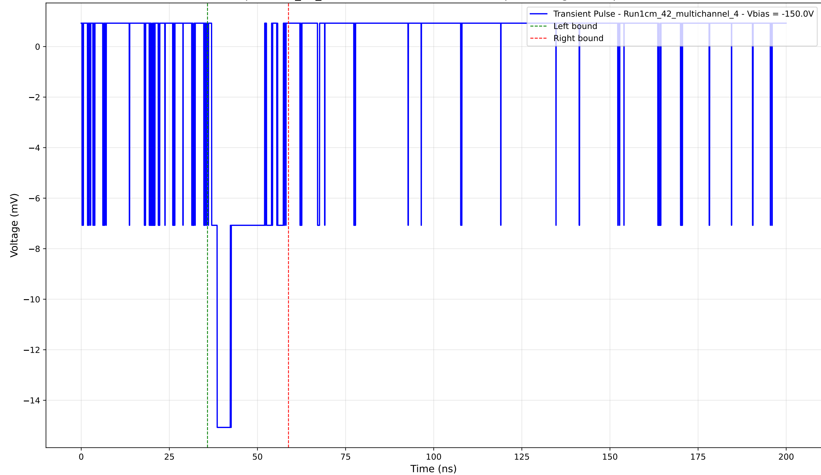
Transient Pulse - Sample: 1cm_42_multichannel - Position: 4610.0 \mu\text{m} - Charge: 3.22 pC - Rise Time: 1.58 ns
