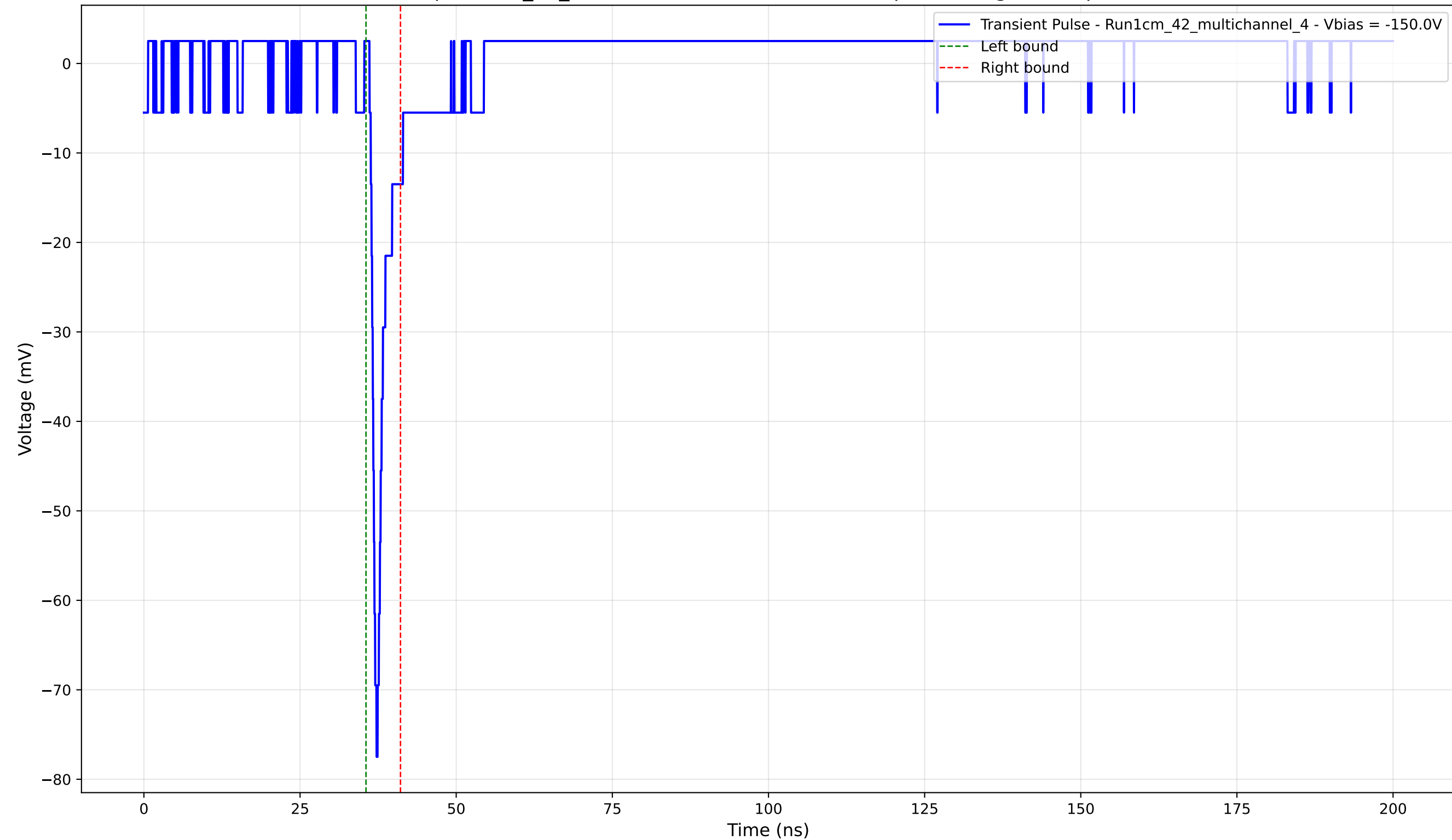
Transient Pulse - Sample: 1cm_42_multichannel - Position: 2210.0 \mu\text{m} - Charge: 3.06 pC - Rise Time: 0.93 ns
