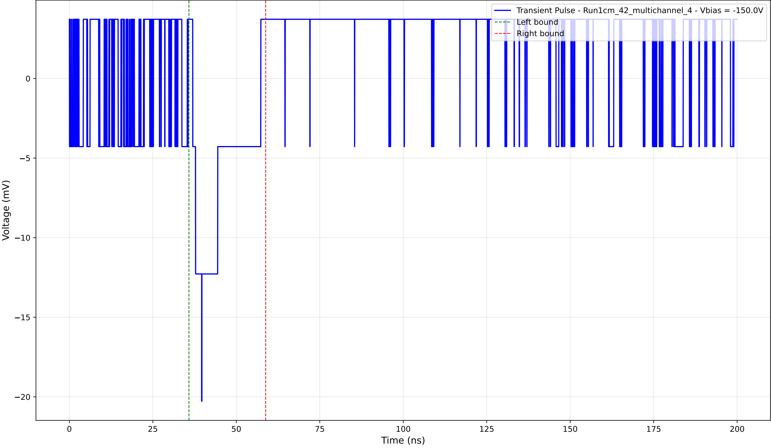
Transient Pulse - Sample: 1cm_42_multichannel - Position: 720.0 \mu\text{m} - Charge: 2.62 pC - Rise Time: 0.00 ns (N/A)
