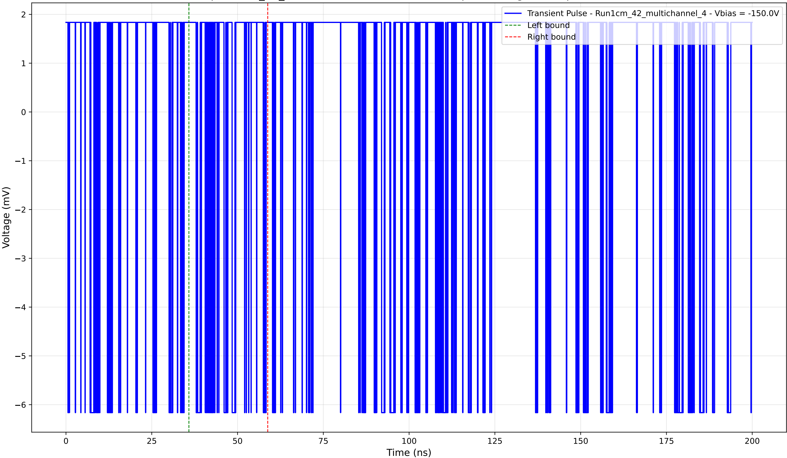
Transient Pulse - Sample: 1cm_42_multichannel - Position: 3415.0 \mu\text{m} - Charge: 0.03 pC - Rise Time: 0.00 ns (N/A)
