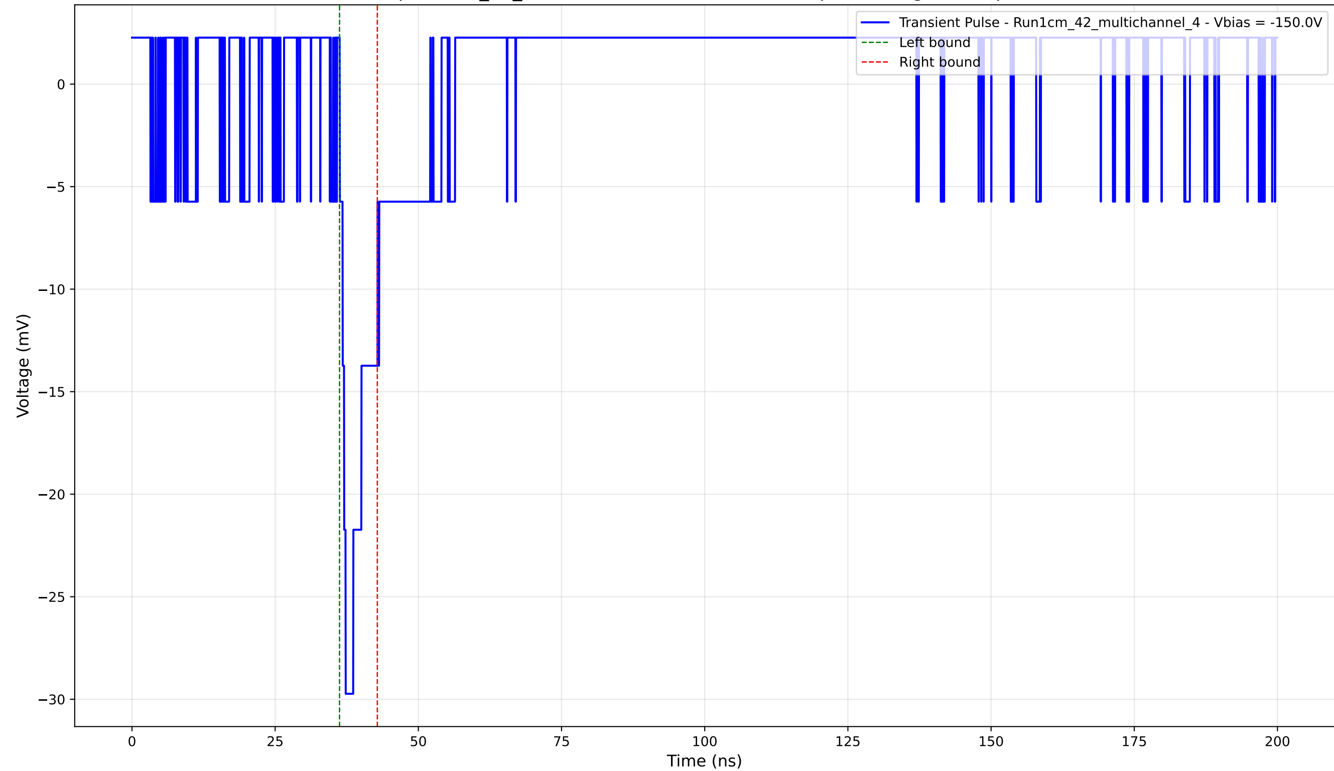
Transient Pulse - Sample: 1cm_42_multichannel - Position: 1635.0 \mu\text{m} - Charge: 2.42 pC - Rise Time: 1.04 ns
