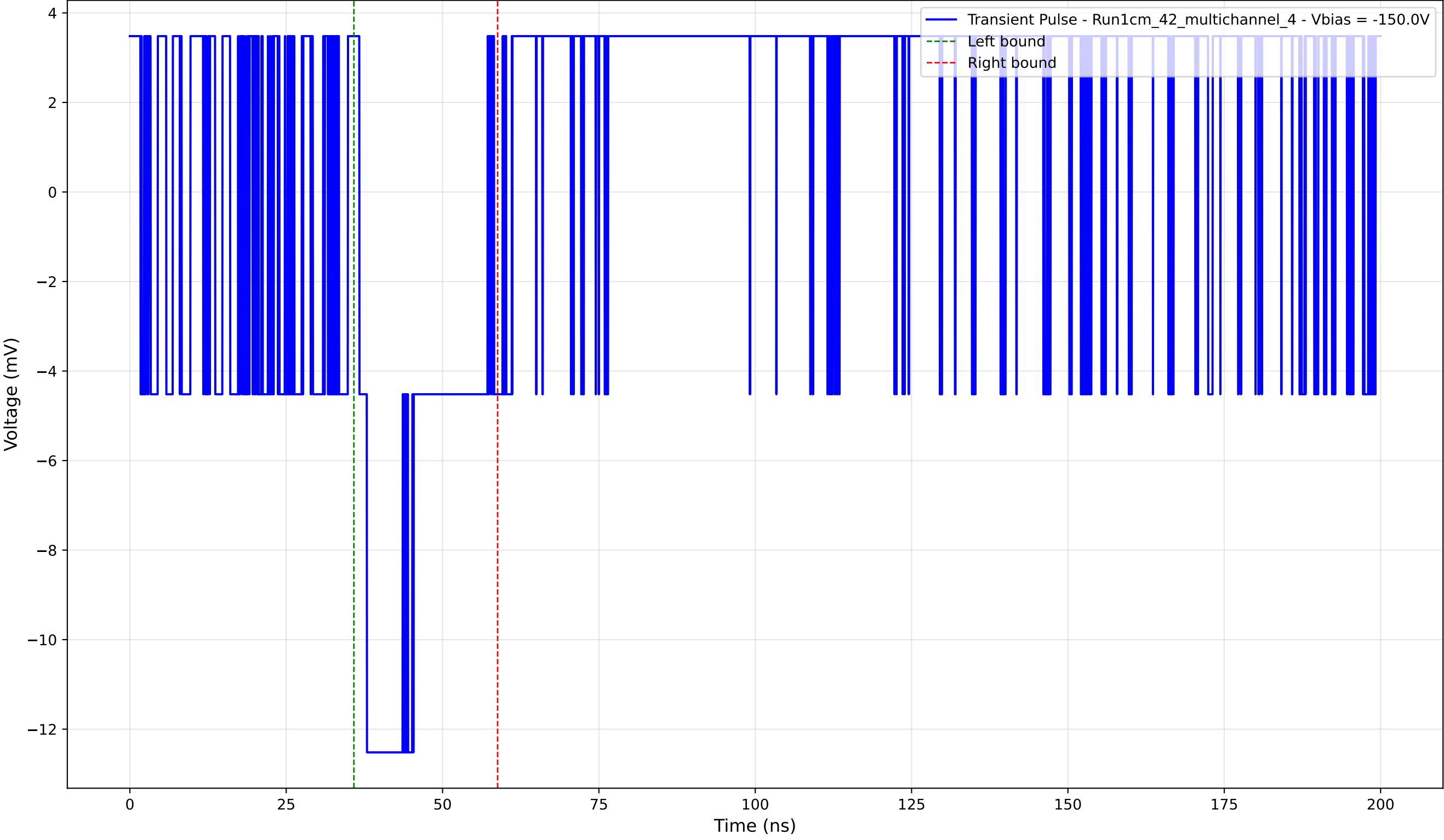
Transient Pulse - Sample: 1cm_42_multichannel - Position: 760.0 \mu\text{m} - Charge: 2.89 pC - Rise Time: 0.00 ns (N/A)
