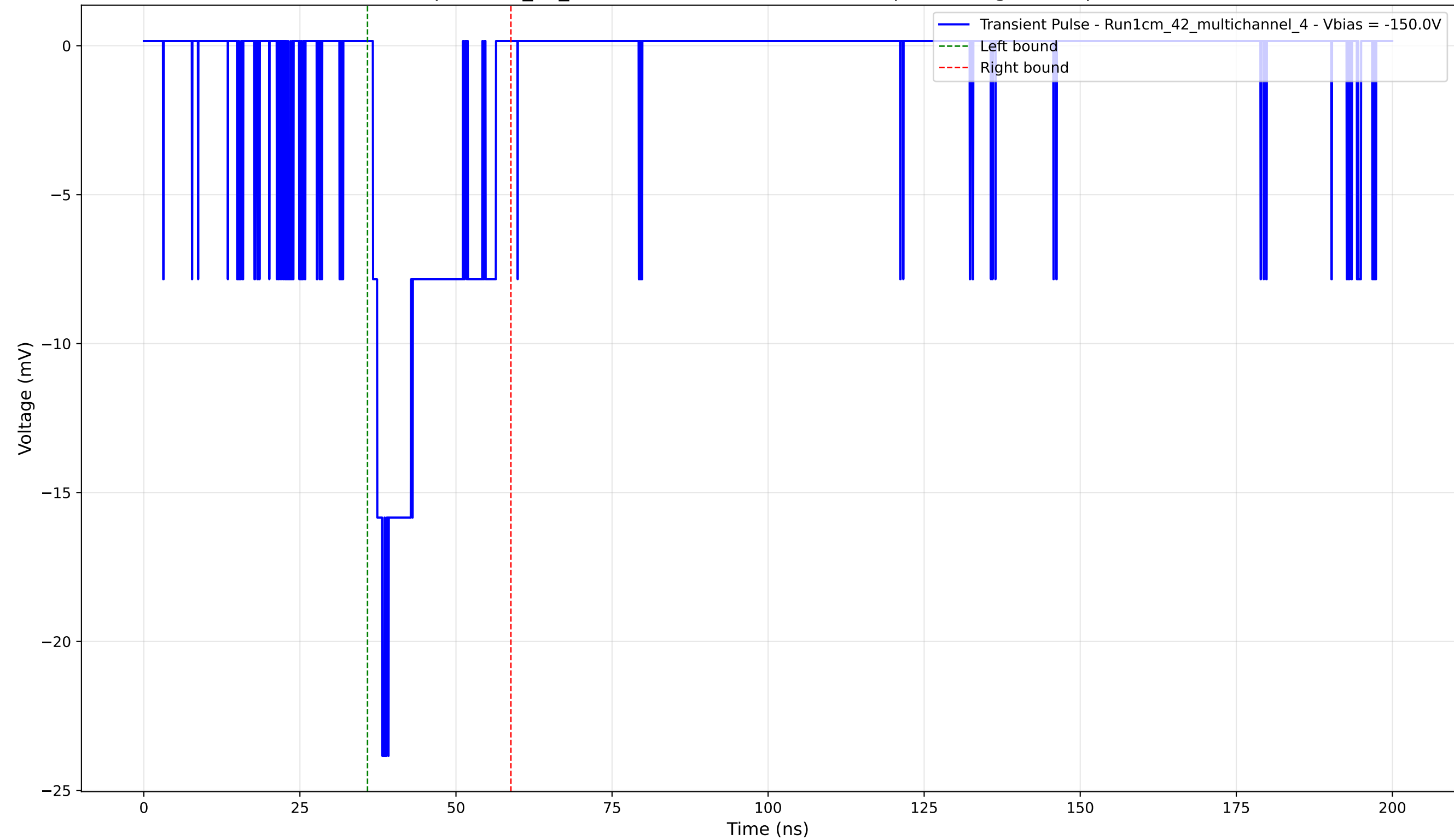
Transient Pulse - Sample: 1cm_42_multichannel - Position: 3590.0 \mu\text{m} - Charge: 3.96 pC - Rise Time: 1.49 ns
