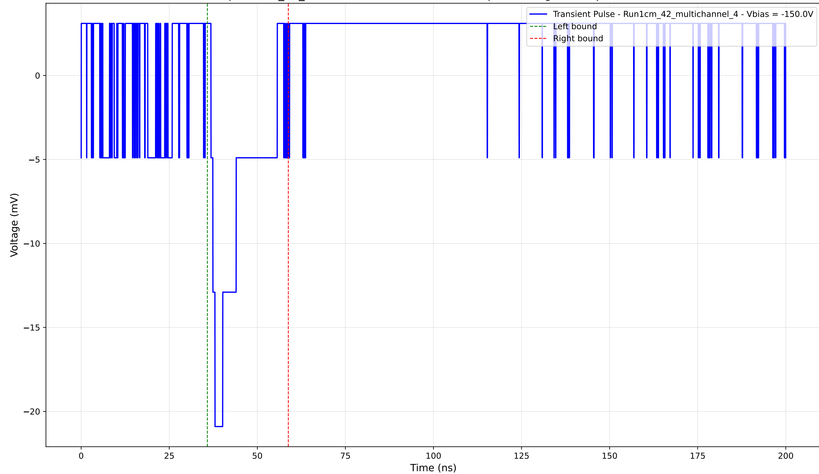
Transient Pulse - Sample: 1cm_42_multichannel - Position: 1090.0 \mu\text{m} - Charge: 3.14 pC - Rise Time: 0.00 ns (N/A)
