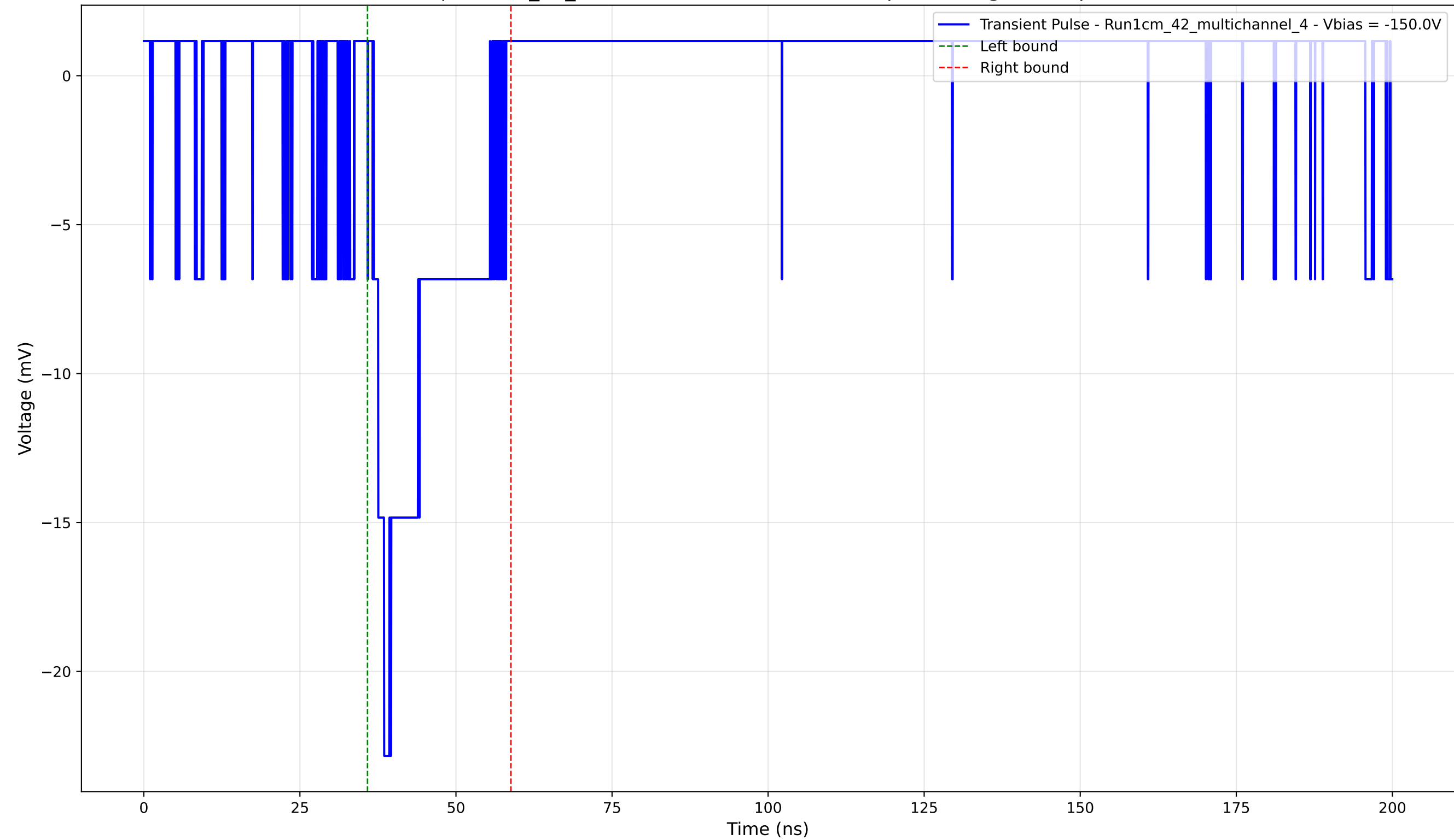
Transient Pulse - Sample: 1cm_42_multichannel - Position: 960.0 \mu\text{m} - Charge: 3.83 pC - Rise Time: 1.66 ns
