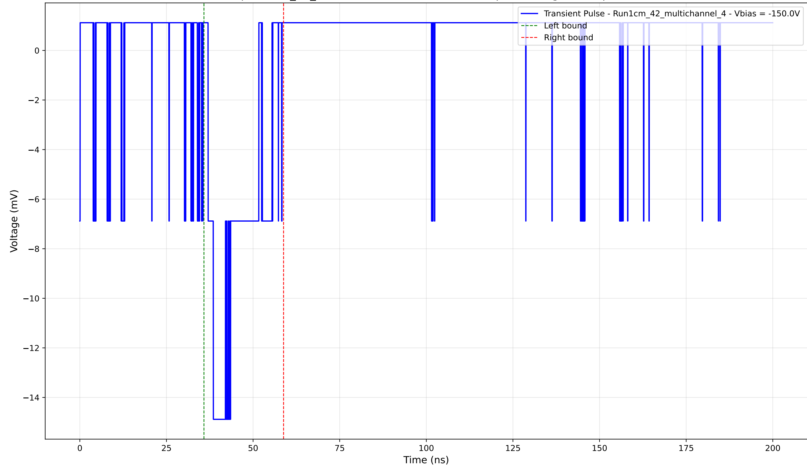
Transient Pulse - Sample: 1cm_42_multichannel - Position: 4750.0 \mu\text{m} - Charge: 3.07 pC - Rise Time: 1.52 ns
