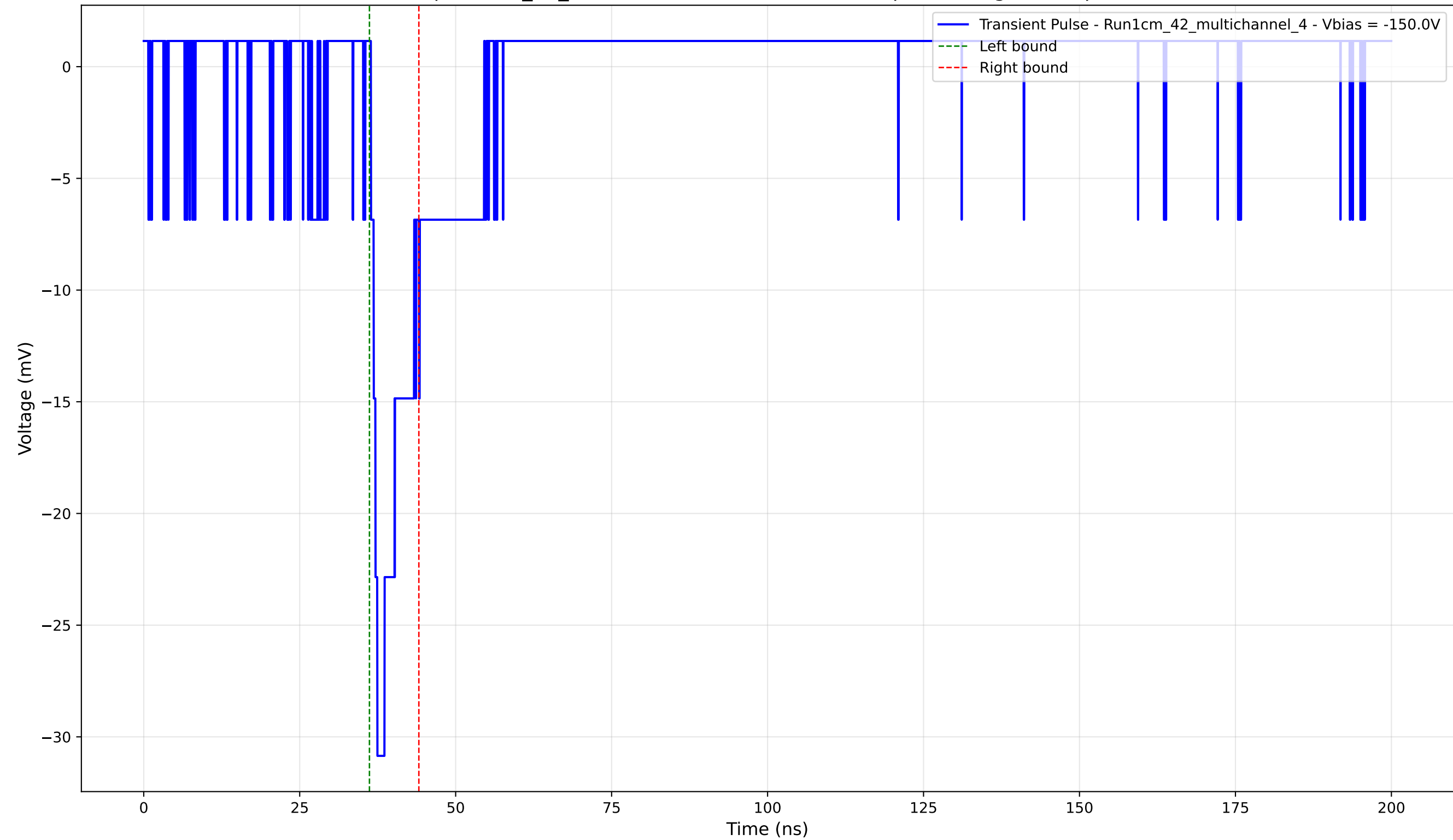
Transient Pulse - Sample: 1cm_42_multichannel - Position: 1555.0 \mu\text{m} - Charge: 2.77 pC - Rise Time: 1.03 ns
