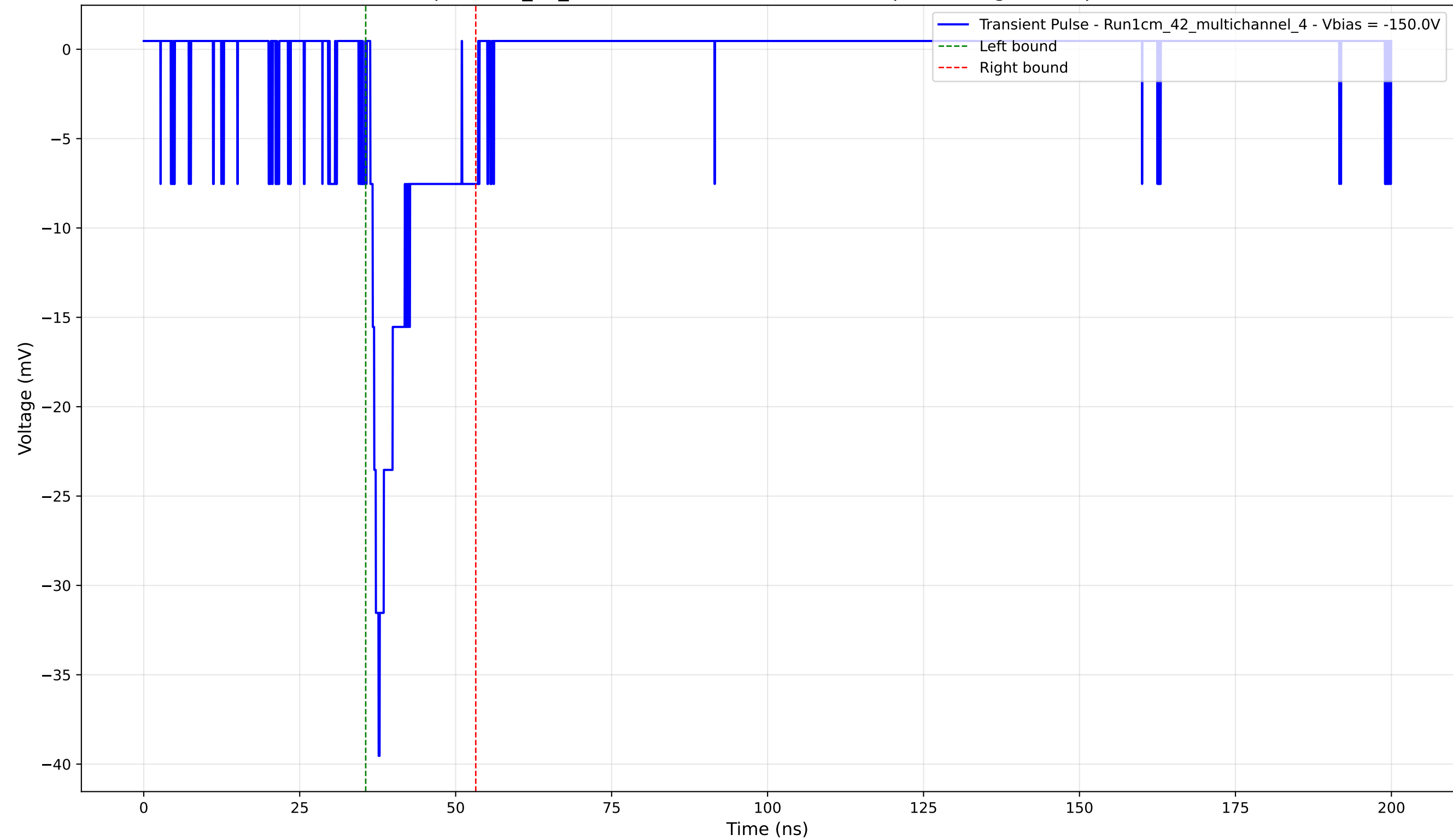
Transient Pulse - Sample: 1cm_42_multichannel - Position: 3060.0 \mu\text{m} - Charge: 4.16 pC - Rise Time: 1.33 ns
