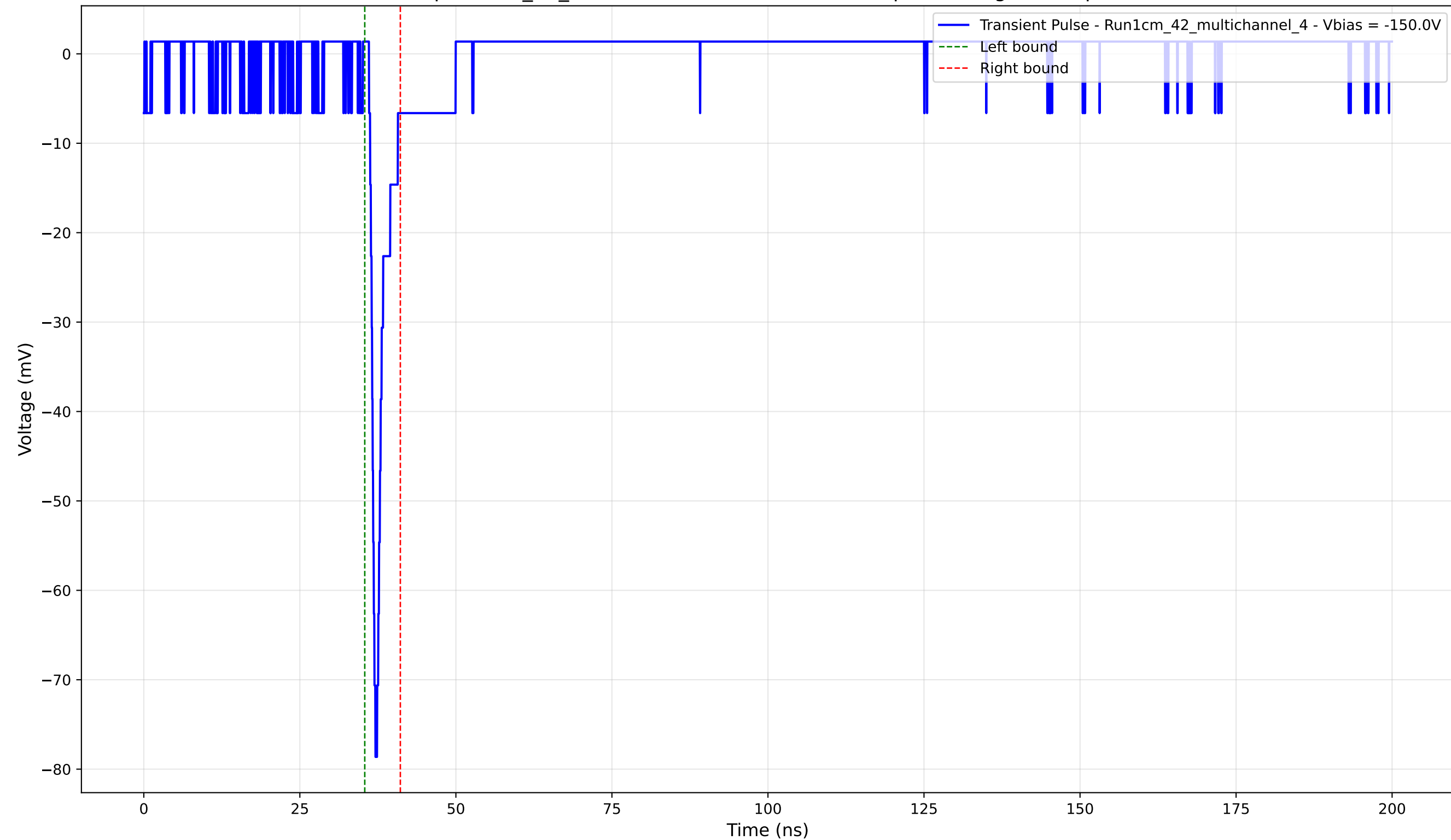
Transient Pulse - Sample: 1cm_42_multichannel - Position: 2310.0 \mu\text{m} - Charge: 3.05 pC - Rise Time: 0.86 ns
