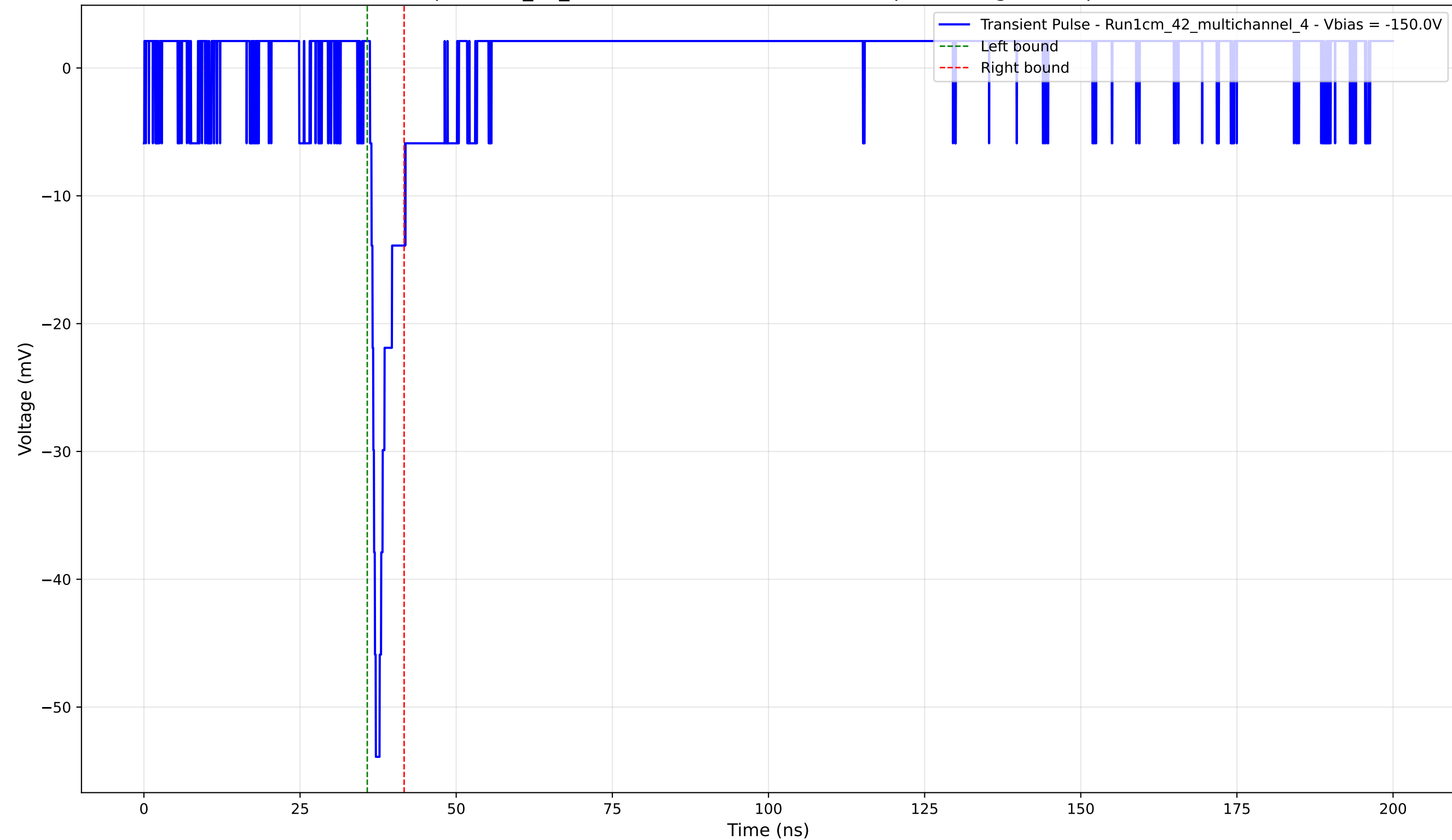
Transient Pulse - Sample: 1cm_42_multichannel - Position: 2710.0 \mu\text{m} - Charge: 2.73 pC - Rise Time: 0.92 ns
