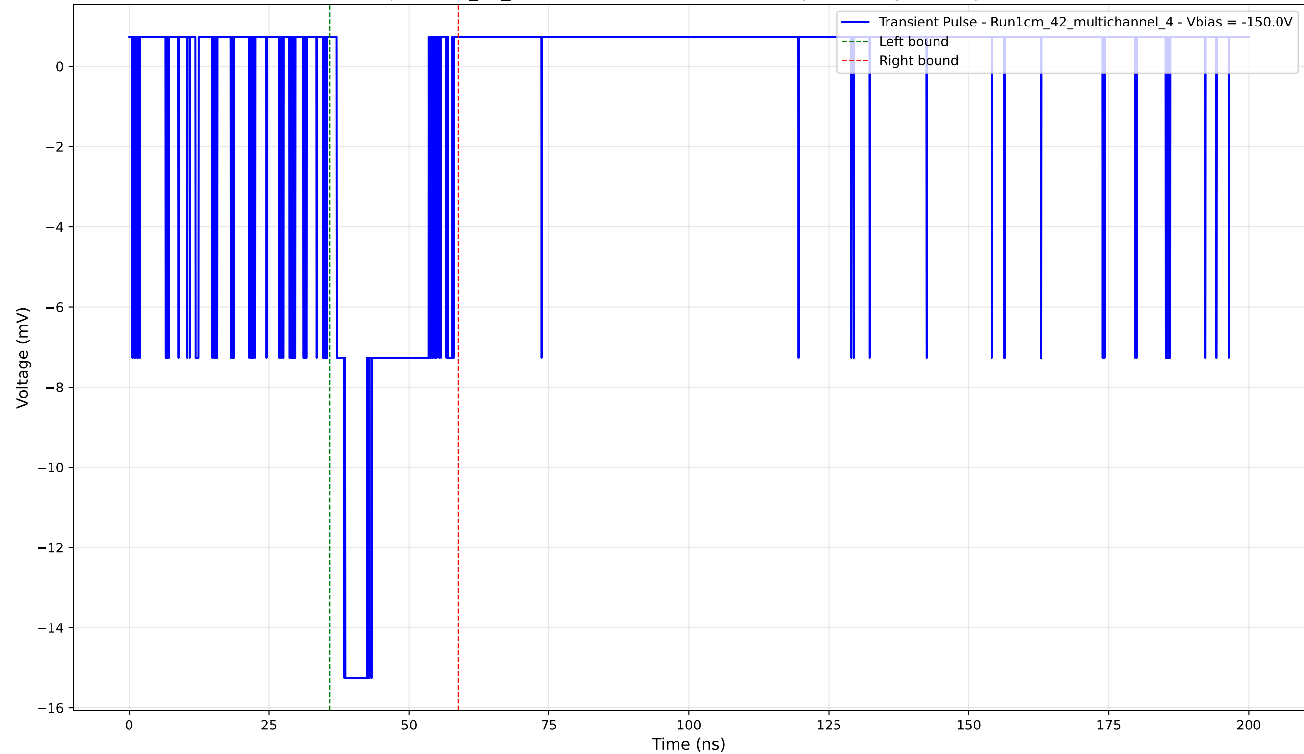
Transient Pulse - Sample: 1cm_42_multichannel - Position: 4600.0 \mu\text{m} - Charge: 3.29 pC - Rise Time: 1.48 ns
