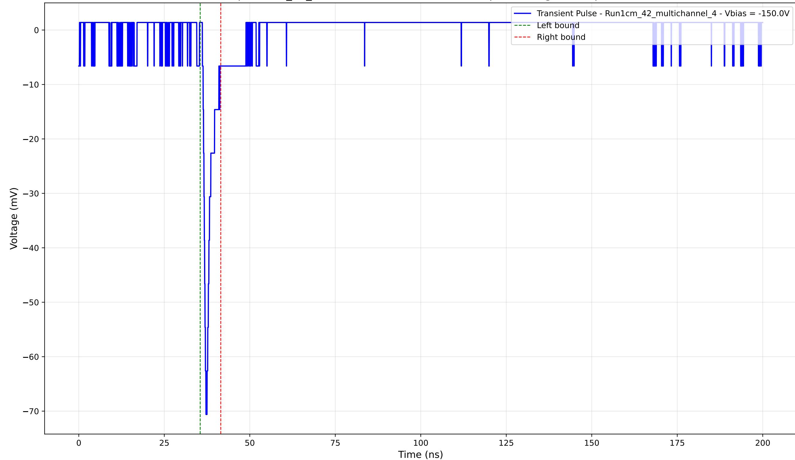
Transient Pulse - Sample: 1cm_42_multichannel - Position: 2175.0 \mu\text{m} - Charge: 3.05 pC - Rise Time: 0.84 ns
