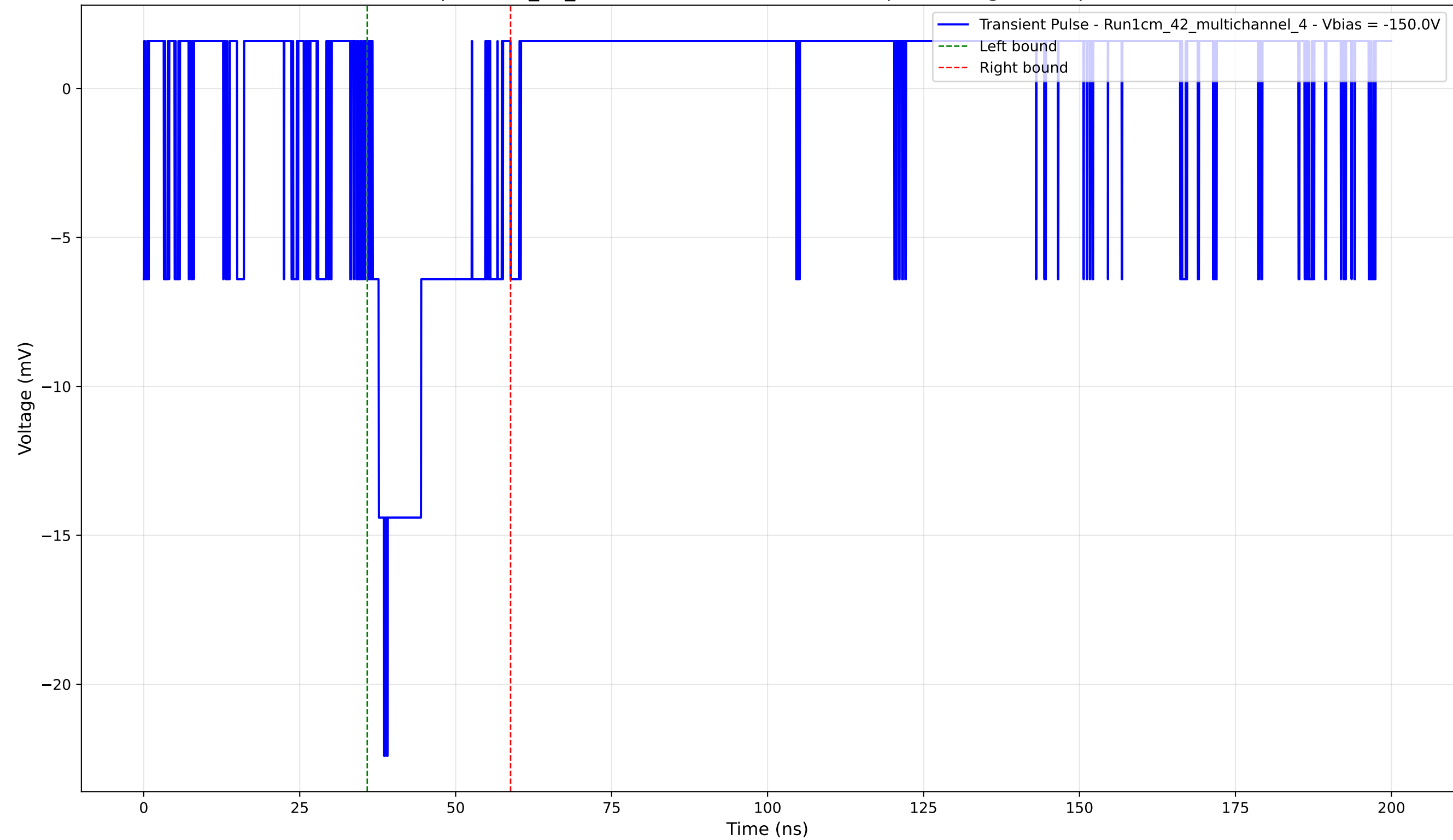
Transient Pulse - Sample: 1cm_42_multichannel - Position: 945.0 \mu\text{m} - Charge: 3.66 pC - Rise Time: 1.84 ns
