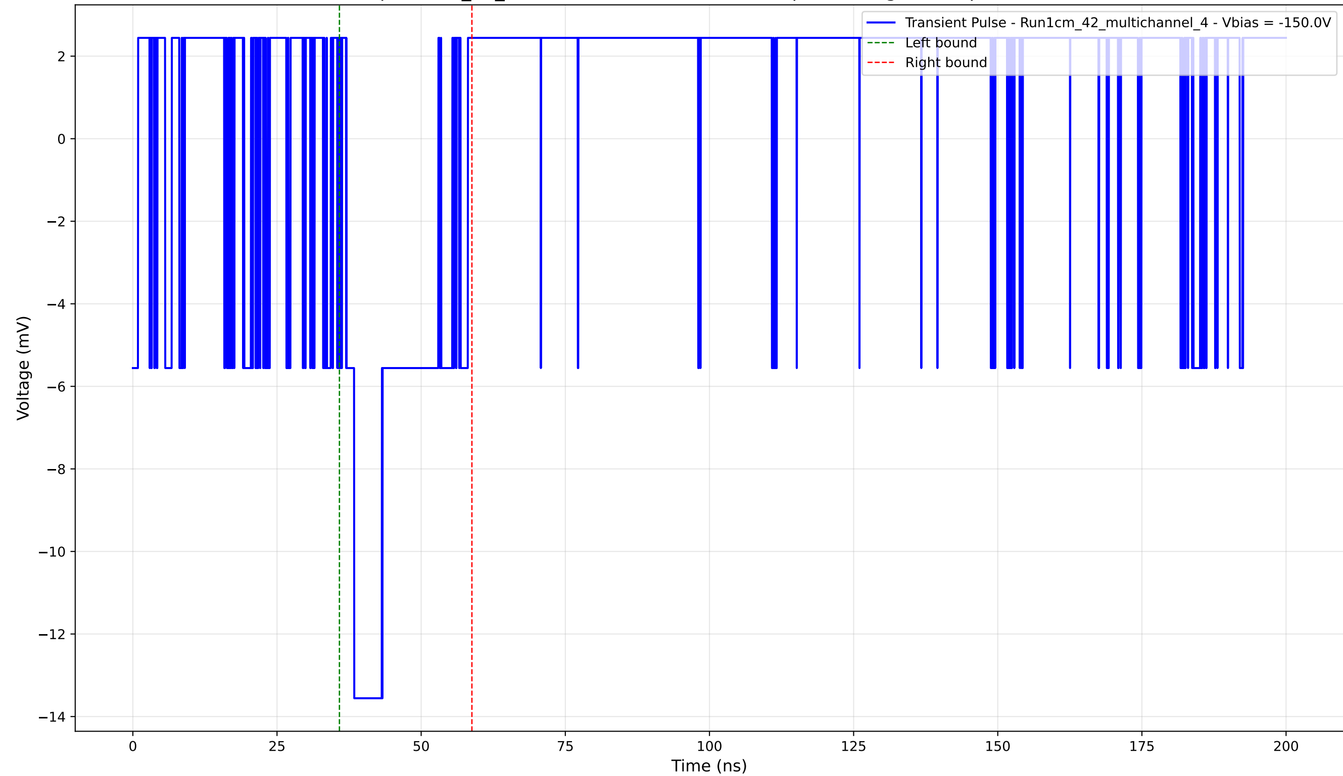
Transient Pulse - Sample: 1cm_42_multichannel - Position: 450.0 \mu\text{m} - Charge: 2.85 pC - Rise Time: 0.00 ns (N/A)
