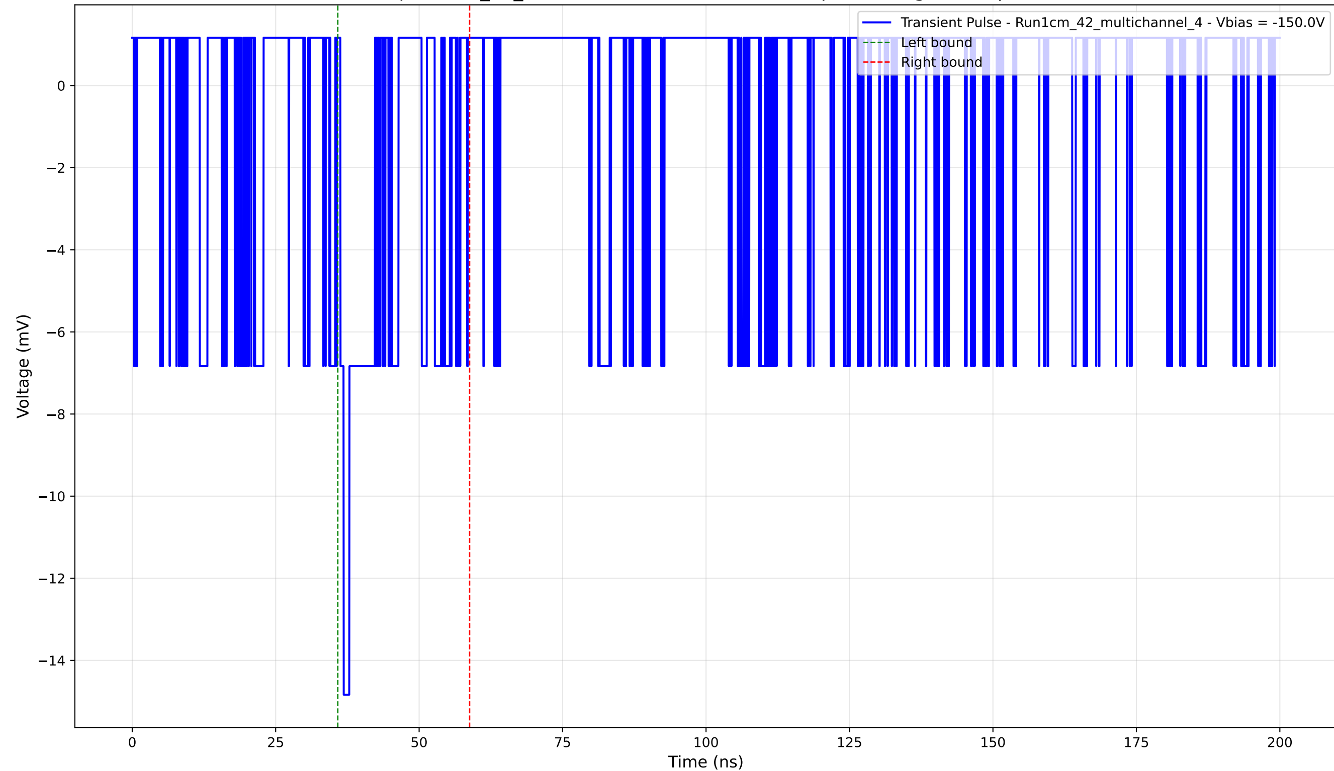
Transient Pulse - Sample: 1cm_42_multichannel - Position: 2420.0 \mu\text{m} - Charge: 1.58 pC - Rise Time: 0.58 ns
