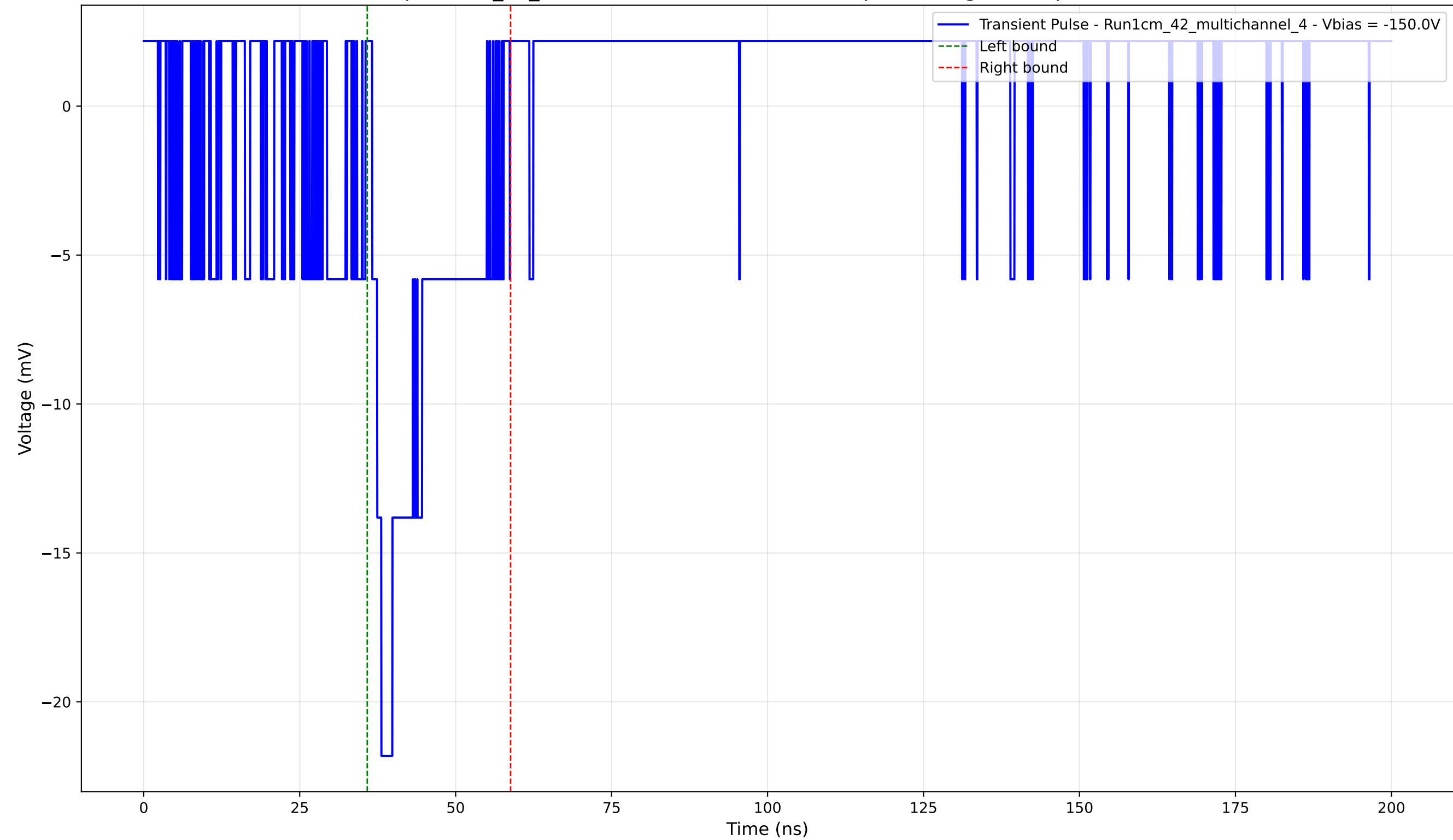
Transient Pulse - Sample: 1cm_42_multichannel - Position: 1065.0 \mu\text{m} - Charge: 3.64 pC - Rise Time: 0.00 ns (N/A)
