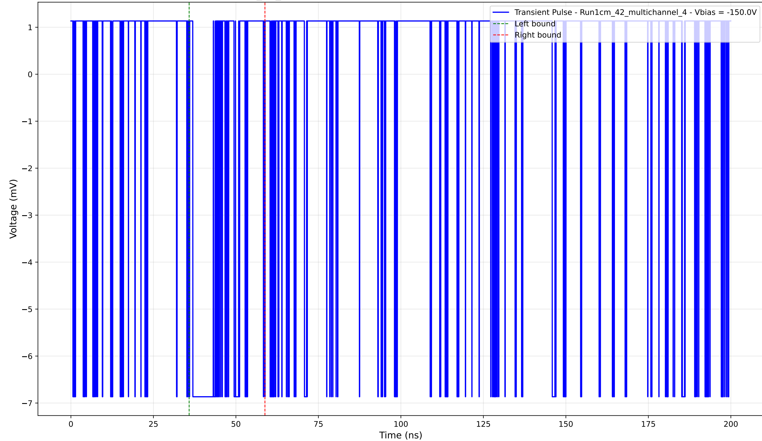
Transient Pulse - Sample: 1cm_42_multichannel - Position: 3430.0 \mu\text{m} - Charge: 1.12 pC - Rise Time: 0.00 ns (N/A)
