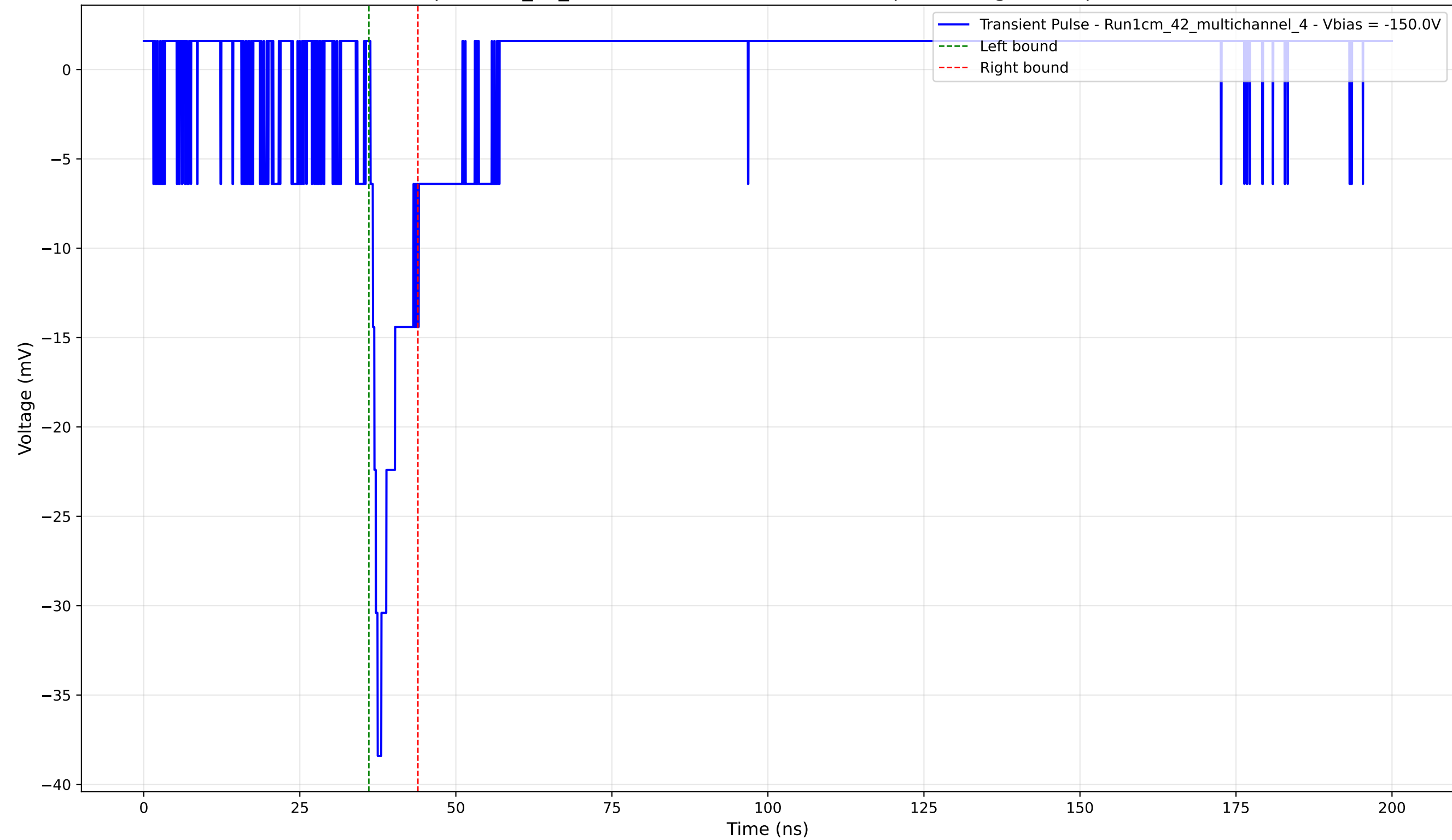
Transient Pulse - Sample: 1cm_42_multichannel - Position: 1685.0 \mu\text{m} - Charge: 2.96 pC - Rise Time: 1.15 ns
