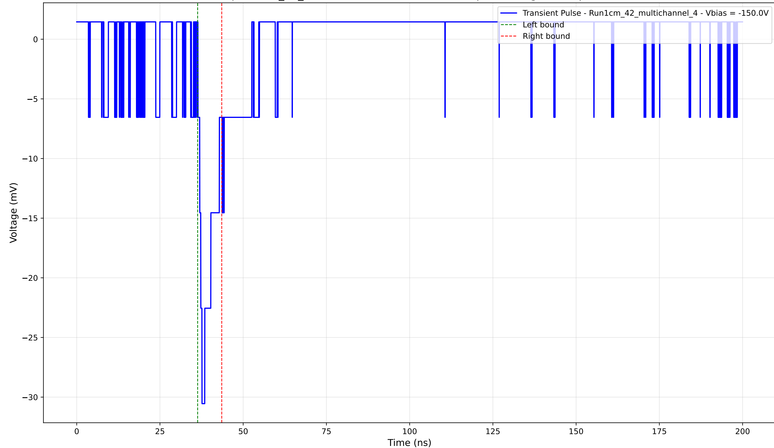
Transient Pulse - Sample: 1cm_42_multichannel - Position: 1470.0 \mu\text{m} - Charge: 2.50 pC - Rise Time: 1.21 ns
