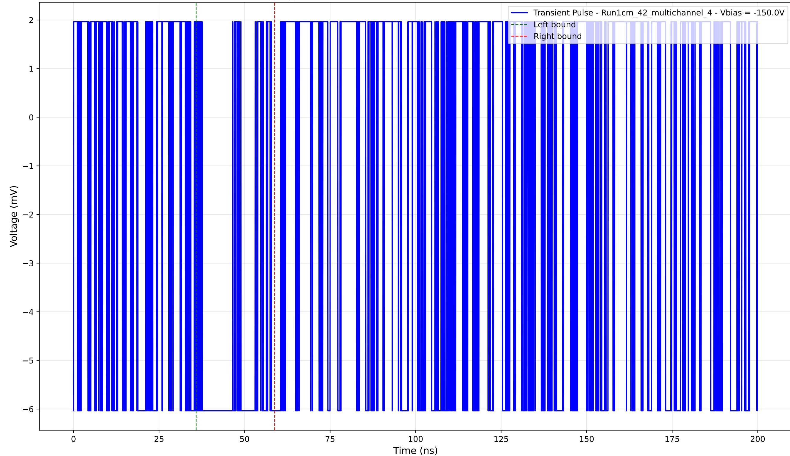
Transient Pulse - Sample: 1cm_42_multichannel - Position: 835.0 \mu\text{m} - Charge: 2.05 pC - Rise Time: 0.00 ns (N/A)
