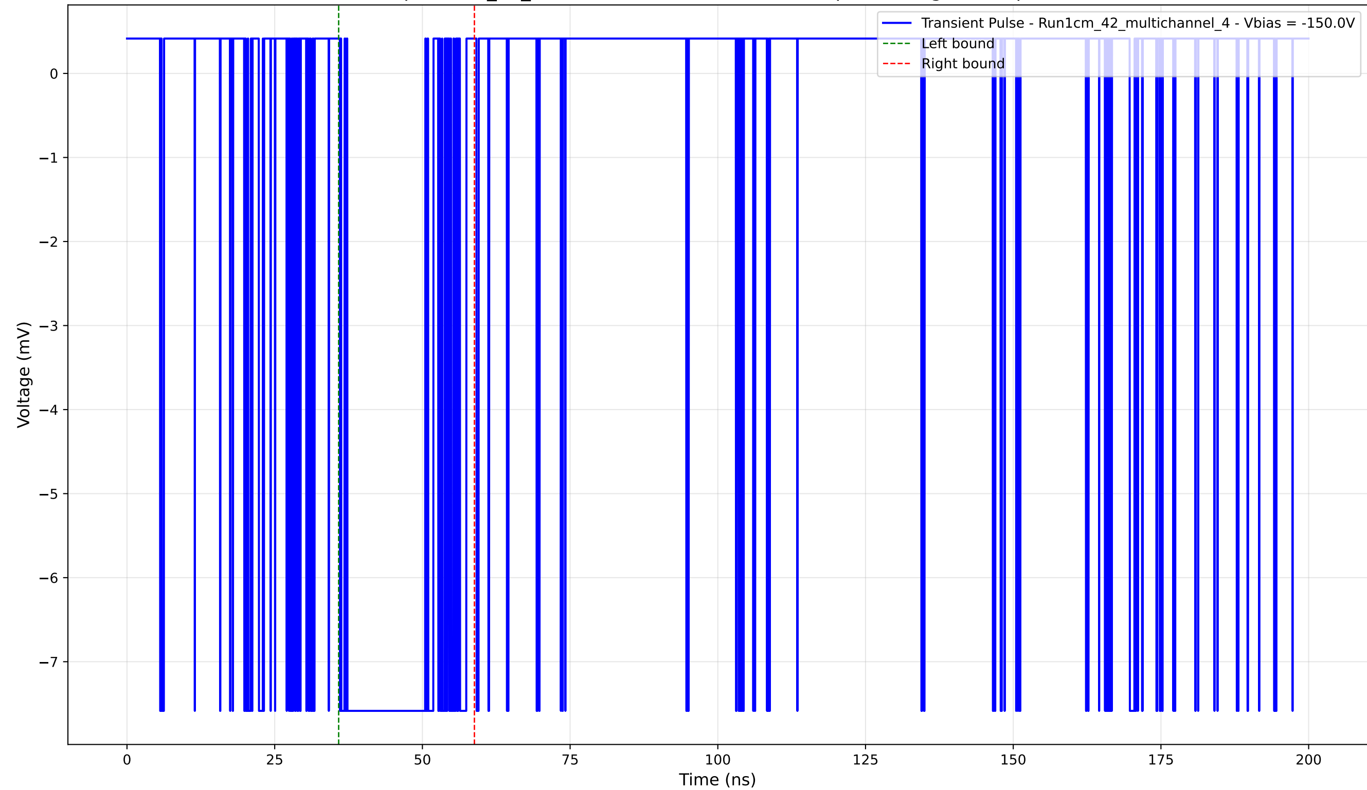
Transient Pulse - Sample: 1cm_42_multichannel - Position: 4850.0 \mu\text{m} - Charge: 2.74 pC - Rise Time: 0.02 ns
