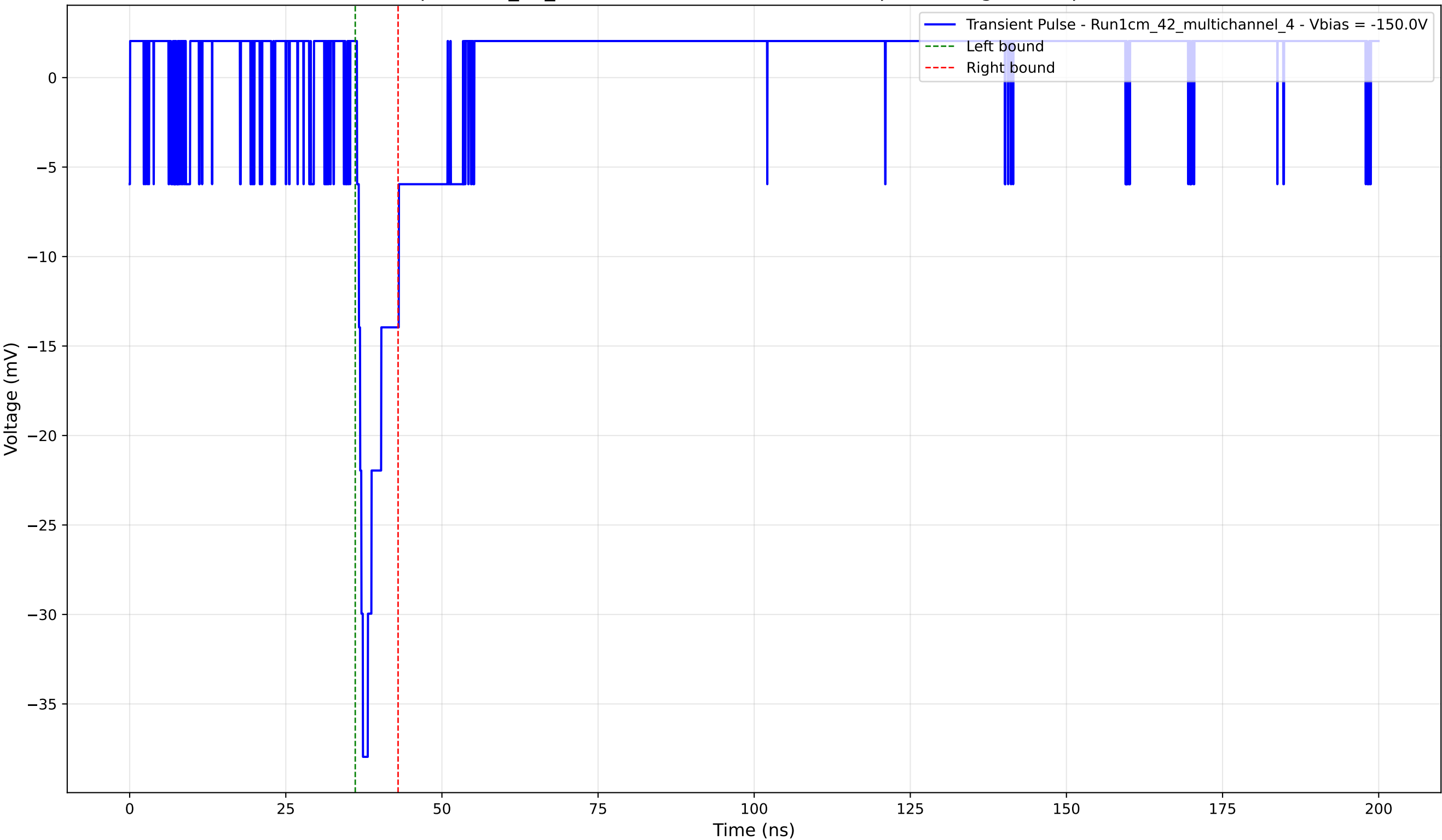
Transient Pulse - Sample: 1cm_42_multichannel - Position: 1735.0 \mu\text{m} - Charge: 2.71 pC - Rise Time: 0.95 ns
