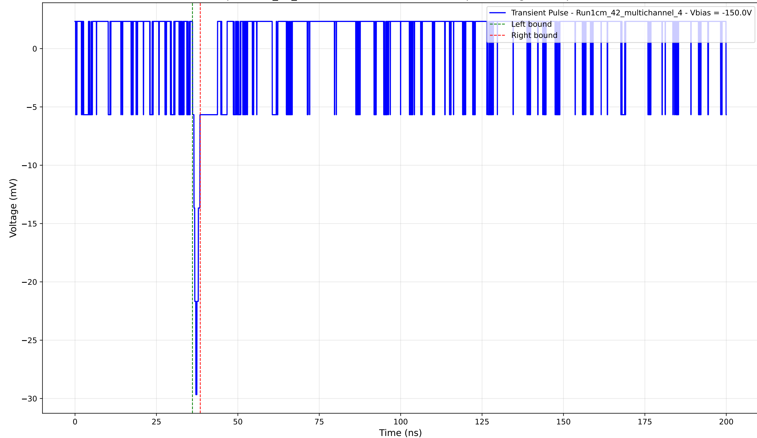
Transient Pulse - Sample: 1cm_42_multichannel - Position: 2430.0 \mu\text{m} - Charge: 0.79 pC - Rise Time: 1.04 ns
