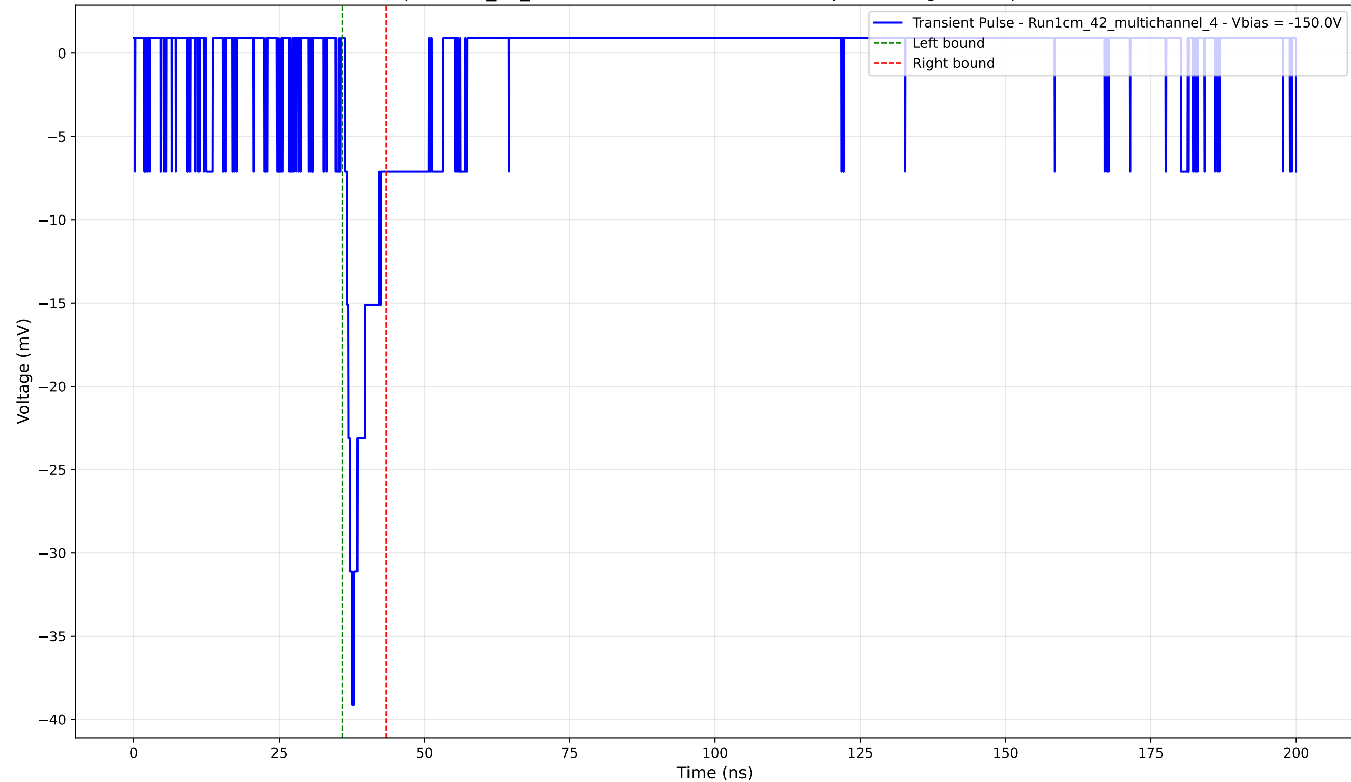
Transient Pulse - Sample: 1cm_42_multichannel - Position: 3045.0 \mu\text{m} - Charge: 2.63 pC - Rise Time: 1.23 ns
