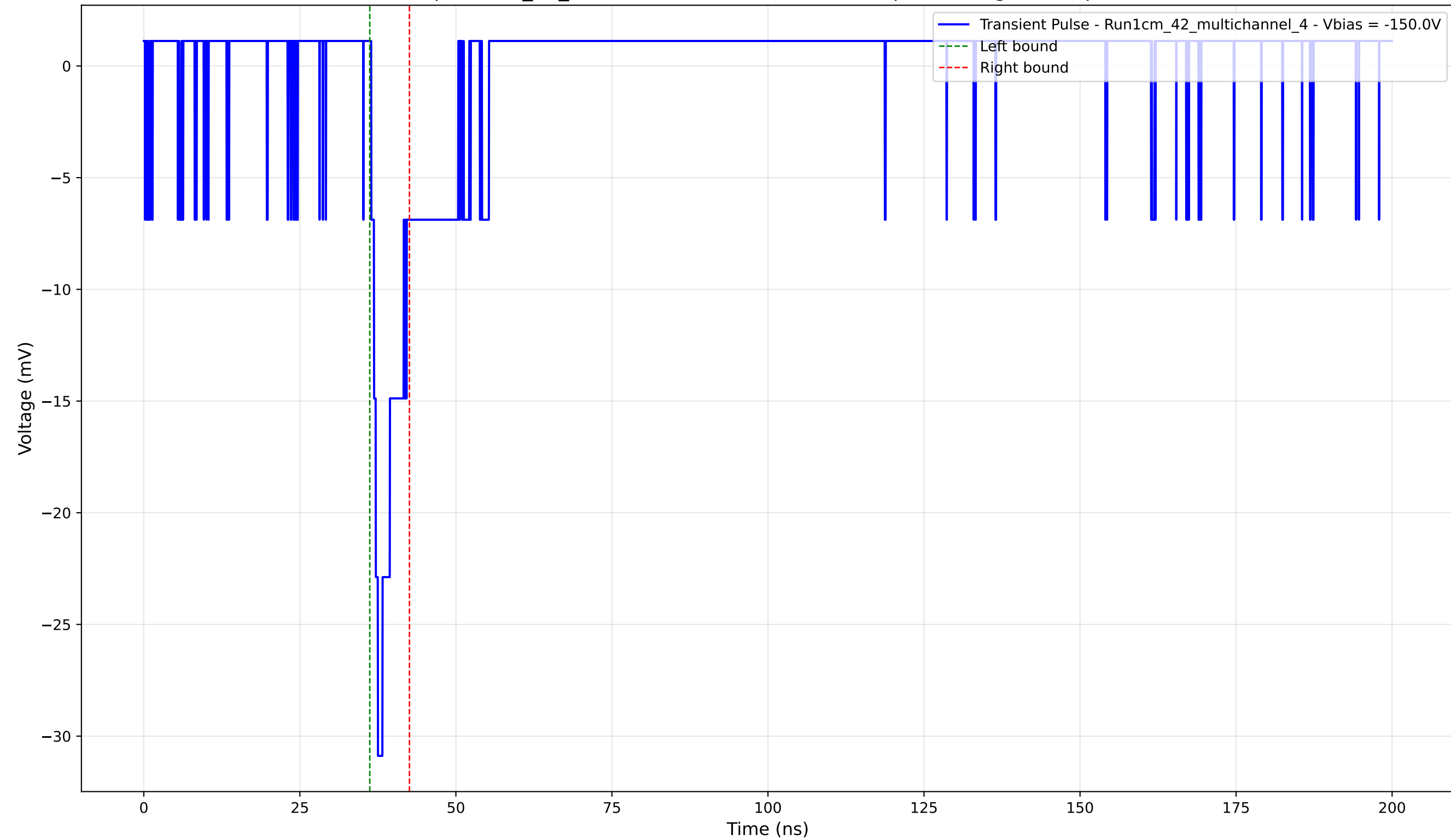
Transient Pulse - Sample: 1cm_42_multichannel - Position: 3150.0 \mu\text{m} - Charge: 2.12 pC - Rise Time: 1.07 ns
