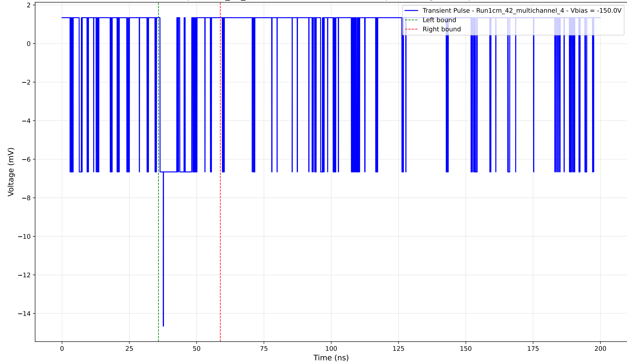
Transient Pulse - Sample: 1cm_42_multichannel - Position: 2855.0 \mu\text{m} - Charge: 1.32 pC - Rise Time: 1.26 ns
