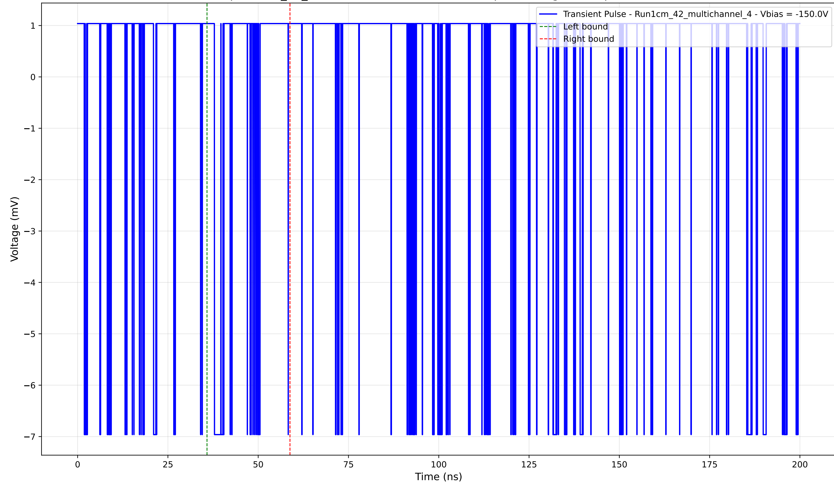
Transient Pulse - Sample: 1cm_42_multichannel - Position: 4420.0 \mu\text{m} - Charge: 0.09 pC - Rise Time: 0.00 ns (N/A)
