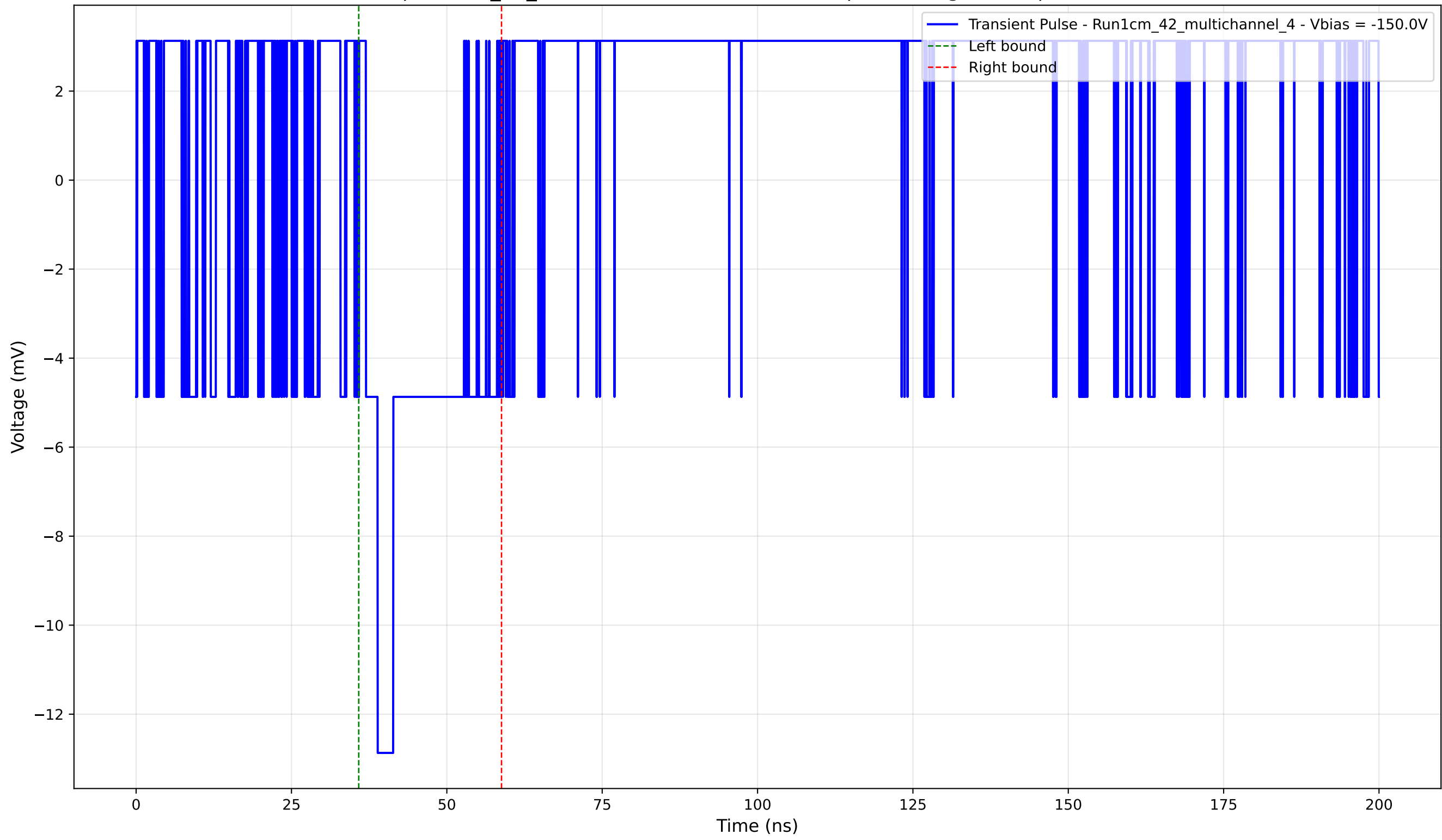
Transient Pulse - Sample: 1cm_42_multichannel - Position: 300.0 \mu\text{m} - Charge: 2.32 pC - Rise Time: 0.00 ns (N/A)
