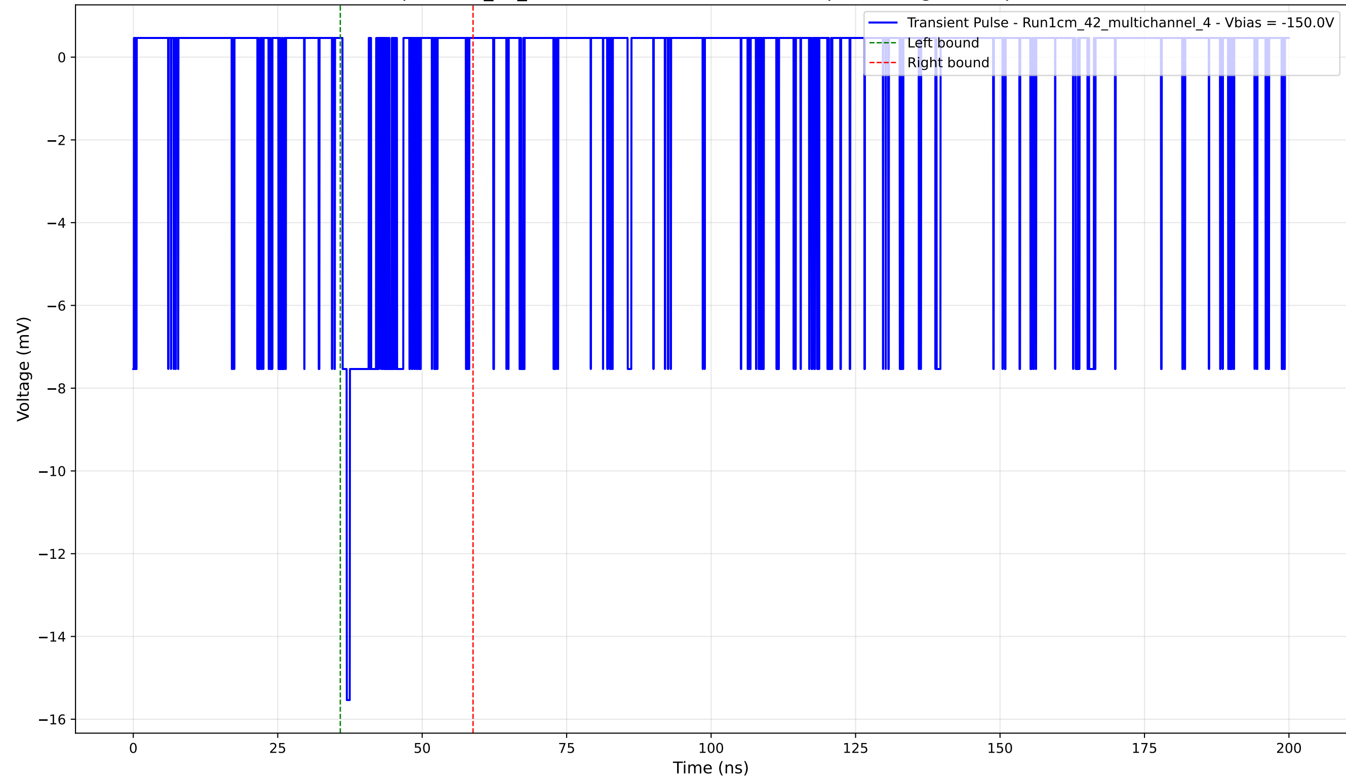
Transient Pulse - Sample: 1cm_42_multichannel - Position: 2355.0 \mu\text{m} - Charge: 1.41 pC - Rise Time: 0.74 ns
