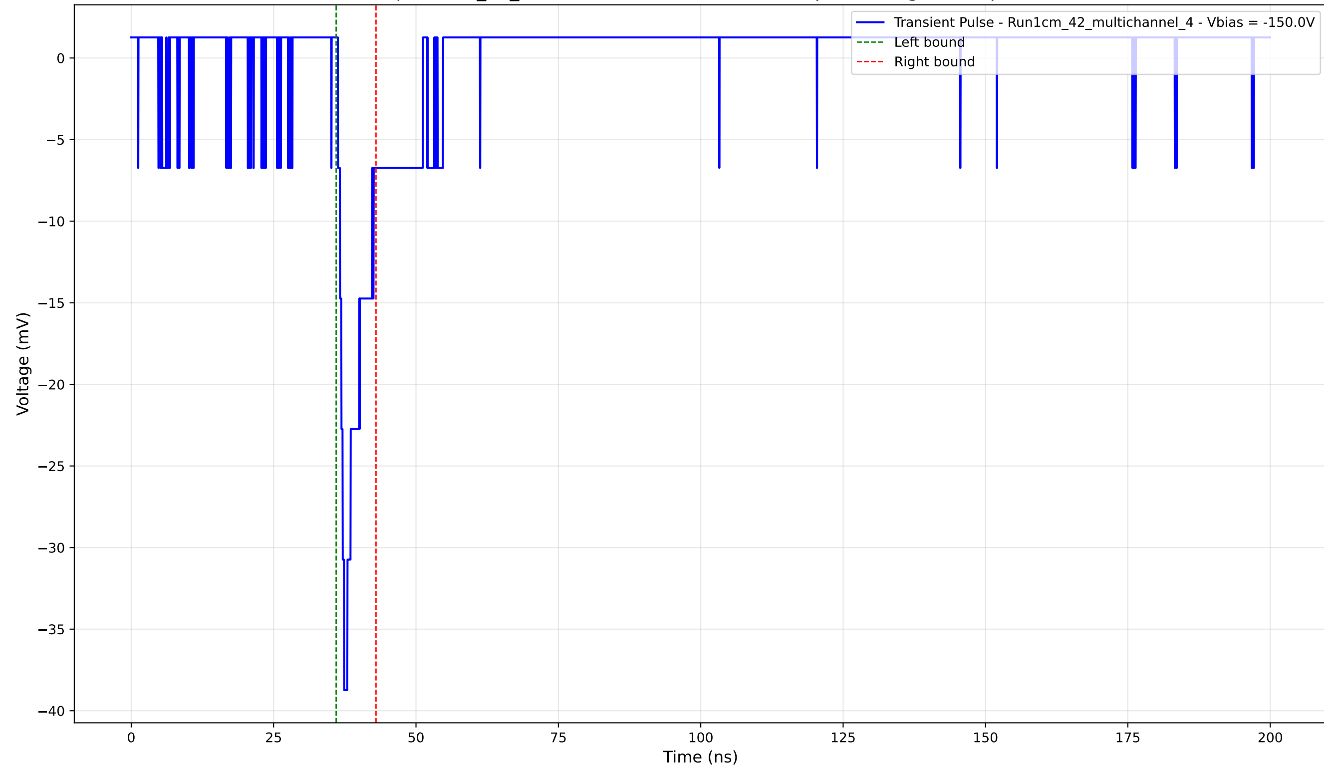
Transient Pulse - Sample: 1cm_42_multichannel - Position: 3025.0 \mu\text{m} - Charge: 2.65 pC - Rise Time: 1.09 ns
