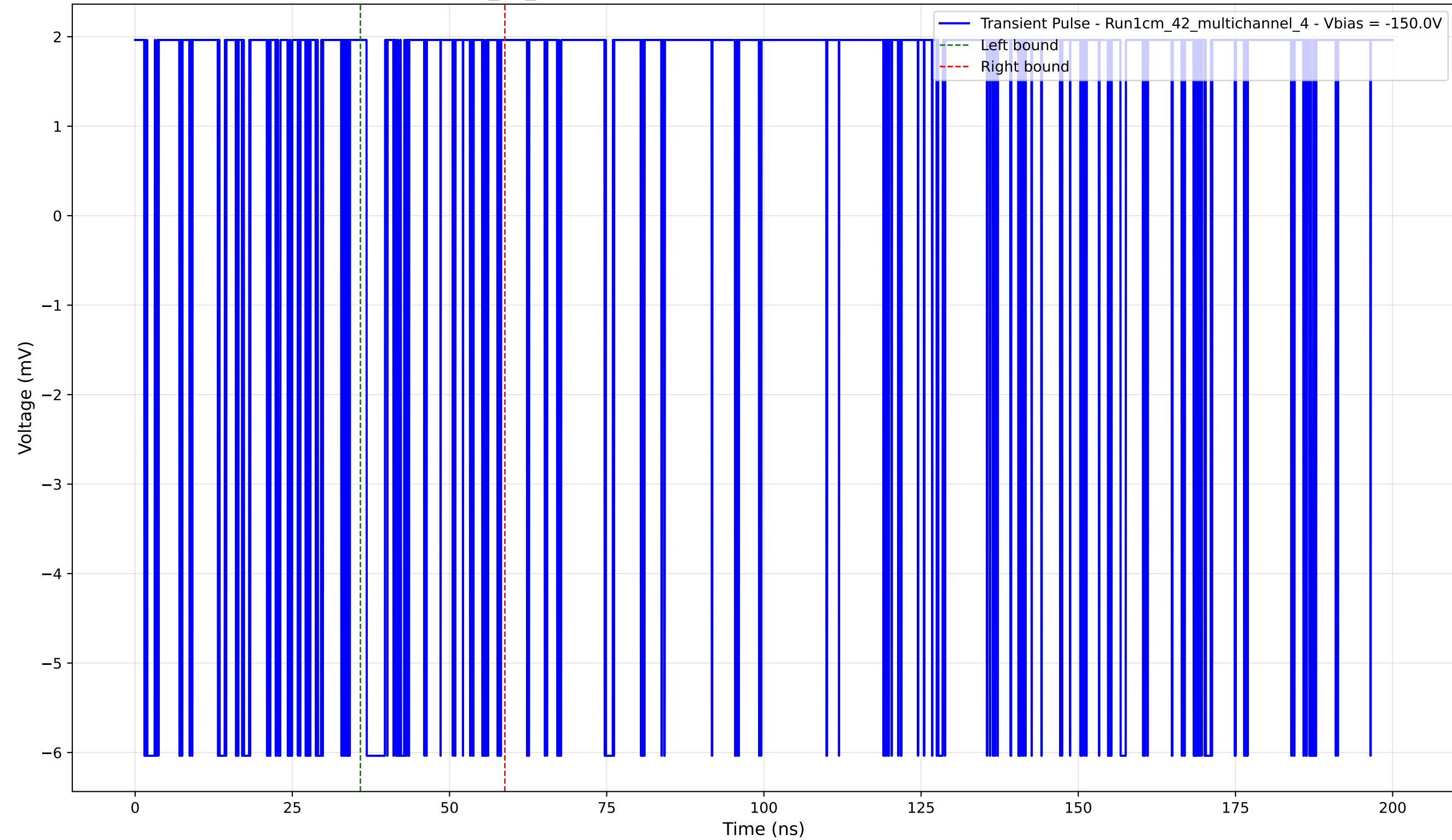
Transient Pulse - Sample: 1cm_42_multichannel - Position: 2890.0 \mu\text{m} - Charge: 0.04 pC - Rise Time: 0.00 ns (N/A)
