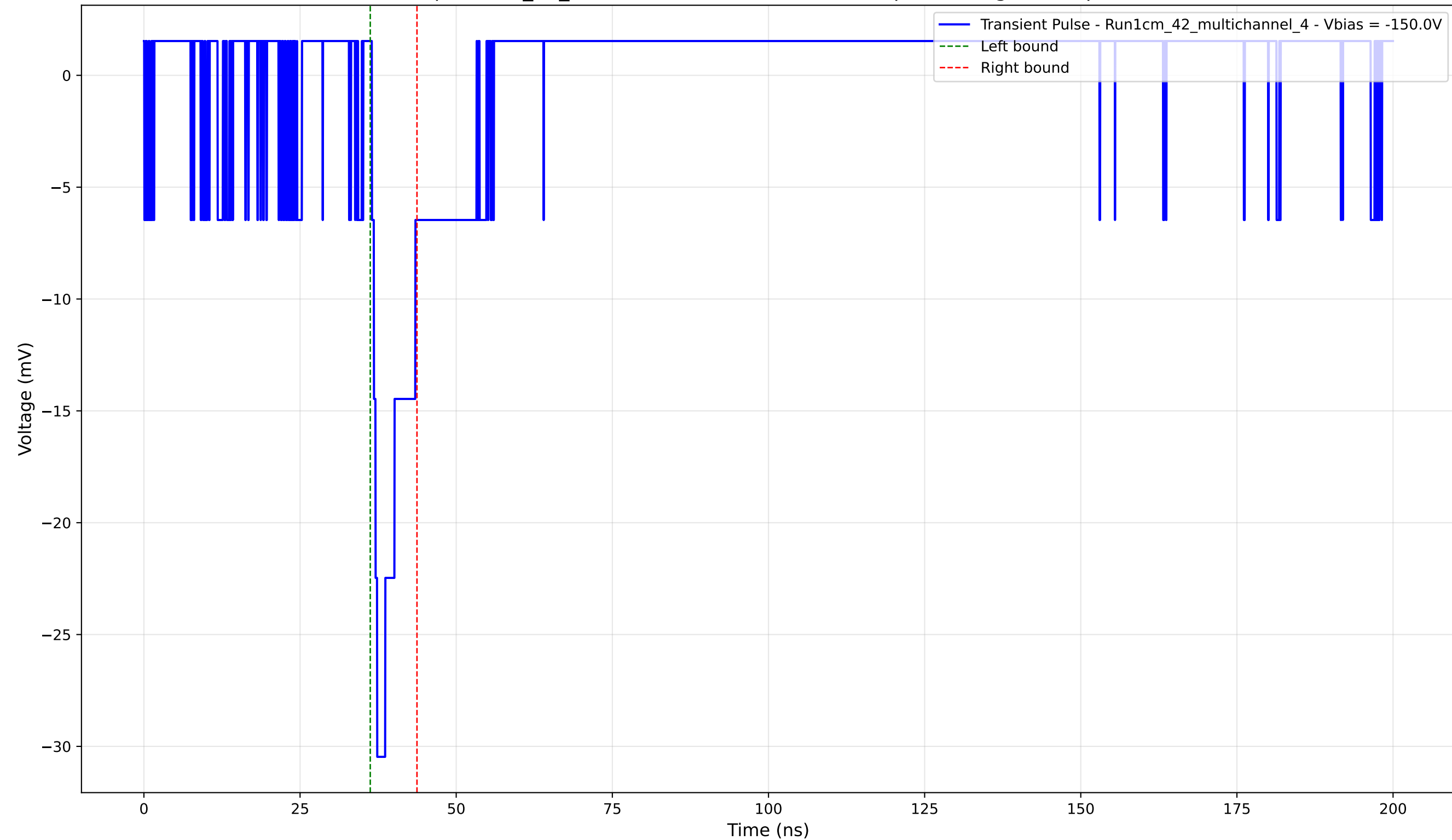
Transient Pulse - Sample: 1cm_42_multichannel - Position: 1615.0 \mu\text{m} - Charge: 2.68 pC - Rise Time: 0.85 ns
