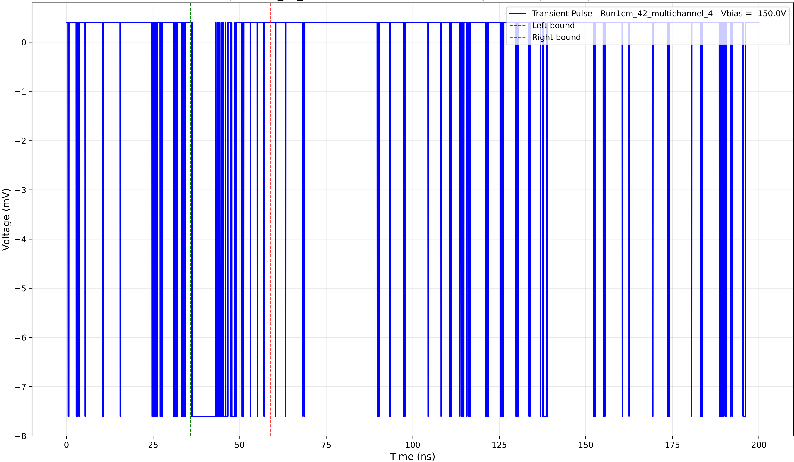
Transient Pulse - Sample: 1cm_42_multichannel - Position: 2930.0 \mu\text{m} - Charge: 1.62 pC - Rise Time: 0.02 ns
