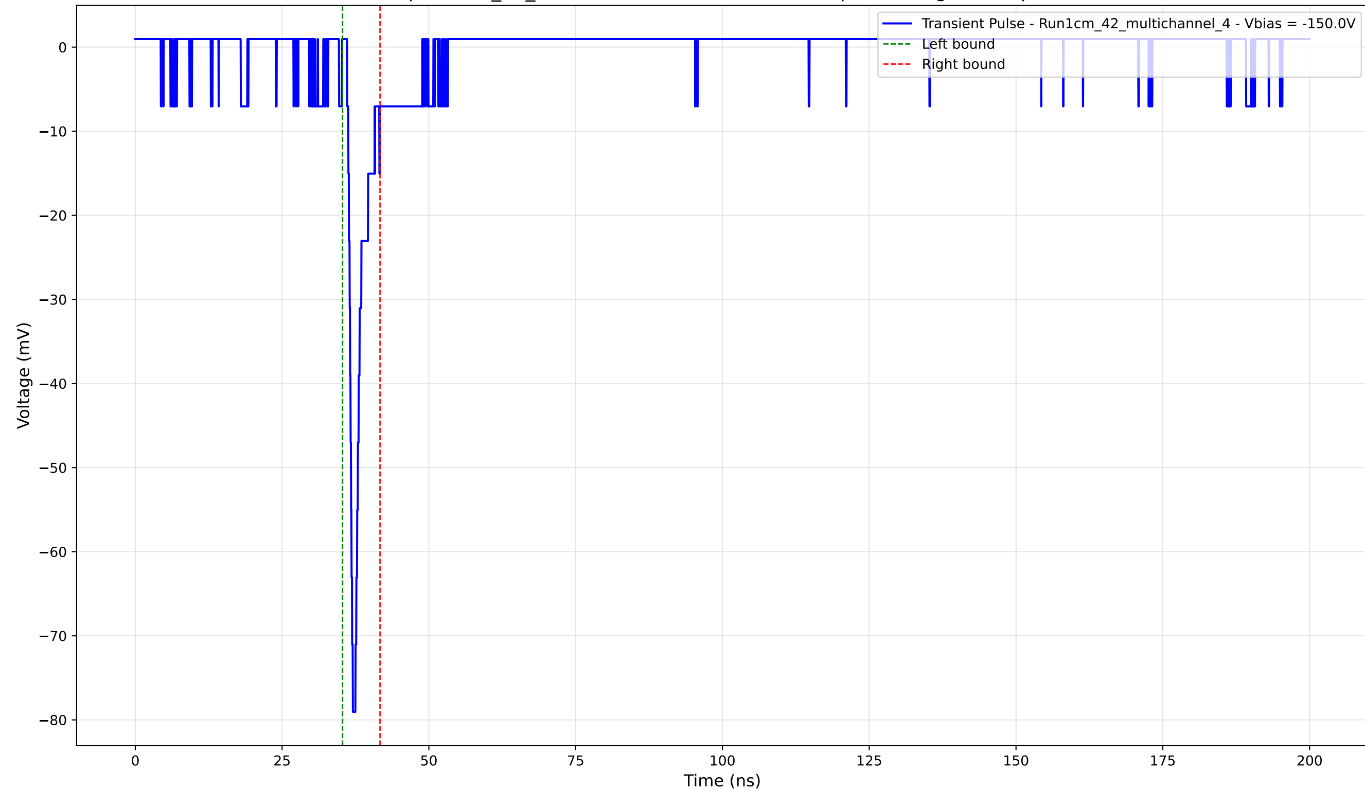
Transient Pulse - Sample: 1cm_42_multichannel - Position: 2495.0 \mu\text{m} - Charge: 3.36 pC - Rise Time: 0.78 ns
