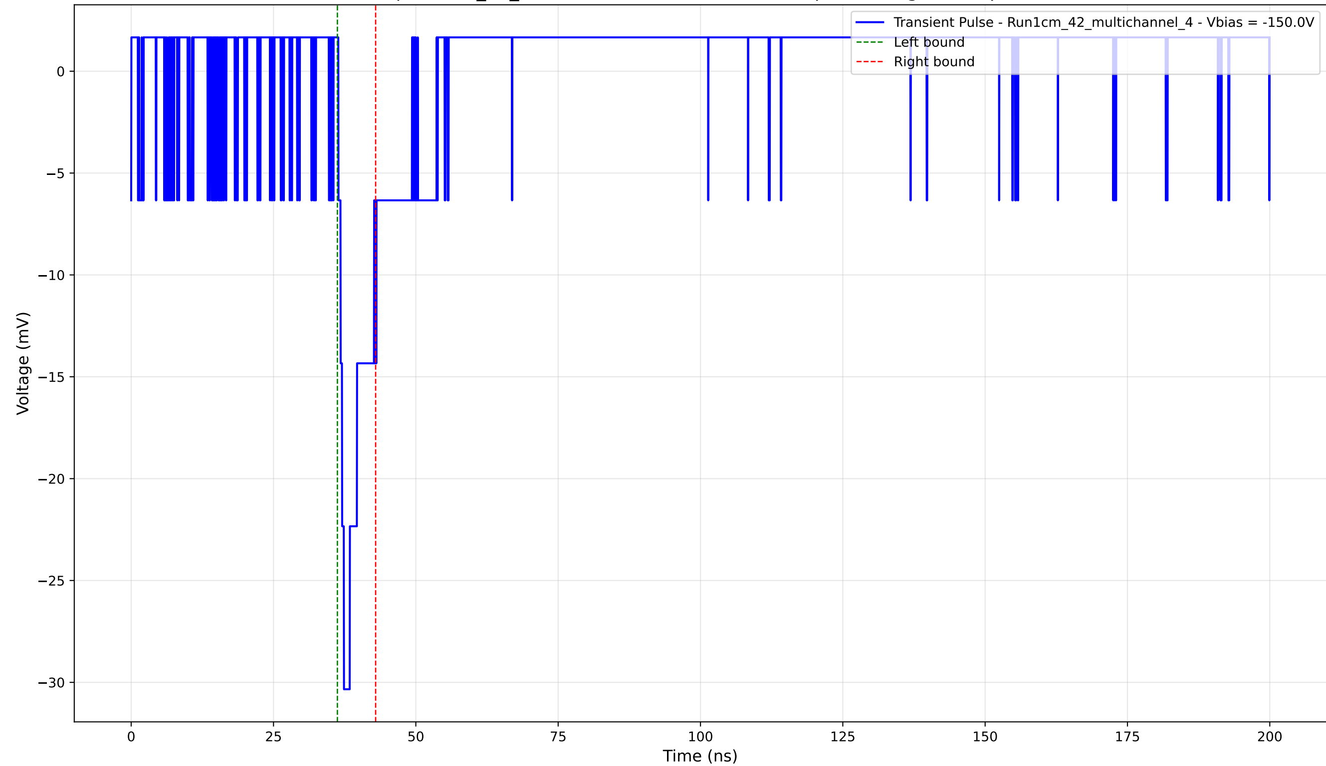
Transient Pulse - Sample: 1cm_42_multichannel - Position: 3140.0 \mu\text{m} - Charge: 2.36 pC - Rise Time: 0.97 ns
