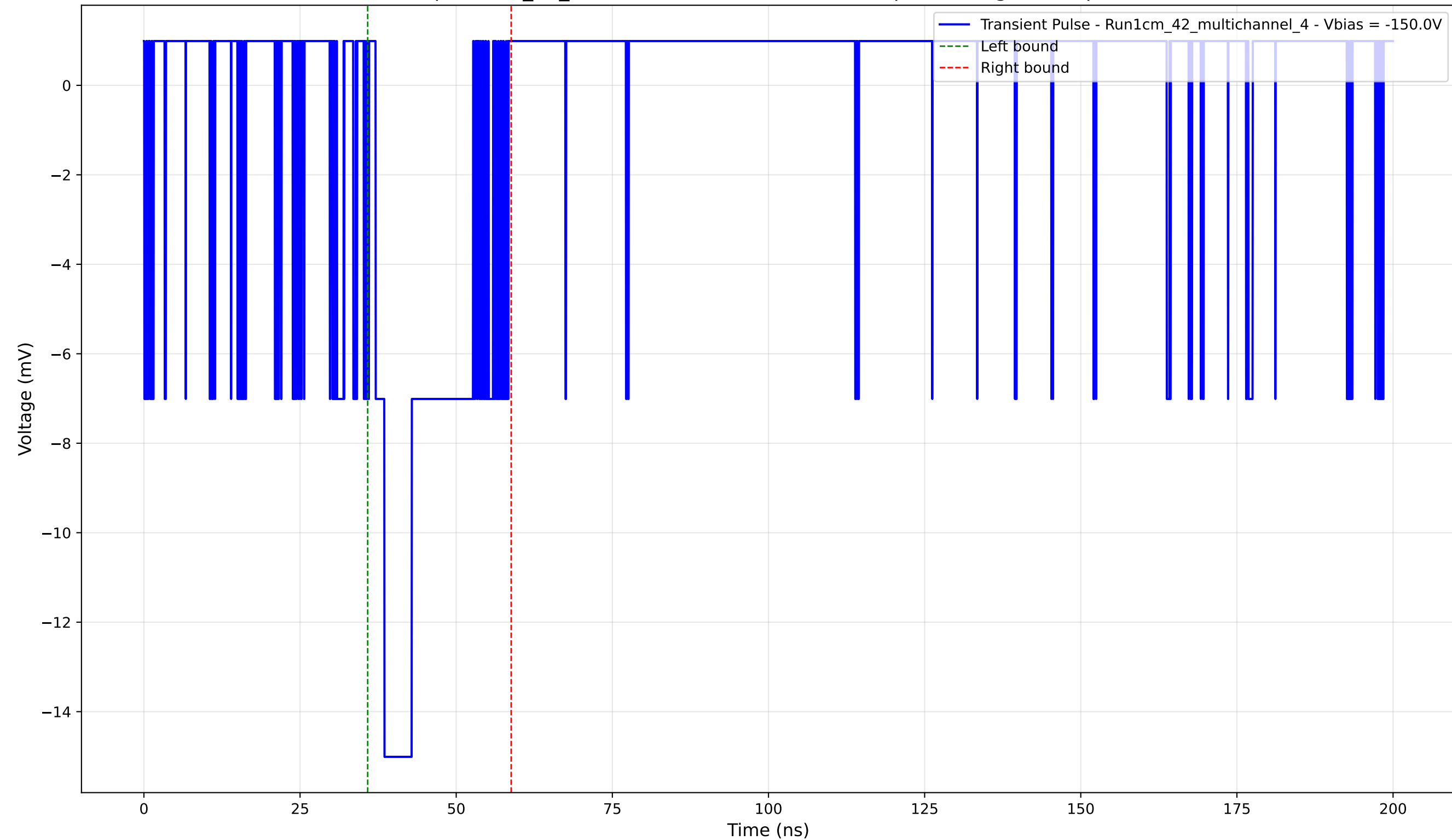
Transient Pulse - Sample: 1cm_42_multichannel - Position: 4315.0 \mu\text{m} - Charge: 3.35 pC - Rise Time: 1.42 ns
