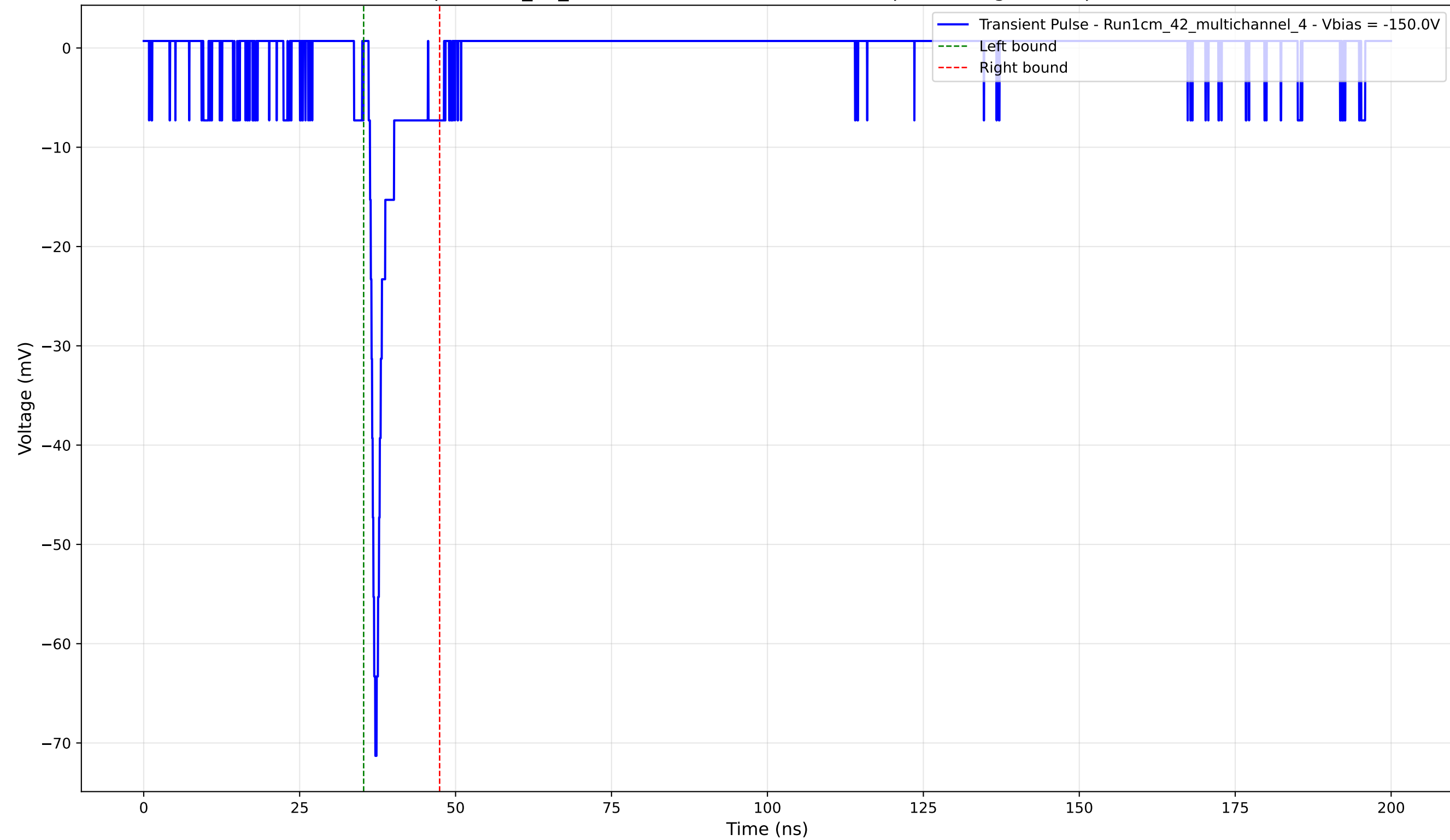
Transient Pulse - Sample: 1cm_42_multichannel - Position: 2320.0 \mu\text{m} - Charge: 3.57 pC - Rise Time: 1.06 ns
