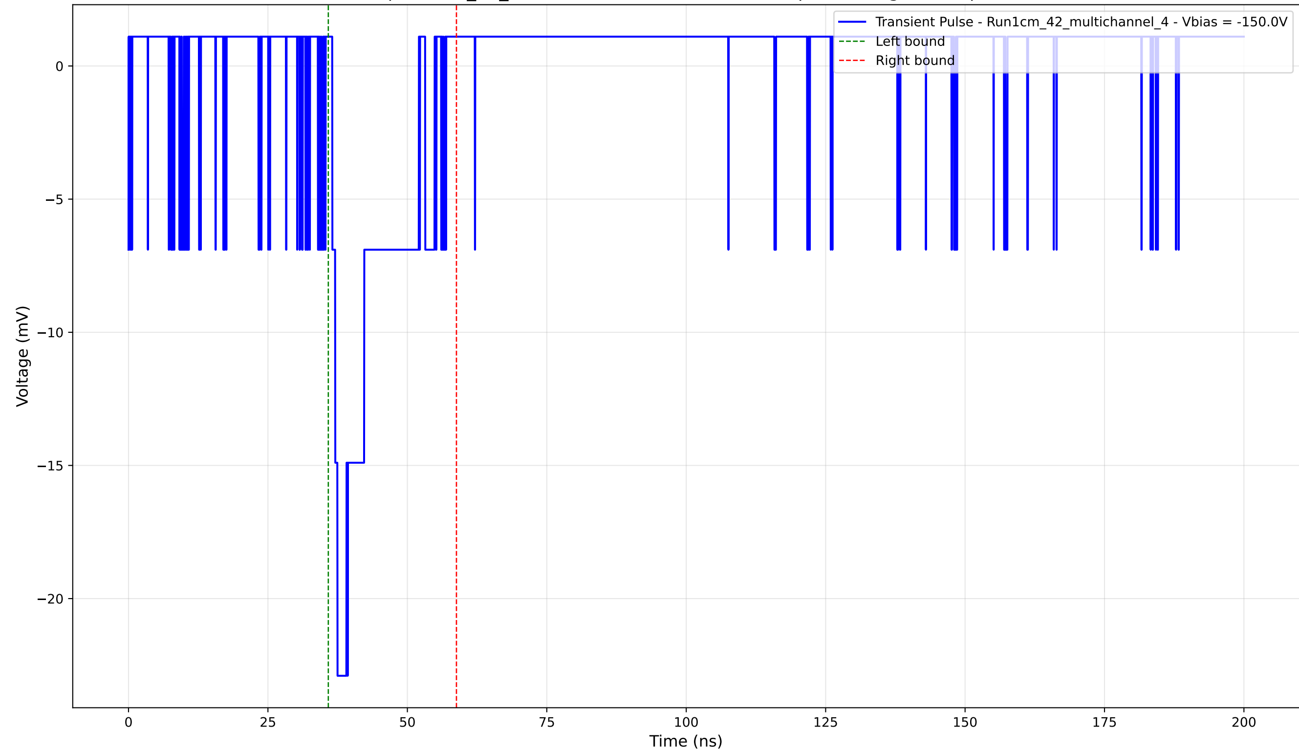
Transient Pulse - Sample: 1cm_42_multichannel - Position: 3325.0 \mu\text{m} - Charge: 3.47 pC - Rise Time: 0.94 ns
