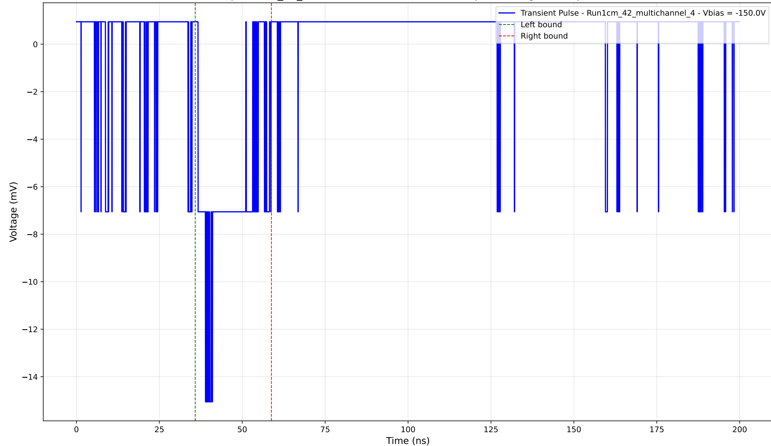
Transient Pulse - Sample: 1cm_42_multichannel - Position: 4815.0 \mu\text{m} - Charge: 2.76 pC - Rise Time: 2.24 ns
