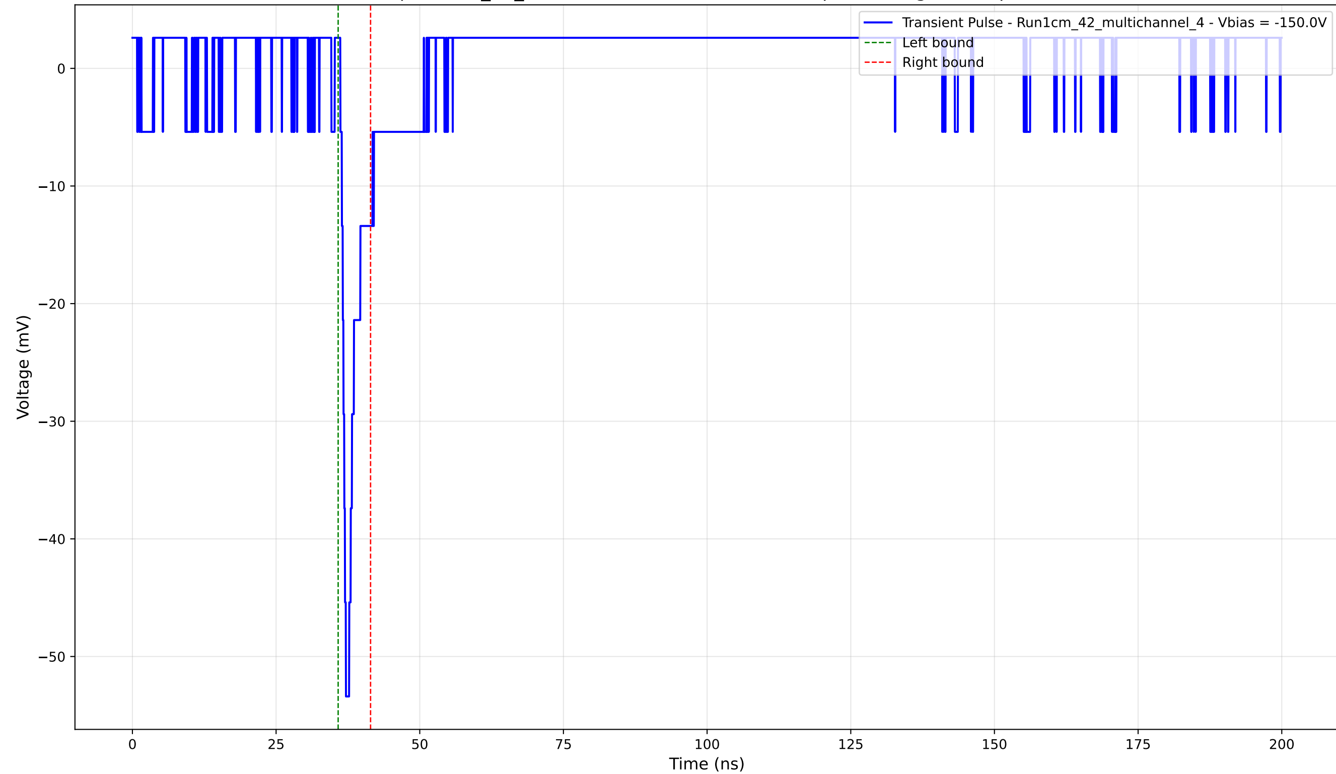
Transient Pulse - Sample: 1cm_42_multichannel - Position: 2715.0 \mu\text{m} - Charge: 2.60 pC - Rise Time: 0.96 ns
