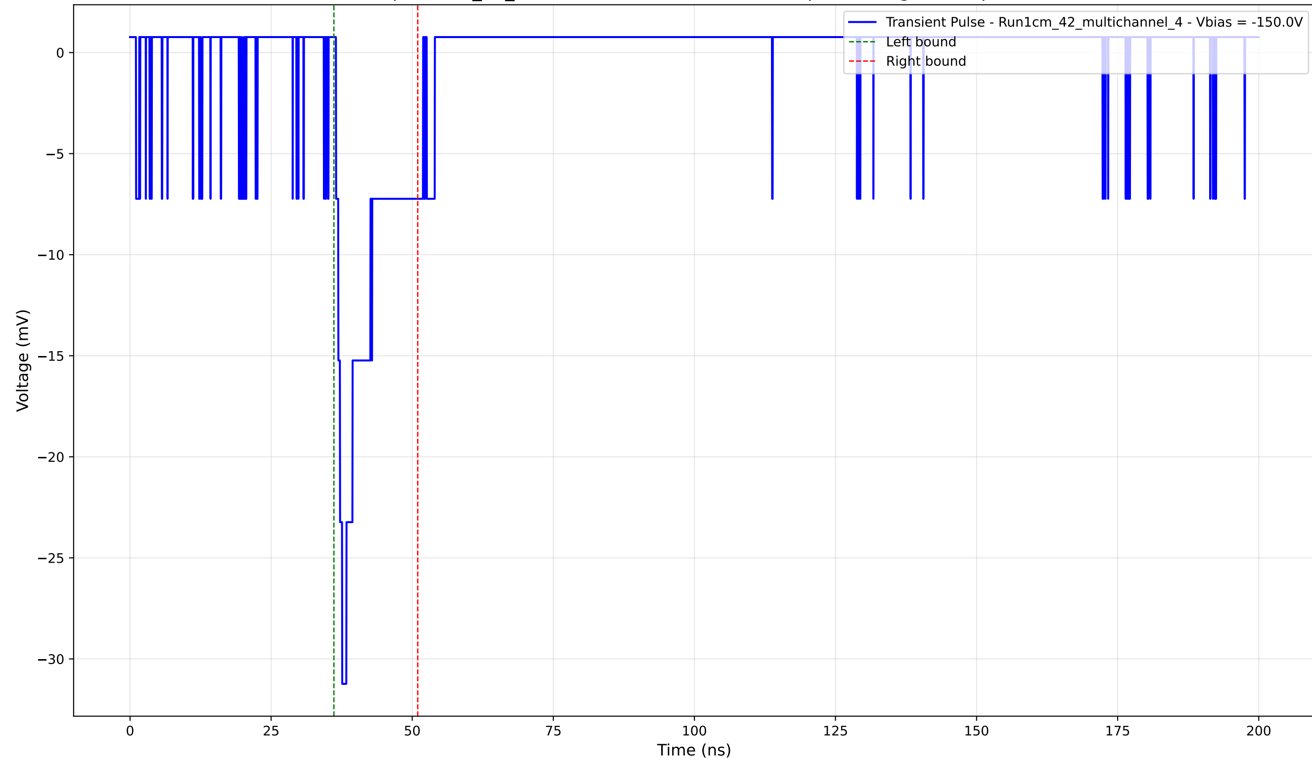
Transient Pulse - Sample: 1cm_42_multichannel - Position: 3200.0 \mu\text{m} - Charge: 3.49 pC - Rise Time: 1.09 ns
