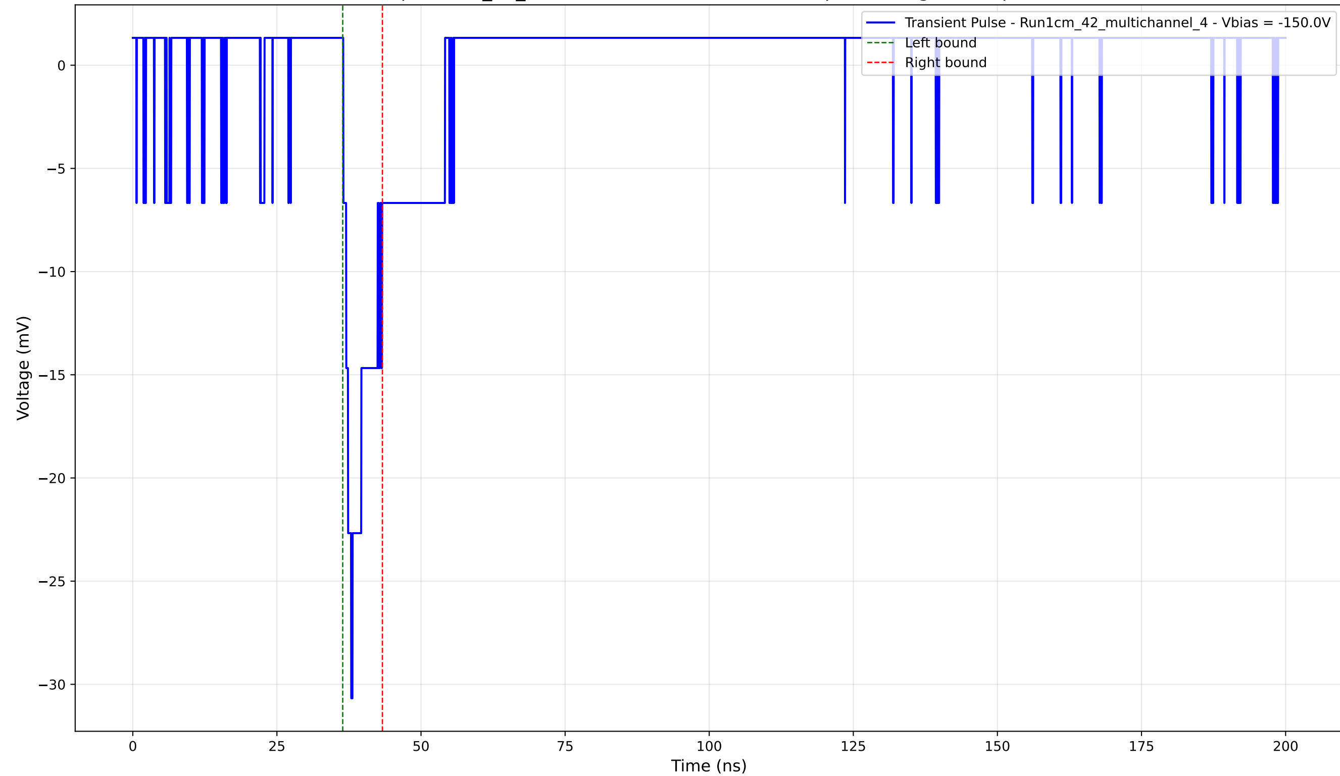
Transient Pulse - Sample: 1cm_42_multichannel - Position: 3305.0 \mu\text{m} - Charge: 2.24 pC - Rise Time: 1.37 ns
