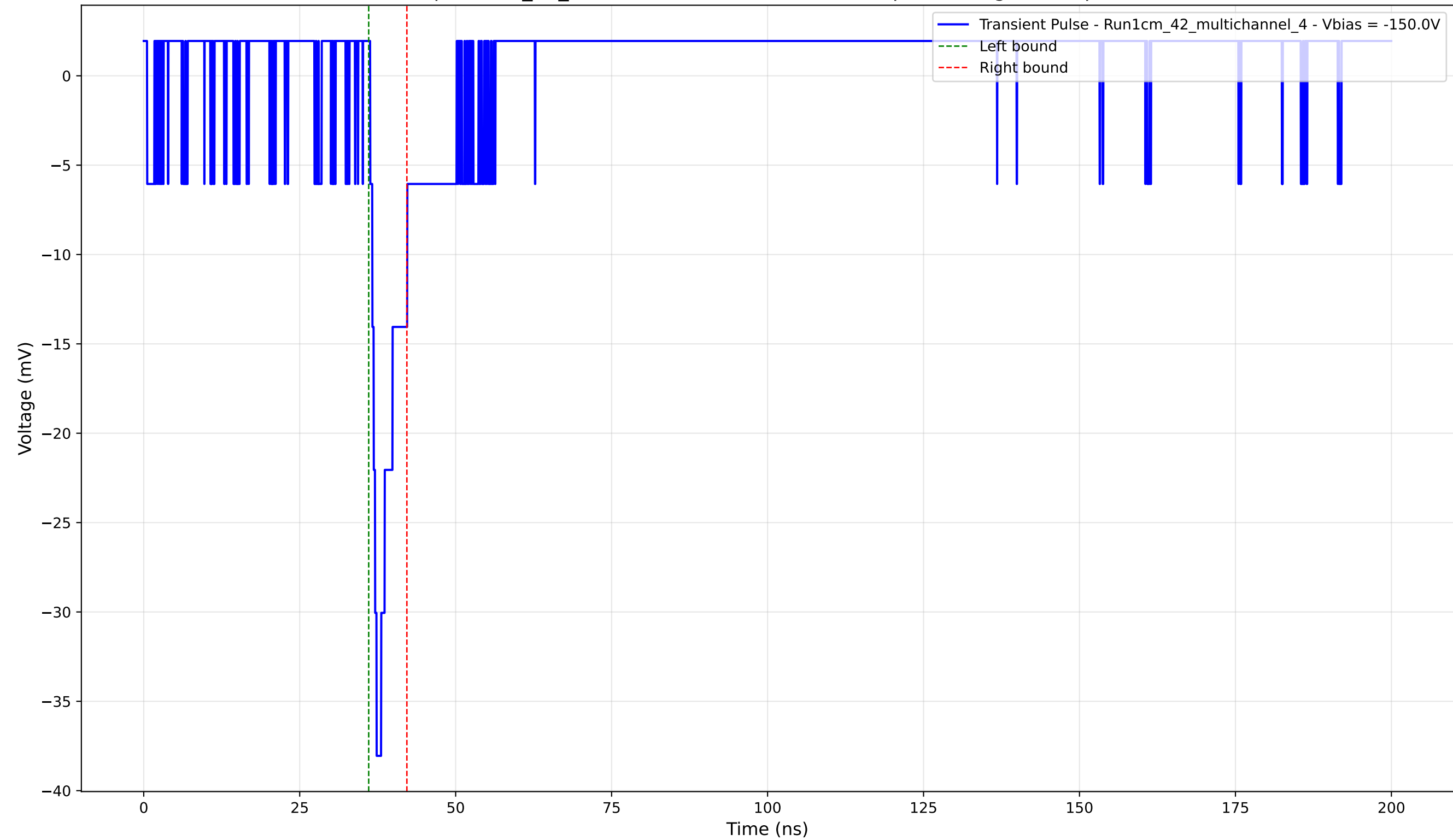
Transient Pulse - Sample: 1cm_42_multichannel - Position: 3005.0 \mu\text{m} - Charge: 2.44 pC - Rise Time: 1.03 ns
