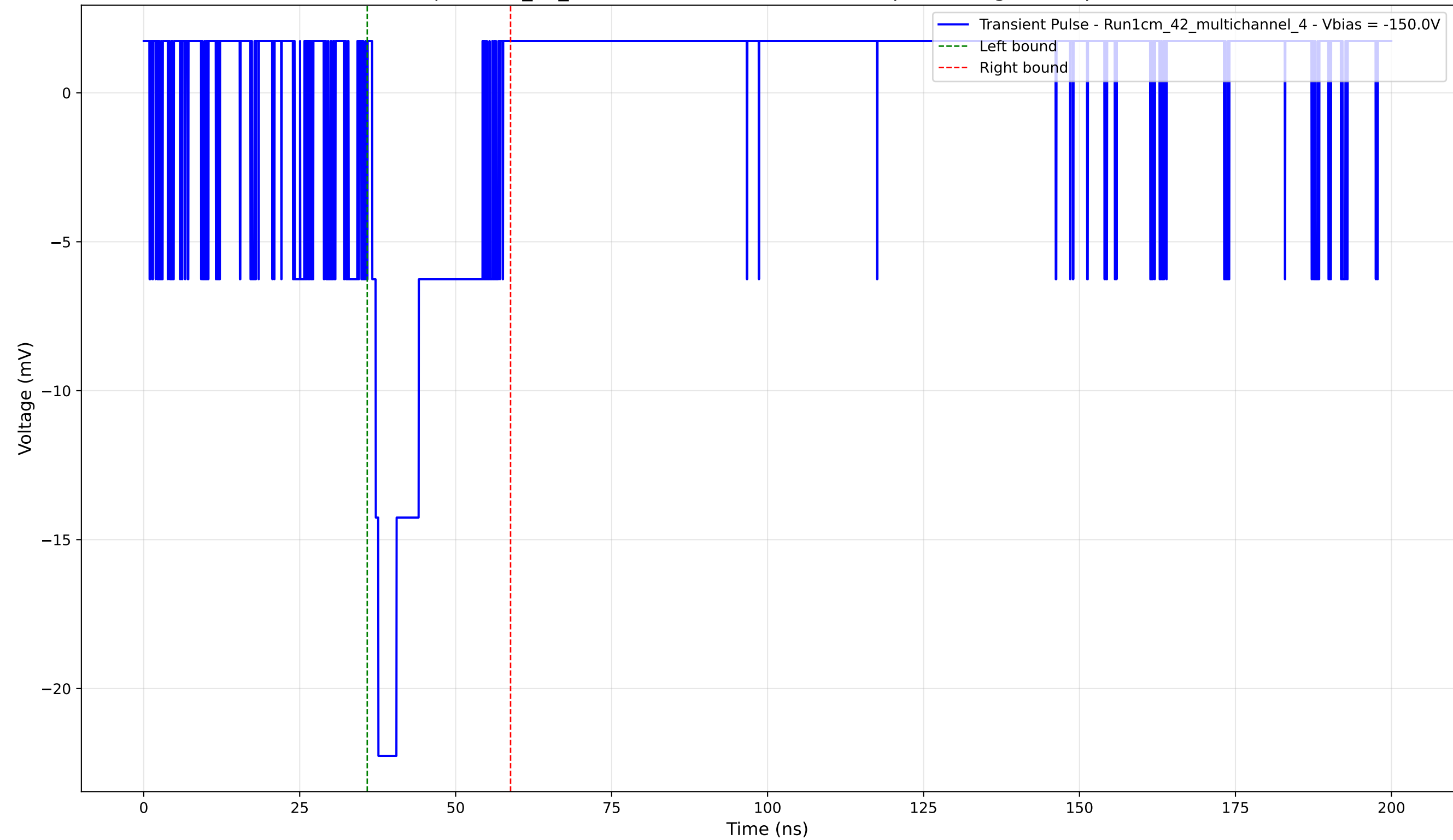
Transient Pulse - Sample: 1cm_42_multichannel - Position: 1270.0 \mu\text{m} - Charge: 3.92 pC - Rise Time: 1.00 ns
