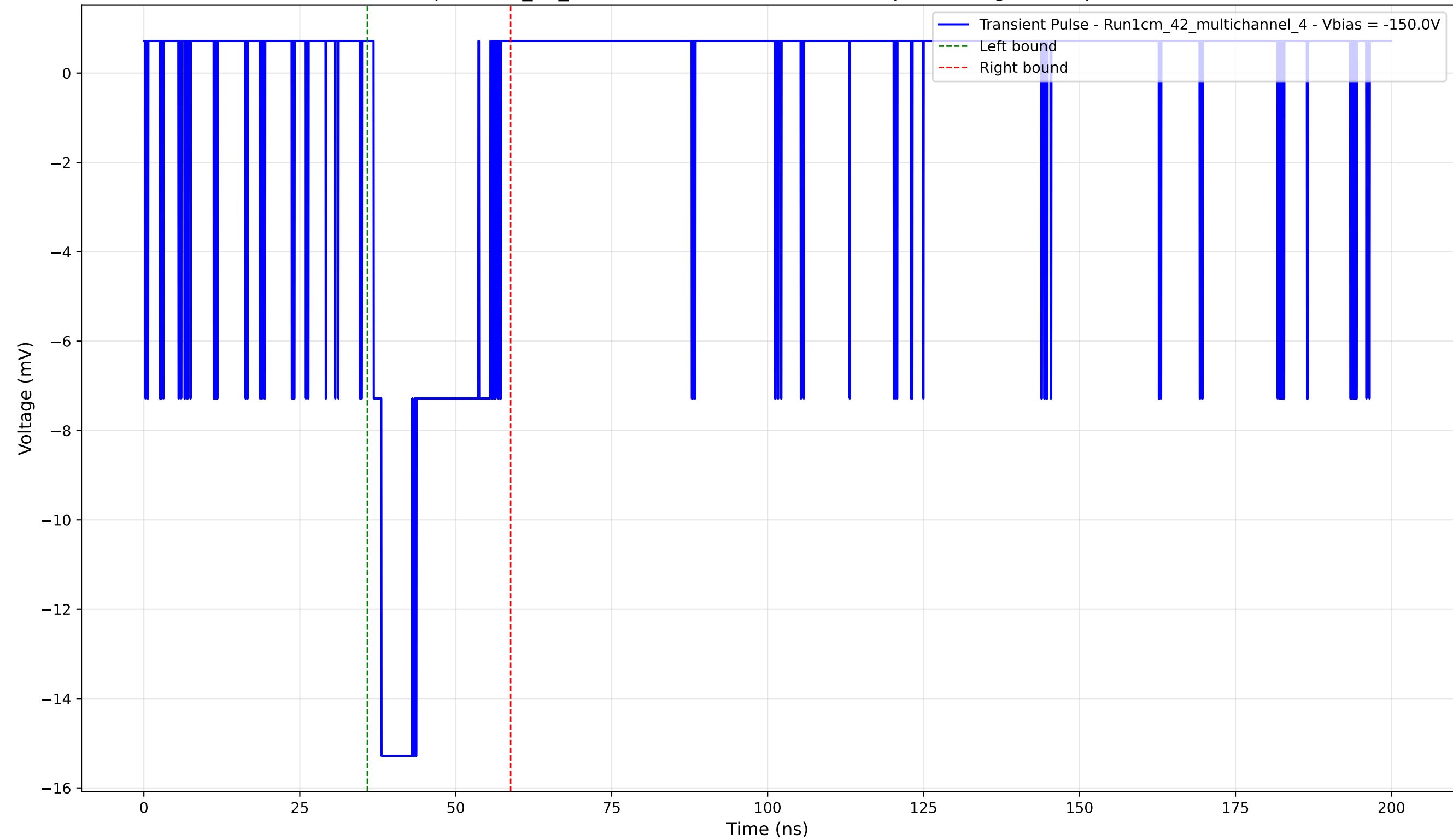
Transient Pulse - Sample: 1cm_42_multichannel - Position: 4115.0 \mu\text{m} - Charge: 3.61 pC - Rise Time: 1.26 ns
