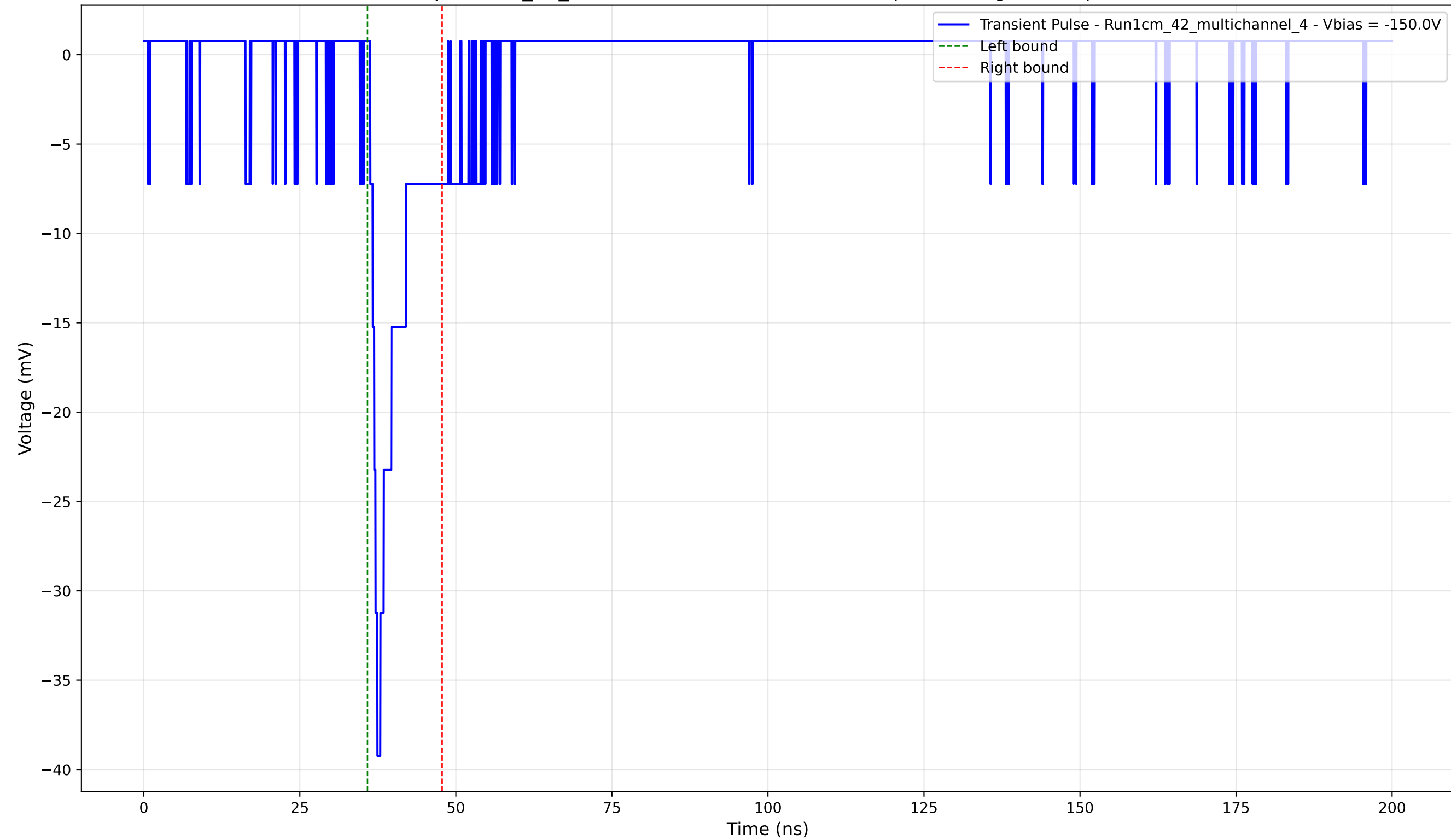
Transient Pulse - Sample: 1cm_42_multichannel - Position: 3020.0 \mu\text{m} - Charge: 3.24 pC - Rise Time: 1.15 ns
