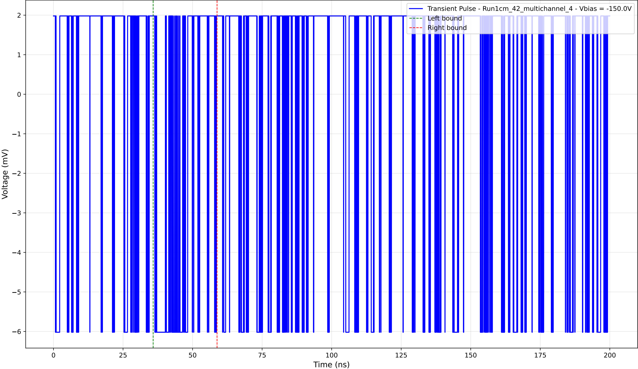
Transient Pulse - Sample: 1cm_42_multichannel - Position: 1390.0 \mu\text{m} - Charge: 0.72 pC - Rise Time: 0.00 ns (N/A)
