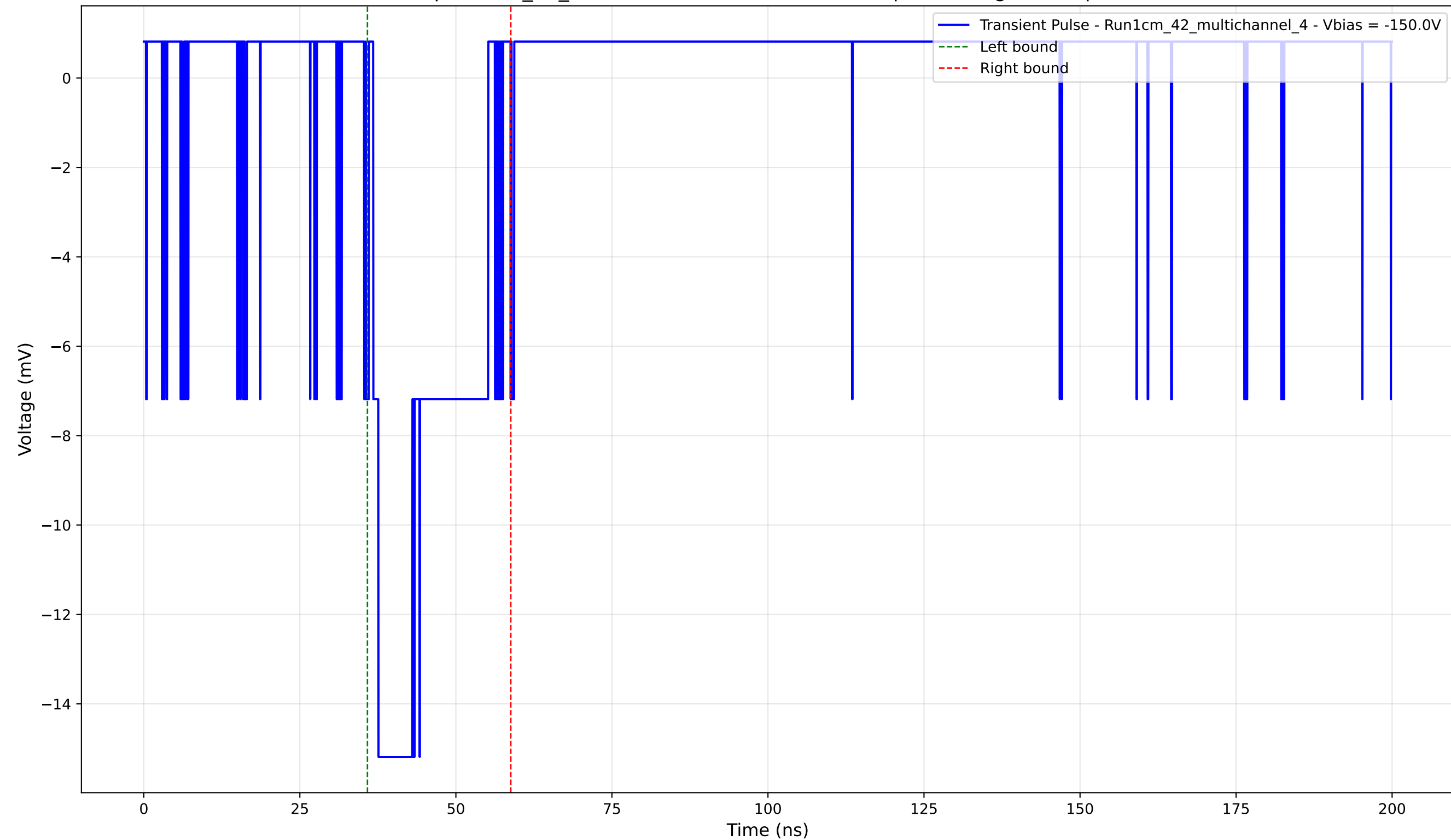
Transient Pulse - Sample: 1cm_42_multichannel - Position: 3785.0 \mu\text{m} - Charge: 3.61 pC - Rise Time: 0.84 ns
