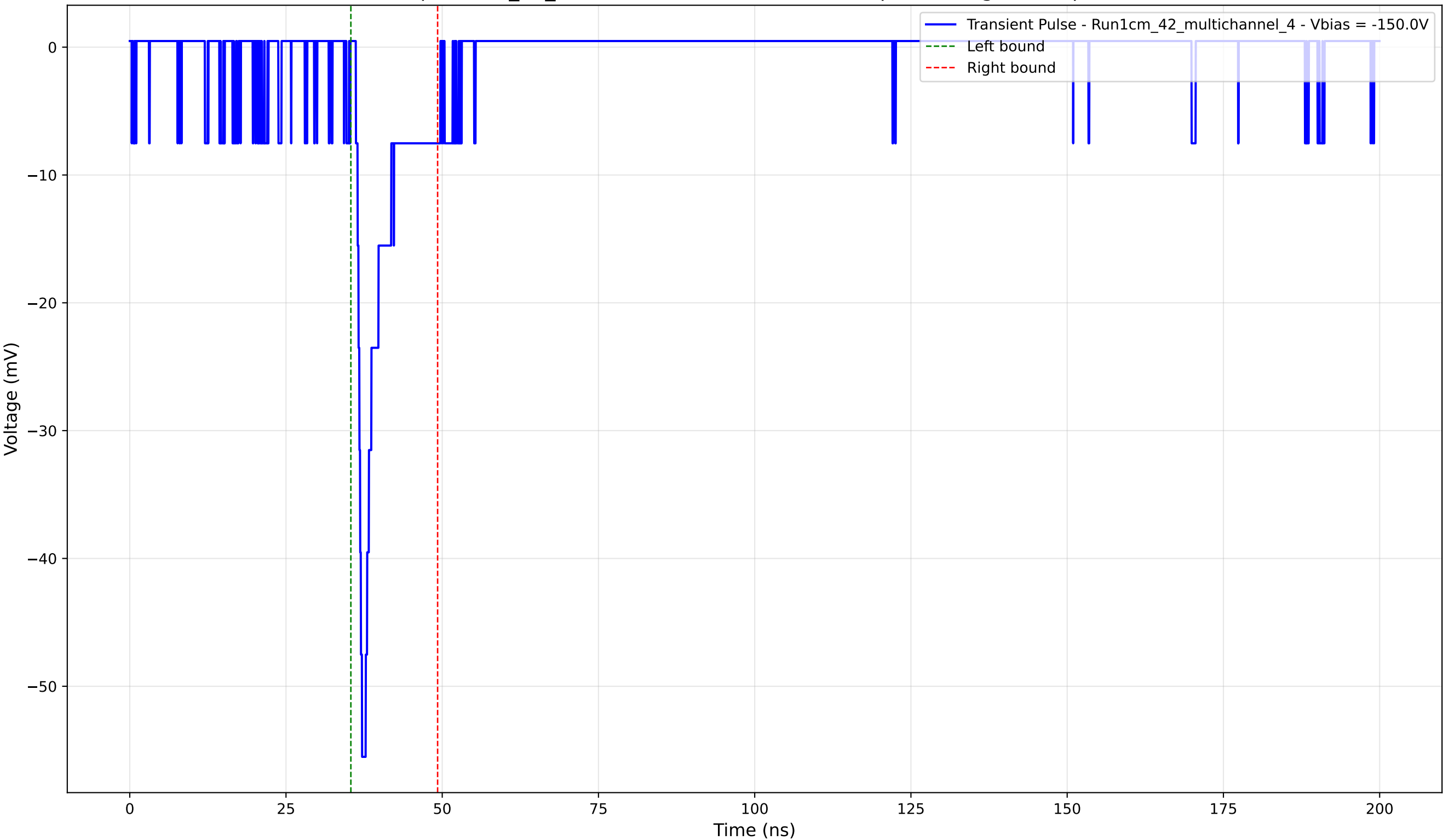
Transient Pulse - Sample: 1cm_42_multichannel - Position: 2735.0 \mu\text{m} - Charge: 4.12 pC - Rise Time: 0.99 ns
