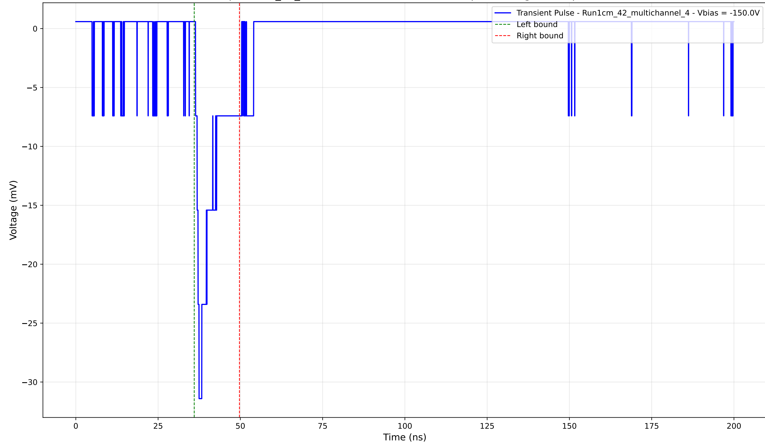
Transient Pulse - Sample: 1cm_42_multichannel - Position: 3180.0 \mu\text{m} - Charge: 3.43 pC - Rise Time: 1.07 ns
