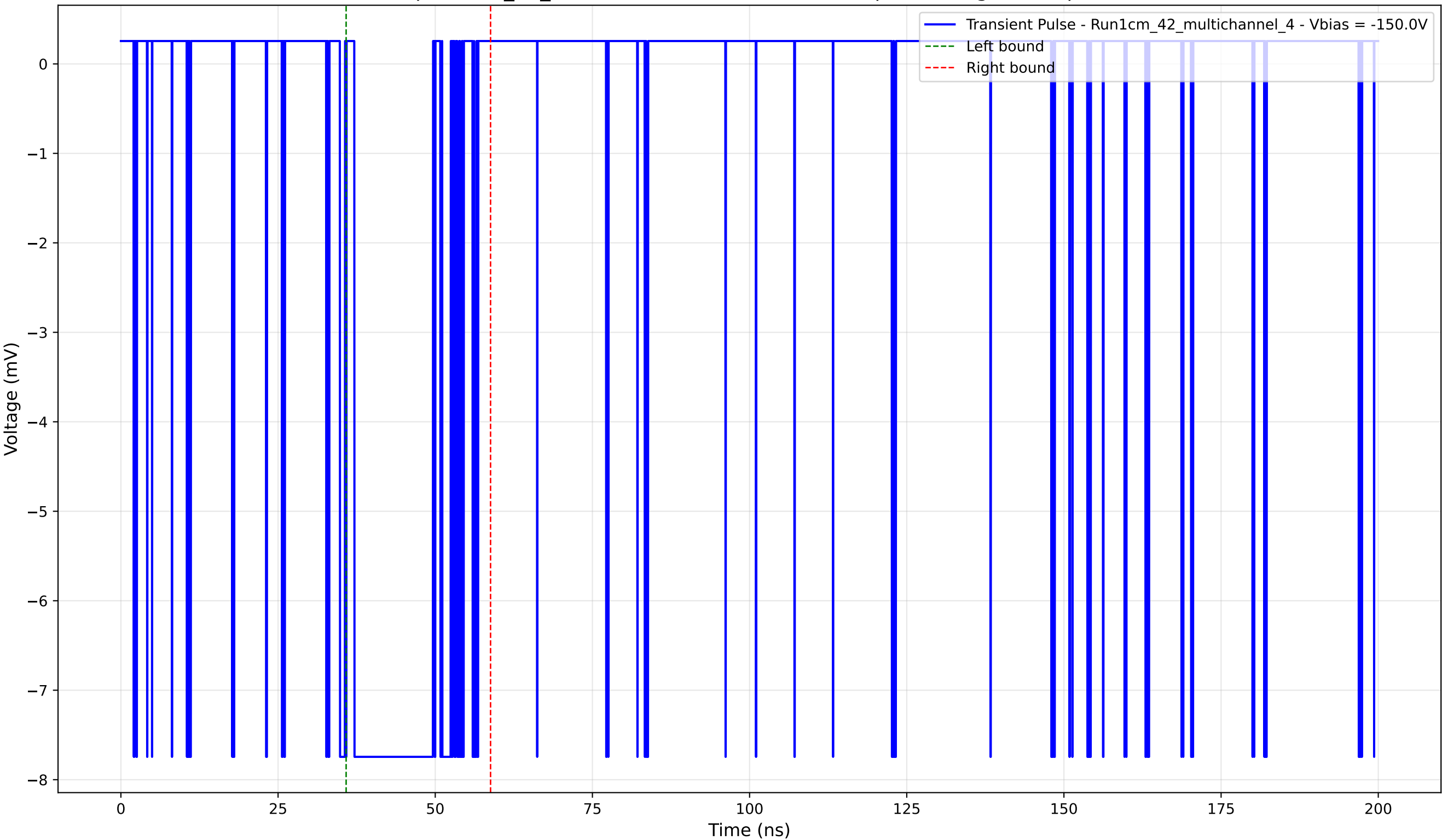
Transient Pulse - Sample: 1cm_42_multichannel - Position: 3855.0 \mu\text{m} - Charge: 2.44 pC - Rise Time: 0.02 ns
