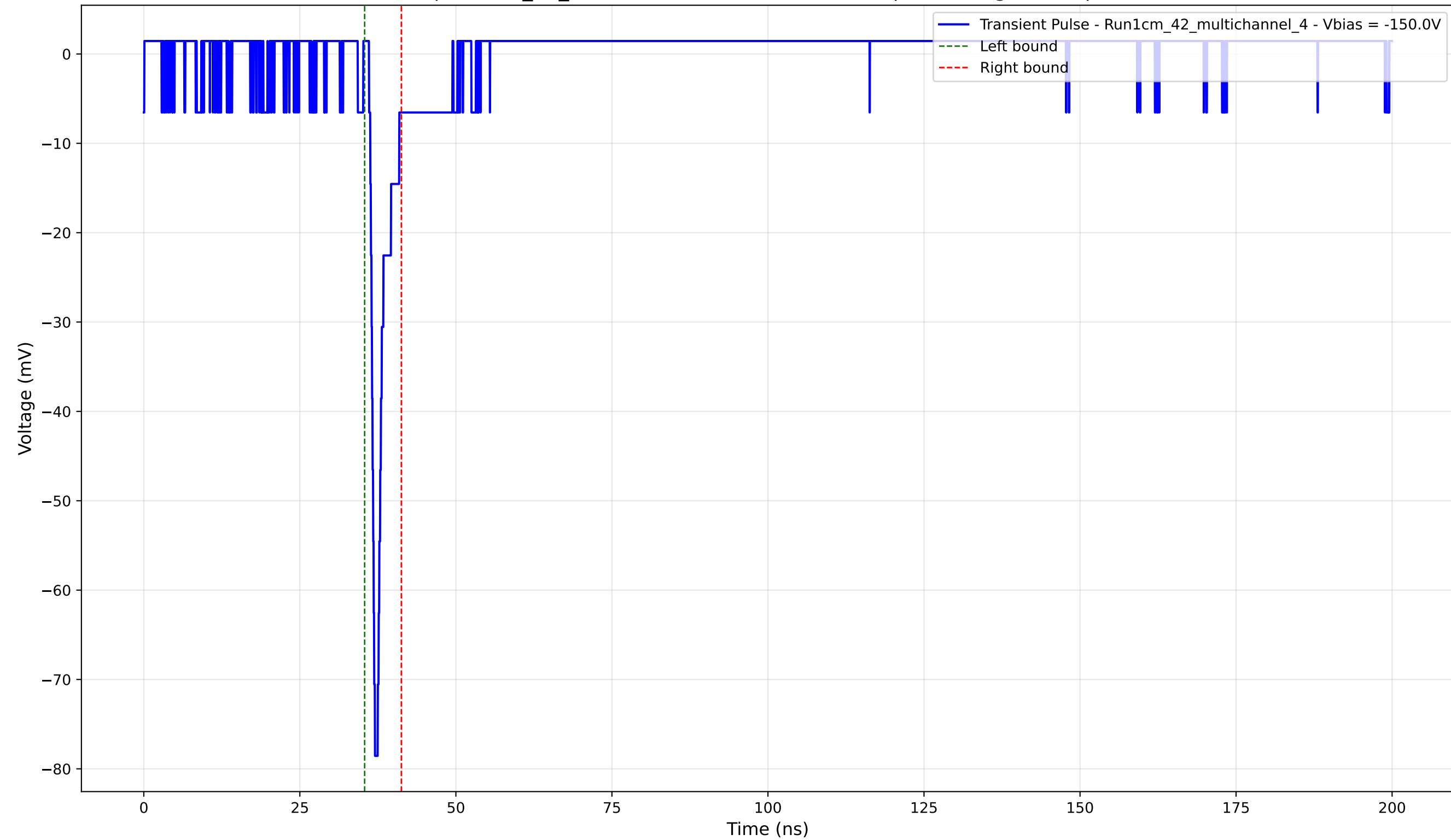
Transient Pulse - Sample: 1cm_42_multichannel - Position: 2470.0 \mu\text{m} - Charge: 3.20 pC - Rise Time: 0.76 ns
