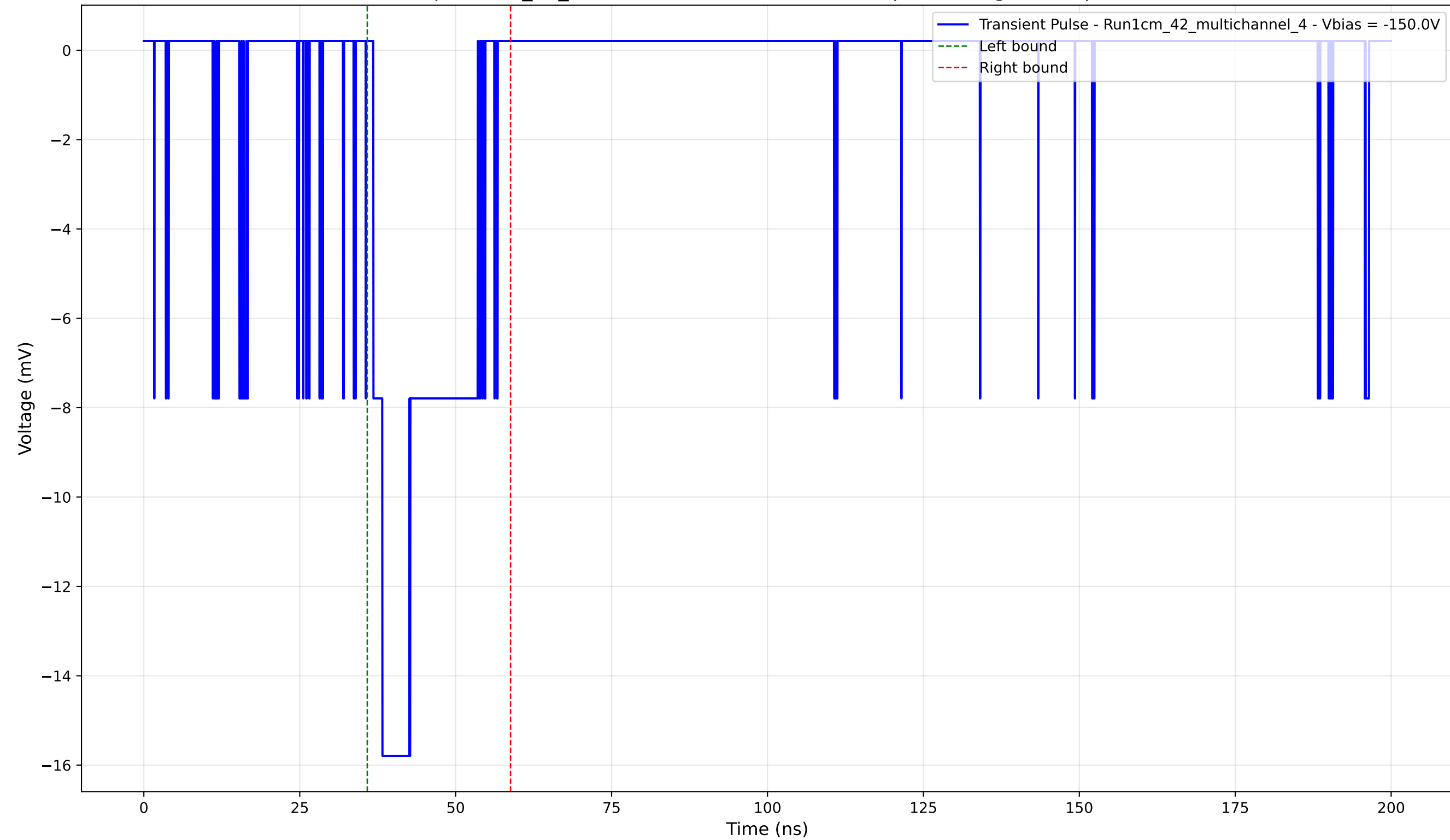
Transient Pulse - Sample: 1cm_42_multichannel - Position: 4100.0 \mu\text{m} - Charge: 3.40 pC - Rise Time: 1.46 ns
