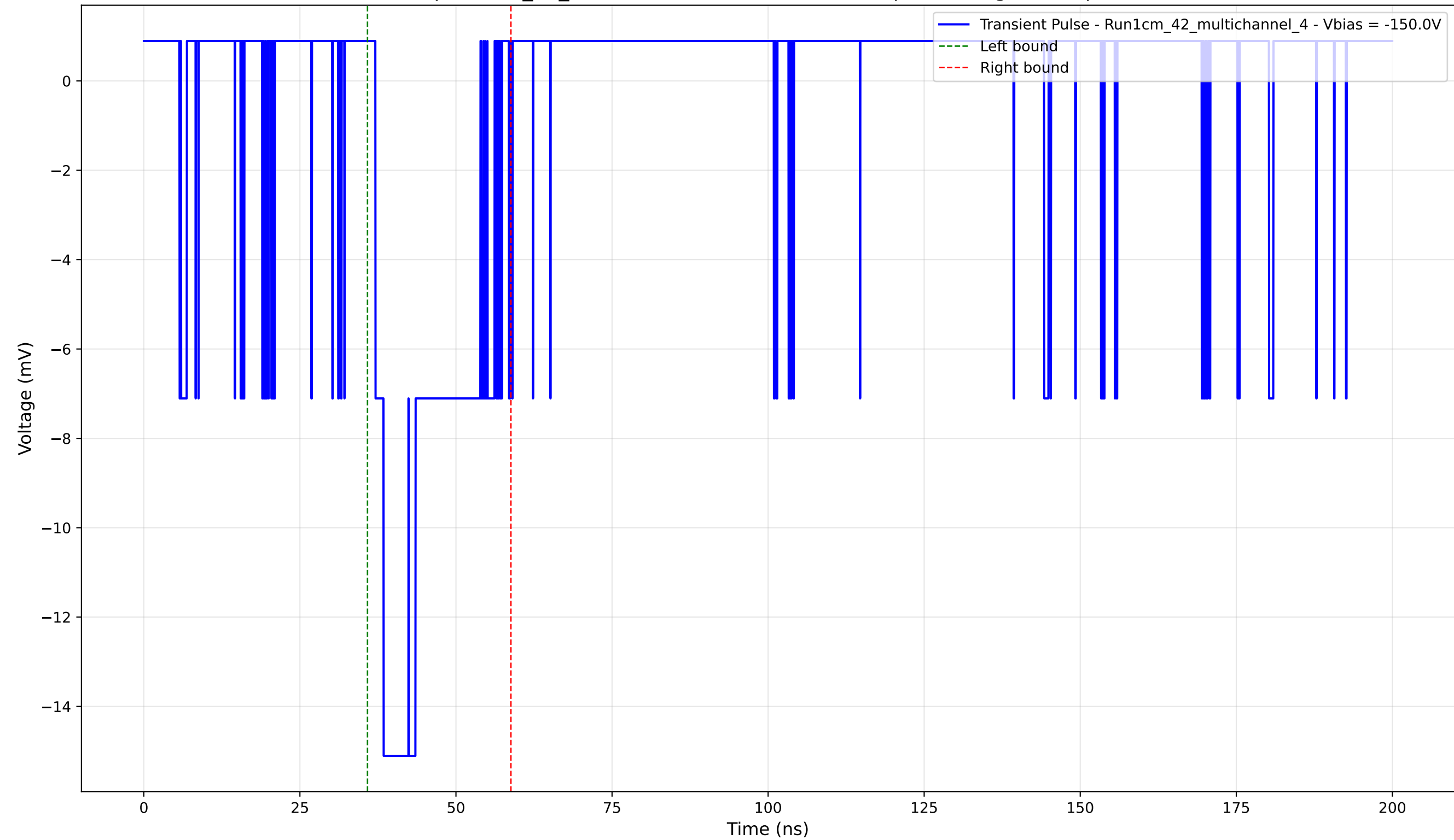
Transient Pulse - Sample: 1cm_42_multichannel - Position: 4255.0 \mu\text{m} - Charge: 3.54 pC - Rise Time: 1.32 ns
