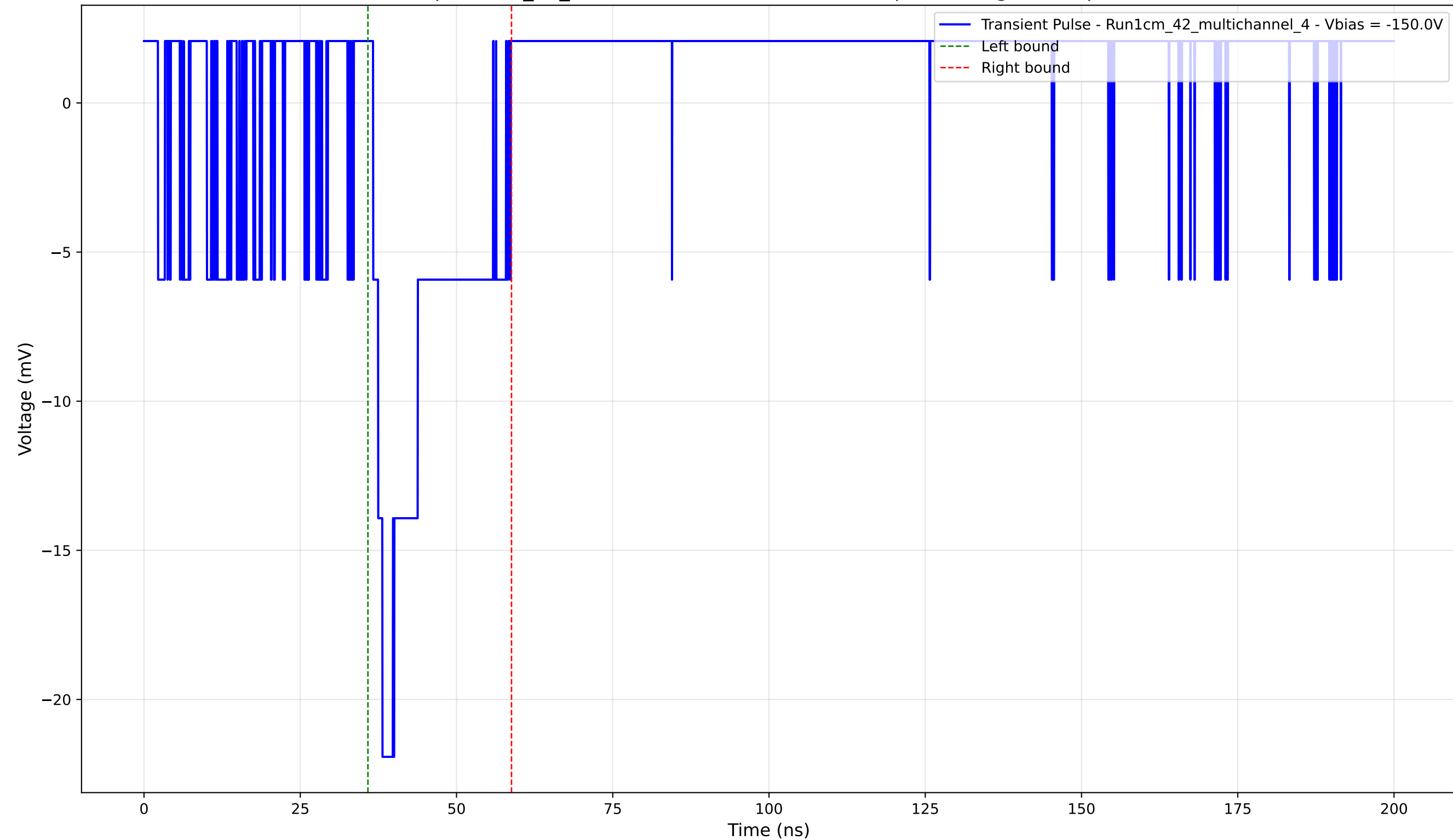
Transient Pulse - Sample: 1cm_42_multichannel - Position: 1105.0 \mu\text{m} - Charge: 3.81 pC - Rise Time: 1.50 ns
