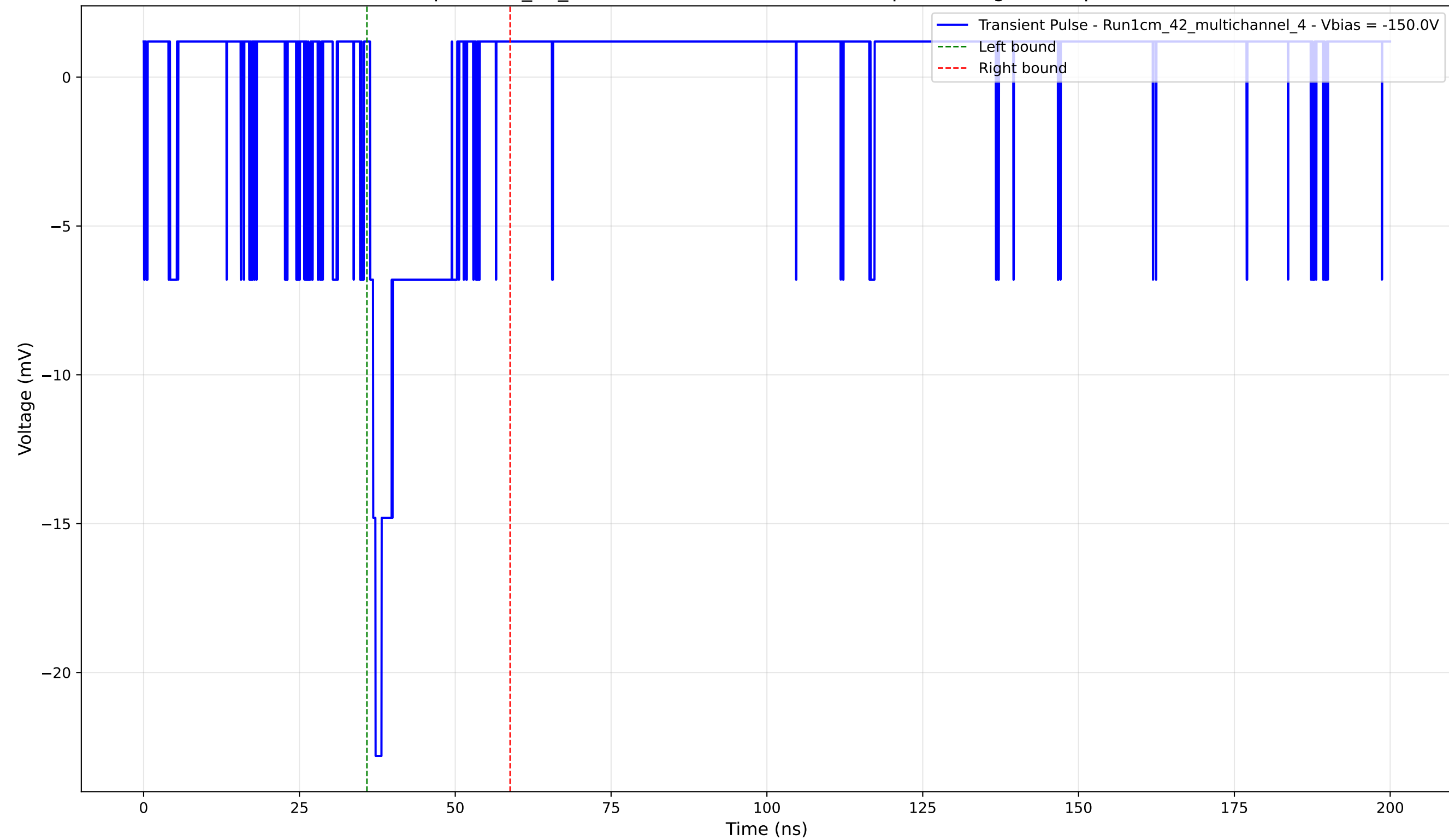
Transient Pulse - Sample: 1cm_42_multichannel - Position: 2945.0 \mu\text{m} - Charge: 2.44 pC - Rise Time: 0.88 ns
