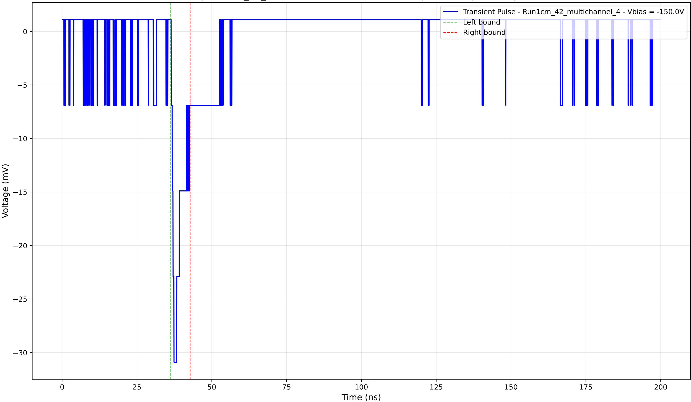
Transient Pulse - Sample: 1cm_42_multichannel - Position: 3105.0 \mu\text{m} - Charge: 2.20 pC - Rise Time: 0.93 ns
