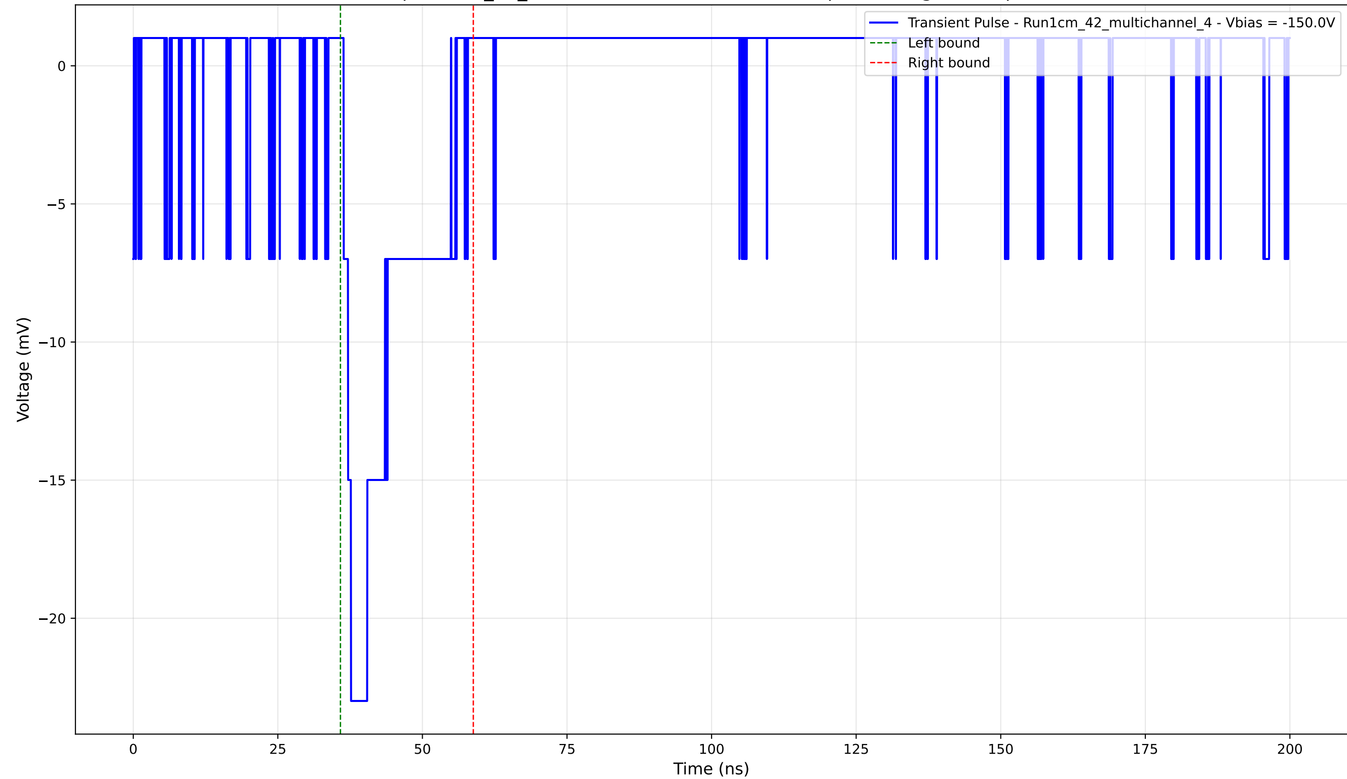
Transient Pulse - Sample: 1cm_42_multichannel - Position: 1265.0 \mu\text{m} - Charge: 4.16 pC - Rise Time: 1.28 ns
