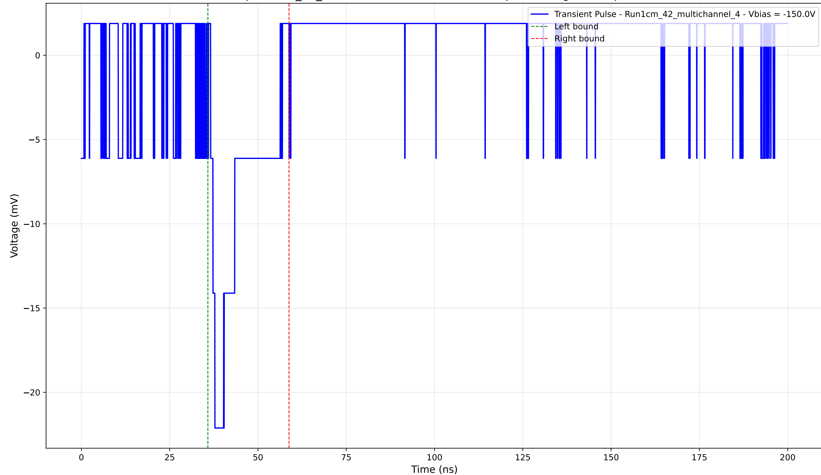
Transient Pulse - Sample: 1cm_42_multichannel - Position: 1185.0 \mu\text{m} - Charge: 3.77 pC - Rise Time: 1.22 ns
