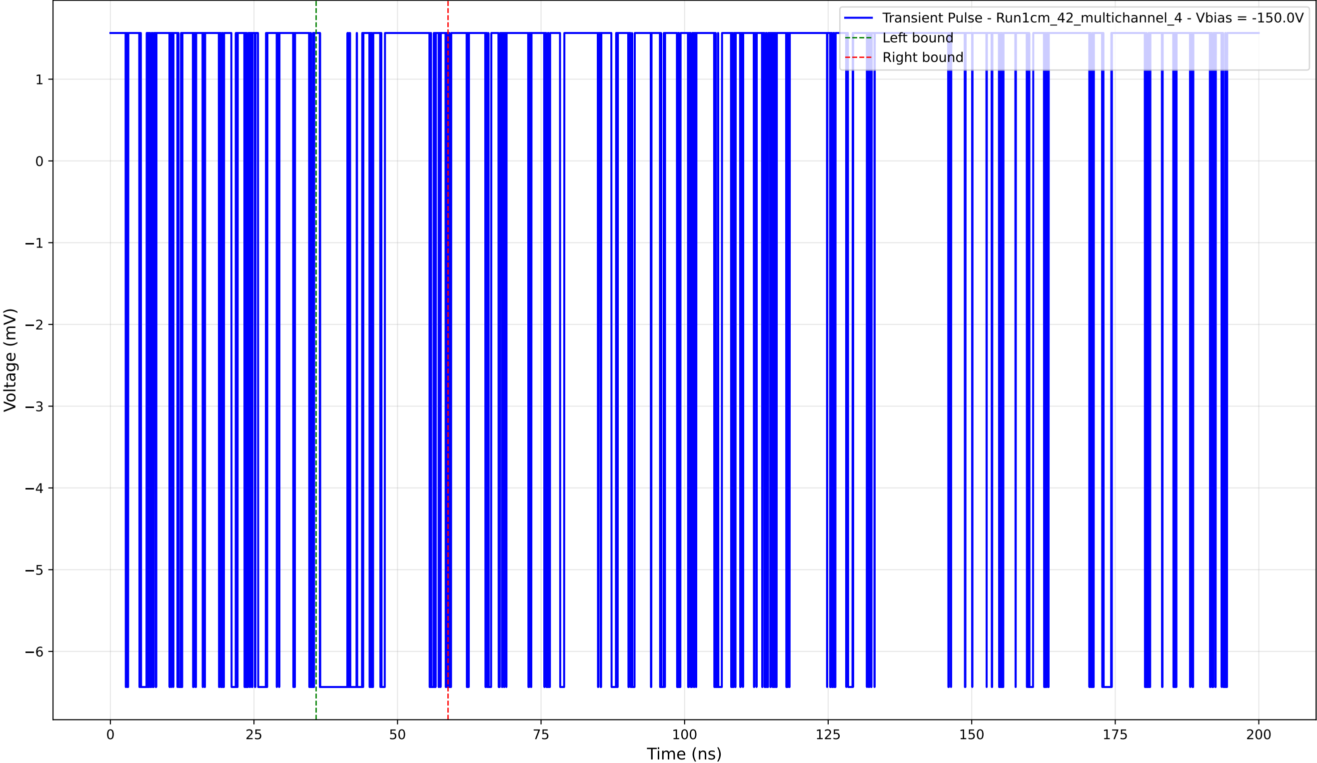
Transient Pulse - Sample: 1cm_42_multichannel - Position: 2860.0 \mu\text{m} - Charge: 0.78 pC - Rise Time: 0.00 ns (N/A)
