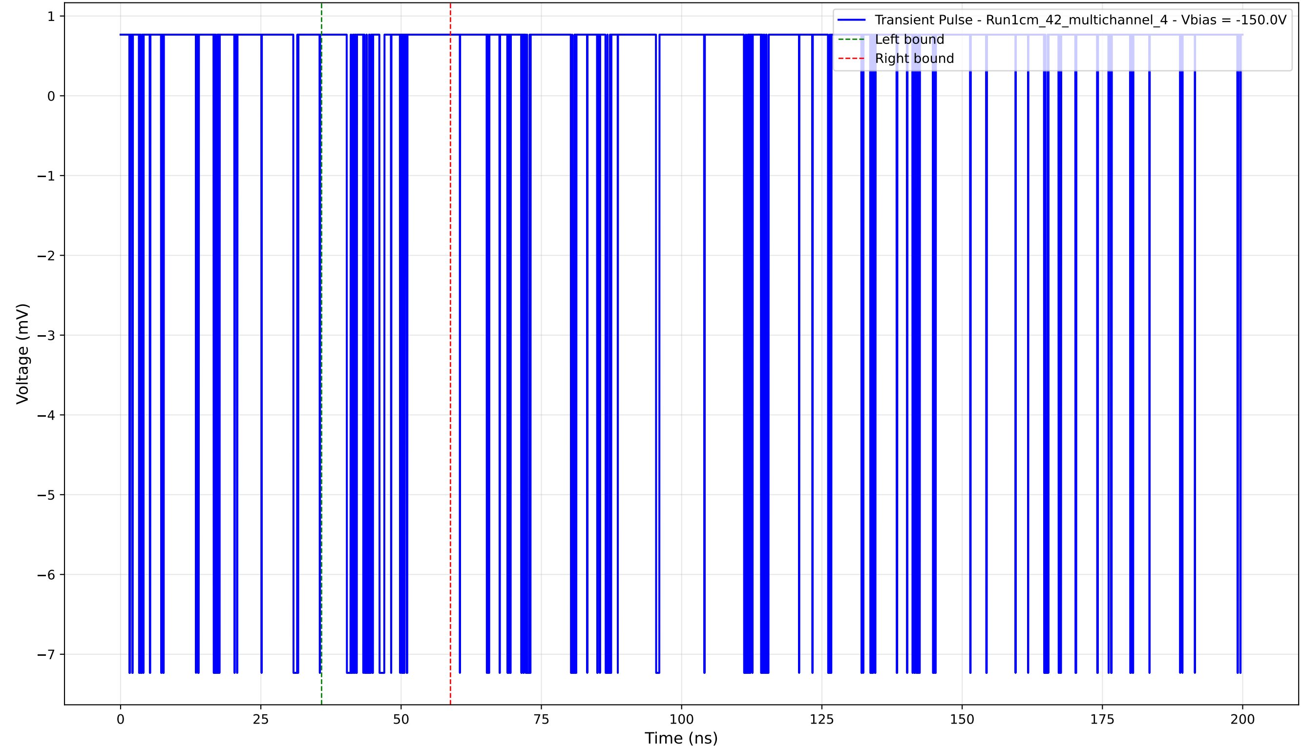
Transient Pulse - Sample: 1cm_42_multichannel - Position: 3885.0 \mu\text{m} - Charge: 0.26 pC - Rise Time: 0.00 ns (N/A)
