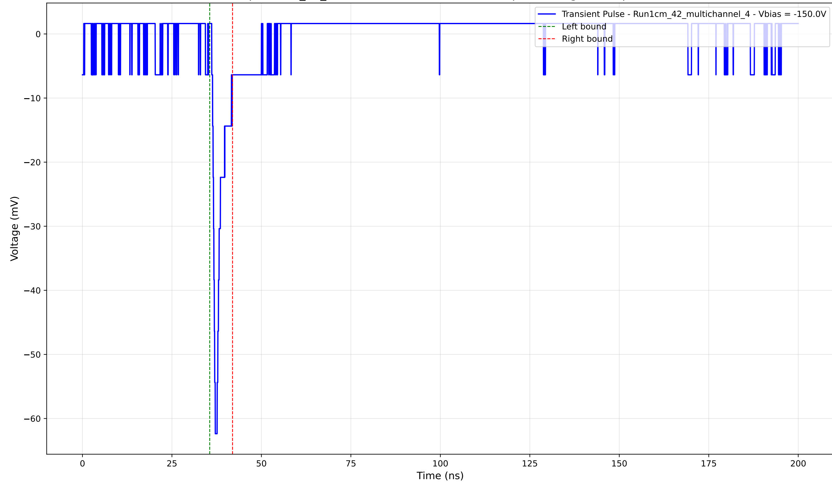
Transient Pulse - Sample: 1cm_42_multichannel - Position: 2150.0 \mu\text{m} - Charge: 3.06 pC - Rise Time: 0.98 ns
