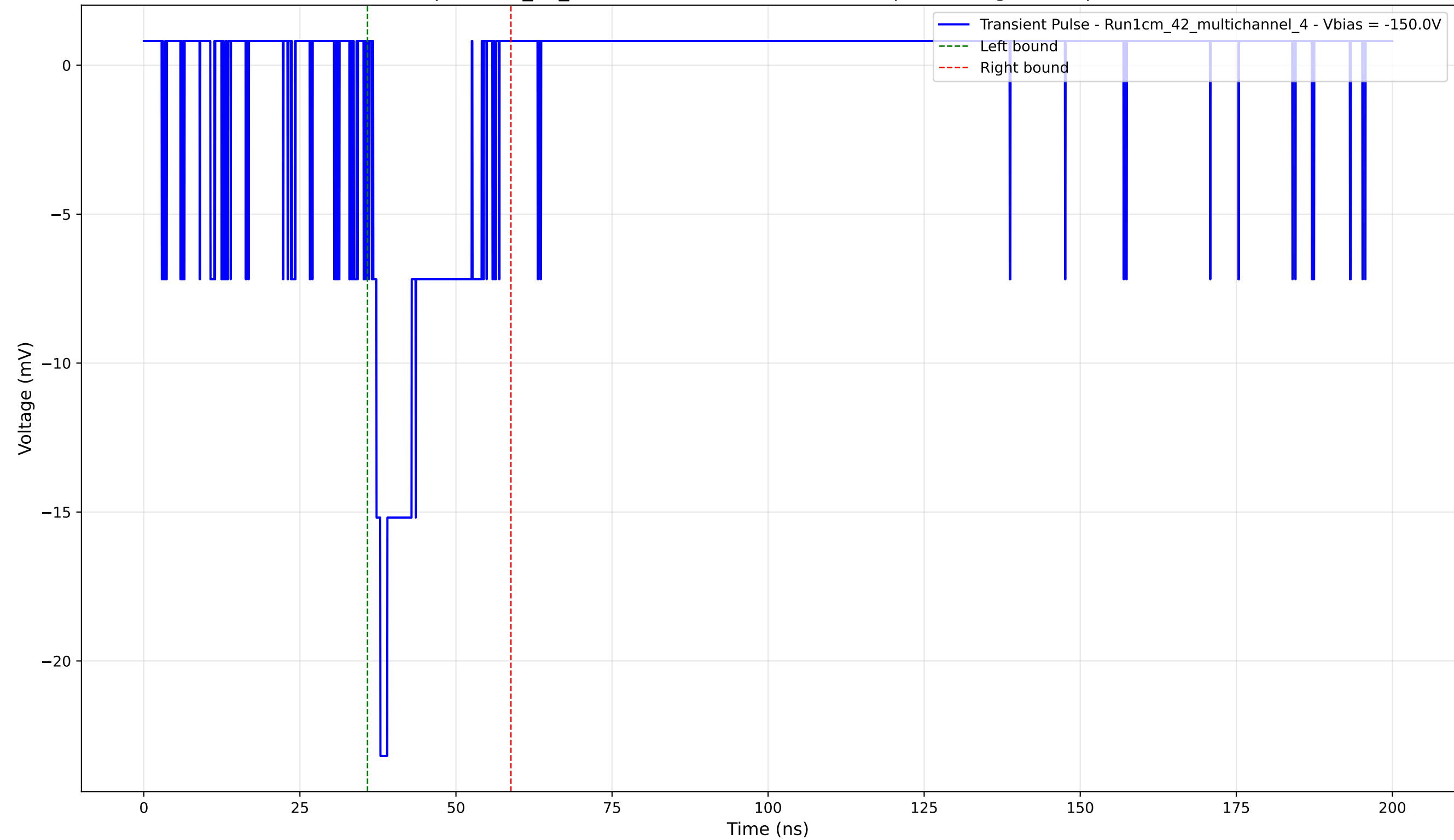
Transient Pulse - Sample: 1cm_42_multichannel - Position: 3535.0 \mu\text{m} - Charge: 3.60 pC - Rise Time: 1.16 ns
