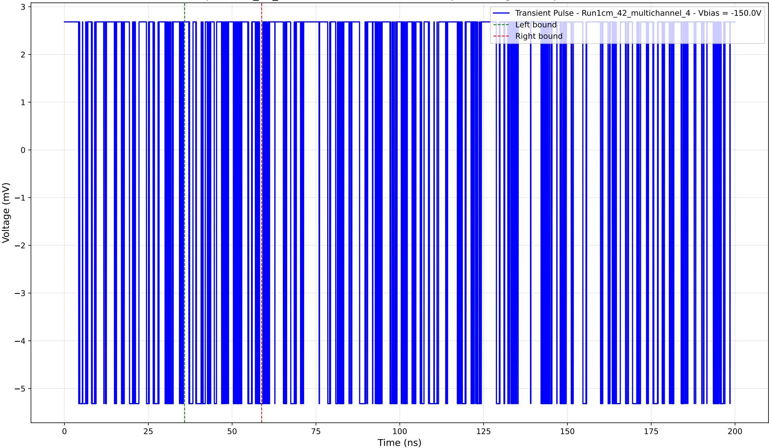
Transient Pulse - Sample: 1cm_42_multichannel - Position: 1375.0 \mu\text{m} - Charge: 0.19 pC - Rise Time: 0.00 ns (N/A)
