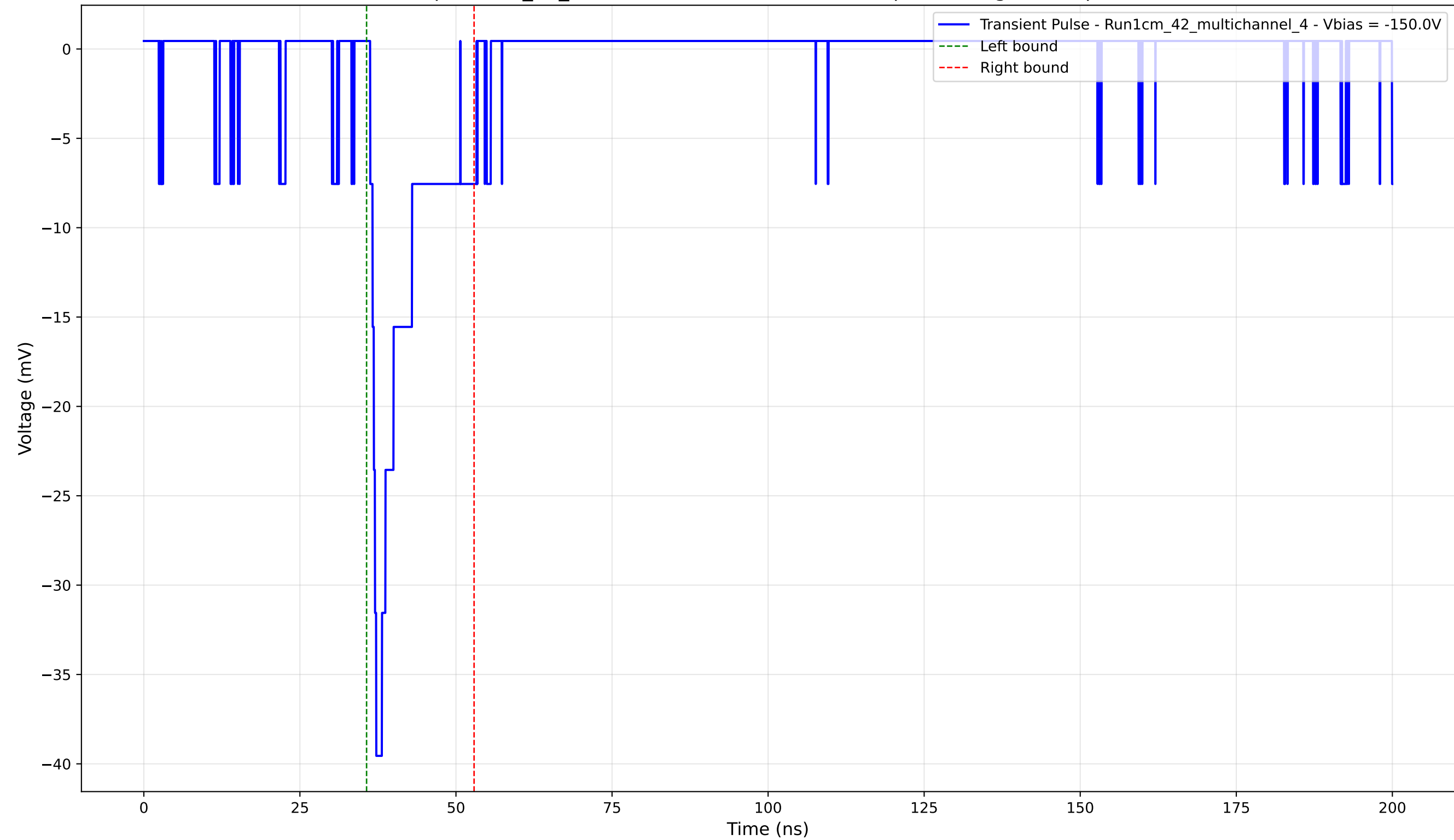
Transient Pulse - Sample: 1cm_42_multichannel - Position: 1790.0 \mu\text{m} - Charge: 4.44 pC - Rise Time: 0.97 ns
