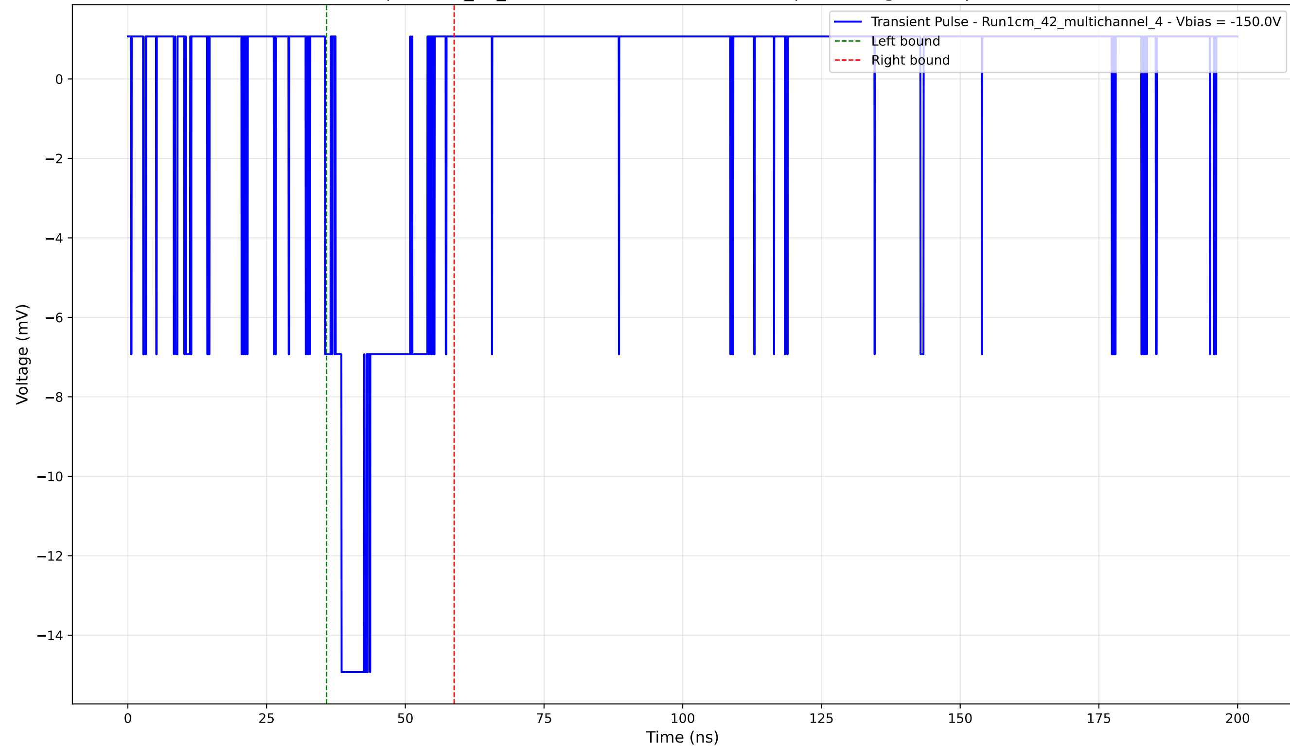
Transient Pulse - Sample: 1cm_42_multichannel - Position: 4525.0 \mu\text{m} - Charge: 3.10 pC - Rise Time: 1.08 ns
