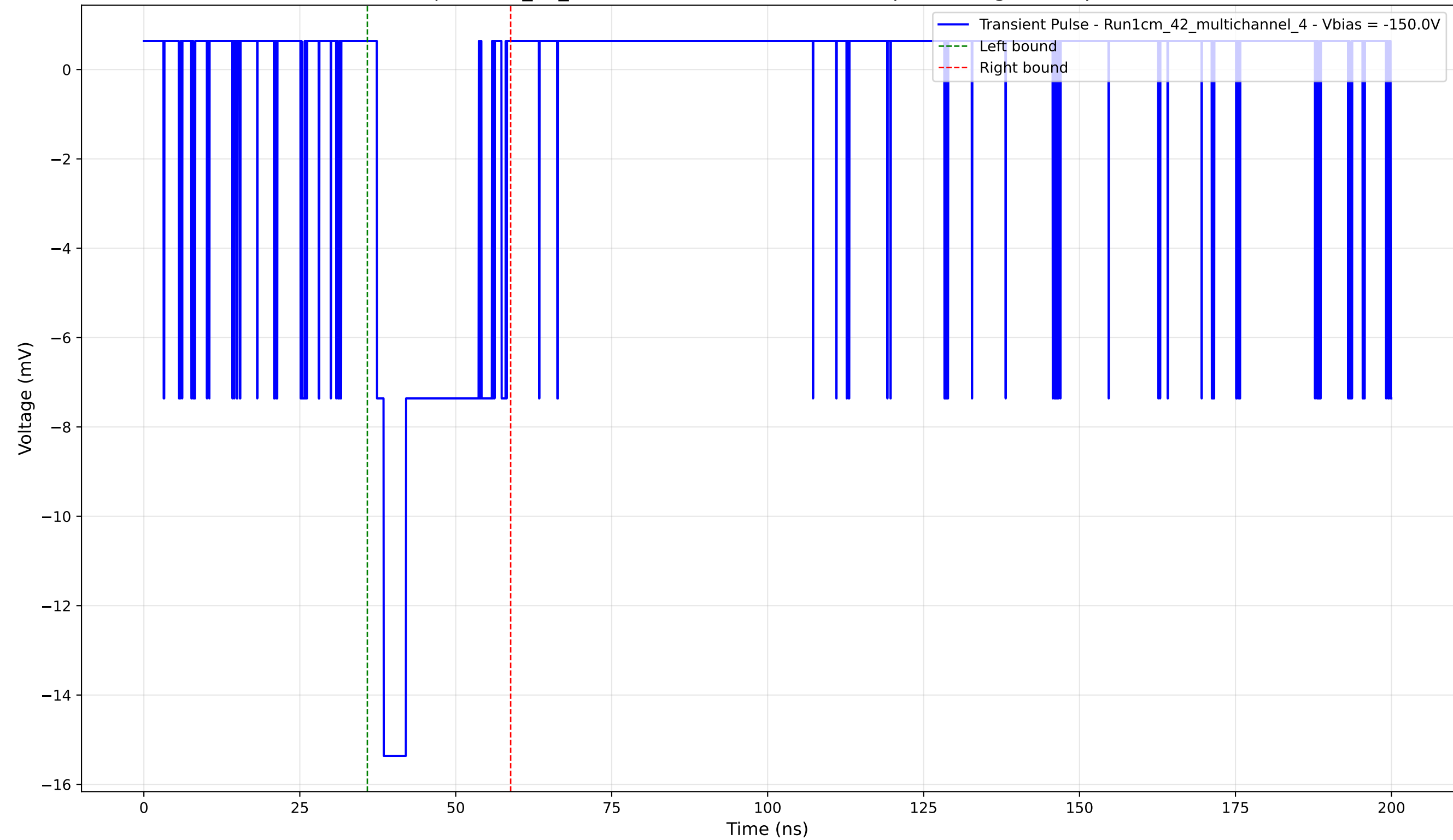
Transient Pulse - Sample: 1cm_42_multichannel - Position: 4330.0 \mu\text{m} - Charge: 3.33 pC - Rise Time: 1.10 ns
