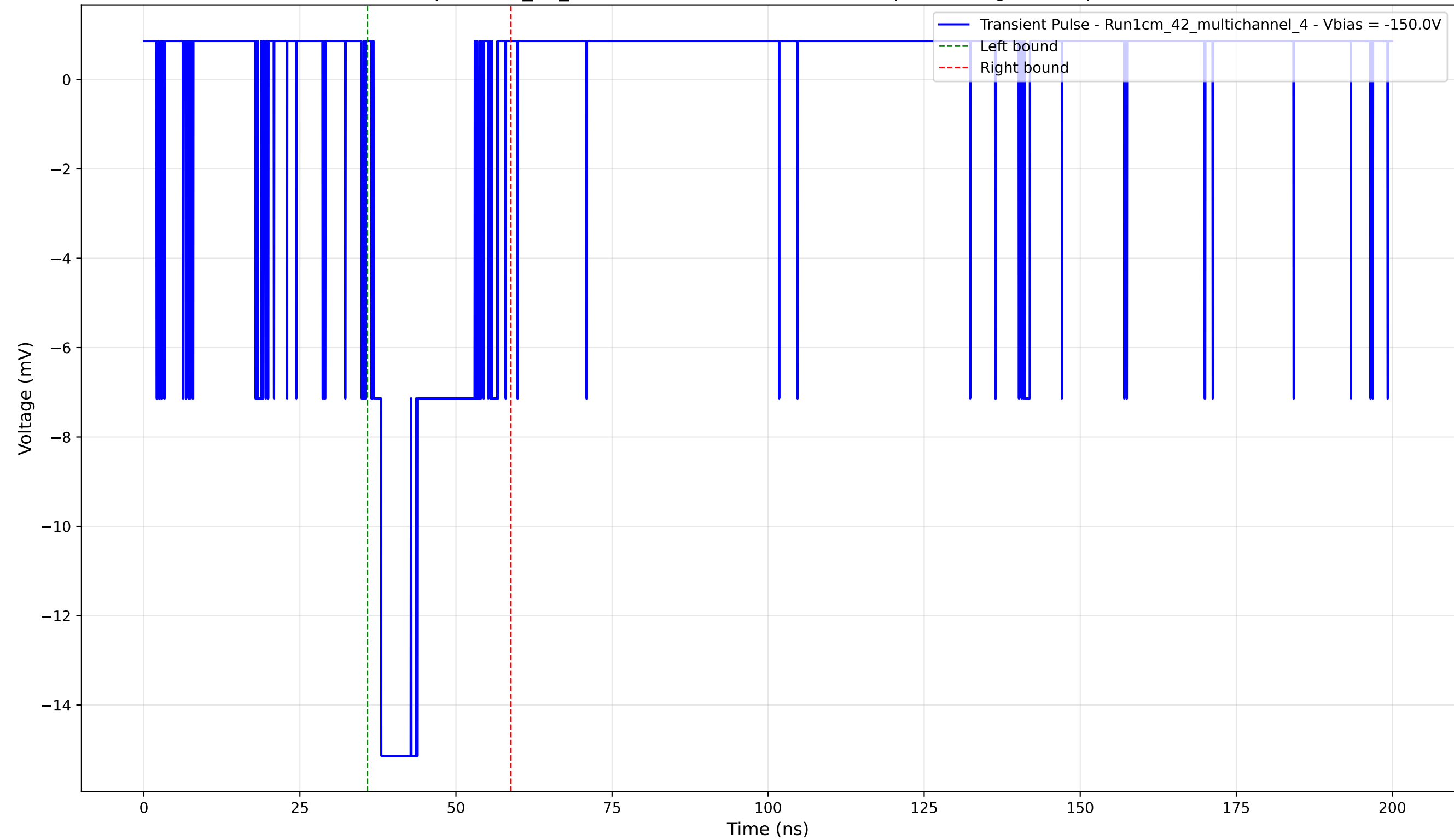
Transient Pulse - Sample: 1cm_42_multichannel - Position: 4020.0 \mu\text{m} - Charge: 3.45 pC - Rise Time: 1.22 ns
