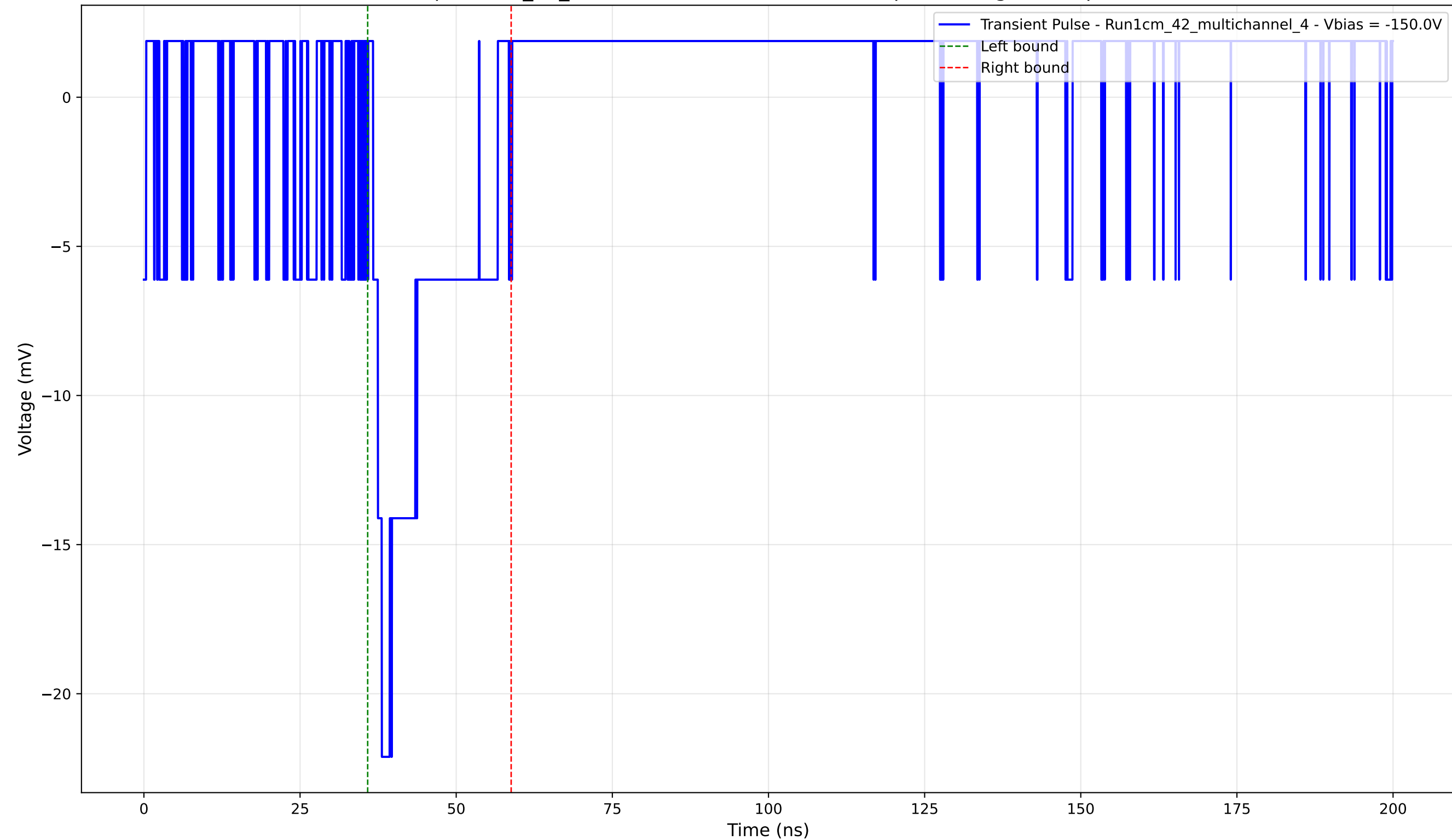
Transient Pulse - Sample: 1cm_42_multichannel - Position: 1115.0 \mu\text{m} - Charge: 3.57 pC - Rise Time: 1.40 ns
