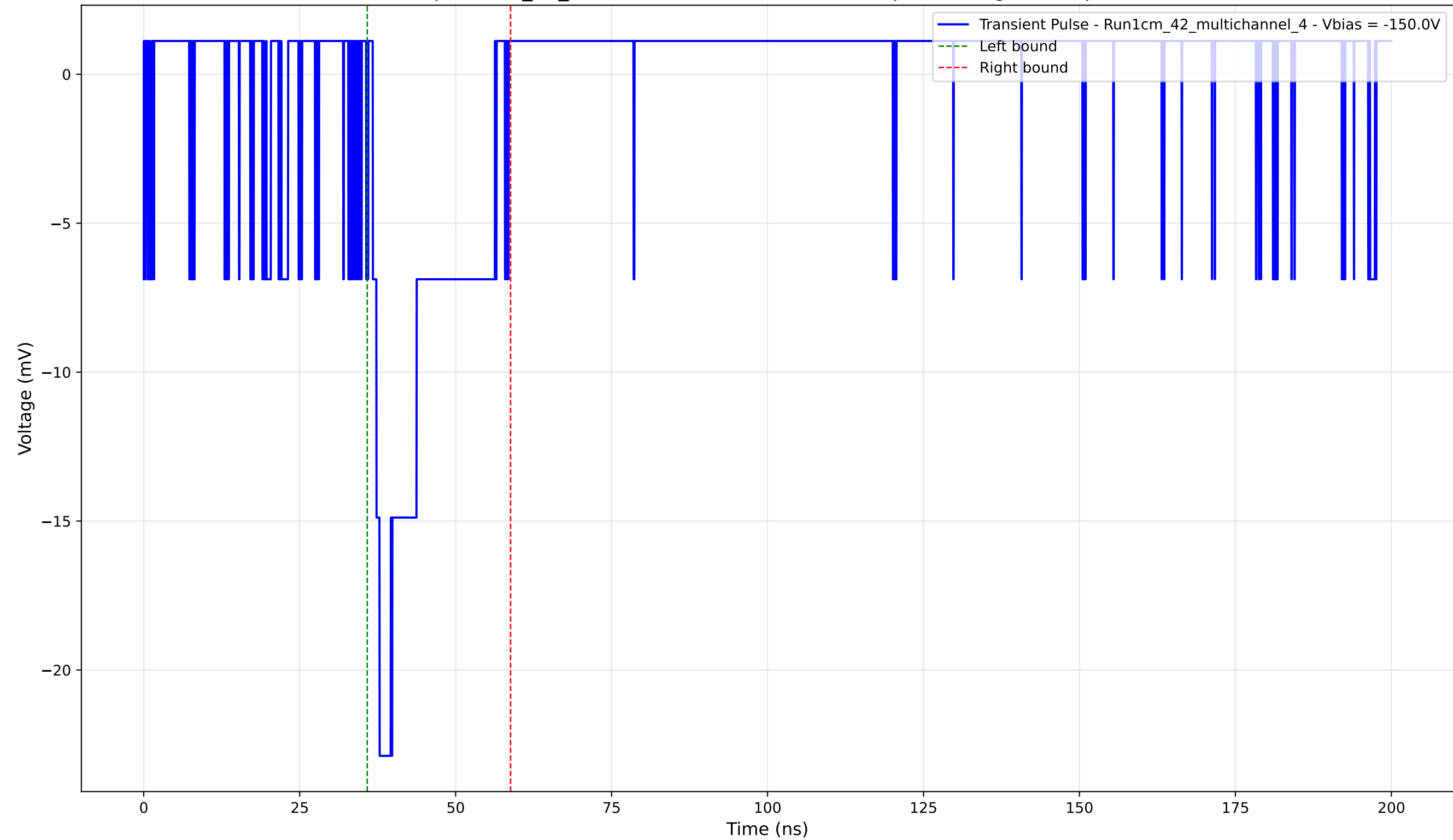
Transient Pulse - Sample: 1cm_42_multichannel - Position: 1165.0 \mu\text{m} - Charge: 4.07 pC - Rise Time: 1.10 ns
