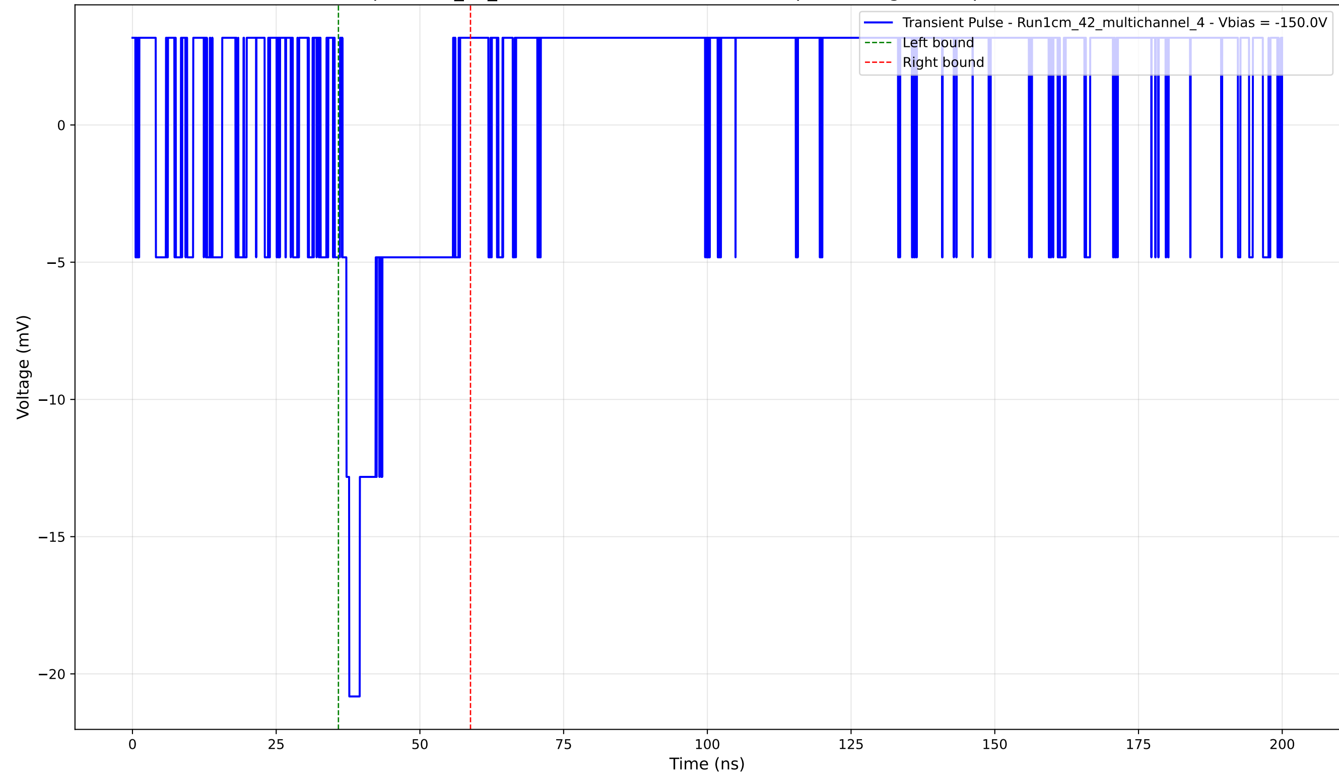
Transient Pulse - Sample: 1cm_42_multichannel - Position: 1305.0 \mu\text{m} - Charge: 2.96 pC - Rise Time: 0.00 ns (N/A)
