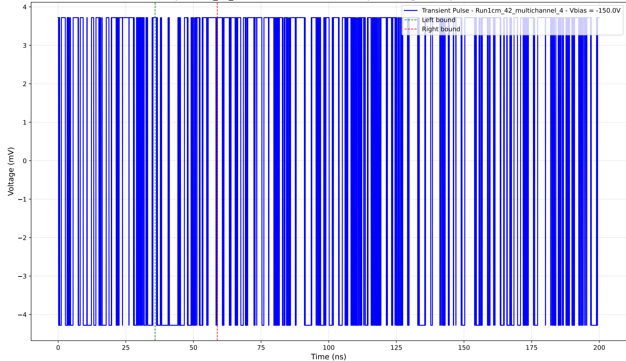
Transient Pulse - Sample: 1cm_42_multichannel - Position: 850.0 \mu\text{m} - Charge: 0.43 pC - Rise Time: 0.00 ns (N/A)
