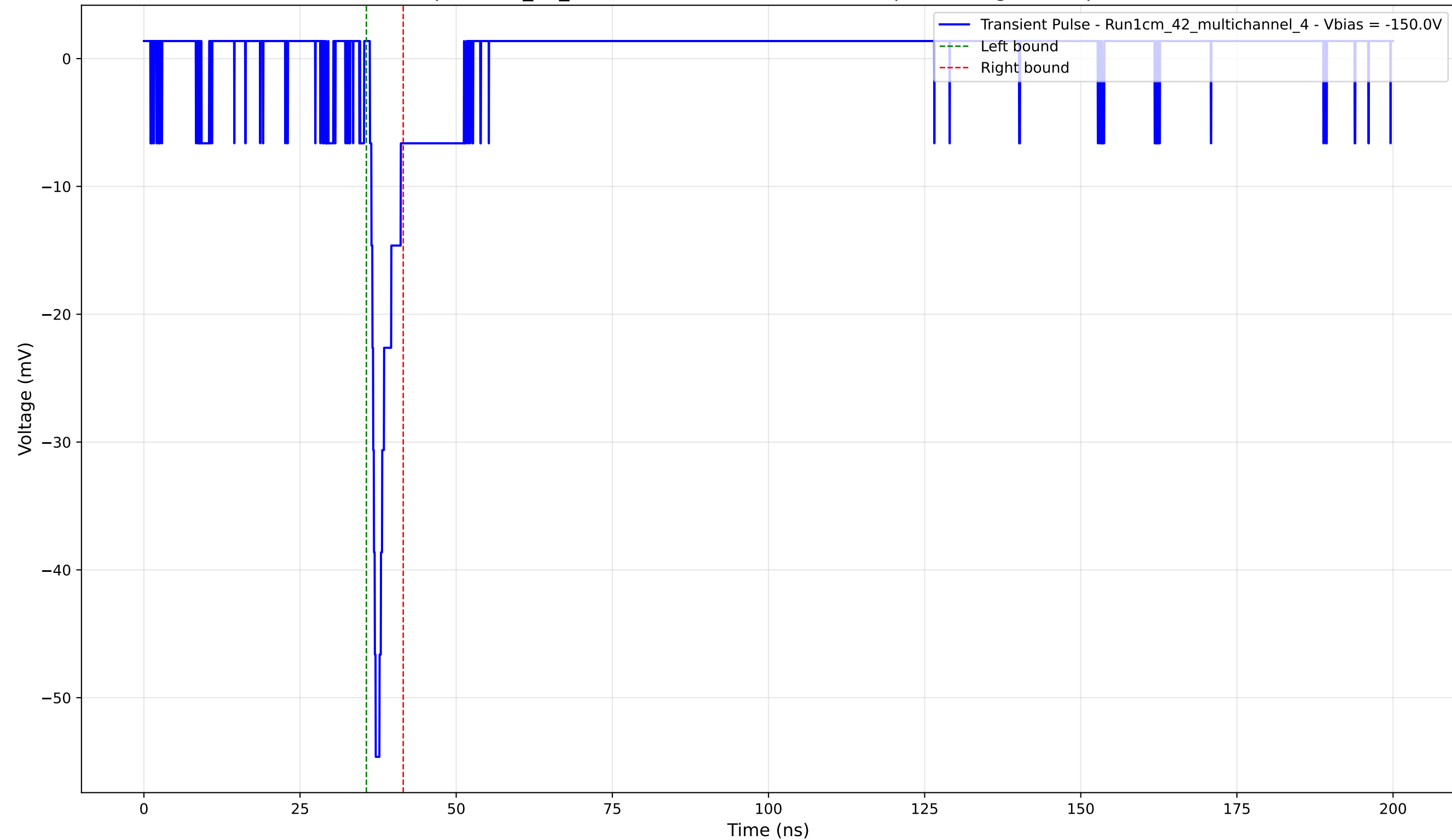
Transient Pulse - Sample: 1cm_42_multichannel - Position: 2680.0 \mu\text{m} - Charge: 2.67 pC - Rise Time: 0.92 ns
