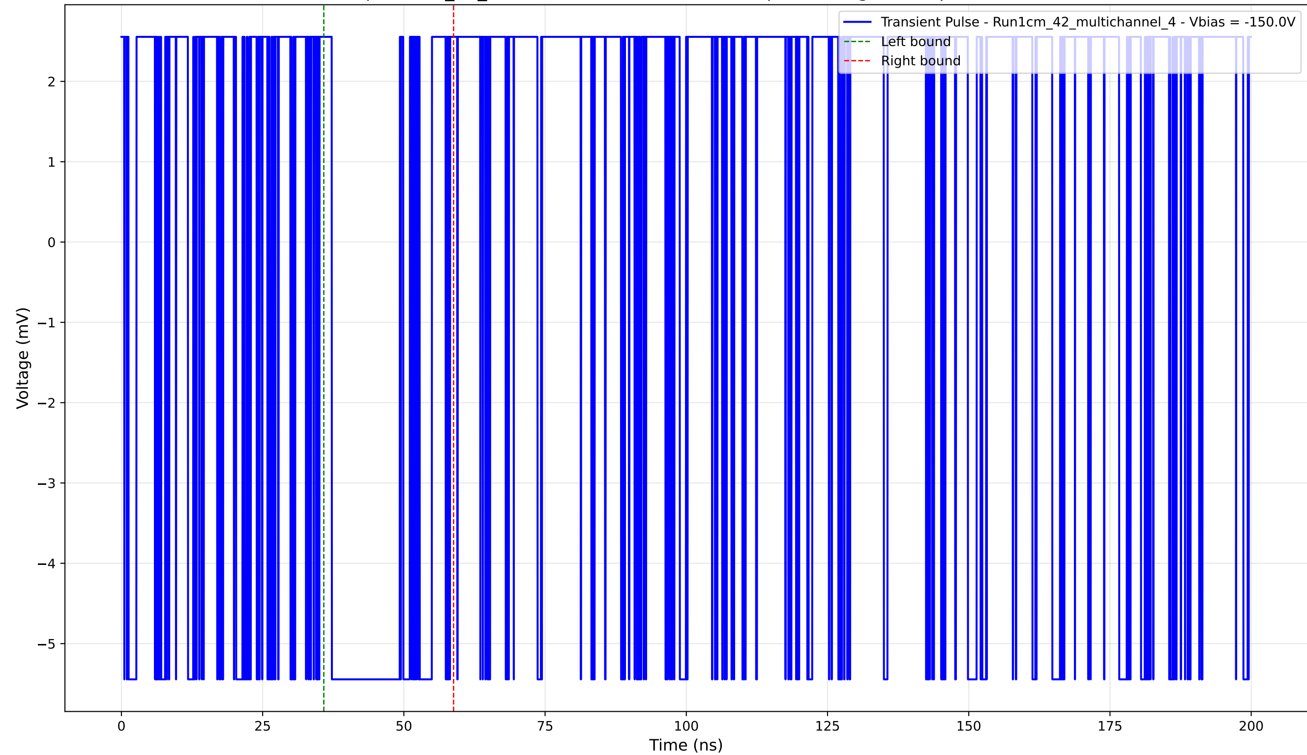
Transient Pulse - Sample: 1cm_42_multichannel - Position: 410.0 \mu\text{m} - Charge: 1.50 pC - Rise Time: 0.00 ns (N/A)
