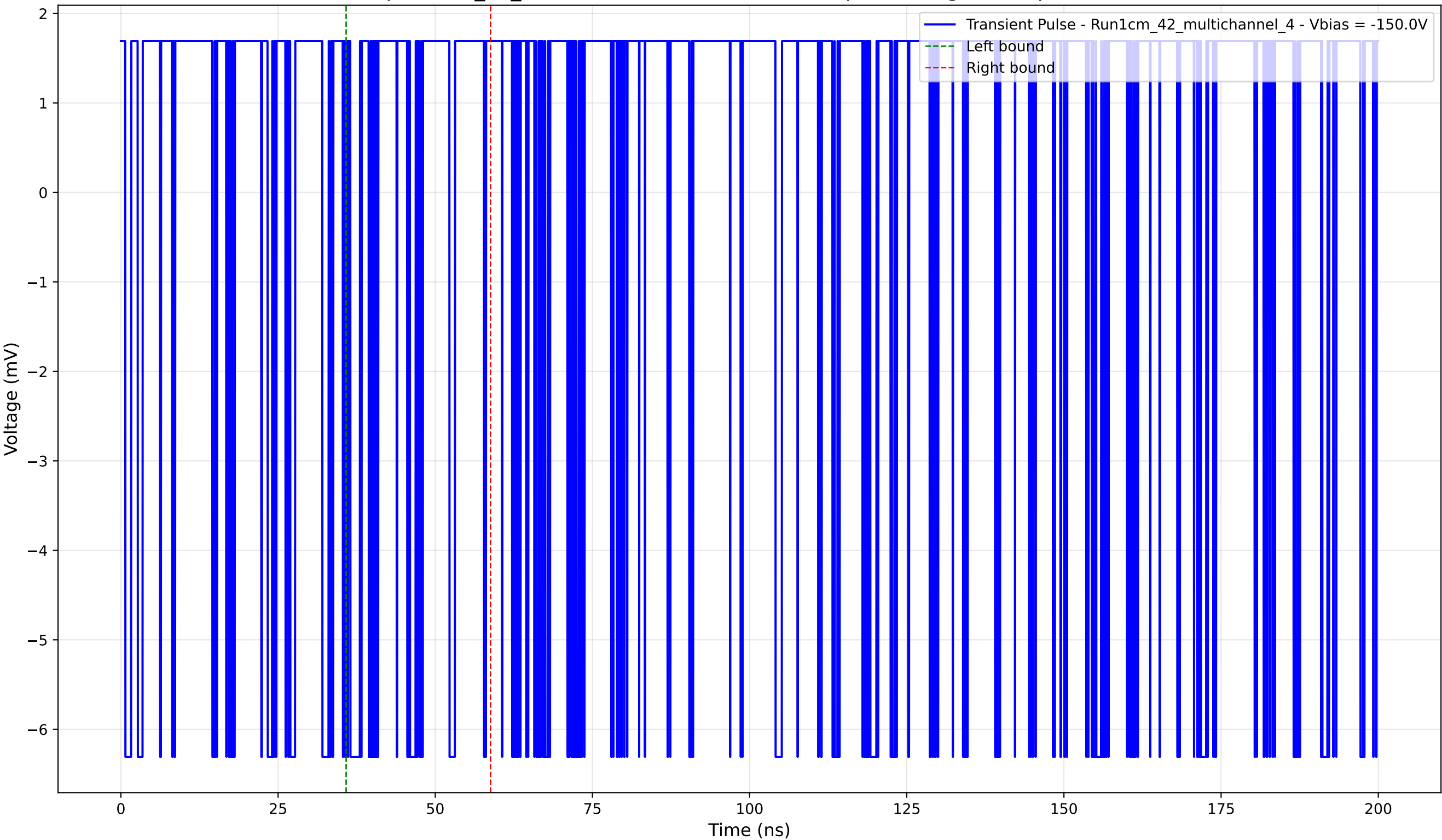
Transient Pulse - Sample: 1cm_42_multichannel - Position: 2375.0 \mu\text{m} - Charge: 0.11 pC - Rise Time: 0.00 ns (N/A)
