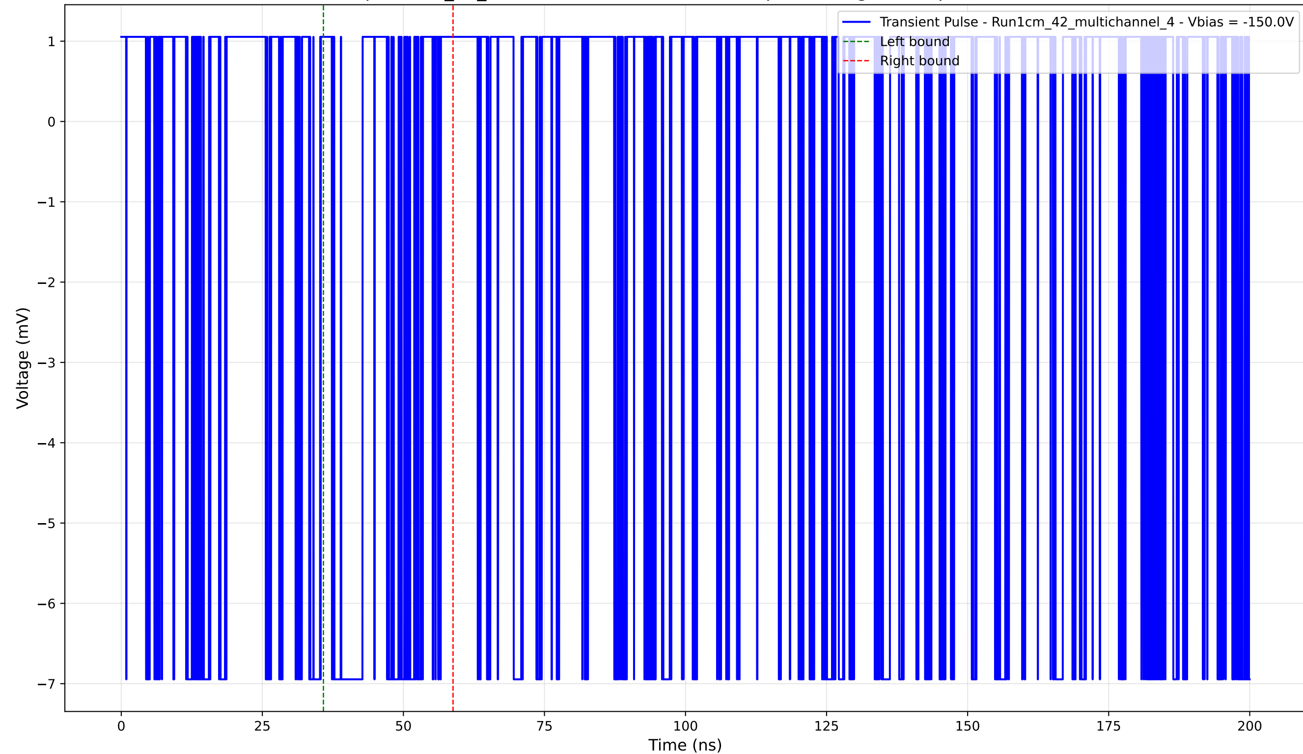
Transient Pulse - Sample: 1cm_42_multichannel - Position: 845.0 \mu\text{m} - Charge: 1.13 pC - Rise Time: 0.00 ns (N/A)
