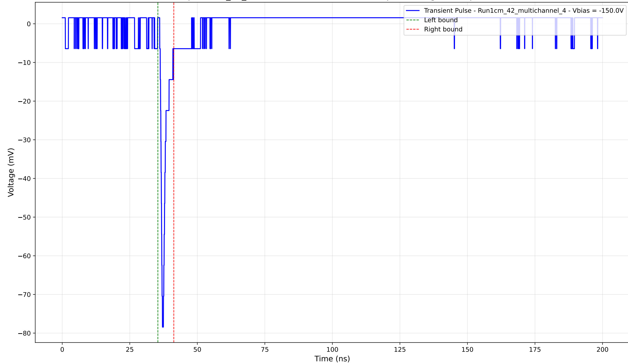
Transient Pulse - Sample: 1cm_42_multichannel - Position: 2275.0 \mu\text{m} - Charge: 3.16 pC - Rise Time: 0.82 ns
