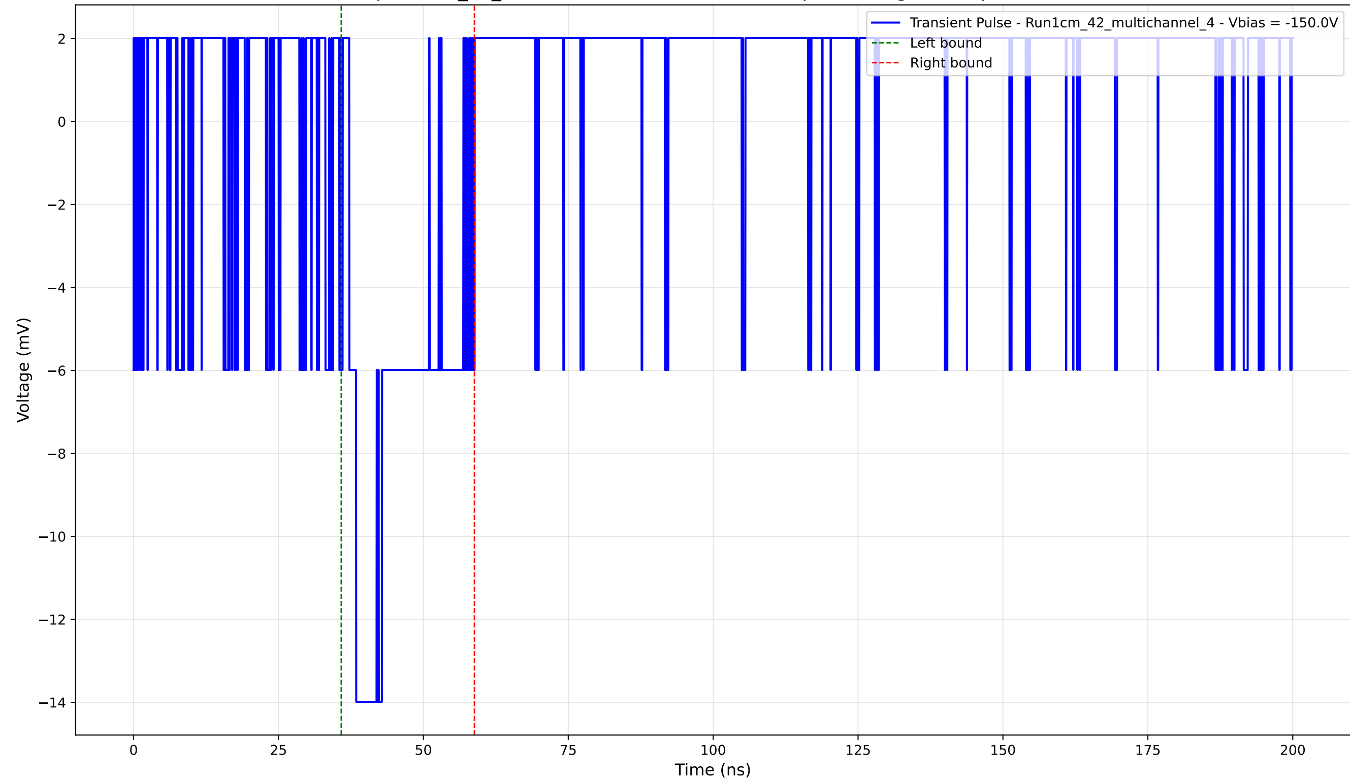
Transient Pulse - Sample: 1cm_42_multichannel - Position: 4335.0 \mu\text{m} - Charge: 3.09 pC - Rise Time: 0.00 ns (N/A)
