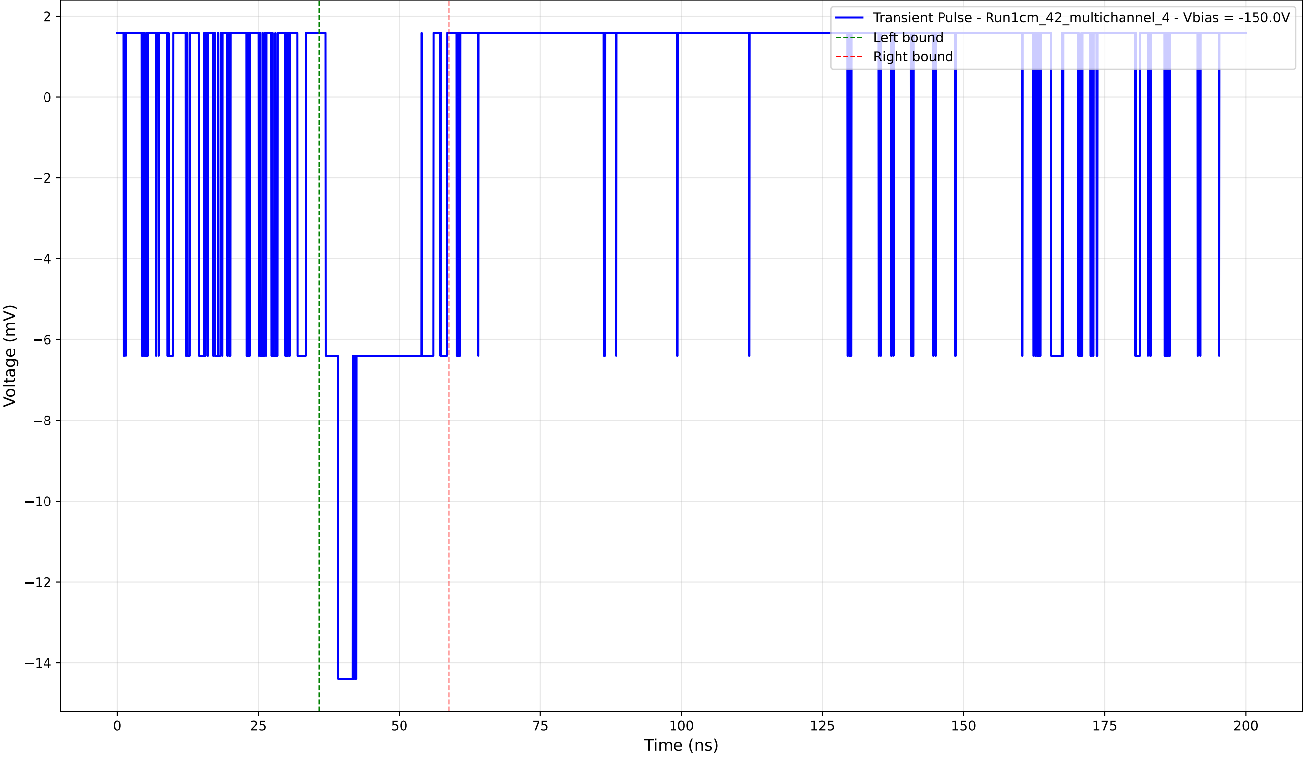
Transient Pulse - Sample: 1cm_42_multichannel - Position: 175.0 \mu\text{m} - Charge: 2.97 pC - Rise Time: 0.00 ns (N/A)
