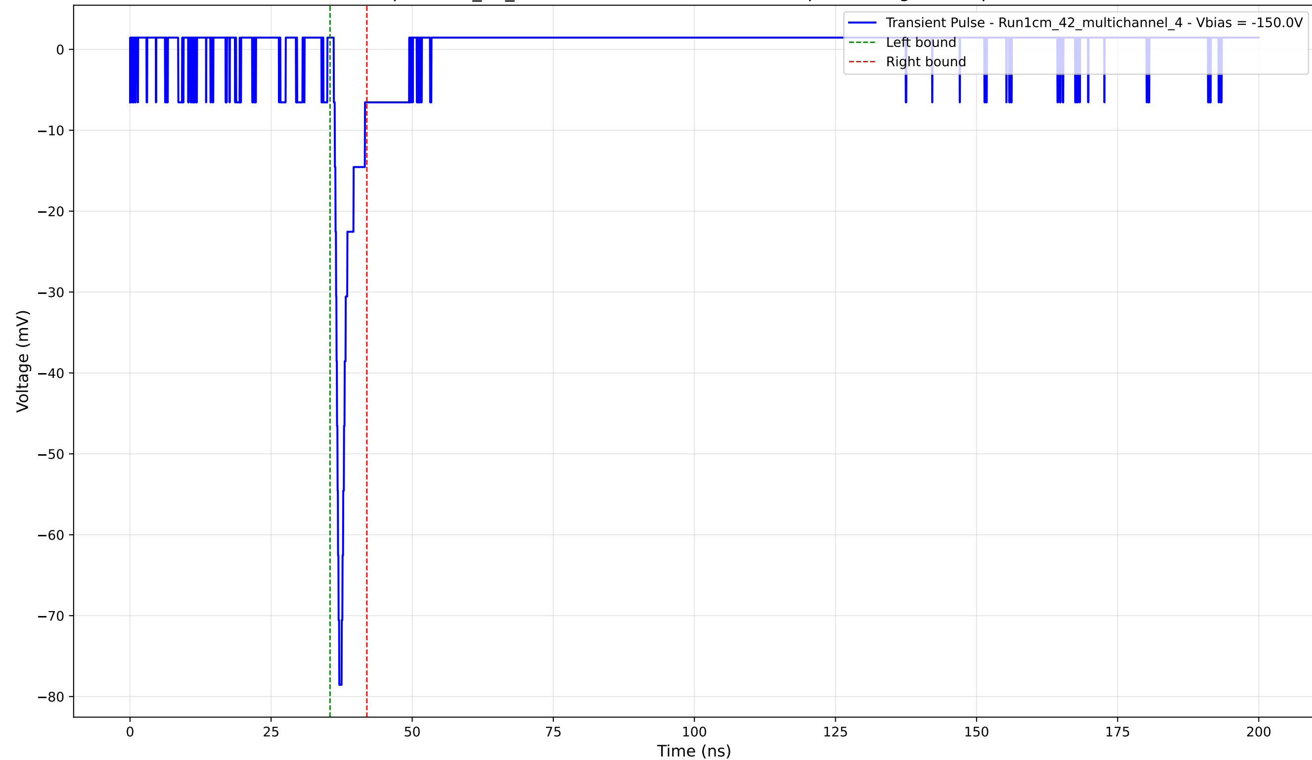
Transient Pulse - Sample: 1cm_42_multichannel - Position: 2505.0 \mu\text{m} - Charge: 3.42 pC - Rise Time: 0.80 ns
