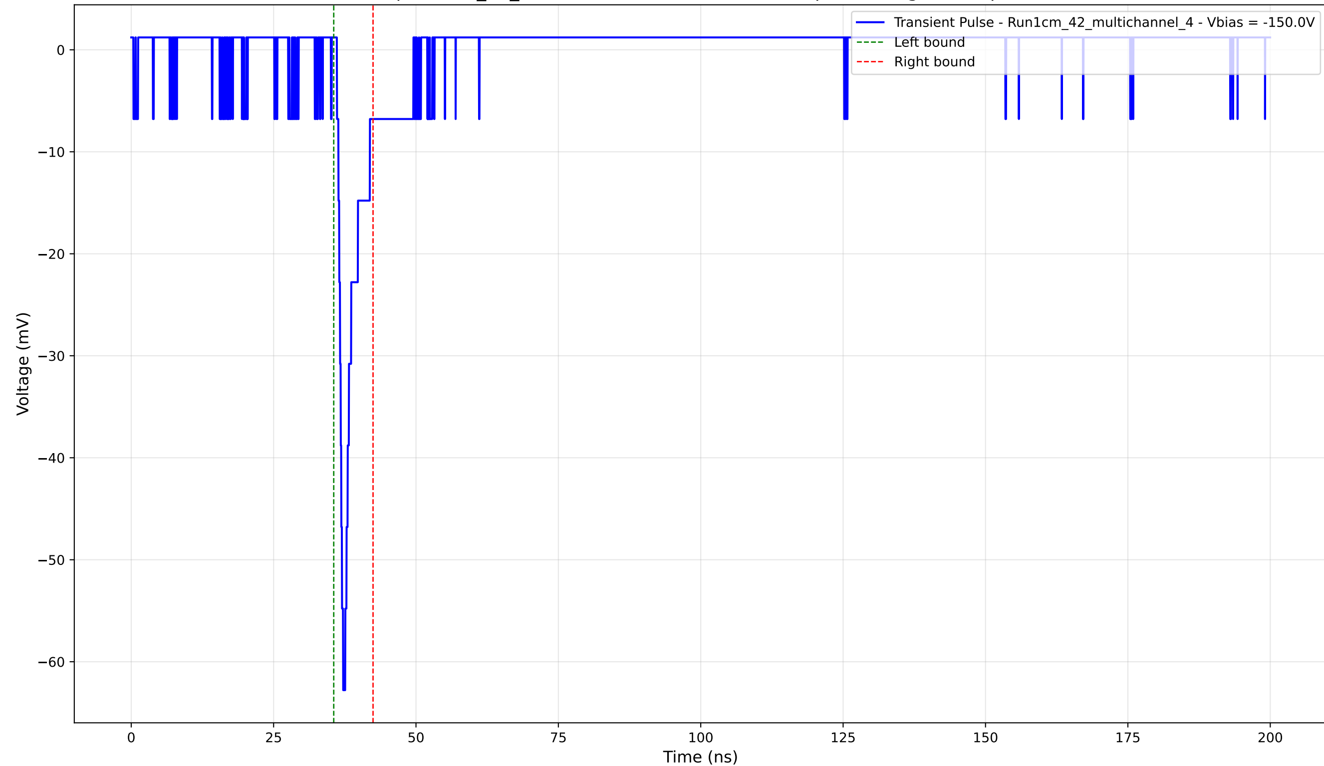
Transient Pulse - Sample: 1cm_42_multichannel - Position: 2115.0 \mu\text{m} - Charge: 3.17 pC - Rise Time: 1.08 ns
