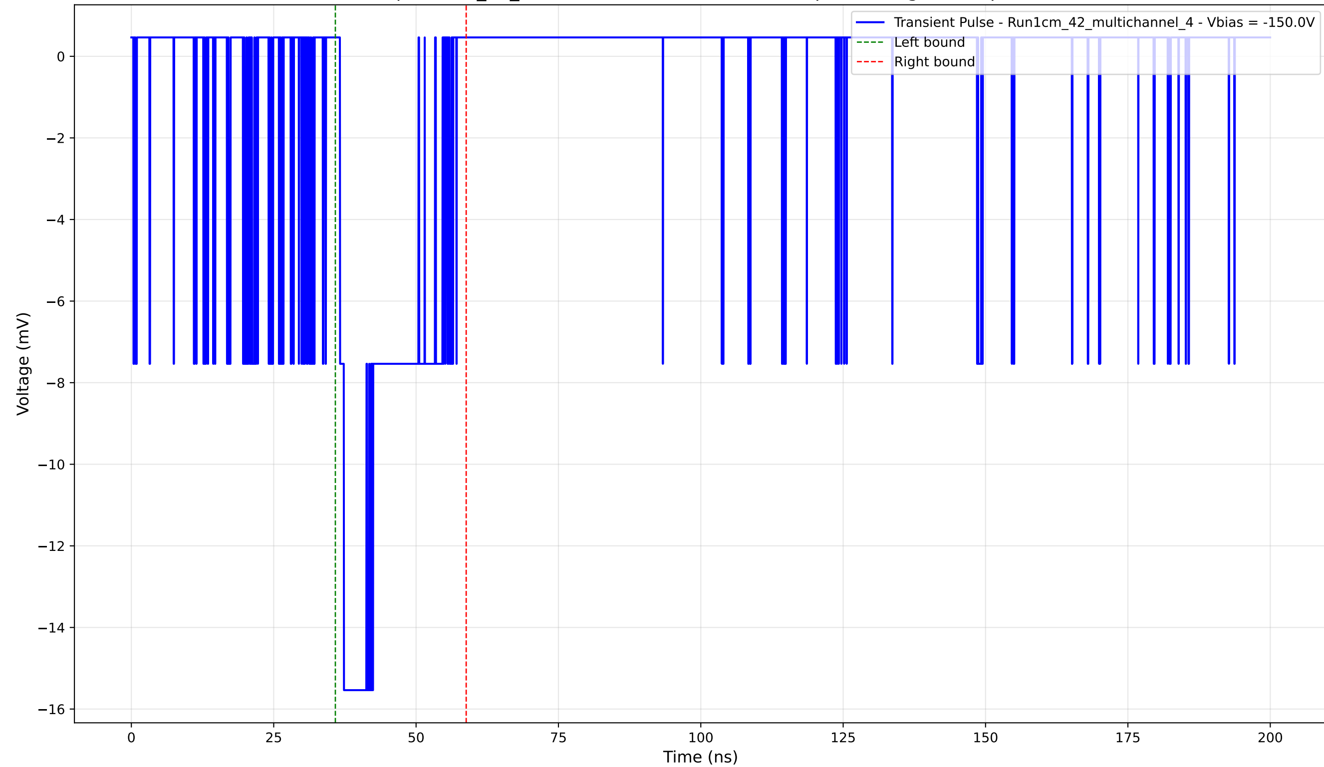
Transient Pulse - Sample: 1cm_42_multichannel - Position: 3460.0 \mu\text{m} - Charge: 3.52 pC - Rise Time: 0.70 ns
