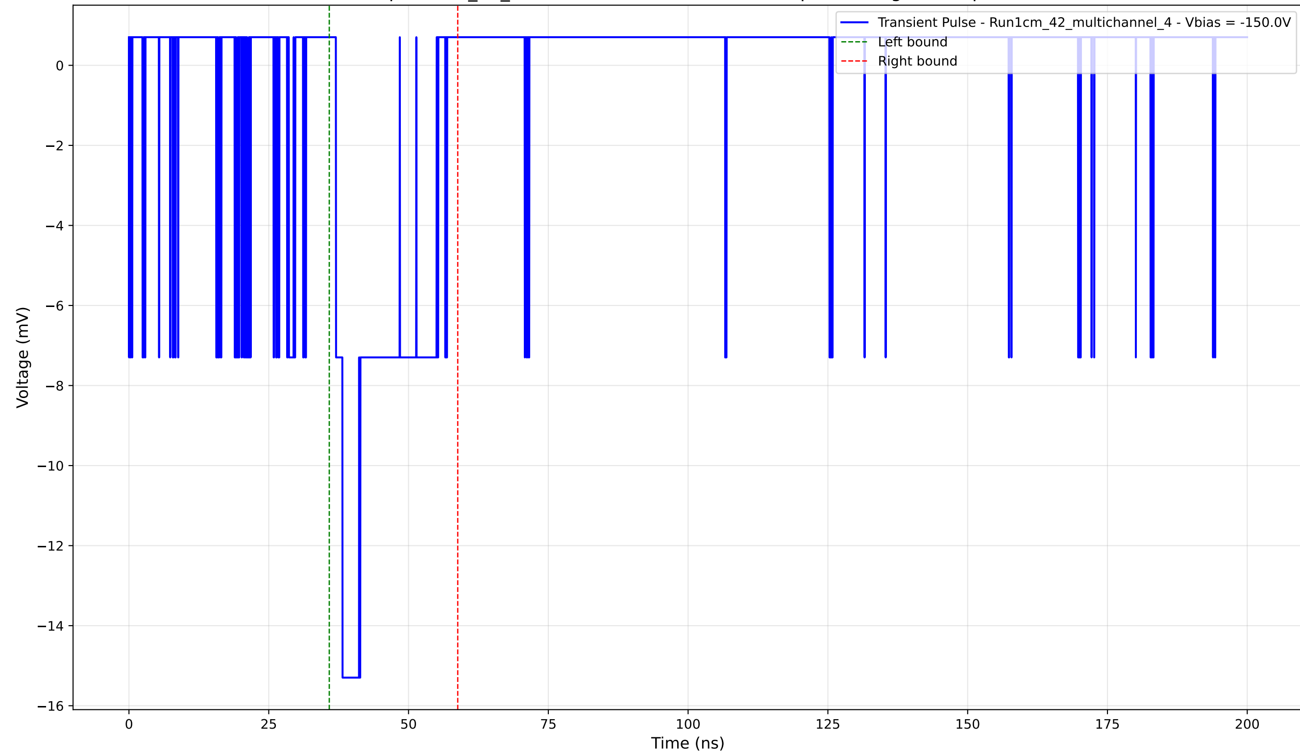
Transient Pulse - Sample: 1cm_42_multichannel - Position: 3965.0 \mu\text{m} - Charge: 3.10 pC - Rise Time: 1.18 ns
