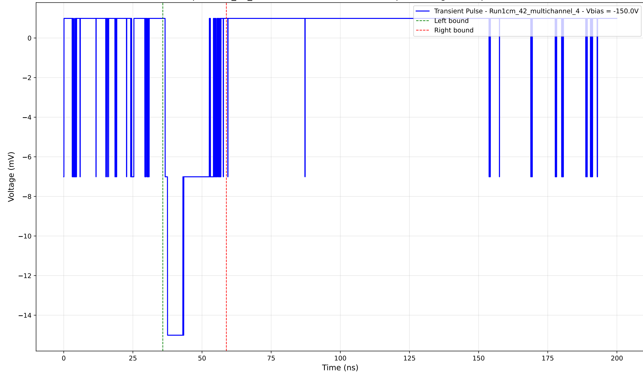
Transient Pulse - Sample: 1cm_42_multichannel - Position: 3710.0 \mu\text{m} - Charge: 3.48 pC - Rise Time: 0.88 ns
