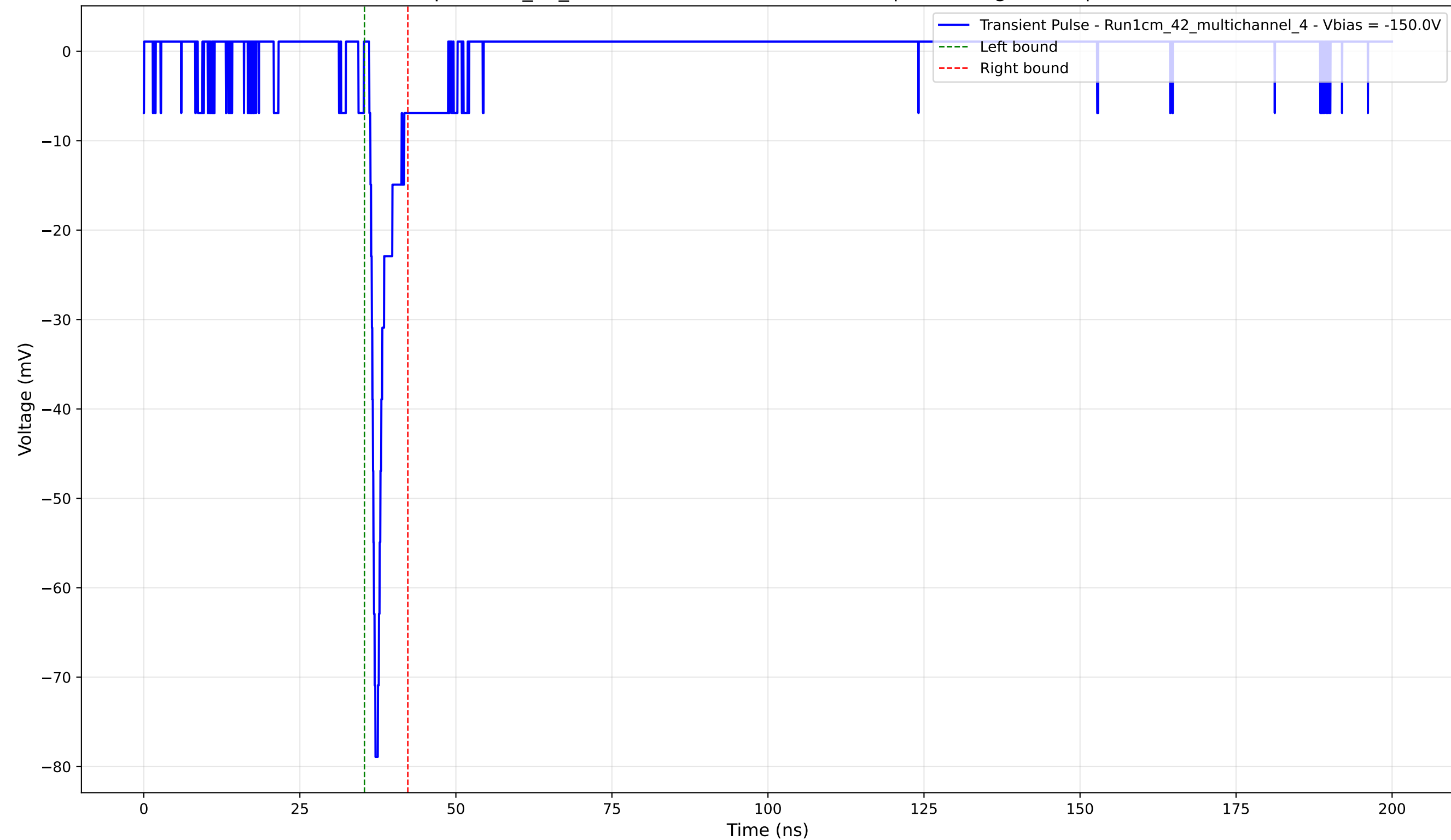
Transient Pulse - Sample: 1cm_42_multichannel - Position: 2230.0 \mu\text{m} - Charge: 3.52 pC - Rise Time: 0.82 ns
