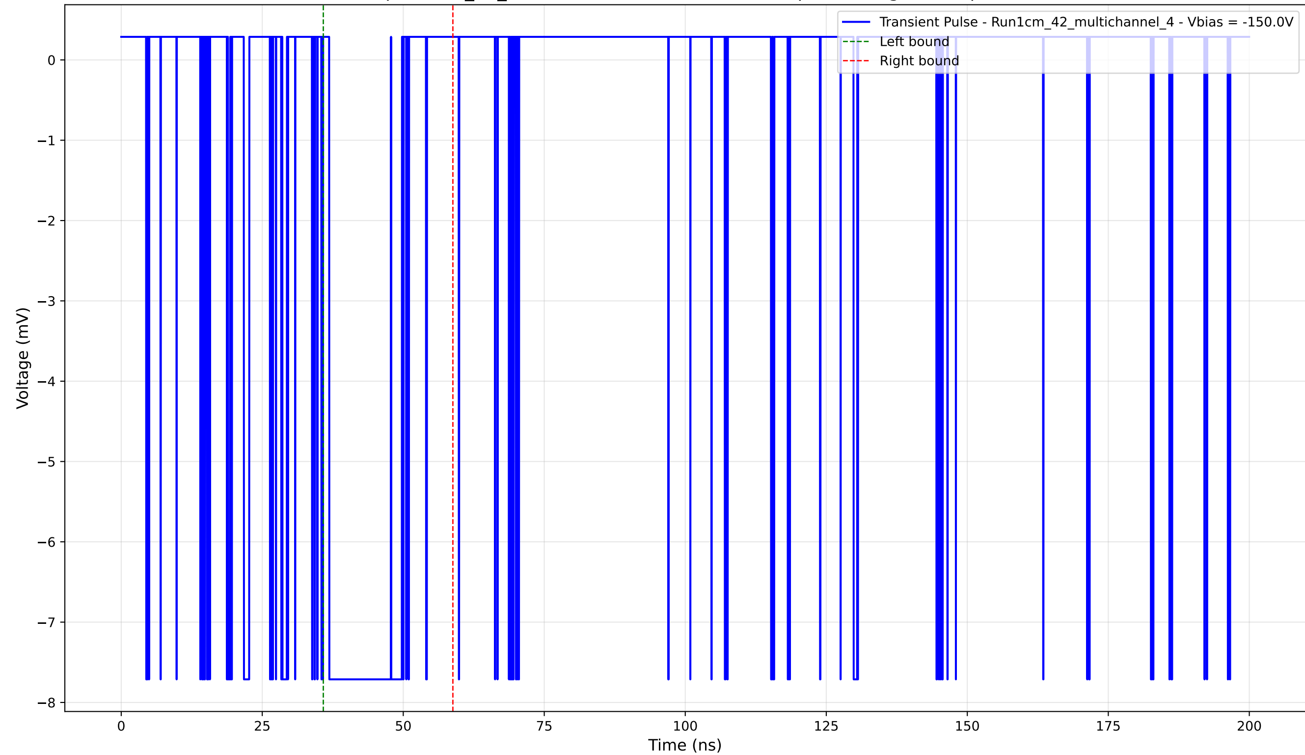
Transient Pulse - Sample: 1cm_42_multichannel - Position: 3445.0 \mu\text{m} - Charge: 1.98 pC - Rise Time: 0.02 ns
