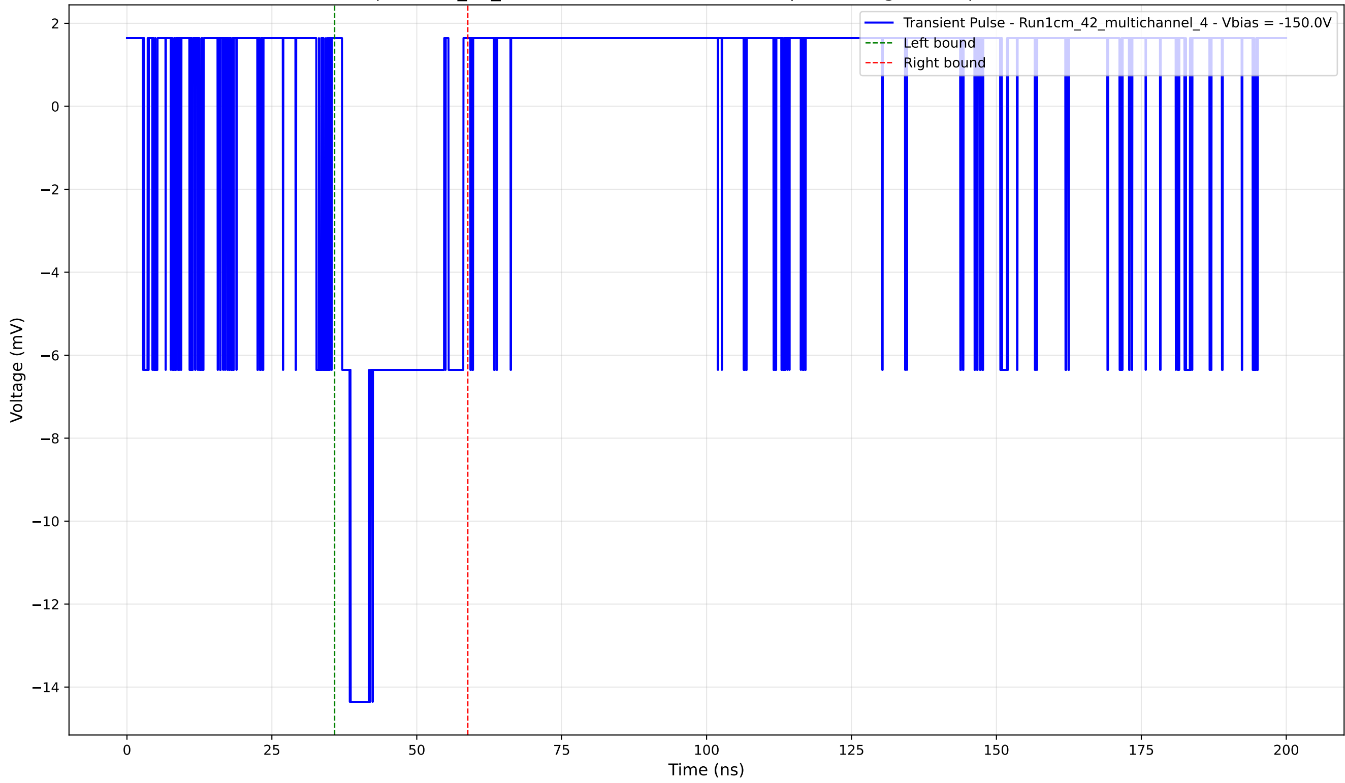
Transient Pulse - Sample: 1cm_42_multichannel - Position: 145.0 \mu\text{m} - Charge: 3.04 pC - Rise Time: 0.00 ns (N/A)
