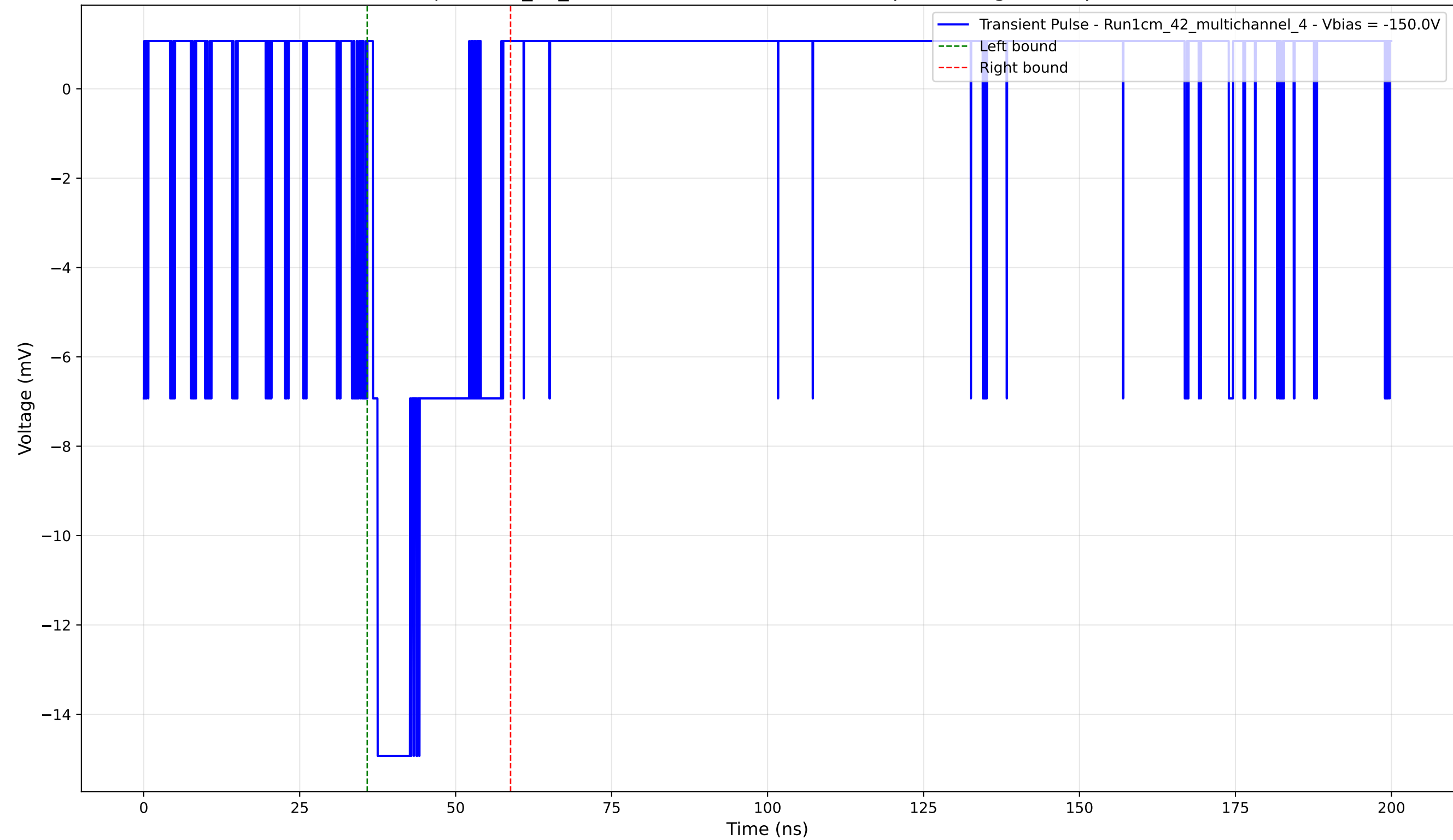
Transient Pulse - Sample: 1cm_42_multichannel - Position: 3655.0 \mu\text{m} - Charge: 3.61 pC - Rise Time: 0.76 ns
