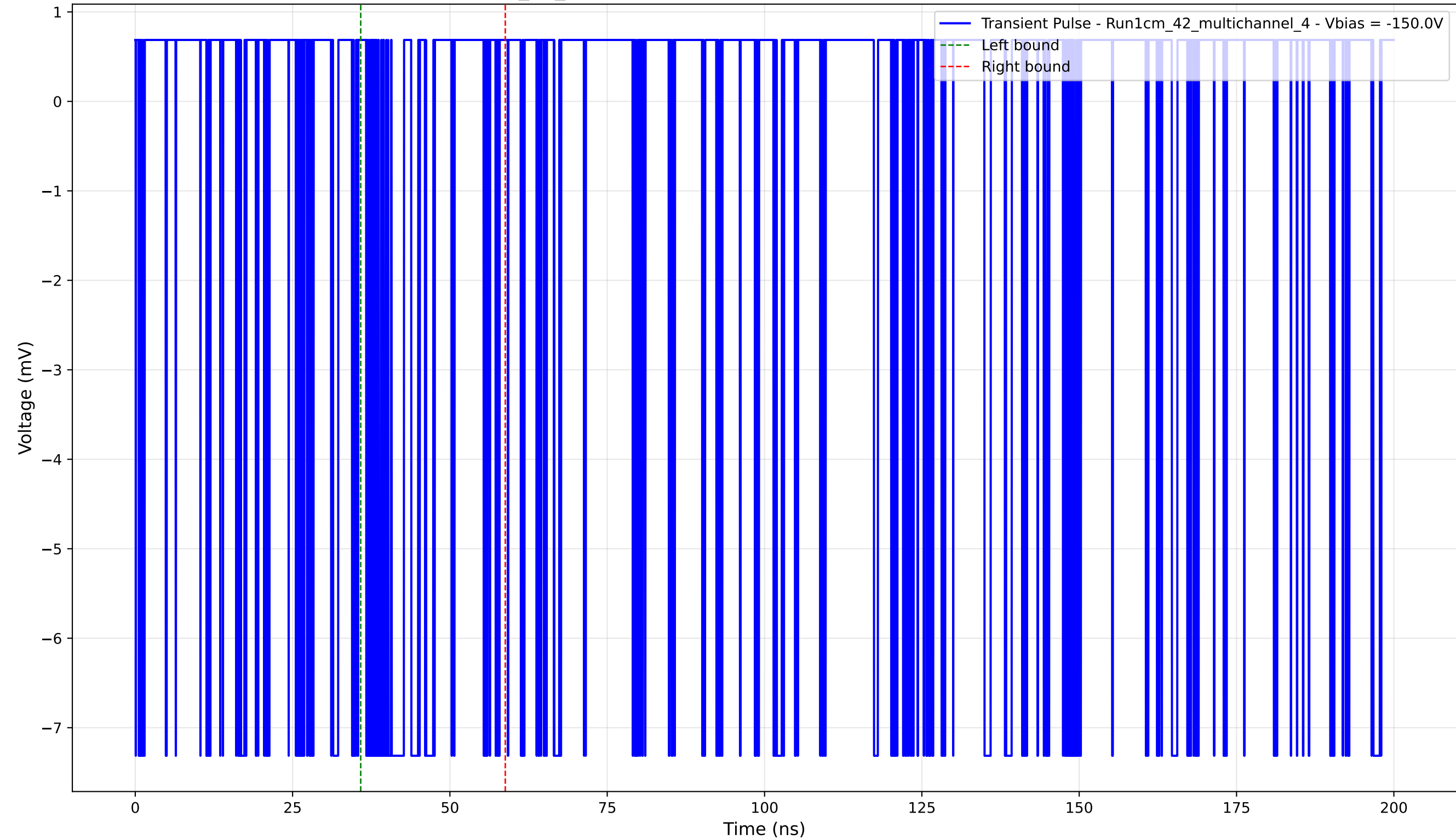
Transient Pulse - Sample: 1cm_42_multichannel - Position: 4375.0 \mu\text{m} - Charge: 1.01 pC - Rise Time: 0.02 ns
