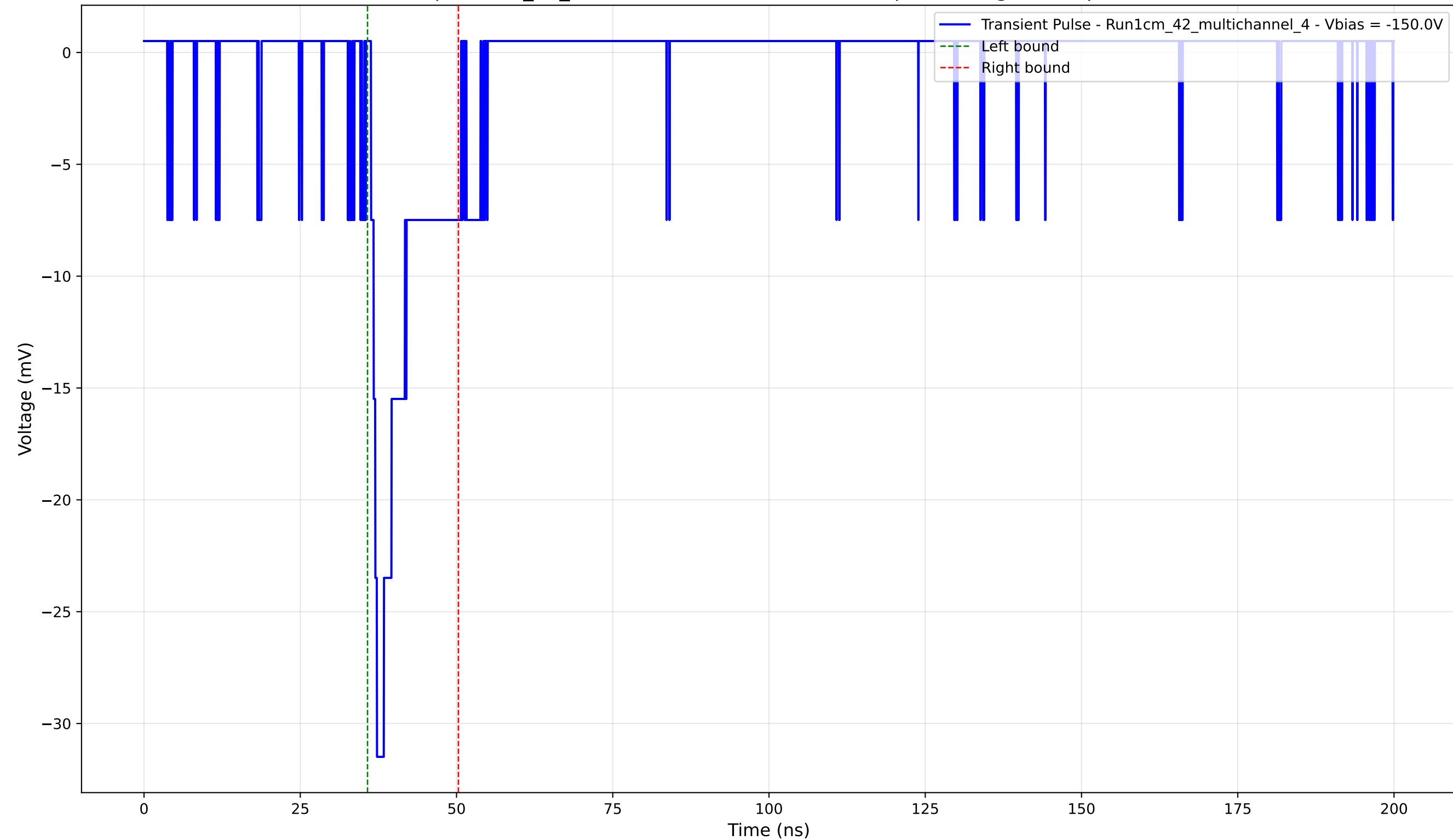
Transient Pulse - Sample: 1cm_42_multichannel - Position: 3075.0 \mu\text{m} - Charge: 3.51 pC - Rise Time: 0.95 ns
