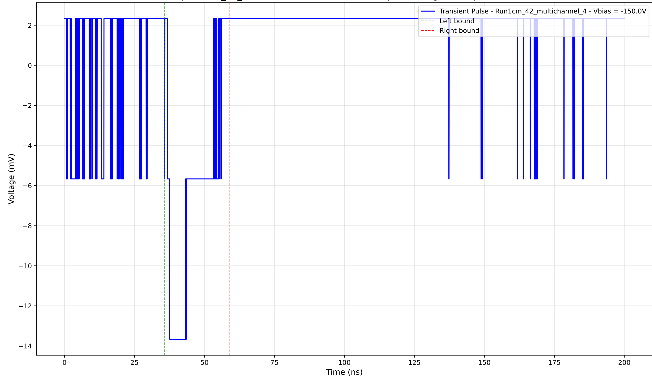
Transient Pulse - Sample: 1cm_42_multichannel - Position: 3675.0 \mu\text{m} - Charge: 2.74 pC - Rise Time: 0.00 ns (N/A)
