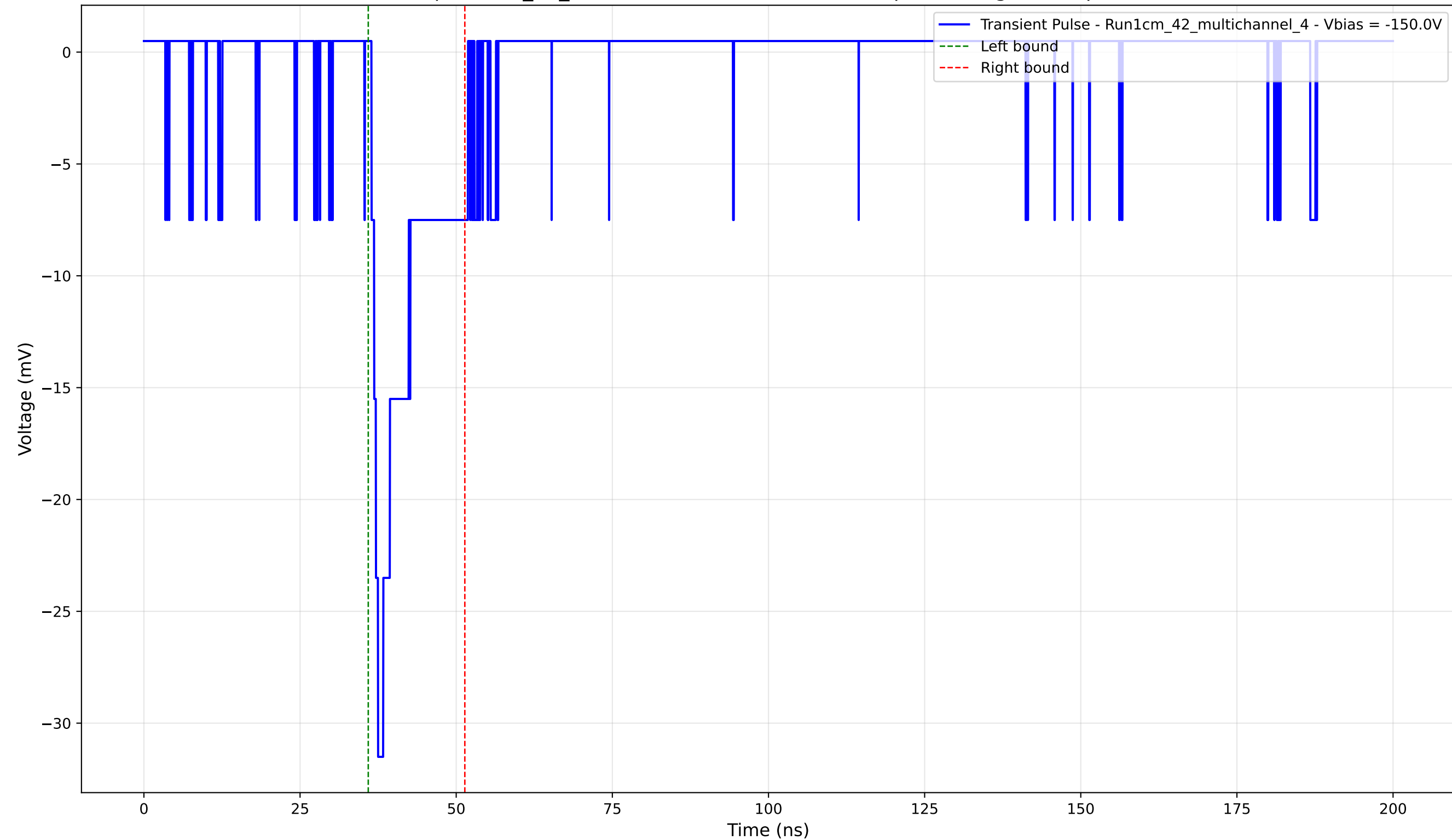
Transient Pulse - Sample: 1cm_42_multichannel - Position: 3155.0 \mu\text{m} - Charge: 3.63 pC - Rise Time: 1.05 ns
