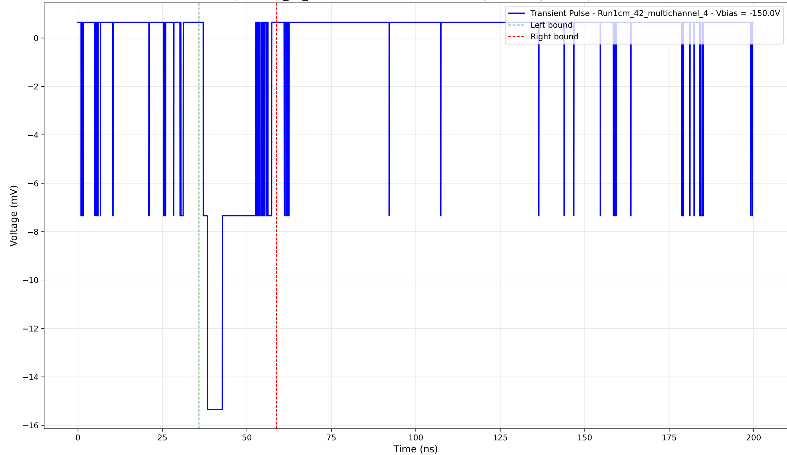
Transient Pulse - Sample: 1cm_42_multichannel - Position: 4215.0 \mu\text{m} - Charge: 3.43 pC - Rise Time: 1.22 ns
