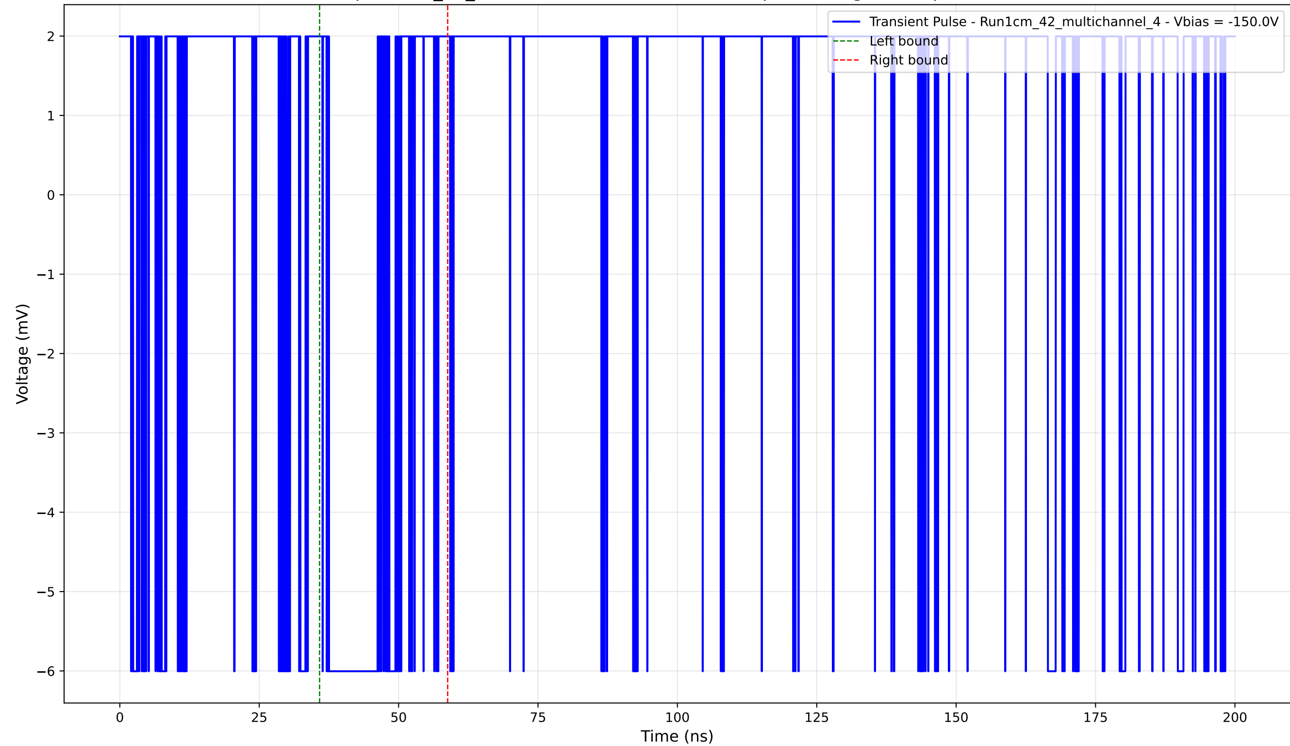
Transient Pulse - Sample: 1cm_42_multichannel - Position: 4865.0 \mu\text{m} - Charge: 1.01 pC - Rise Time: 0.00 ns (N/A)
