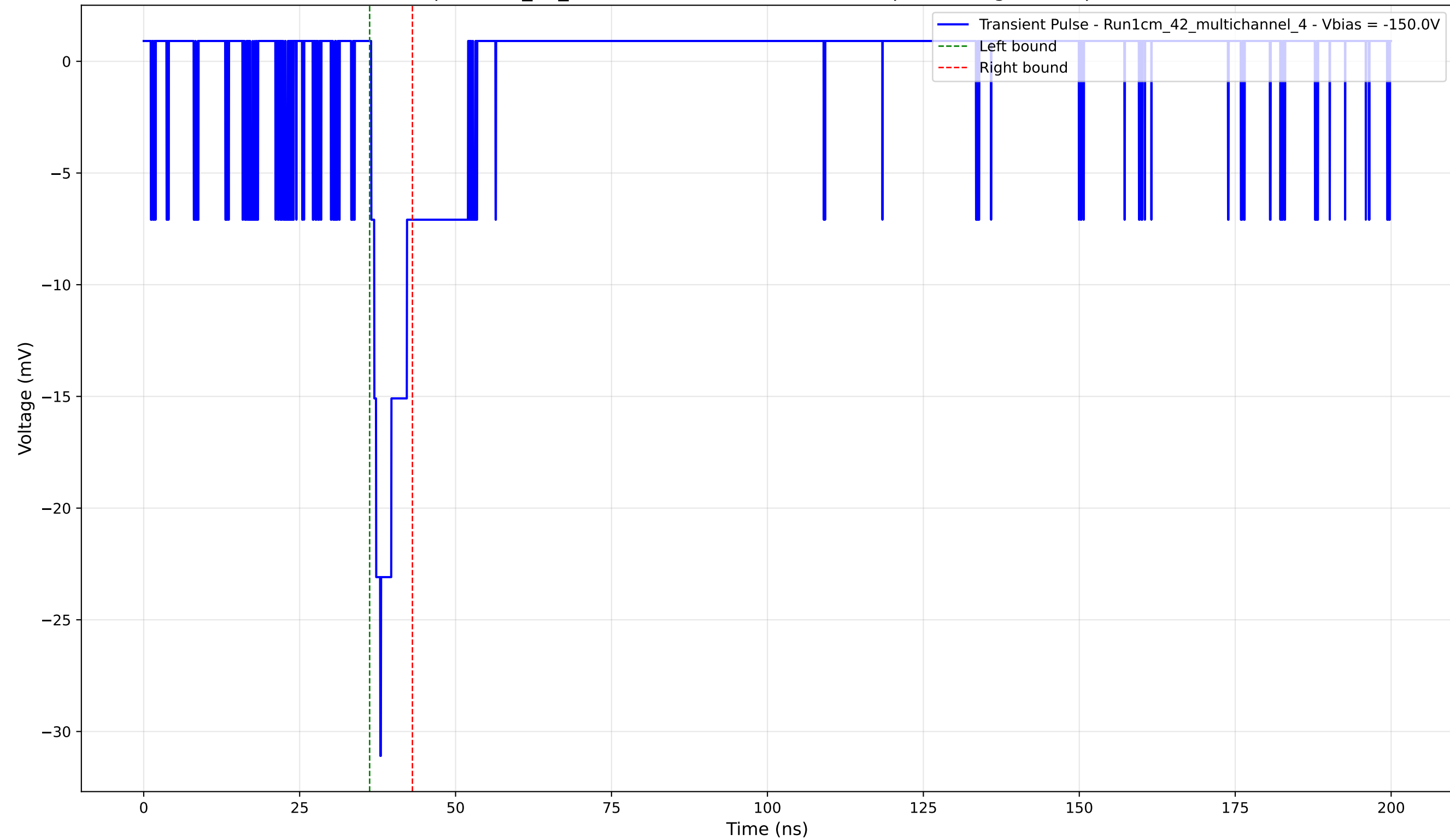
Transient Pulse - Sample: 1cm_42_multichannel - Position: 3260.0 \mu\text{m} - Charge: 2.18 pC - Rise Time: 1.45 ns
