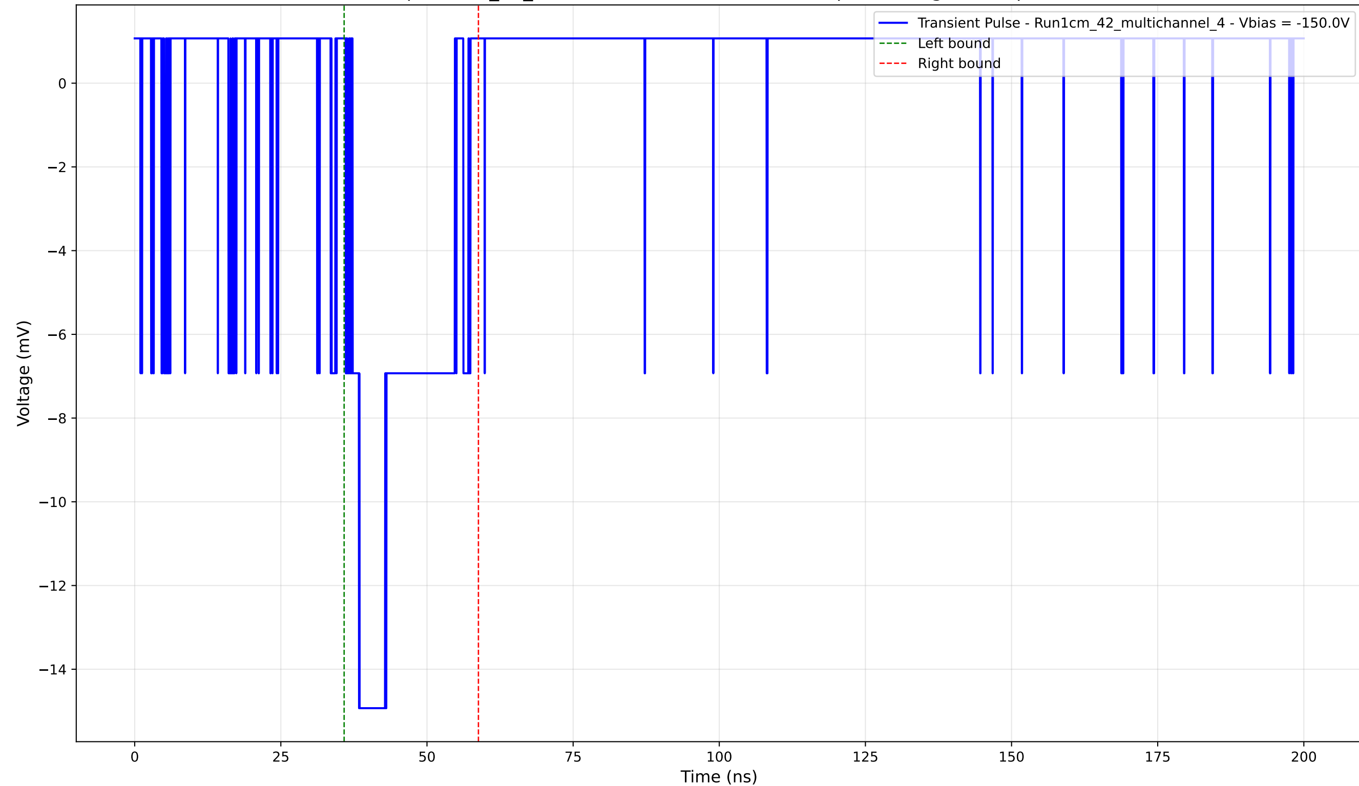
Transient Pulse - Sample: 1cm_42_multichannel - Position: 4245.0 \mu\text{m} - Charge: 3.33 pC - Rise Time: 1.10 ns
