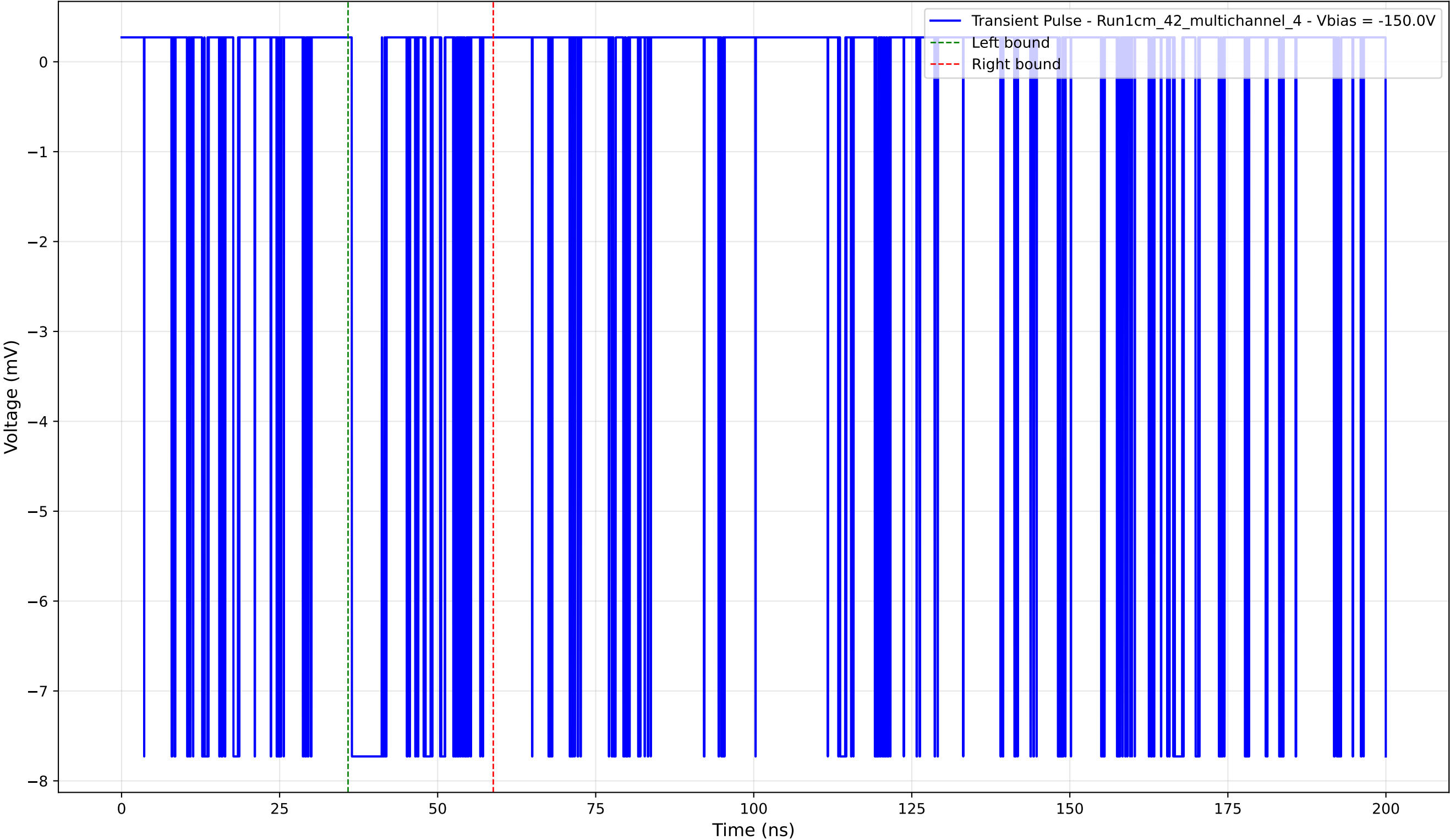
Transient Pulse - Sample: 1cm_42_multichannel - Position: 1880.0 \mu\text{m} - Charge: 1.34 pC - Rise Time: 0.02 ns
