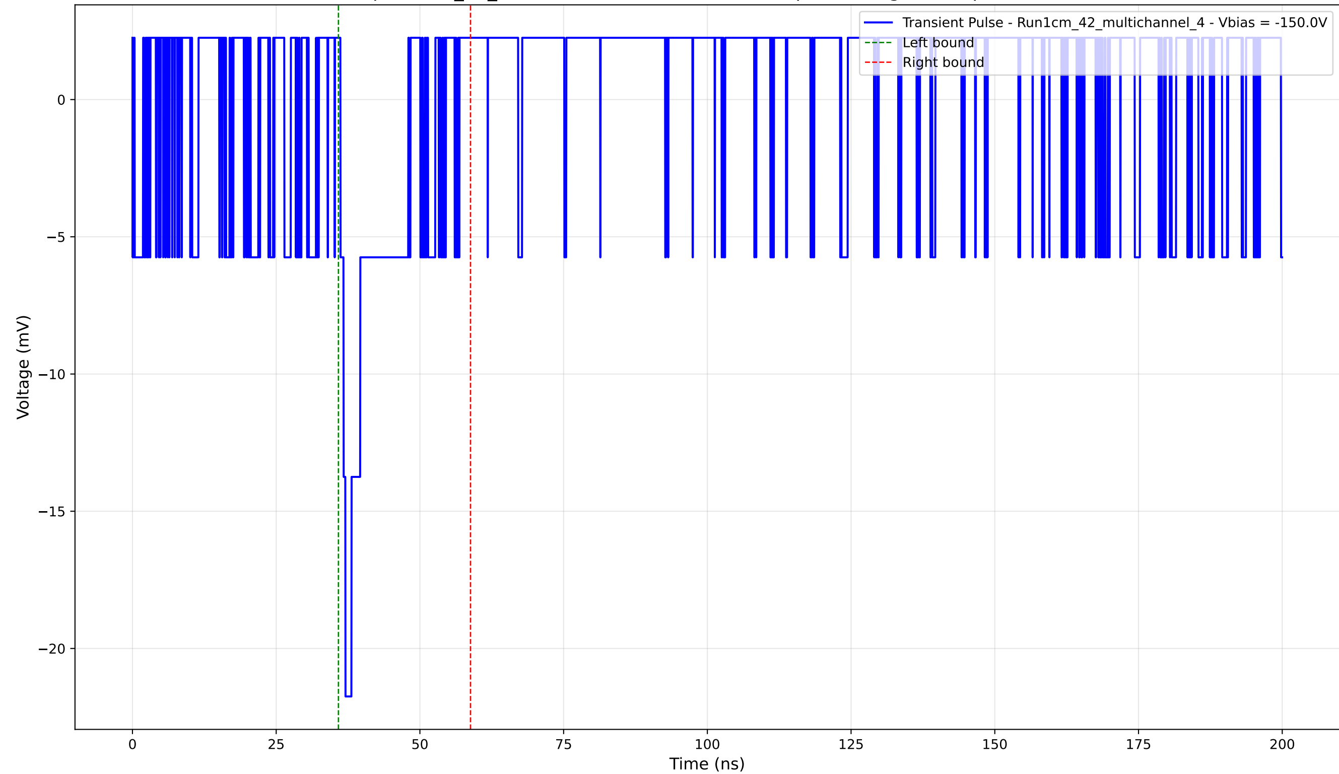
Transient Pulse - Sample: 1cm_42_multichannel - Position: 1930.0 \mu\text{m} - Charge: 2.06 pC - Rise Time: 0.00 ns (N/A)
