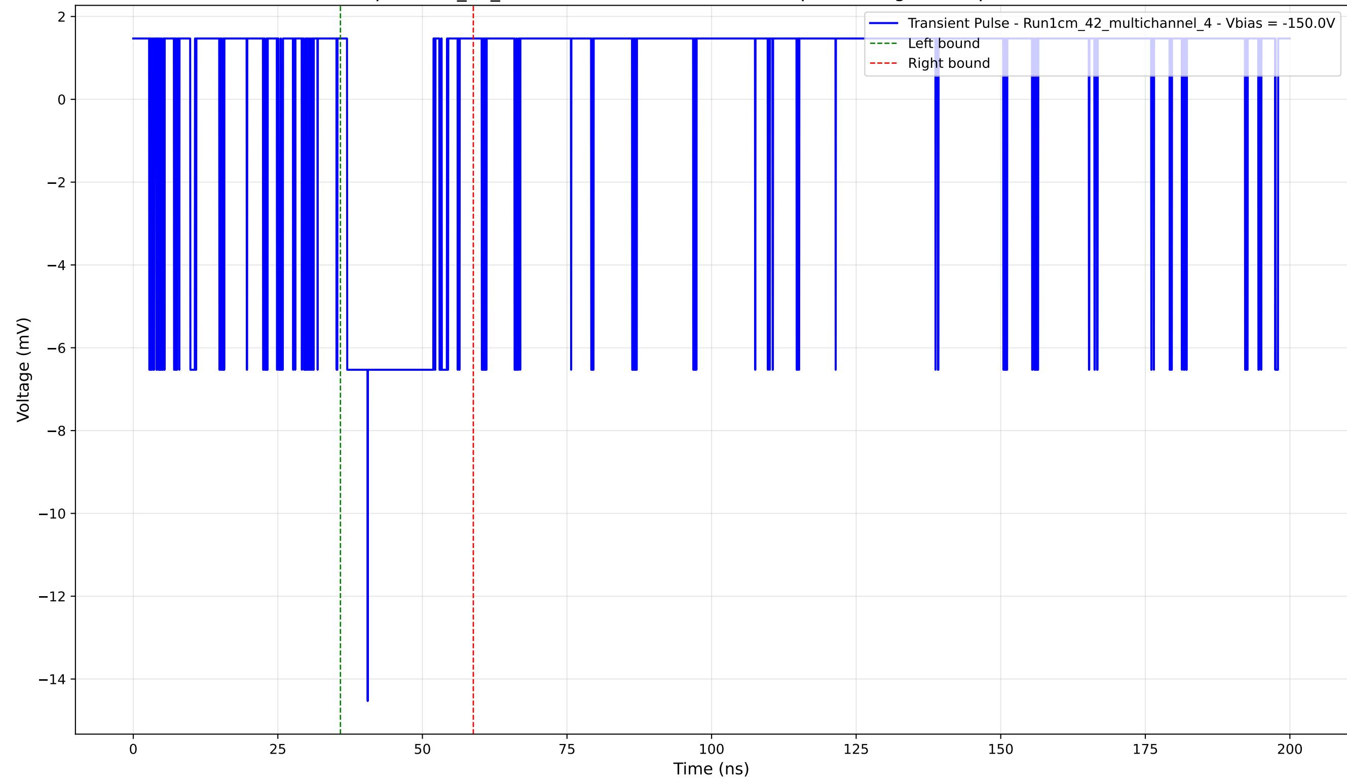
Transient Pulse - Sample: 1cm_42_multichannel - Position: 4840.0 \mu\text{m} - Charge: 1.97 pC - Rise Time: 0.00 ns (N/A)
