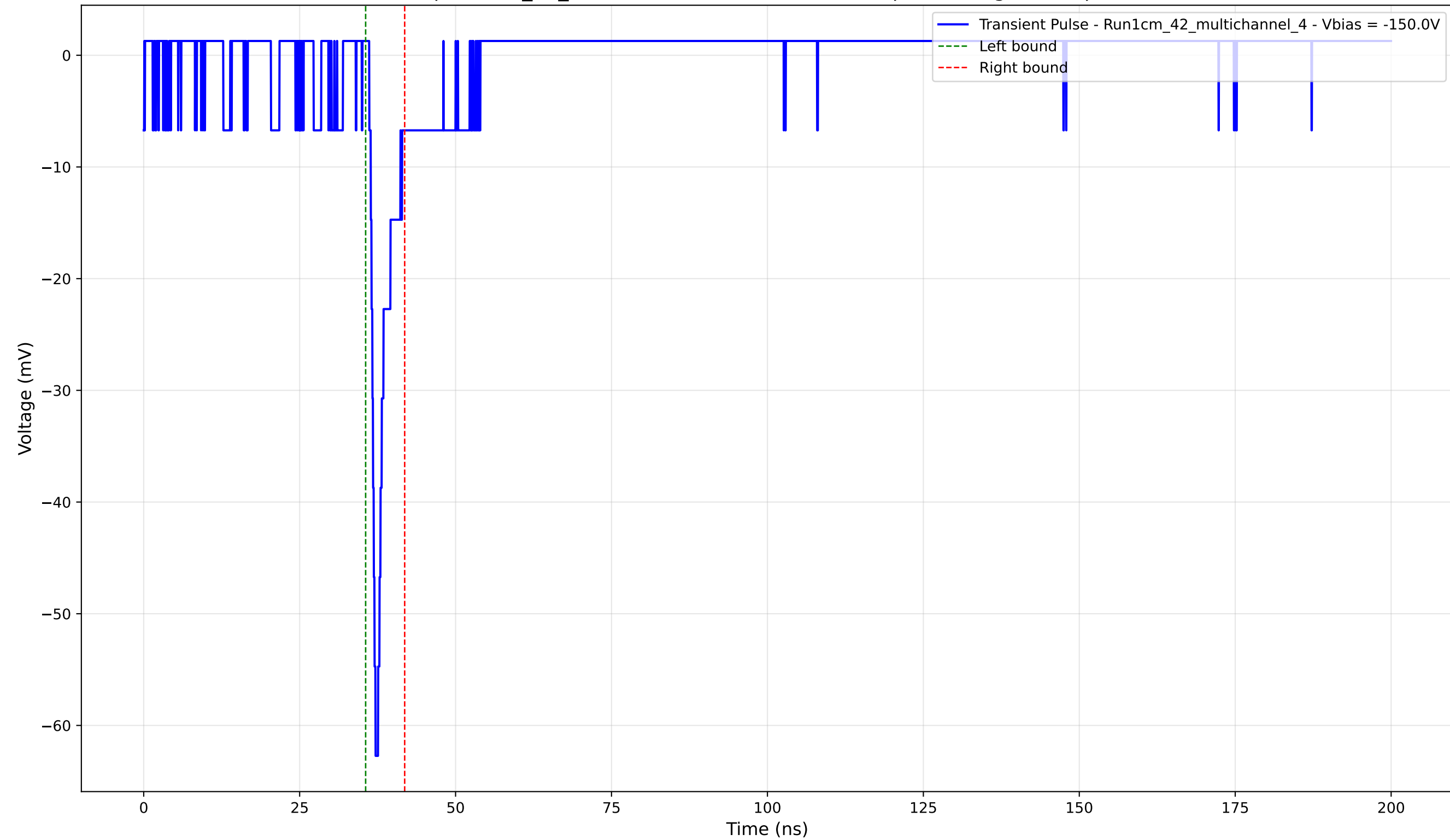
Transient Pulse - Sample: 1cm_42_multichannel - Position: 2635.0 \mu\text{m} - Charge: 2.90 pC - Rise Time: 1.00 ns
