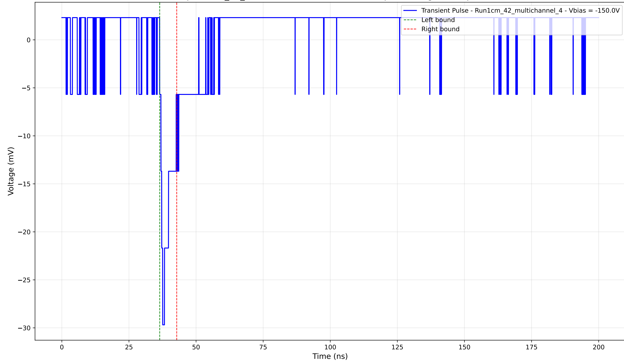
Transient Pulse - Sample: 1cm_42_multichannel - Position: 3225.0 \mu\text{m} - Charge: 2.17 pC - Rise Time: 1.14 ns
