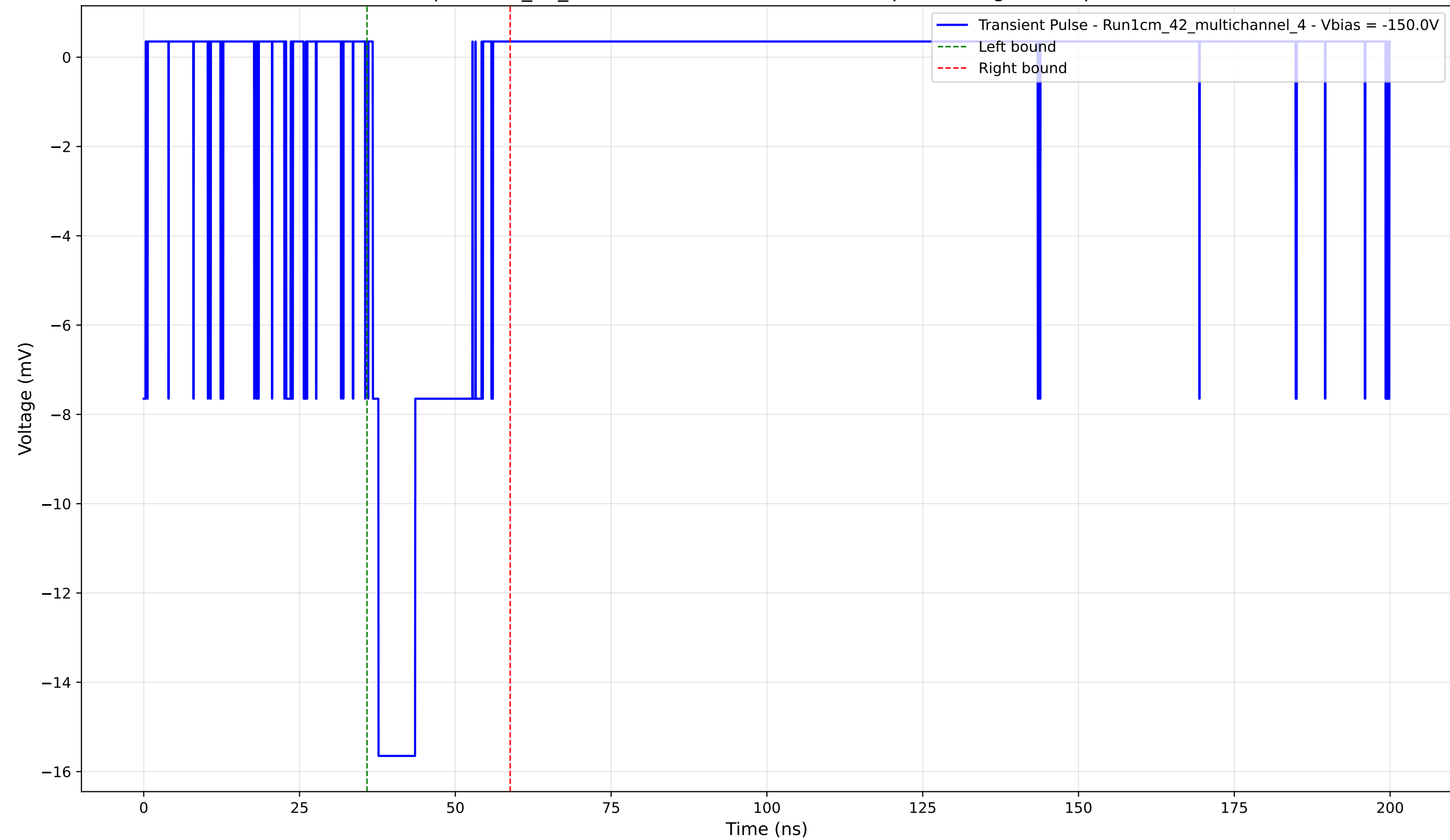
Transient Pulse - Sample: 1cm_42_multichannel - Position: 3760.0 \mu\text{m} - Charge: 3.62 pC - Rise Time: 0.92 ns
