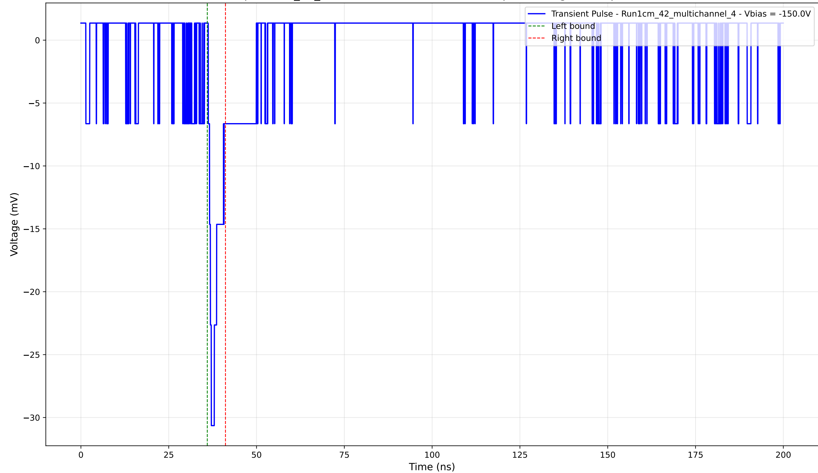
Transient Pulse - Sample: 1cm_42_multichannel - Position: 1935.0 \mu\text{m} - Charge: 1.73 pC - Rise Time: 0.87 ns
