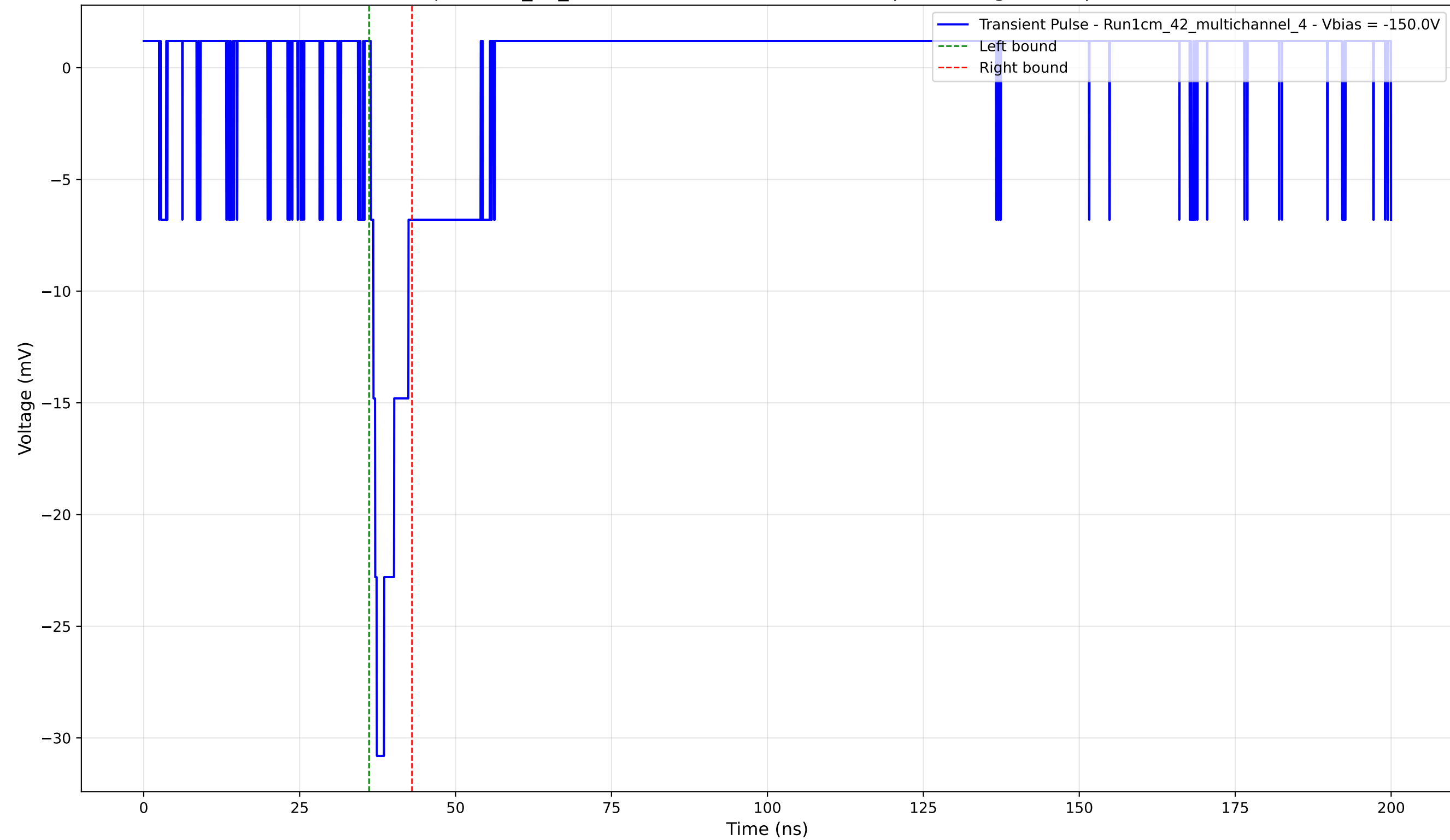
Transient Pulse - Sample: 1cm_42_multichannel - Position: 1575.0 \mu\text{m} - Charge: 2.46 pC - Rise Time: 0.95 ns
