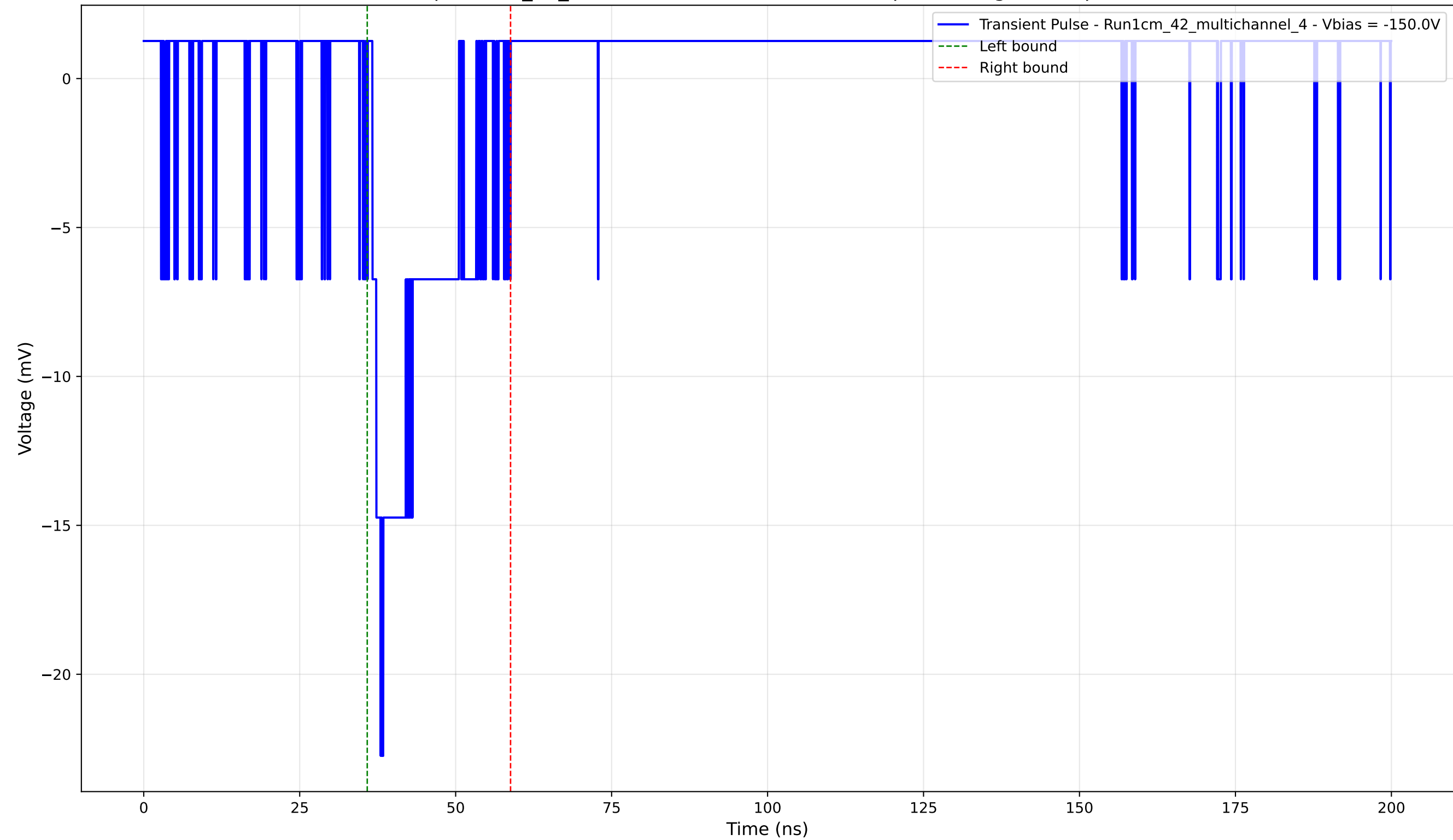
Transient Pulse - Sample: 1cm_42_multichannel - Position: 3465.0 \mu\text{m} - Charge: 3.17 pC - Rise Time: 1.34 ns
