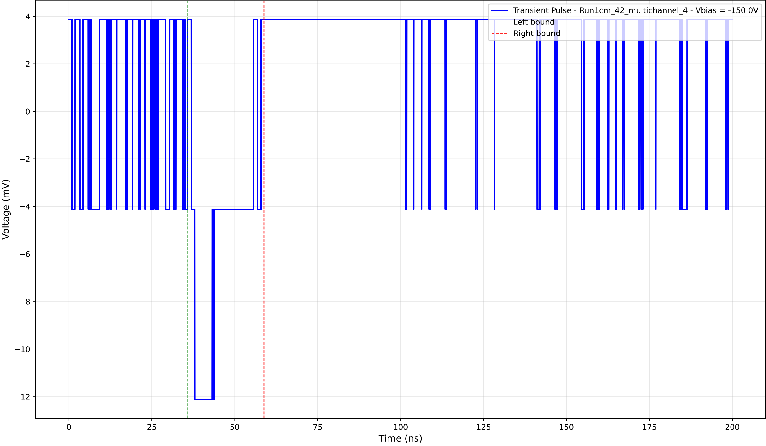
Transient Pulse - Sample: 1cm_42_multichannel - Position: 535.0 \mu\text{m} - Charge: 2.31 pC - Rise Time: 0.00 ns (N/A)
