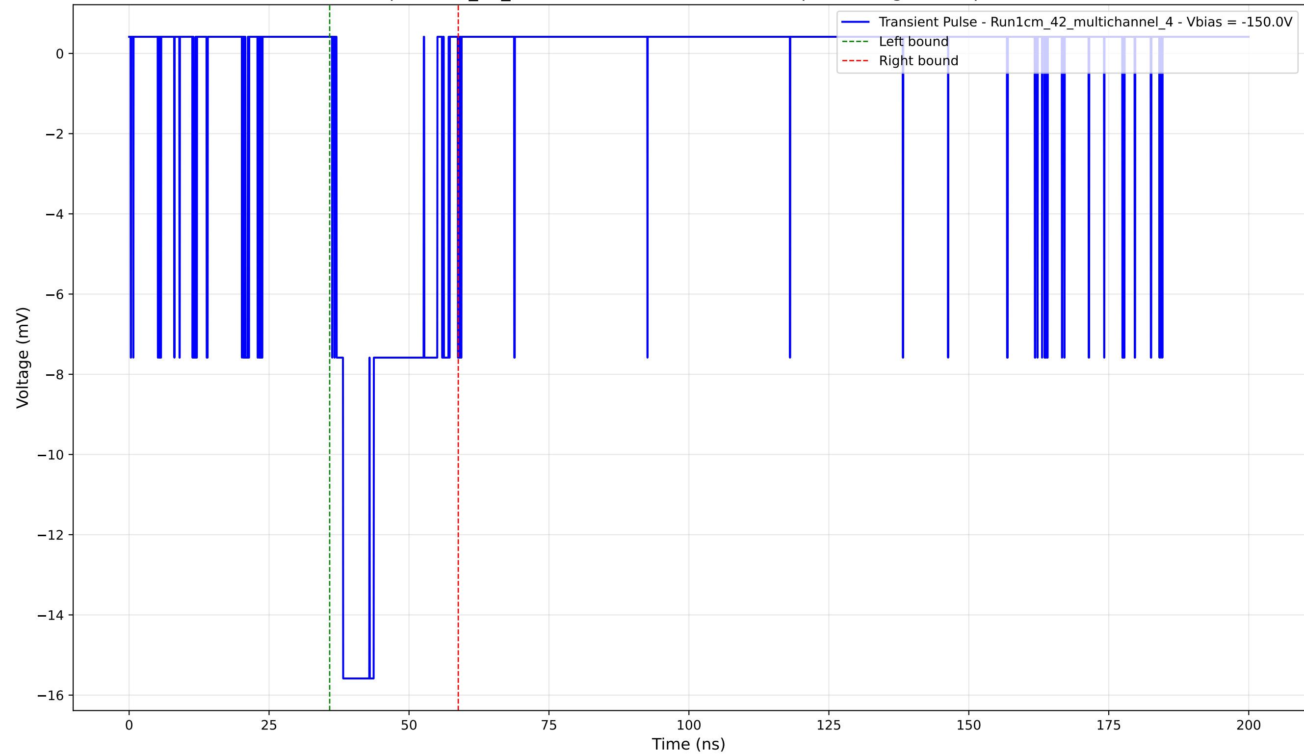
Transient Pulse - Sample: 1cm_42_multichannel - Position: 4095.0 \mu\text{m} - Charge: 3.75 pC - Rise Time: 1.18 ns
