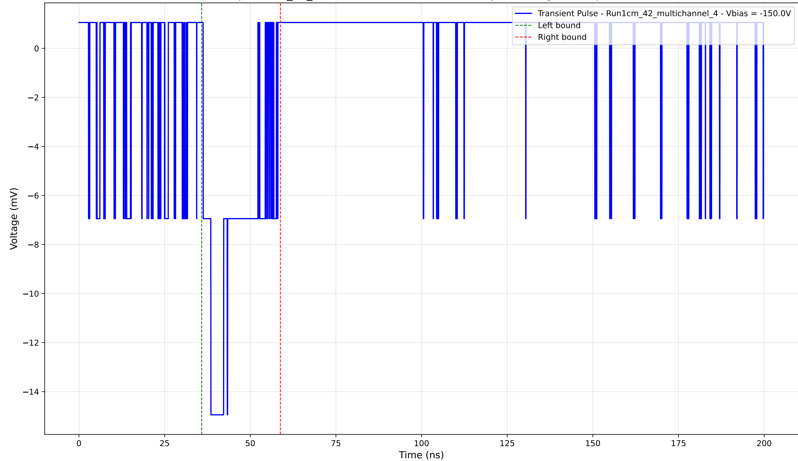
Transient Pulse - Sample: 1cm_42_multichannel - Position: 4650.0 \mu\text{m} - Charge: 3.30 pC - Rise Time: 2.26 ns
