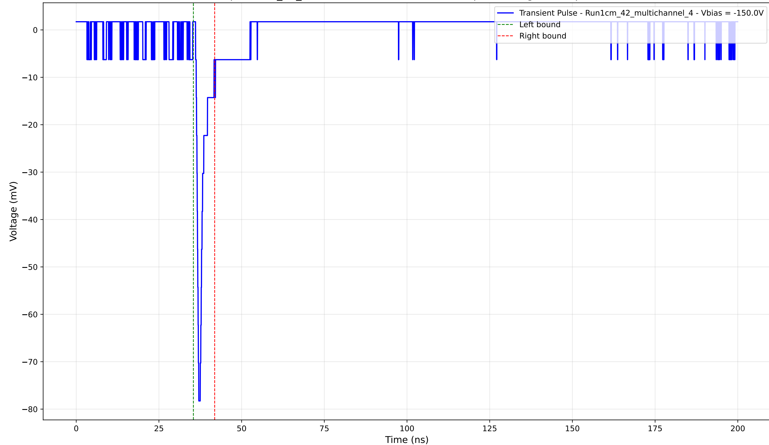
Transient Pulse - Sample: 1cm_42_multichannel - Position: 2260.0 \mu\text{m} - Charge: 3.43 pC - Rise Time: 0.78 ns
