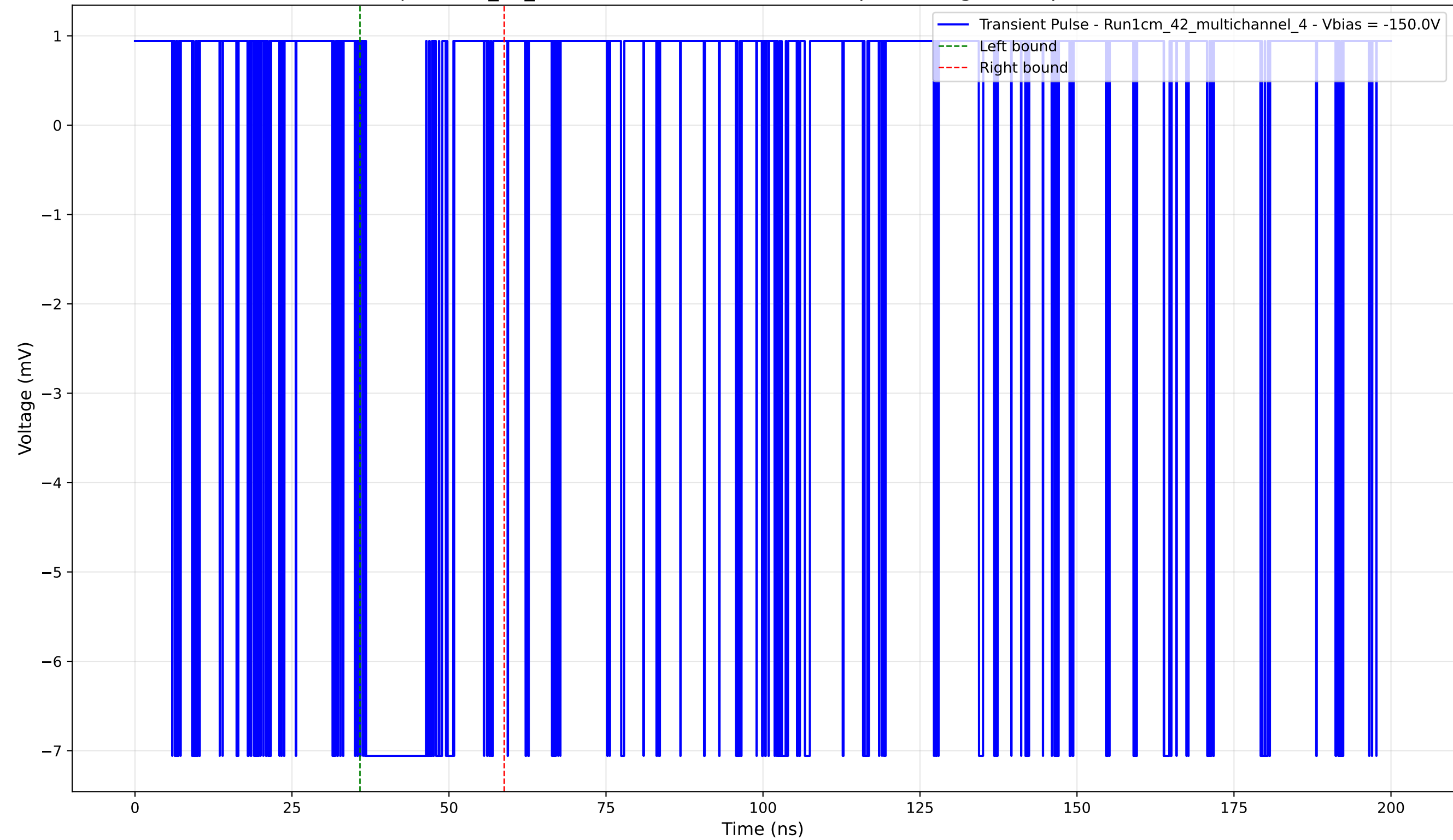
Transient Pulse - Sample: 1cm_42_multichannel - Position: 3435.0 \mu\text{m} - Charge: 1.68 pC - Rise Time: 0.00 ns (N/A)
