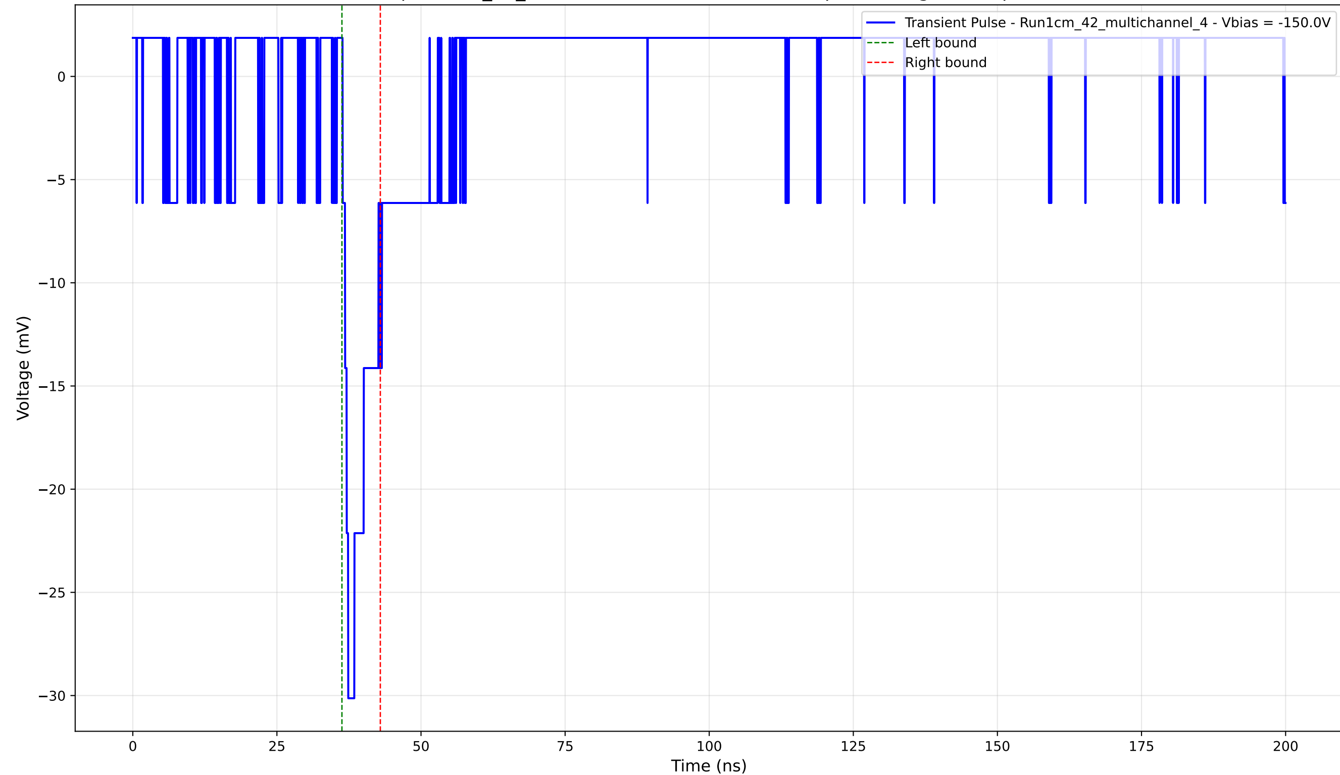
Transient Pulse - Sample: 1cm_42_multichannel - Position: 1600.0 \mu\text{m} - Charge: 2.40 pC - Rise Time: 0.97 ns
