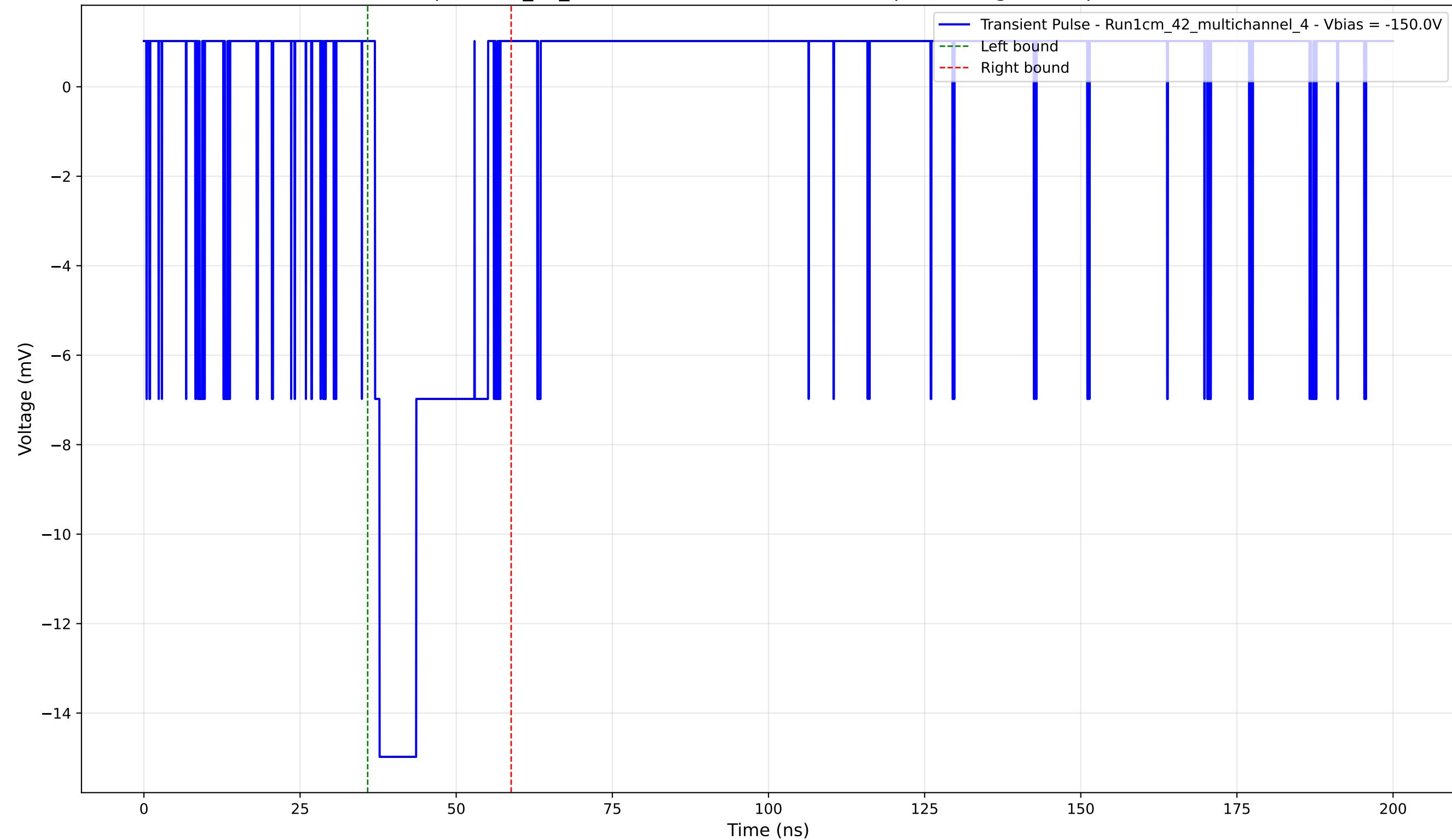
Transient Pulse - Sample: 1cm_42_multichannel - Position: 3810.0 \mu\text{m} - Charge: 3.45 pC - Rise Time: 0.74 ns
