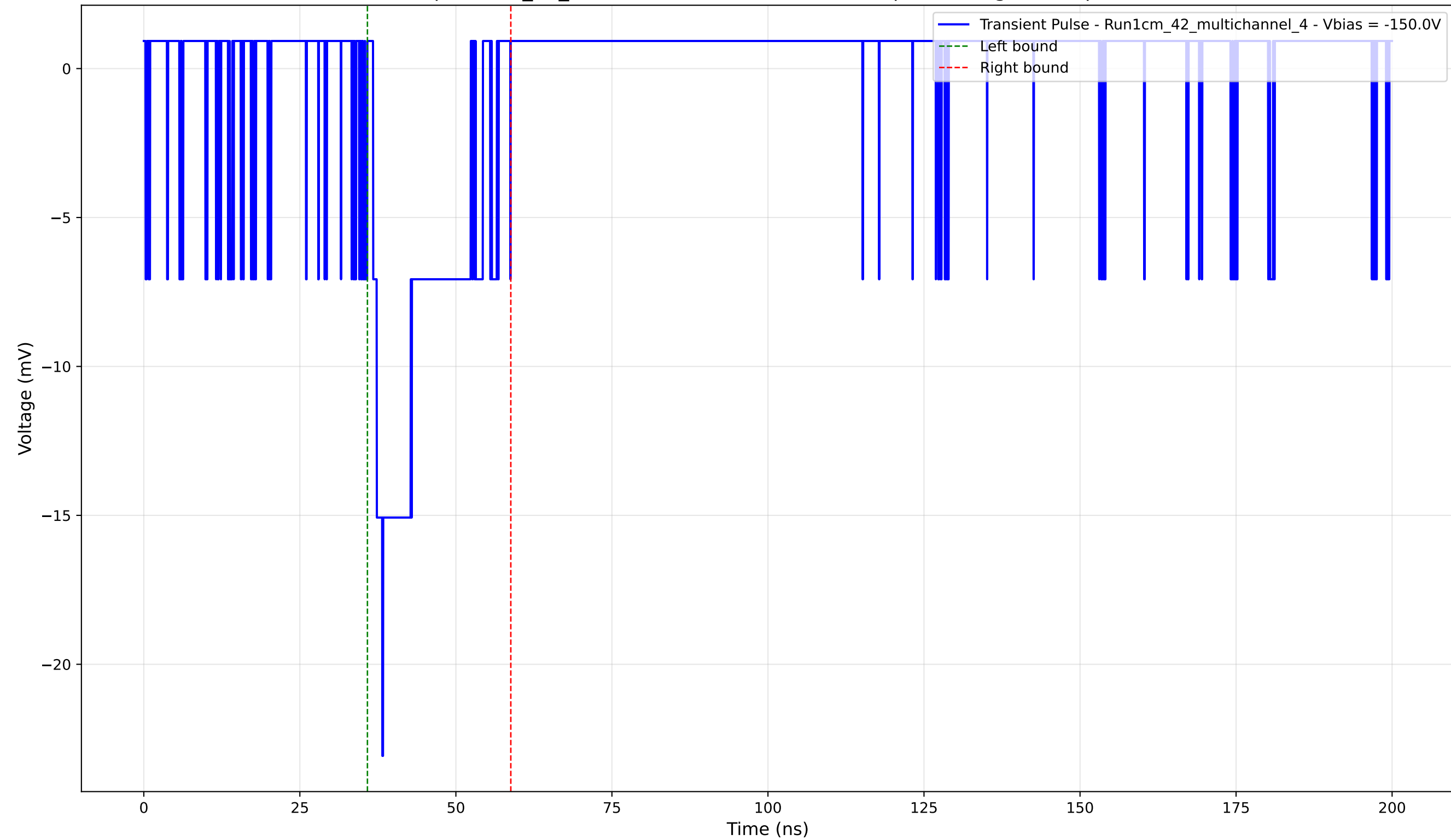
Transient Pulse - Sample: 1cm_42_multichannel - Position: 3580.0 \mu\text{m} - Charge: 3.38 pC - Rise Time: 1.48 ns
