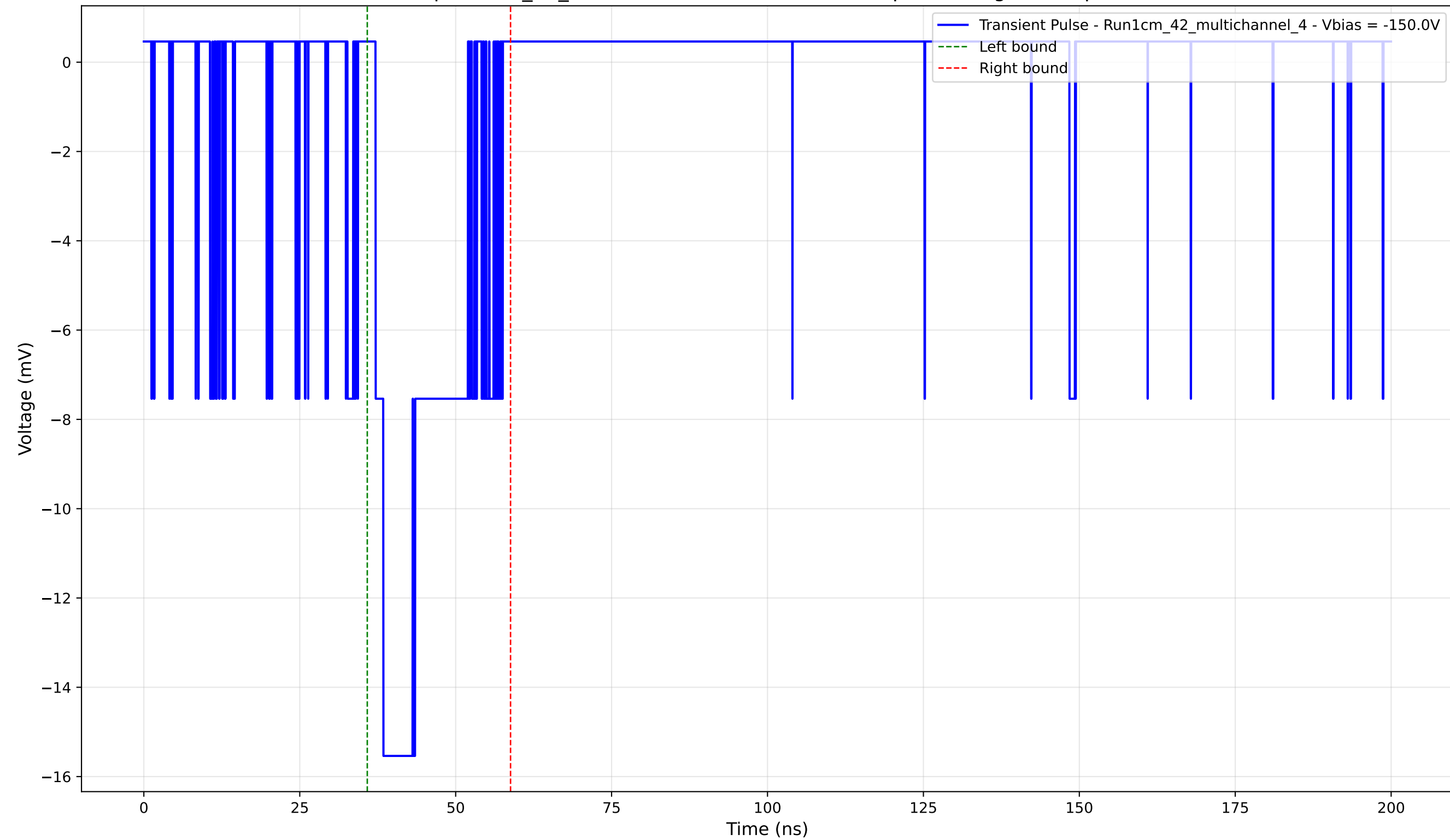
Transient Pulse - Sample: 1cm_42_multichannel - Position: 4615.0 \mu\text{m} - Charge: 3.50 pC - Rise Time: 1.26 ns
