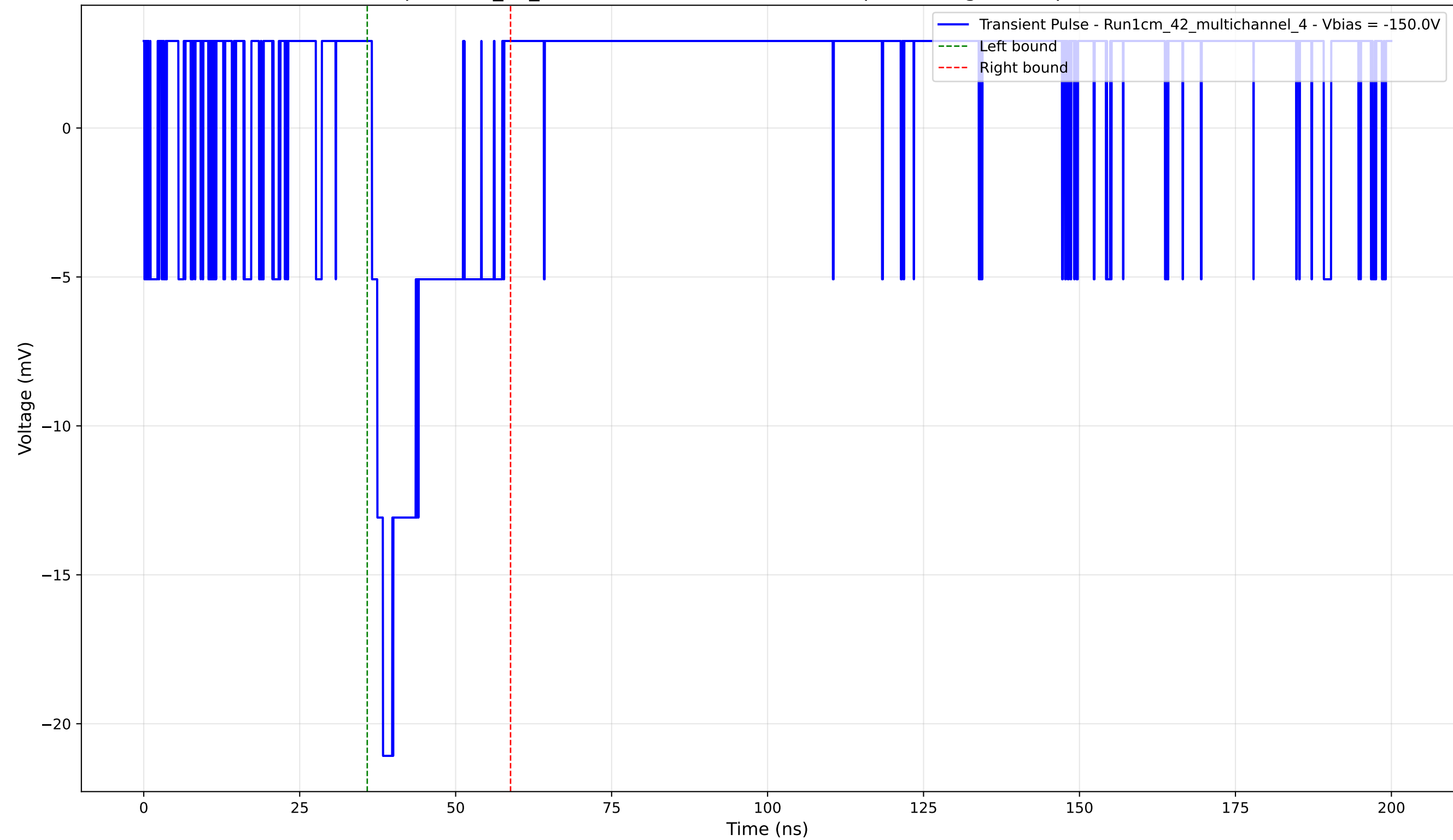
Transient Pulse - Sample: 1cm_42_multichannel - Position: 1040.0 \mu\text{m} - Charge: 3.24 pC - Rise Time: 0.00 ns (N/A)
