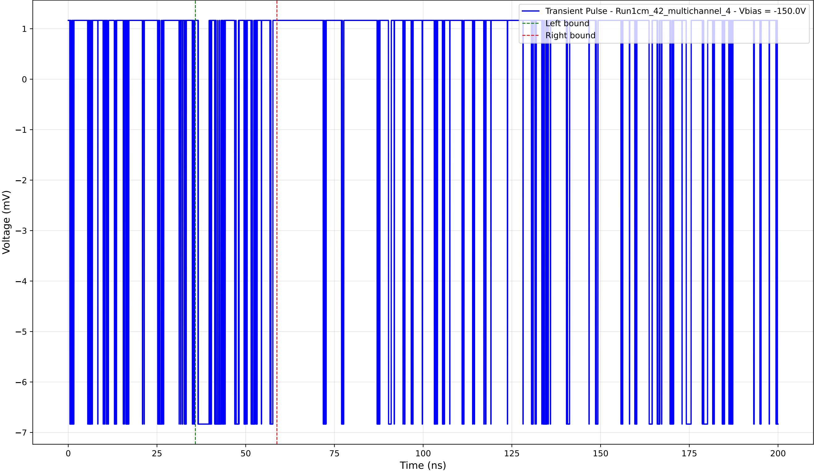
Transient Pulse - Sample: 1cm_42_multichannel - Position: 2875.0 \mu\text{m} - Charge: 0.86 pC - Rise Time: 0.00 ns (N/A)
