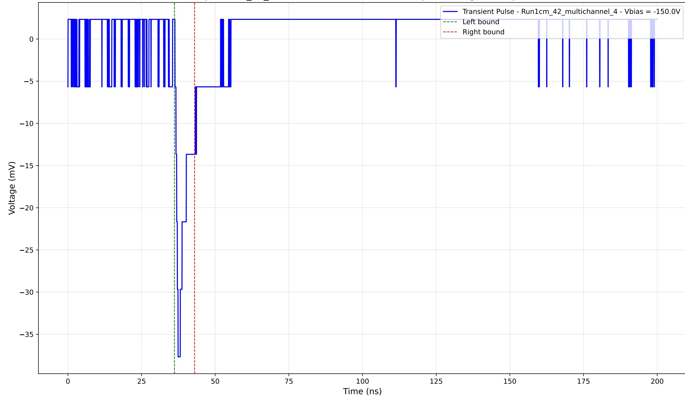
Transient Pulse - Sample: 1cm_42_multichannel - Position: 1715.0 \mu\text{m} - Charge: 2.66 pC - Rise Time: 1.05 ns
