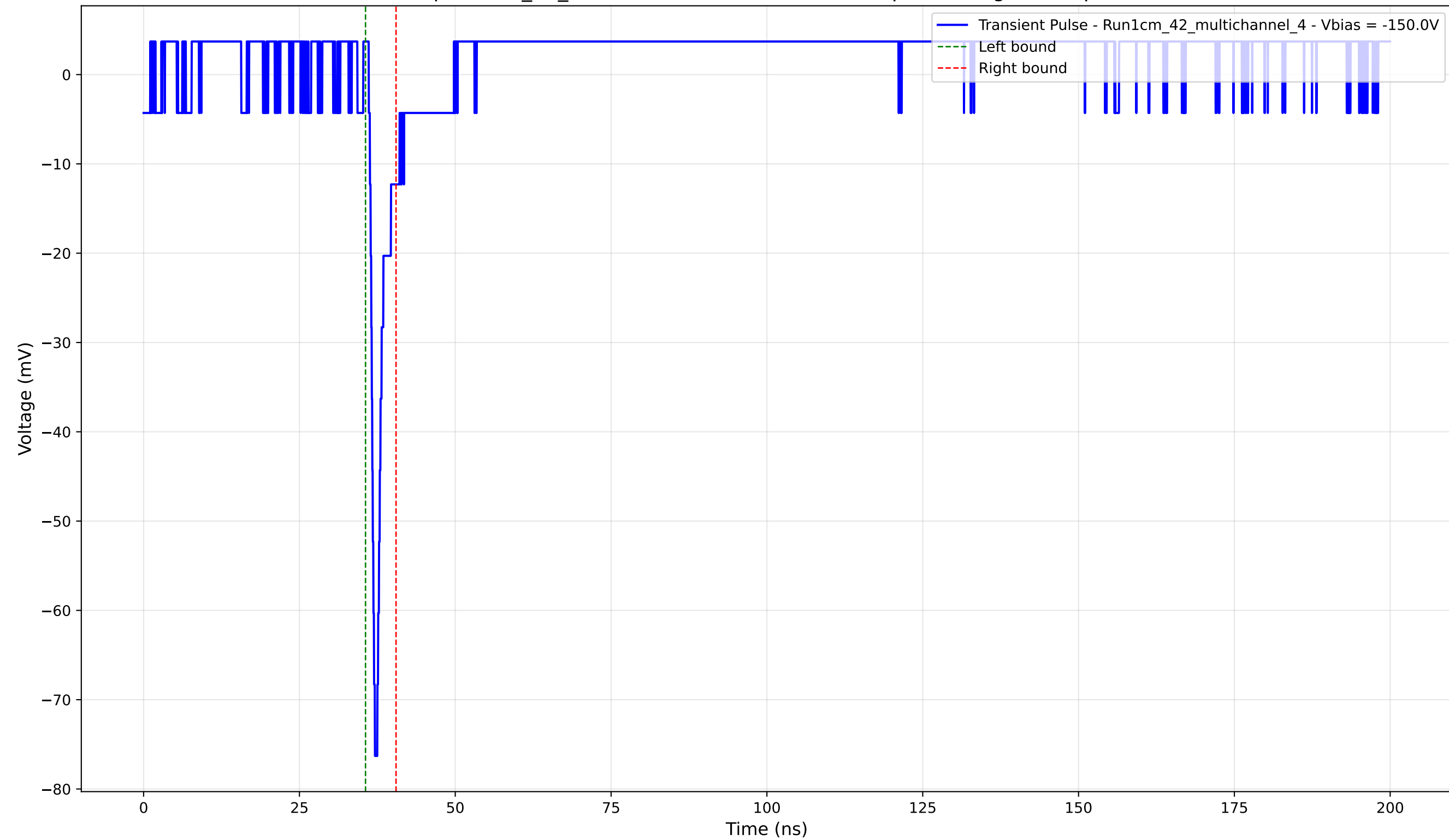
Transient Pulse - Sample: 1cm_42_multichannel - Position: 2255.0 \mu\text{m} - Charge: 2.80 pC - Rise Time: 0.81 ns
