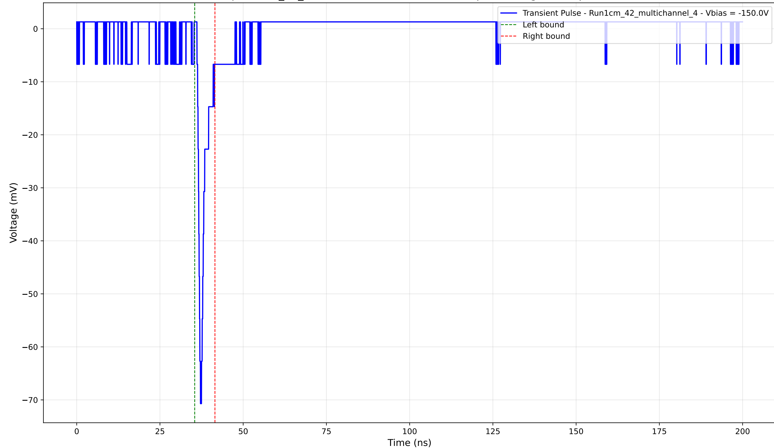
Transient Pulse - Sample: 1cm_42_multichannel - Position: 2580.0 \mu\text{m} - Charge: 3.03 pC - Rise Time: 0.86 ns
