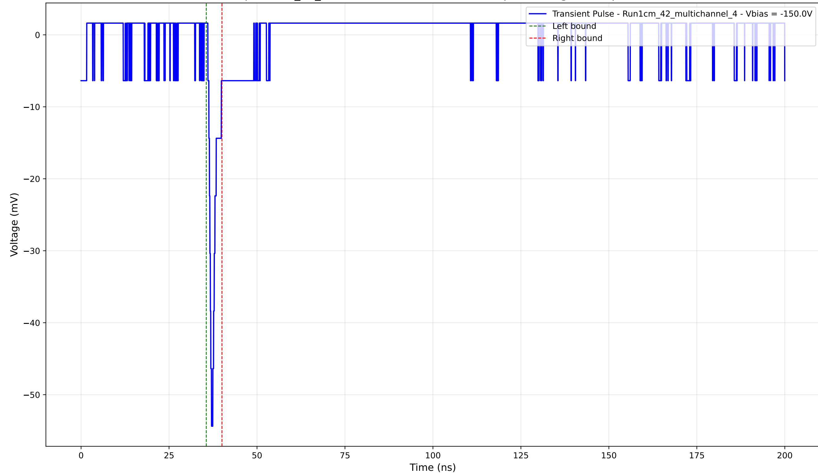
Transient Pulse - Sample: 1cm_42_multichannel - Position: 2330.0 \mu\text{m} - Charge: 1.97 pC - Rise Time: 1.02 ns
