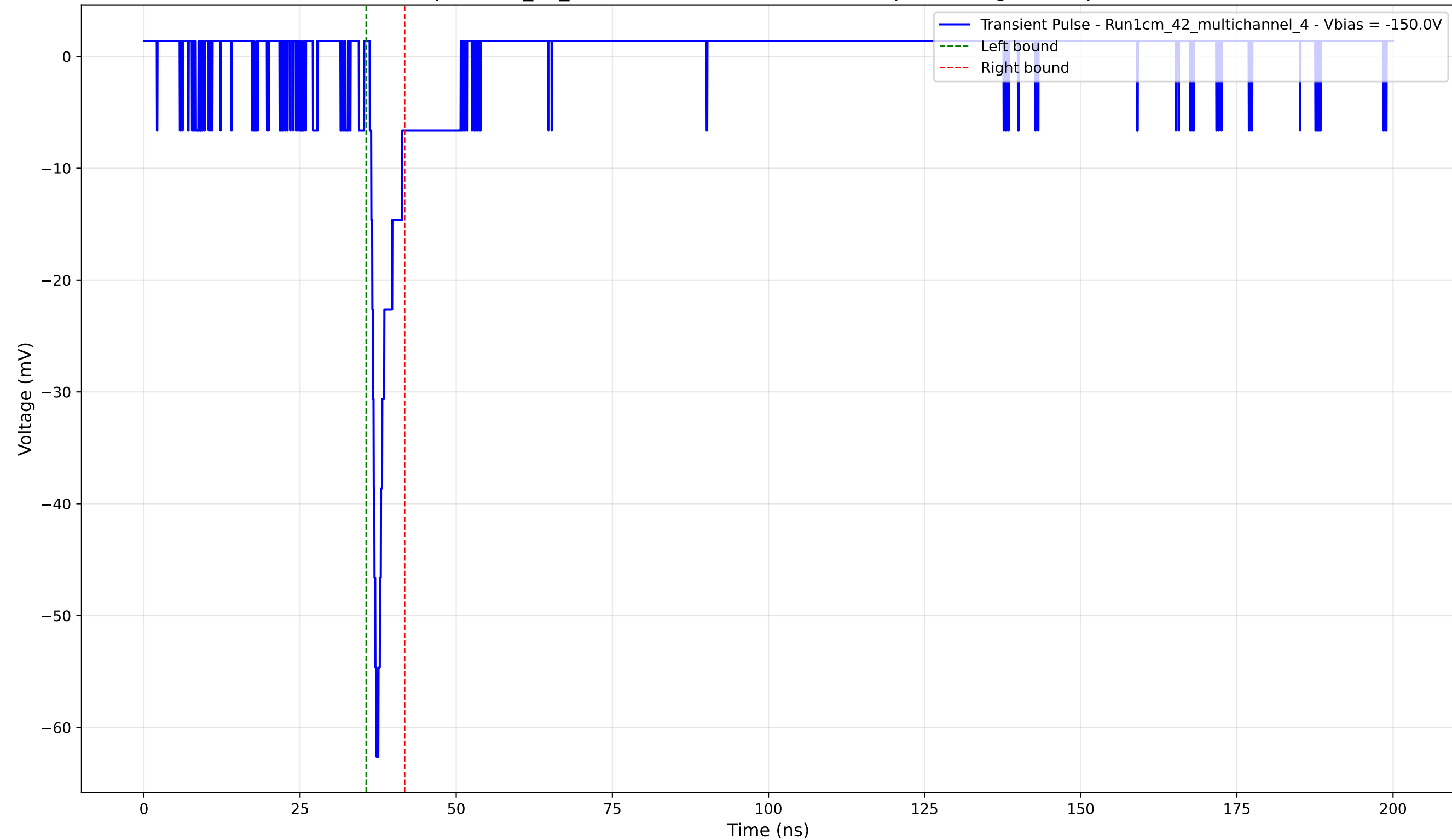
Transient Pulse - Sample: 1cm_42_multichannel - Position: 2650.0 \mu\text{m} - Charge: 2.87 pC - Rise Time: 1.06 ns
