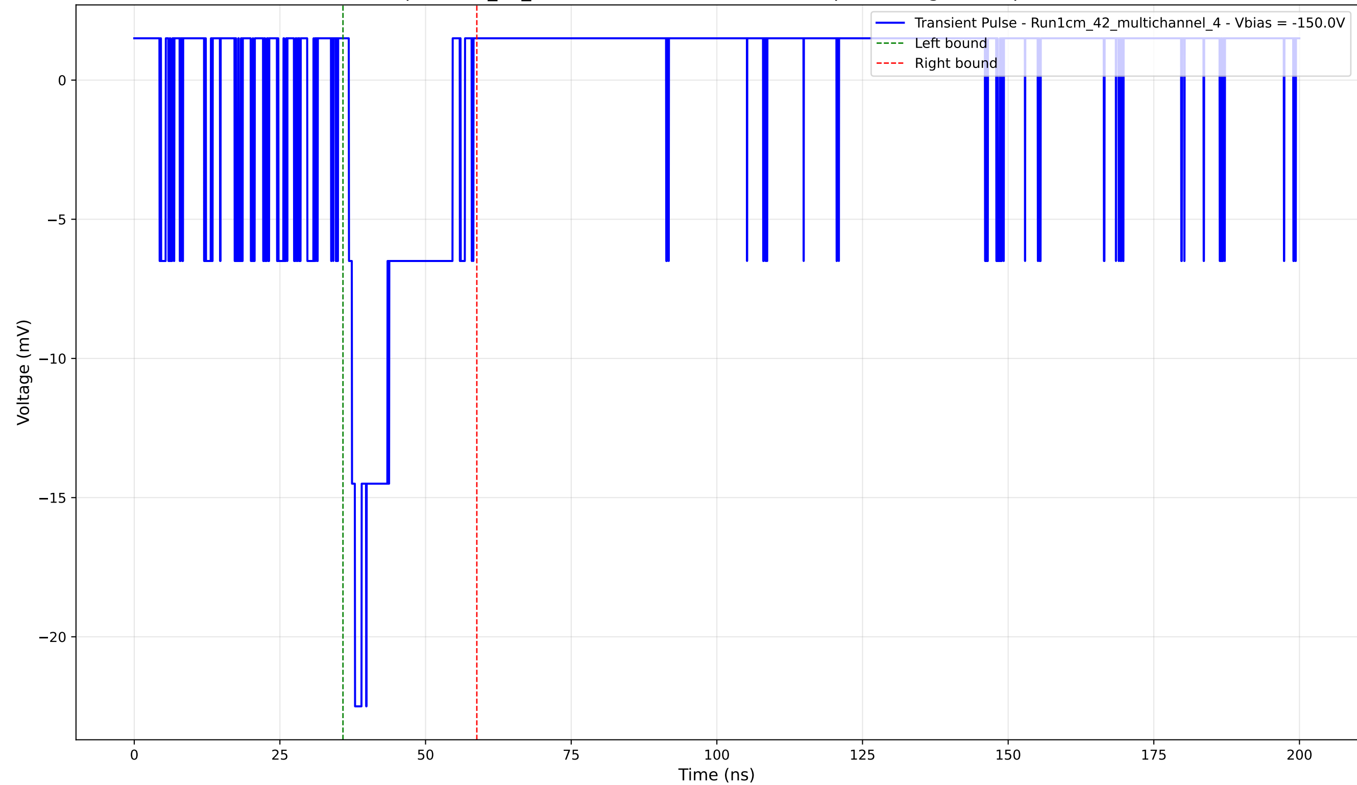
Transient Pulse - Sample: 1cm_42_multichannel - Position: 1120.0 \mu\text{m} - Charge: 3.50 pC - Rise Time: 1.06 ns
