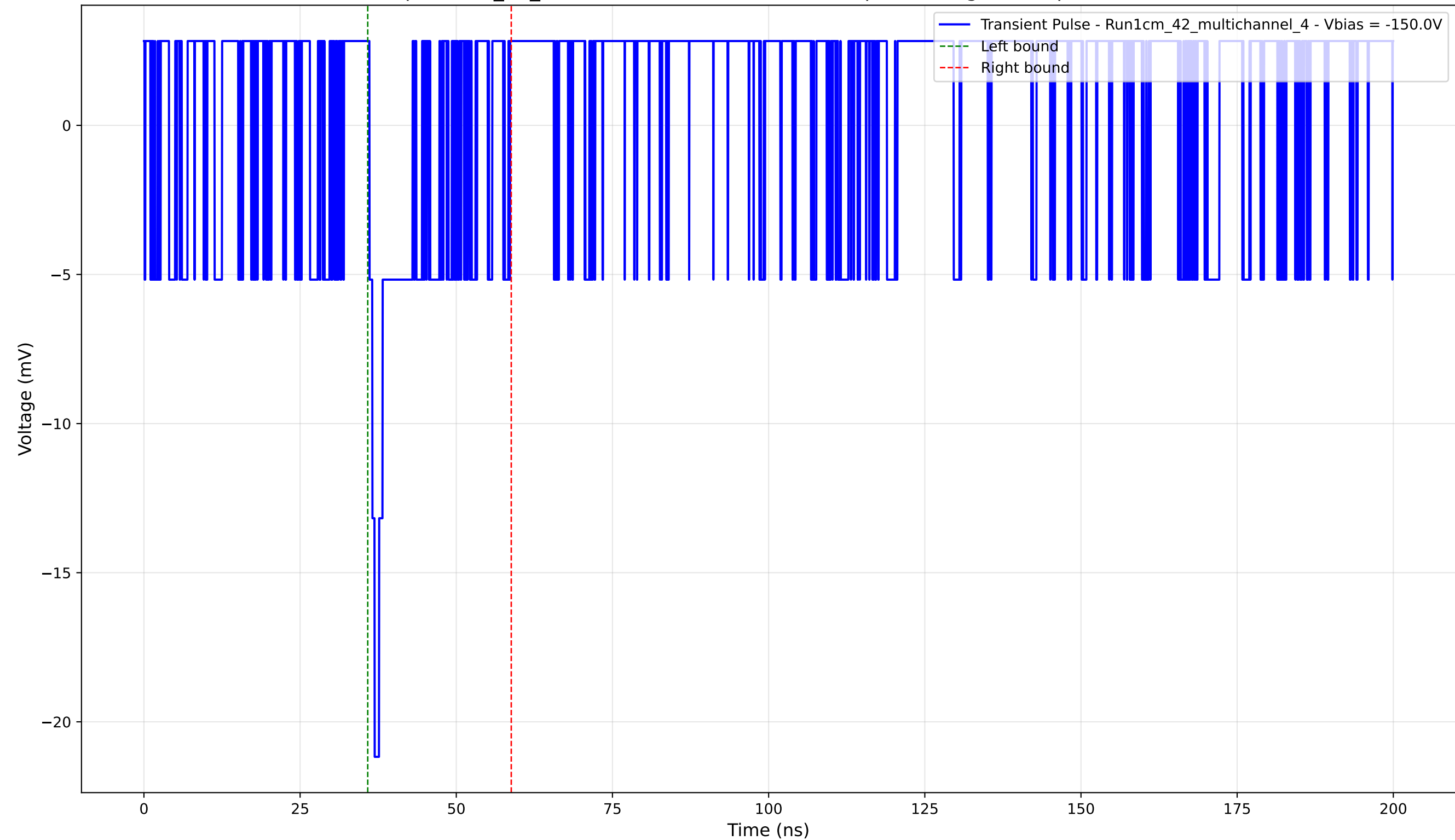
Transient Pulse - Sample: 1cm_42_multichannel - Position: 2345.0 \mu\text{m} - Charge: 1.37 pC - Rise Time: 0.00 ns (N/A)
