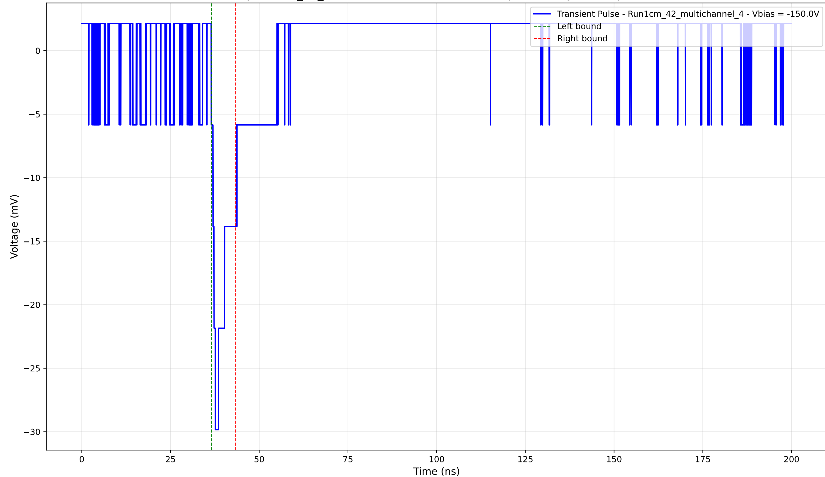
Transient Pulse - Sample: 1cm_42_multichannel - Position: 1465.0 \mu\text{m} - Charge: 2.45 pC - Rise Time: 1.18 ns
