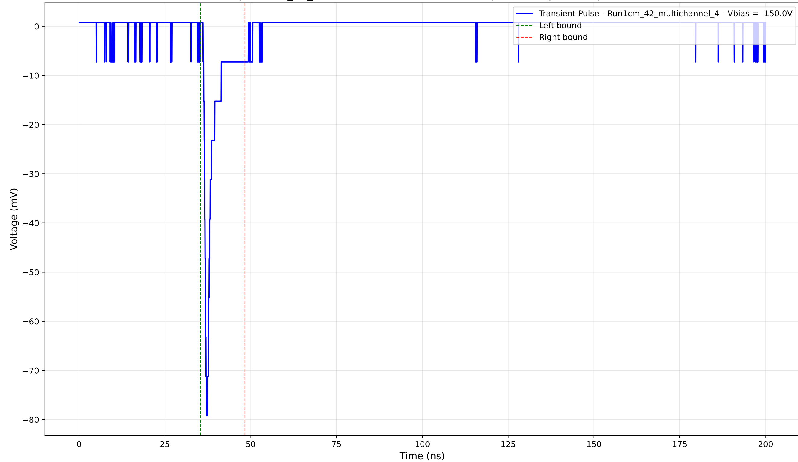
Transient Pulse - Sample: 1cm_42_multichannel - Position: 2510.0 \mu\text{m} - Charge: 4.34 pC - Rise Time: 0.82 ns
