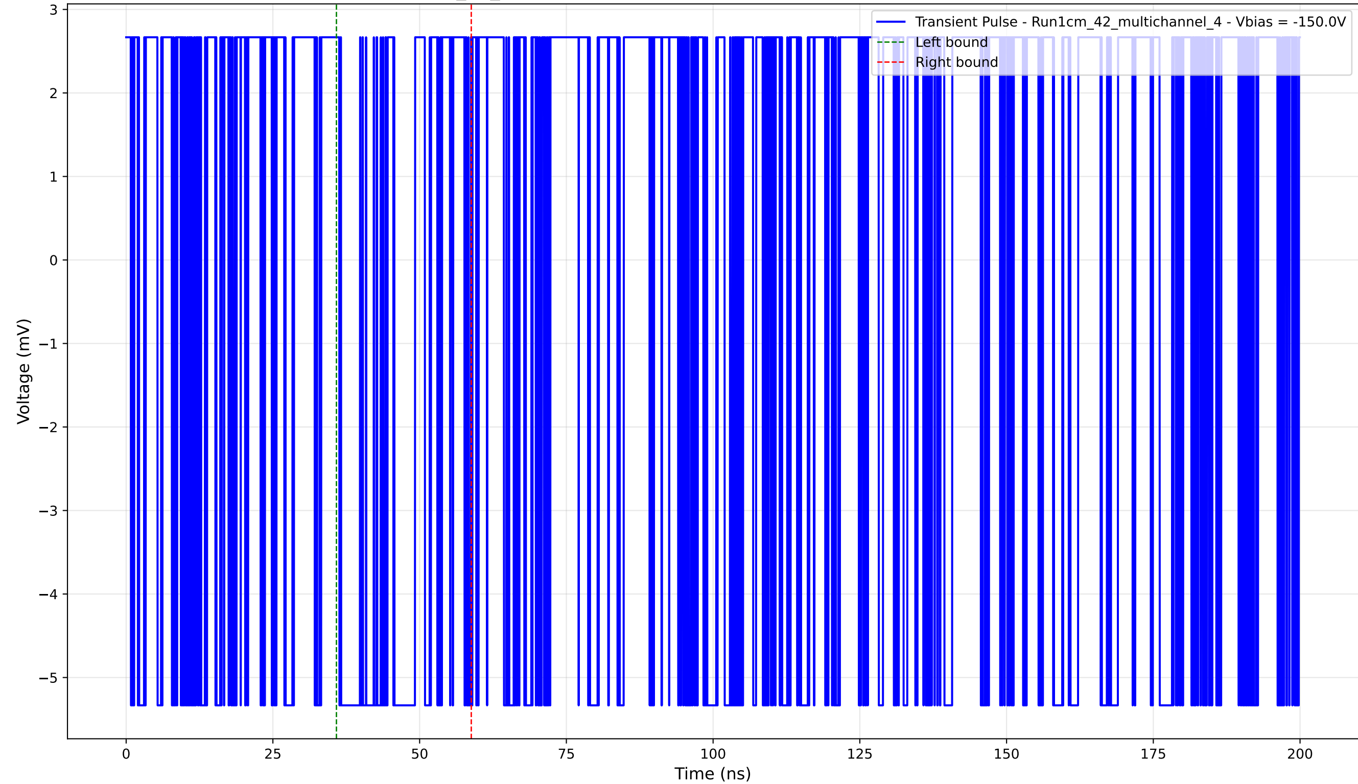
Transient Pulse - Sample: 1cm_42_multichannel - Position: 1350.0 \mu\text{m} - Charge: 0.96 pC - Rise Time: 0.00 ns (N/A)
