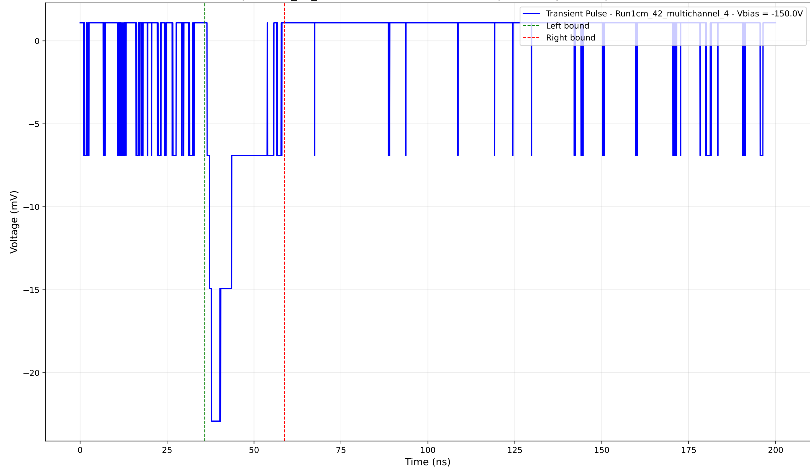
Transient Pulse - Sample: 1cm_42_multichannel - Position: 1200.0 \mu\text{m} - Charge: 4.18 pC - Rise Time: 1.28 ns
