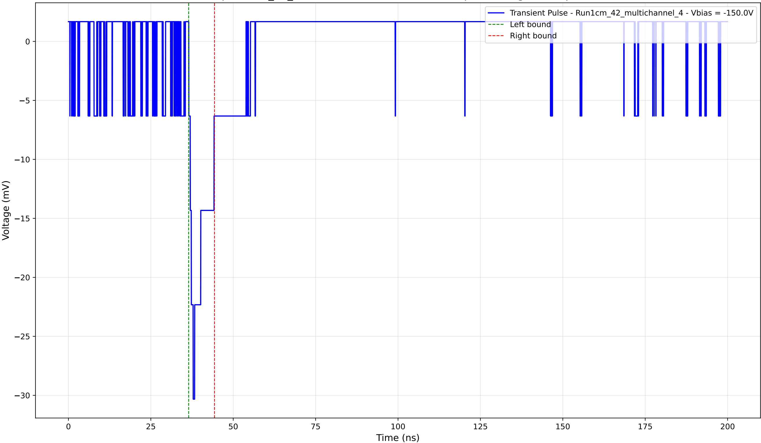
Transient Pulse - Sample: 1cm_42_multichannel - Position: 1455.0 \mu\text{m} - Charge: 2.67 pC - Rise Time: 1.33 ns
