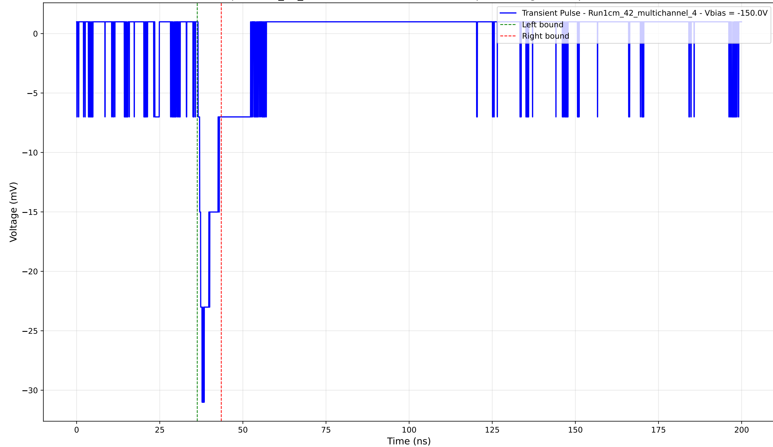
Transient Pulse - Sample: 1cm_42_multichannel - Position: 3295.0 \mu\text{m} - Charge: 2.37 pC - Rise Time: 1.21 ns
