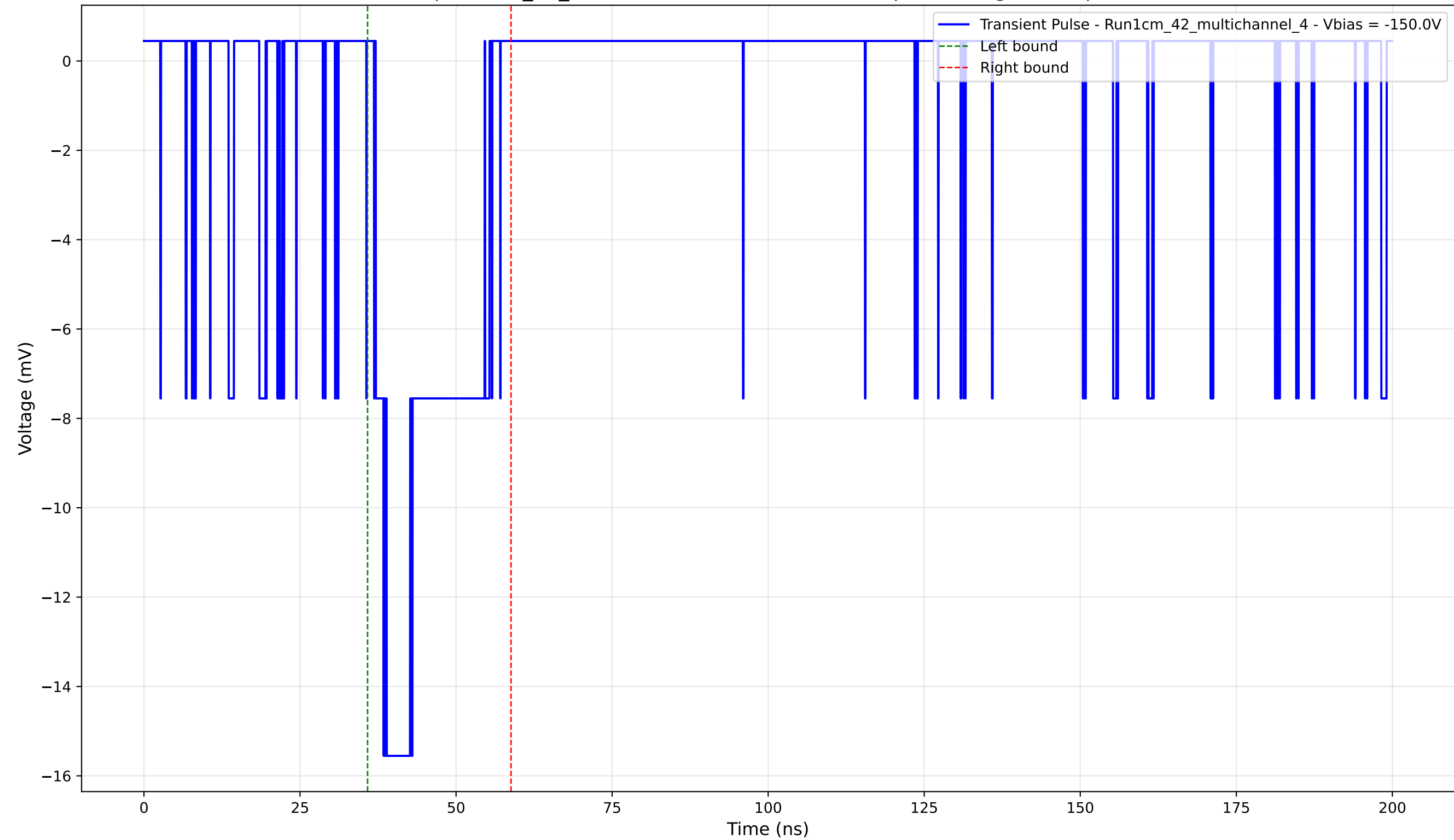
Transient Pulse - Sample: 1cm_42_multichannel - Position: 4700.0 \mu\text{m} - Charge: 3.39 pC - Rise Time: 1.28 ns
