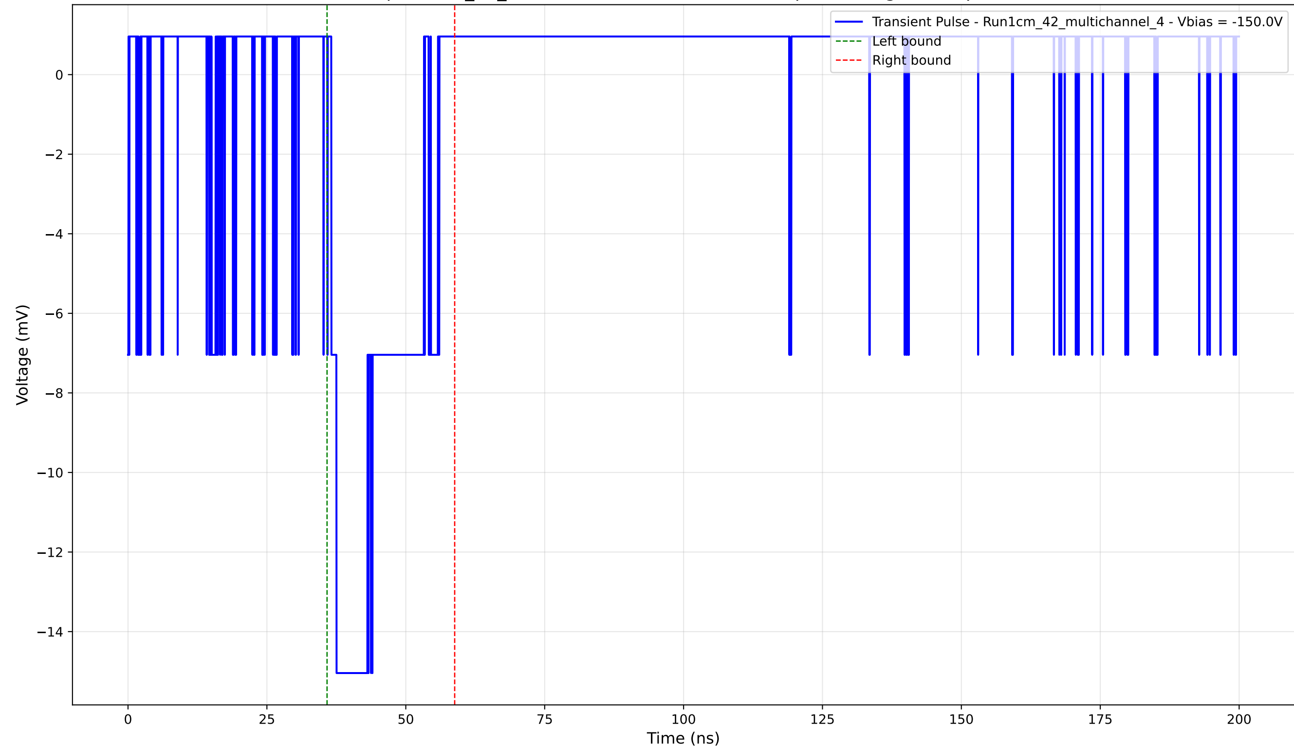
Transient Pulse - Sample: 1cm_42_multichannel - Position: 3750.0 \mu\text{m} - Charge: 3.45 pC - Rise Time: 0.94 ns
