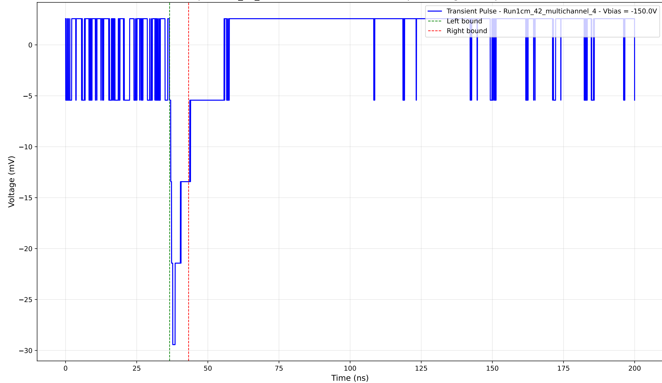
Transient Pulse - Sample: 1cm_42_multichannel - Position: 1460.0 \mu\text{m} - Charge: 2.38 pC - Rise Time: 1.22 ns
