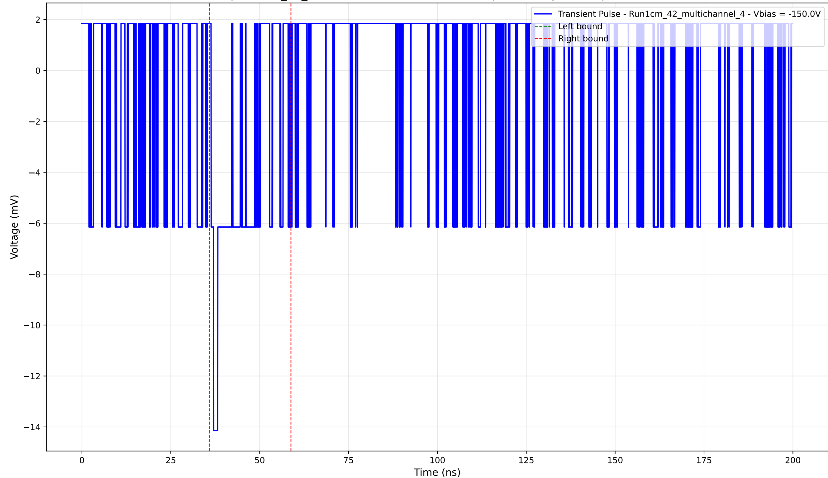
Transient Pulse - Sample: 1cm_42_multichannel - Position: 1920.0 \mu\text{m} - Charge: 1.67 pC - Rise Time: 0.00 ns (N/A)
