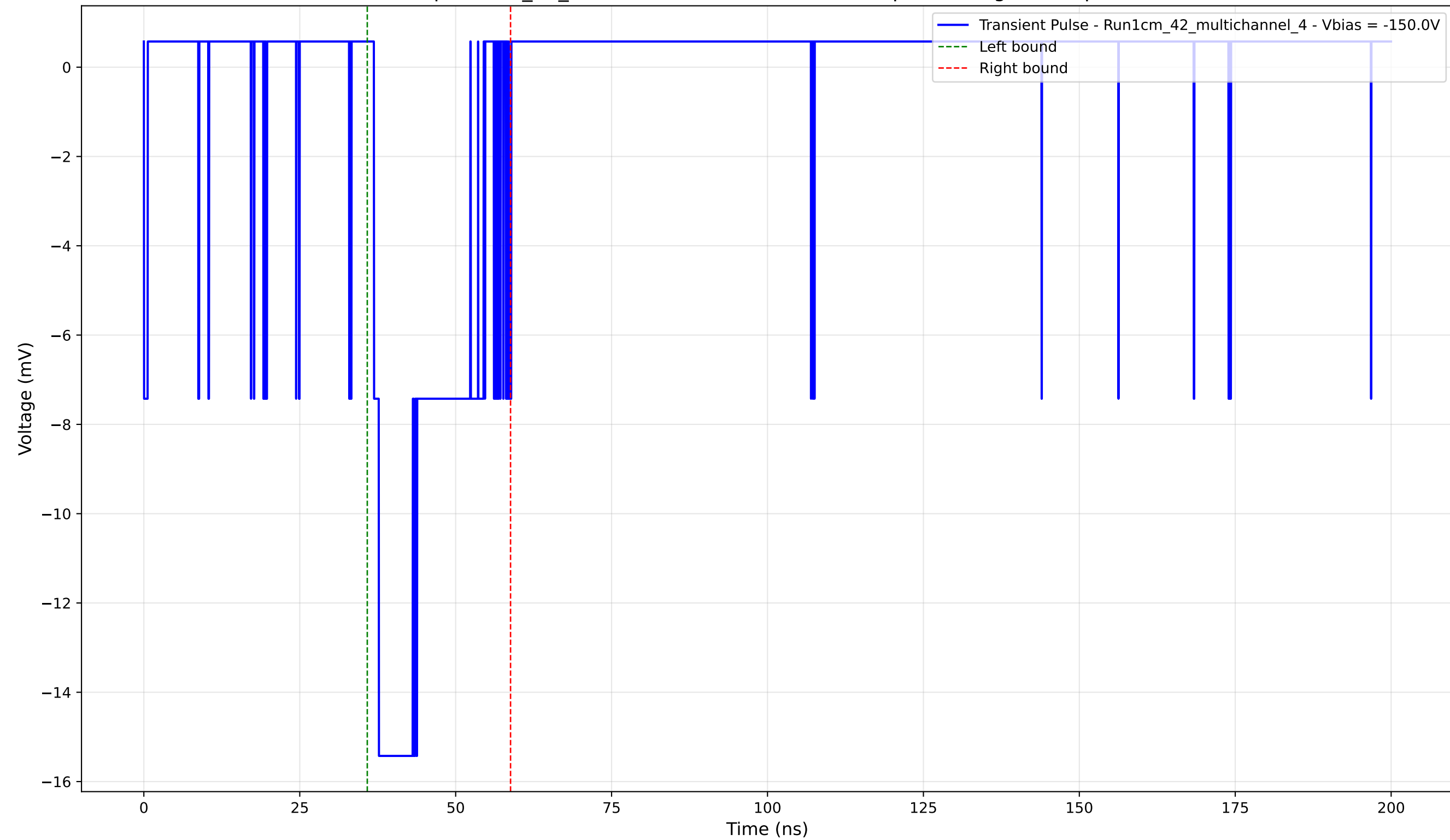
Transient Pulse - Sample: 1cm_42_multichannel - Position: 3805.0 \mu\text{m} - Charge: 3.63 pC - Rise Time: 0.80 ns
