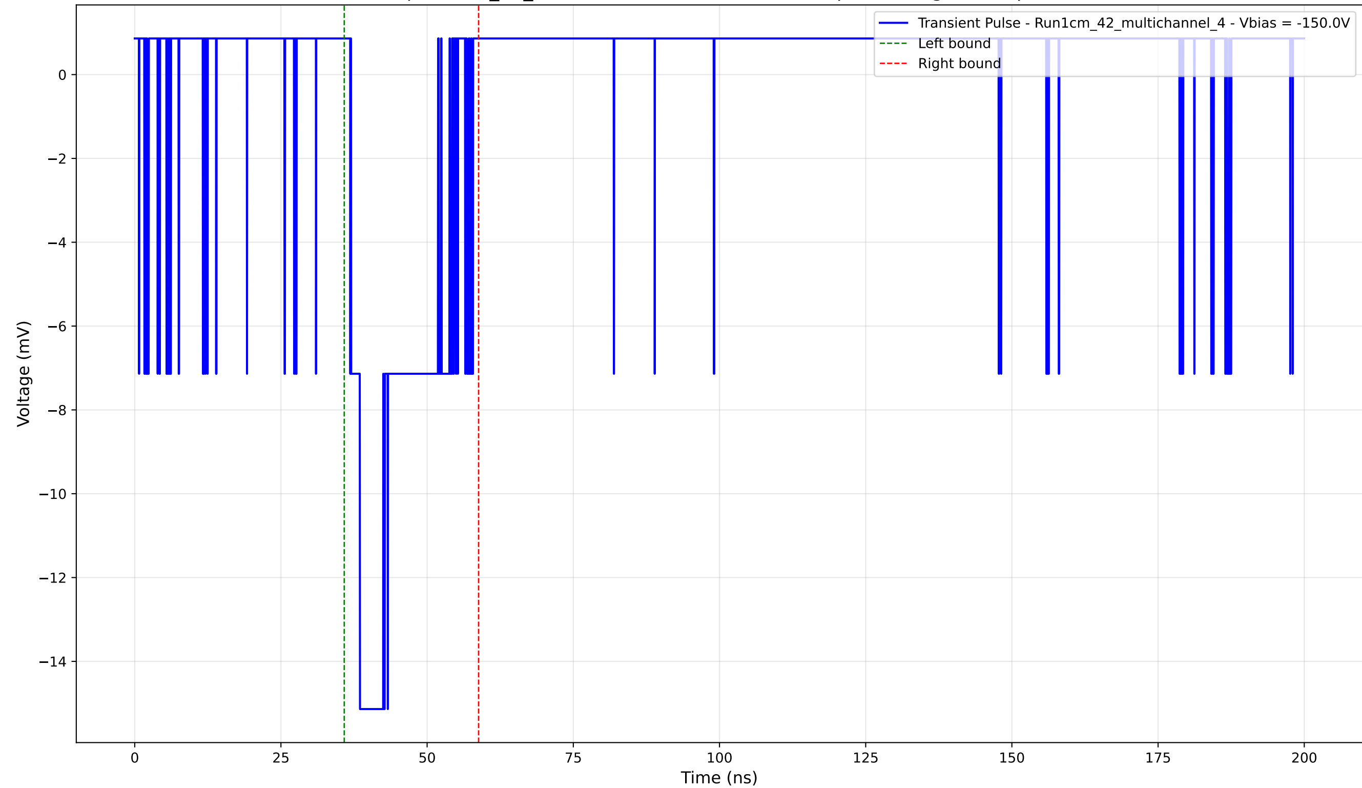
Transient Pulse - Sample: 1cm_42_multichannel - Position: 4685.0 \mu\text{m} - Charge: 3.17 pC - Rise Time: 1.52 ns
