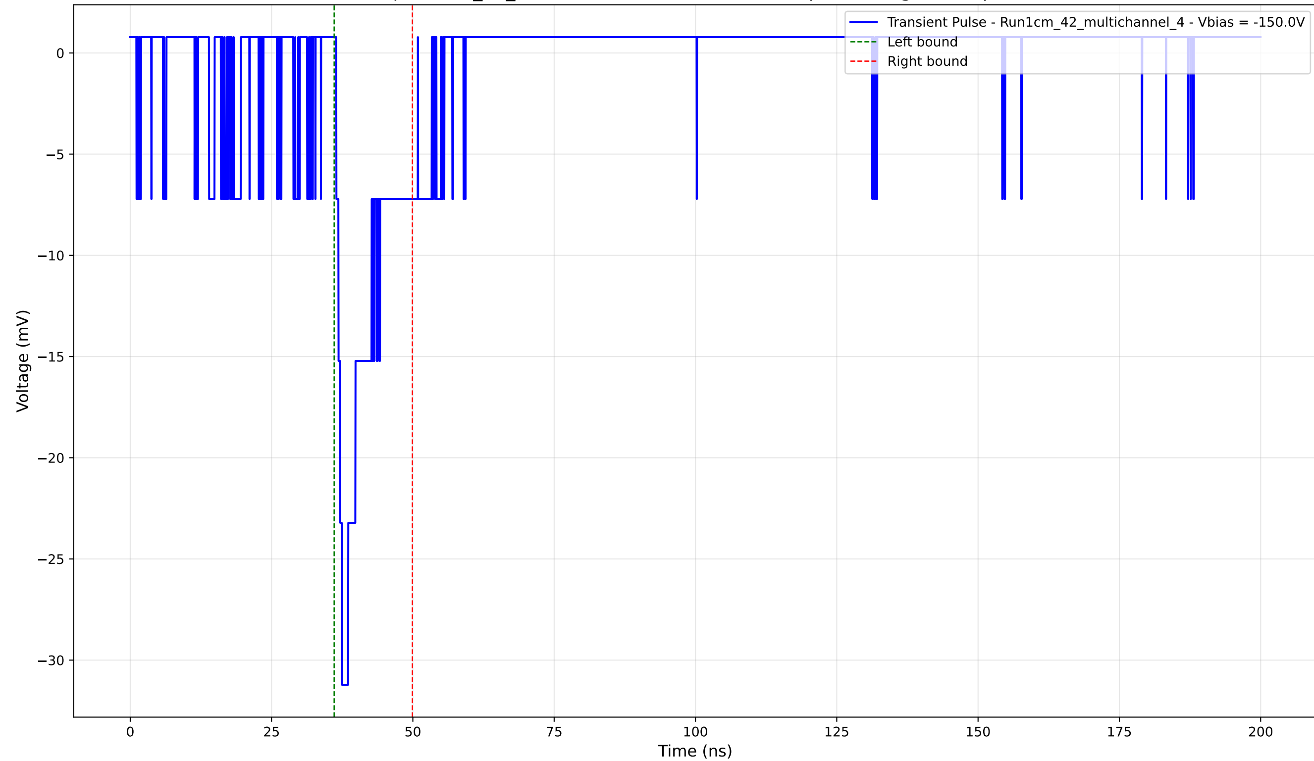
Transient Pulse - Sample: 1cm_42_multichannel - Position: 1560.0 \mu\text{m} - Charge: 3.57 pC - Rise Time: 0.99 ns
