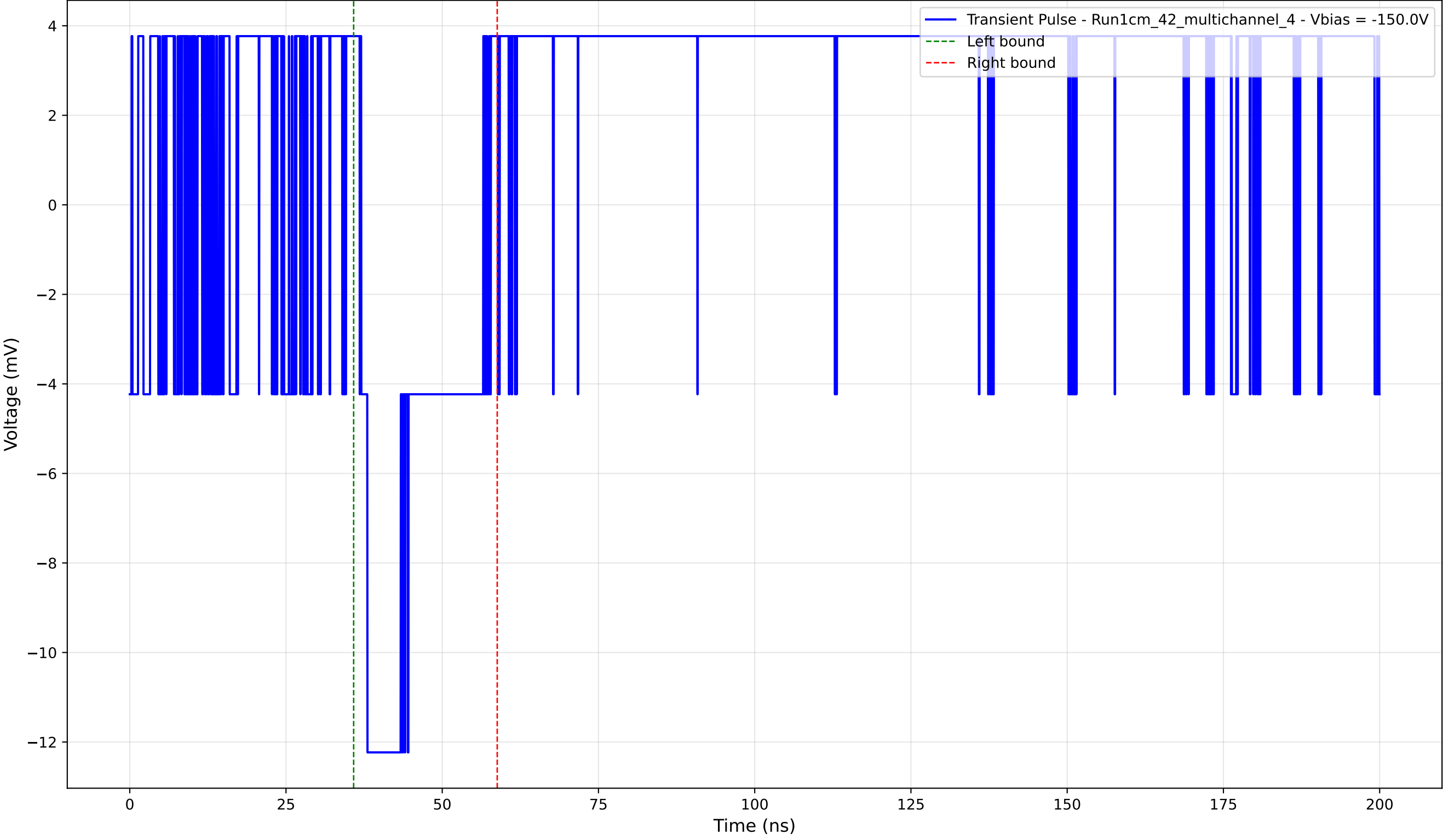
Transient Pulse - Sample: 1cm_42_multichannel - Position: 550.0 \mu\text{m} - Charge: 2.41 pC - Rise Time: 0.00 ns (N/A)
