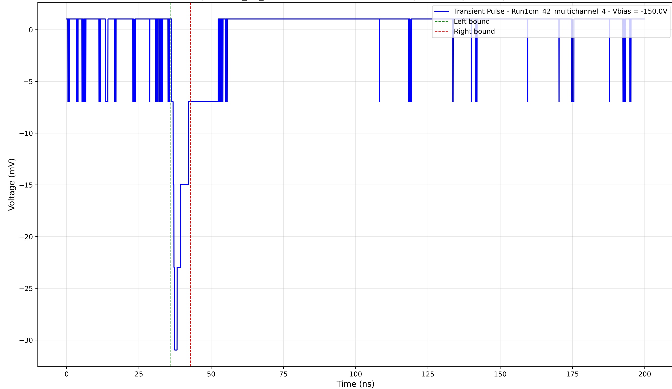
Transient Pulse - Sample: 1cm_42_multichannel - Position: 3115.0 \mu\text{m} - Charge: 2.23 pC - Rise Time: 1.05 ns
