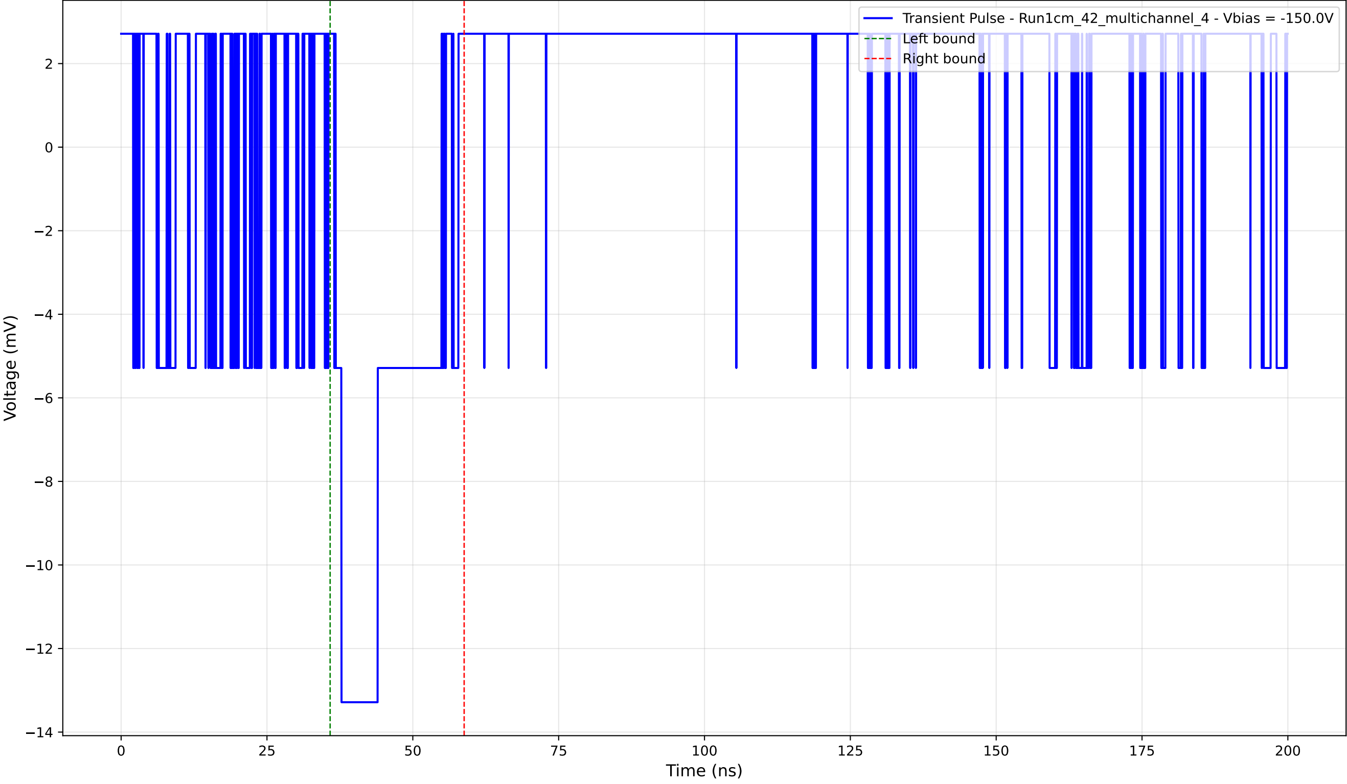
Transient Pulse - Sample: 1cm_42_multichannel - Position: 795.0 \mu\text{m} - Charge: 2.92 pC - Rise Time: 0.00 ns (N/A)
