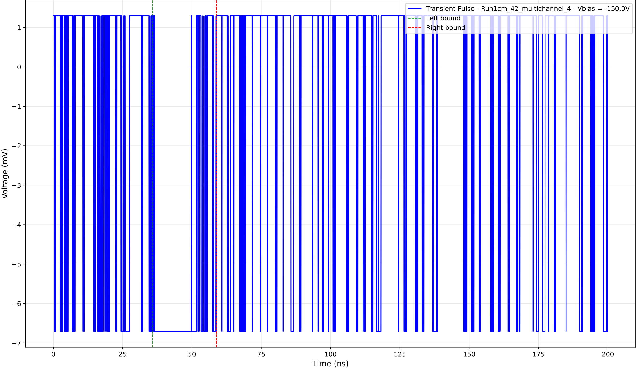
Transient Pulse - Sample: 1cm_42_multichannel - Position: 1415.0 \mu\text{m} - Charge: 2.38 pC - Rise Time: 0.00 ns (N/A)
