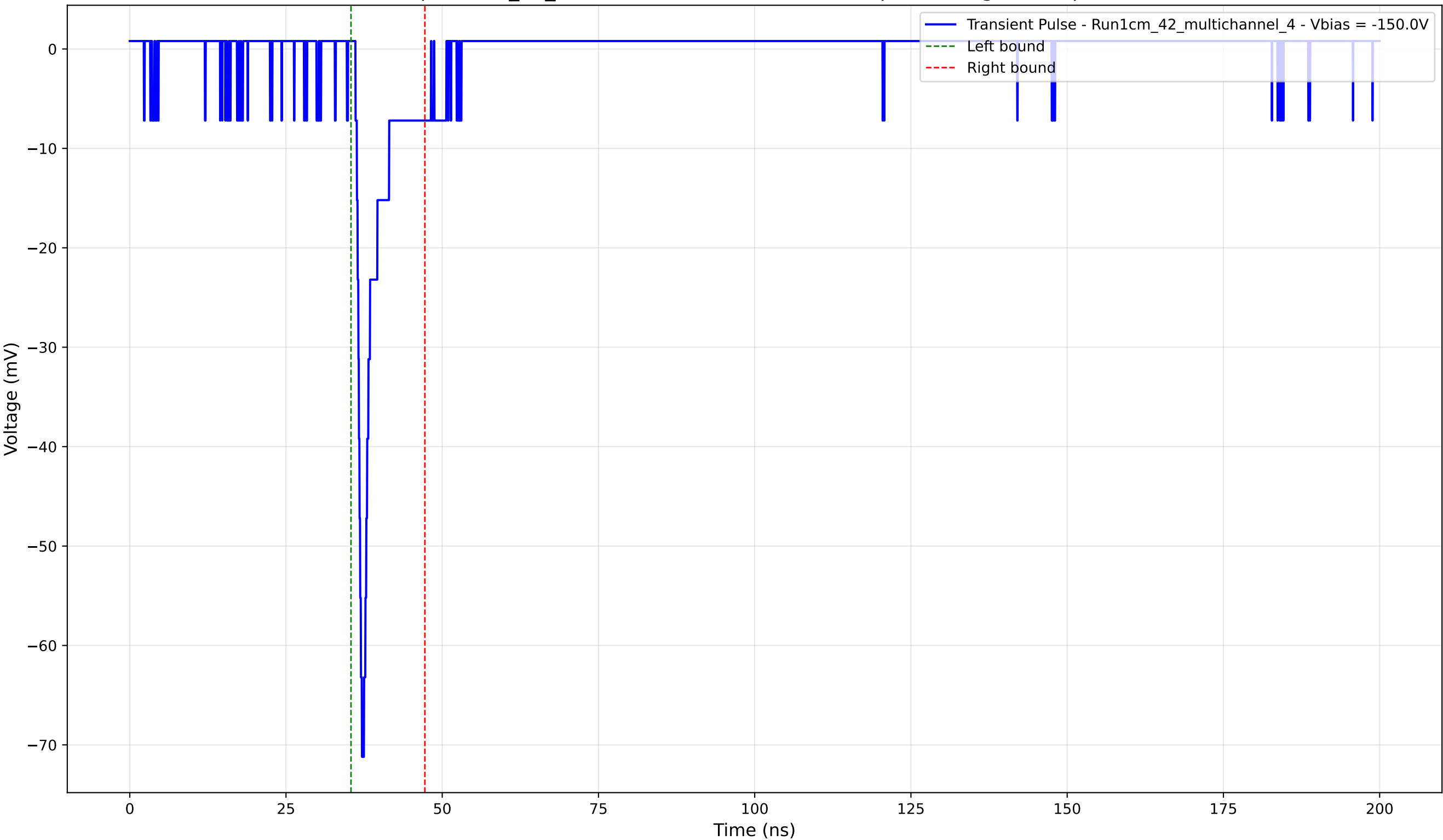
Transient Pulse - Sample: 1cm_42_multichannel - Position: 2570.0 \mu\text{m} - Charge: 3.98 pC - Rise Time: 1.02 ns
