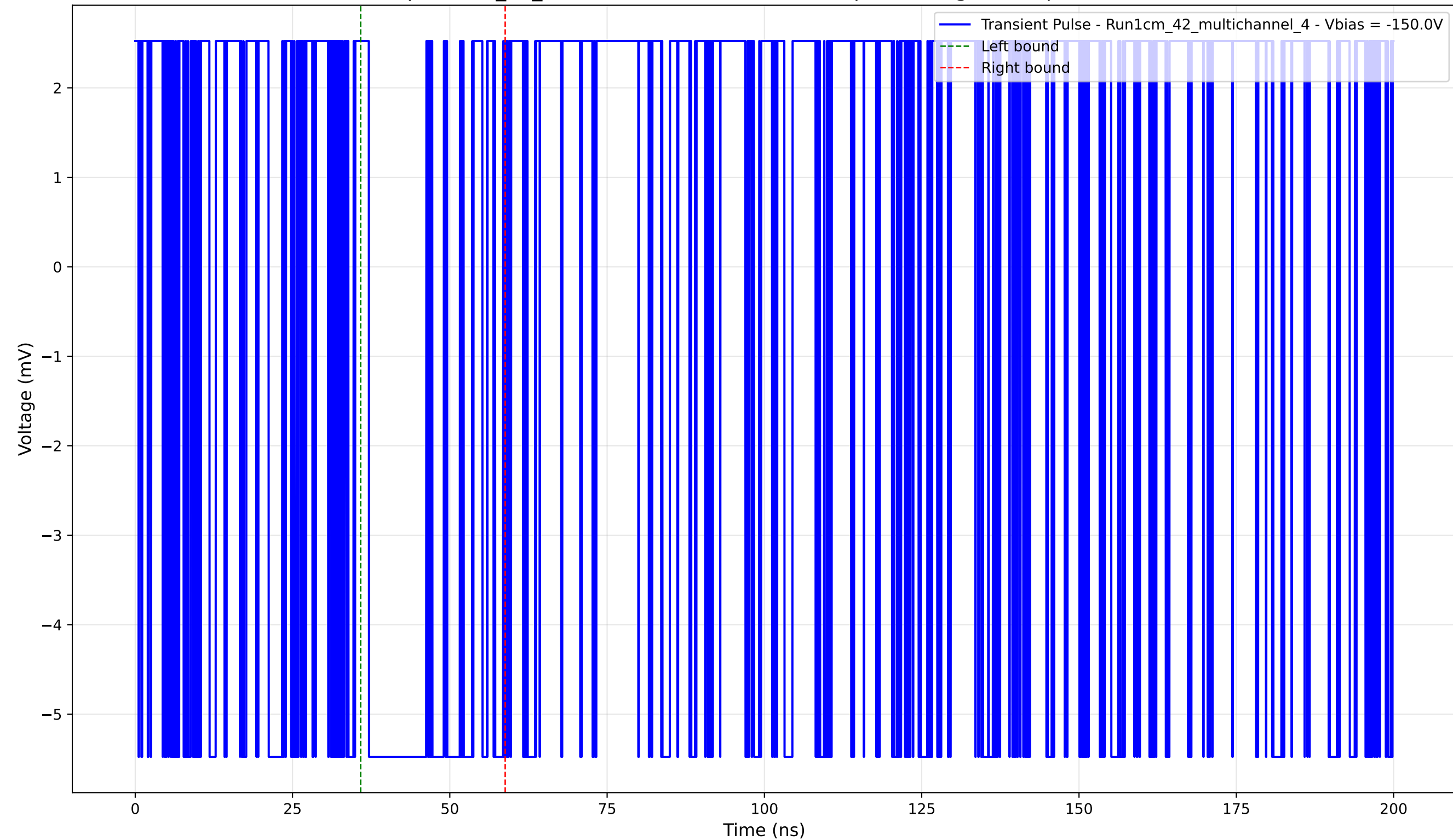
Transient Pulse - Sample: 1cm_42_multichannel - Position: 400.0 \mu\text{m} - Charge: 1.64 pC - Rise Time: 0.00 ns (N/A)
