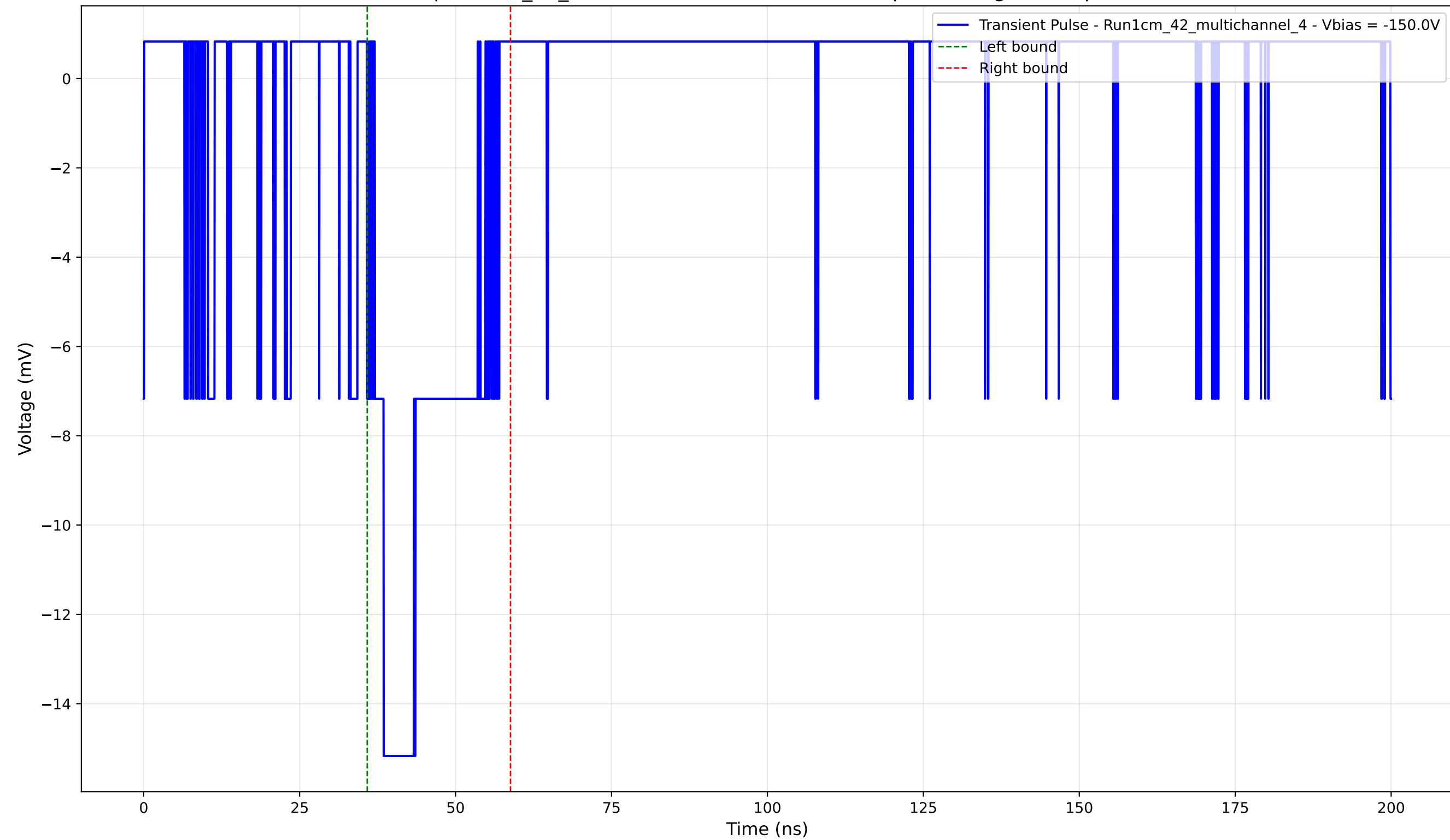
Transient Pulse - Sample: 1cm_42_multichannel - Position: 4500.0 \mu\text{m} - Charge: 3.46 pC - Rise Time: 1.42 ns
