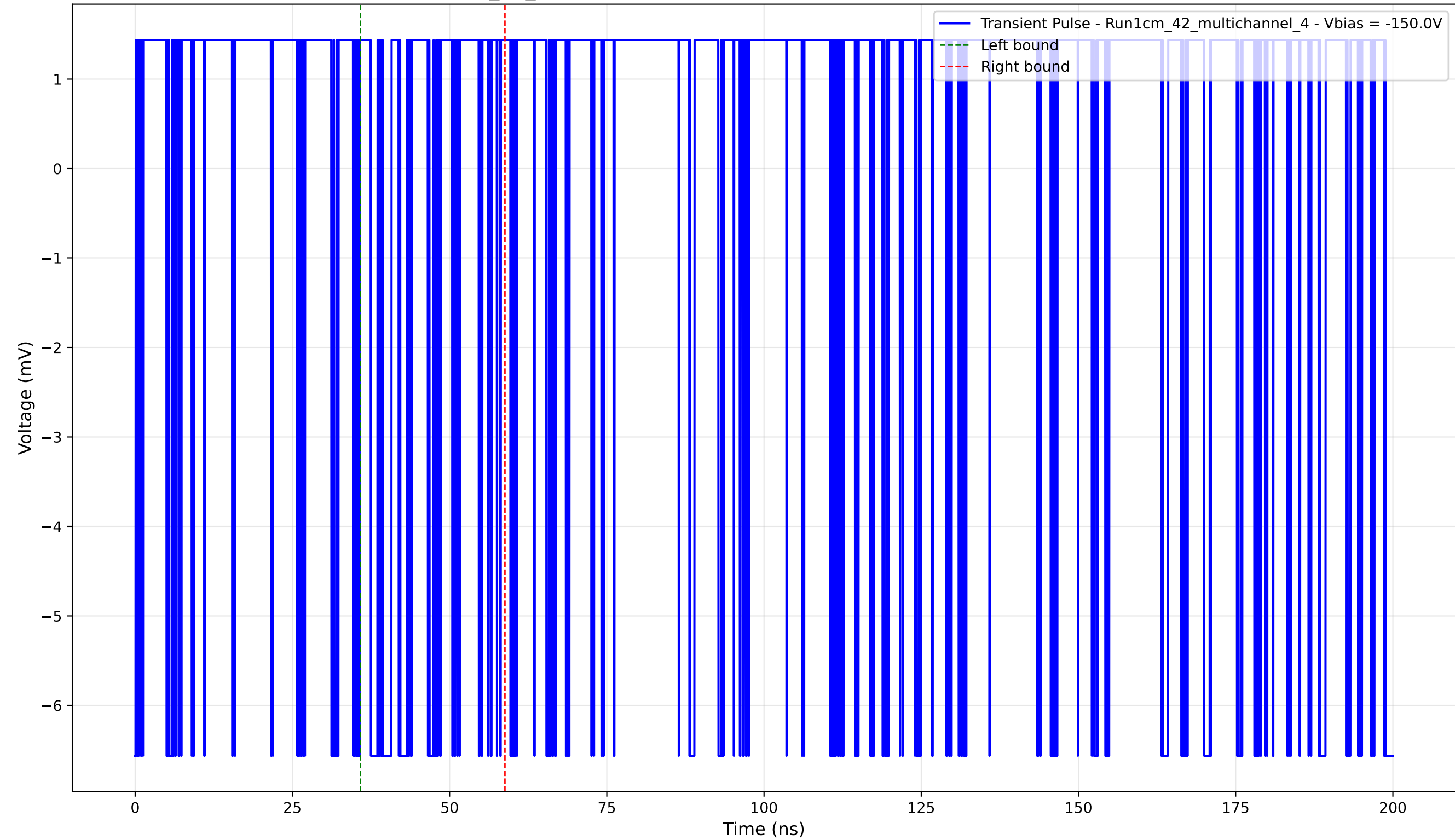
Transient Pulse - Sample: 1cm_42_multichannel - Position: 3385.0 \mu\text{m} - Charge: 0.46 pC - Rise Time: 0.00 ns (N/A)
