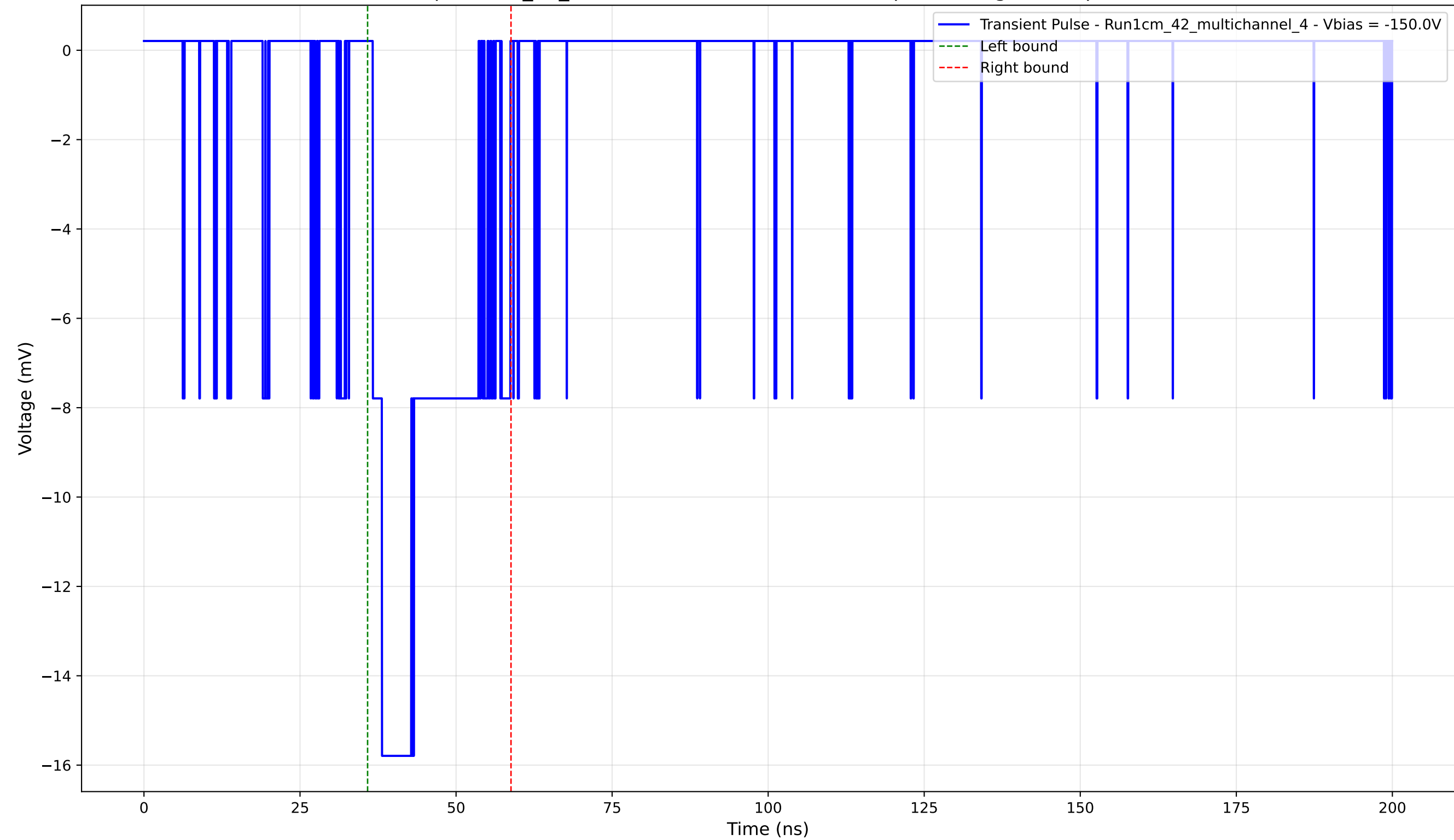
Transient Pulse - Sample: 1cm_42_multichannel - Position: 4125.0 \mu\text{m} - Charge: 3.92 pC - Rise Time: 1.48 ns
