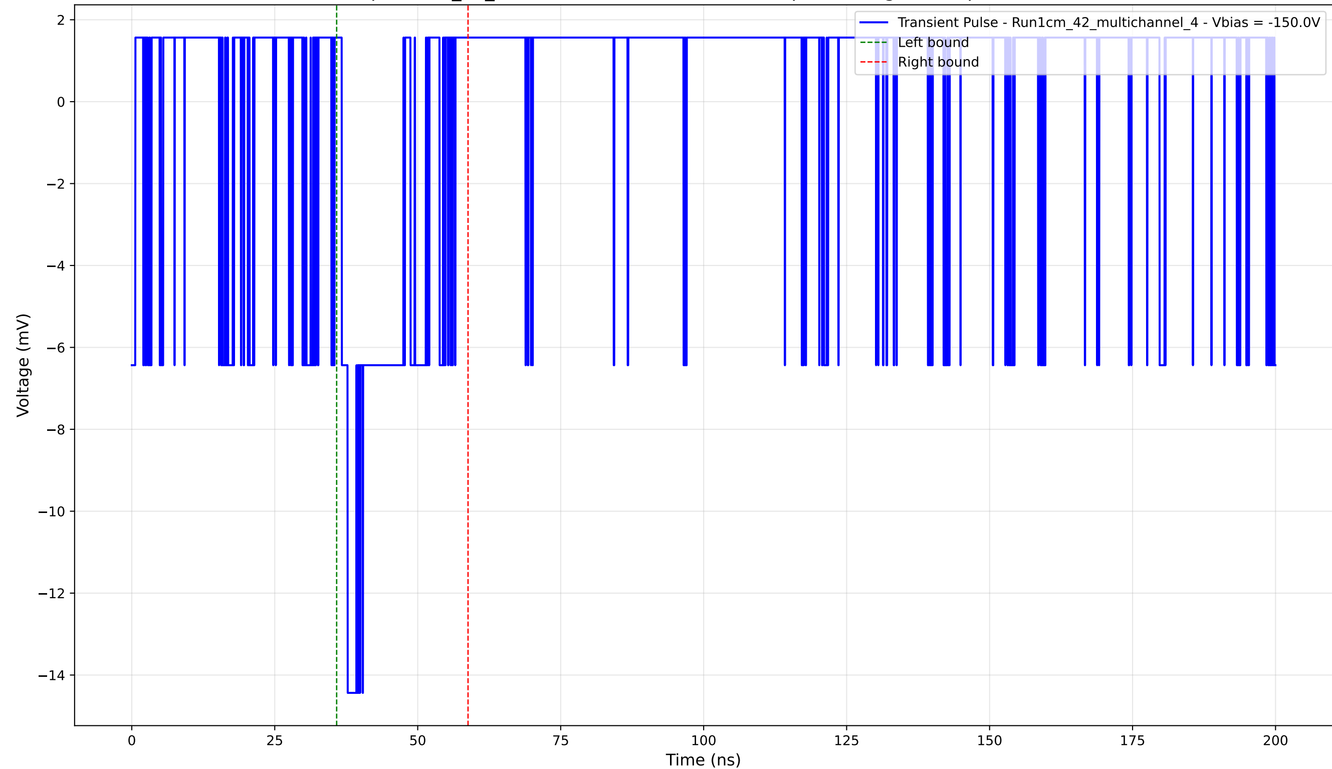
Transient Pulse - Sample: 1cm_42_multichannel - Position: 3450.0 \mu\text{m} - Charge: 2.01 pC - Rise Time: 0.00 ns (N/A)
