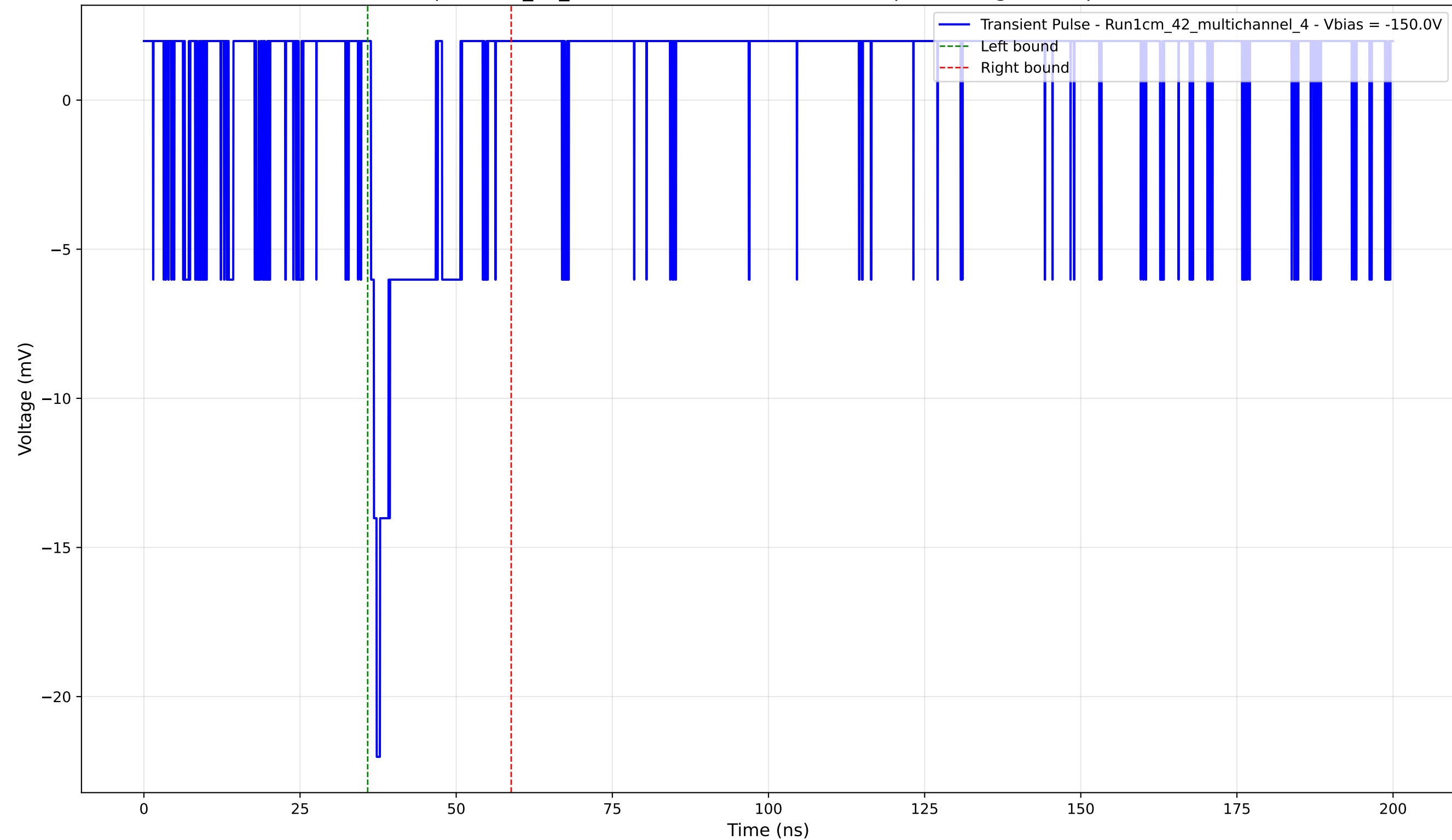
Transient Pulse - Sample: 1cm_42_multichannel - Position: 2845.0 \mu\text{m} - Charge: 1.85 pC - Rise Time: 0.92 ns
