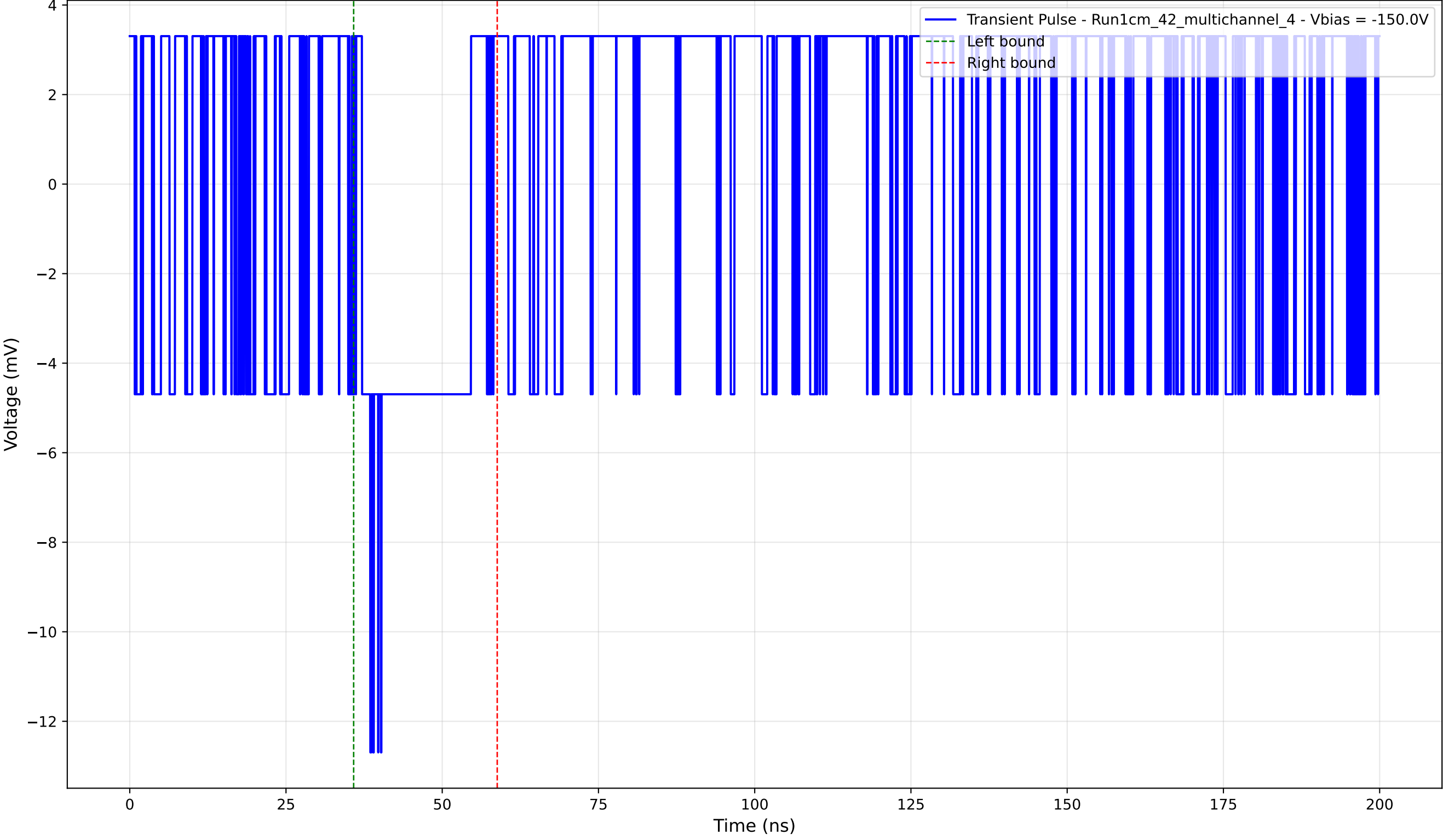
Transient Pulse - Sample: 1cm_42_multichannel - Position: 815.0 \mu\text{m} - Charge: 1.43 pC - Rise Time: 0.00 ns (N/A)
