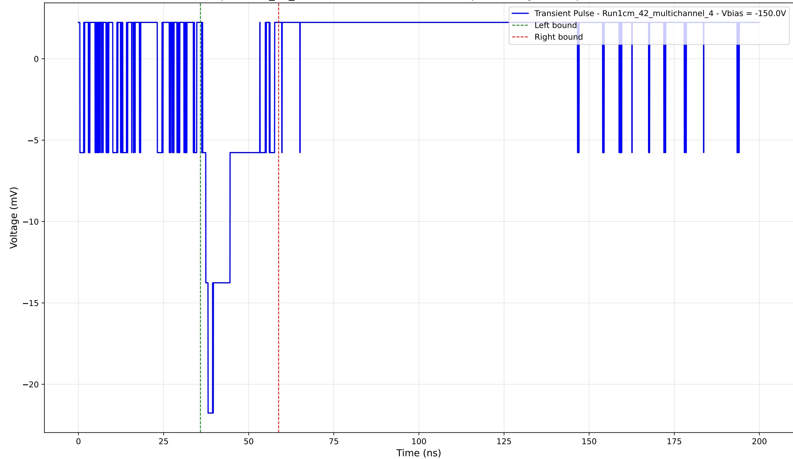
Transient Pulse - Sample: 1cm_42_multichannel - Position: 1125.0 \mu\text{m} - Charge: 3.57 pC - Rise Time: 0.00 ns (N/A)
