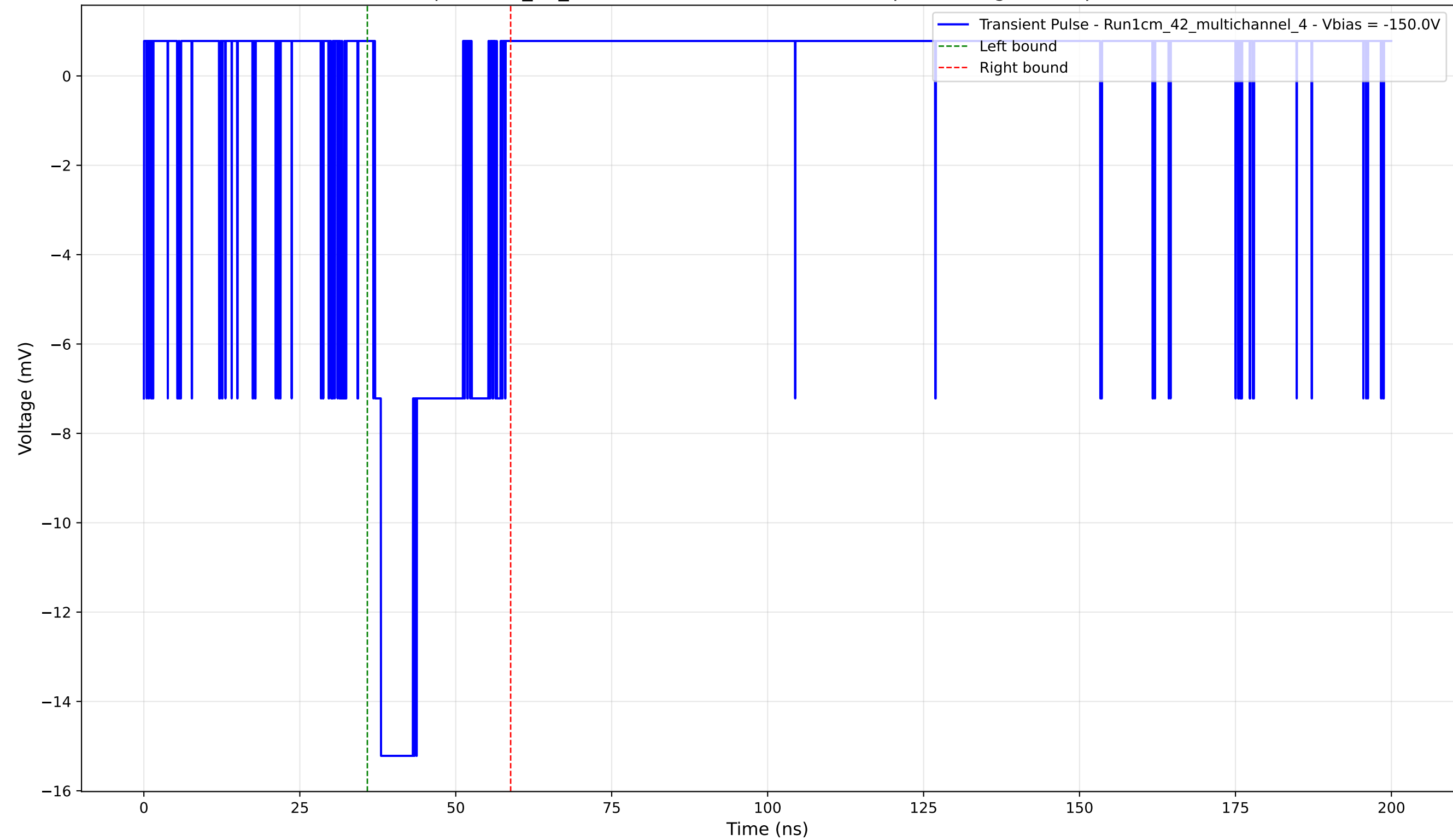
Transient Pulse - Sample: 1cm_42_multichannel - Position: 4010.0 \mu\text{m} - Charge: 3.46 pC - Rise Time: 0.96 ns
