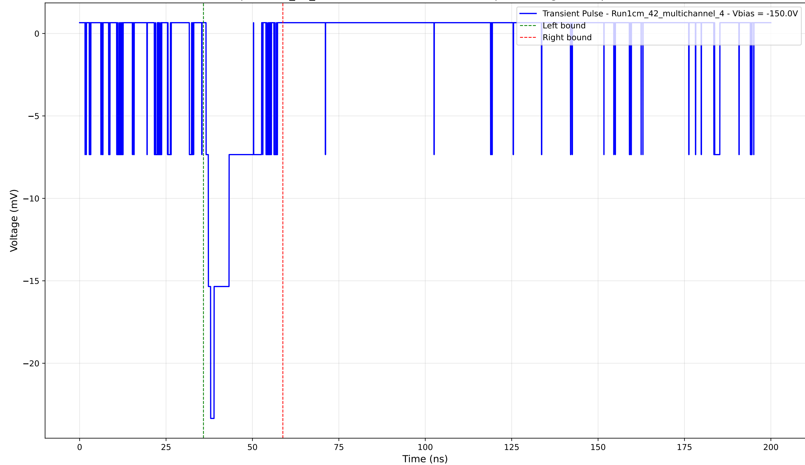
Transient Pulse - Sample: 1cm_42_multichannel - Position: 3550.0 \mu\text{m} - Charge: 3.71 pC - Rise Time: 1.33 ns
