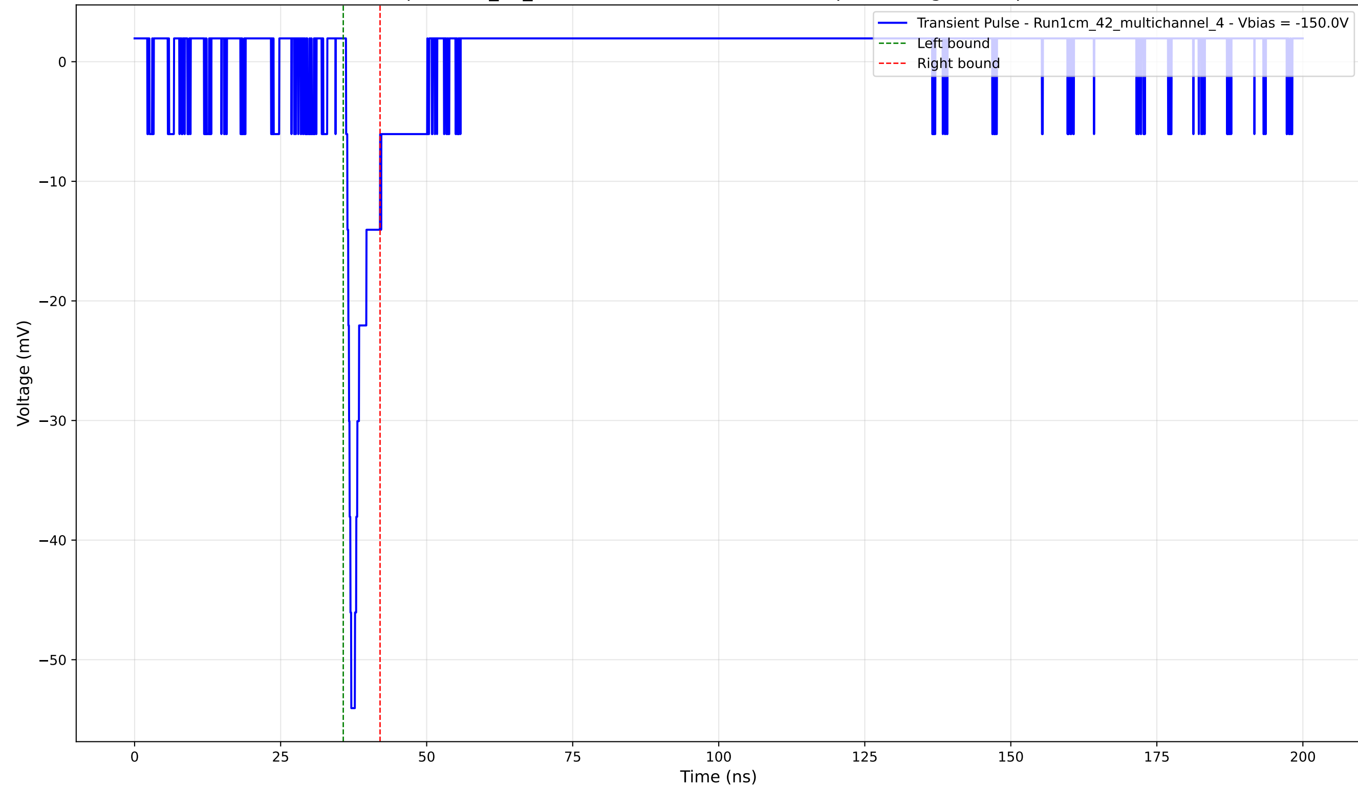
Transient Pulse - Sample: 1cm_42_multichannel - Position: 2665.0 \mu\text{m} - Charge: 2.83 pC - Rise Time: 0.88 ns
