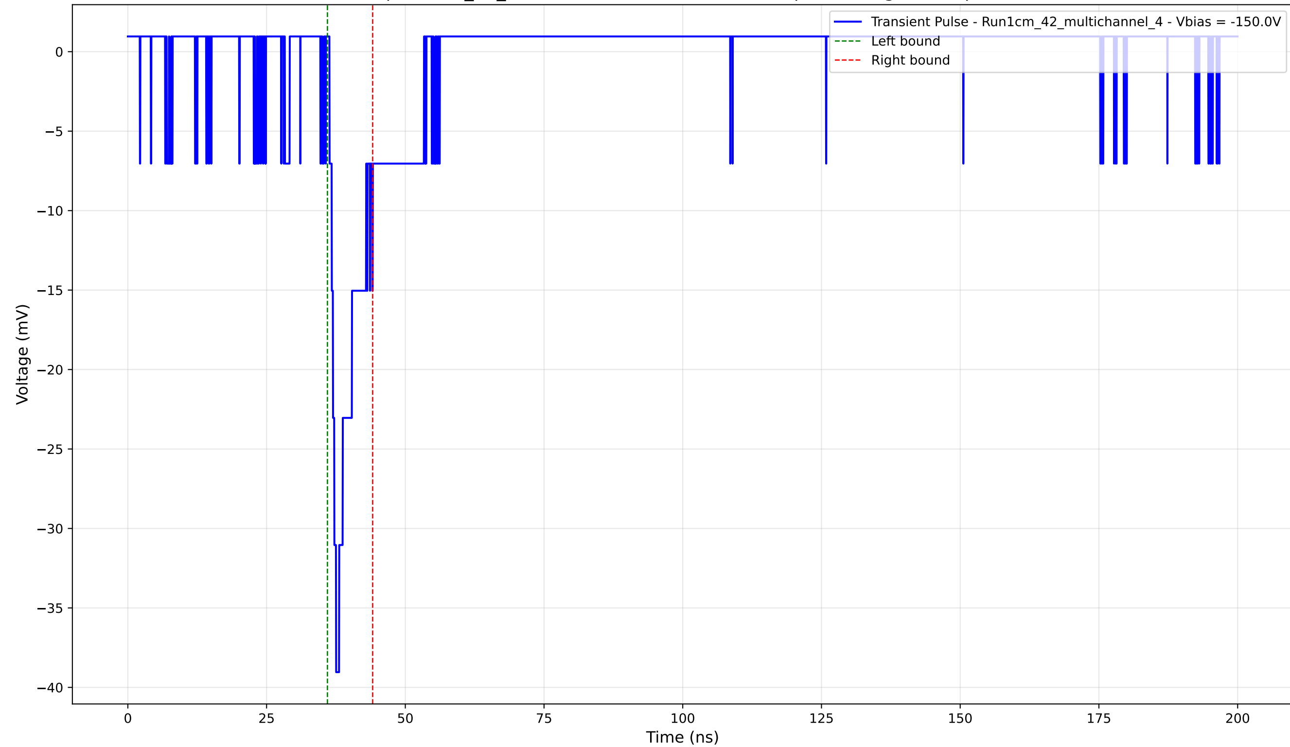
Transient Pulse - Sample: 1cm_42_multichannel - Position: 1660.0 \mu\text{m} - Charge: 3.00 pC - Rise Time: 1.19 ns
