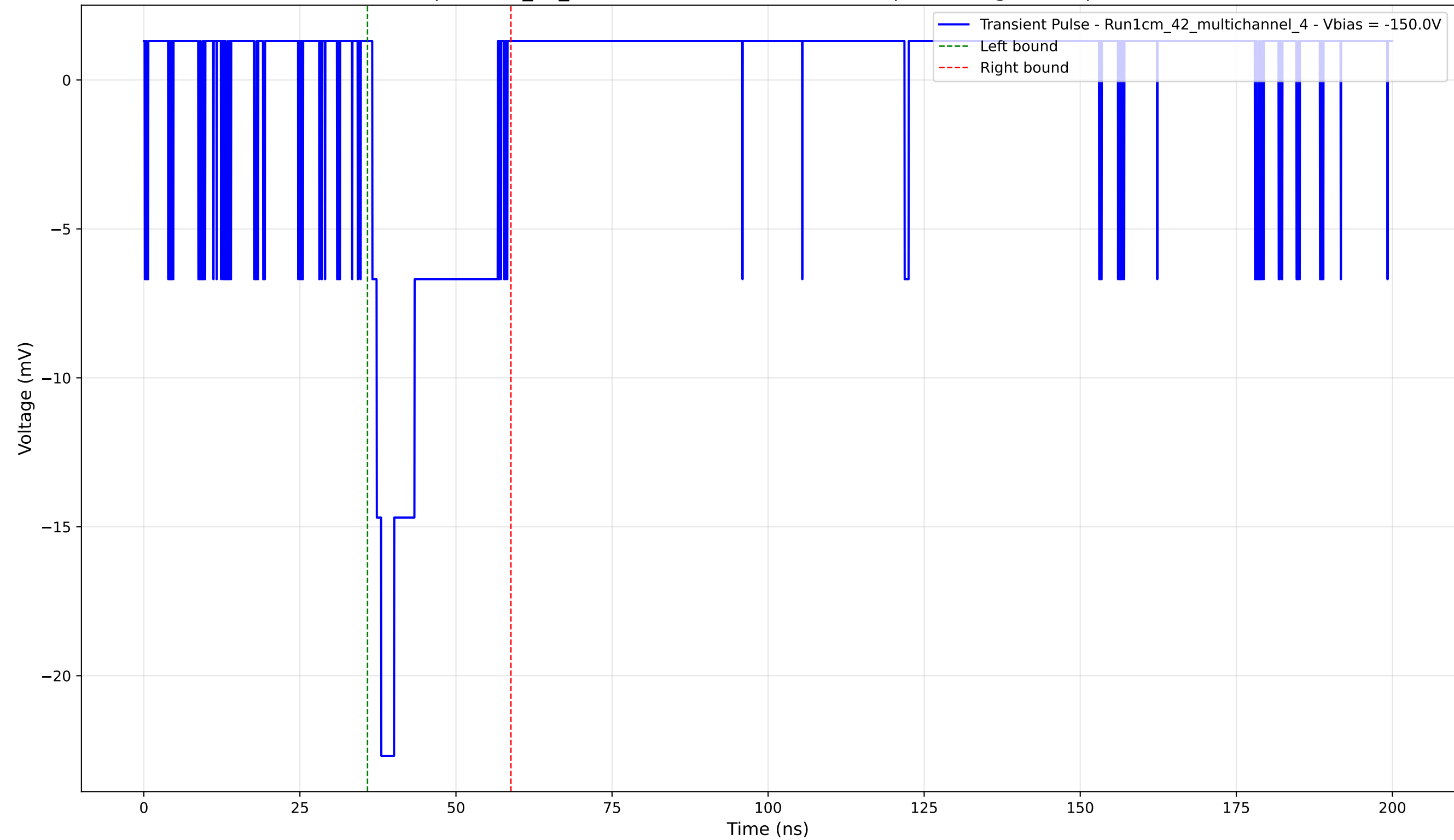
Transient Pulse - Sample: 1cm_42_multichannel - Position: 1150.0 \mu\text{m} - Charge: 3.99 pC - Rise Time: 1.44 ns
