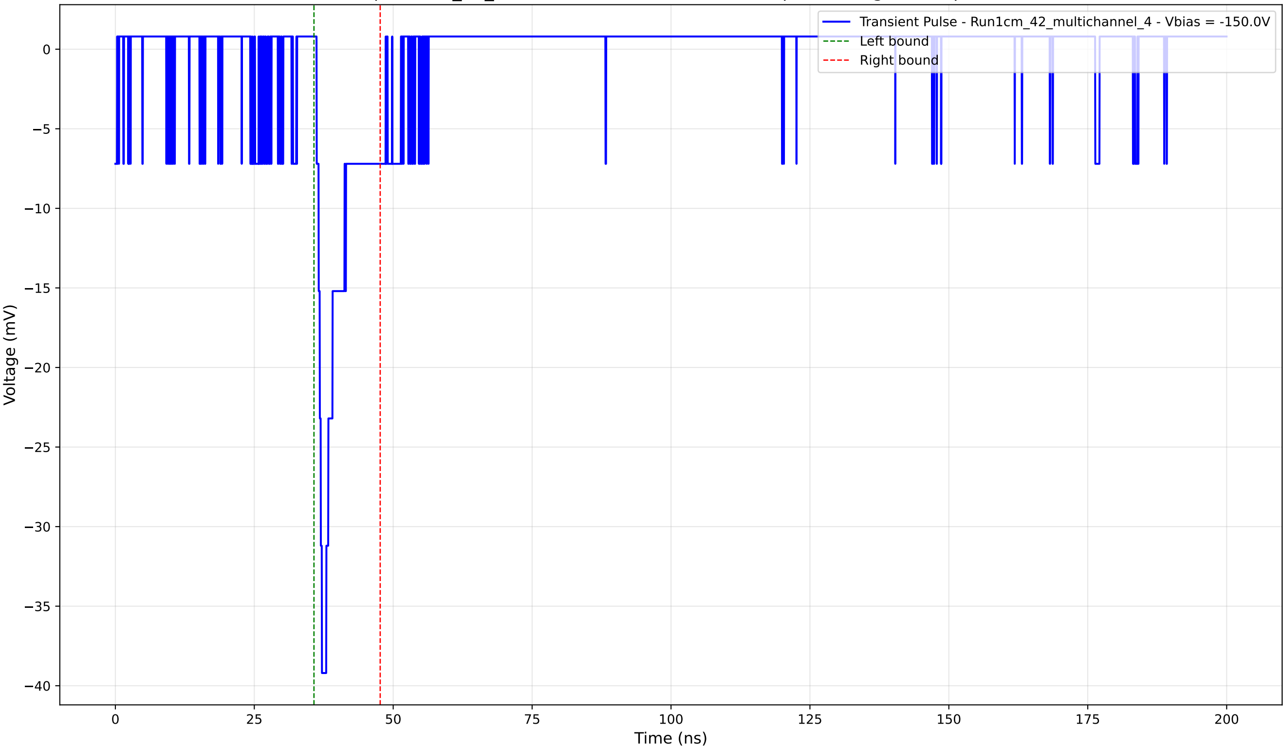
Transient Pulse - Sample: 1cm_42_multichannel - Position: 2825.0 \mu\text{m} - Charge: 3.12 pC - Rise Time: 0.95 ns
