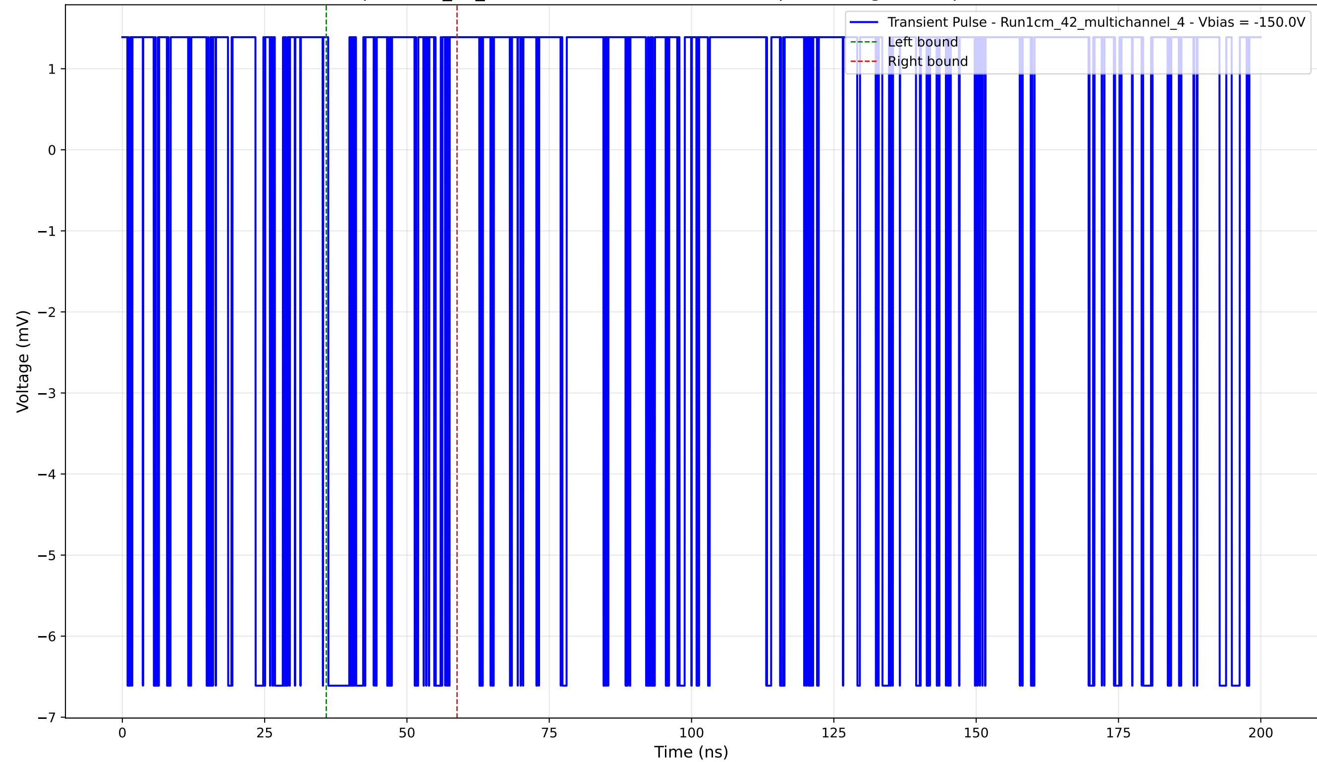
Transient Pulse - Sample: 1cm_42_multichannel - Position: 2370.0 \mu\text{m} - Charge: 0.76 pC - Rise Time: 0.00 ns (N/A)
