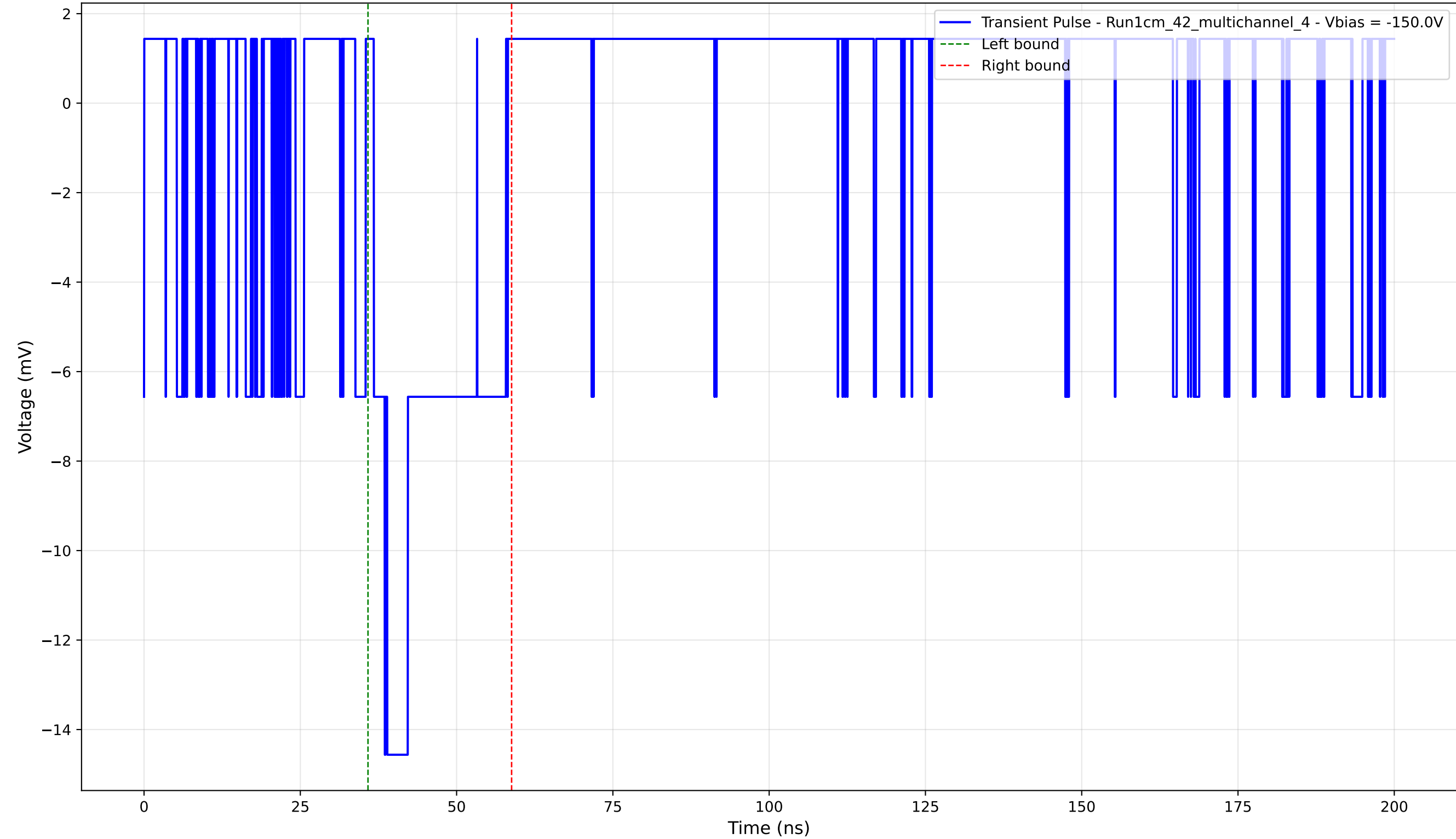
Transient Pulse - Sample: 1cm_42_multichannel - Position: 430.0 \mu\text{m} - Charge: 3.28 pC - Rise Time: 1.76 ns
