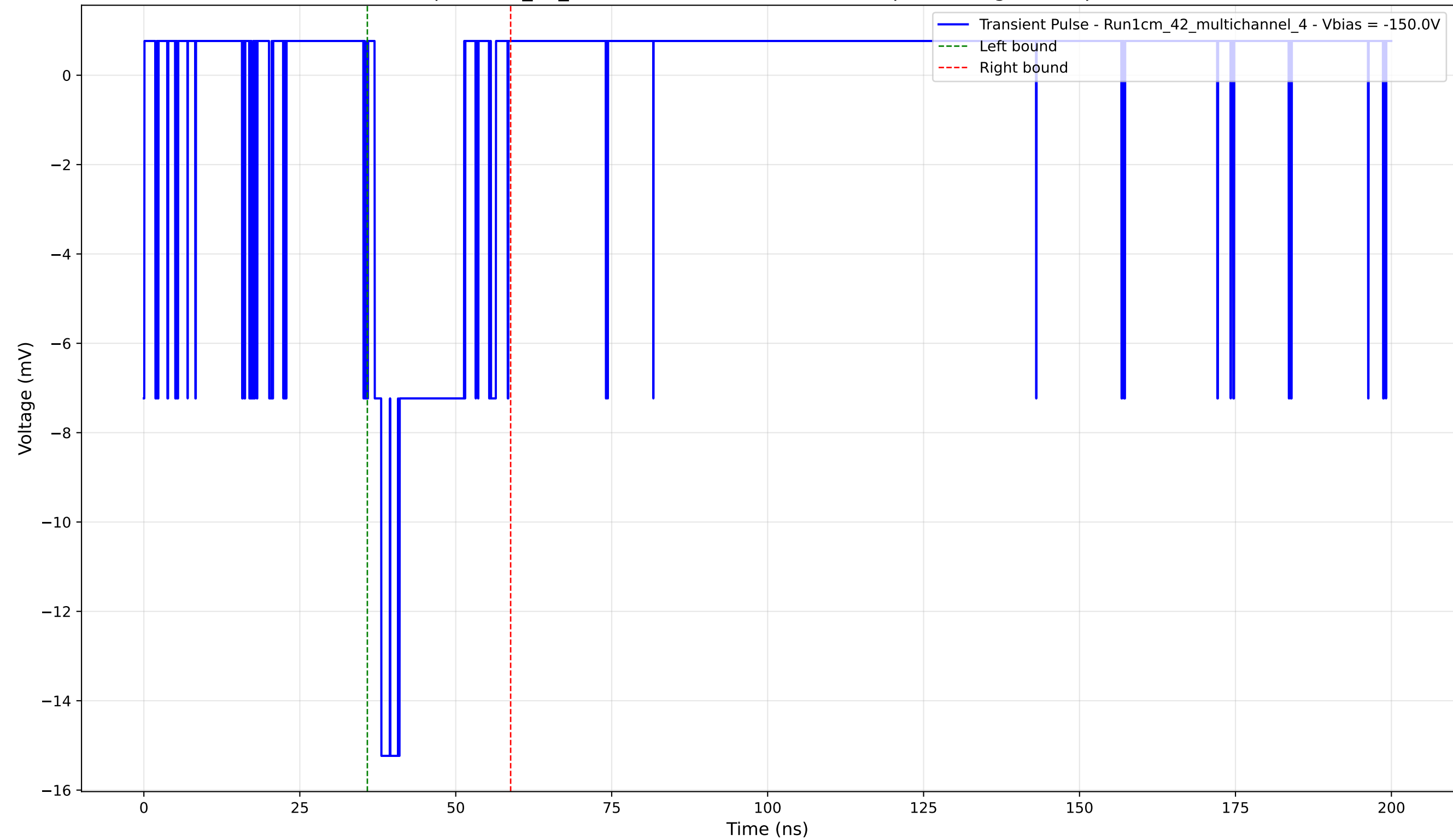
Transient Pulse - Sample: 1cm_42_multichannel - Position: 3845.0 \mu\text{m} - Charge: 2.61 pC - Rise Time: 1.08 ns
