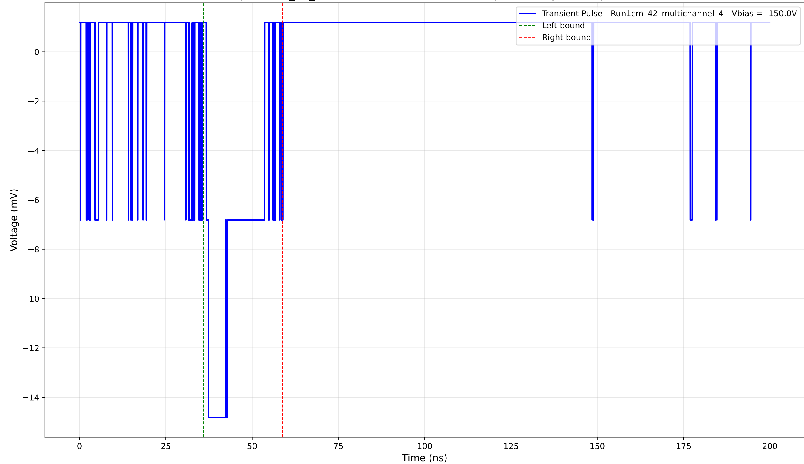
Transient Pulse - Sample: 1cm_42_multichannel - Position: 3605.0 \mu\text{m} - Charge: 3.15 pC - Rise Time: 0.72 ns
