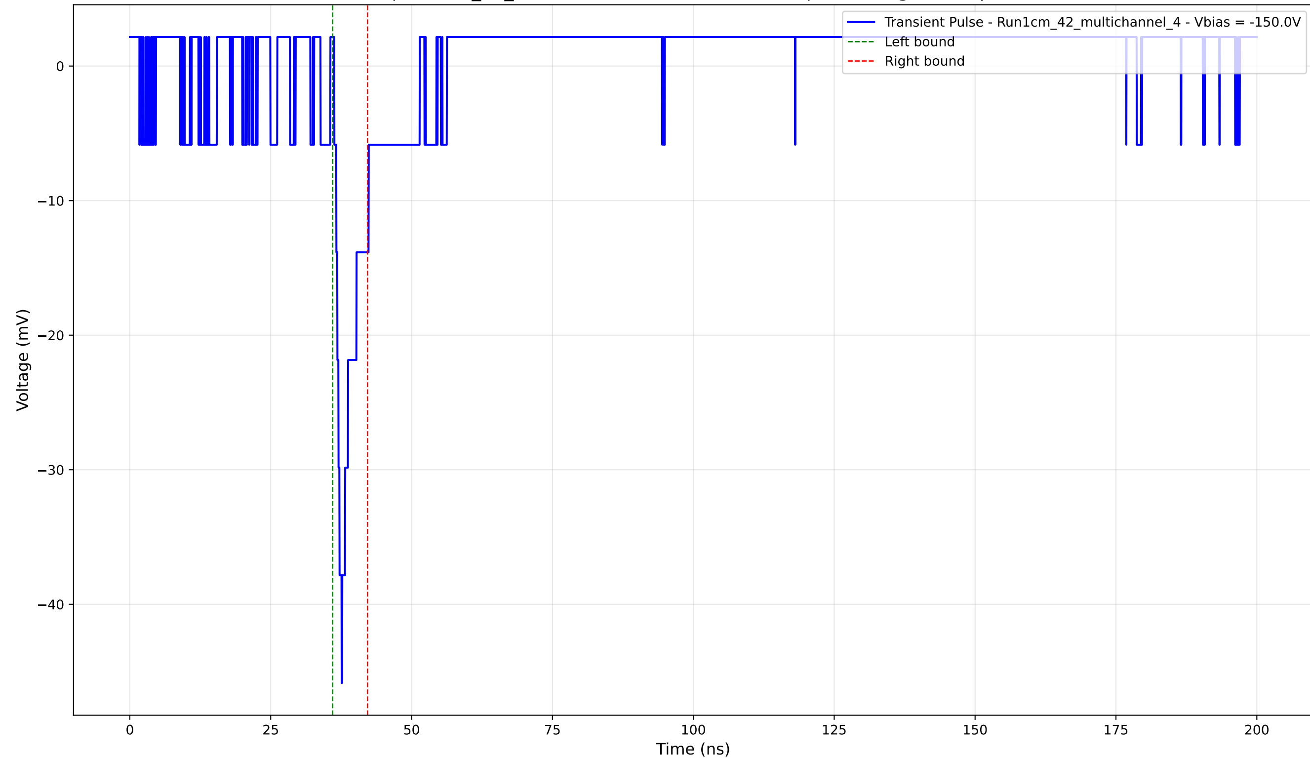
Transient Pulse - Sample: 1cm_42_multichannel - Position: 1795.0 \mu\text{m} - Charge: 2.56 pC - Rise Time: 1.31 ns
