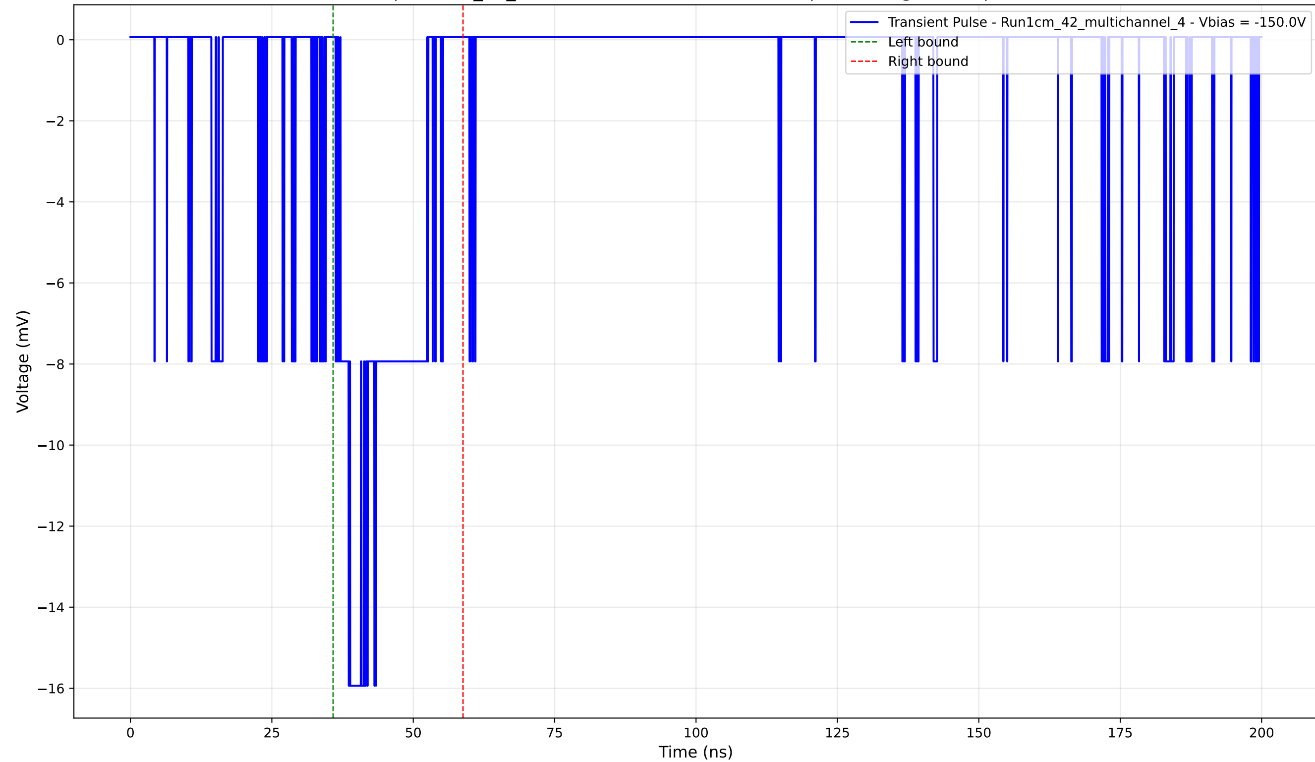
Transient Pulse - Sample: 1cm_42_multichannel - Position: 4800.0 \mu\text{m} - Charge: 3.07 pC - Rise Time: 1.44 ns
