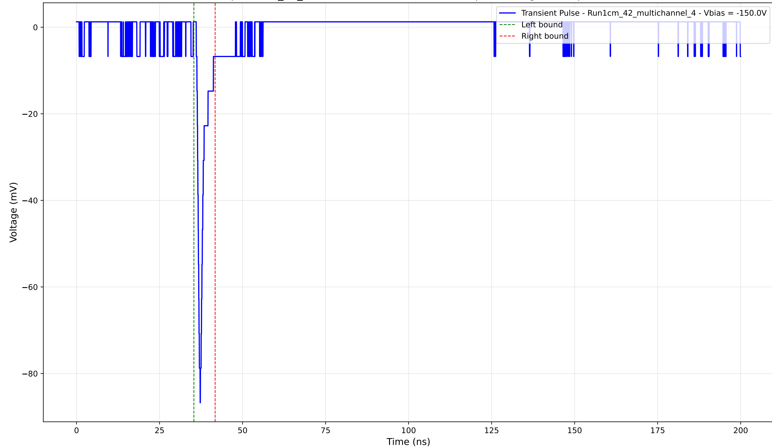
Transient Pulse - Sample: 1cm_42_multichannel - Position: 2475.0 \mu\text{m} - Charge: 3.42 pC - Rise Time: 0.74 ns
