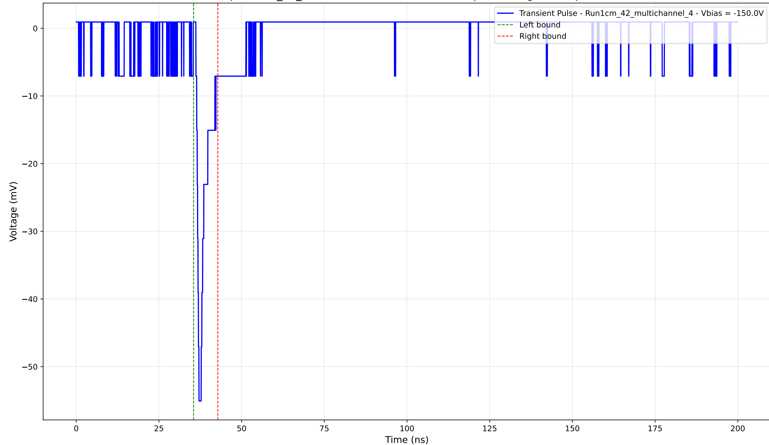
Transient Pulse - Sample: 1cm_42_multichannel - Position: 2695.0 \mu\text{m} - Charge: 3.12 pC - Rise Time: 0.93 ns
