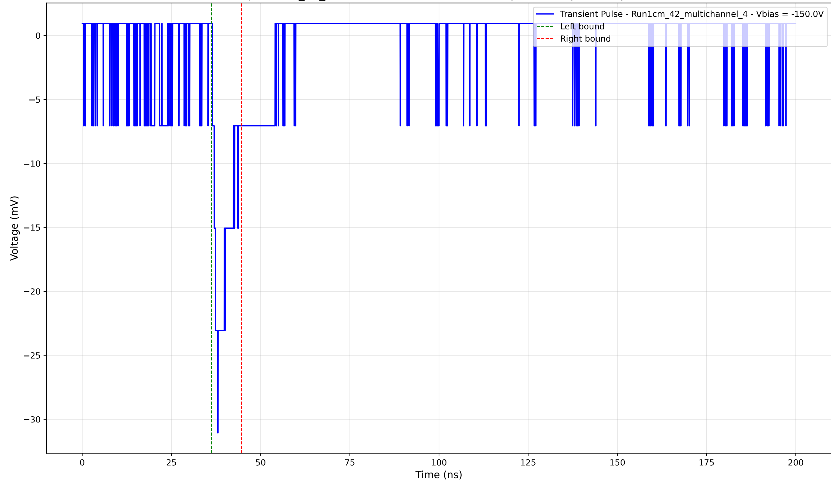
Transient Pulse - Sample: 1cm_42_multichannel - Position: 3280.0 \mu\text{m} - Charge: 2.52 pC - Rise Time: 1.43 ns
