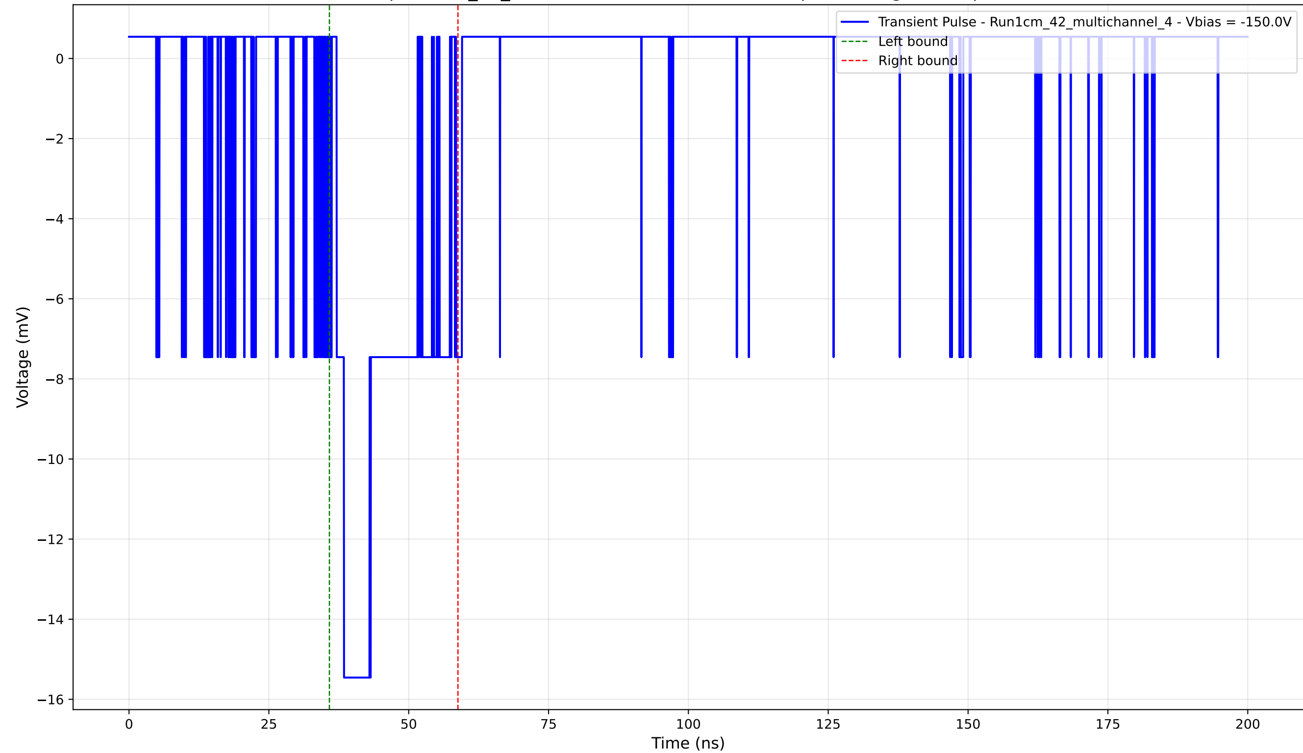
Transient Pulse - Sample: 1cm_42_multichannel - Position: 4325.0 \mu\text{m} - Charge: 3.69 pC - Rise Time: 1.32 ns
