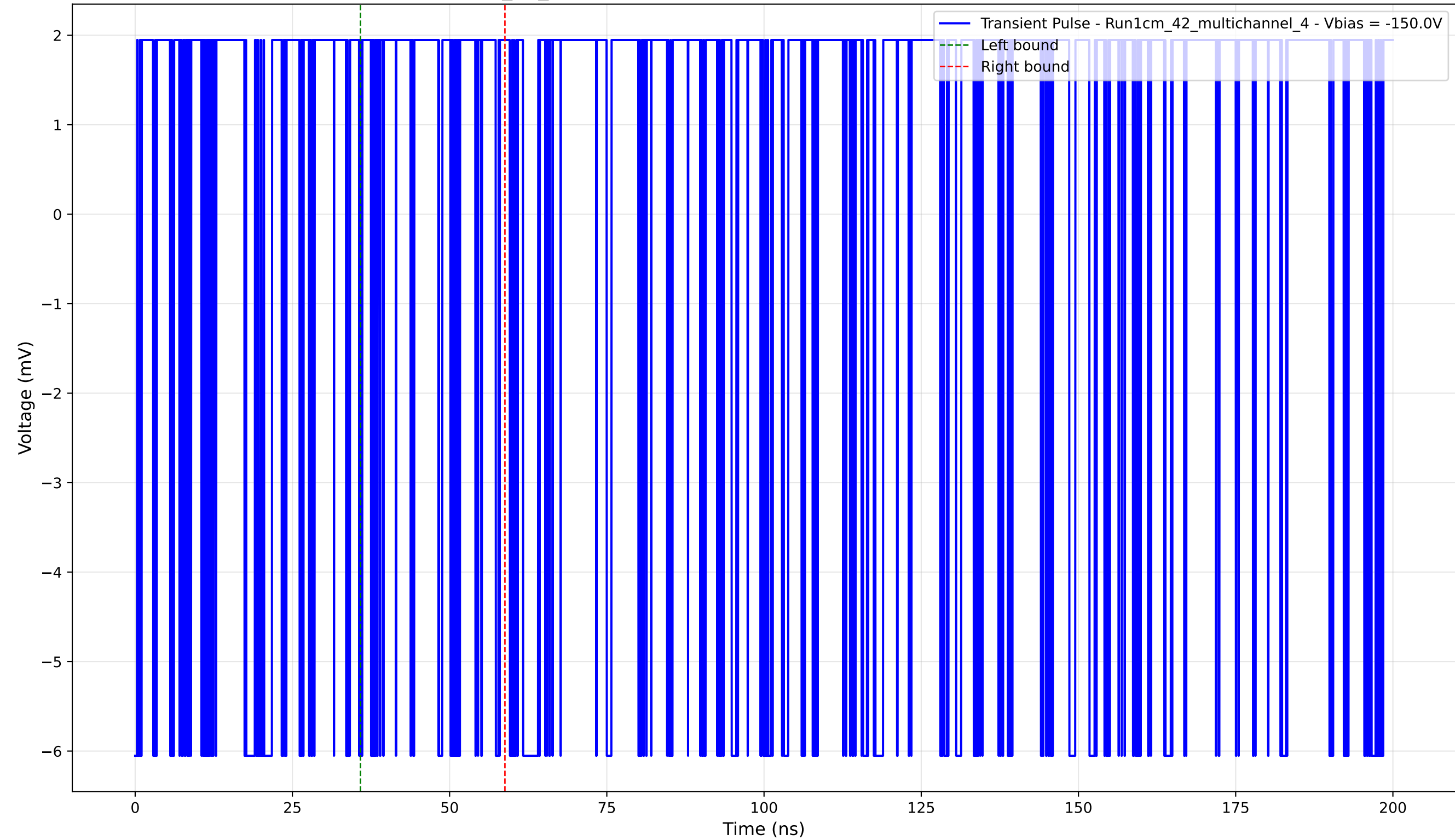
Transient Pulse - Sample: 1cm_42_multichannel - Position: 40.0 \mu\text{m} - Charge: 0.35 pC - Rise Time: 0.00 ns (N/A)
