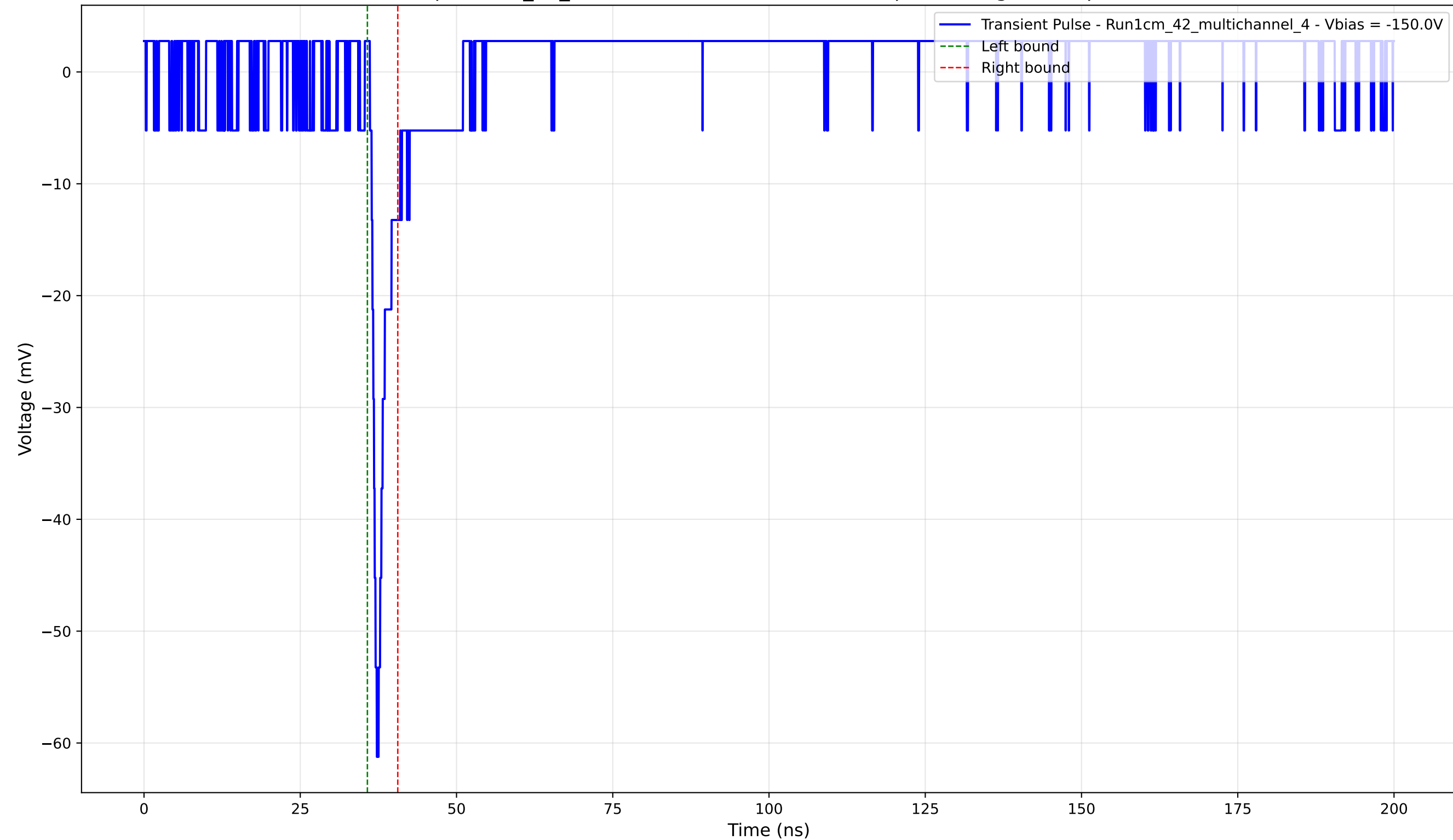
Transient Pulse - Sample: 1cm_42_multichannel - Position: 2655.0 \mu\text{m} - Charge: 2.46 pC - Rise Time: 0.84 ns
