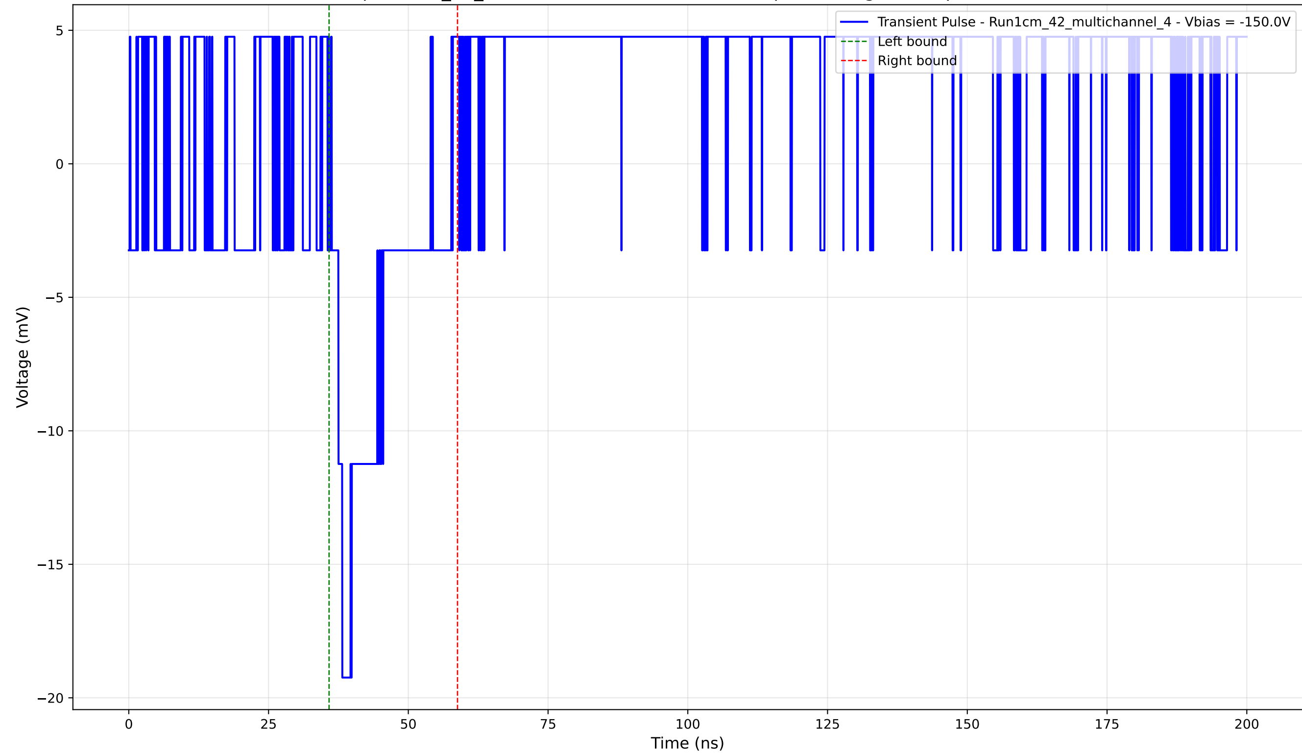
Transient Pulse - Sample: 1cm_42_multichannel - Position: 1010.0 \mu\text{m} - Charge: 2.74 pC - Rise Time: 0.00 ns (N/A)
