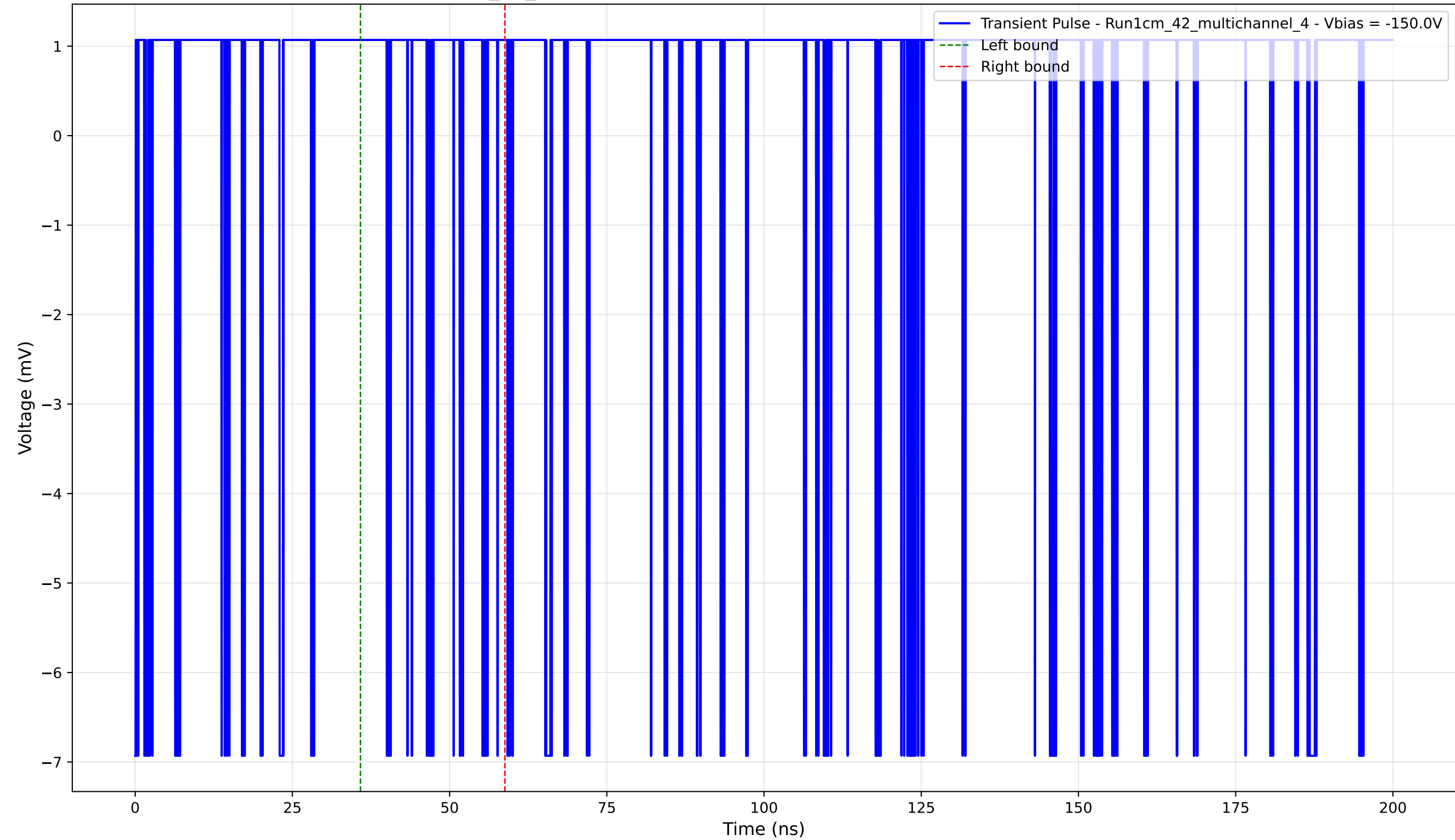
Transient Pulse - Sample: 1cm_42_multichannel - Position: 3905.0 \mu\text{m} - Charge: 0.16 pC - Rise Time: 0.00 ns (N/A)
