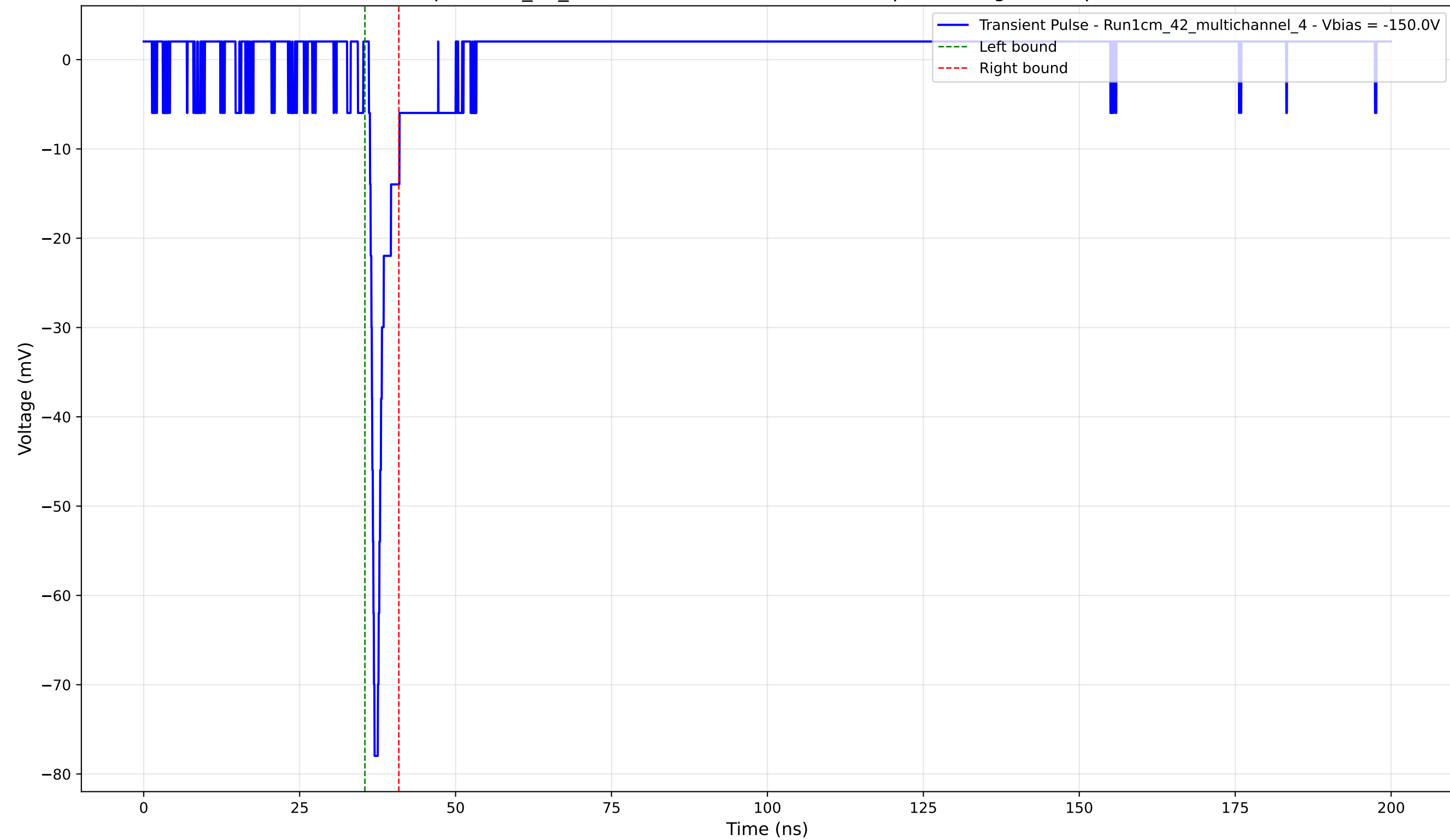
Transient Pulse - Sample: 1cm_42_multichannel - Position: 2490.0 \mu\text{m} - Charge: 3.16 pC - Rise Time: 0.74 ns
