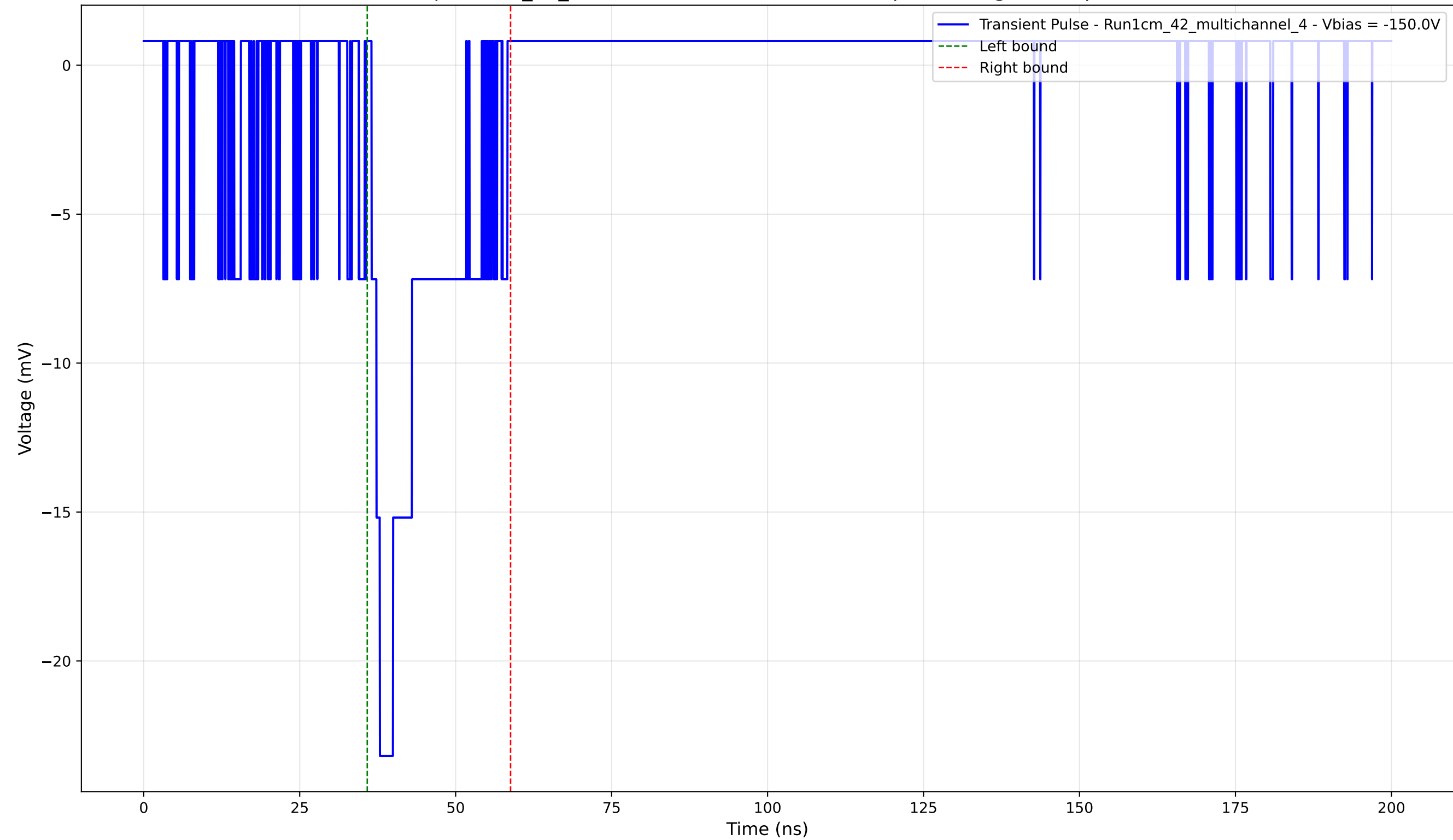
Transient Pulse - Sample: 1cm_42_multichannel - Position: 3565.0 \mu\text{m} - Charge: 3.96 pC - Rise Time: 1.34 ns
