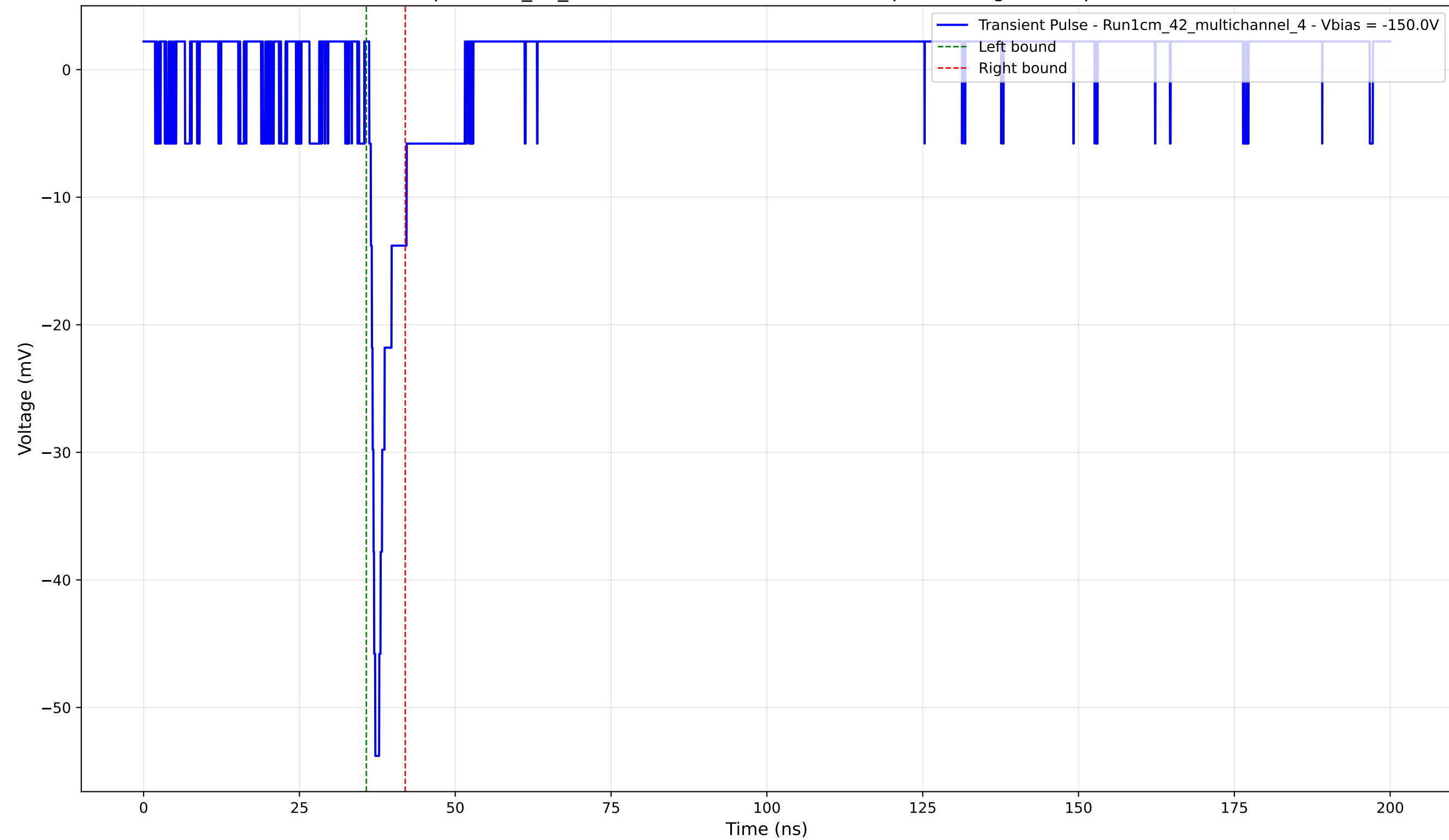
Transient Pulse - Sample: 1cm_42_multichannel - Position: 2035.0 \mu\text{m} - Charge: 2.84 pC - Rise Time: 0.96 ns
