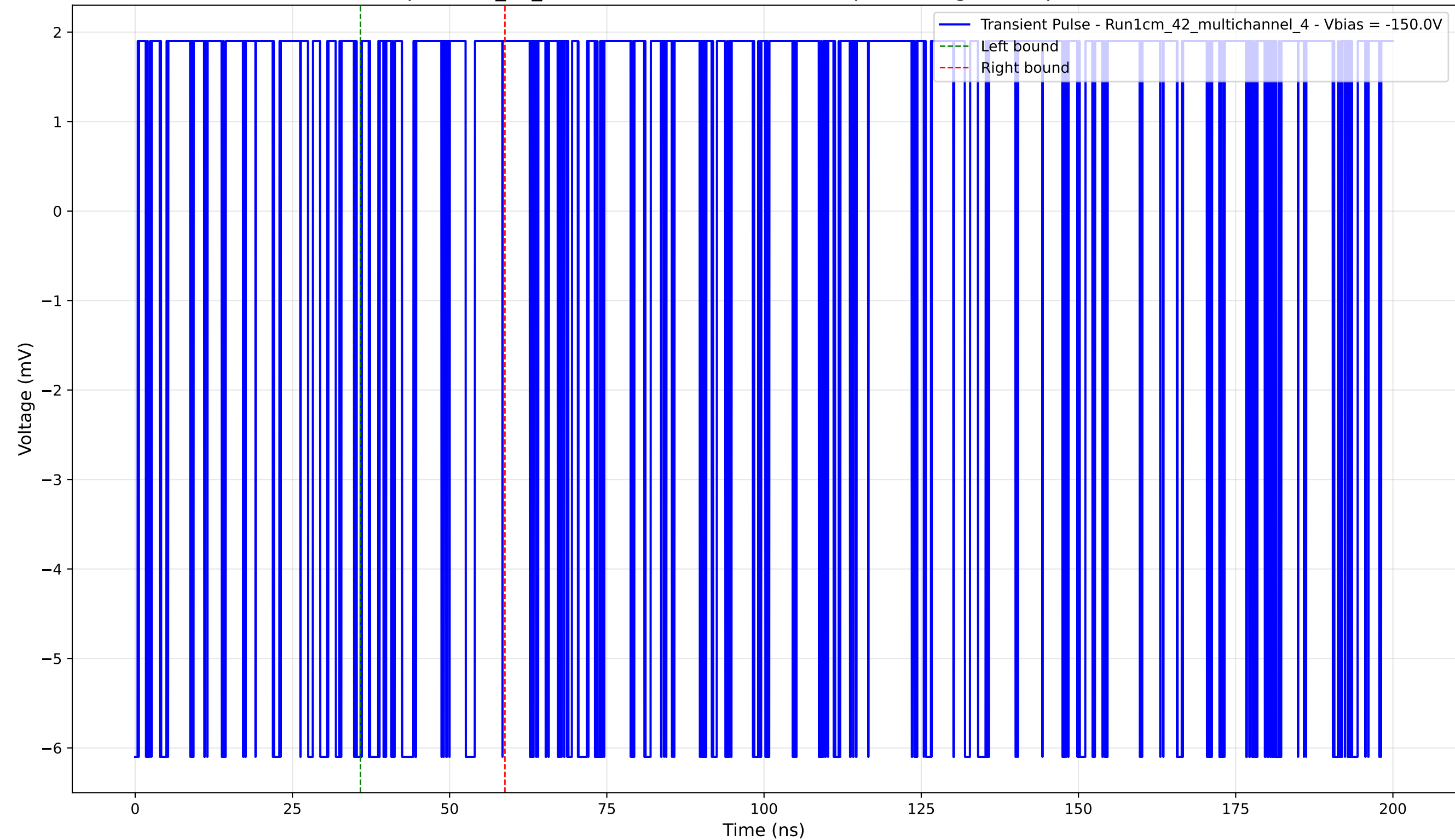
Transient Pulse - Sample: 1cm_42_multichannel - Position: 880.0 \mu\text{m} - Charge: 0.11 pC - Rise Time: 0.00 ns (N/A)
