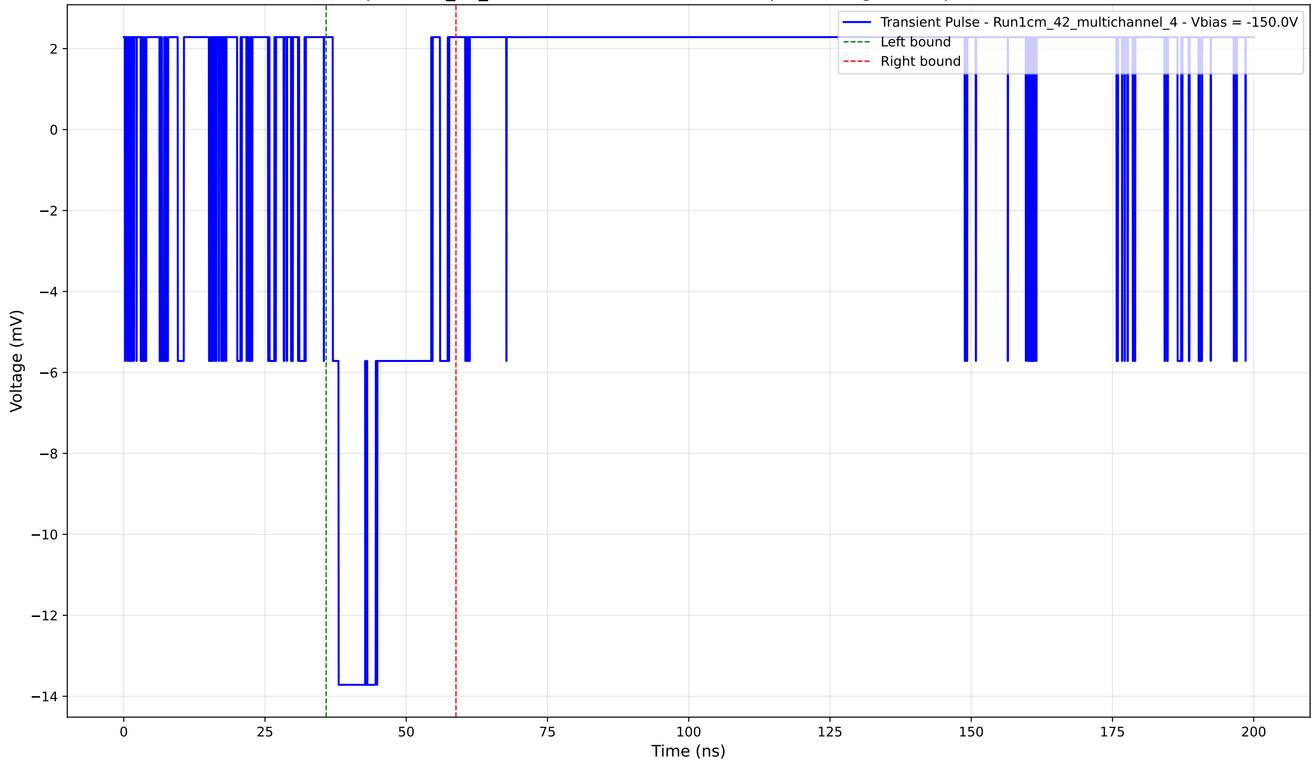
Transient Pulse - Sample: 1cm_42_multichannel - Position: 490.0 \mu\text{m} - Charge: 3.07 pC - Rise Time: 0.00 ns (N/A)
