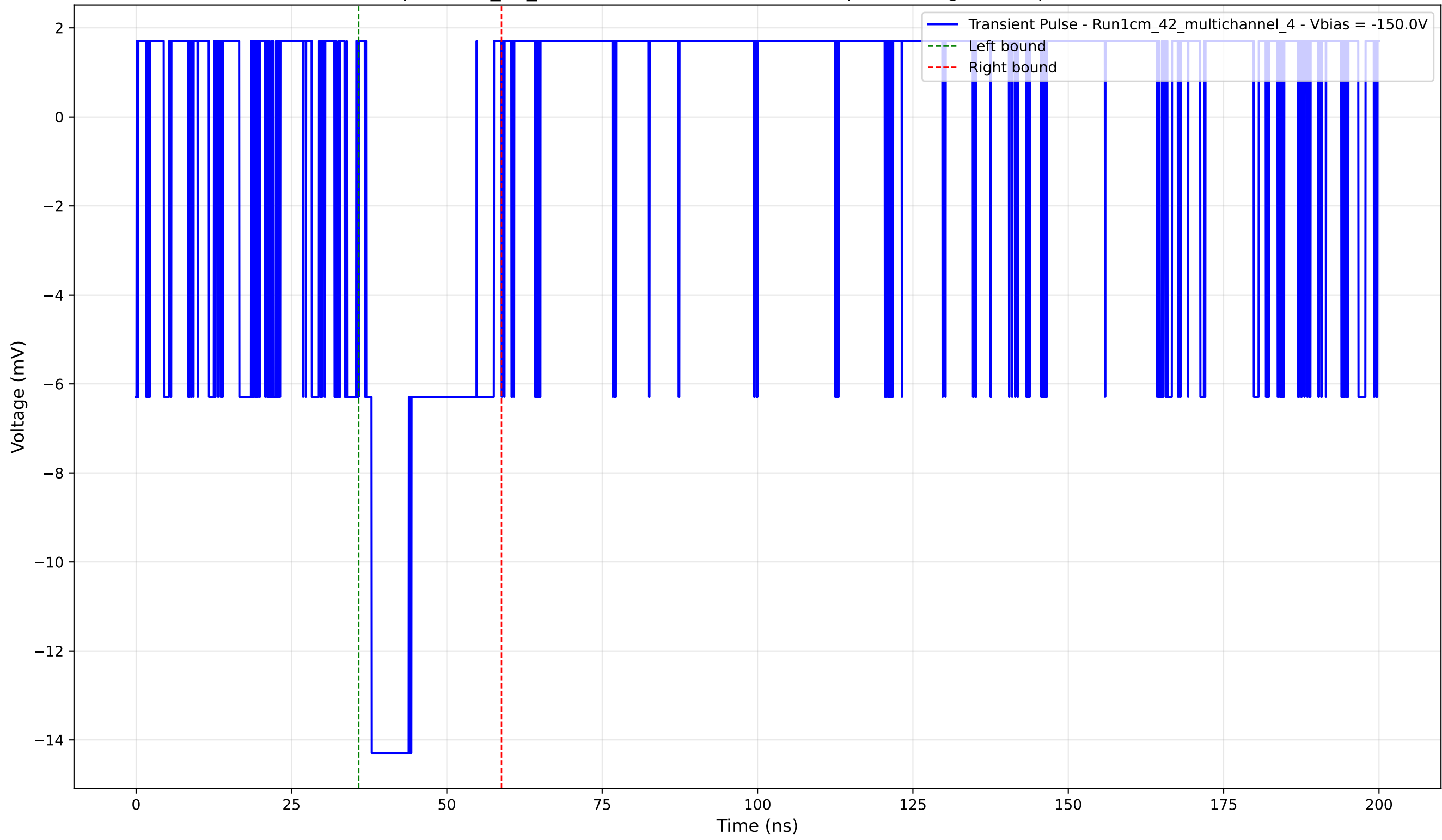
Transient Pulse - Sample: 1cm_42_multichannel - Position: 665.0 \mu\text{m} - Charge: 3.50 pC - Rise Time: 0.00 ns (N/A)
