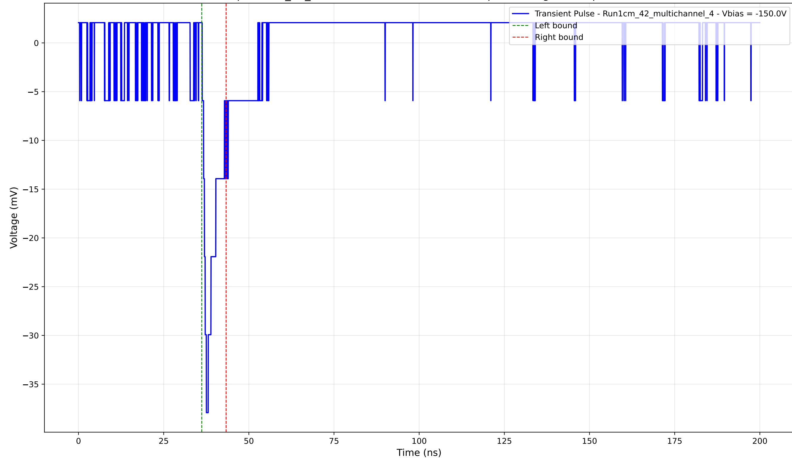
Transient Pulse - Sample: 1cm_42_multichannel - Position: 1680.0 \mu\text{m} - Charge: 2.74 pC - Rise Time: 1.23 ns
