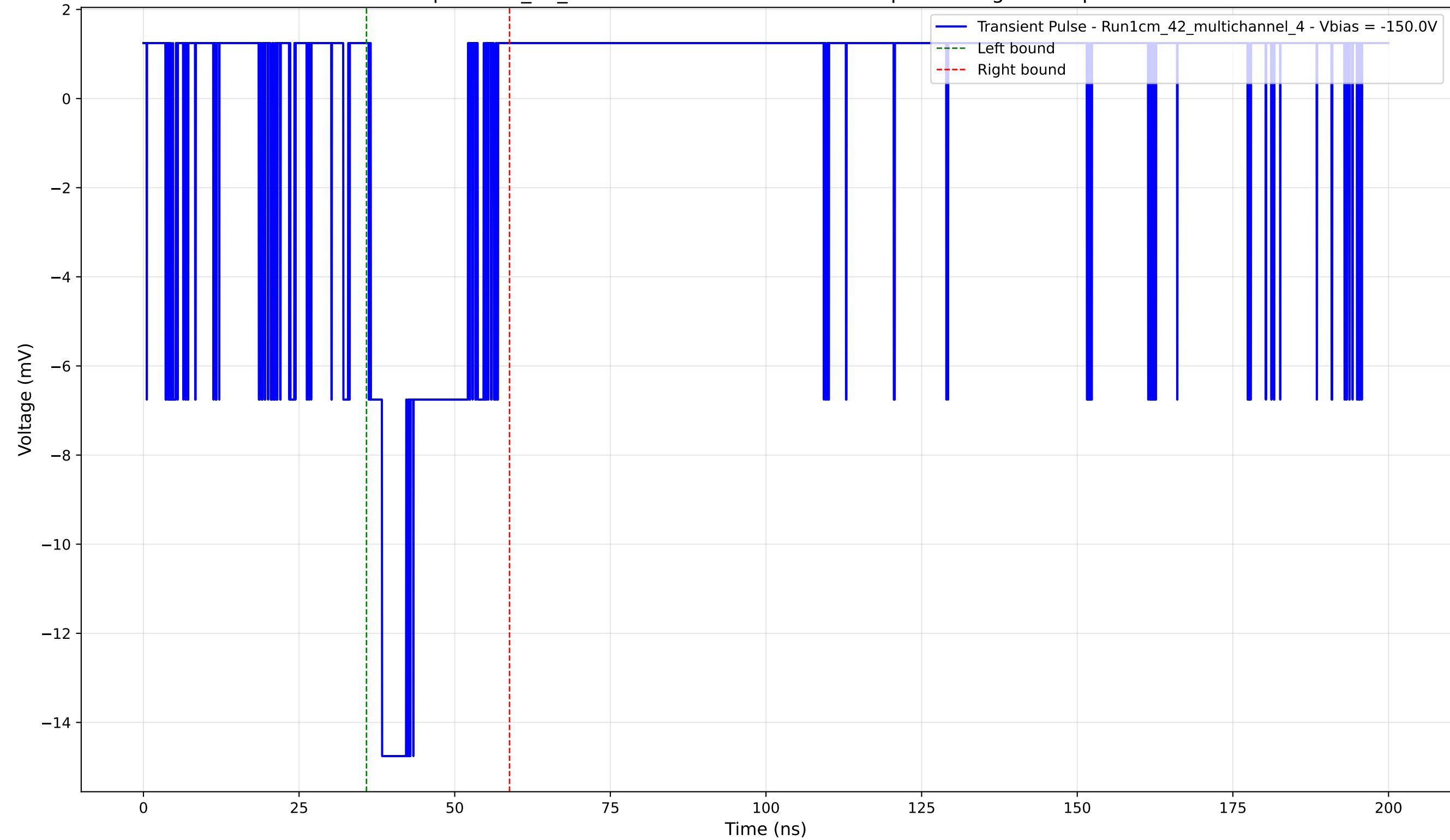
Transient Pulse - Sample: 1cm_42_multichannel - Position: 4575.0 \mu\text{m} - Charge: 3.00 pC - Rise Time: 1.82 ns
