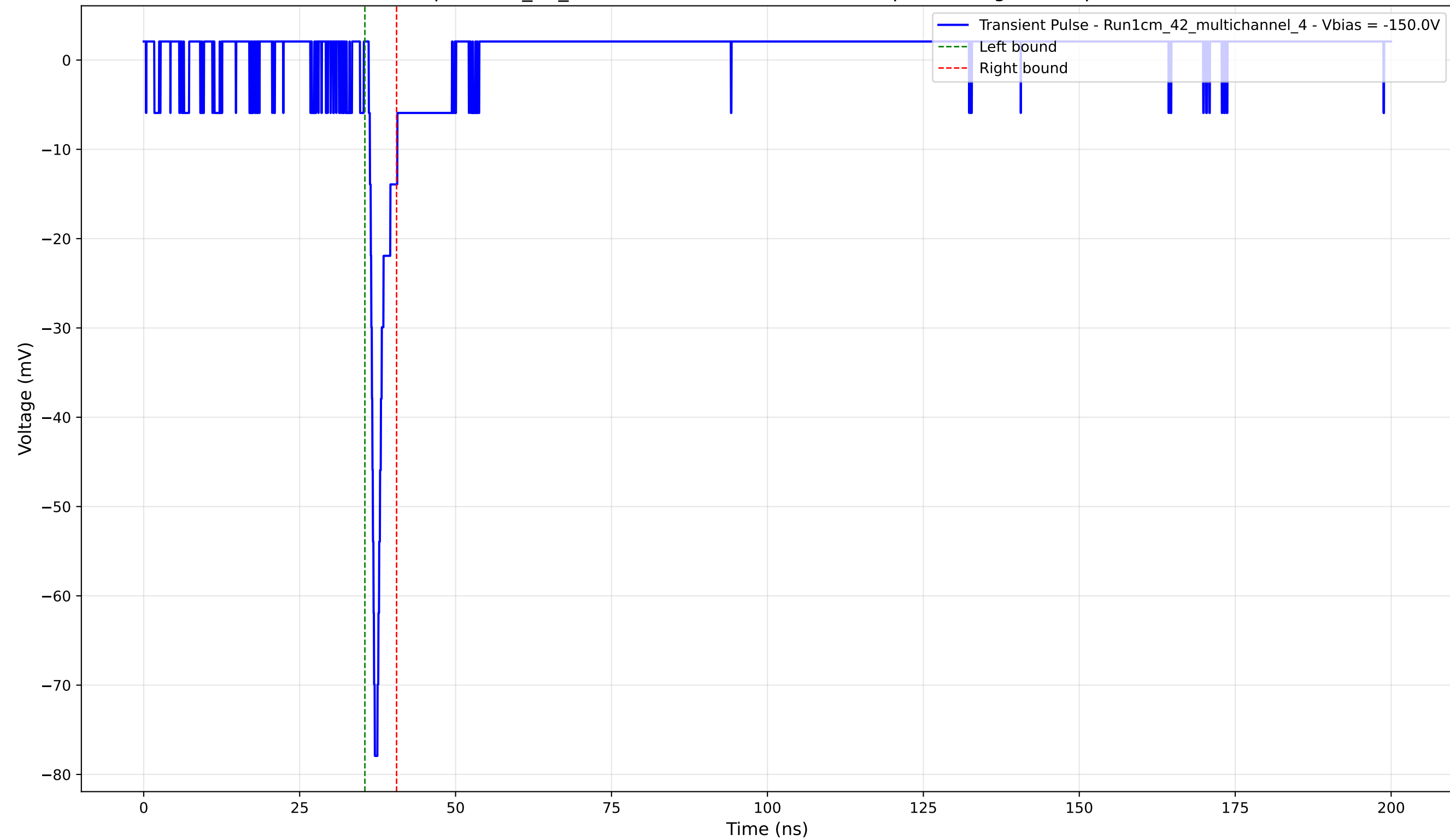
Transient Pulse - Sample: 1cm_42_multichannel - Position: 2285.0 \mu\text{m} - Charge: 2.99 pC - Rise Time: 0.80 ns
