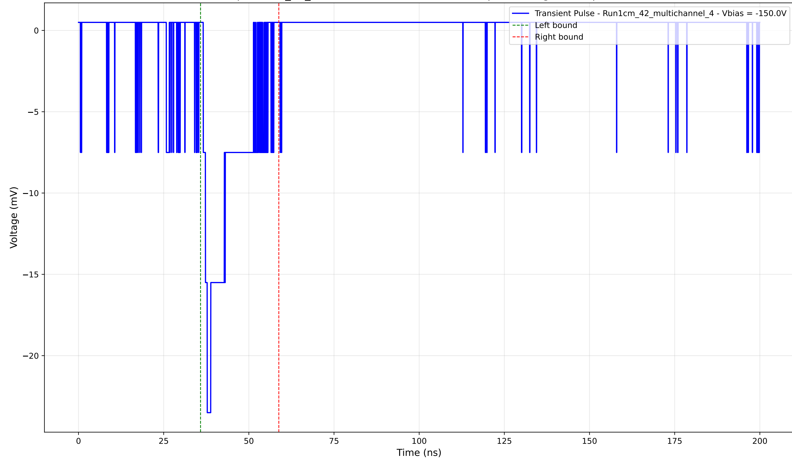
Transient Pulse - Sample: 1cm_42_multichannel - Position: 3530.0 \mu\text{m} - Charge: 3.71 pC - Rise Time: 1.17 ns
