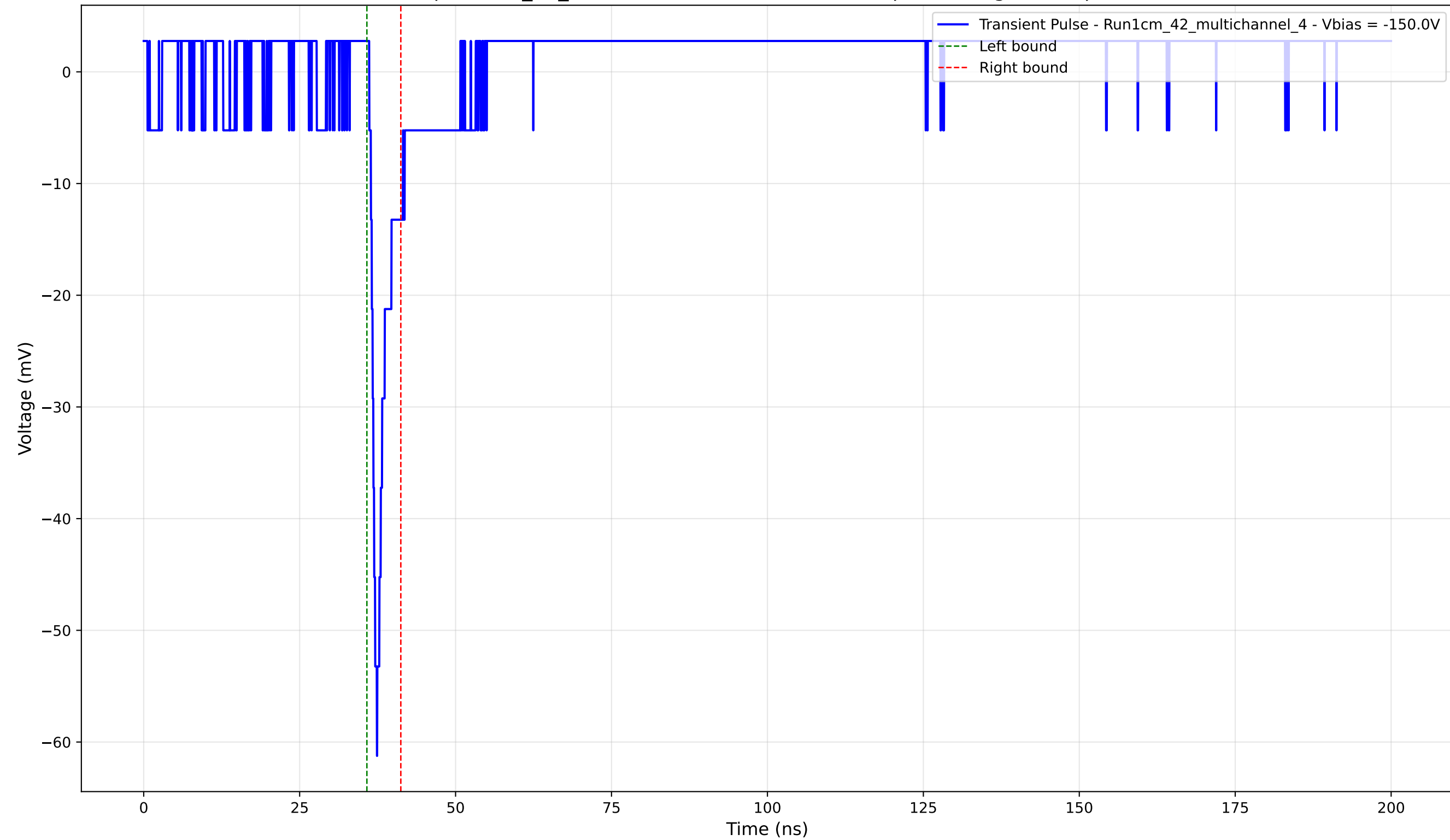
Transient Pulse - Sample: 1cm_42_multichannel - Position: 2065.0 \mu\text{m} - Charge: 2.61 pC - Rise Time: 0.98 ns
