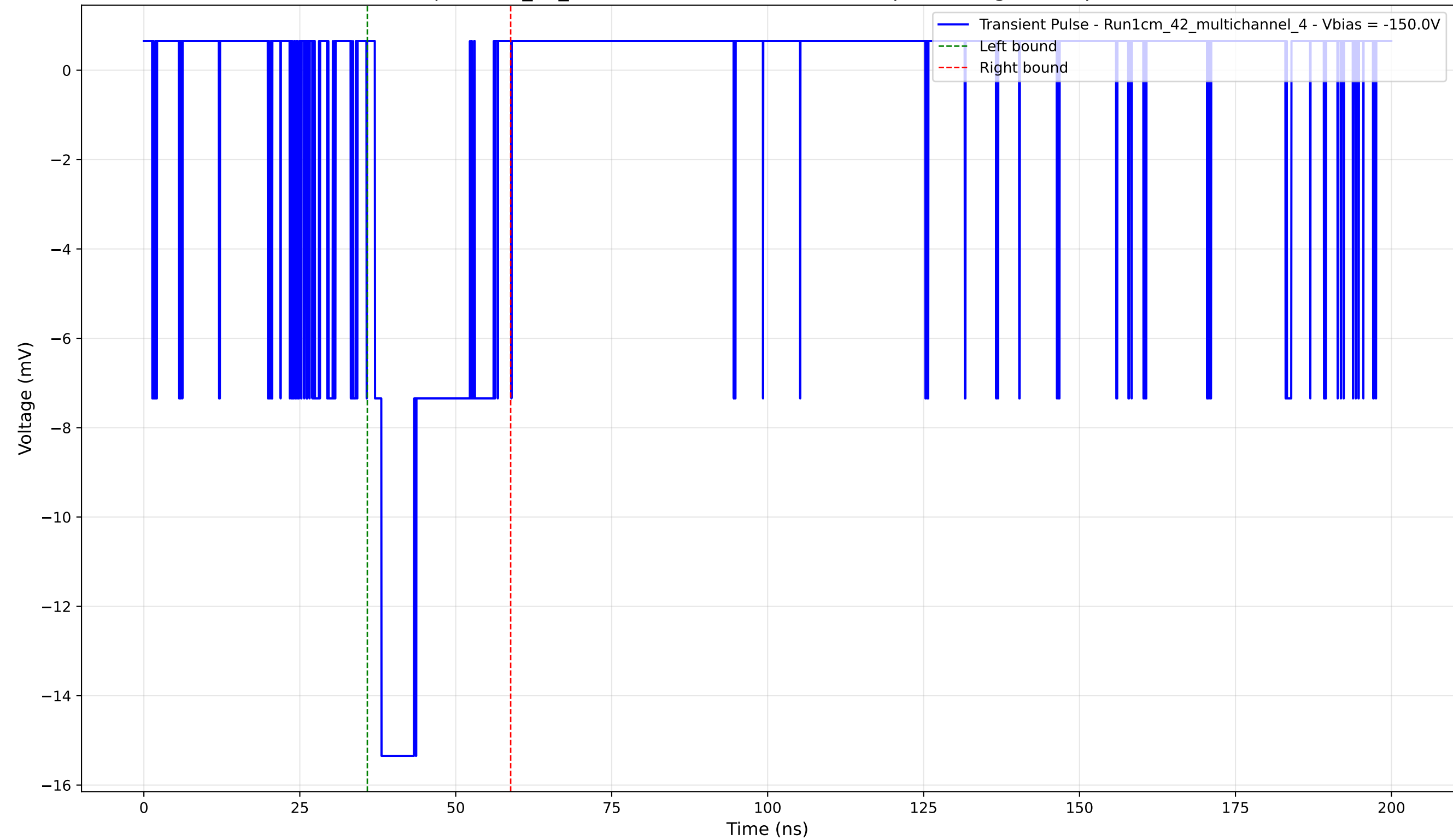
Transient Pulse - Sample: 1cm_42_multichannel - Position: 4120.0 \mu\text{m} - Charge: 3.58 pC - Rise Time: 1.06 ns
