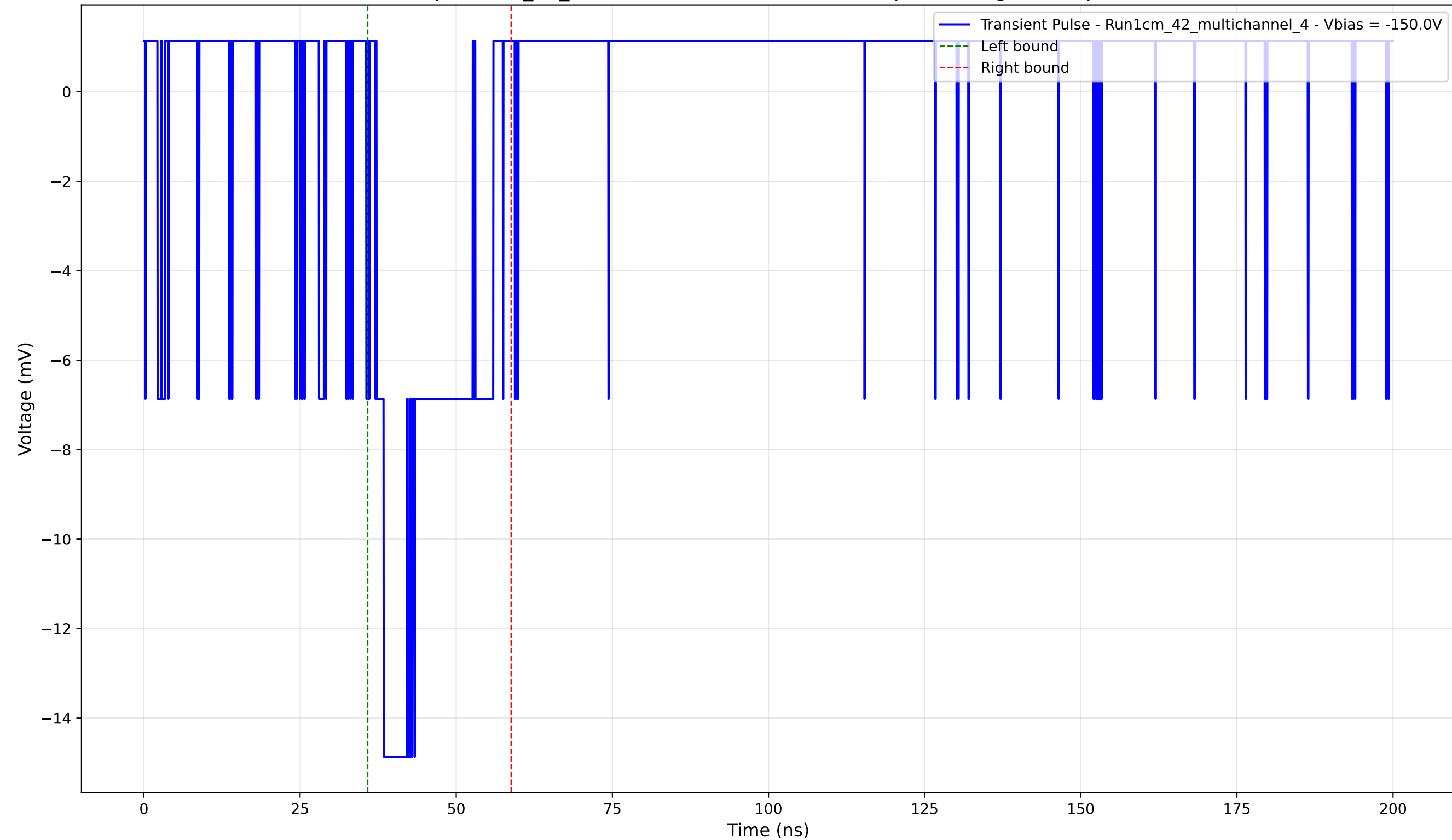
Transient Pulse - Sample: 1cm_42_multichannel - Position: 4185.0 \mu\text{m} - Charge: 3.20 pC - Rise Time: 1.16 ns
