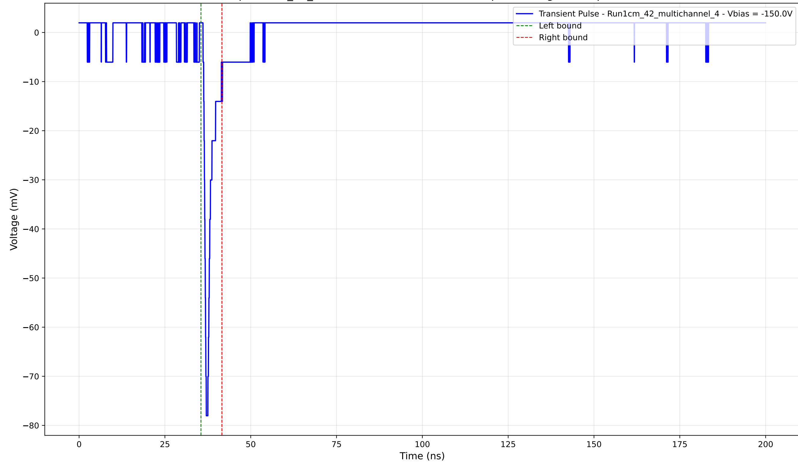
Transient Pulse - Sample: 1cm_42_multichannel - Position: 2245.0 \mu\text{m} - Charge: 3.39 pC - Rise Time: 0.76 ns
