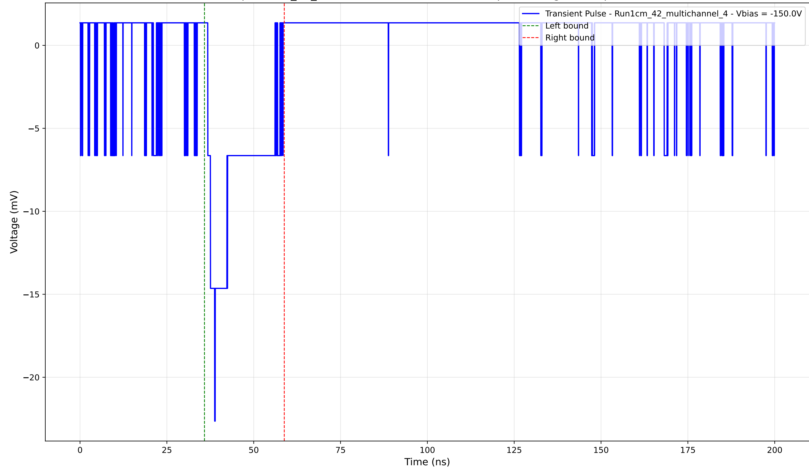
Transient Pulse - Sample: 1cm_42_multichannel - Position: 3685.0 \mu\text{m} - Charge: 3.50 pC - Rise Time: 2.00 ns
