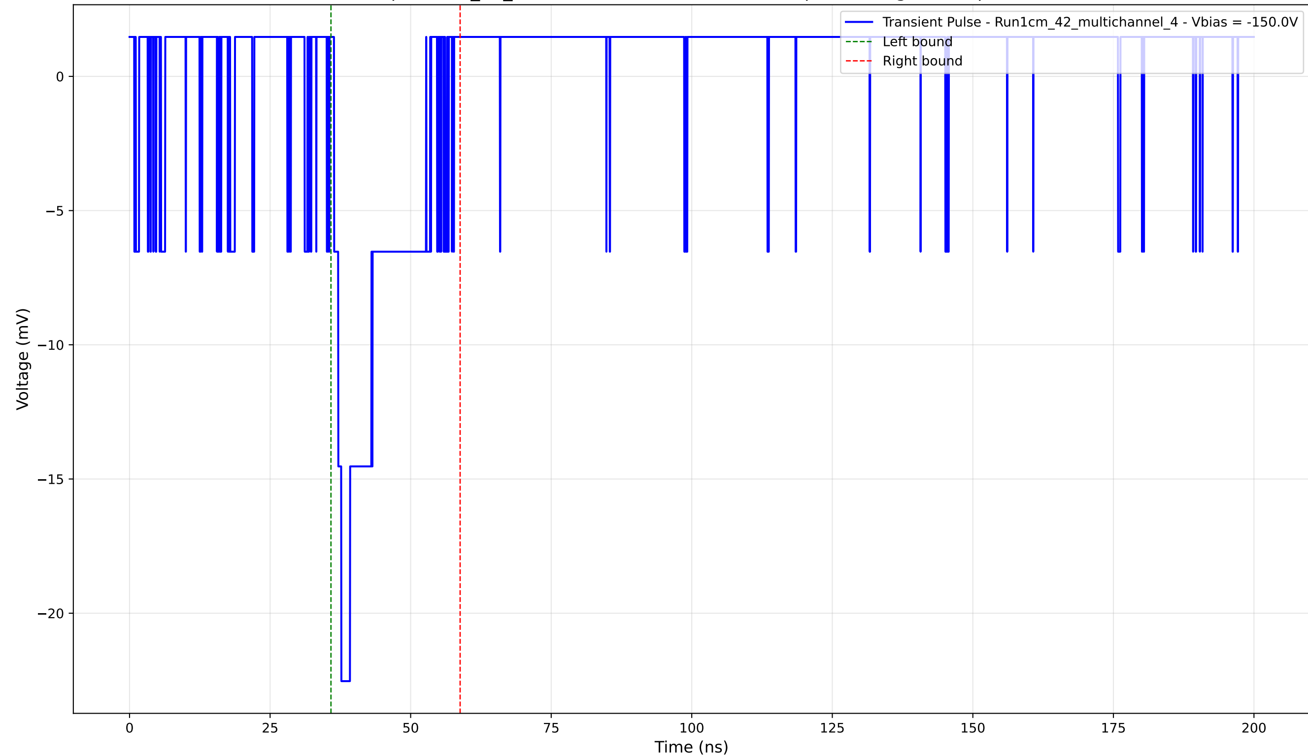
Transient Pulse - Sample: 1cm_42_multichannel - Position: 3480.0 \mu\text{m} - Charge: 3.42 pC - Rise Time: 1.30 ns
