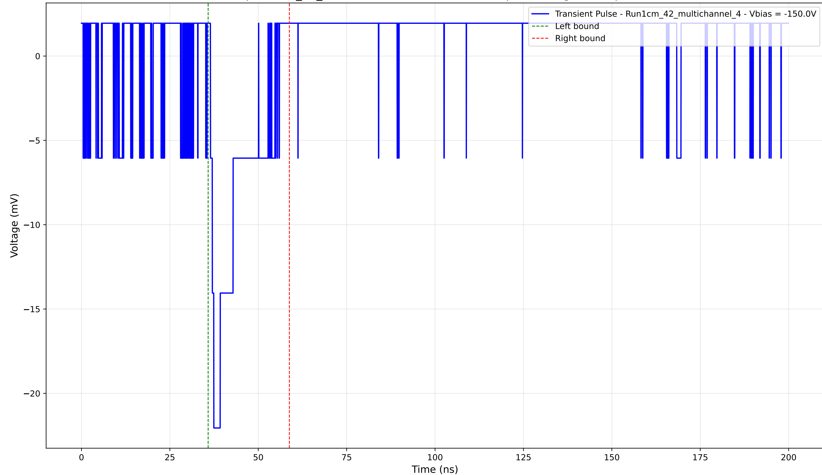
Transient Pulse - Sample: 1cm_42_multichannel - Position: 3315.0 \mu\text{m} - Charge: 3.22 pC - Rise Time: 0.96 ns
