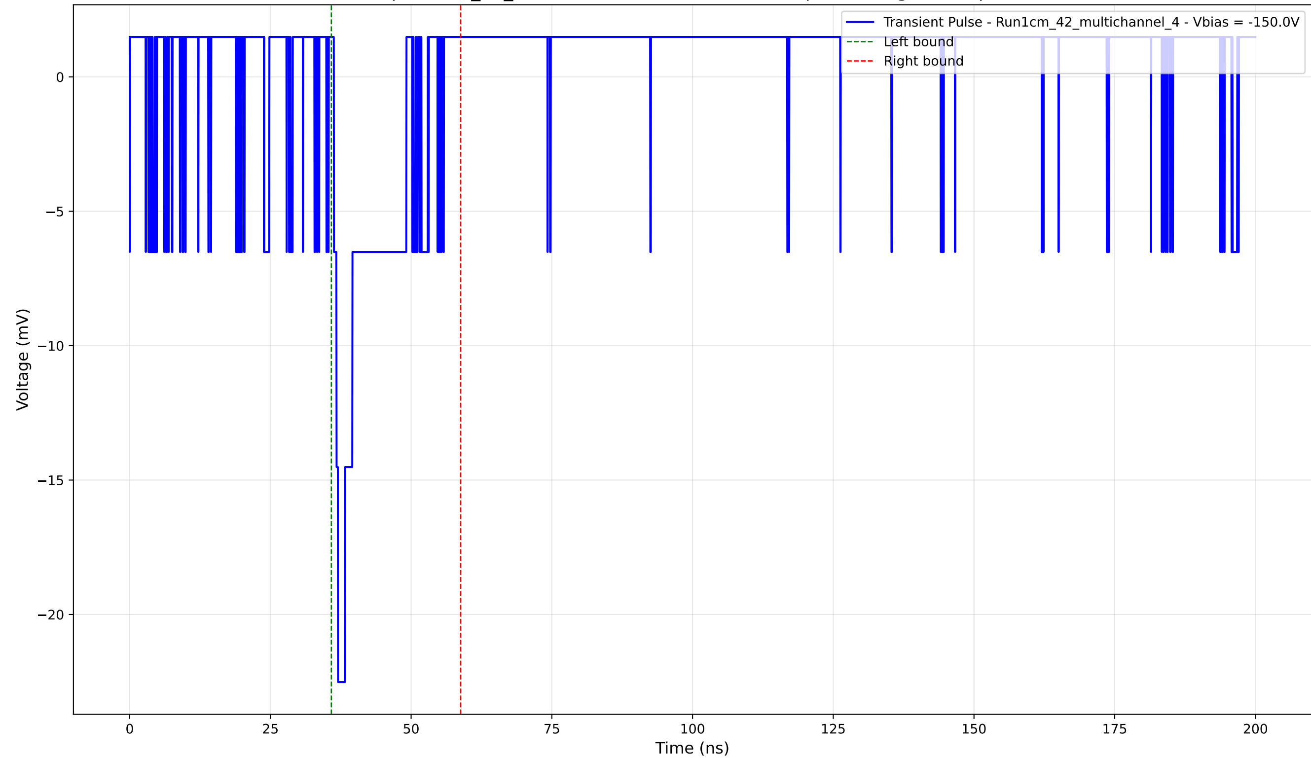
Transient Pulse - Sample: 1cm_42_multichannel - Position: 2840.0 \mu\text{m} - Charge: 2.44 pC - Rise Time: 0.74 ns
