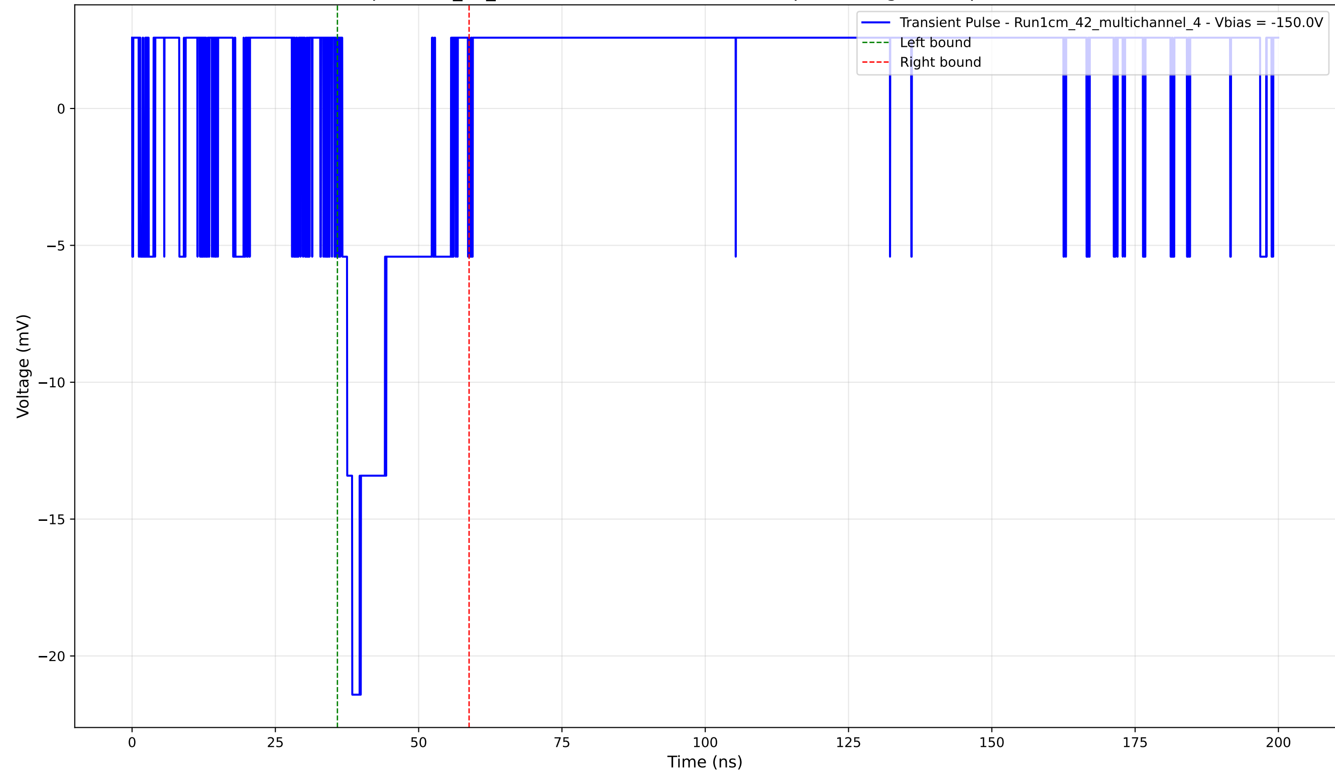
Transient Pulse - Sample: 1cm_42_multichannel - Position: 1060.0 \mu\text{m} - Charge: 3.26 pC - Rise Time: 0.00 ns (N/A)
