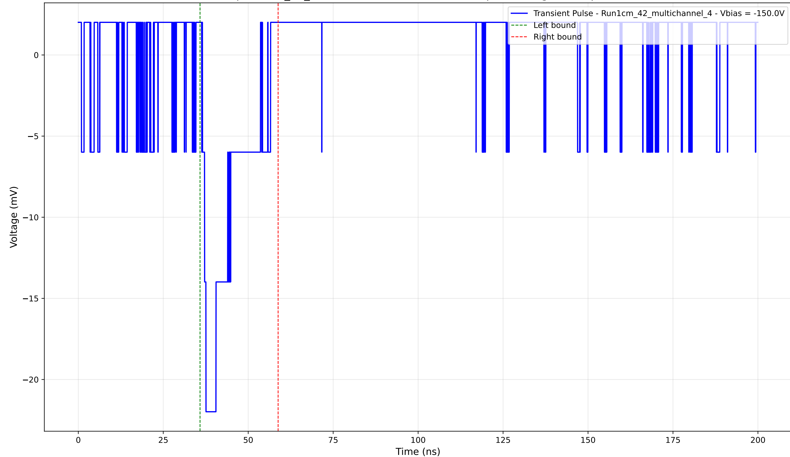
Transient Pulse - Sample: 1cm_42_multichannel - Position: 1260.0 \mu\text{m} - Charge: 3.87 pC - Rise Time: 1.04 ns
