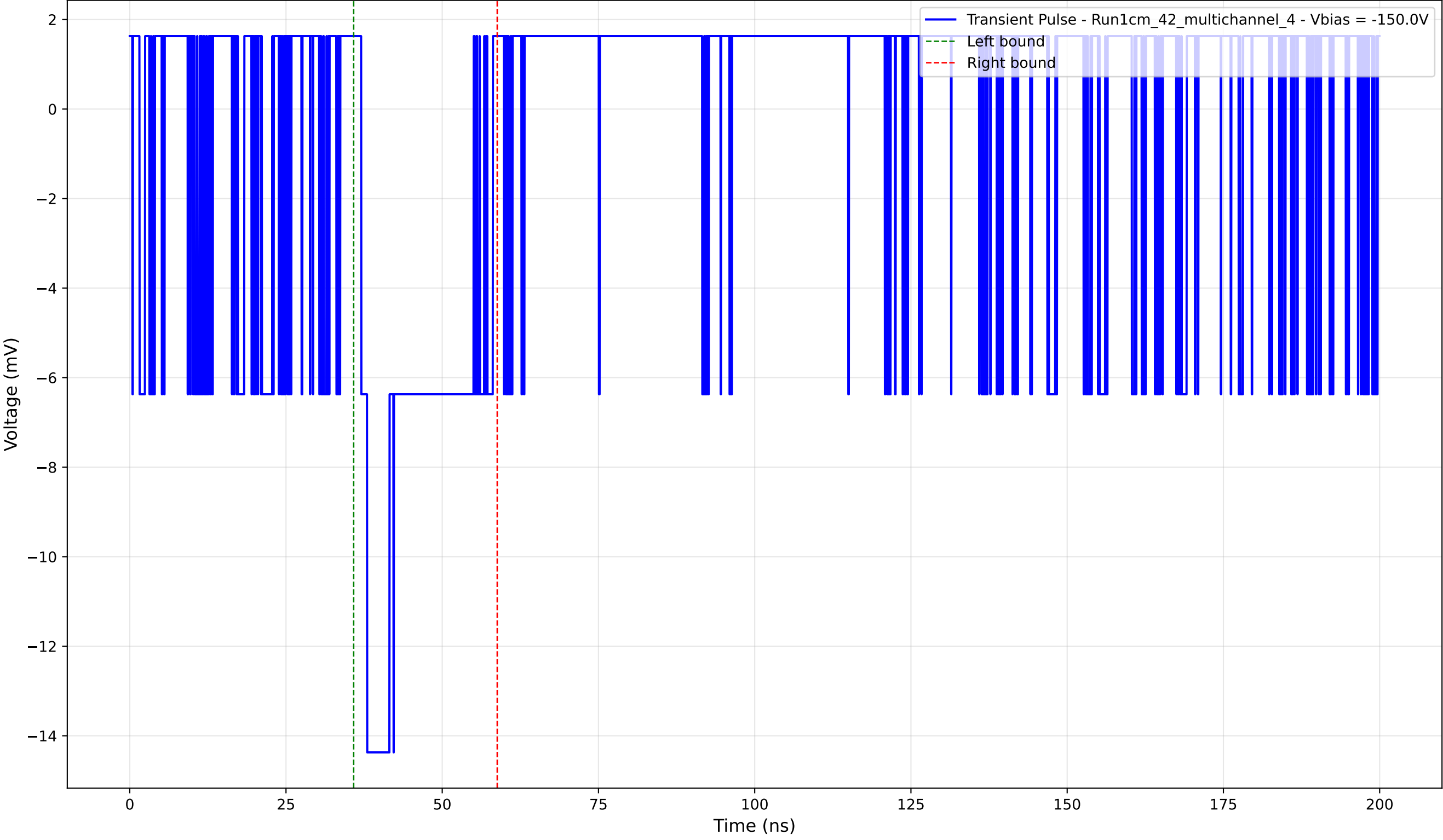
Transient Pulse - Sample: 1cm_42_multichannel - Position: 925.0 \mu\text{m} - Charge: 3.10 pC - Rise Time: 0.00 ns (N/A)
