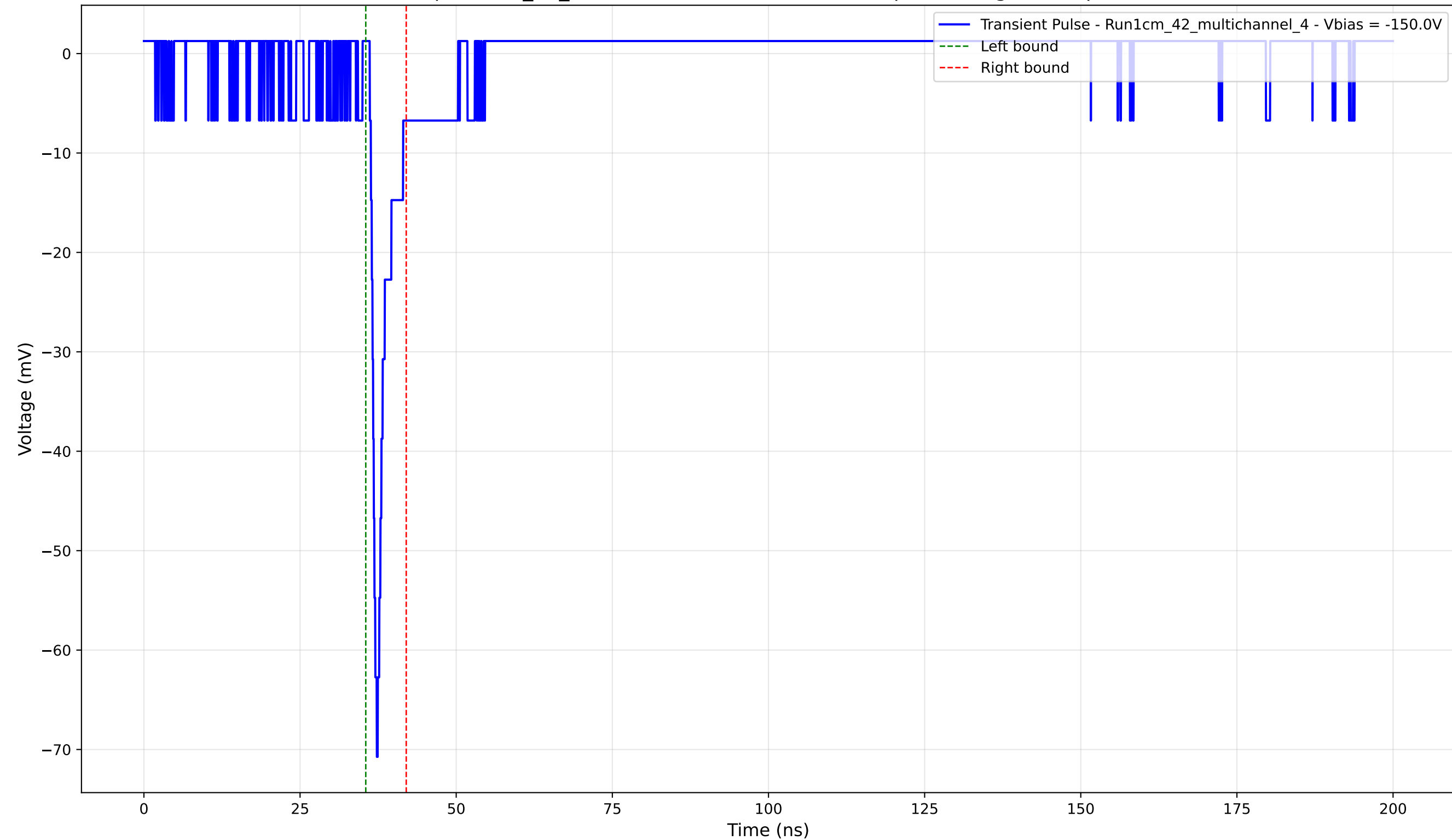
Transient Pulse - Sample: 1cm_42_multichannel - Position: 2165.0 \mu\text{m} - Charge: 3.13 pC - Rise Time: 0.96 ns
