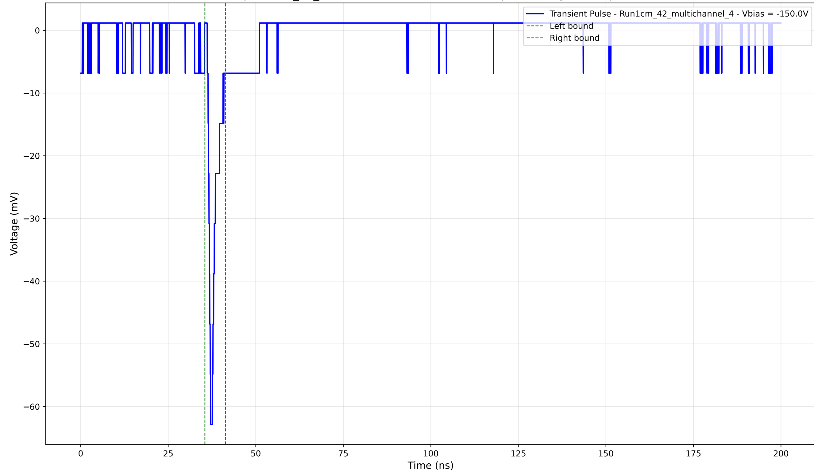
Transient Pulse - Sample: 1cm_42_multichannel - Position: 2615.0 \mu\text{m} - Charge: 2.80 pC - Rise Time: 0.98 ns
