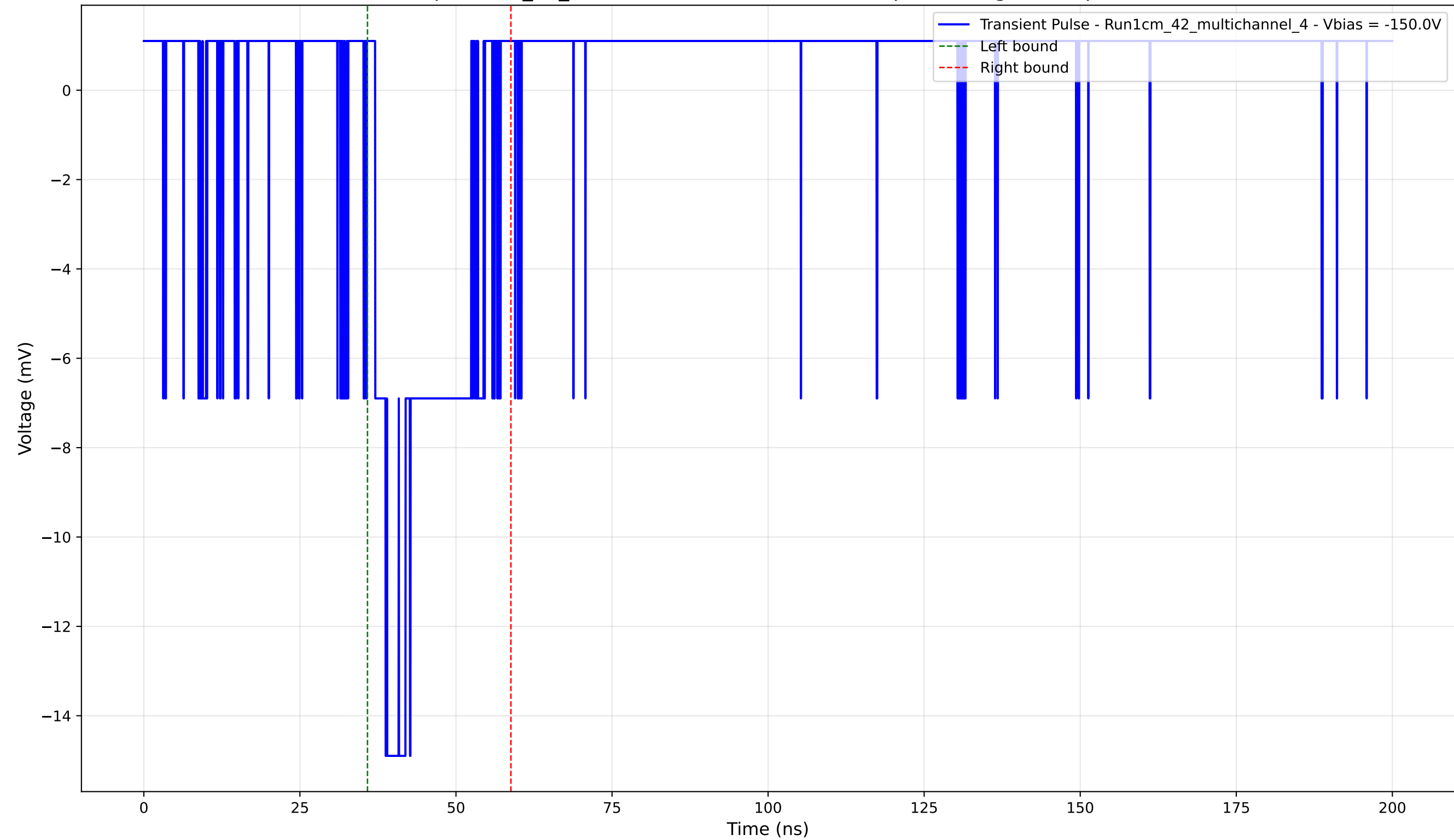
Transient Pulse - Sample: 1cm_42_multichannel - Position: 4805.0 \mu\text{m} - Charge: 2.81 pC - Rise Time: 1.68 ns
