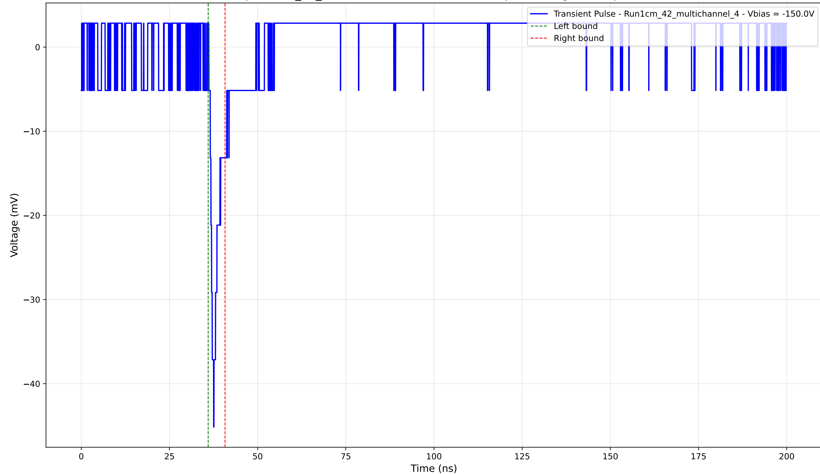
Transient Pulse - Sample: 1cm_42_multichannel - Position: 1945.0 \mu\text{m} - Charge: 1.98 pC - Rise Time: 1.37 ns
