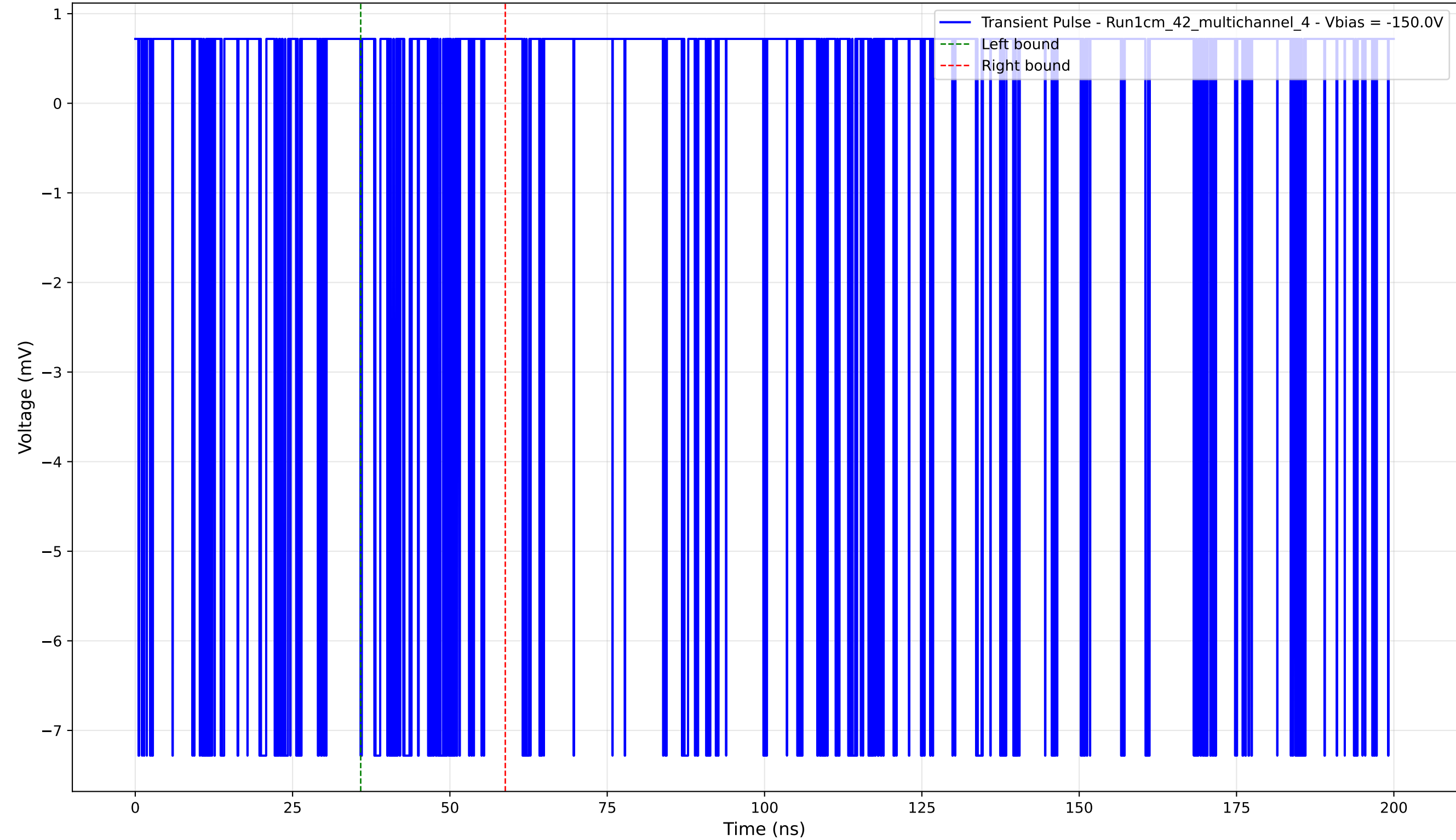
Transient Pulse - Sample: 1cm_42_multichannel - Position: 4395.0 \mu\text{m} - Charge: 0.80 pC - Rise Time: 0.02 ns
