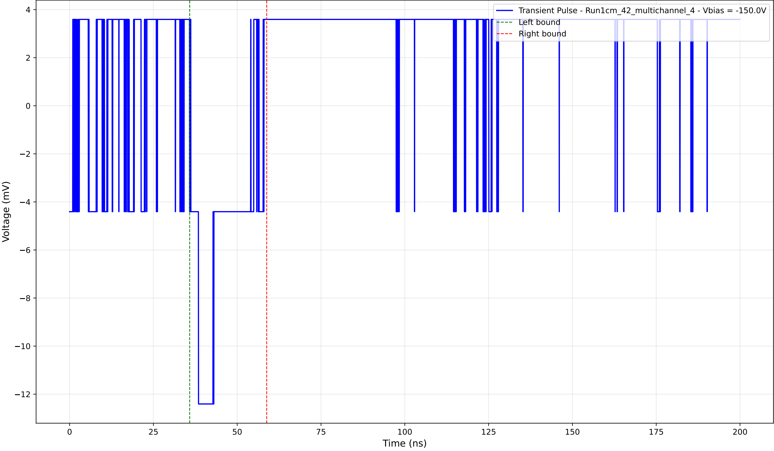
Transient Pulse - Sample: 1cm_42_multichannel - Position: 160.0 \mu\text{m} - Charge: 2.32 pC - Rise Time: 0.00 ns (N/A)
