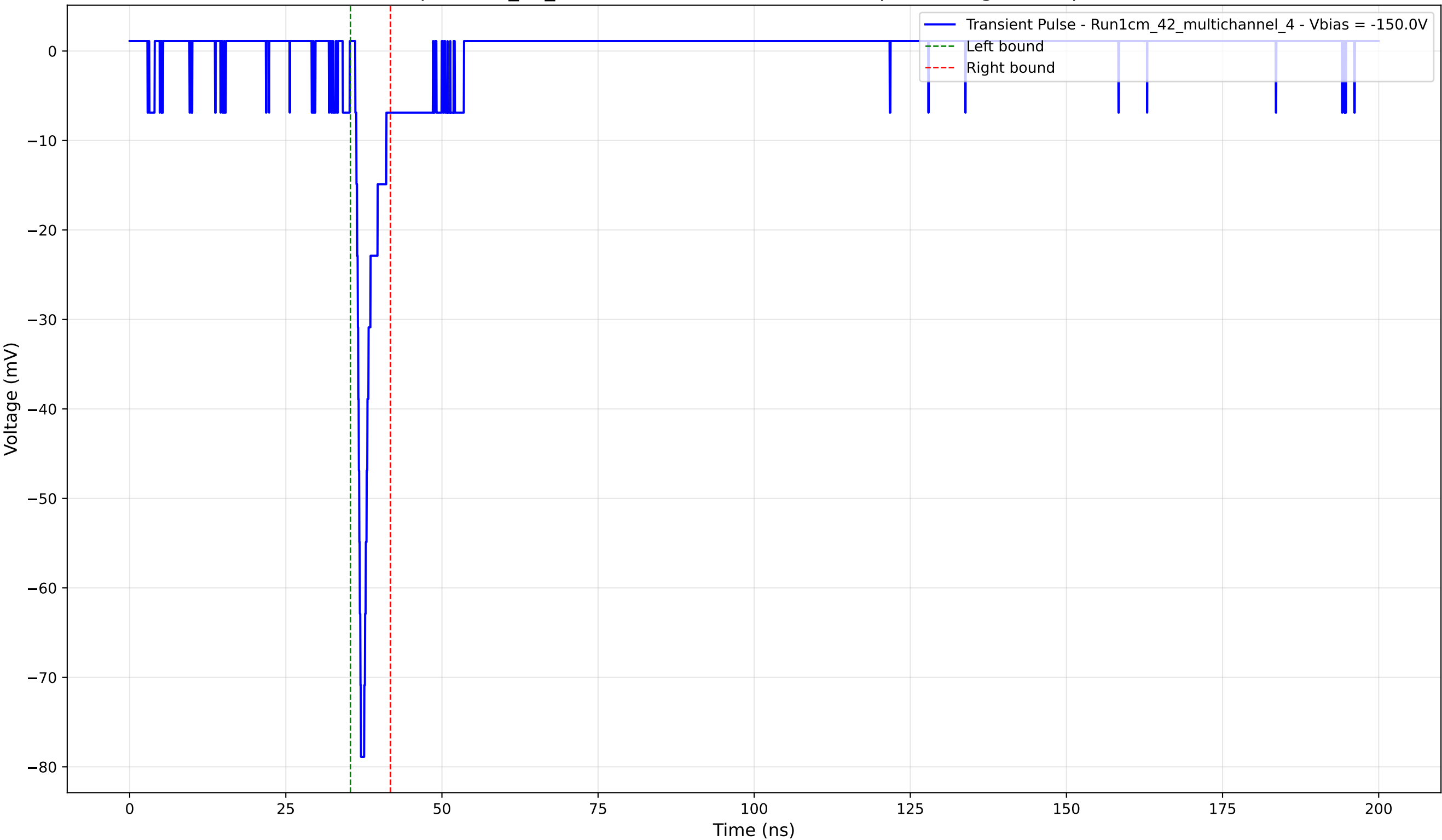
Transient Pulse - Sample: 1cm_42_multichannel - Position: 2250.0 \mu\text{m} - Charge: 3.41 pC - Rise Time: 0.74 ns
