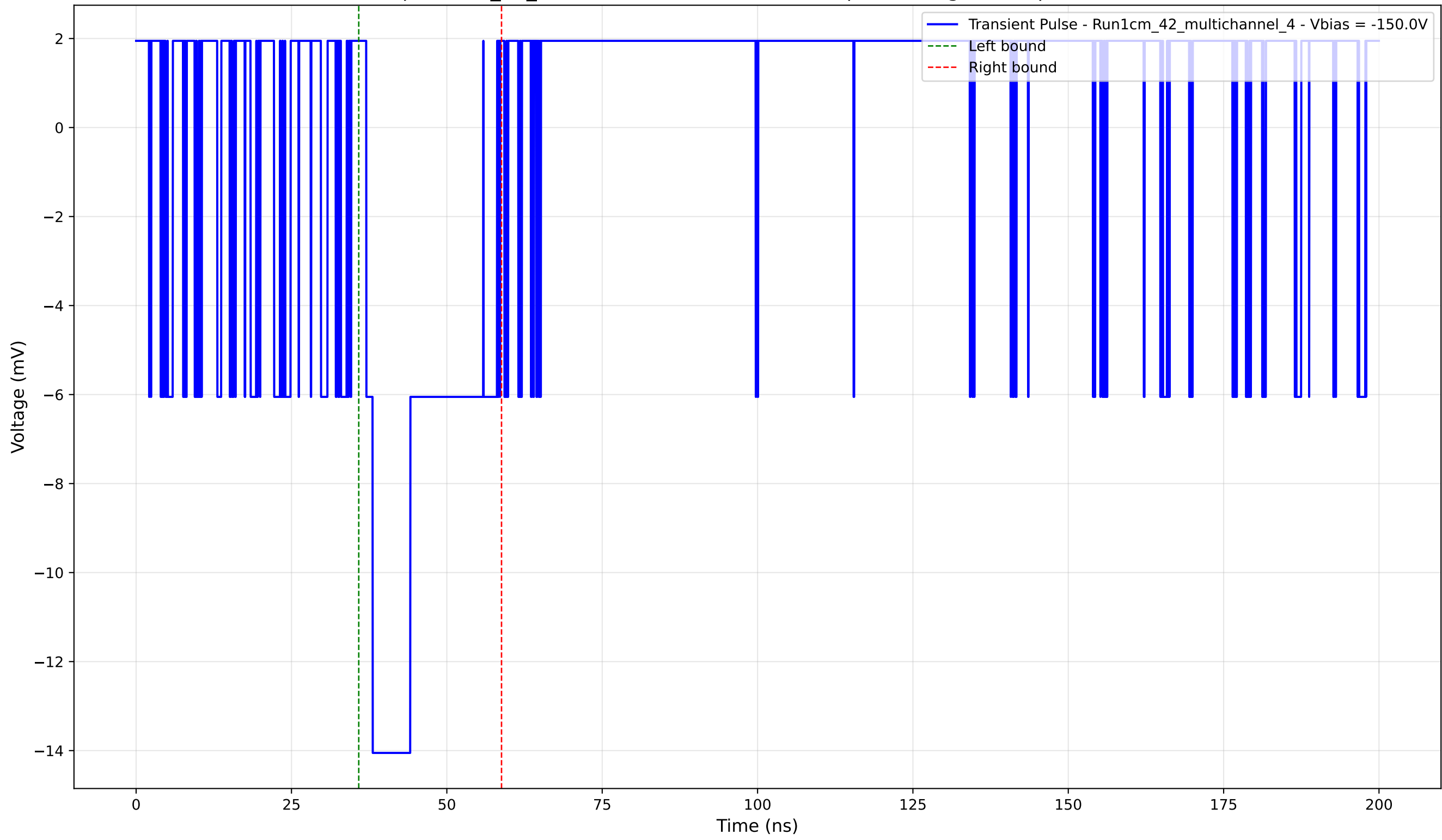
Transient Pulse - Sample: 1cm_42_multichannel - Position: 485.0 \mu\text{m} - Charge: 3.46 pC - Rise Time: 0.00 ns (N/A)
