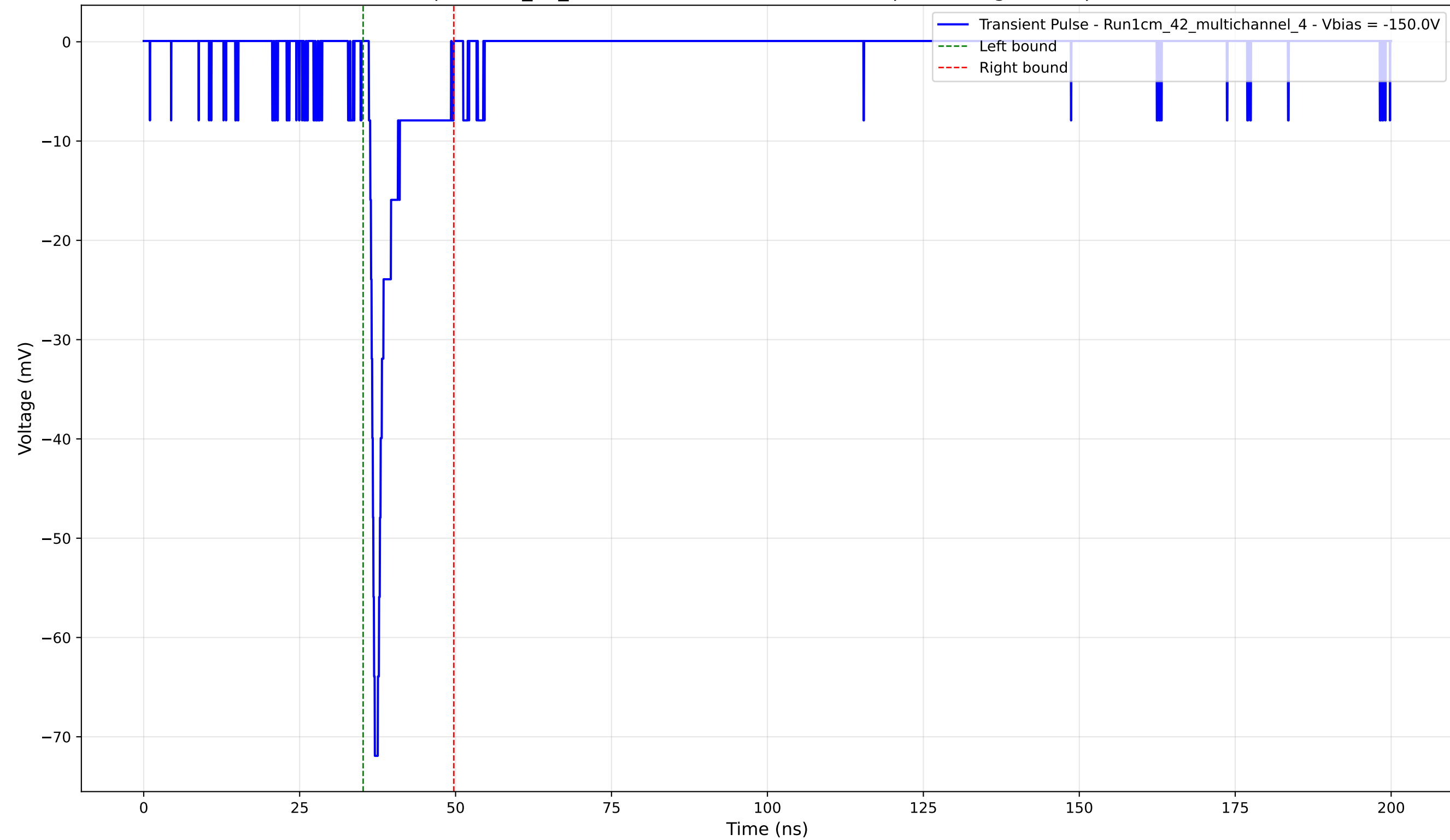
Transient Pulse - Sample: 1cm_42_multichannel - Position: 2550.0 \mu\text{m} - Charge: 4.51 pC - Rise Time: 0.94 ns
