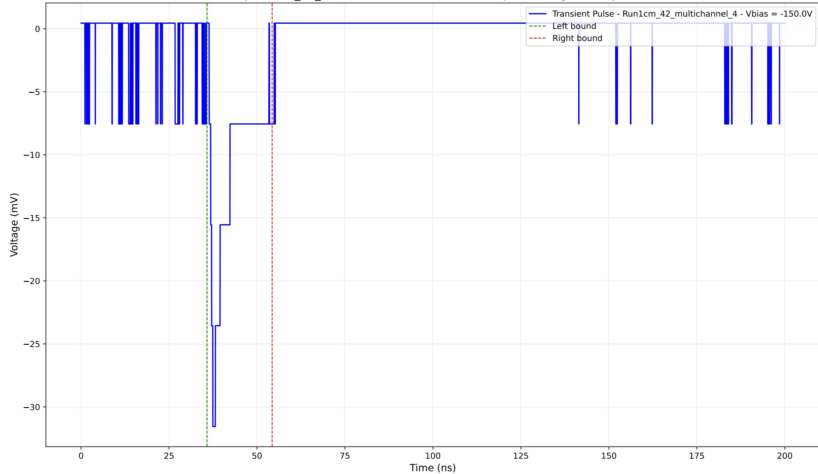
Transient Pulse - Sample: 1cm_42_multichannel - Position: 3160.0 \mu\text{m} - Charge: 4.05 pC - Rise Time: 1.05 ns
