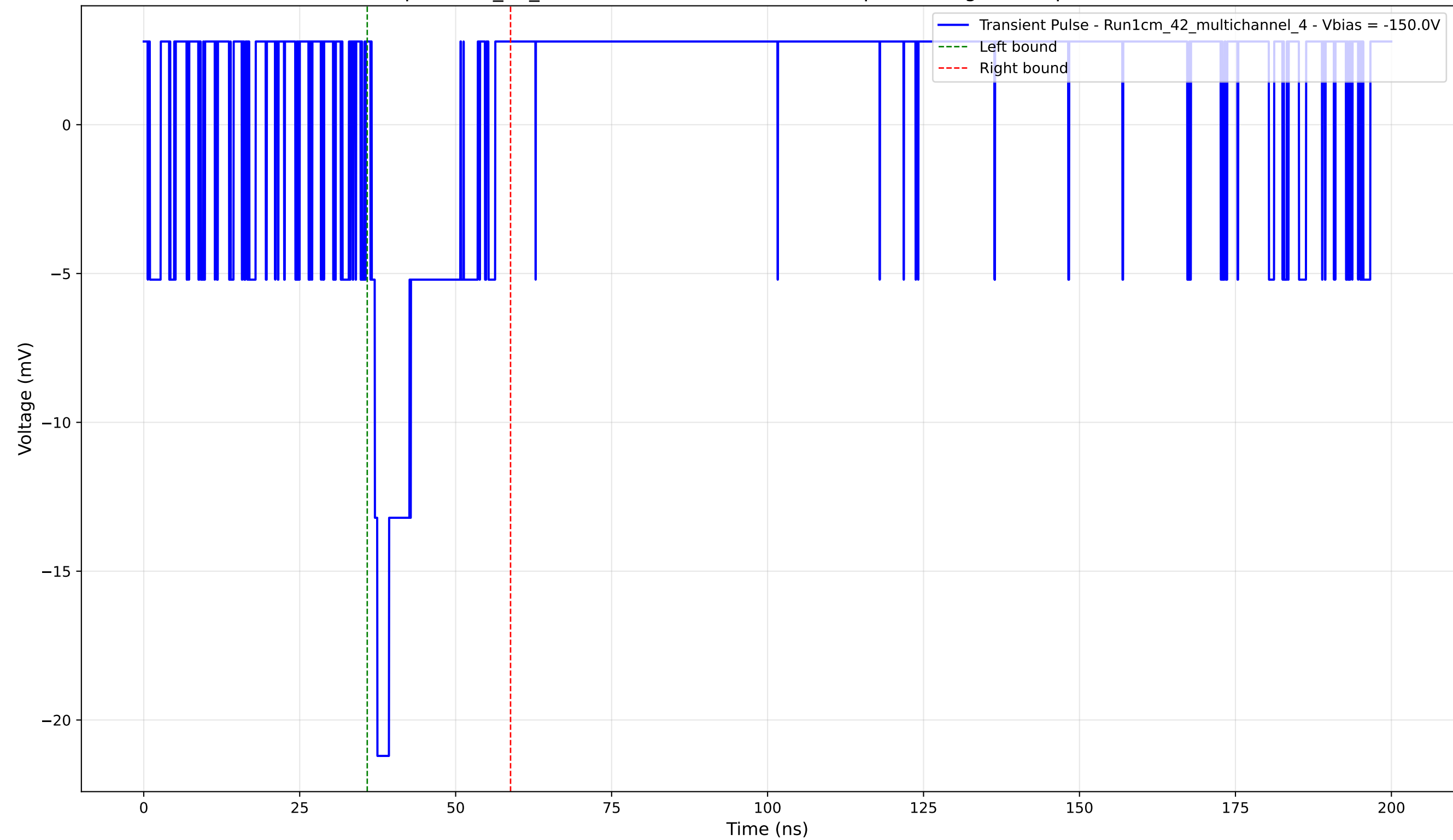
Transient Pulse - Sample: 1cm_42_multichannel - Position: 1440.0 \mu\text{m} - Charge: 2.84 pC - Rise Time: 0.00 ns (N/A)
