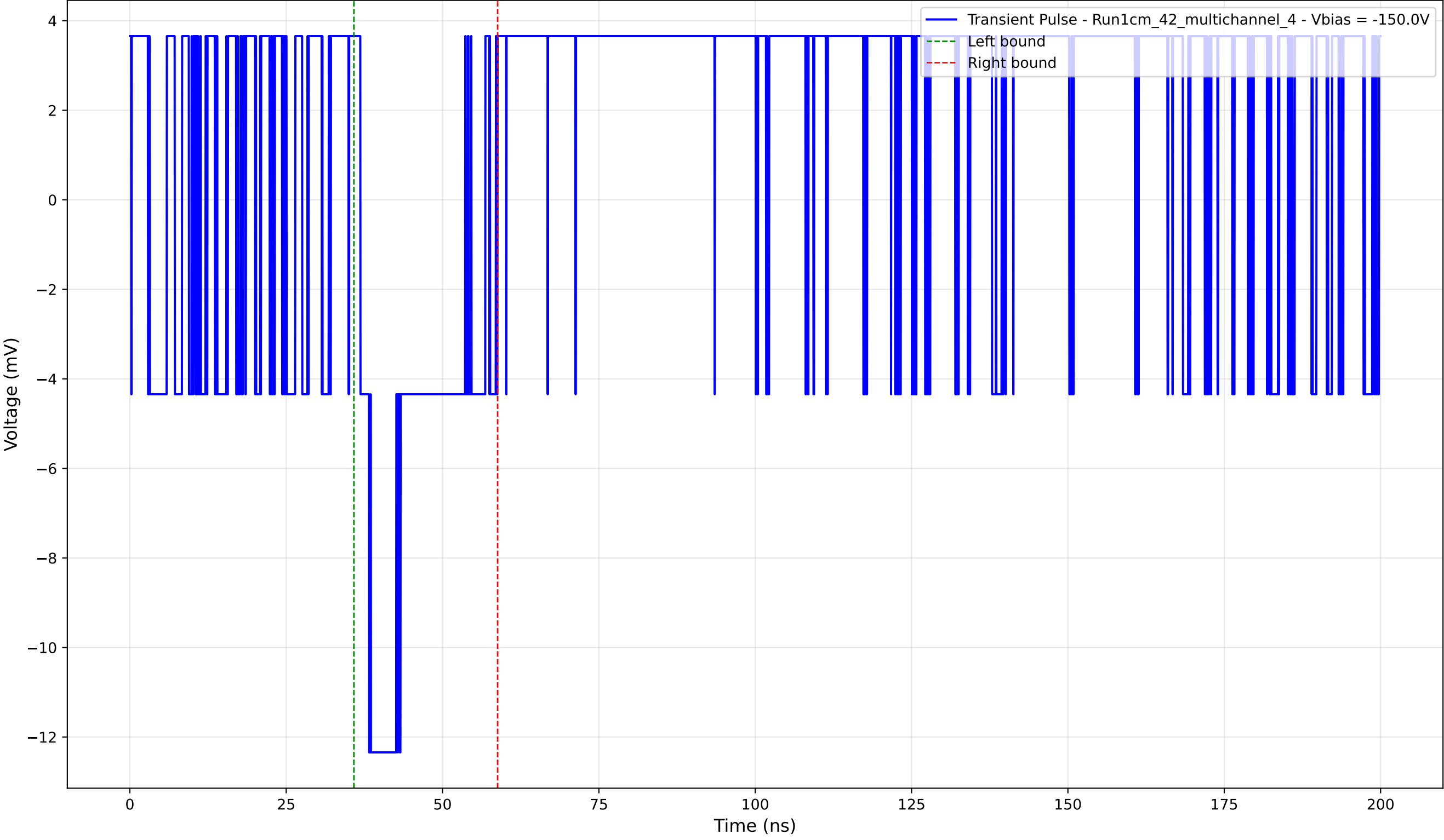
Transient Pulse - Sample: 1cm_42_multichannel - Position: 260.0 \mu\text{m} - Charge: 2.37 pC - Rise Time: 0.00 ns (N/A)
