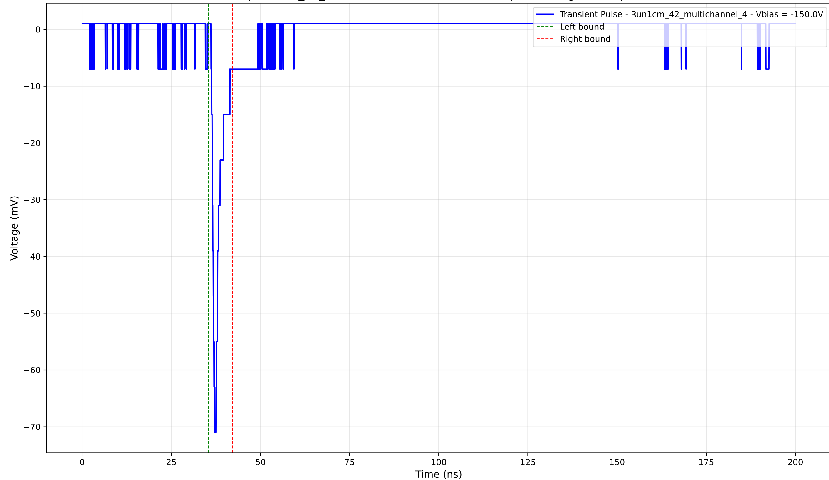
Transient Pulse - Sample: 1cm_42_multichannel - Position: 2170.0 \mu\text{m} - Charge: 3.28 pC - Rise Time: 0.80 ns
