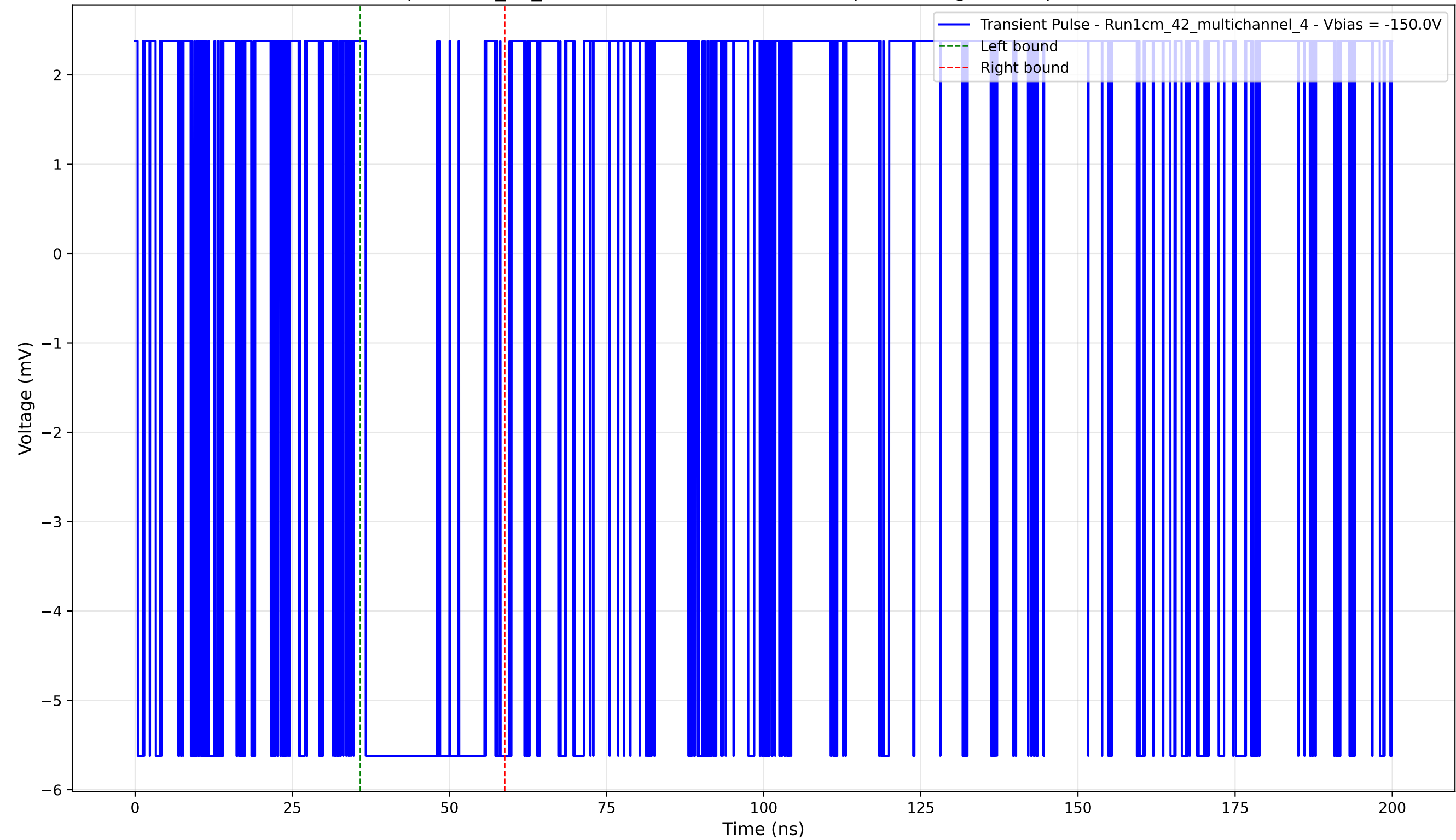
Transient Pulse - Sample: 1cm_42_multichannel - Position: 825.0 \mu\text{m} - Charge: 2.10 pC - Rise Time: 0.00 ns (N/A)
