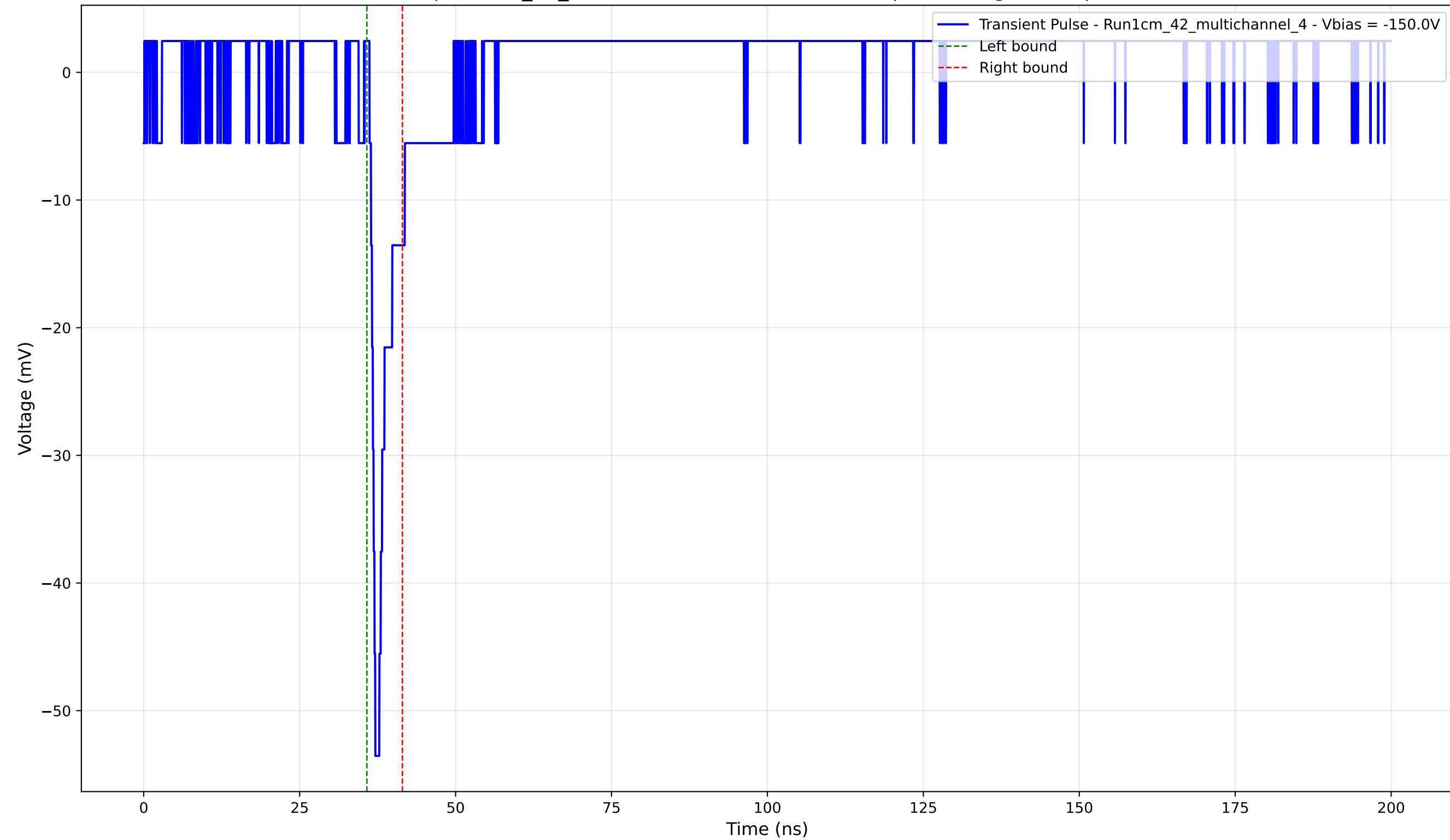
Transient Pulse - Sample: 1cm_42_multichannel - Position: 2725.0 \mu\text{m} - Charge: 2.67 pC - Rise Time: 0.92 ns
