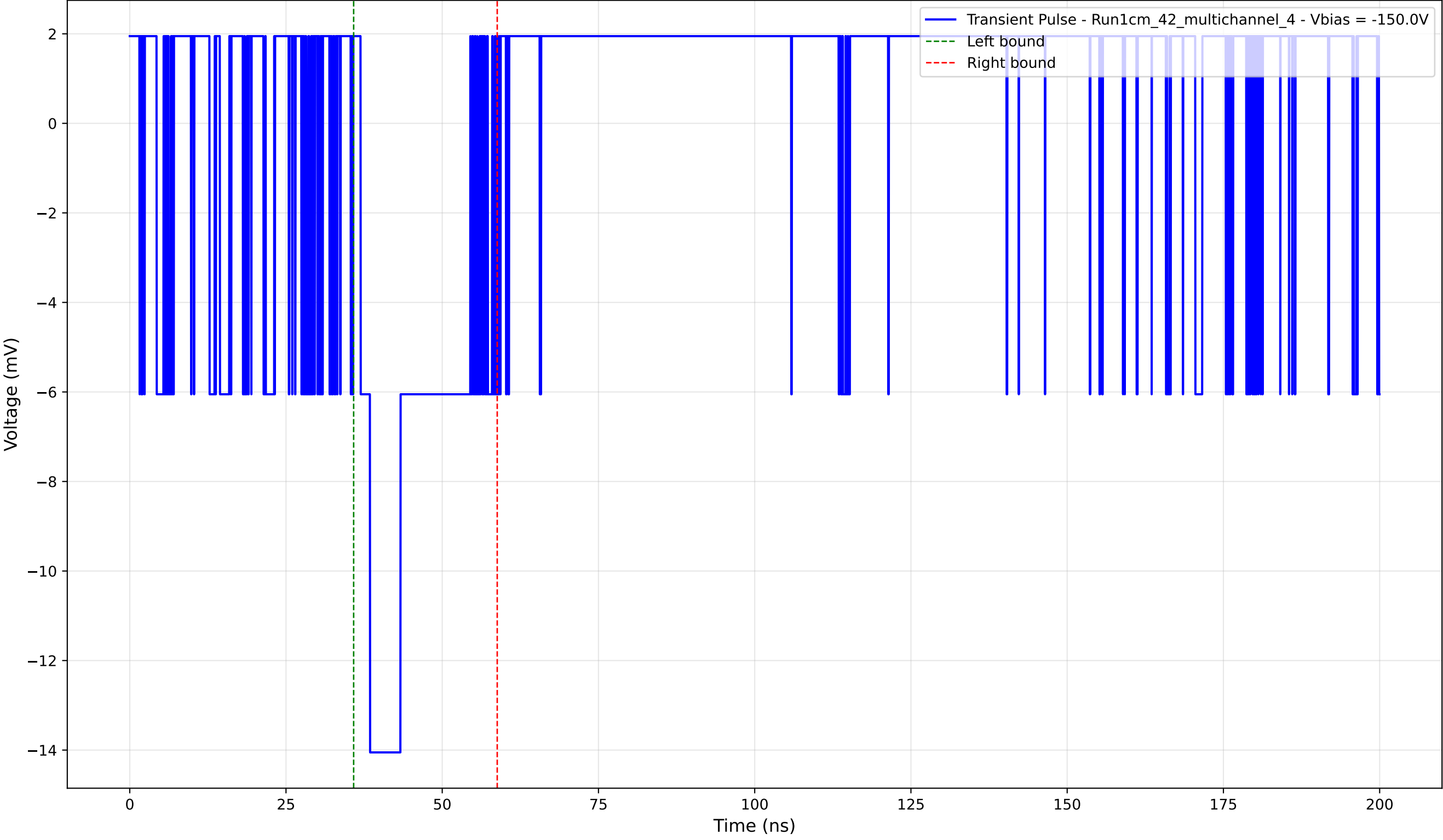
Transient Pulse - Sample: 1cm_42_multichannel - Position: 440.0 \mu\text{m} - Charge: 3.16 pC - Rise Time: 0.00 ns (N/A)
