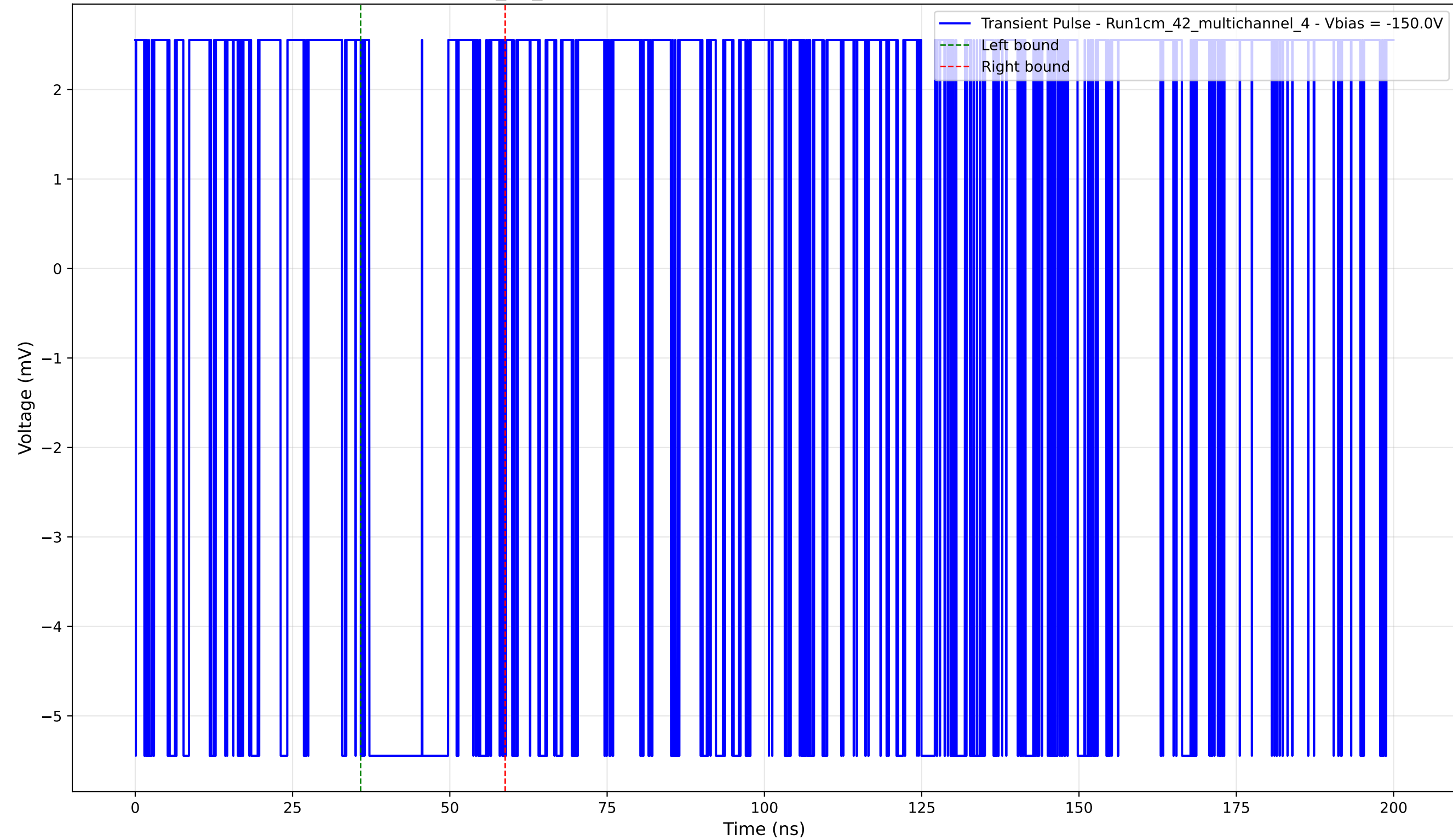
Transient Pulse - Sample: 1cm_42_multichannel - Position: 900.0 \mu\text{m} - Charge: 1.25 pC - Rise Time: 0.00 ns (N/A)
