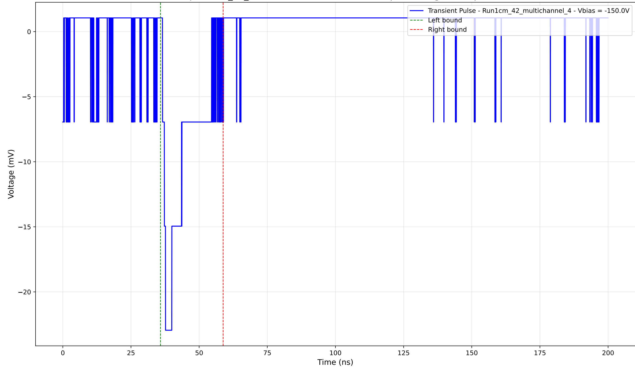
Transient Pulse - Sample: 1cm_42_multichannel - Position: 1230.0 \mu\text{m} - Charge: 4.01 pC - Rise Time: 1.12 ns
