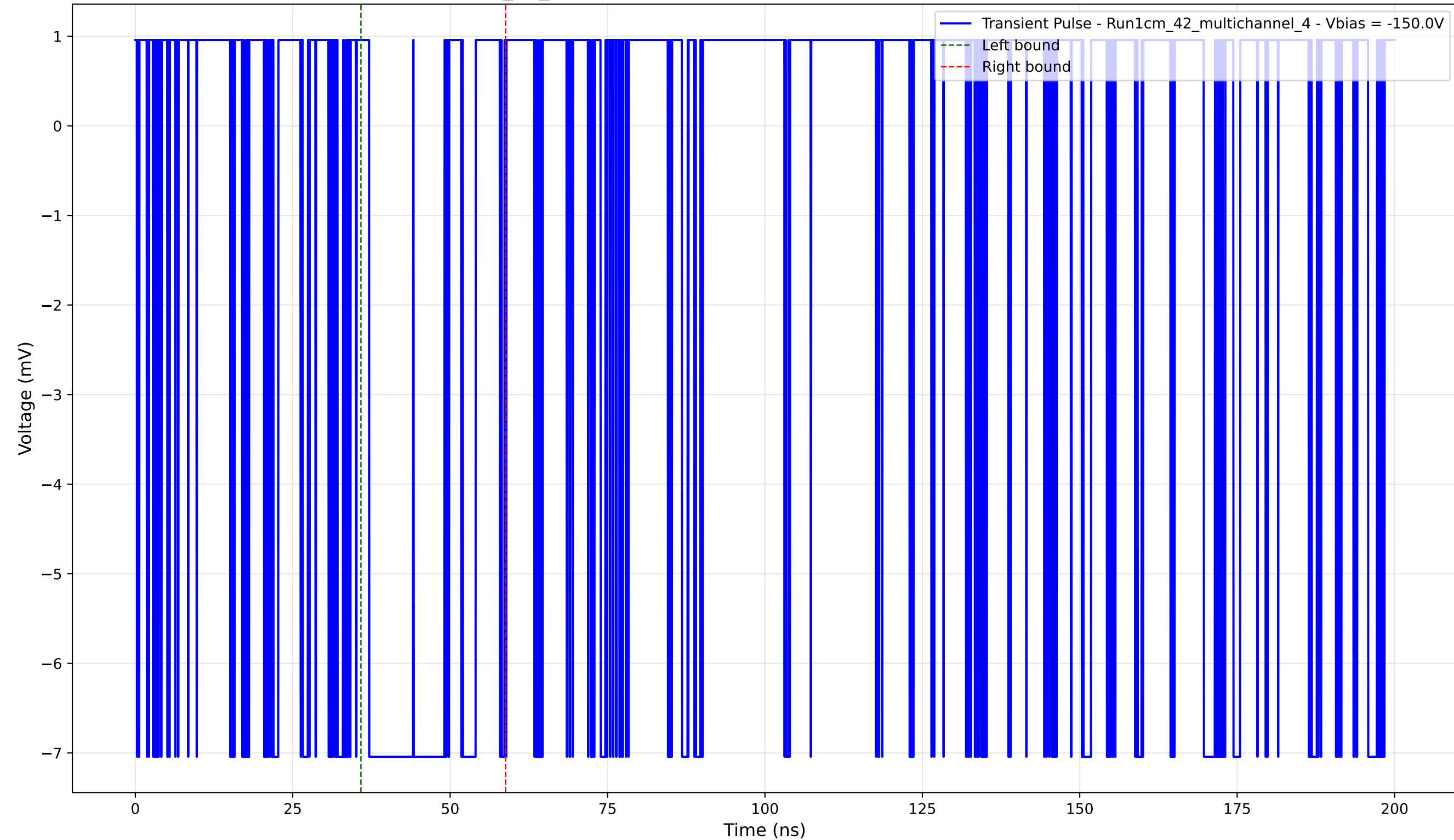
Transient Pulse - Sample: 1cm_42_multichannel - Position: 80.0 \mu\text{m} - Charge: 1.97 pC - Rise Time: 0.00 ns (N/A)
