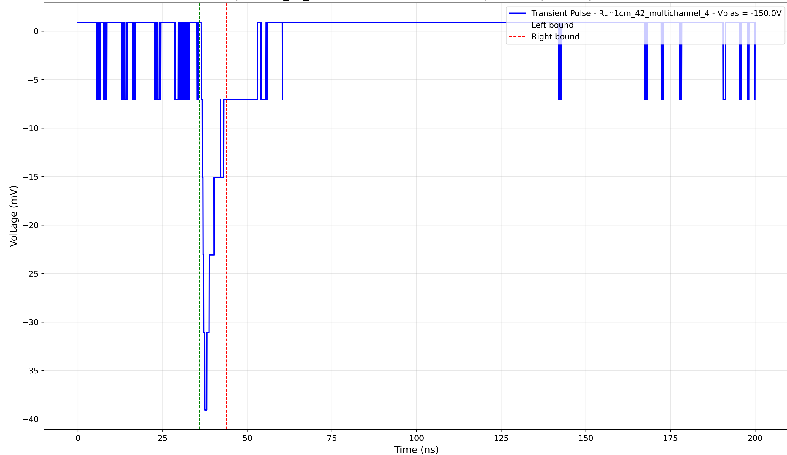
Transient Pulse - Sample: 1cm_42_multichannel - Position: 1710.0 \mu\text{m} - Charge: 2.95 pC - Rise Time: 1.07 ns
