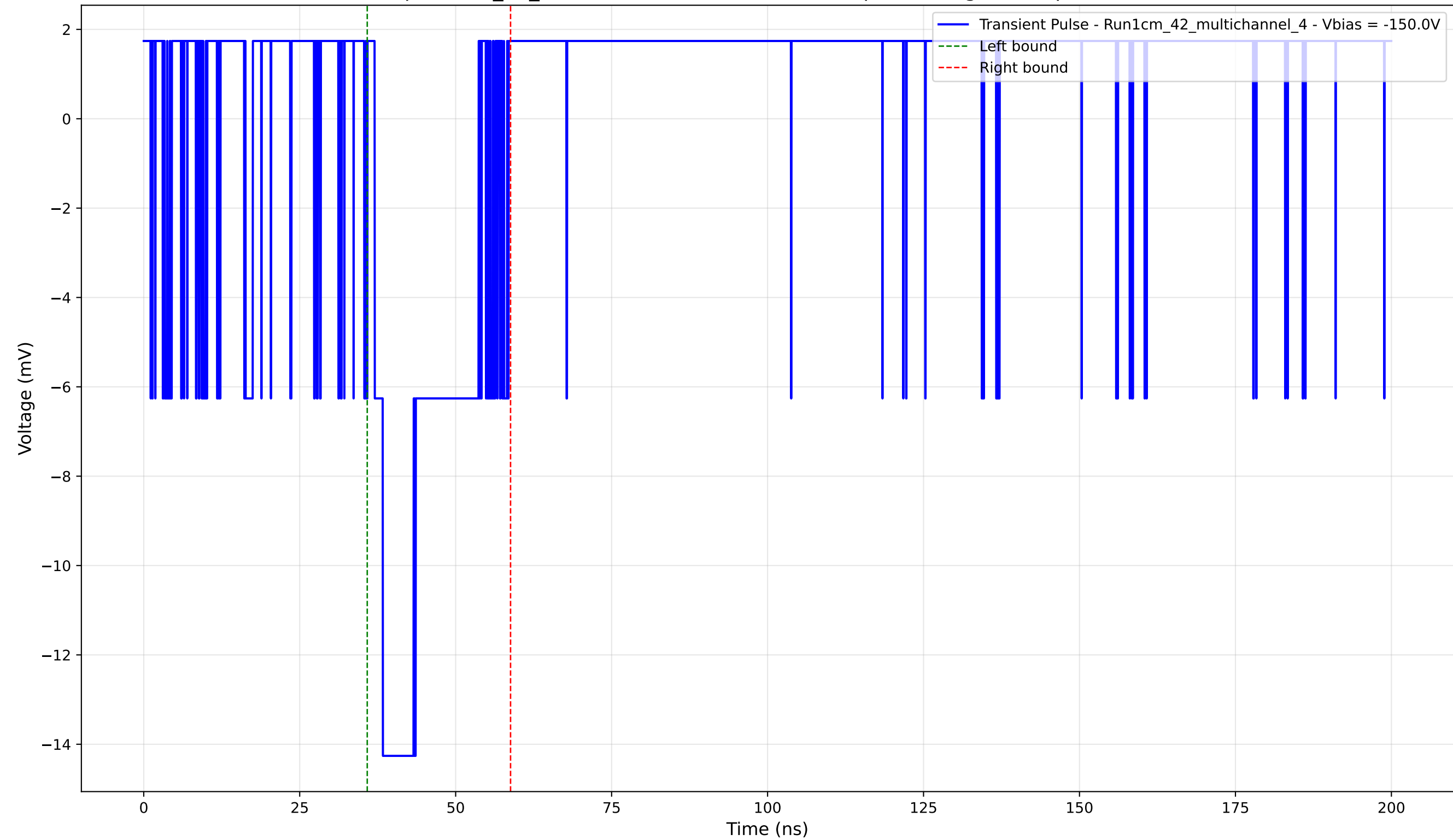
Transient Pulse - Sample: 1cm_42_multichannel - Position: 4290.0 \mu\text{m} - Charge: 3.07 pC - Rise Time: 0.00 ns (N/A)
