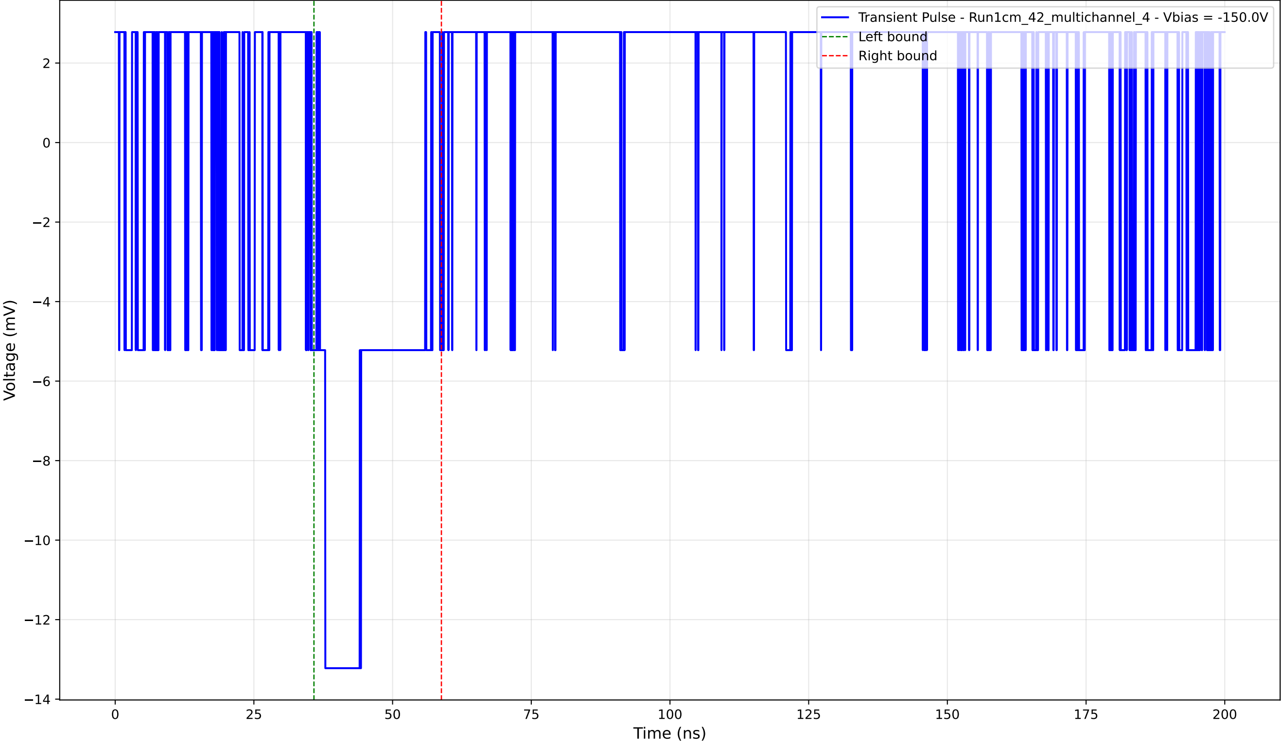
Transient Pulse - Sample: 1cm_42_multichannel - Position: 685.0 \mu\text{m} - Charge: 3.10 pC - Rise Time: 0.00 ns (N/A)
