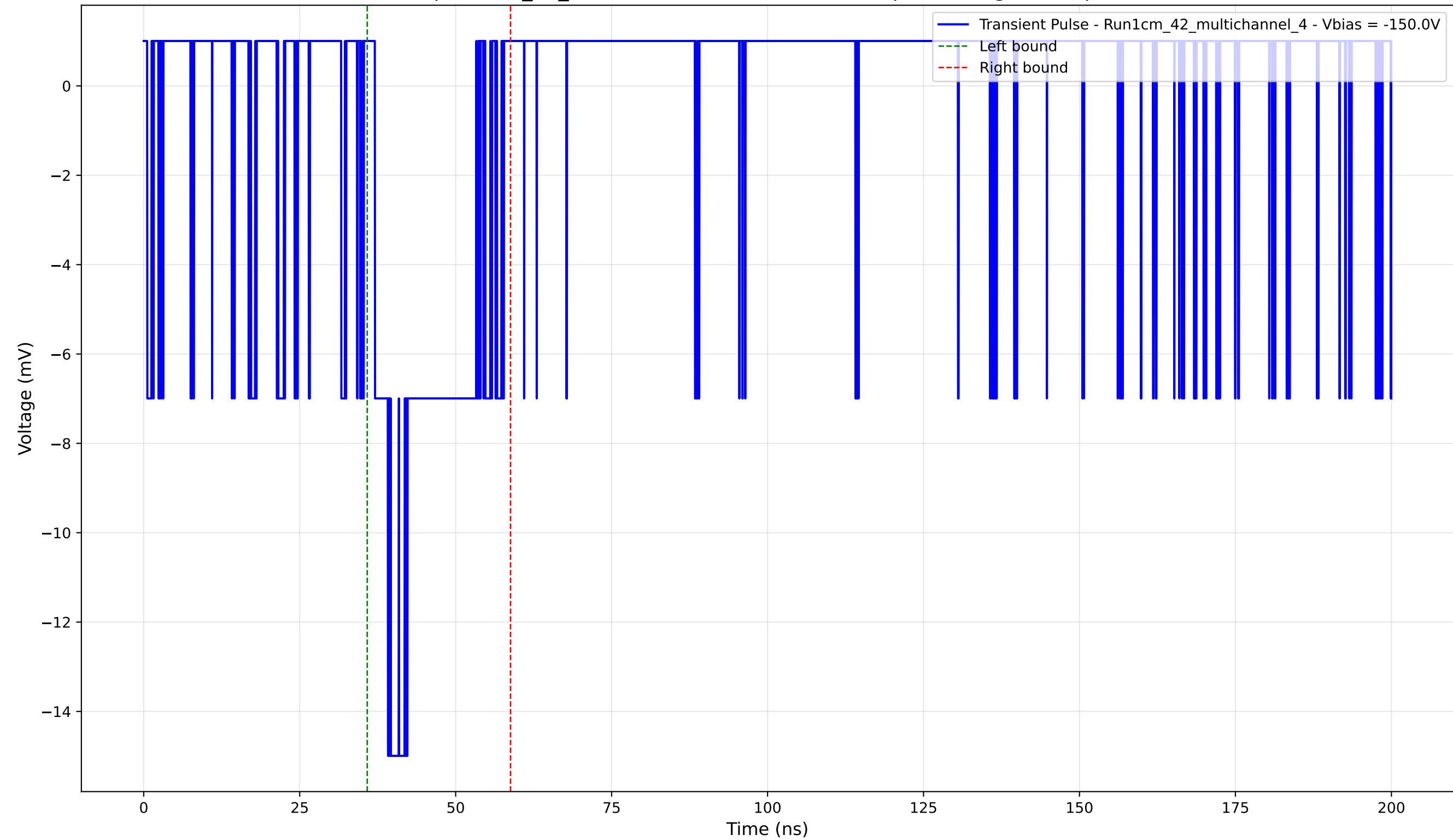
Transient Pulse - Sample: 1cm_42_multichannel - Position: 4340.0 \mu\text{m} - Charge: 2.98 pC - Rise Time: 2.10 ns
