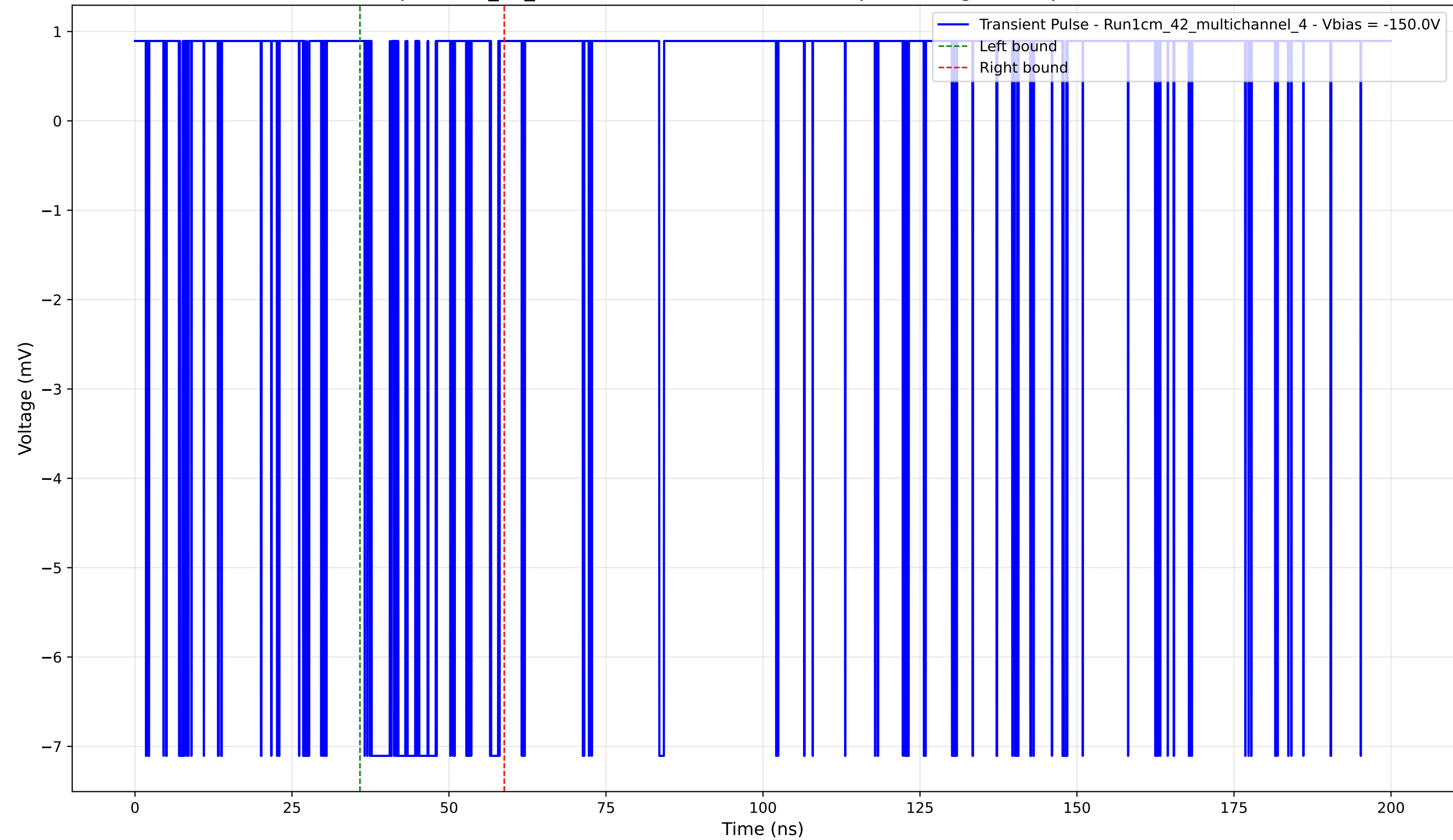
Transient Pulse - Sample: 1cm_42_multichannel - Position: 3870.0 \mu\text{m} - Charge: 1.40 pC - Rise Time: 0.00 ns (N/A)
