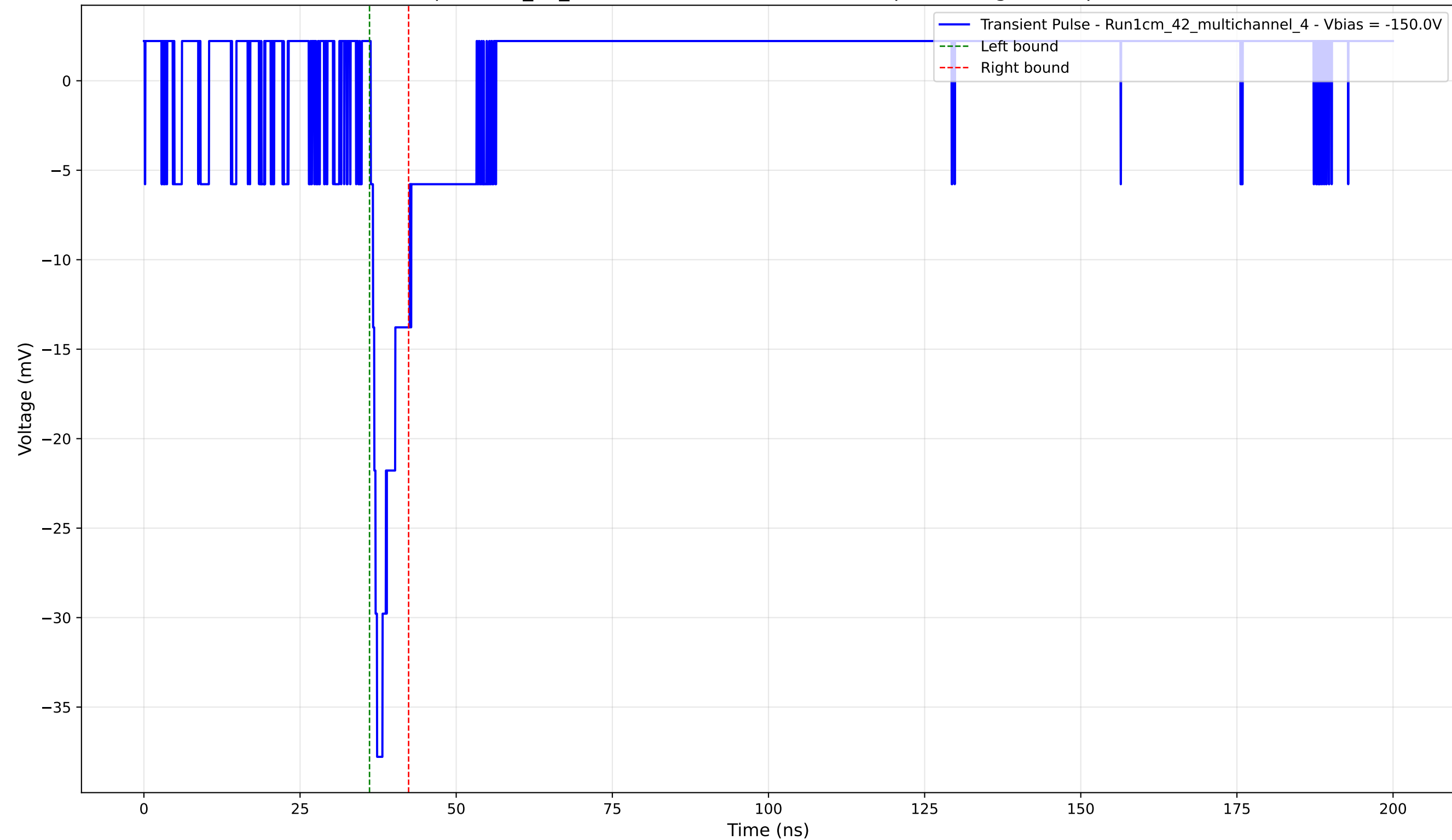
Transient Pulse - Sample: 1cm_42_multichannel - Position: 1740.0 \mu\text{m} - Charge: 2.56 pC - Rise Time: 1.01 ns
