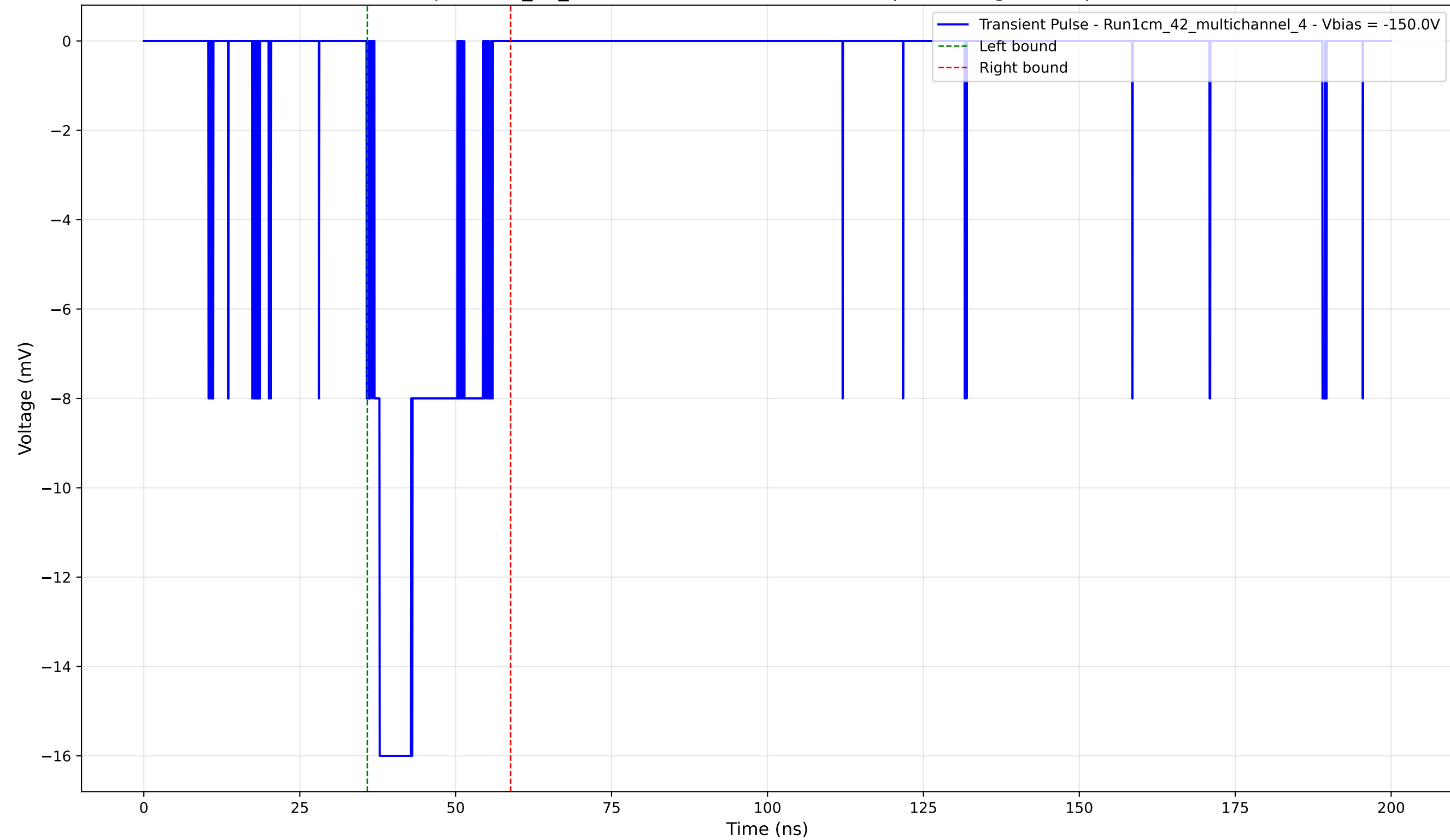
Transient Pulse - Sample: 1cm_42_multichannel - Position: 3825.0 \mu\text{m} - Charge: 3.73 pC - Rise Time: 0.84 ns
