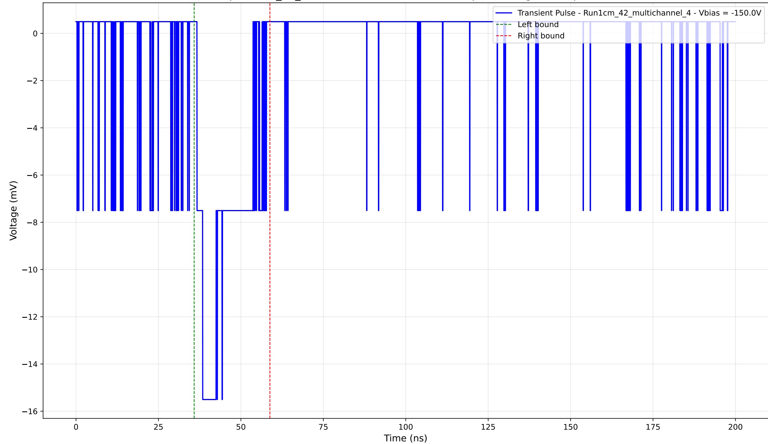
Transient Pulse - Sample: 1cm_42_multichannel - Position: 4570.0 \mu\text{m} - Charge: 3.50 pC - Rise Time: 1.74 ns
