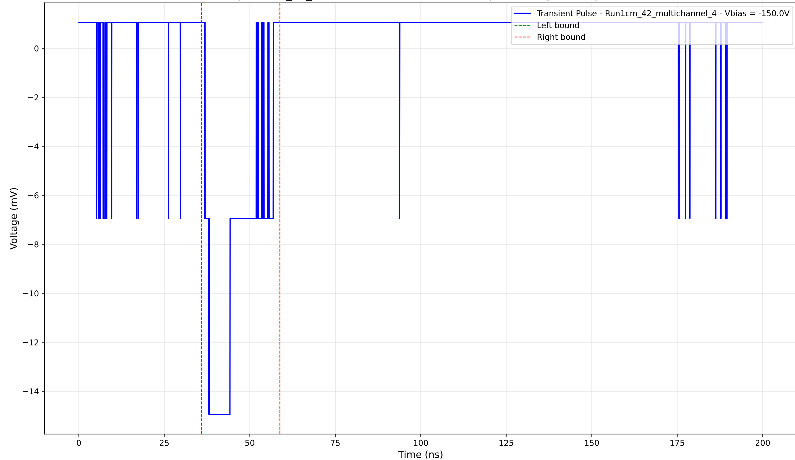
Transient Pulse - Sample: 1cm_42_multichannel - Position: 4030.0 \mu\text{m} - Charge: 3.58 pC - Rise Time: 1.12 ns
