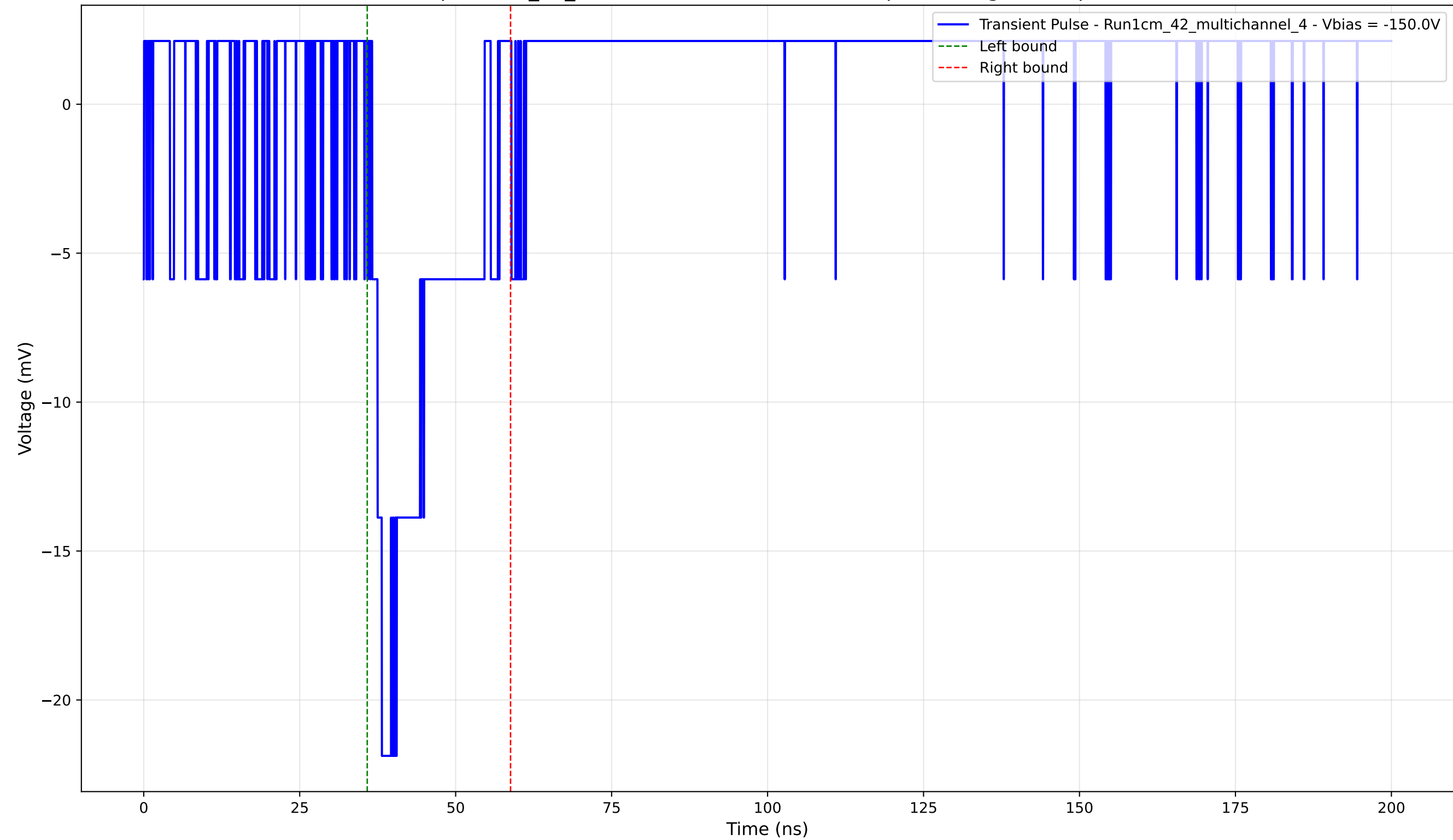
Transient Pulse - Sample: 1cm_42_multichannel - Position: 990.0 \mu\text{m} - Charge: 3.61 pC - Rise Time: 1.56 ns
