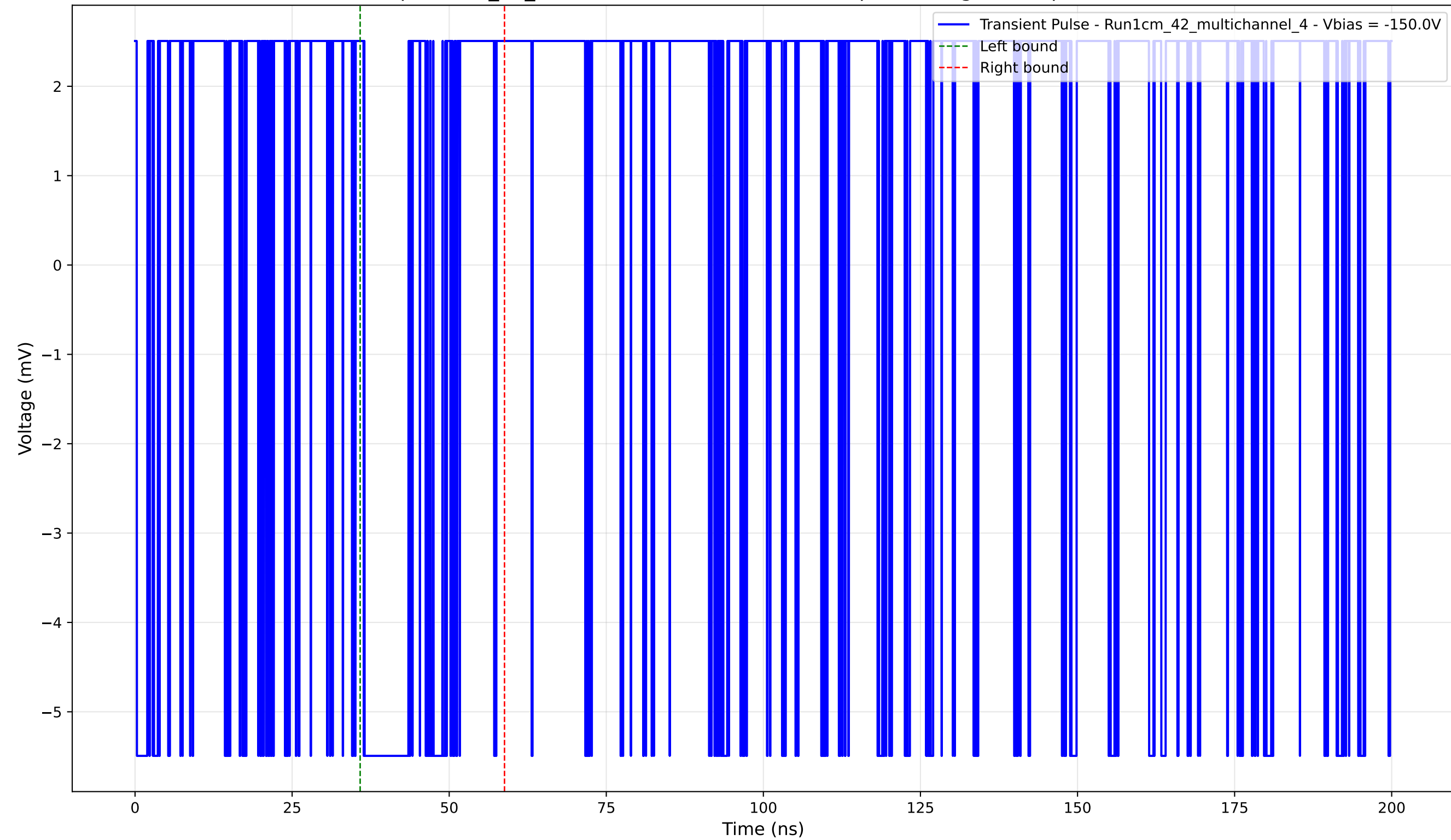
Transient Pulse - Sample: 1cm_42_multichannel - Position: 2925.0 \mu\text{m} - Charge: 0.64 pC - Rise Time: 0.00 ns (N/A)
