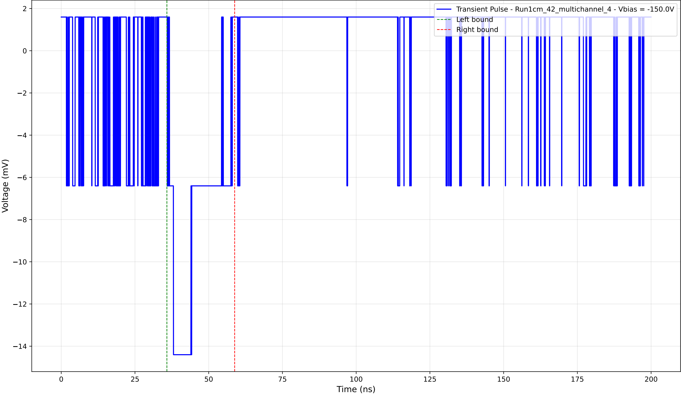
Transient Pulse - Sample: 1cm_42_multichannel - Position: 530.0 \mu\text{m} - Charge: 3.63 pC - Rise Time: 0.00 ns (N/A)
