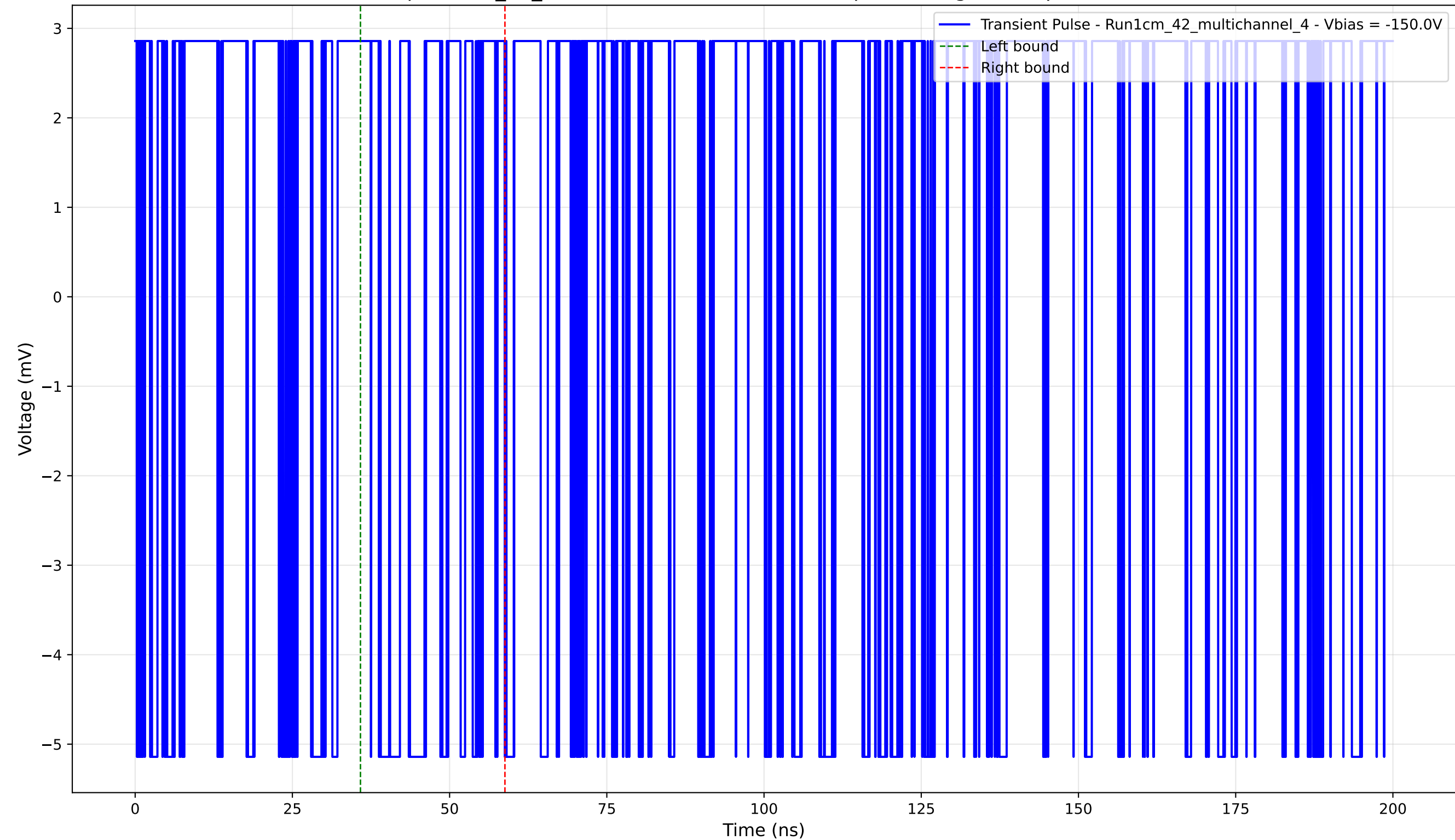
Transient Pulse - Sample: 1cm_42_multichannel - Position: 365.0 \mu\text{m} - Charge: 0.07 pC - Rise Time: 0.00 ns (N/A)
