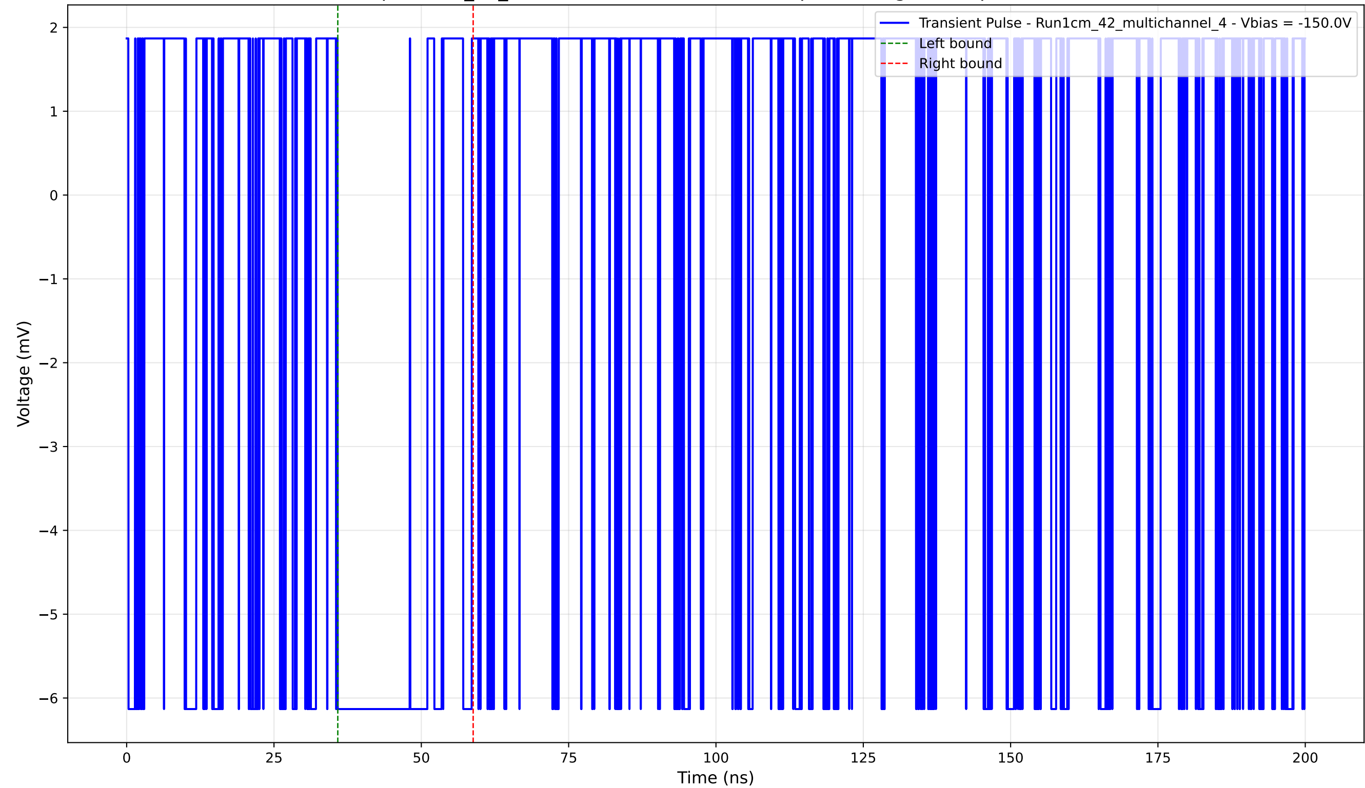
Transient Pulse - Sample: 1cm_42_multichannel - Position: 315.0 \mu\text{m} - Charge: 2.00 pC - Rise Time: 0.00 ns (N/A)
