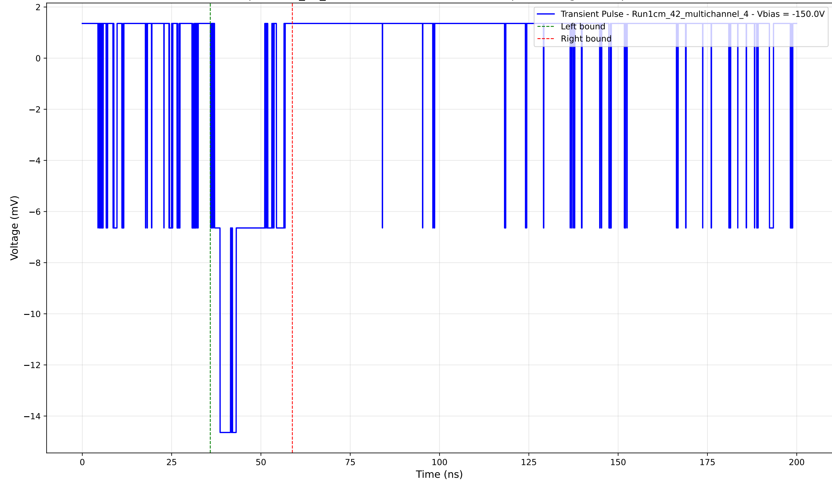
Transient Pulse - Sample: 1cm_42_multichannel - Position: 4485.0 \mu\text{m} - Charge: 2.98 pC - Rise Time: 1.56 ns
