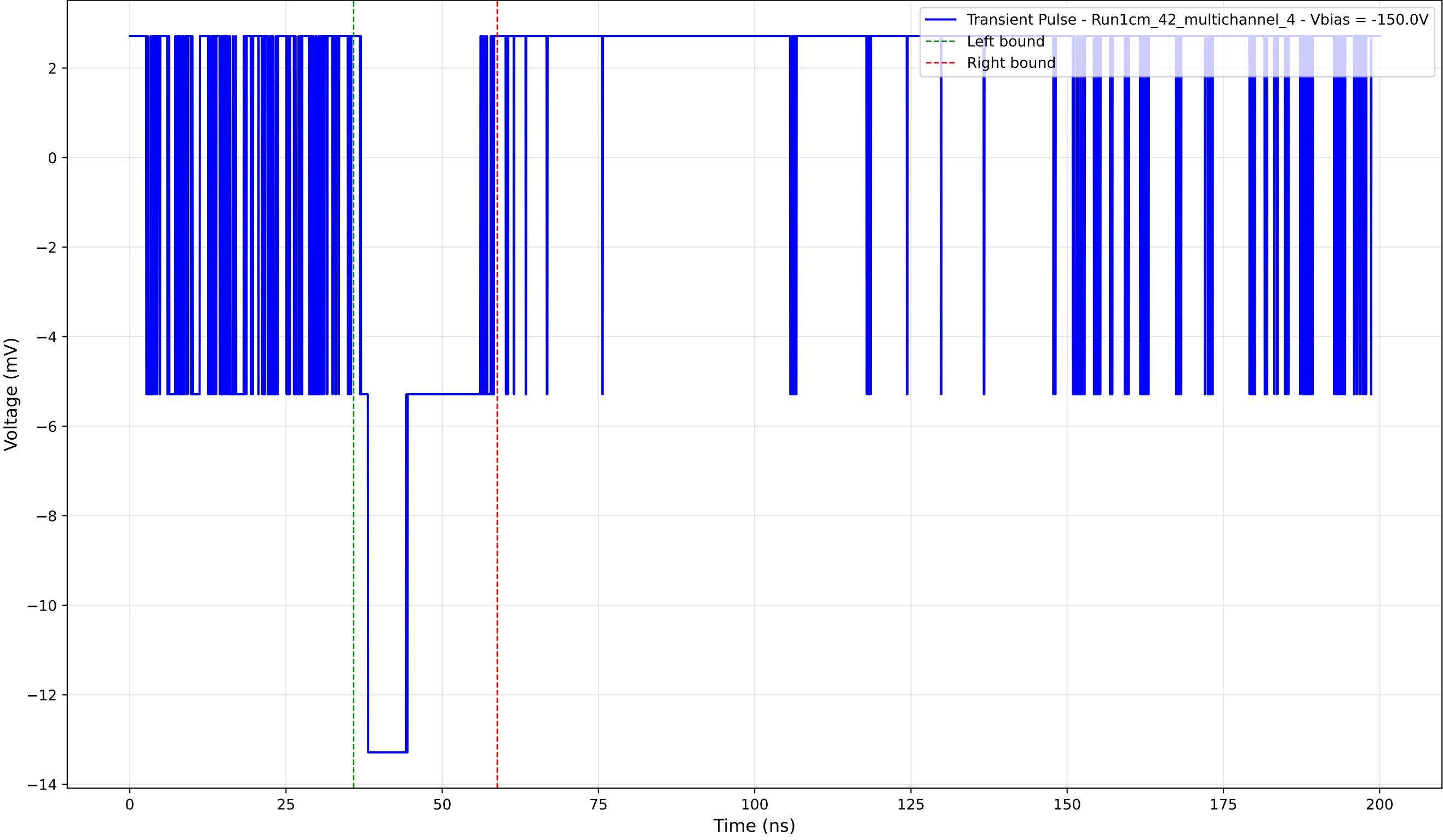
Transient Pulse - Sample: 1cm_42_multichannel - Position: 510.0 \mu\text{m} - Charge: 3.08 pC - Rise Time: 0.00 ns (N/A)
