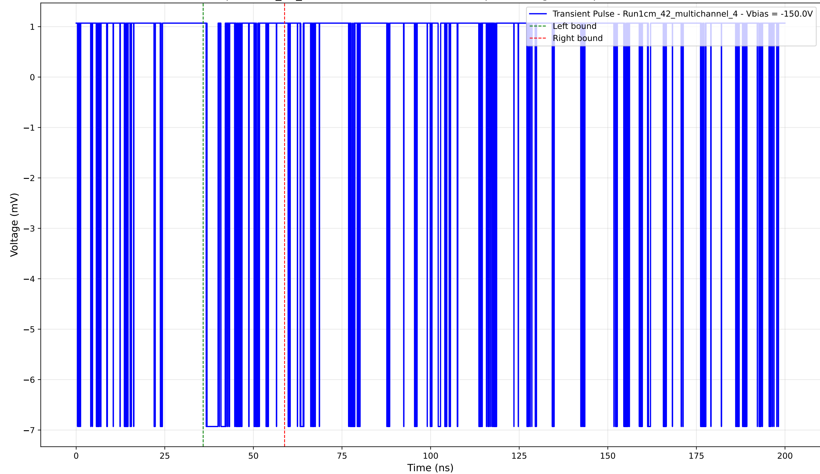
Transient Pulse - Sample: 1cm_42_multichannel - Position: 3420.0 \mu\text{m} - Charge: 0.73 pC - Rise Time: 0.00 ns (N/A)
