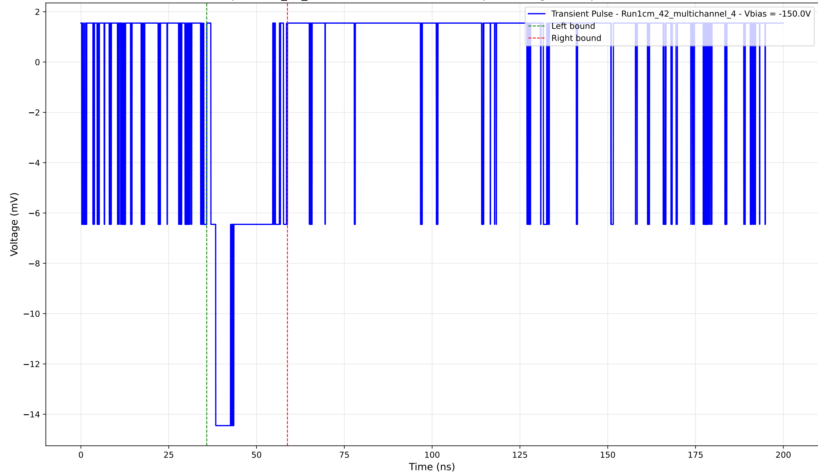
Transient Pulse - Sample: 1cm_42_multichannel - Position: 210.0 \mu\text{m} - Charge: 3.30 pC - Rise Time: 0.00 ns (N/A)
