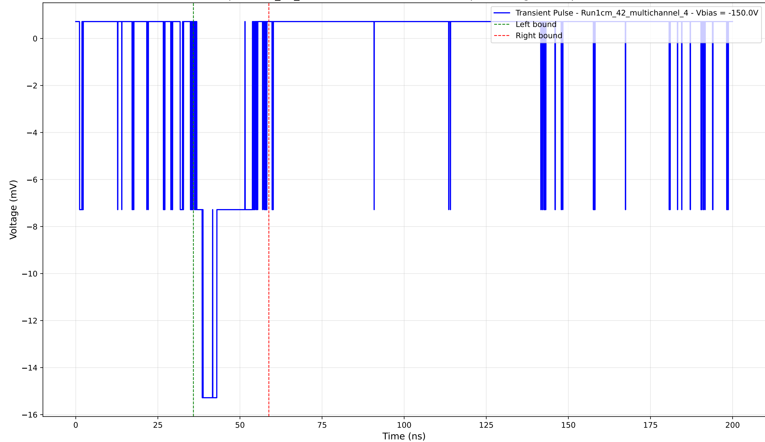
Transient Pulse - Sample: 1cm_42_multichannel - Position: 4690.0 \mu\text{m} - Charge: 3.27 pC - Rise Time: 1.66 ns
