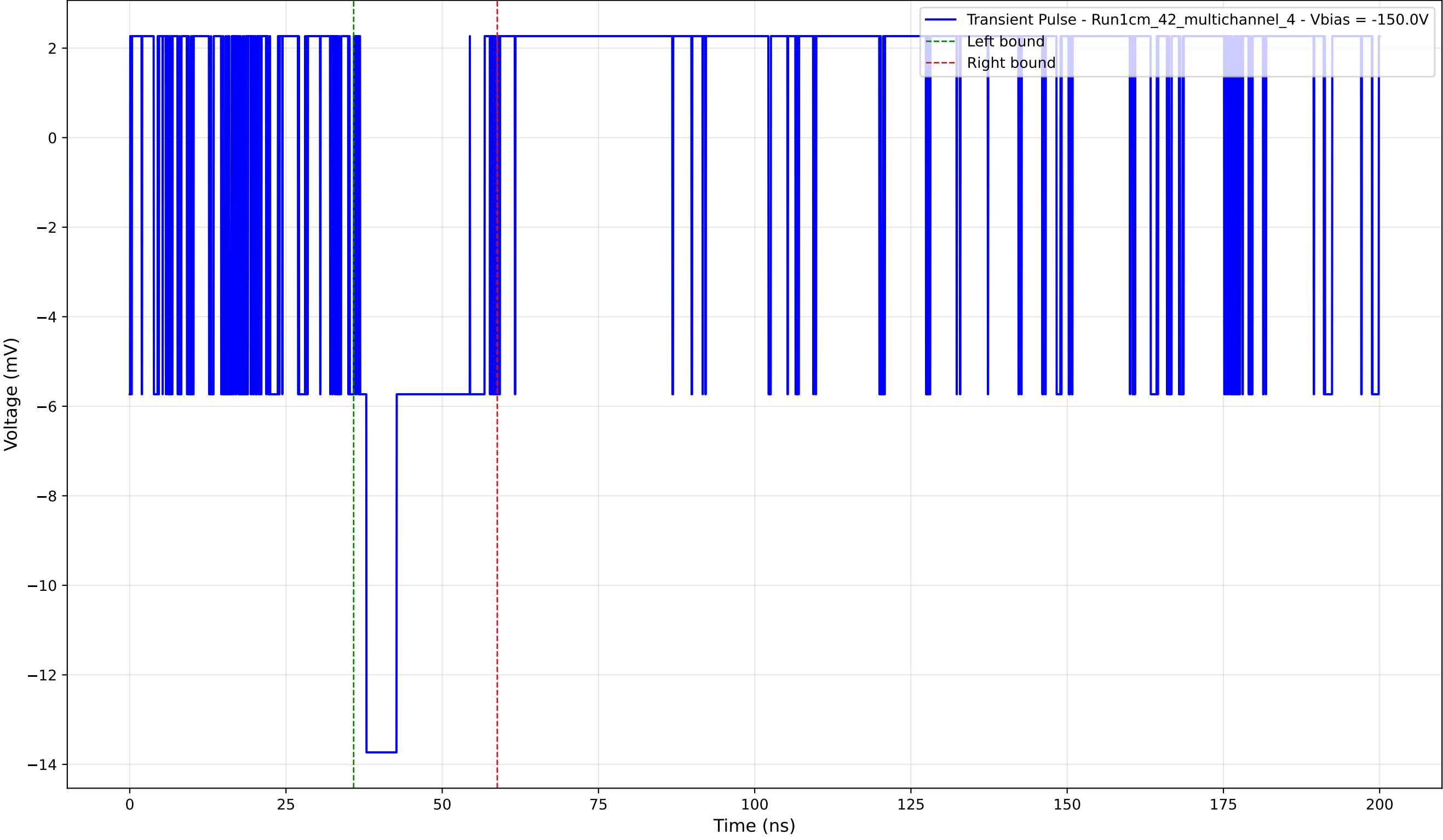
Transient Pulse - Sample: 1cm_42_multichannel - Position: 800.0 \mu\text{m} - Charge: 3.03 pC - Rise Time: 0.00 ns (N/A)
