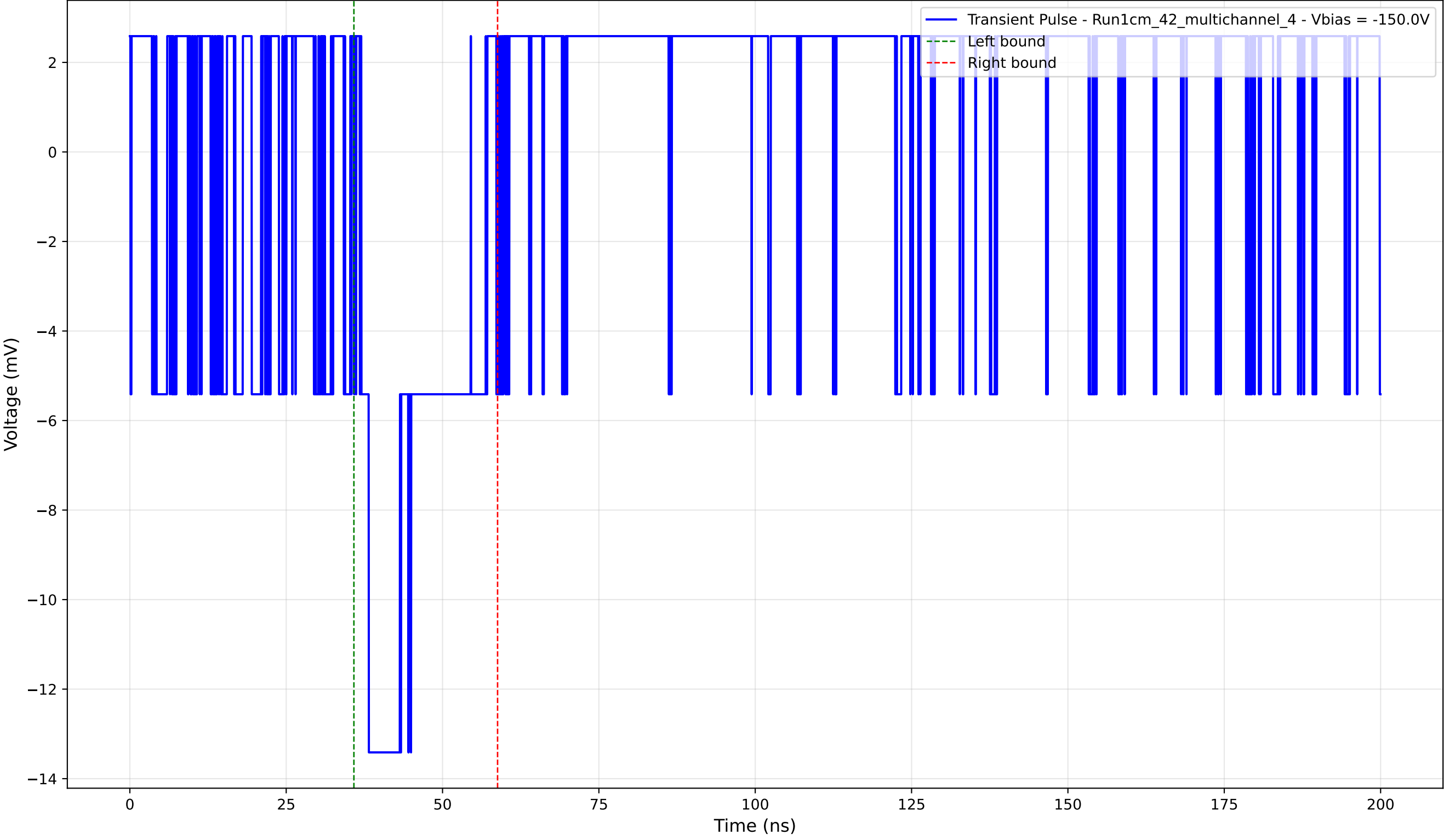
Transient Pulse - Sample: 1cm_42_multichannel - Position: 515.0 \mu\text{m} - Charge: 2.90 pC - Rise Time: 0.00 ns (N/A)
