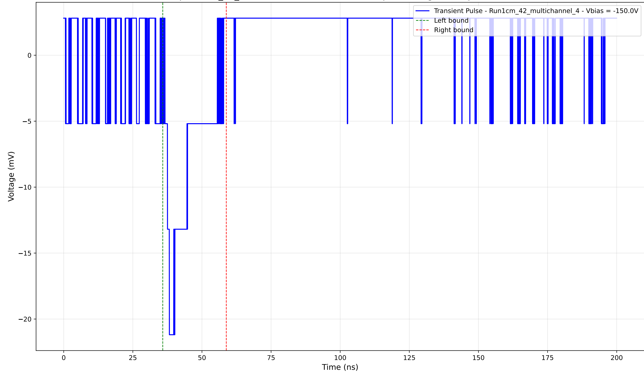
Transient Pulse - Sample: 1cm_42_multichannel - Position: 1020.0 \mu\text{m} - Charge: 3.43 pC - Rise Time: 0.00 ns (N/A)
