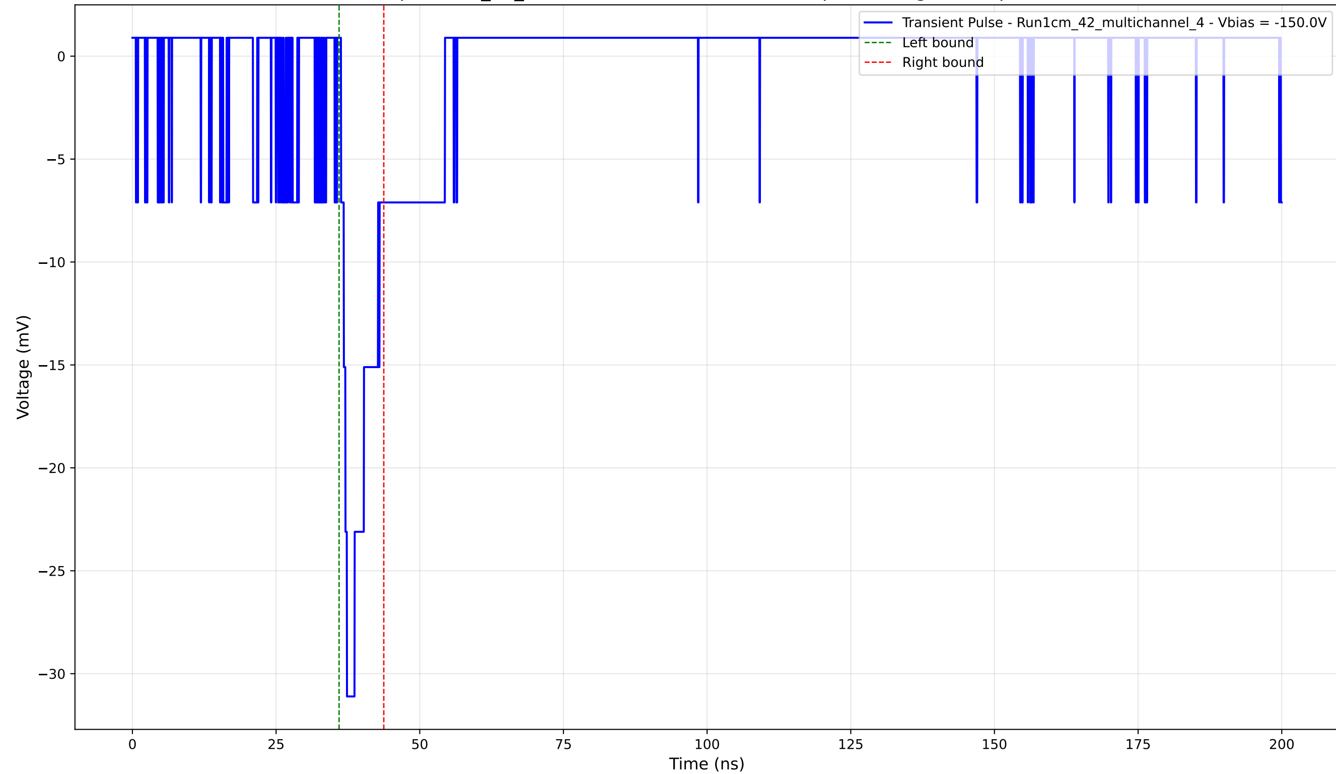
Transient Pulse - Sample: 1cm_42_multichannel - Position: 1620.0 \mu\text{m} - Charge: 2.75 pC - Rise Time: 1.03 ns
