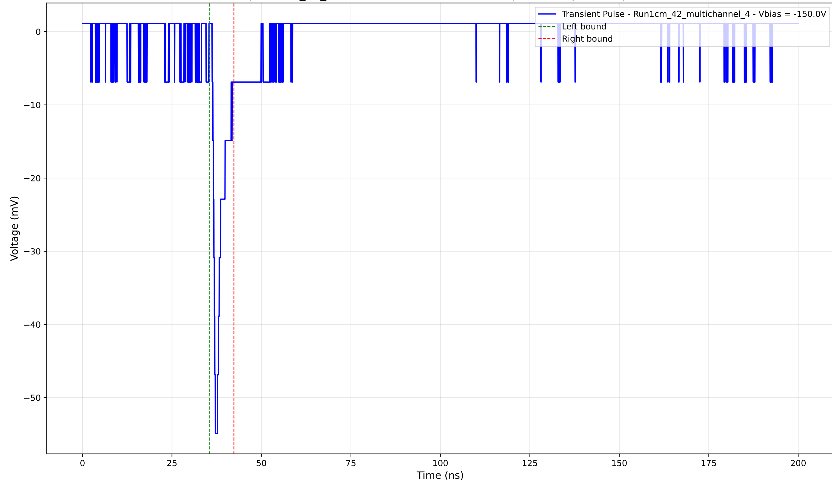
Transient Pulse - Sample: 1cm_42_multichannel - Position: 2700.0 \mu\text{m} - Charge: 2.96 pC - Rise Time: 0.90 ns
