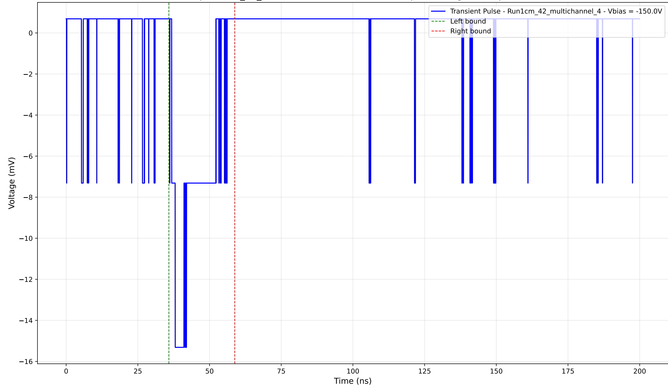
Transient Pulse - Sample: 1cm_42_multichannel - Position: 3840.0 \mu\text{m} - Charge: 2.78 pC - Rise Time: 1.24 ns
