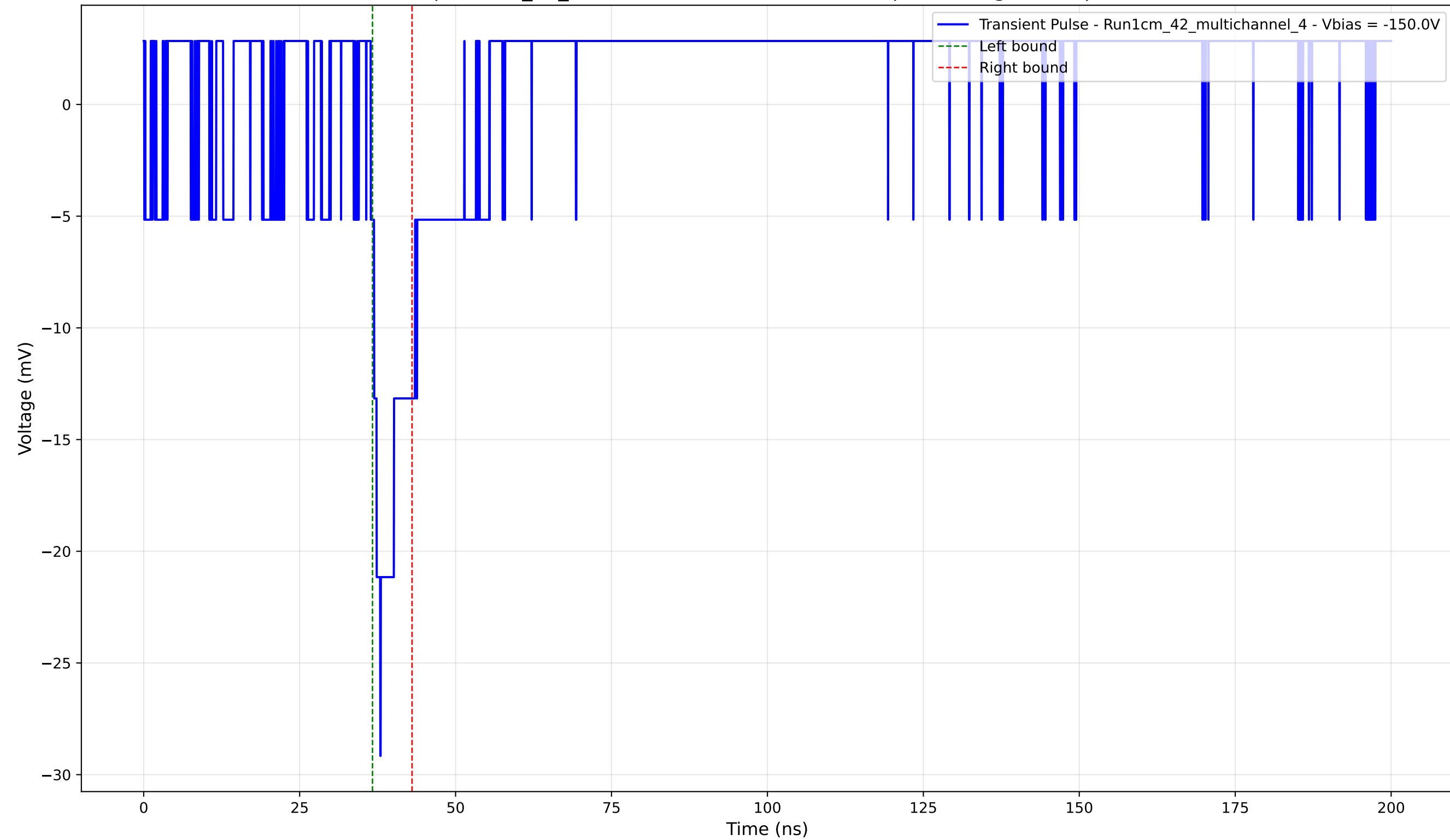
Transient Pulse - Sample: 1cm_42_multichannel - Position: 1450.0 \mu\text{m} - Charge: 2.09 pC - Rise Time: 1.54 ns
