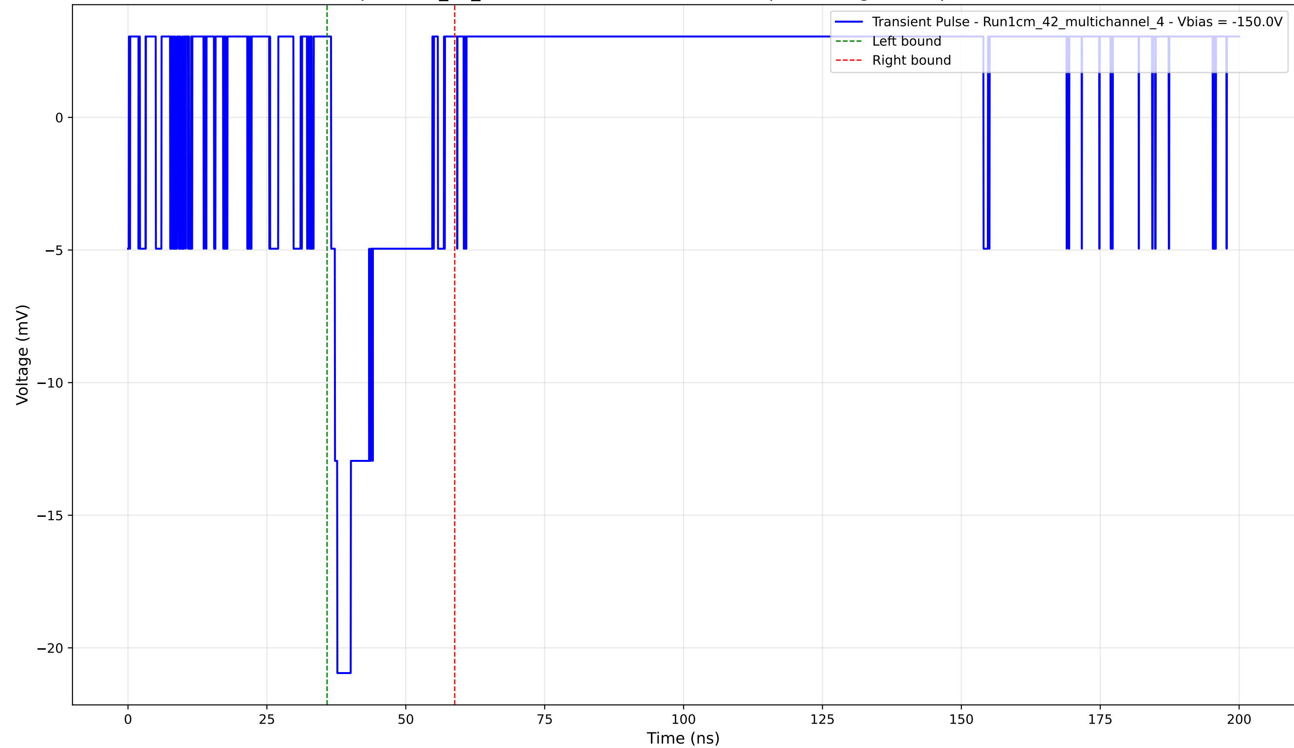
Transient Pulse - Sample: 1cm_42_multichannel - Position: 1250.0 \mu\text{m} - Charge: 3.15 pC - Rise Time: 0.00 ns (N/A)
