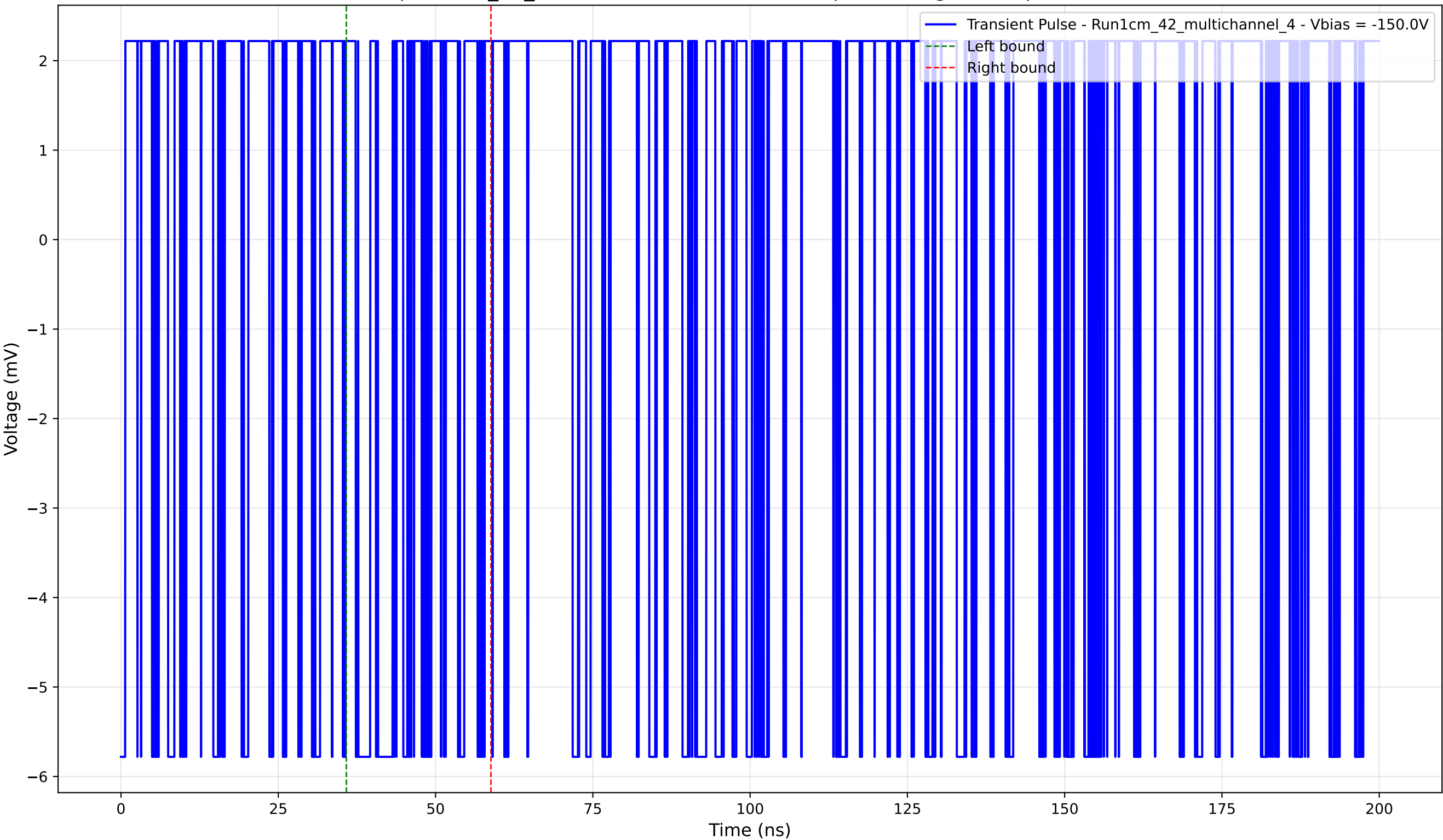
Transient Pulse - Sample: 1cm_42_multichannel - Position: 65.0 \mu\text{m} - Charge: 0.42 pC - Rise Time: 0.00 ns (N/A)
