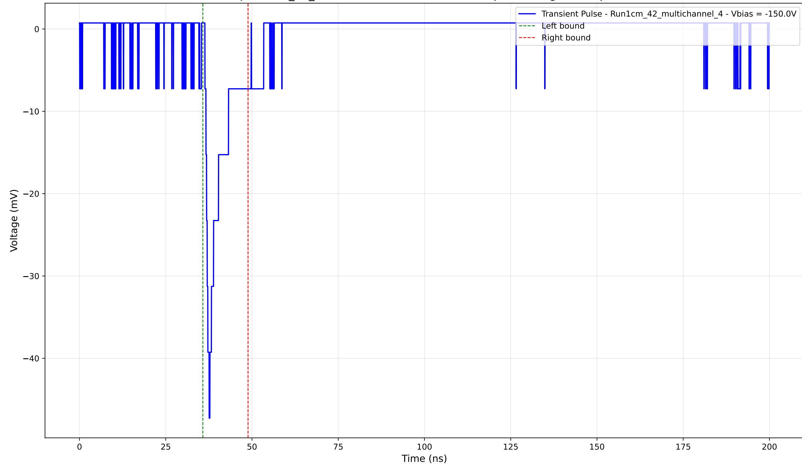
Transient Pulse - Sample: 1cm_42_multichannel - Position: 1780.0 \mu\text{m} - Charge: 3.91 pC - Rise Time: 1.23 ns
