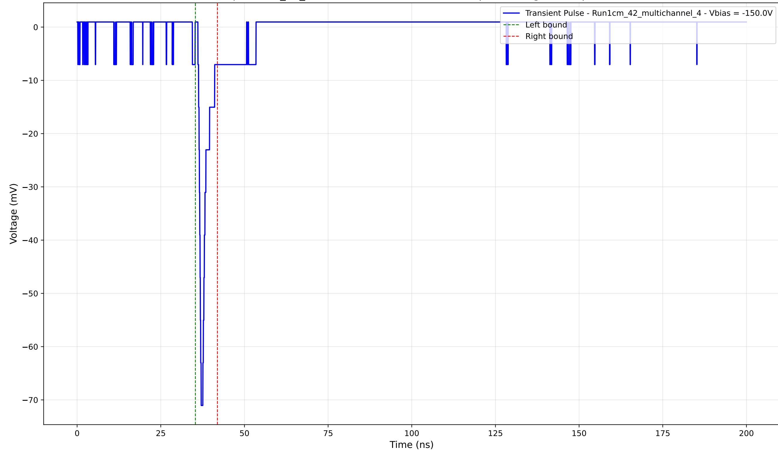
Transient Pulse - Sample: 1cm_42_multichannel - Position: 2220.0 \mu\text{m} - Charge: 3.22 pC - Rise Time: 0.78 ns
