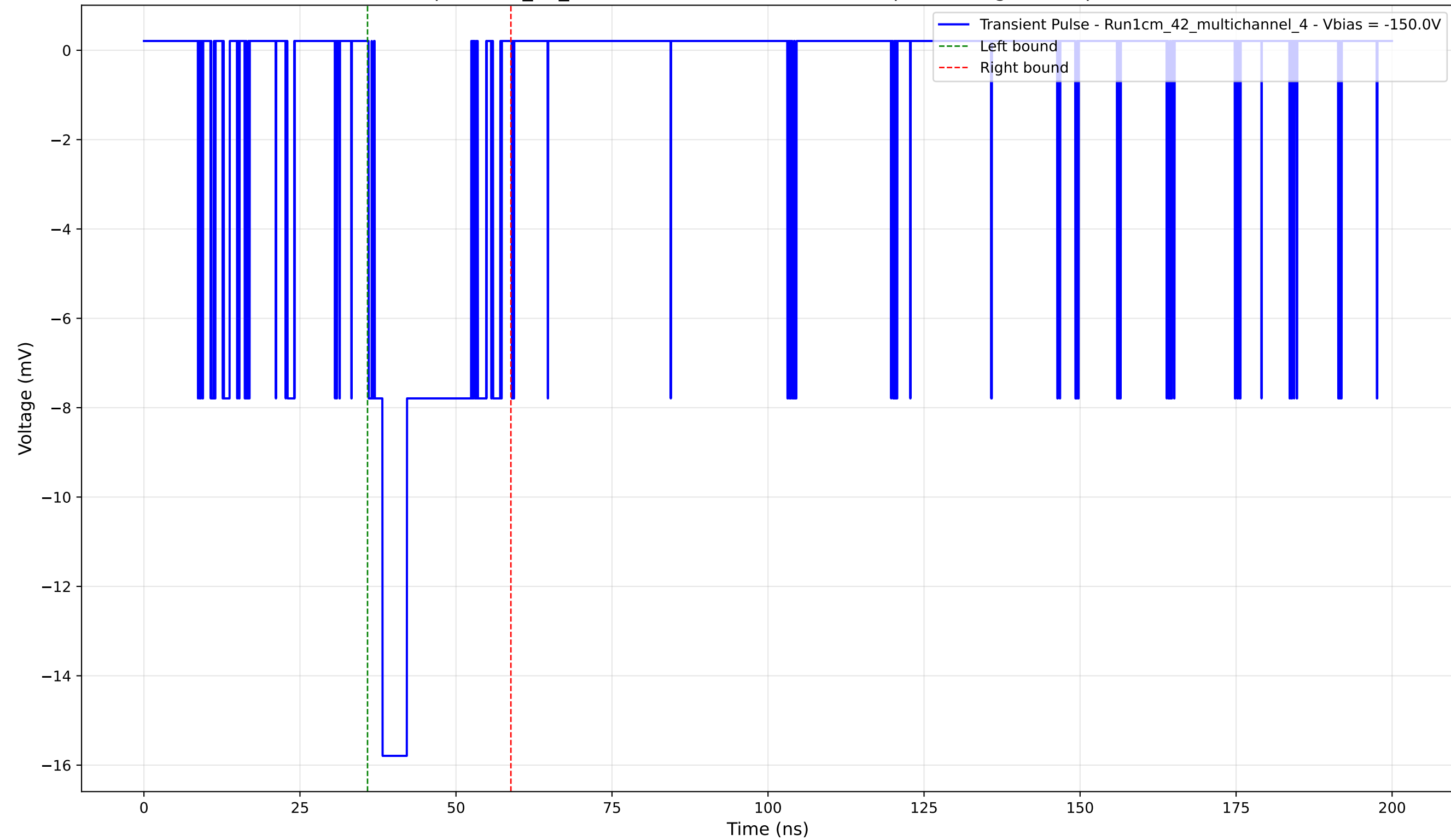
Transient Pulse - Sample: 1cm_42_multichannel - Position: 4745.0 \mu\text{m} - Charge: 3.66 pC - Rise Time: 1.26 ns
