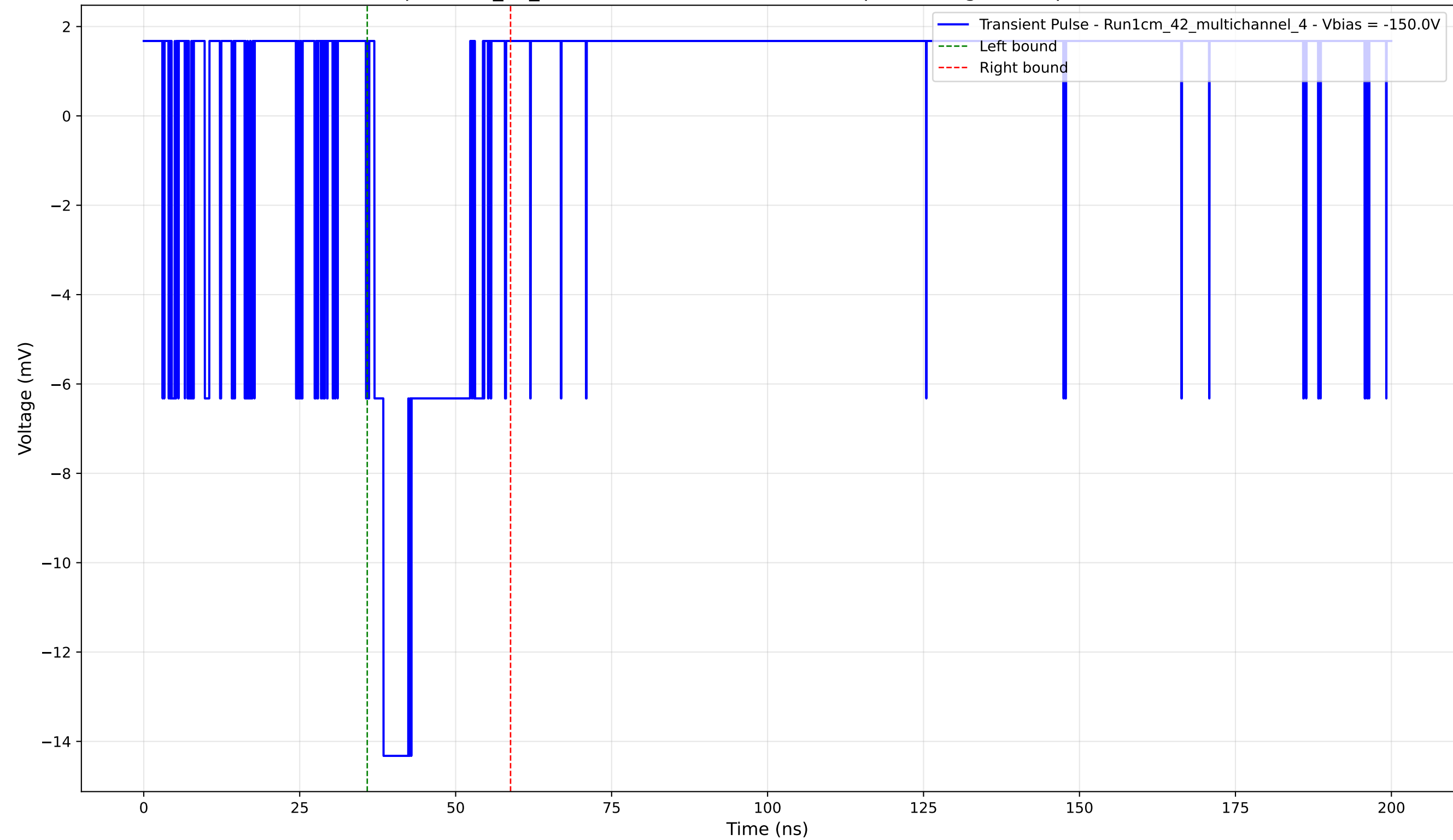
Transient Pulse - Sample: 1cm_42_multichannel - Position: 4675.0 \mu\text{m} - Charge: 2.70 pC - Rise Time: 0.00 ns (N/A)
