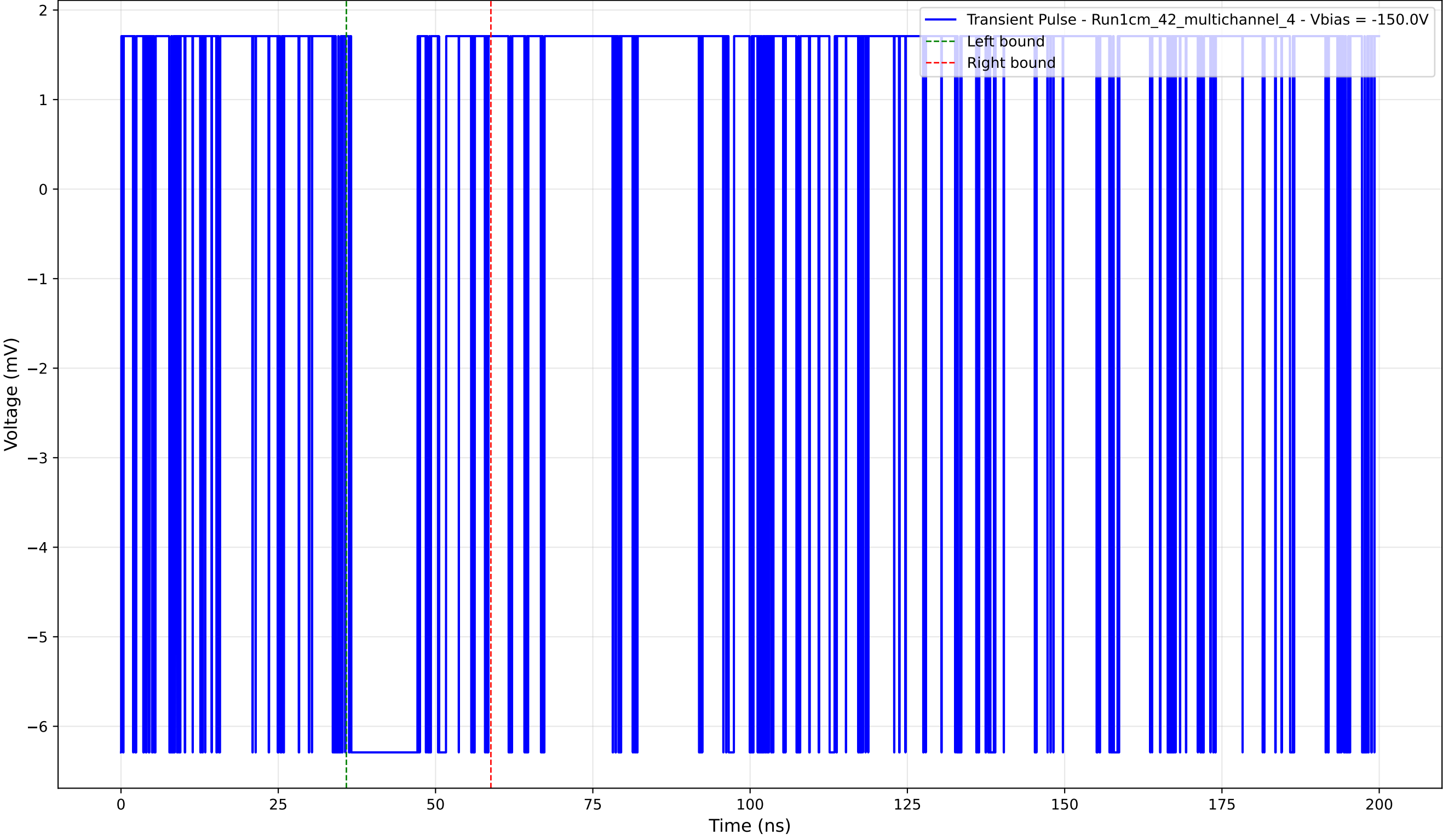
Transient Pulse - Sample: 1cm_42_multichannel - Position: 3360.0 \mu\text{m} - Charge: 1.34 pC - Rise Time: 0.00 ns (N/A)
