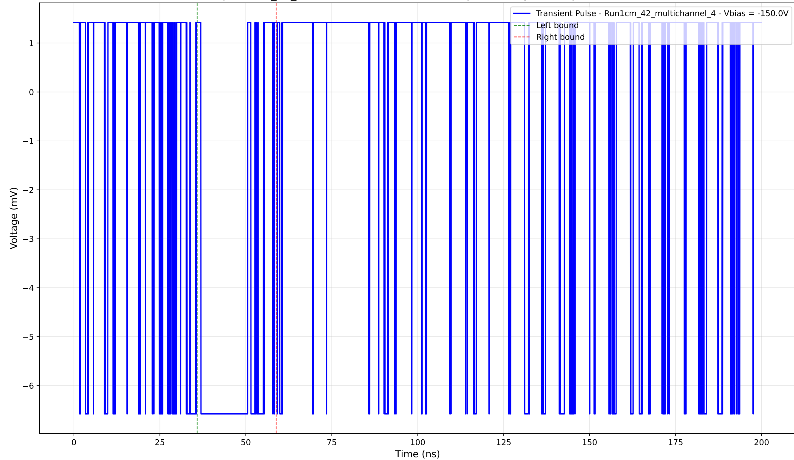
Transient Pulse - Sample: 1cm_42_multichannel - Position: 105.0 \mu\text{m} - Charge: 2.11 pC - Rise Time: 0.00 ns (N/A)
