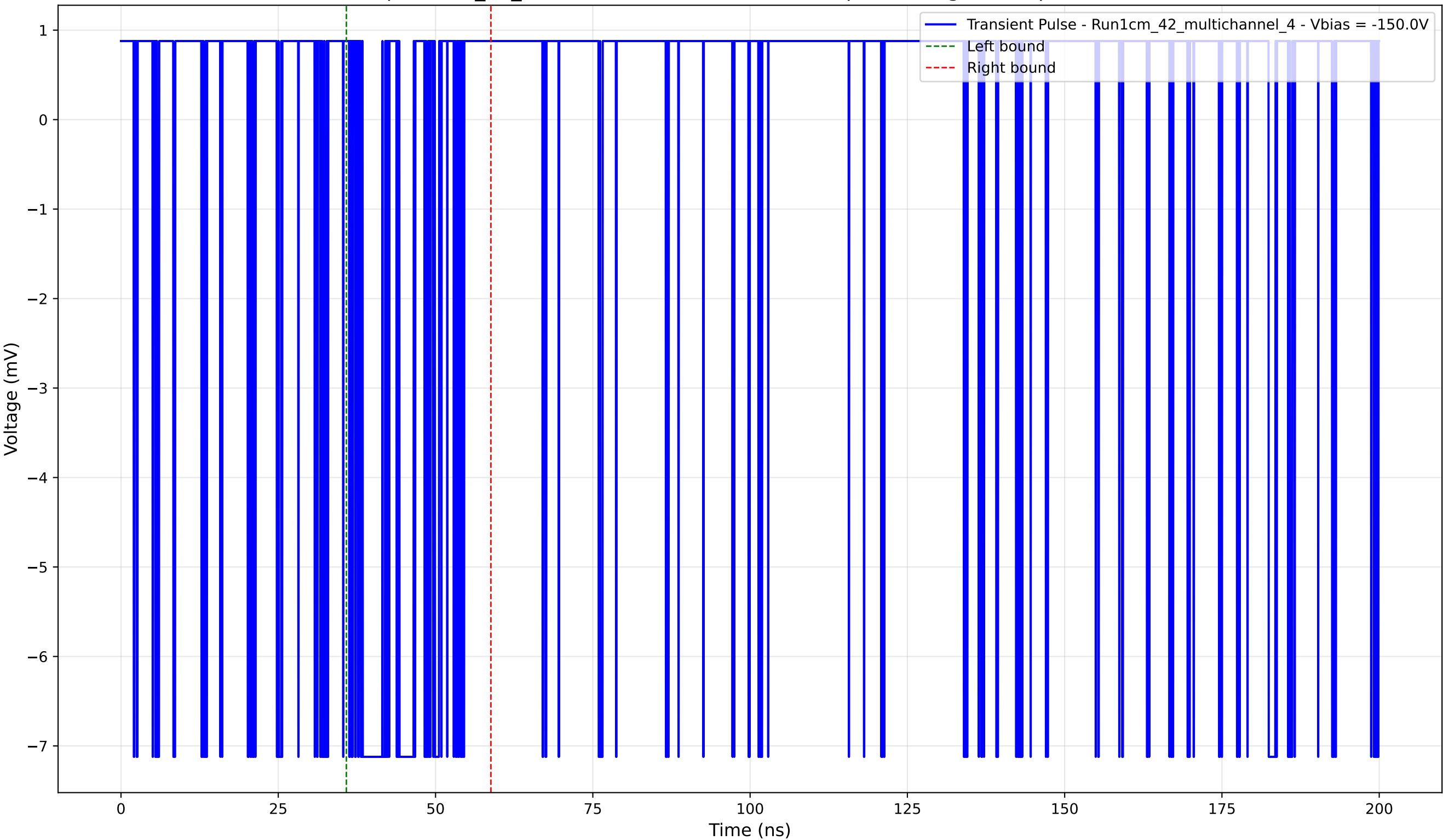
Transient Pulse - Sample: 1cm_42_multichannel - Position: 4875.0 \mu\text{m} - Charge: 1.07 pC - Rise Time: 0.00 ns (N/A)
