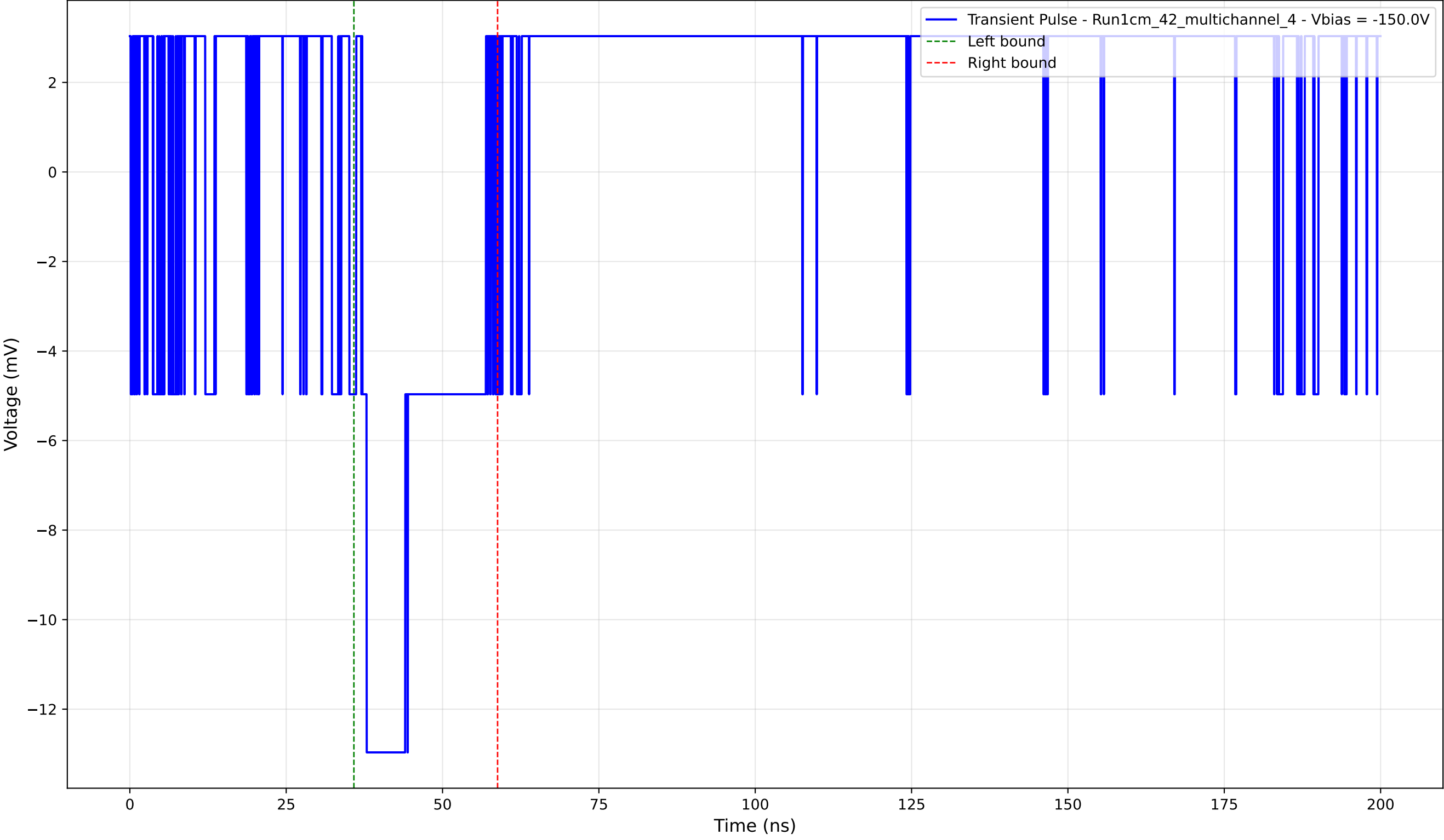
Transient Pulse - Sample: 1cm_42_multichannel - Position: 700.0 \mu\text{m} - Charge: 2.94 pC - Rise Time: 0.00 ns (N/A)
