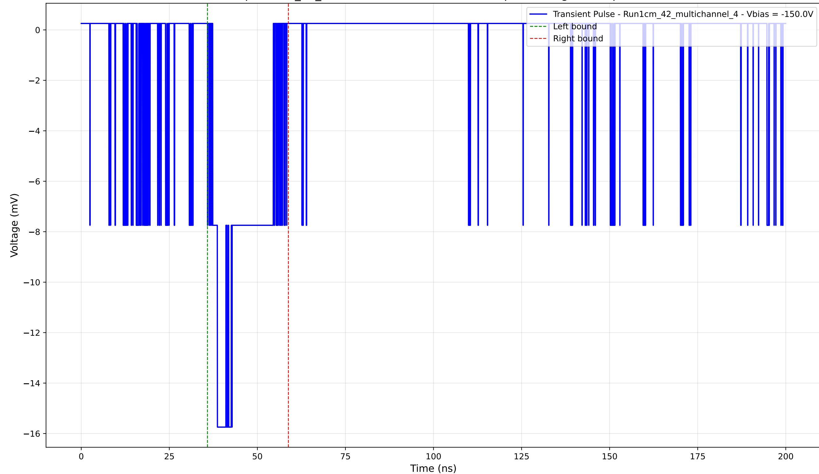
Transient Pulse - Sample: 1cm_42_multichannel - Position: 4475.0 \mu\text{m} - Charge: 3.48 pC - Rise Time: 1.34 ns
