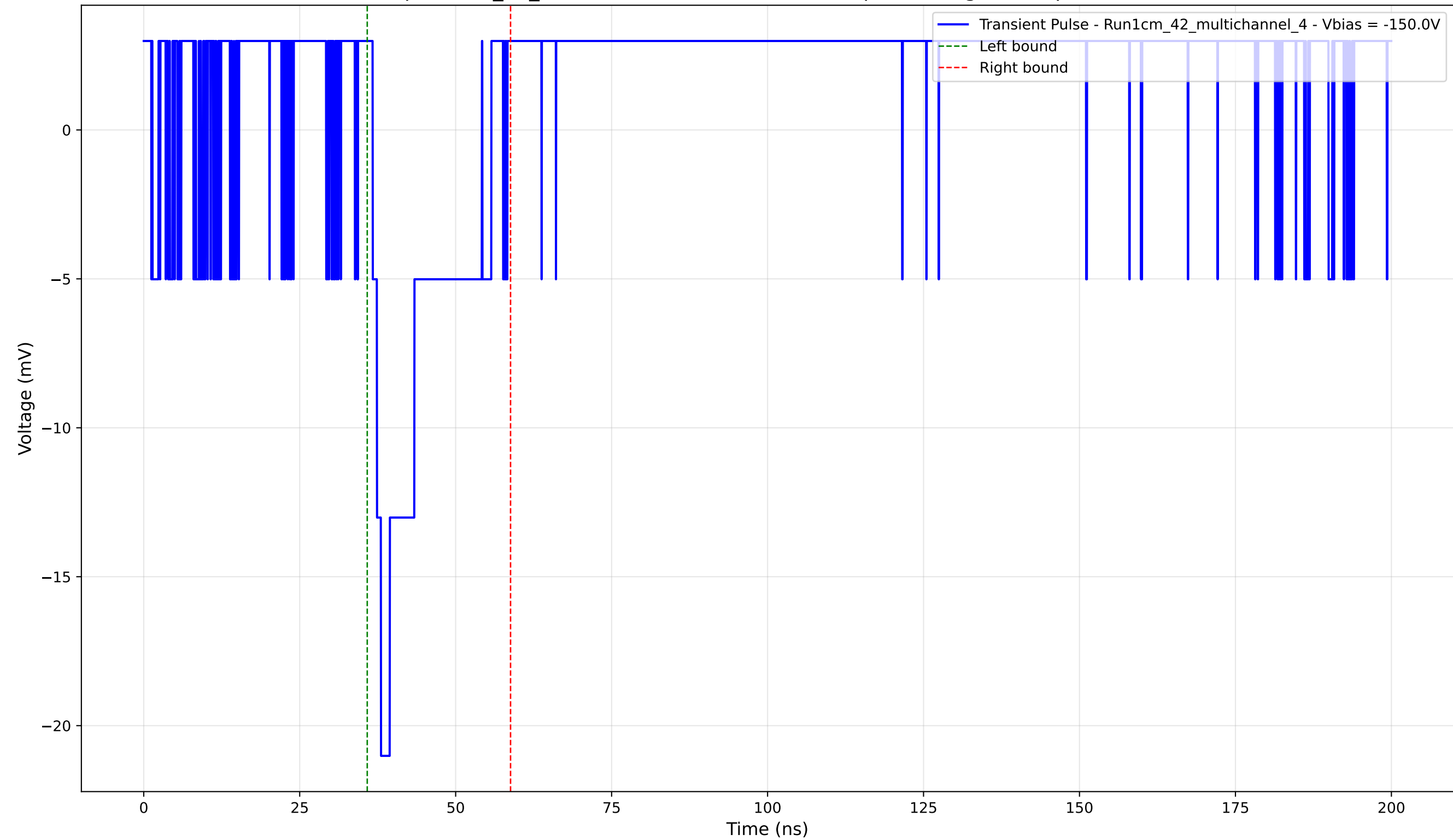
Transient Pulse - Sample: 1cm_42_multichannel - Position: 1140.0 \mu\text{m} - Charge: 2.94 pC - Rise Time: 0.00 ns (N/A)
