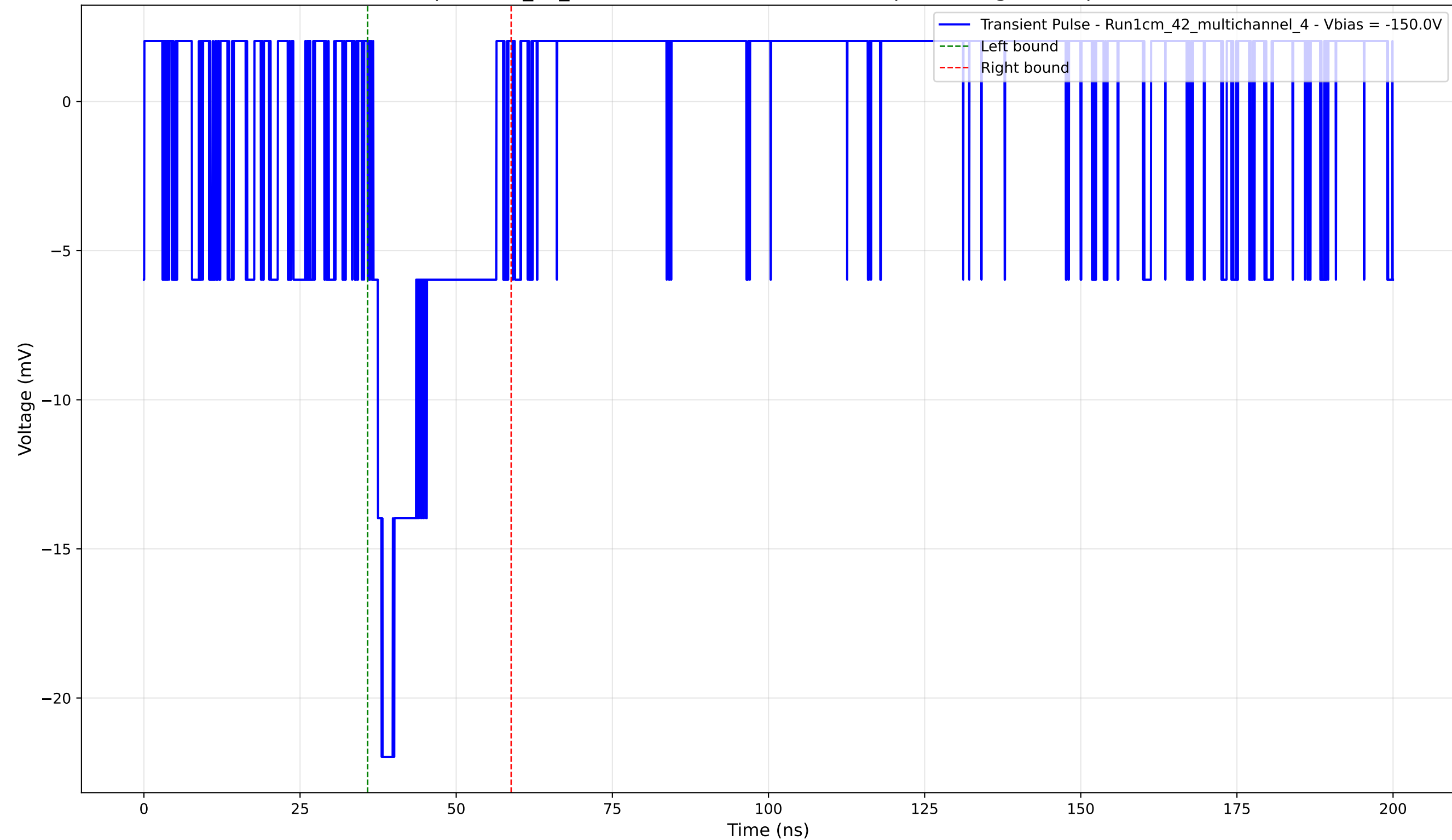
Transient Pulse - Sample: 1cm_42_multichannel - Position: 1045.0 \mu\text{m} - Charge: 3.78 pC - Rise Time: 1.32 ns
