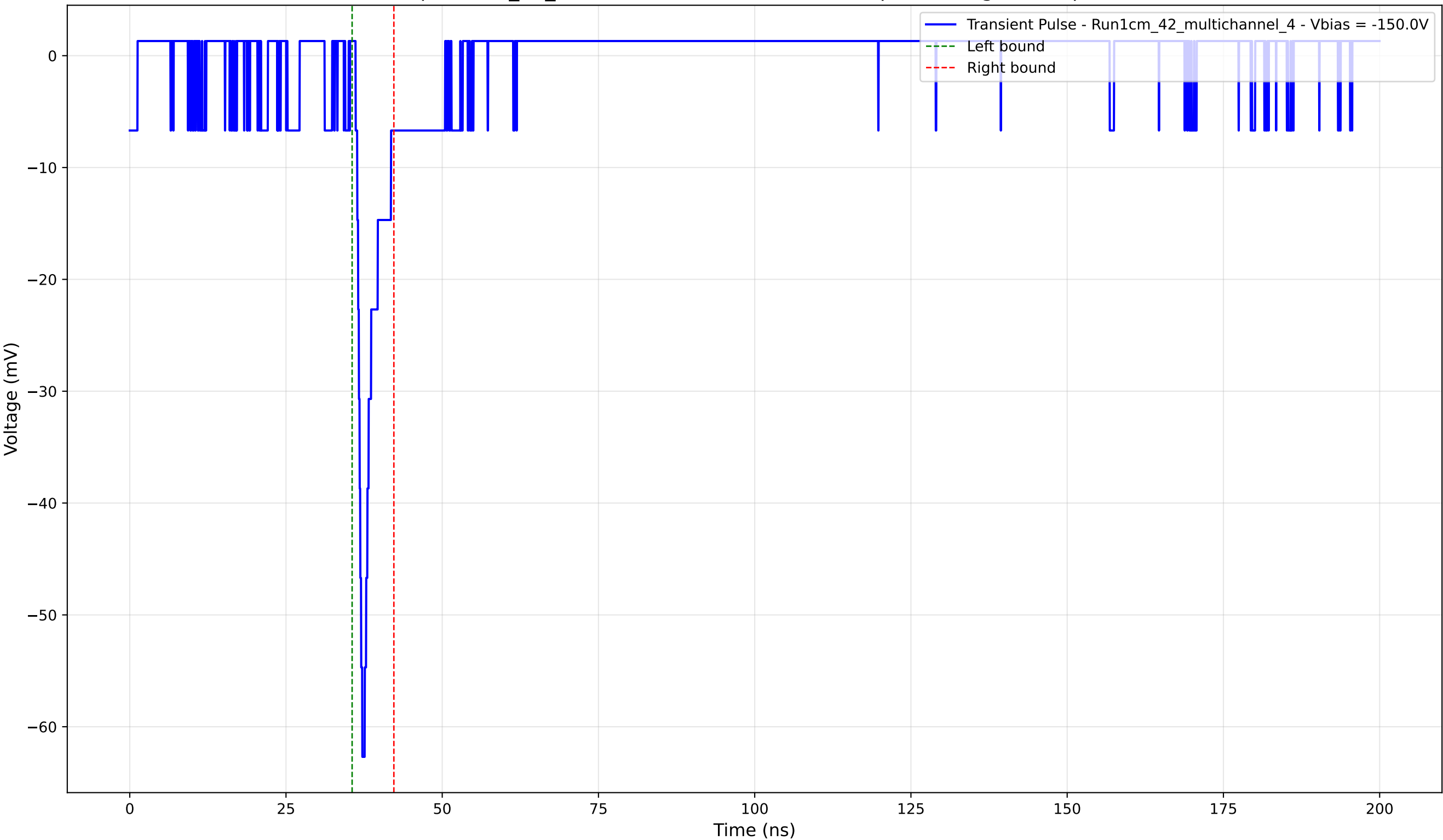
Transient Pulse - Sample: 1cm_42_multichannel - Position: 2100.0 \mu\text{m} - Charge: 3.09 pC - Rise Time: 1.06 ns
