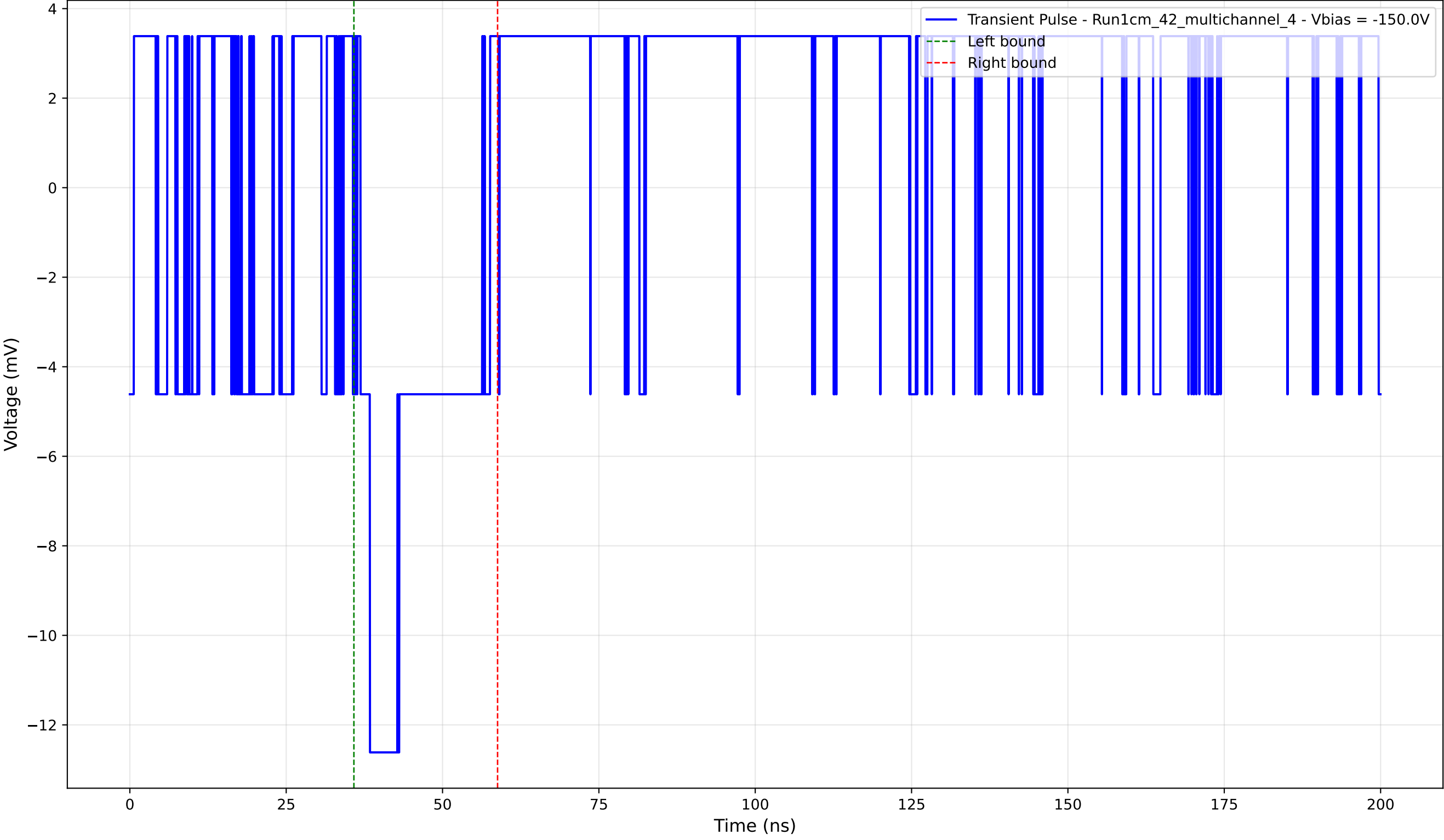
Transient Pulse - Sample: 1cm_42_multichannel - Position: 245.0 \mu\text{m} - Charge: 2.50 pC - Rise Time: 0.00 ns (N/A)
