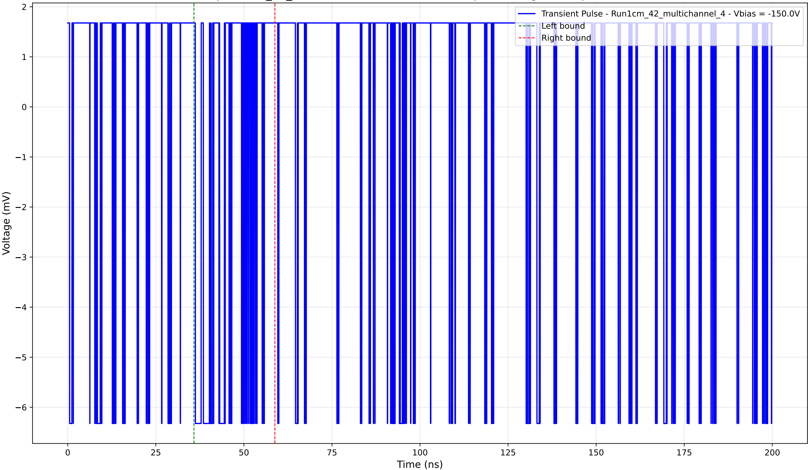
Transient Pulse - Sample: 1cm_42_multichannel - Position: 2885.0 \mu\text{m} - Charge: 0.54 pC - Rise Time: 0.00 ns (N/A)
