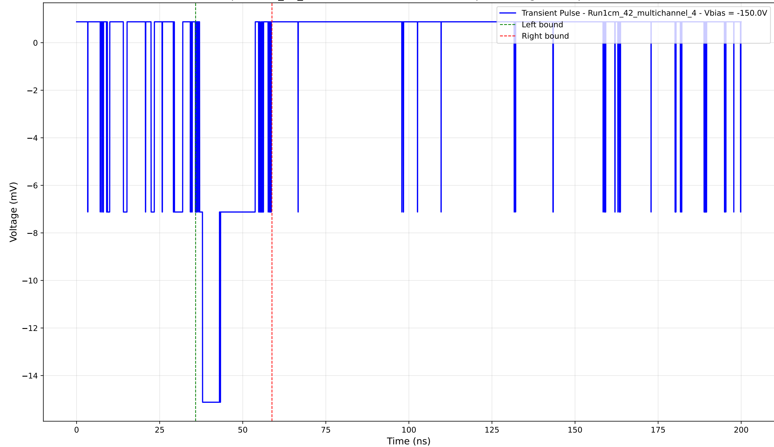
Transient Pulse - Sample: 1cm_42_multichannel - Position: 4015.0 \mu\text{m} - Charge: 3.34 pC - Rise Time: 0.90 ns
