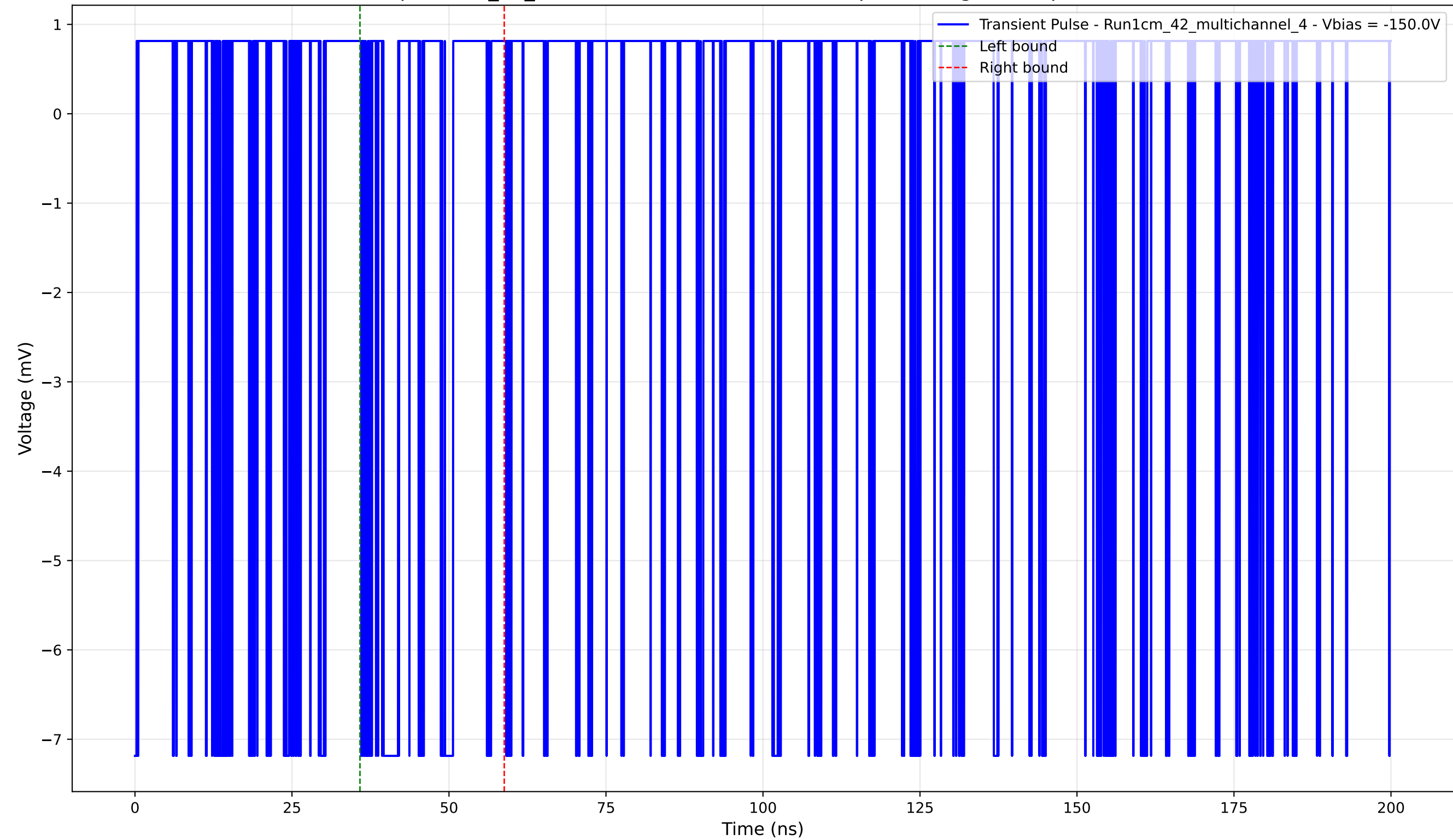
Transient Pulse - Sample: 1cm_42_multichannel - Position: 4405.0 \mu\text{m} - Charge: 0.67 pC - Rise Time: 0.00 ns (N/A)
