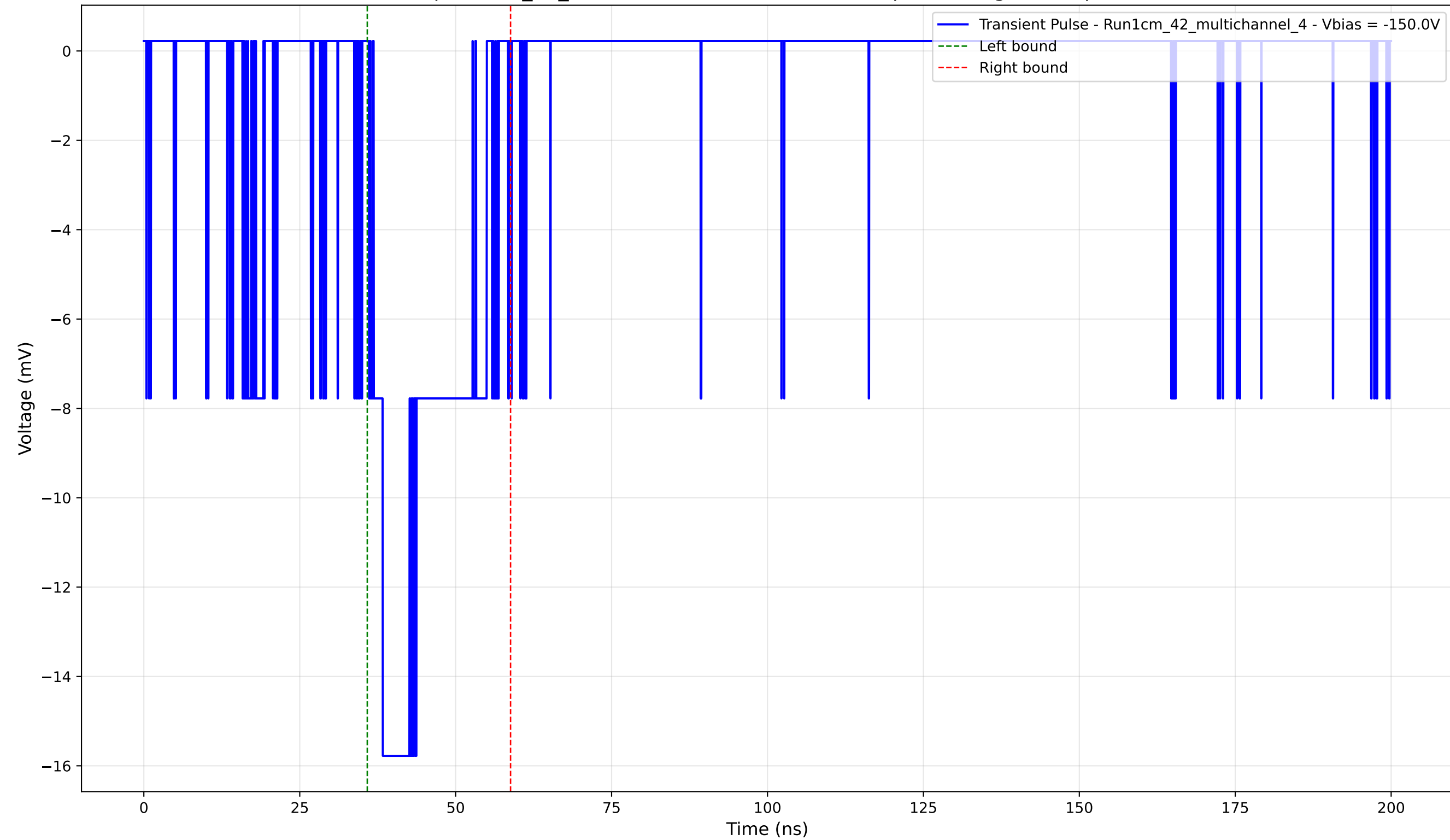
Transient Pulse - Sample: 1cm_42_multichannel - Position: 4285.0 \mu\text{m} - Charge: 3.78 pC - Rise Time: 1.46 ns
