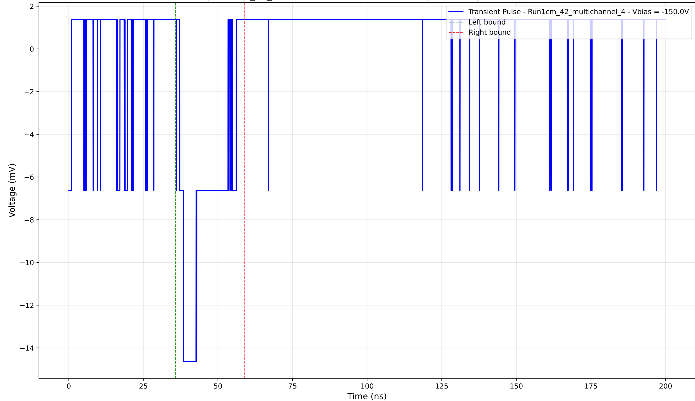
Transient Pulse - Sample: 1cm_42_multichannel - Position: 4230.0 \mu\text{m} - Charge: 2.96 pC - Rise Time: 1.26 ns
