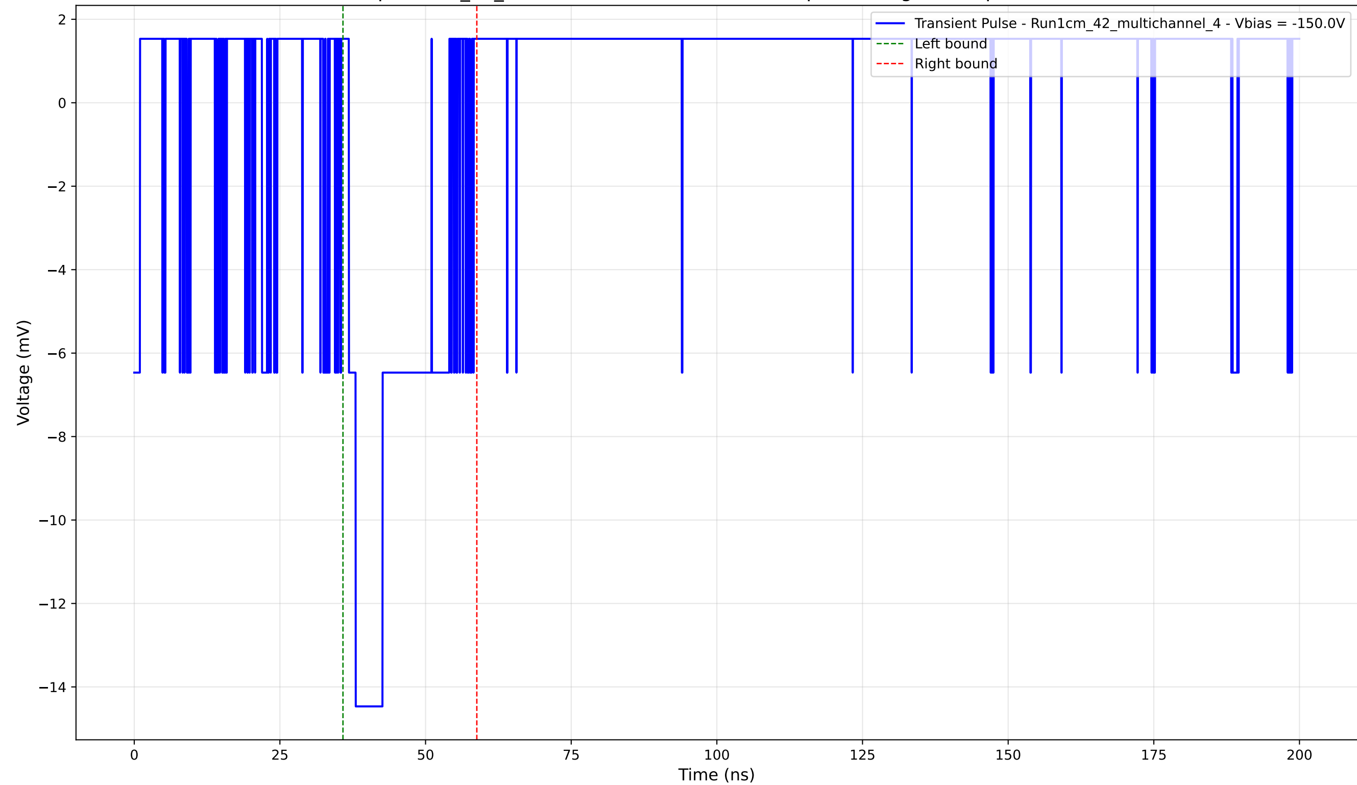
Transient Pulse - Sample: 1cm_42_multichannel - Position: 4040.0 \mu\text{m} - Charge: 2.99 pC - Rise Time: 0.00 ns (N/A)
