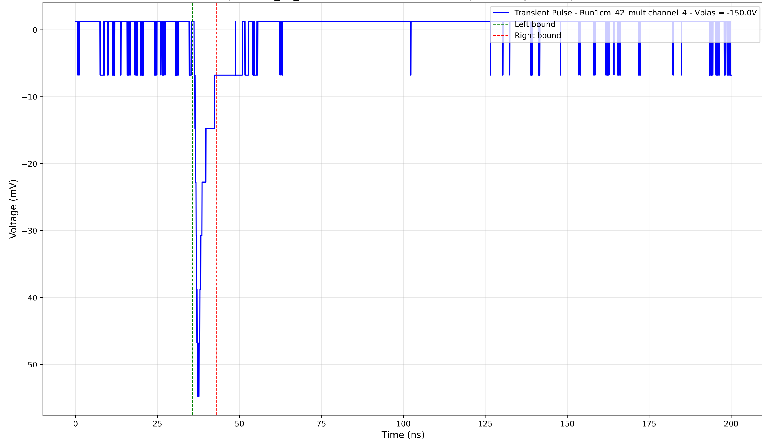
Transient Pulse - Sample: 1cm_42_multichannel - Position: 2765.0 \mu\text{m} - Charge: 3.04 pC - Rise Time: 1.12 ns
