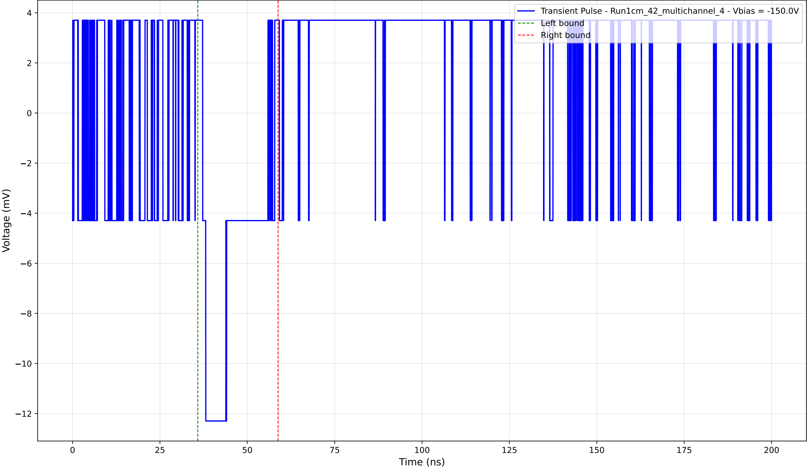
Transient Pulse - Sample: 1cm_42_multichannel - Position: 505.0 \mu\text{m} - Charge: 2.40 pC - Rise Time: 0.00 ns (N/A)
