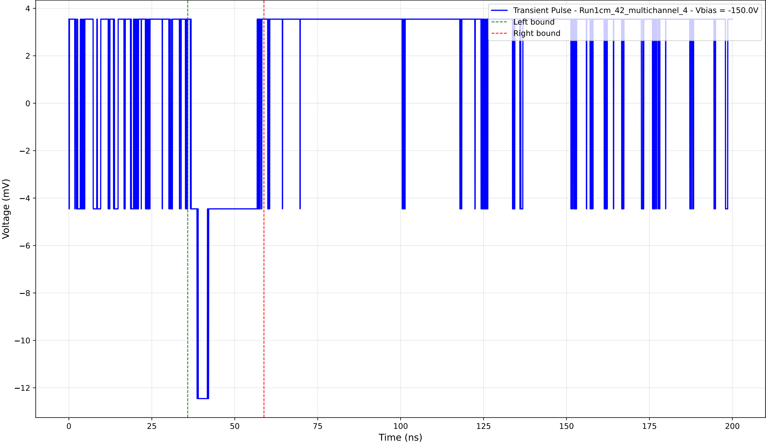
Transient Pulse - Sample: 1cm_42_multichannel - Position: 200.0 \mu\text{m} - Charge: 2.18 pC - Rise Time: 0.00 ns (N/A)
