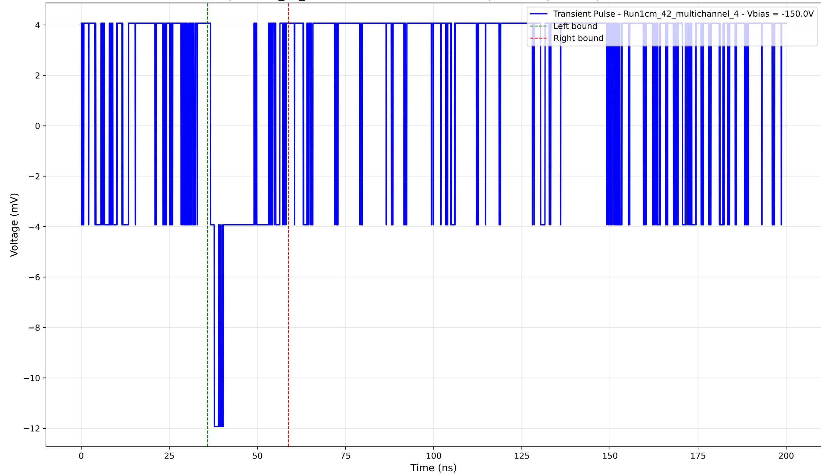
Transient Pulse - Sample: 1cm_42_multichannel - Position: 1325.0 \mu\text{m} - Charge: 1.38 pC - Rise Time: 0.00 ns (N/A)
