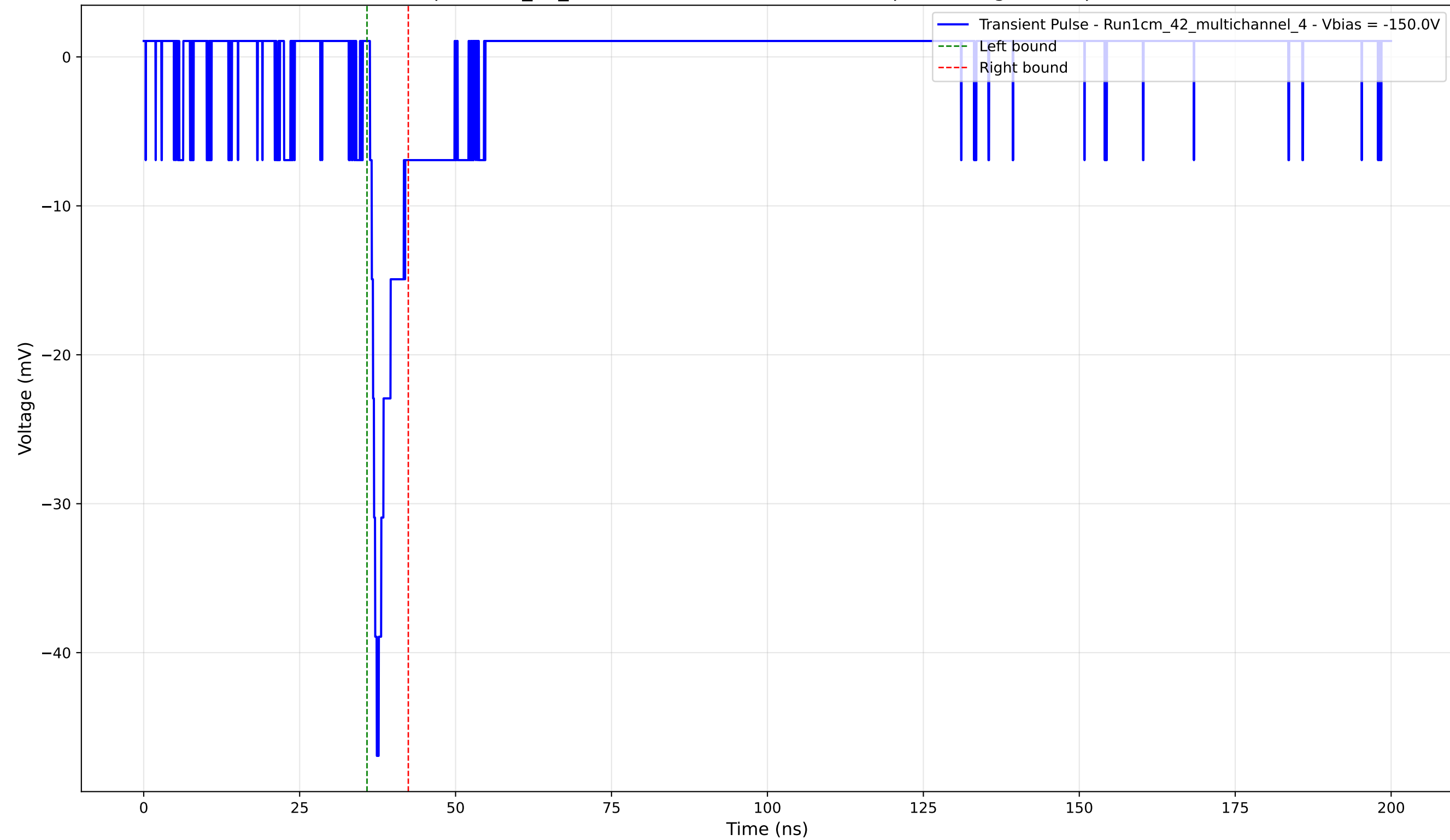
Transient Pulse - Sample: 1cm_42_multichannel - Position: 2820.0 \mu\text{m} - Charge: 2.57 pC - Rise Time: 1.09 ns
