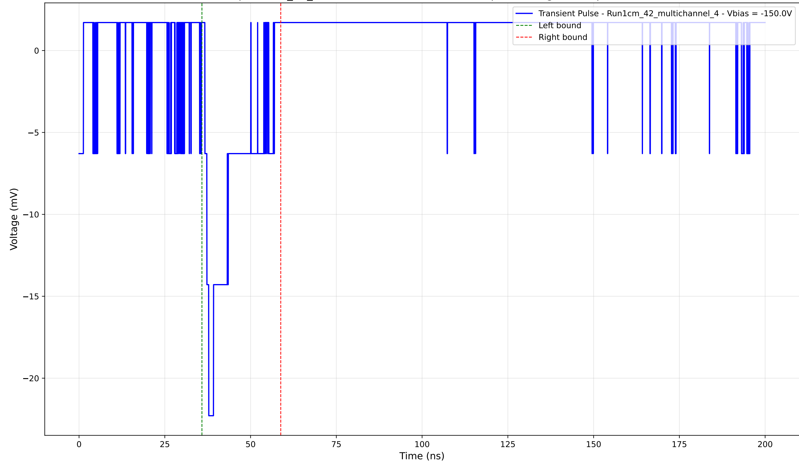
Transient Pulse - Sample: 1cm_42_multichannel - Position: 3520.0 \mu\text{m} - Charge: 3.49 pC - Rise Time: 1.14 ns
