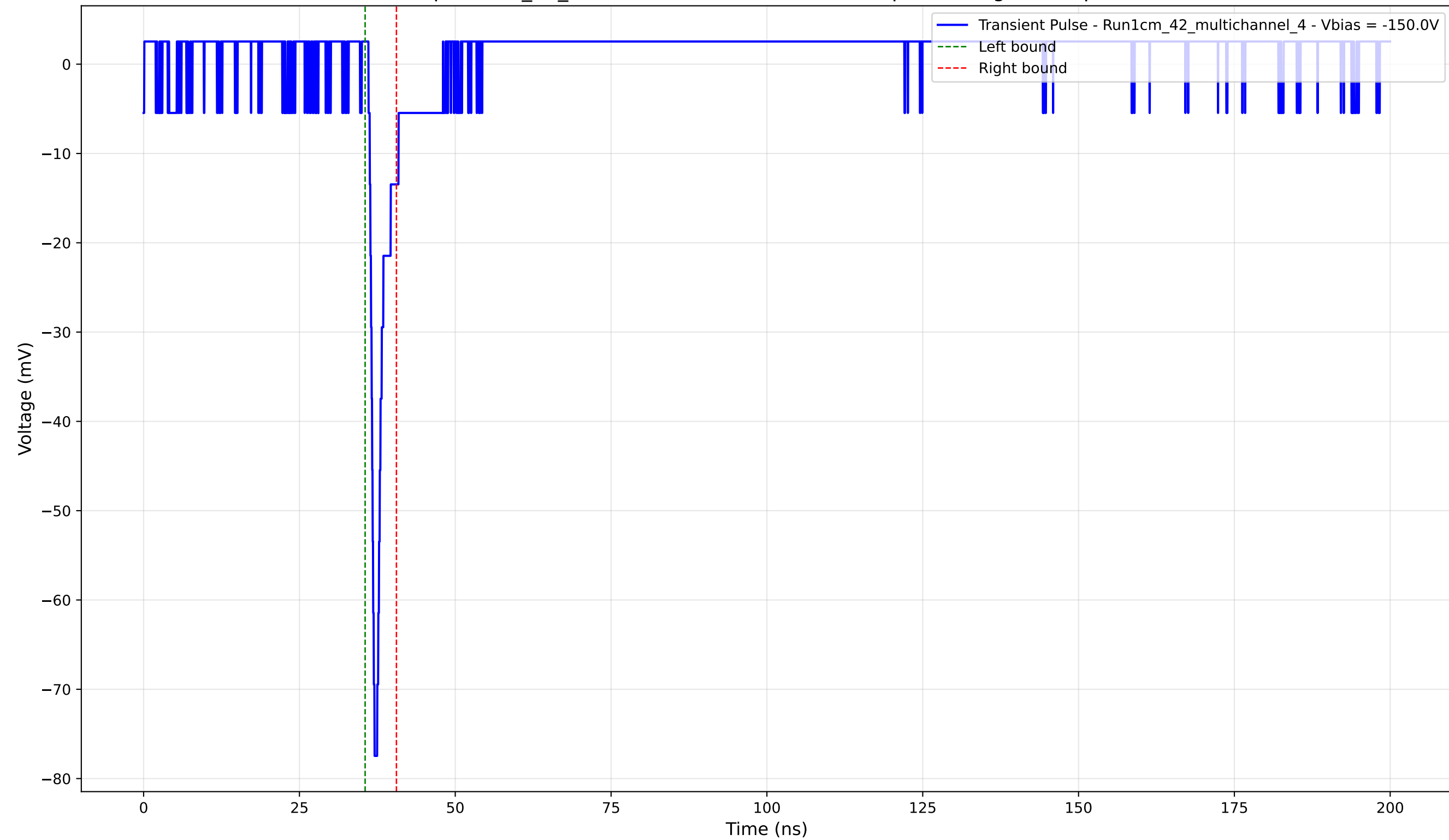
Transient Pulse - Sample: 1cm_42_multichannel - Position: 2500.0 \mu\text{m} - Charge: 2.98 pC - Rise Time: 0.77 ns
