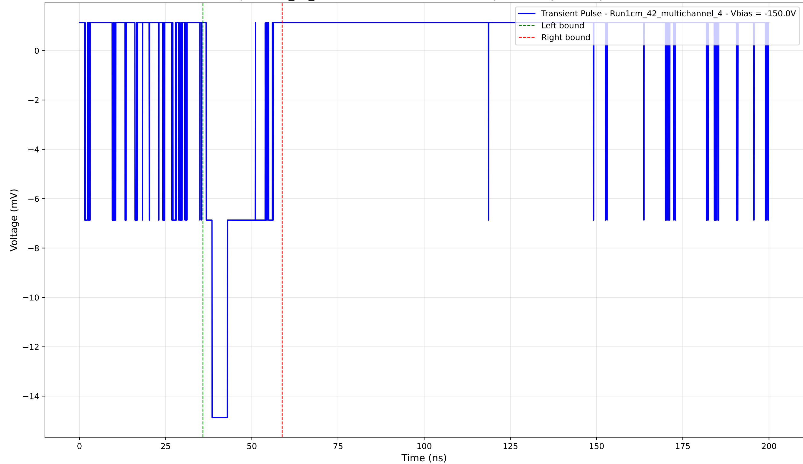
Transient Pulse - Sample: 1cm_42_multichannel - Position: 4560.0 \mu\text{m} - Charge: 3.20 pC - Rise Time: 1.72 ns
