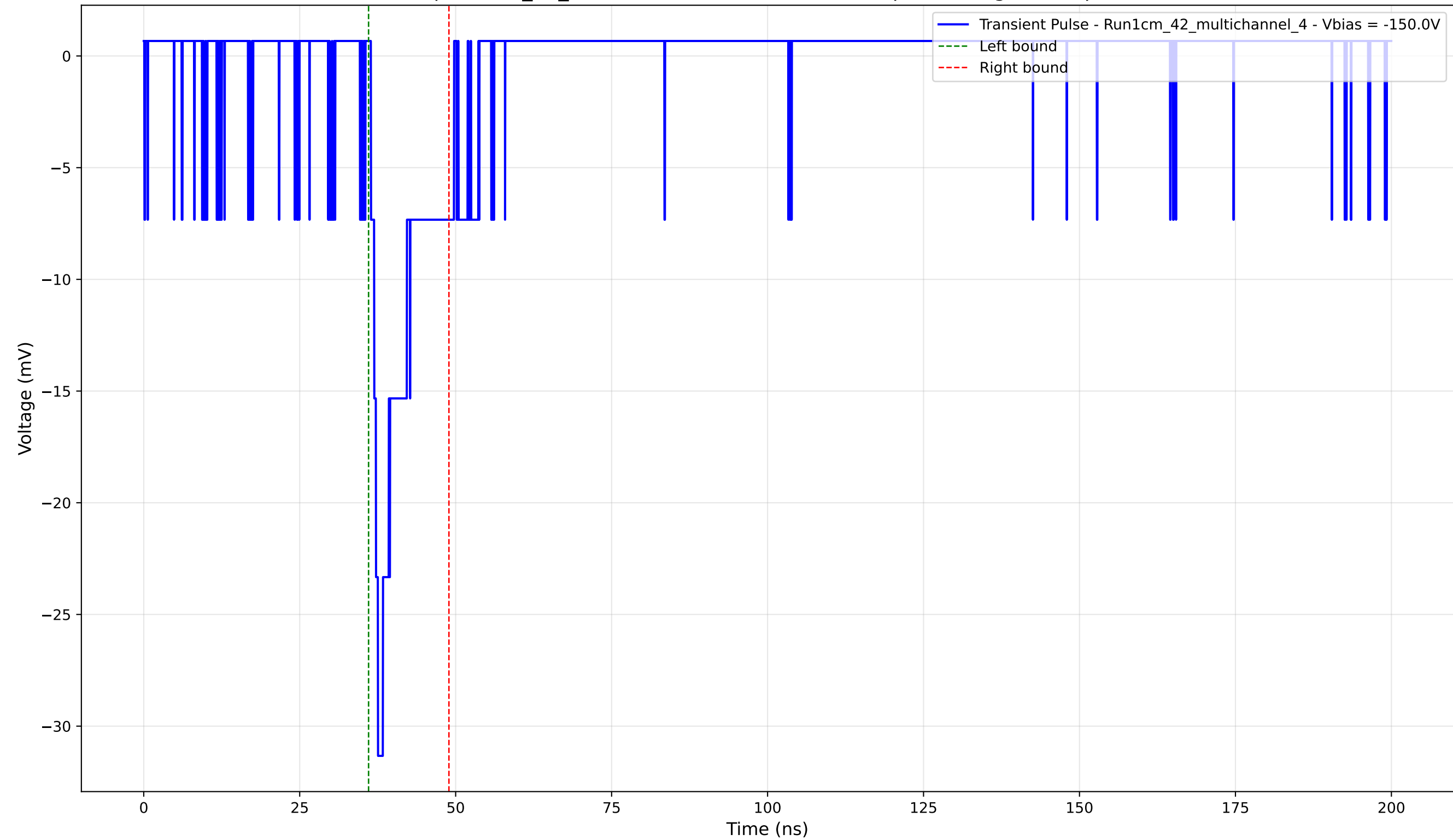
Transient Pulse - Sample: 1cm_42_multichannel - Position: 3215.0 \mu\text{m} - Charge: 3.14 pC - Rise Time: 1.13 ns
