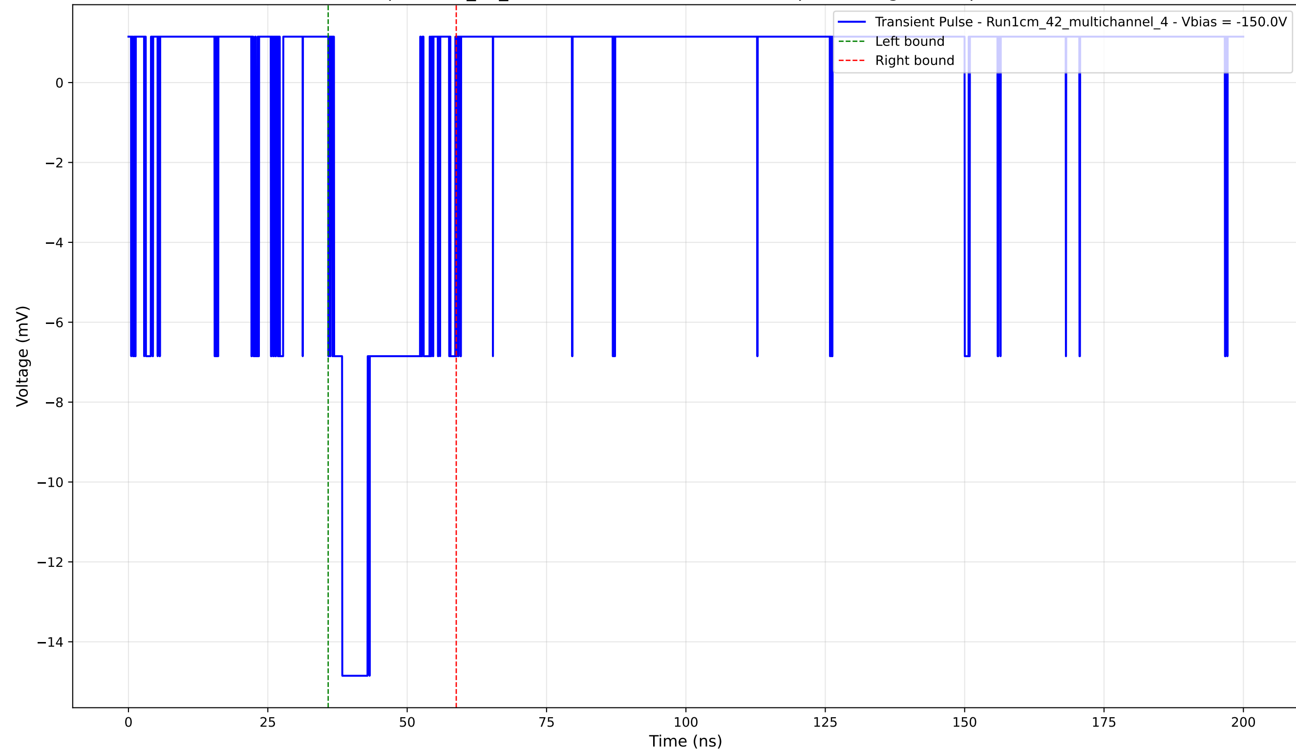
Transient Pulse - Sample: 1cm_42_multichannel - Position: 4240.0 \mu\text{m} - Charge: 3.17 pC - Rise Time: 1.48 ns
