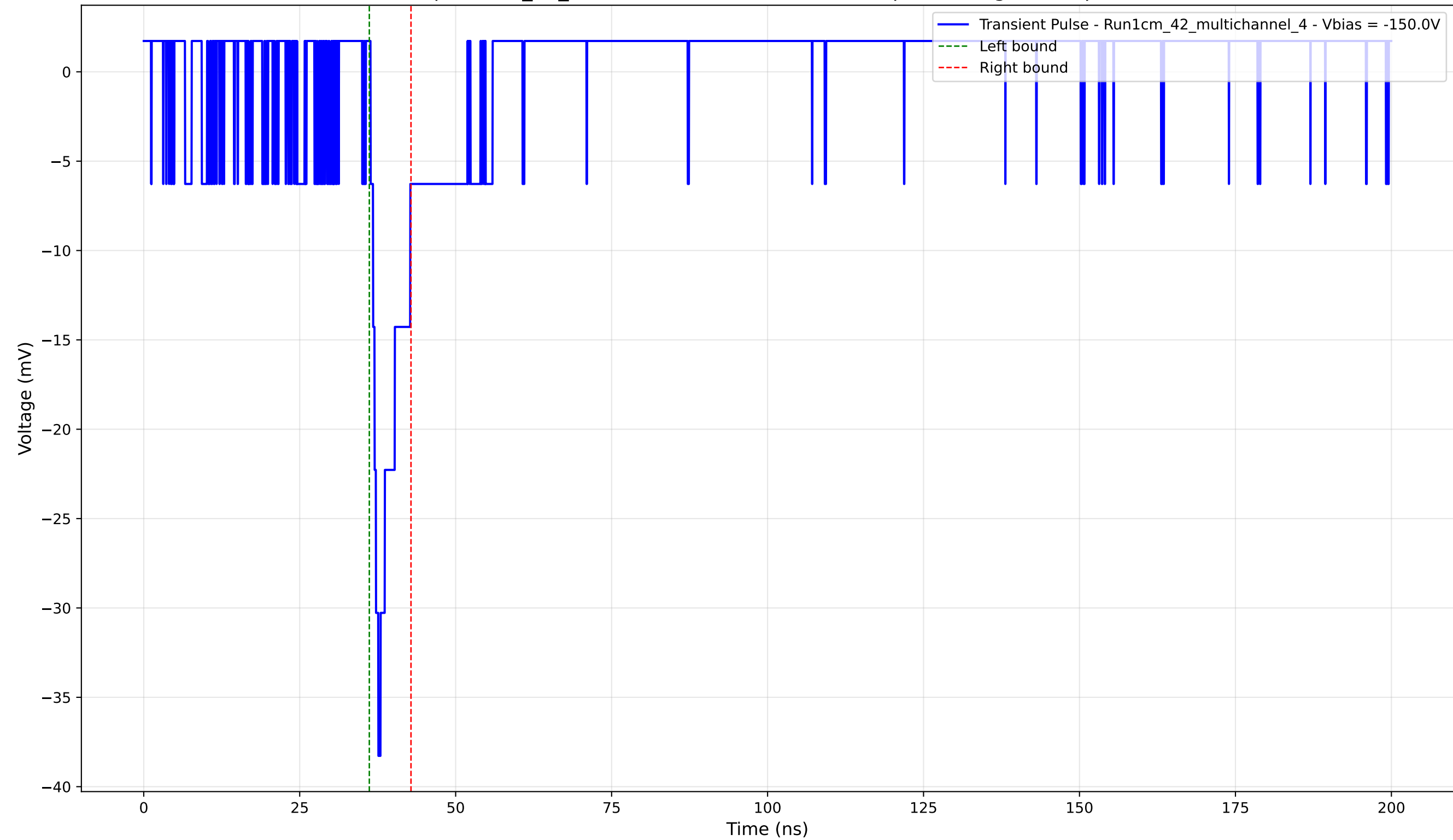
Transient Pulse - Sample: 1cm_42_multichannel - Position: 1665.0 \mu\text{m} - Charge: 2.56 pC - Rise Time: 1.25 ns
