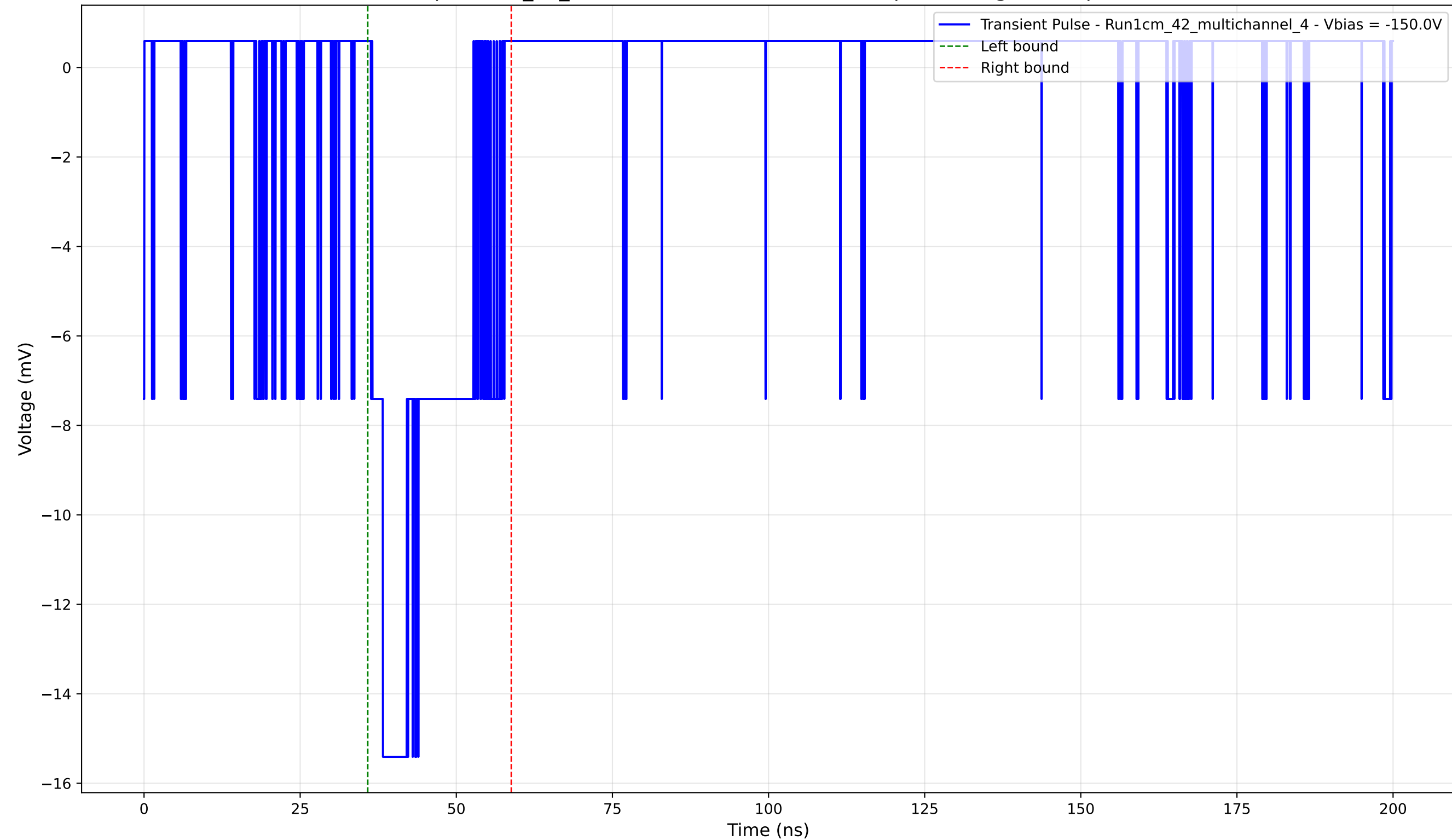
Transient Pulse - Sample: 1cm_42_multichannel - Position: 4320.0 \mu\text{m} - Charge: 3.50 pC - Rise Time: 1.70 ns
