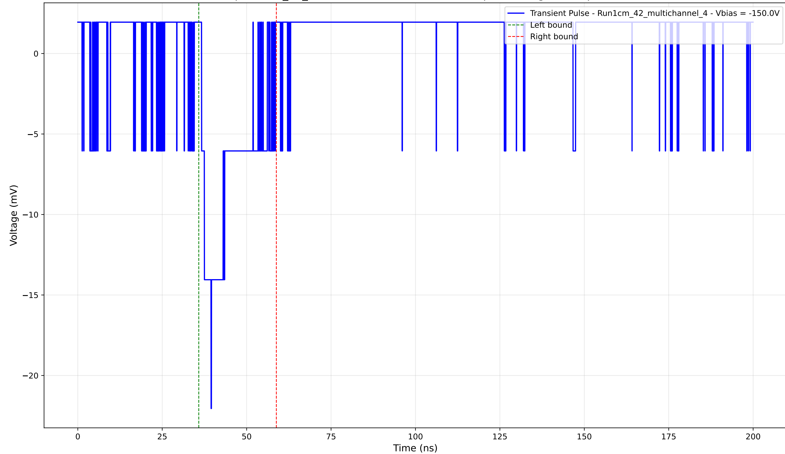
Transient Pulse - Sample: 1cm_42_multichannel - Position: 3690.0 \mu\text{m} - Charge: 3.23 pC - Rise Time: 2.82 ns
