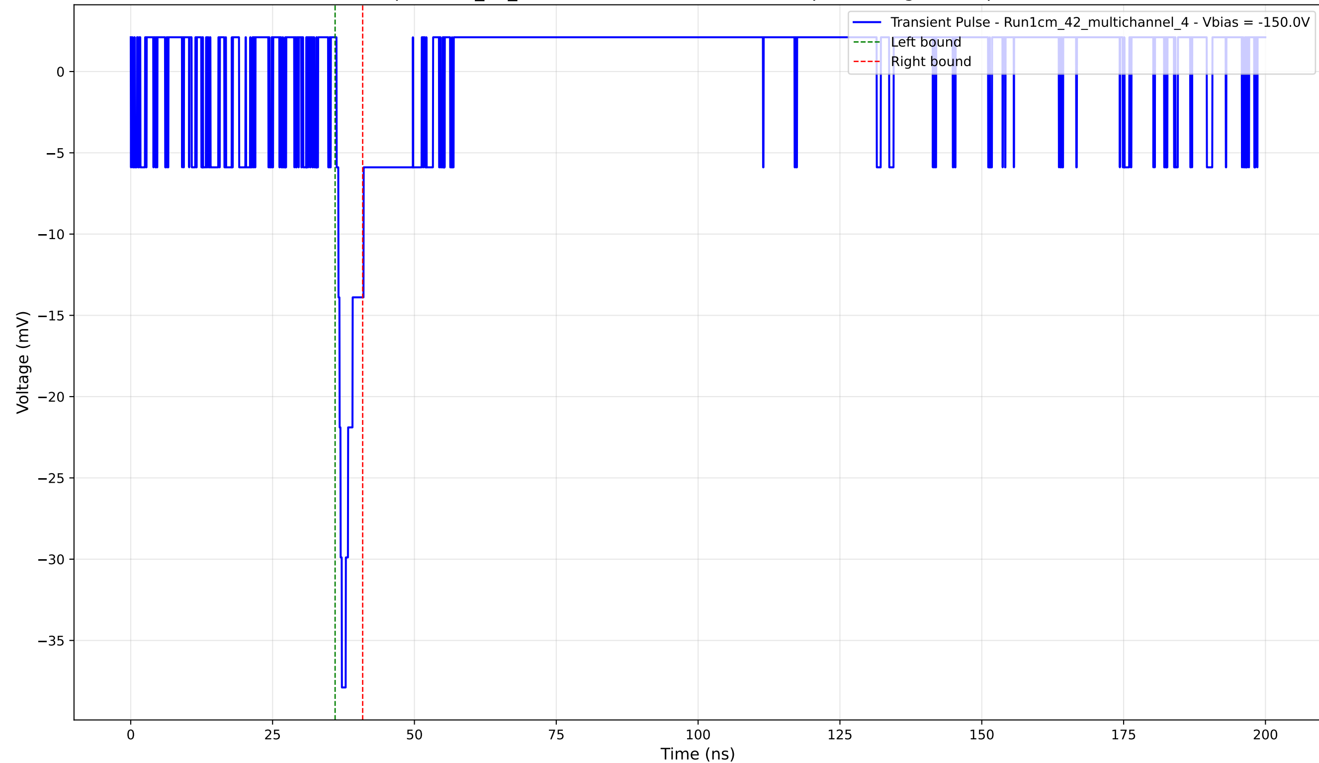
Transient Pulse - Sample: 1cm_42_multichannel - Position: 1940.0 \mu\text{m} - Charge: 1.91 pC - Rise Time: 0.93 ns
