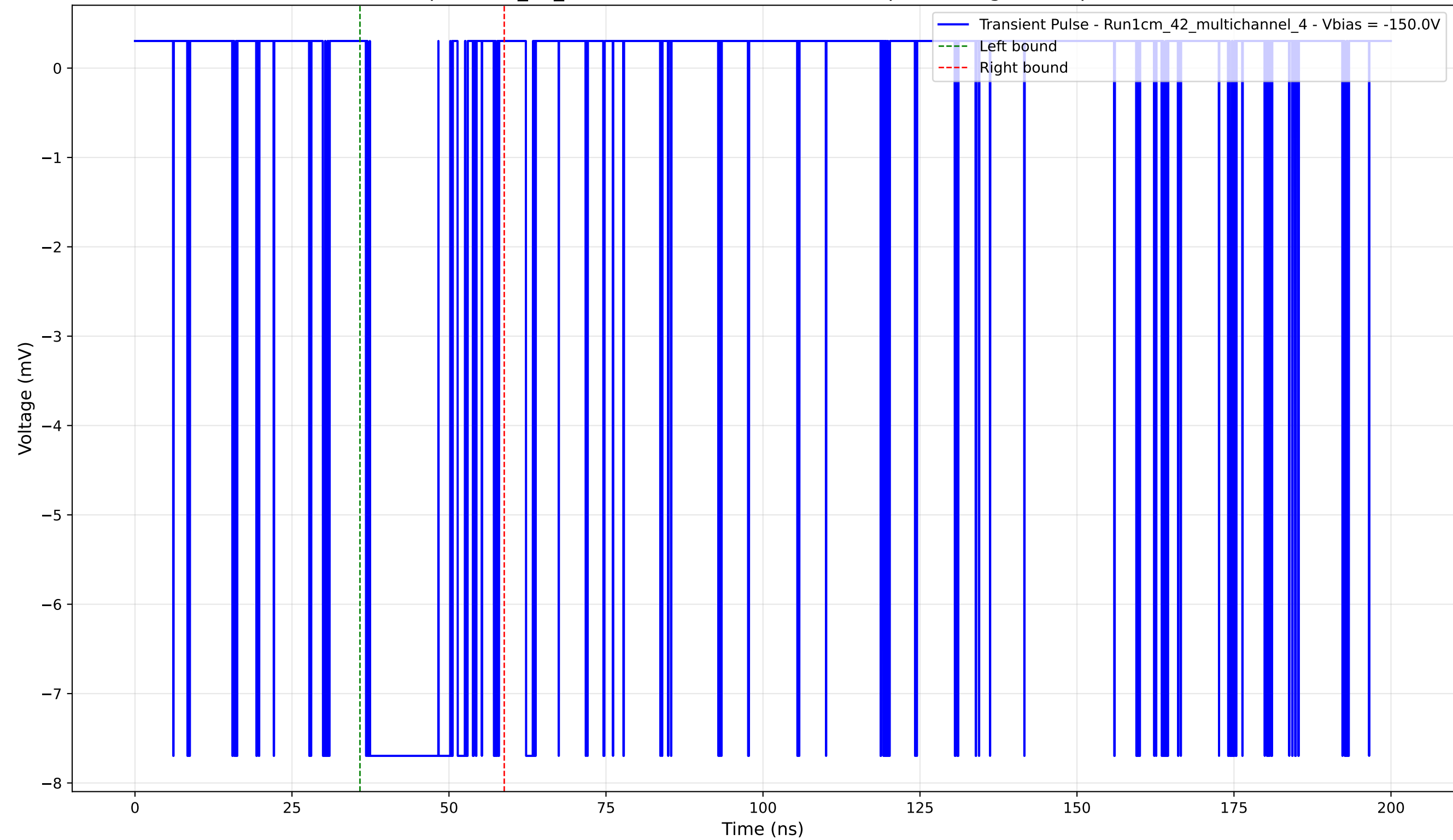
Transient Pulse - Sample: 1cm_42_multichannel - Position: 4860.0 \mu\text{m} - Charge: 2.38 pC - Rise Time: 0.02 ns
