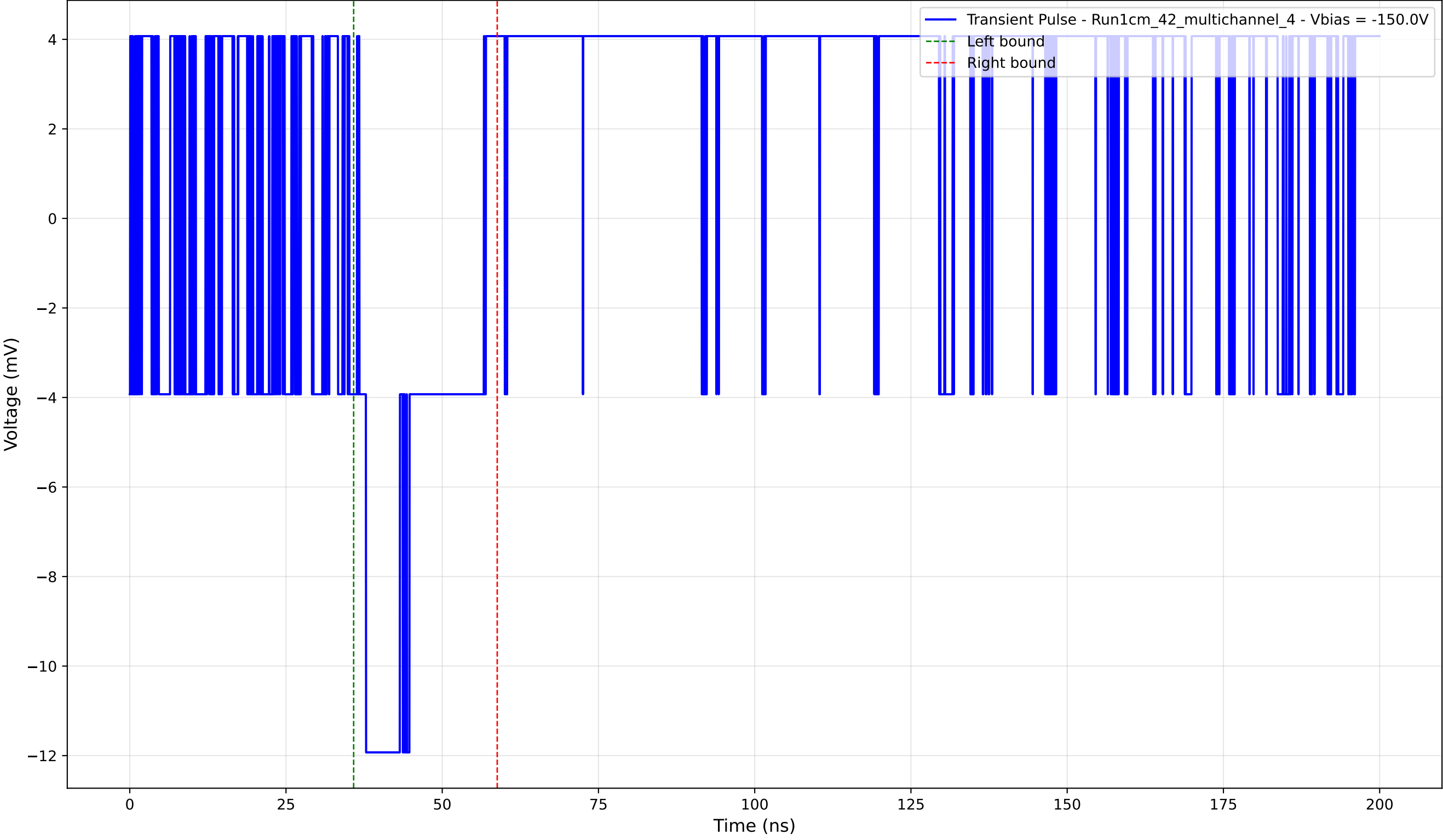
Transient Pulse - Sample: 1cm_42_multichannel - Position: 785.0 \mu\text{m} - Charge: 2.47 pC - Rise Time: 0.00 ns (N/A)
