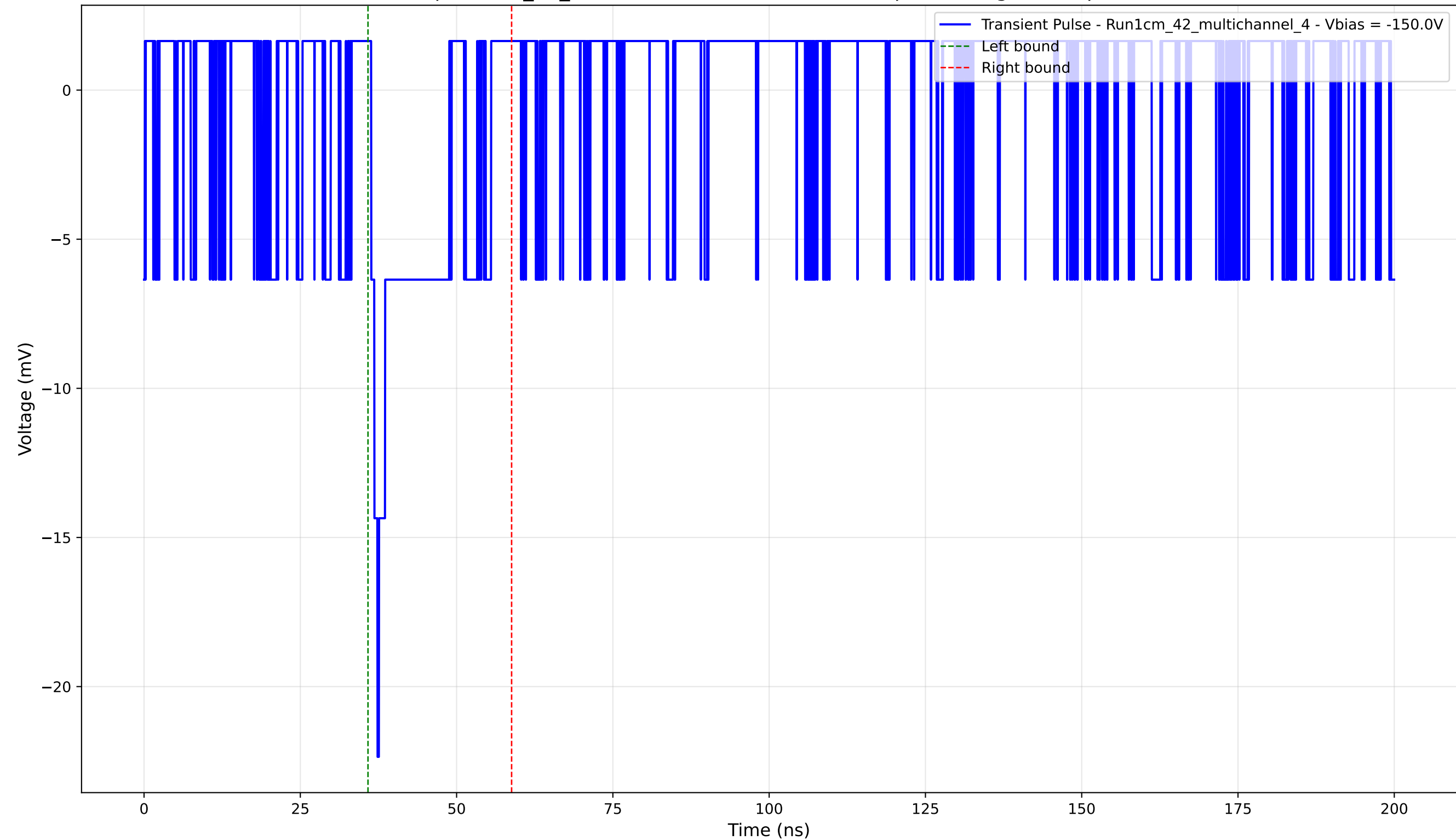
Transient Pulse - Sample: 1cm_42_multichannel - Position: 1925.0 \mu\text{m} - Charge: 2.09 pC - Rise Time: 1.02 ns
