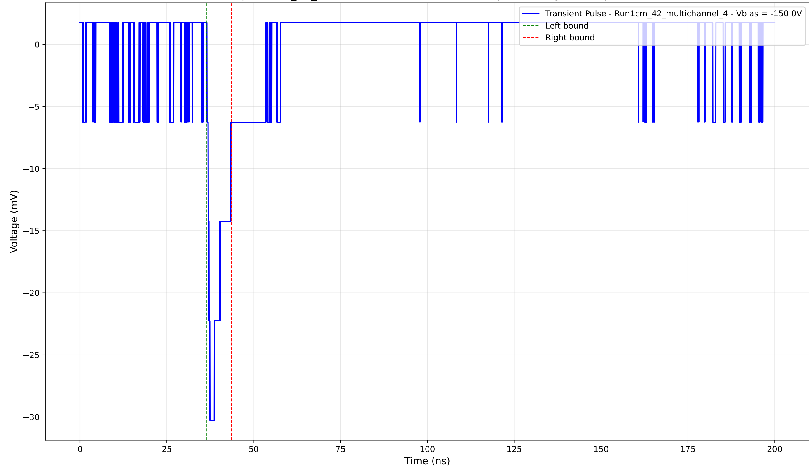
Transient Pulse - Sample: 1cm_42_multichannel - Position: 1545.0 \mu\text{m} - Charge: 2.64 pC - Rise Time: 0.89 ns
