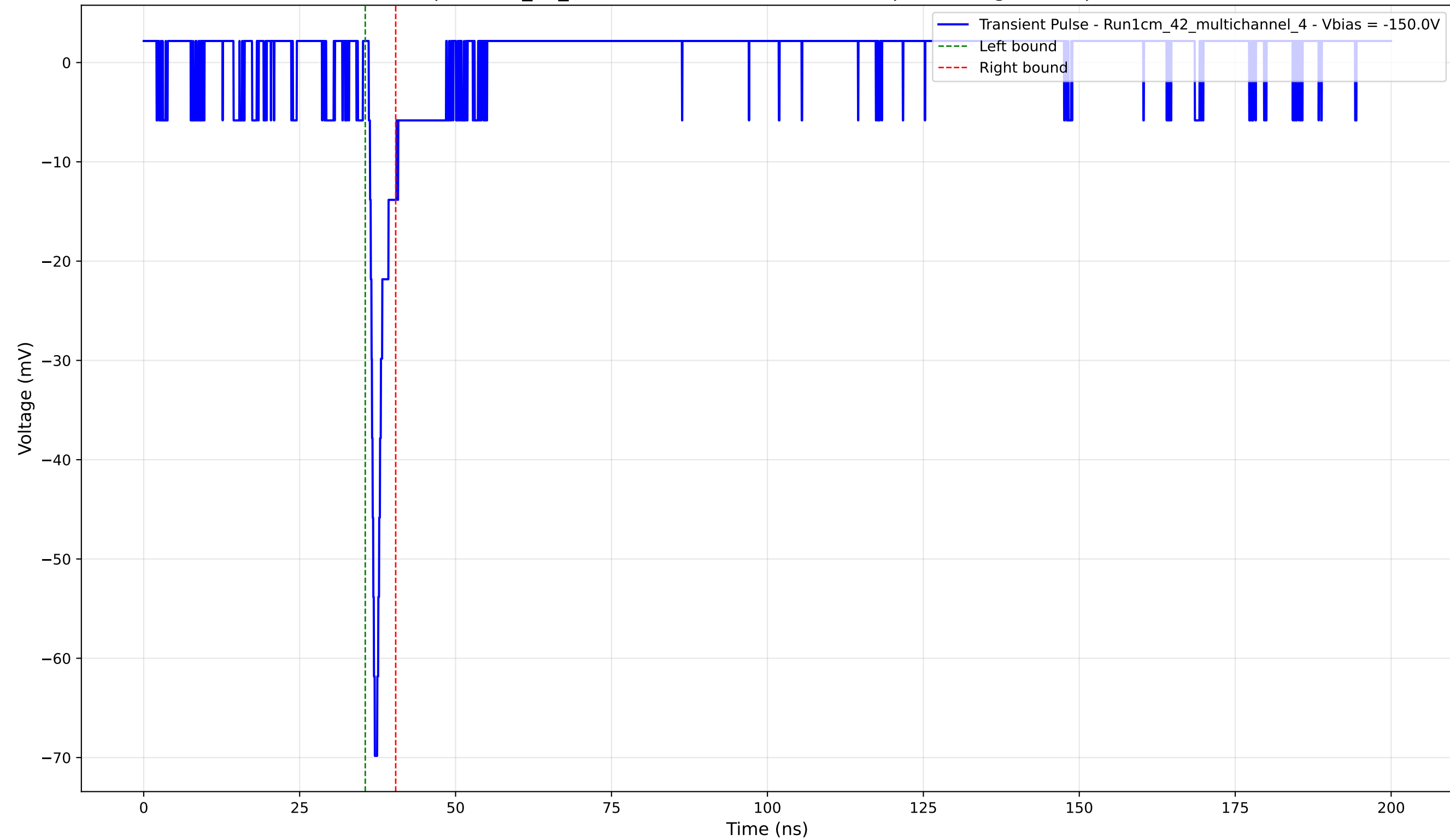
Transient Pulse - Sample: 1cm_42_multichannel - Position: 2315.0 \mu\text{m} - Charge: 2.61 pC - Rise Time: 0.78 ns
