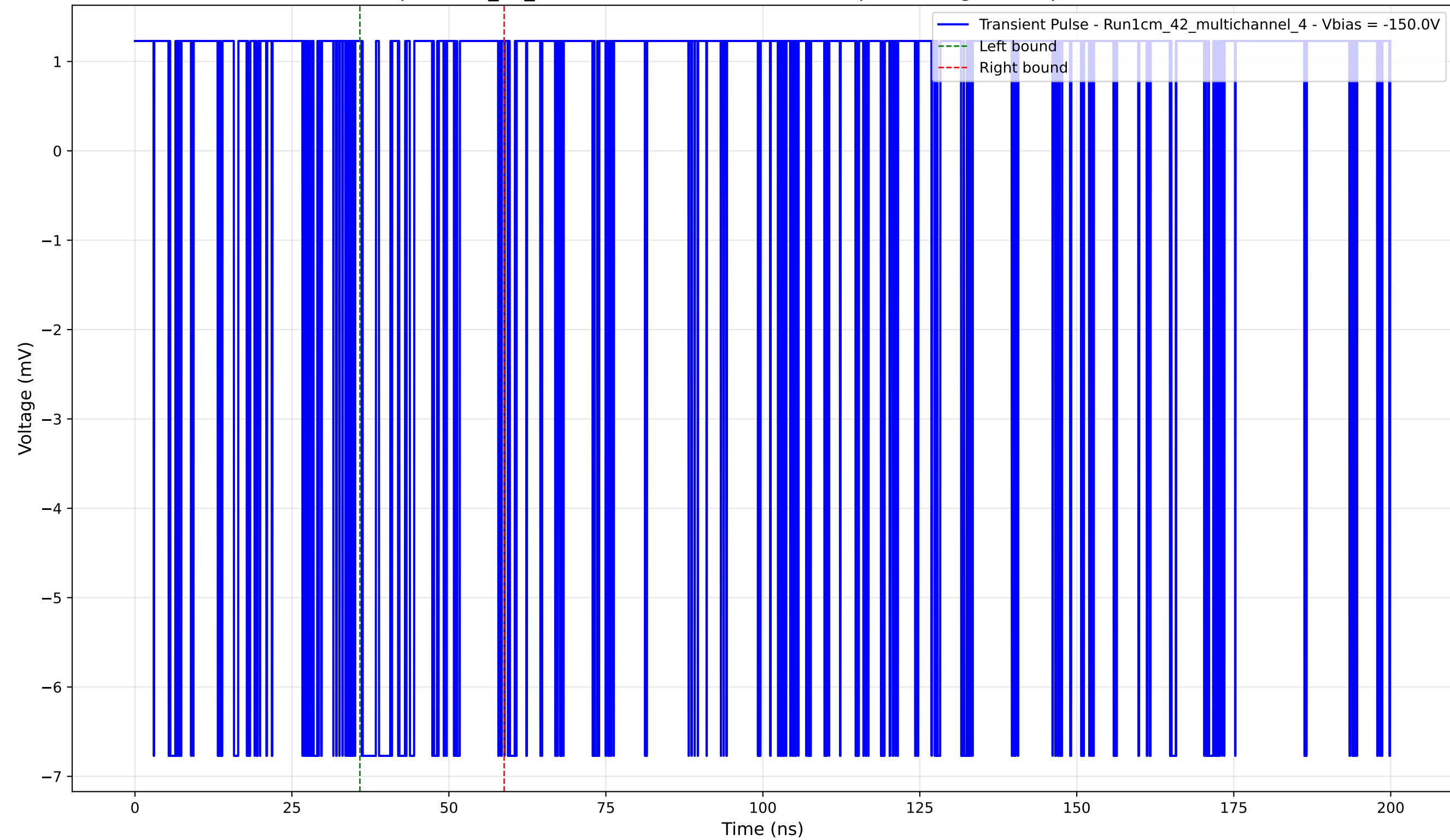
Transient Pulse - Sample: 1cm_42_multichannel - Position: 2365.0 \mu\text{m} - Charge: 0.71 pC - Rise Time: 0.00 ns (N/A)
