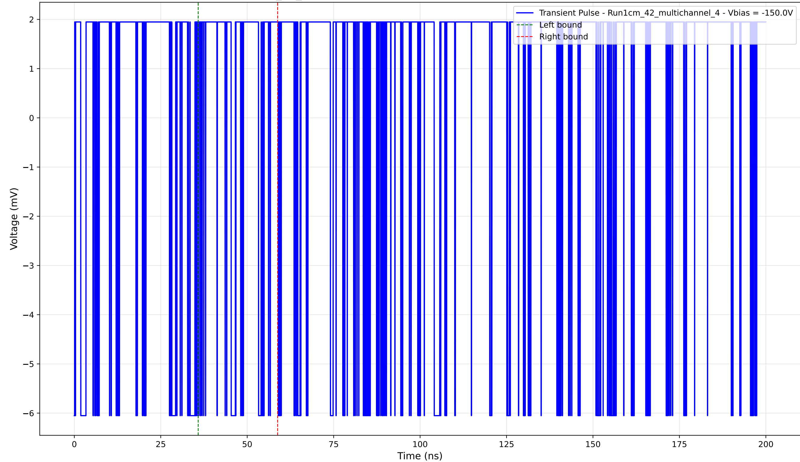
Transient Pulse - Sample: 1cm_42_multichannel - Position: 30.0 \mu\text{m} - Charge: 0.31 pC - Rise Time: 0.00 ns (N/A)
