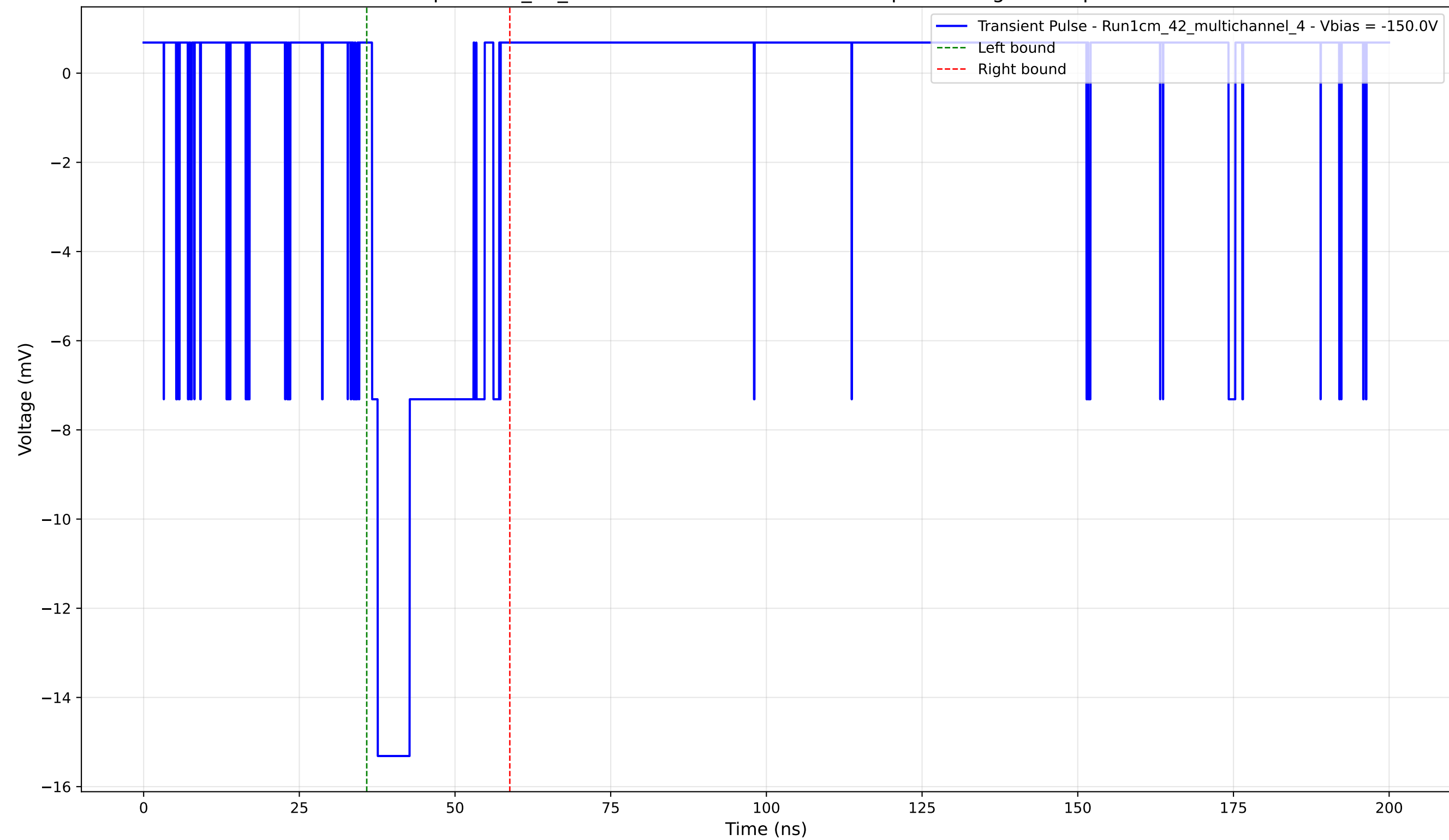
Transient Pulse - Sample: 1cm_42_multichannel - Position: 3705.0 \mu\text{m} - Charge: 3.54 pC - Rise Time: 0.92 ns
