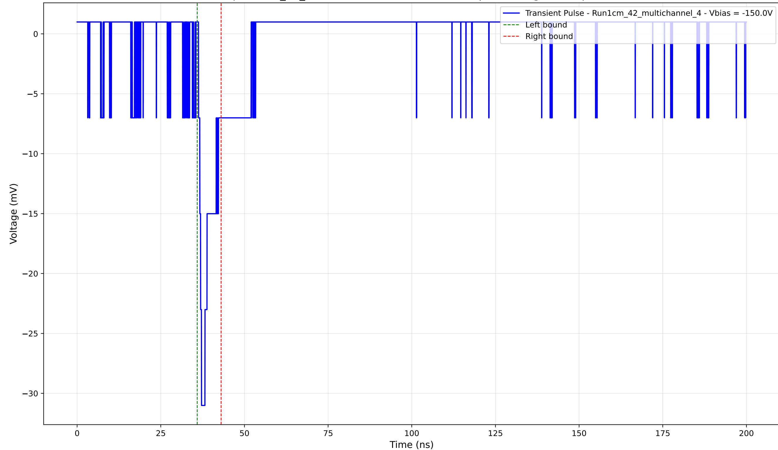
Transient Pulse - Sample: 1cm_42_multichannel - Position: 2955.0 \mu\text{m} - Charge: 2.28 pC - Rise Time: 0.89 ns
