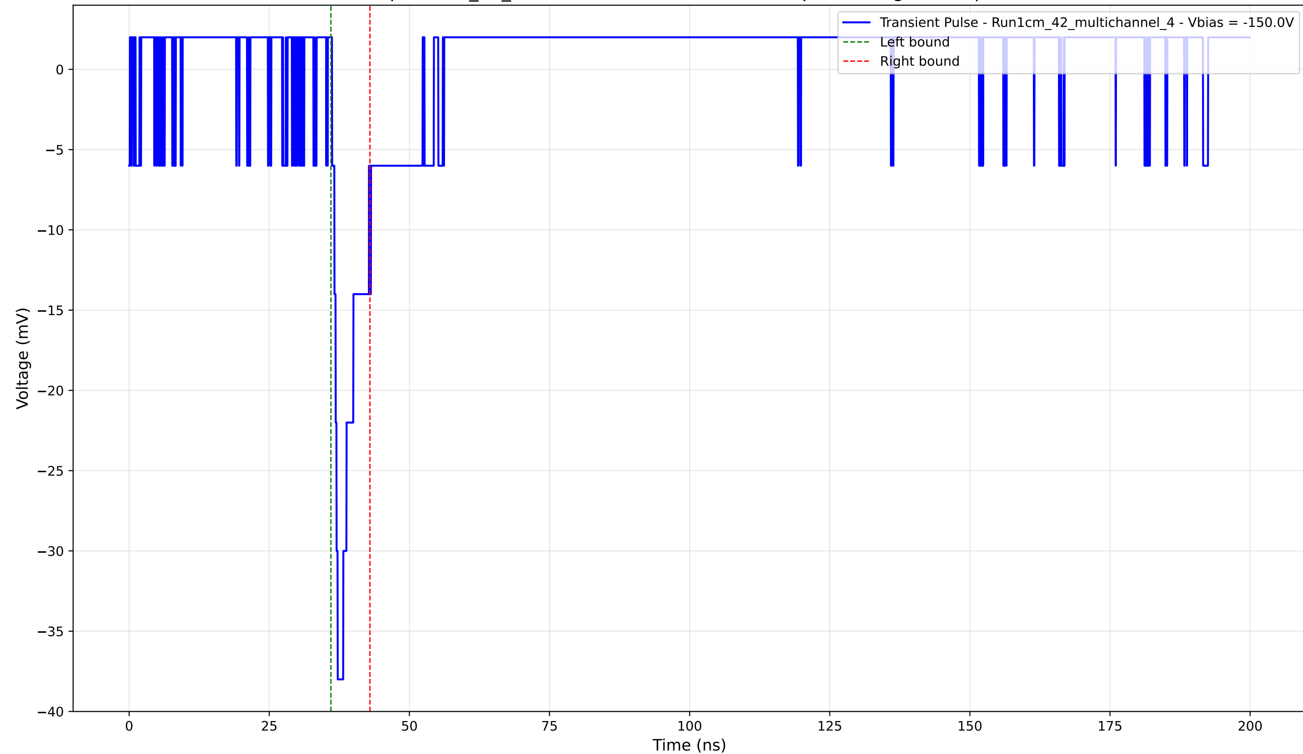
Transient Pulse - Sample: 1cm_42_multichannel - Position: 1800.0 \mu\text{m} - Charge: 2.76 pC - Rise Time: 1.01 ns
