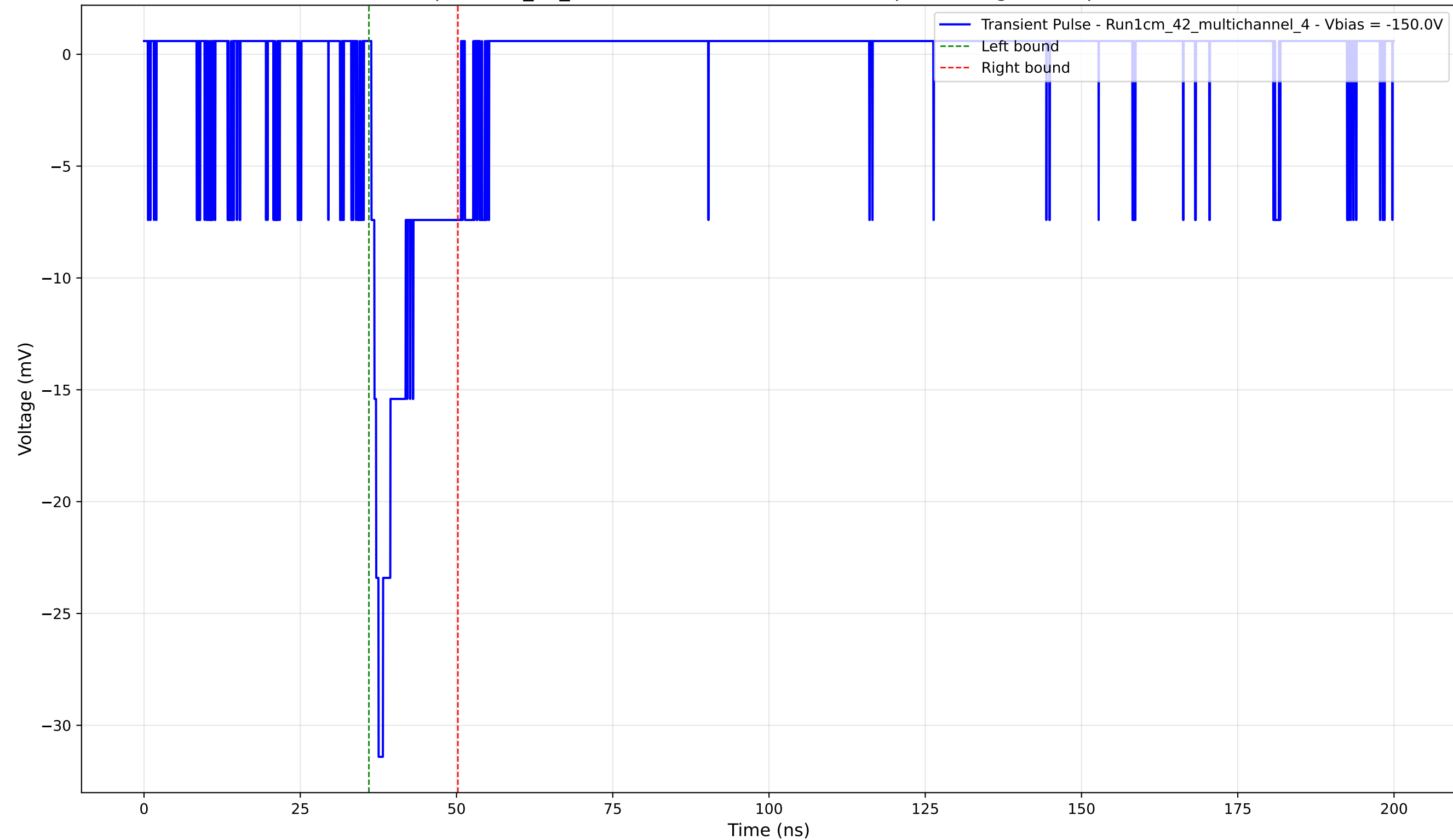
Transient Pulse - Sample: 1cm_42_multichannel - Position: 3165.0 \mu\text{m} - Charge: 3.36 pC - Rise Time: 1.15 ns
