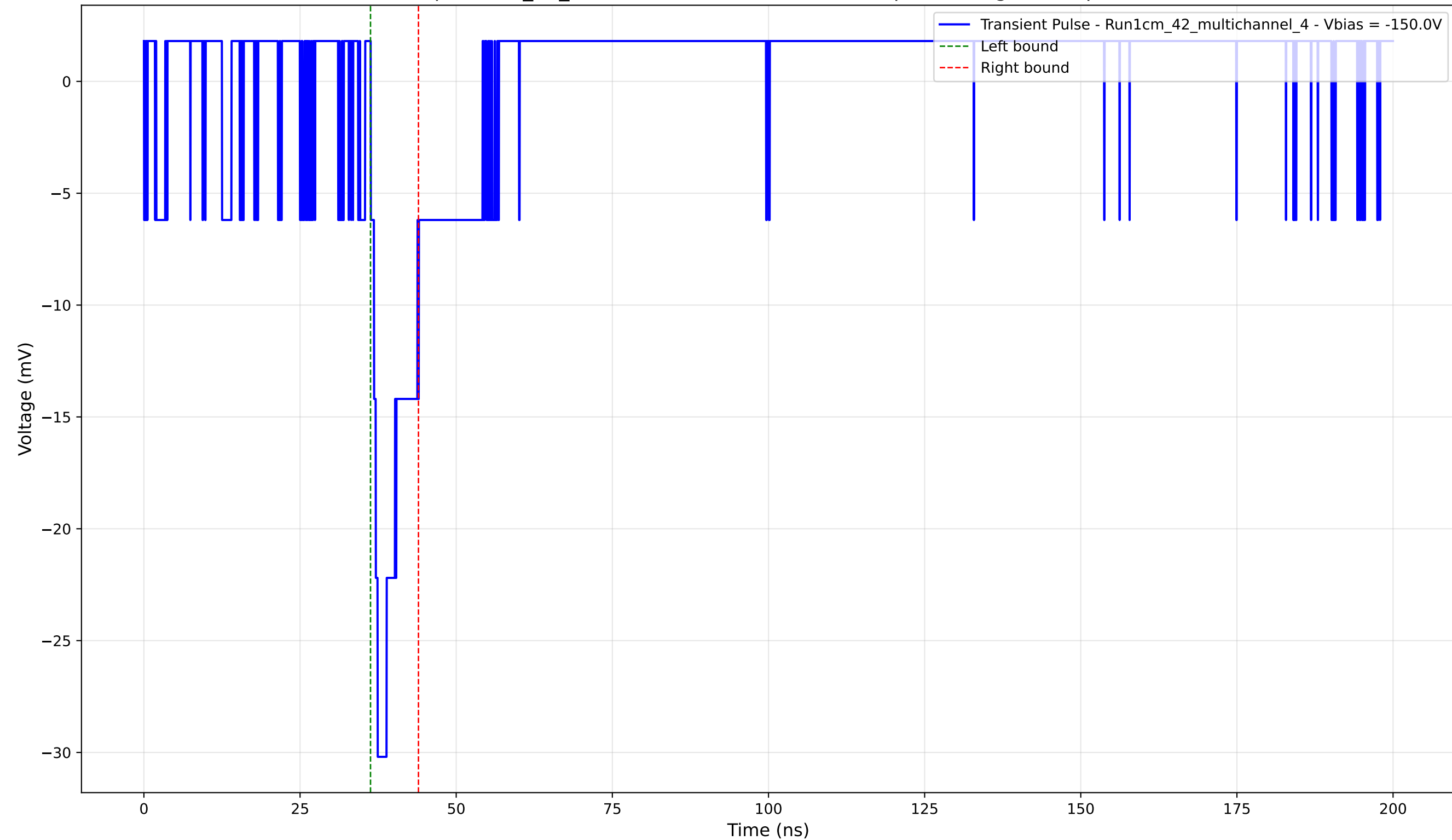
Transient Pulse - Sample: 1cm_42_multichannel - Position: 1535.0 \mu\text{m} - Charge: 2.81 pC - Rise Time: 1.11 ns
