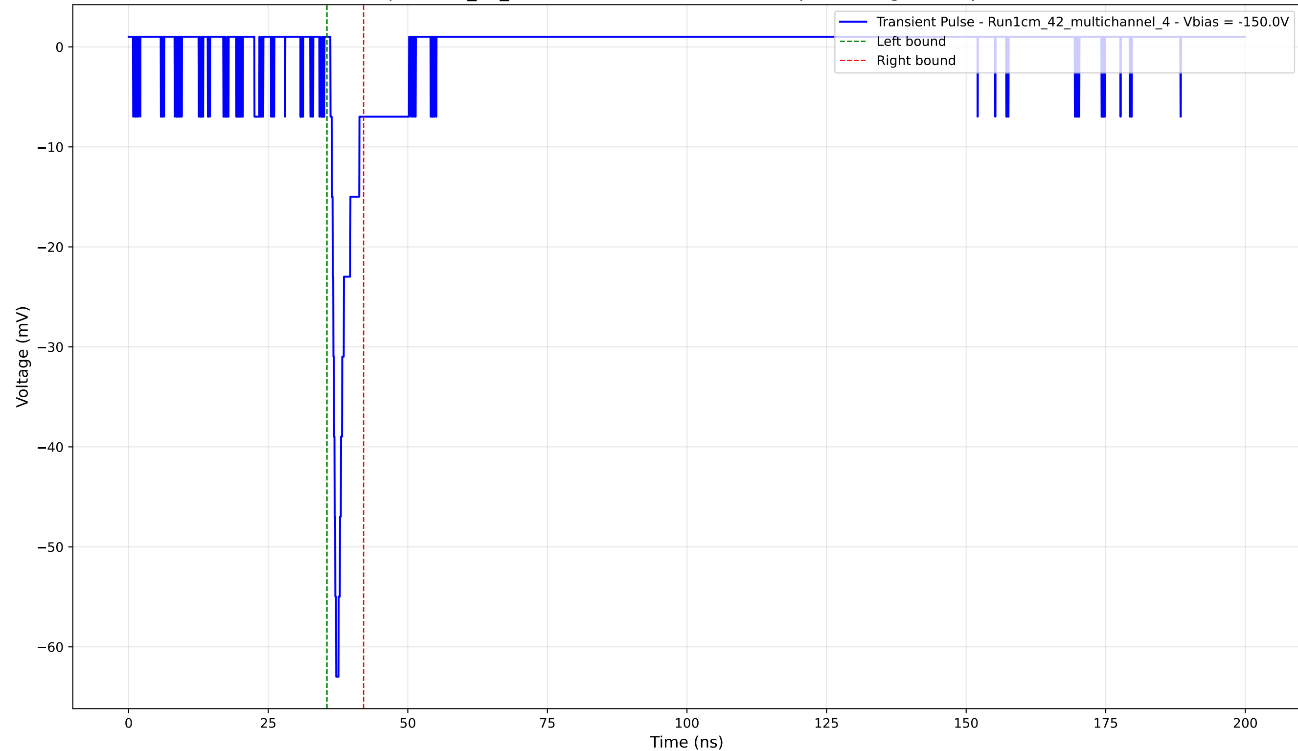
Transient Pulse - Sample: 1cm_42_multichannel - Position: 2120.0 \mu\text{m} - Charge: 3.04 pC - Rise Time: 1.02 ns
