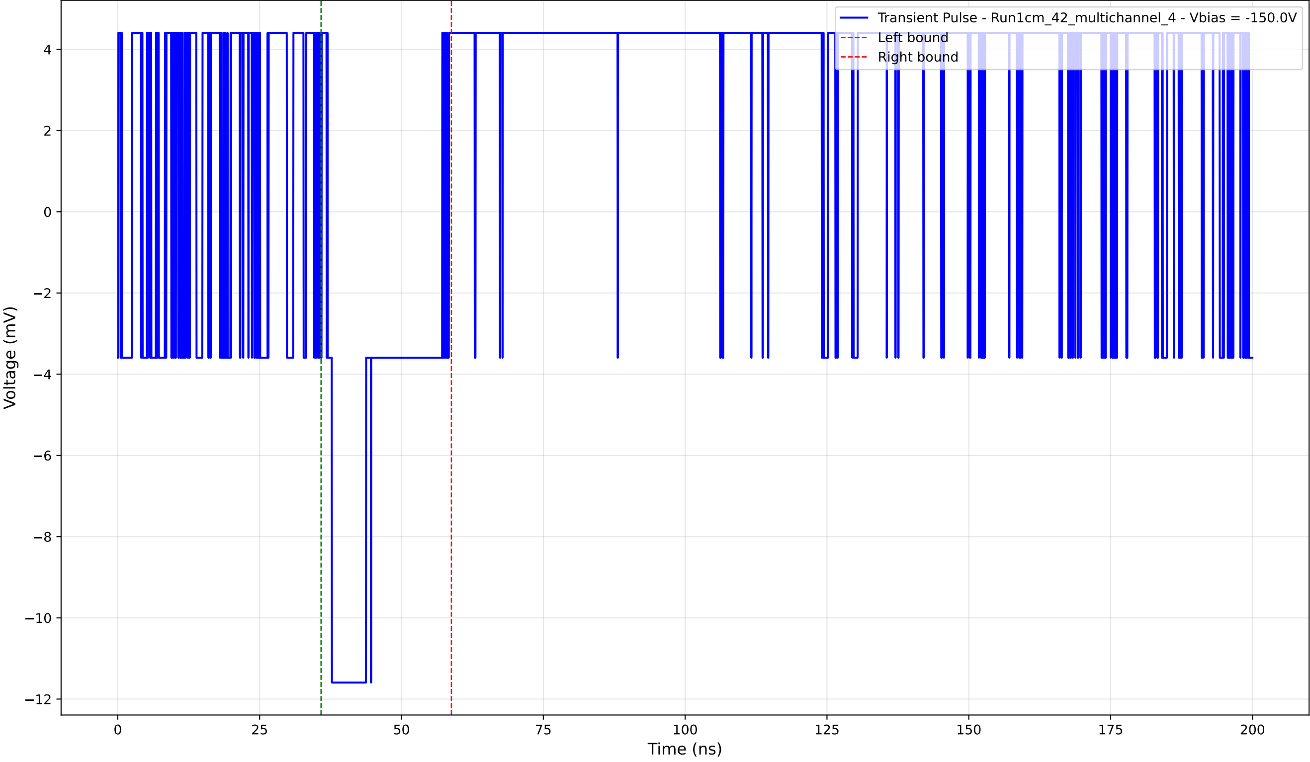
Transient Pulse - Sample: 1cm_42_multichannel - Position: 715.0 \mu\text{m} - Charge: 2.33 pC - Rise Time: 0.00 ns (N/A)
