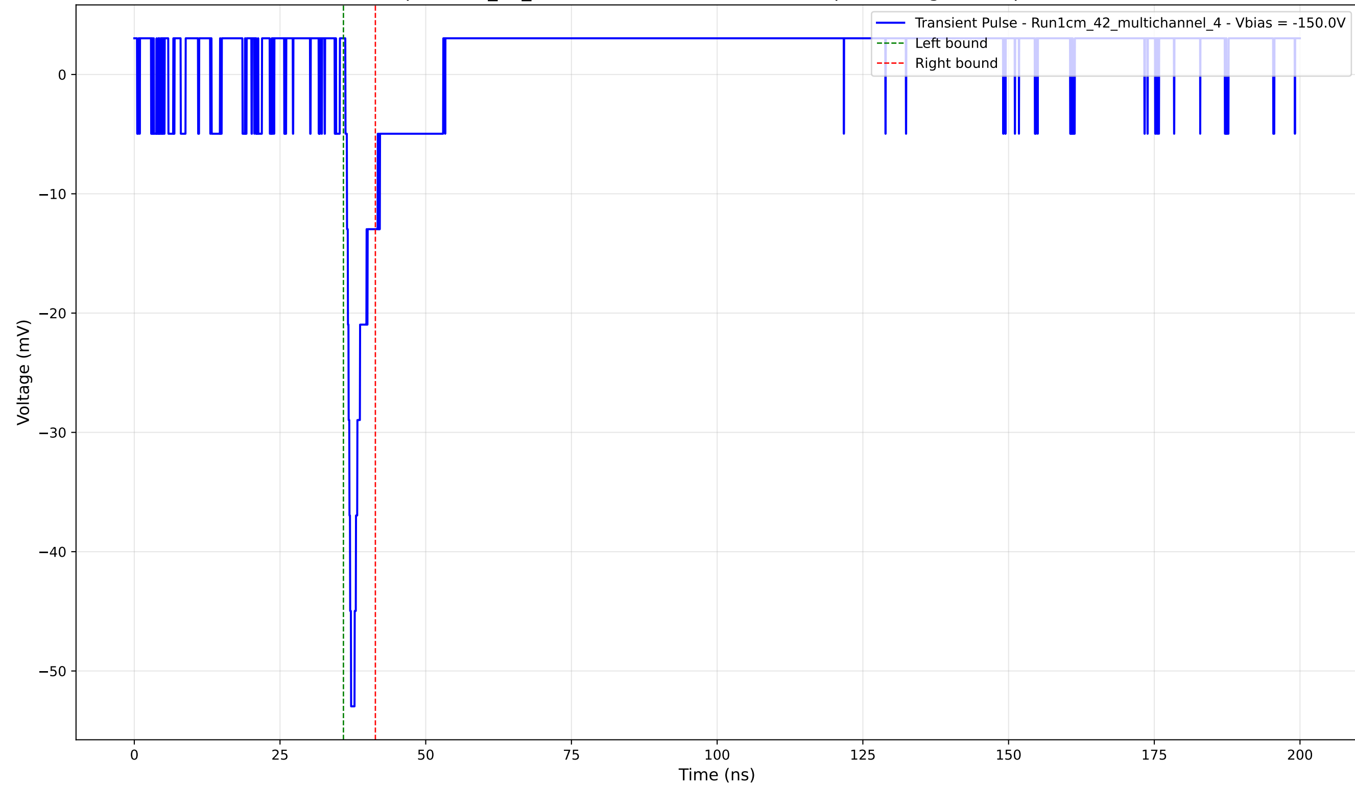
Transient Pulse - Sample: 1cm_42_multichannel - Position: 2010.0 \mu\text{m} - Charge: 2.59 pC - Rise Time: 0.72 ns
