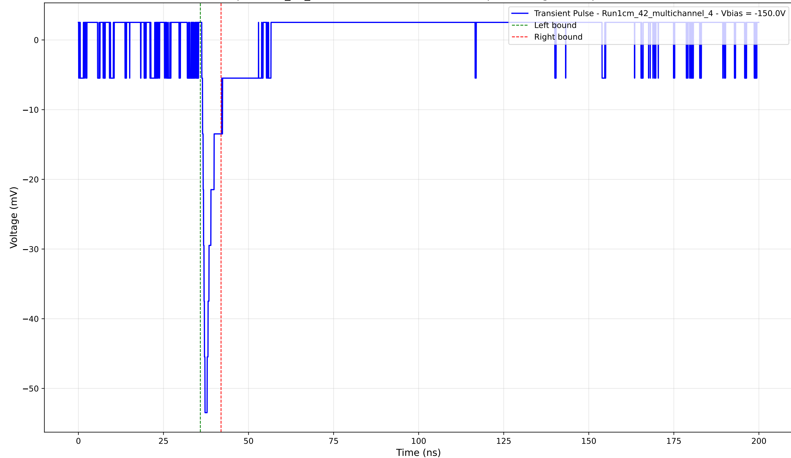
Transient Pulse - Sample: 1cm_42_multichannel - Position: 1985.0 \mu\text{m} - Charge: 2.84 pC - Rise Time: 0.94 ns
