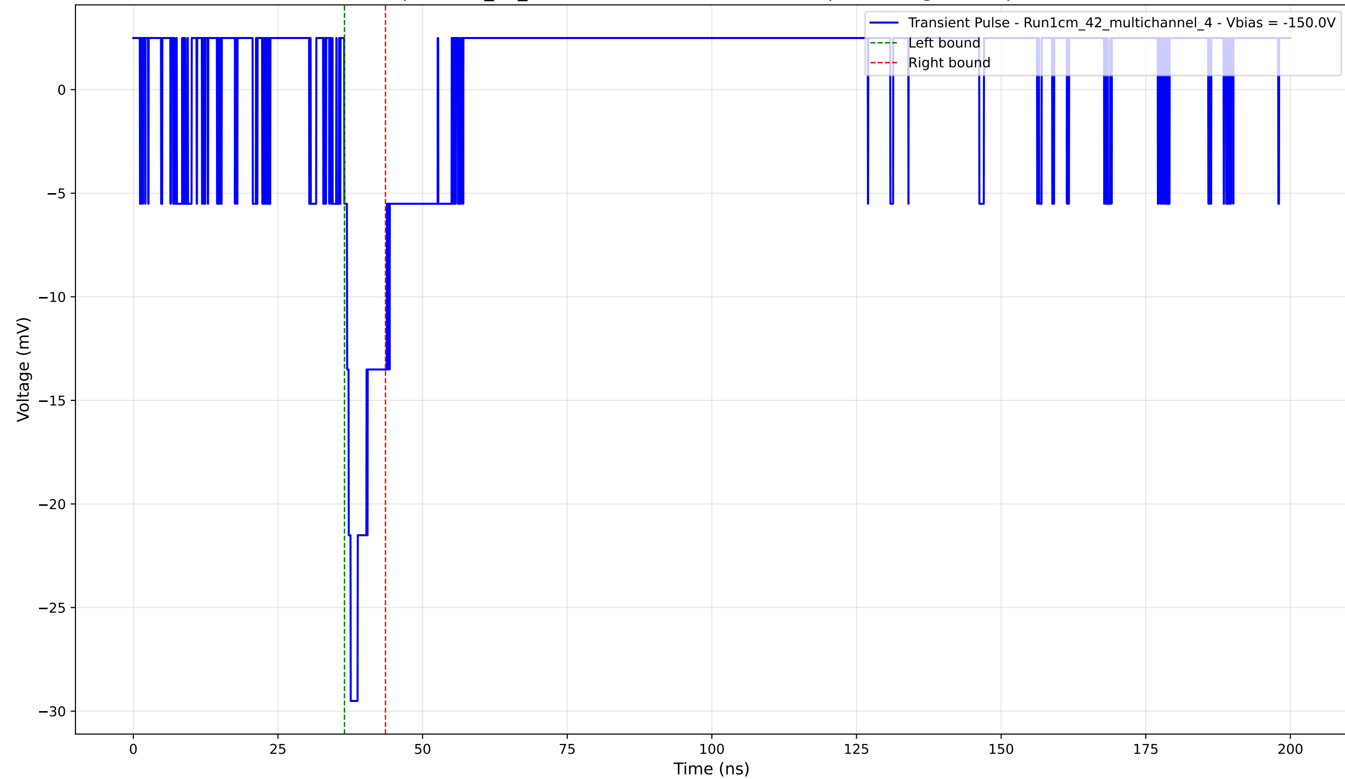
Transient Pulse - Sample: 1cm_42_multichannel - Position: 1485.0 \mu\text{m} - Charge: 2.55 pC - Rise Time: 1.12 ns
