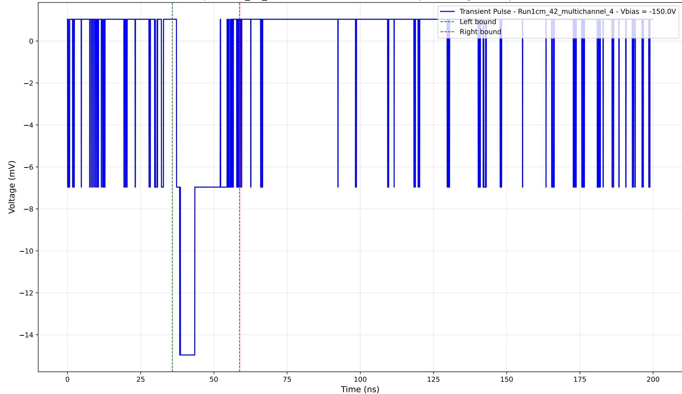
Transient Pulse - Sample: 1cm_42_multichannel - Position: 4580.0 \mu\text{m} - Charge: 3.37 pC - Rise Time: 1.10 ns
