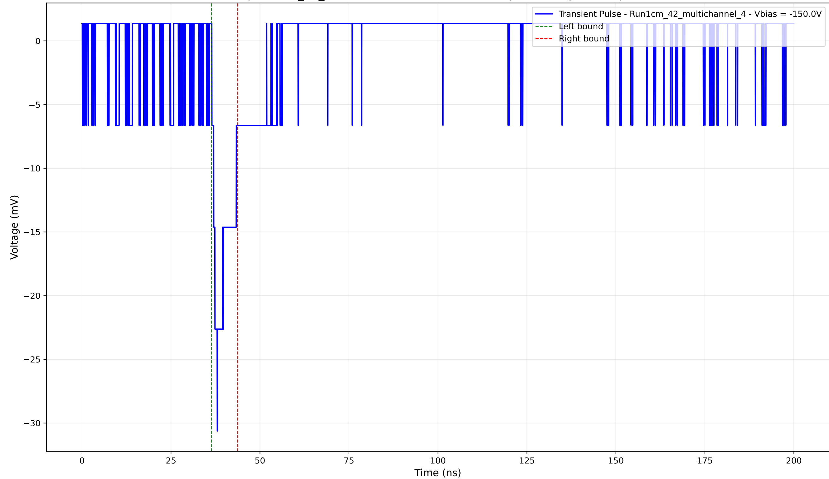
Transient Pulse - Sample: 1cm_42_multichannel - Position: 3300.0 \mu\text{m} - Charge: 2.35 pC - Rise Time: 1.51 ns
