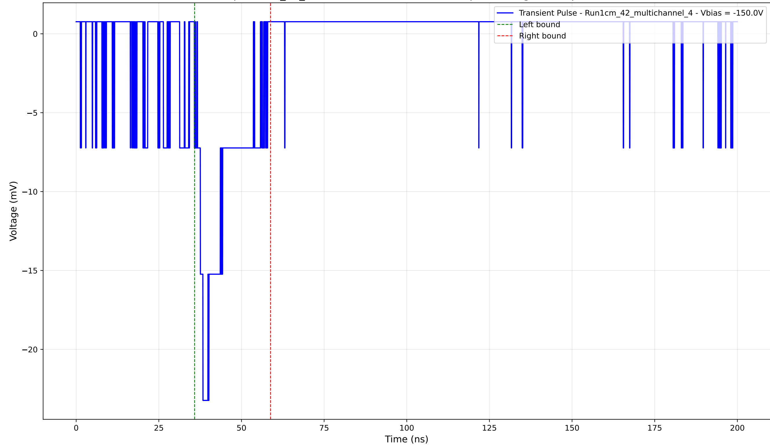
Transient Pulse - Sample: 1cm_42_multichannel - Position: 980.0 \mu\text{m} - Charge: 4.19 pC - Rise Time: 1.66 ns
