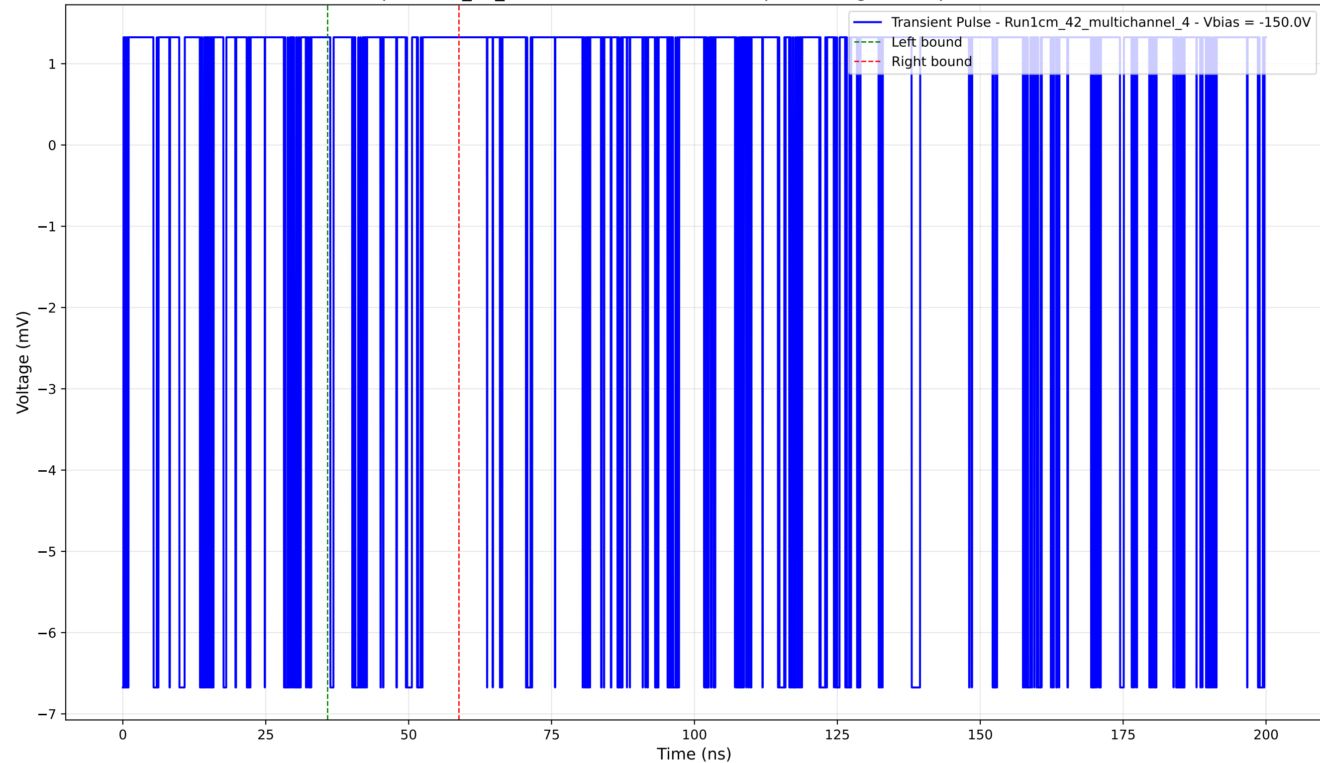
Transient Pulse - Sample: 1cm_42_multichannel - Position: 5.0 \mu\text{m} - Charge: 0.12 pC - Rise Time: 0.00 ns (N/A)
