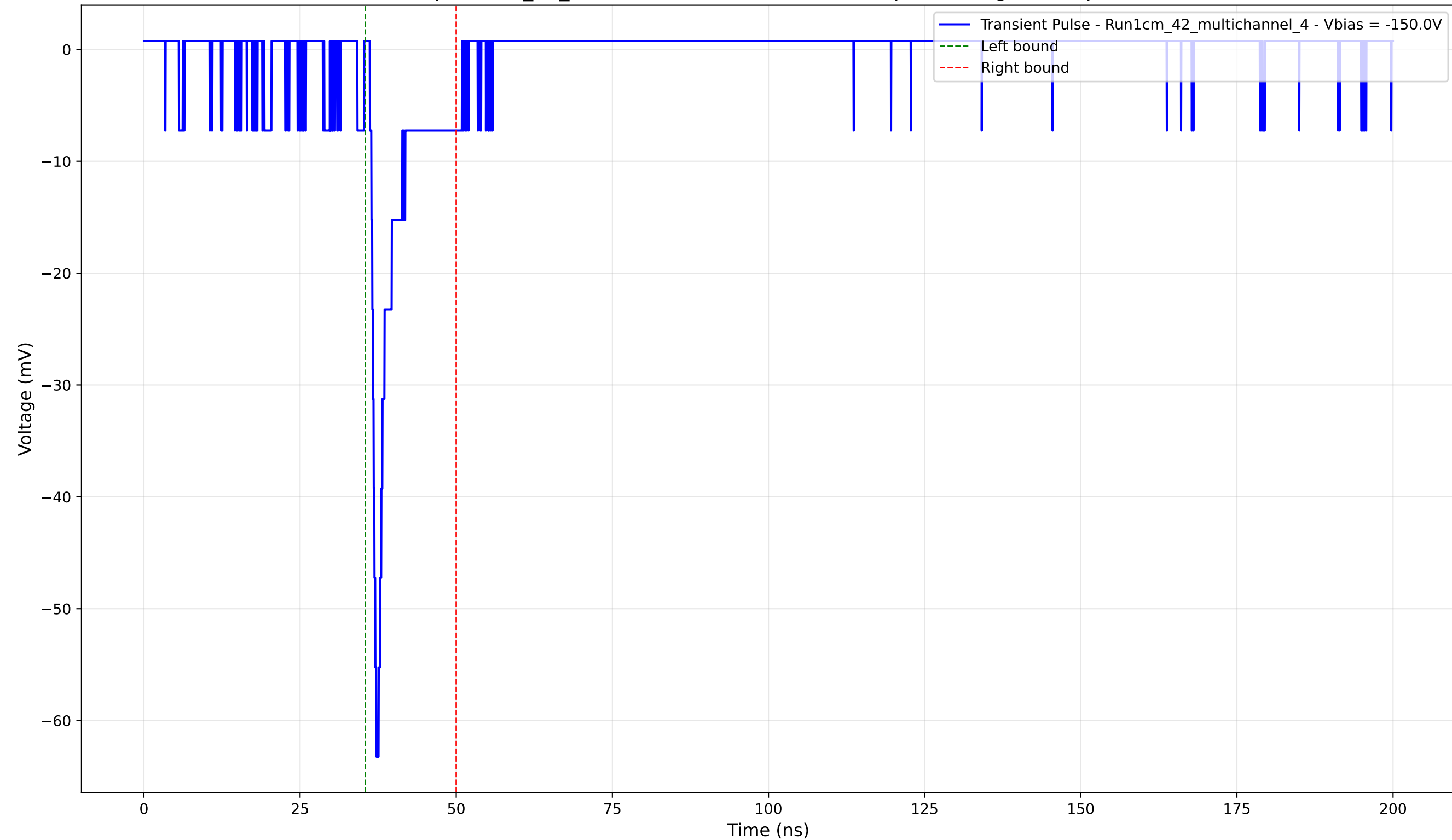
Transient Pulse - Sample: 1cm_42_multichannel - Position: 2105.0 \mu\text{m} - Charge: 4.20 pC - Rise Time: 1.04 ns
