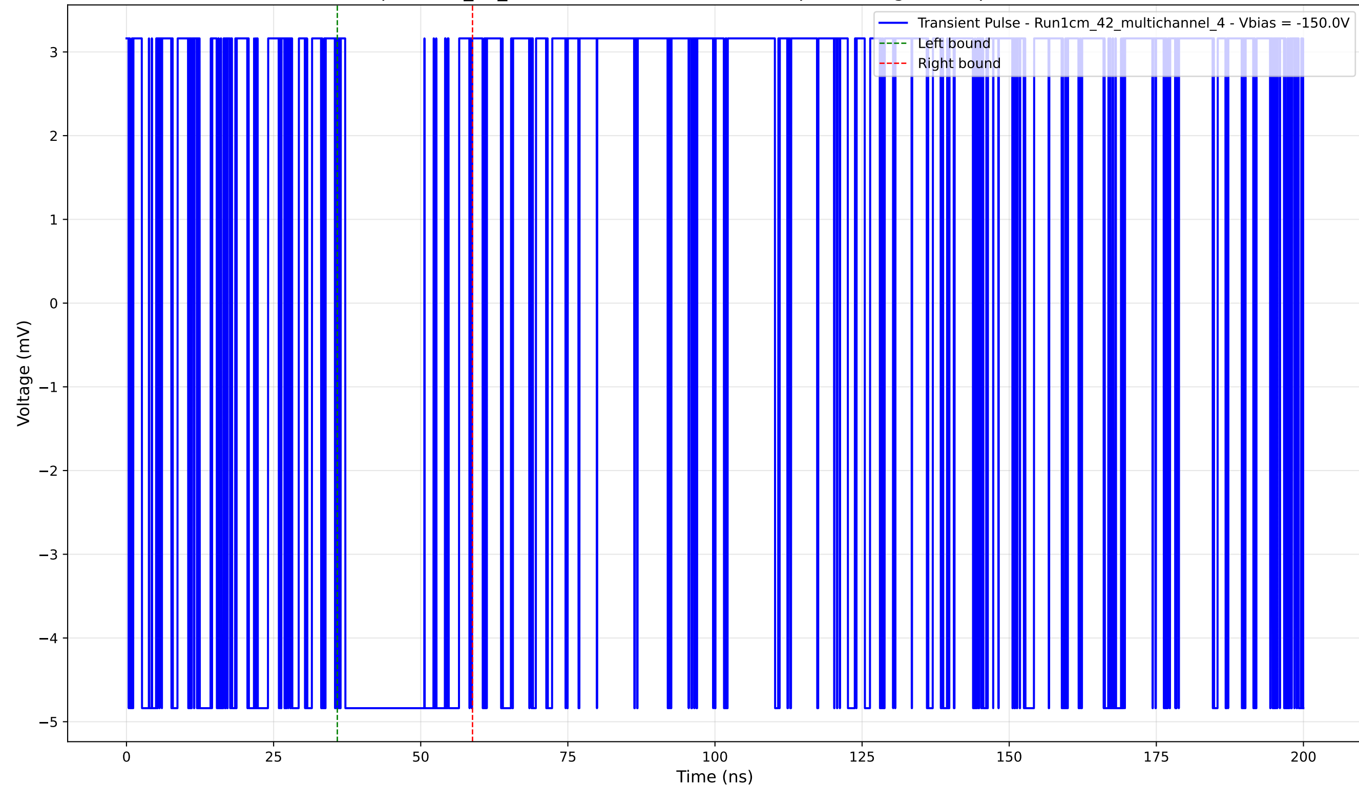
Transient Pulse - Sample: 1cm_42_multichannel - Position: 915.0 \mu\text{m} - Charge: 1.64 pC - Rise Time: 0.00 ns (N/A)
