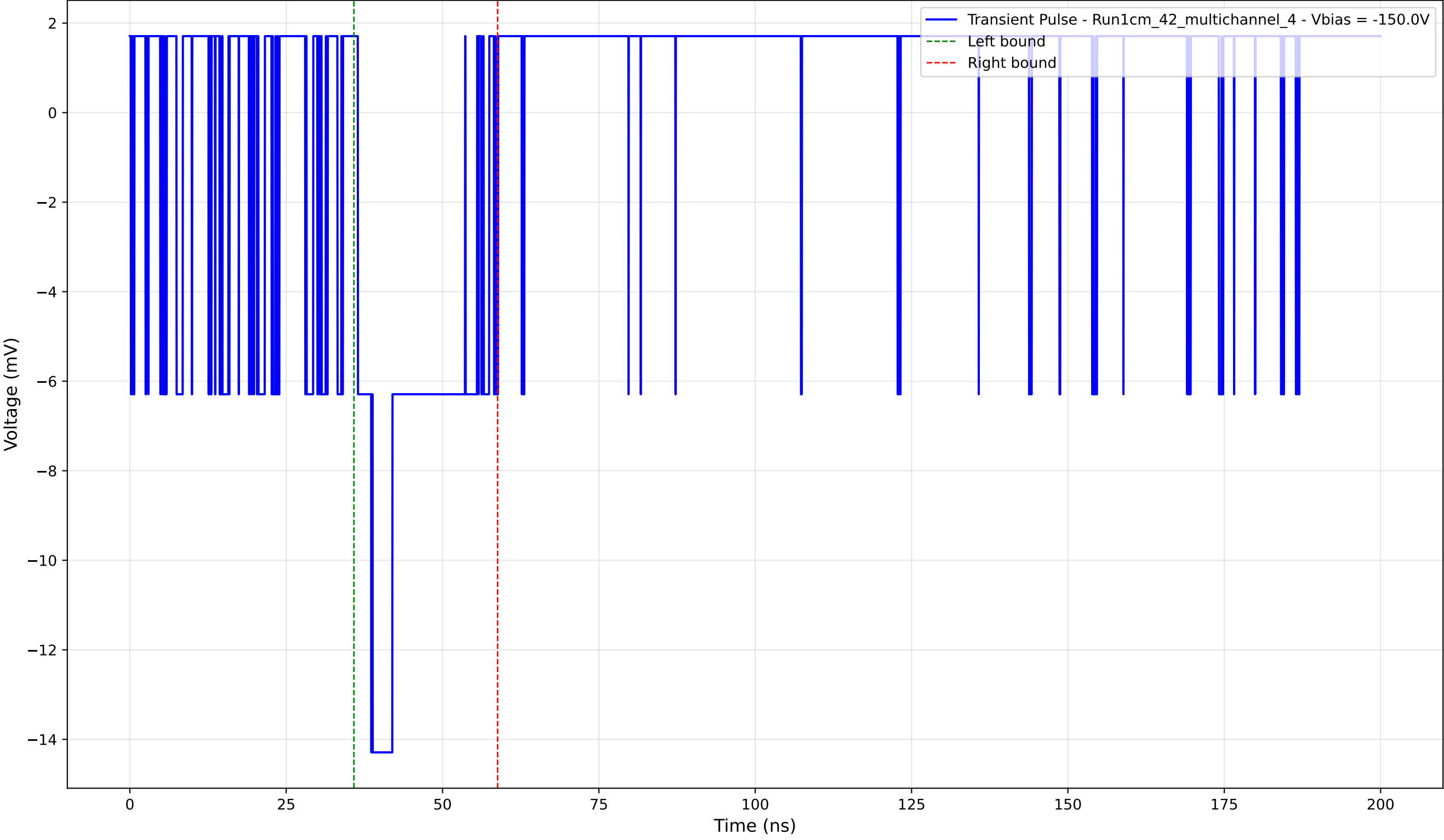
Transient Pulse - Sample: 1cm_42_multichannel - Position: 140.0 \mu\text{m} - Charge: 3.07 pC - Rise Time: 0.00 ns (N/A)
