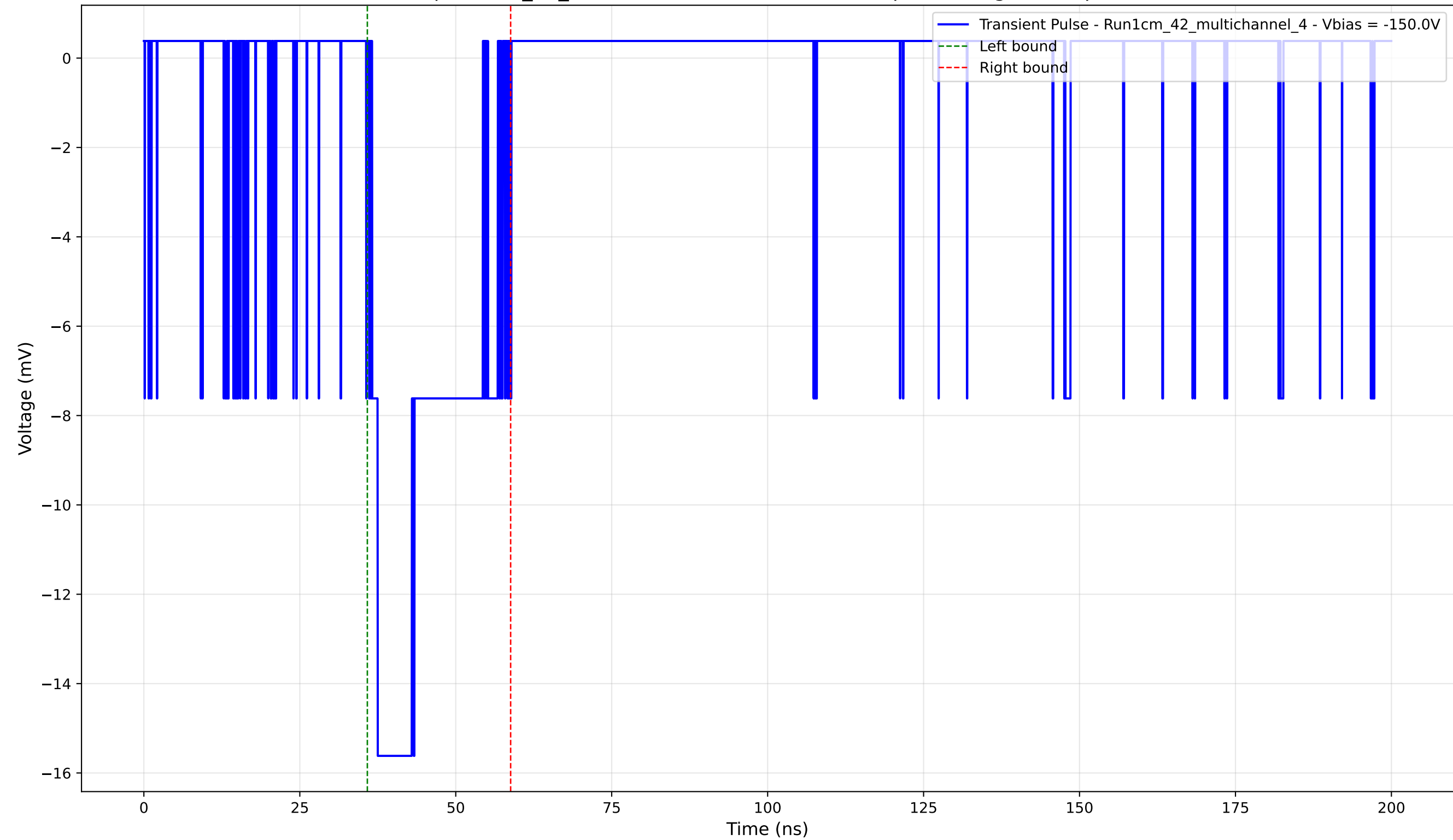
Transient Pulse - Sample: 1cm_42_multichannel - Position: 3620.0 \mu\text{m} - Charge: 4.00 pC - Rise Time: 0.90 ns
