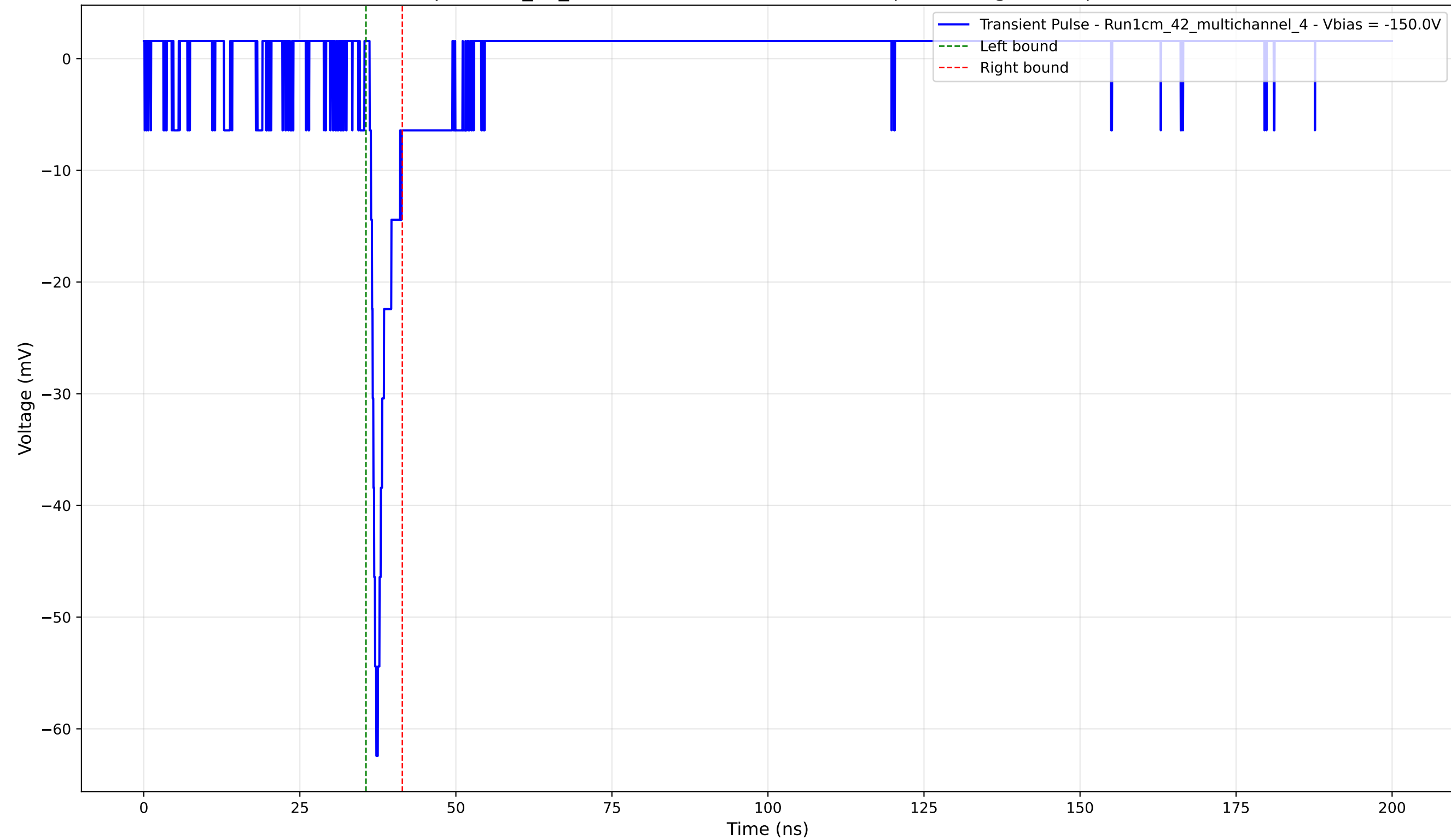
Transient Pulse - Sample: 1cm_42_multichannel - Position: 2660.0 \mu\text{m} - Charge: 2.76 pC - Rise Time: 1.06 ns
