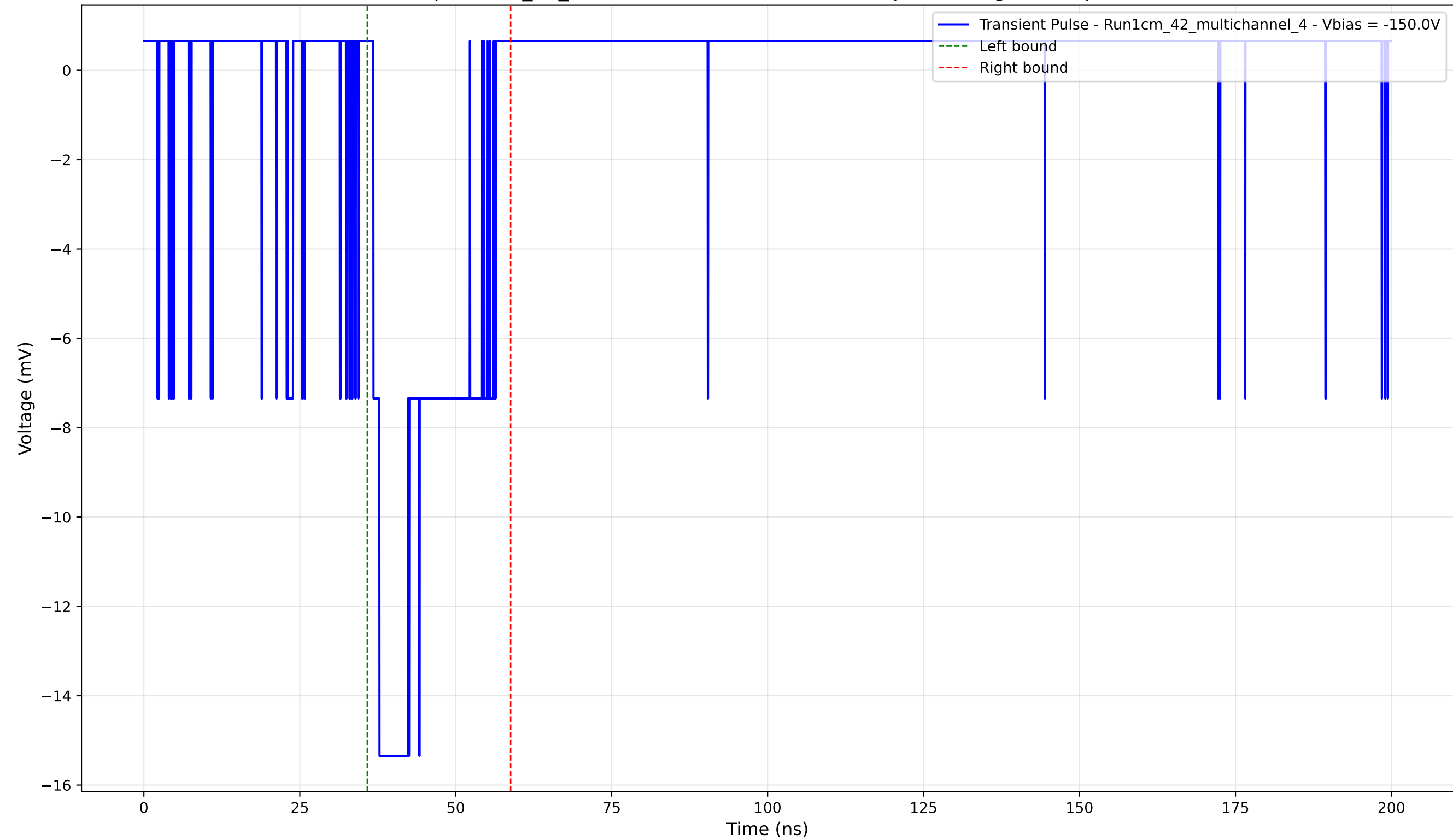
Transient Pulse - Sample: 1cm_42_multichannel - Position: 3815.0 \mu\text{m} - Charge: 3.52 pC - Rise Time: 0.98 ns
