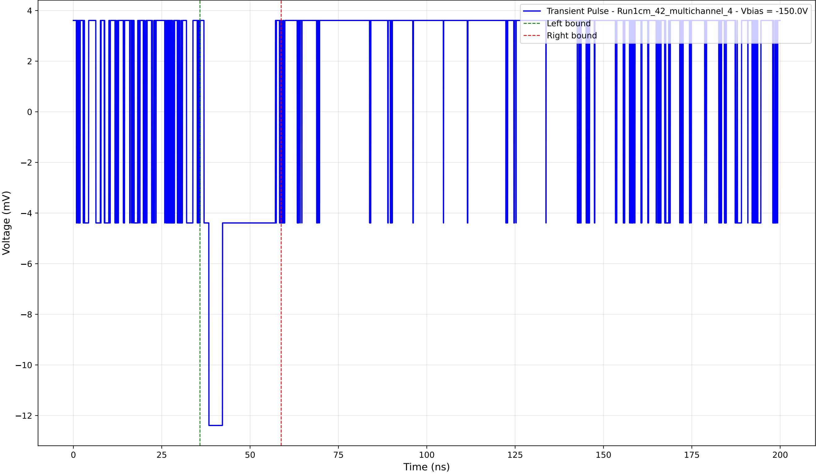
Transient Pulse - Sample: 1cm_42_multichannel - Position: 230.0 \mu\text{m} - Charge: 2.25 pC - Rise Time: 0.00 ns (N/A)
