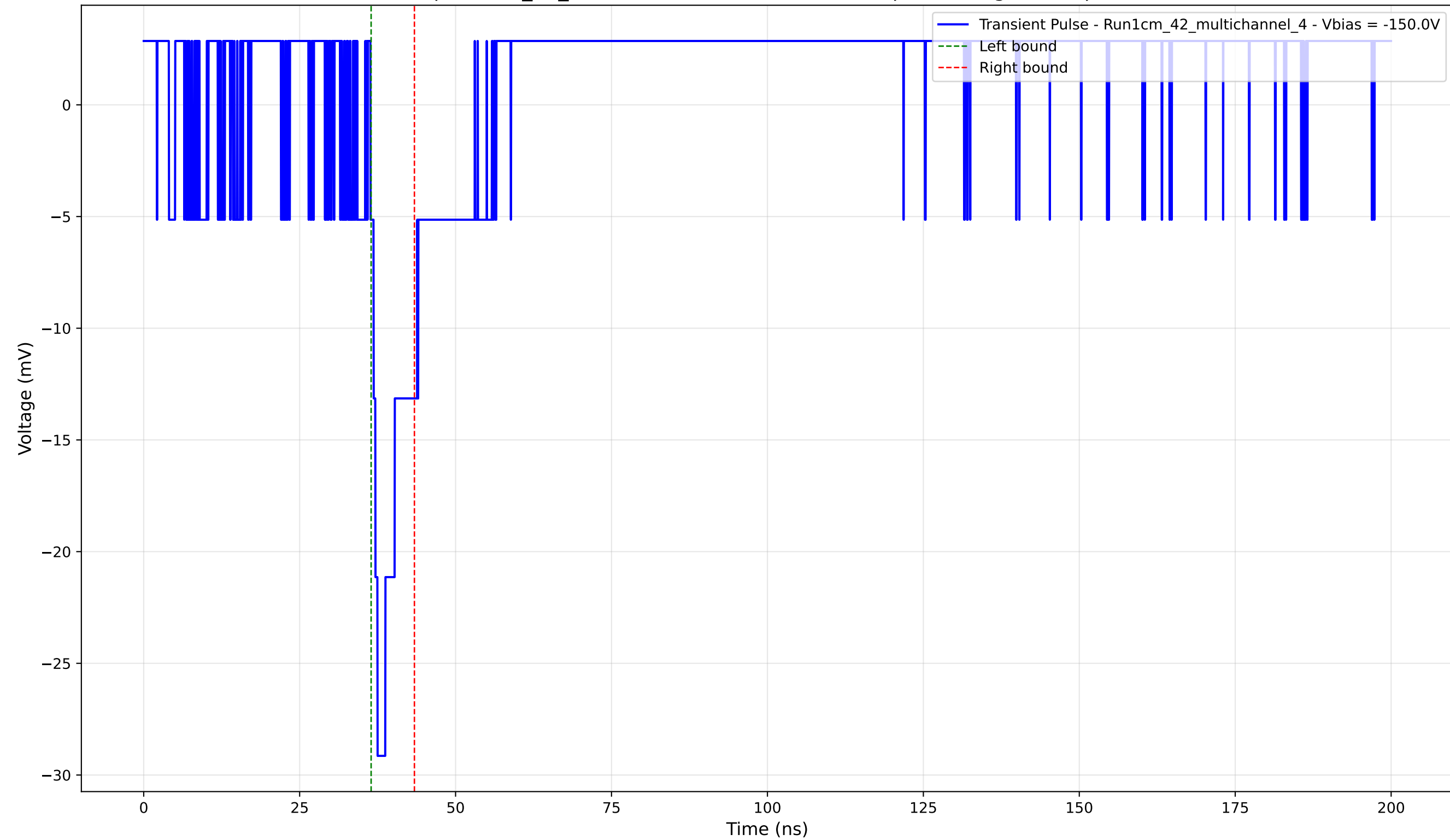
Transient Pulse - Sample: 1cm_42_multichannel - Position: 1525.0 \mu\text{m} - Charge: 2.46 pC - Rise Time: 1.14 ns
