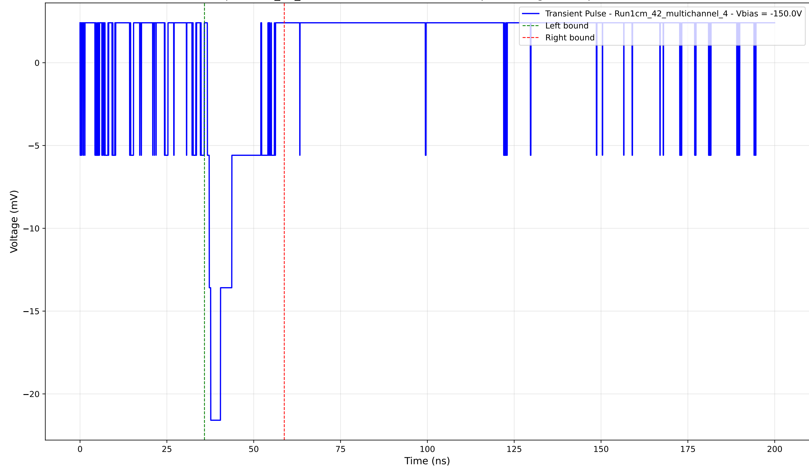
Transient Pulse - Sample: 1cm_42_multichannel - Position: 1245.0 \mu\text{m} - Charge: 3.44 pC - Rise Time: 0.00 ns (N/A)
