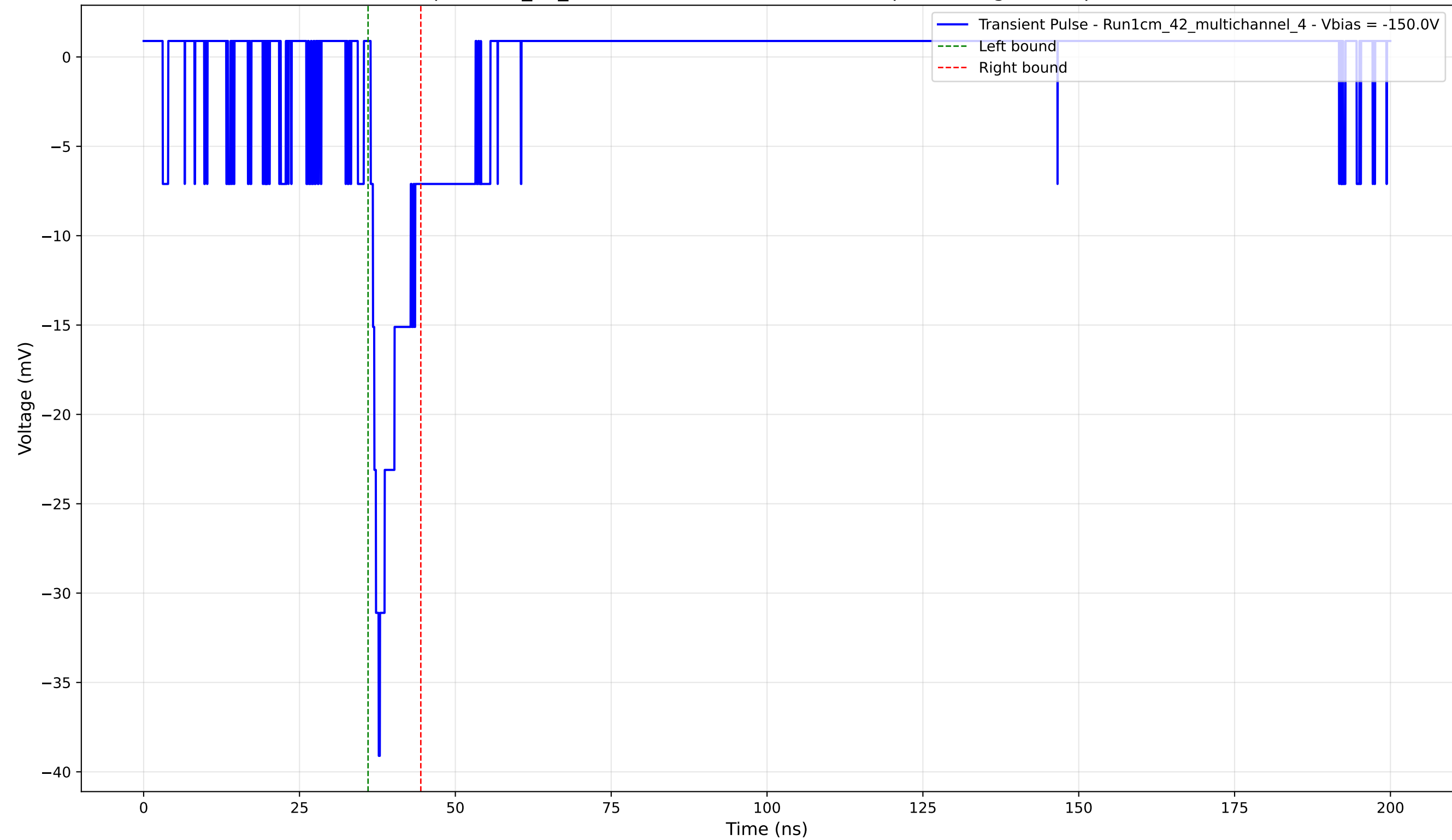
Transient Pulse - Sample: 1cm_42_multichannel - Position: 1640.0 \mu\text{m} - Charge: 2.94 pC - Rise Time: 1.29 ns
