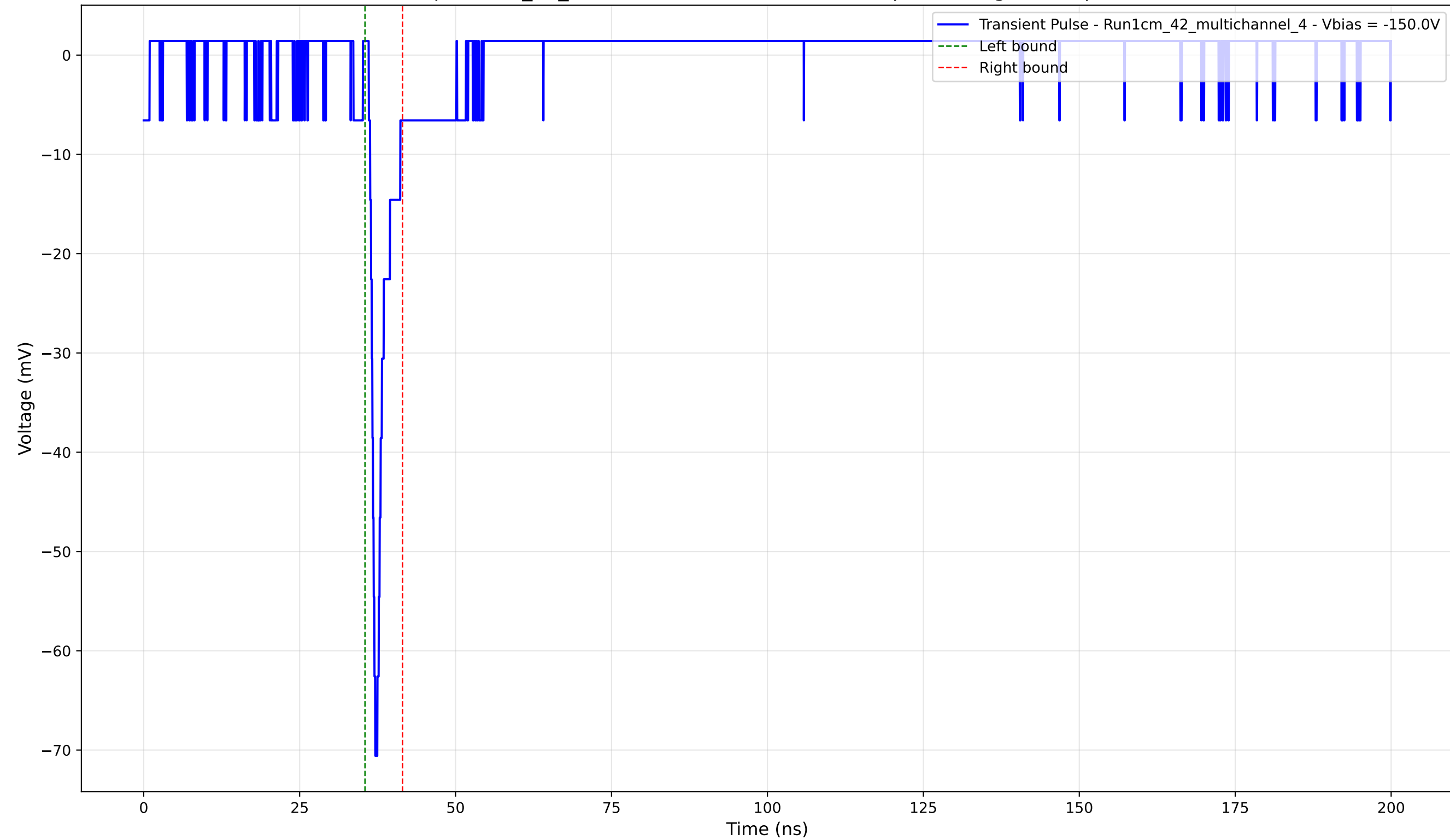
Transient Pulse - Sample: 1cm_42_multichannel - Position: 2555.0 \mu\text{m} - Charge: 3.02 pC - Rise Time: 0.84 ns
