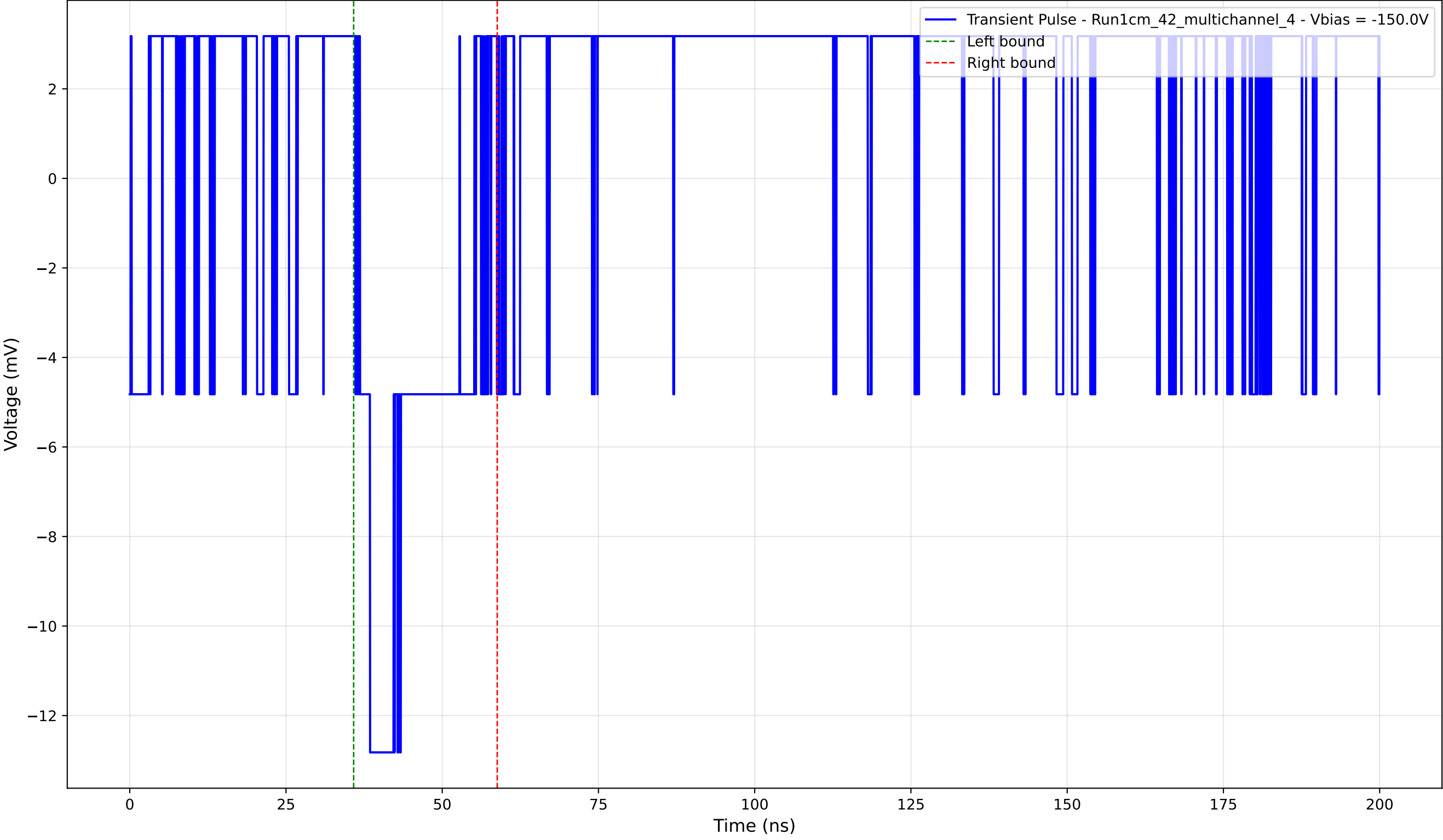
Transient Pulse - Sample: 1cm_42_multichannel - Position: 155.0 \mu\text{m} - Charge: 2.35 pC - Rise Time: 0.00 ns (N/A)
