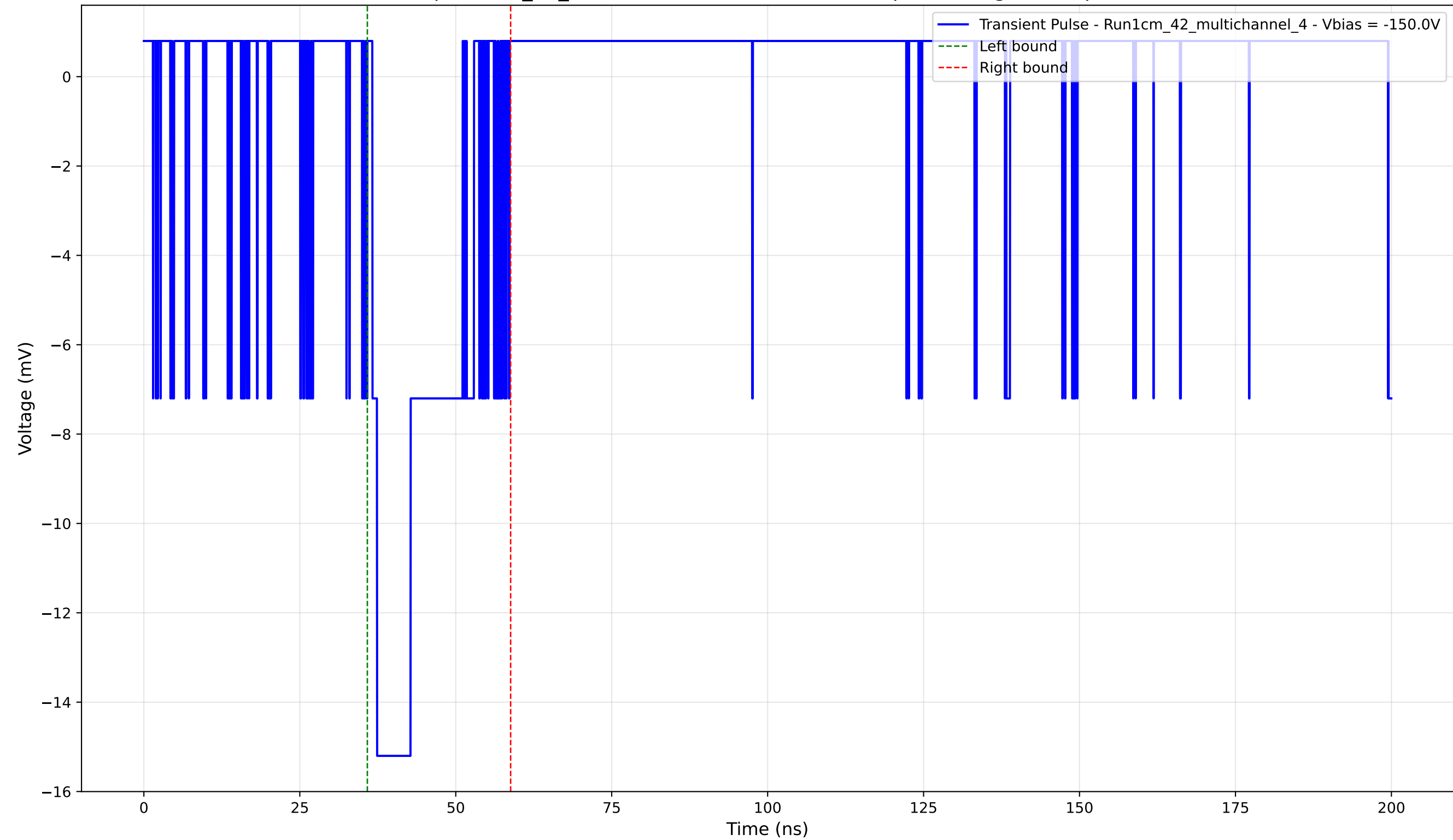
Transient Pulse - Sample: 1cm_42_multichannel - Position: 3595.0 \mu\text{m} - Charge: 3.35 pC - Rise Time: 0.76 ns
