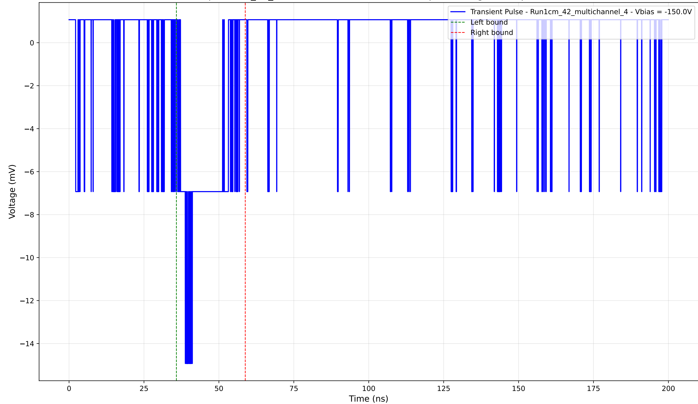
Transient Pulse - Sample: 1cm_42_multichannel - Position: 4460.0 \mu\text{m} - Charge: 2.45 pC - Rise Time: 1.60 ns
