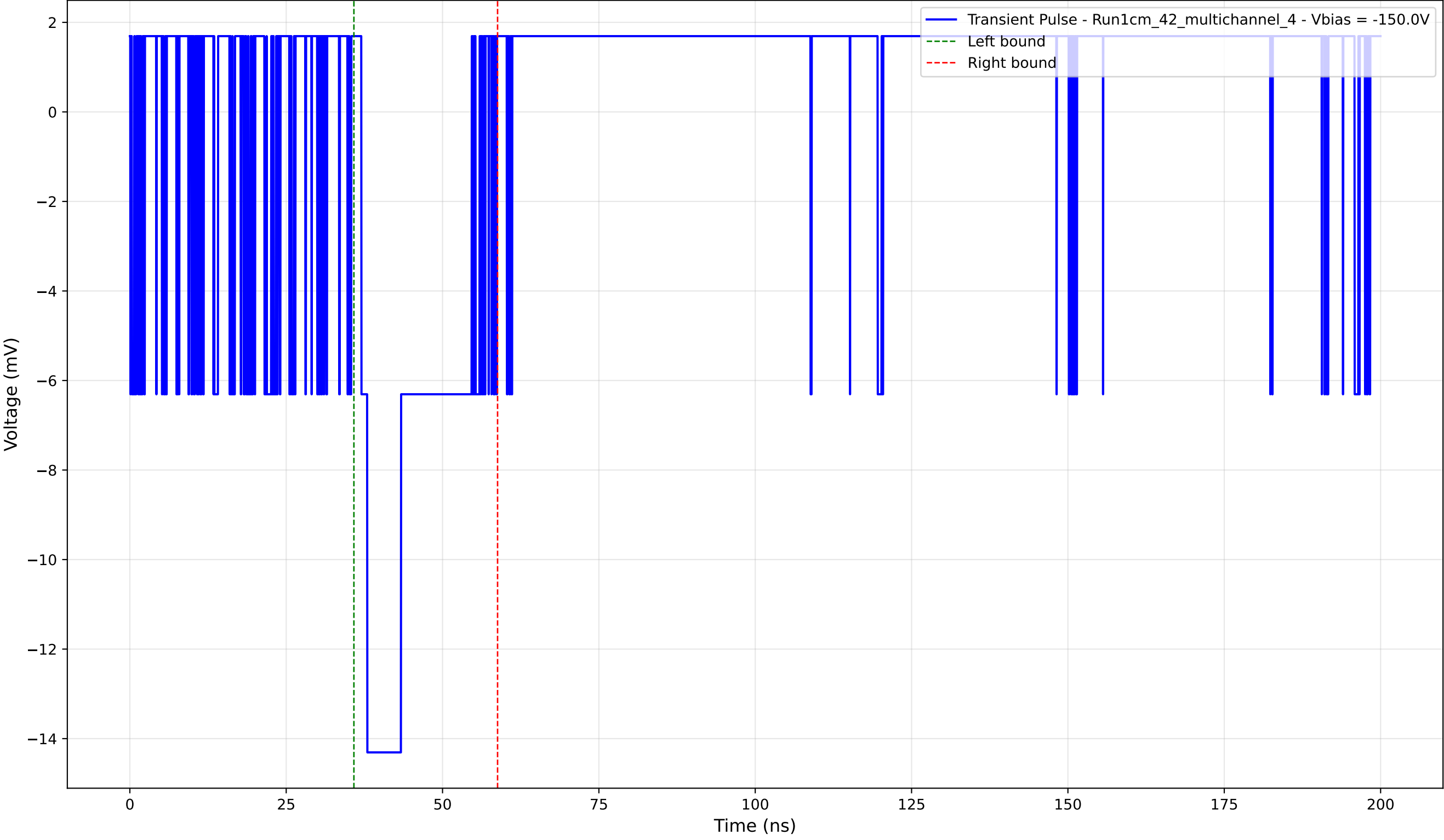
Transient Pulse - Sample: 1cm_42_multichannel - Position: 620.0 \mu\text{m} - Charge: 3.17 pC - Rise Time: 0.00 ns (N/A)
