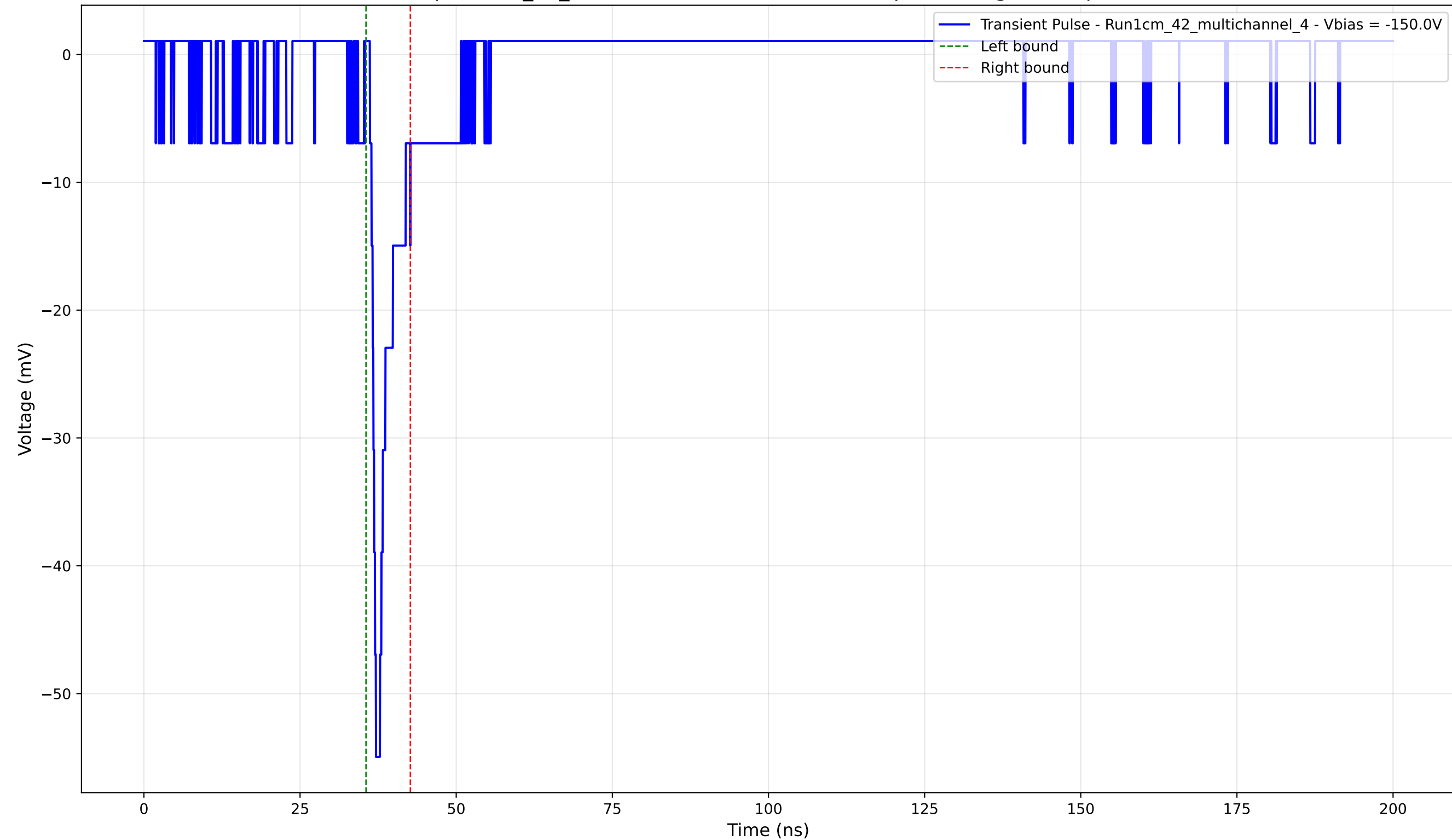
Transient Pulse - Sample: 1cm_42_multichannel - Position: 2045.0 \mu\text{m} - Charge: 3.08 pC - Rise Time: 0.96 ns
