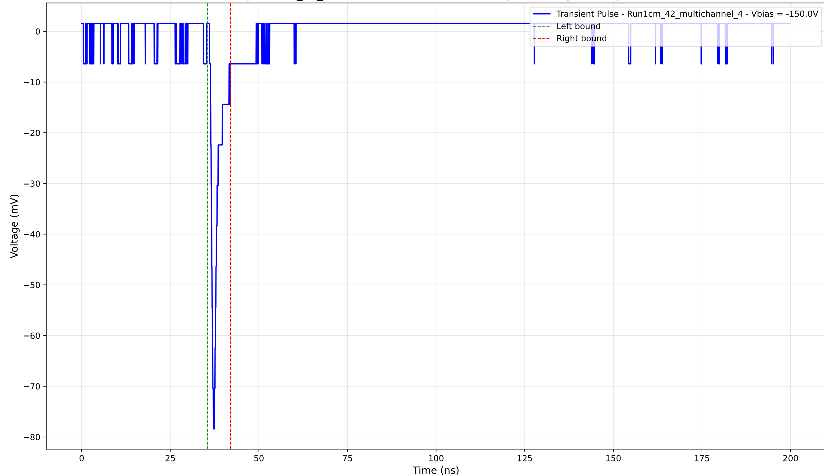
Transient Pulse - Sample: 1cm_42_multichannel - Position: 2535.0 \mu\text{m} - Charge: 3.37 pC - Rise Time: 0.86 ns
