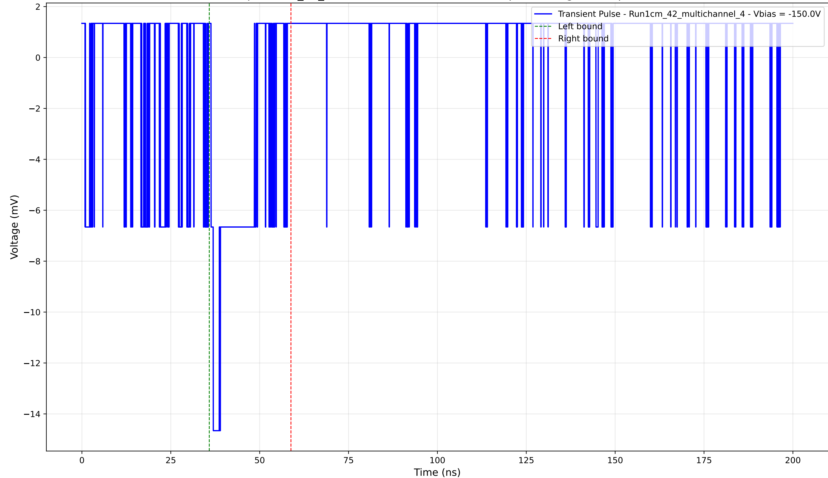
Transient Pulse - Sample: 1cm_42_multichannel - Position: 2940.0 \mu\text{m} - Charge: 2.00 pC - Rise Time: 0.64 ns
