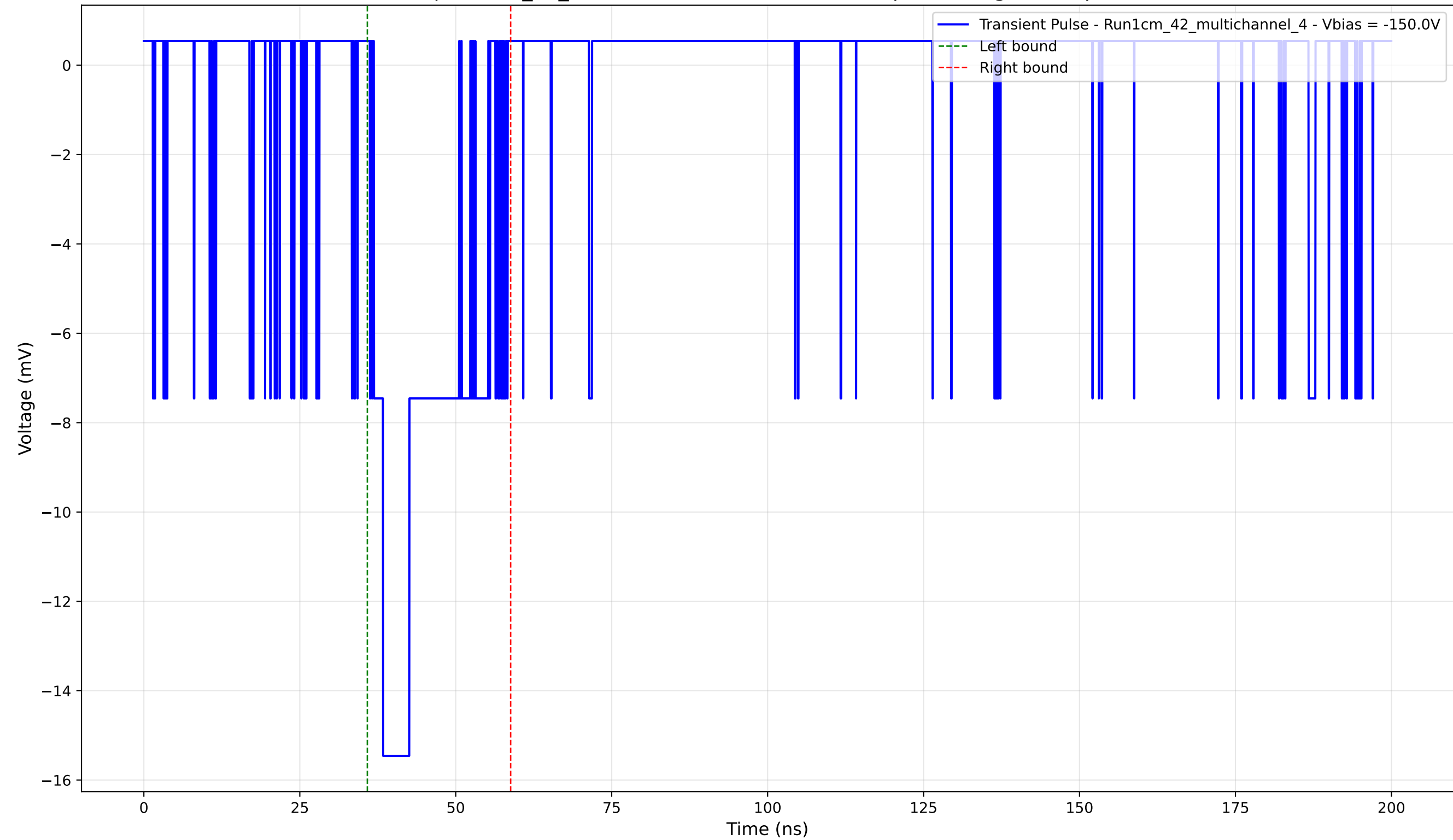
Transient Pulse - Sample: 1cm_42_multichannel - Position: 4695.0 \mu\text{m} - Charge: 3.46 pC - Rise Time: 1.48 ns
