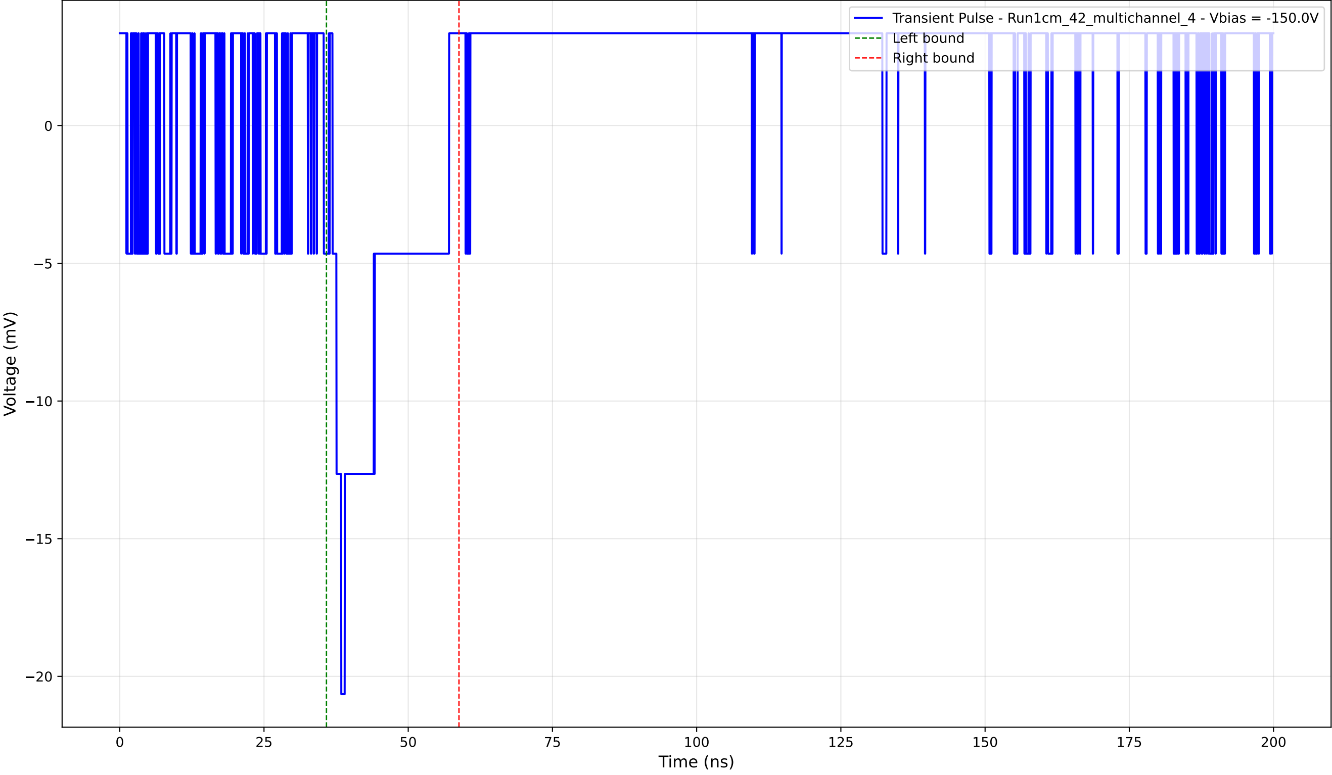
Transient Pulse - Sample: 1cm_42_multichannel - Position: 995.0 \mu\text{m} - Charge: 2.92 pC - Rise Time: 0.00 ns (N/A)
