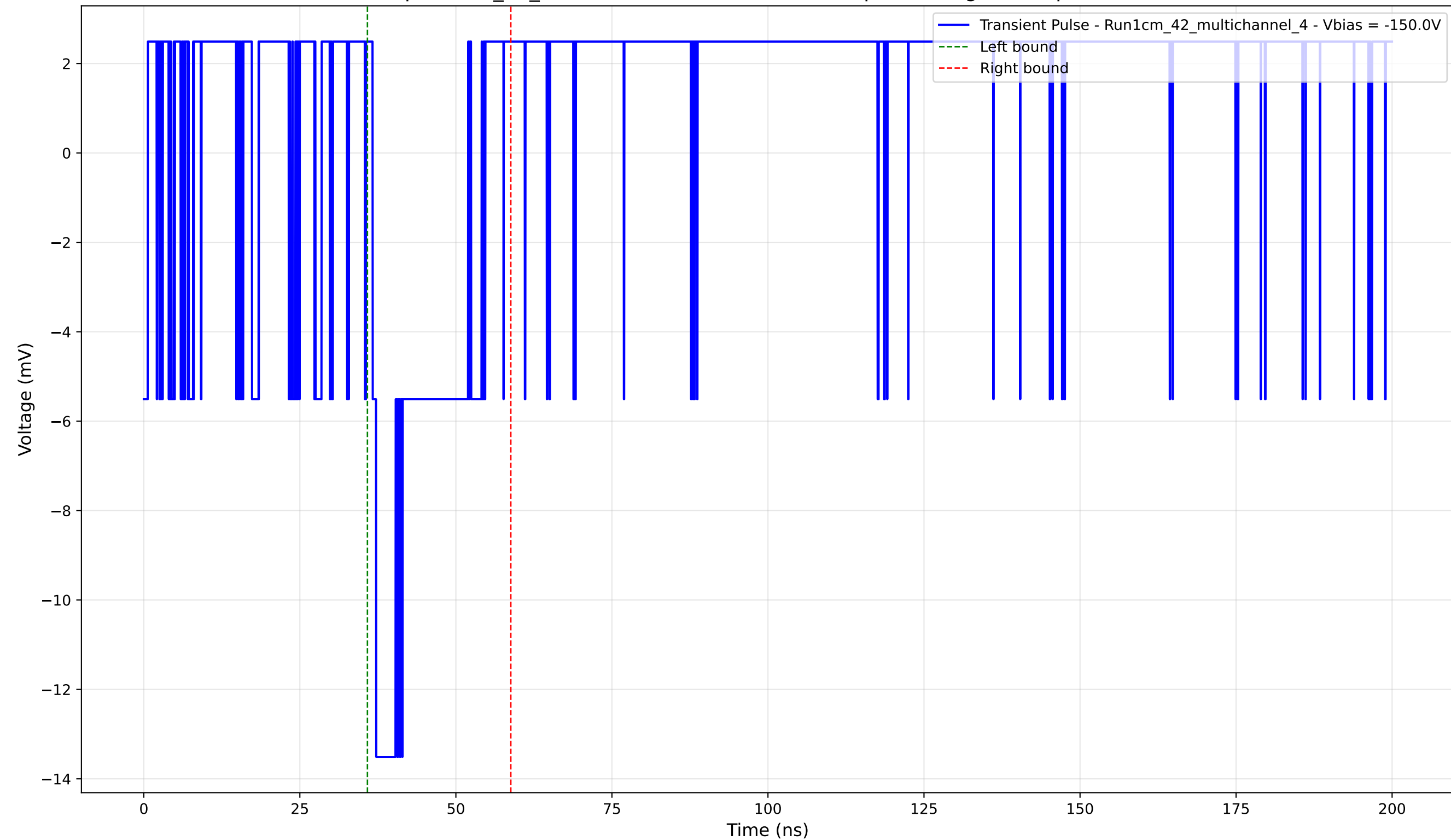
Transient Pulse - Sample: 1cm_42_multichannel - Position: 3340.0 \mu\text{m} - Charge: 2.23 pC - Rise Time: 0.00 ns (N/A)
