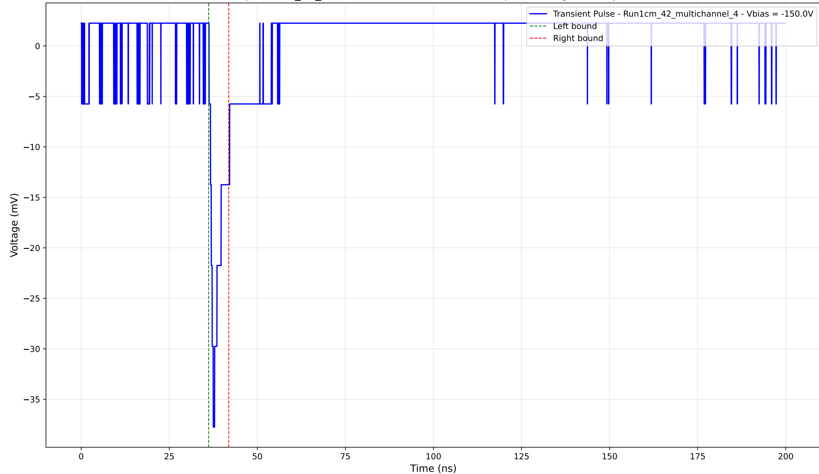
Transient Pulse - Sample: 1cm_42_multichannel - Position: 3050.0 \mu\text{m} - Charge: 2.20 pC - Rise Time: 1.19 ns
