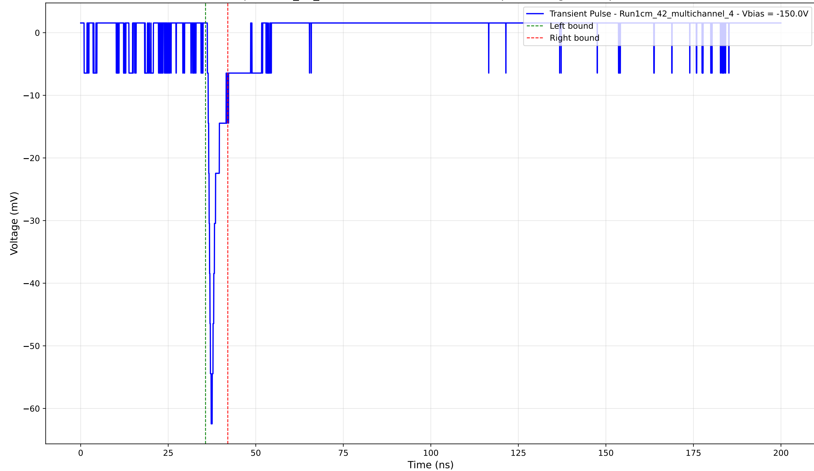
Transient Pulse - Sample: 1cm_42_multichannel - Position: 2675.0 \mu\text{m} - Charge: 2.93 pC - Rise Time: 1.08 ns
