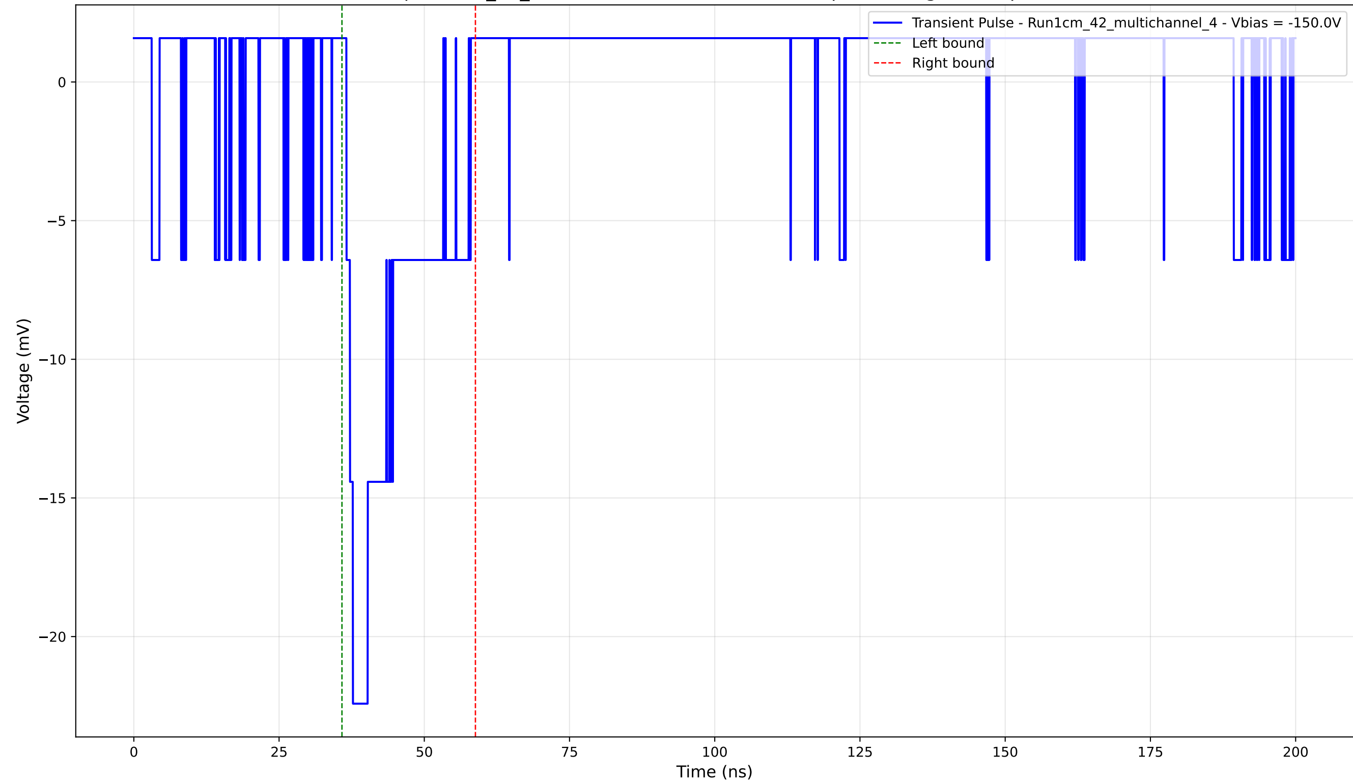
Transient Pulse - Sample: 1cm_42_multichannel - Position: 1235.0 \mu\text{m} - Charge: 4.17 pC - Rise Time: 1.12 ns
