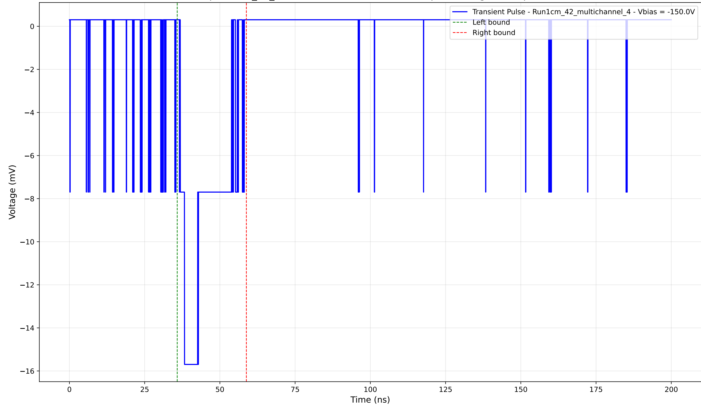
Transient Pulse - Sample: 1cm_42_multichannel - Position: 4150.0 \mu\text{m} - Charge: 3.59 pC - Rise Time: 1.42 ns
