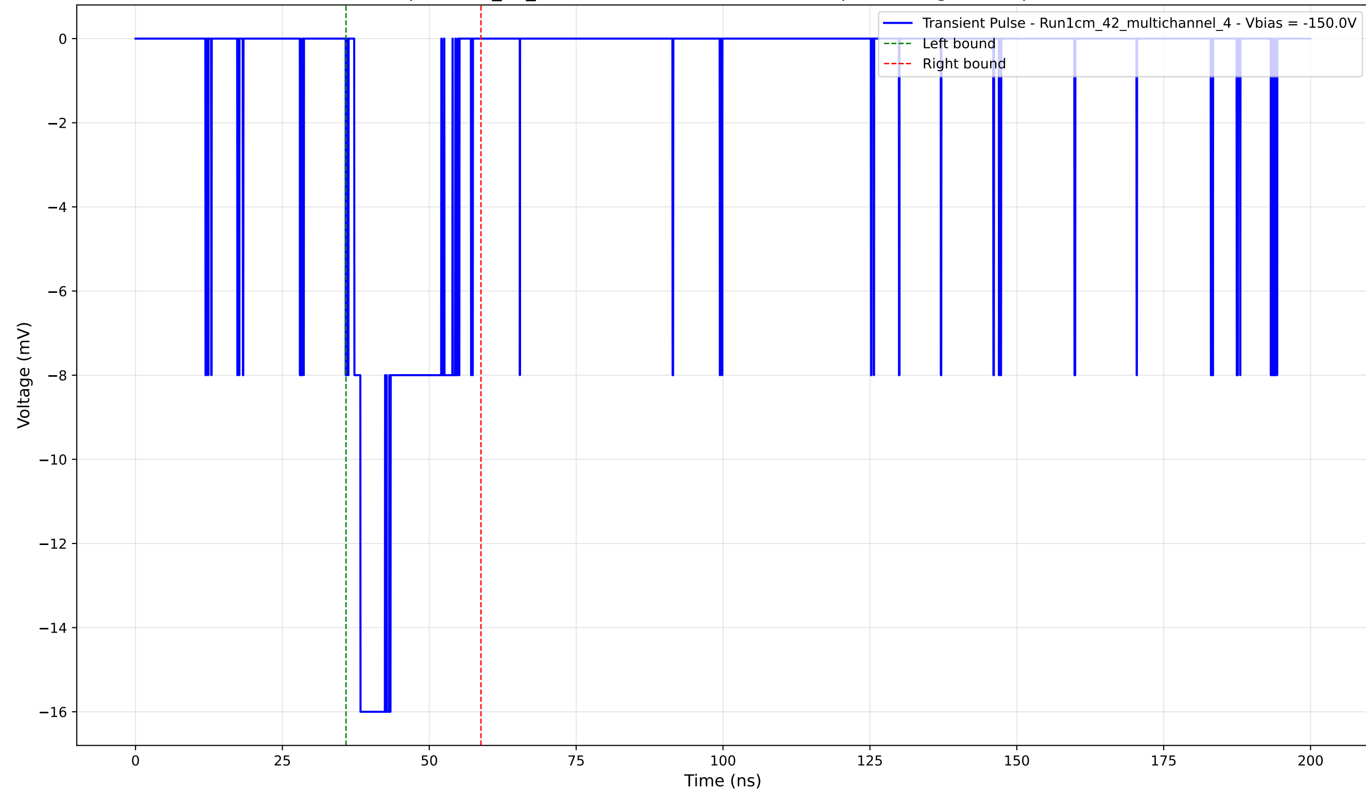
Transient Pulse - Sample: 1cm_42_multichannel - Position: 4250.0 \mu\text{m} - Charge: 3.60 pC - Rise Time: 1.06 ns
