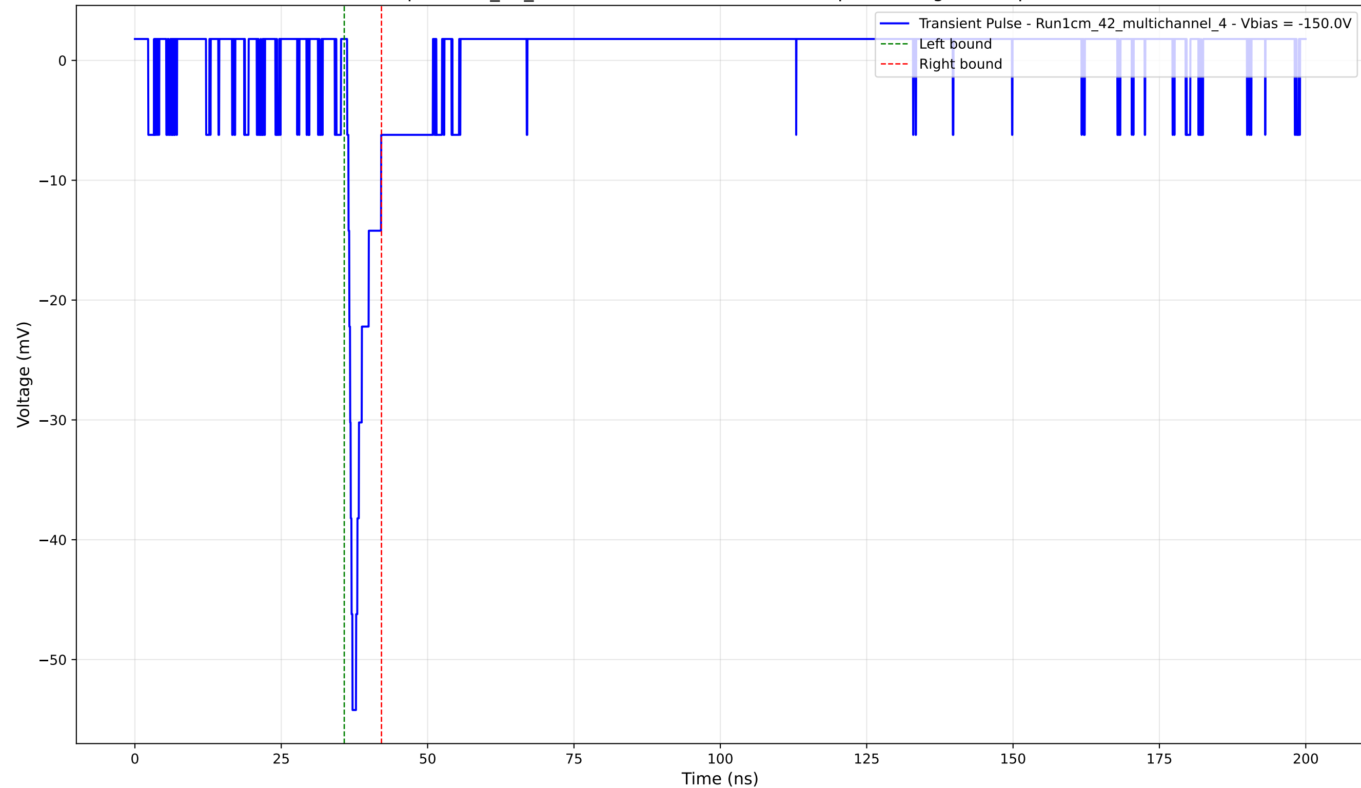
Transient Pulse - Sample: 1cm_42_multichannel - Position: 2745.0 \mu\text{m} - Charge: 2.94 pC - Rise Time: 0.90 ns
