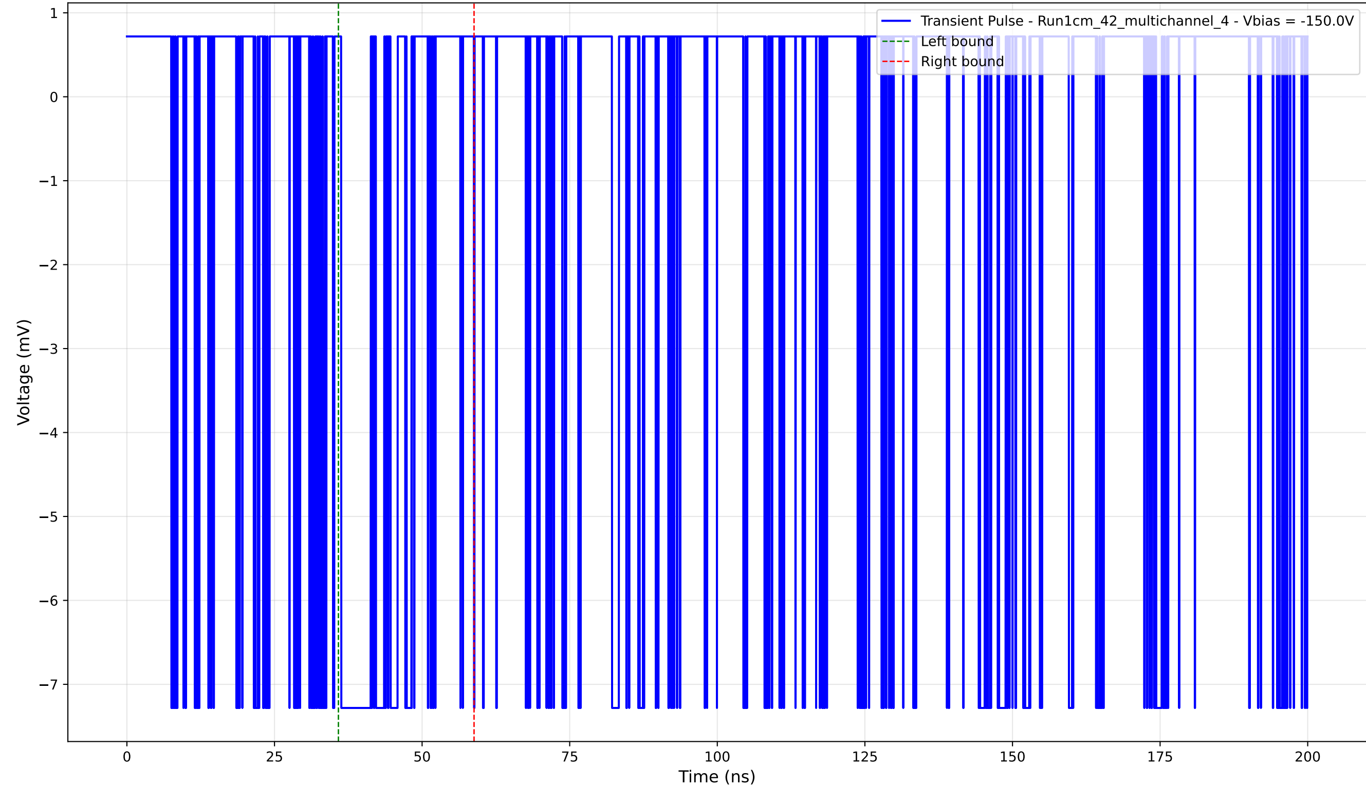
Transient Pulse - Sample: 1cm_42_multichannel - Position: 2415.0 \mu\text{m} - Charge: 1.25 pC - Rise Time: 0.02 ns
