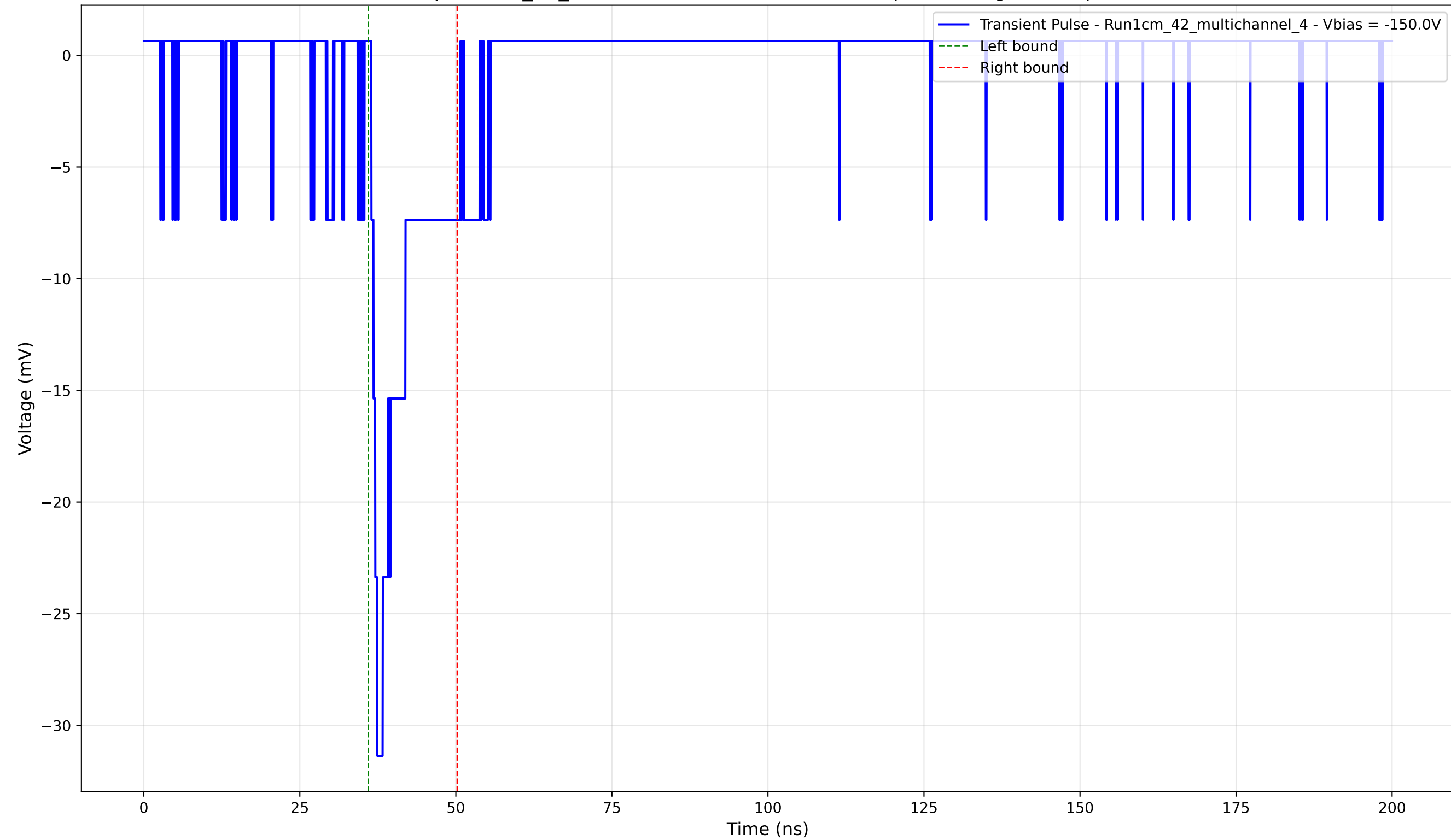
Transient Pulse - Sample: 1cm_42_multichannel - Position: 3120.0 \mu\text{m} - Charge: 3.34 pC - Rise Time: 0.95 ns
