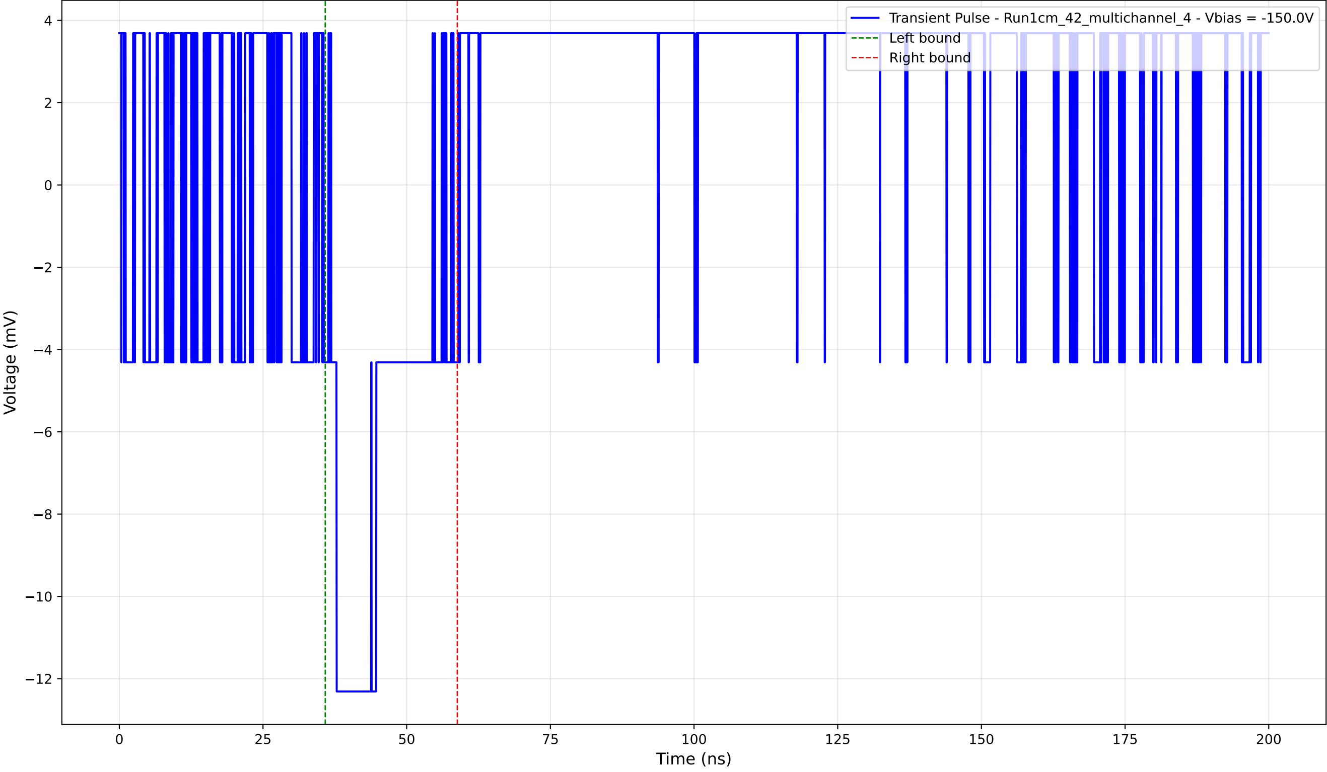
Transient Pulse - Sample: 1cm_42_multichannel - Position: 725.0 \mu\text{m} - Charge: 2.89 pC - Rise Time: 0.00 ns (N/A)
