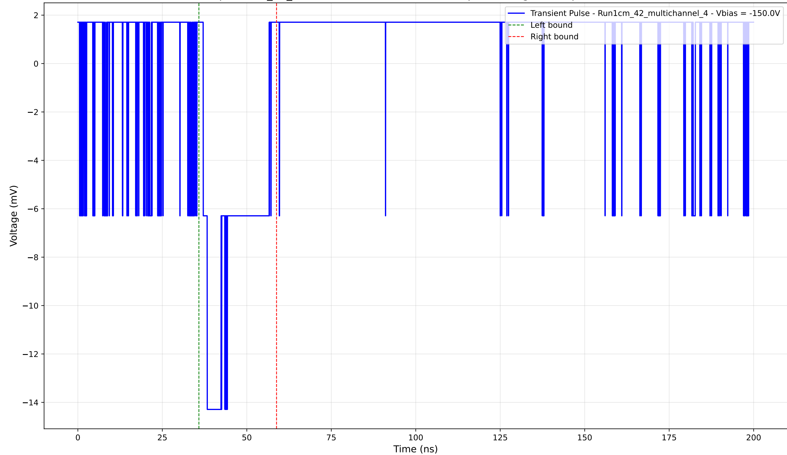
Transient Pulse - Sample: 1cm_42_multichannel - Position: 4515.0 \mu\text{m} - Charge: 3.07 pC - Rise Time: 0.00 ns (N/A)
