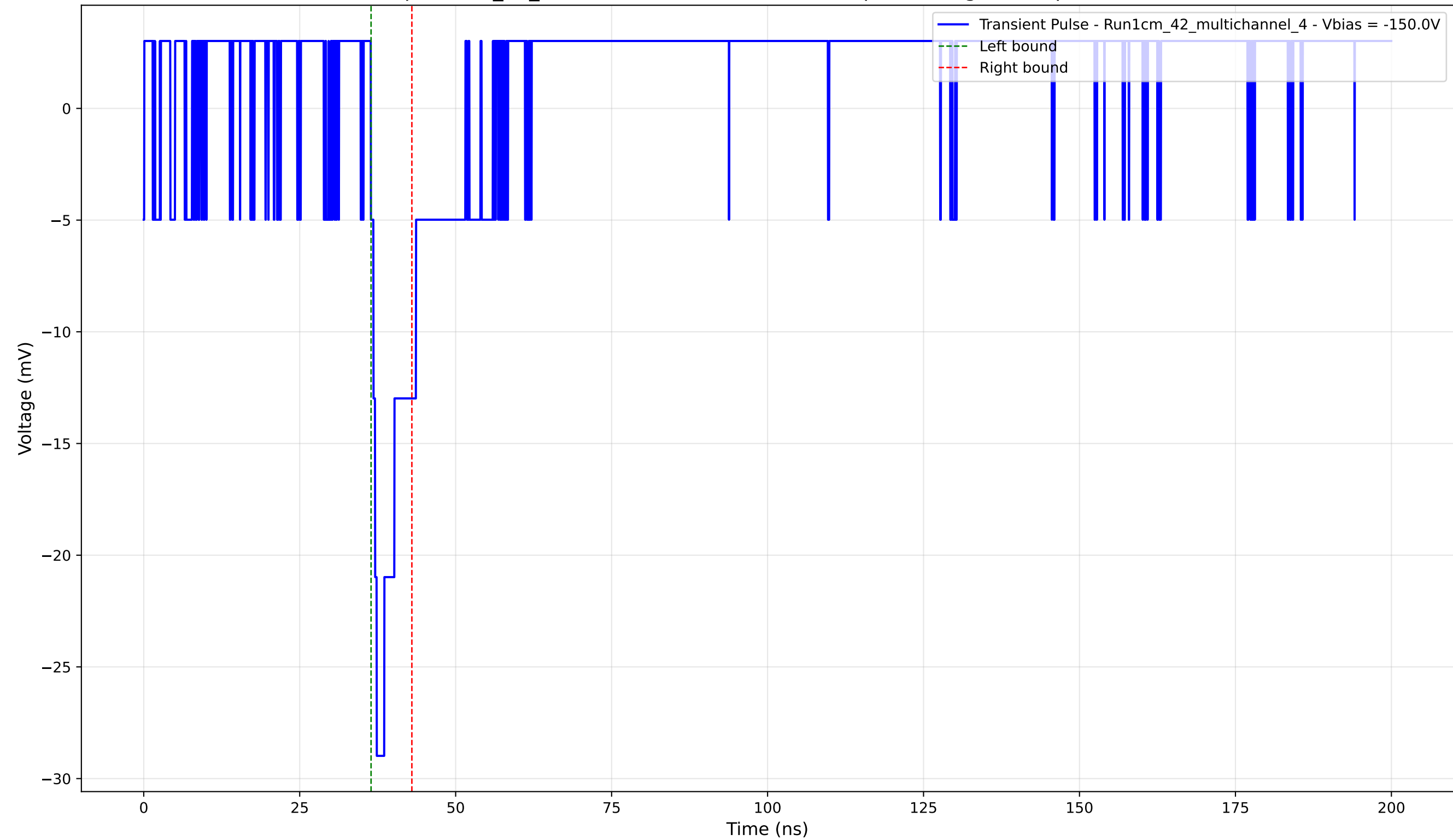
Transient Pulse - Sample: 1cm_42_multichannel - Position: 1605.0 \mu\text{m} - Charge: 2.33 pC - Rise Time: 0.00 ns (N/A)
