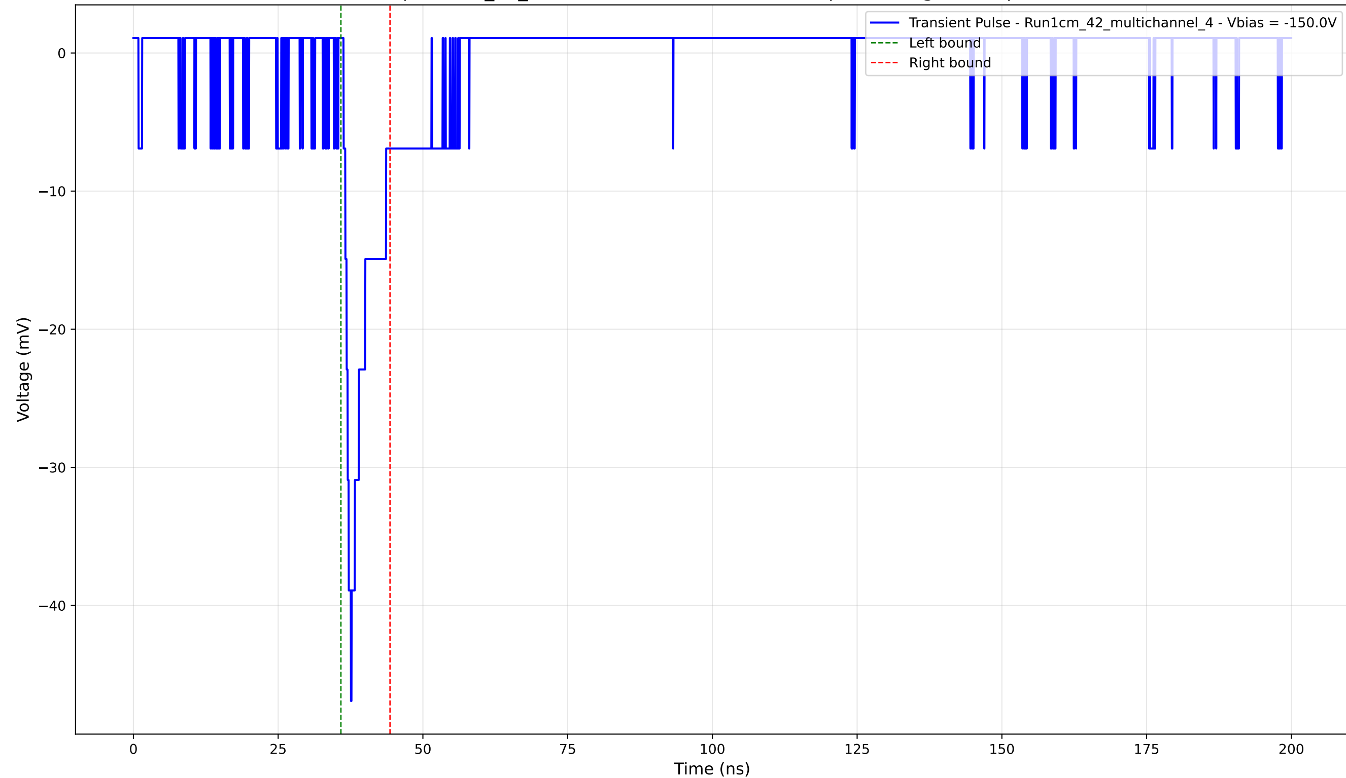
Transient Pulse - Sample: 1cm_42_multichannel - Position: 1785.0 \mu\text{m} - Charge: 3.24 pC - Rise Time: 1.27 ns
