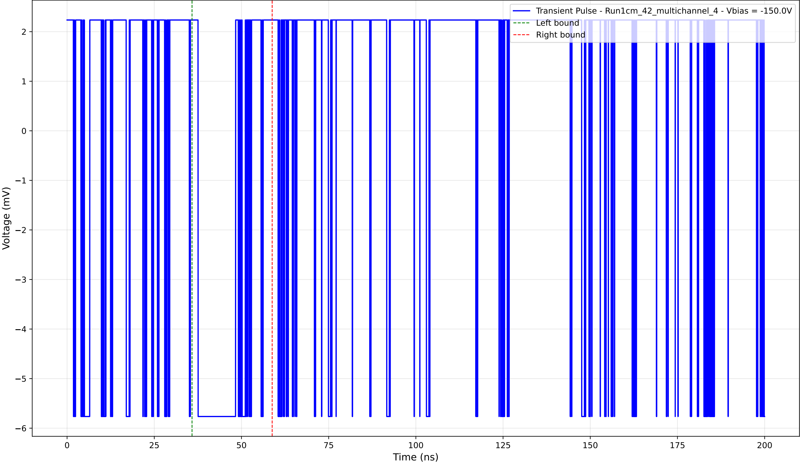
Transient Pulse - Sample: 1cm_42_multichannel - Position: 4440.0 \mu\text{m} - Charge: 1.17 pC - Rise Time: 0.00 ns (N/A)
