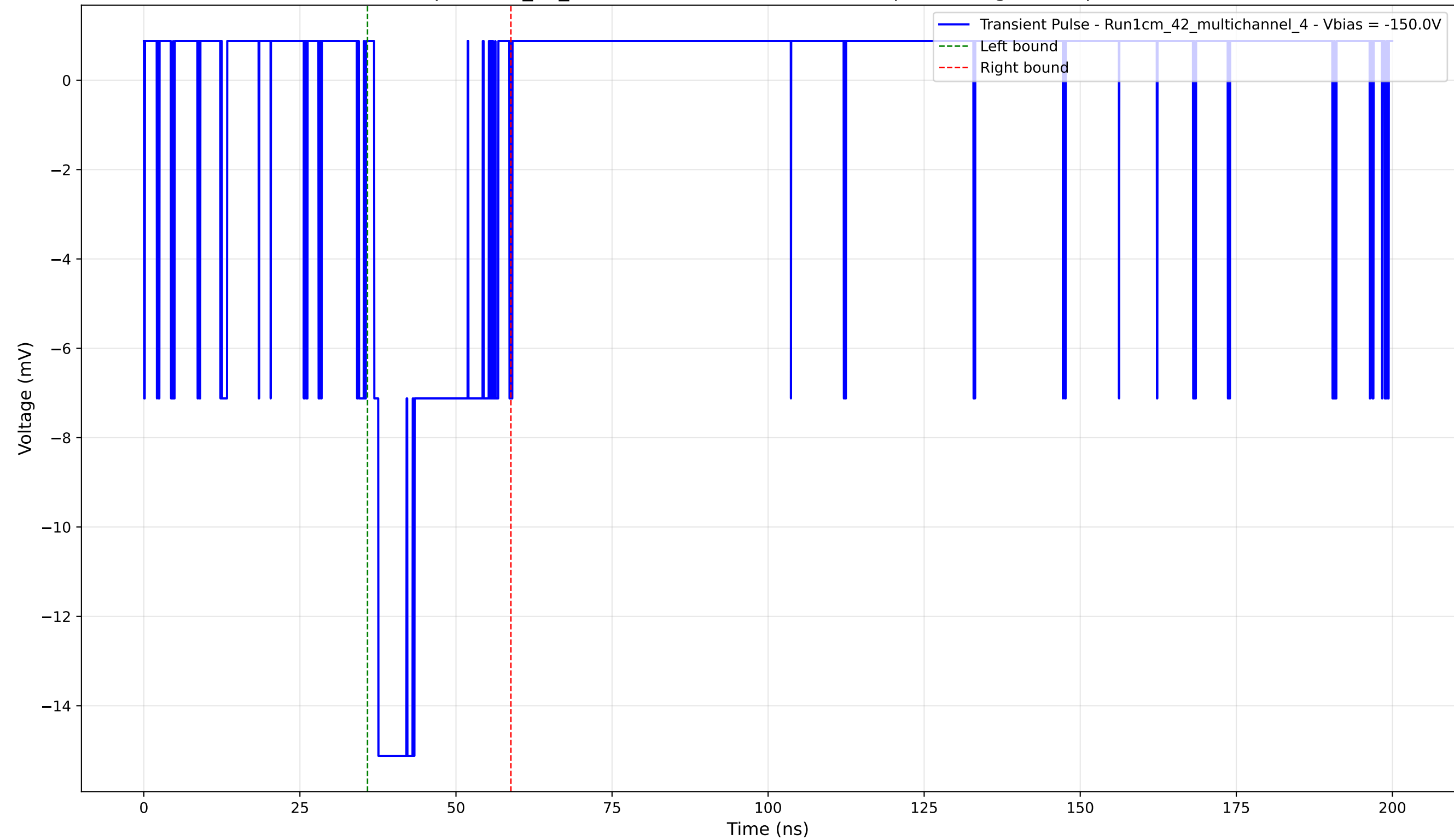
Transient Pulse - Sample: 1cm_42_multichannel - Position: 3725.0 \mu\text{m} - Charge: 3.58 pC - Rise Time: 0.68 ns
