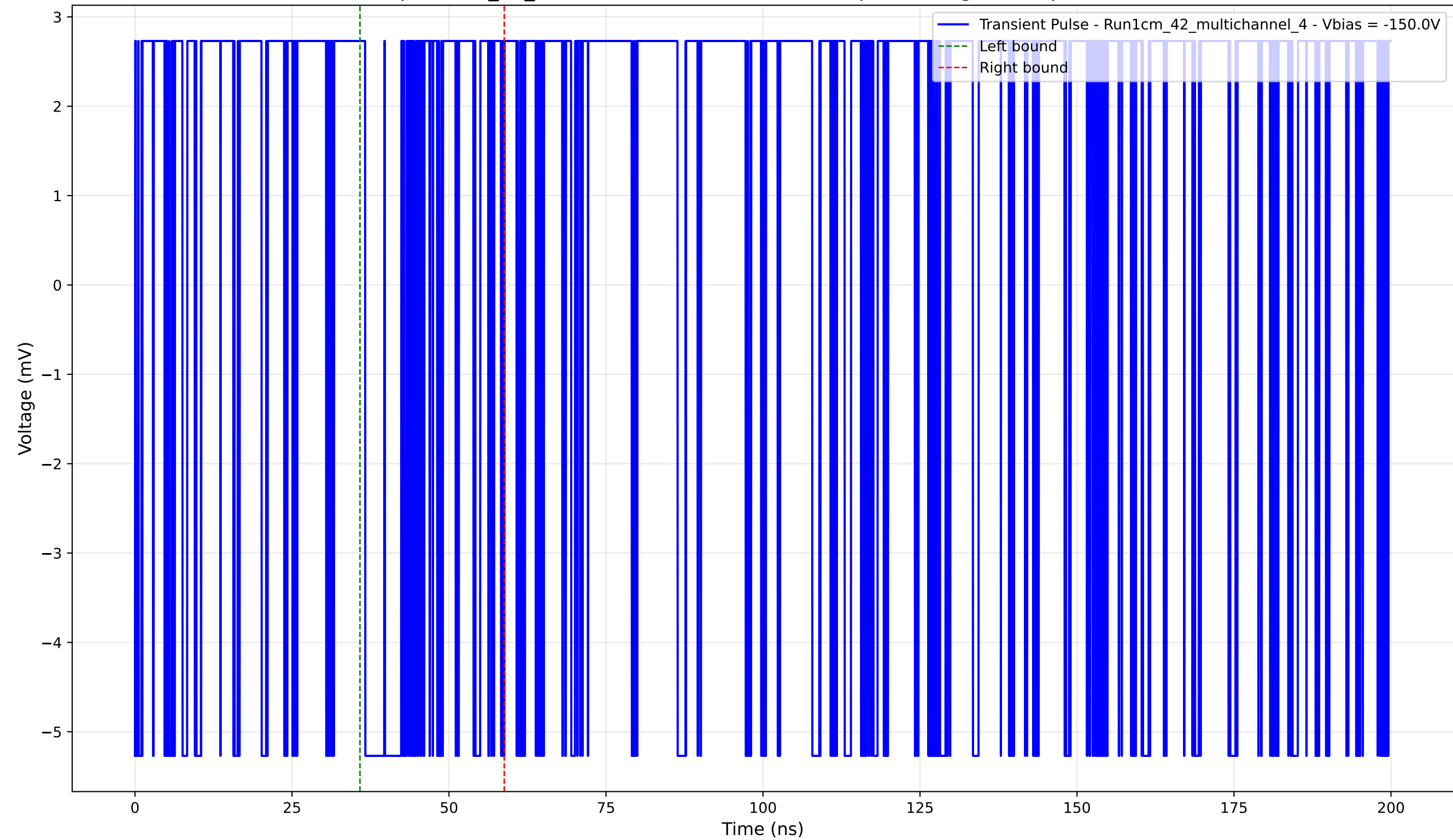
Transient Pulse - Sample: 1cm_42_multichannel - Position: 1855.0 \mu\text{m} - Charge: 0.33 pC - Rise Time: 0.00 ns (N/A)
