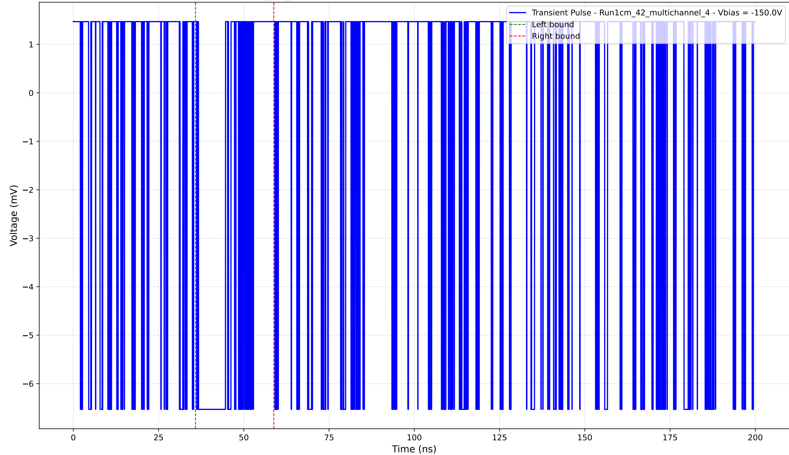
Transient Pulse - Sample: 1cm_42_multichannel - Position: 1405.0 \mu\text{m} - Charge: 1.11 pC - Rise Time: 0.00 ns (N/A)
