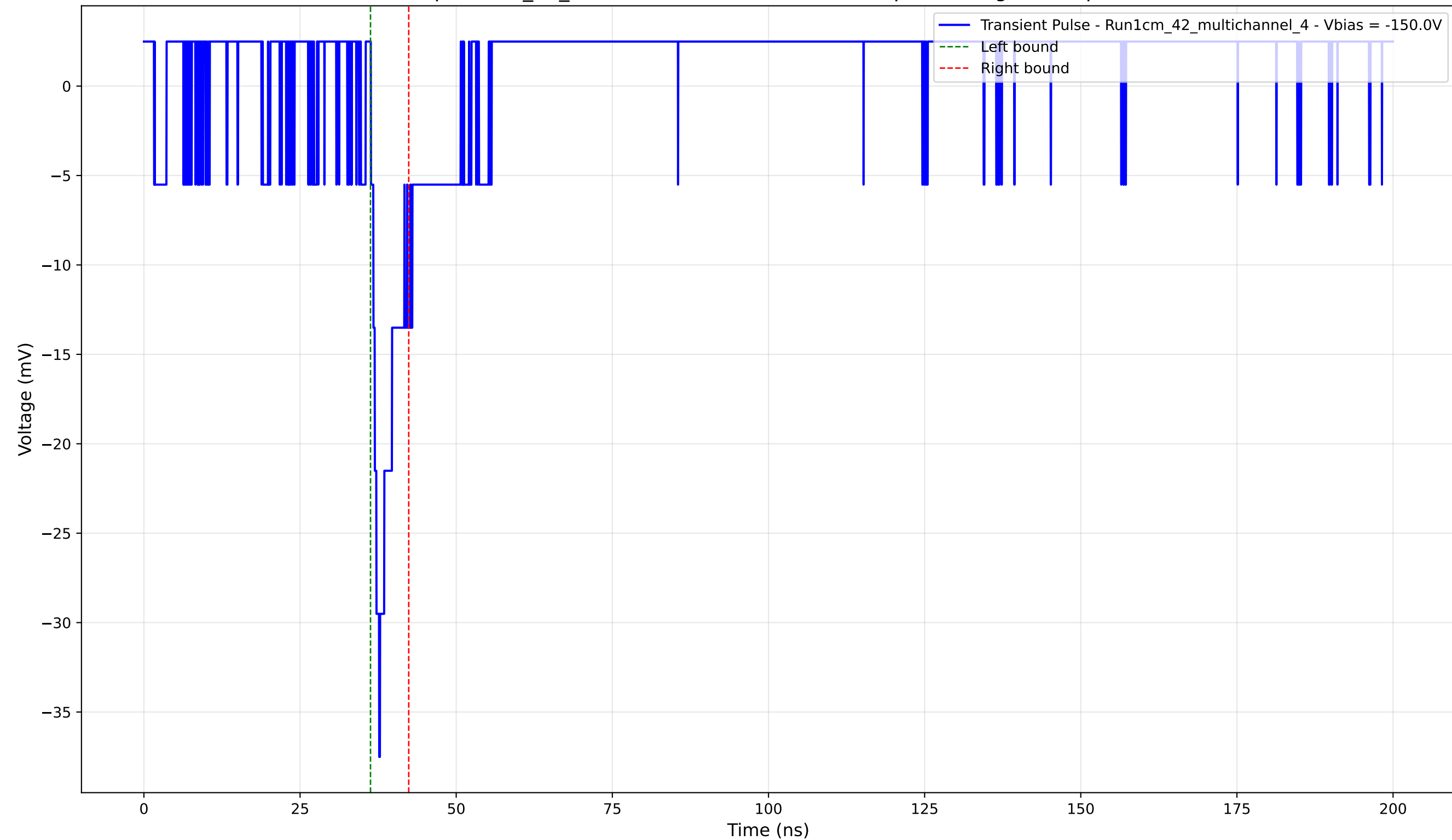
Transient Pulse - Sample: 1cm_42_multichannel - Position: 3065.0 \mu\text{m} - Charge: 2.22 pC - Rise Time: 1.33 ns
