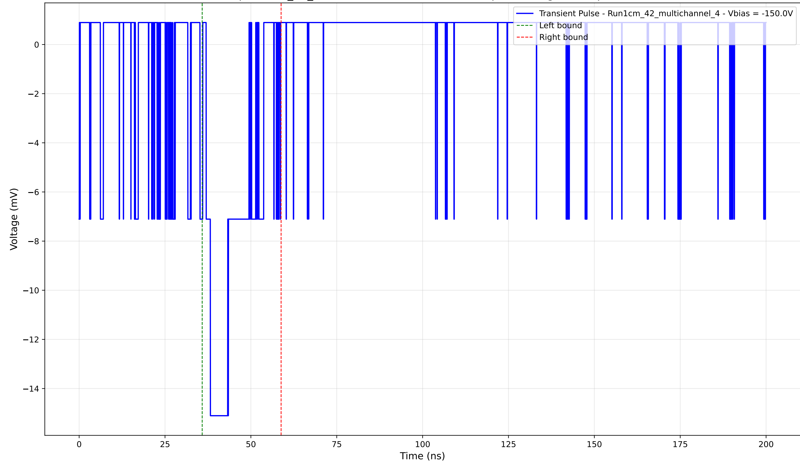
Transient Pulse - Sample: 1cm_42_multichannel - Position: 4530.0 \mu\text{m} - Charge: 3.05 pC - Rise Time: 1.24 ns
