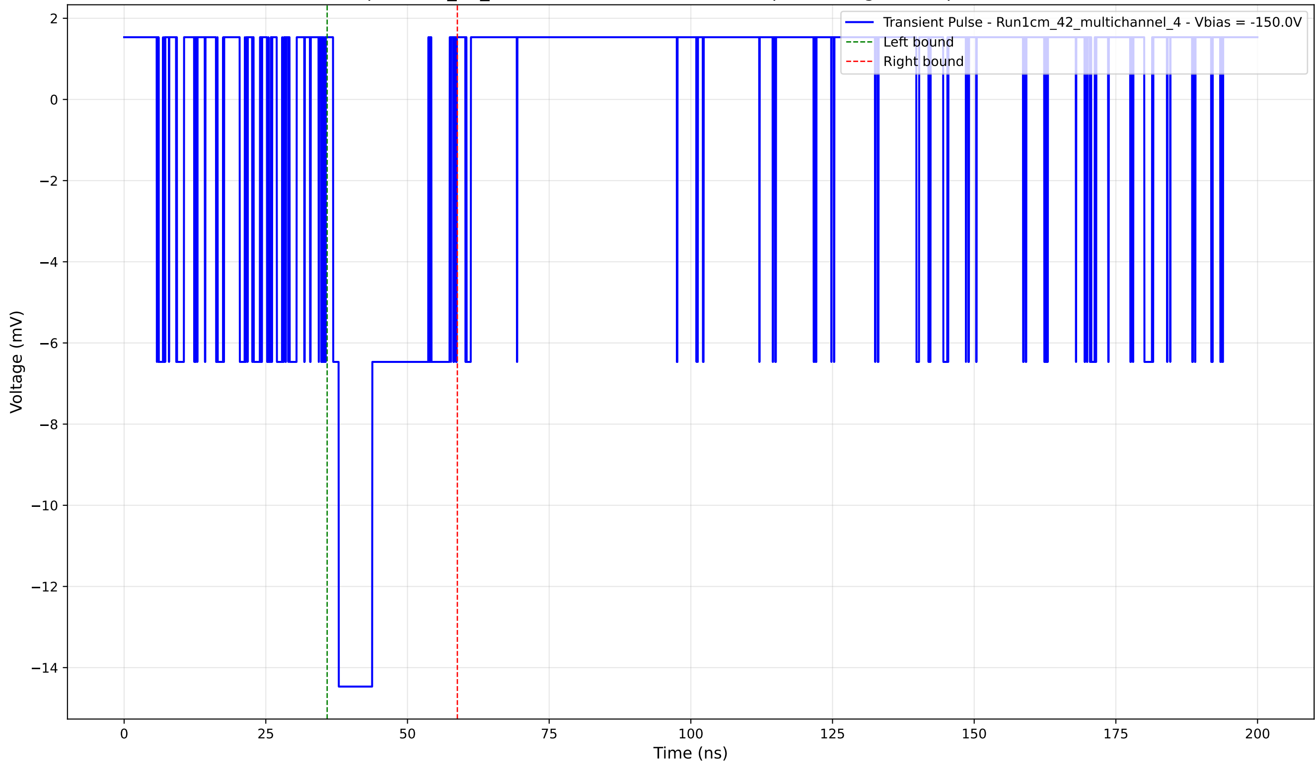
Transient Pulse - Sample: 1cm_42_multichannel - Position: 580.0 \mu\text{m} - Charge: 3.54 pC - Rise Time: 0.00 ns (N/A)
