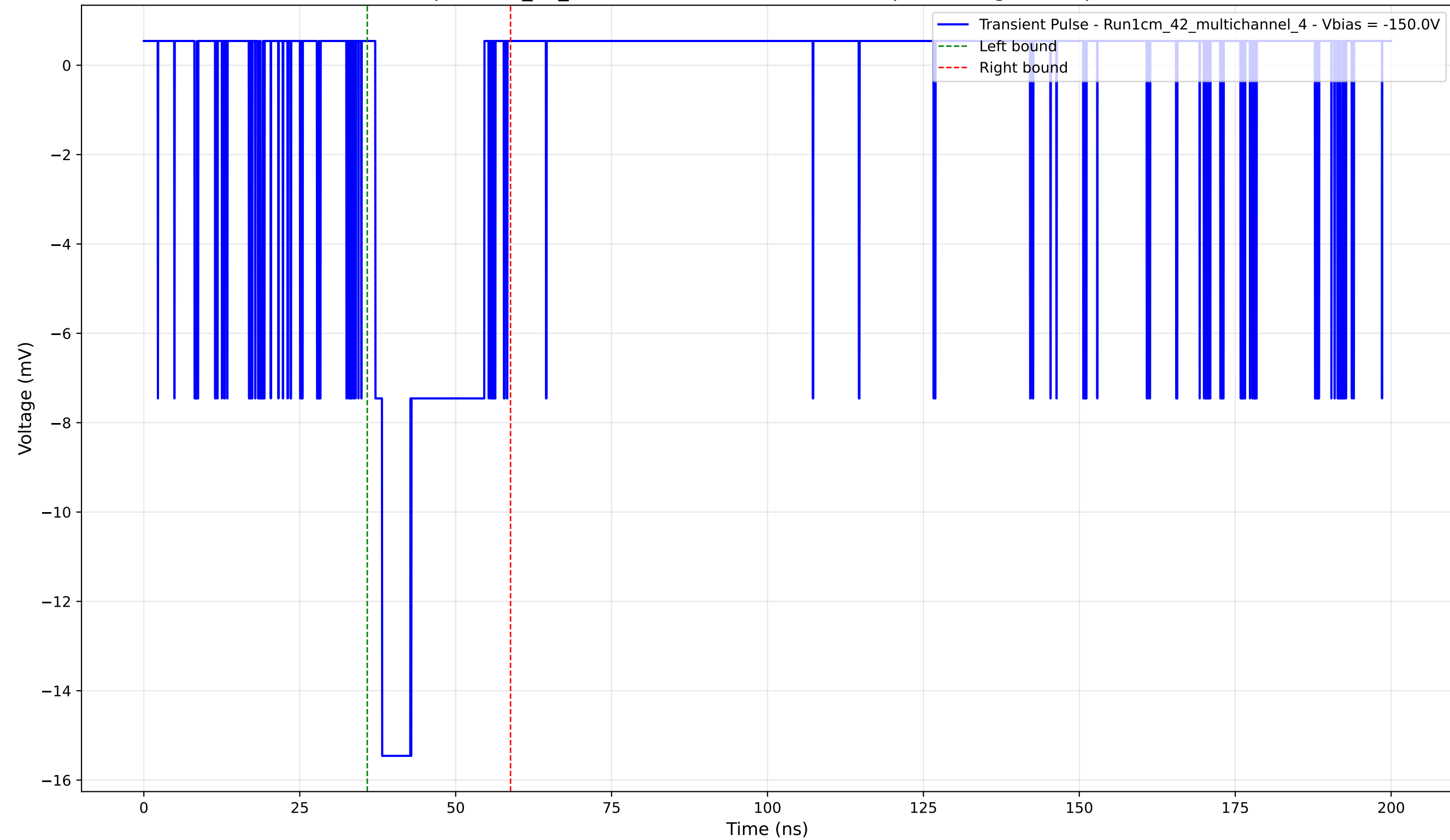
Transient Pulse - Sample: 1cm_42_multichannel - Position: 4545.0 \mu\text{m} - Charge: 3.43 pC - Rise Time: 1.10 ns
