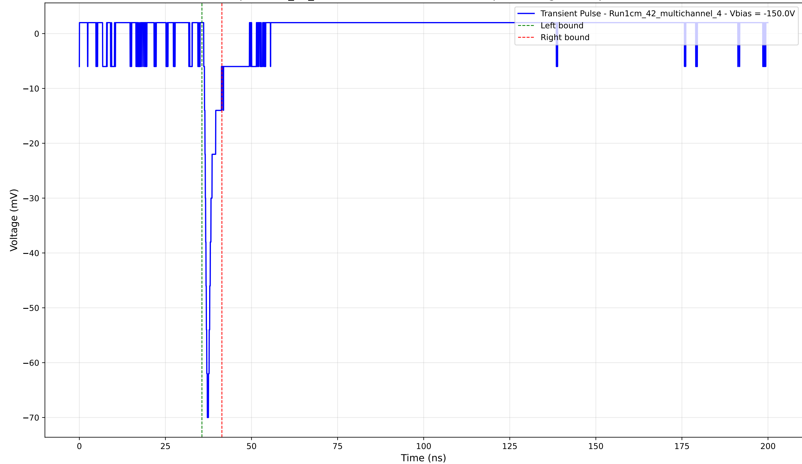
Transient Pulse - Sample: 1cm_42_multichannel - Position: 2185.0 \mu\text{m} - Charge: 3.00 pC - Rise Time: 0.84 ns
