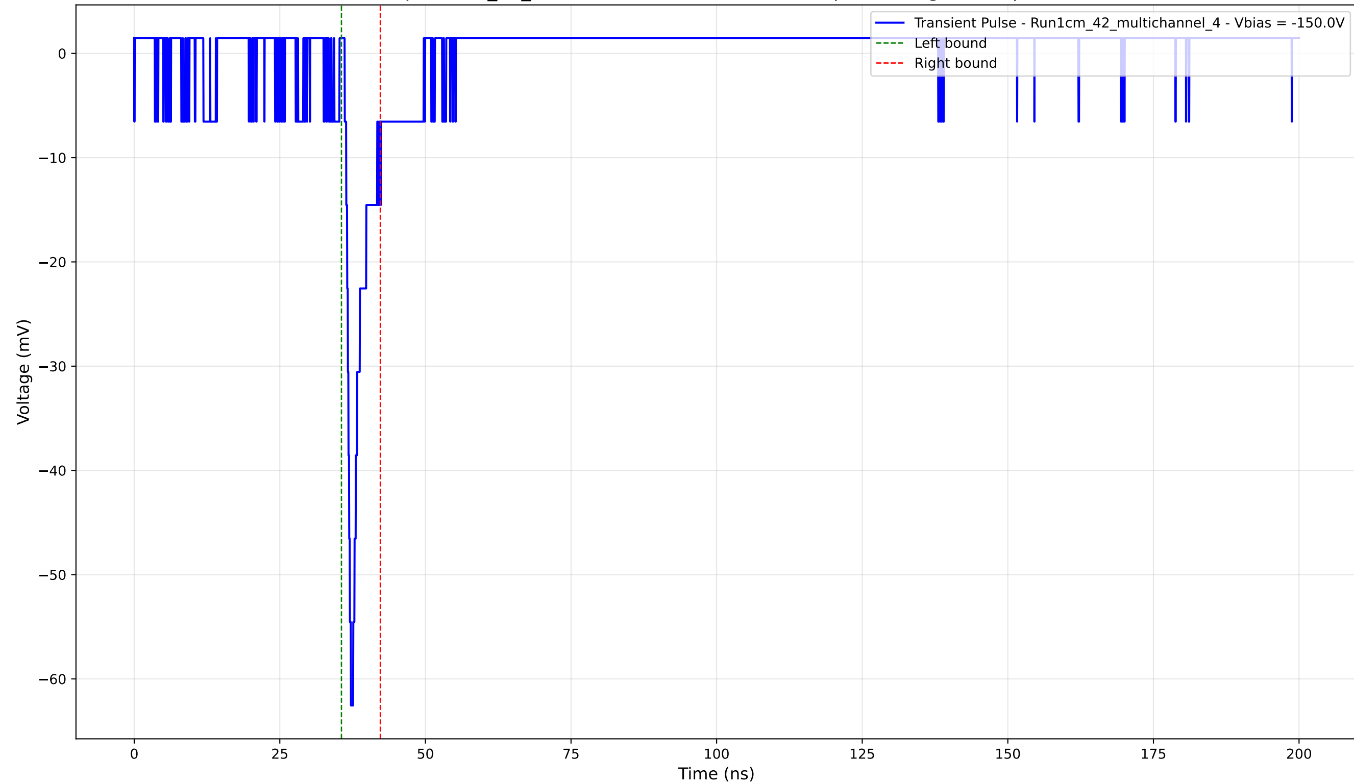
Transient Pulse - Sample: 1cm_42_multichannel - Position: 2095.0 \mu\text{m} - Charge: 3.14 pC - Rise Time: 1.06 ns
