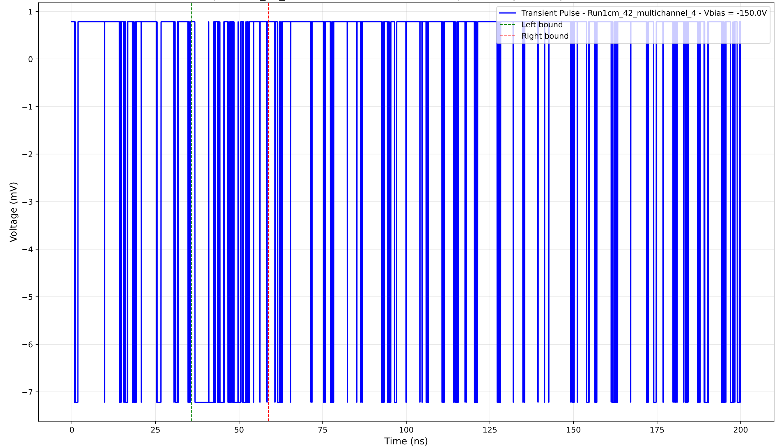
Transient Pulse - Sample: 1cm_42_multichannel - Position: 3365.0 \mu\text{m} - Charge: 1.57 pC - Rise Time: 0.00 ns (N/A)
