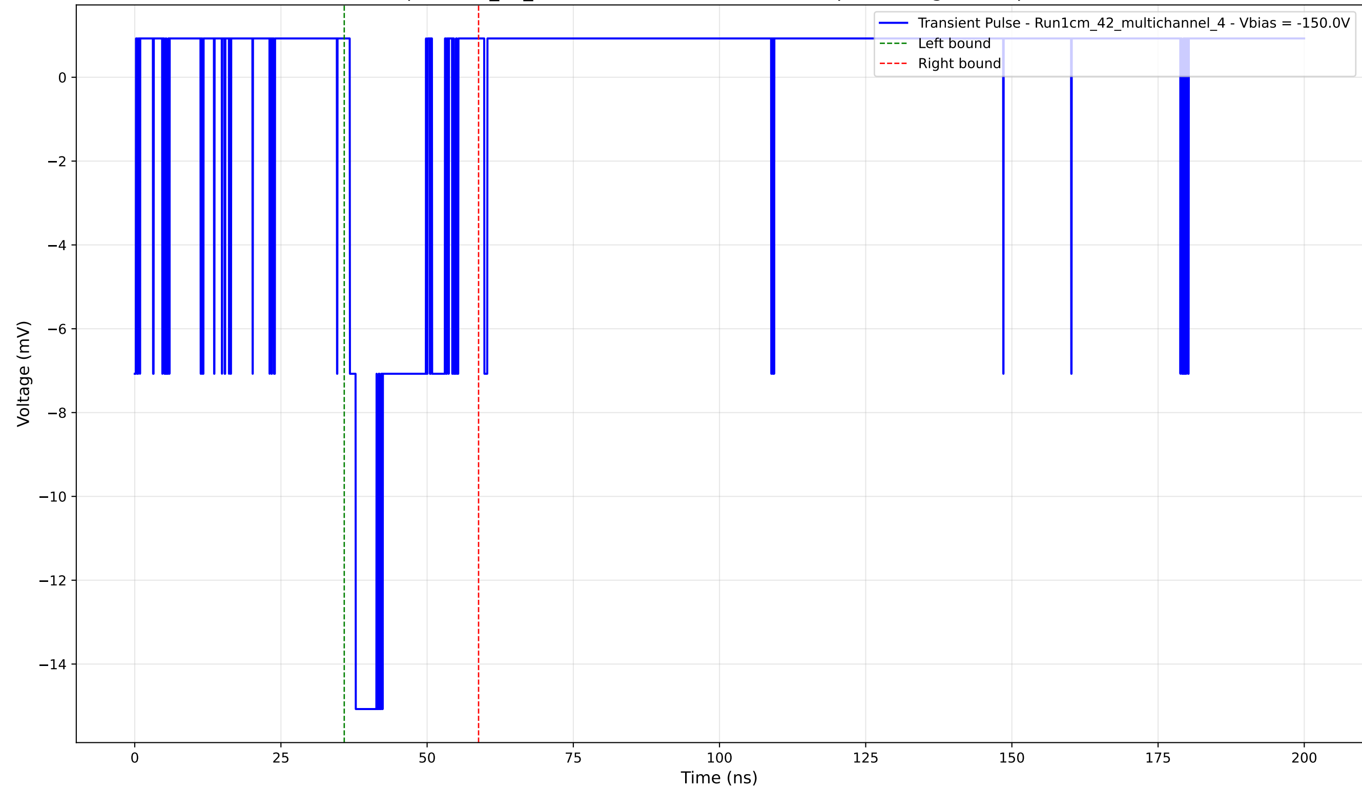
Transient Pulse - Sample: 1cm_42_multichannel - Position: 3835.0 \mu\text{m} - Charge: 2.89 pC - Rise Time: 1.02 ns
