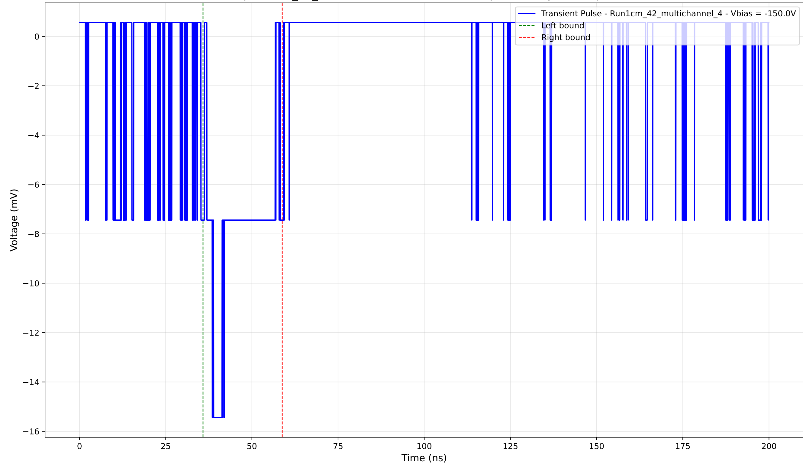
Transient Pulse - Sample: 1cm_42_multichannel - Position: 240.0 \mu\text{m} - Charge: 3.55 pC - Rise Time: 1.58 ns
