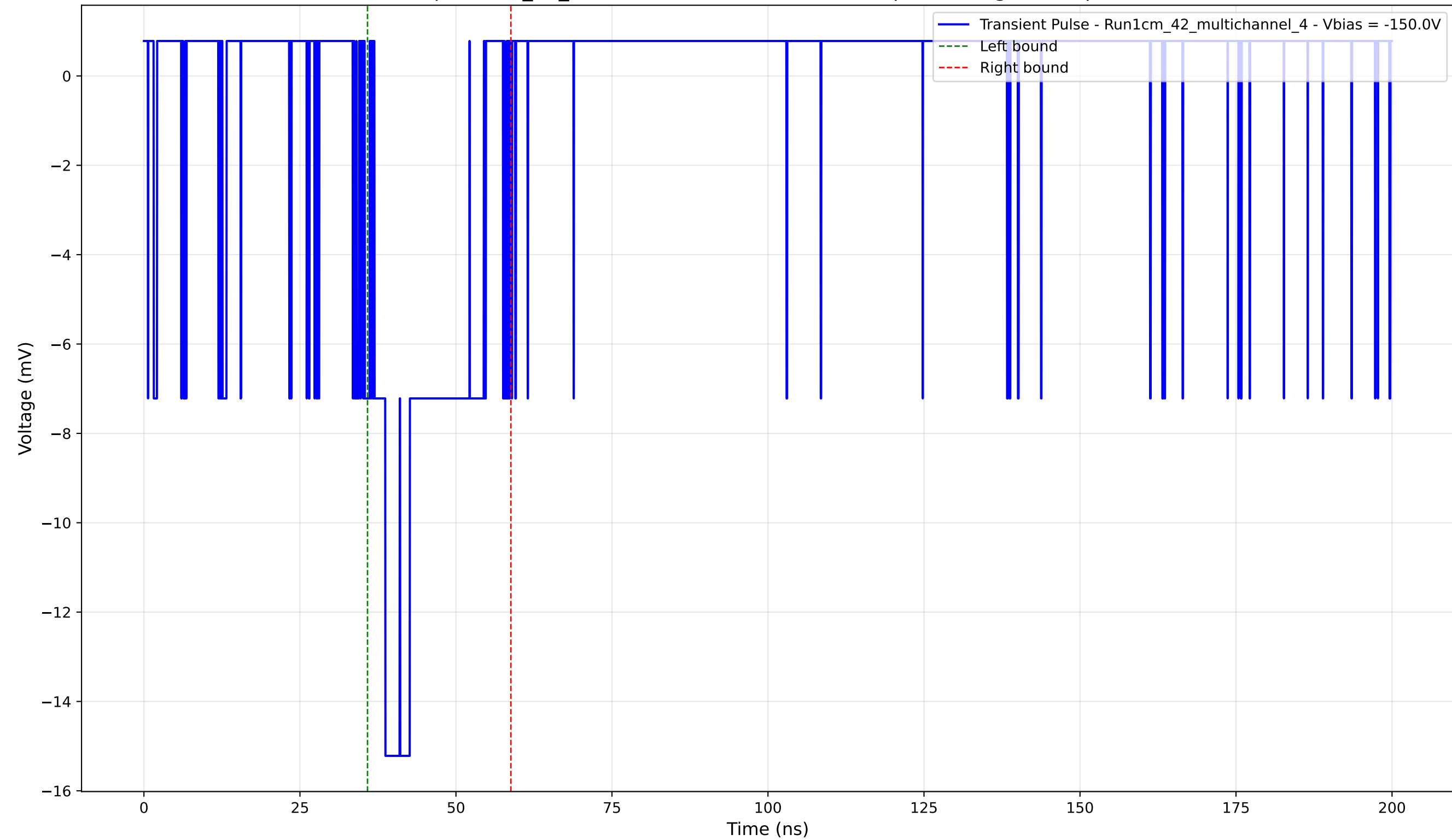
Transient Pulse - Sample: 1cm_42_multichannel - Position: 4640.0 \mu\text{m} - Charge: 3.28 pC - Rise Time: 1.76 ns
