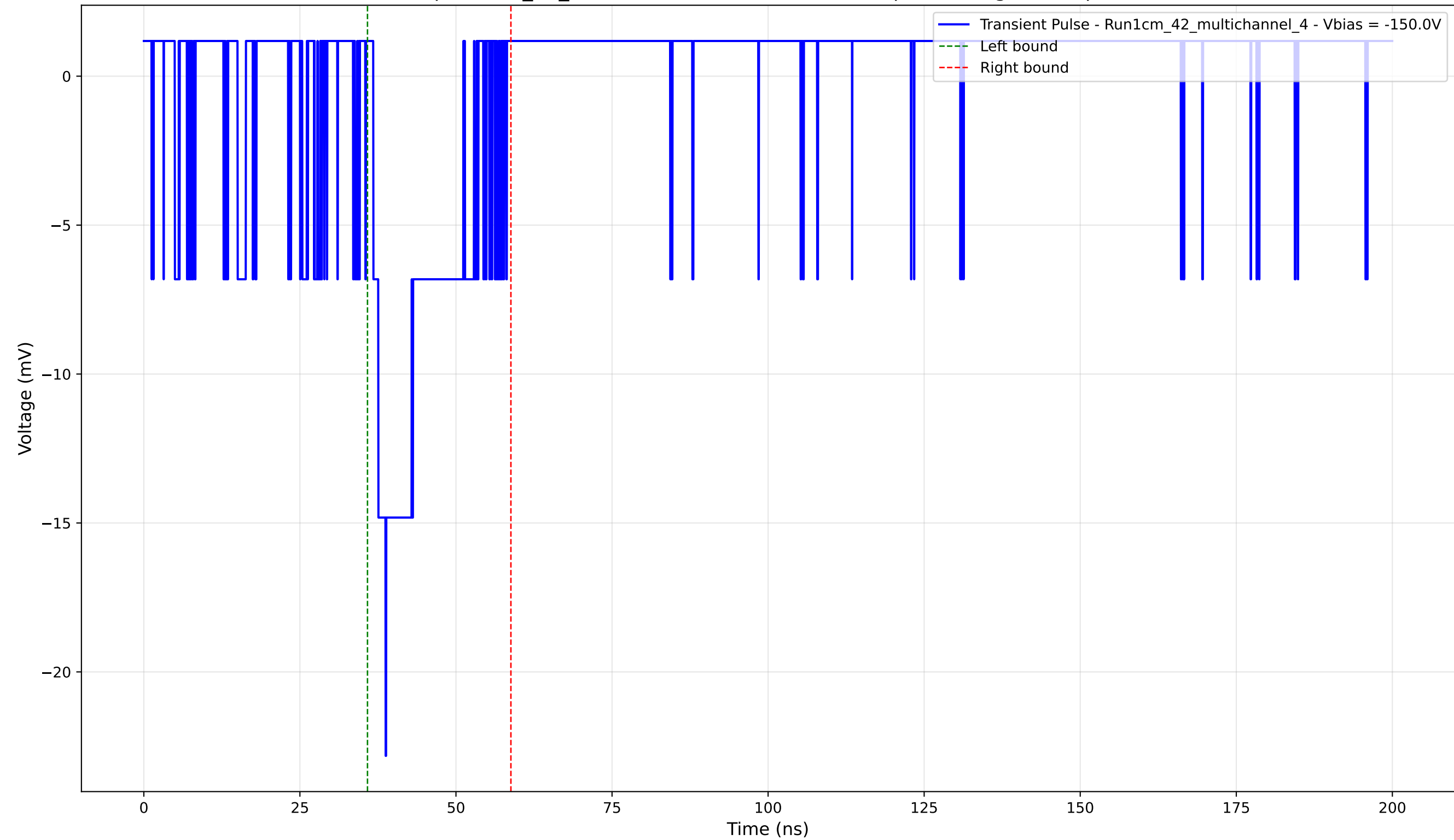
Transient Pulse - Sample: 1cm_42_multichannel - Position: 3695.0 \mu\text{m} - Charge: 3.26 pC - Rise Time: 1.98 ns
