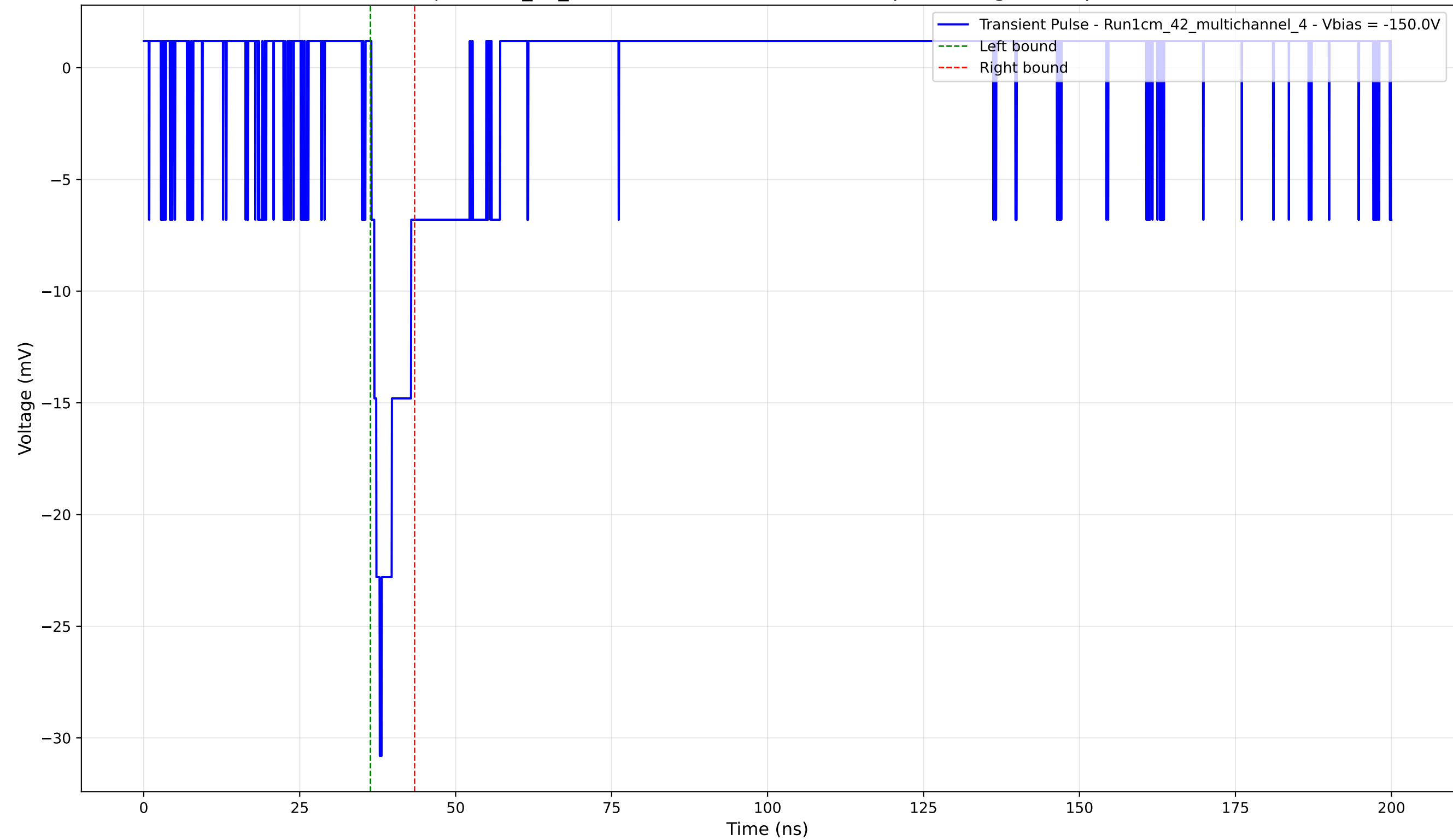
Transient Pulse - Sample: 1cm_42_multichannel - Position: 3285.0 \mu\text{m} - Charge: 2.33 pC - Rise Time: 1.33 ns
