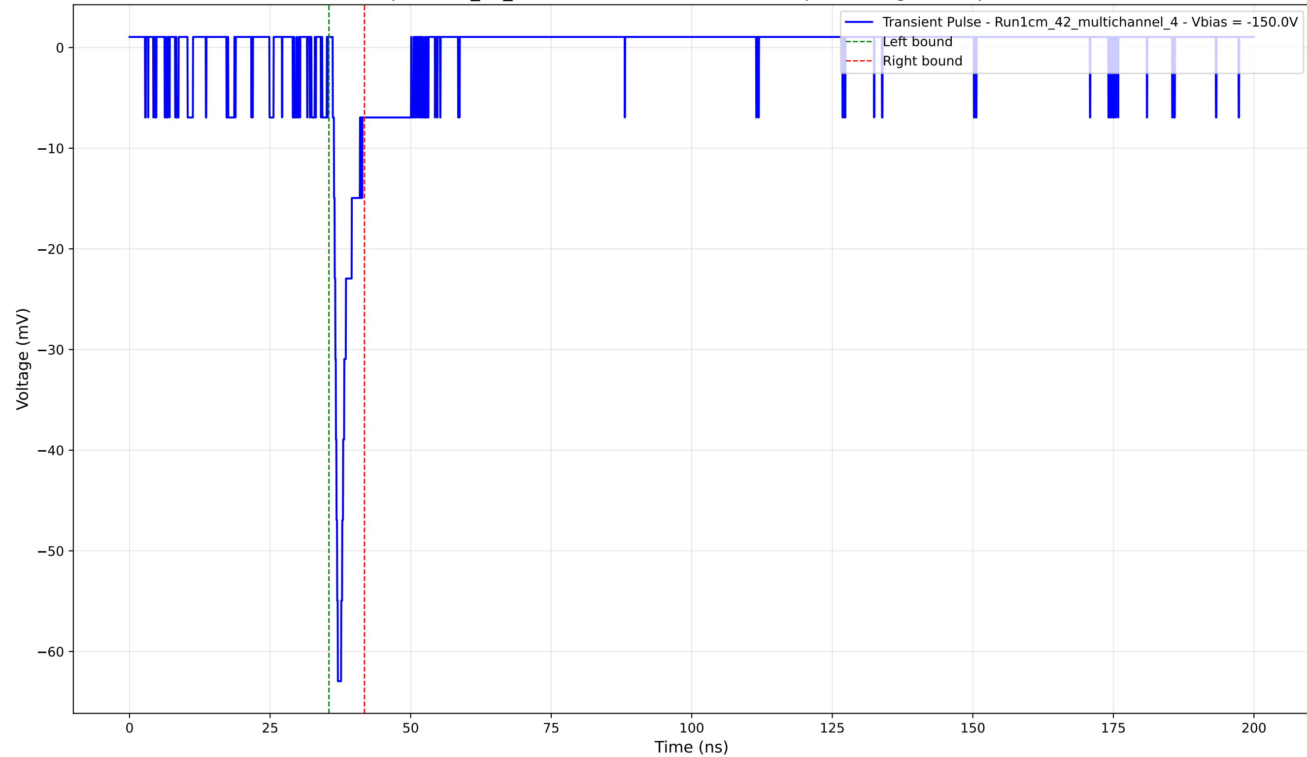
Transient Pulse - Sample: 1cm_42_multichannel - Position: 2590.0 \mu\text{m} - Charge: 2.98 pC - Rise Time: 0.90 ns
