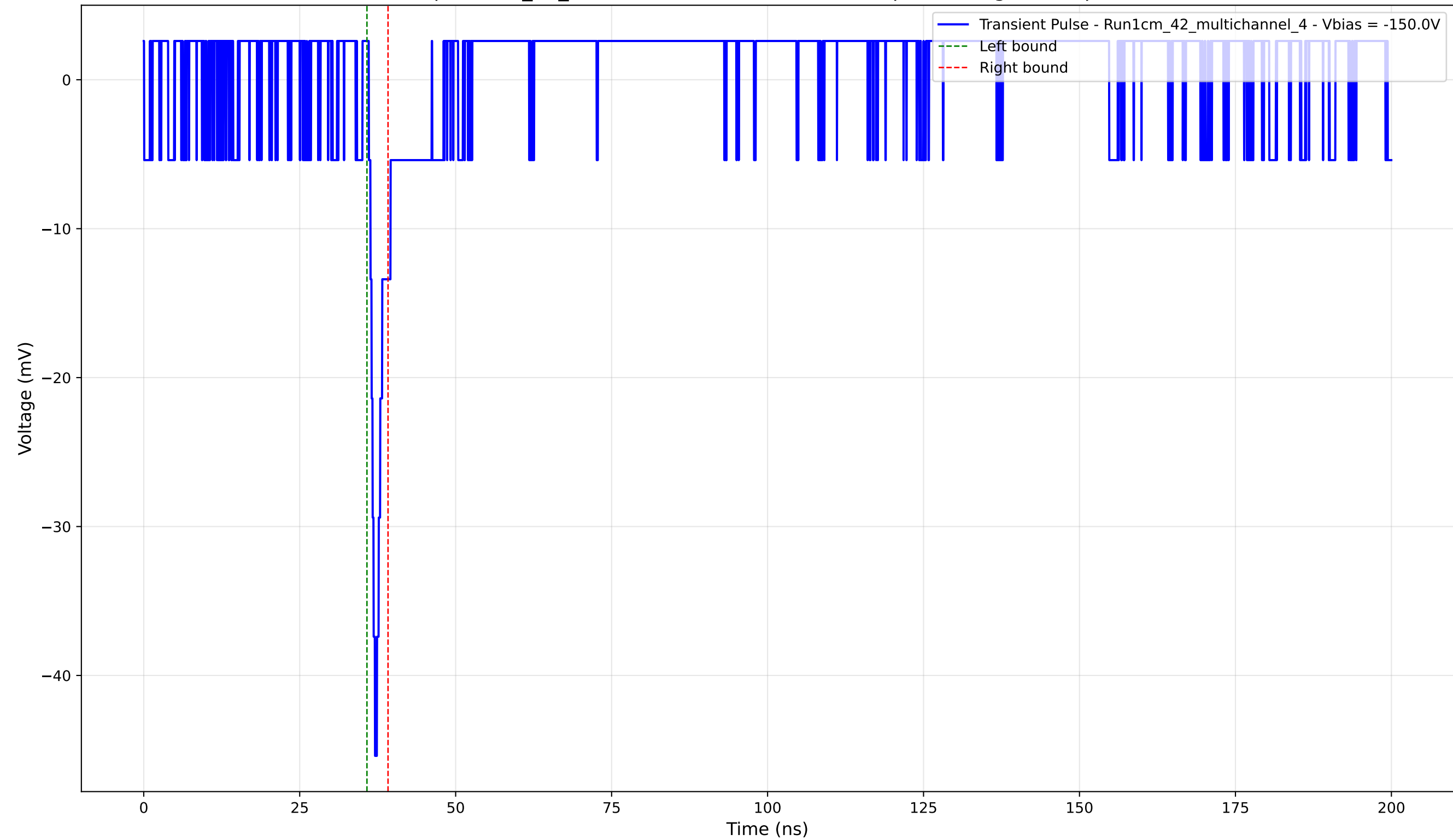
Transient Pulse - Sample: 1cm_42_multichannel - Position: 2335.0 \mu\text{m} - Charge: 1.42 pC - Rise Time: 0.99 ns
