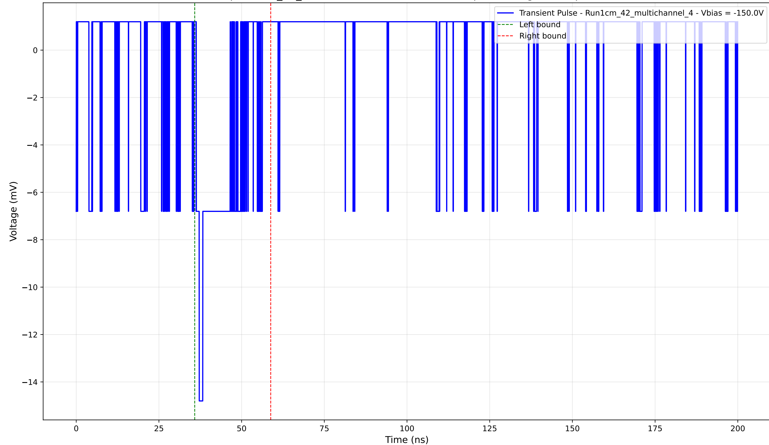
Transient Pulse - Sample: 1cm_42_multichannel - Position: 2935.0 \mu\text{m} - Charge: 1.99 pC - Rise Time: 0.90 ns
