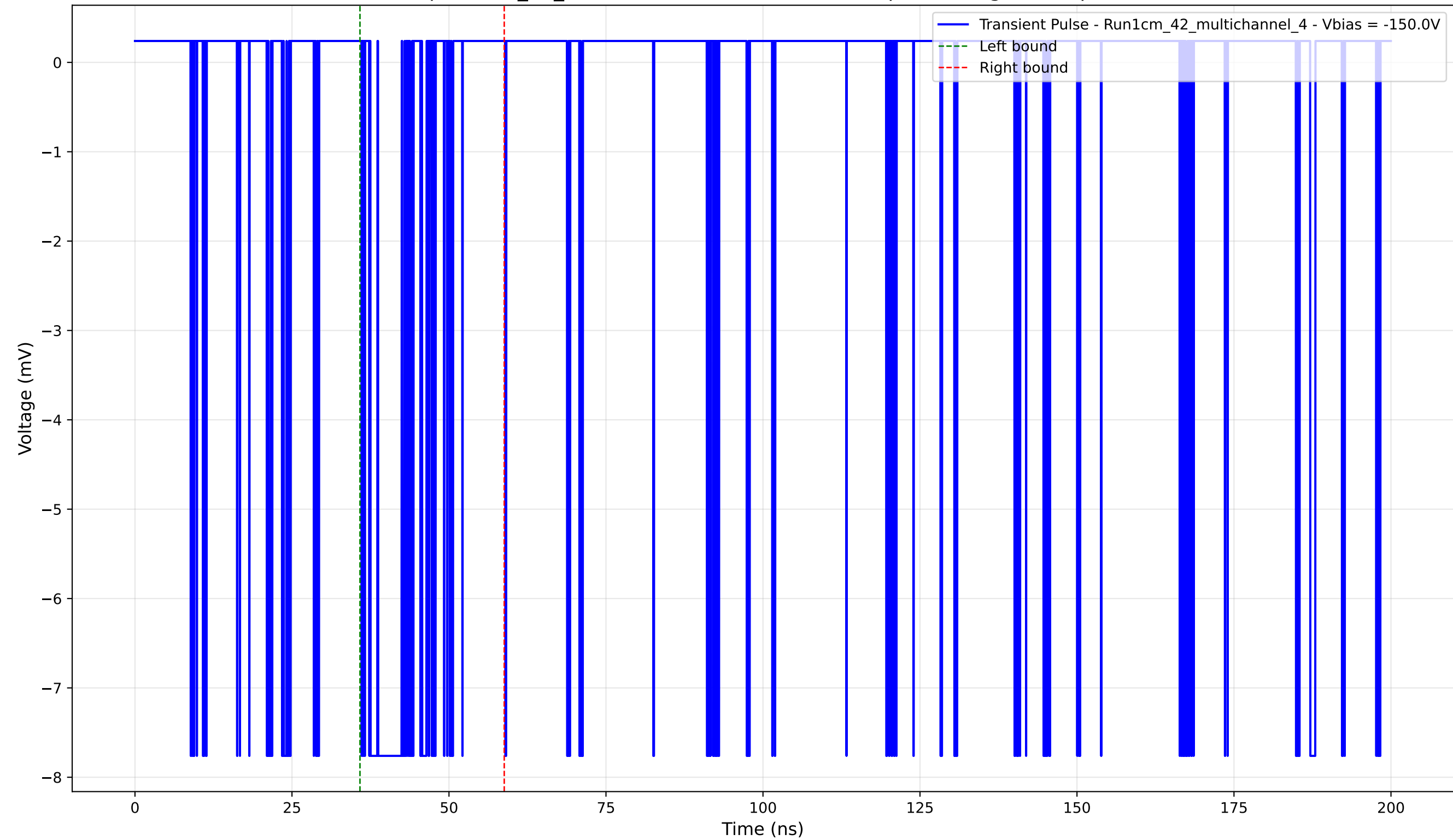
Transient Pulse - Sample: 1cm_42_multichannel - Position: 3875.0 \mu\text{m} - Charge: 1.19 pC - Rise Time: 0.02 ns
