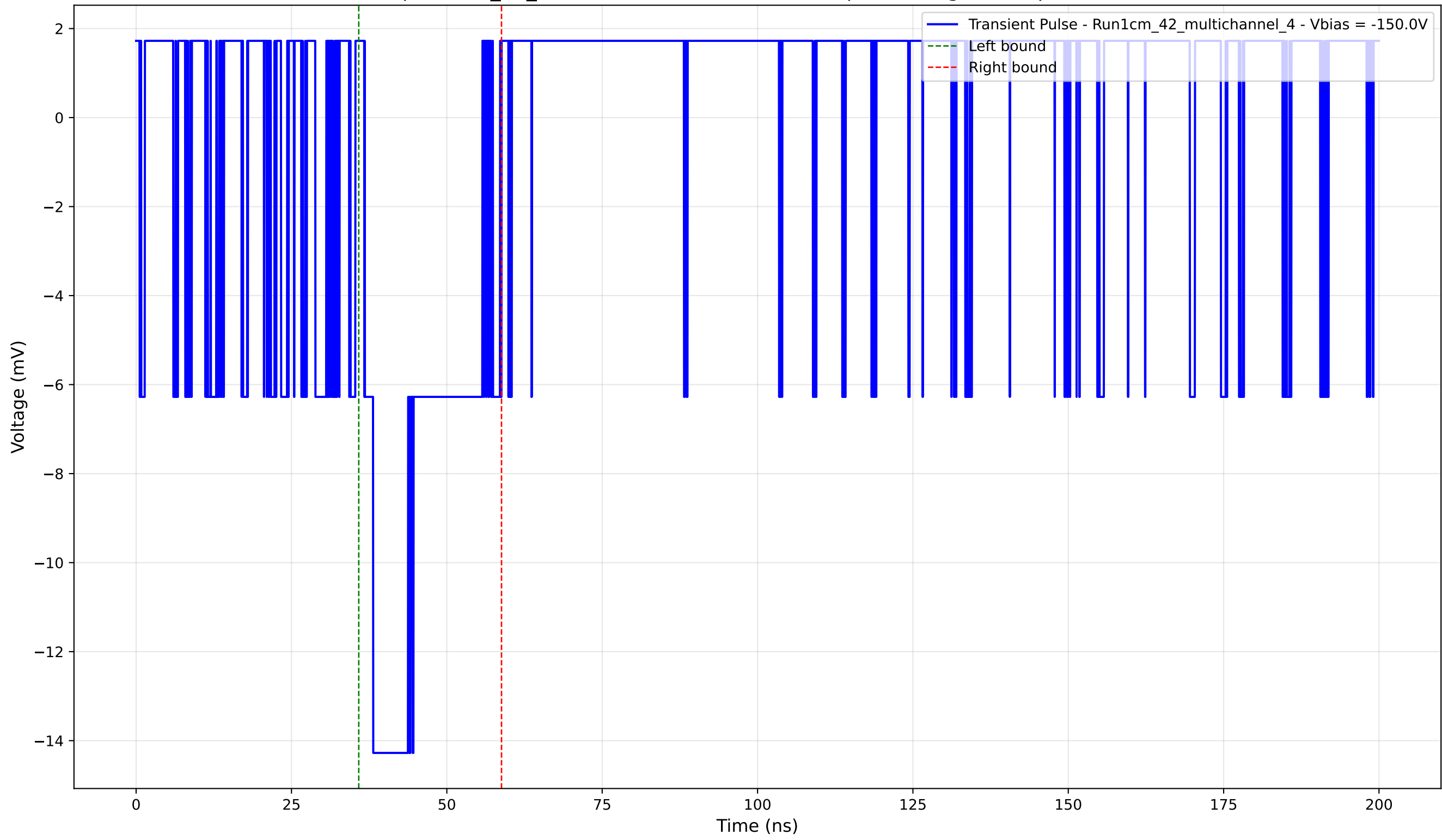
Transient Pulse - Sample: 1cm_42_multichannel - Position: 545.0 \mu\text{m} - Charge: 3.48 pC - Rise Time: 0.00 ns (N/A)
