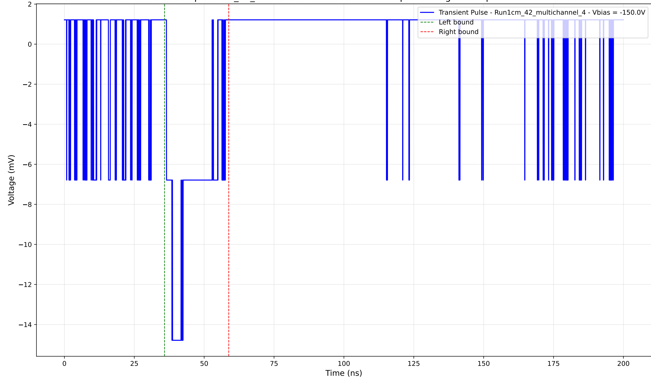
Transient Pulse - Sample: 1cm_42_multichannel - Position: 4785.0 \mu\text{m} - Charge: 3.12 pC - Rise Time: 1.96 ns
