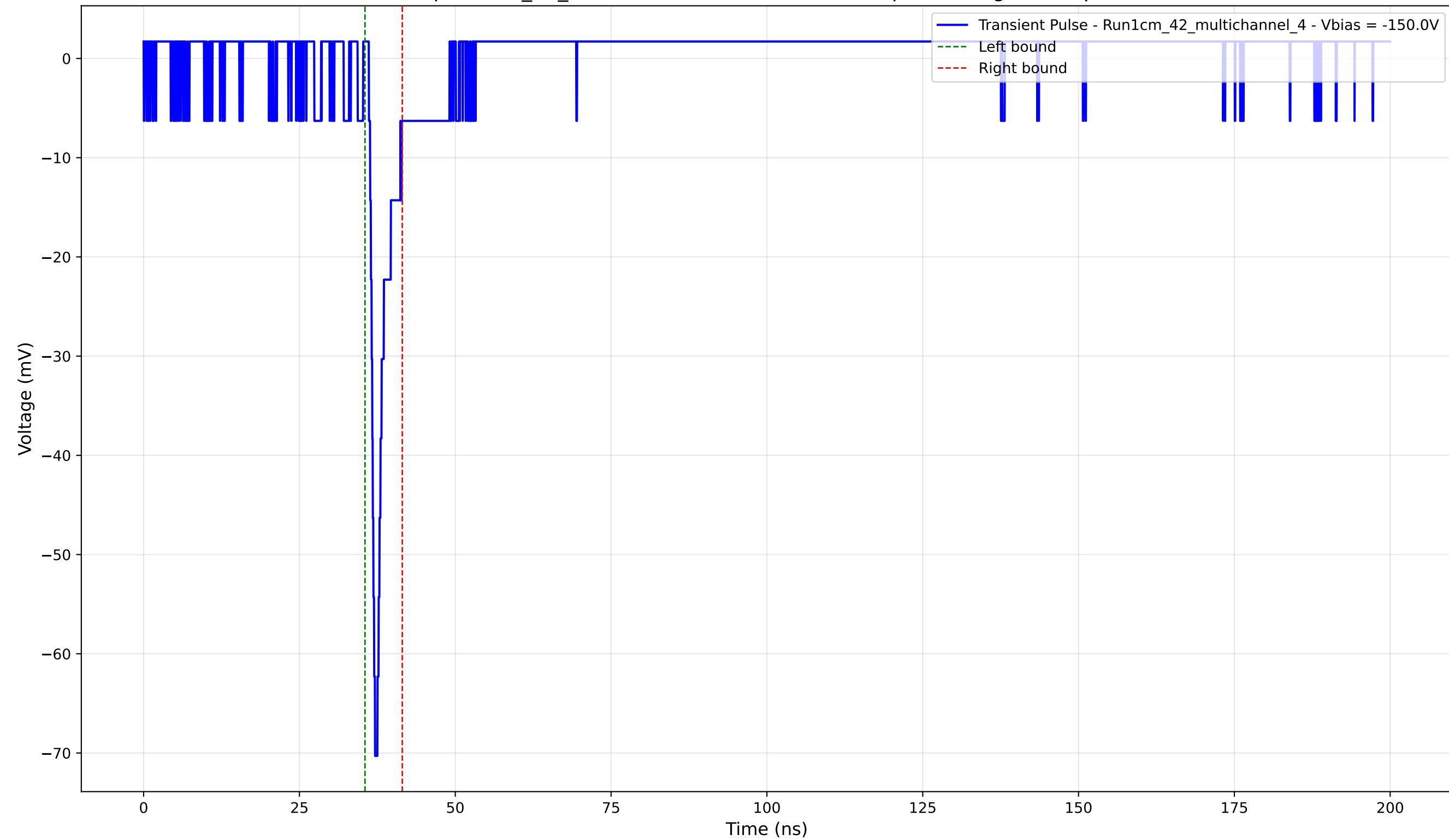
Transient Pulse - Sample: 1cm_42_multichannel - Position: 2205.0 \mu\text{m} - Charge: 3.06 pC - Rise Time: 0.80 ns
