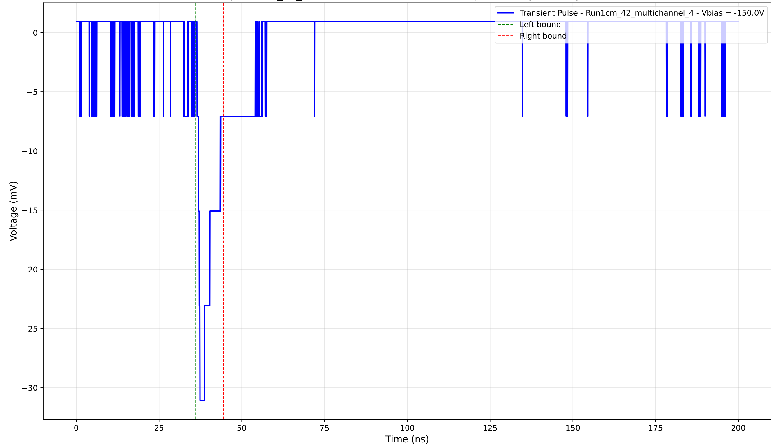
Transient Pulse - Sample: 1cm_42_multichannel - Position: 1540.0 \mu\text{m} - Charge: 2.96 pC - Rise Time: 0.91 ns
