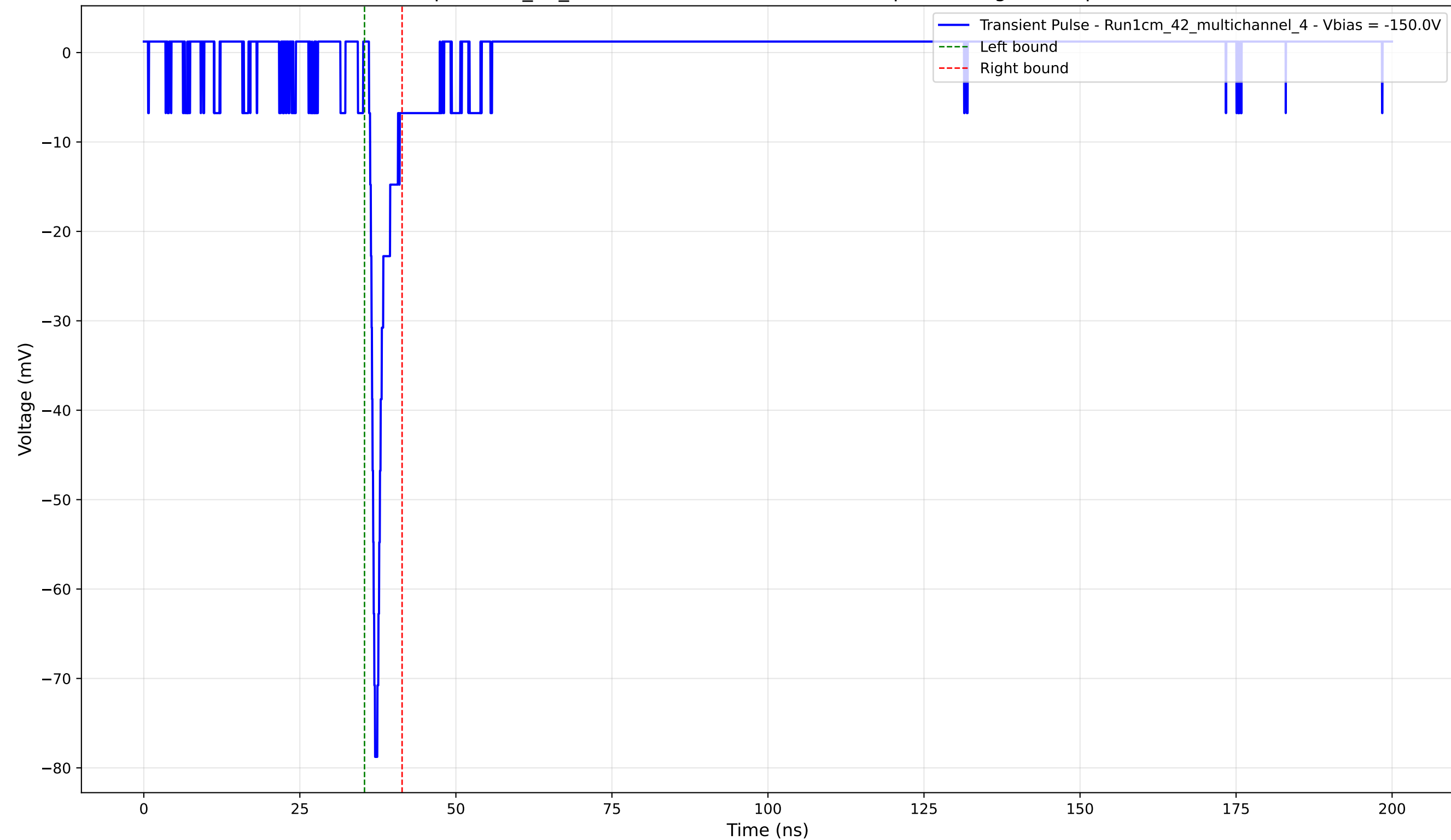
Transient Pulse - Sample: 1cm_42_multichannel - Position: 2460.0 \mu\text{m} - Charge: 3.17 pC - Rise Time: 0.80 ns
