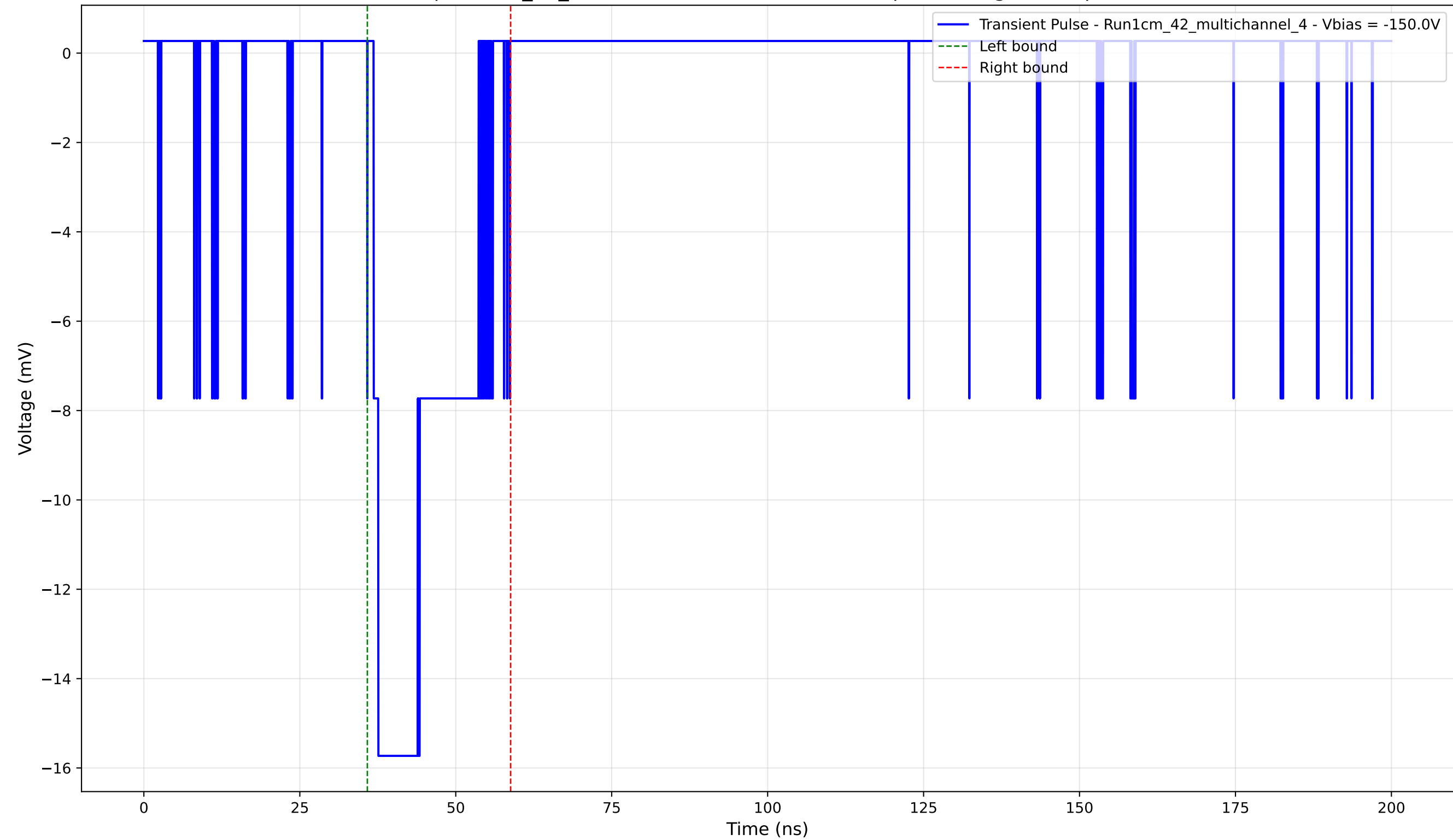
Transient Pulse - Sample: 1cm_42_multichannel - Position: 3745.0 \mu\text{m} - Charge: 3.83 pC - Rise Time: 0.76 ns
