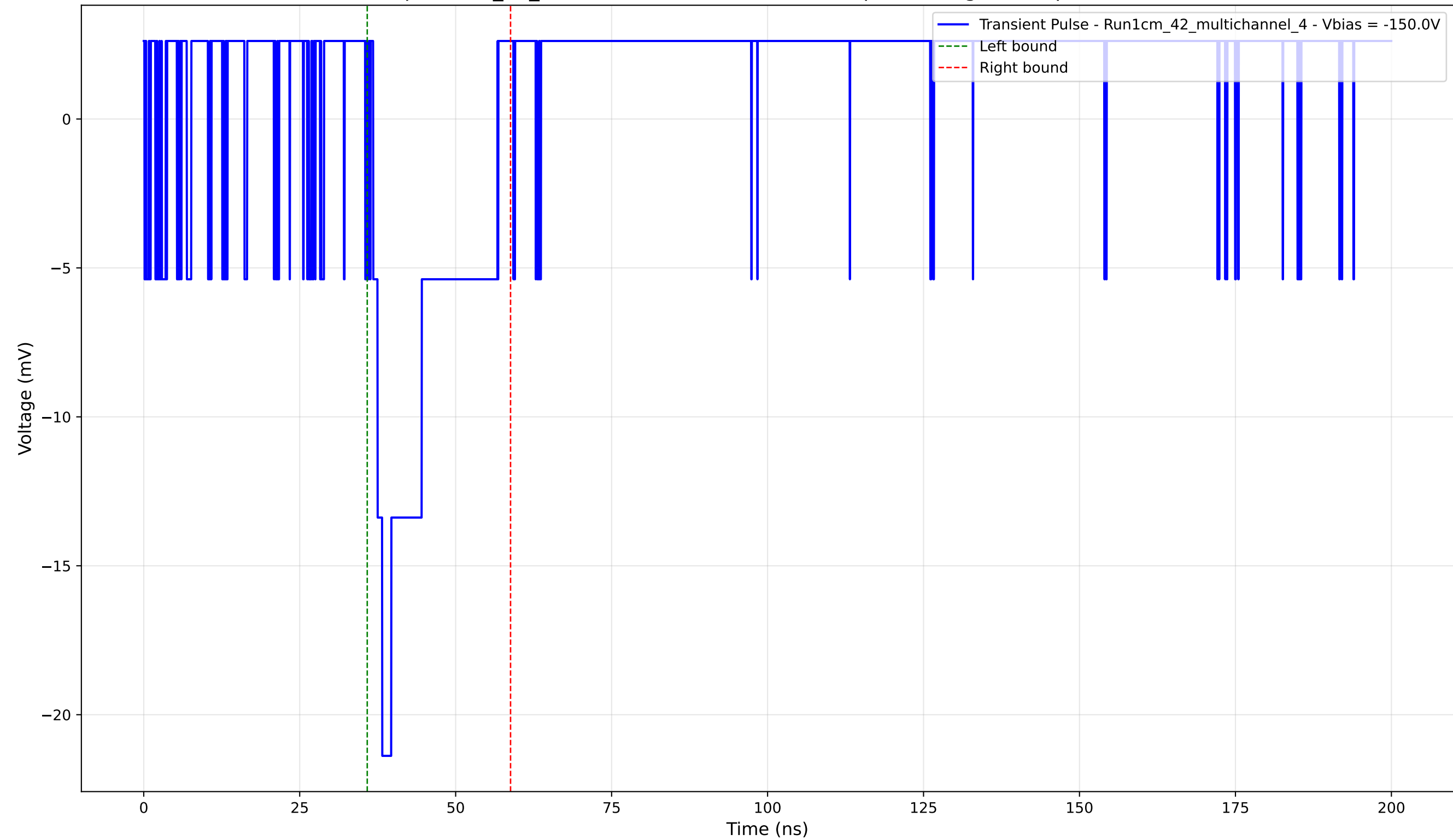
Transient Pulse - Sample: 1cm_42_multichannel - Position: 1015.0 \mu\text{m} - Charge: 3.41 pC - Rise Time: 0.00 ns (N/A)
