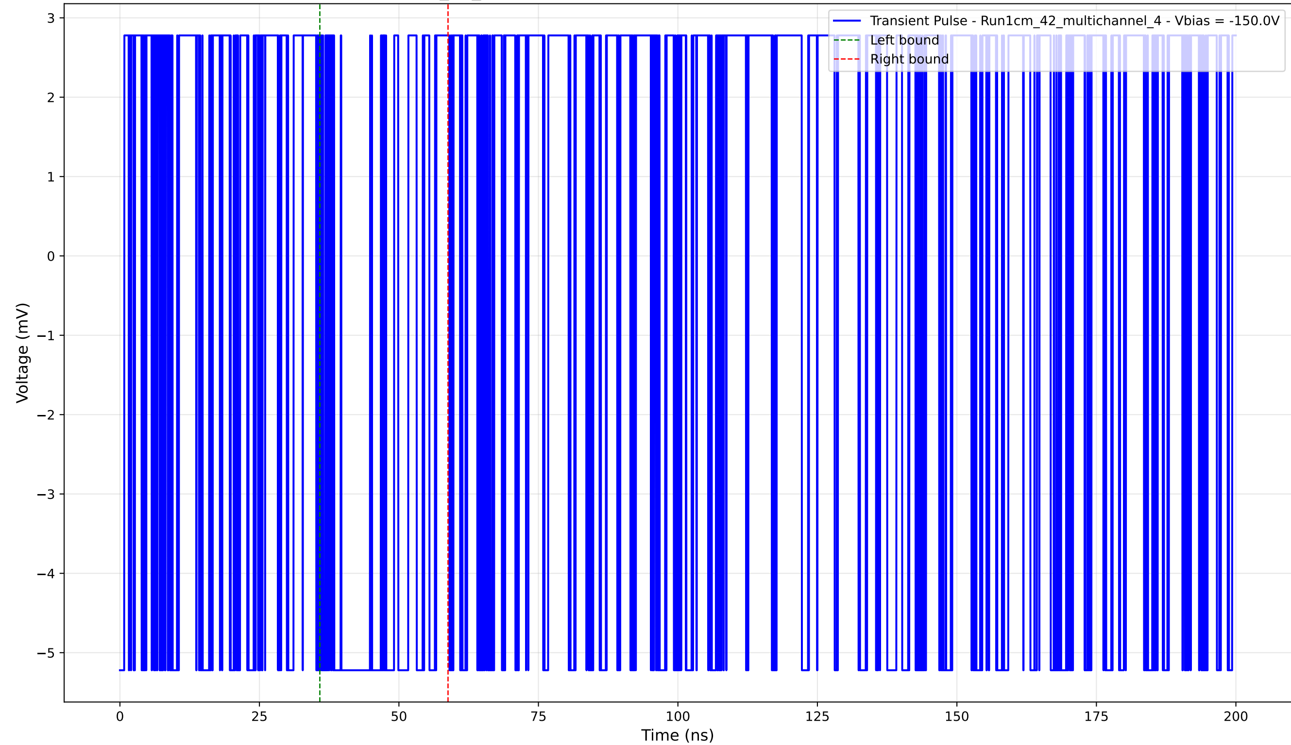
Transient Pulse - Sample: 1cm_42_multichannel - Position: 395.0 \mu\text{m} - Charge: 1.21 pC - Rise Time: 0.00 ns (N/A)
