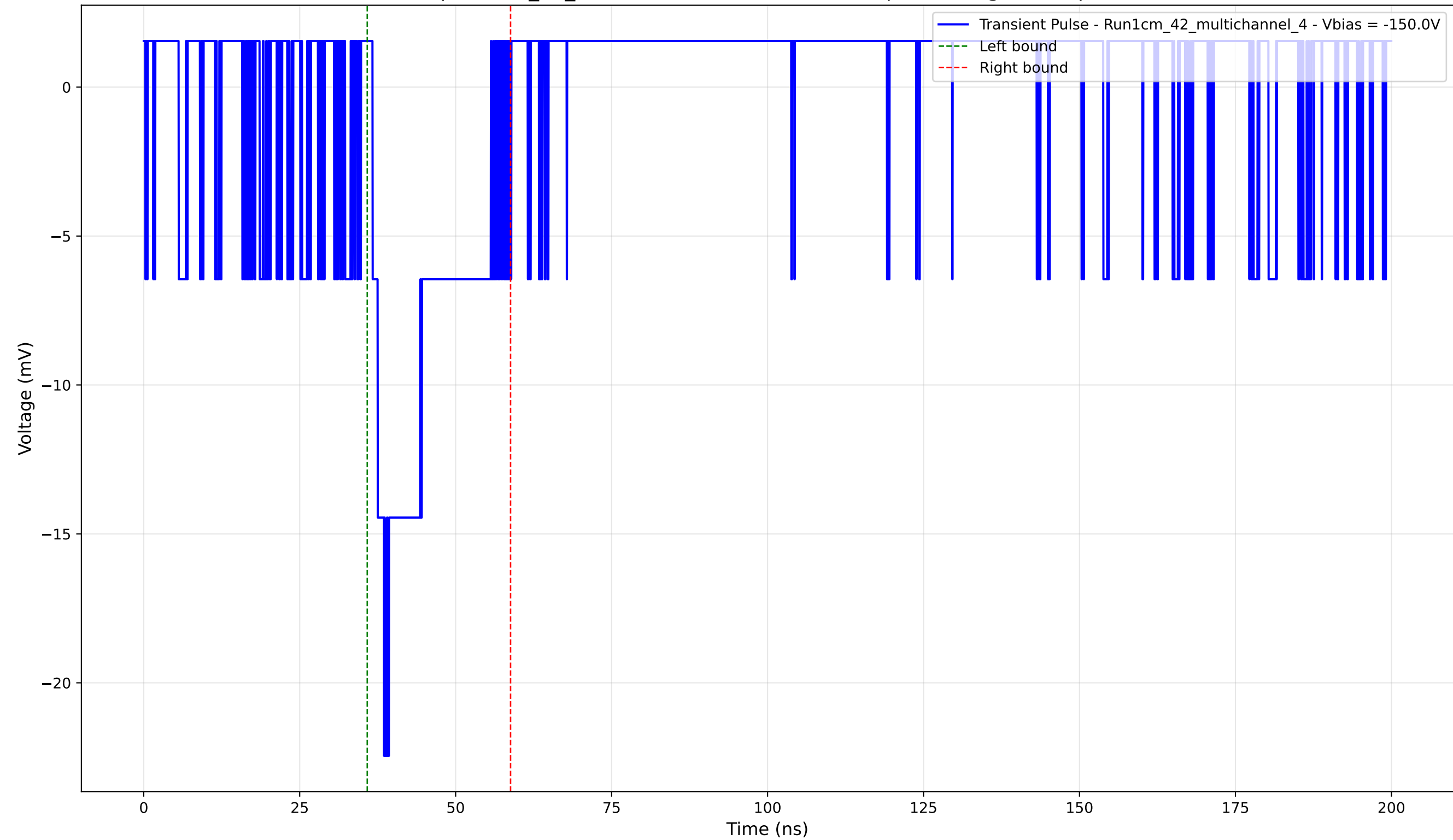
Transient Pulse - Sample: 1cm_42_multichannel - Position: 975.0 \mu\text{m} - Charge: 3.81 pC - Rise Time: 1.88 ns
