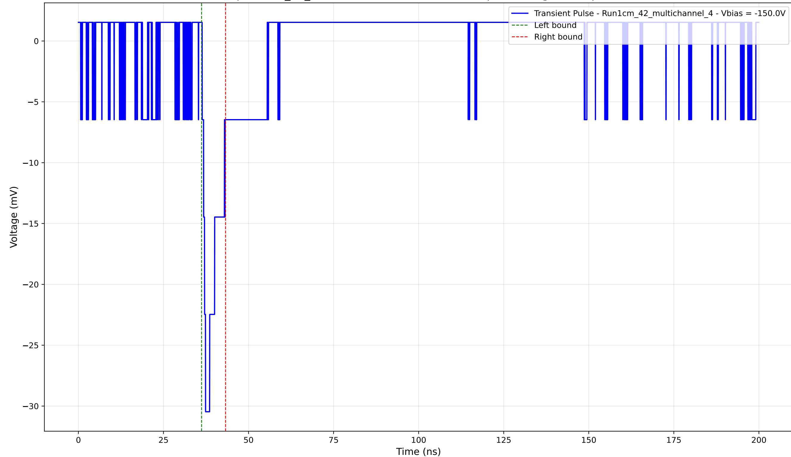
Transient Pulse - Sample: 1cm_42_multichannel - Position: 1590.0 \mu\text{m} - Charge: 2.55 pC - Rise Time: 0.99 ns
