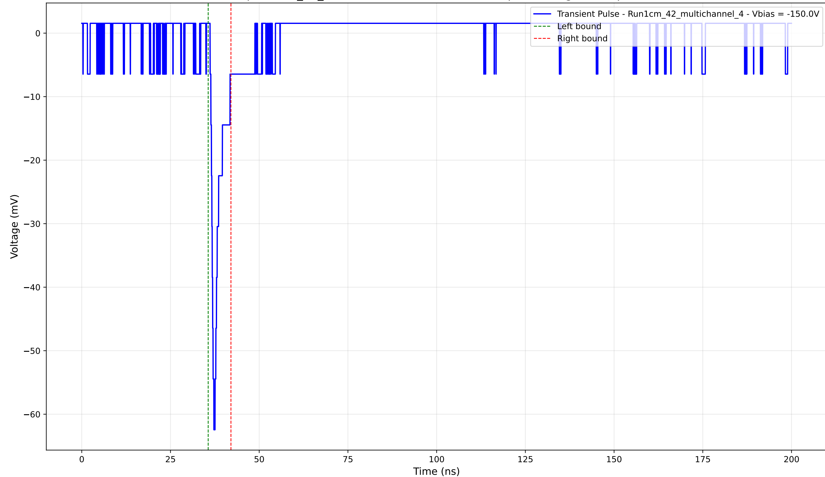
Transient Pulse - Sample: 1cm_42_multichannel - Position: 2135.0 \mu\text{m} - Charge: 2.98 pC - Rise Time: 1.06 ns
