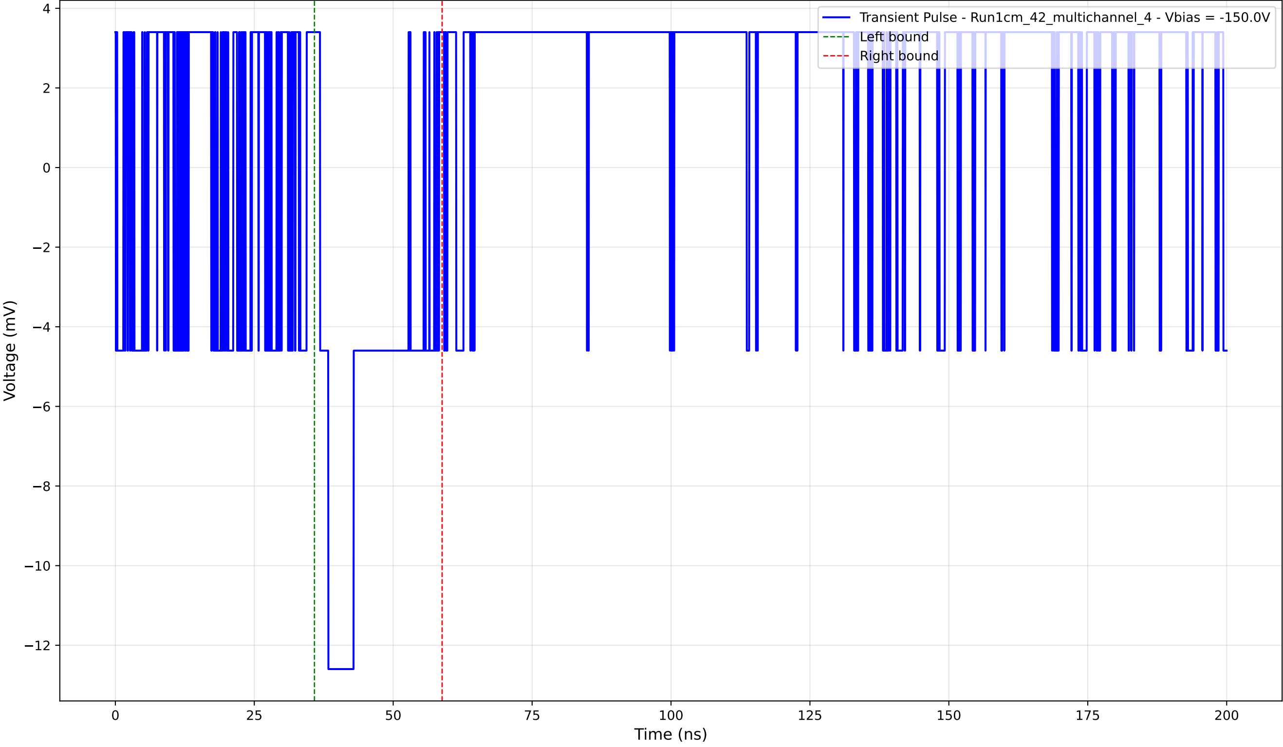
Transient Pulse - Sample: 1cm_42_multichannel - Position: 270.0 \mu\text{m} - Charge: 2.48 pC - Rise Time: 0.00 ns (N/A)
