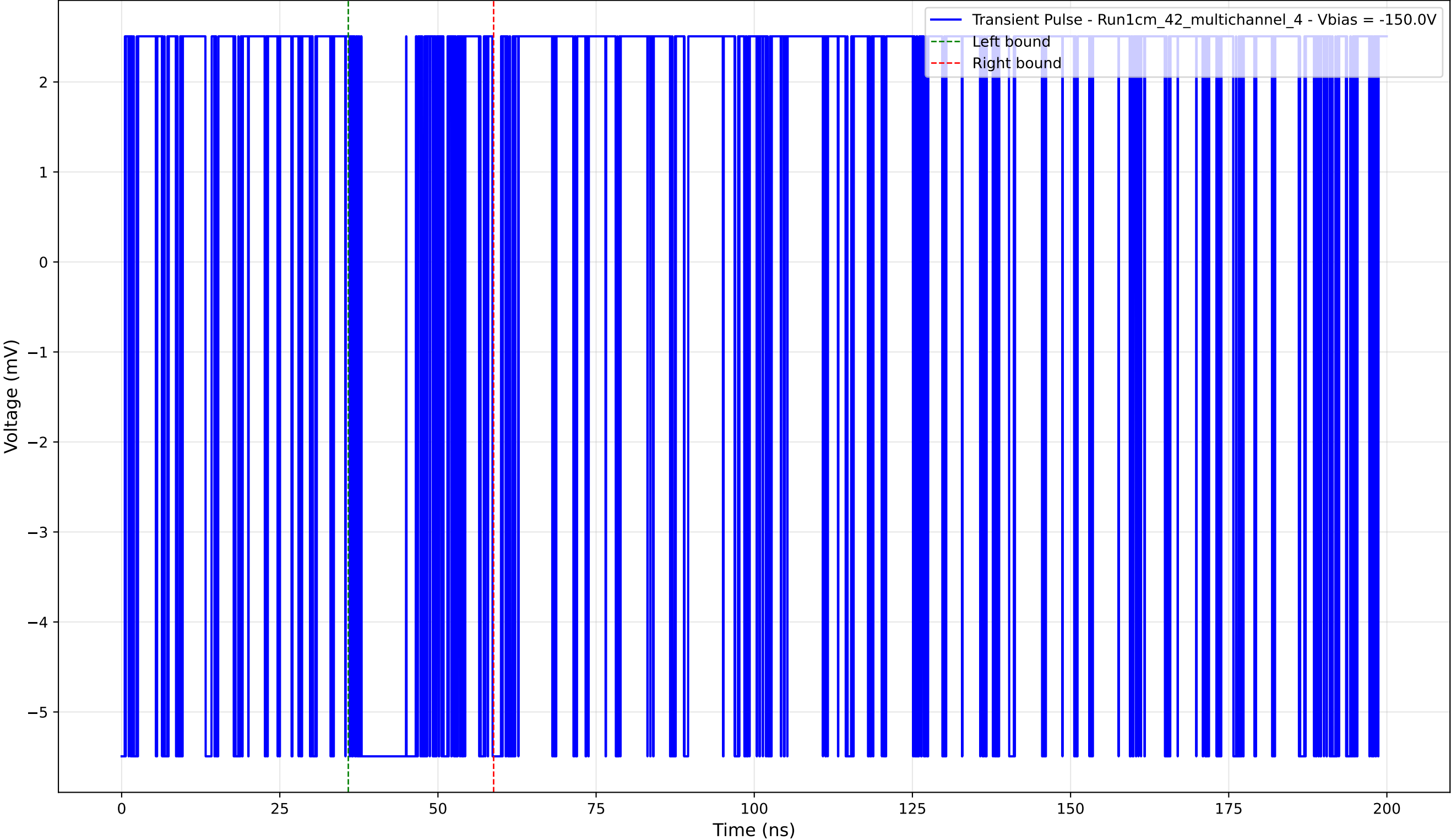
Transient Pulse - Sample: 1cm_42_multichannel - Position: 4370.0 \mu\text{m} - Charge: 1.03 pC - Rise Time: 0.00 ns (N/A)
