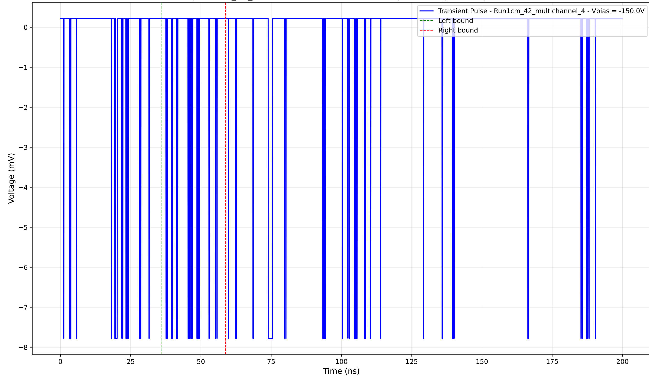
Transient Pulse - Sample: 1cm_42_multichannel - Position: 3915.0 \mu\text{m} - Charge: 0.23 pC - Rise Time: 0.02 ns
