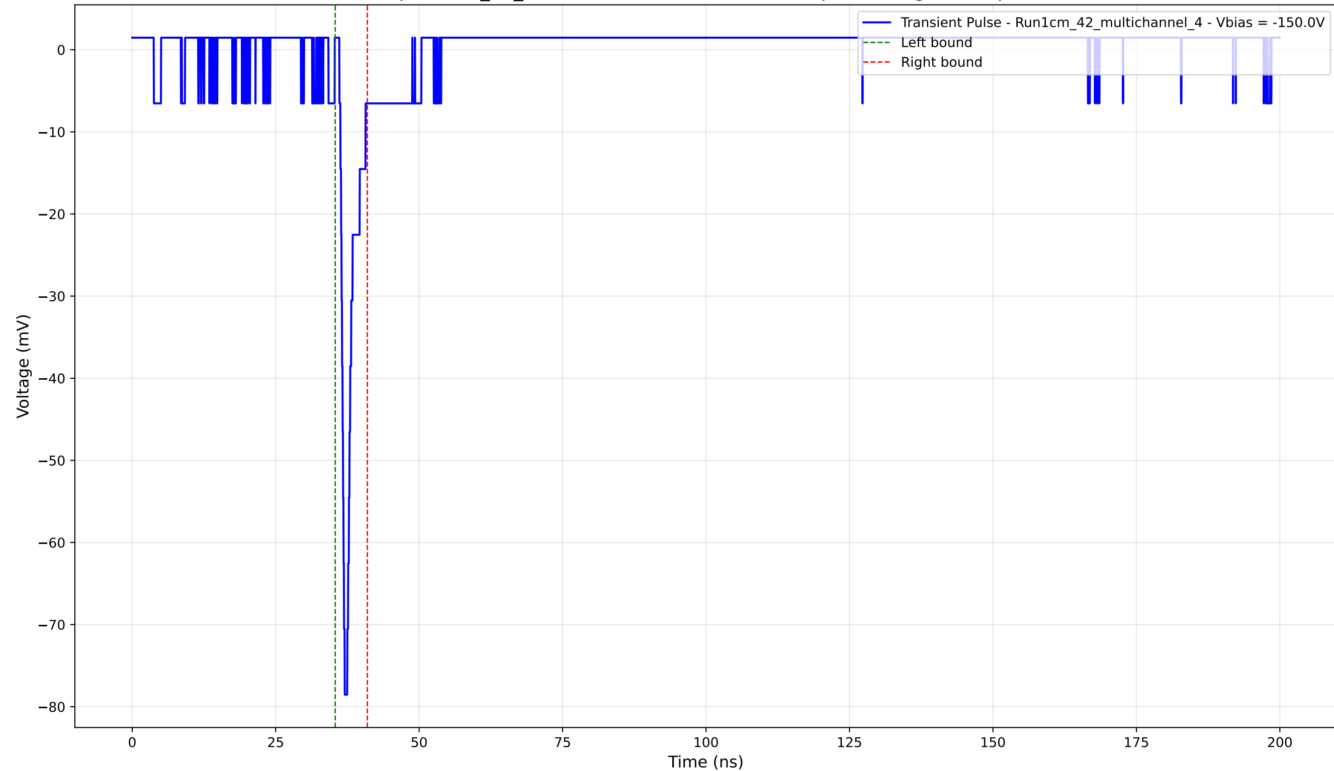
Transient Pulse - Sample: 1cm_42_multichannel - Position: 2290.0 \mu\text{m} - Charge: 3.13 pC - Rise Time: 0.76 ns
