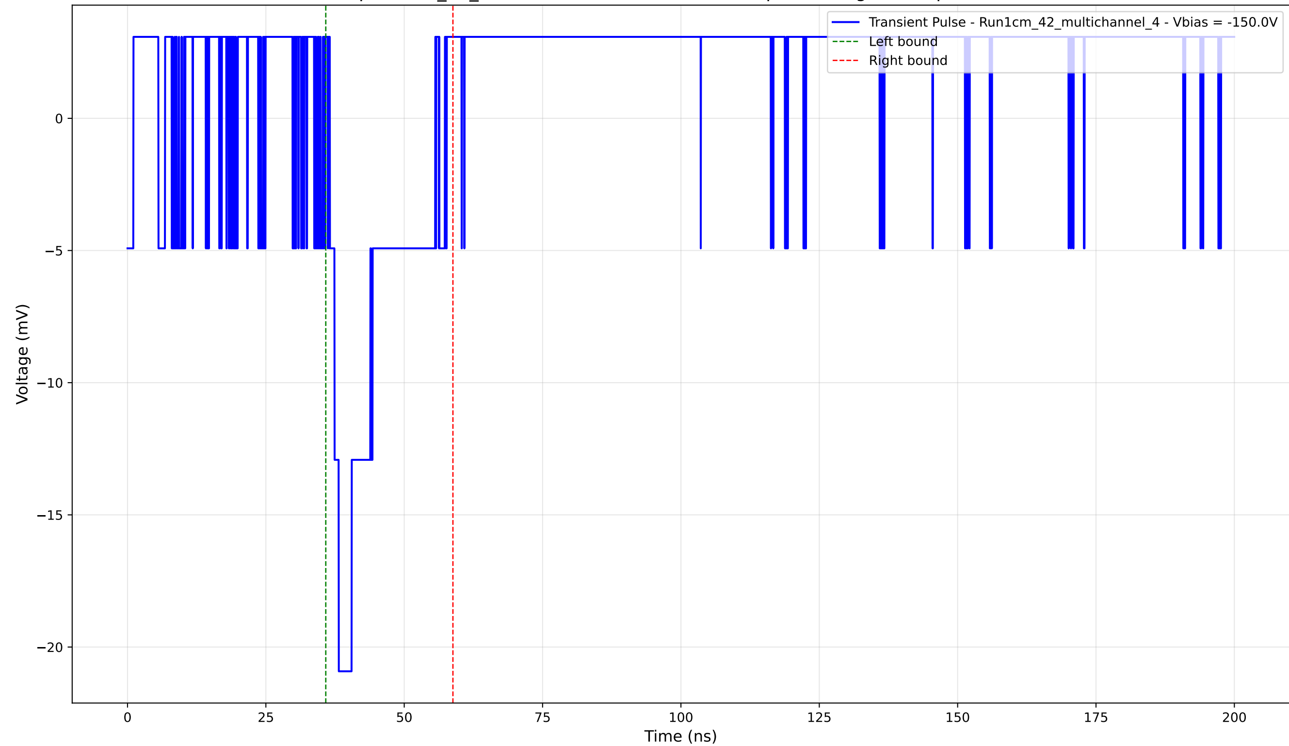
Transient Pulse - Sample: 1cm_42_multichannel - Position: 1035.0 \mu\text{m} - Charge: 3.30 pC - Rise Time: 0.00 ns (N/A)
