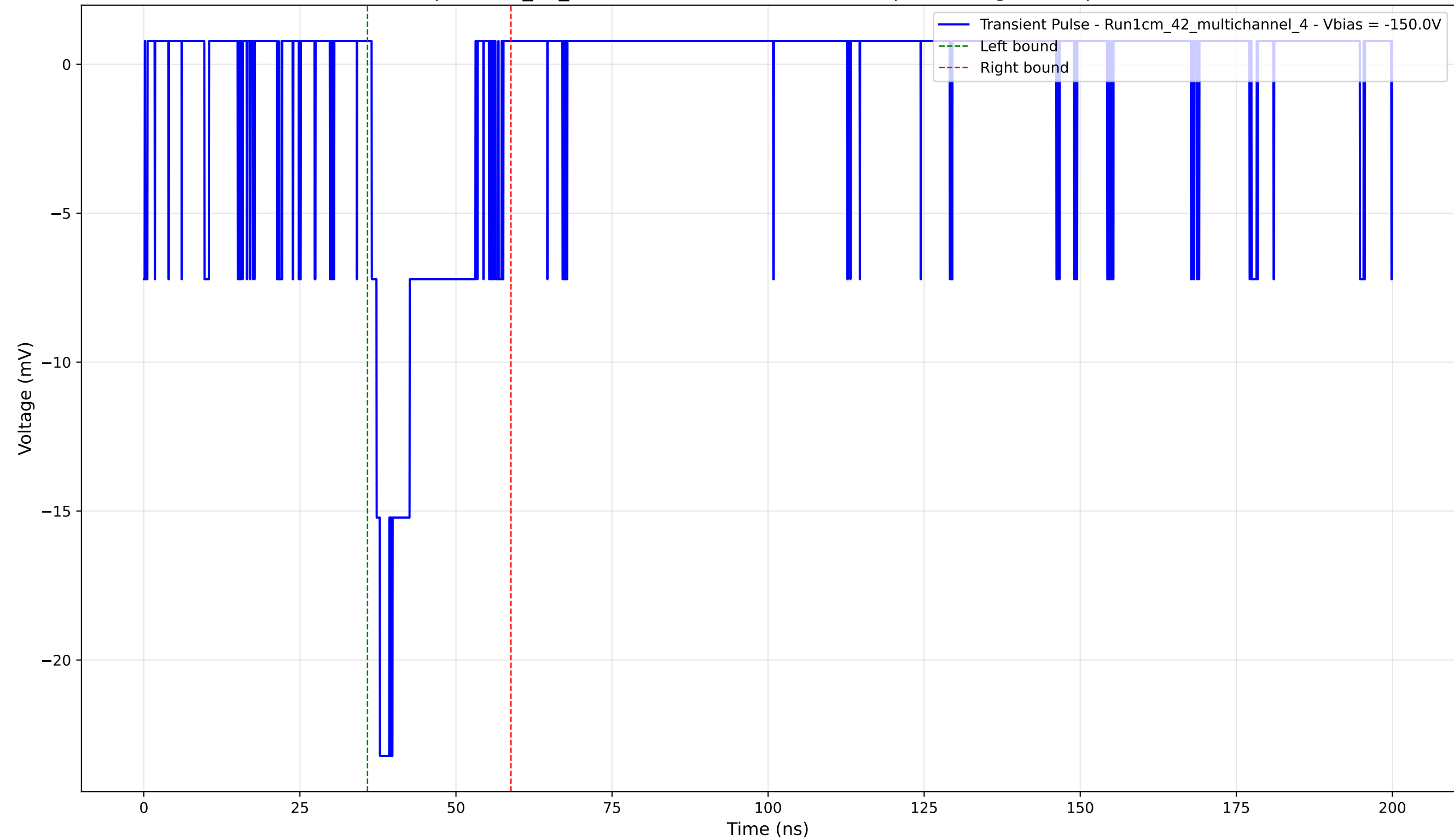
Transient Pulse - Sample: 1cm_42_multichannel - Position: 3510.0 \mu\text{m} - Charge: 3.68 pC - Rise Time: 1.32 ns
