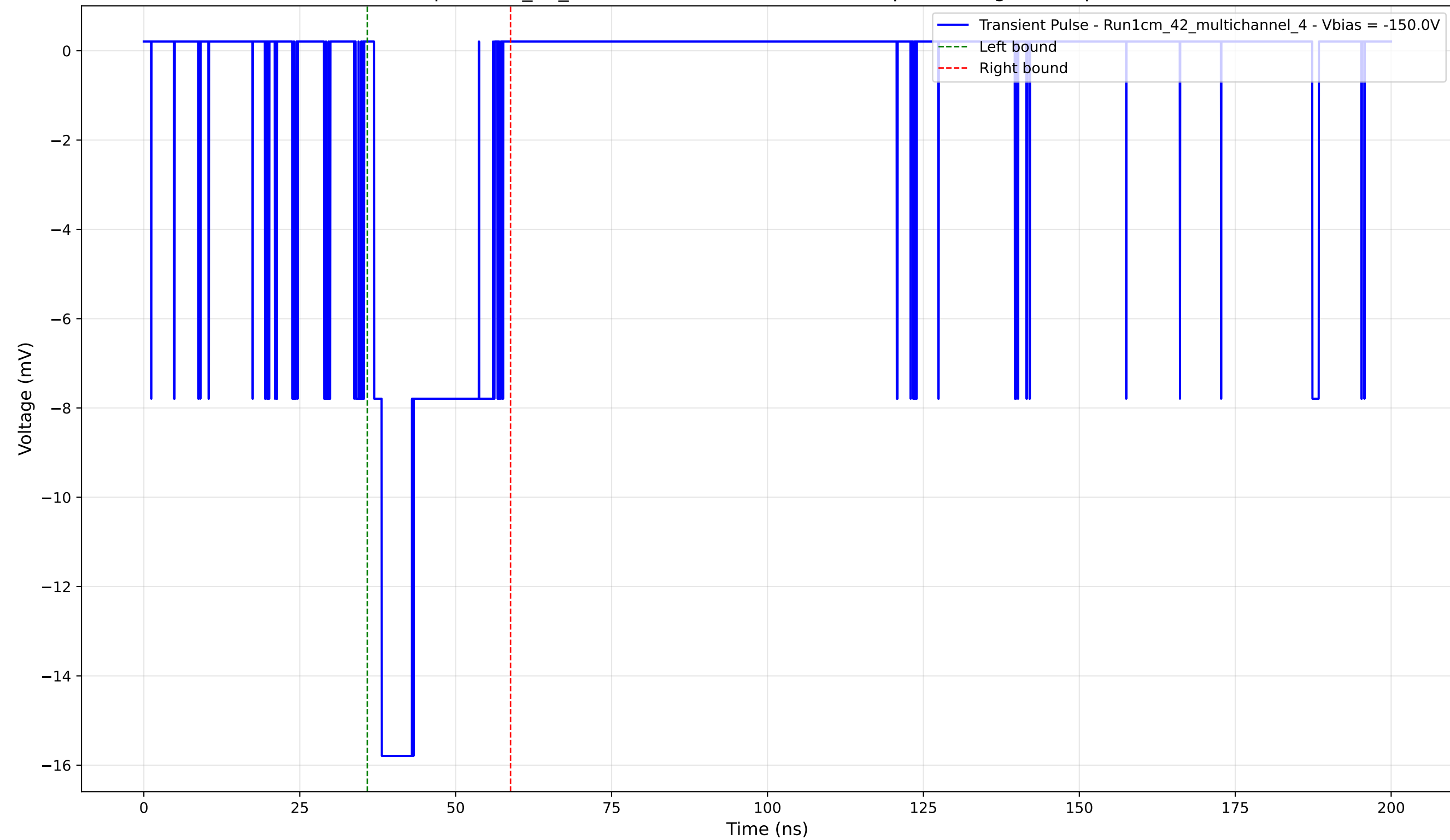
Transient Pulse - Sample: 1cm_42_multichannel - Position: 4035.0 \mu\text{m} - Charge: 3.86 pC - Rise Time: 1.24 ns
