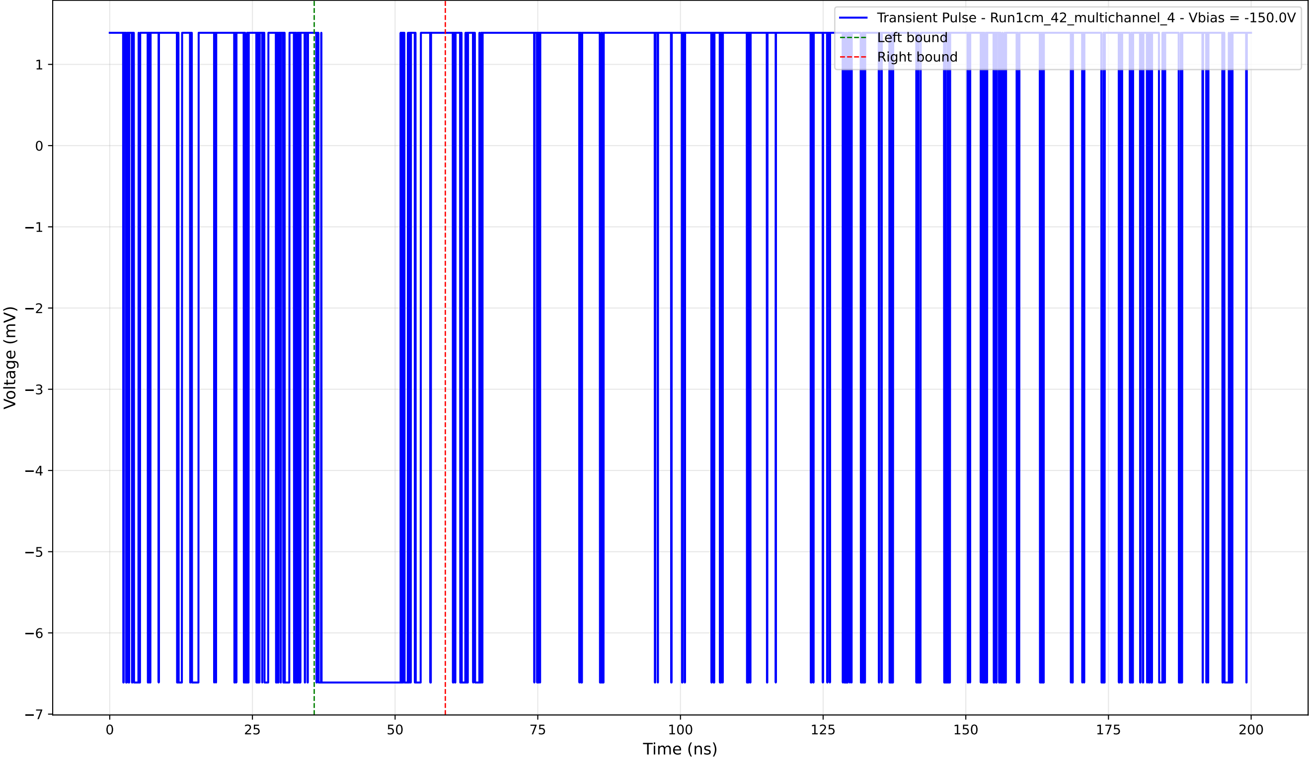
Transient Pulse - Sample: 1cm_42_multichannel - Position: 4450.0 \mu\text{m} - Charge: 2.03 pC - Rise Time: 0.00 ns (N/A)
