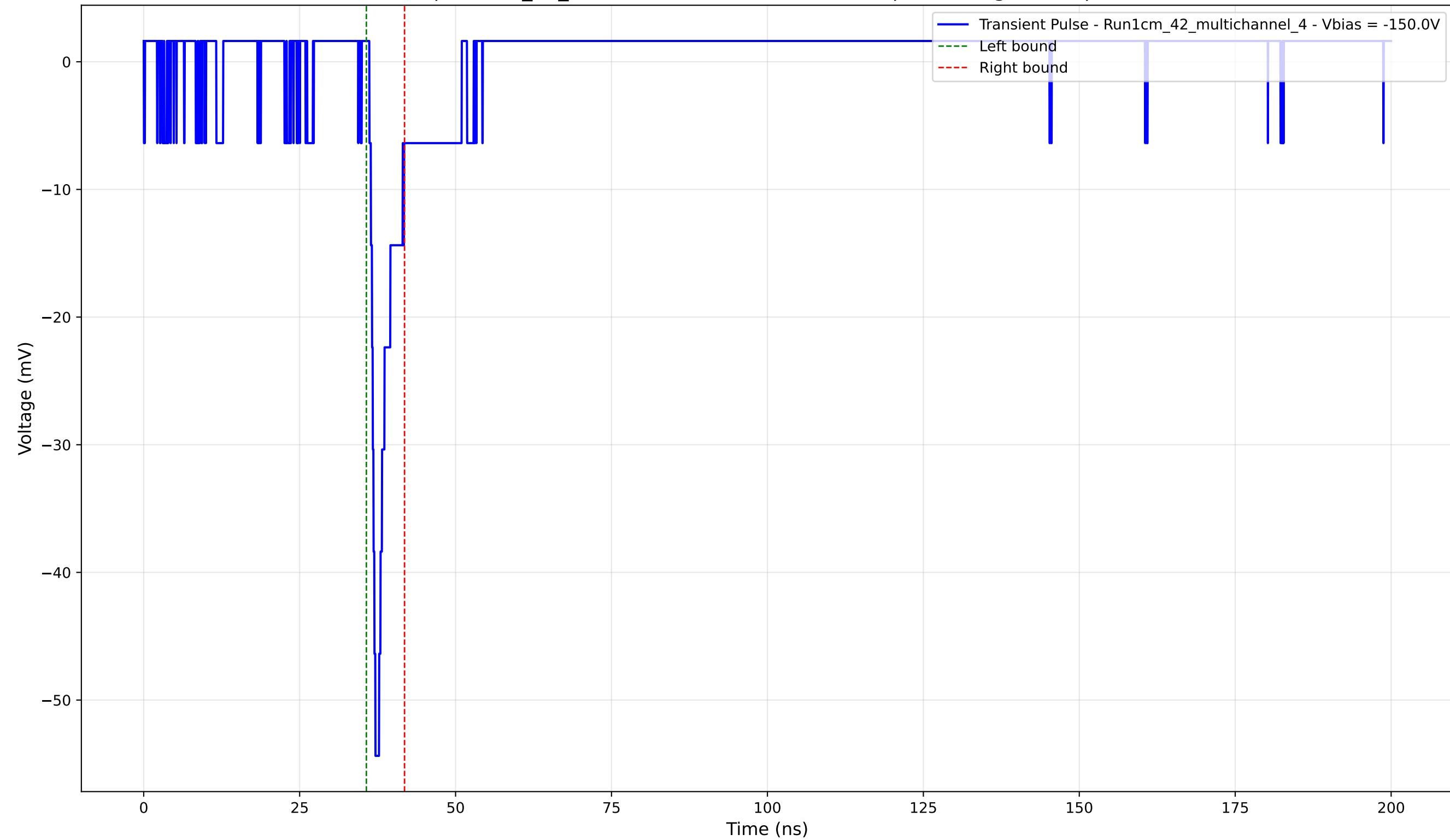
Transient Pulse - Sample: 1cm_42_multichannel - Position: 2070.0 \mu\text{m} - Charge: 2.78 pC - Rise Time: 0.96 ns
