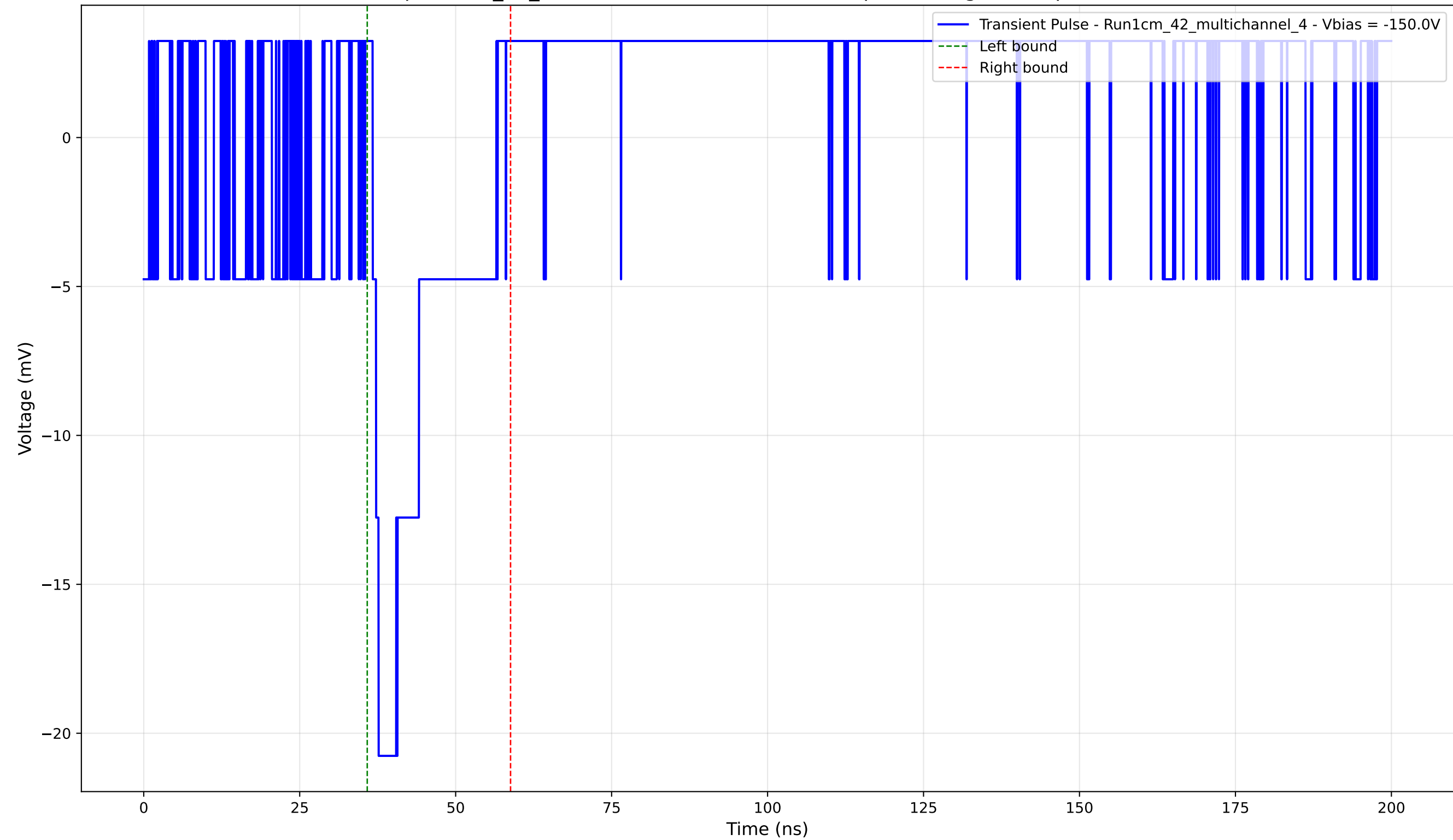
Transient Pulse - Sample: 1cm_42_multichannel - Position: 1215.0 \mu\text{m} - Charge: 3.29 pC - Rise Time: 0.00 ns (N/A)
