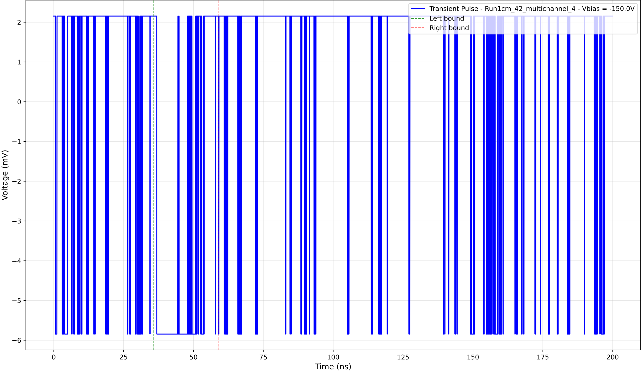
Transient Pulse - Sample: 1cm_42_multichannel - Position: 3440.0 \mu\text{m} - Charge: 1.26 pC - Rise Time: 0.00 ns (N/A)
