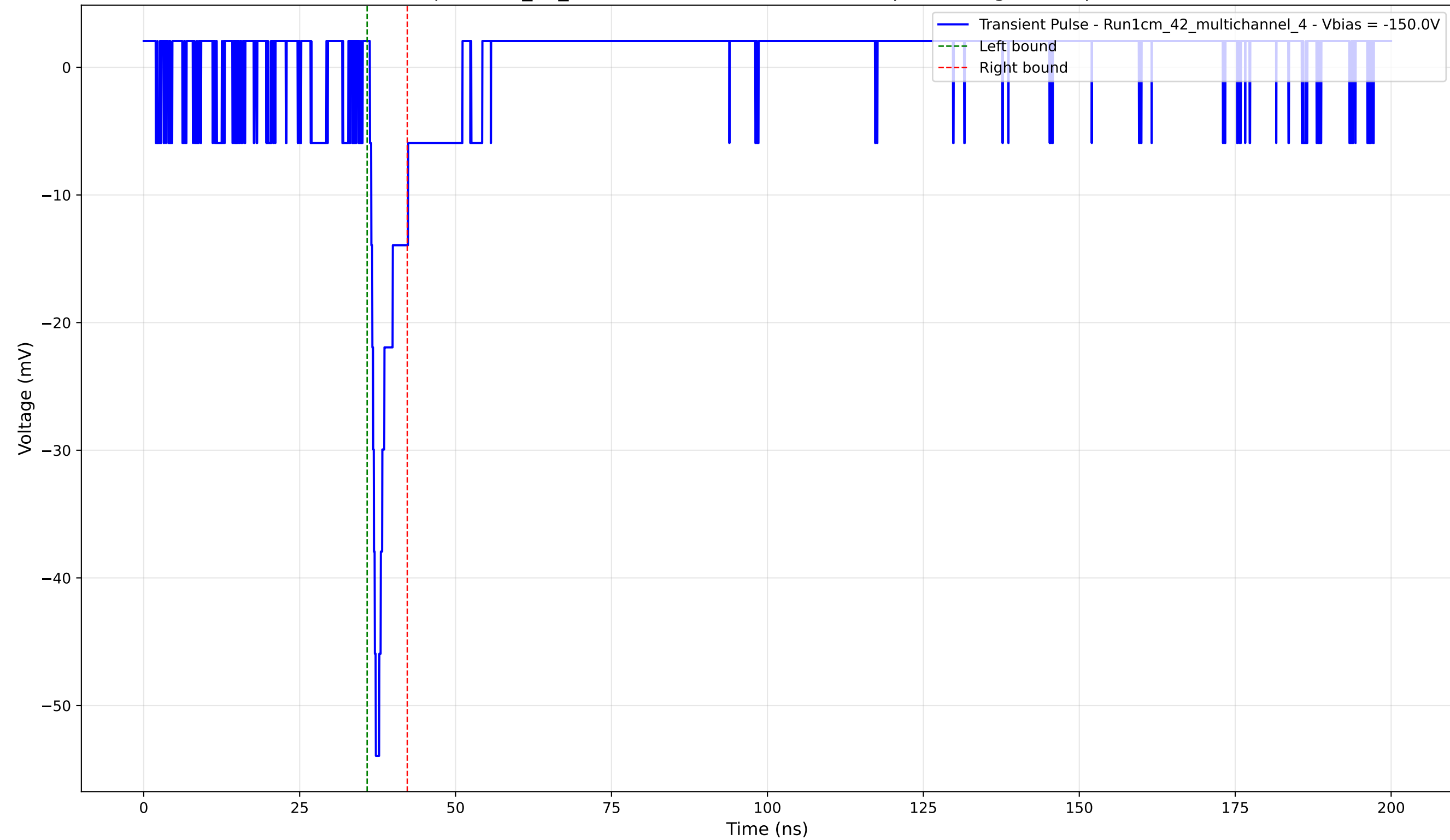
Transient Pulse - Sample: 1cm_42_multichannel - Position: 2760.0 \mu\text{m} - Charge: 2.89 pC - Rise Time: 0.94 ns
