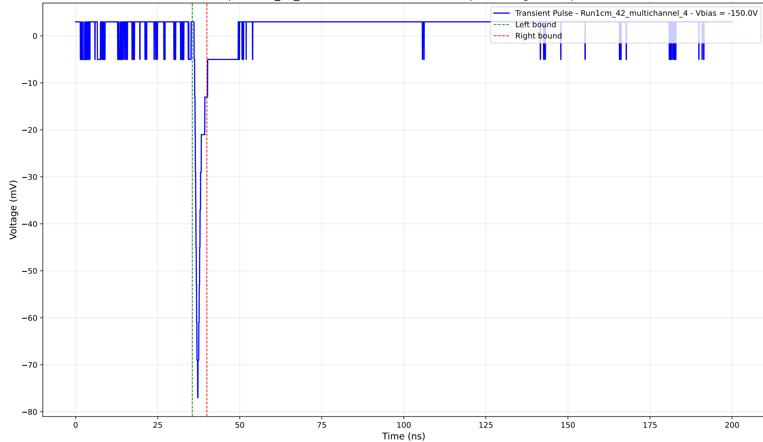
Transient Pulse - Sample: 1cm_42_multichannel - Position: 2455.0 \mu\text{m} - Charge: 2.55 pC - Rise Time: 0.93 ns
