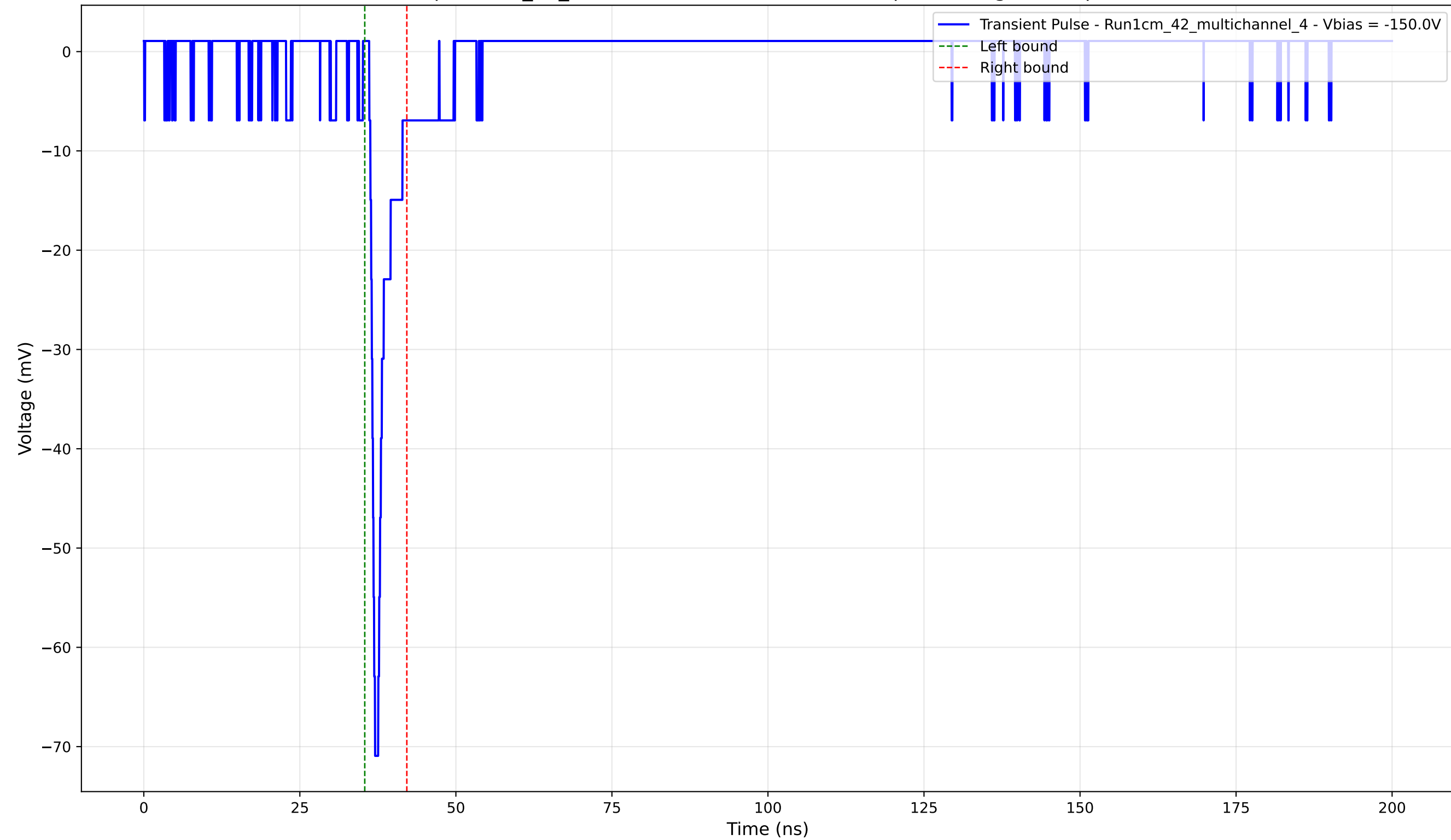
Transient Pulse - Sample: 1cm_42_multichannel - Position: 2530.0 \mu\text{m} - Charge: 3.27 pC - Rise Time: 0.76 ns
