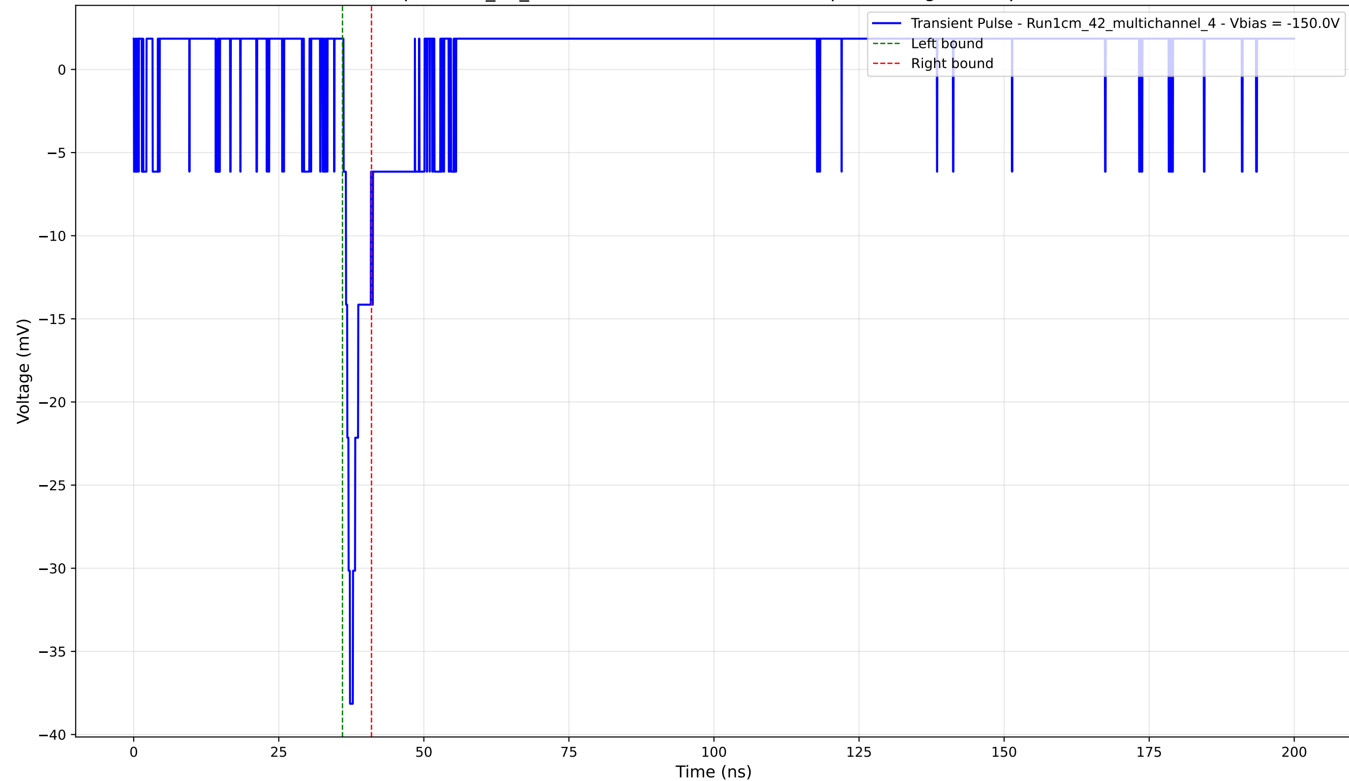
Transient Pulse - Sample: 1cm_42_multichannel - Position: 2830.0 \mu\text{m} - Charge: 1.84 pC - Rise Time: 1.11 ns
