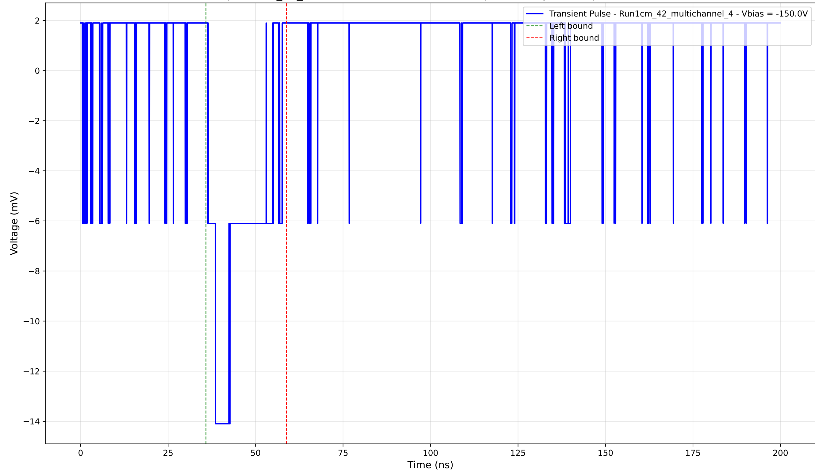
Transient Pulse - Sample: 1cm_42_multichannel - Position: 4740.0 \mu\text{m} - Charge: 2.90 pC - Rise Time: 0.00 ns (N/A)
