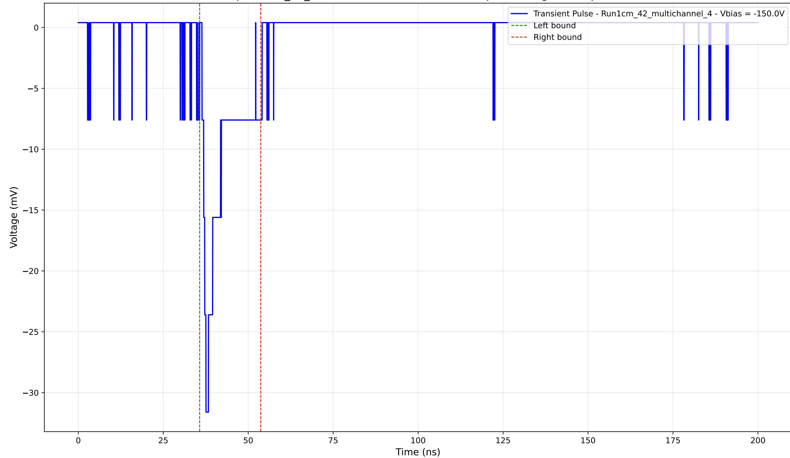
Transient Pulse - Sample: 1cm_42_multichannel - Position: 3190.0 \mu\text{m} - Charge: 3.93 pC - Rise Time: 1.17 ns
