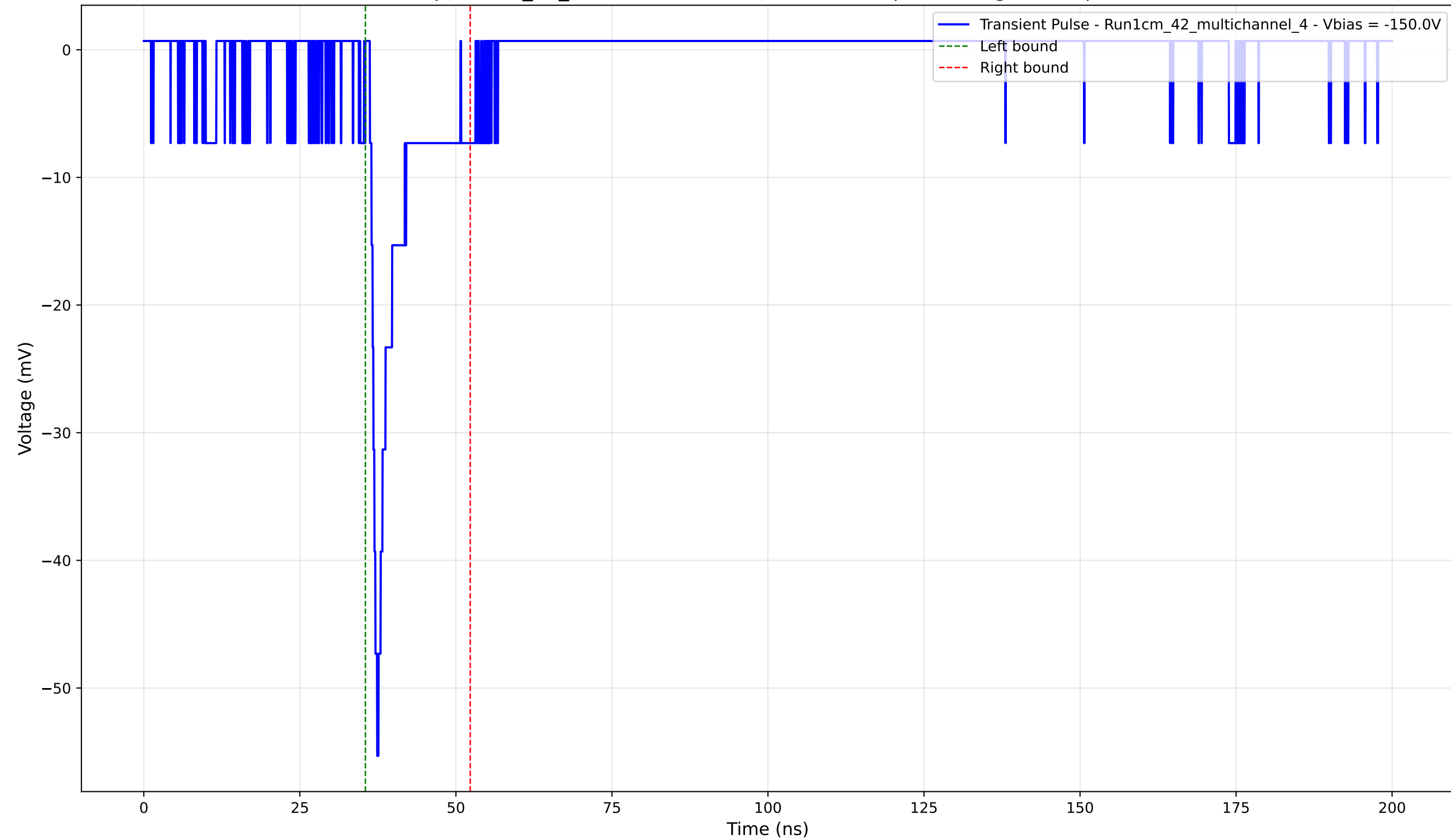
Transient Pulse - Sample: 1cm_42_multichannel - Position: 2785.0 \mu\text{m} - Charge: 4.39 pC - Rise Time: 1.17 ns
