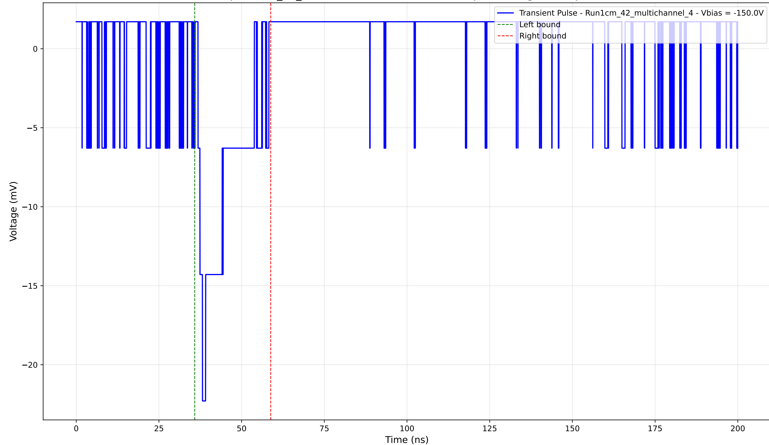
Transient Pulse - Sample: 1cm_42_multichannel - Position: 1085.0 \mu\text{m} - Charge: 3.61 pC - Rise Time: 1.36 ns
