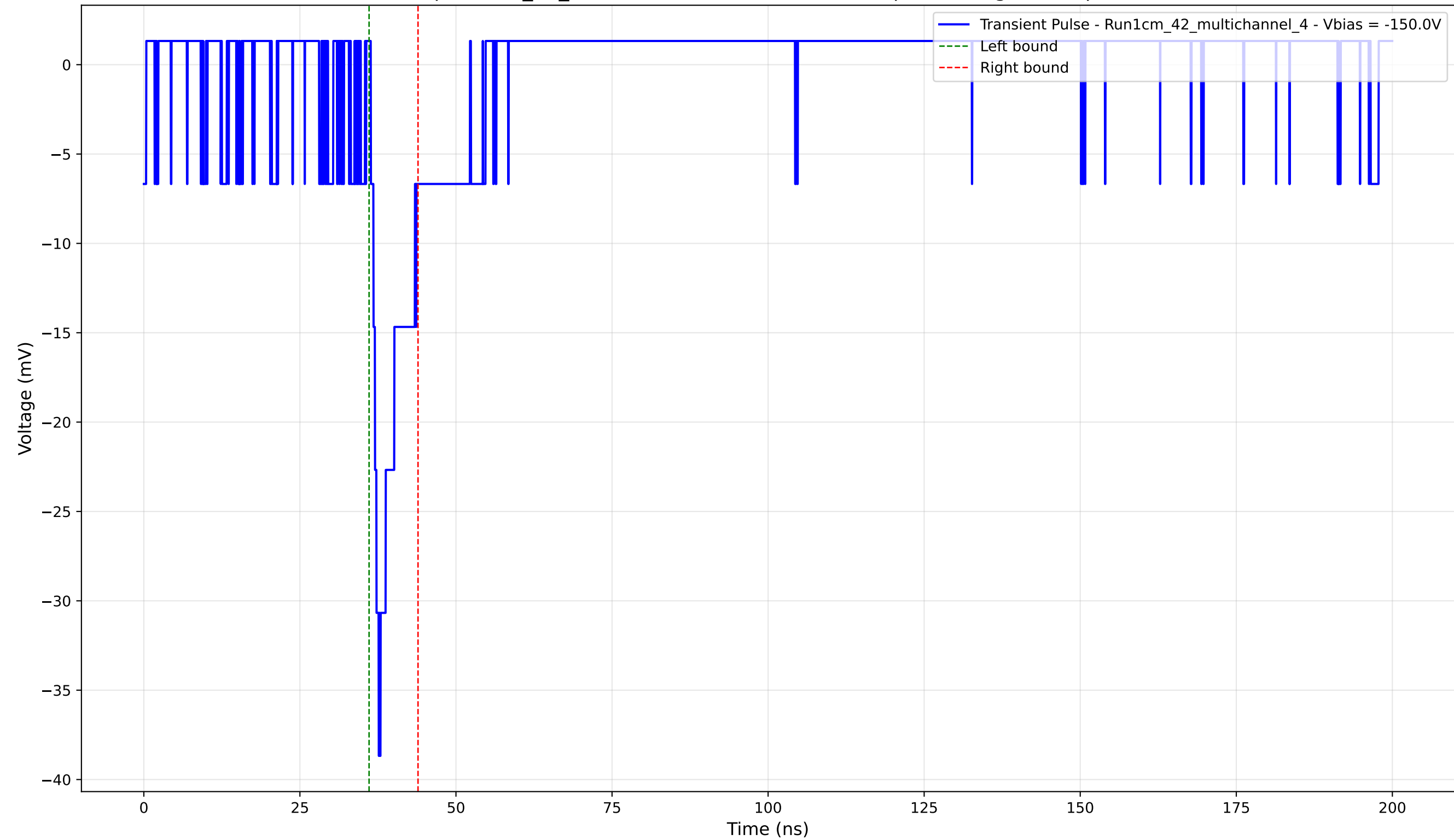
Transient Pulse - Sample: 1cm_42_multichannel - Position: 1655.0 \mu\text{m} - Charge: 2.84 pC - Rise Time: 1.27 ns
