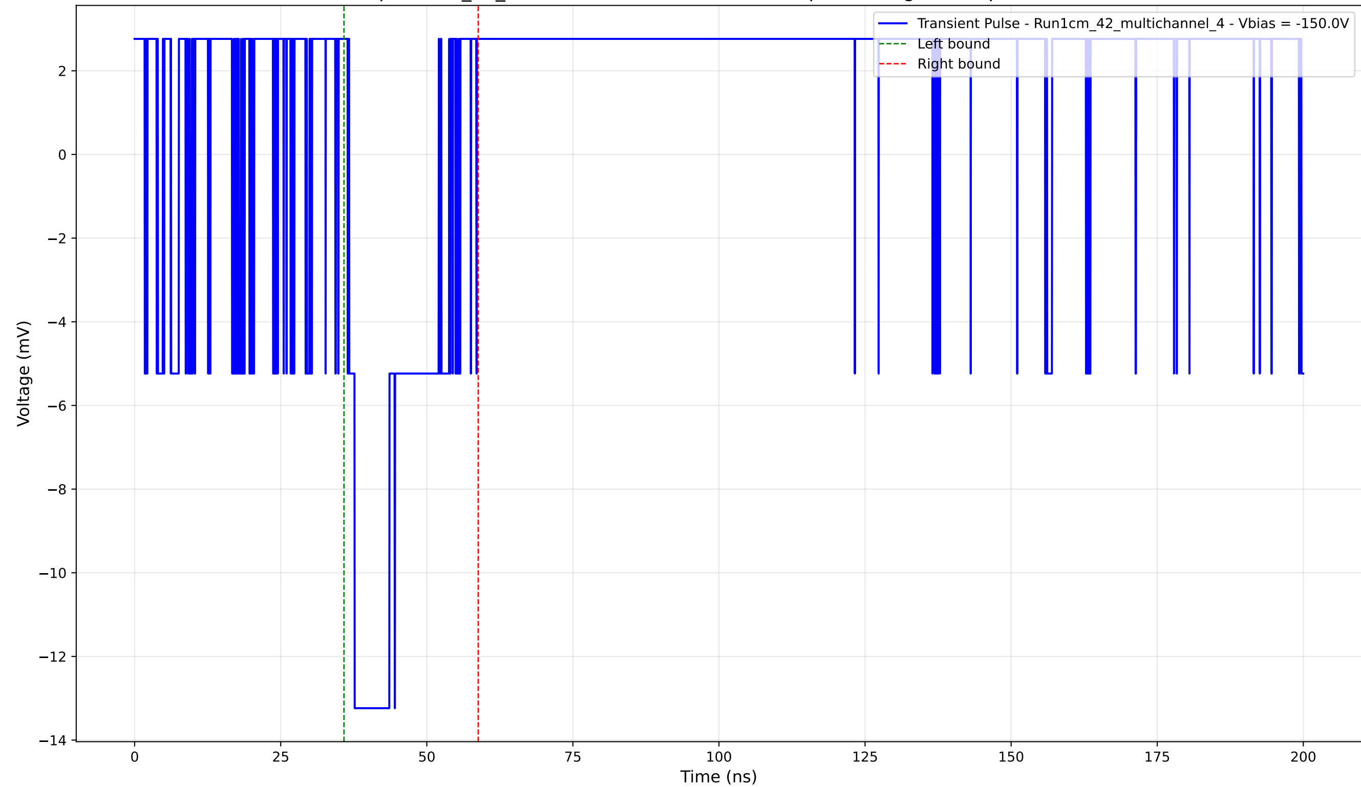
Transient Pulse - Sample: 1cm_42_multichannel - Position: 3780.0 \mu\text{m} - Charge: 2.56 pC - Rise Time: 0.00 ns (N/A)
