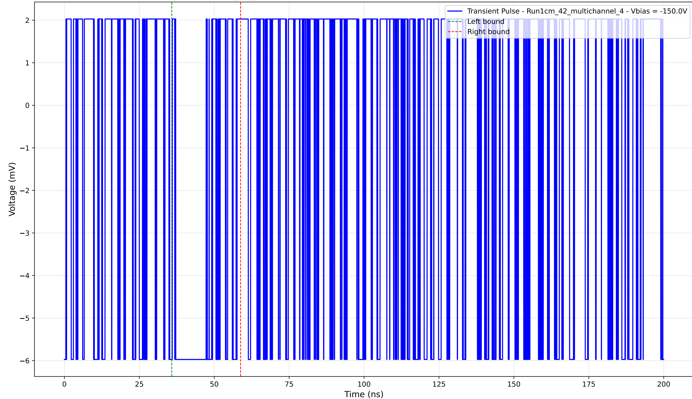
Transient Pulse - Sample: 1cm_42_multichannel - Position: 1340.0 \mu\text{m} - Charge: 1.48 pC - Rise Time: 0.00 ns (N/A)
