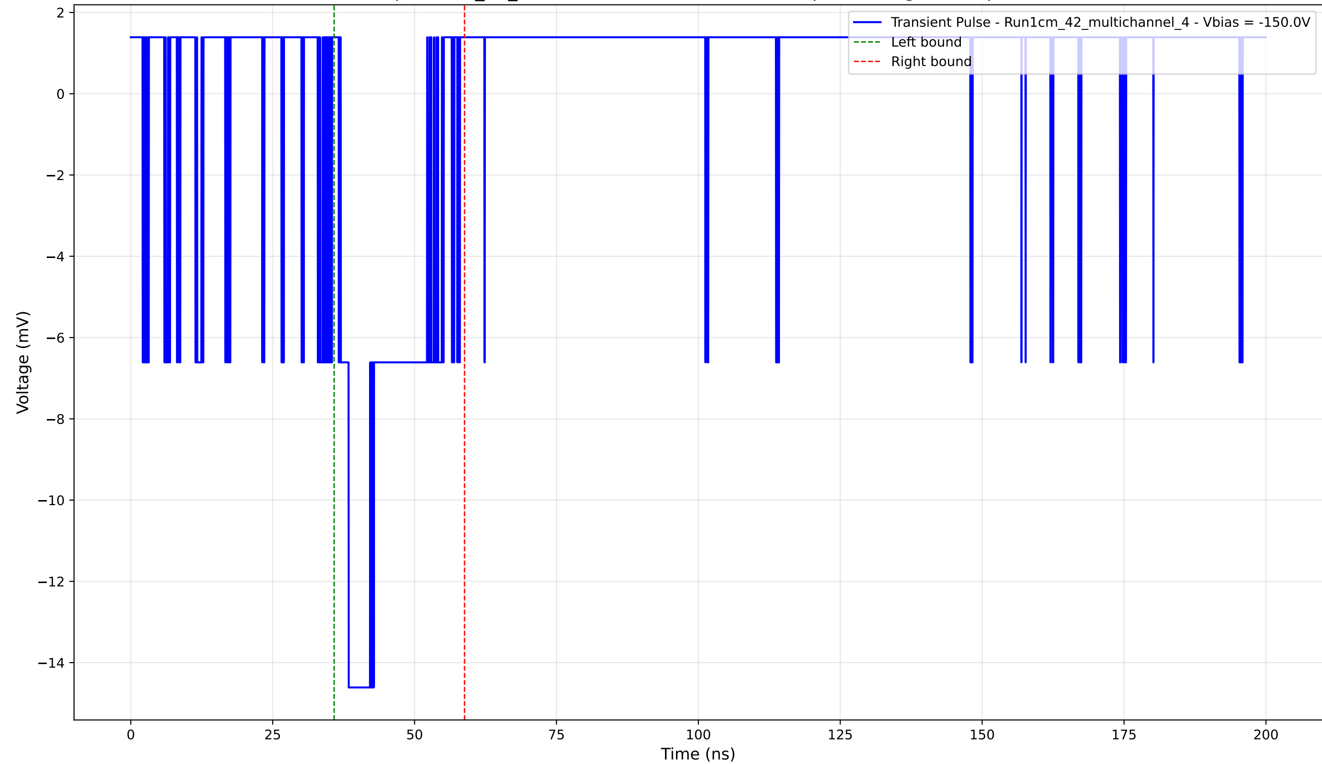
Transient Pulse - Sample: 1cm_42_multichannel - Position: 4670.0 \mu\text{m} - Charge: 2.95 pC - Rise Time: 1.40 ns
