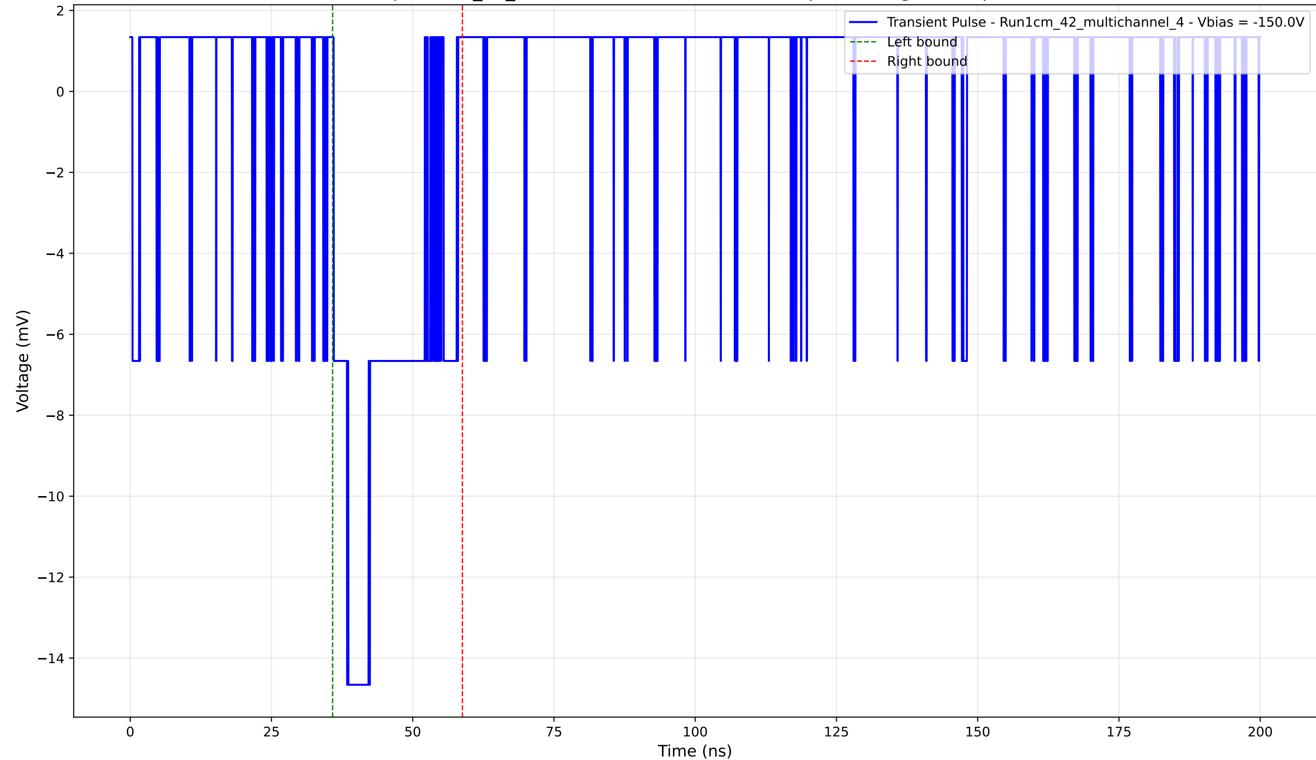
Transient Pulse - Sample: 1cm_42_multichannel - Position: 4795.0 \mu\text{m} - Charge: 3.22 pC - Rise Time: 2.38 ns
