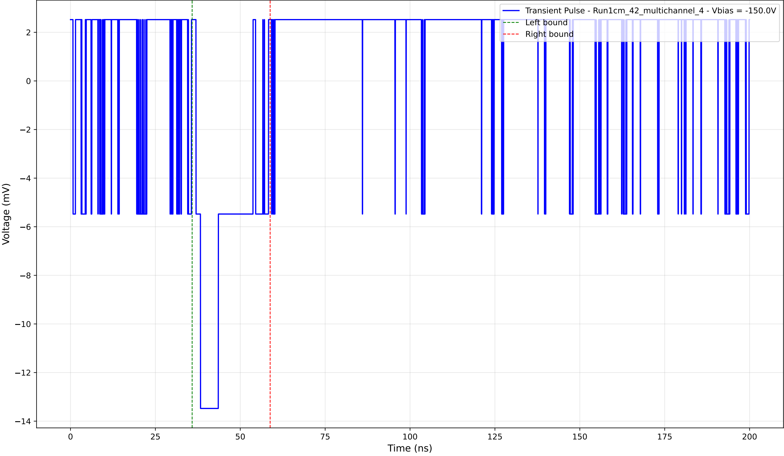
Transient Pulse - Sample: 1cm_42_multichannel - Position: 460.0 \mu\text{m} - Charge: 2.96 pC - Rise Time: 0.00 ns (N/A)
