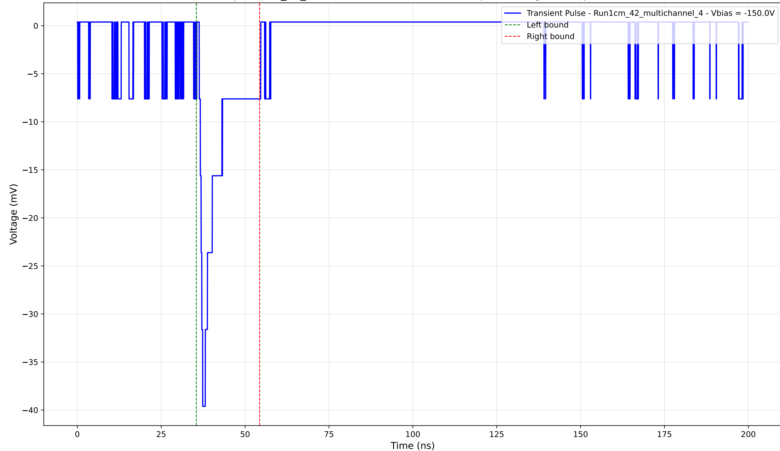
Transient Pulse - Sample: 1cm_42_multichannel - Position: 1725.0 \mu\text{m} - Charge: 4.74 pC - Rise Time: 1.03 ns
