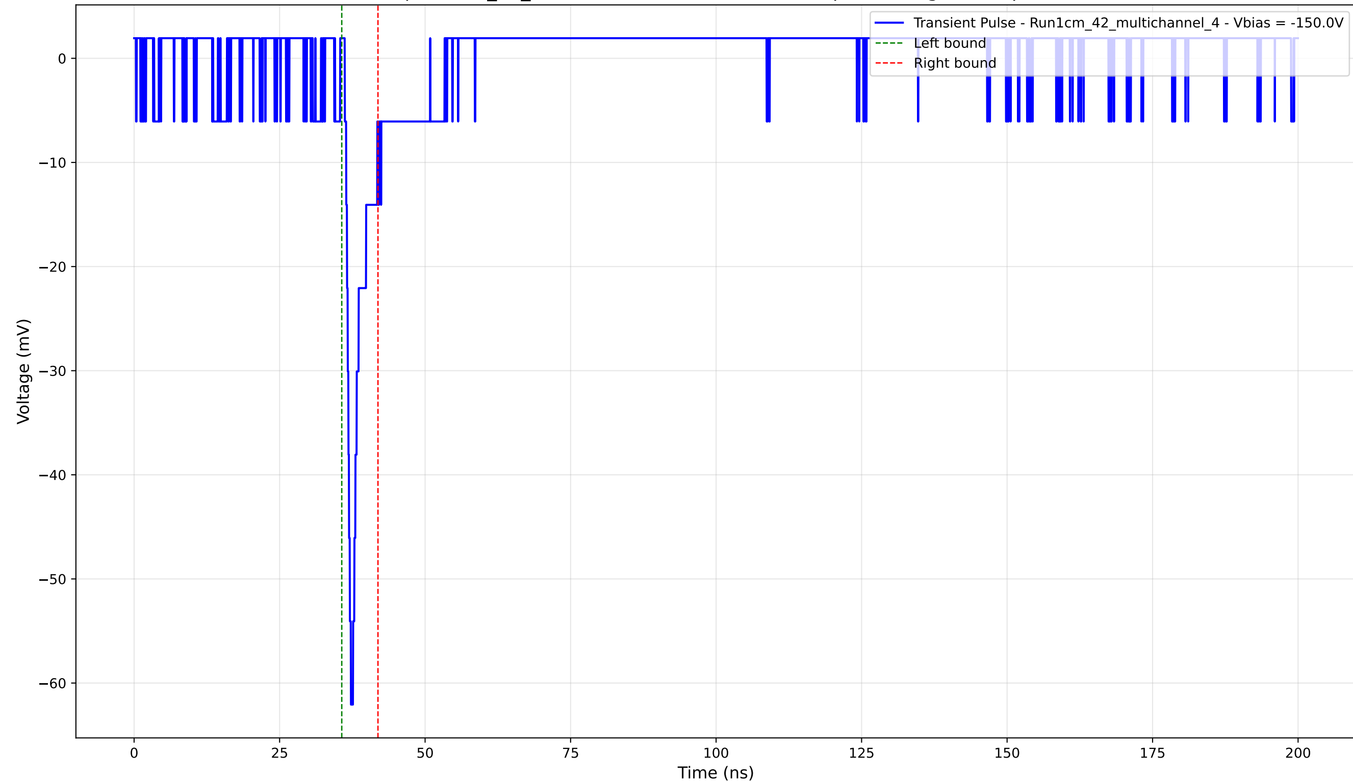
Transient Pulse - Sample: 1cm_42_multichannel - Position: 2080.0 \mu\text{m} - Charge: 2.94 pC - Rise Time: 0.82 ns
