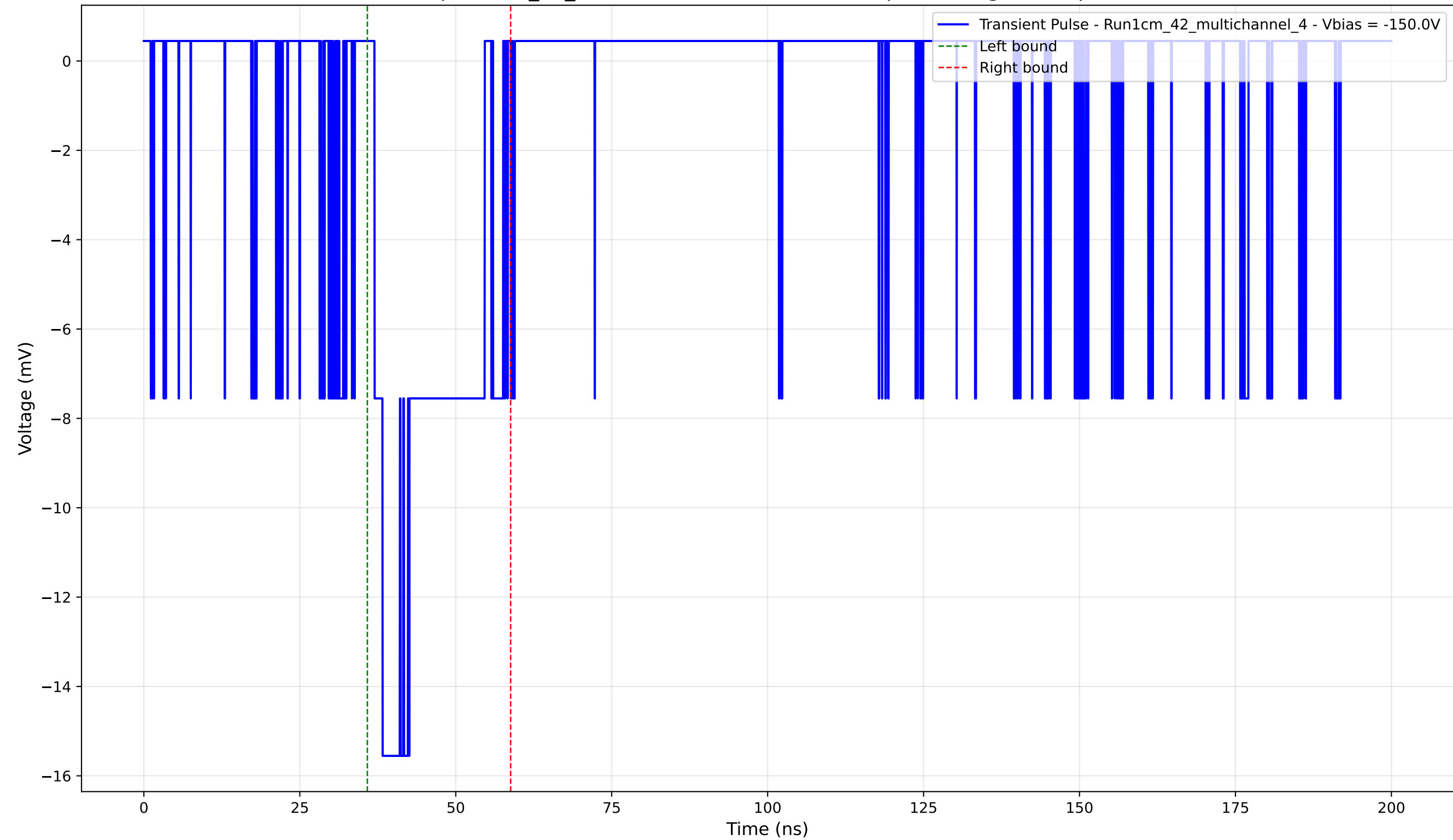
Transient Pulse - Sample: 1cm_42_multichannel - Position: 185.0 \mu\text{m} - Charge: 3.55 pC - Rise Time: 1.30 ns
