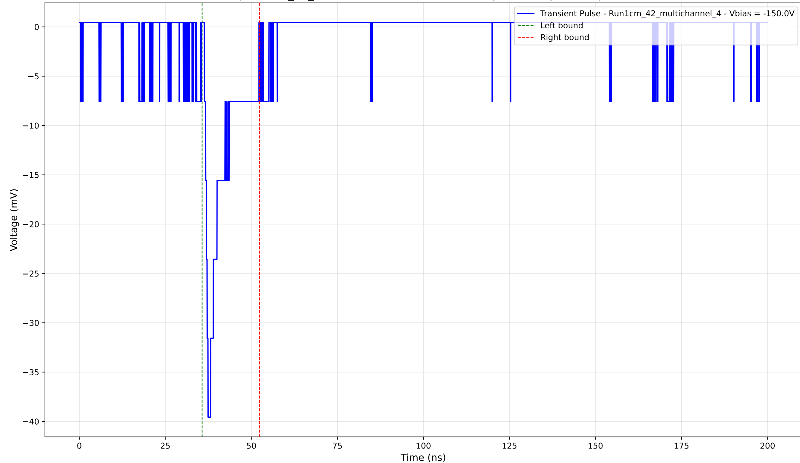
Transient Pulse - Sample: 1cm_42_multichannel - Position: 1720.0 \mu\text{m} - Charge: 4.37 pC - Rise Time: 1.05 ns
