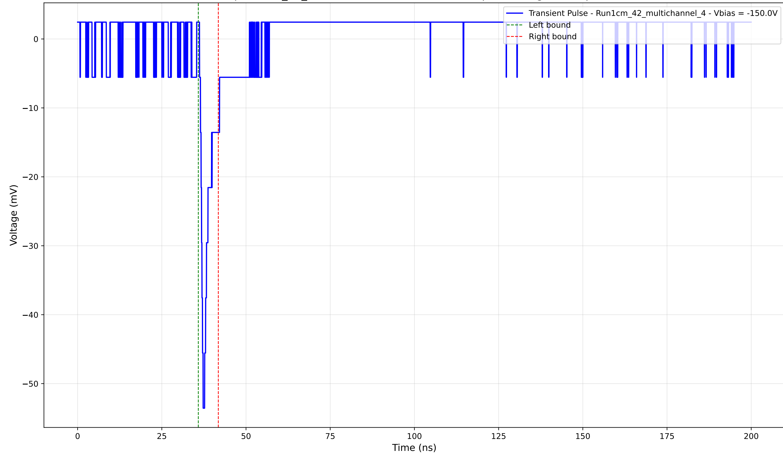
Transient Pulse - Sample: 1cm_42_multichannel - Position: 2775.0 \mu\text{m} - Charge: 2.70 pC - Rise Time: 1.06 ns
