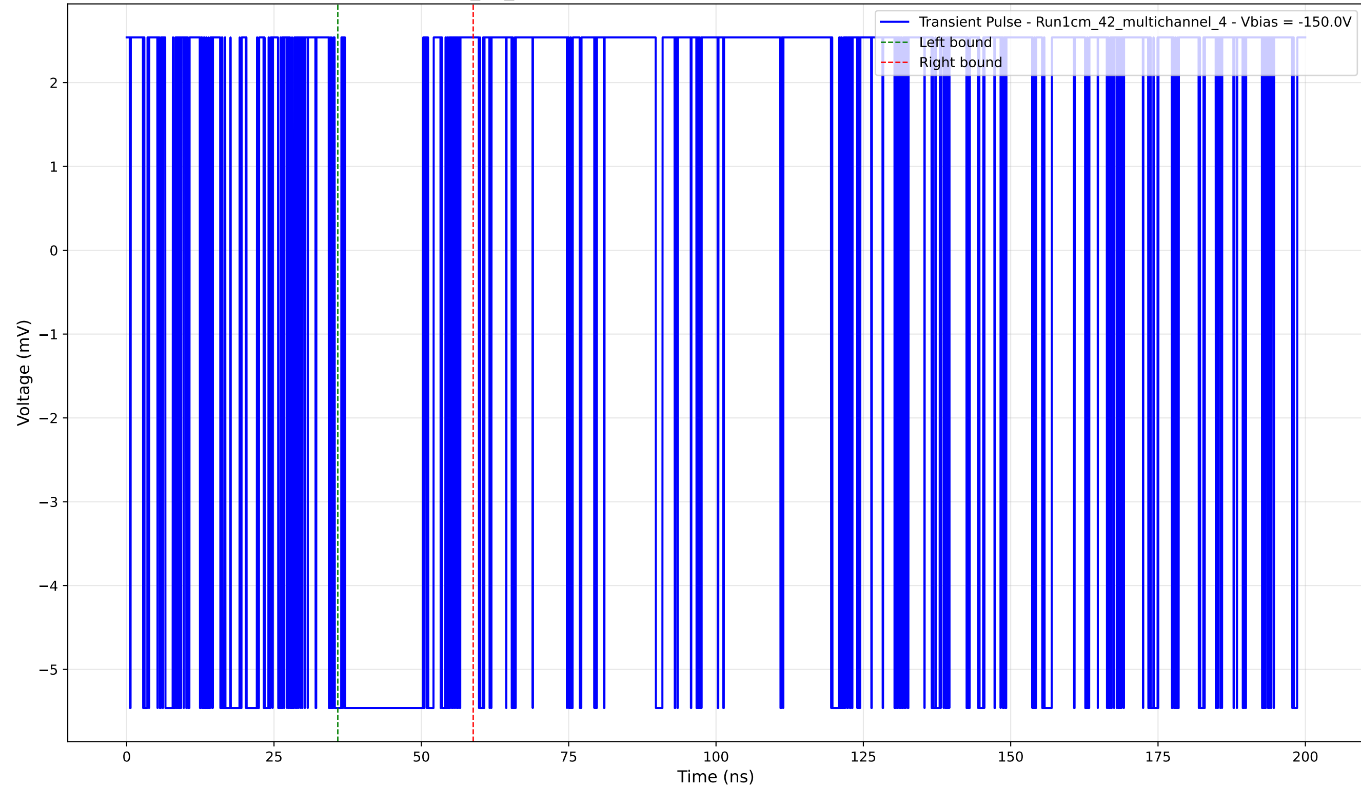
Transient Pulse - Sample: 1cm_42_multichannel - Position: 85.0 \mu\text{m} - Charge: 1.52 pC - Rise Time: 0.00 ns (N/A)
