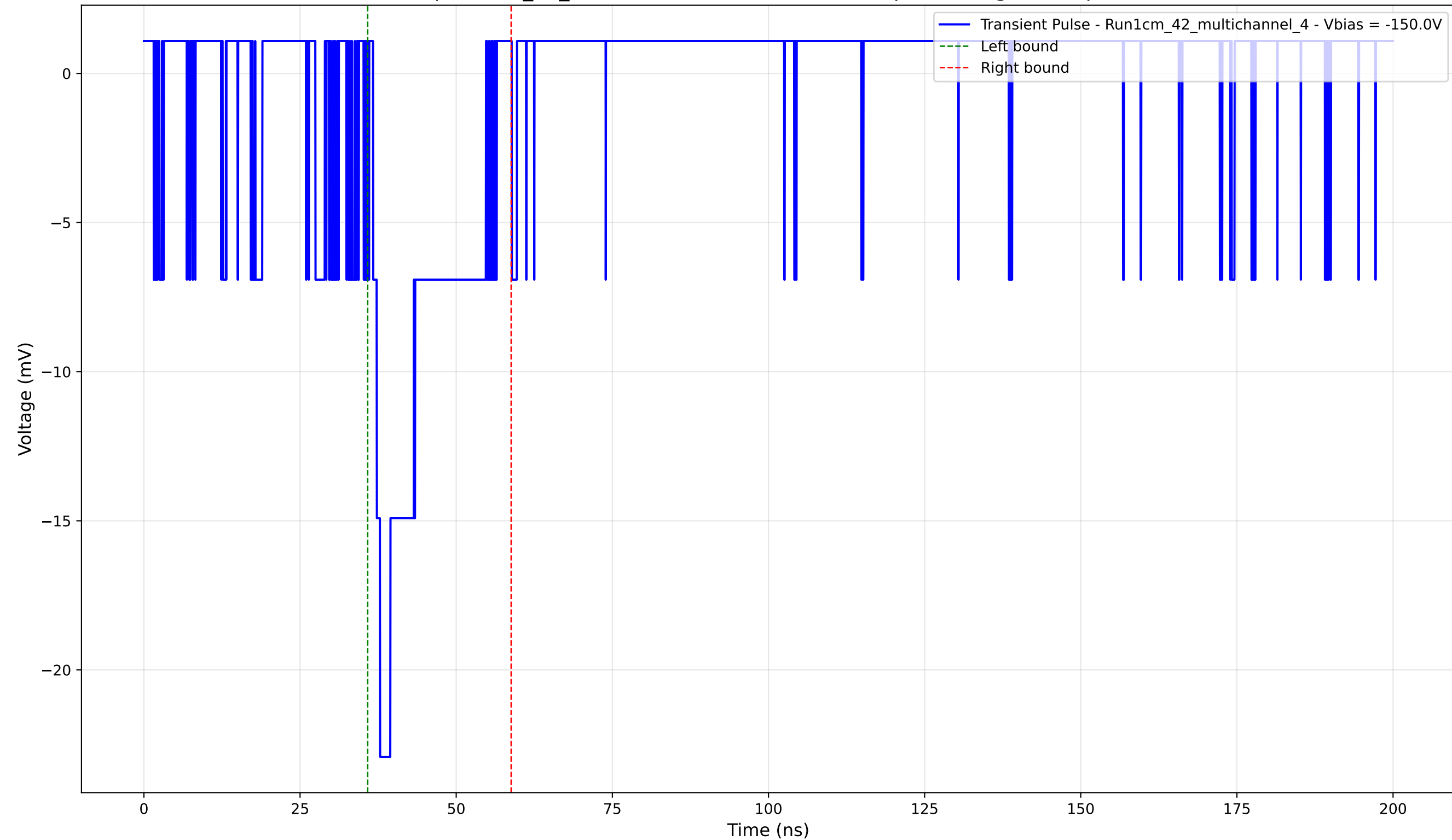
Transient Pulse - Sample: 1cm_42_multichannel - Position: 3515.0 \mu\text{m} - Charge: 3.81 pC - Rise Time: 1.12 ns
