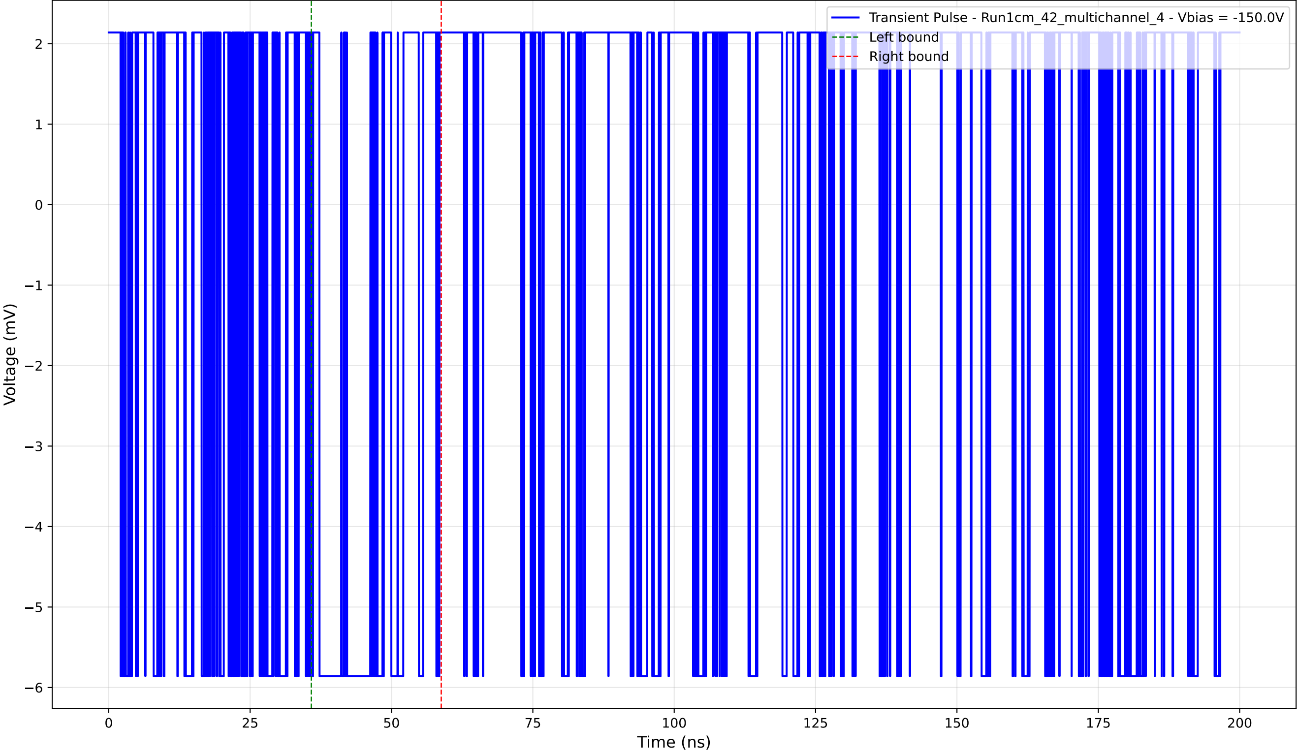
Transient Pulse - Sample: 1cm_42_multichannel - Position: 75.0 \mu\text{m} - Charge: 1.23 pC - Rise Time: 0.00 ns (N/A)
