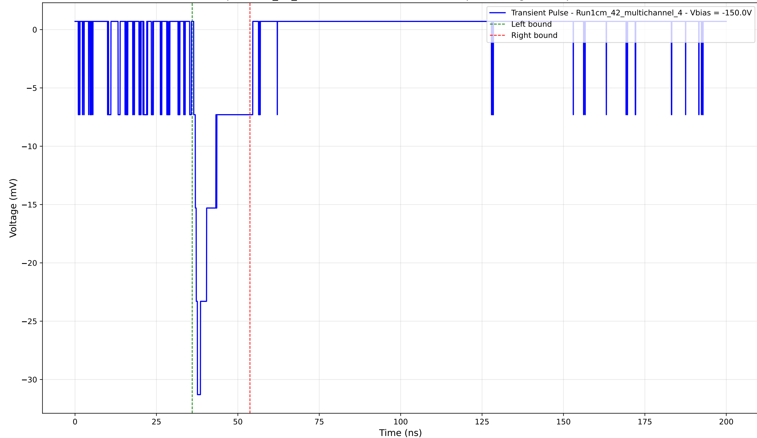
Transient Pulse - Sample: 1cm_42_multichannel - Position: 1495.0 \mu\text{m} - Charge: 4.21 pC - Rise Time: 1.15 ns
