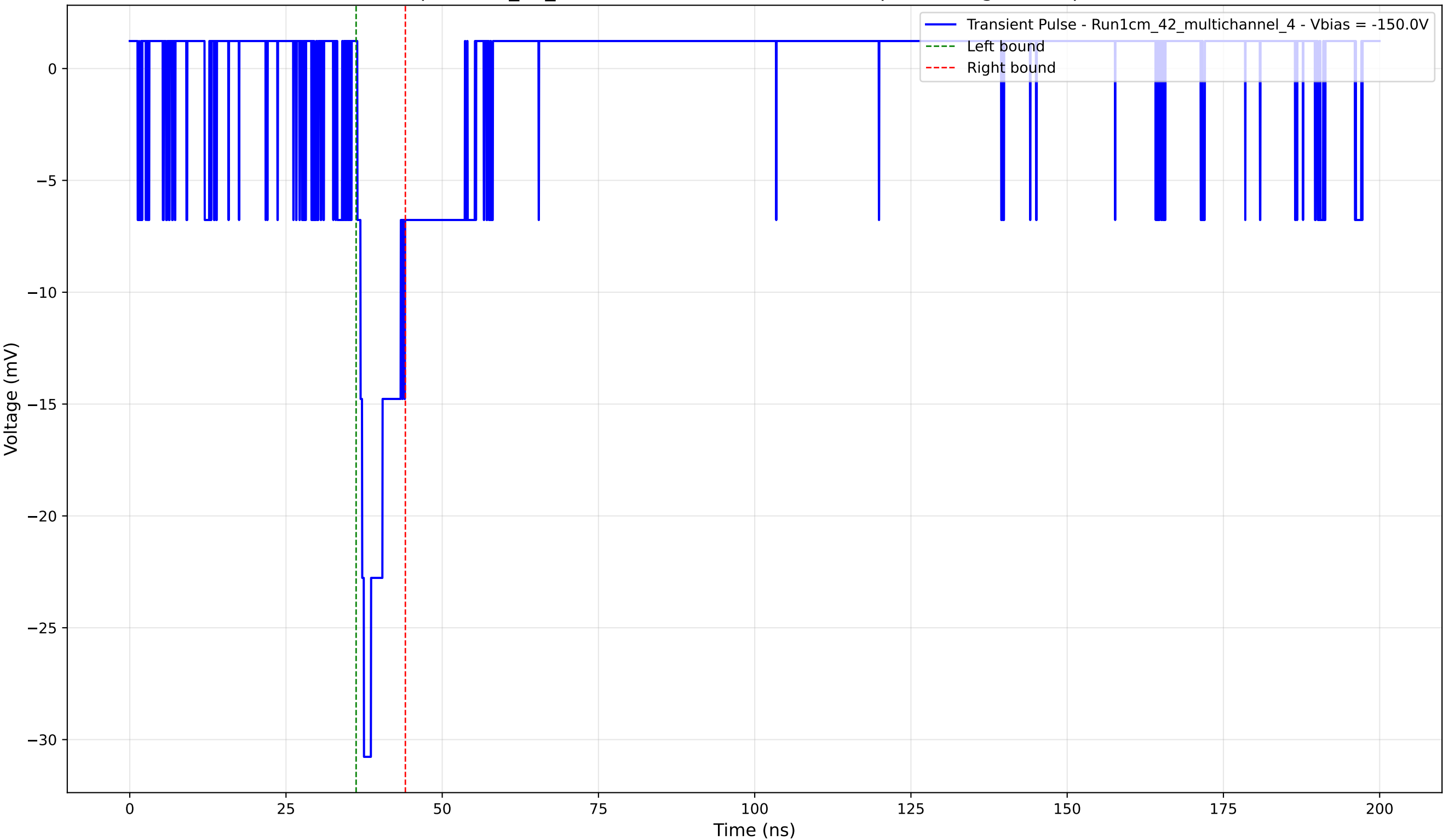
Transient Pulse - Sample: 1cm_42_multichannel - Position: 1520.0 \mu\text{m} - Charge: 2.80 pC - Rise Time: 1.05 ns
