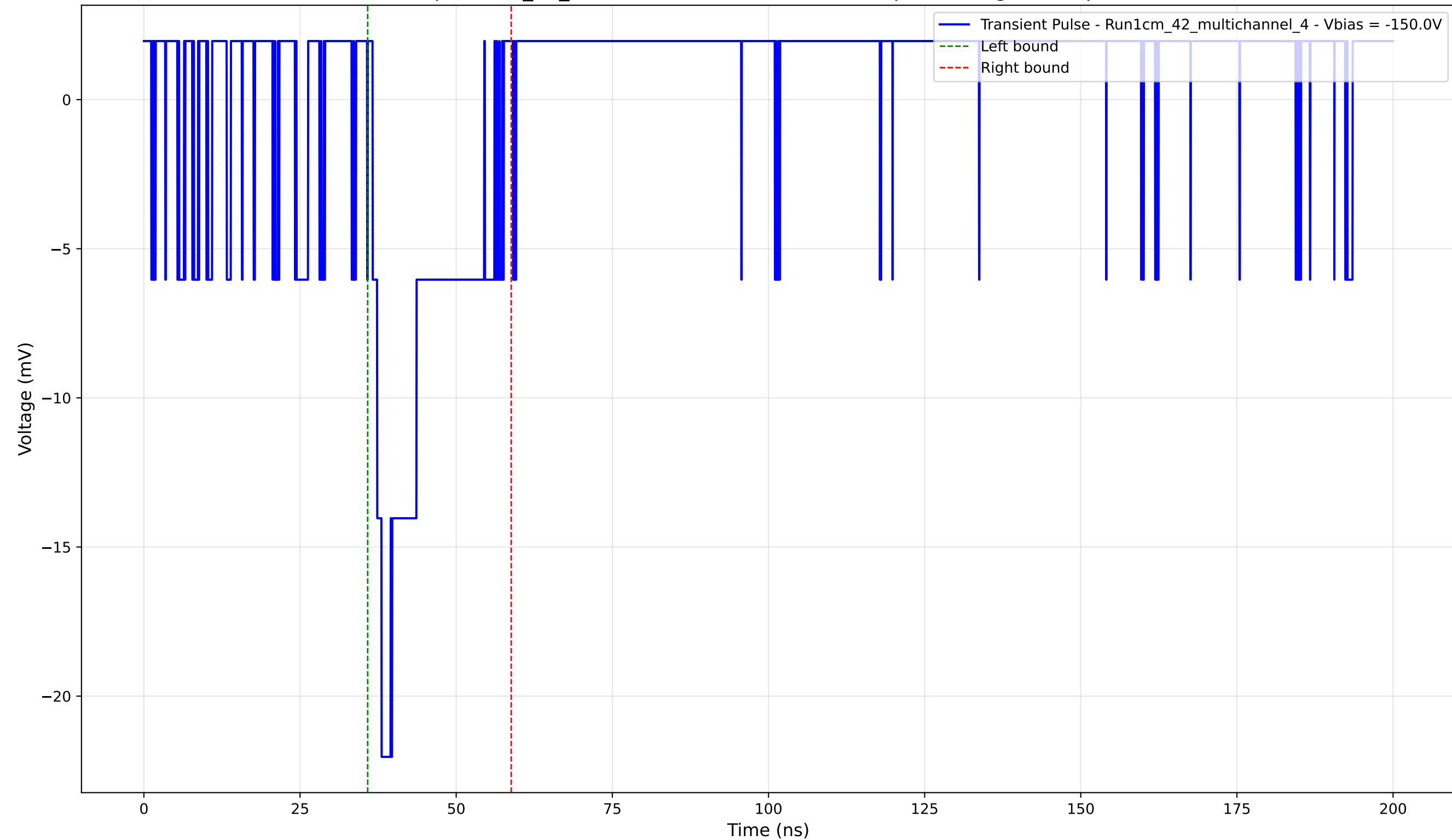
Transient Pulse - Sample: 1cm_42_multichannel - Position: 1130.0 \mu\text{m} - Charge: 3.64 pC - Rise Time: 1.44 ns
