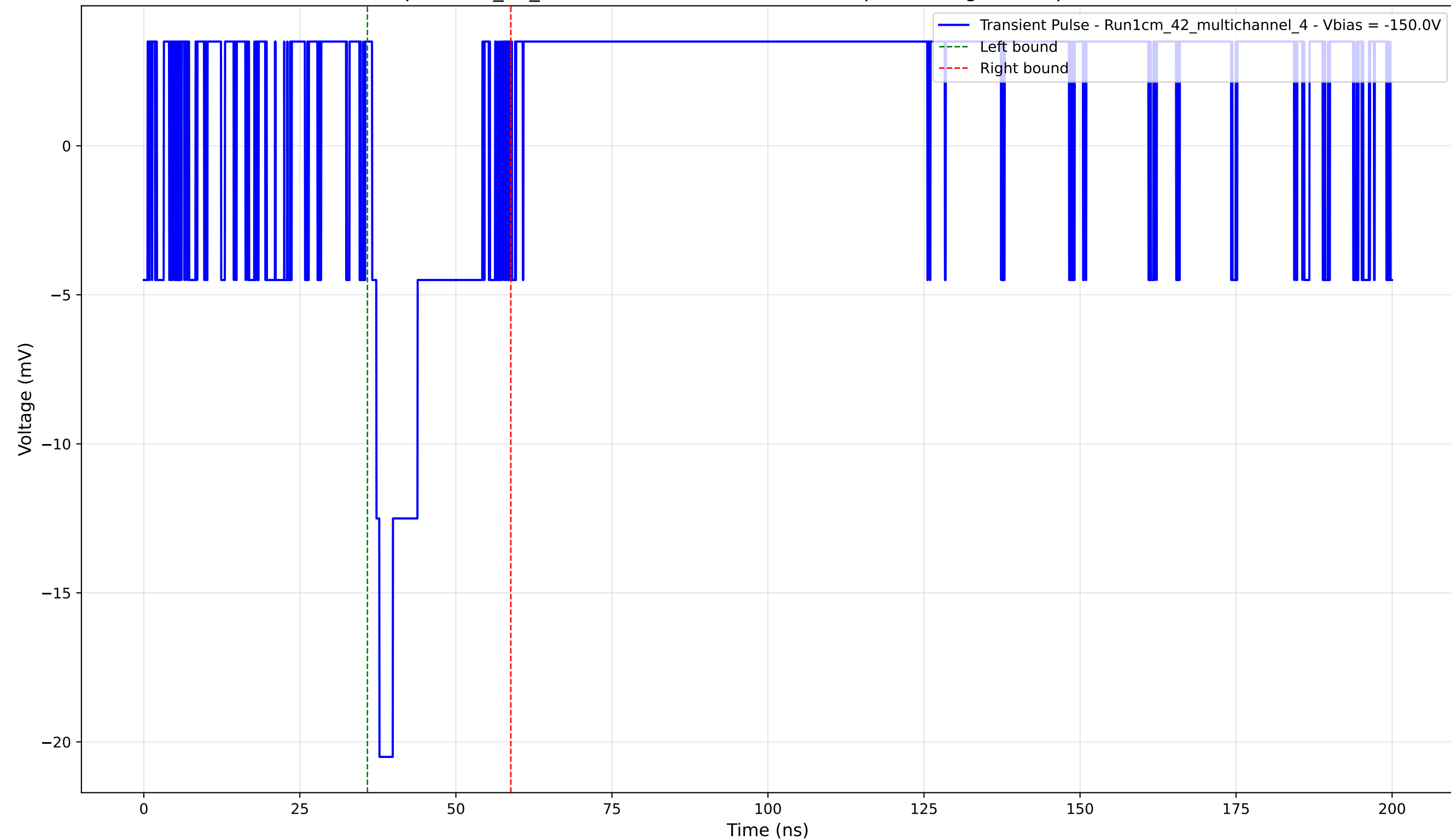
Transient Pulse - Sample: 1cm_42_multichannel - Position: 1195.0 \mu\text{m} - Charge: 2.98 pC - Rise Time: 0.00 ns (N/A)
