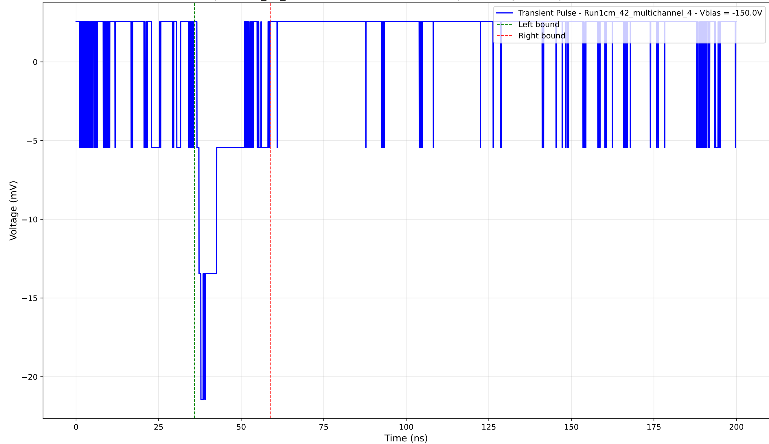
Transient Pulse - Sample: 1cm_42_multichannel - Position: 1310.0 \mu\text{m} - Charge: 2.92 pC - Rise Time: 0.00 ns (N/A)
