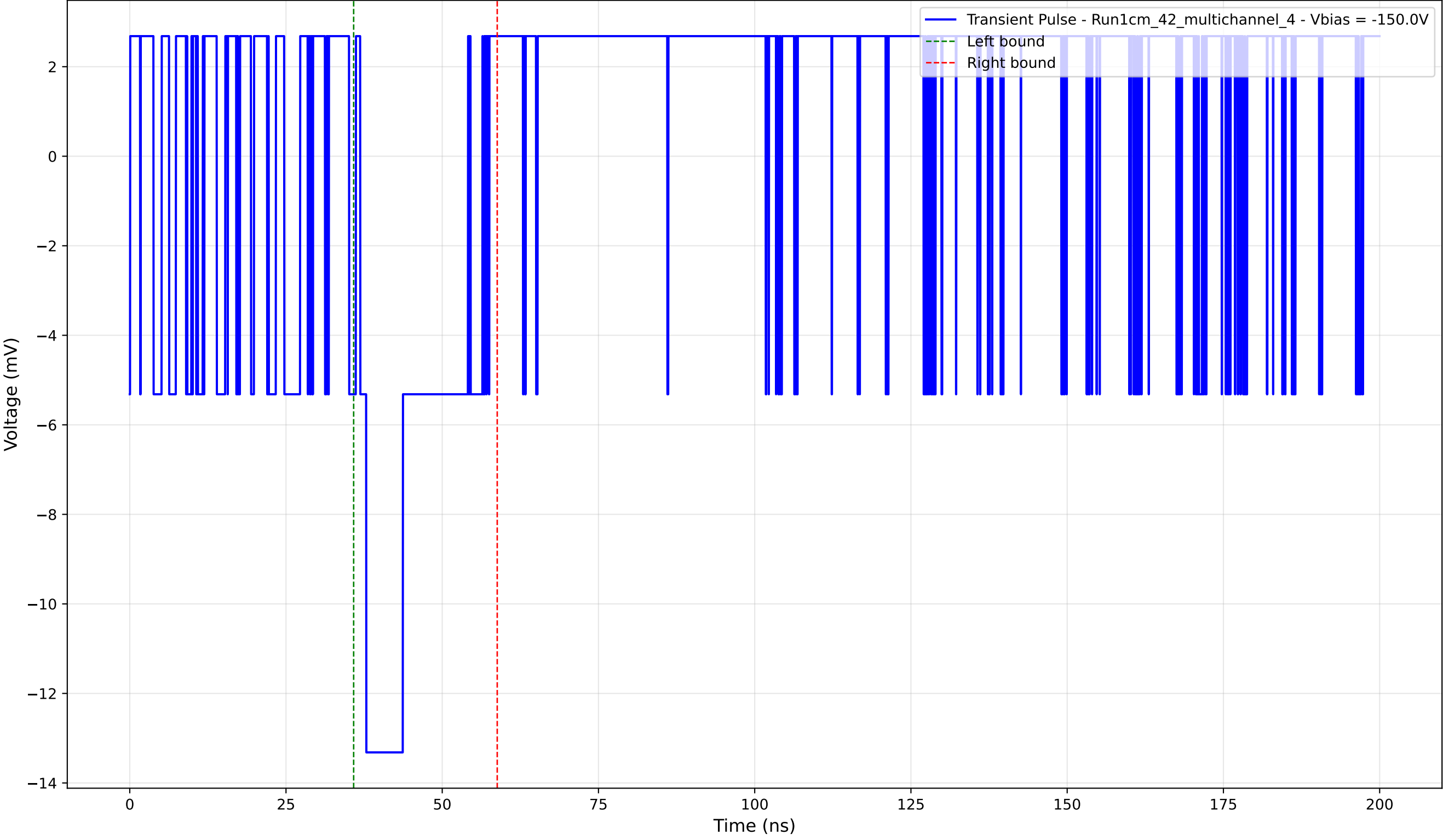
Transient Pulse - Sample: 1cm_42_multichannel - Position: 705.0 \mu\text{m} - Charge: 2.92 pC - Rise Time: 0.00 ns (N/A)
