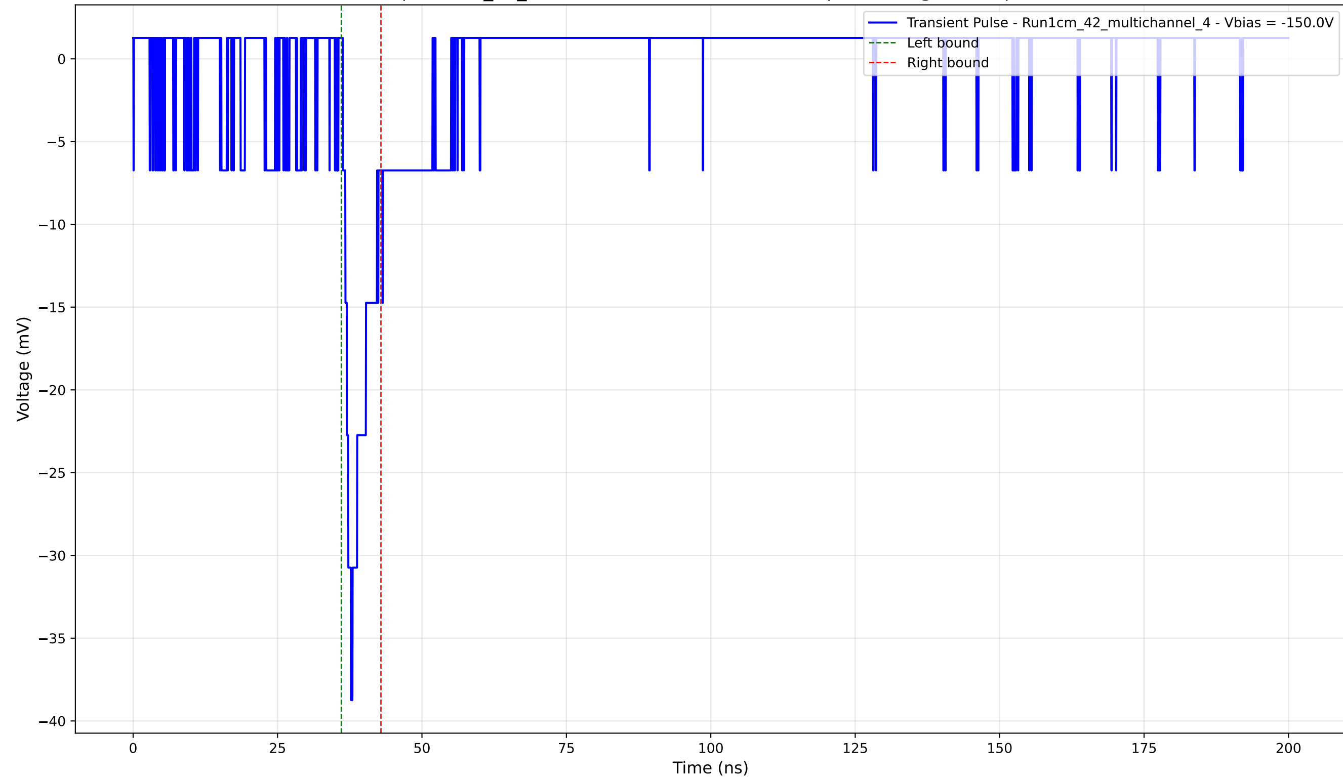
Transient Pulse - Sample: 1cm_42_multichannel - Position: 1645.0 \mu\text{m} - Charge: 2.59 pC - Rise Time: 1.39 ns
