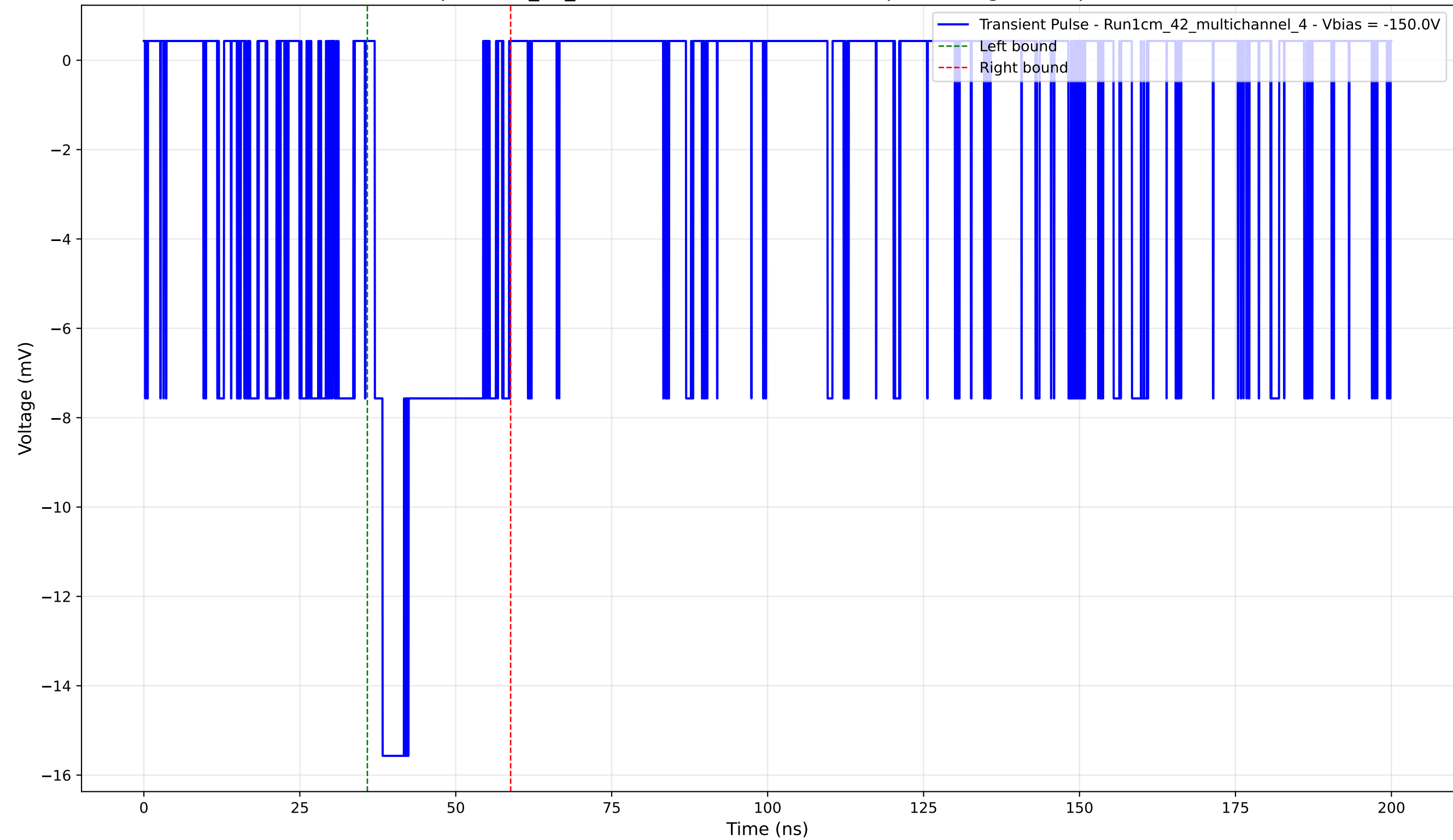
Transient Pulse - Sample: 1cm_42_multichannel - Position: 180.0 \mu\text{m} - Charge: 3.62 pC - Rise Time: 1.26 ns
