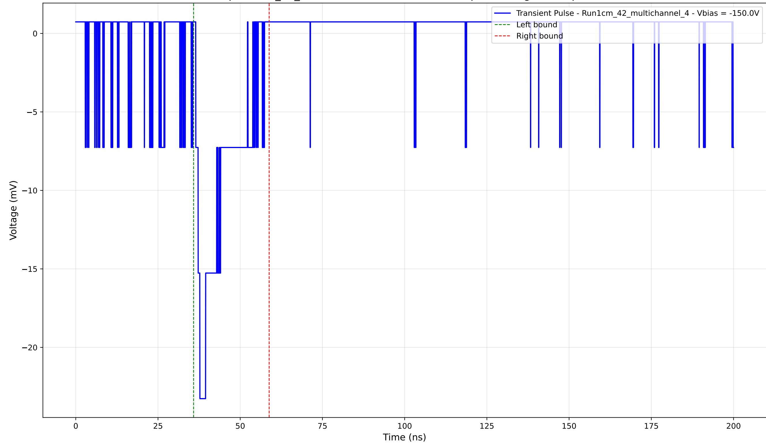
Transient Pulse - Sample: 1cm_42_multichannel - Position: 3495.0 \mu\text{m} - Charge: 3.92 pC - Rise Time: 1.26 ns
