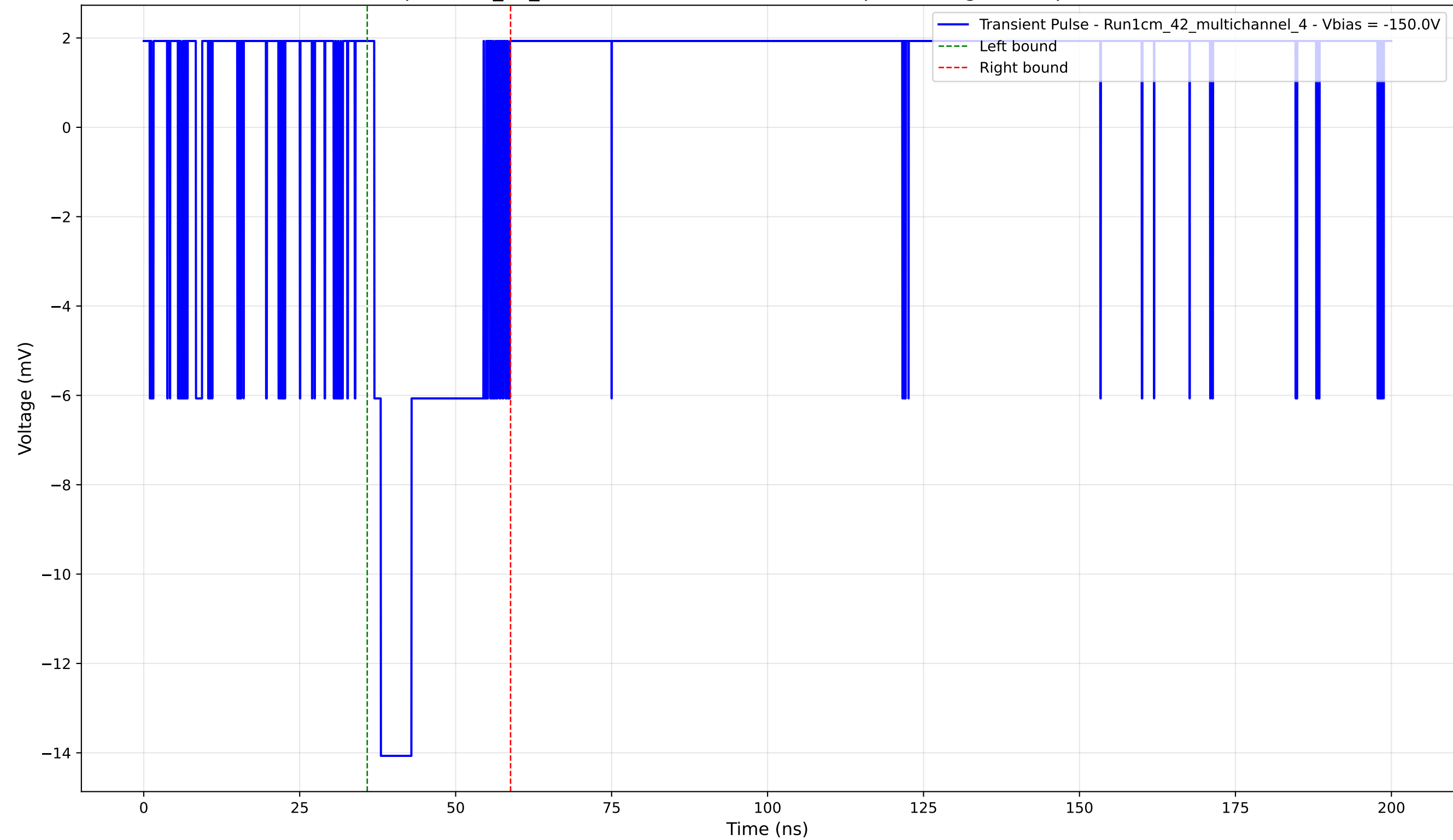
Transient Pulse - Sample: 1cm_42_multichannel - Position: 3975.0 \mu\text{m} - Charge: 3.05 pC - Rise Time: 0.00 ns (N/A)
