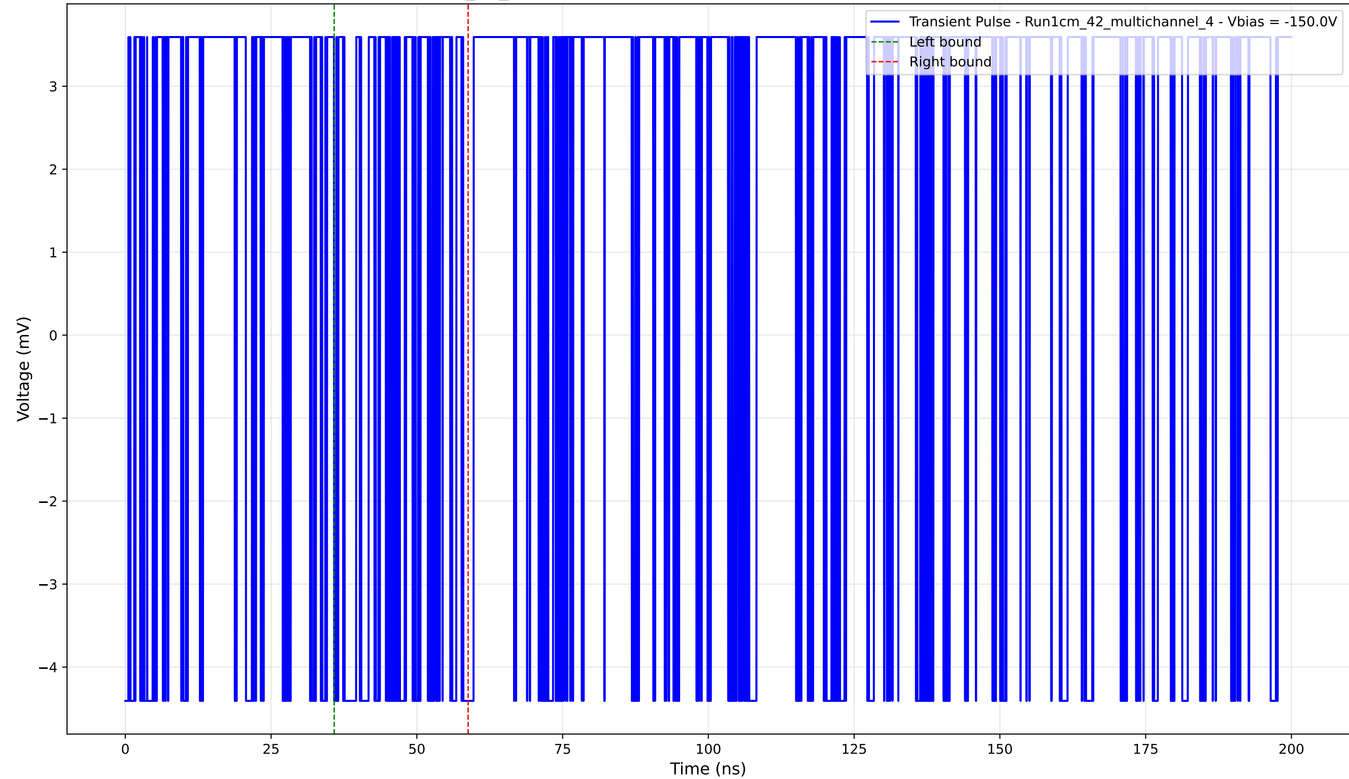
Transient Pulse - Sample: 1cm_42_multichannel - Position: 70.0 \mu\text{m} - Charge: 0.06 pC - Rise Time: 0.00 ns (N/A)
