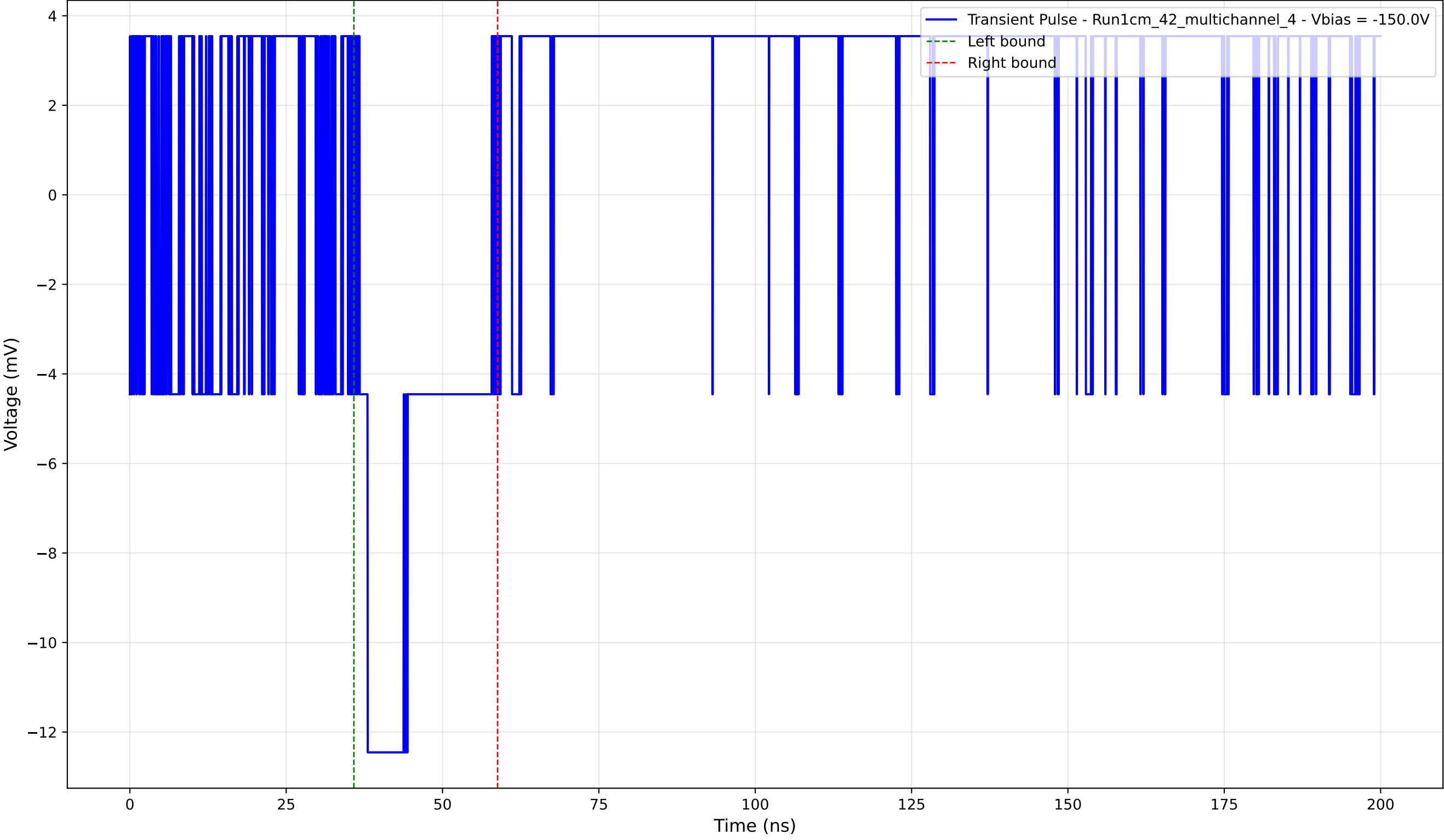
Transient Pulse - Sample: 1cm_42_multichannel - Position: 575.0 \mu\text{m} - Charge: 2.82 pC - Rise Time: 0.00 ns (N/A)
