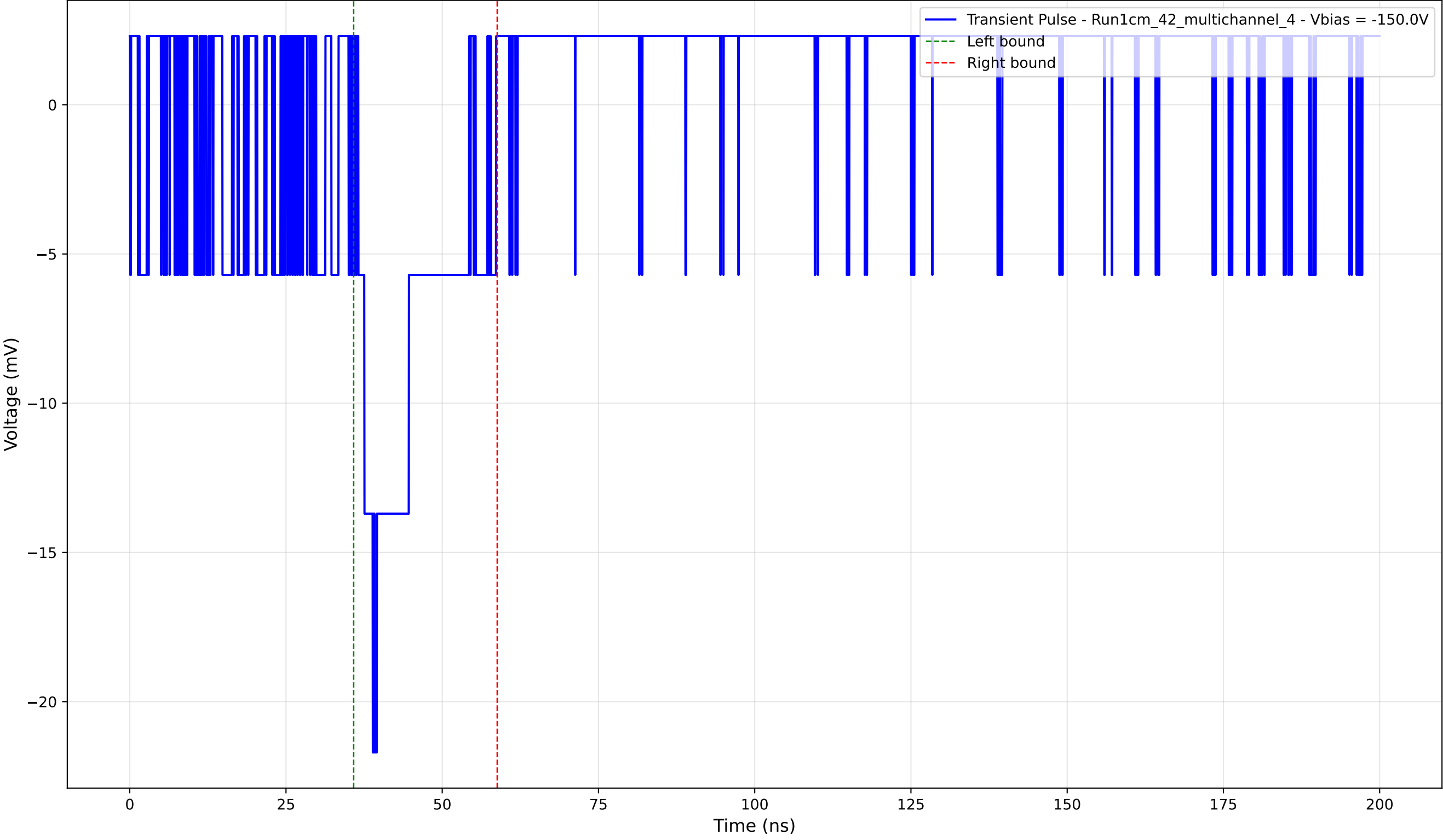
Transient Pulse - Sample: 1cm_42_multichannel - Position: 950.0 \mu\text{m} - Charge: 3.57 pC - Rise Time: 0.00 ns (N/A)
