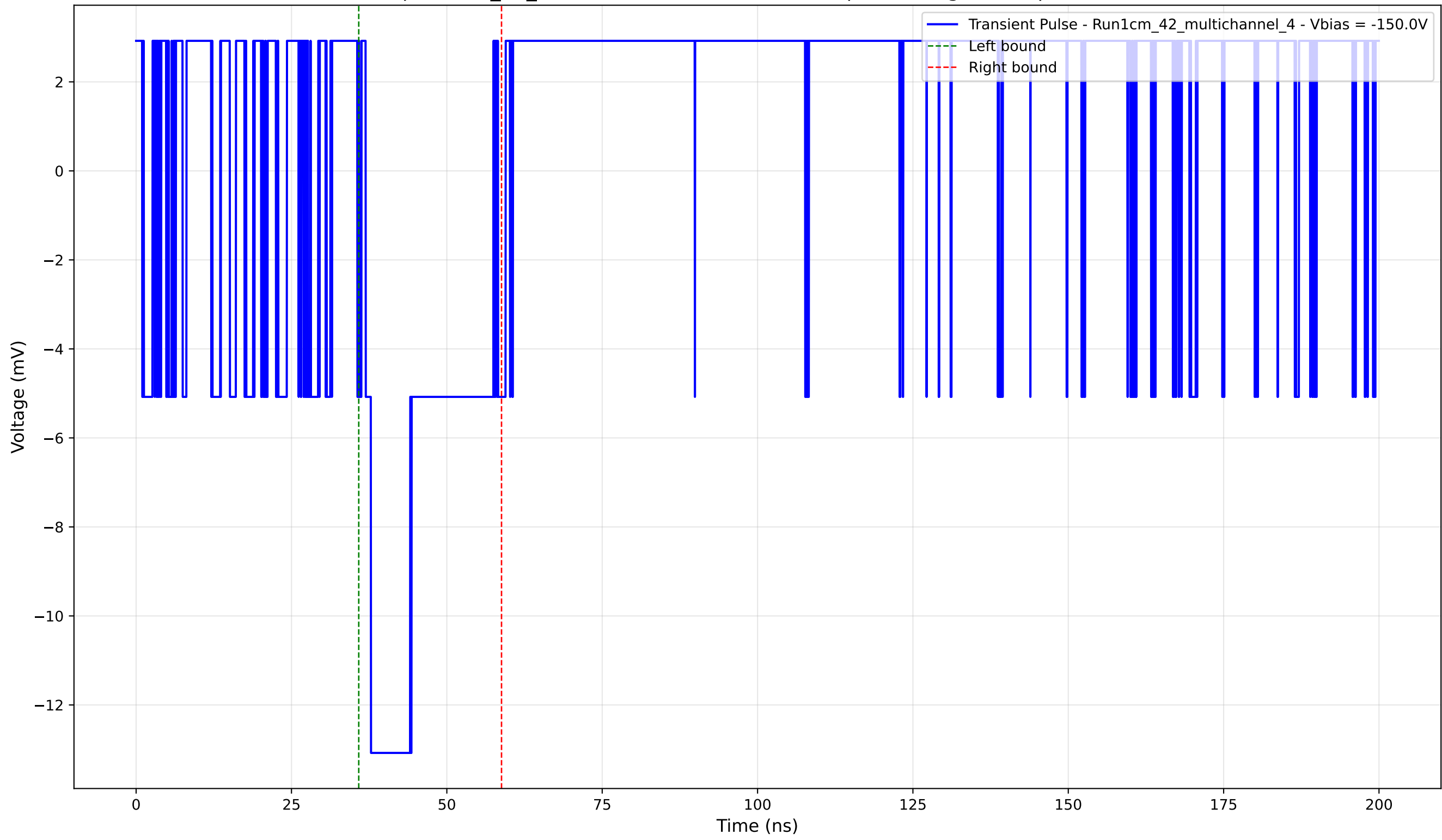
Transient Pulse - Sample: 1cm_42_multichannel - Position: 730.0 \mu\text{m} - Charge: 3.16 pC - Rise Time: 0.00 ns (N/A)
