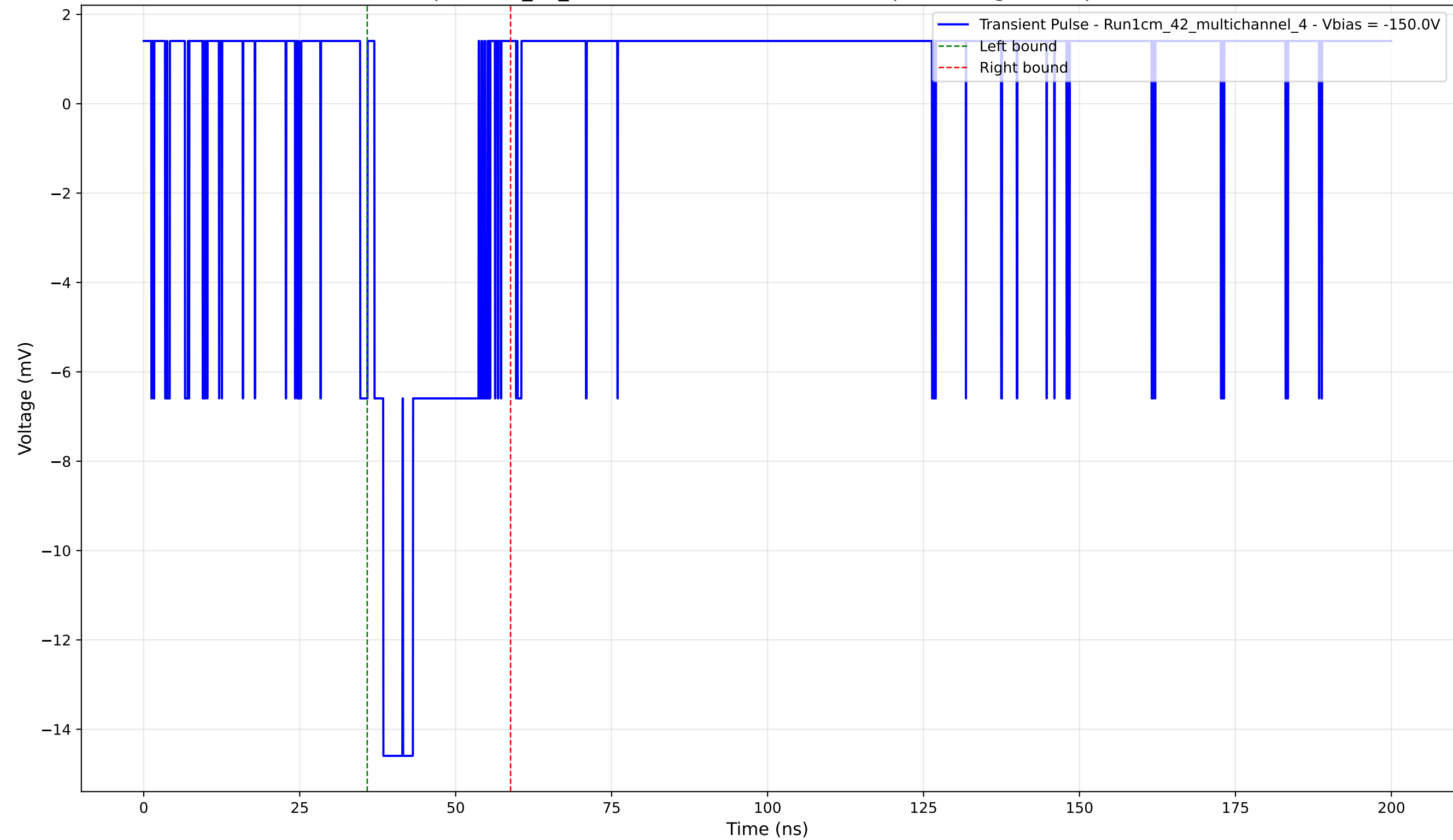
Transient Pulse - Sample: 1cm_42_multichannel - Position: 4155.0 \mu\text{m} - Charge: 3.01 pC - Rise Time: 1.44 ns
