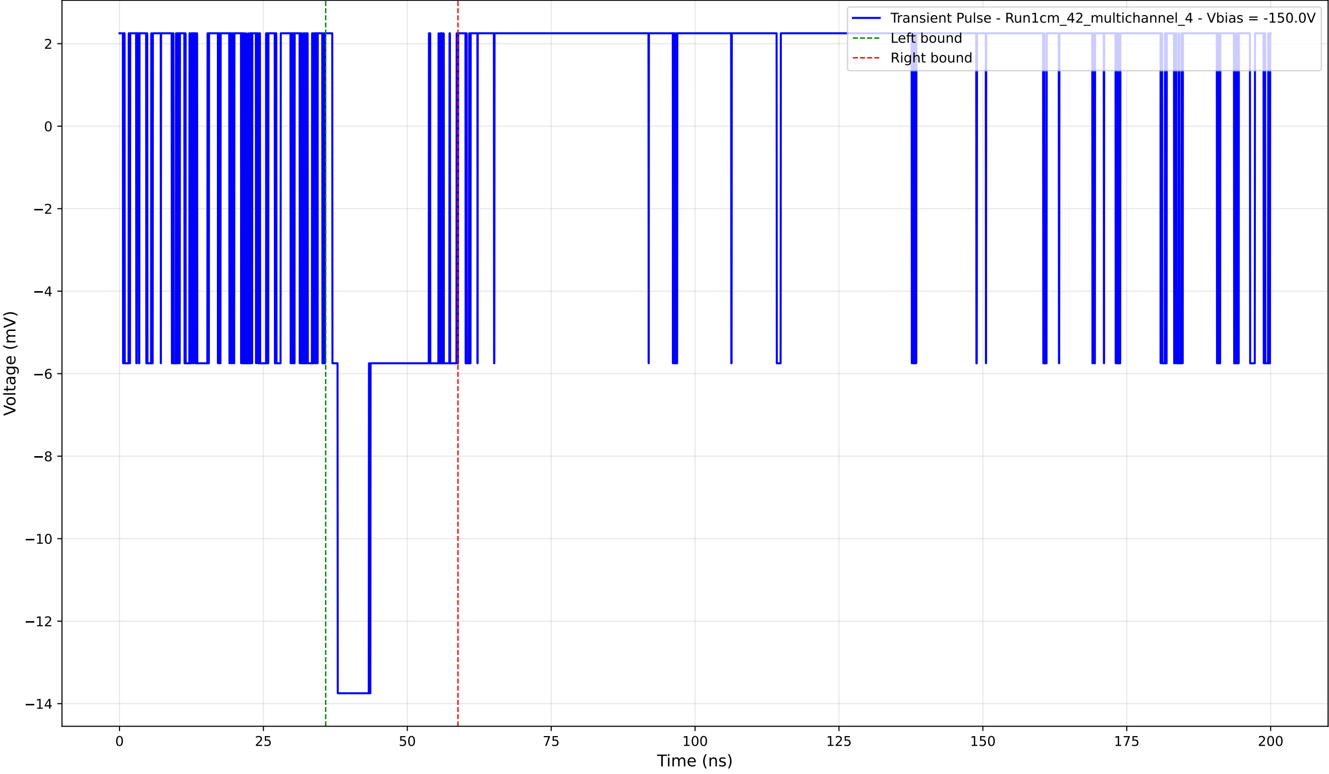
Transient Pulse - Sample: 1cm_42_multichannel - Position: 615.0 \mu\text{m} - Charge: 3.23 pC - Rise Time: 0.00 ns (N/A)
