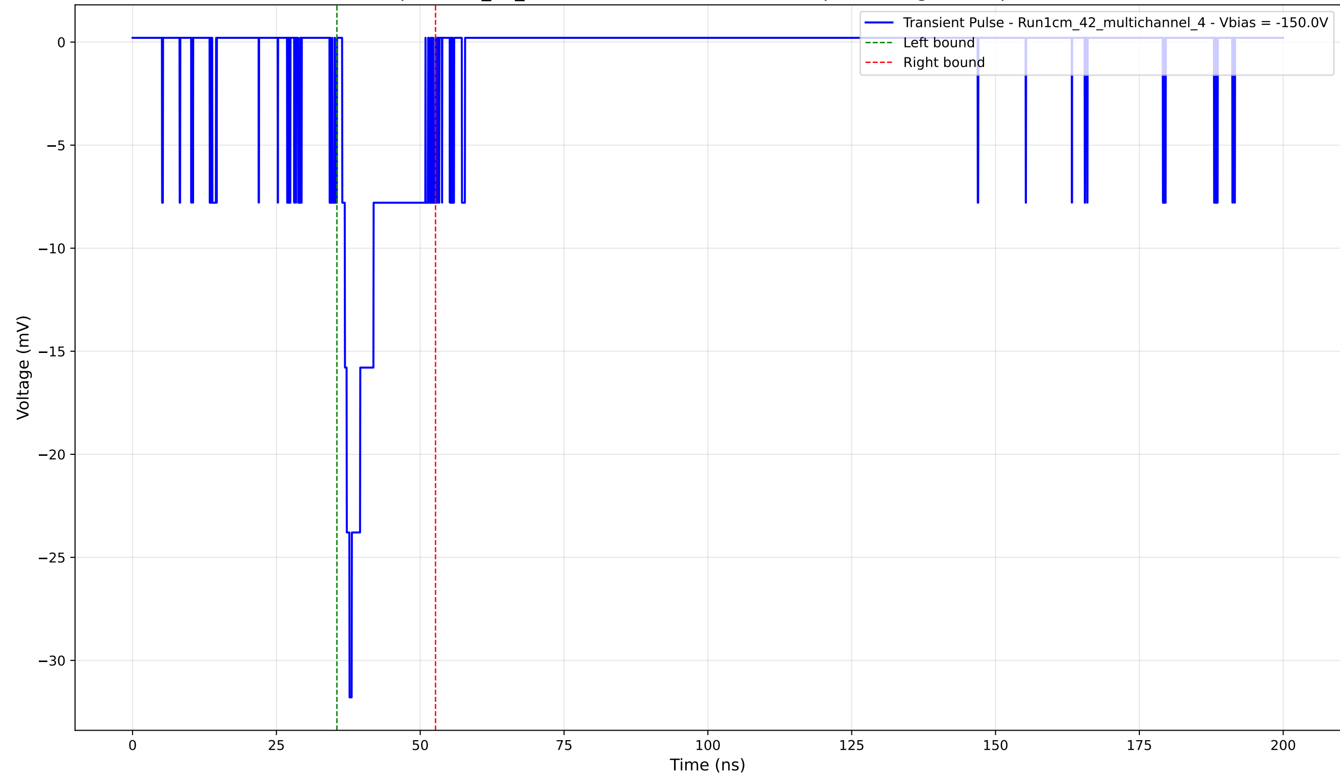
Transient Pulse - Sample: 1cm_42_multichannel - Position: 3175.0 \mu\text{m} - Charge: 3.68 pC - Rise Time: 1.27 ns
