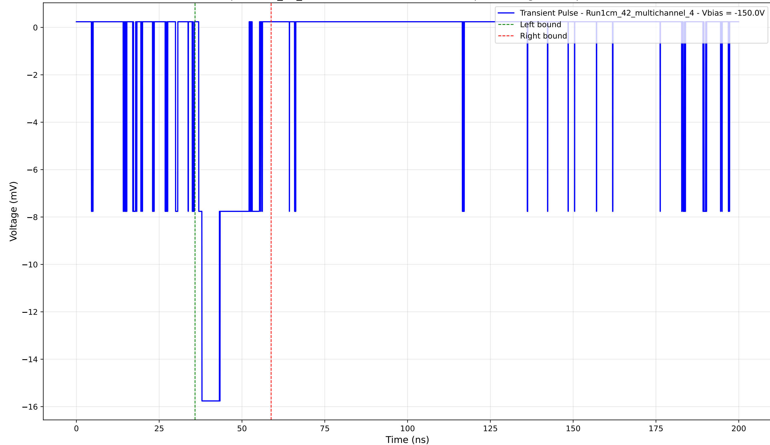
Transient Pulse - Sample: 1cm_42_multichannel - Position: 3990.0 \mu\text{m} - Charge: 3.65 pC - Rise Time: 0.98 ns
