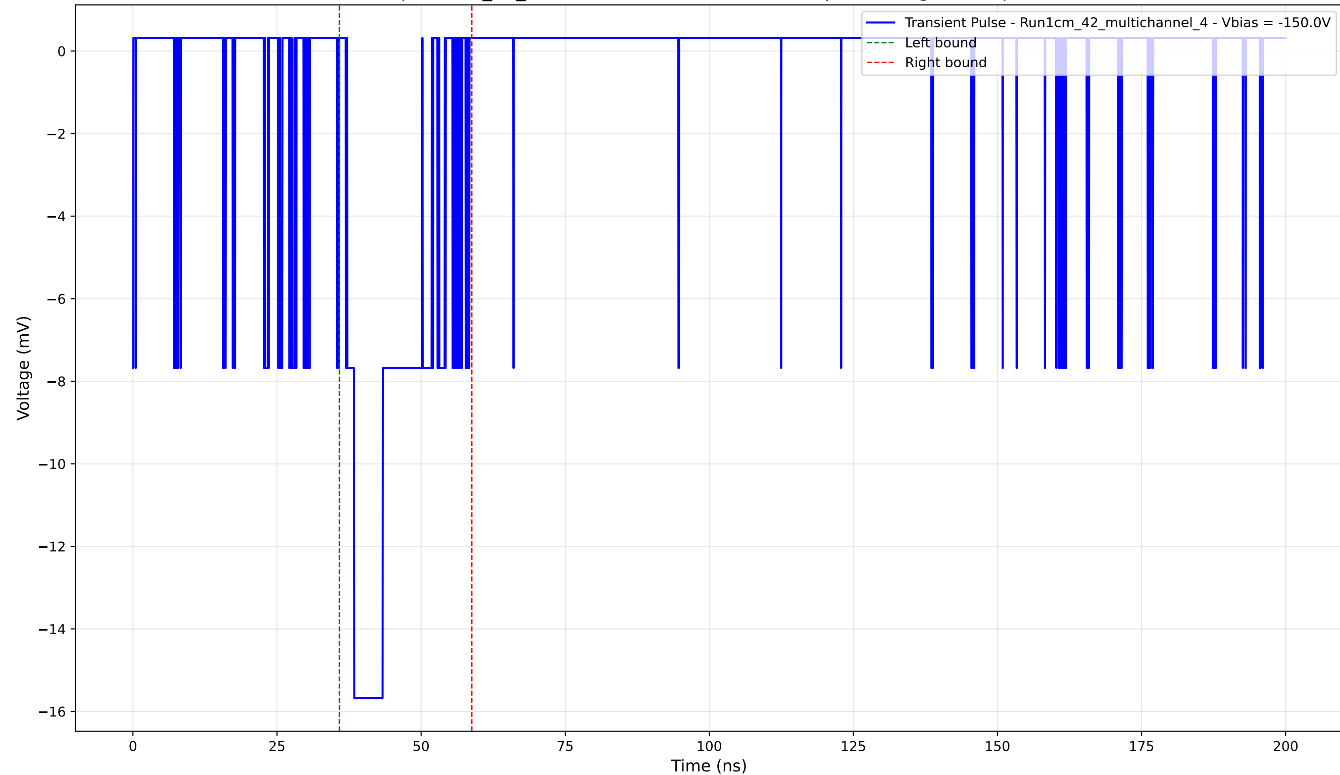
Transient Pulse - Sample: 1cm_42_multichannel - Position: 4535.0 \mu\text{m} - Charge: 3.41 pC - Rise Time: 1.22 ns
