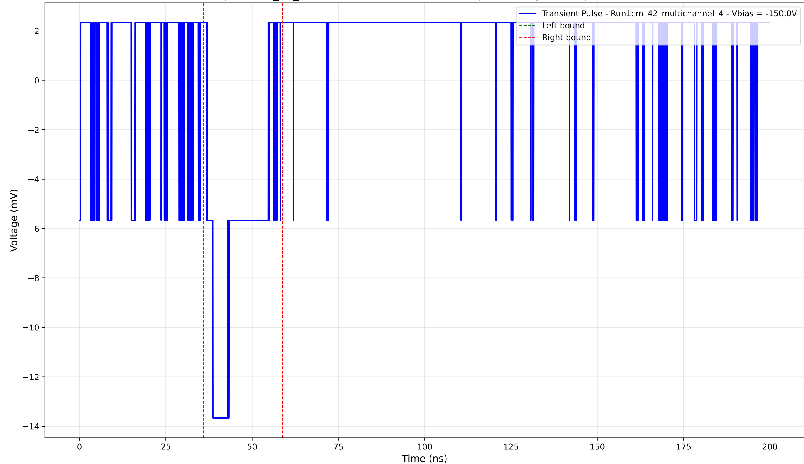
Transient Pulse - Sample: 1cm_42_multichannel - Position: 4510.0 \mu\text{m} - Charge: 2.60 pC - Rise Time: 0.00 ns (N/A)
