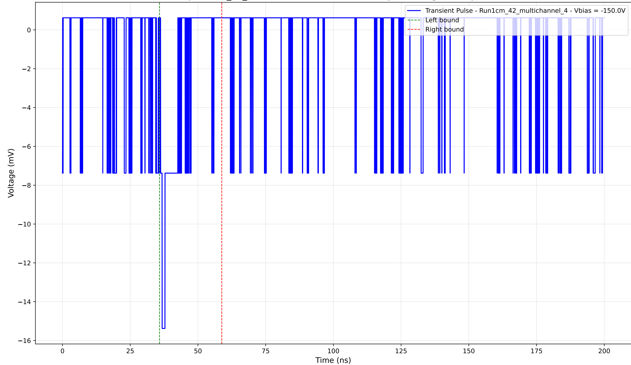
Transient Pulse - Sample: 1cm_42_multichannel - Position: 2350.0 \mu\text{m} - Charge: 1.25 pC - Rise Time: 0.58 ns
