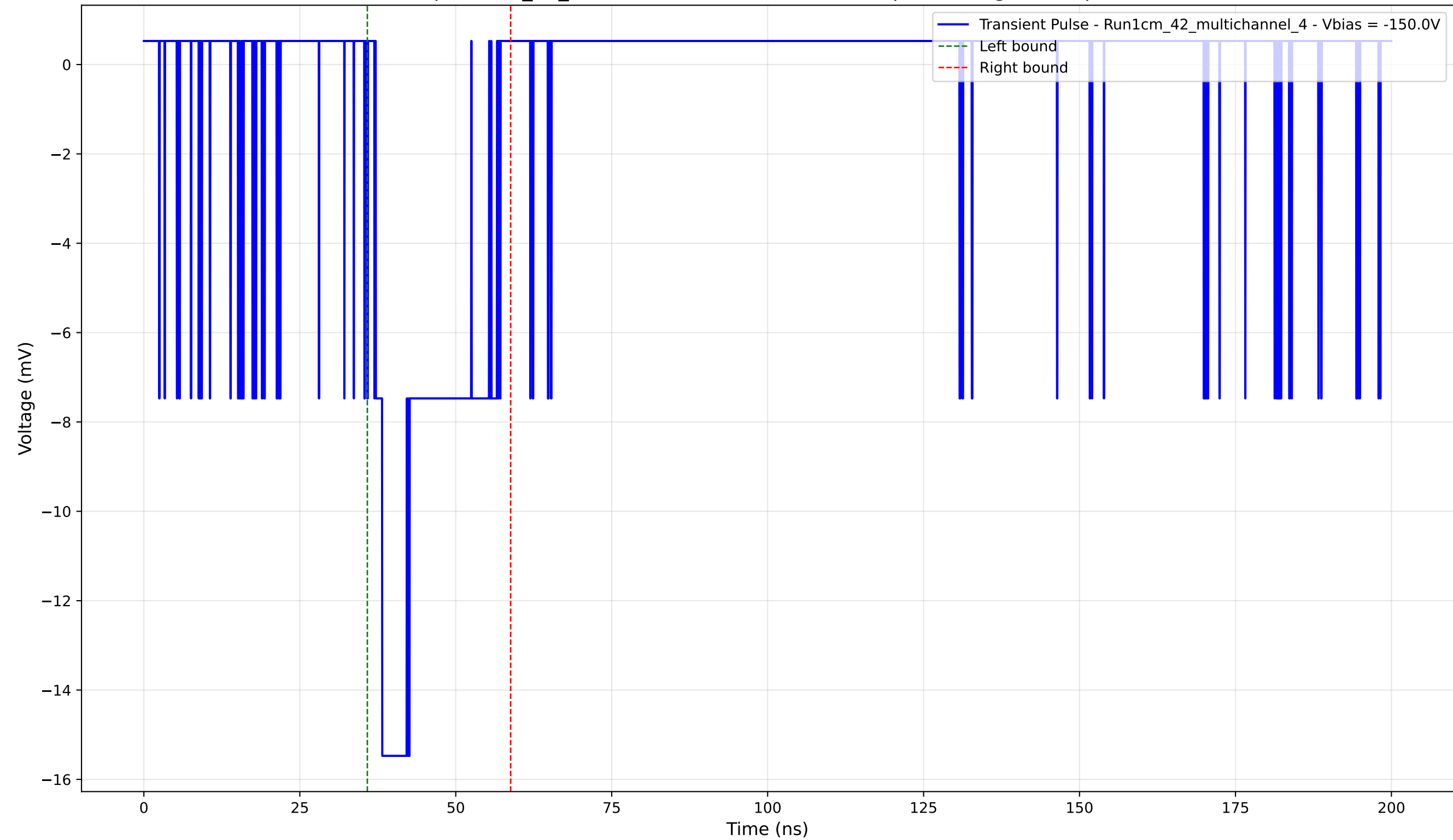
Transient Pulse - Sample: 1cm_42_multichannel - Position: 4105.0 \mu\text{m} - Charge: 3.56 pC - Rise Time: 1.04 ns
