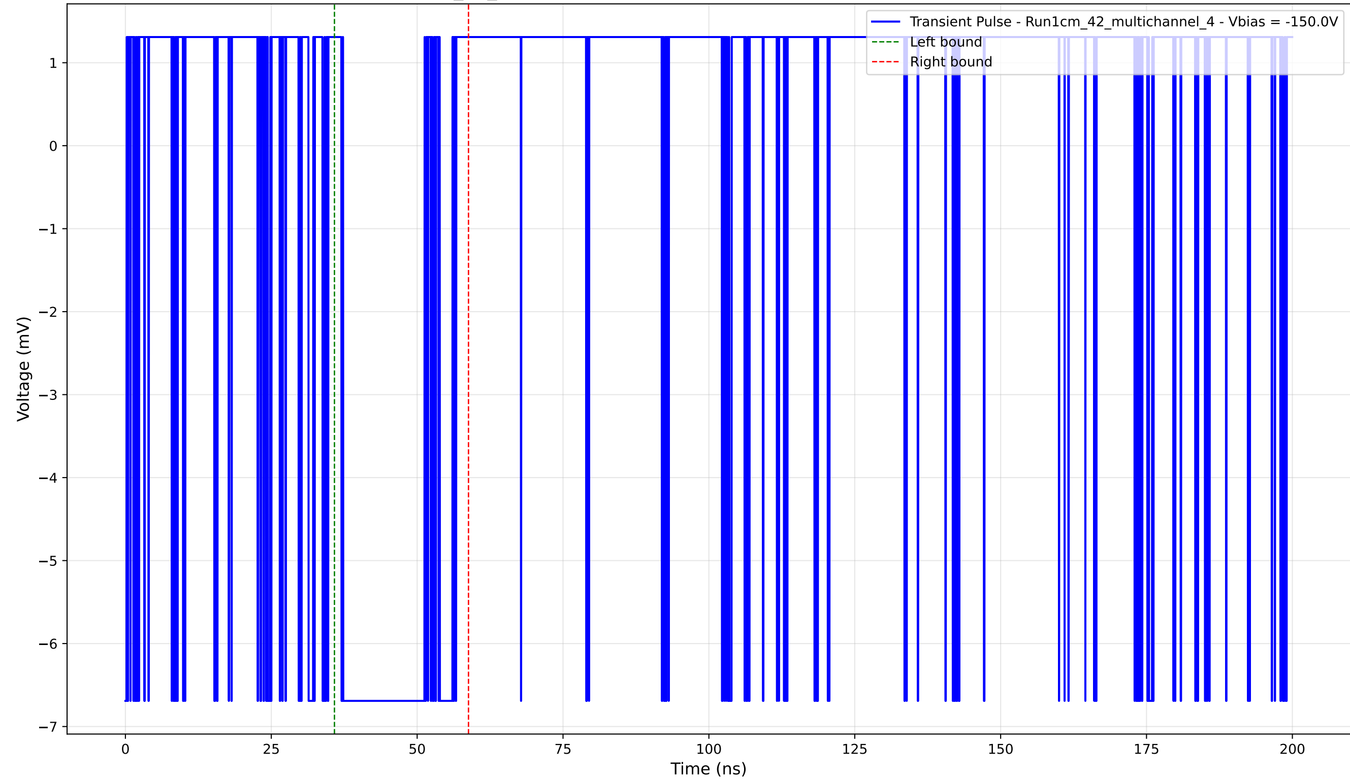
Transient Pulse - Sample: 1cm_42_multichannel - Position: 4455.0 \mu\text{m} - Charge: 2.19 pC - Rise Time: 0.00 ns (N/A)
