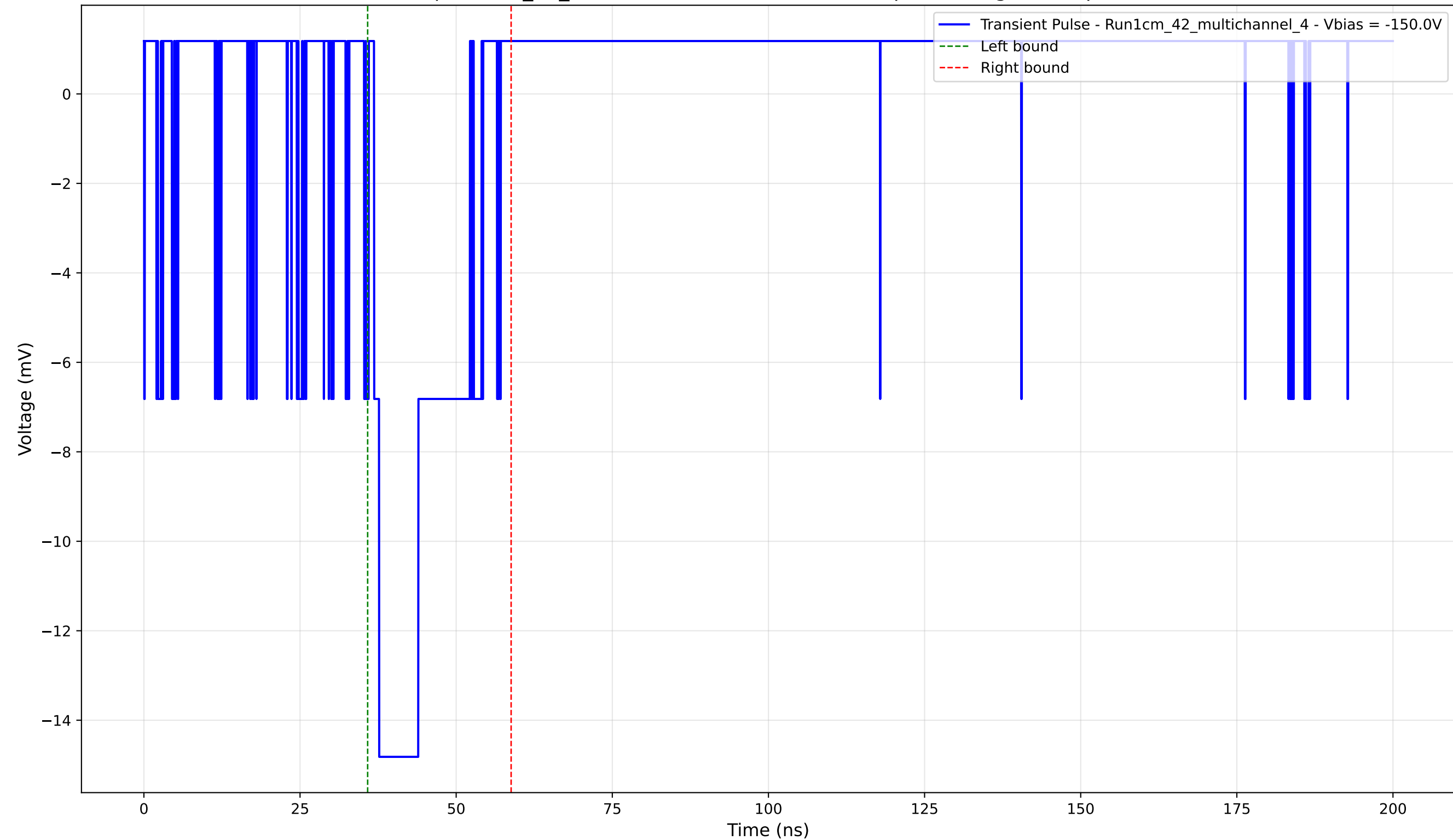
Transient Pulse - Sample: 1cm_42_multichannel - Position: 3800.0 \mu\text{m} - Charge: 3.26 pC - Rise Time: 0.82 ns
