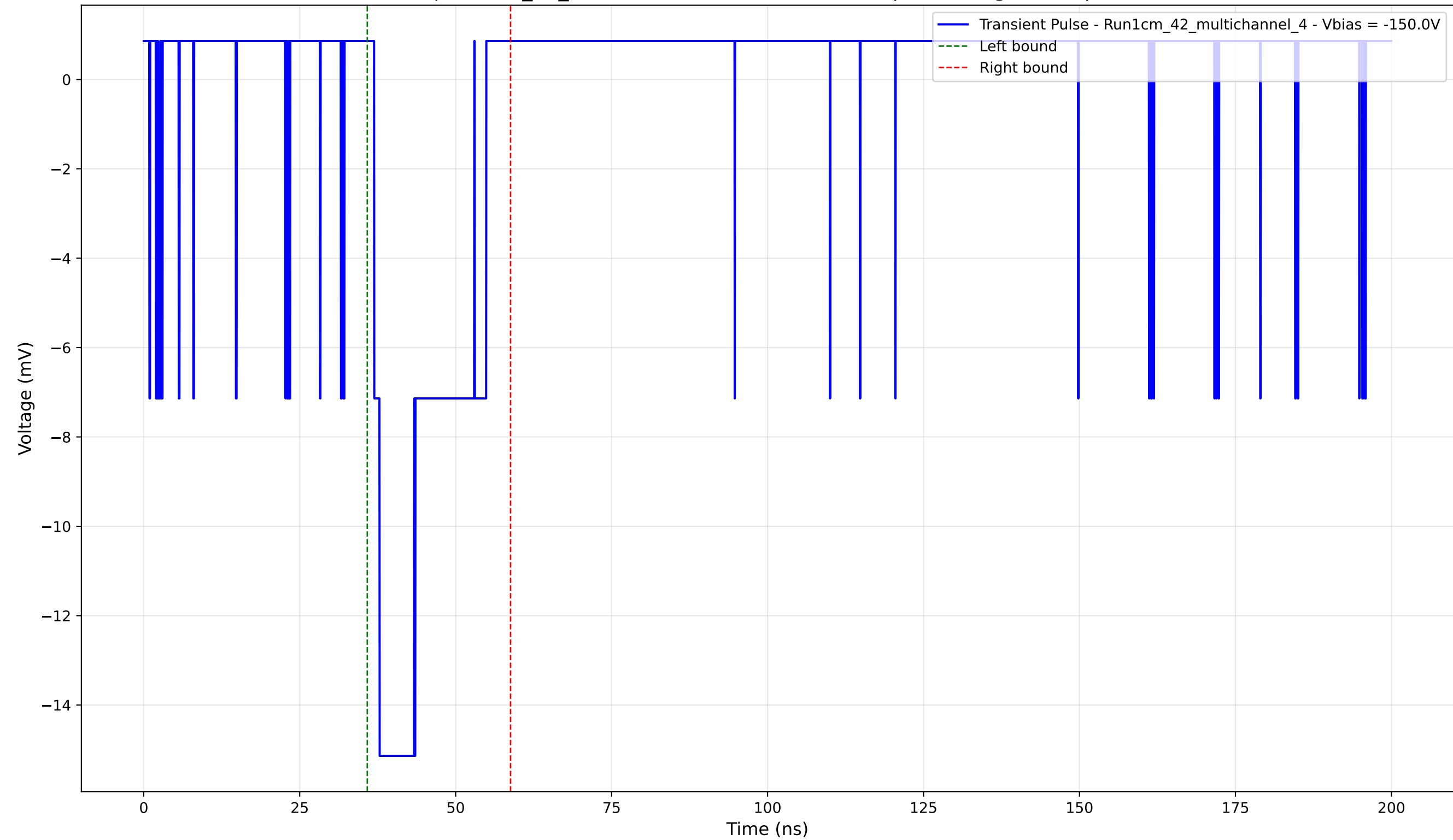
Transient Pulse - Sample: 1cm_42_multichannel - Position: 3820.0 \mu\text{m} - Charge: 3.38 pC - Rise Time: 0.88 ns
