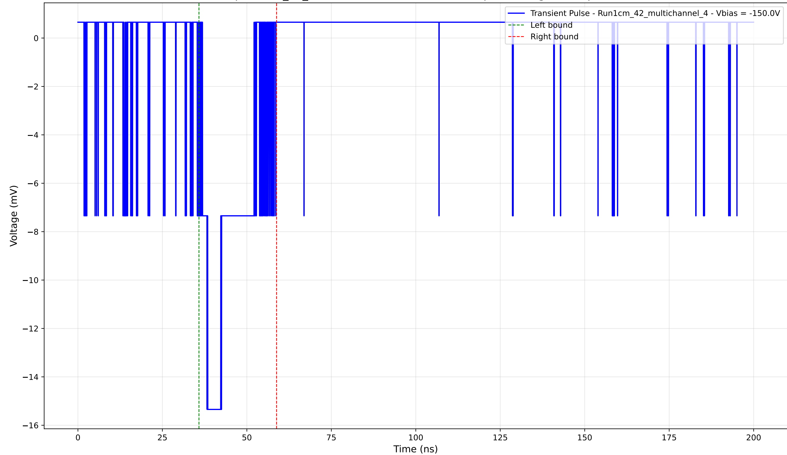
Transient Pulse - Sample: 1cm_42_multichannel - Position: 4160.0 \mu\text{m} - Charge: 3.21 pC - Rise Time: 1.36 ns
