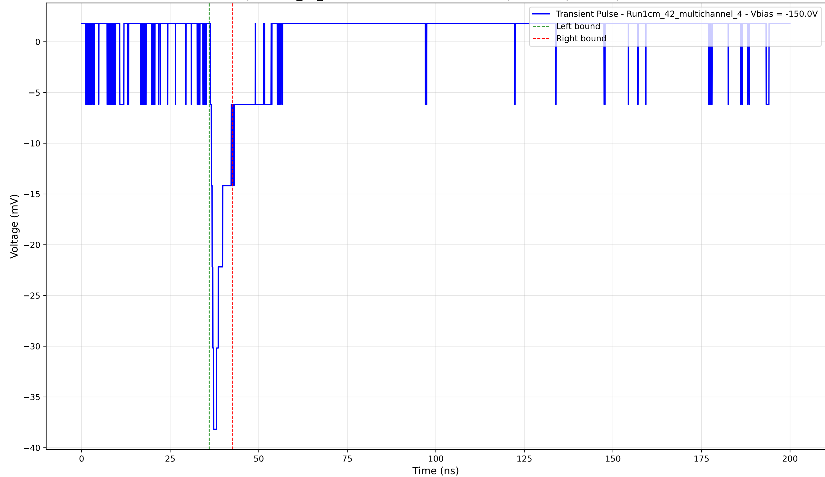
Transient Pulse - Sample: 1cm_42_multichannel - Position: 2985.0 \mu\text{m} - Charge: 2.54 pC - Rise Time: 0.95 ns
