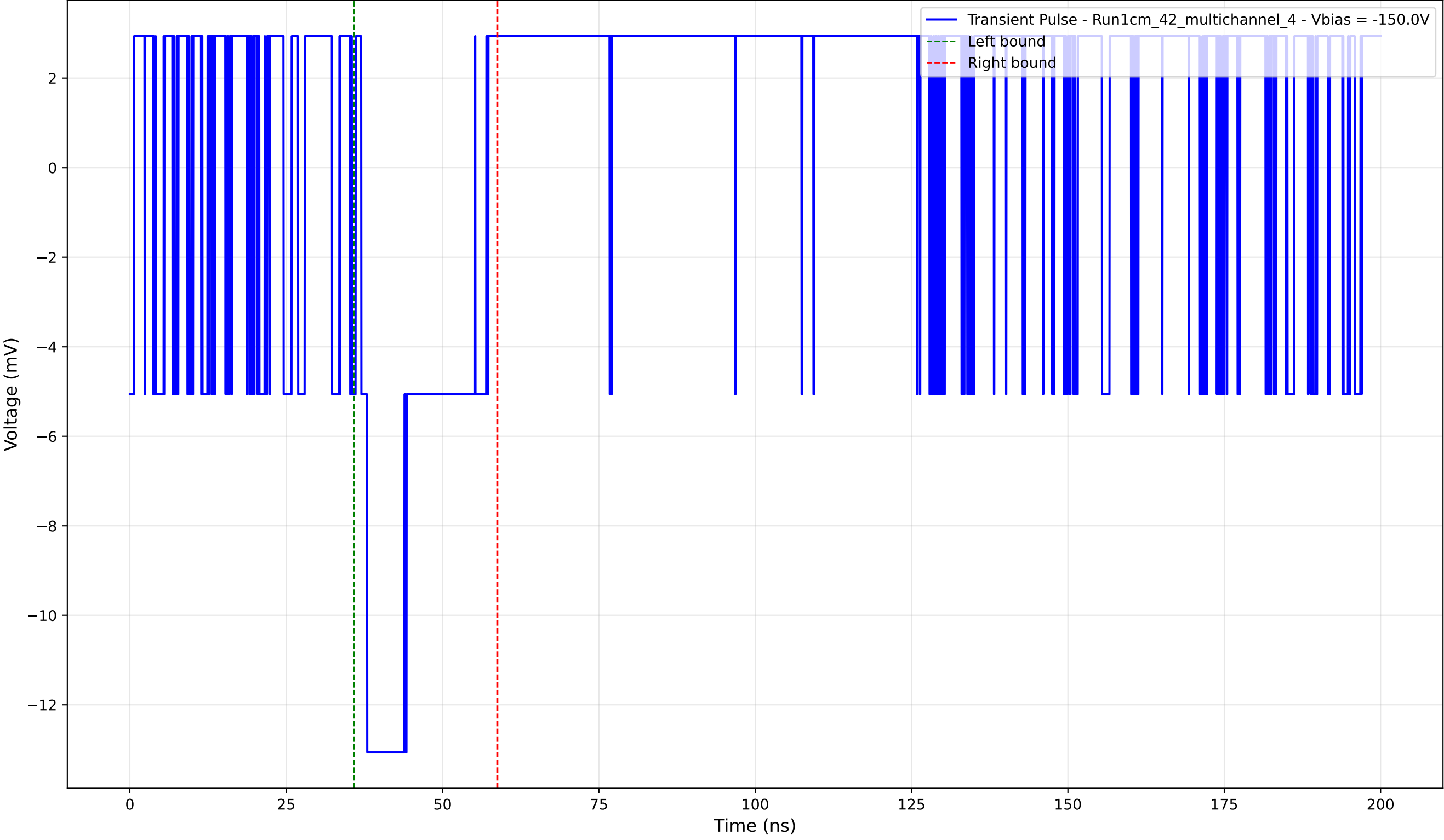
Transient Pulse - Sample: 1cm_42_multichannel - Position: 525.0 \mu\text{m} - Charge: 2.89 pC - Rise Time: 0.00 ns (N/A)
