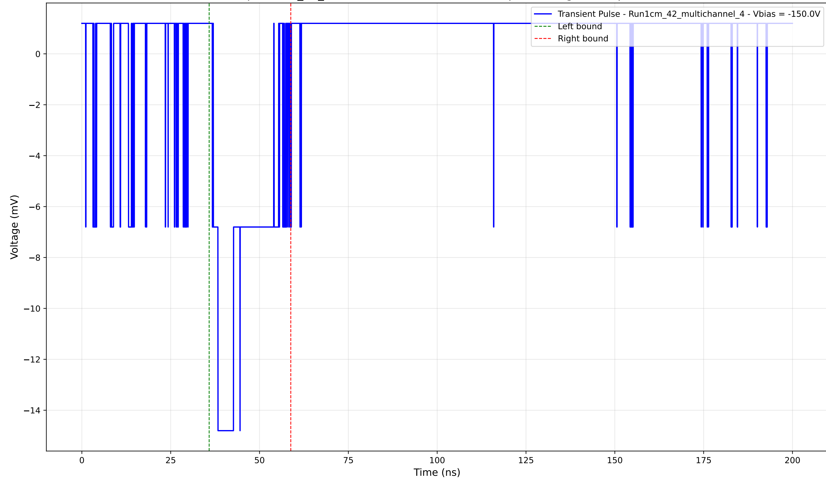
Transient Pulse - Sample: 1cm_42_multichannel - Position: 4210.0 \mu\text{m} - Charge: 3.29 pC - Rise Time: 1.32 ns
