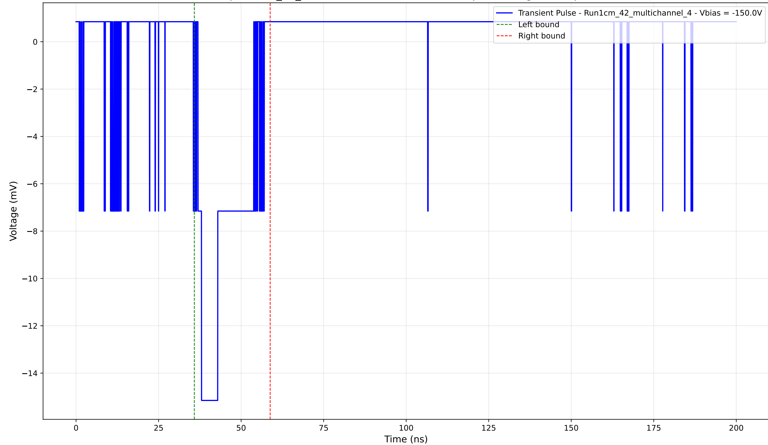
Transient Pulse - Sample: 1cm_42_multichannel - Position: 4065.0 \mu\text{m} - Charge: 3.40 pC - Rise Time: 1.08 ns
