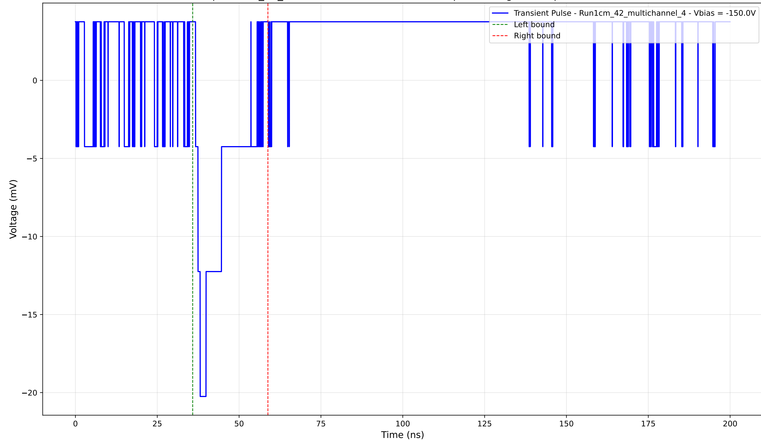
Transient Pulse - Sample: 1cm_42_multichannel - Position: 1030.0 \mu\text{m} - Charge: 2.85 pC - Rise Time: 0.00 ns (N/A)
