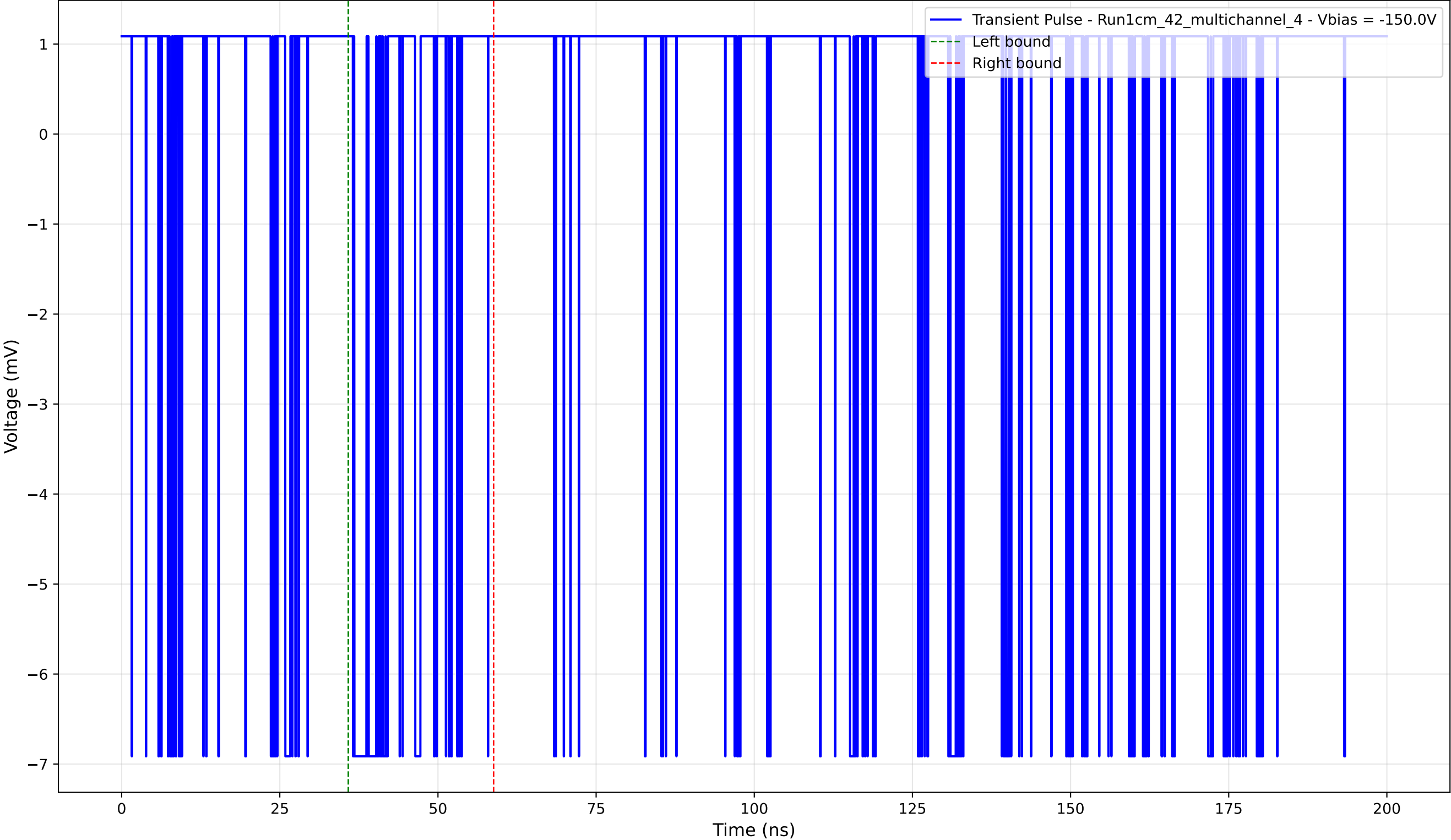
Transient Pulse - Sample: 1cm_42_multichannel - Position: 2915.0 \mu\text{m} - Charge: 0.55 pC - Rise Time: 0.00 ns (N/A)
