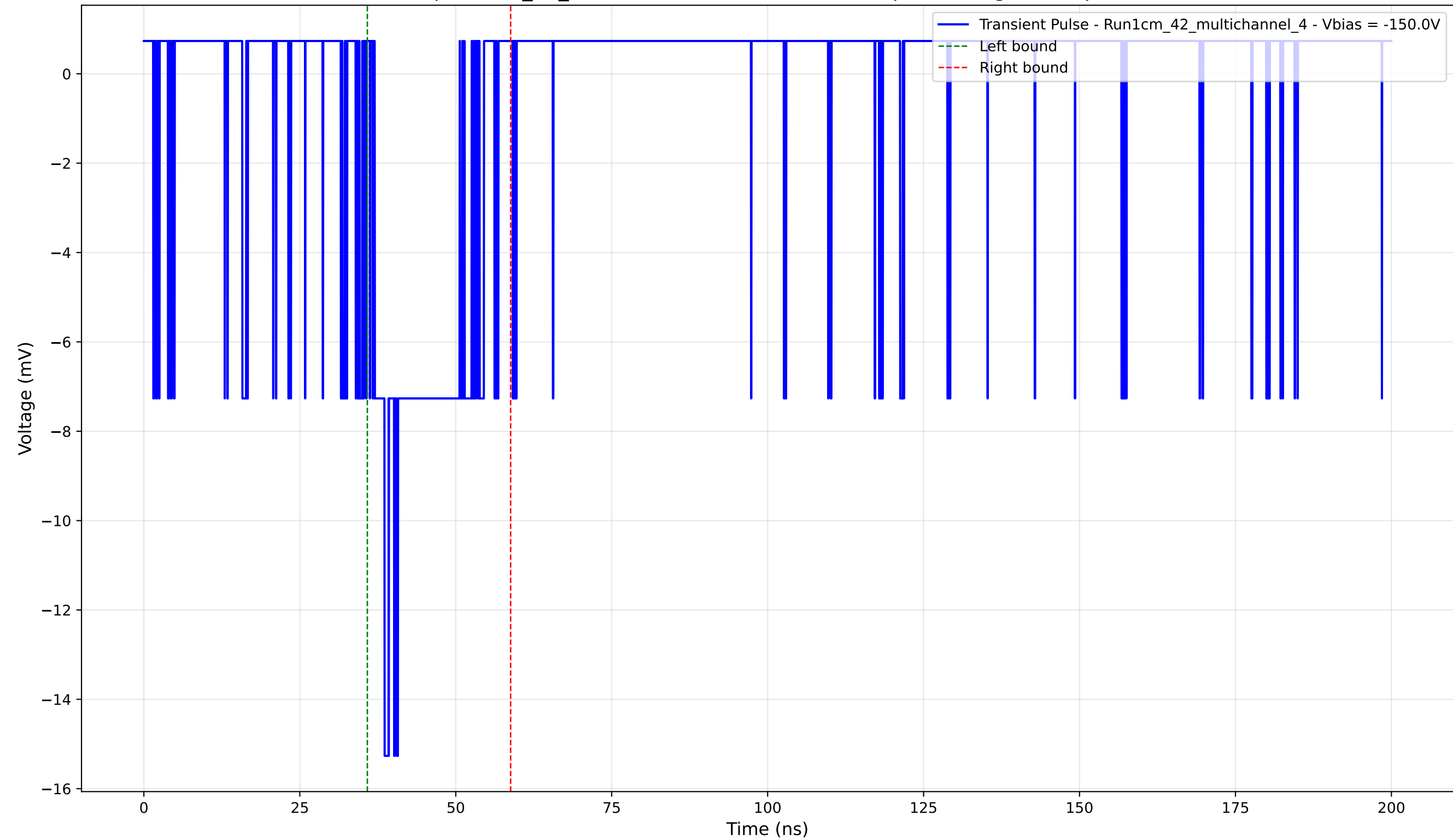
Transient Pulse - Sample: 1cm_42_multichannel - Position: 4825.0 \mu\text{m} - Charge: 2.57 pC - Rise Time: 1.58 ns
