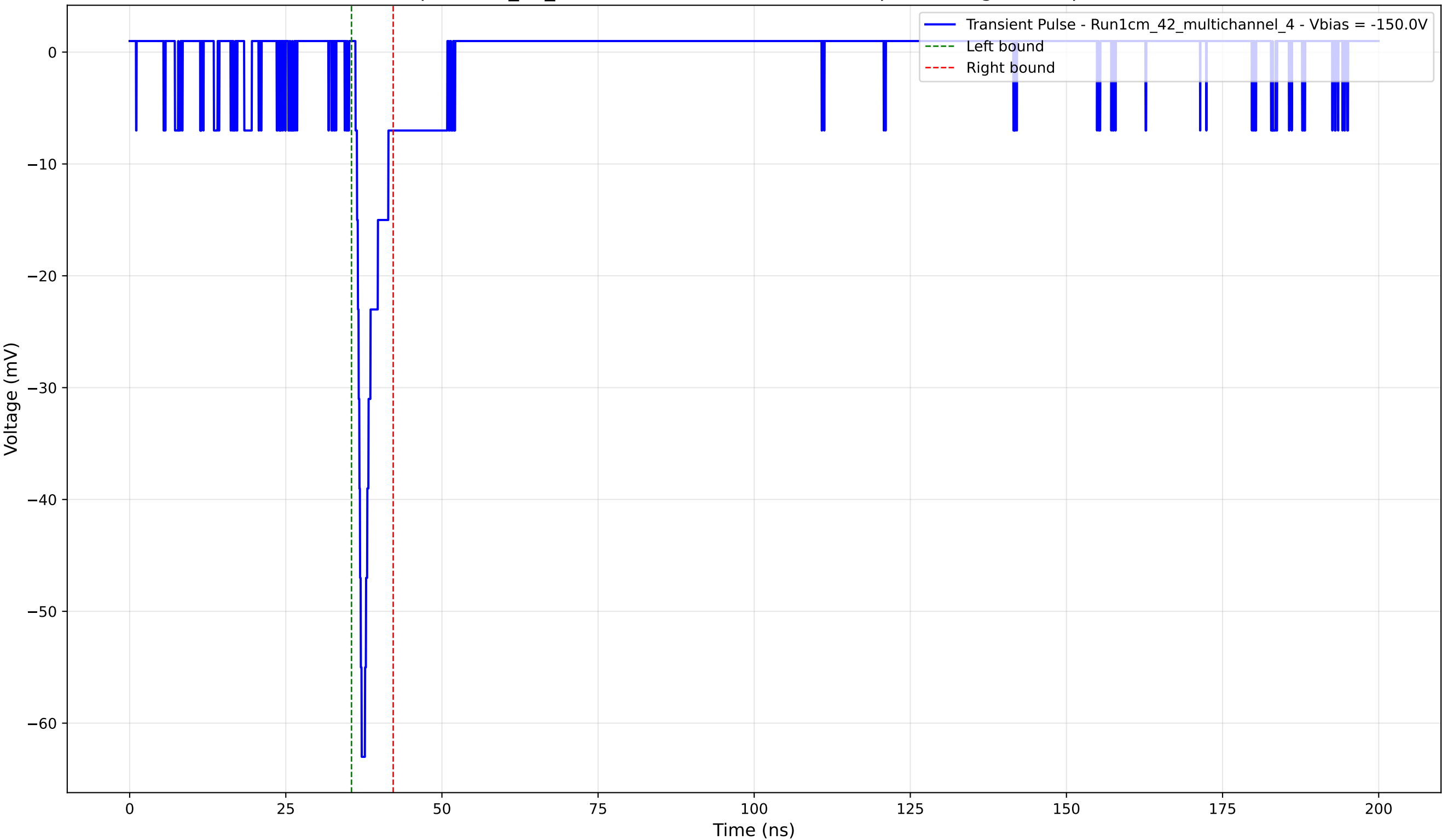
Transient Pulse - Sample: 1cm_42_multichannel - Position: 2125.0 \mu\text{m} - Charge: 3.09 pC - Rise Time: 0.98 ns
