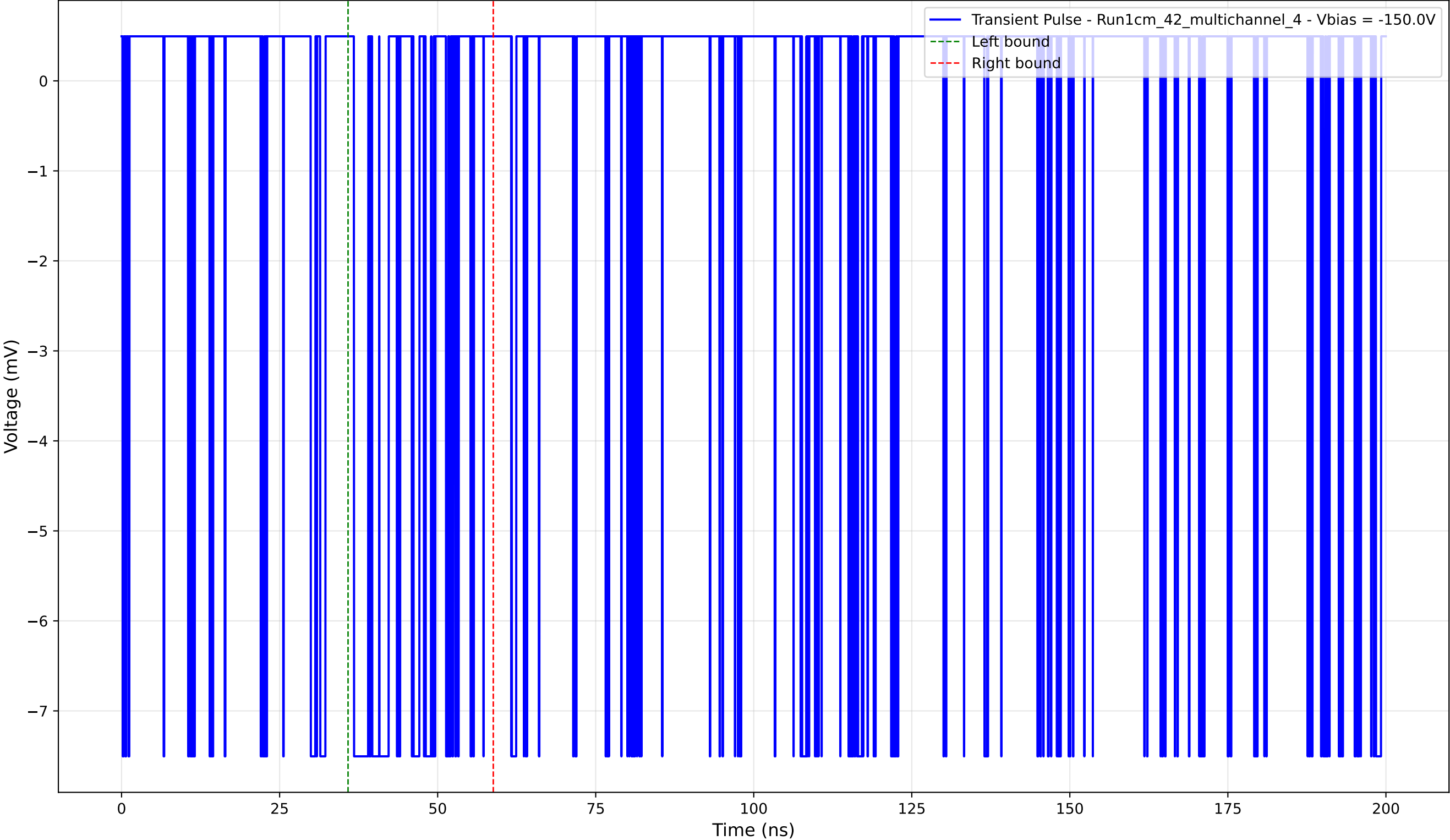
Transient Pulse - Sample: 1cm_42_multichannel - Position: 2905.0 \mu\text{m} - Charge: 1.21 pC - Rise Time: 0.02 ns
