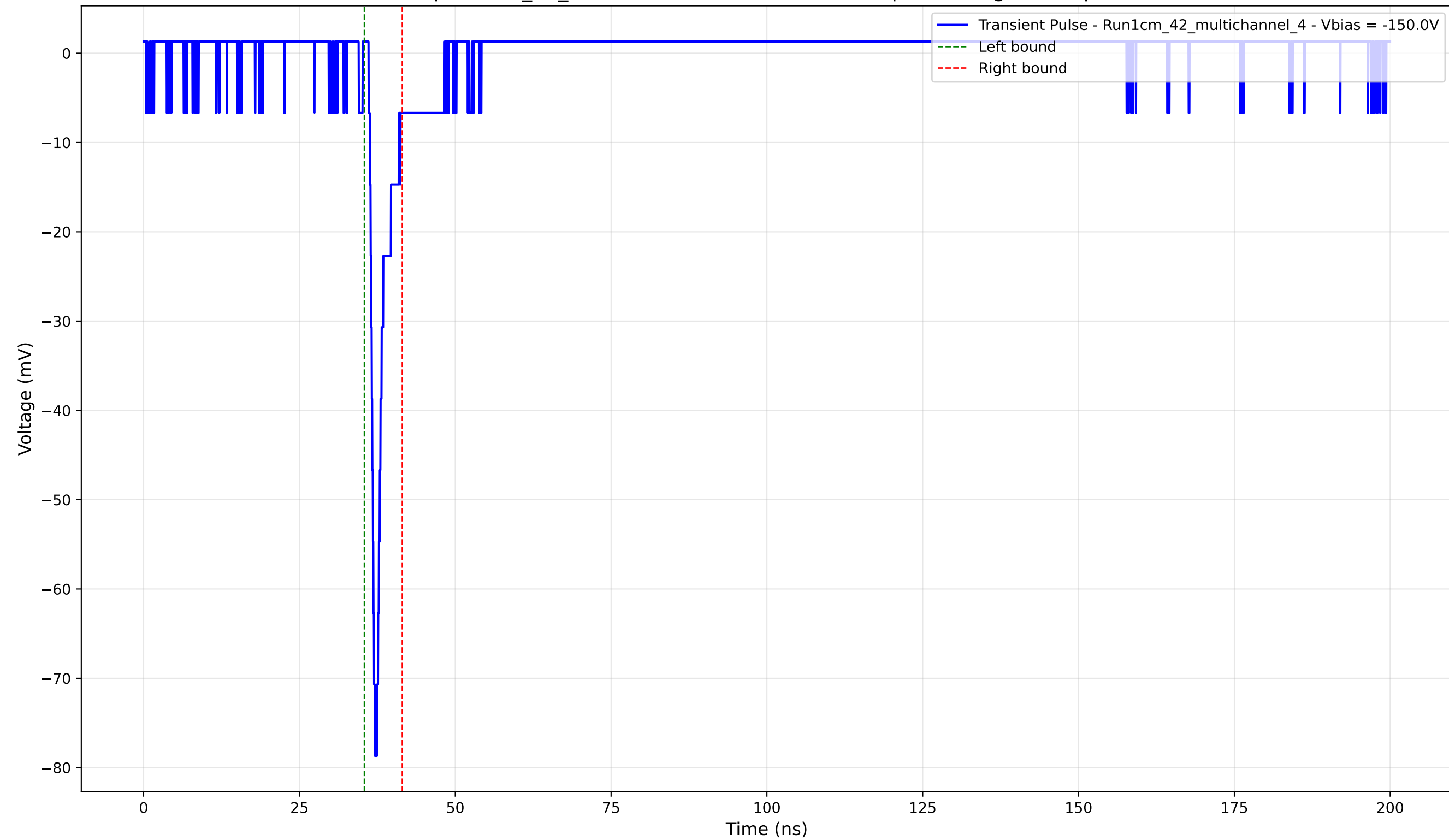
Transient Pulse - Sample: 1cm_42_multichannel - Position: 2520.0 \mu\text{m} - Charge: 3.23 pC - Rise Time: 0.82 ns
