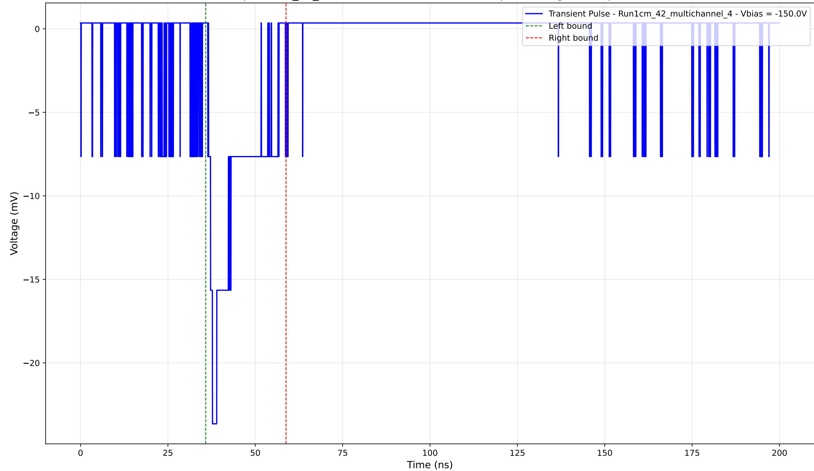
Transient Pulse - Sample: 1cm_42_multichannel - Position: 3475.0 \mu\text{m} - Charge: 4.10 pC - Rise Time: 1.11 ns
