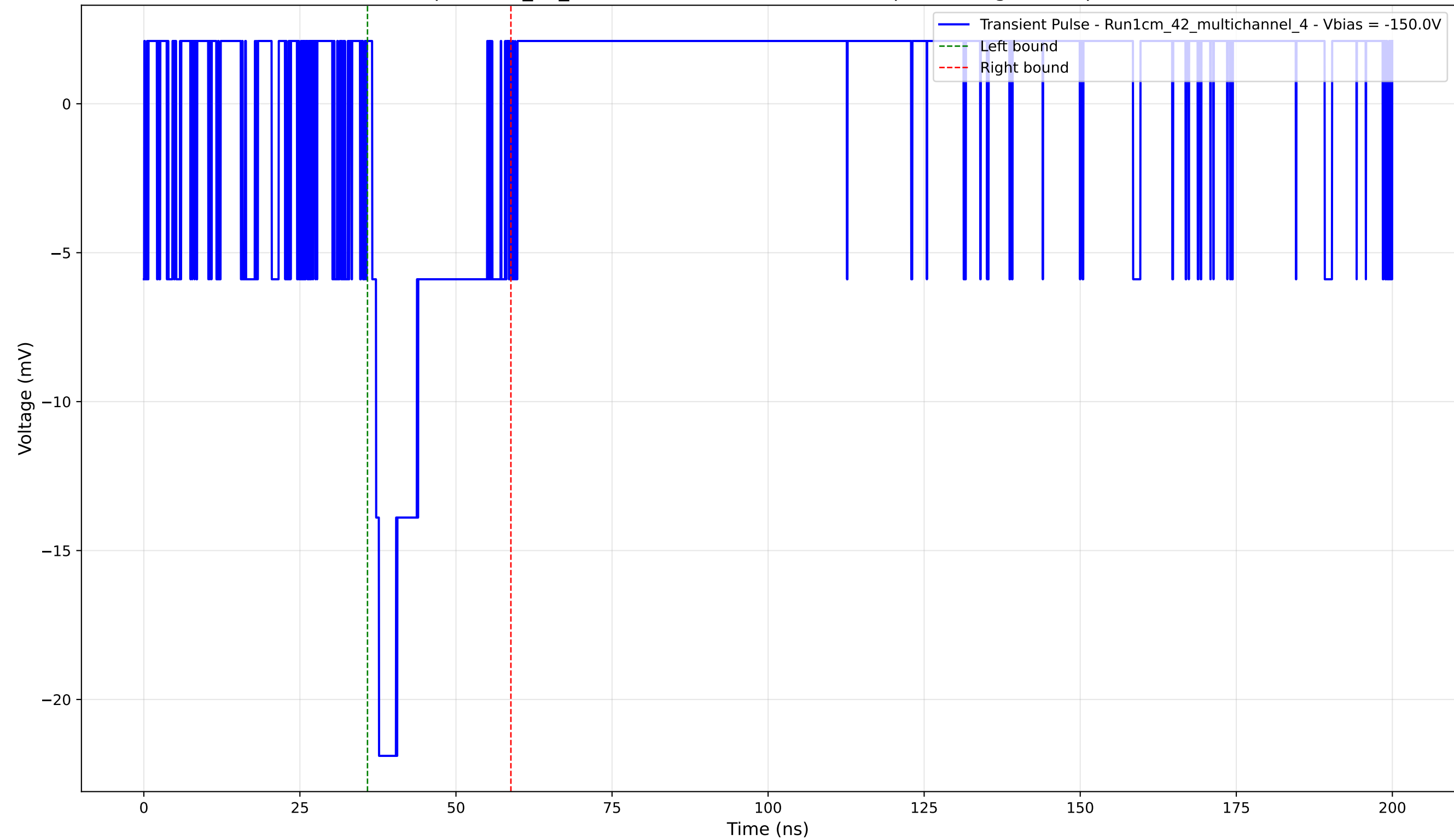
Transient Pulse - Sample: 1cm_42_multichannel - Position: 1205.0 \mu\text{m} - Charge: 3.92 pC - Rise Time: 1.10 ns
