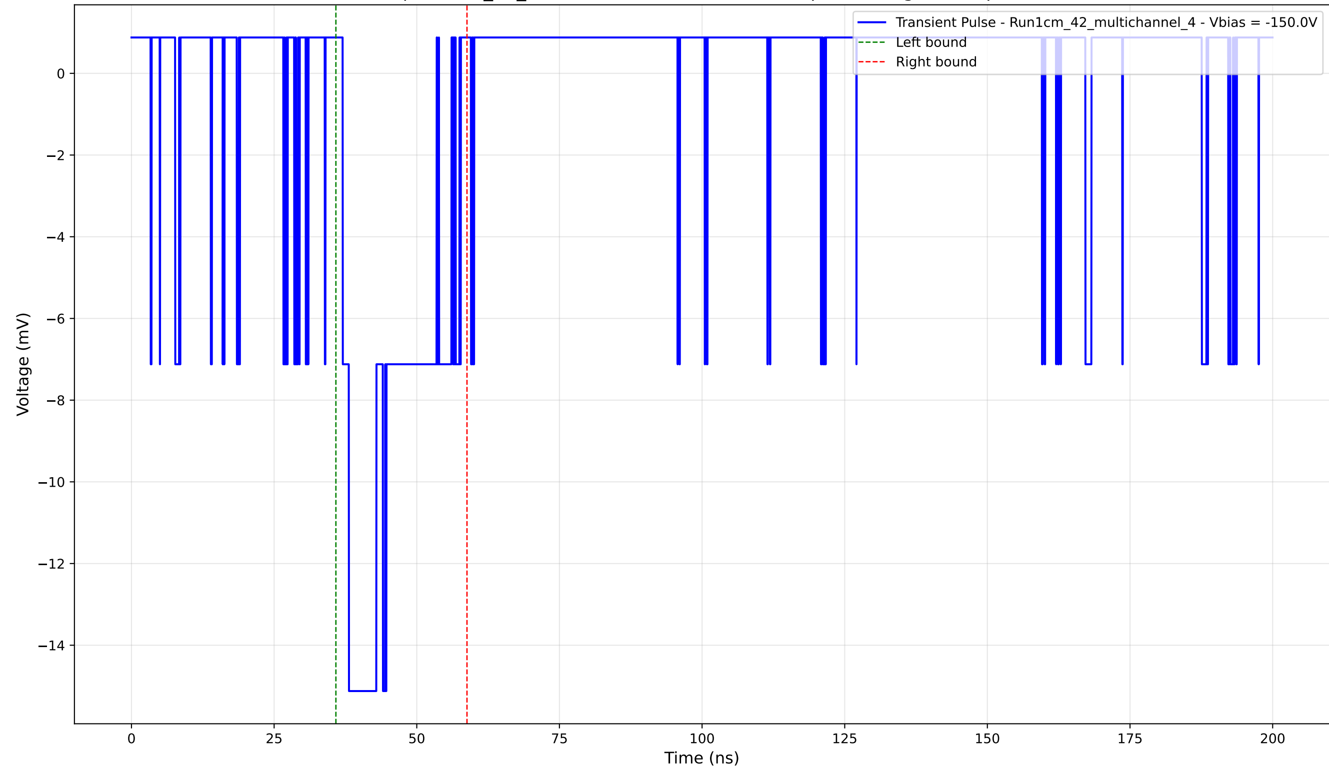
Transient Pulse - Sample: 1cm_42_multichannel - Position: 610.0 \mu\text{m} - Charge: 3.67 pC - Rise Time: 1.10 ns
