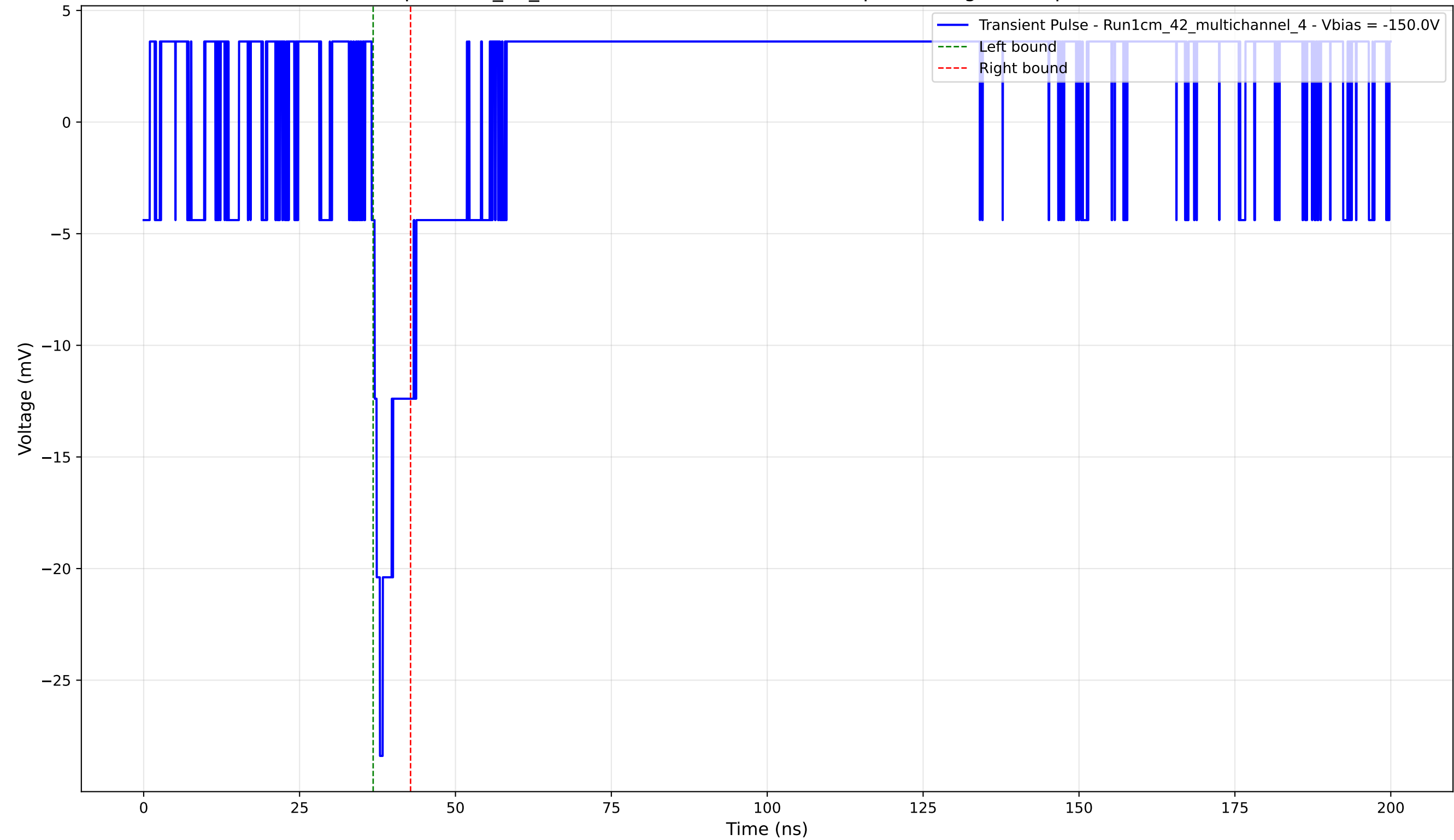
Transient Pulse - Sample: 1cm_42_multichannel - Position: 1445.0 \mu\text{m} - Charge: 1.92 pC - Rise Time: 0.00 ns (N/A)
