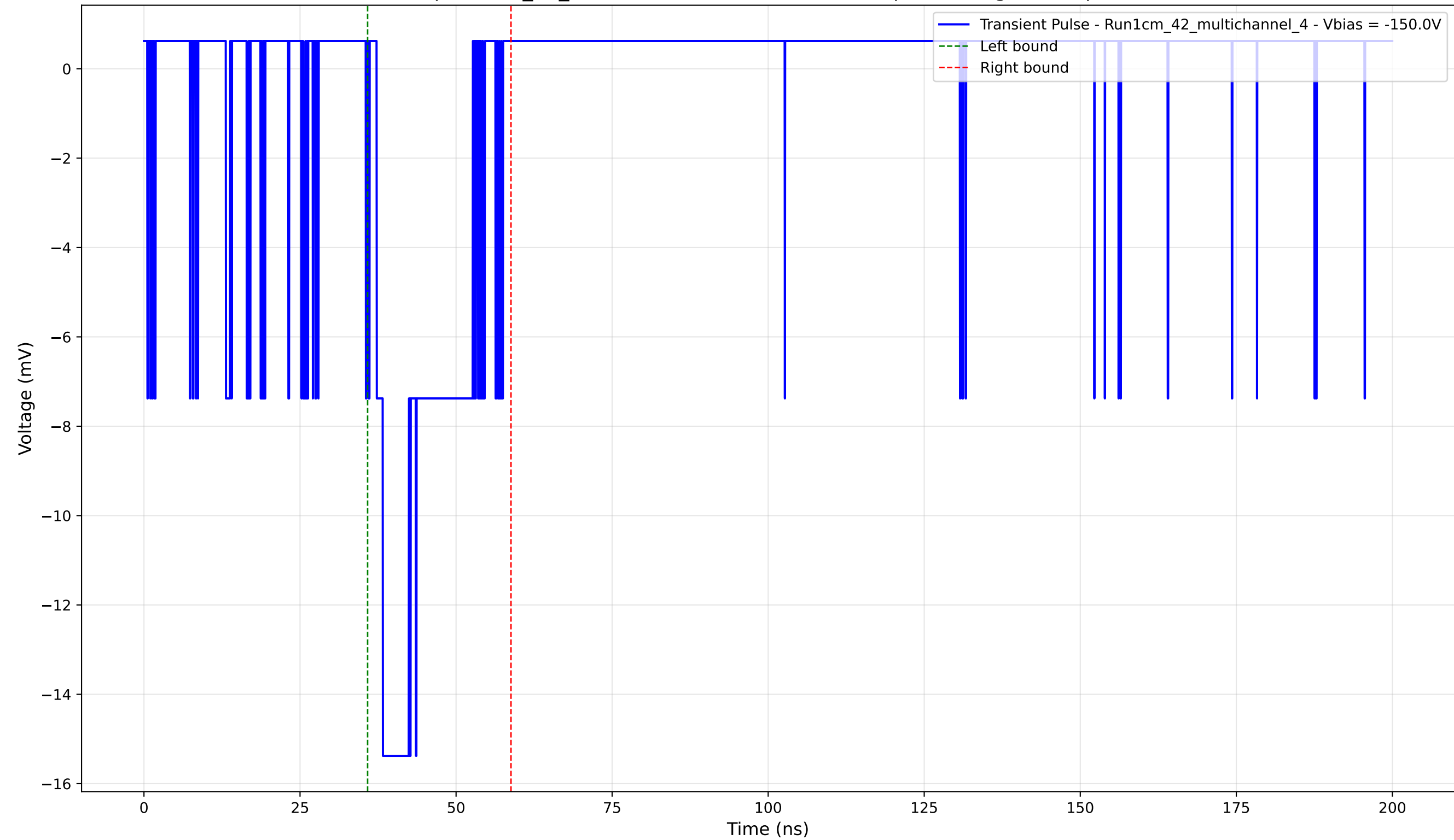
Transient Pulse - Sample: 1cm_42_multichannel - Position: 4165.0 \mu\text{m} - Charge: 3.20 pC - Rise Time: 1.00 ns
