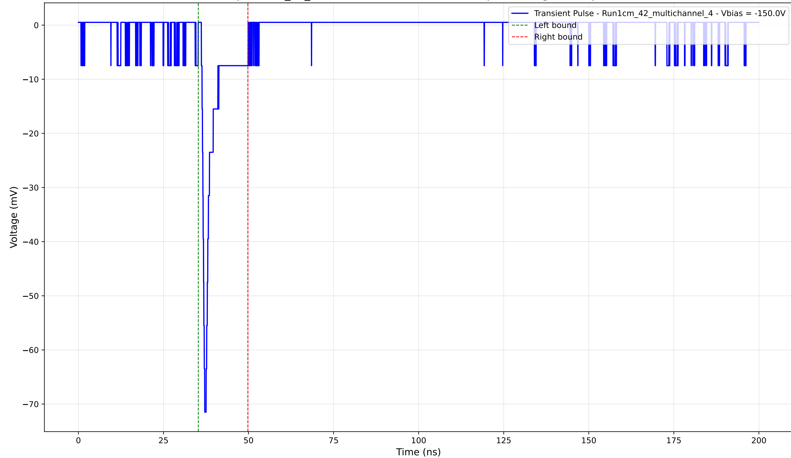
Transient Pulse - Sample: 1cm_42_multichannel - Position: 2195.0 \mu\text{m} - Charge: 4.42 pC - Rise Time: 0.98 ns
