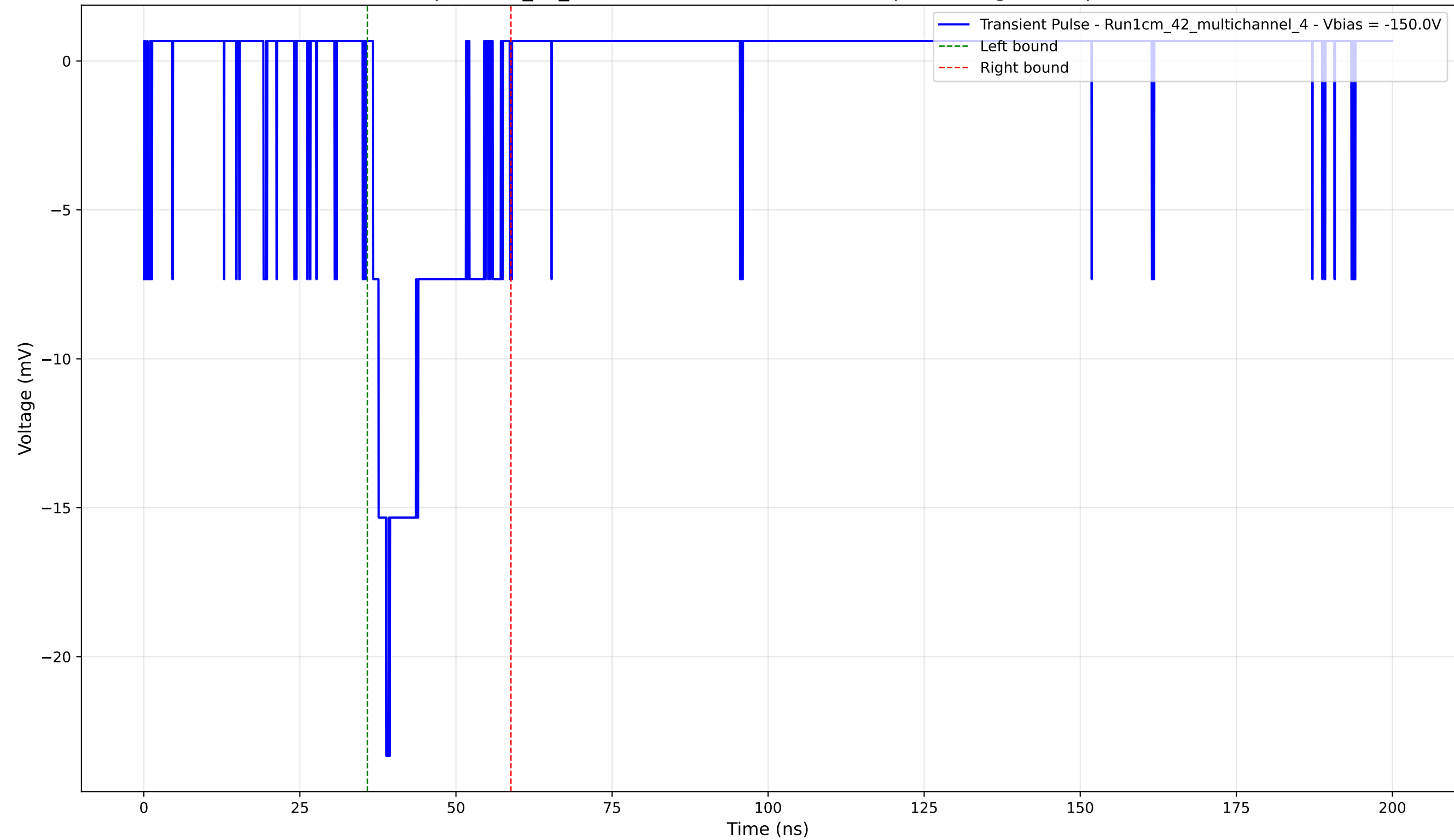
Transient Pulse - Sample: 1cm_42_multichannel - Position: 3740.0 \mu\text{m} - Charge: 3.87 pC - Rise Time: 2.12 ns
