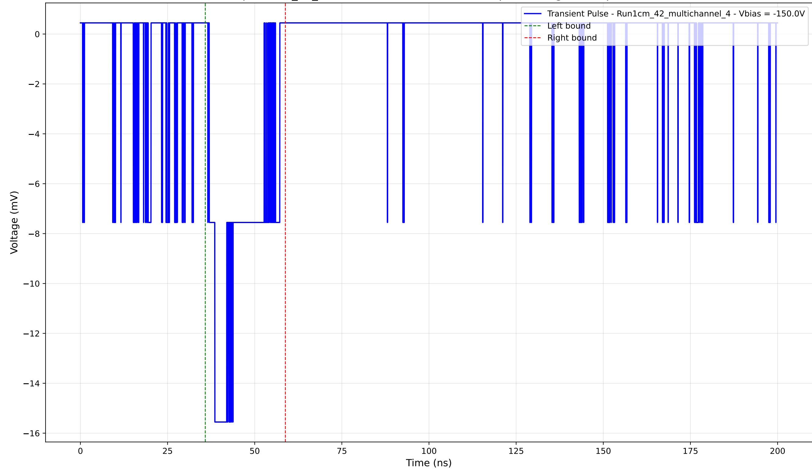
Transient Pulse - Sample: 1cm_42_multichannel - Position: 4705.0 \mu\text{m} - Charge: 3.48 pC - Rise Time: 1.62 ns
