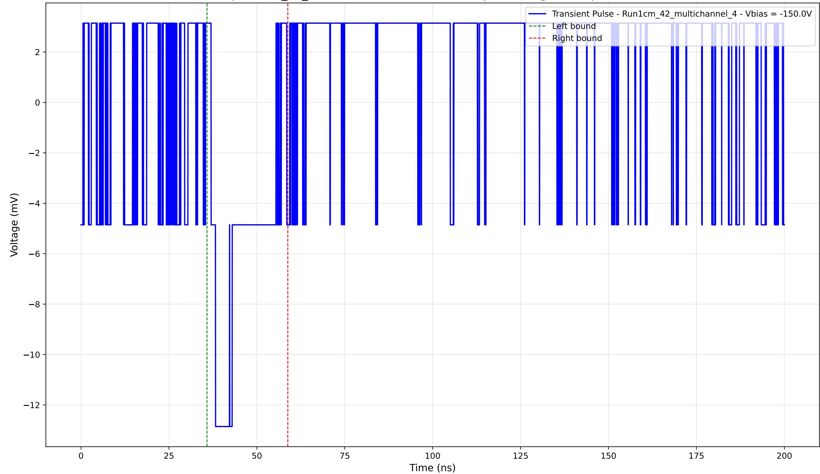
Transient Pulse - Sample: 1cm_42_multichannel - Position: 255.0 \mu\text{m} - Charge: 2.46 pC - Rise Time: 0.00 ns (N/A)
