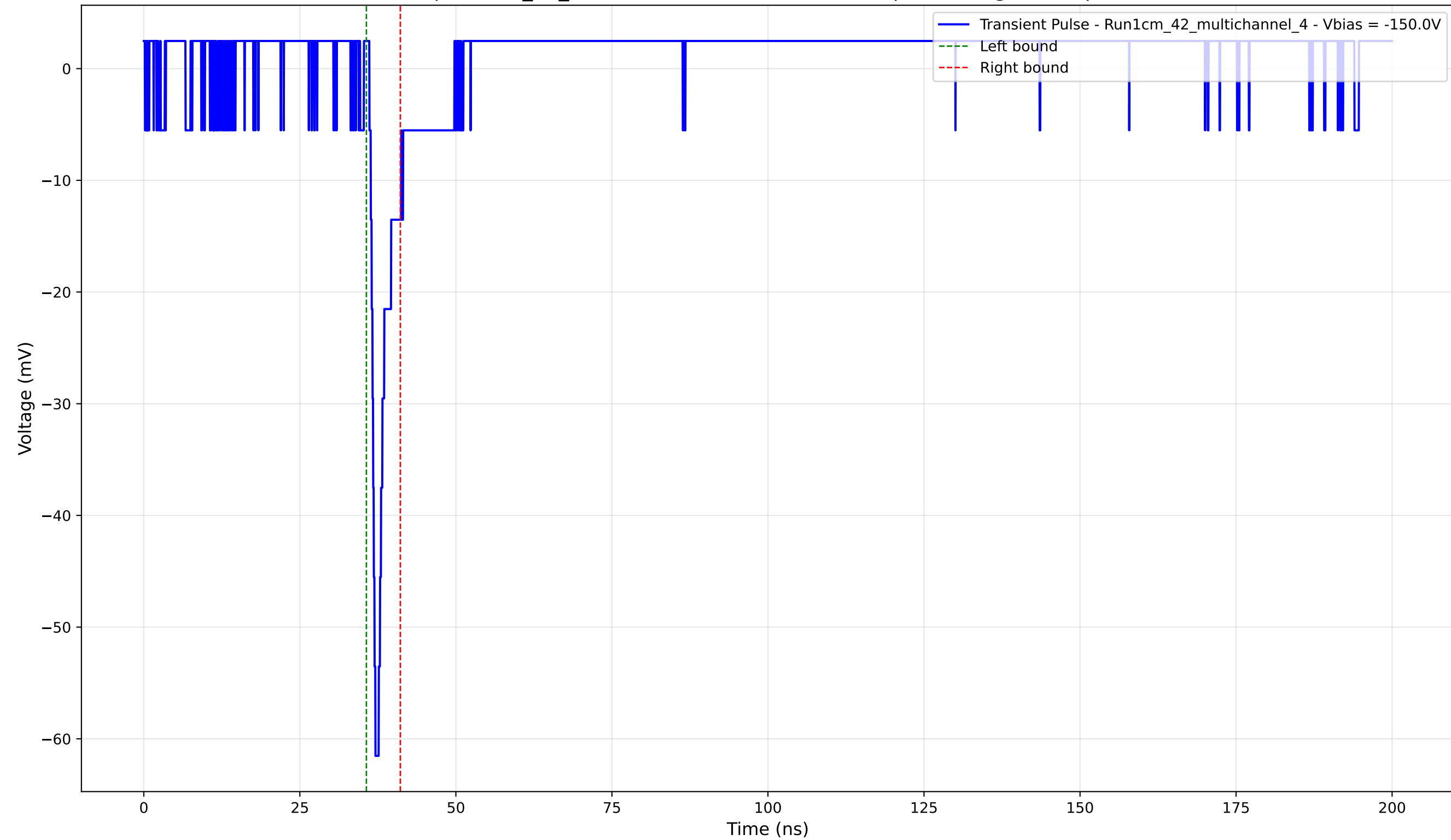
Transient Pulse - Sample: 1cm_42_multichannel - Position: 2625.0 \mu\text{m} - Charge: 2.74 pC - Rise Time: 0.76 ns
