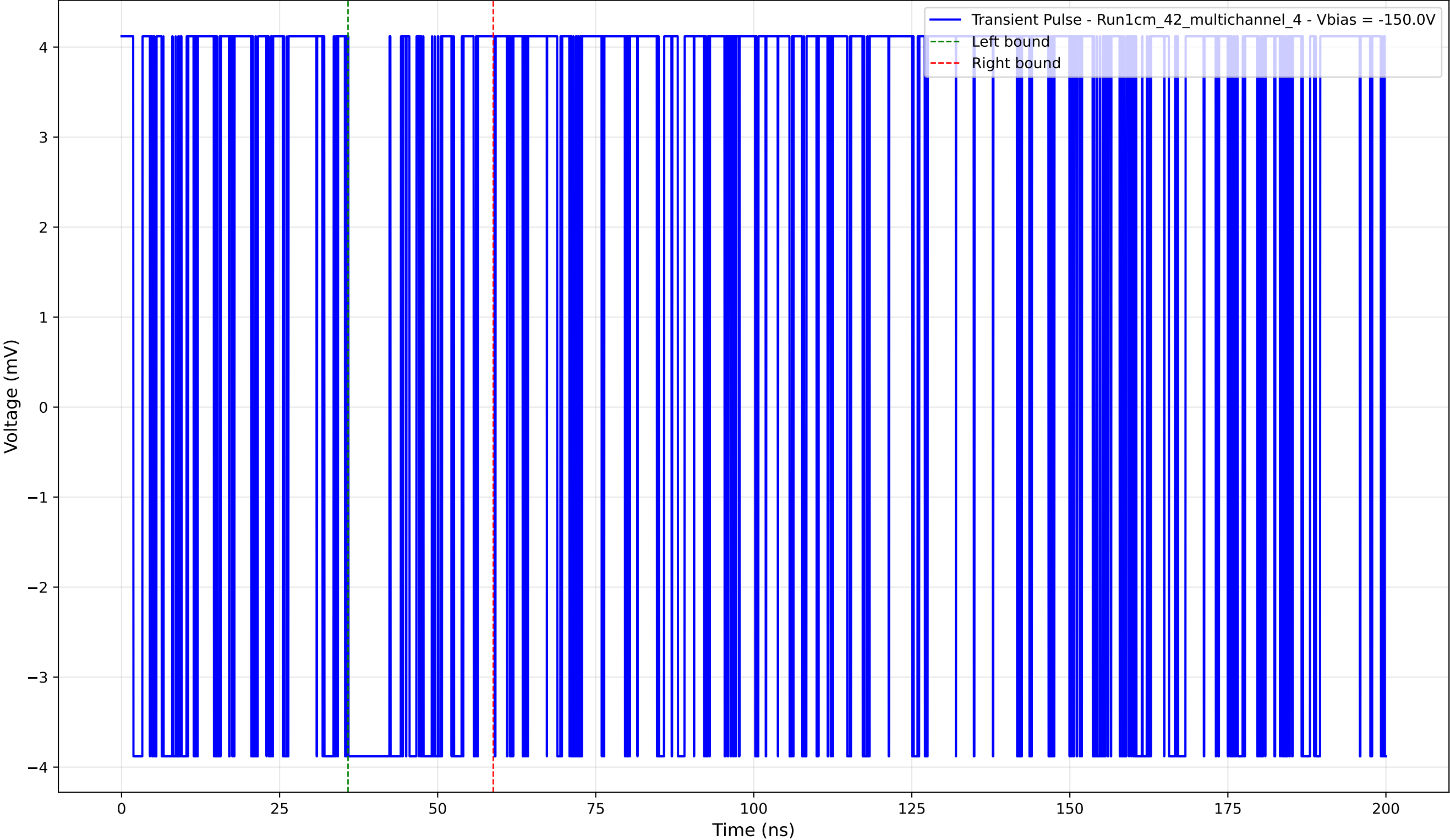
Transient Pulse - Sample: 1cm_42_multichannel - Position: 1845.0 \mu\text{m} - Charge: 0.43 pC - Rise Time: 0.00 ns (N/A)
