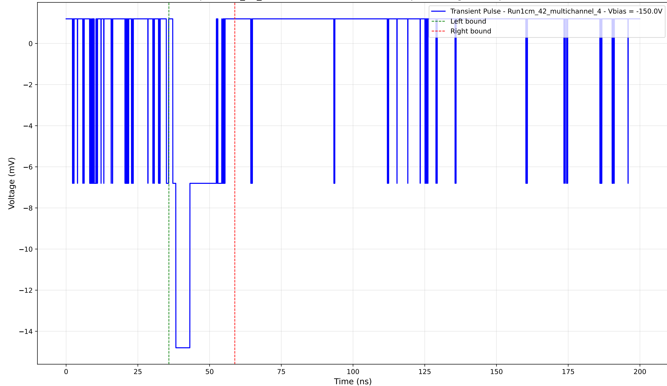
Transient Pulse - Sample: 1cm_42_multichannel - Position: 4310.0 \mu\text{m} - Charge: 3.02 pC - Rise Time: 1.08 ns
