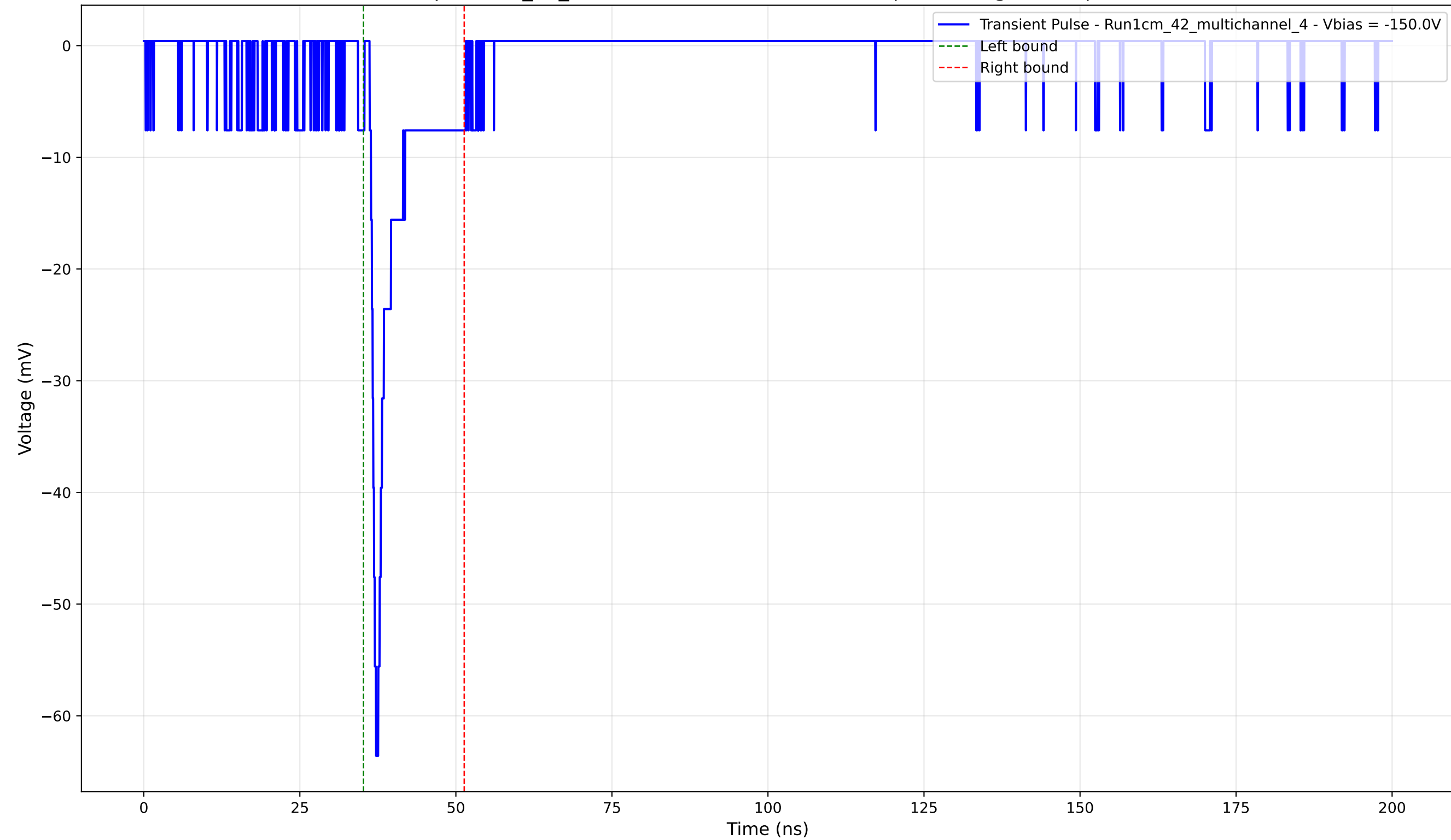
Transient Pulse - Sample: 1cm_42_multichannel - Position: 2645.0 \mu\text{m} - Charge: 4.53 pC - Rise Time: 1.02 ns
