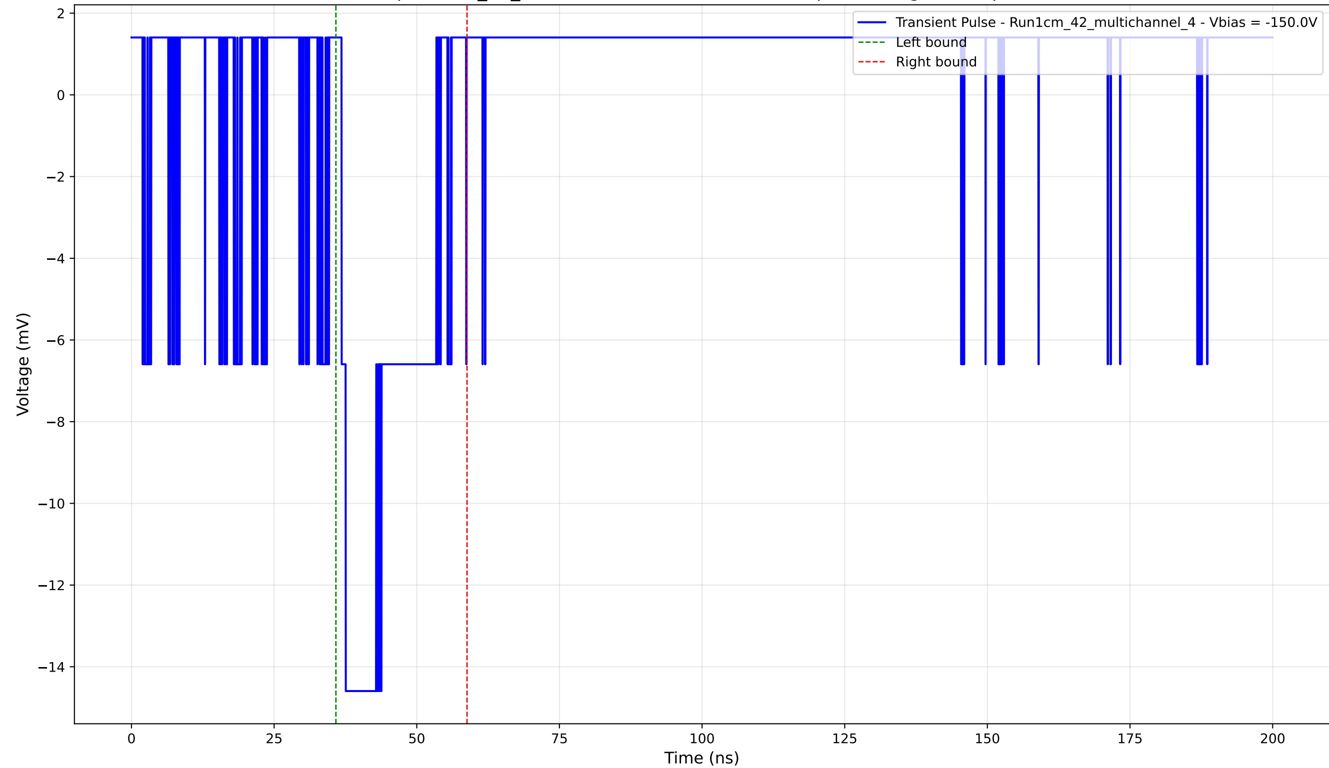
Transient Pulse - Sample: 1cm_42_multichannel - Position: 3730.0 \mu\text{m} - Charge: 3.08 pC - Rise Time: 0.74 ns
