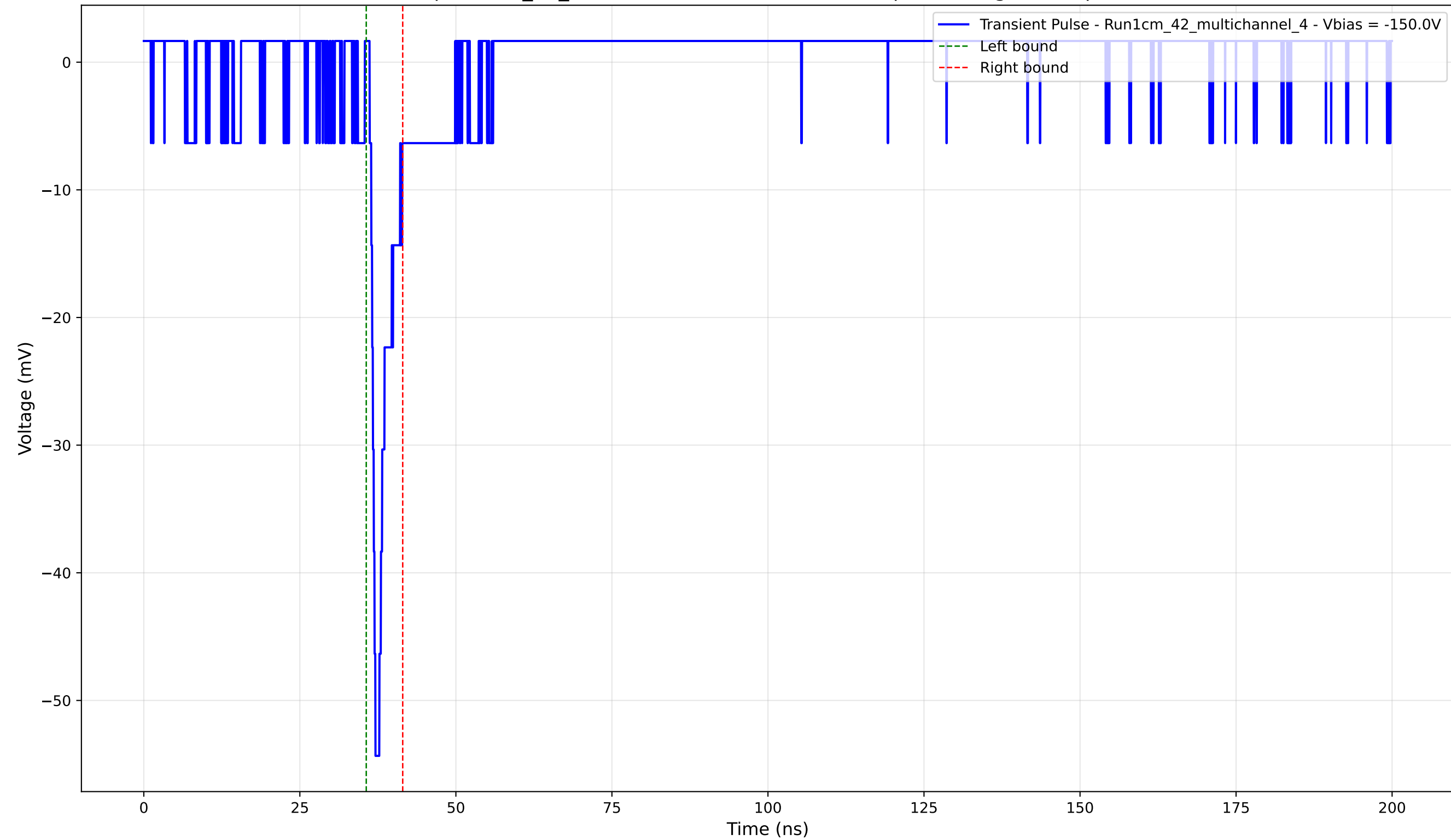
Transient Pulse - Sample: 1cm_42_multichannel - Position: 2705.0 \mu\text{m} - Charge: 2.73 pC - Rise Time: 0.92 ns
