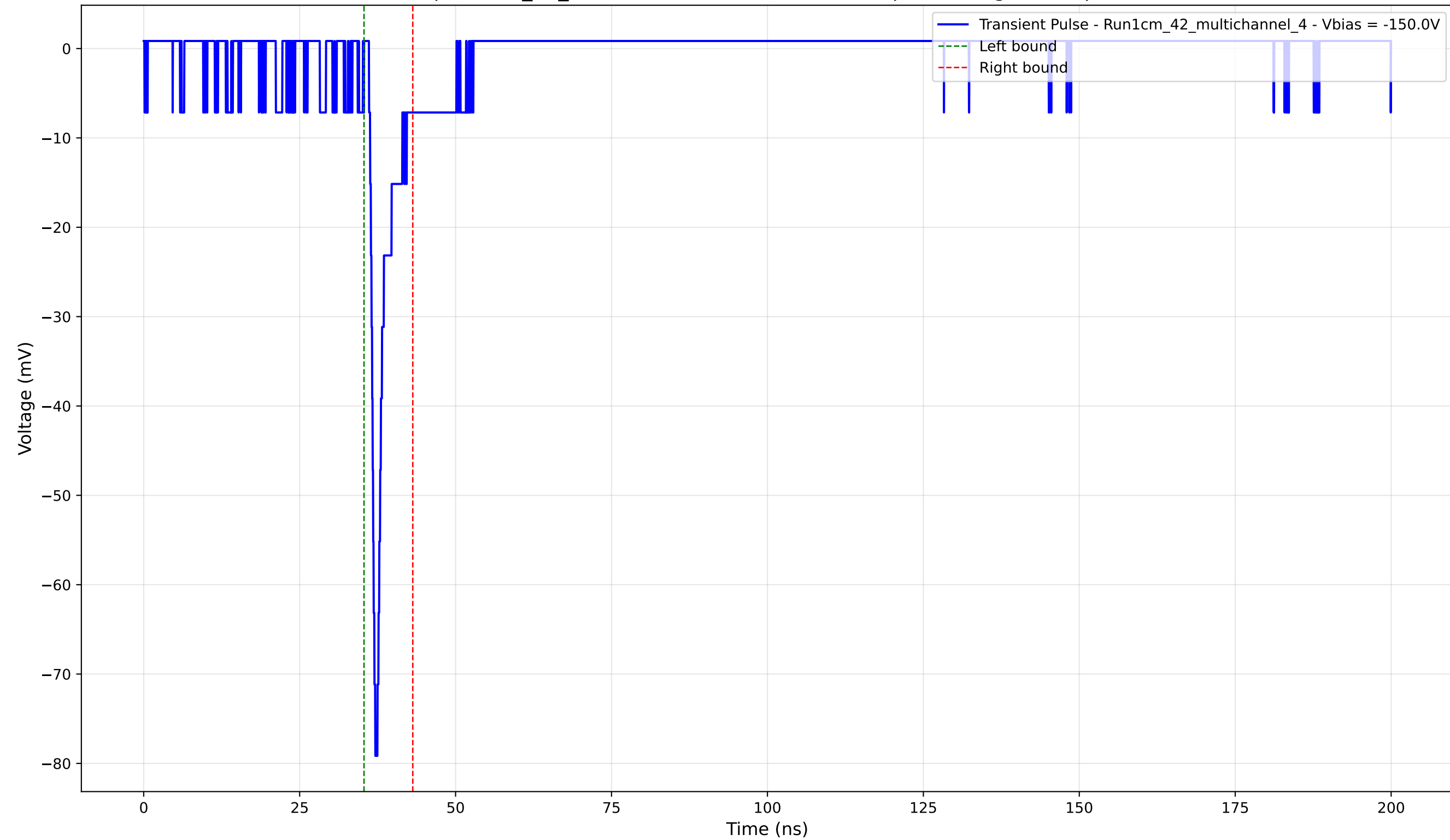
Transient Pulse - Sample: 1cm_42_multichannel - Position: 2240.0 \mu\text{m} - Charge: 3.65 pC - Rise Time: 0.84 ns
