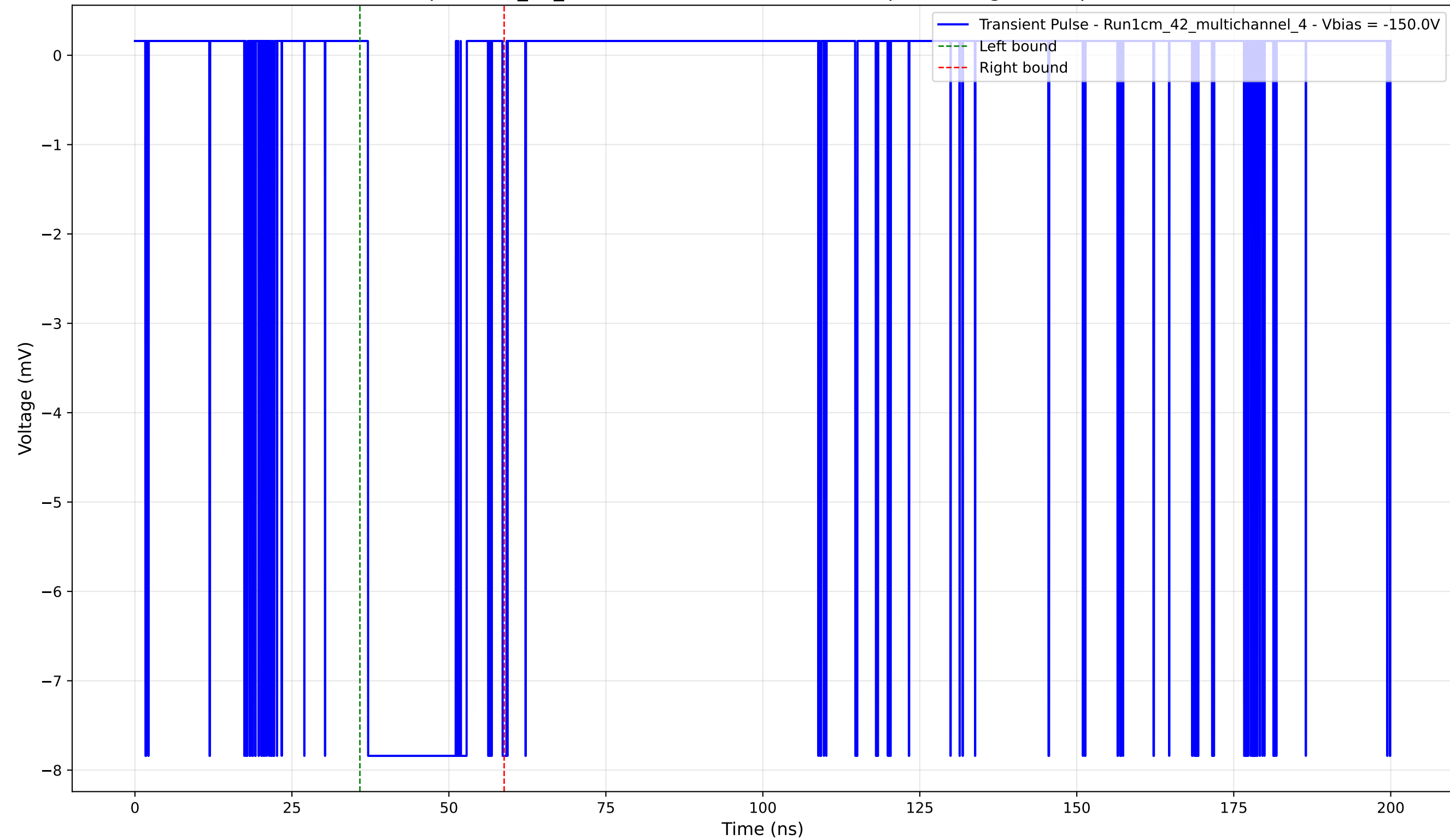
Transient Pulse - Sample: 1cm_42_multichannel - Position: 4855.0 \mu\text{m} - Charge: 2.48 pC - Rise Time: 0.02 ns
