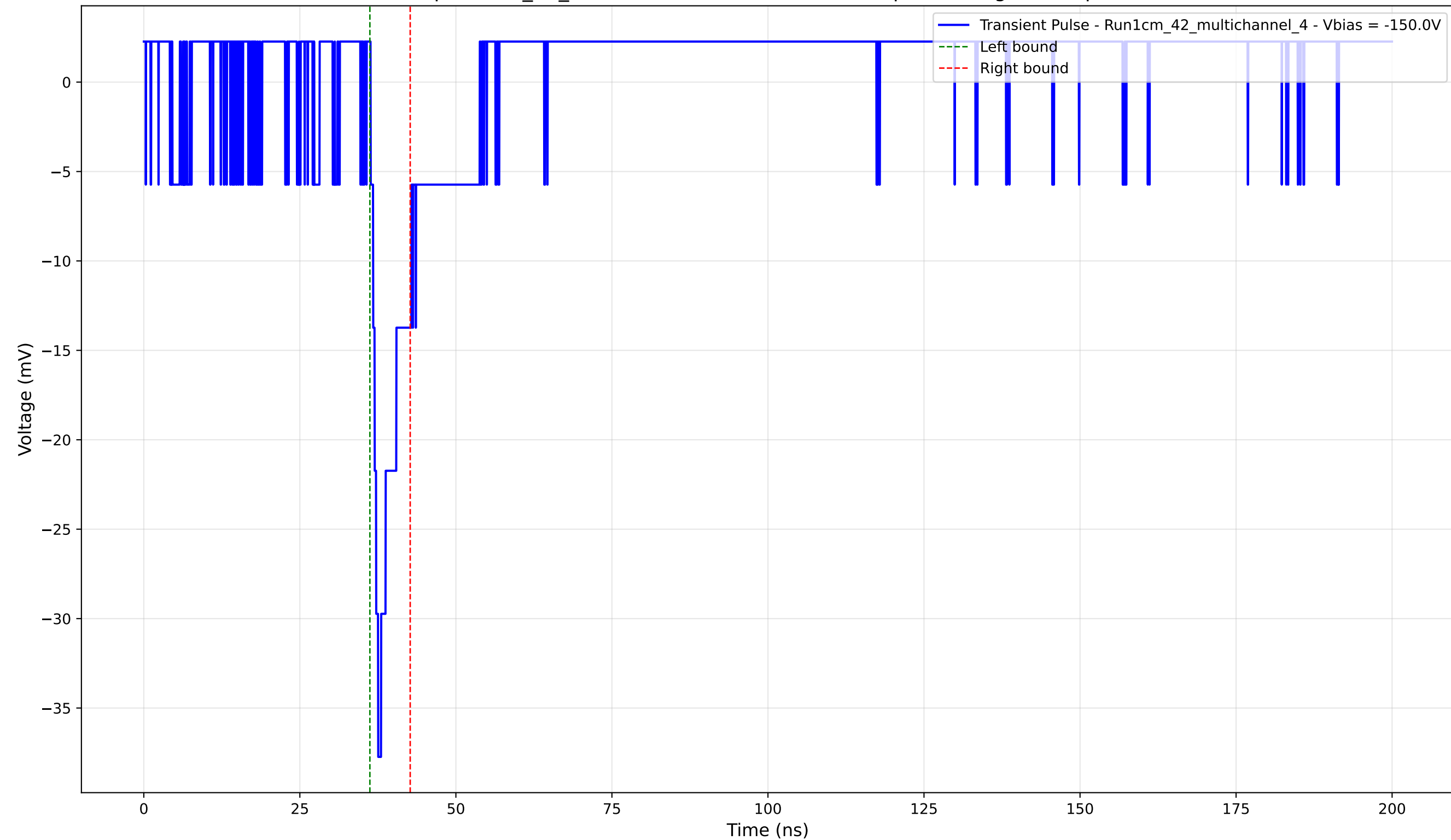
Transient Pulse - Sample: 1cm_42_multichannel - Position: 1670.0 \mu\text{m} - Charge: 2.55 pC - Rise Time: 1.21 ns
