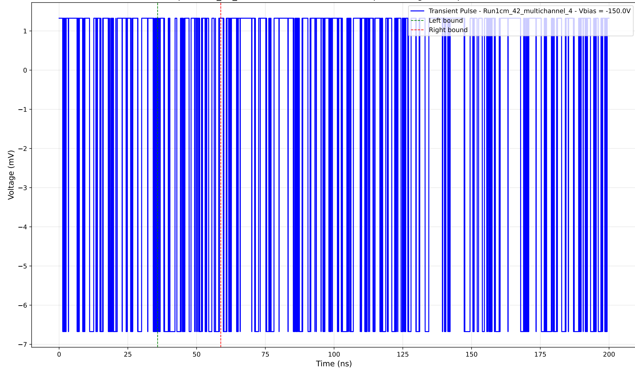
Transient Pulse - Sample: 1cm_42_multichannel - Position: 870.0 \mu\text{m} - Charge: 1.22 pC - Rise Time: 0.00 ns (N/A)
