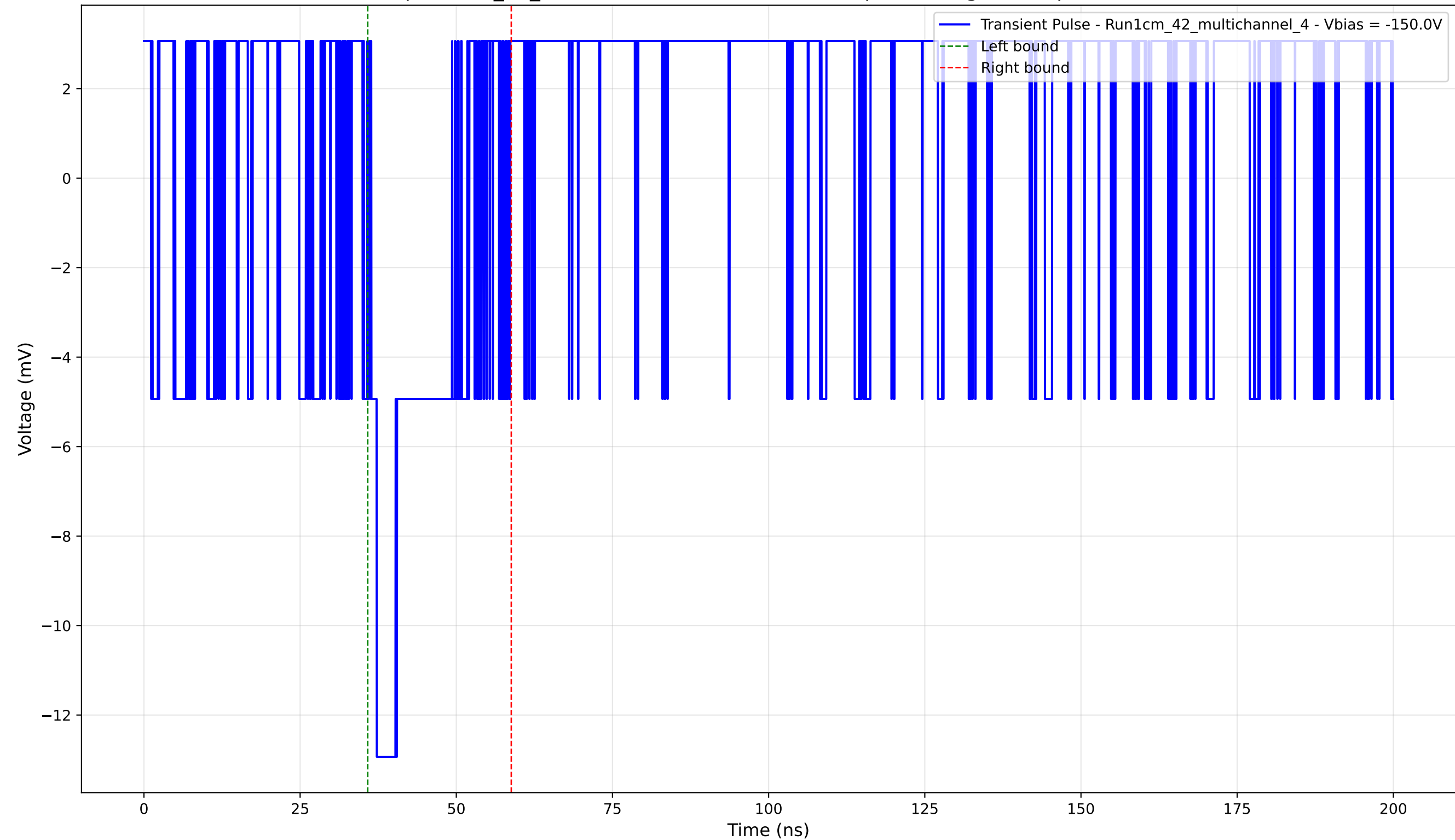
Transient Pulse - Sample: 1cm_42_multichannel - Position: 1425.0 \mu\text{m} - Charge: 1.87 pC - Rise Time: 0.00 ns (N/A)
