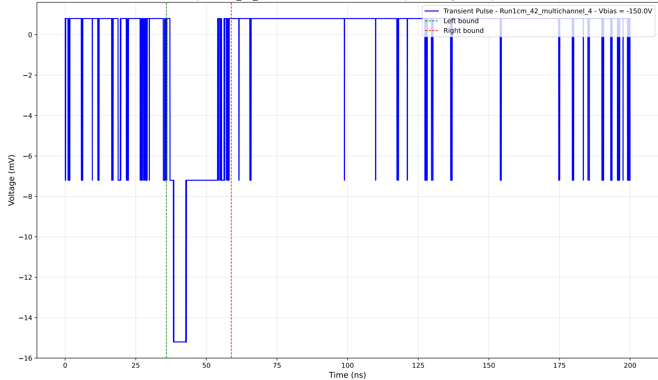
Transient Pulse - Sample: 1cm_42_multichannel - Position: 4505.0 \mu\text{m} - Charge: 3.40 pC - Rise Time: 1.24 ns
