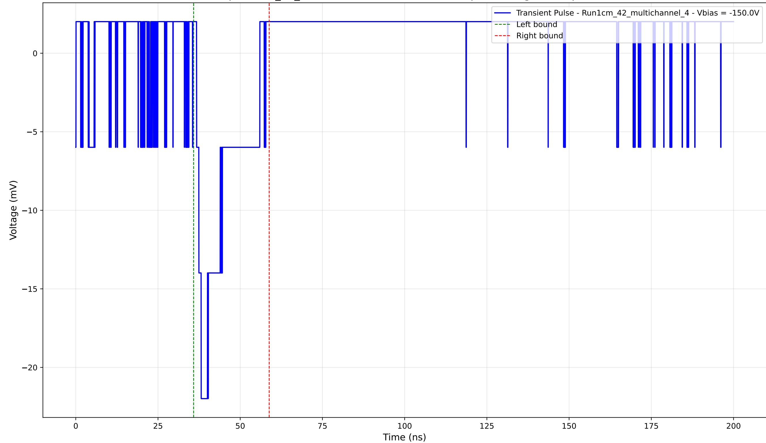
Transient Pulse - Sample: 1cm_42_multichannel - Position: 1005.0 \mu\text{m} - Charge: 3.61 pC - Rise Time: 1.40 ns
