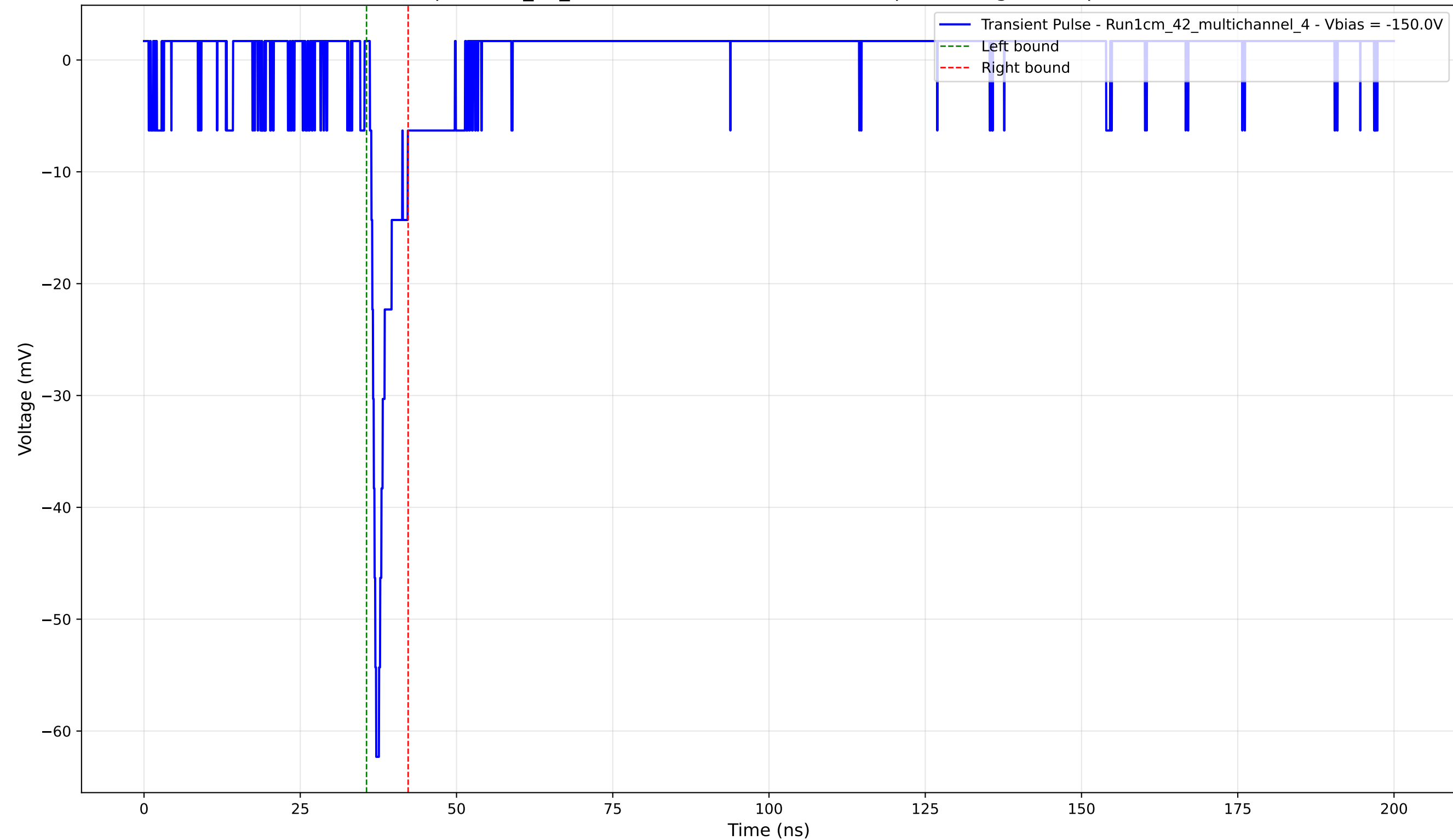
Transient Pulse - Sample: 1cm_42_multichannel - Position: 2640.0 \mu\text{m} - Charge: 3.07 pC - Rise Time: 1.00 ns
