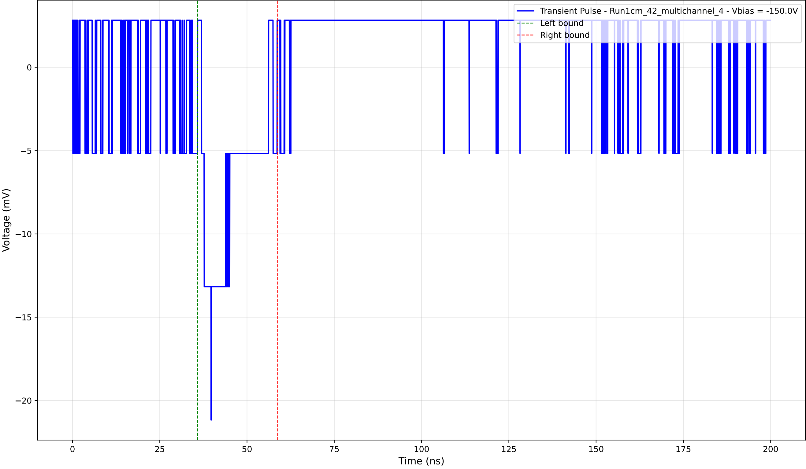
Transient Pulse - Sample: 1cm_42_multichannel - Position: 765.0 \mu\text{m} - Charge: 3.05 pC - Rise Time: 0.00 ns (N/A)
