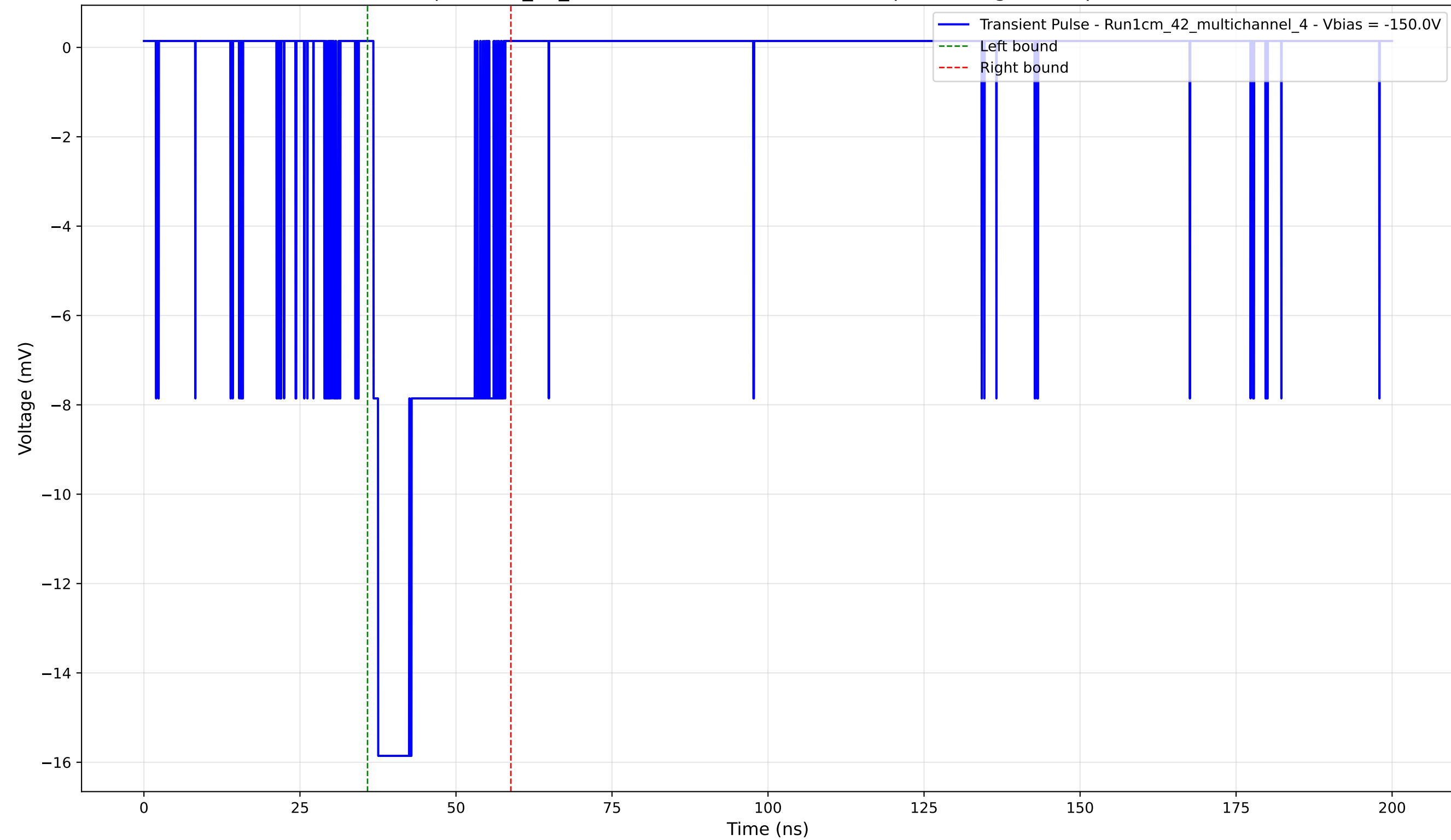
Transient Pulse - Sample: 1cm_42_multichannel - Position: 3625.0 \mu\text{m} - Charge: 3.94 pC - Rise Time: 0.76 ns
