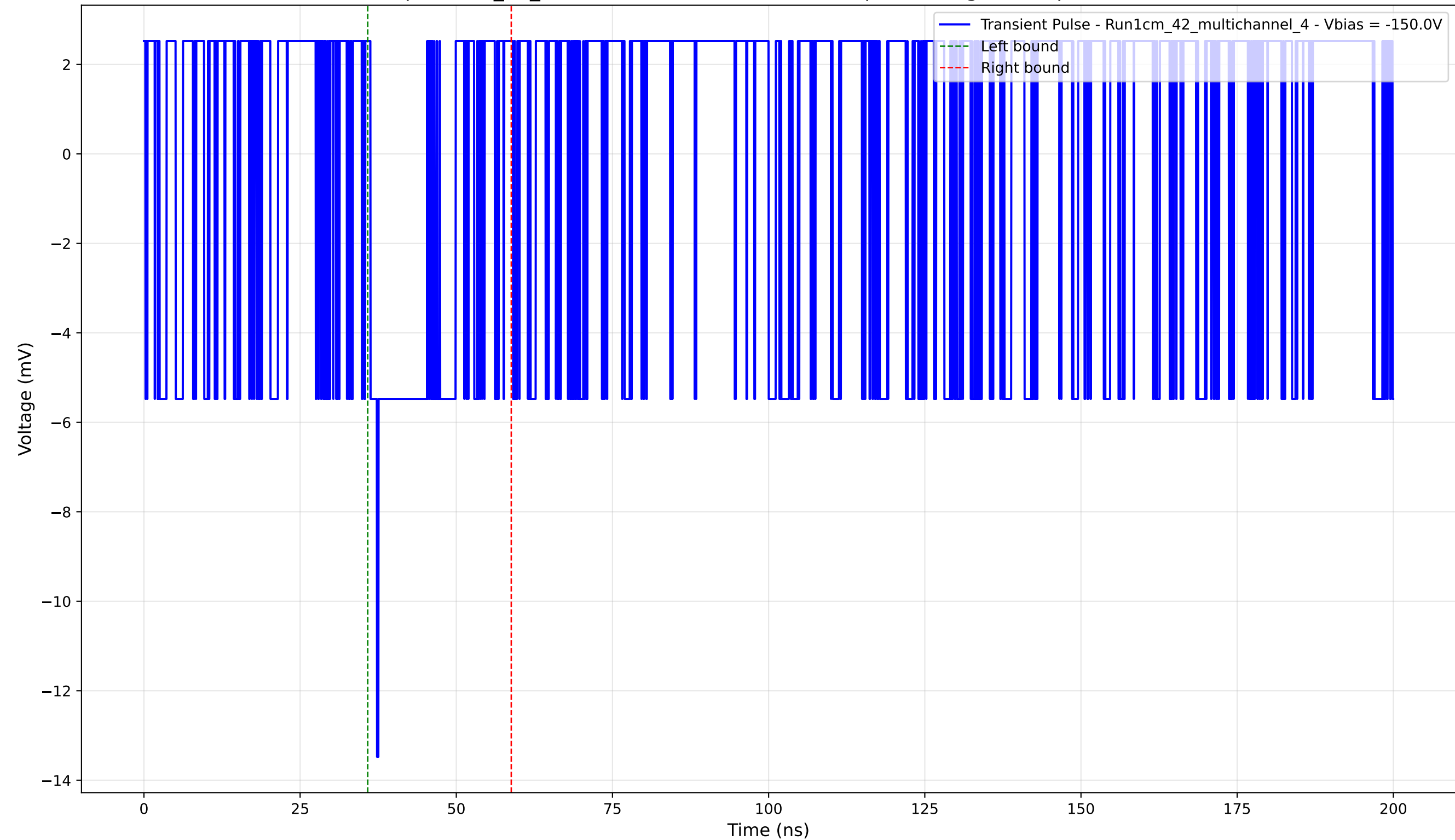
Transient Pulse - Sample: 1cm_42_multichannel - Position: 1915.0 \mu\text{m} - Charge: 1.20 pC - Rise Time: 0.00 ns (N/A)
