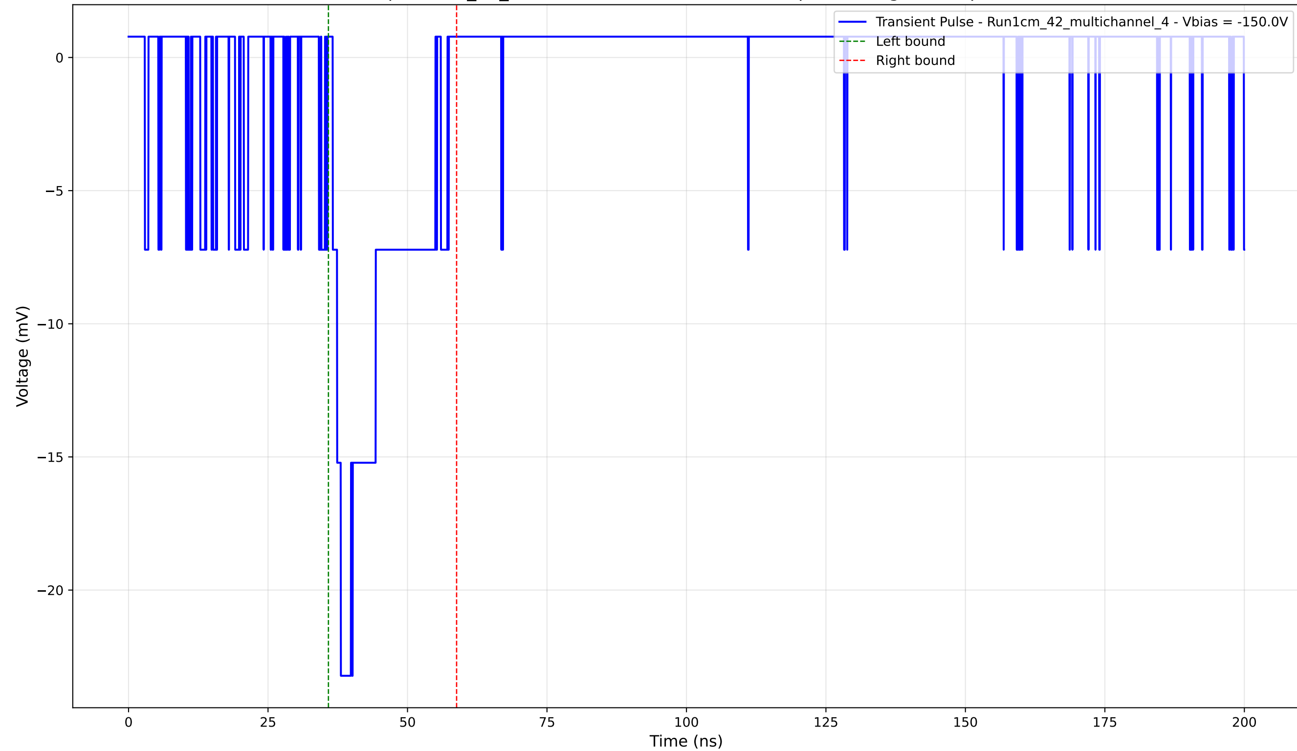
Transient Pulse - Sample: 1cm_42_multichannel - Position: 1110.0 \mu\text{m} - Charge: 4.23 pC - Rise Time: 1.46 ns
