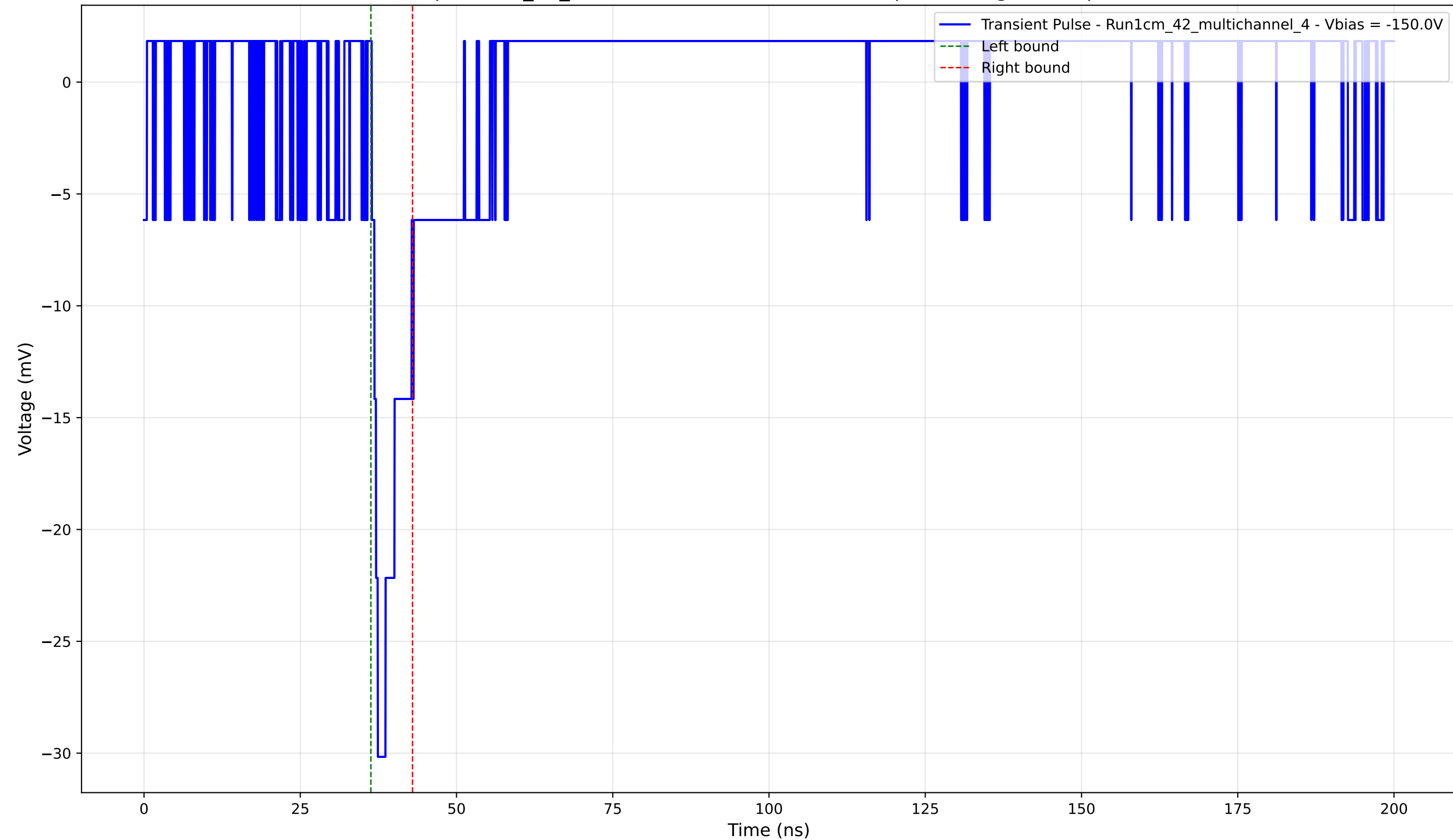
Transient Pulse - Sample: 1cm_42_multichannel - Position: 1580.0 \mu\text{m} - Charge: 2.43 pC - Rise Time: 0.97 ns
