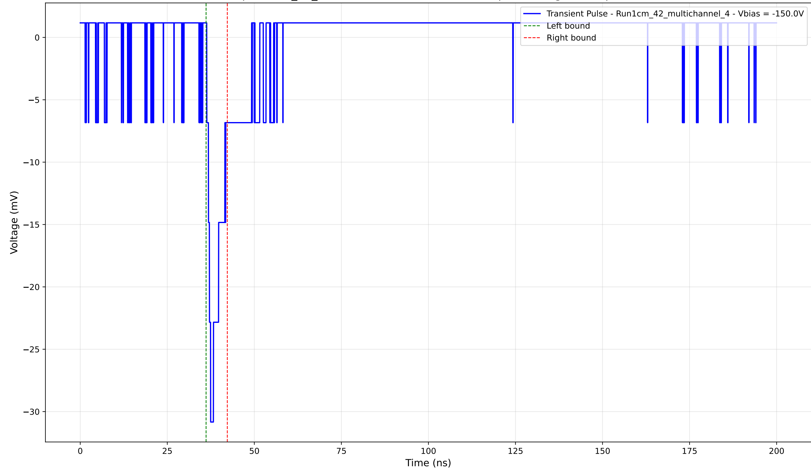
Transient Pulse - Sample: 1cm_42_multichannel - Position: 3125.0 \mu\text{m} - Charge: 2.13 pC - Rise Time: 1.11 ns
