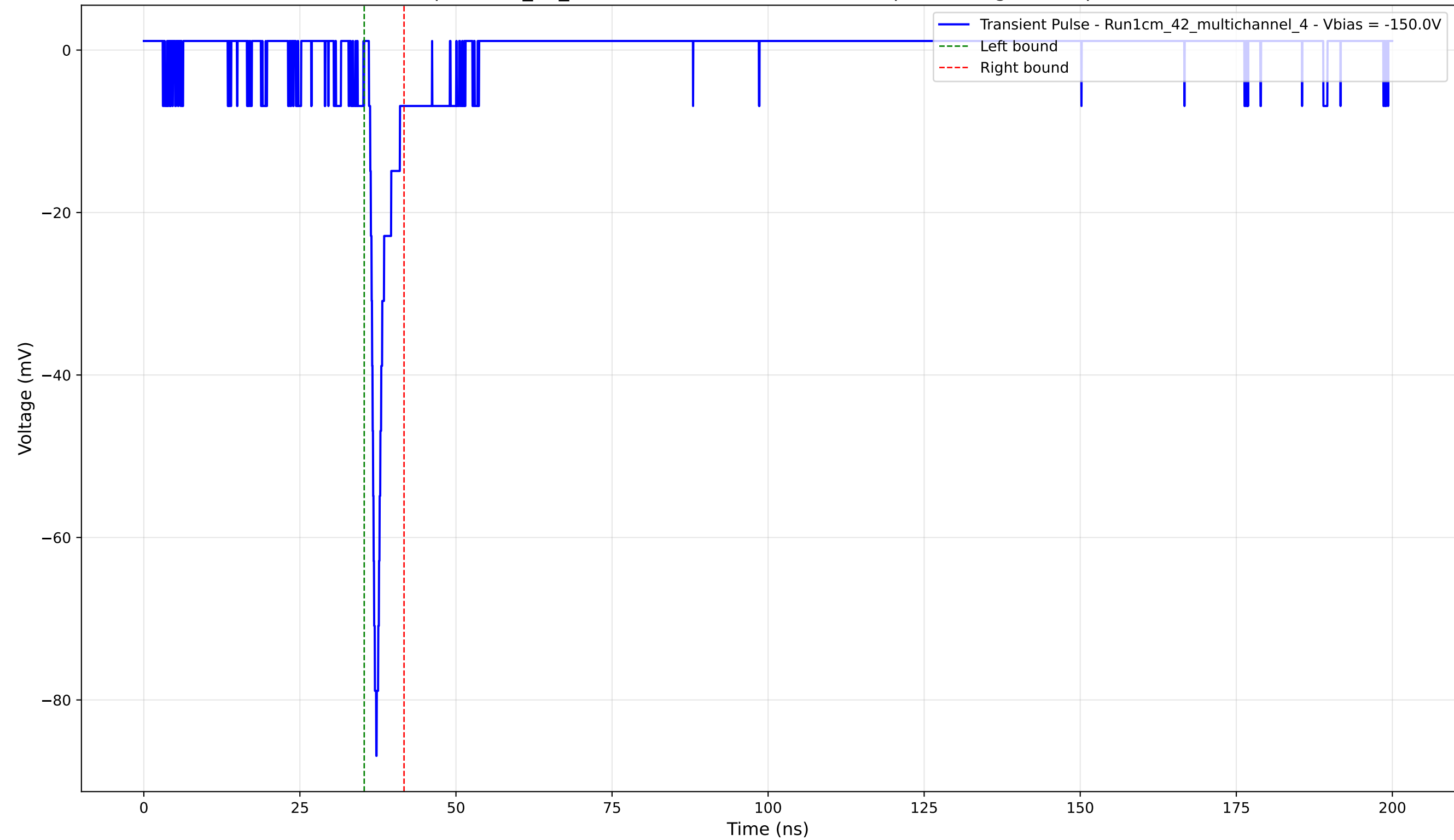
Transient Pulse - Sample: 1cm_42_multichannel - Position: 2480.0 \mu\text{m} - Charge: 3.40 pC - Rise Time: 0.76 ns
