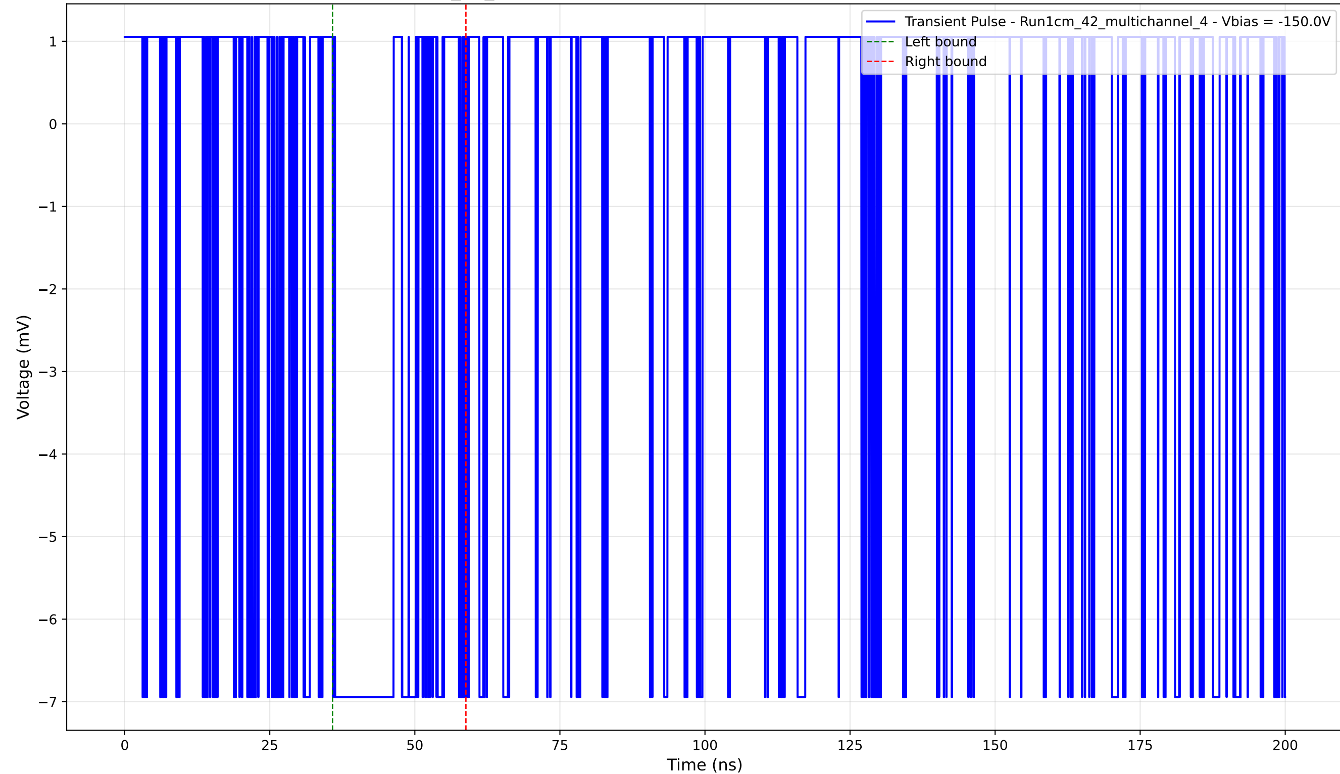
Transient Pulse - Sample: 1cm_42_multichannel - Position: 1410.0 \mu\text{m} - Charge: 1.91 pC - Rise Time: 0.00 ns (N/A)
