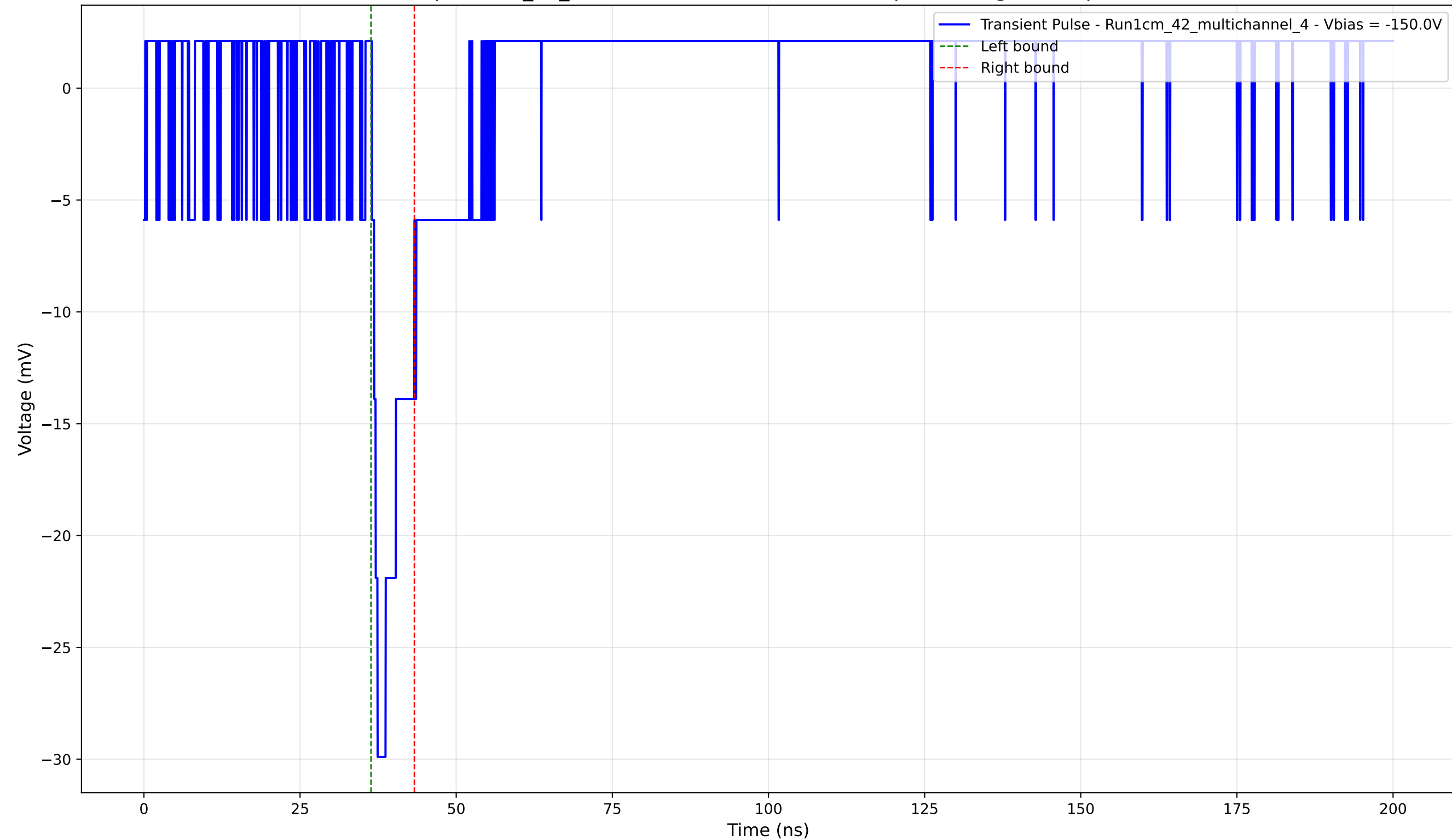
Transient Pulse - Sample: 1cm_42_multichannel - Position: 1570.0 \mu\text{m} - Charge: 2.55 pC - Rise Time: 0.92 ns
