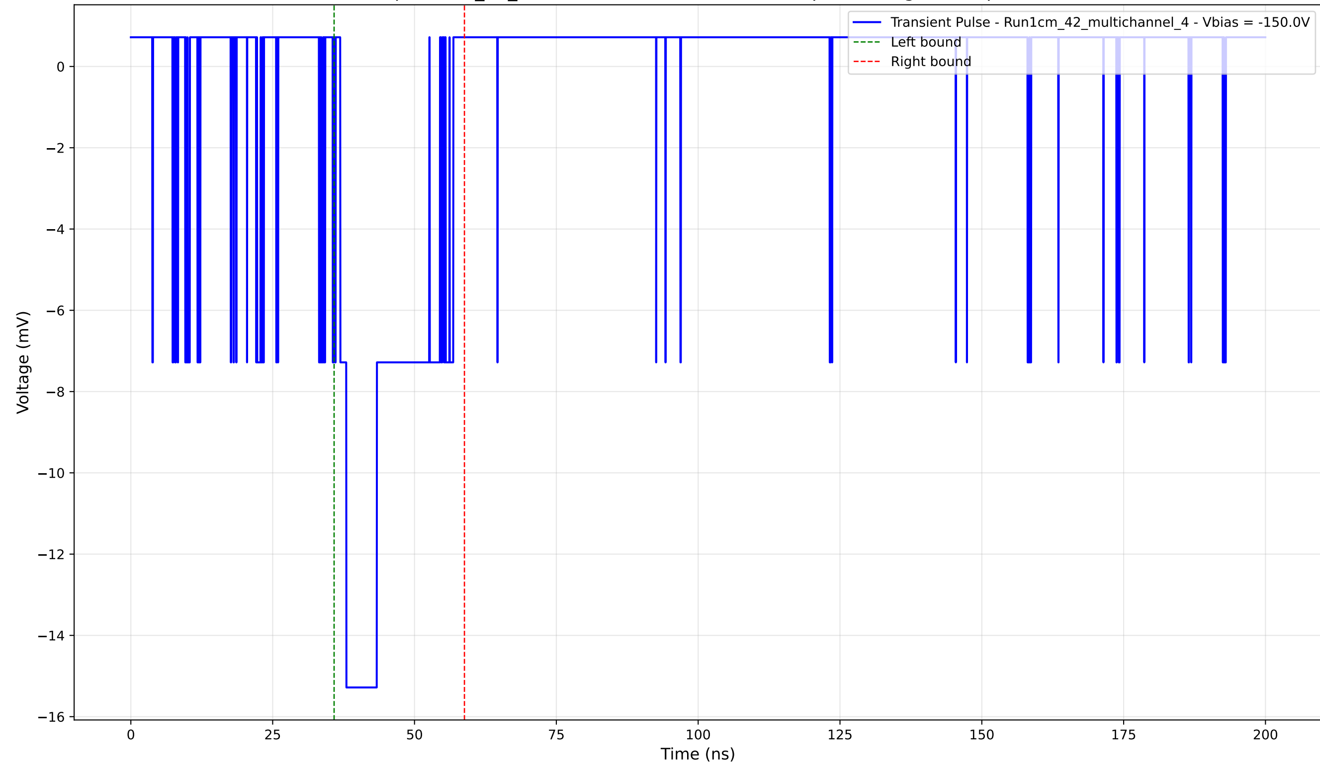
Transient Pulse - Sample: 1cm_42_multichannel - Position: 4075.0 \mu\text{m} - Charge: 3.62 pC - Rise Time: 1.08 ns
