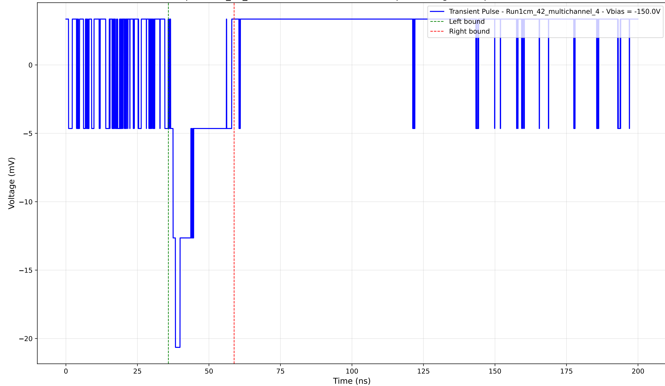
Transient Pulse - Sample: 1cm_42_multichannel - Position: 1025.0 \mu\text{m} - Charge: 3.27 pC - Rise Time: 0.00 ns (N/A)
