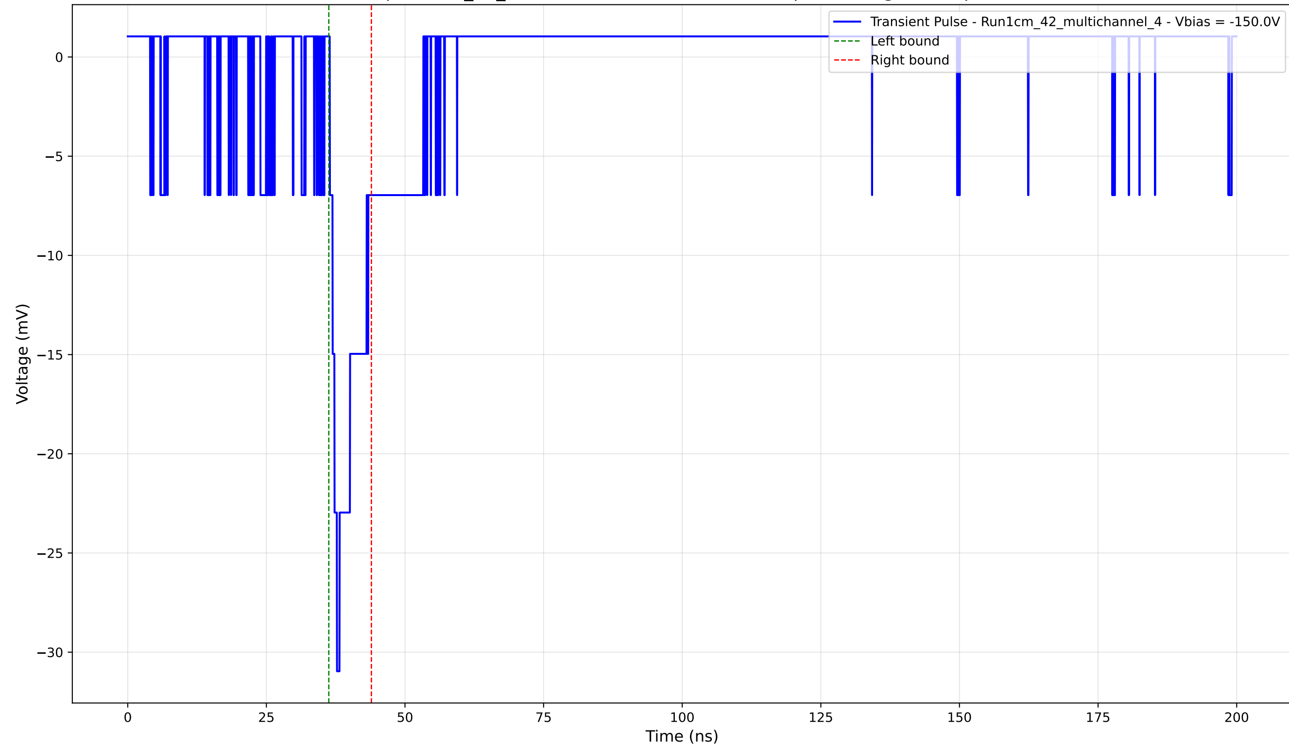
Transient Pulse - Sample: 1cm_42_multichannel - Position: 3290.0 \mu\text{m} - Charge: 2.57 pC - Rise Time: 1.29 ns
