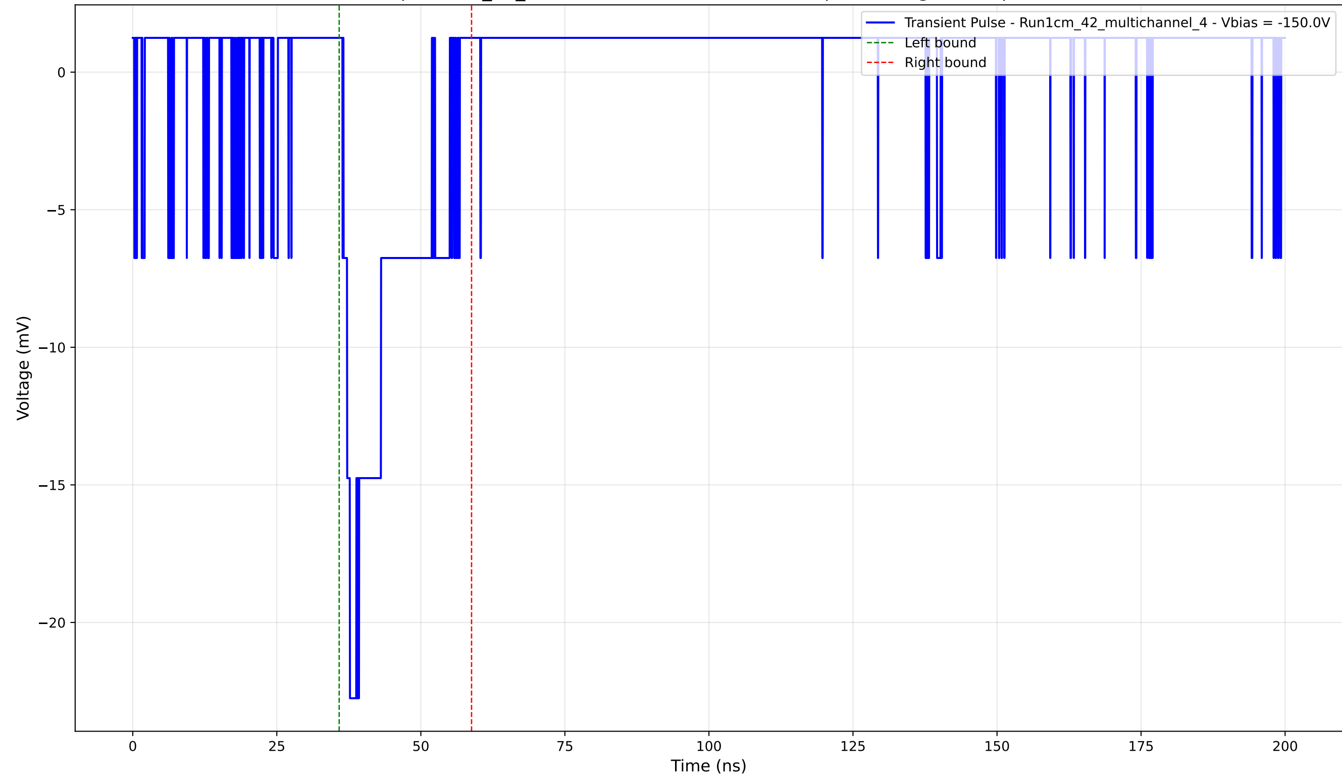
Transient Pulse - Sample: 1cm_42_multichannel - Position: 3500.0 \mu\text{m} - Charge: 3.61 pC - Rise Time: 1.12 ns
