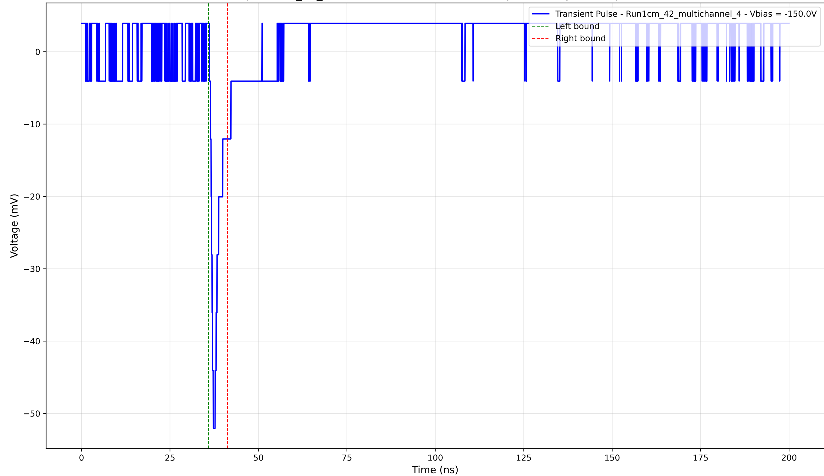
Transient Pulse - Sample: 1cm_42_multichannel - Position: 1990.0 \mu\text{m} - Charge: 2.48 pC - Rise Time: 0.78 ns
