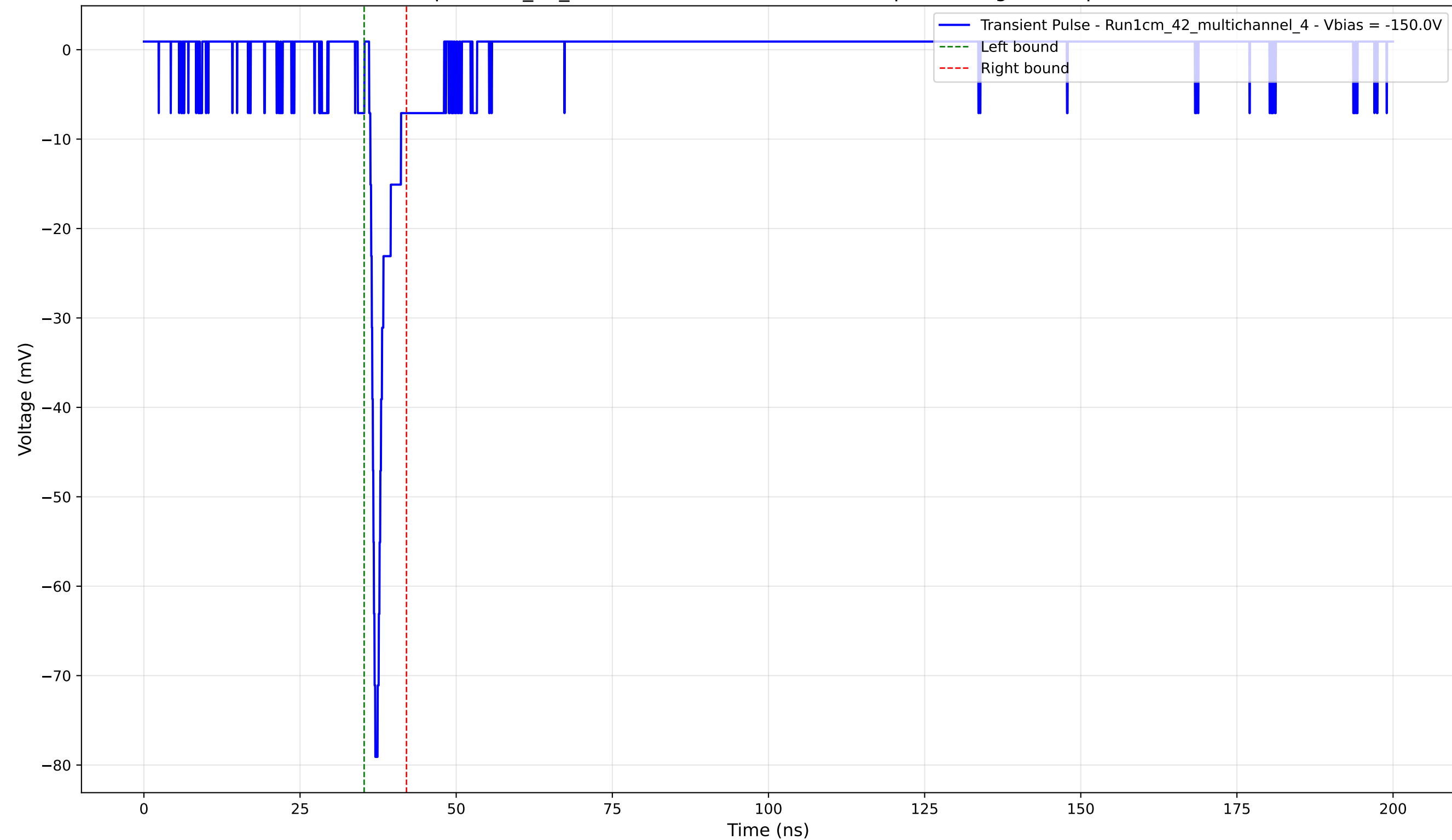
Transient Pulse - Sample: 1cm_42_multichannel - Position: 2305.0 \mu\text{m} - Charge: 3.37 pC - Rise Time: 0.80 ns
