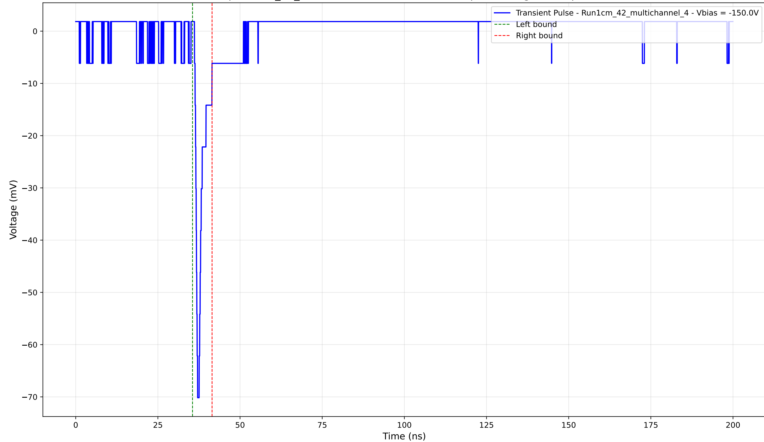
Transient Pulse - Sample: 1cm_42_multichannel - Position: 2565.0 \mu\text{m} - Charge: 3.09 pC - Rise Time: 0.78 ns
