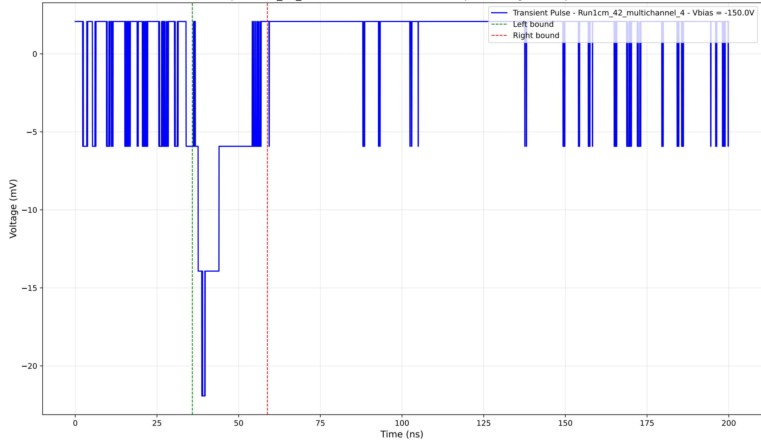
Transient Pulse - Sample: 1cm_42_multichannel - Position: 965.0 \mu\text{m} - Charge: 3.40 pC - Rise Time: 2.00 ns
