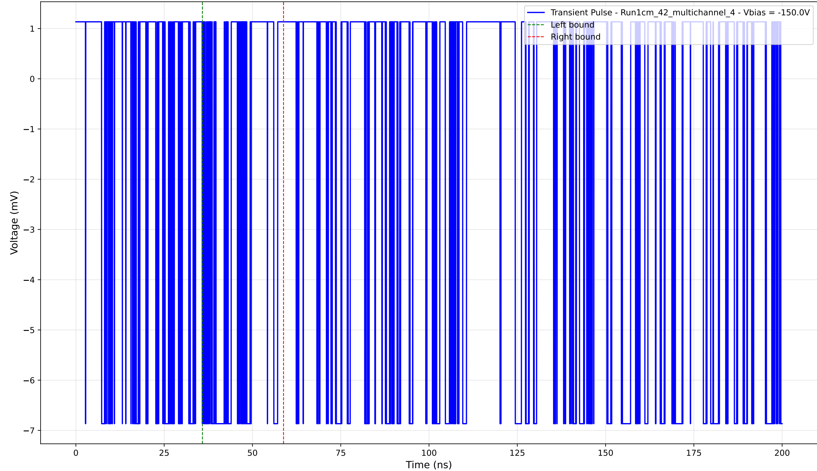
Transient Pulse - Sample: 1cm_42_multichannel - Position: 350.0 \mu\text{m} - Charge: 1.00 pC - Rise Time: 0.00 ns (N/A)
