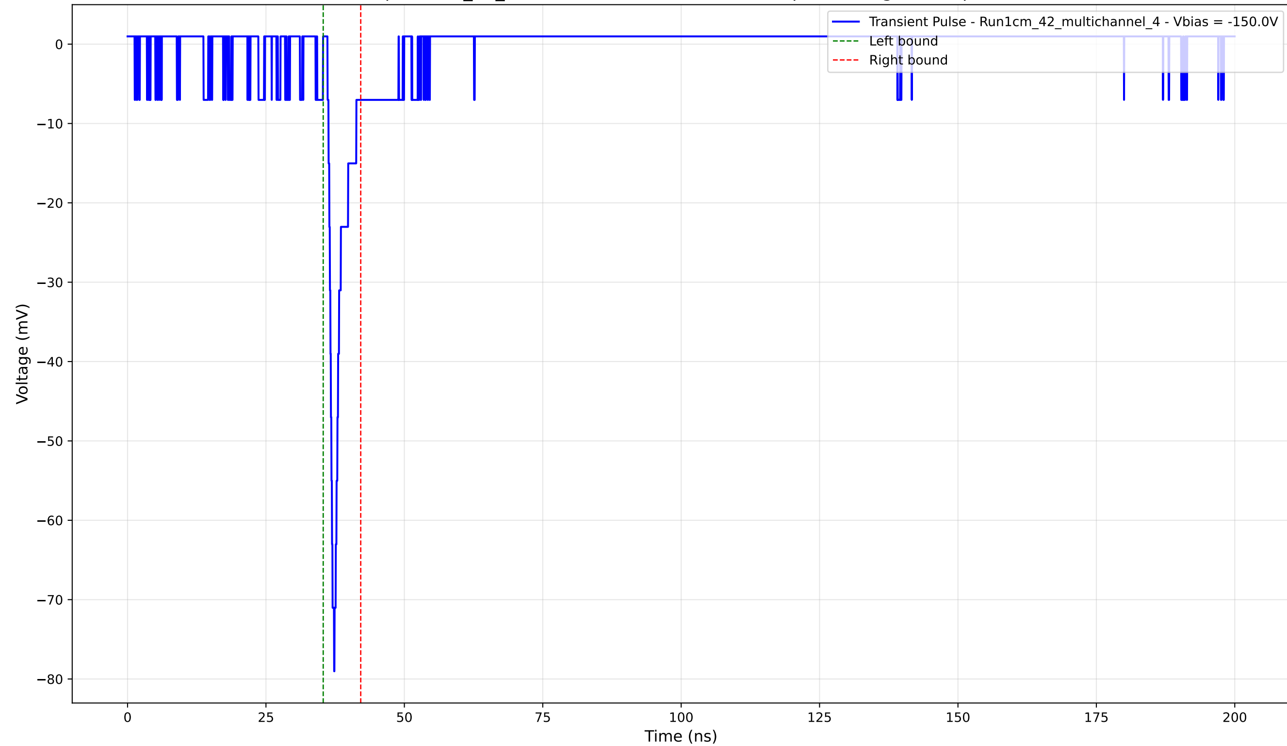
Transient Pulse - Sample: 1cm_42_multichannel - Position: 2215.0 \mu\text{m} - Charge: 3.36 pC - Rise Time: 1.02 ns
