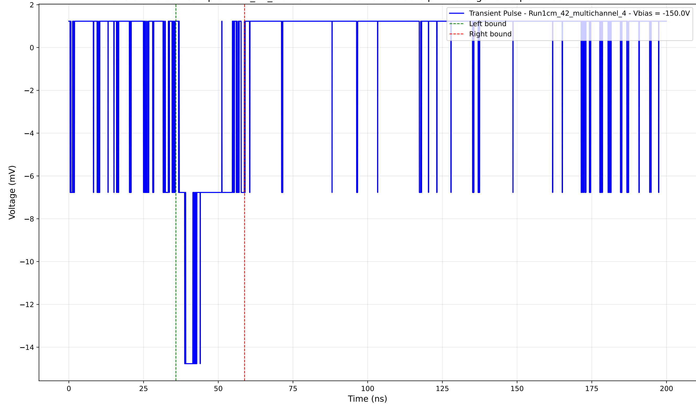
Transient Pulse - Sample: 1cm_42_multichannel - Position: 4480.0 \mu\text{m} - Charge: 3.18 pC - Rise Time: 1.84 ns
