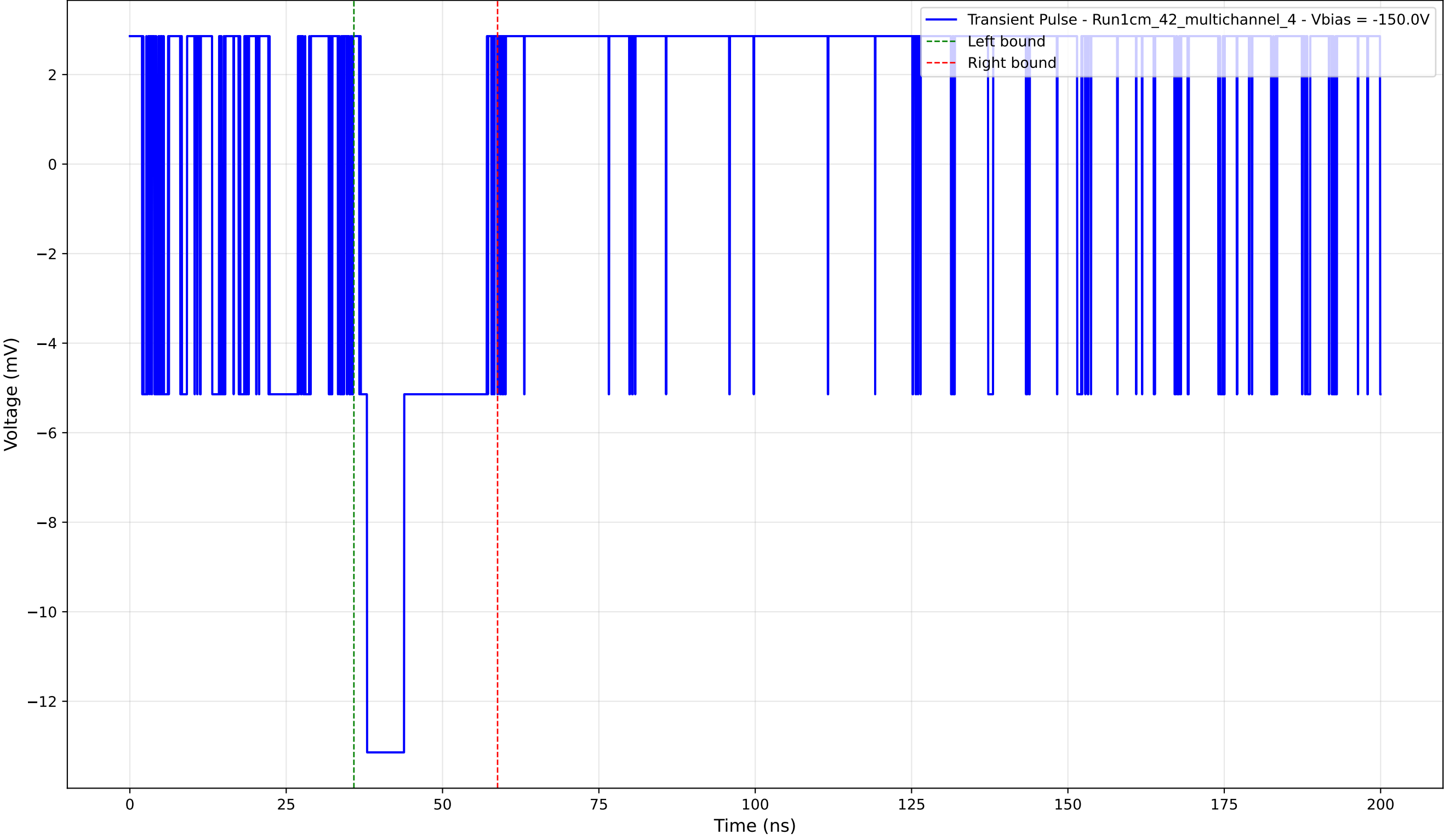
Transient Pulse - Sample: 1cm_42_multichannel - Position: 565.0 \mu\text{m} - Charge: 2.93 pC - Rise Time: 0.00 ns (N/A)
