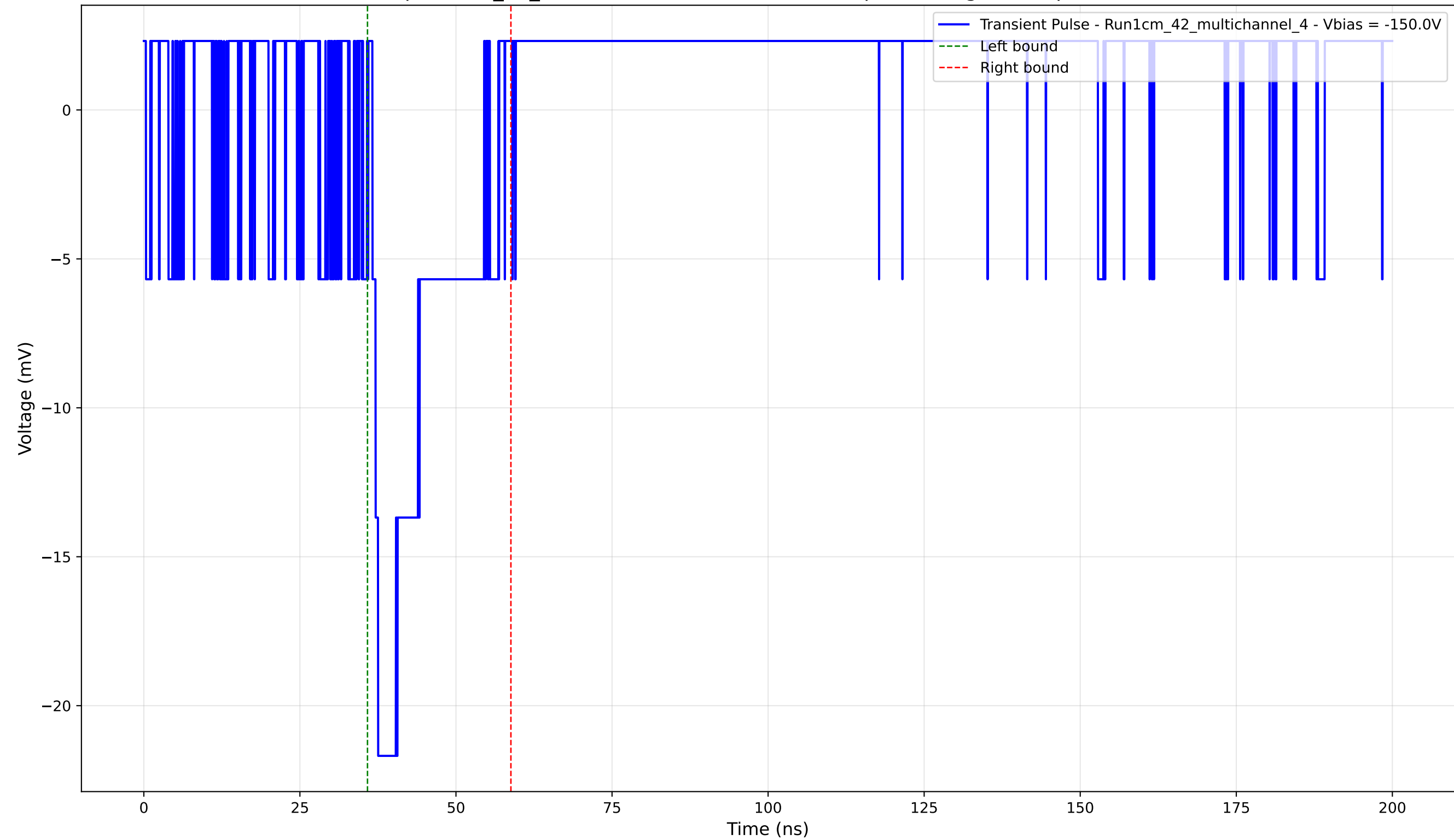
Transient Pulse - Sample: 1cm_42_multichannel - Position: 1275.0 \mu\text{m} - Charge: 3.70 pC - Rise Time: 0.00 ns (N/A)
