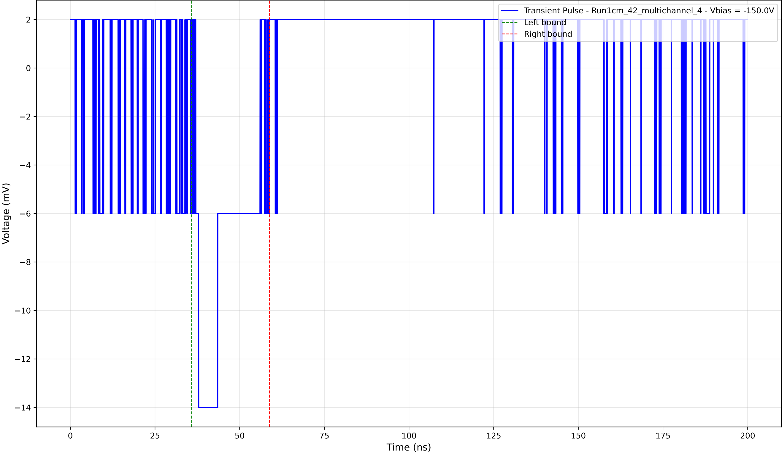
Transient Pulse - Sample: 1cm_42_multichannel - Position: 645.0 \mu\text{m} - Charge: 3.25 pC - Rise Time: 0.00 ns (N/A)
