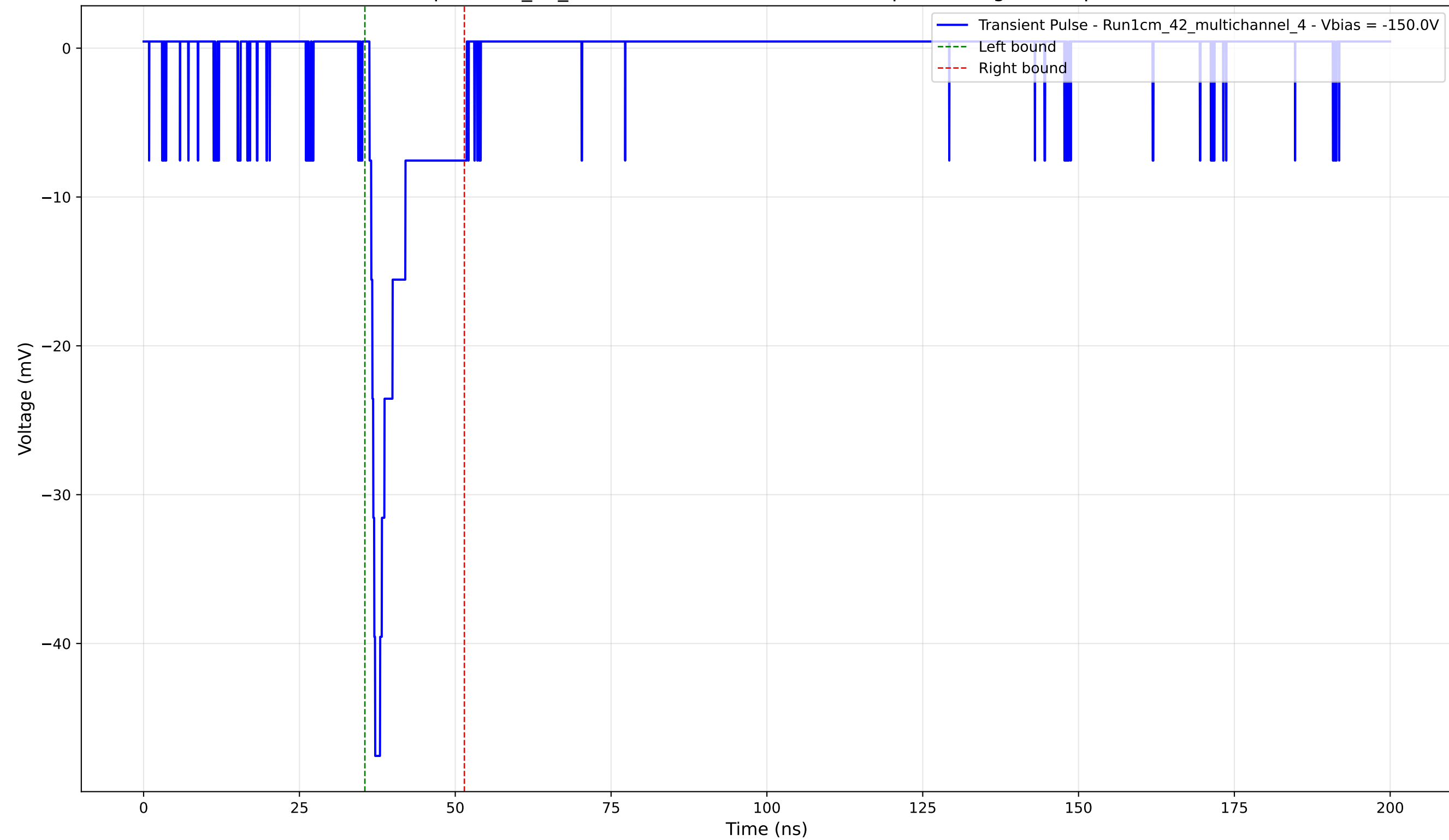
Transient Pulse - Sample: 1cm_42_multichannel - Position: 2810.0 \mu\text{m} - Charge: 4.30 pC - Rise Time: 0.91 ns
