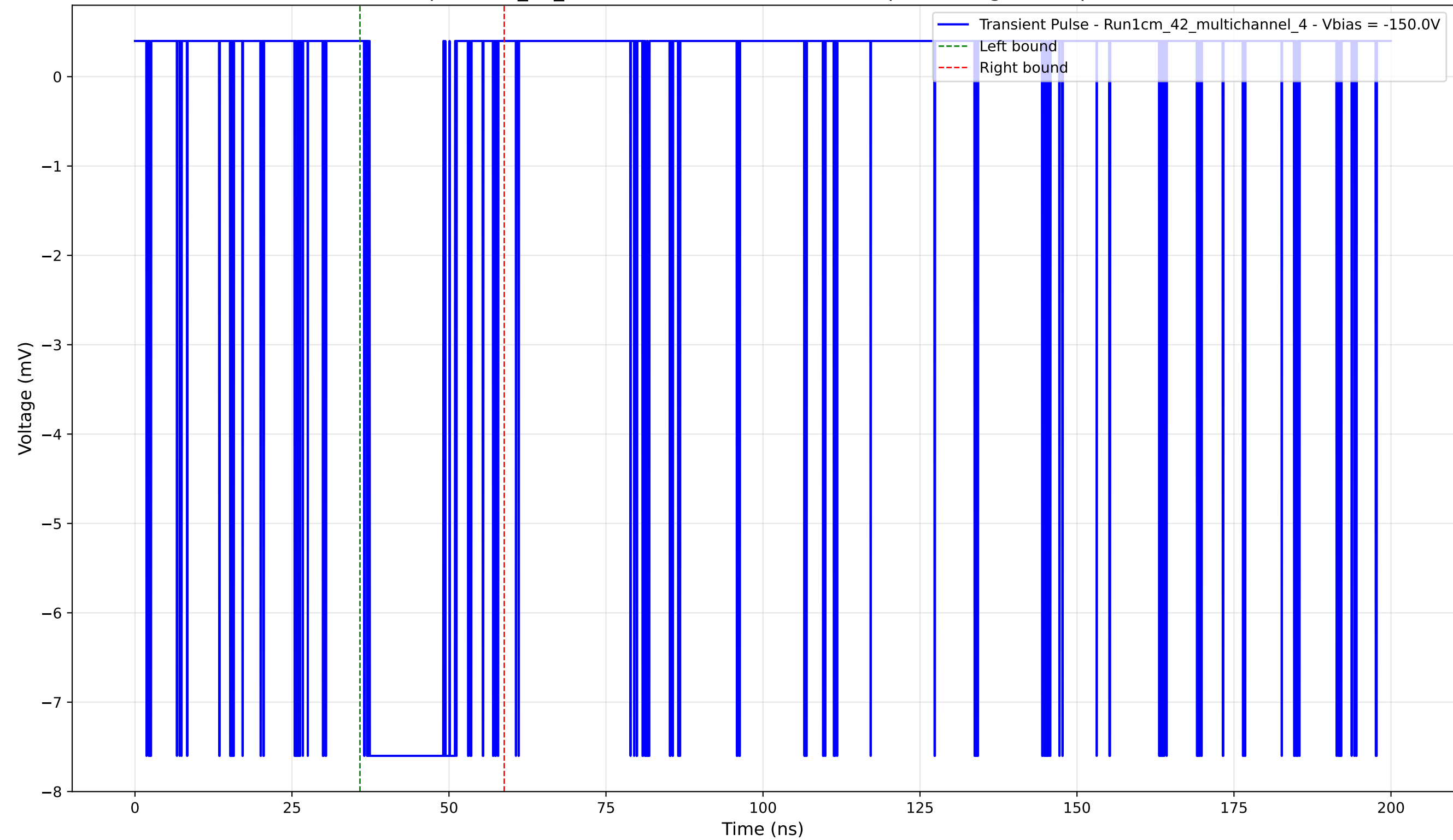
Transient Pulse - Sample: 1cm_42_multichannel - Position: 4445.0 \mu\text{m} - Charge: 2.15 pC - Rise Time: 0.02 ns
