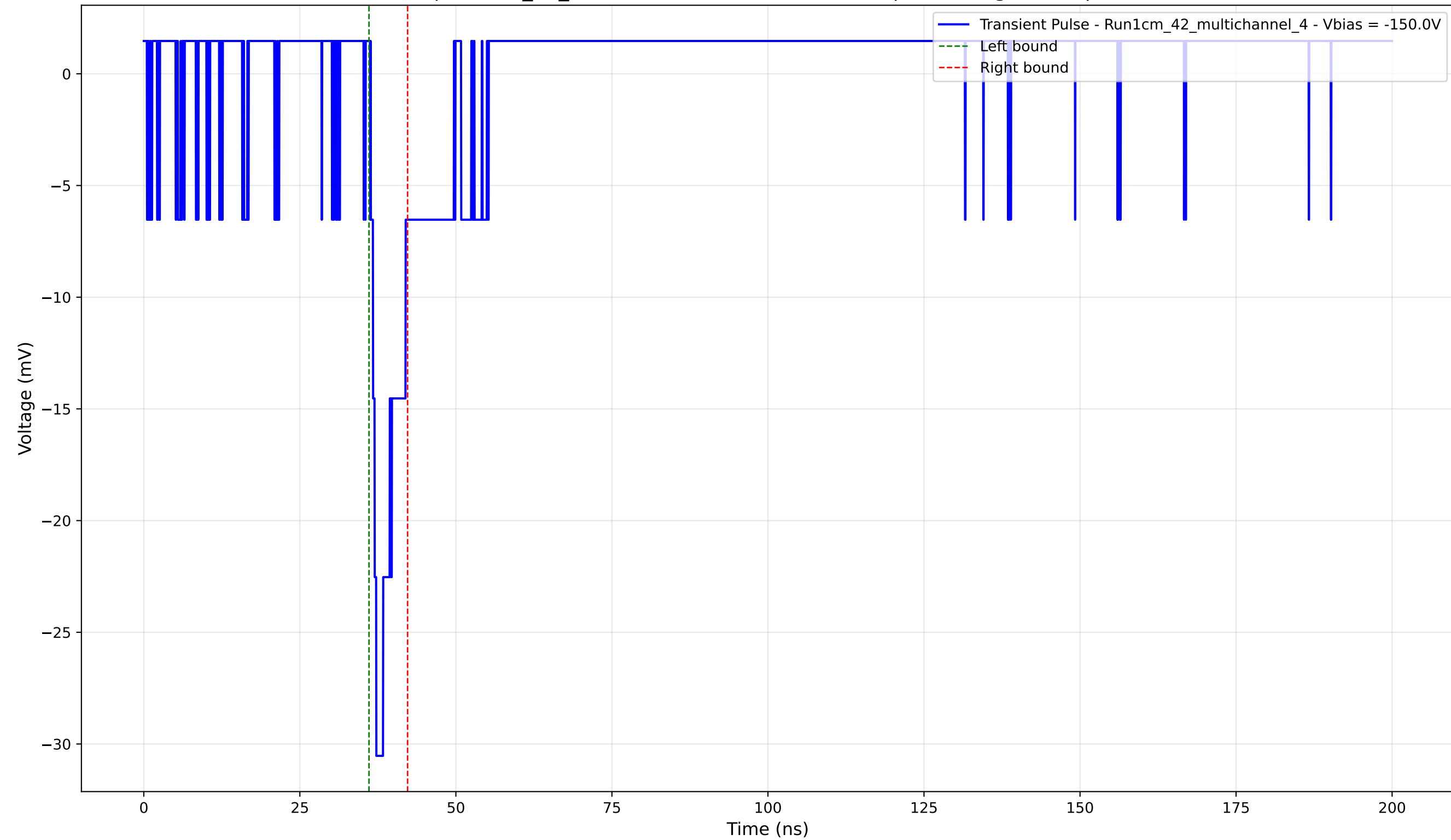
Transient Pulse - Sample: 1cm_42_multichannel - Position: 3070.0 \mu\text{m} - Charge: 2.19 pC - Rise Time: 0.89 ns
