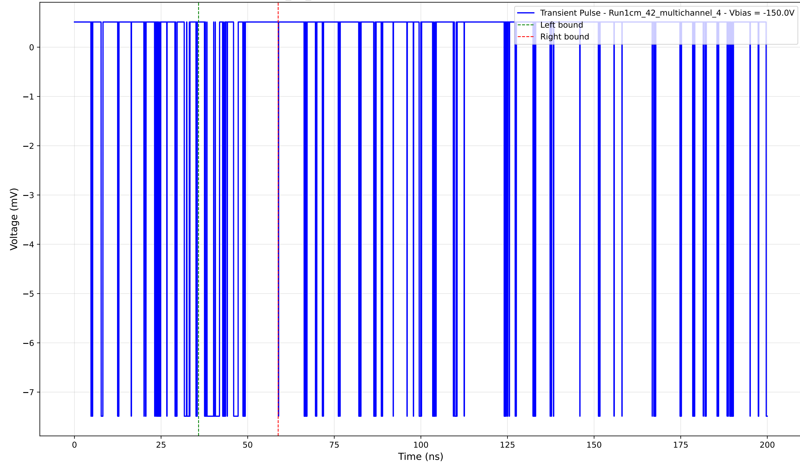
Transient Pulse - Sample: 1cm_42_multichannel - Position: 3930.0 \mu\text{m} - Charge: 0.82 pC - Rise Time: 0.02 ns
