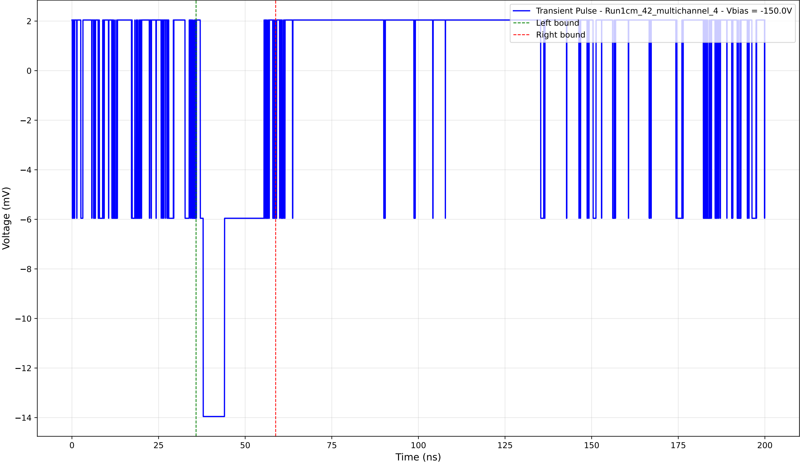
Transient Pulse - Sample: 1cm_42_multichannel - Position: 585.0 \mu\text{m} - Charge: 3.19 pC - Rise Time: 0.00 ns (N/A)
