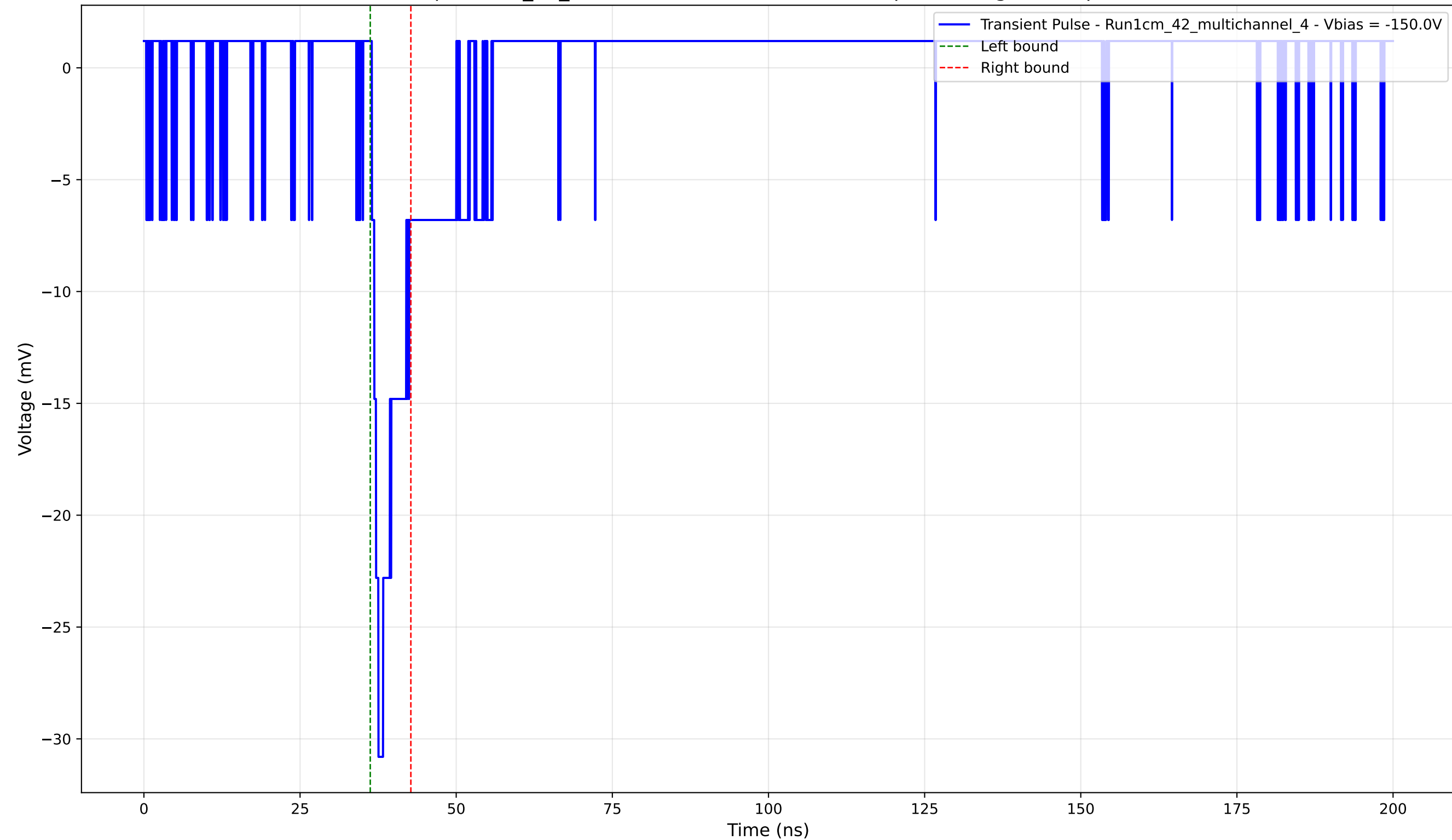
Transient Pulse - Sample: 1cm_42_multichannel - Position: 3185.0 \mu\text{m} - Charge: 2.19 pC - Rise Time: 1.05 ns
