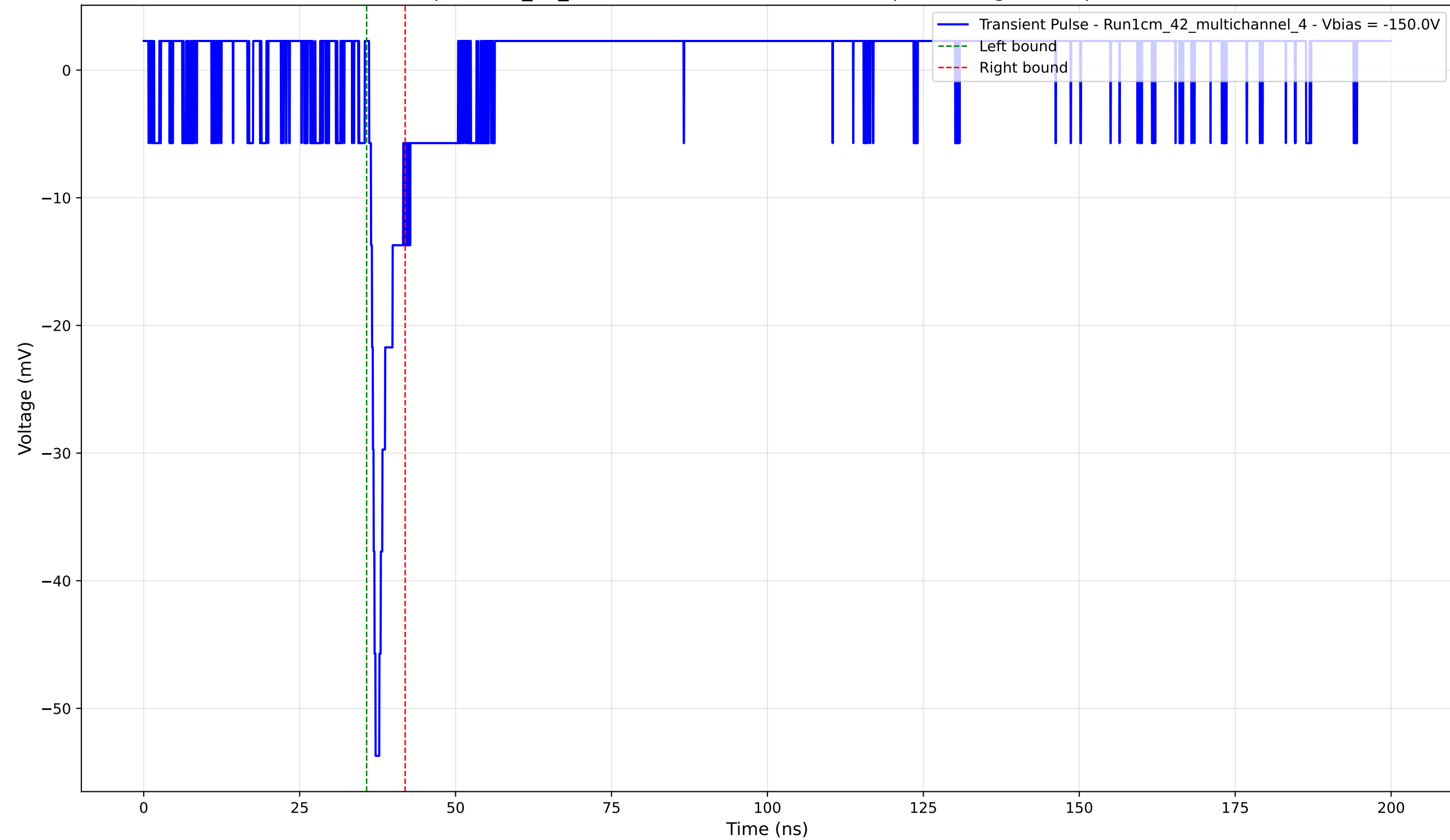
Transient Pulse - Sample: 1cm_42_multichannel - Position: 2730.0 \mu\text{m} - Charge: 2.82 pC - Rise Time: 1.02 ns
