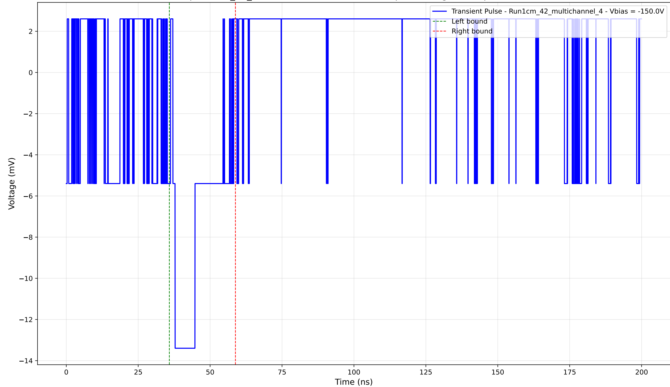
Transient Pulse - Sample: 1cm_42_multichannel - Position: 745.0 \mu\text{m} - Charge: 3.26 pC - Rise Time: 0.00 ns (N/A)
