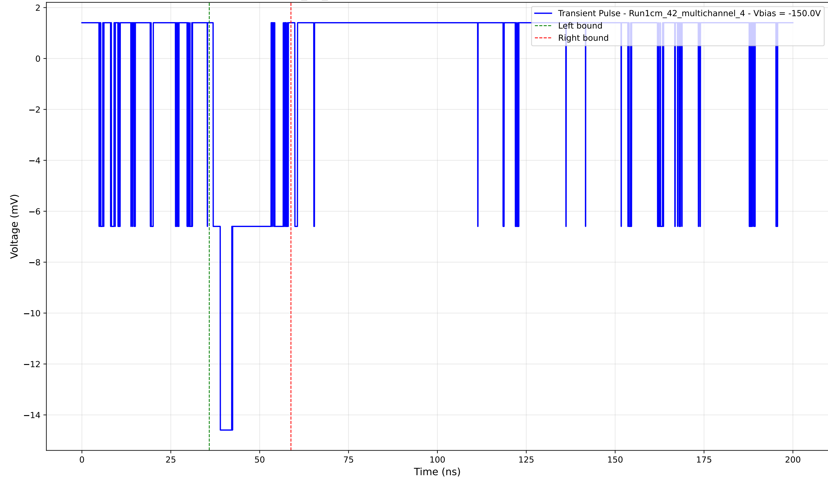
Transient Pulse - Sample: 1cm_42_multichannel - Position: 135.0 \mu\text{m} - Charge: 3.06 pC - Rise Time: 2.02 ns
