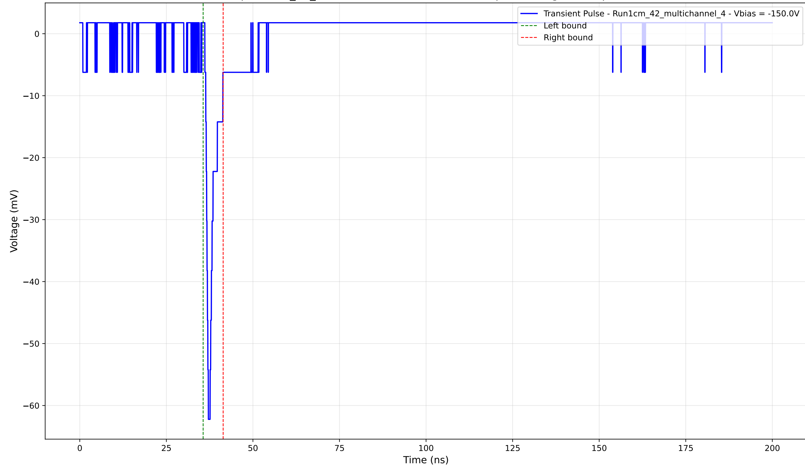
Transient Pulse - Sample: 1cm_42_multichannel - Position: 2155.0 \mu\text{m} - Charge: 2.87 pC - Rise Time: 1.00 ns
