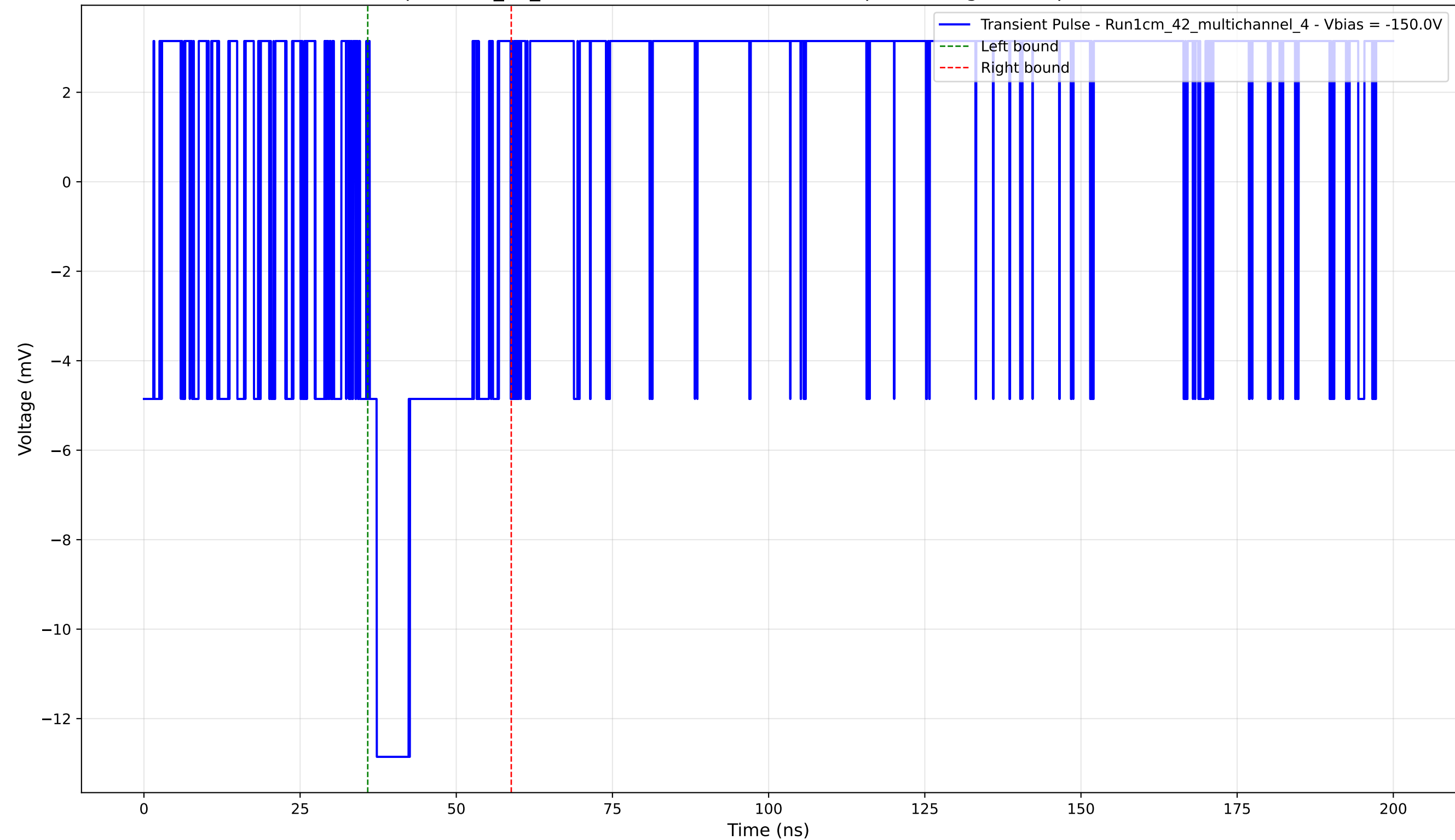
Transient Pulse - Sample: 1cm_42_multichannel - Position: 1315.0 \mu\text{m} - Charge: 2.55 pC - Rise Time: 0.00 ns (N/A)
