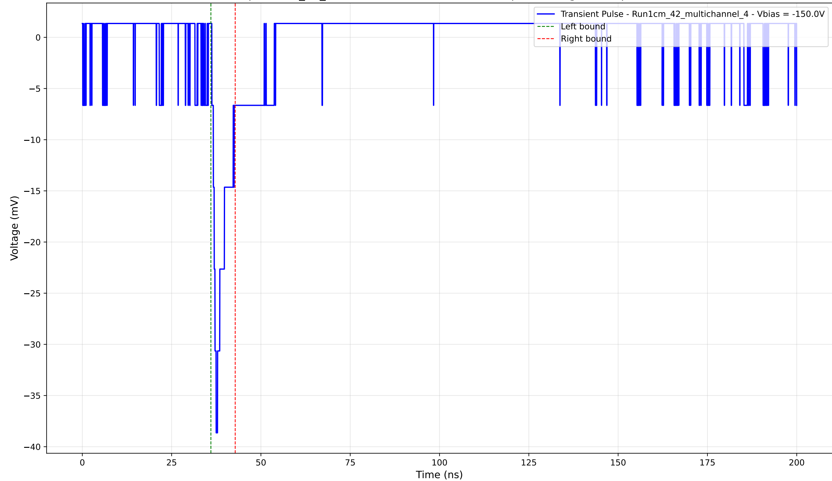
Transient Pulse - Sample: 1cm_42_multichannel - Position: 3030.0 \mu\text{m} - Charge: 2.51 pC - Rise Time: 1.21 ns
