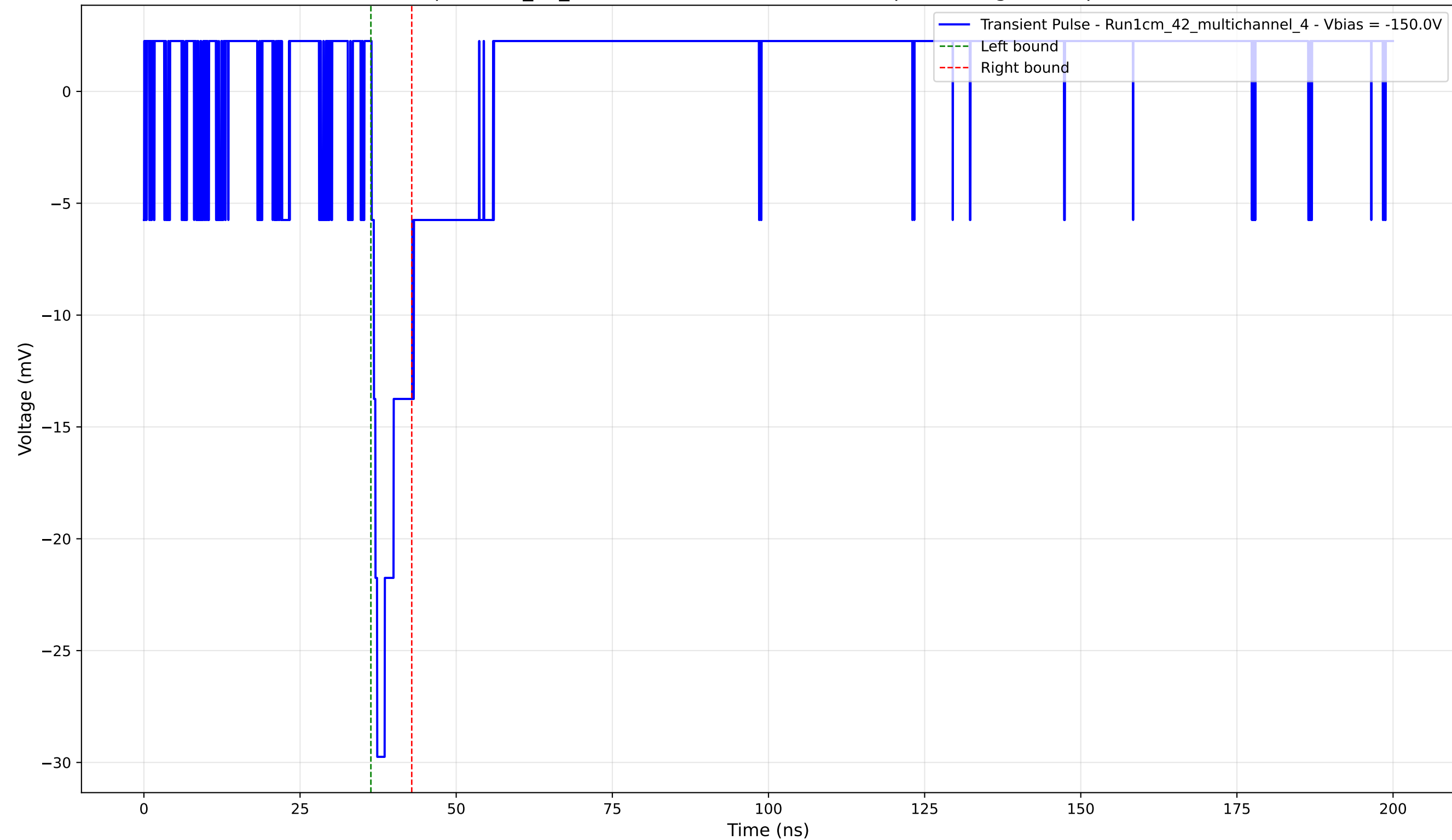
Transient Pulse - Sample: 1cm_42_multichannel - Position: 1630.0 \mu\text{m} - Charge: 2.37 pC - Rise Time: 0.90 ns
