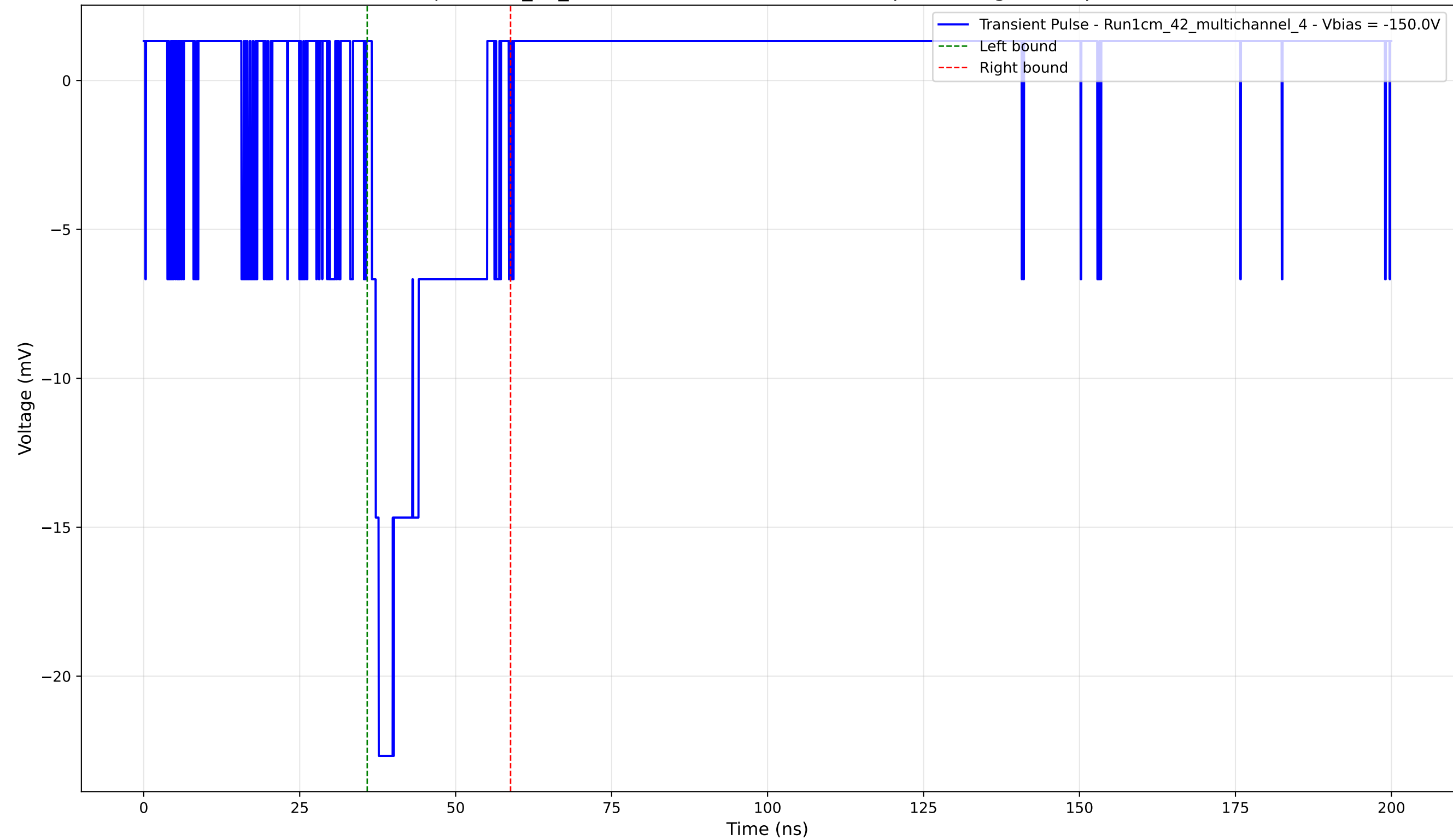
Transient Pulse - Sample: 1cm_42_multichannel - Position: 1295.0 \mu\text{m} - Charge: 3.97 pC - Rise Time: 1.12 ns
