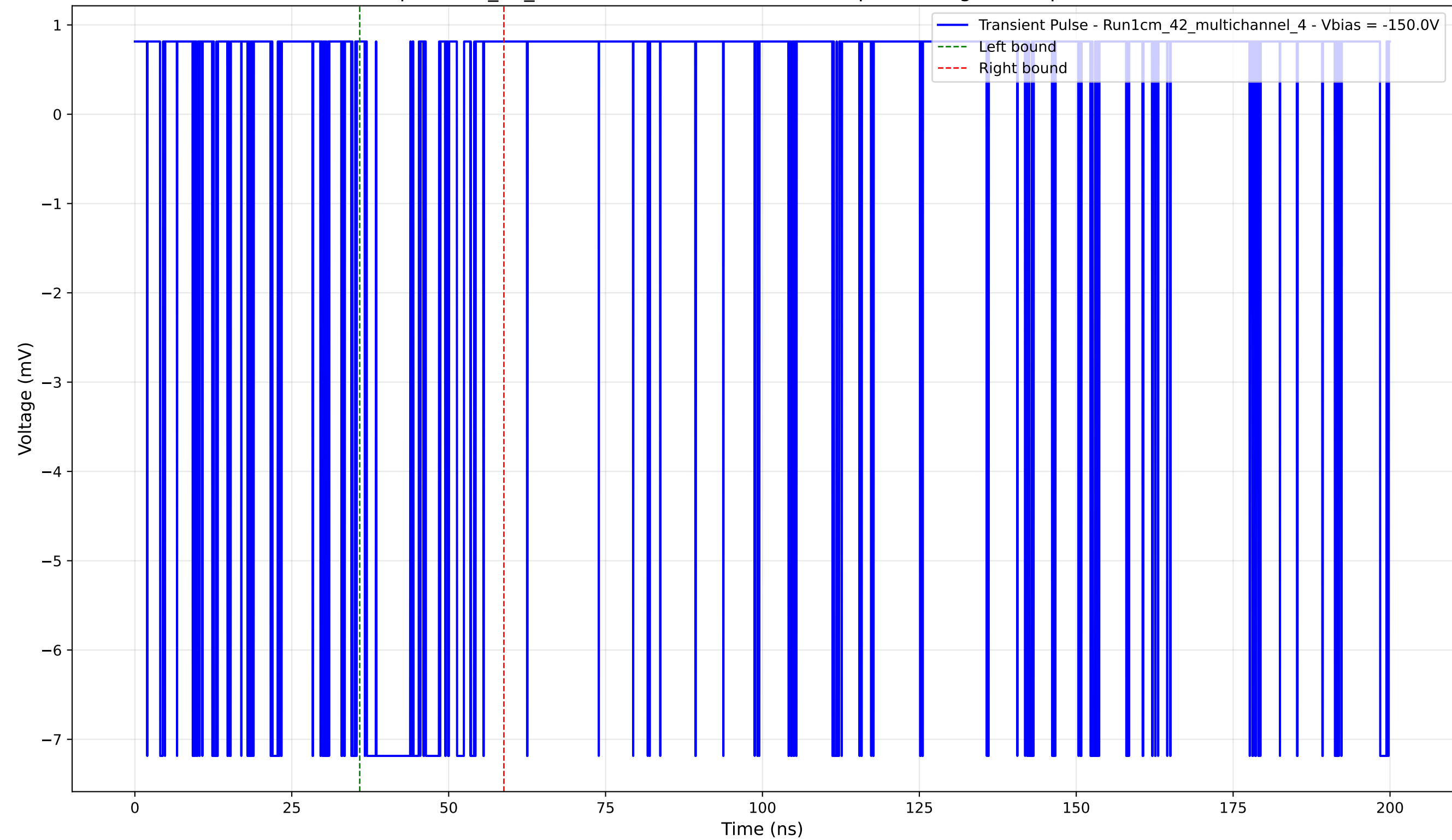
Transient Pulse - Sample: 1cm_42_multichannel - Position: 4365.0 \mu\text{m} - Charge: 1.64 pC - Rise Time: 0.00 ns (N/A)
