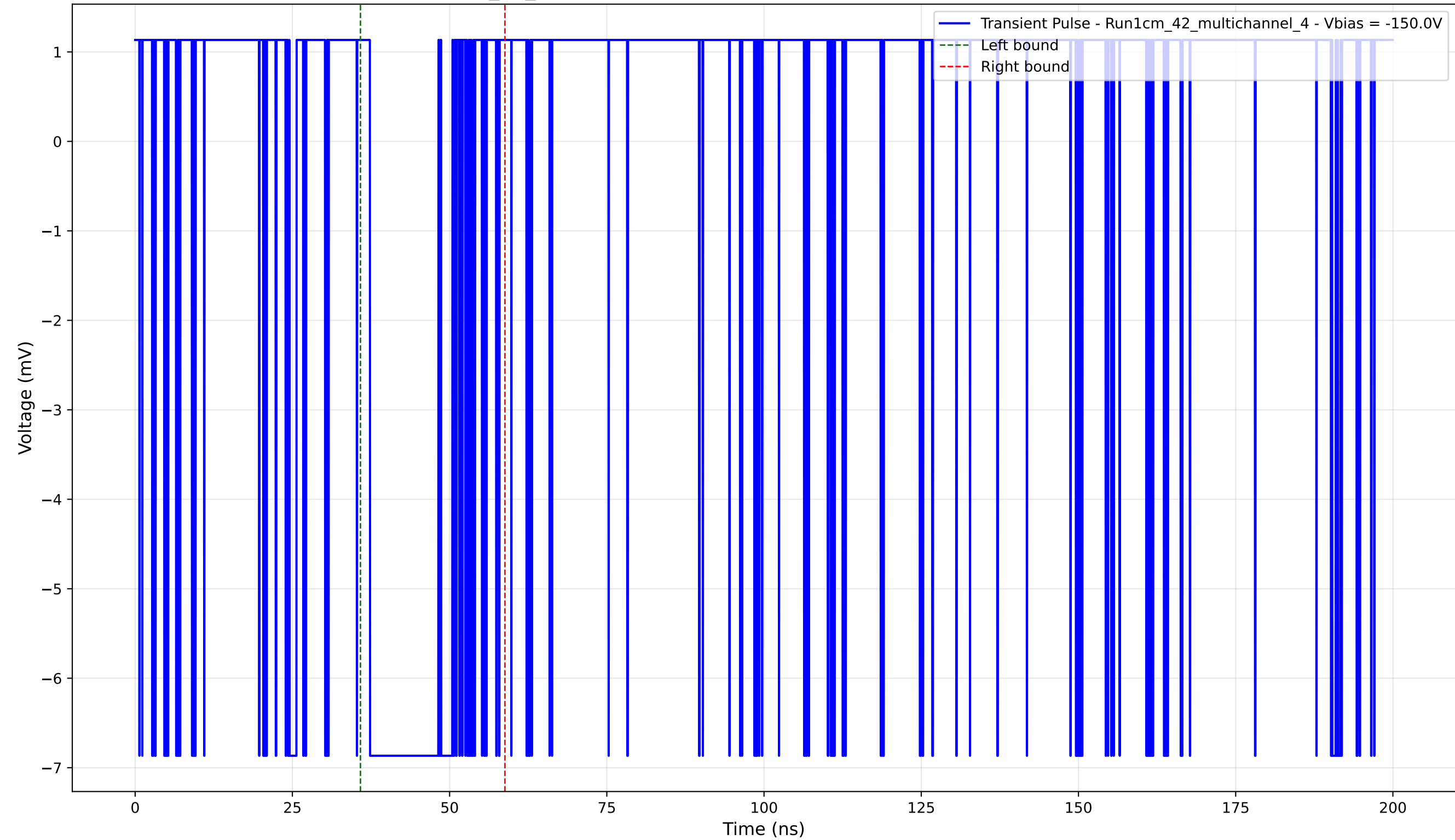
Transient Pulse - Sample: 1cm_42_multichannel - Position: 3945.0 \mu\text{m} - Charge: 1.84 pC - Rise Time: 0.00 ns (N/A)
