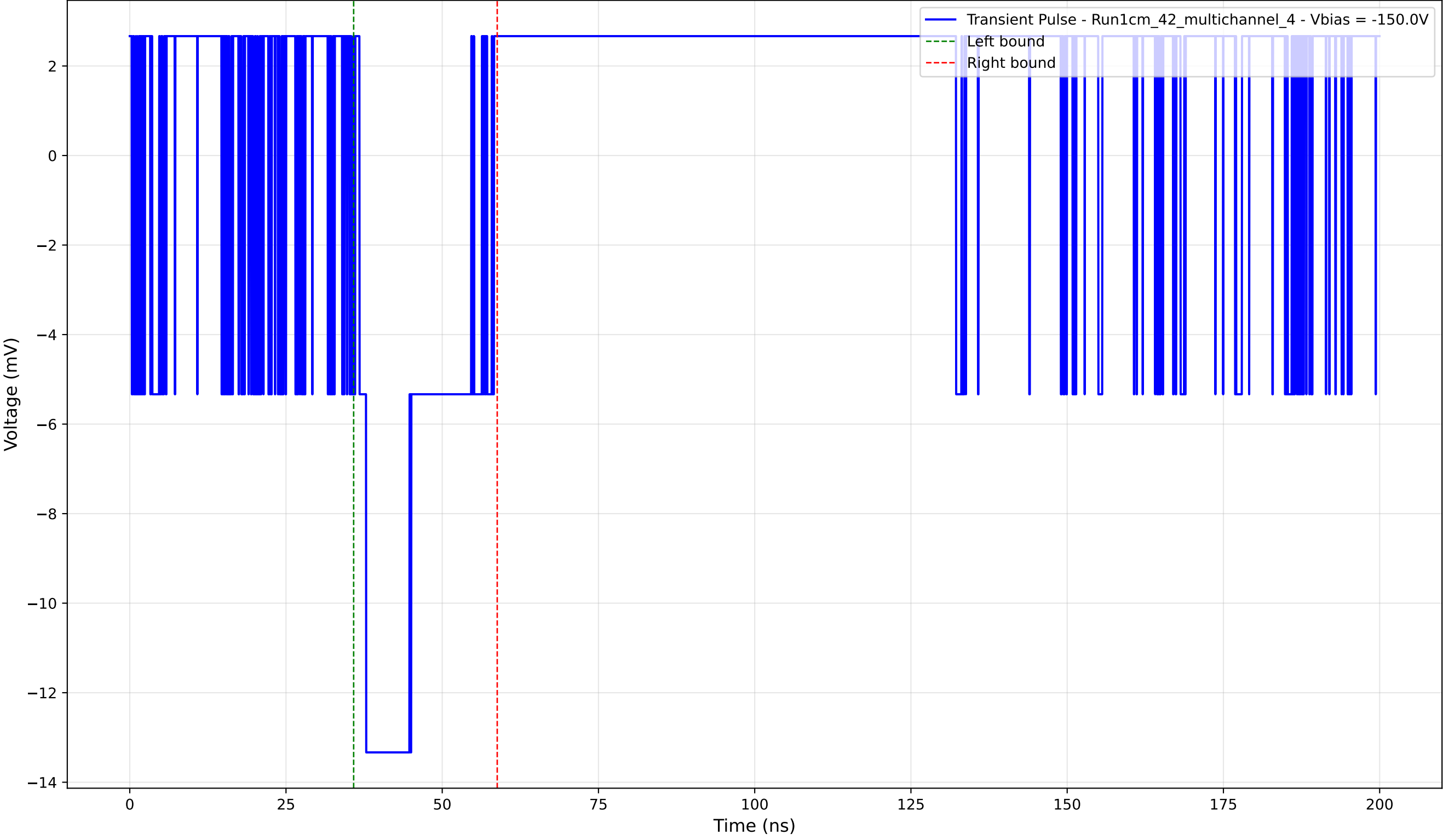
Transient Pulse - Sample: 1cm_42_multichannel - Position: 690.0 \mu\text{m} - Charge: 3.23 pC - Rise Time: 0.00 ns (N/A)
