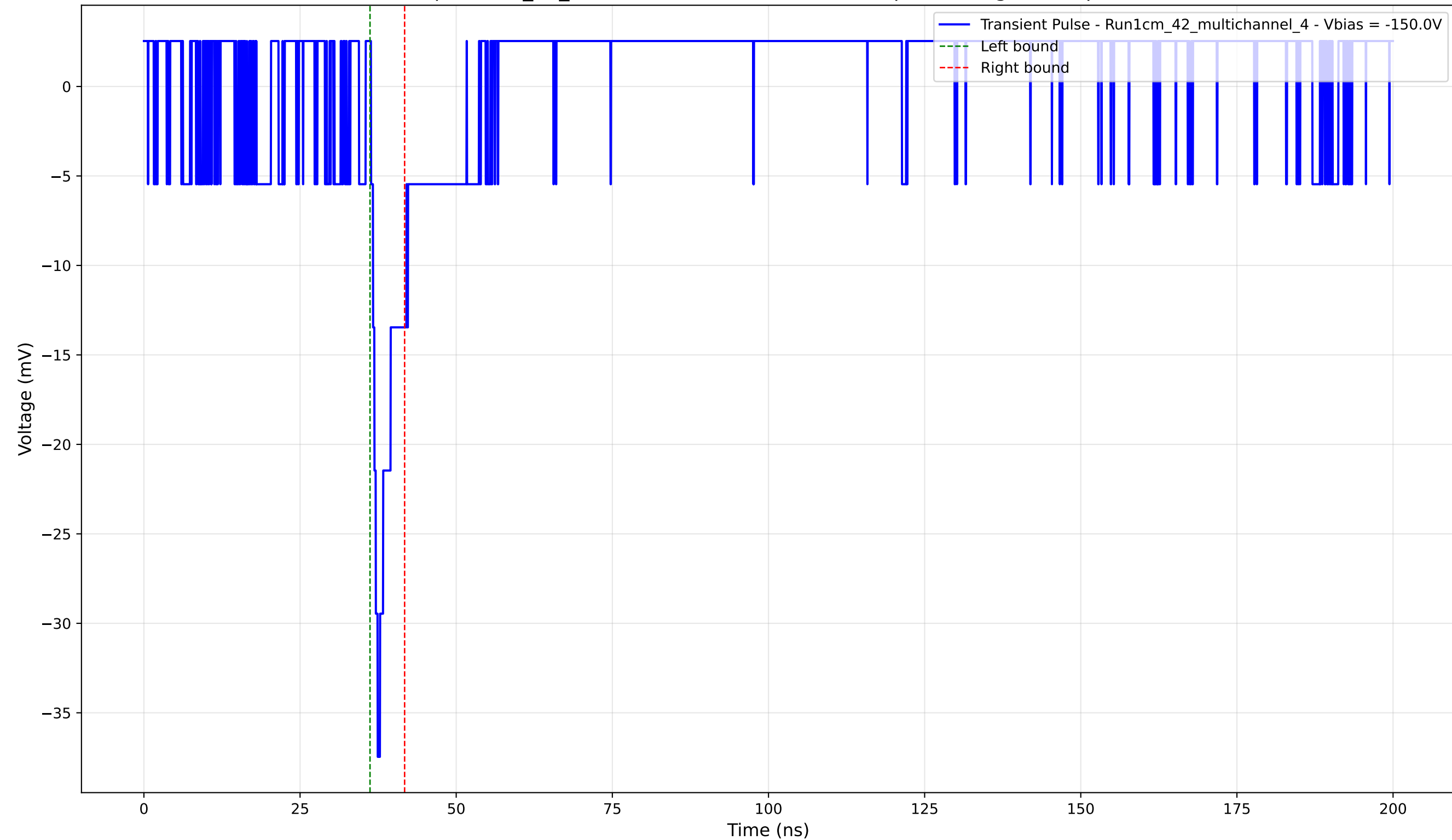
Transient Pulse - Sample: 1cm_42_multichannel - Position: 1815.0 \mu\text{m} - Charge: 2.06 pC - Rise Time: 1.07 ns
