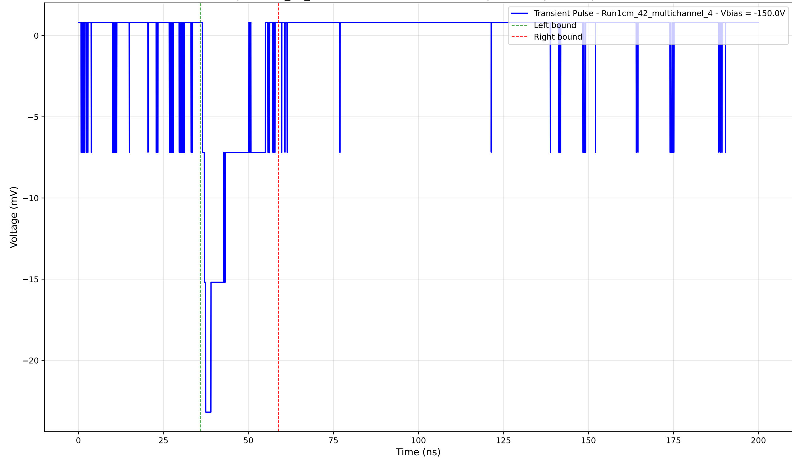
Transient Pulse - Sample: 1cm_42_multichannel - Position: 3320.0 \mu\text{m} - Charge: 3.84 pC - Rise Time: 1.00 ns
