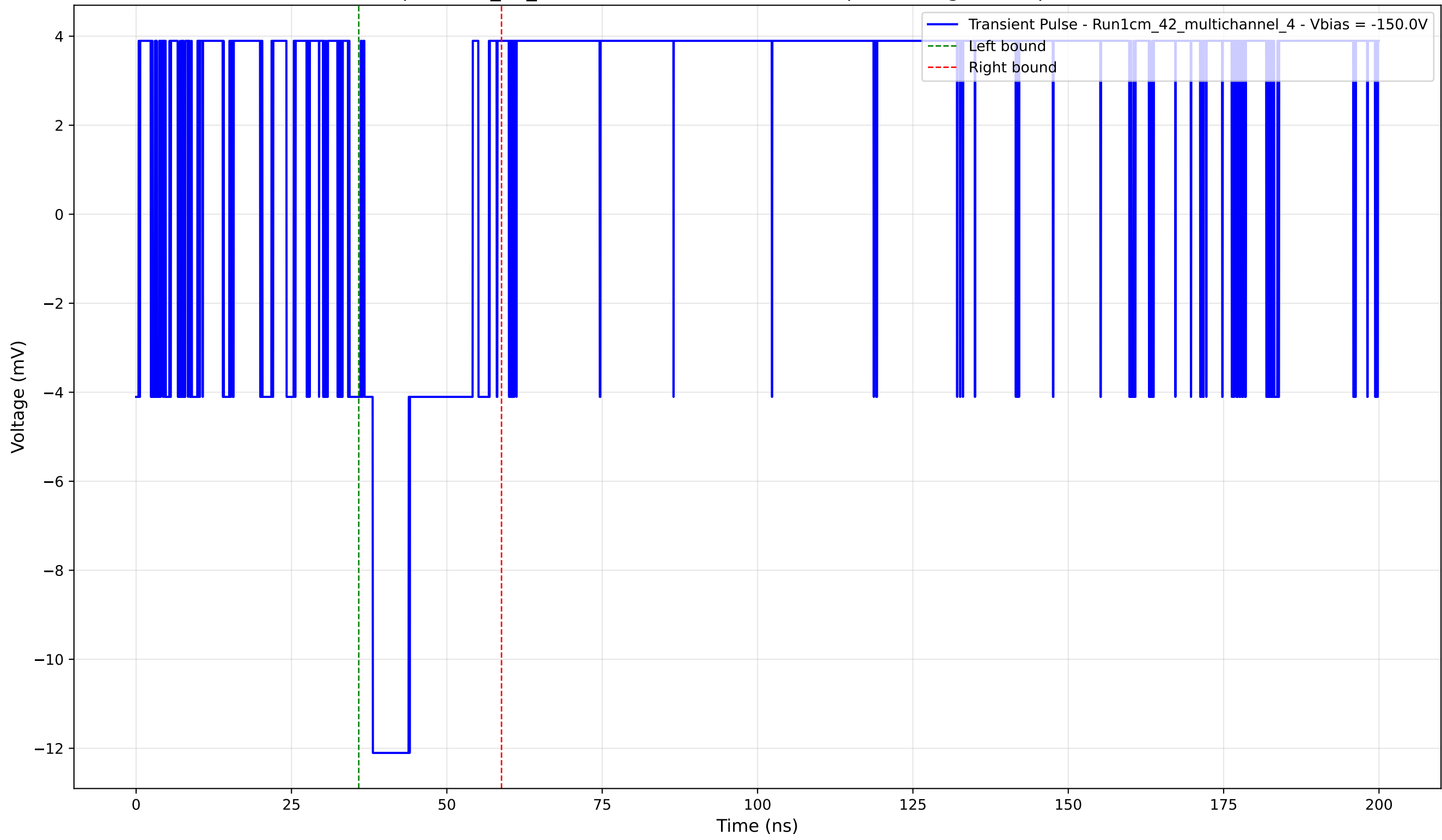
Transient Pulse - Sample: 1cm_42_multichannel - Position: 520.0 \mu\text{m} - Charge: 2.32 pC - Rise Time: 0.00 ns (N/A)
