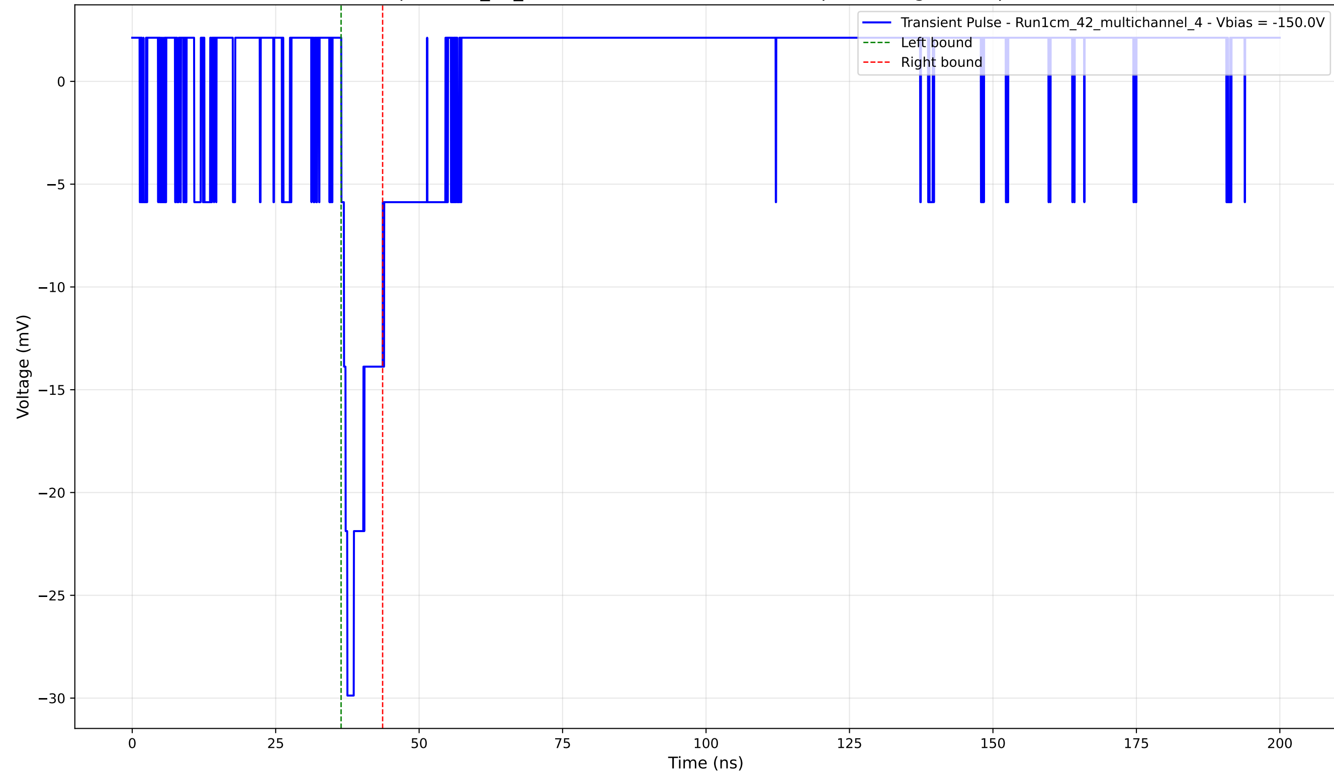
Transient Pulse - Sample: 1cm_42_multichannel - Position: 1510.0 \mu\text{m} - Charge: 2.61 pC - Rise Time: 1.06 ns
