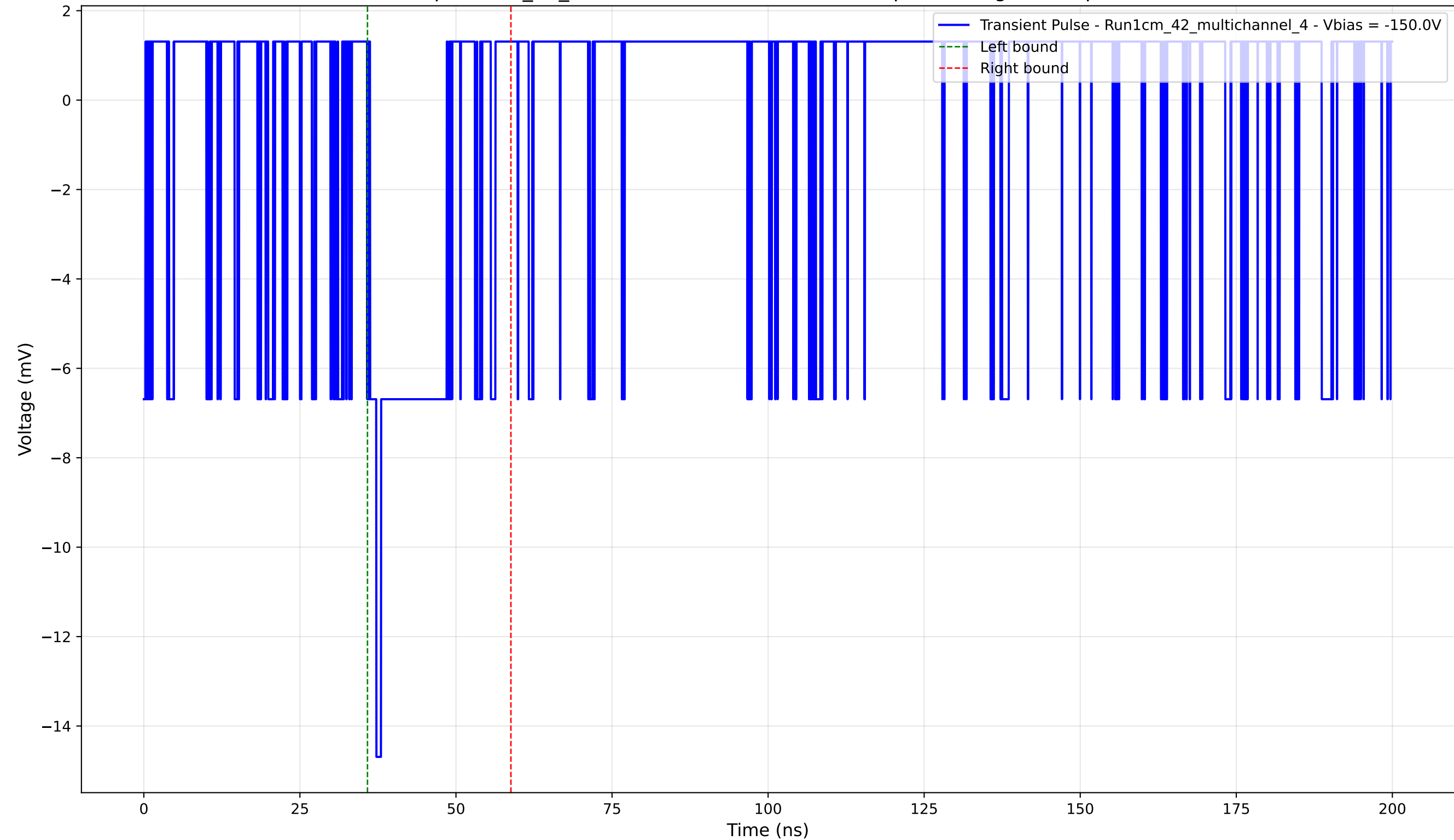
Transient Pulse - Sample: 1cm_42_multichannel - Position: 1840.0 \mu\text{m} - Charge: 1.87 pC - Rise Time: 1.02 ns
