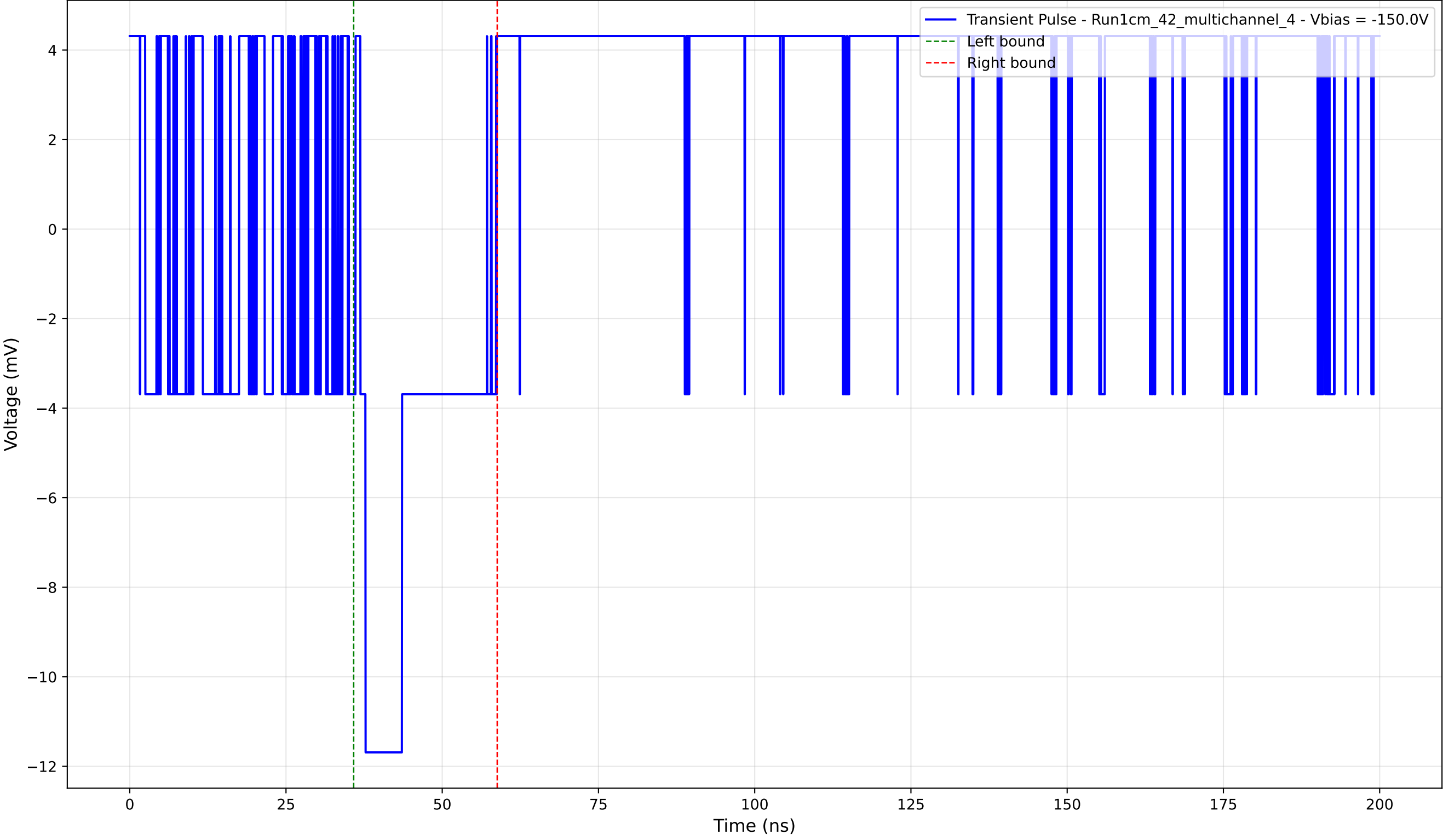
Transient Pulse - Sample: 1cm_42_multichannel - Position: 790.0 \mu\text{m} - Charge: 2.47 pC - Rise Time: 0.00 ns (N/A)
