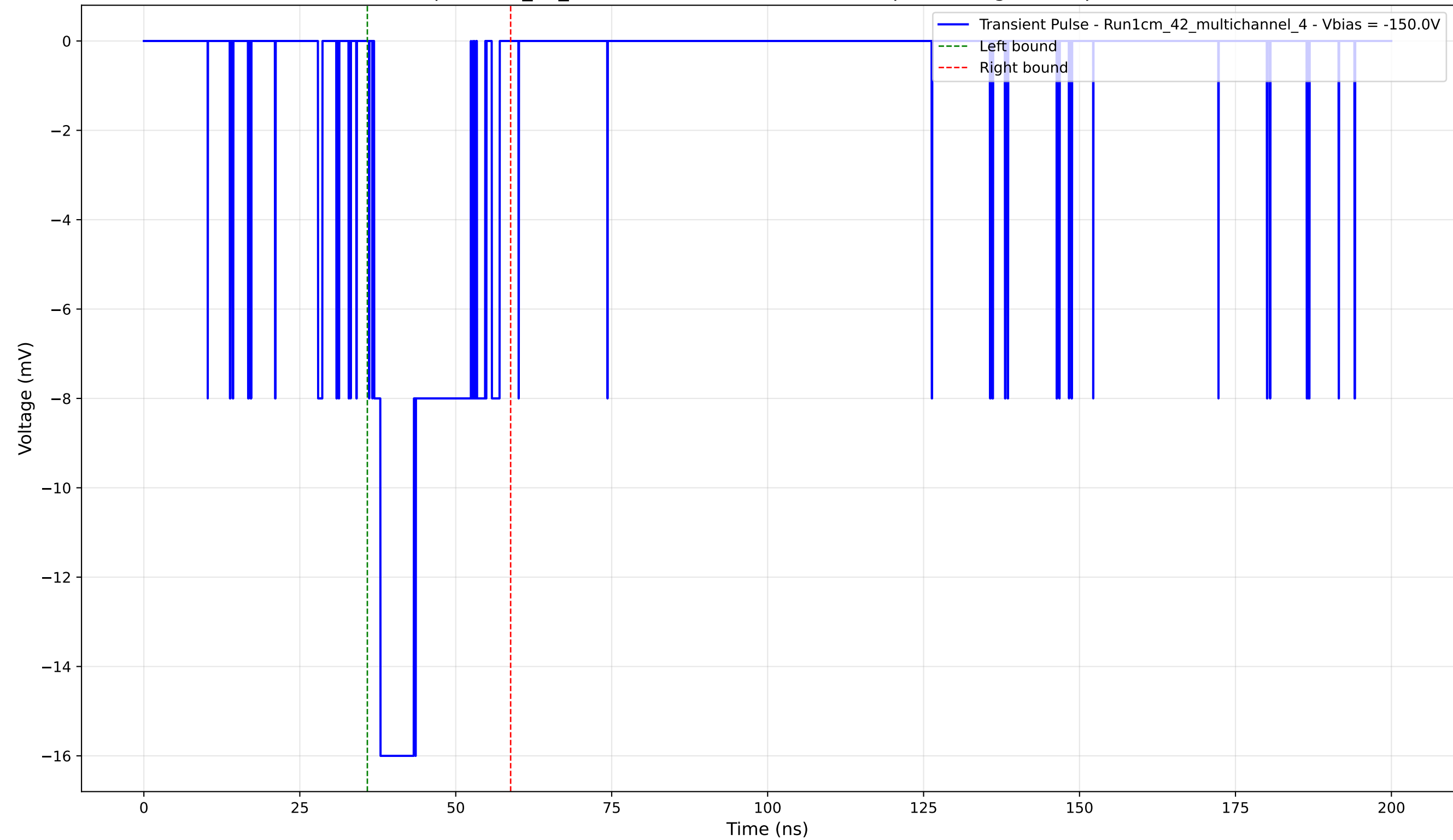
Transient Pulse - Sample: 1cm_42_multichannel - Position: 3985.0 \mu\text{m} - Charge: 3.91 pC - Rise Time: 1.02 ns
