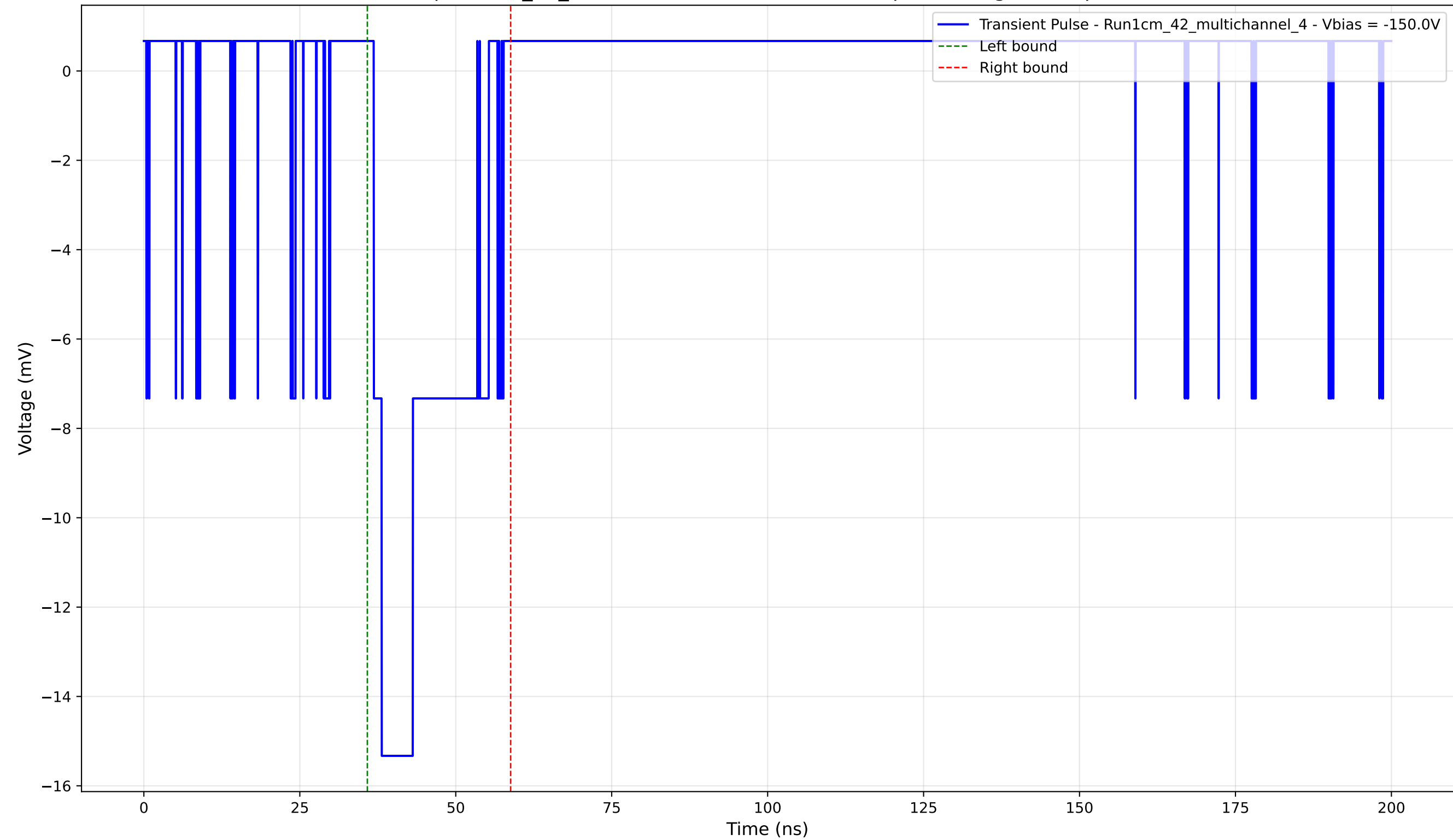
Transient Pulse - Sample: 1cm_42_multichannel - Position: 4025.0 \mu\text{m} - Charge: 3.54 pC - Rise Time: 1.28 ns
