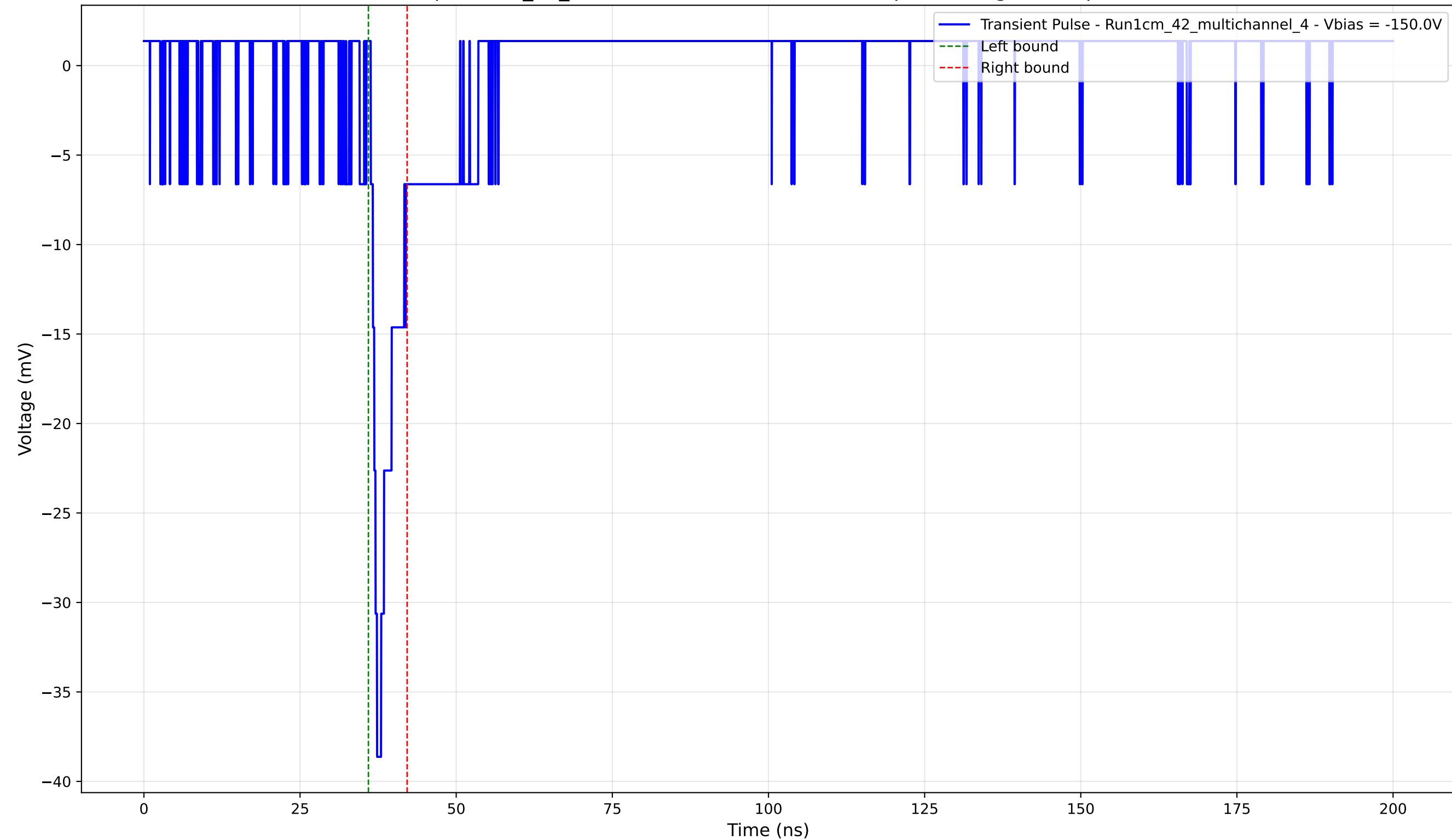
Transient Pulse - Sample: 1cm_42_multichannel - Position: 2970.0 \mu\text{m} - Charge: 2.34 pC - Rise Time: 1.01 ns
