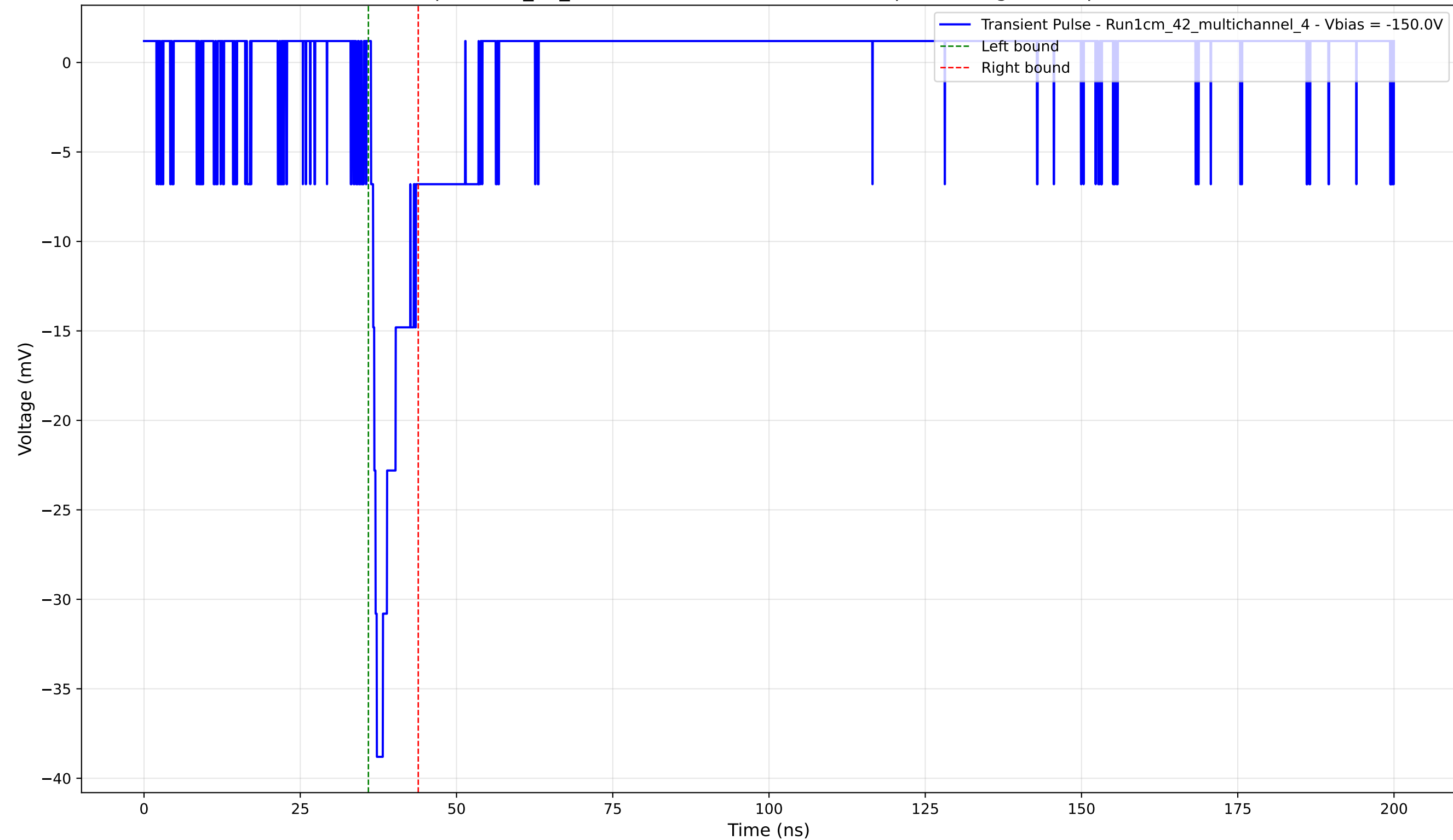
Transient Pulse - Sample: 1cm_42_multichannel - Position: 1760.0 \mu\text{m} - Charge: 3.08 pC - Rise Time: 0.93 ns
