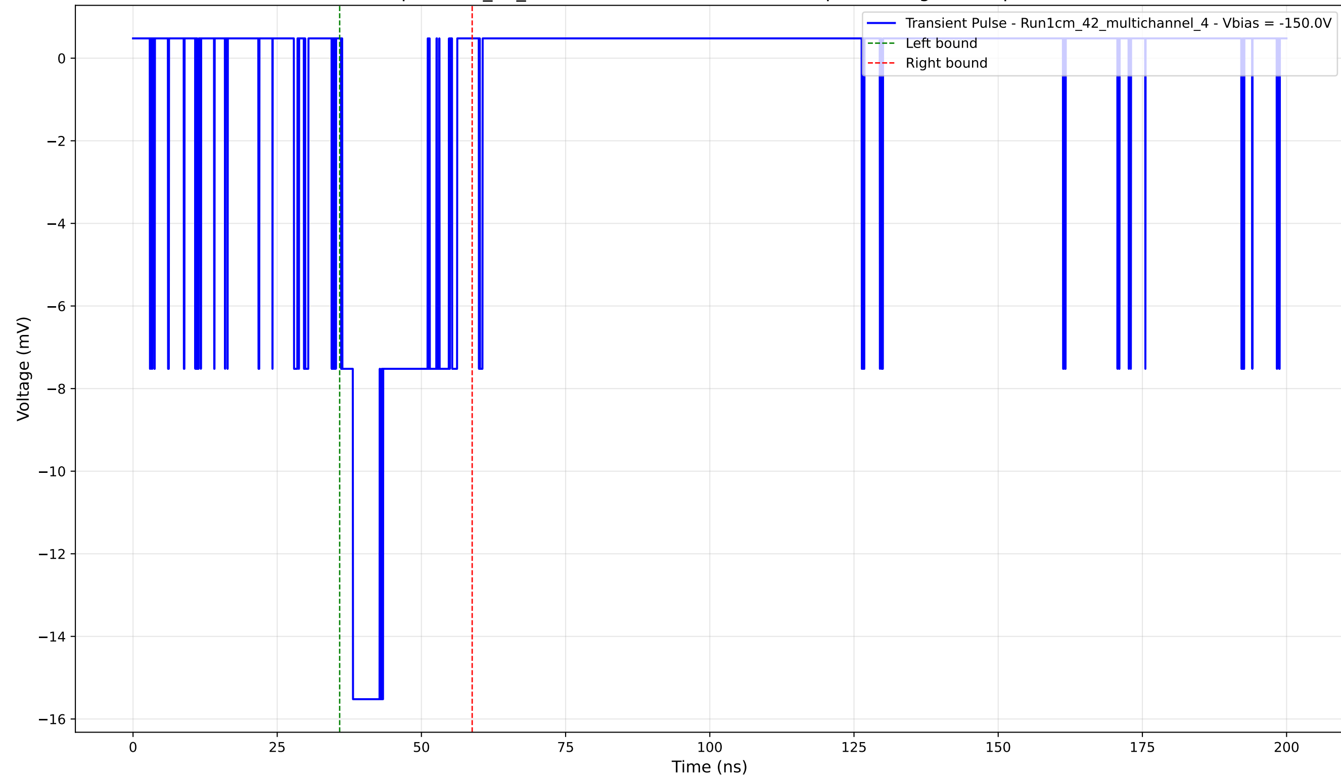
Transient Pulse - Sample: 1cm_42_multichannel - Position: 4080.0 \mu\text{m} - Charge: 3.67 pC - Rise Time: 1.86 ns
