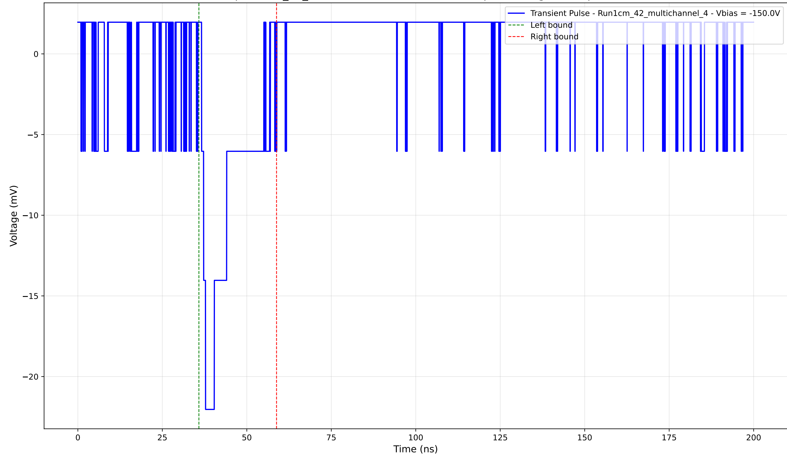
Transient Pulse - Sample: 1cm_42_multichannel - Position: 1190.0 \mu\text{m} - Charge: 3.84 pC - Rise Time: 1.18 ns
