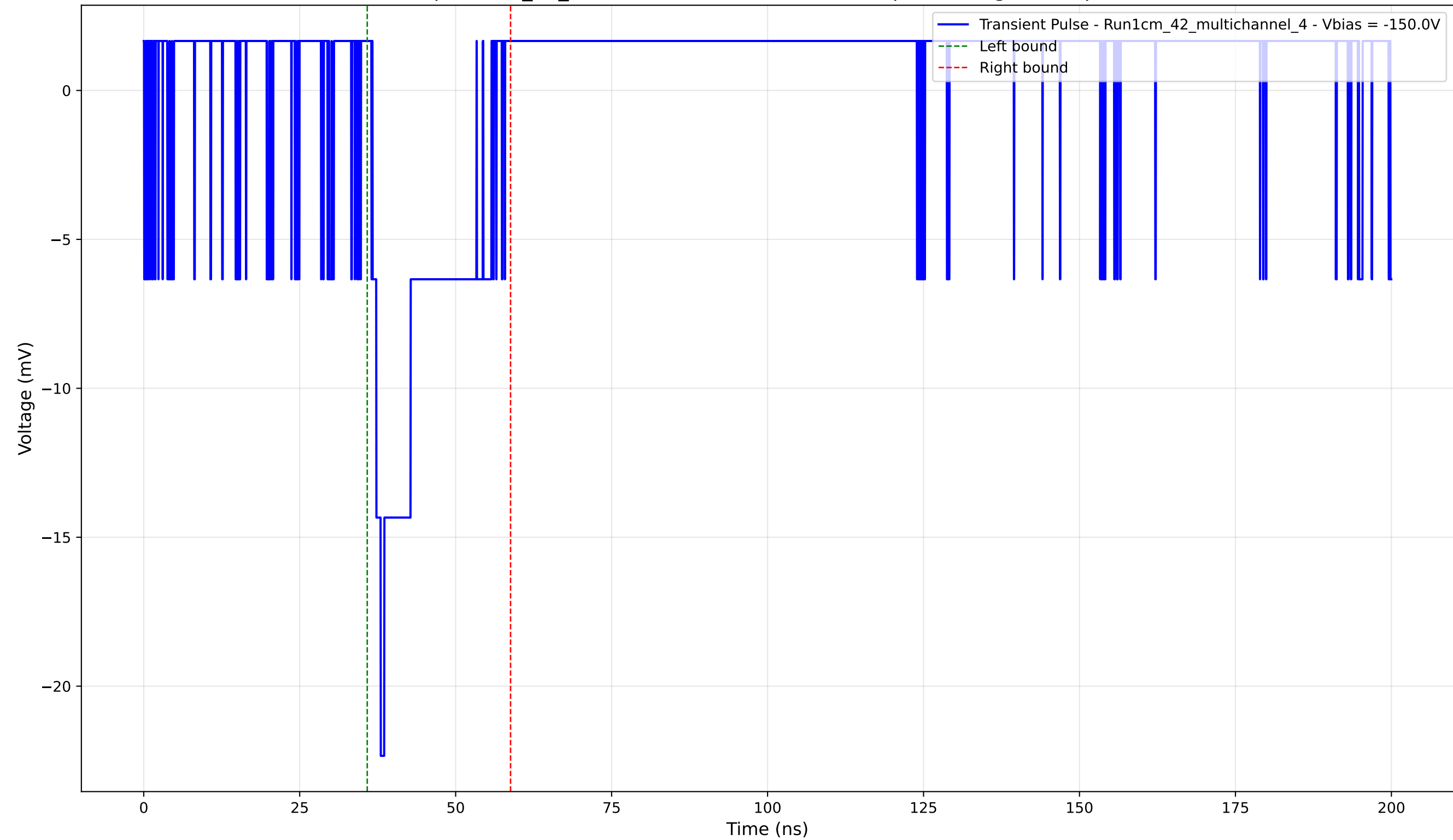
Transient Pulse - Sample: 1cm_42_multichannel - Position: 3570.0 \mu\text{m} - Charge: 3.31 pC - Rise Time: 1.32 ns
