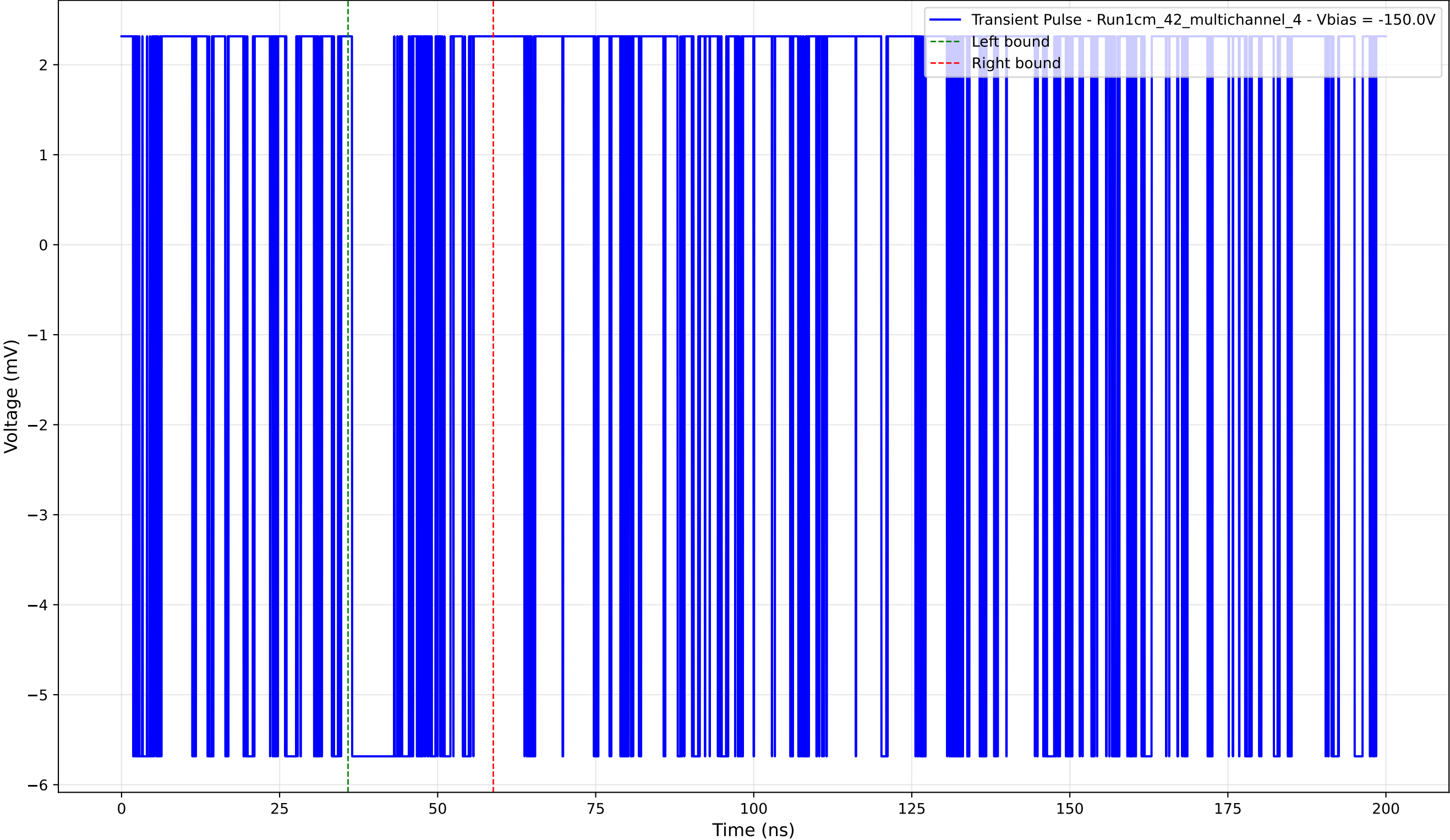
Transient Pulse - Sample: 1cm_42_multichannel - Position: 1910.0 \mu\text{m} - Charge: 1.13 pC - Rise Time: 0.00 ns (N/A)
