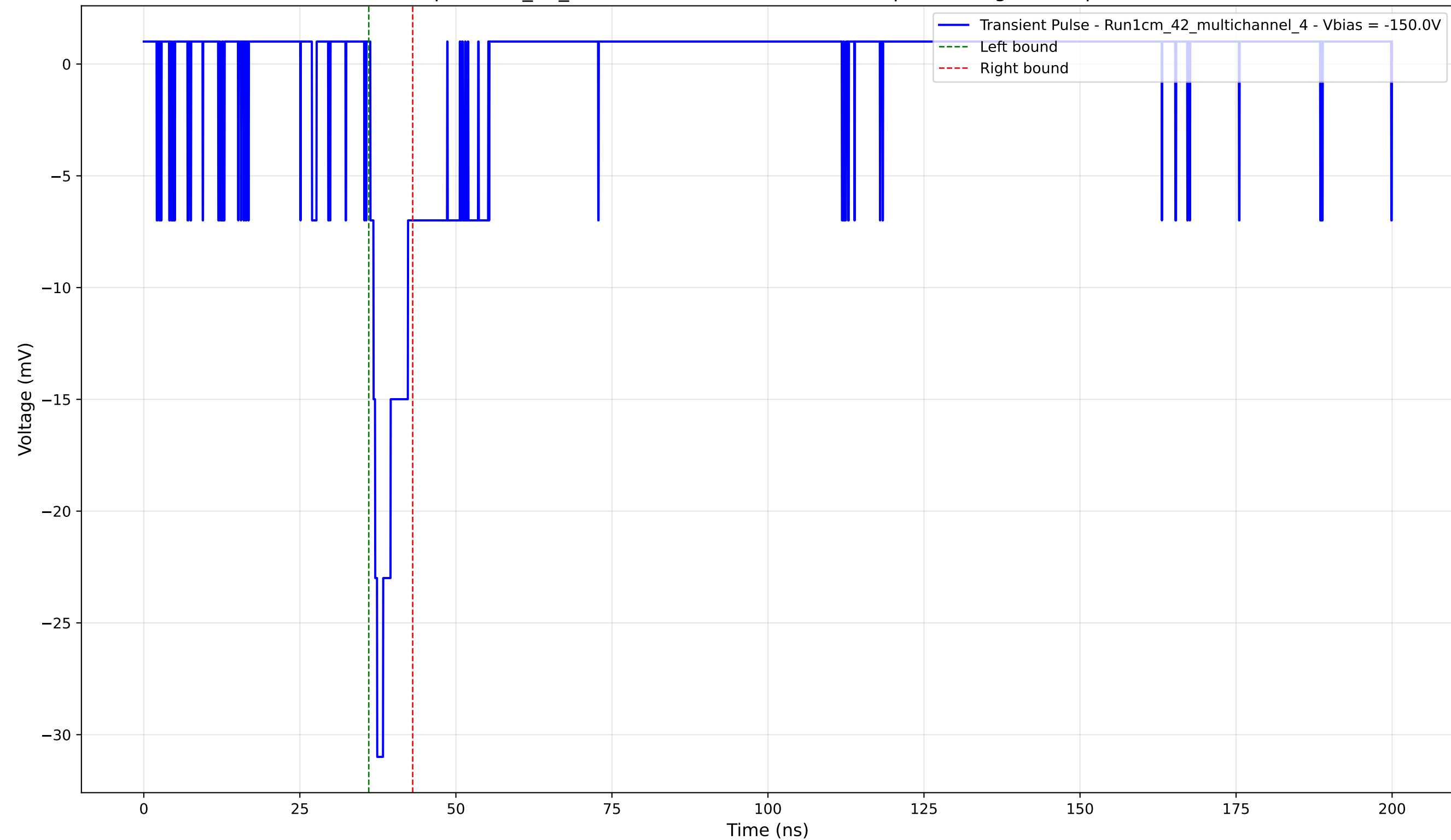
Transient Pulse - Sample: 1cm_42_multichannel - Position: 3135.0 \mu\text{m} - Charge: 2.38 pC - Rise Time: 1.09 ns
