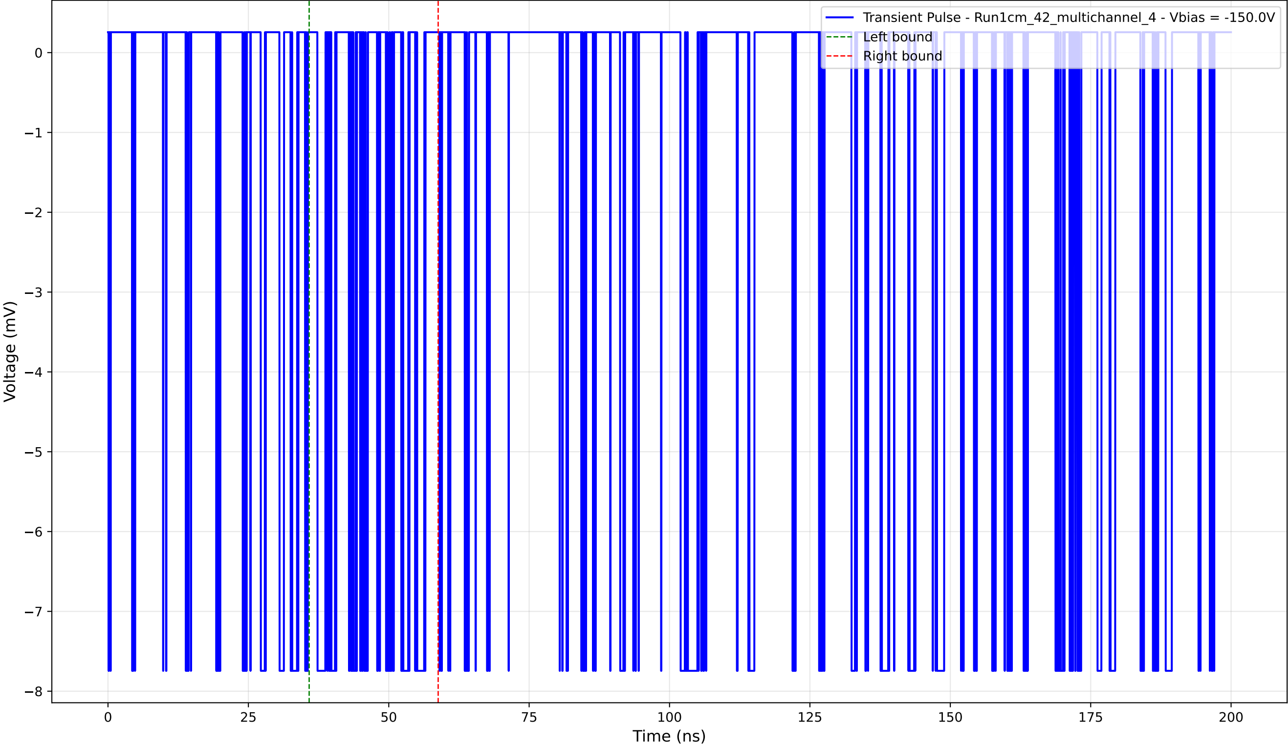
Transient Pulse - Sample: 1cm_42_multichannel - Position: 1875.0 \mu\text{m} - Charge: 1.19 pC - Rise Time: 0.02 ns
