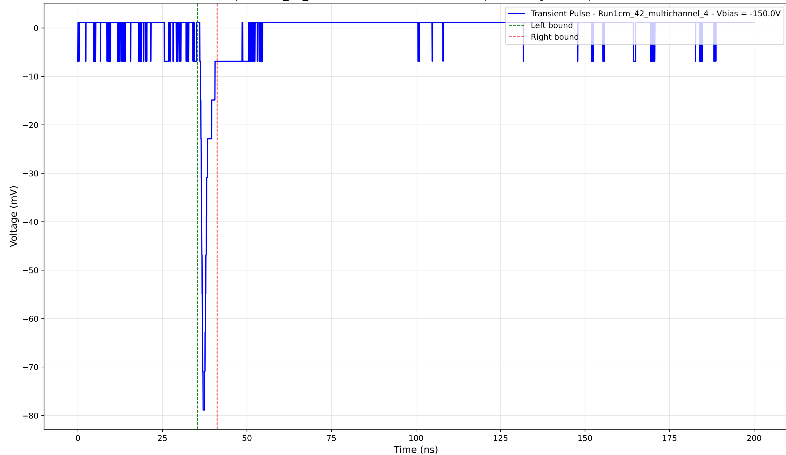
Transient Pulse - Sample: 1cm_42_multichannel - Position: 2465.0 \mu\text{m} - Charge: 3.16 pC - Rise Time: 0.80 ns
