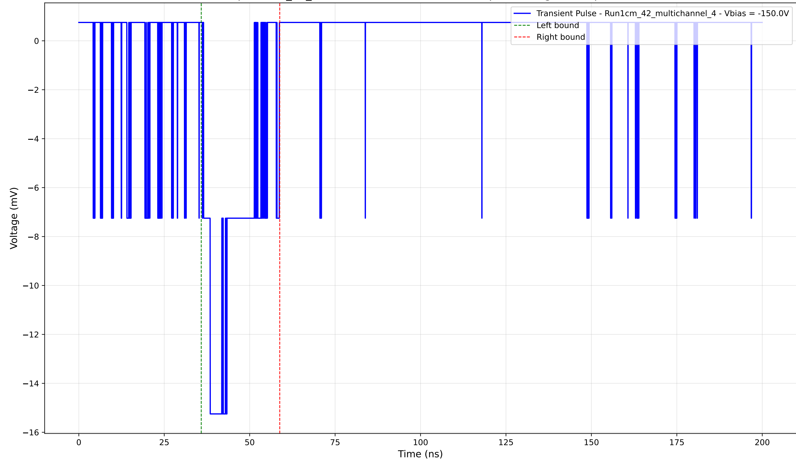
Transient Pulse - Sample: 1cm_42_multichannel - Position: 4680.0 \mu\text{m} - Charge: 3.30 pC - Rise Time: 1.94 ns
