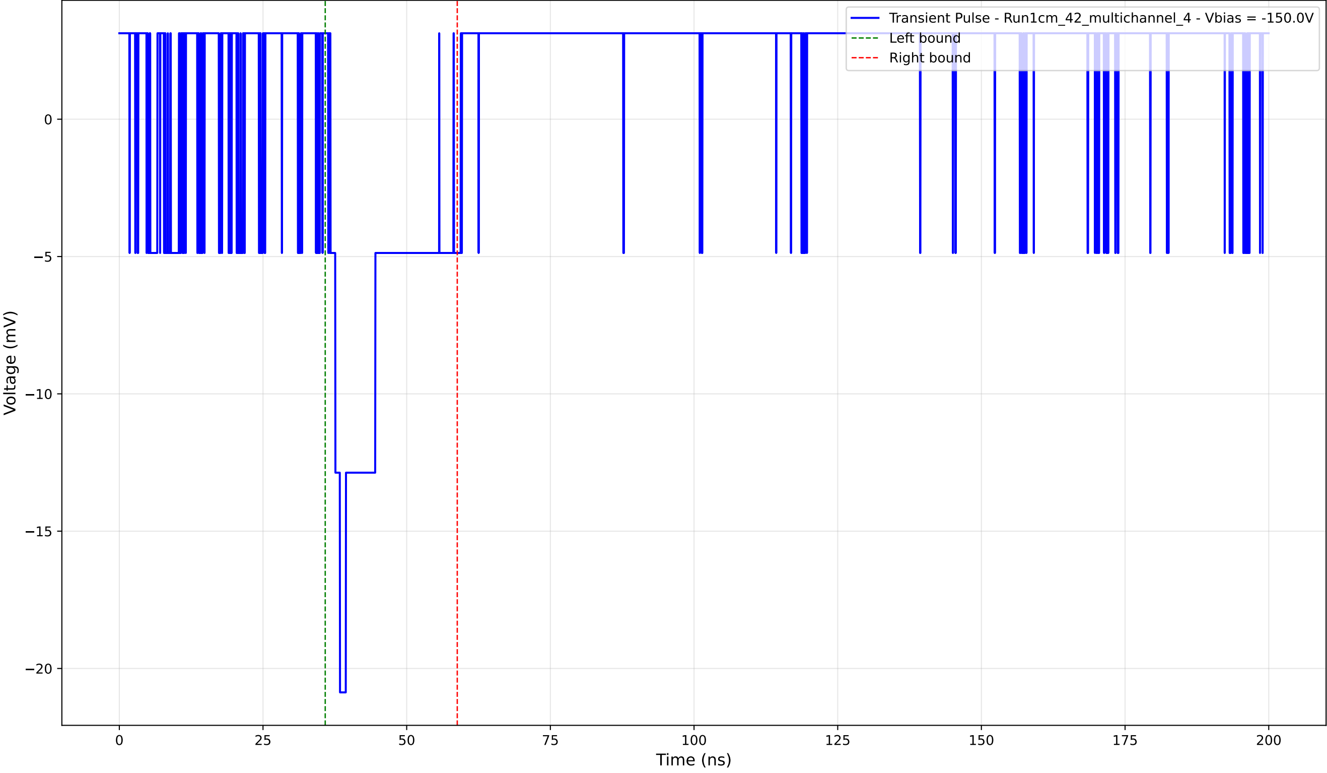
Transient Pulse - Sample: 1cm_42_multichannel - Position: 955.0 \mu\text{m} - Charge: 3.37 pC - Rise Time: 0.00 ns (N/A)
