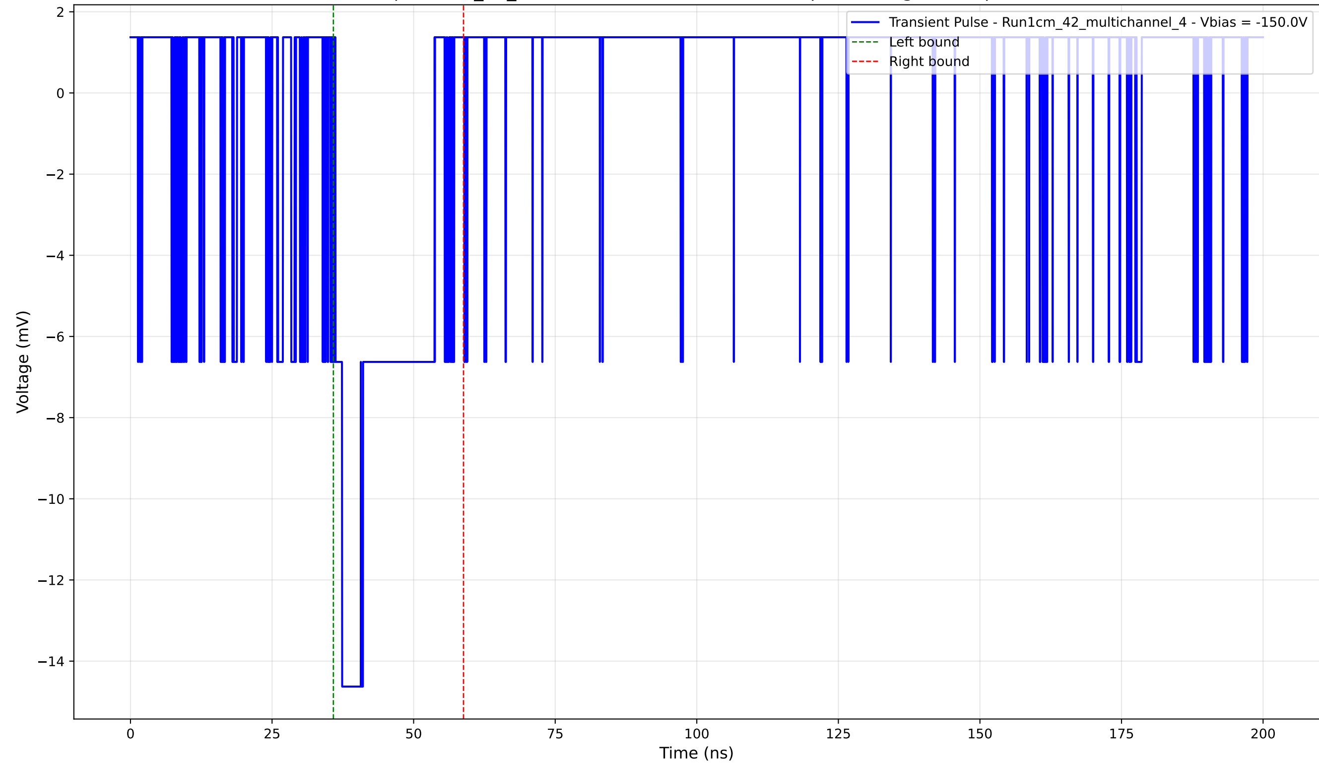
Transient Pulse - Sample: 1cm_42_multichannel - Position: 3455.0 \mu\text{m} - Charge: 2.97 pC - Rise Time: 1.18 ns
