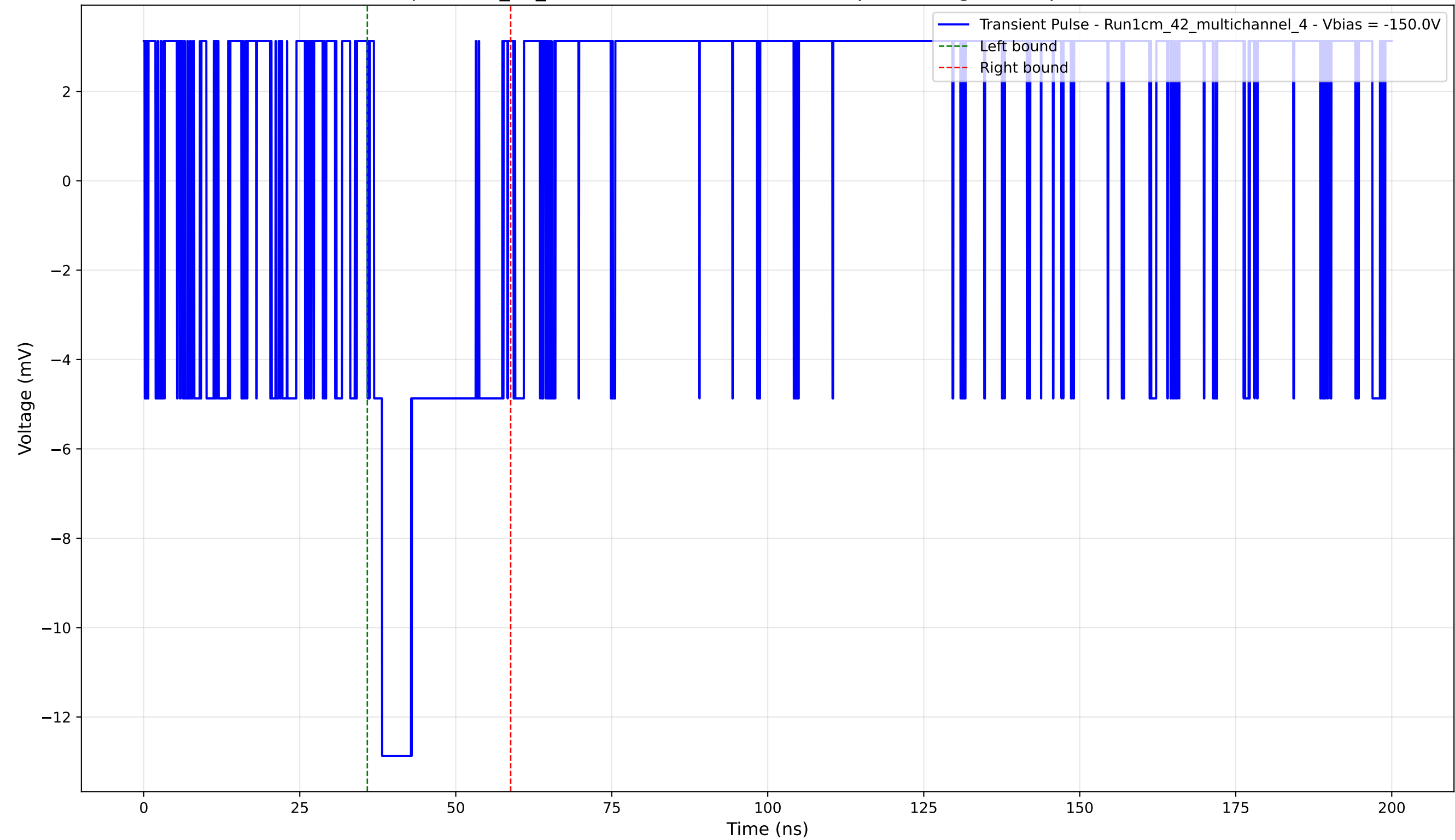
Transient Pulse - Sample: 1cm_42_multichannel - Position: 265.0 \mu\text{m} - Charge: 2.63 pC - Rise Time: 0.00 ns (N/A)
