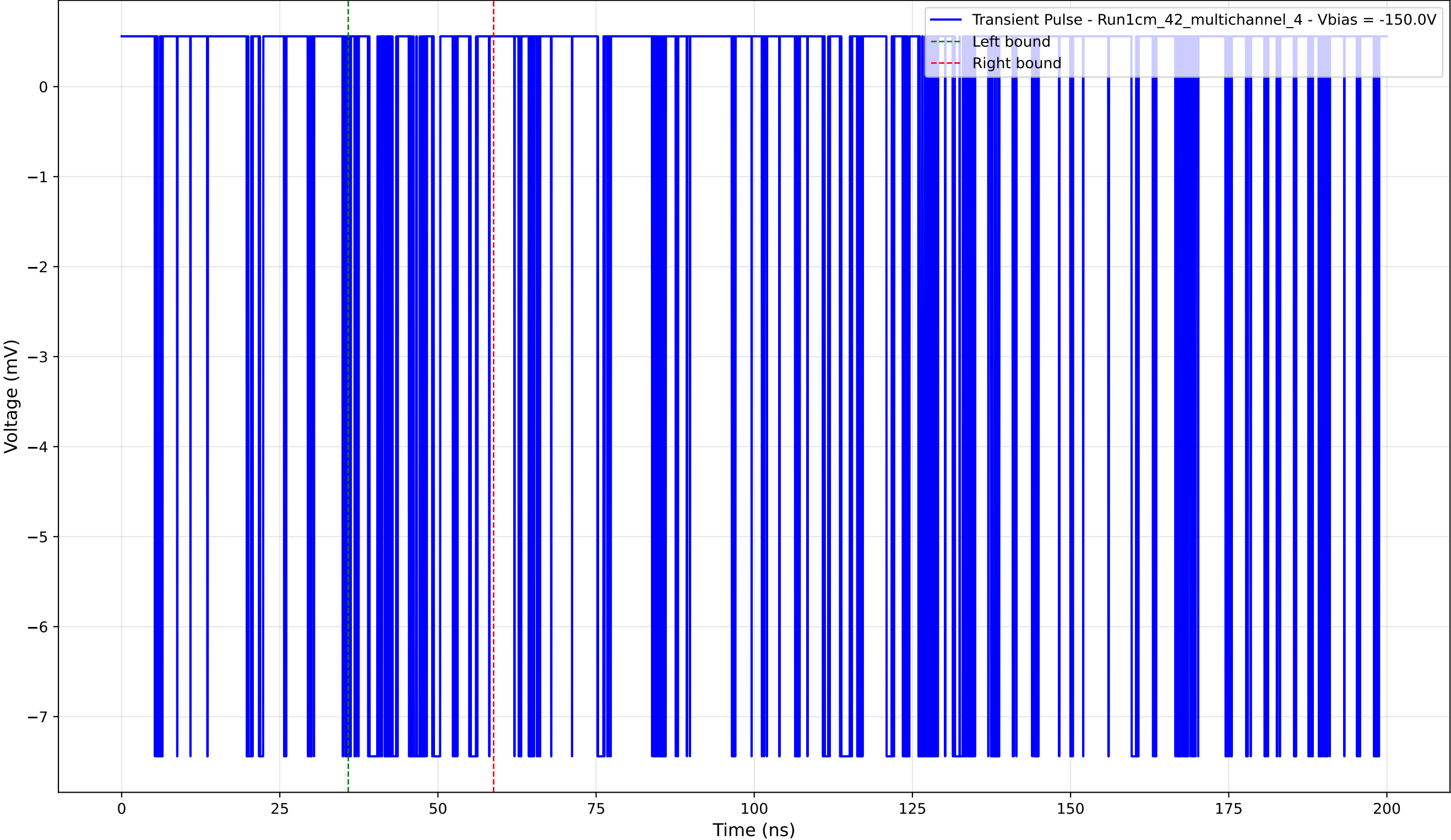
Transient Pulse - Sample: 1cm_42_multichannel - Position: 4415.0 \mu\text{m} - Charge: 1.05 pC - Rise Time: 0.02 ns
