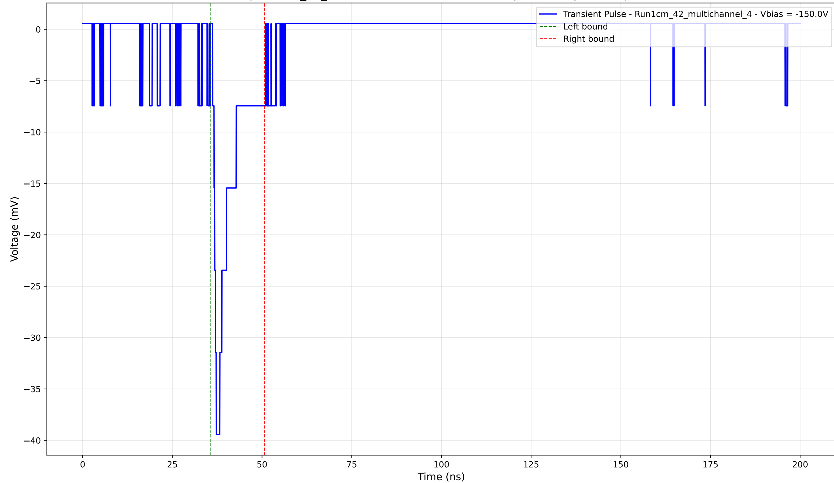
Transient Pulse - Sample: 1cm_42_multichannel - Position: 1775.0 \mu\text{m} - Charge: 4.13 pC - Rise Time: 1.01 ns
