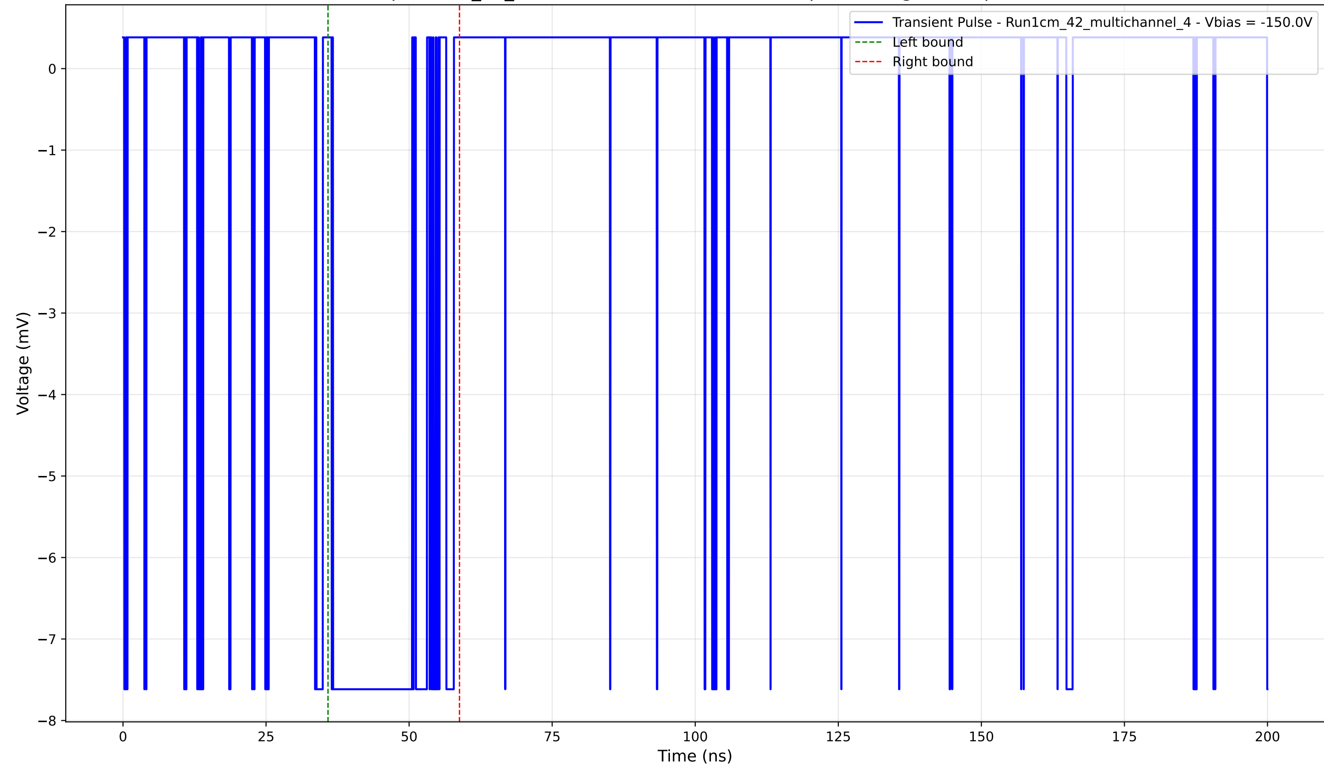
Transient Pulse - Sample: 1cm_42_multichannel - Position: 4845.0 \mu\text{m} - Charge: 2.78 pC - Rise Time: 0.02 ns
