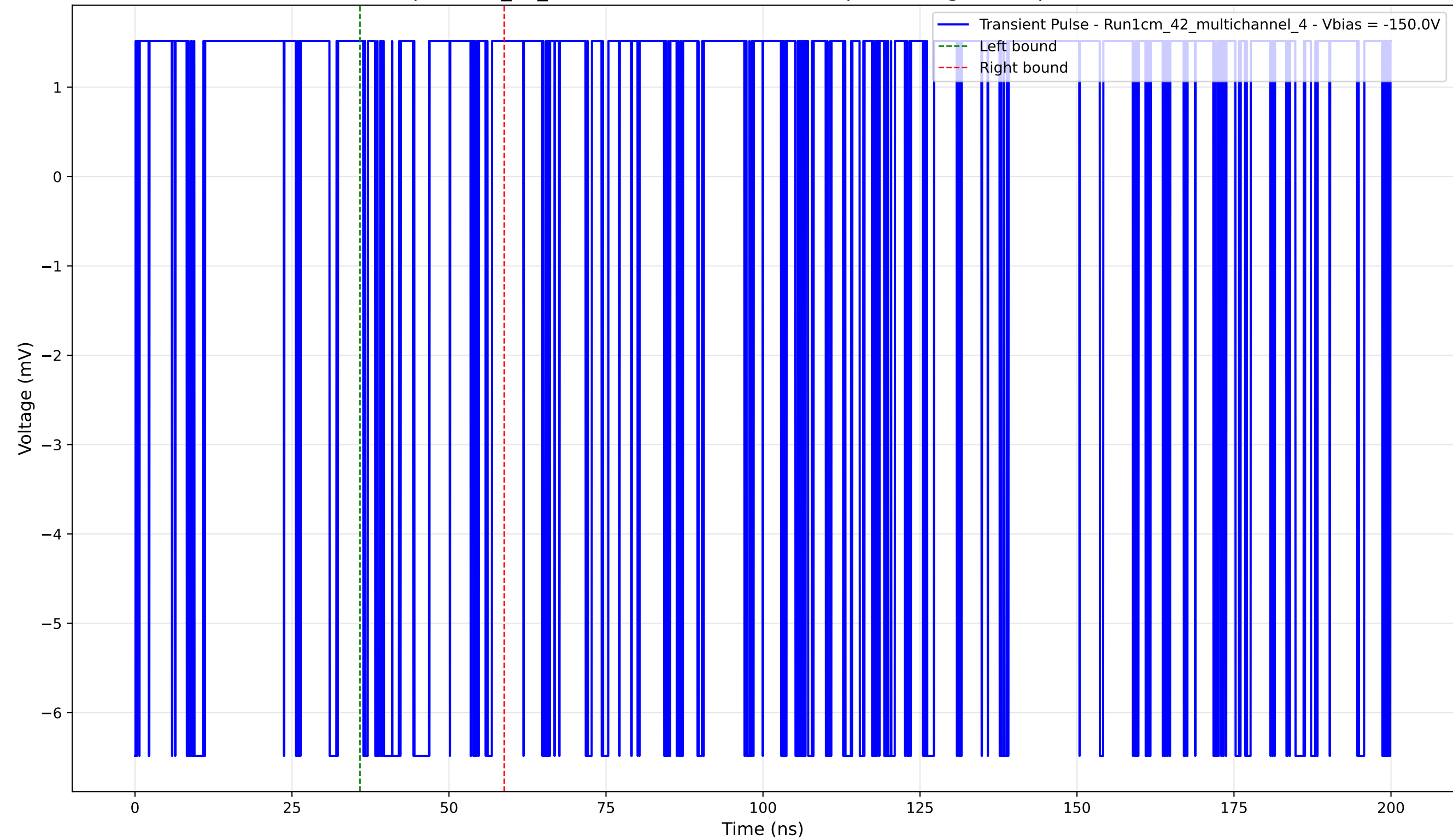
Transient Pulse - Sample: 1cm_42_multichannel - Position: 55.0 \mu\text{m} - Charge: 0.59 pC - Rise Time: 0.00 ns (N/A)
