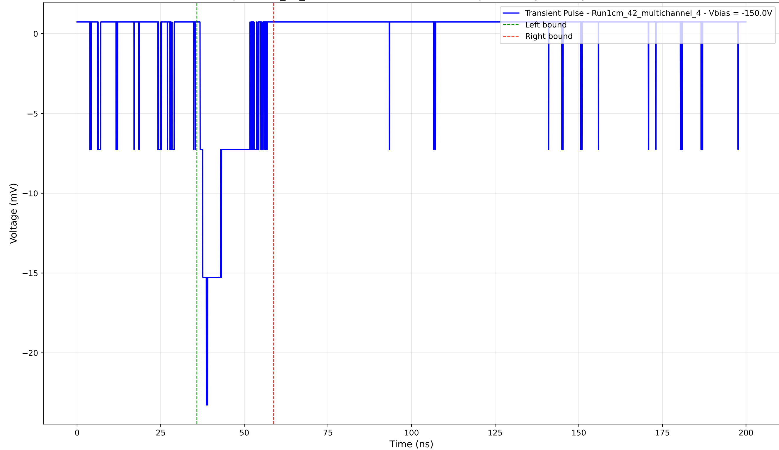
Transient Pulse - Sample: 1cm_42_multichannel - Position: 3735.0 \mu\text{m} - Charge: 3.37 pC - Rise Time: 1.88 ns
