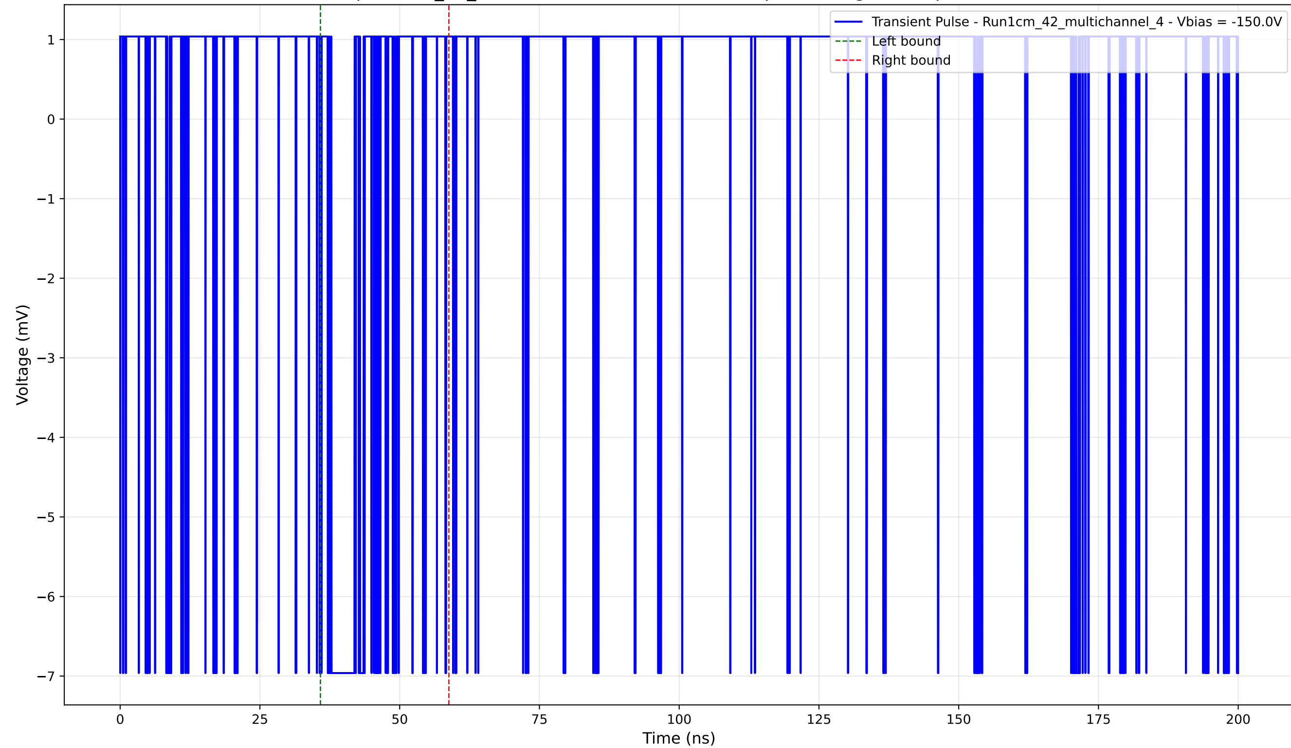
Transient Pulse - Sample: 1cm_42_multichannel - Position: 3935.0 \mu\text{m} - Charge: 0.76 pC - Rise Time: 0.00 ns (N/A)
