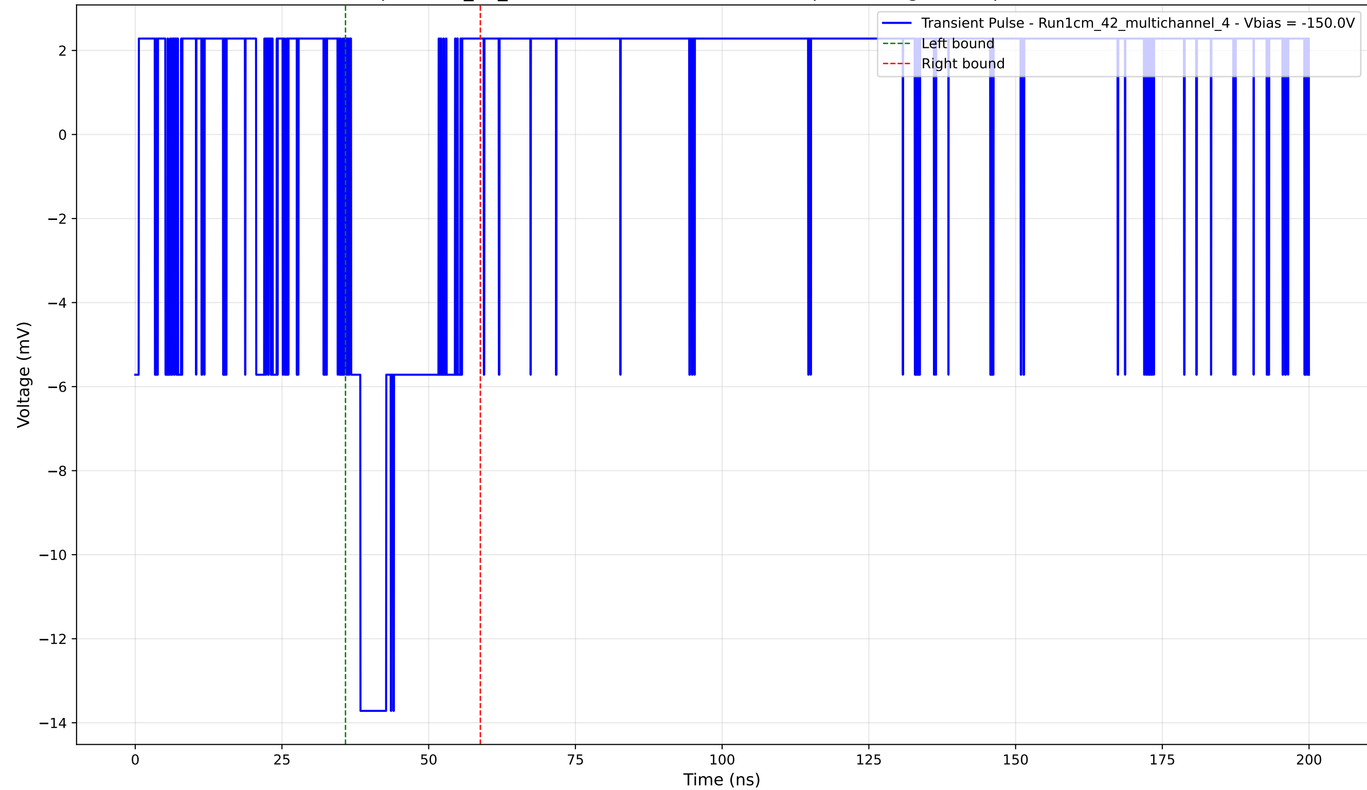
Transient Pulse - Sample: 1cm_42_multichannel - Position: 4305.0 \mu\text{m} - Charge: 2.63 pC - Rise Time: 0.00 ns (N/A)
