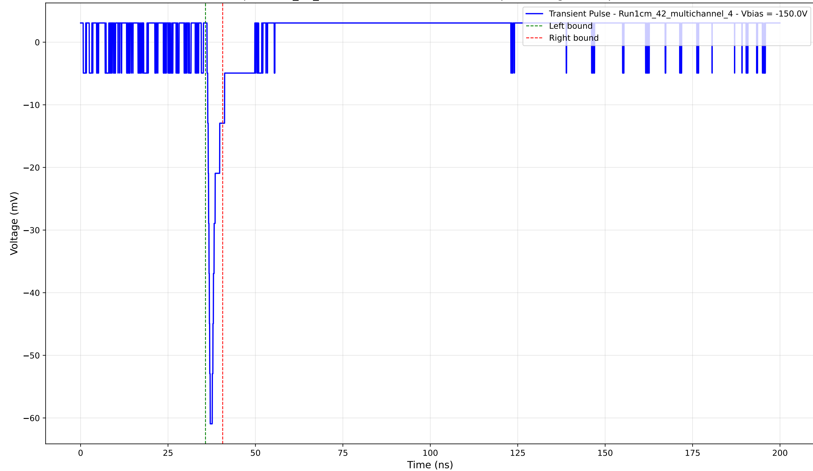
Transient Pulse - Sample: 1cm_42_multichannel - Position: 2605.0 \mu\text{m} - Charge: 2.59 pC - Rise Time: 0.72 ns
