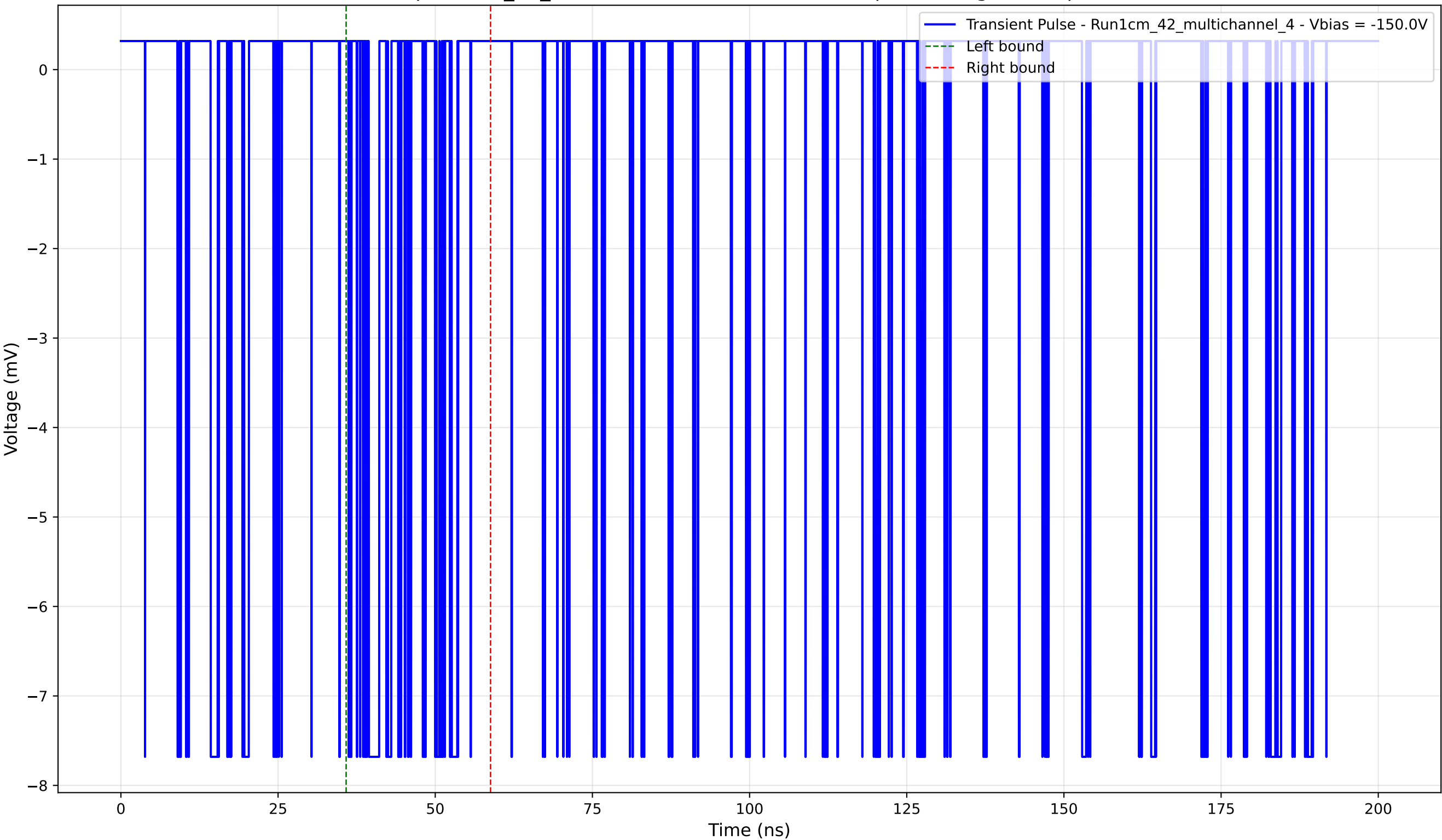
Transient Pulse - Sample: 1cm_42_multichannel - Position: 3920.0 \mu\text{m} - Charge: 0.94 pC - Rise Time: 0.02 ns
