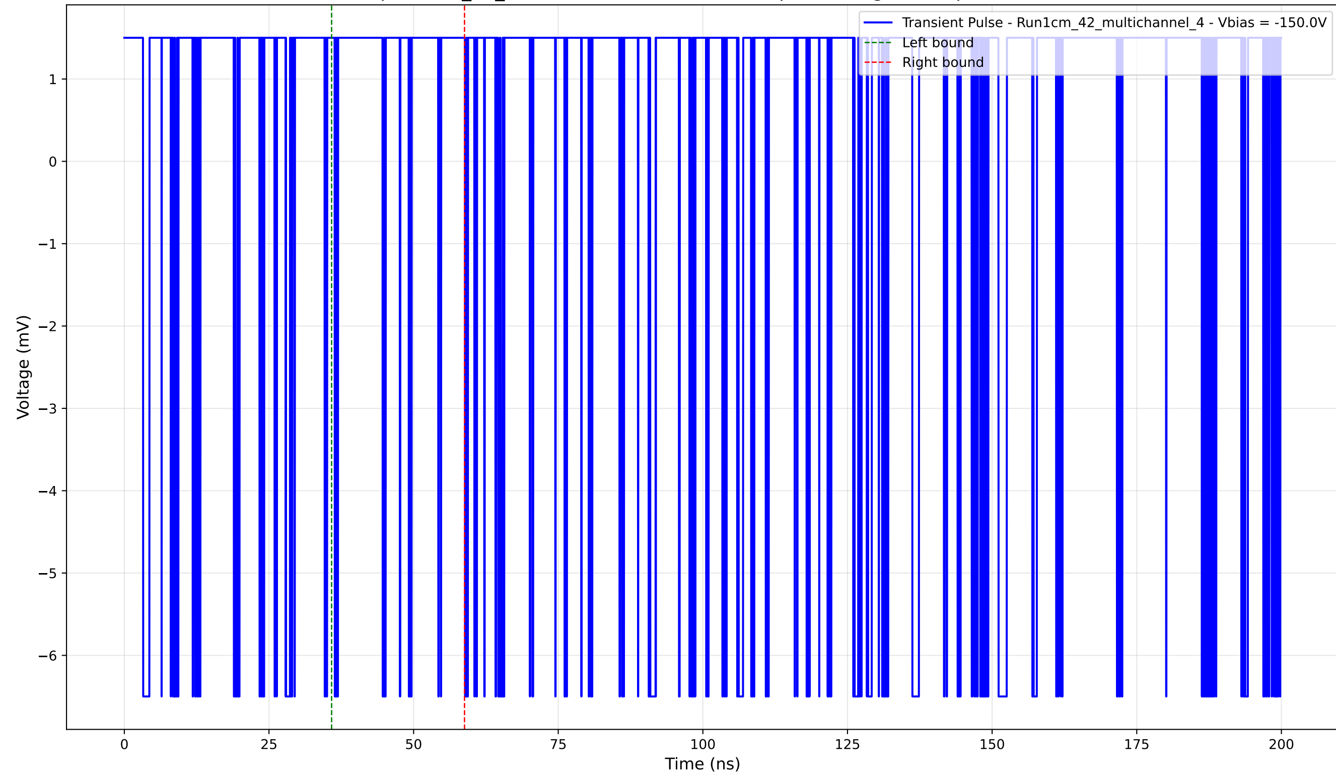
Transient Pulse - Sample: 1cm_42_multichannel - Position: 45.0 \mu\text{m} - Charge: 0.46 pC - Rise Time: 0.00 ns (N/A)
