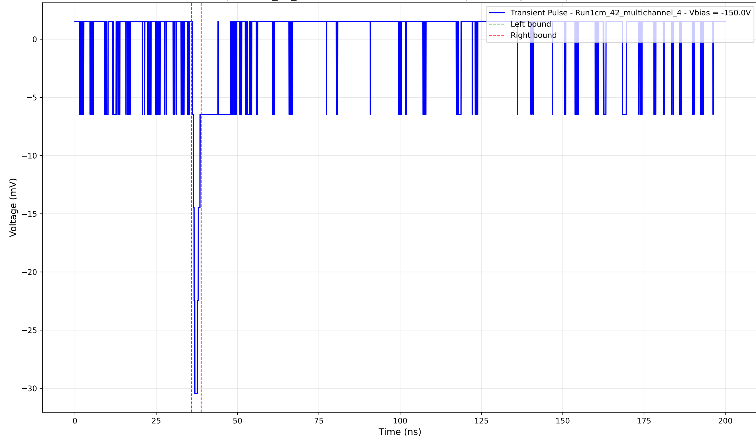
Transient Pulse - Sample: 1cm_42_multichannel - Position: 2340.0 \mu\text{m} - Charge: 0.99 pC - Rise Time: 0.81 ns
