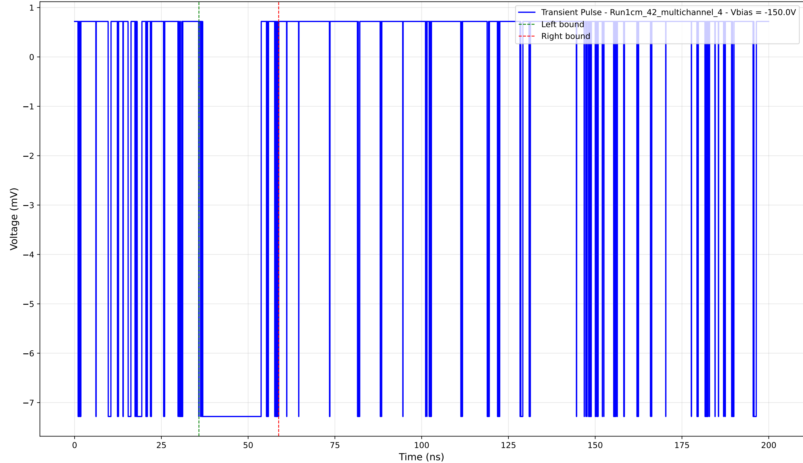
Transient Pulse - Sample: 1cm_42_multichannel - Position: 95.0 \mu\text{m} - Charge: 2.58 pC - Rise Time: 0.02 ns
