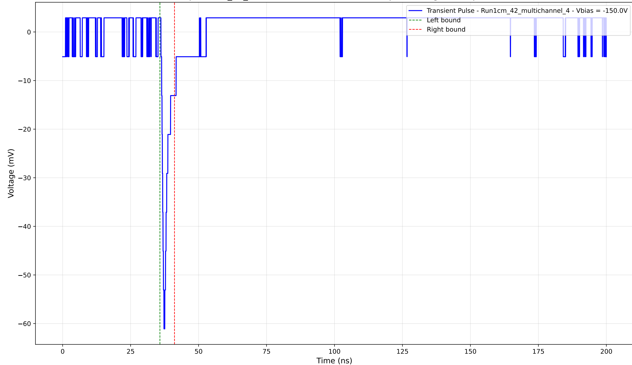
Transient Pulse - Sample: 1cm_42_multichannel - Position: 2085.0 \mu\text{m} - Charge: 2.66 pC - Rise Time: 0.86 ns
