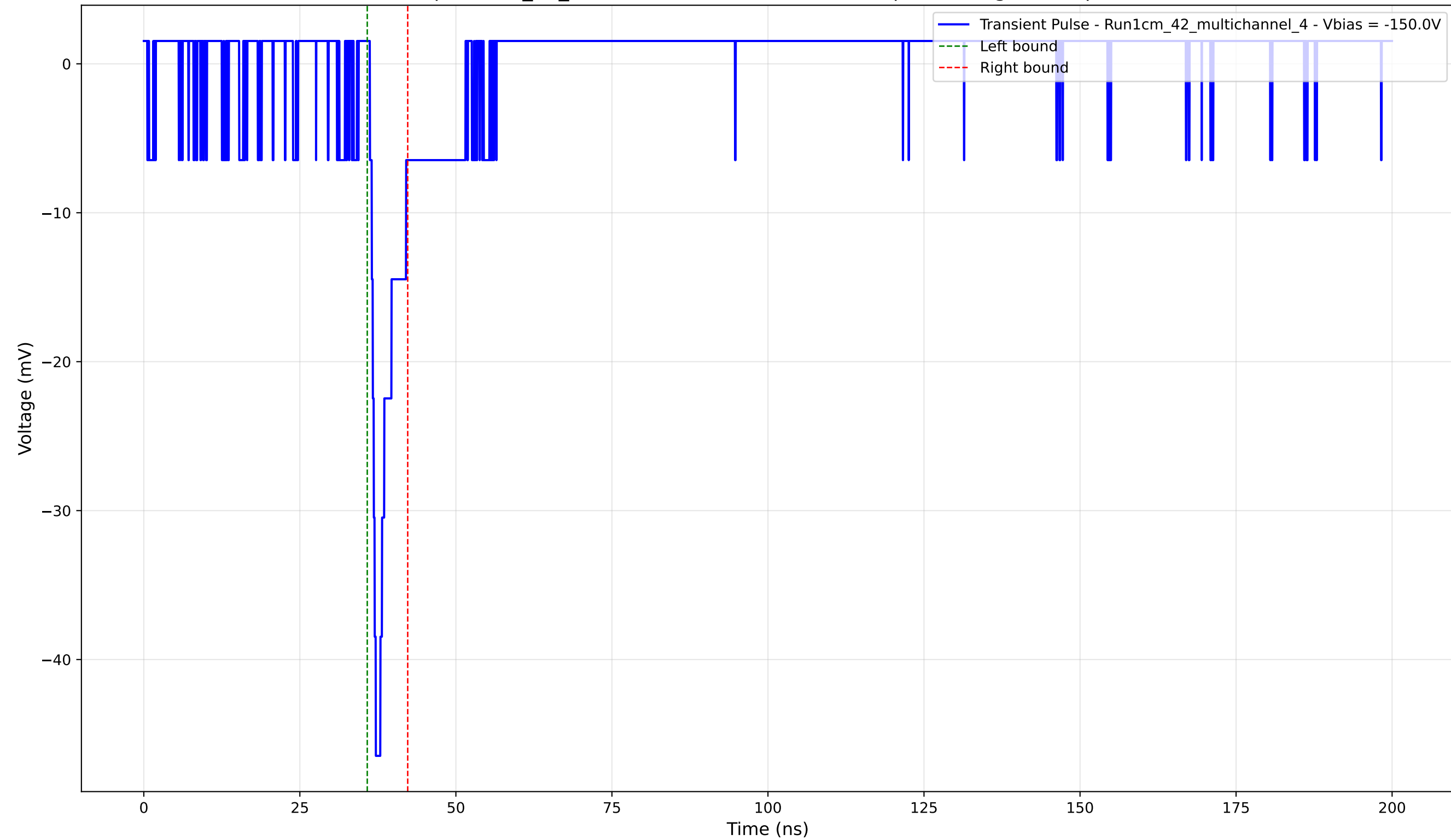
Transient Pulse - Sample: 1cm_42_multichannel - Position: 2800.0 \mu\text{m} - Charge: 2.71 pC - Rise Time: 0.95 ns
