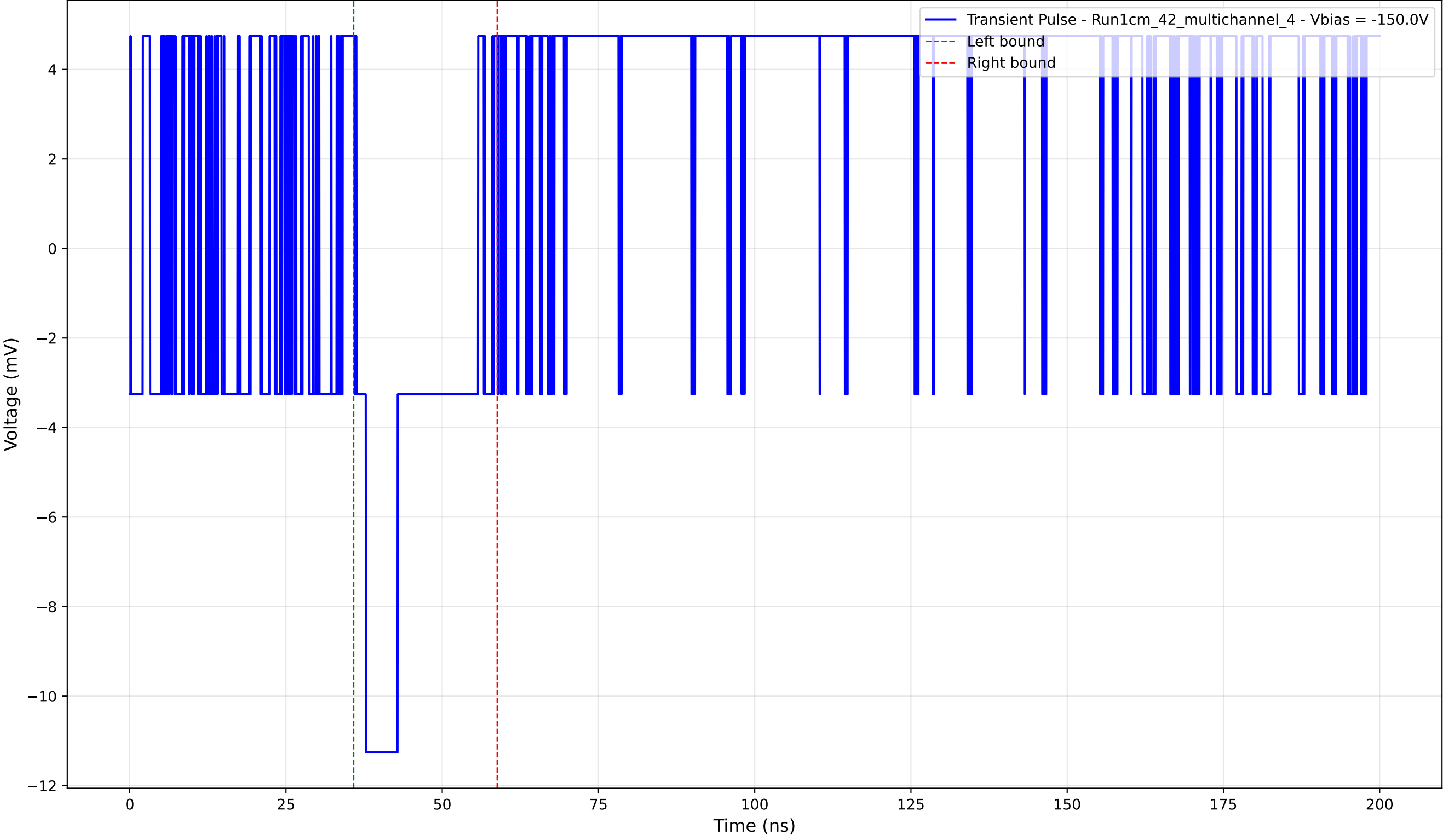
Transient Pulse - Sample: 1cm_42_multichannel - Position: 930.0 \mu\text{m} - Charge: 1.99 pC - Rise Time: 0.00 ns (N/A)
