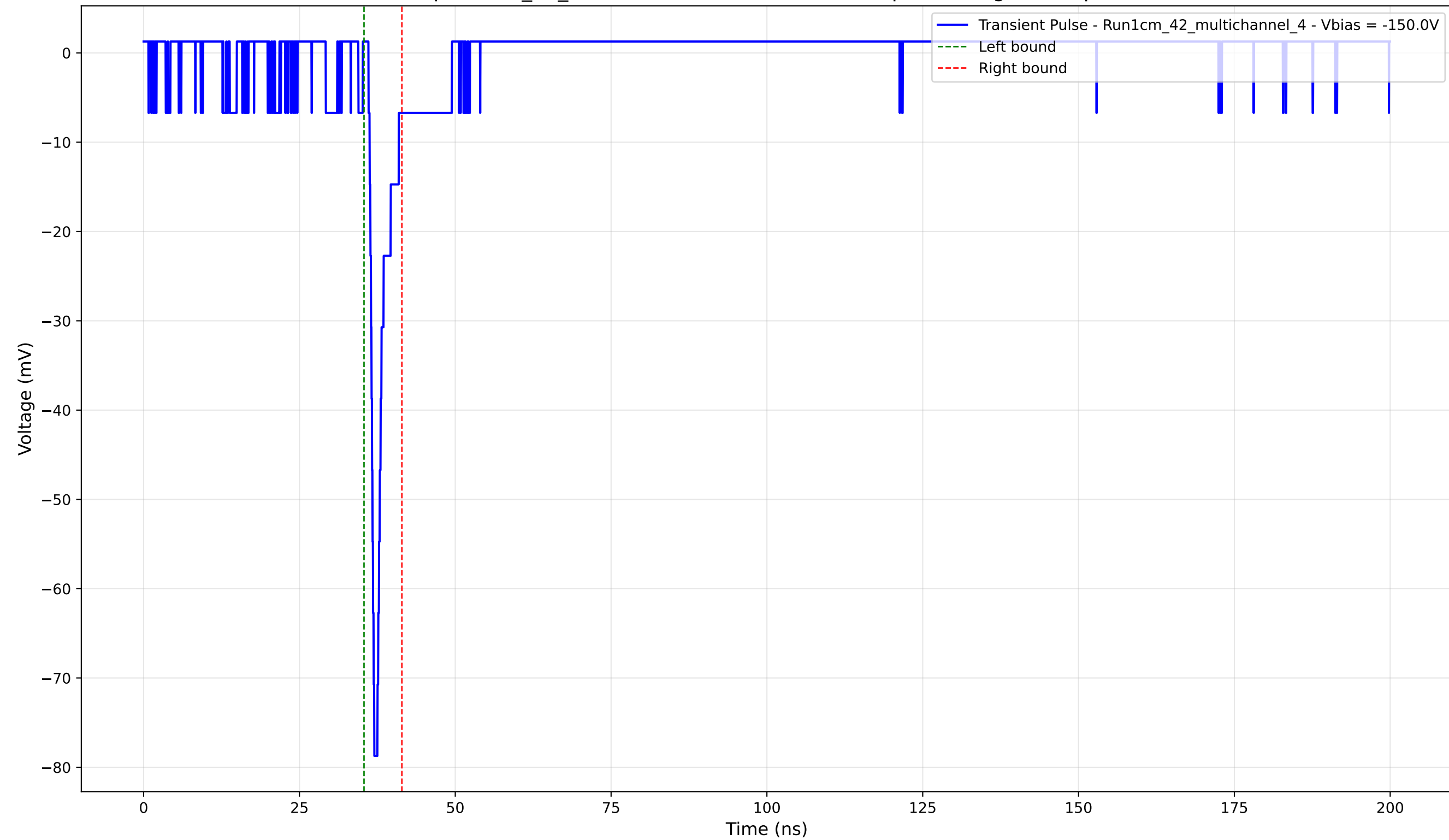
Transient Pulse - Sample: 1cm_42_multichannel - Position: 2295.0 \mu\text{m} - Charge: 3.32 pC - Rise Time: 0.76 ns
