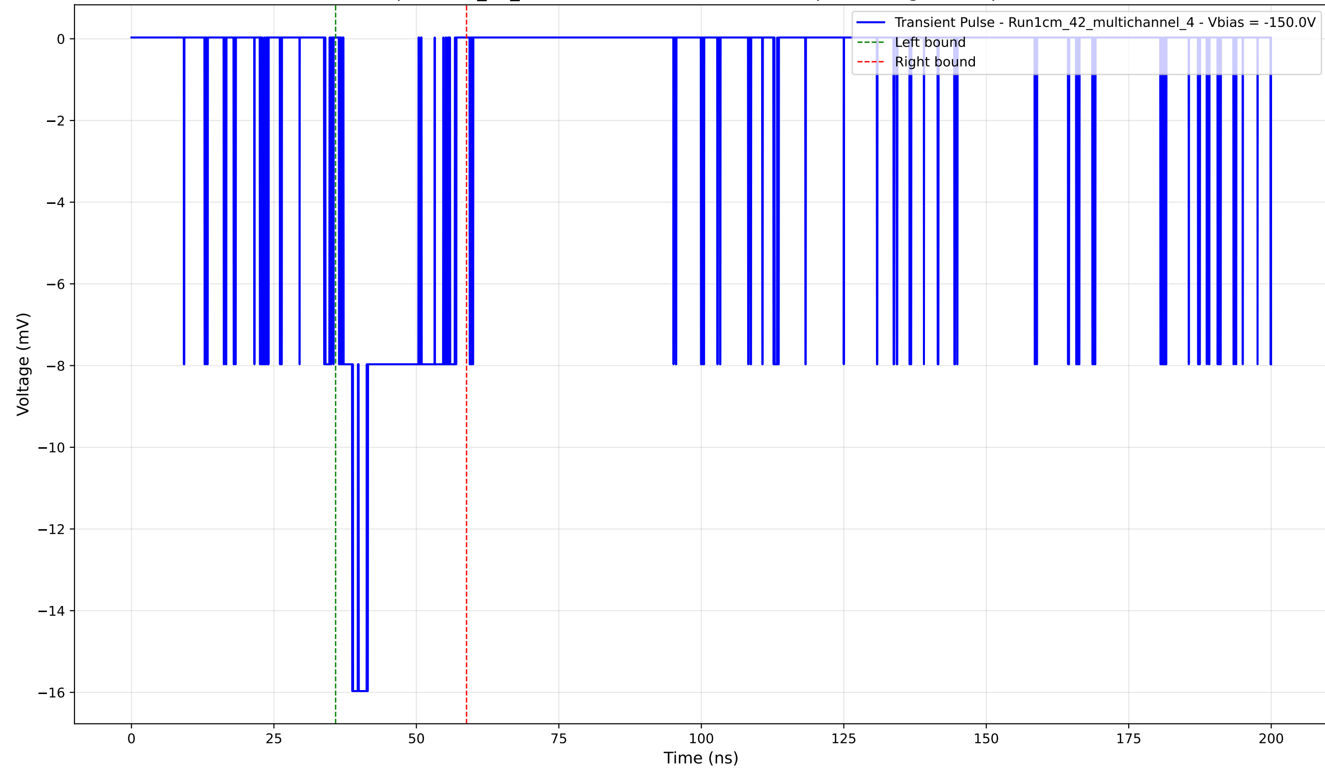
Transient Pulse - Sample: 1cm_42_multichannel - Position: 4470.0 \mu\text{m} - Charge: 3.48 pC - Rise Time: 1.52 ns
