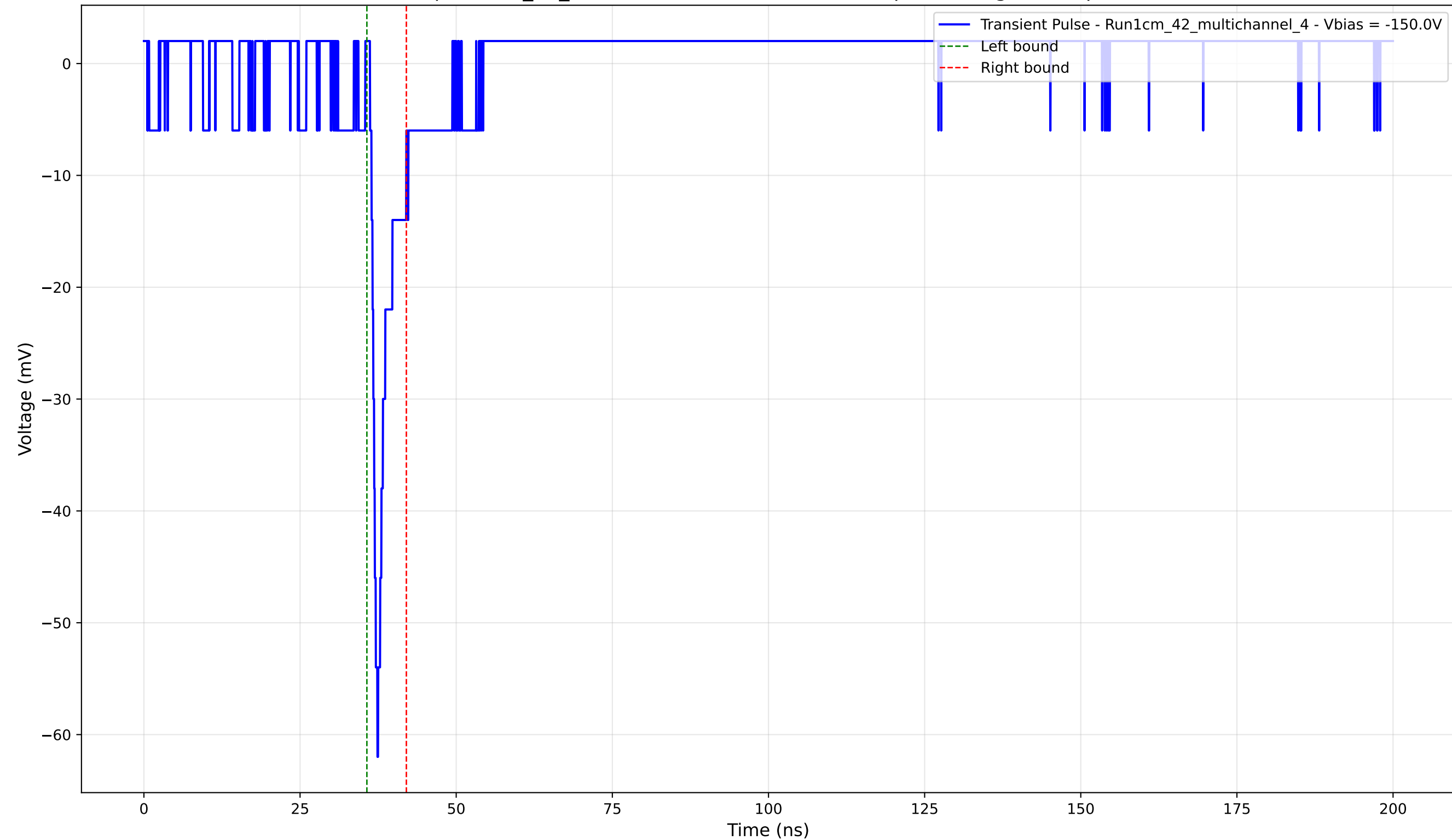
Transient Pulse - Sample: 1cm_42_multichannel - Position: 2040.0 \mu\text{m} - Charge: 2.91 pC - Rise Time: 0.96 ns
