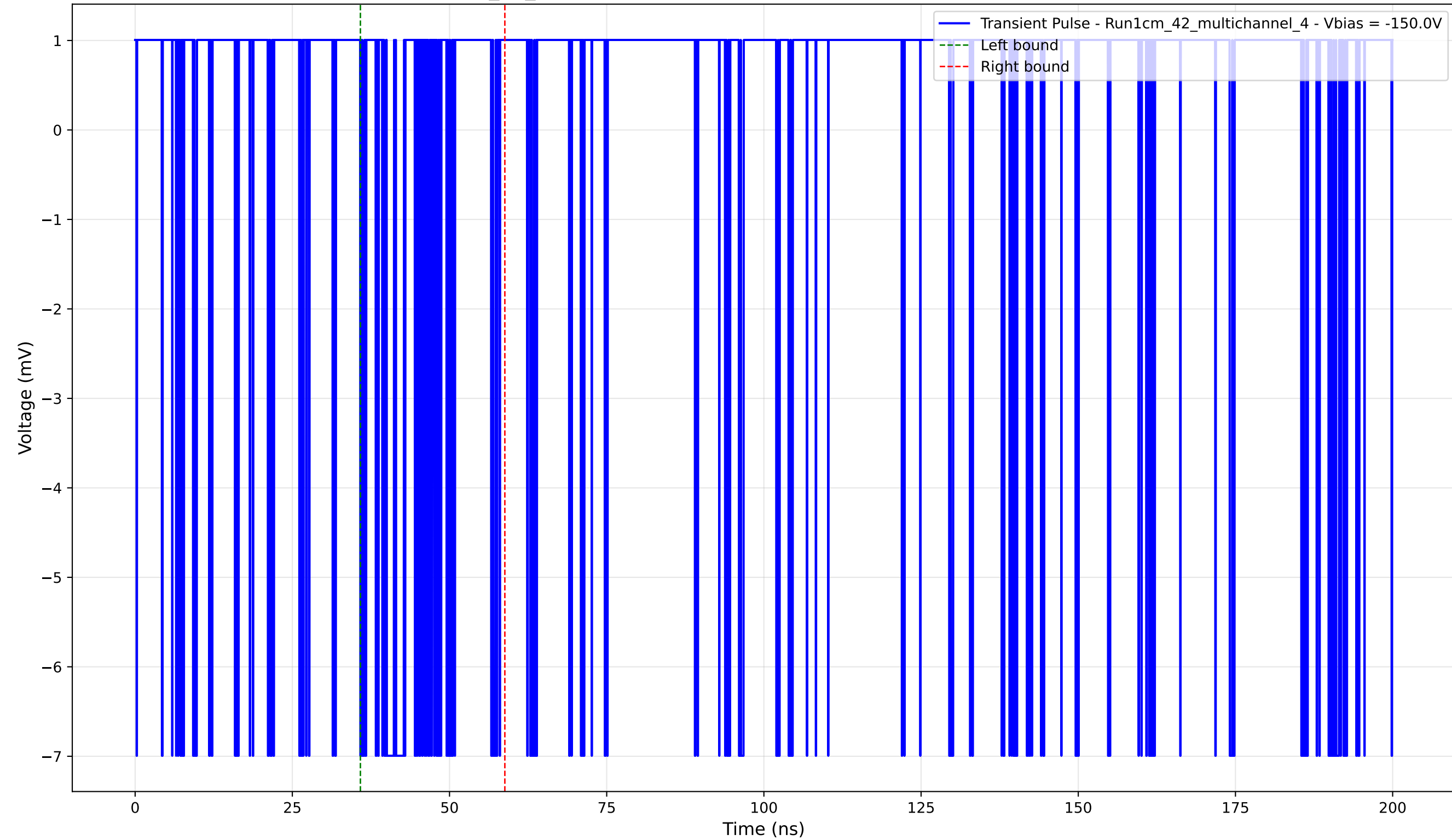
Transient Pulse - Sample: 1cm_42_multichannel - Position: 3895.0 \mu\text{m} - Charge: 0.63 pC - Rise Time: 0.00 ns (N/A)
