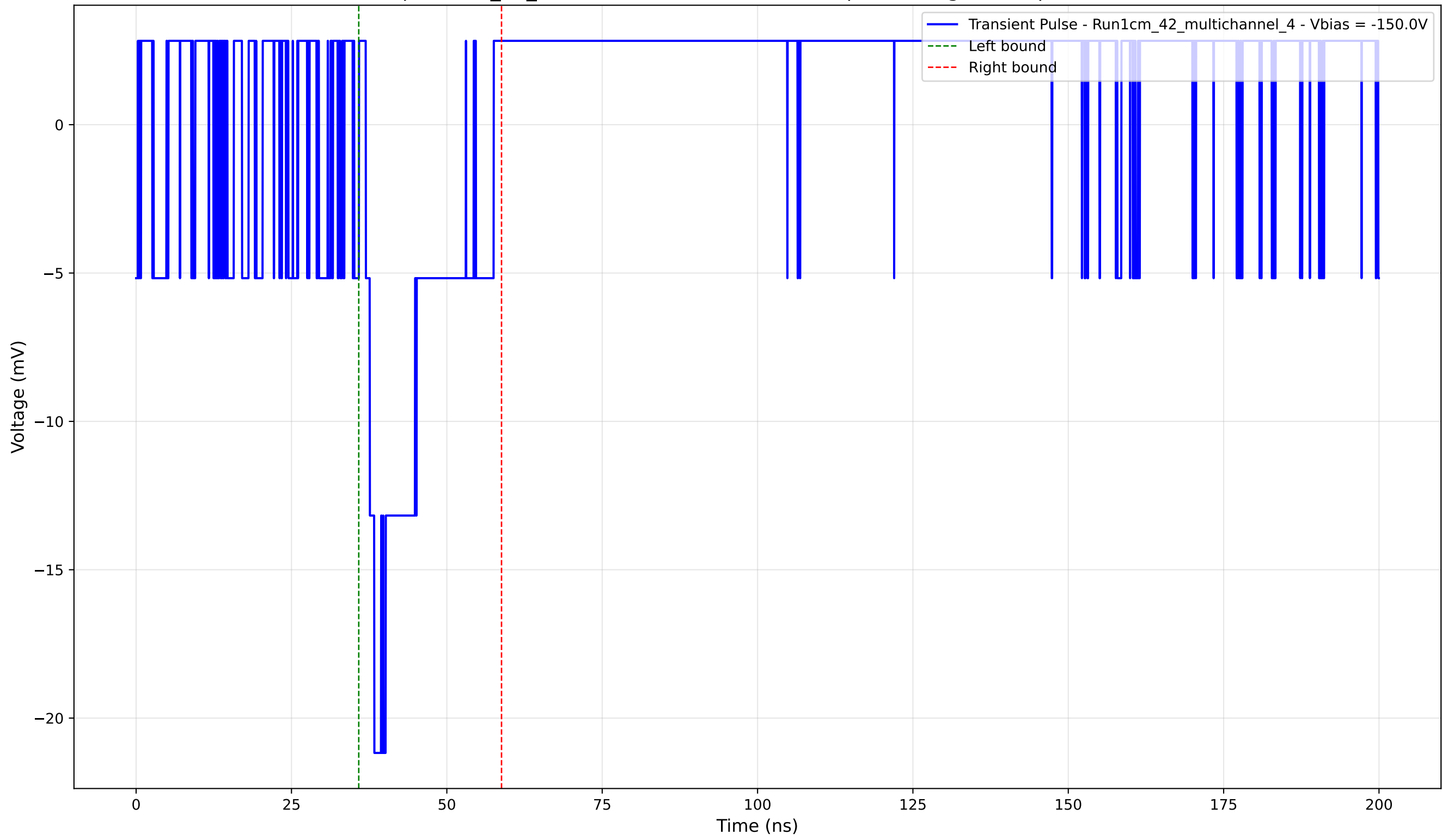
Transient Pulse - Sample: 1cm_42_multichannel - Position: 985.0 \mu\text{m} - Charge: 3.41 pC - Rise Time: 0.00 ns (N/A)
