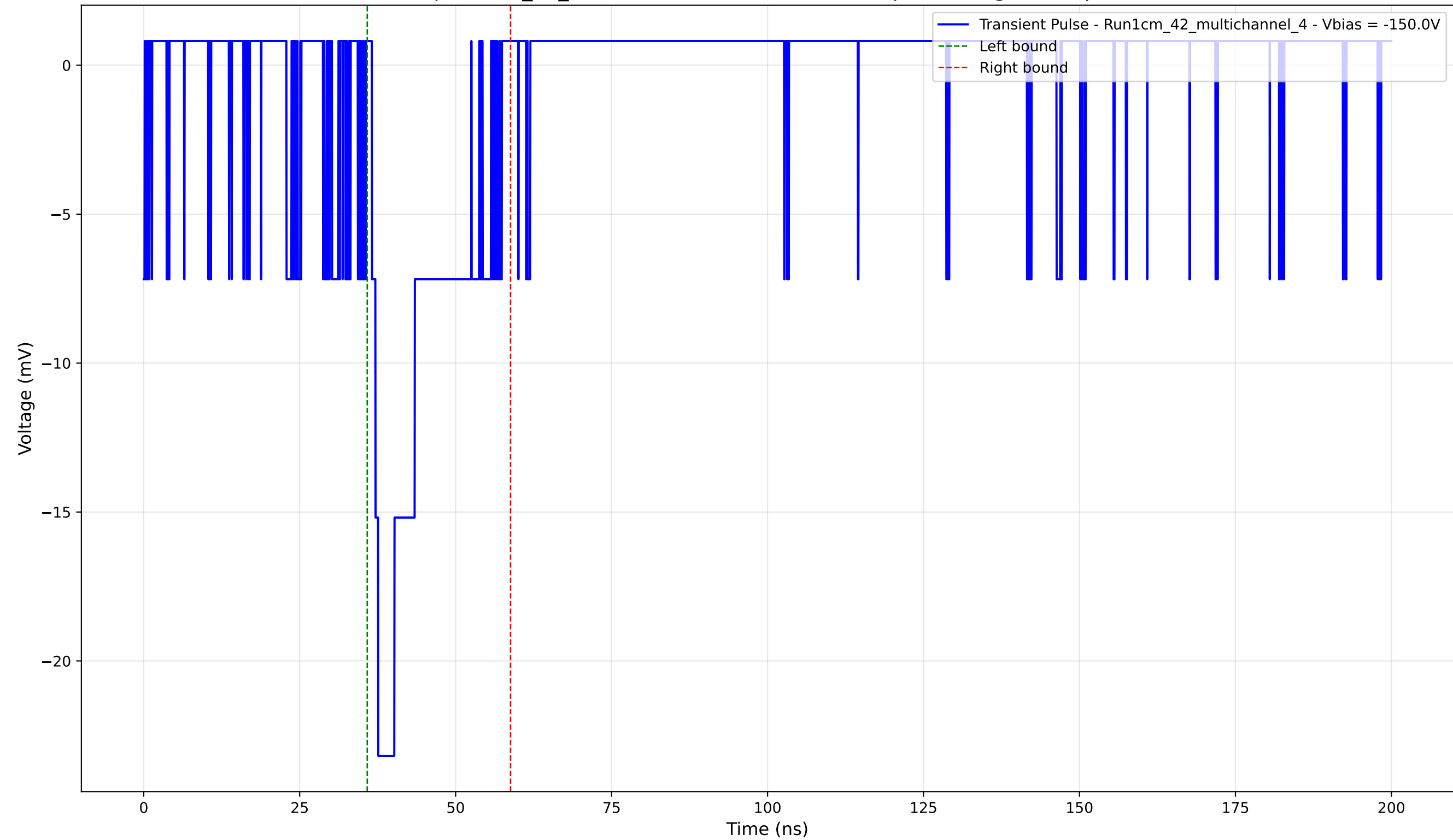
Transient Pulse - Sample: 1cm_42_multichannel - Position: 1290.0 \mu\text{m} - Charge: 4.18 pC - Rise Time: 1.02 ns
