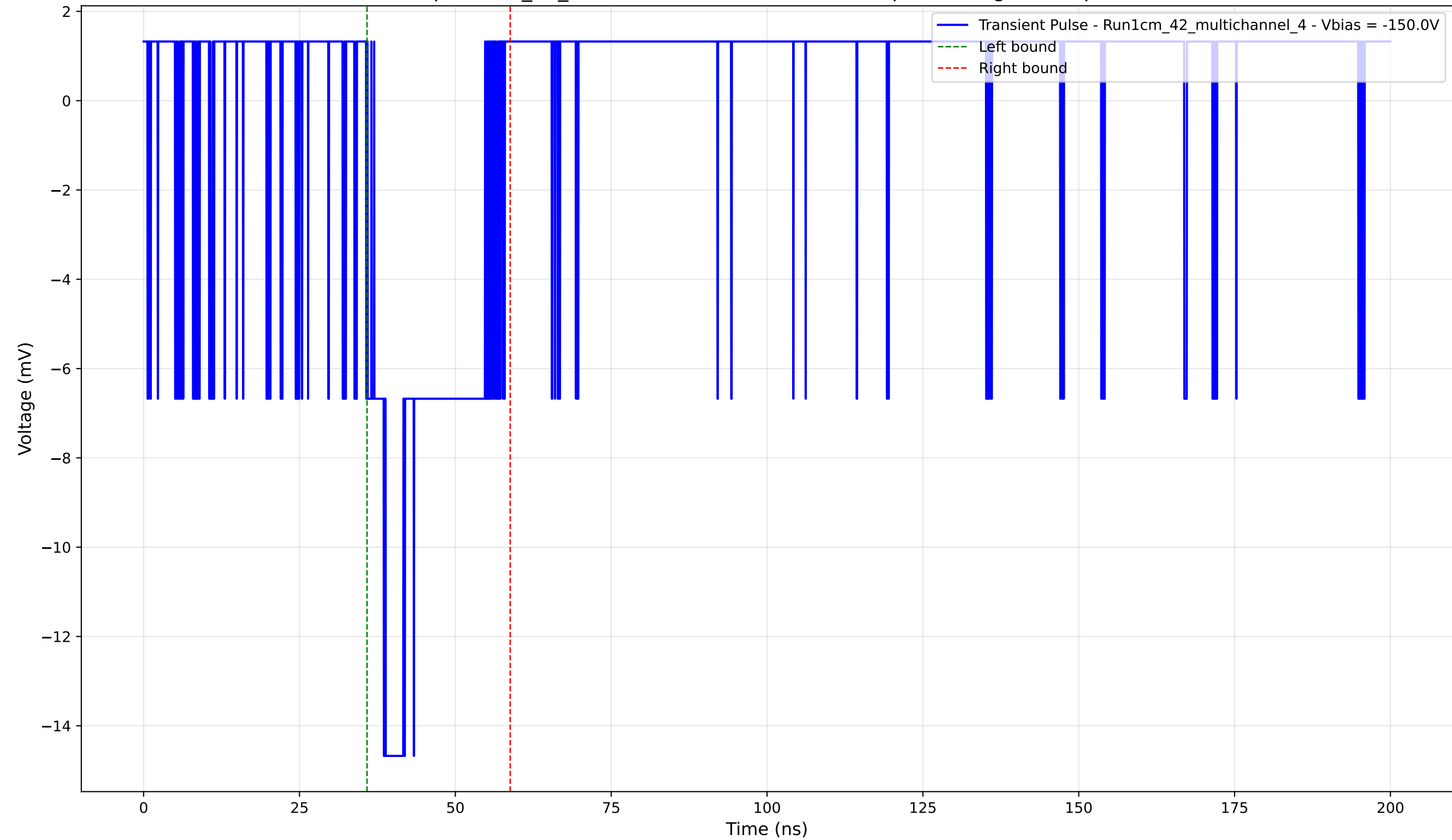
Transient Pulse - Sample: 1cm_42_multichannel - Position: 4725.0 \mu\text{m} - Charge: 3.12 pC - Rise Time: 1.54 ns
