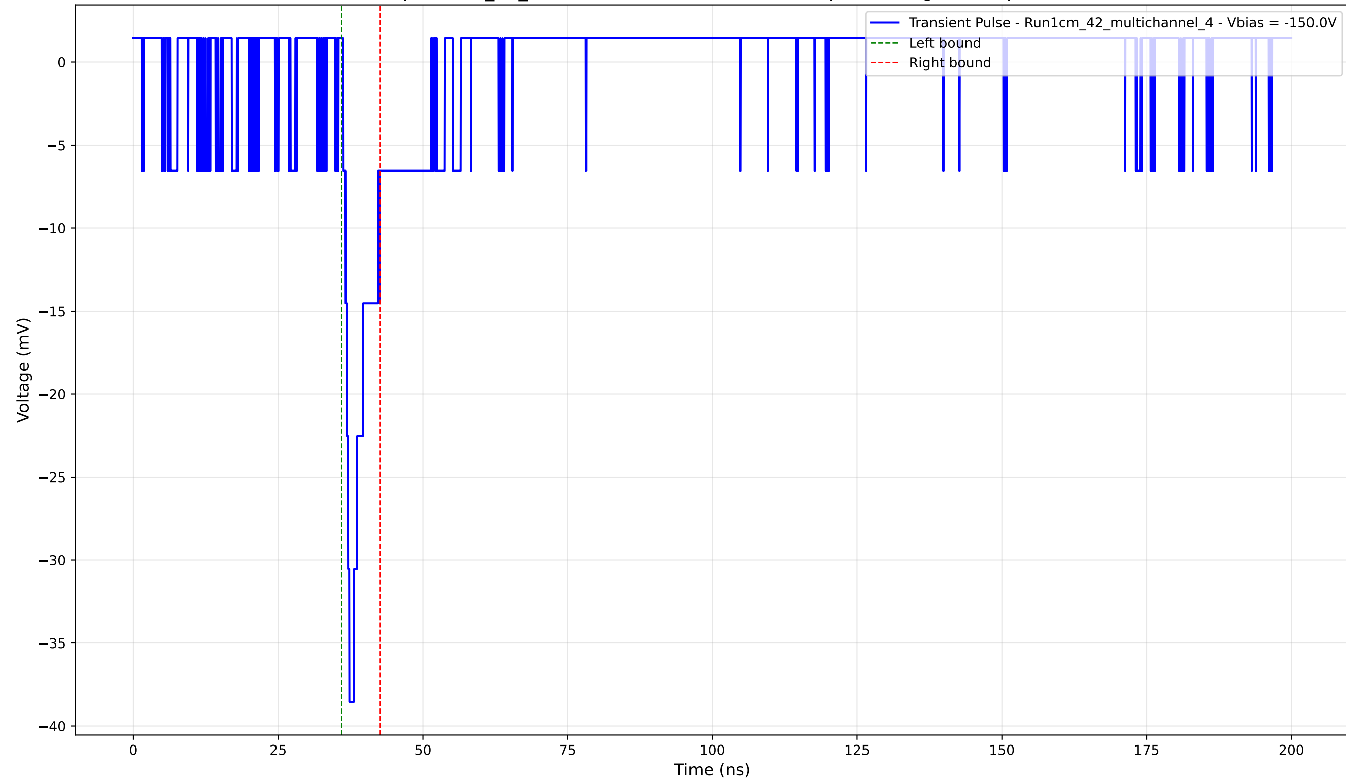
Transient Pulse - Sample: 1cm_42_multichannel - Position: 2990.0 \mu\text{m} - Charge: 2.56 pC - Rise Time: 1.01 ns
