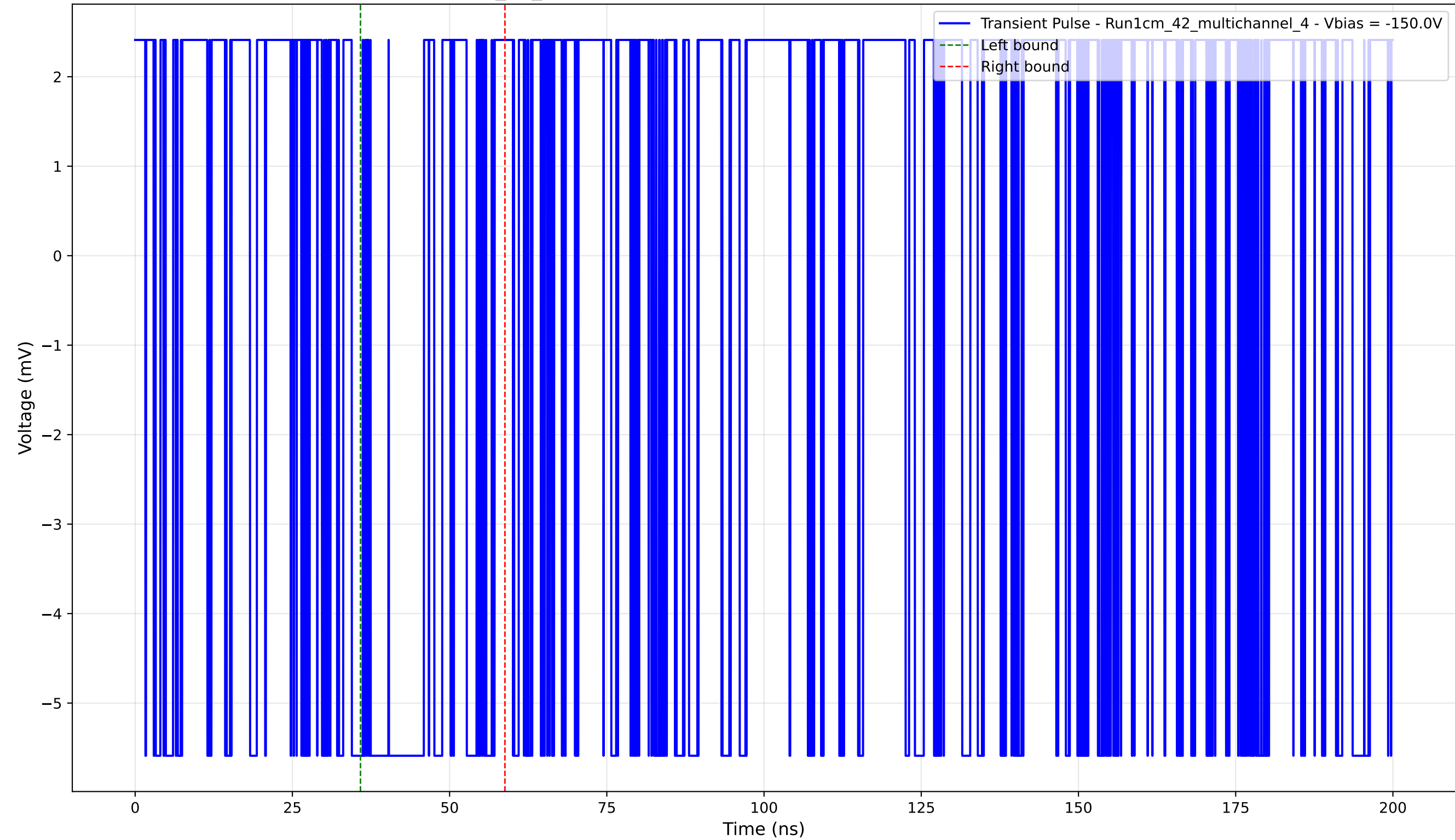
Transient Pulse - Sample: 1cm_42_multichannel - Position: 335.0 \mu\text{m} - Charge: 1.22 pC - Rise Time: 0.00 ns (N/A)
