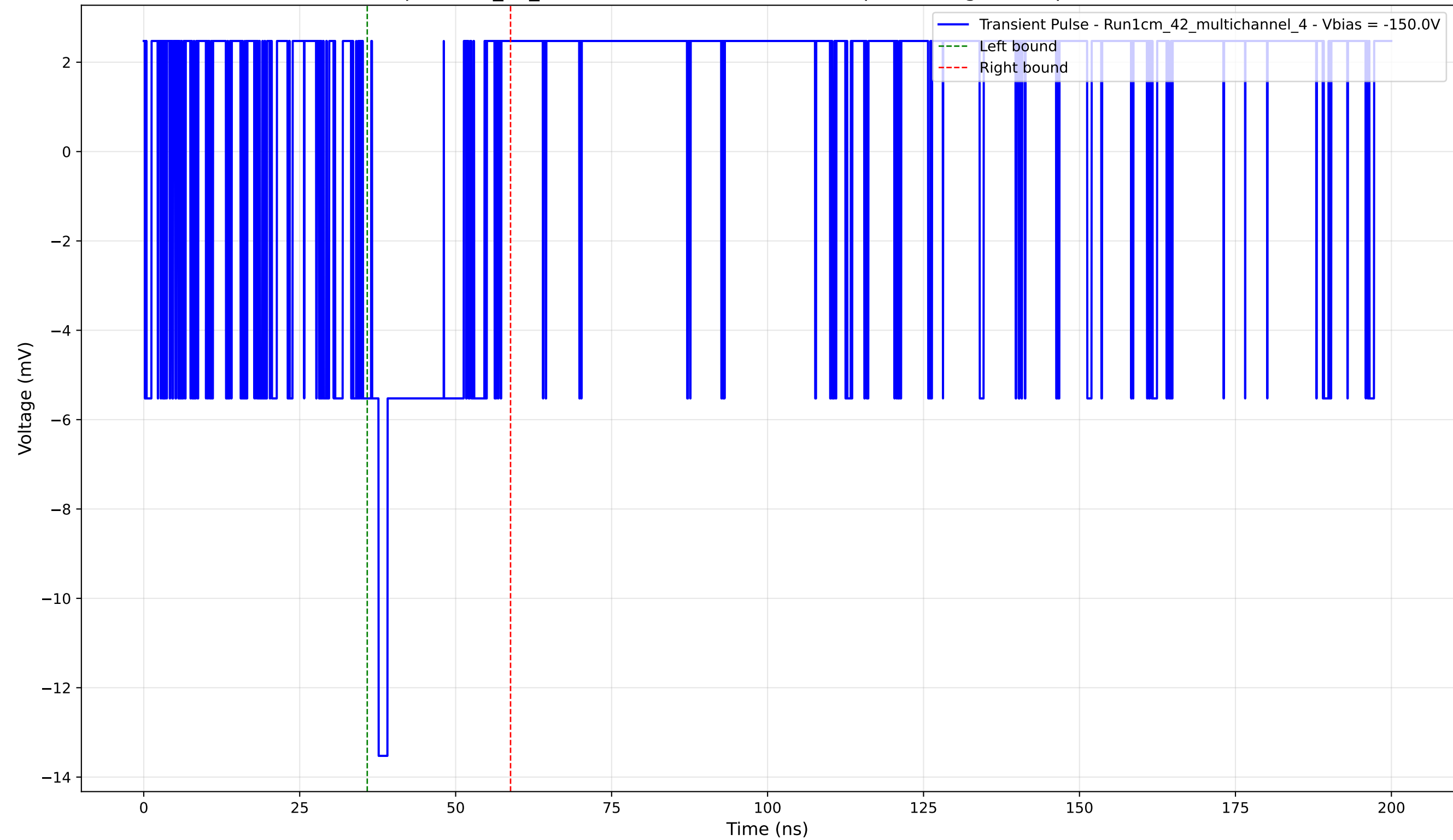
Transient Pulse - Sample: 1cm_42_multichannel - Position: 1420.0 \mu\text{m} - Charge: 1.99 pC - Rise Time: 0.00 ns (N/A)
