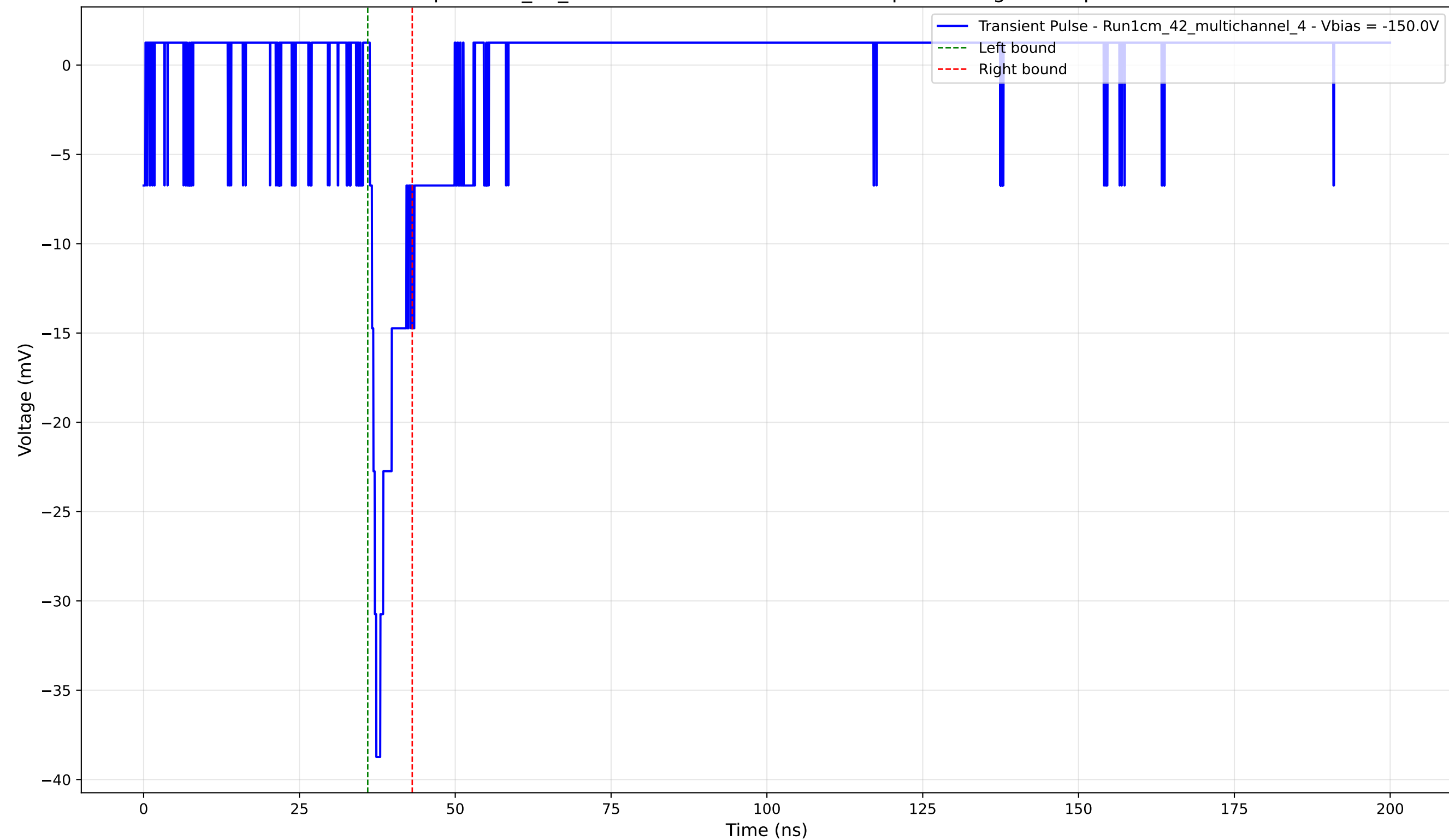
Transient Pulse - Sample: 1cm_42_multichannel - Position: 2995.0 \mu\text{m} - Charge: 2.63 pC - Rise Time: 1.03 ns
