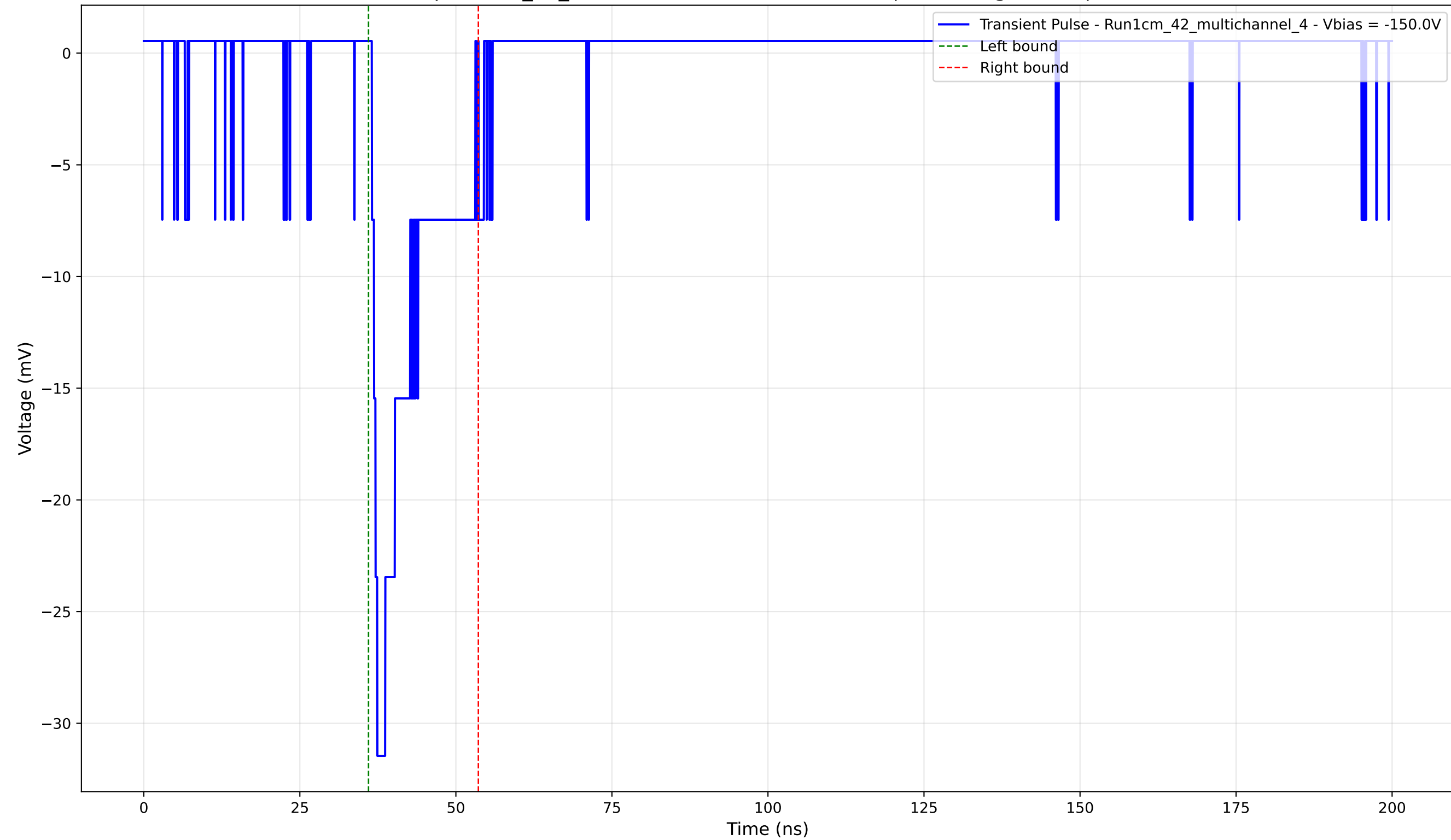
Transient Pulse - Sample: 1cm_42_multichannel - Position: 1550.0 \mu\text{m} - Charge: 4.23 pC - Rise Time: 0.87 ns
