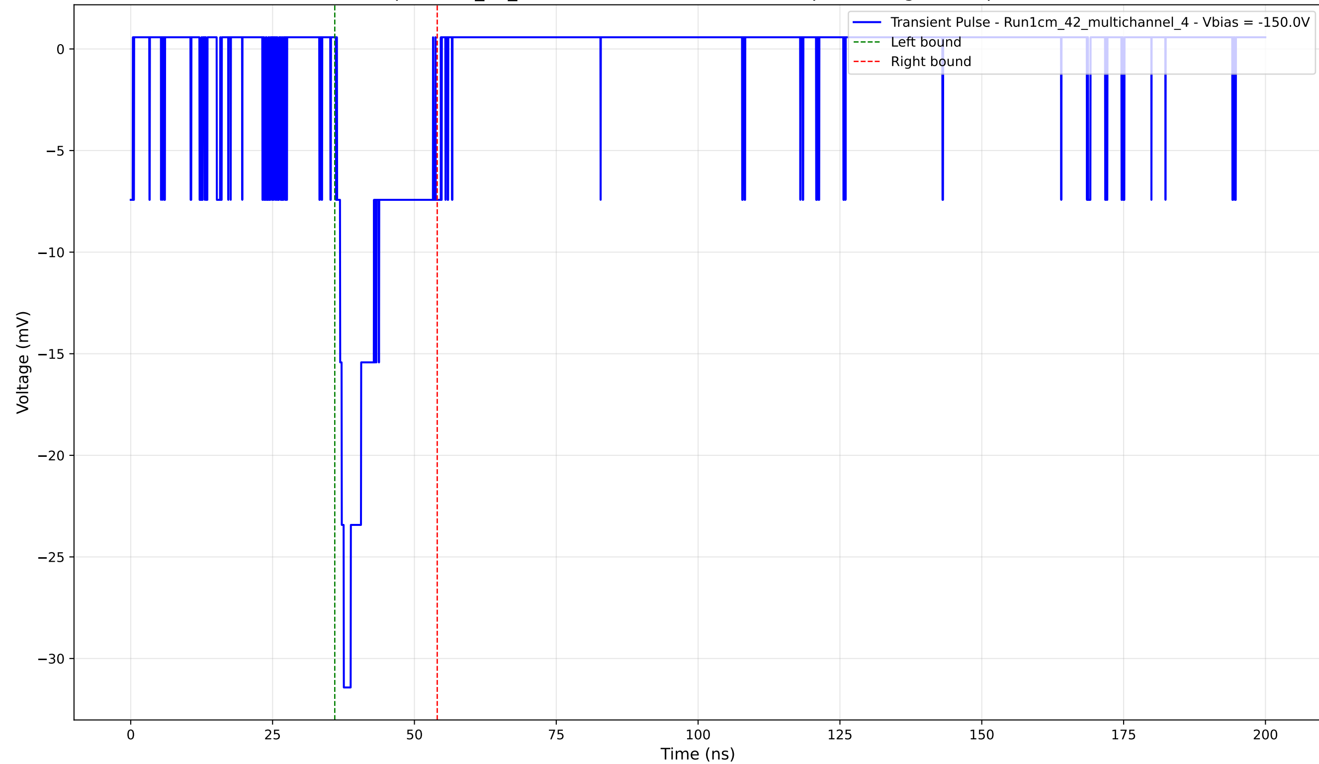
Transient Pulse - Sample: 1cm_42_multichannel - Position: 1515.0 \mu\text{m} - Charge: 4.35 pC - Rise Time: 1.19 ns
