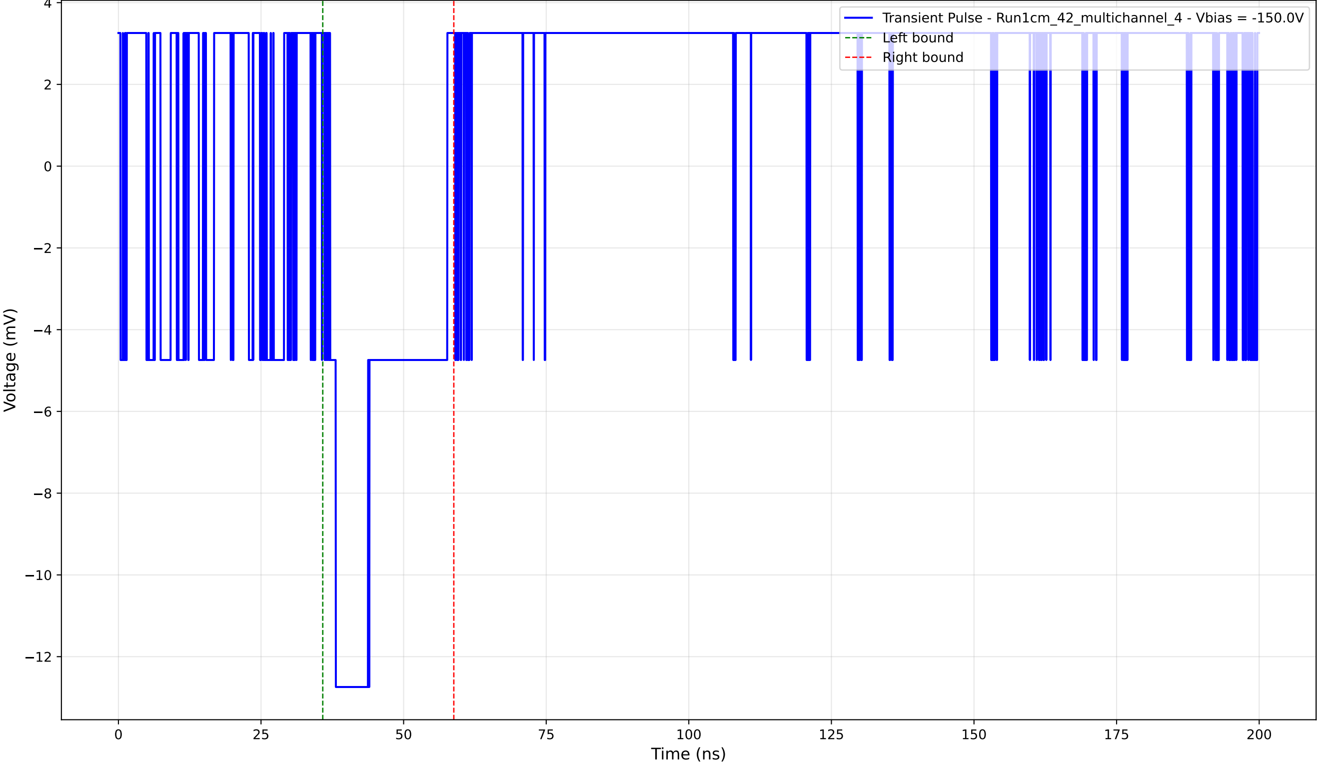
Transient Pulse - Sample: 1cm_42_multichannel - Position: 555.0 \mu\text{m} - Charge: 2.76 pC - Rise Time: 0.00 ns (N/A)
