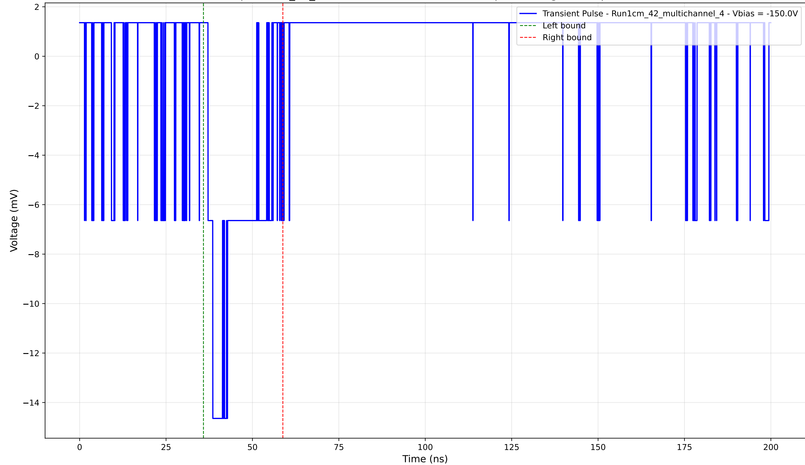
Transient Pulse - Sample: 1cm_42_multichannel - Position: 4730.0 \mu\text{m} - Charge: 2.89 pC - Rise Time: 1.40 ns
