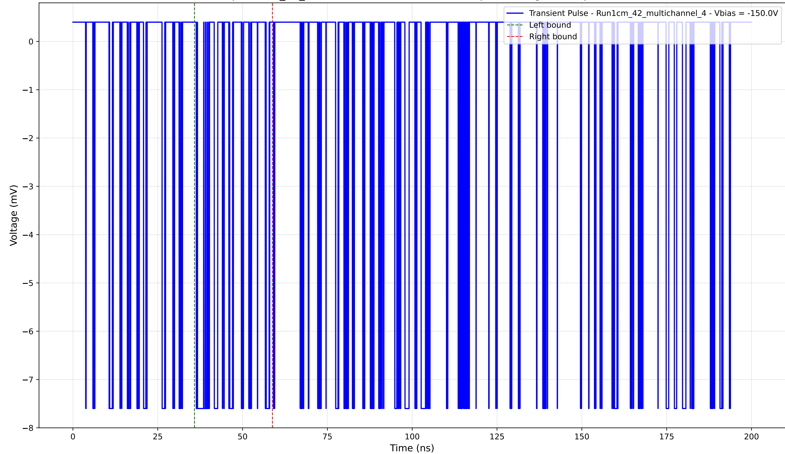
Transient Pulse - Sample: 1cm_42_multichannel - Position: 1895.0 \mu\text{m} - Charge: 1.09 pC - Rise Time: 0.02 ns
