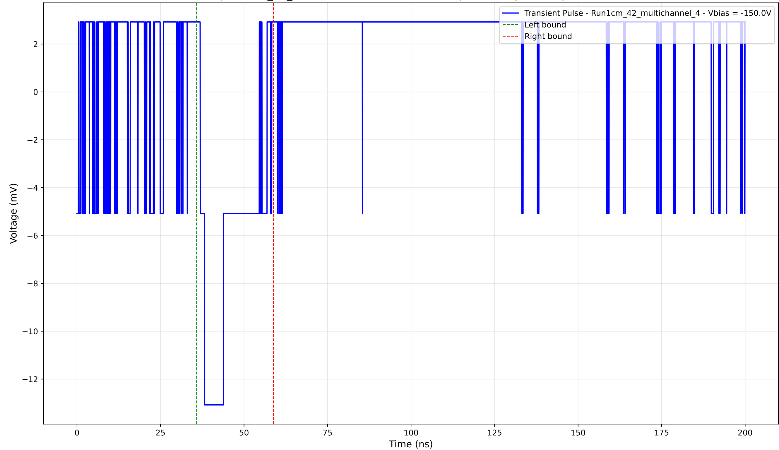
Transient Pulse - Sample: 1cm_42_multichannel - Position: 475.0 \mu\text{m} - Charge: 2.74 pC - Rise Time: 0.00 ns (N/A)
