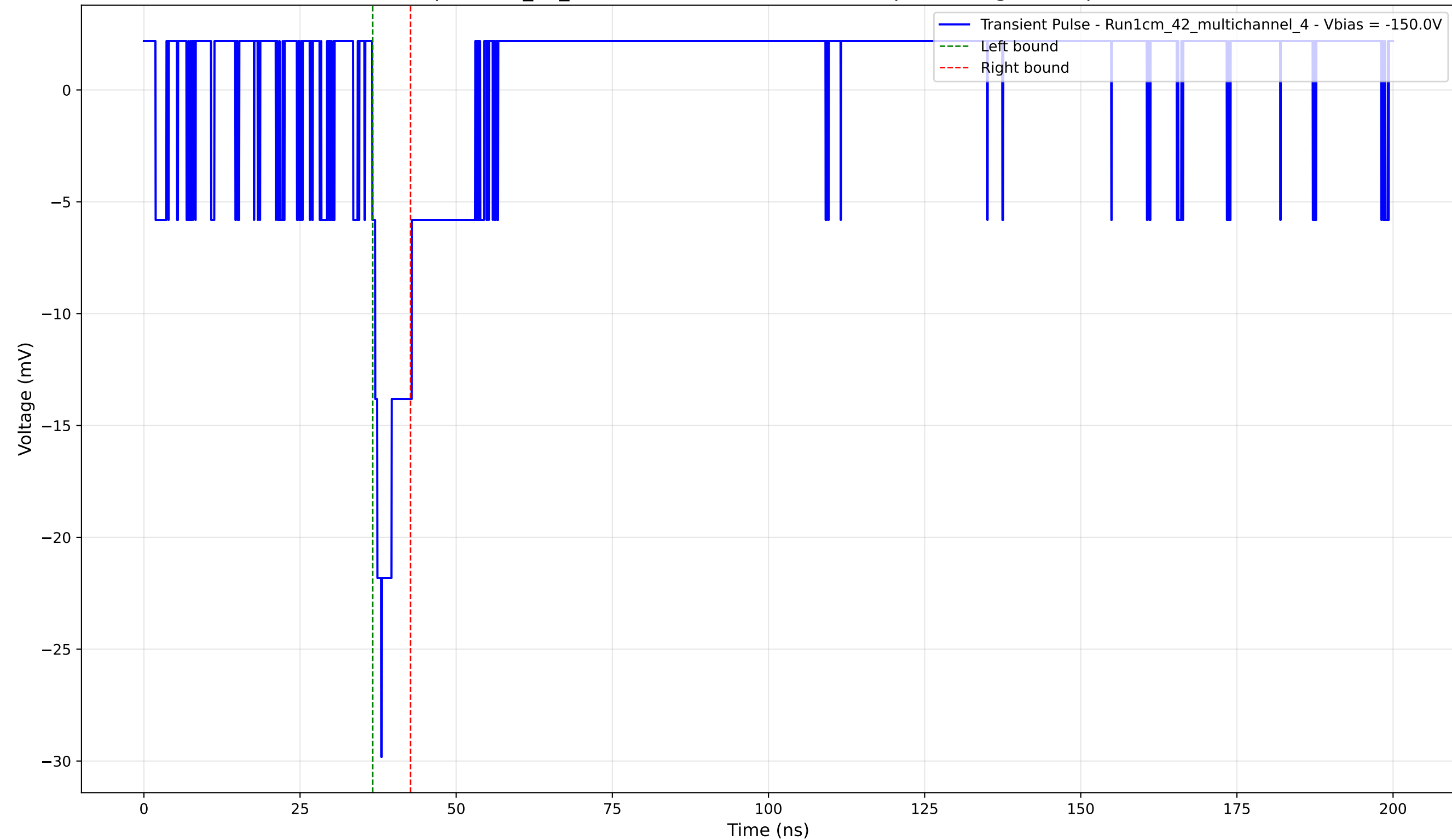
Transient Pulse - Sample: 1cm_42_multichannel - Position: 3310.0 \mu\text{m} - Charge: 2.00 pC - Rise Time: 1.44 ns
