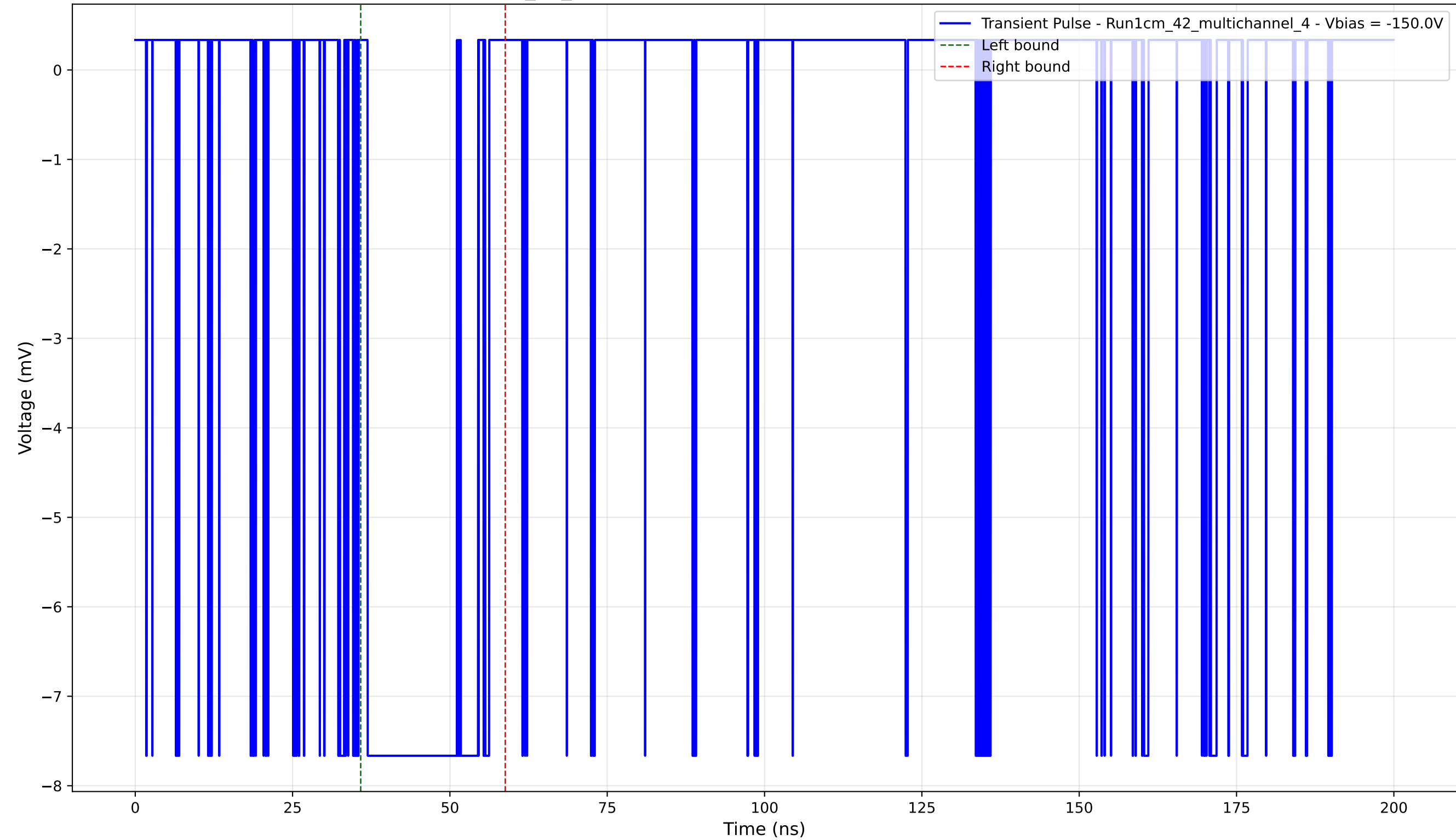
Transient Pulse - Sample: 1cm_42_multichannel - Position: 100.0 \mu\text{m} - Charge: 2.75 pC - Rise Time: 0.02 ns
