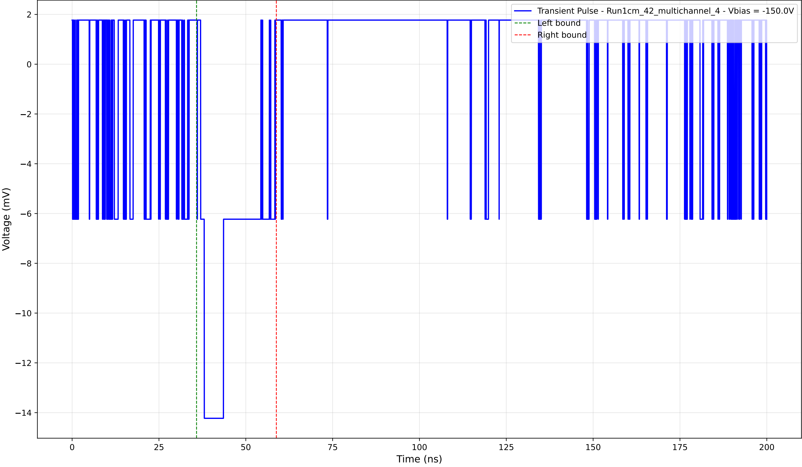
Transient Pulse - Sample: 1cm_42_multichannel - Position: 465.0 \mu\text{m} - Charge: 3.46 pC - Rise Time: 0.00 ns (N/A)
