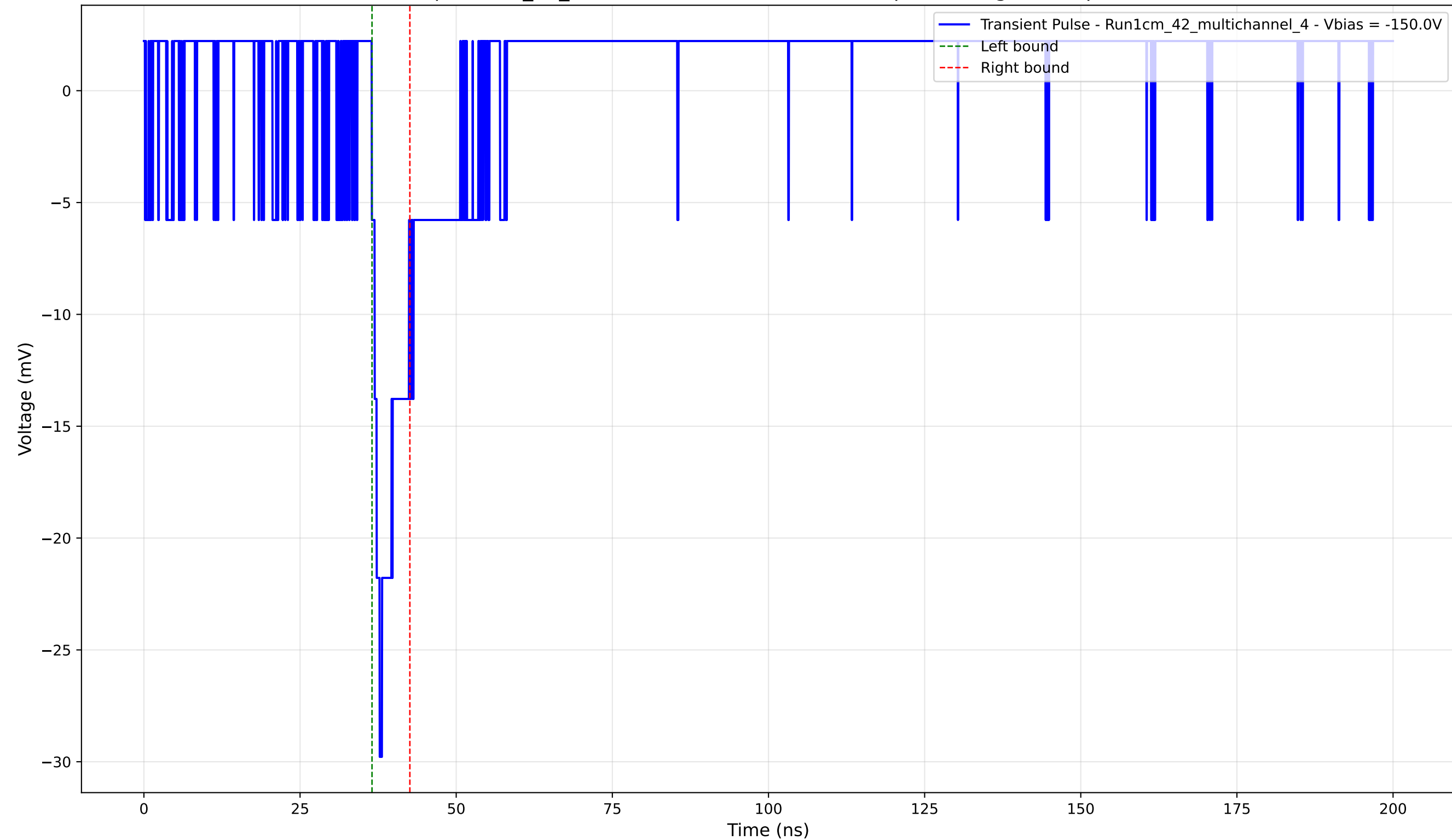
Transient Pulse - Sample: 1cm_42_multichannel - Position: 3240.0 \mu\text{m} - Charge: 2.03 pC - Rise Time: 1.28 ns
