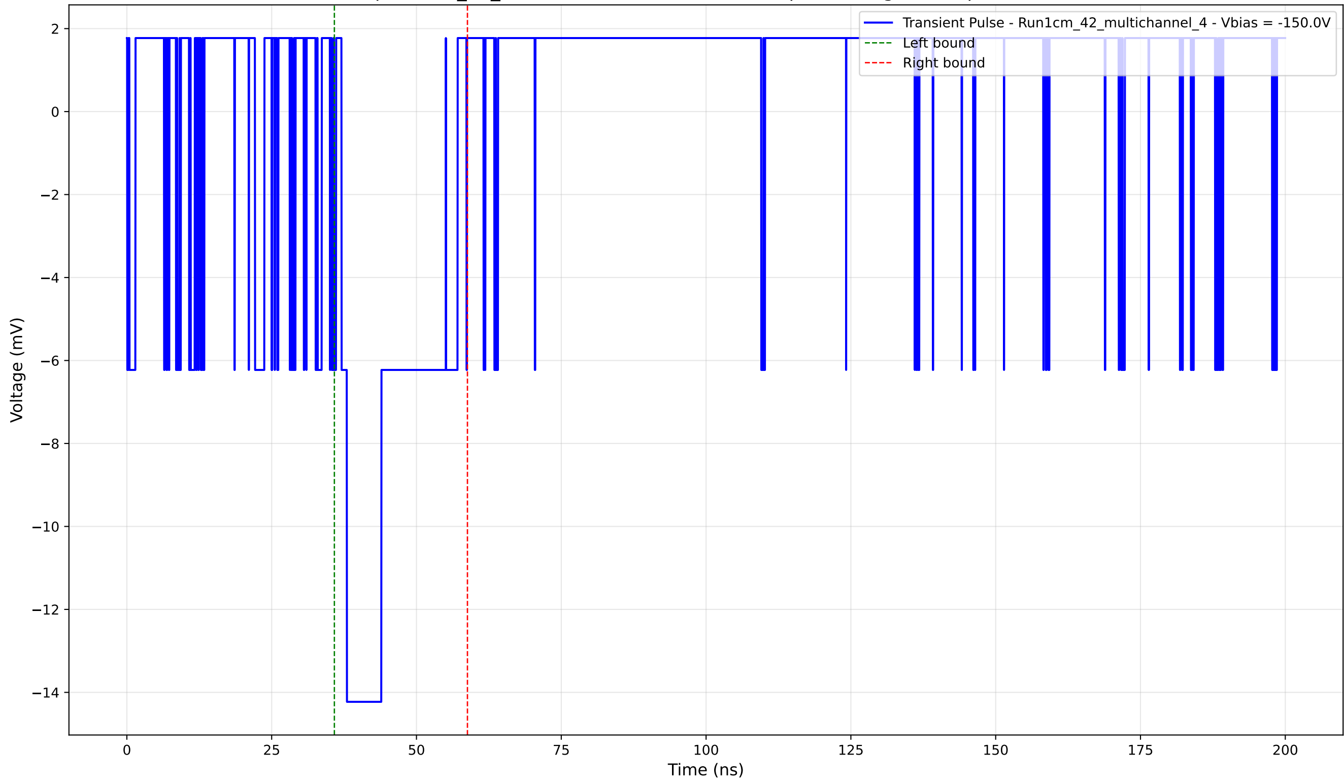
Transient Pulse - Sample: 1cm_42_multichannel - Position: 500.0 \mu\text{m} - Charge: 3.40 pC - Rise Time: 0.00 ns (N/A)
