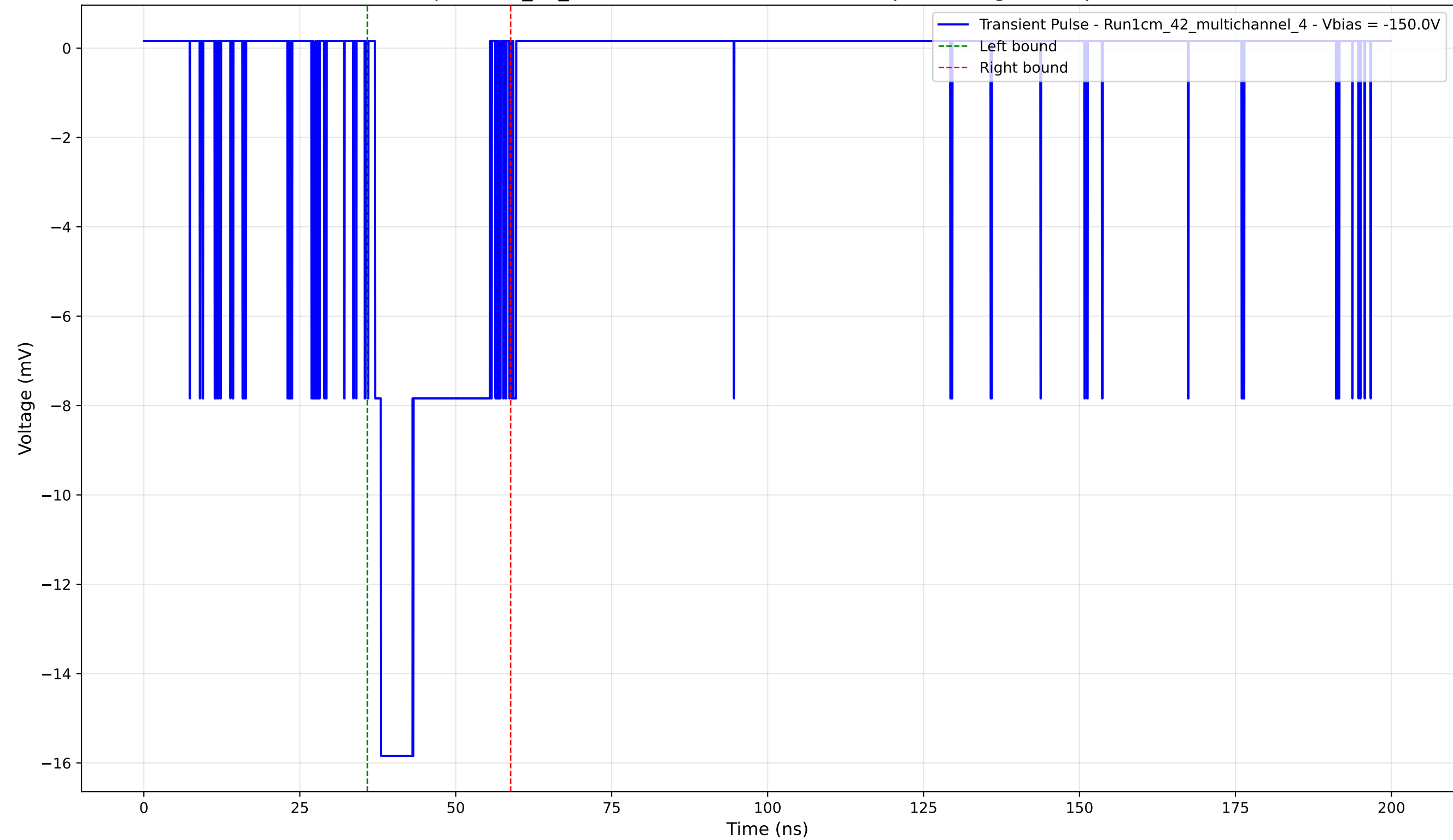
Transient Pulse - Sample: 1cm_42_multichannel - Position: 3995.0 \mu\text{m} - Charge: 3.87 pC - Rise Time: 0.96 ns
