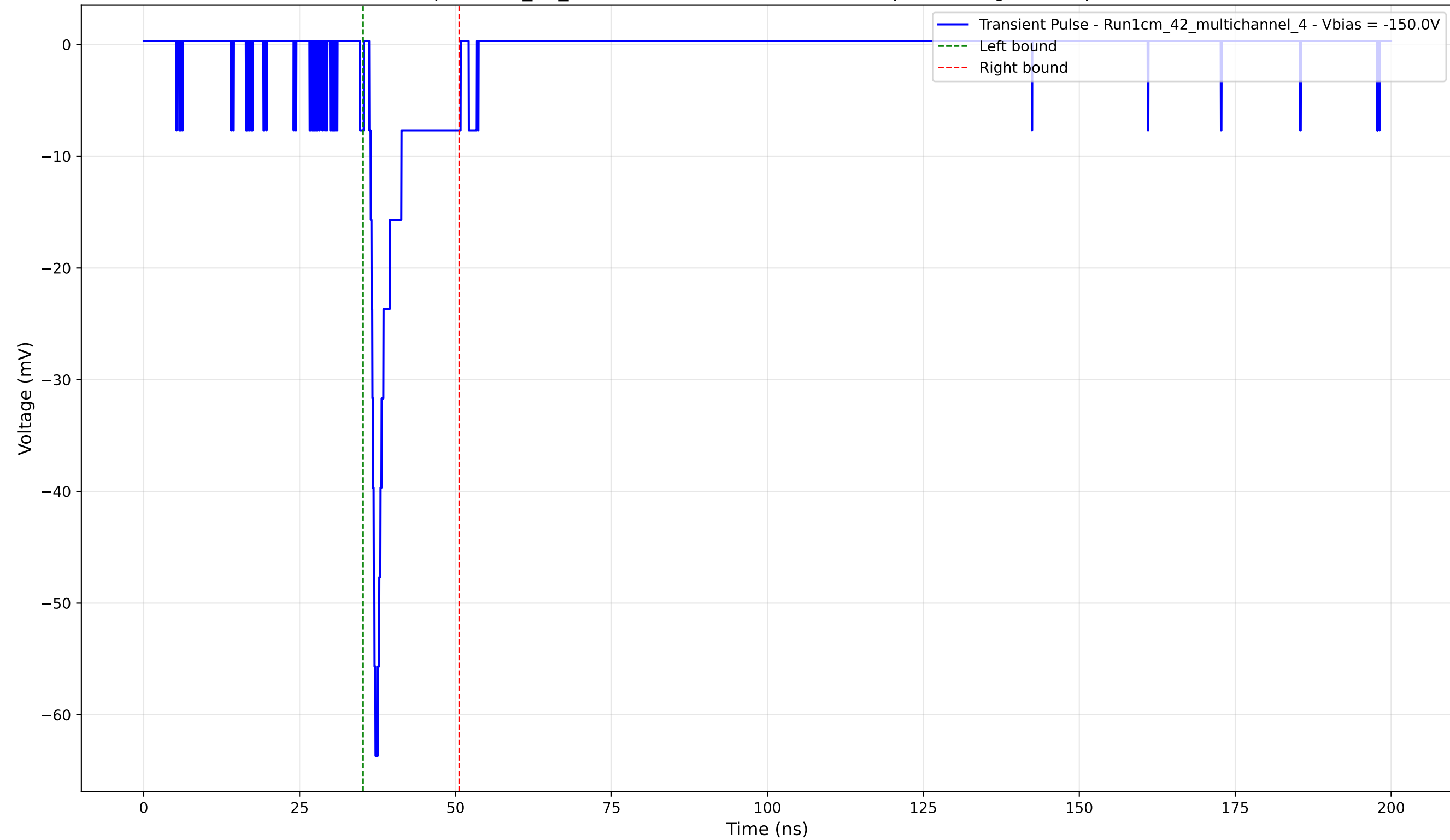
Transient Pulse - Sample: 1cm_42_multichannel - Position: 2630.0 \mu\text{m} - Charge: 4.34 pC - Rise Time: 1.00 ns
