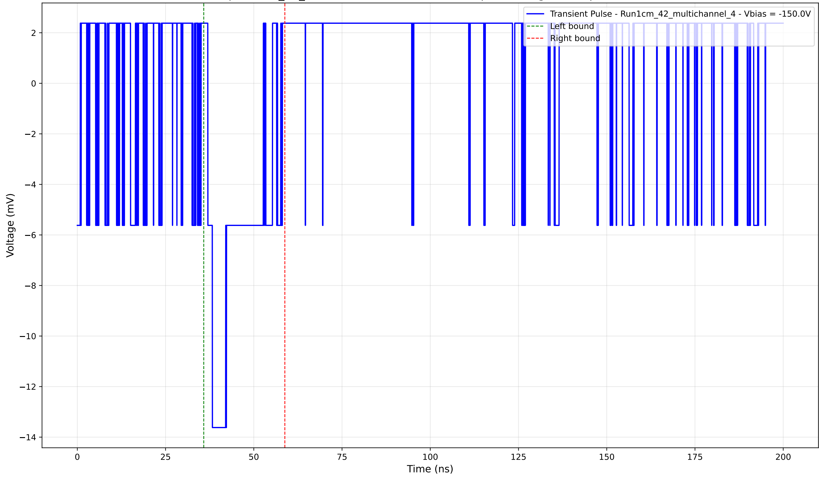
Transient Pulse - Sample: 1cm_42_multichannel - Position: 170.0 \mu\text{m} - Charge: 2.60 pC - Rise Time: 0.00 ns (N/A)
