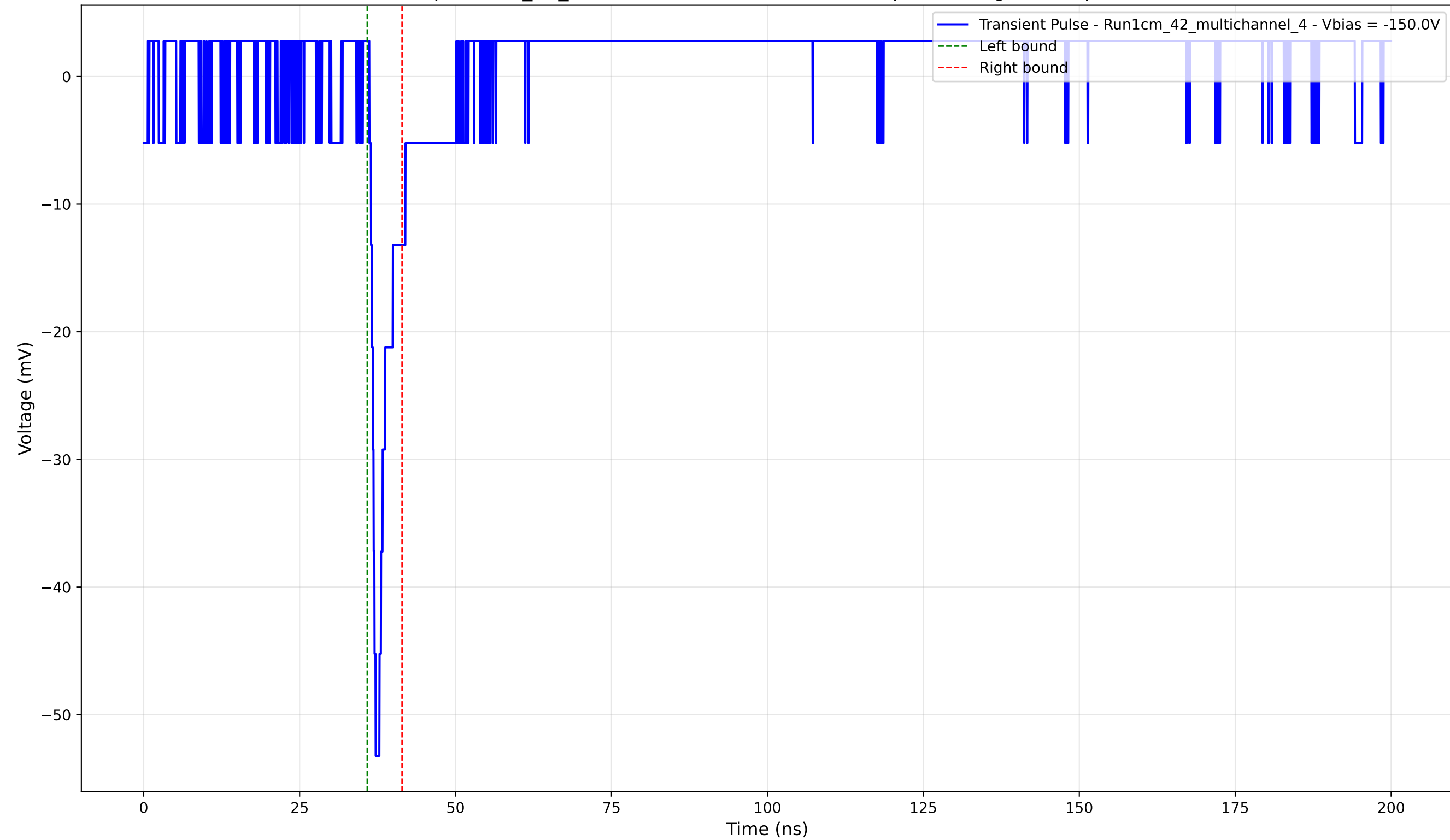
Transient Pulse - Sample: 1cm_42_multichannel - Position: 2020.0 \mu\text{m} - Charge: 2.68 pC - Rise Time: 0.76 ns
