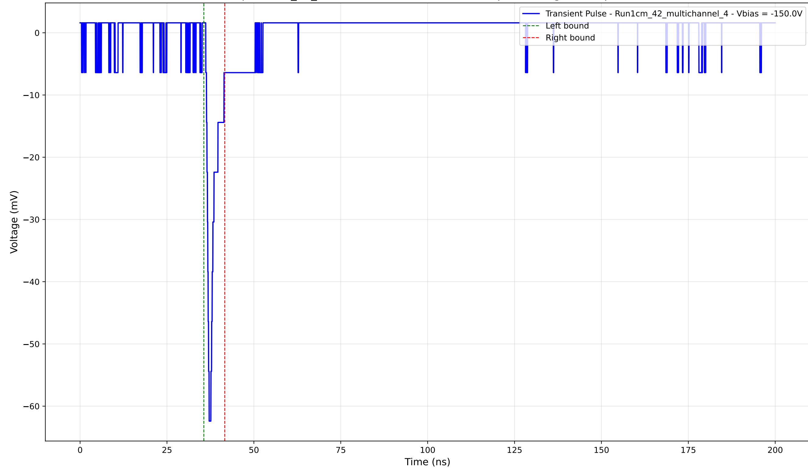
Transient Pulse - Sample: 1cm_42_multichannel - Position: 2145.0 \mu\text{m} - Charge: 2.94 pC - Rise Time: 0.96 ns
