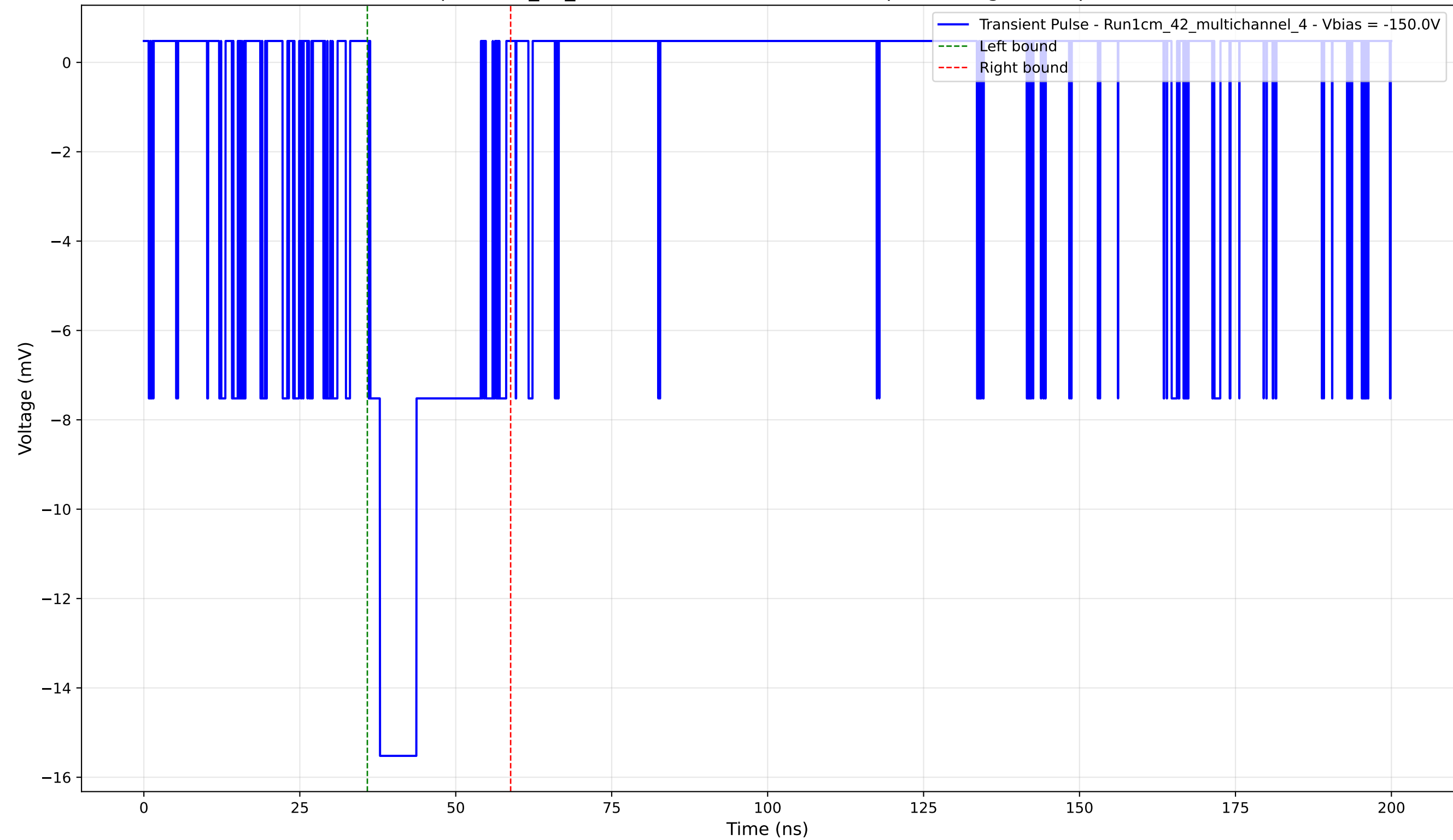
Transient Pulse - Sample: 1cm_42_multichannel - Position: 680.0 \mu\text{m} - Charge: 4.04 pC - Rise Time: 1.56 ns
