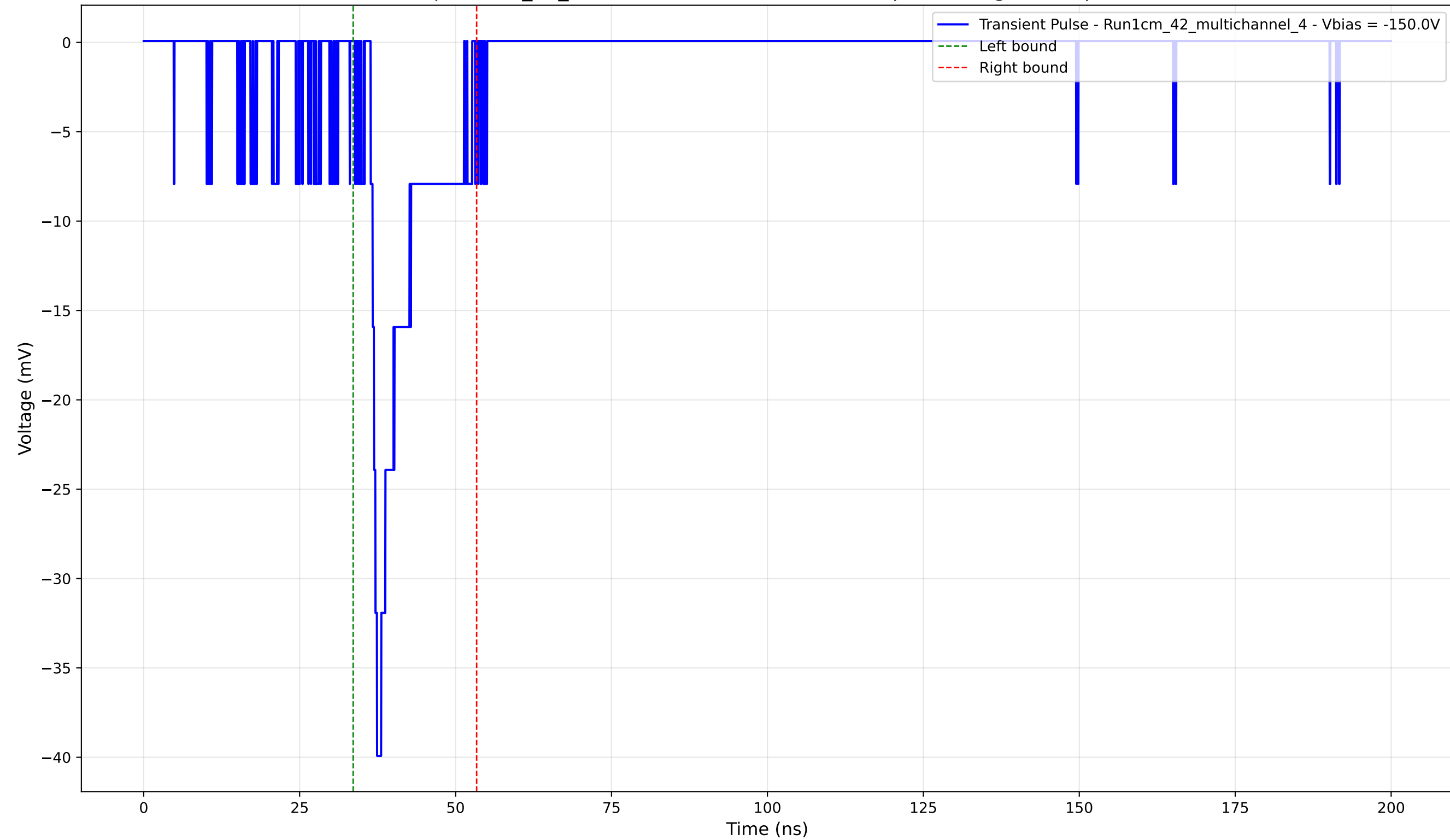
Transient Pulse - Sample: 1cm_42_multichannel - Position: 1705.0 \mu\text{m} - Charge: 4.53 pC - Rise Time: 1.03 ns
