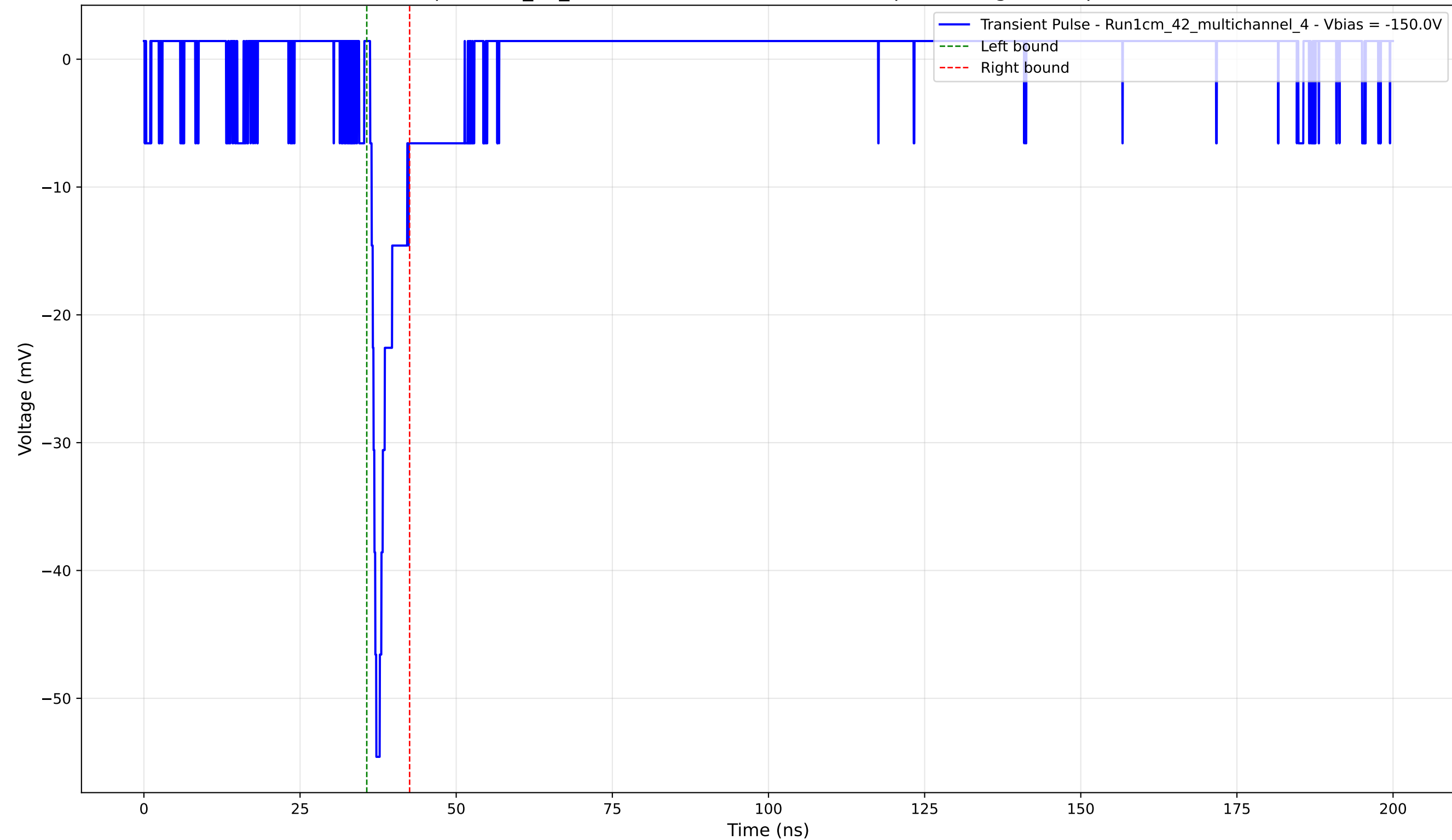
Transient Pulse - Sample: 1cm_42_multichannel - Position: 2755.0 \mu\text{m} - Charge: 2.98 pC - Rise Time: 0.98 ns
