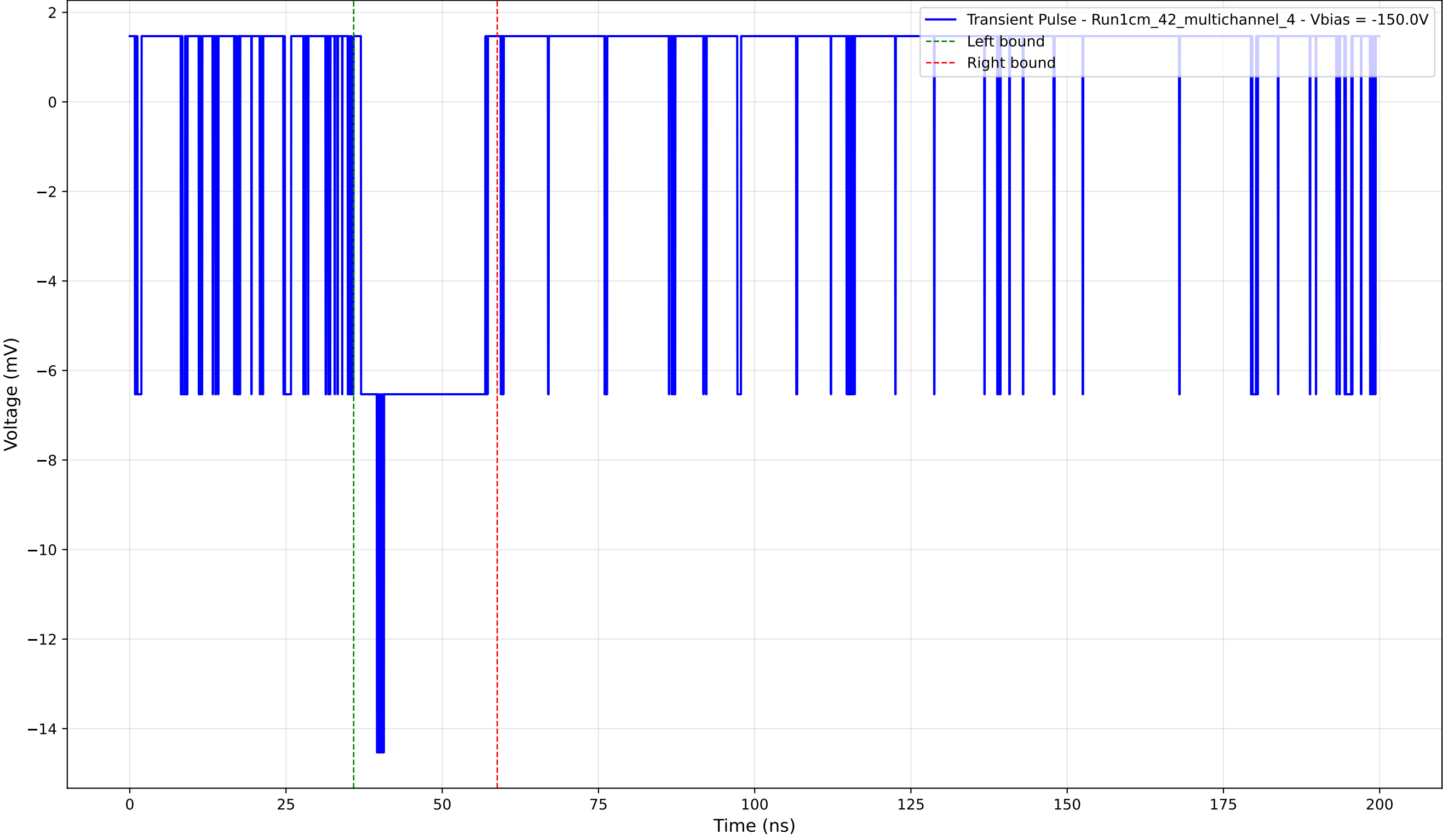
Transient Pulse - Sample: 1cm_42_multichannel - Position: 110.0 \mu\text{m} - Charge: 2.67 pC - Rise Time: 0.00 ns (N/A)
