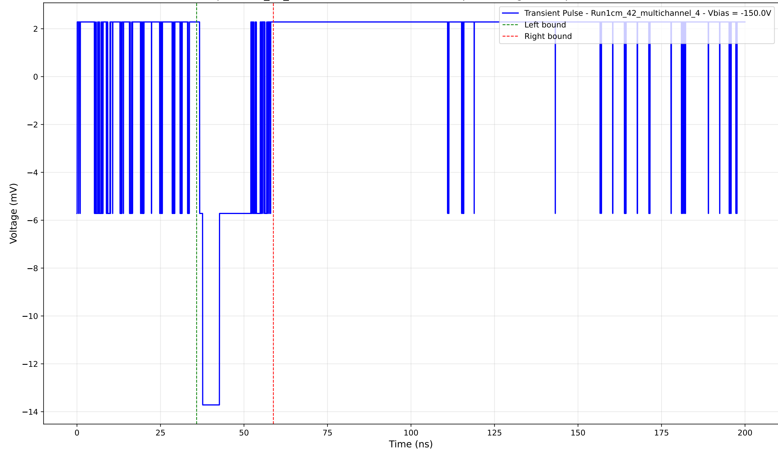
Transient Pulse - Sample: 1cm_42_multichannel - Position: 3720.0 \mu\text{m} - Charge: 2.78 pC - Rise Time: 0.00 ns (N/A)
