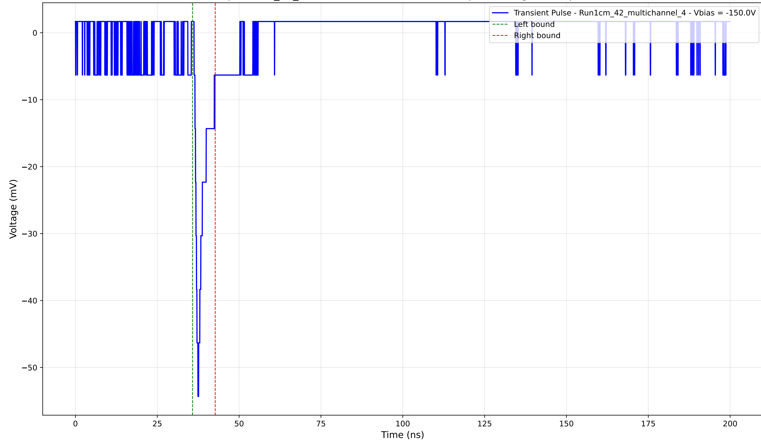
Transient Pulse - Sample: 1cm_42_multichannel - Position: 1960.0 \mu\text{m} - Charge: 2.99 pC - Rise Time: 1.18 ns
