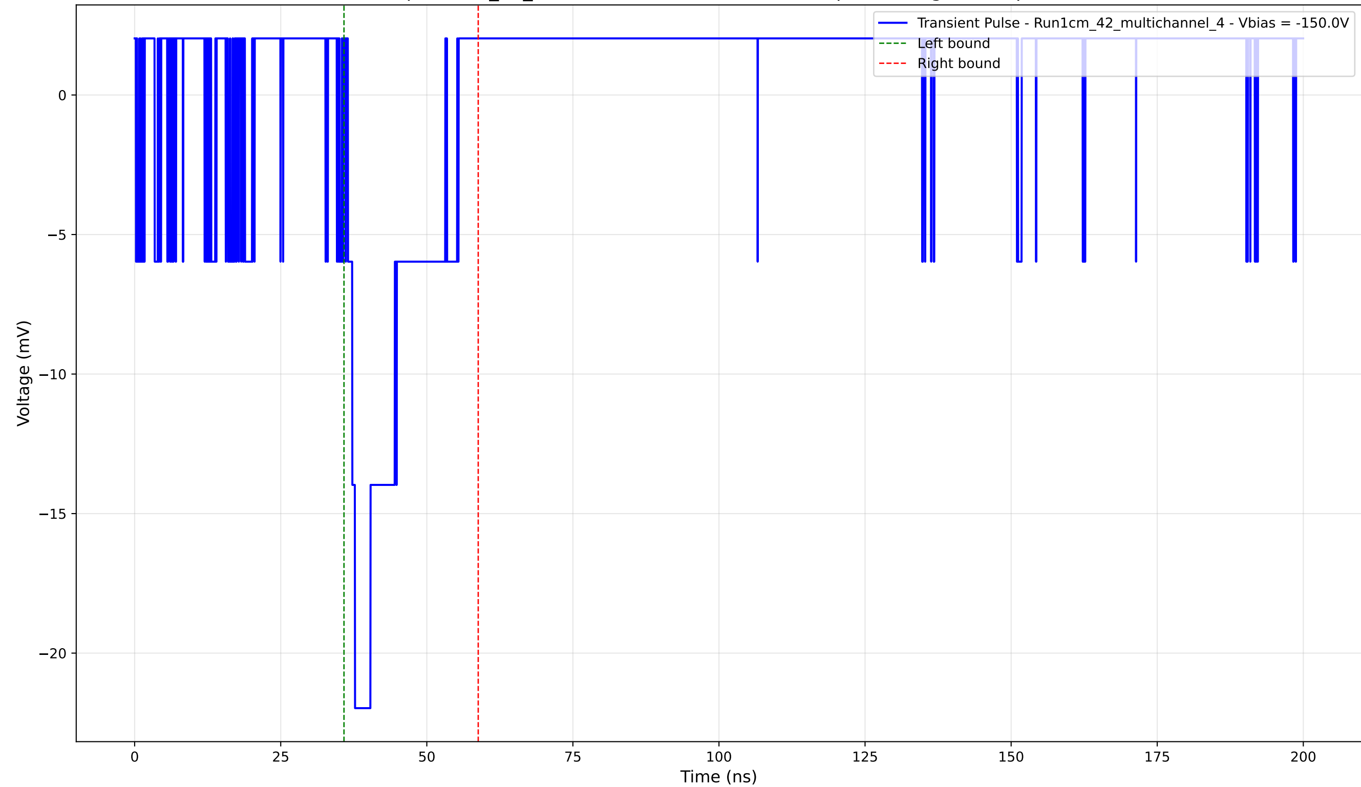
Transient Pulse - Sample: 1cm_42_multichannel - Position: 1225.0 \mu\text{m} - Charge: 3.68 pC - Rise Time: 1.22 ns
