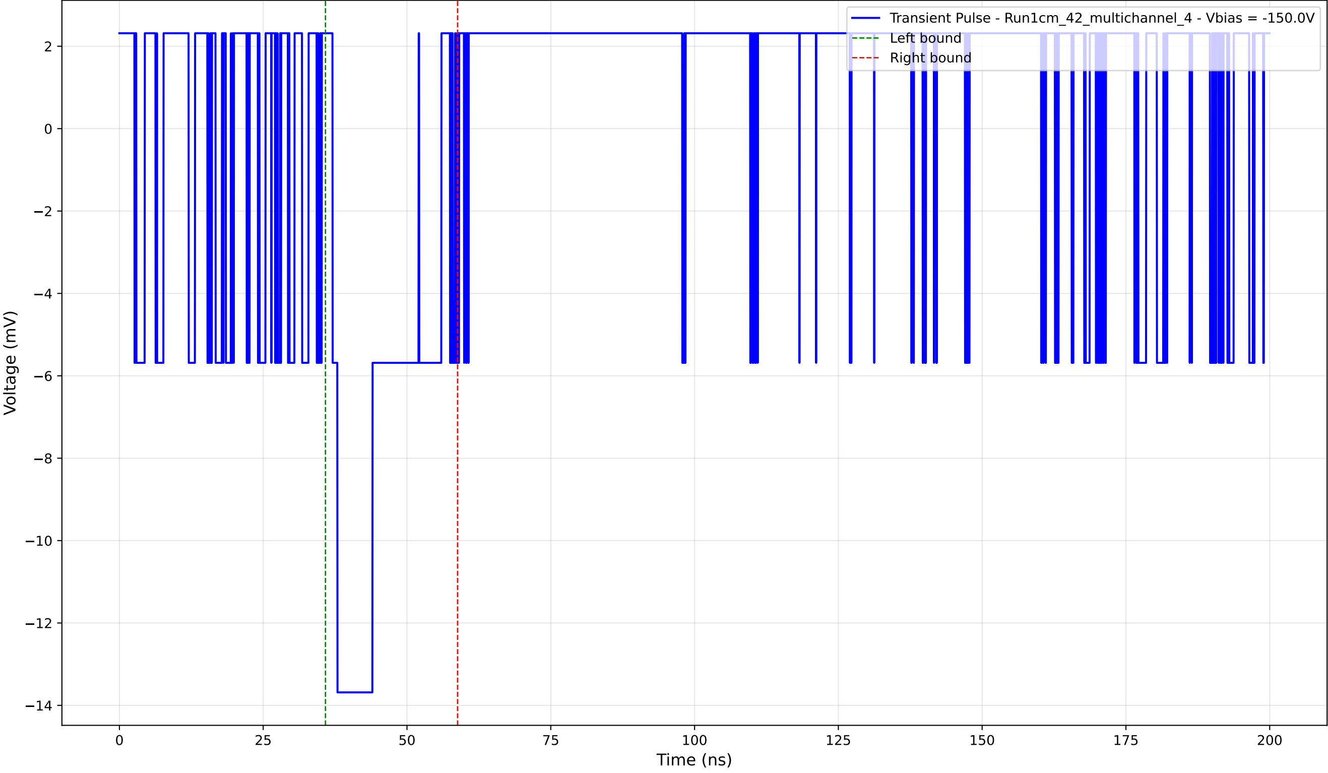
Transient Pulse - Sample: 1cm_42_multichannel - Position: 590.0 \mu\text{m} - Charge: 3.09 pC - Rise Time: 0.00 ns (N/A)
