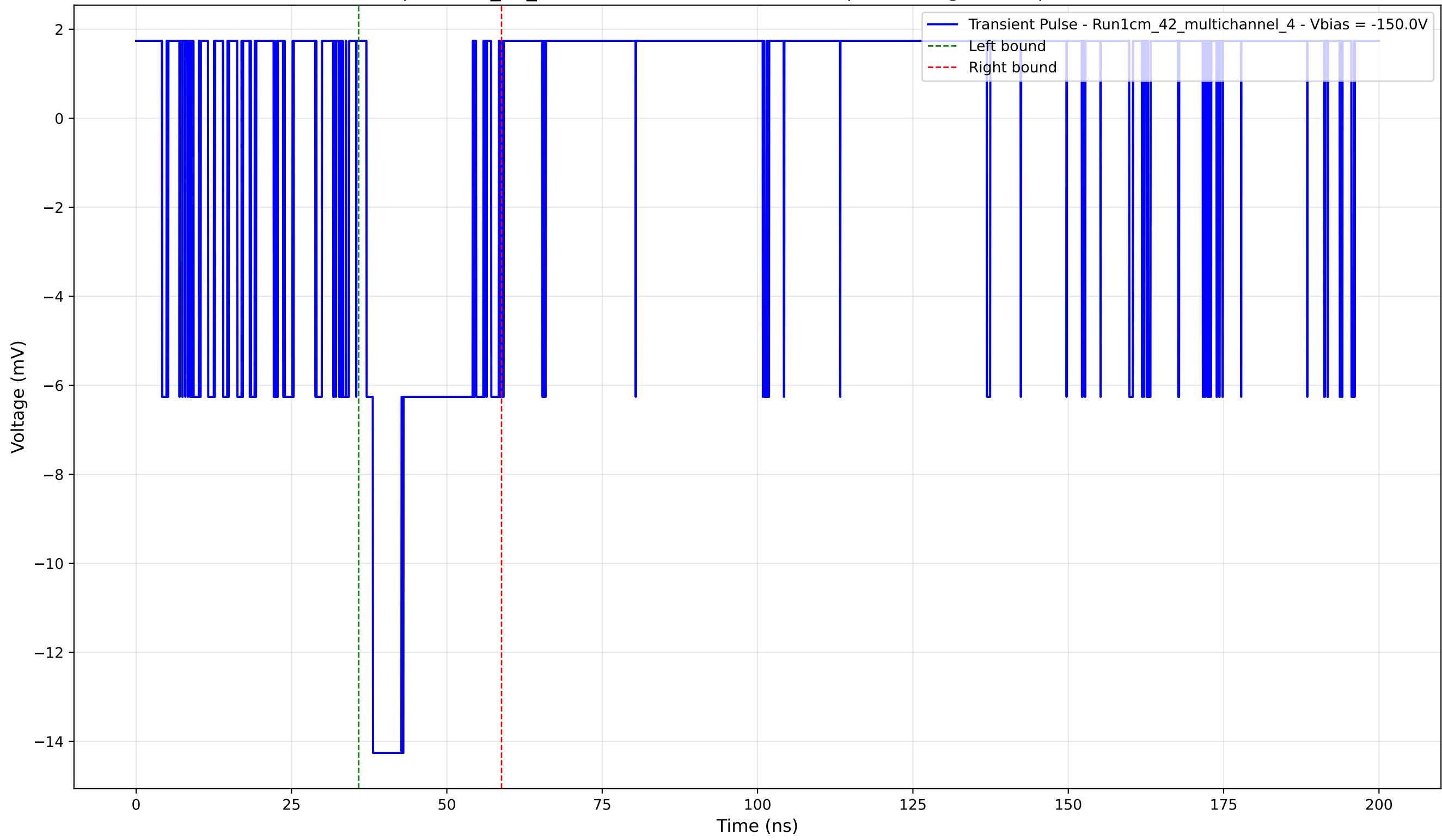
Transient Pulse - Sample: 1cm_42_multichannel - Position: 445.0 \mu\text{m} - Charge: 3.17 pC - Rise Time: 0.00 ns (N/A)
