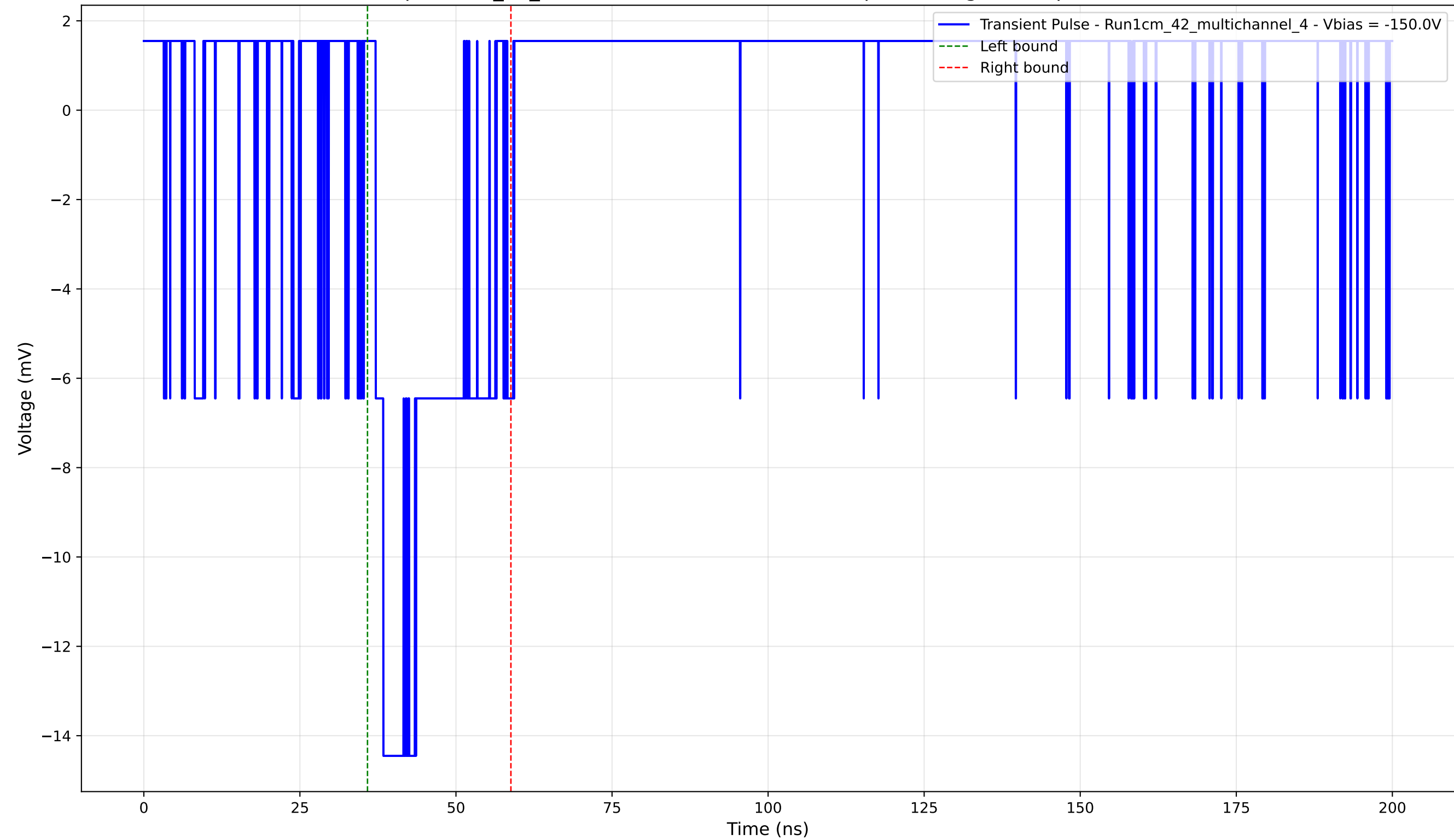
Transient Pulse - Sample: 1cm_42_multichannel - Position: 4565.0 \mu\text{m} - Charge: 3.21 pC - Rise Time: 0.00 ns (N/A)
