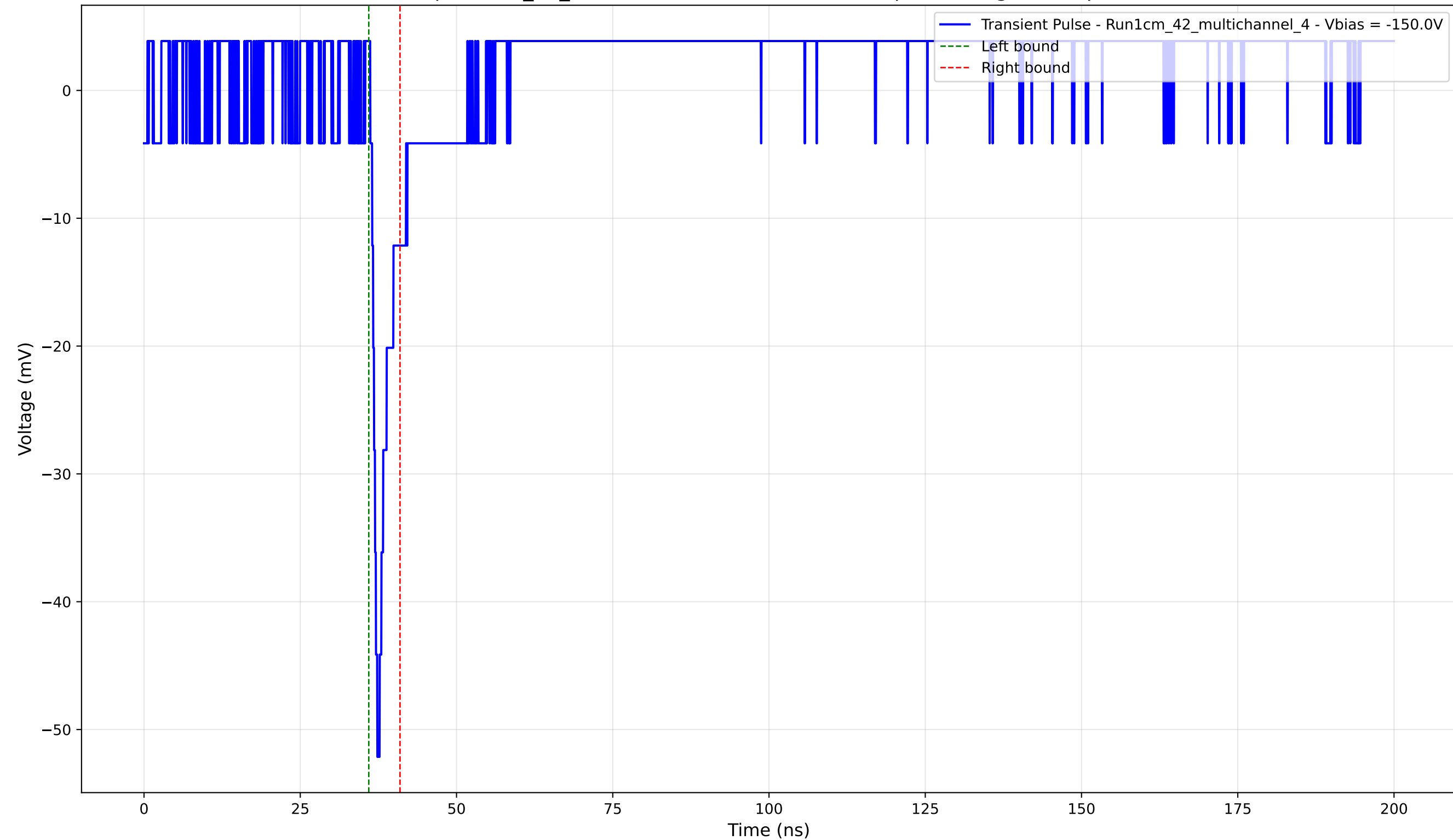
Transient Pulse - Sample: 1cm_42_multichannel - Position: 1965.0 \mu\text{m} - Charge: 2.34 pC - Rise Time: 0.84 ns
