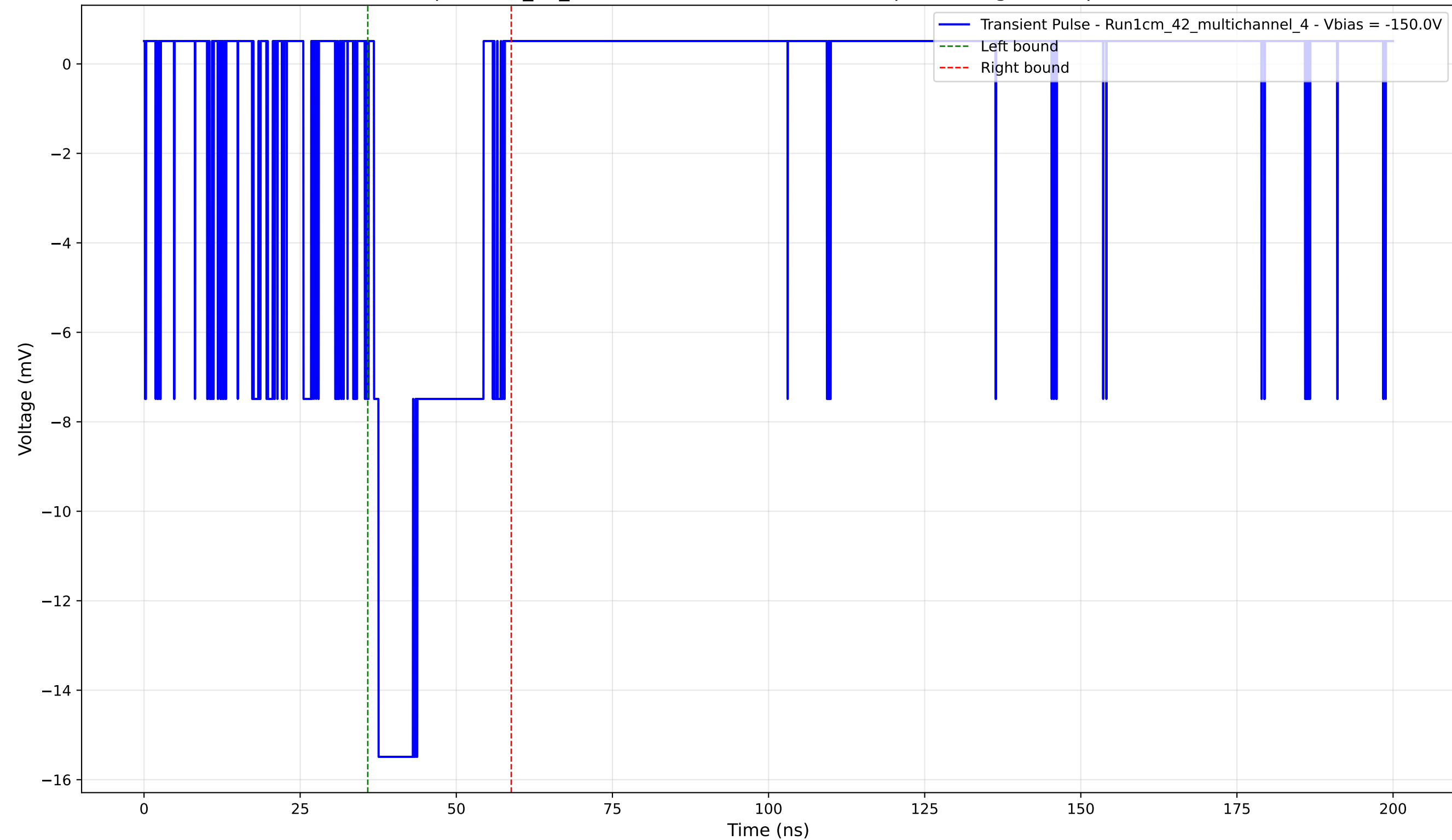
Transient Pulse - Sample: 1cm_42_multichannel - Position: 3755.0 \mu\text{m} - Charge: 3.76 pC - Rise Time: 0.74 ns
