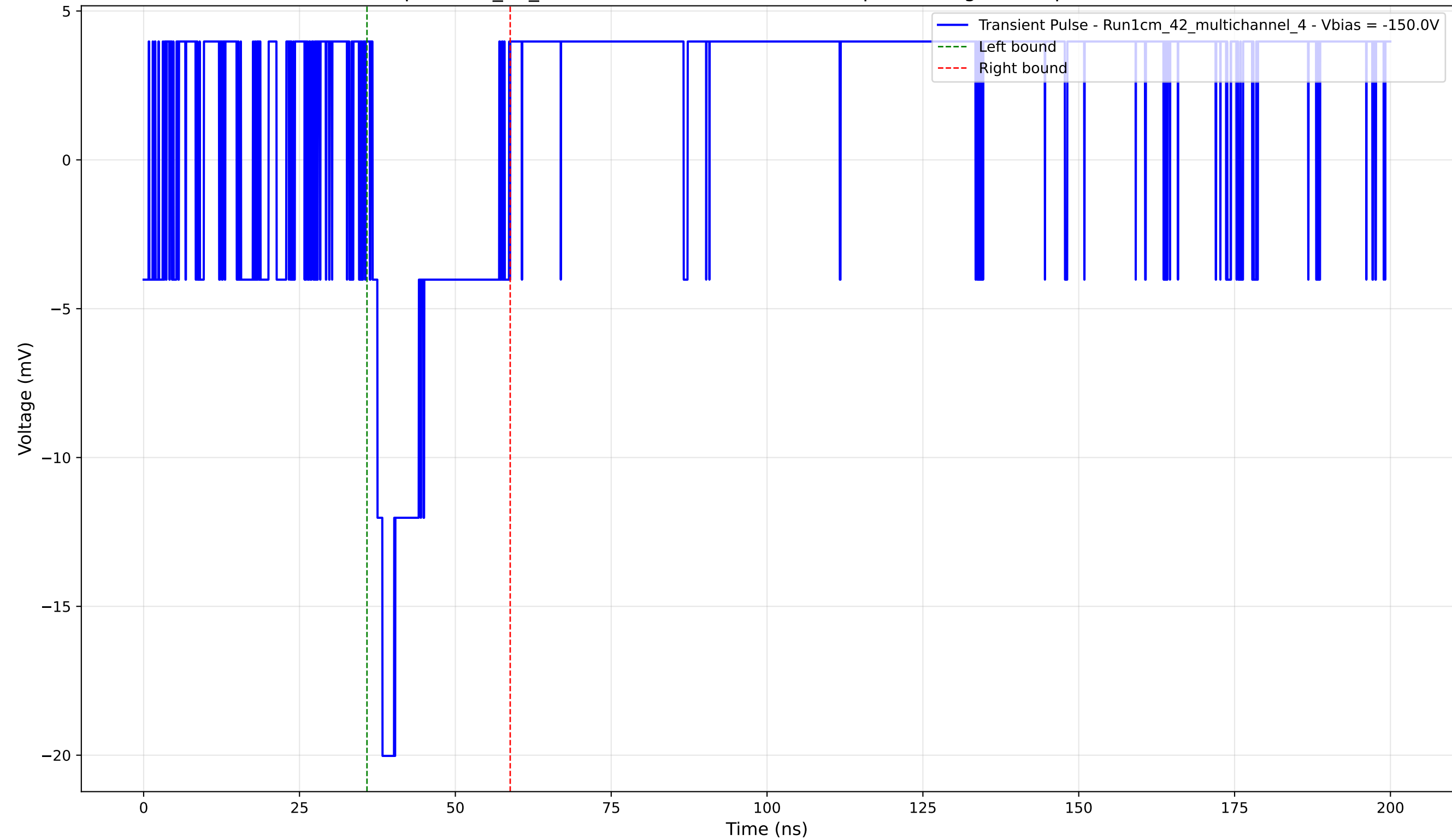
Transient Pulse - Sample: 1cm_42_multichannel - Position: 1000.0 \mu\text{m} - Charge: 3.04 pC - Rise Time: 0.00 ns (N/A)
