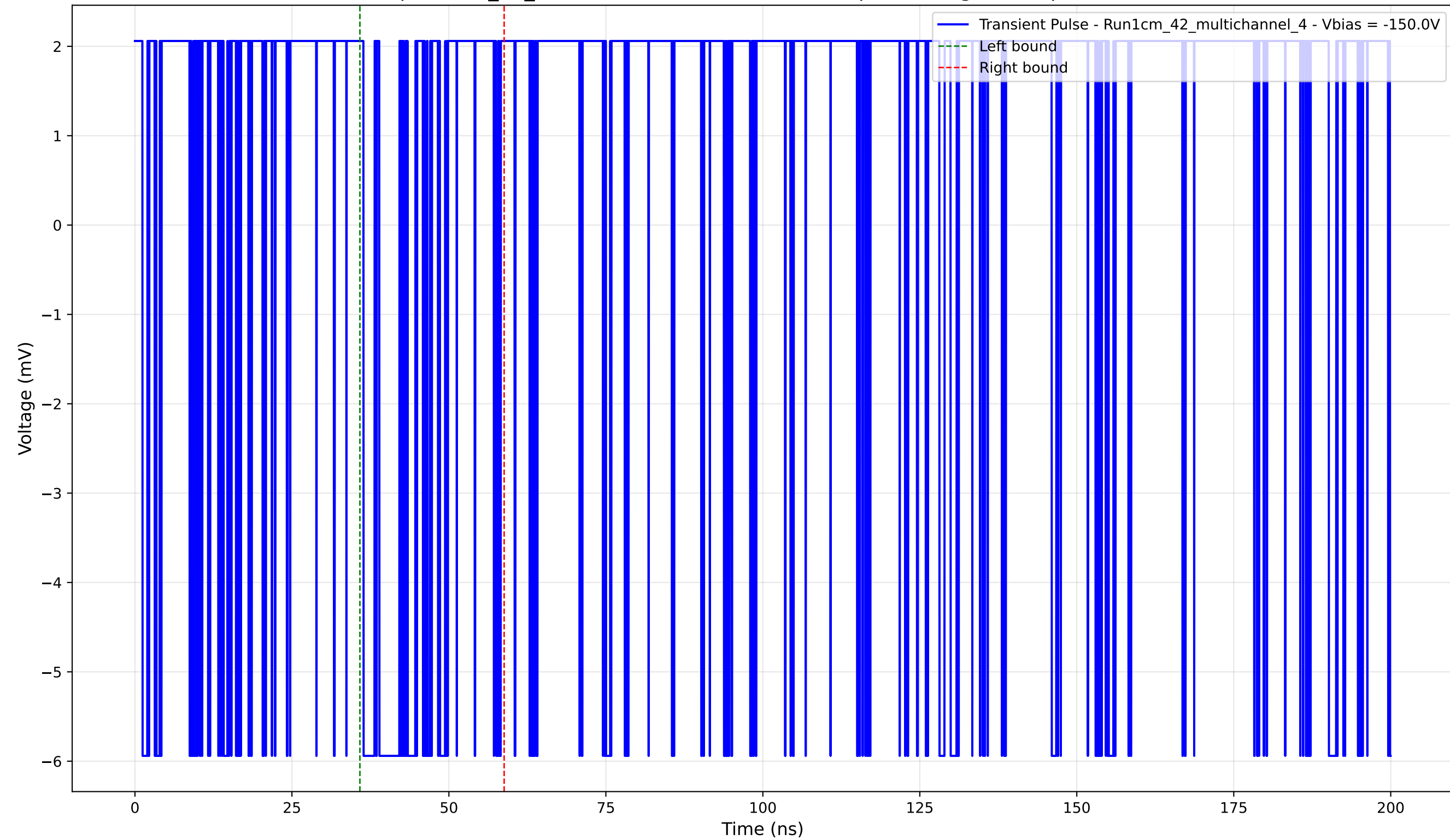
Transient Pulse - Sample: 1cm_42_multichannel - Position: 4430.0 \mu\text{m} - Charge: 0.67 pC - Rise Time: 0.00 ns (N/A)
