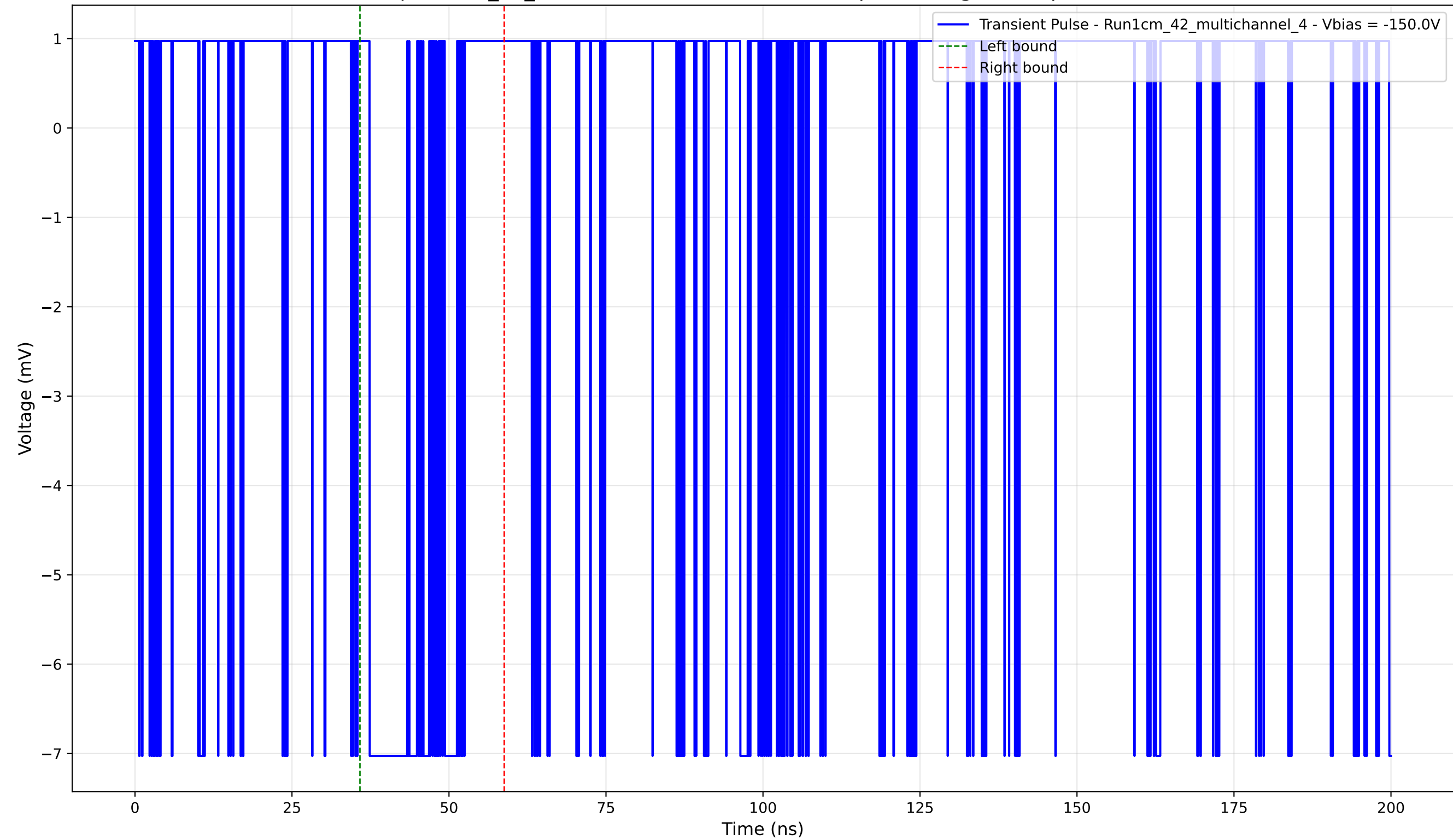
Transient Pulse - Sample: 1cm_42_multichannel - Position: 4870.0 \mu\text{m} - Charge: 1.51 pC - Rise Time: 0.00 ns (N/A)
