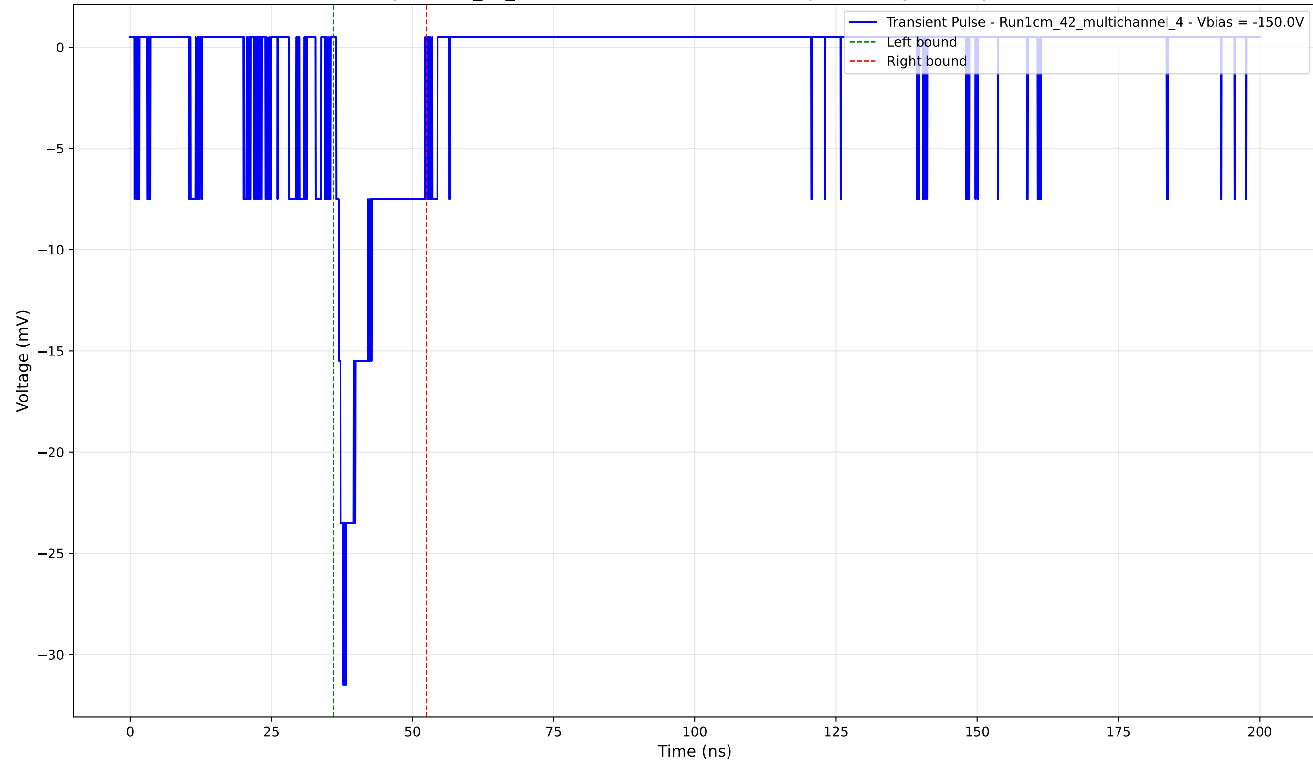
Transient Pulse - Sample: 1cm_42_multichannel - Position: 3270.0 \mu\text{m} - Charge: 3.75 pC - Rise Time: 1.29 ns
