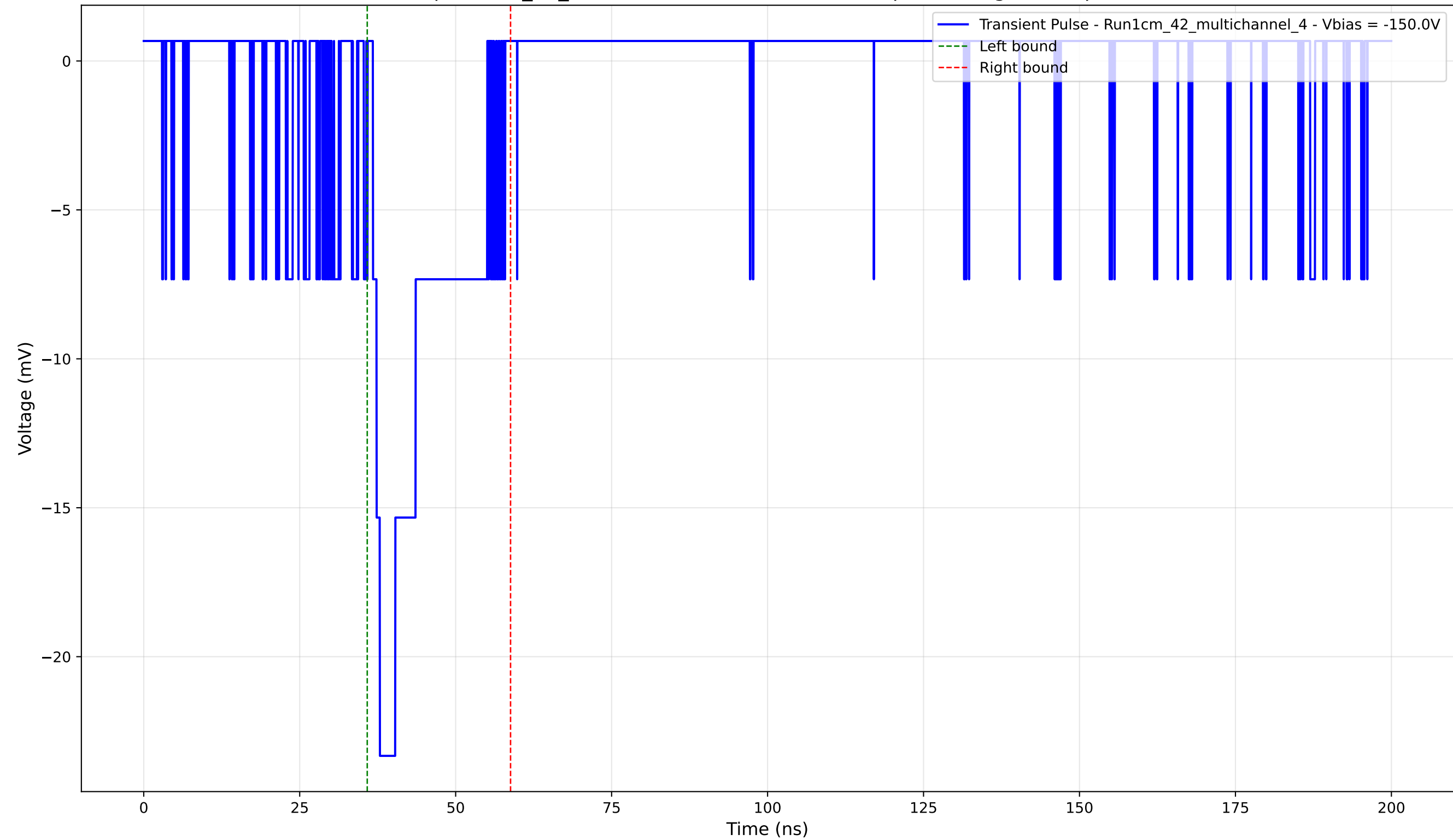
Transient Pulse - Sample: 1cm_42_multichannel - Position: 1170.0 \mu\text{m} - Charge: 4.28 pC - Rise Time: 1.12 ns
