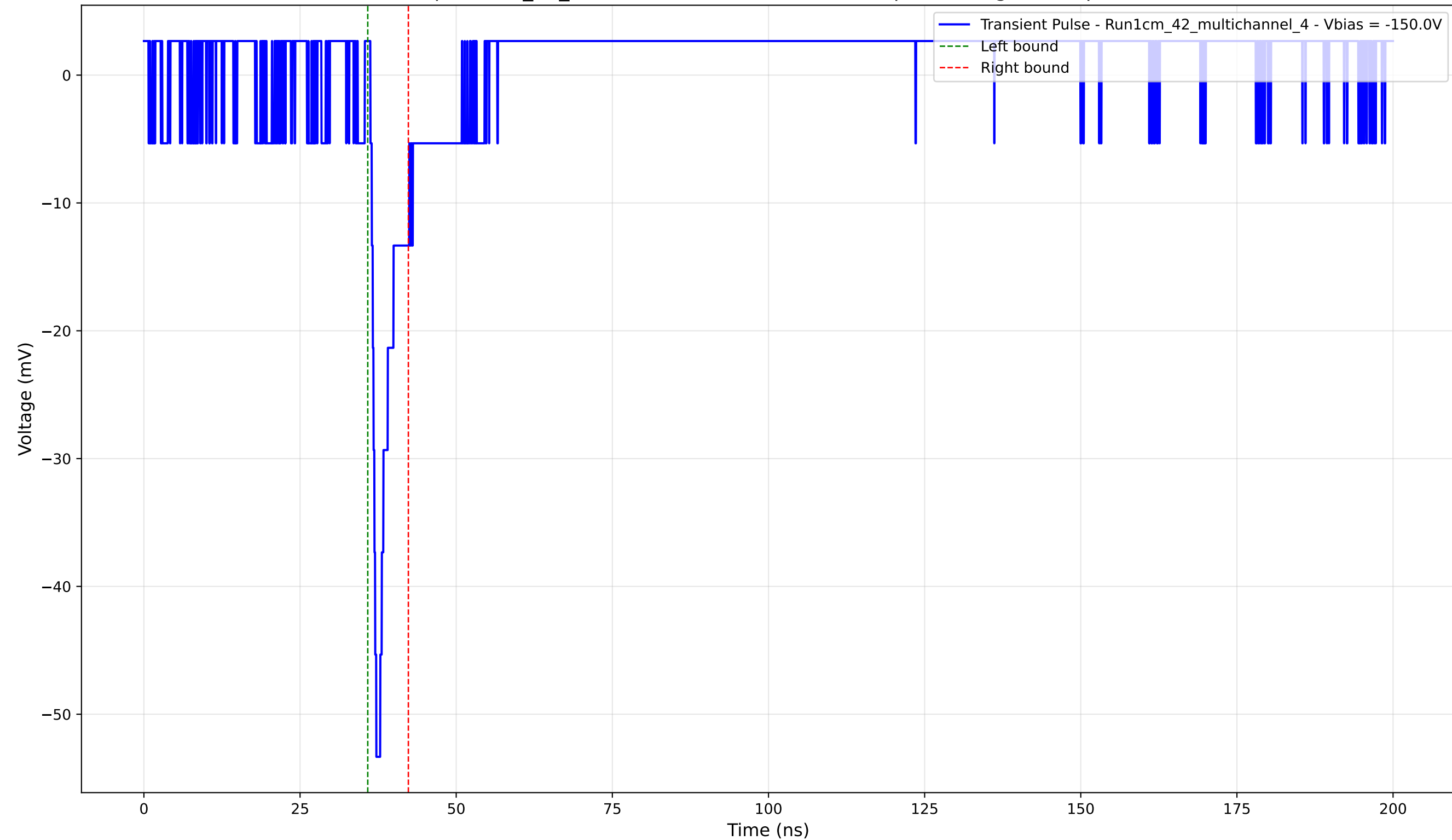
Transient Pulse - Sample: 1cm_42_multichannel - Position: 2000.0 \mu\text{m} - Charge: 2.97 pC - Rise Time: 0.74 ns
