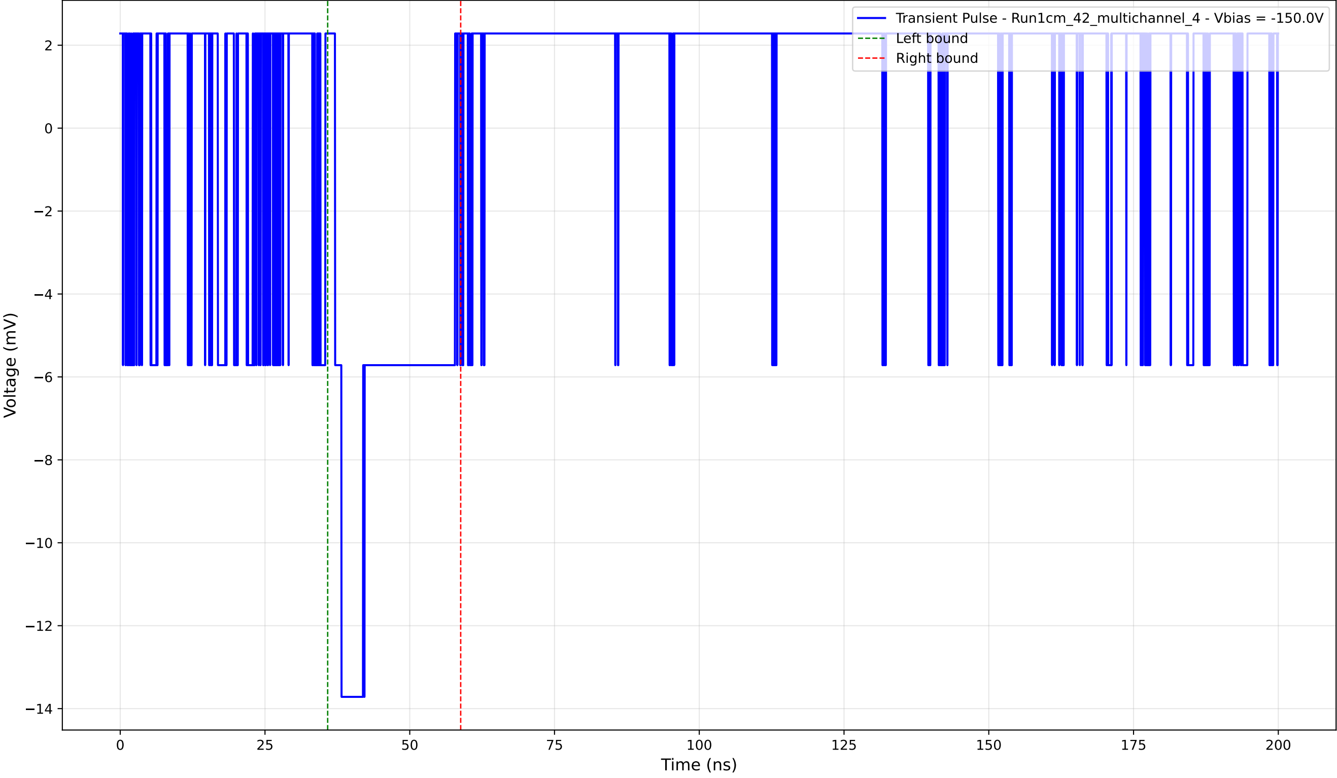
Transient Pulse - Sample: 1cm_42_multichannel - Position: 225.0 \mu\text{m} - Charge: 2.89 pC - Rise Time: 0.00 ns (N/A)
