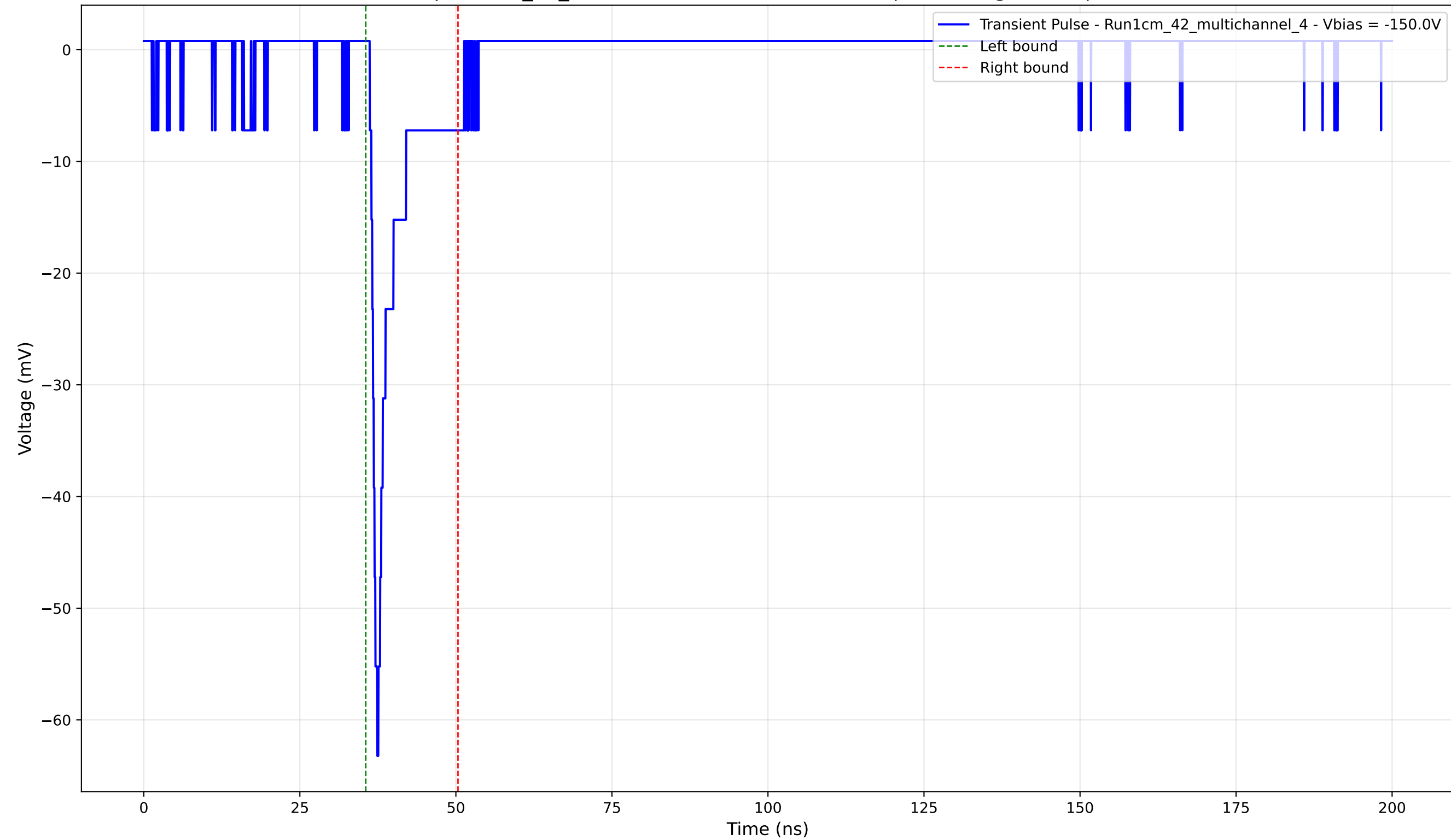
Transient Pulse - Sample: 1cm_42_multichannel - Position: 2060.0 \mu\text{m} - Charge: 4.34 pC - Rise Time: 1.20 ns
