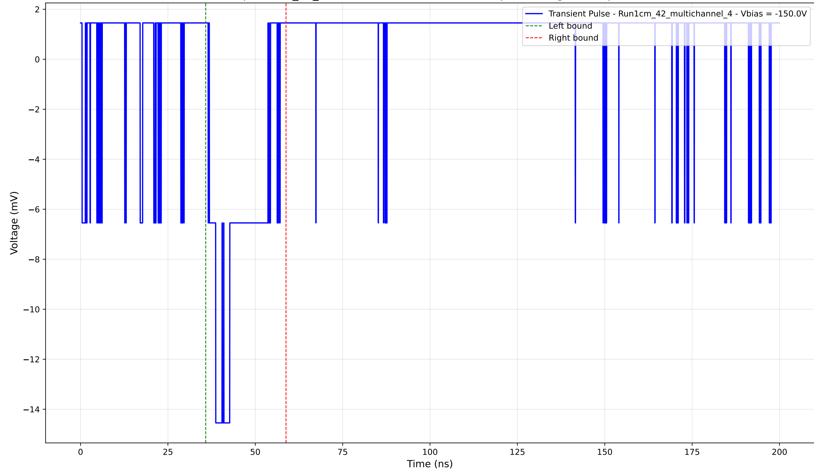
Transient Pulse - Sample: 1cm_42_multichannel - Position: 4790.0 \mu\text{m} - Charge: 2.78 pC - Rise Time: 1.84 ns
