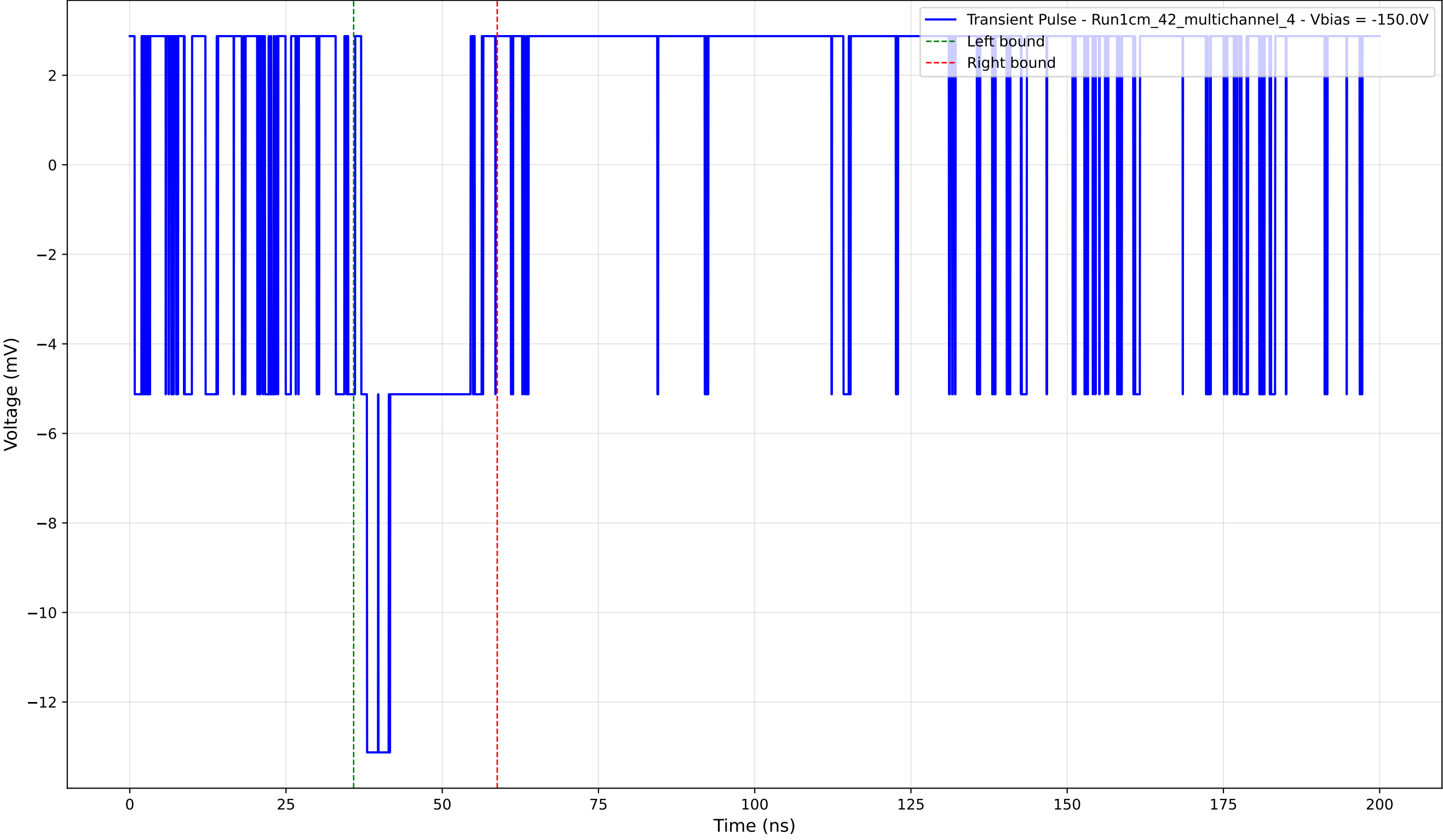
Transient Pulse - Sample: 1cm_42_multichannel - Position: 810.0 \mu\text{m} - Charge: 2.31 pC - Rise Time: 0.00 ns (N/A)
