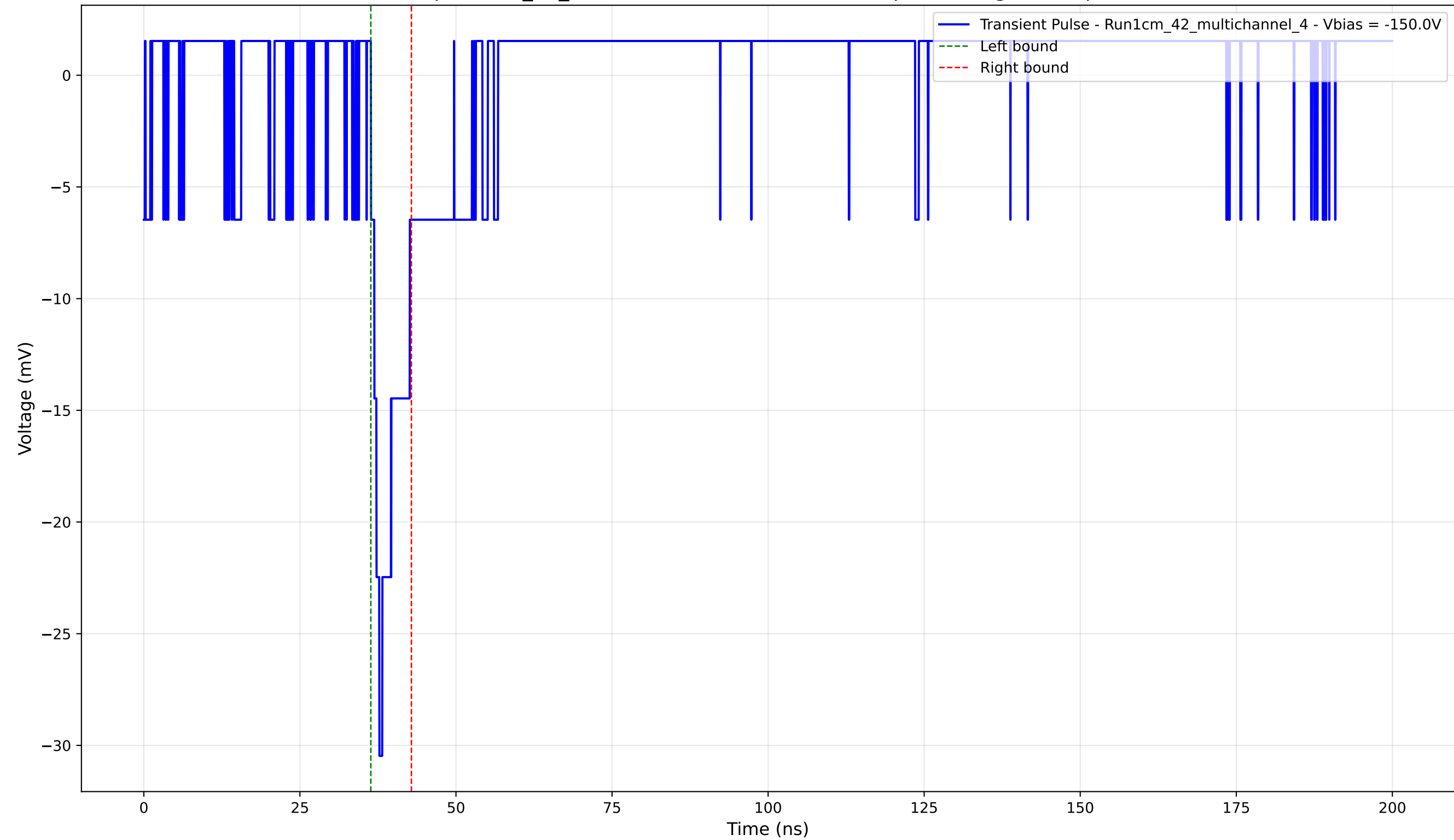
Transient Pulse - Sample: 1cm_42_multichannel - Position: 3245.0 \mu\text{m} - Charge: 2.20 pC - Rise Time: 1.35 ns
