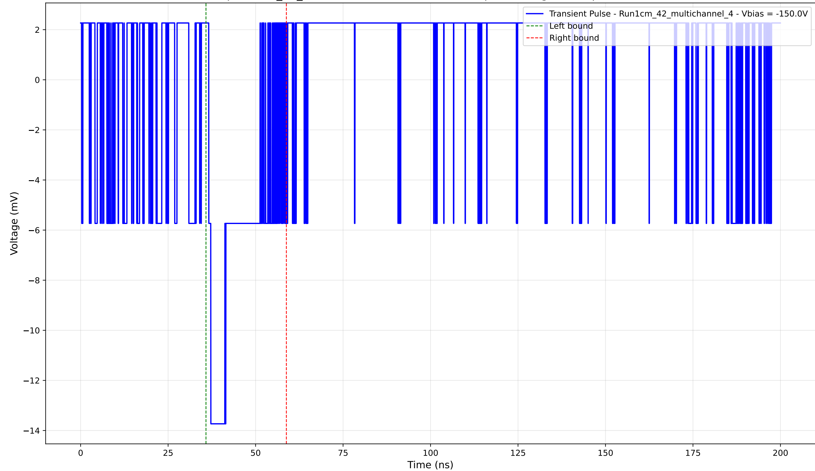
Transient Pulse - Sample: 1cm_42_multichannel - Position: 1430.0 \mu\text{m} - Charge: 2.59 pC - Rise Time: 0.00 ns (N/A)
