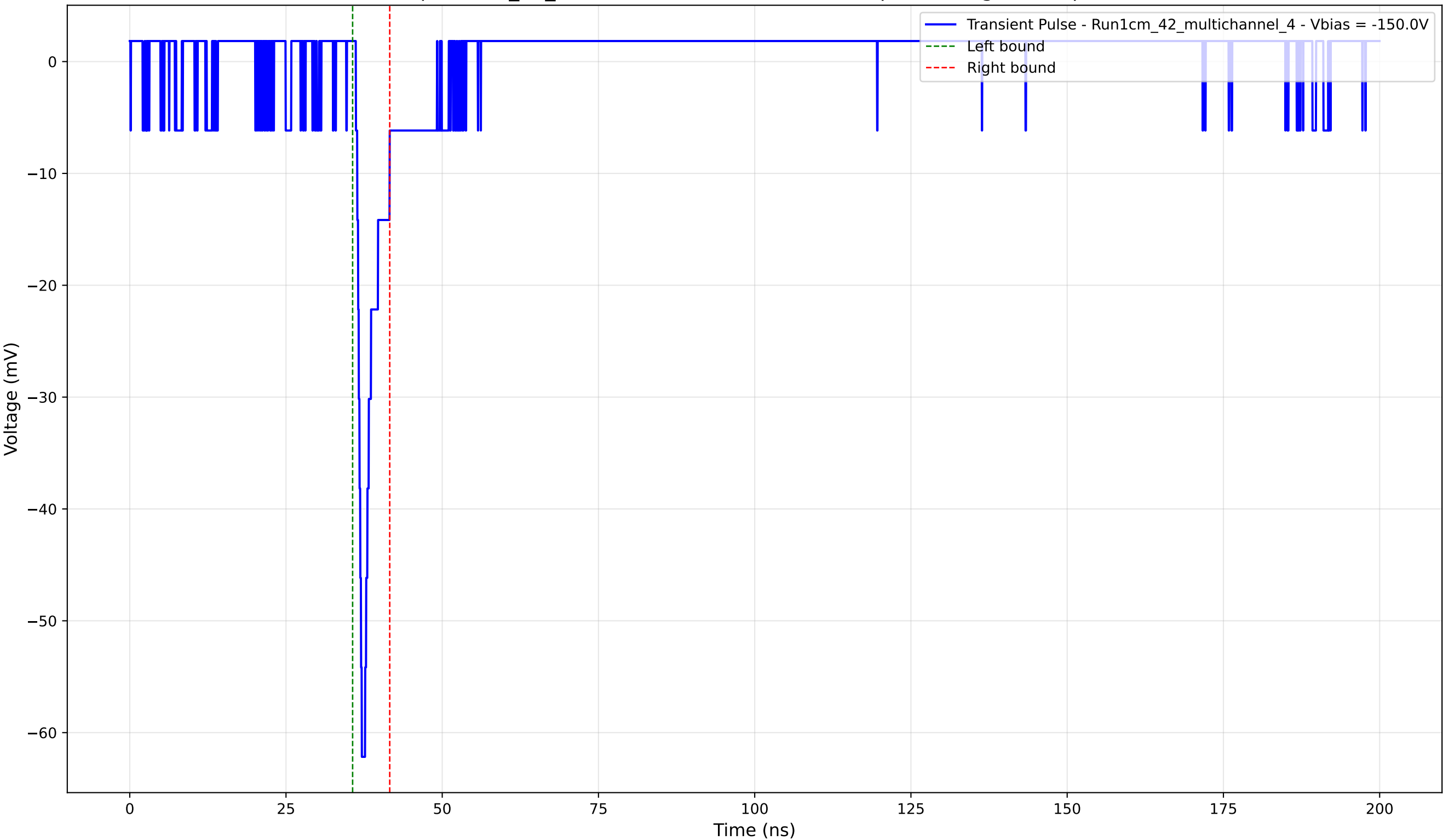
Transient Pulse - Sample: 1cm_42_multichannel - Position: 2130.0 \mu\text{m} - Charge: 2.94 pC - Rise Time: 0.74 ns
