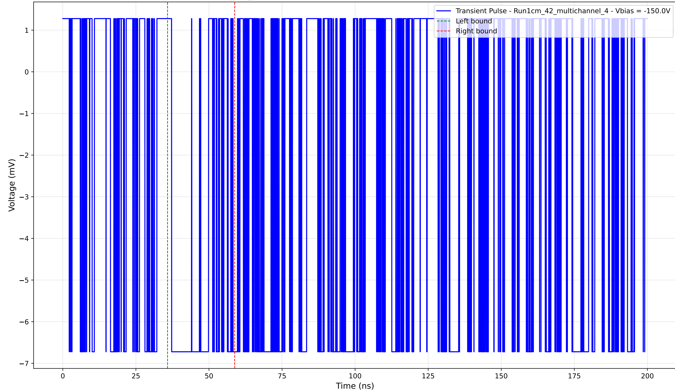
Transient Pulse - Sample: 1cm_42_multichannel - Position: 330.0 \mu\text{m} - Charge: 2.06 pC - Rise Time: 0.00 ns (N/A)
