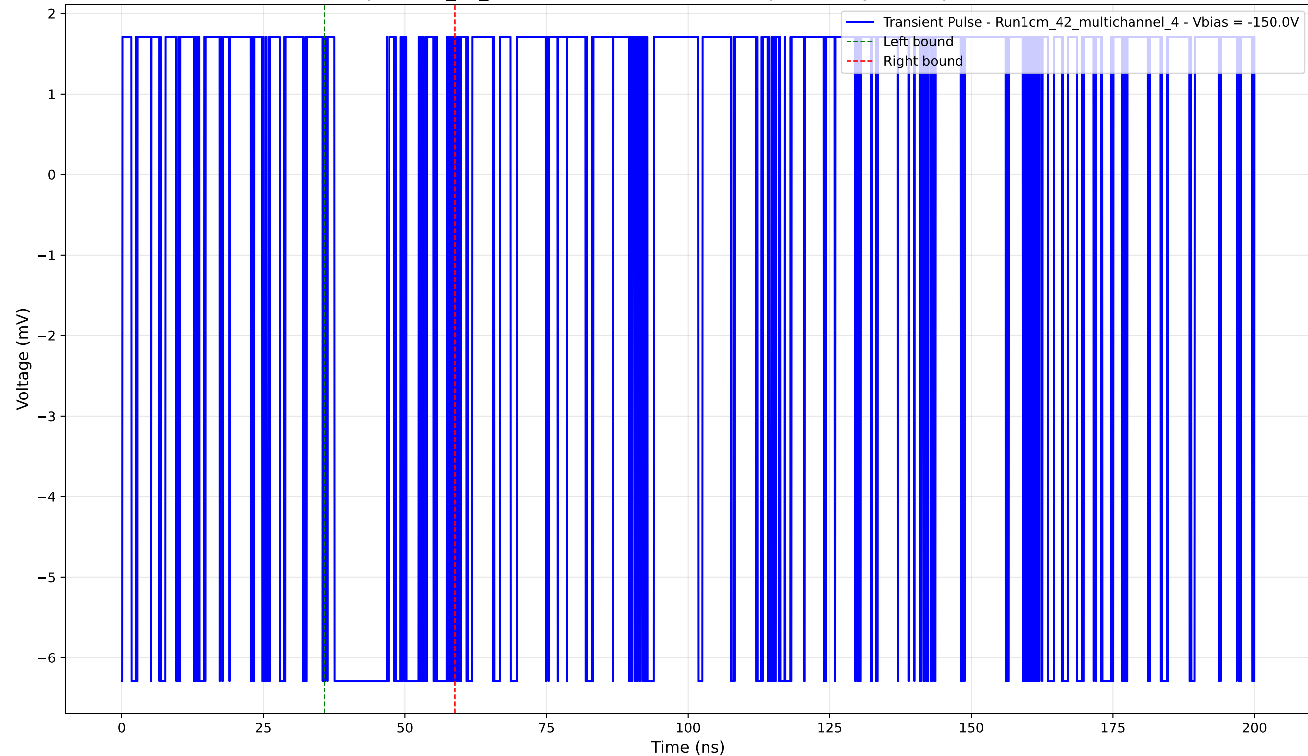
Transient Pulse - Sample: 1cm_42_multichannel - Position: 905.0 \mu\text{m} - Charge: 1.86 pC - Rise Time: 0.00 ns (N/A)
