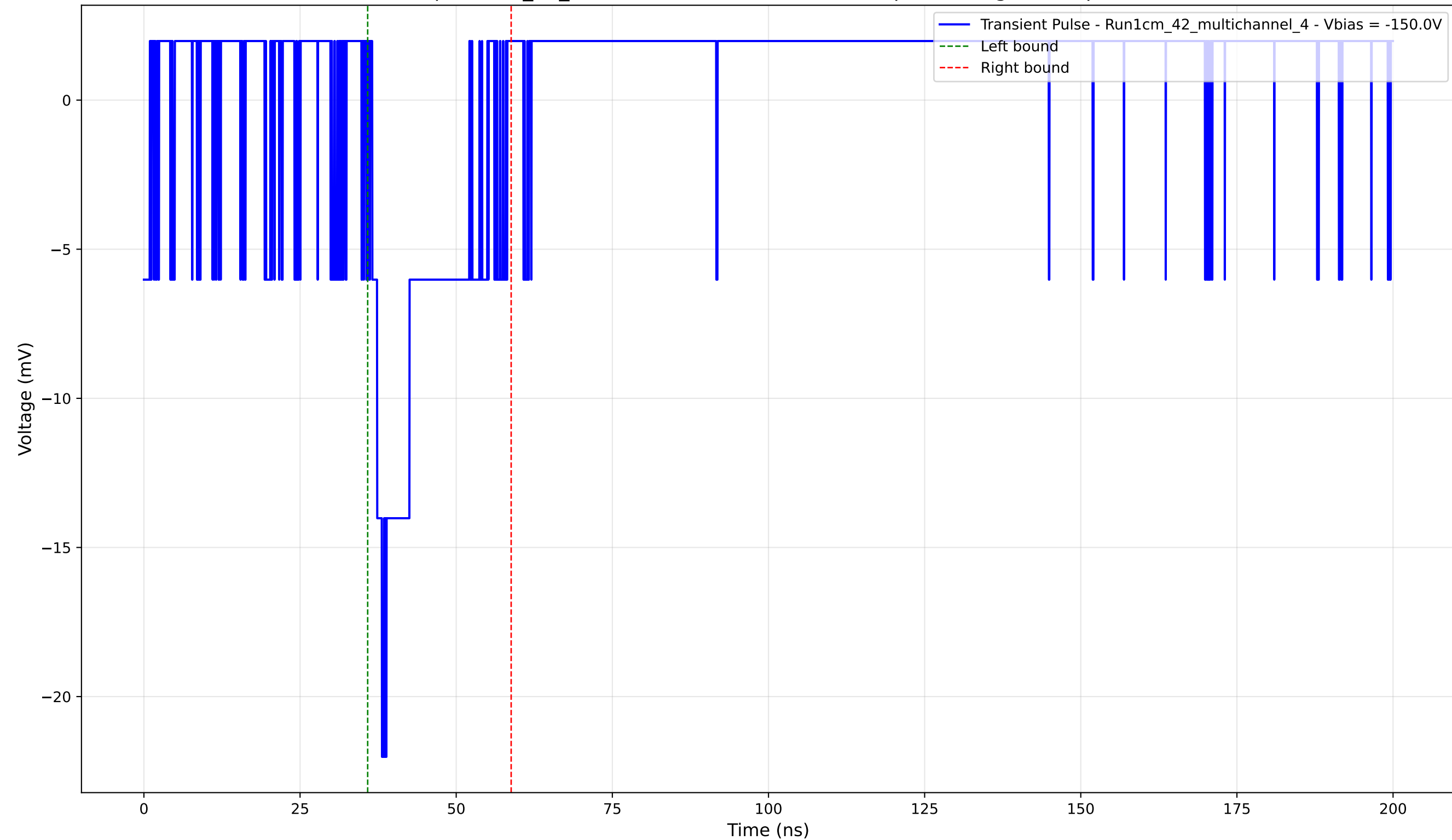
Transient Pulse - Sample: 1cm_42_multichannel - Position: 3585.0 \mu\text{m} - Charge: 3.16 pC - Rise Time: 1.56 ns
