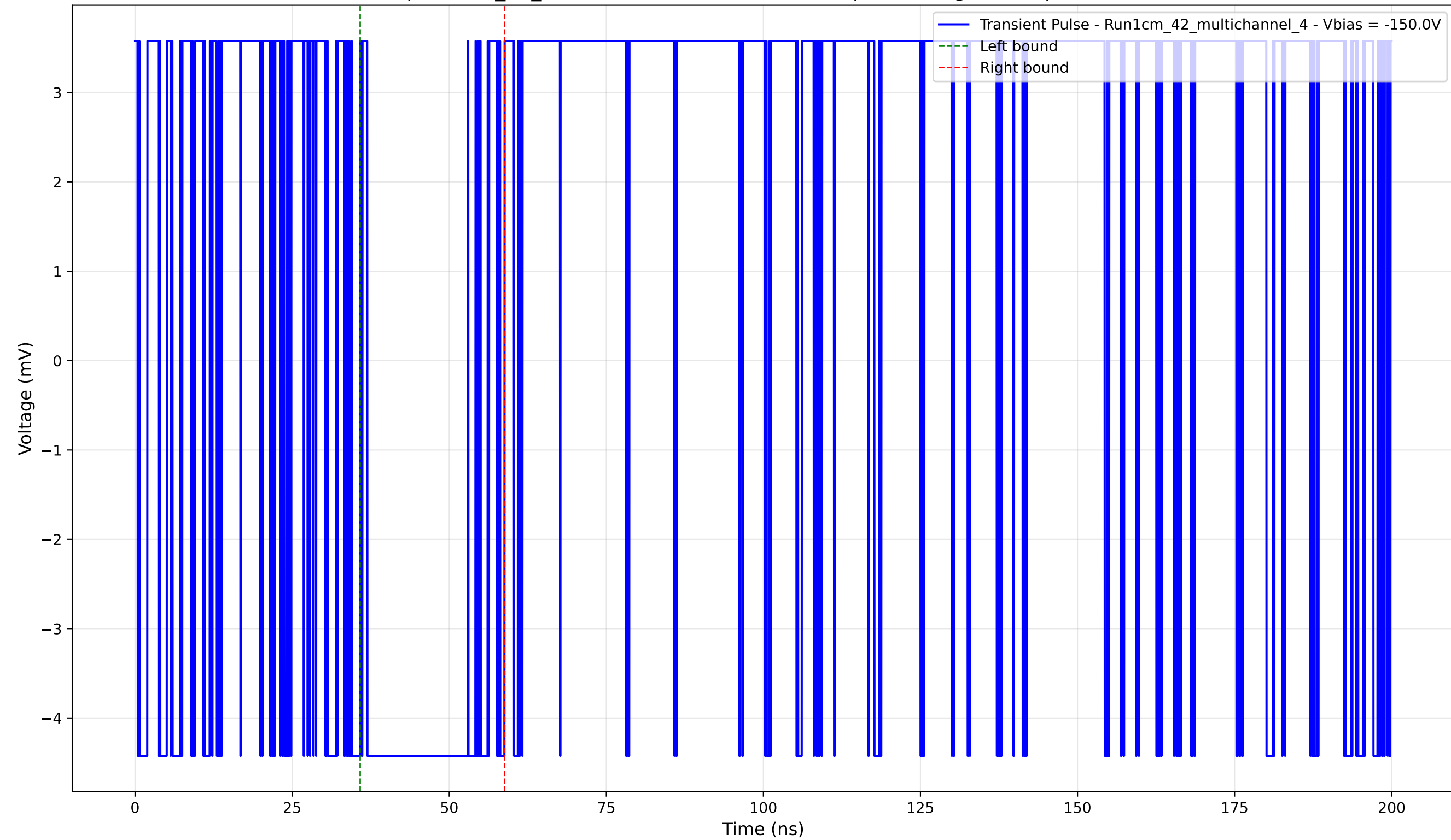
Transient Pulse - Sample: 1cm_42_multichannel - Position: 305.0 \mu\text{m} - Charge: 1.59 pC - Rise Time: 0.00 ns (N/A)
