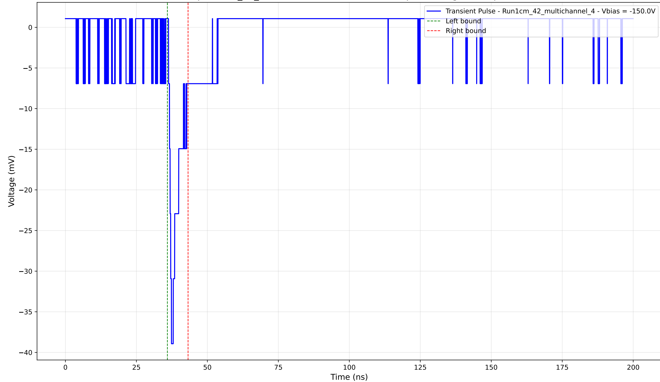
Transient Pulse - Sample: 1cm_42_multichannel - Position: 2975.0 \mu\text{m} - Charge: 2.67 pC - Rise Time: 1.03 ns
