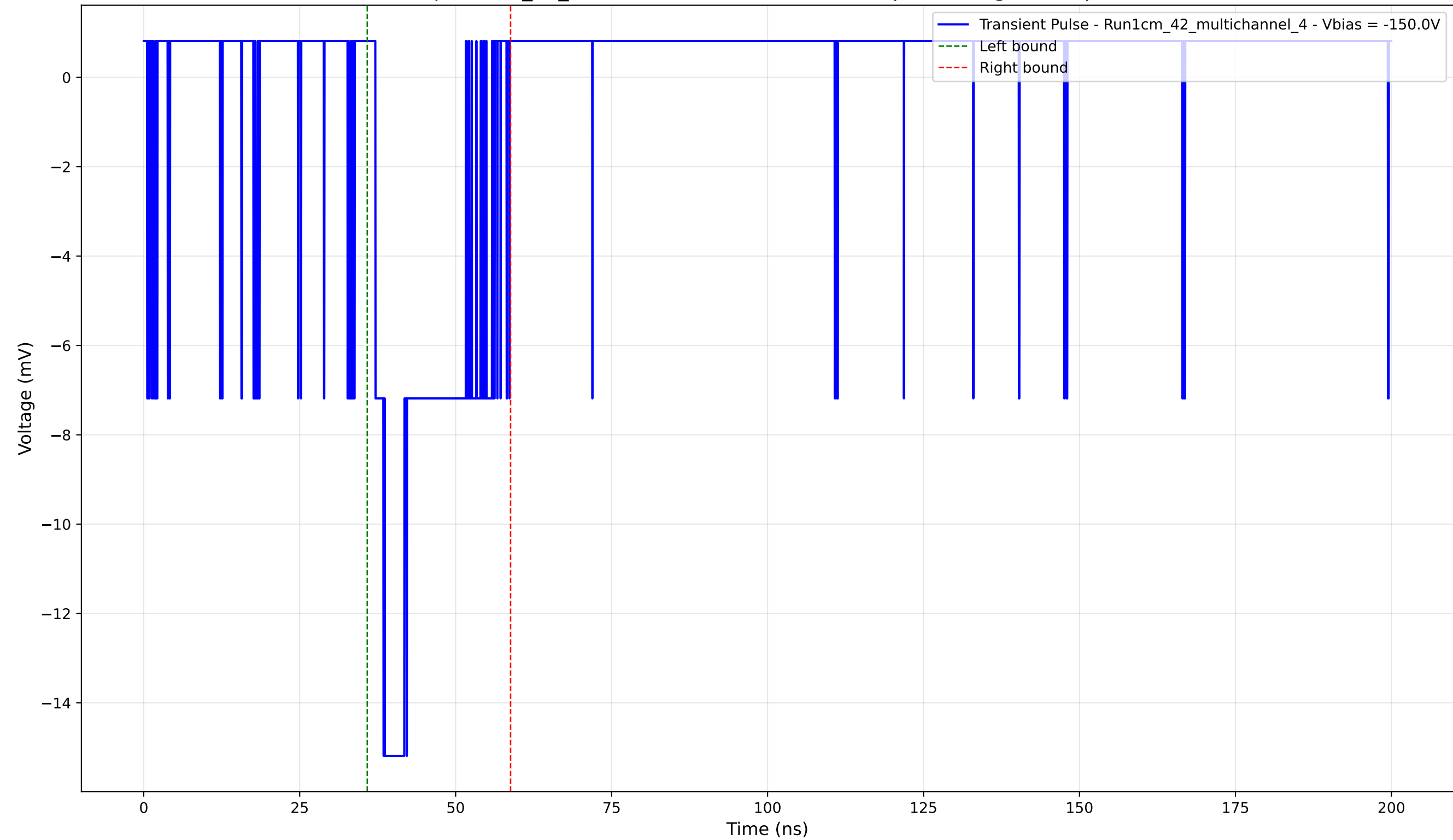
Transient Pulse - Sample: 1cm_42_multichannel - Position: 4660.0 \mu\text{m} - Charge: 3.09 pC - Rise Time: 1.30 ns
