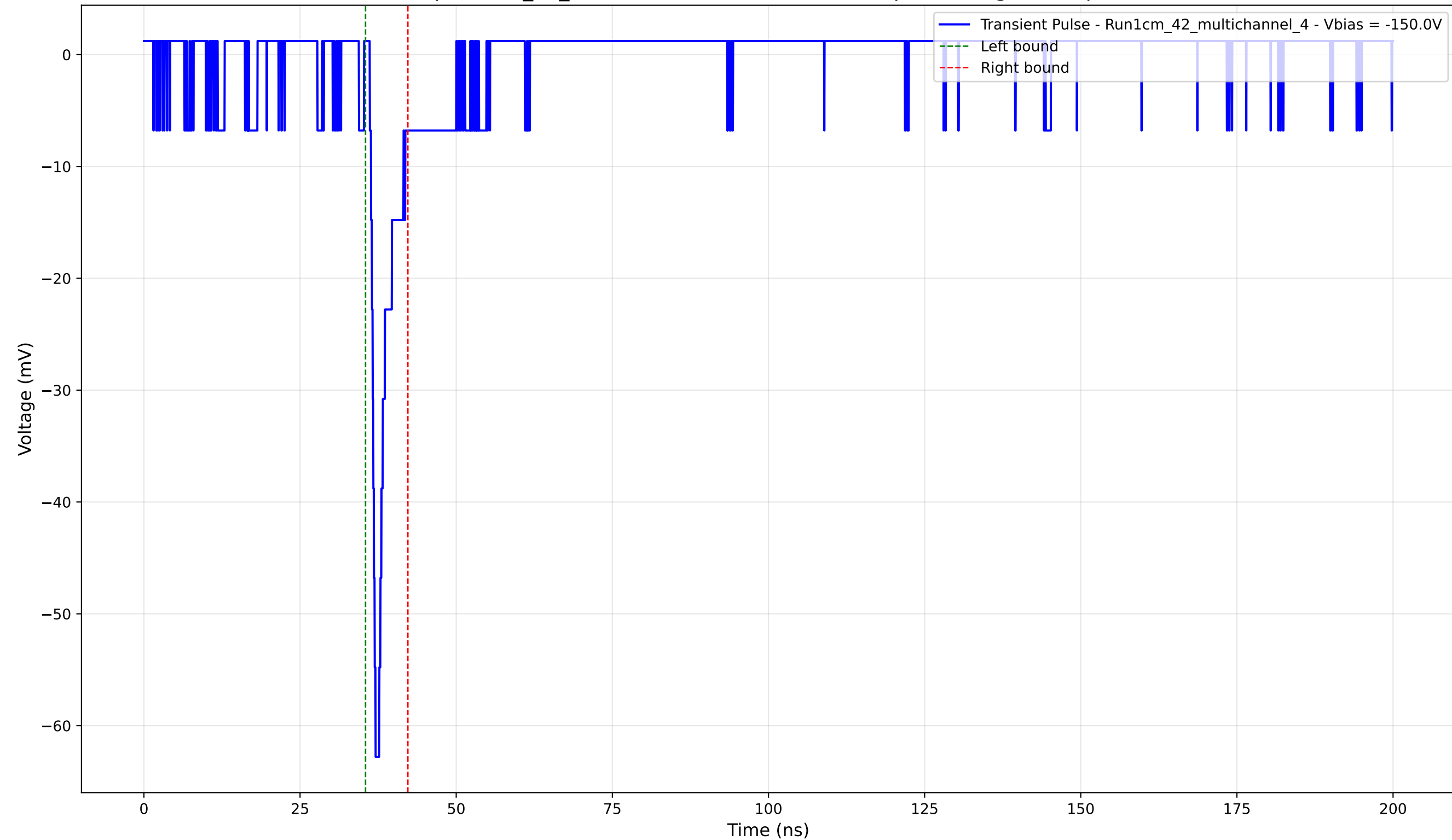
Transient Pulse - Sample: 1cm_42_multichannel - Position: 2160.0 \mu\text{m} - Charge: 3.17 pC - Rise Time: 0.92 ns
