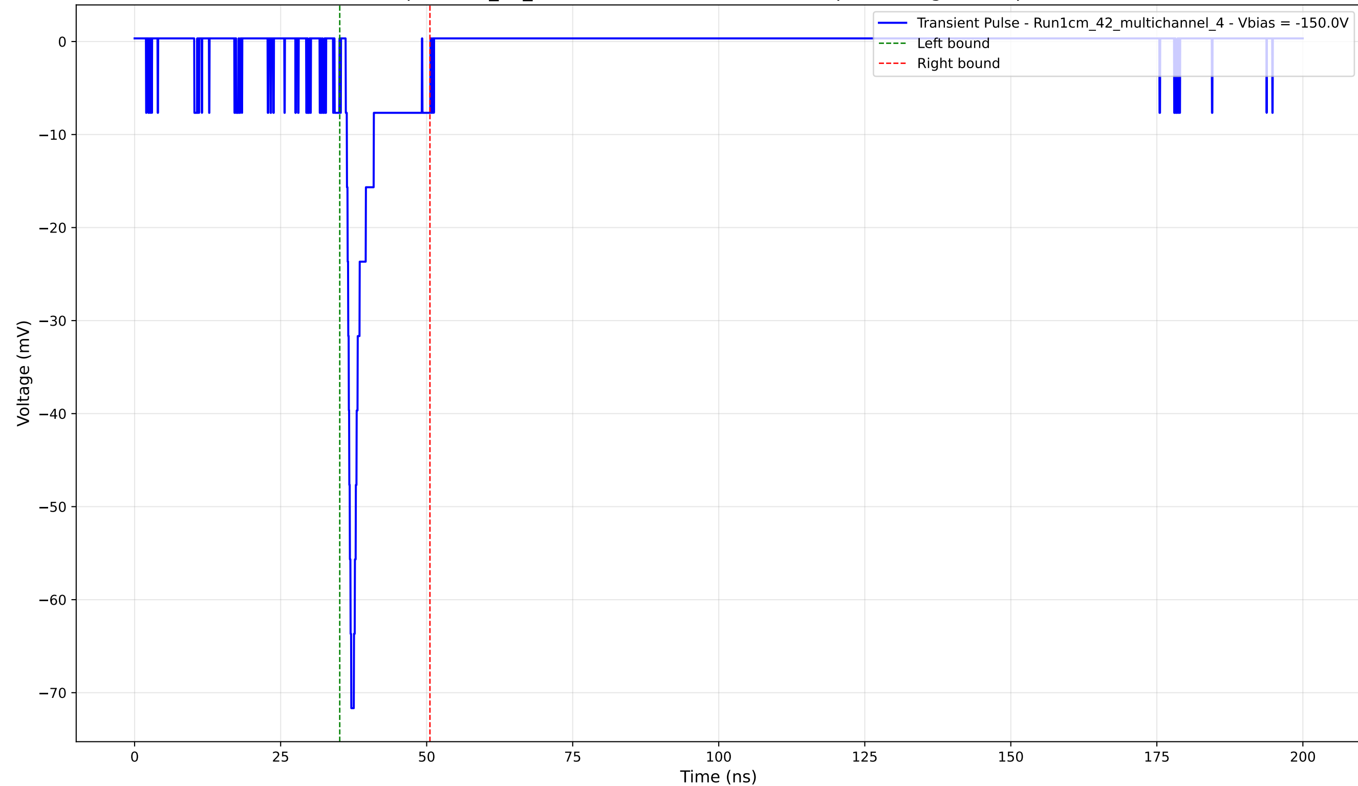
Transient Pulse - Sample: 1cm_42_multichannel - Position: 2560.0 \mu\text{m} - Charge: 4.56 pC - Rise Time: 0.94 ns
