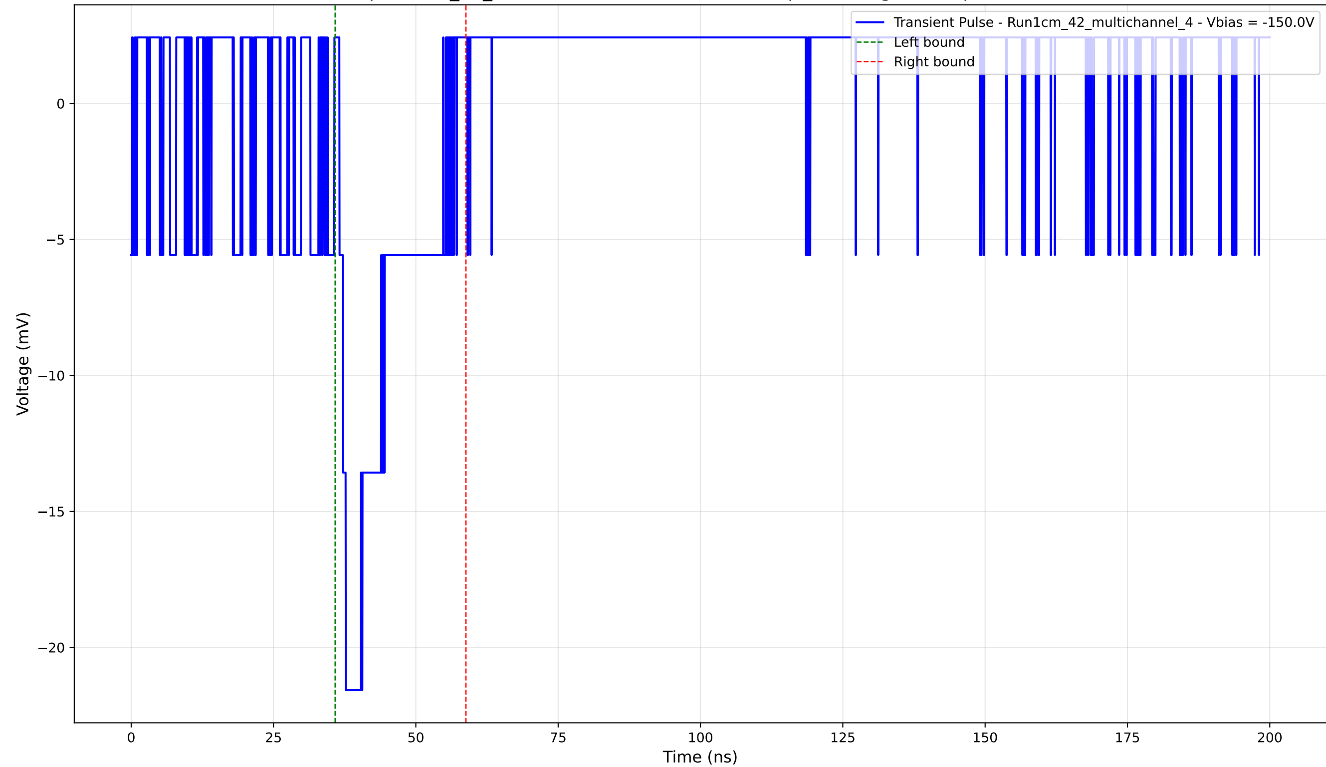
Transient Pulse - Sample: 1cm_42_multichannel - Position: 1210.0 \mu\text{m} - Charge: 3.62 pC - Rise Time: 0.00 ns (N/A)
