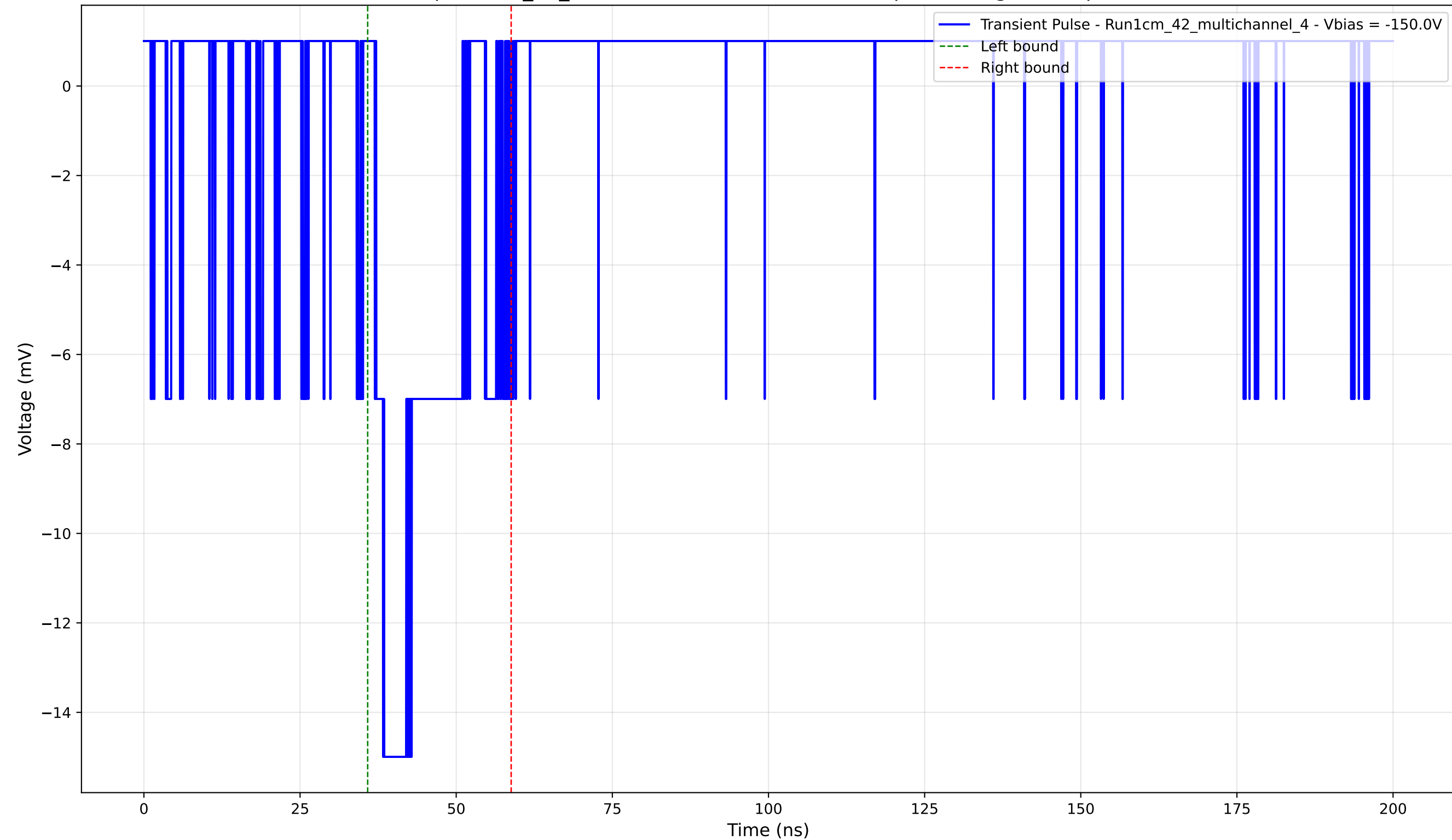
Transient Pulse - Sample: 1cm_42_multichannel - Position: 4635.0 \mu\text{m} - Charge: 2.95 pC - Rise Time: 1.10 ns
