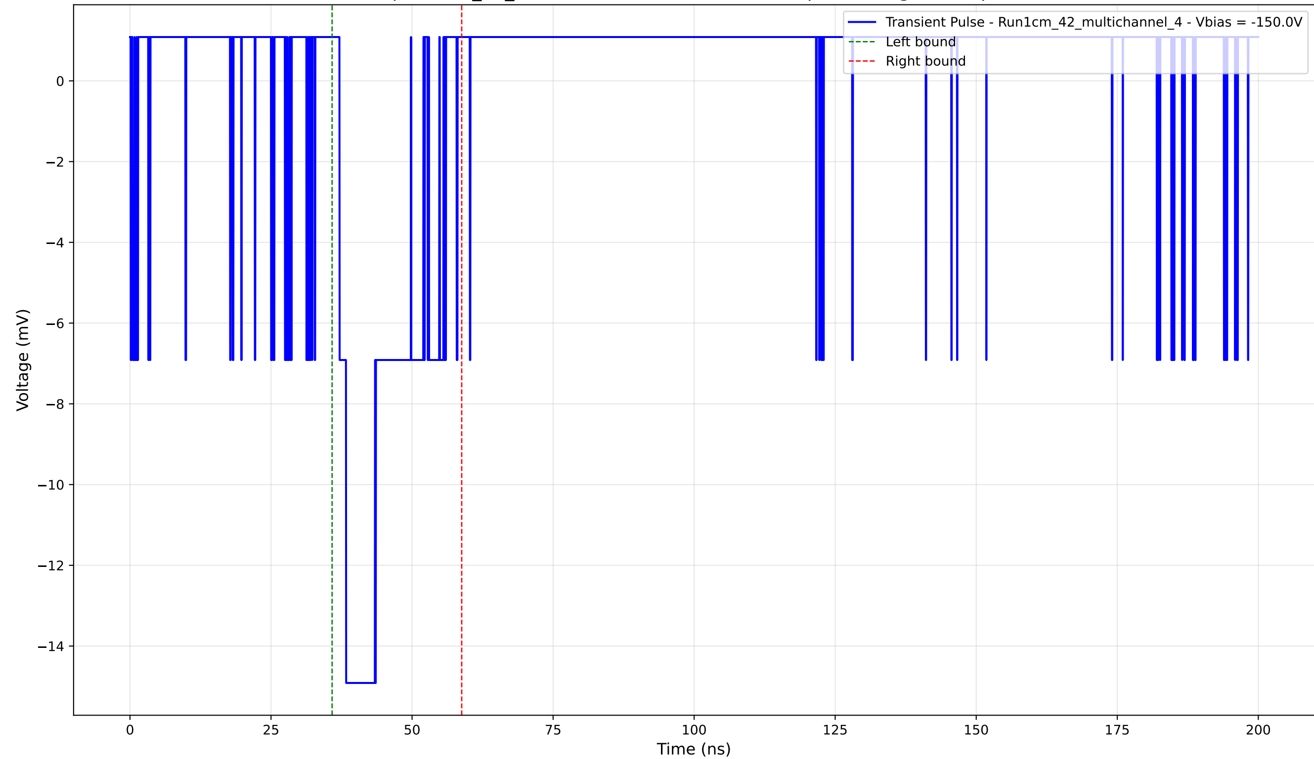
Transient Pulse - Sample: 1cm_42_multichannel - Position: 4205.0 \mu\text{m} - Charge: 3.22 pC - Rise Time: 1.18 ns
