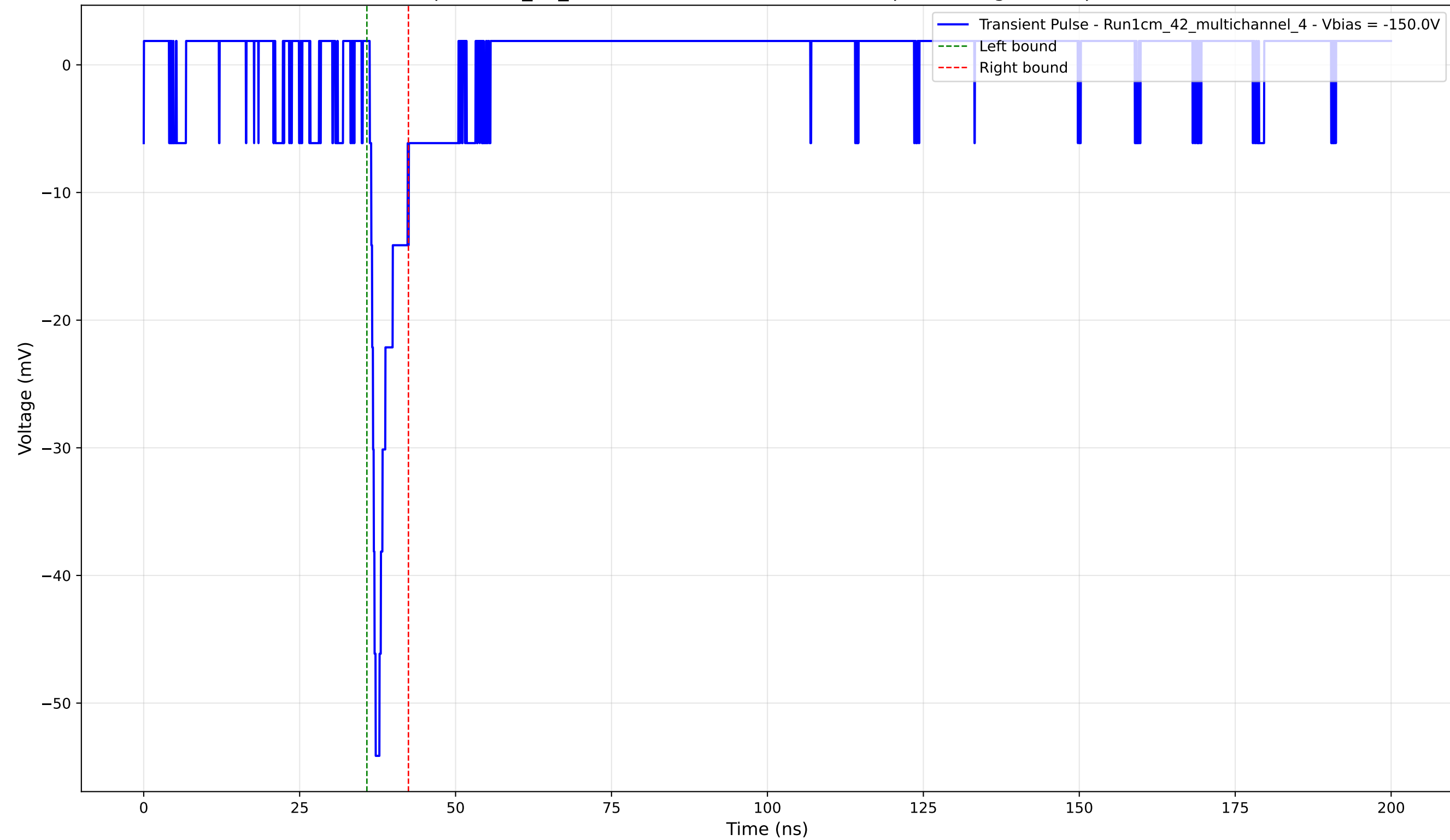
Transient Pulse - Sample: 1cm_42_multichannel - Position: 2005.0 \mu\text{m} - Charge: 3.02 pC - Rise Time: 0.94 ns
