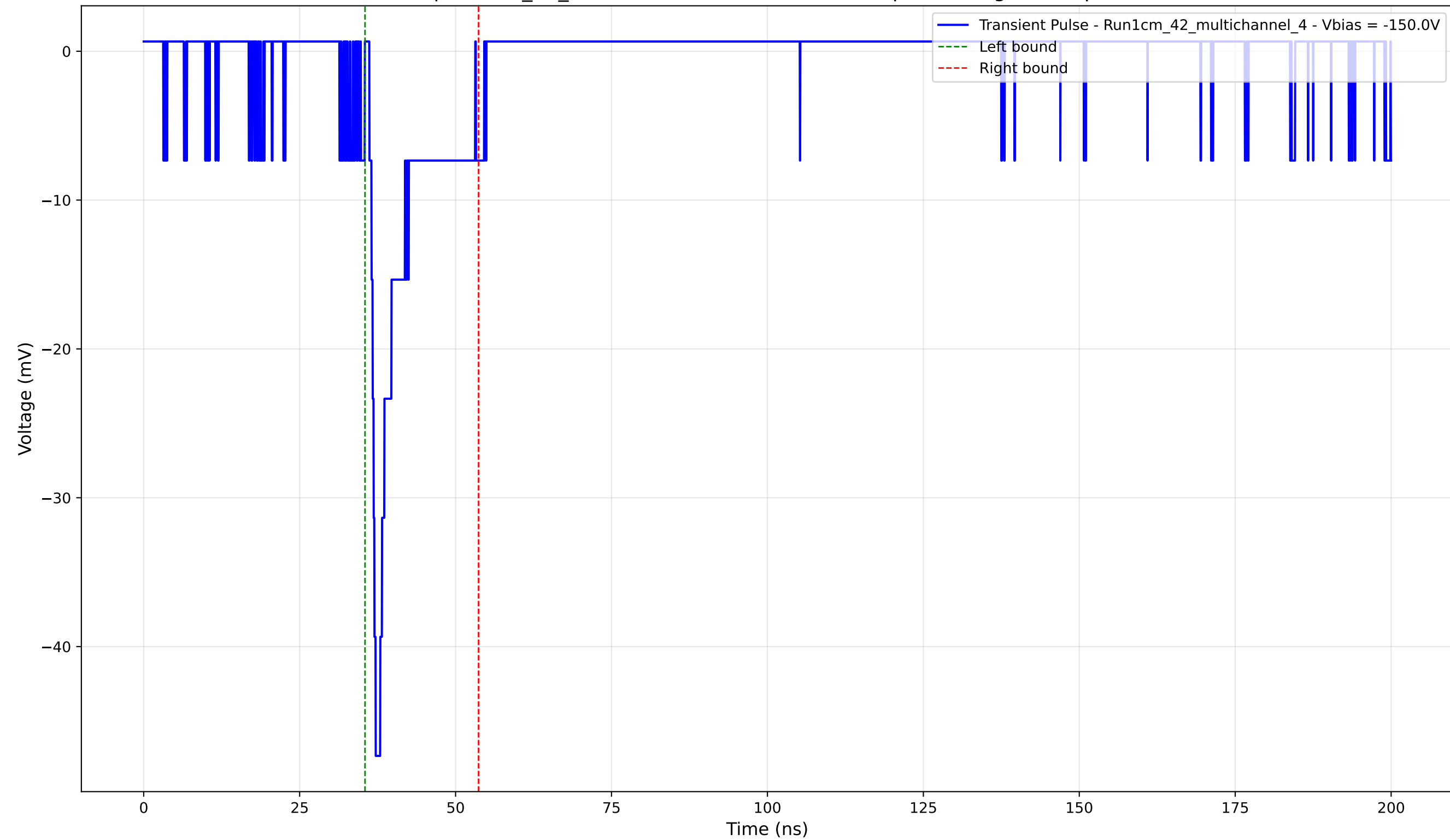
Transient Pulse - Sample: 1cm_42_multichannel - Position: 2795.0 \mu\text{m} - Charge: 4.52 pC - Rise Time: 1.01 ns
