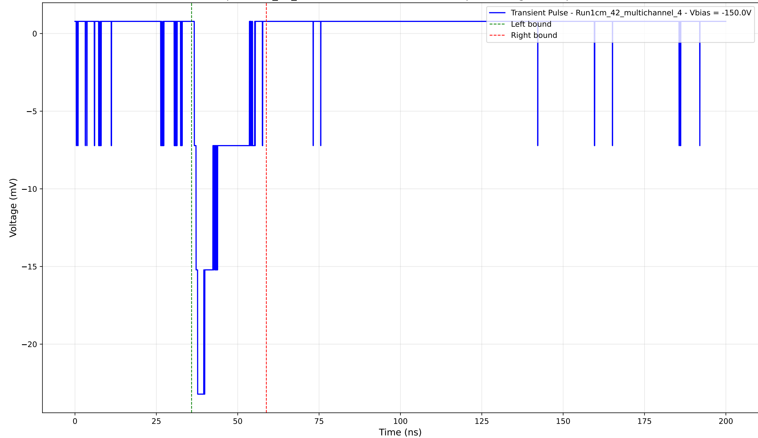
Transient Pulse - Sample: 1cm_42_multichannel - Position: 3505.0 \mu\text{m} - Charge: 3.79 pC - Rise Time: 1.04 ns
