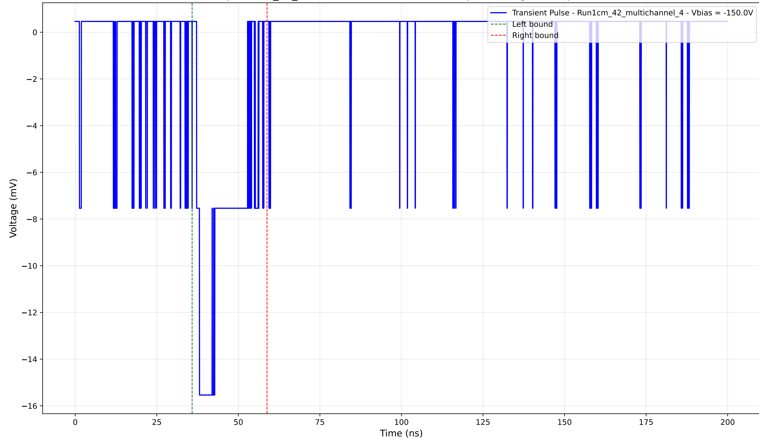
Transient Pulse - Sample: 1cm_42_multichannel - Position: 3970.0 \mu\text{m} - Charge: 3.29 pC - Rise Time: 0.90 ns
