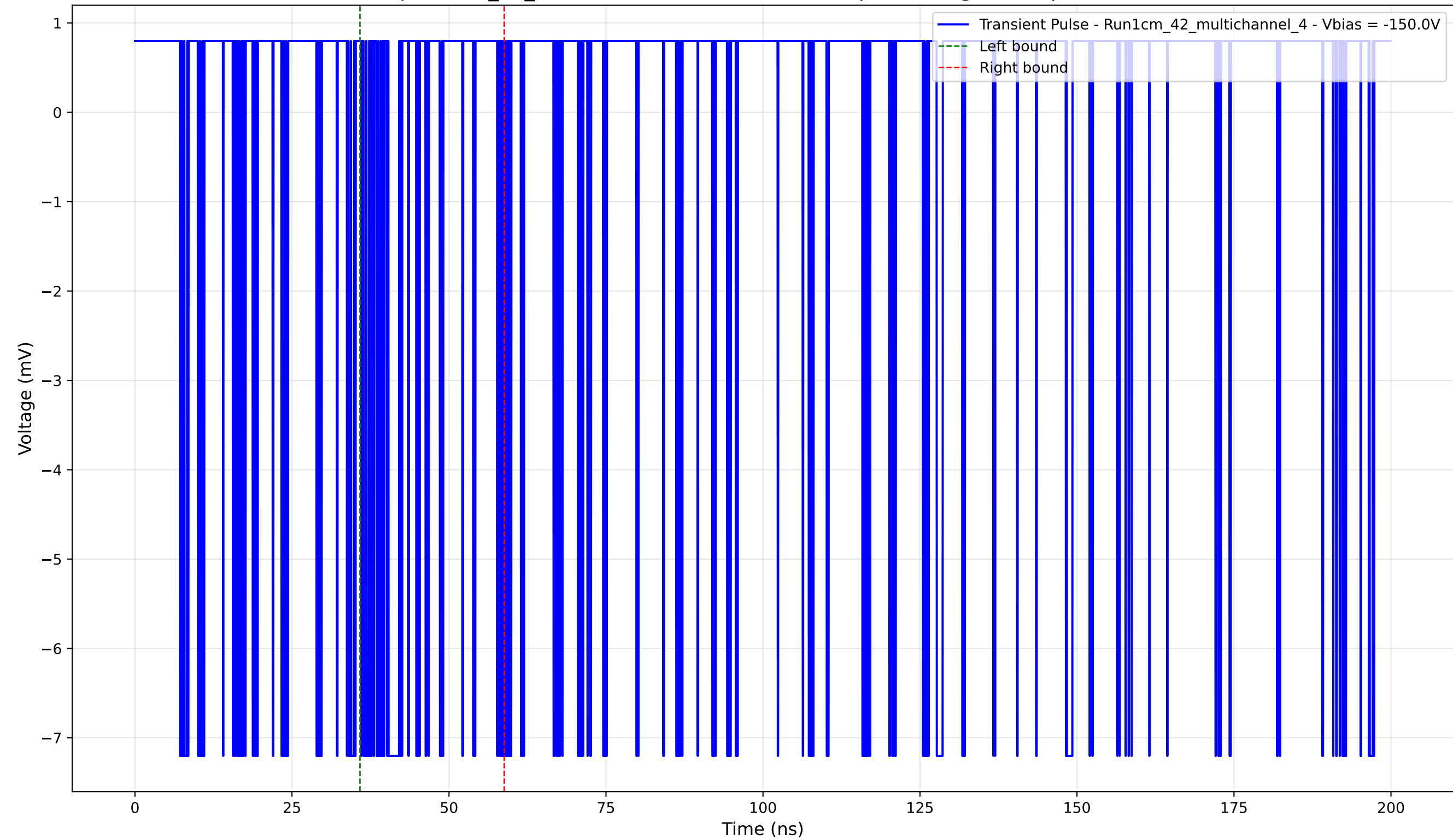
Transient Pulse - Sample: 1cm_42_multichannel - Position: 3380.0 \mu\text{m} - Charge: 0.58 pC - Rise Time: 0.00 ns (N/A)
