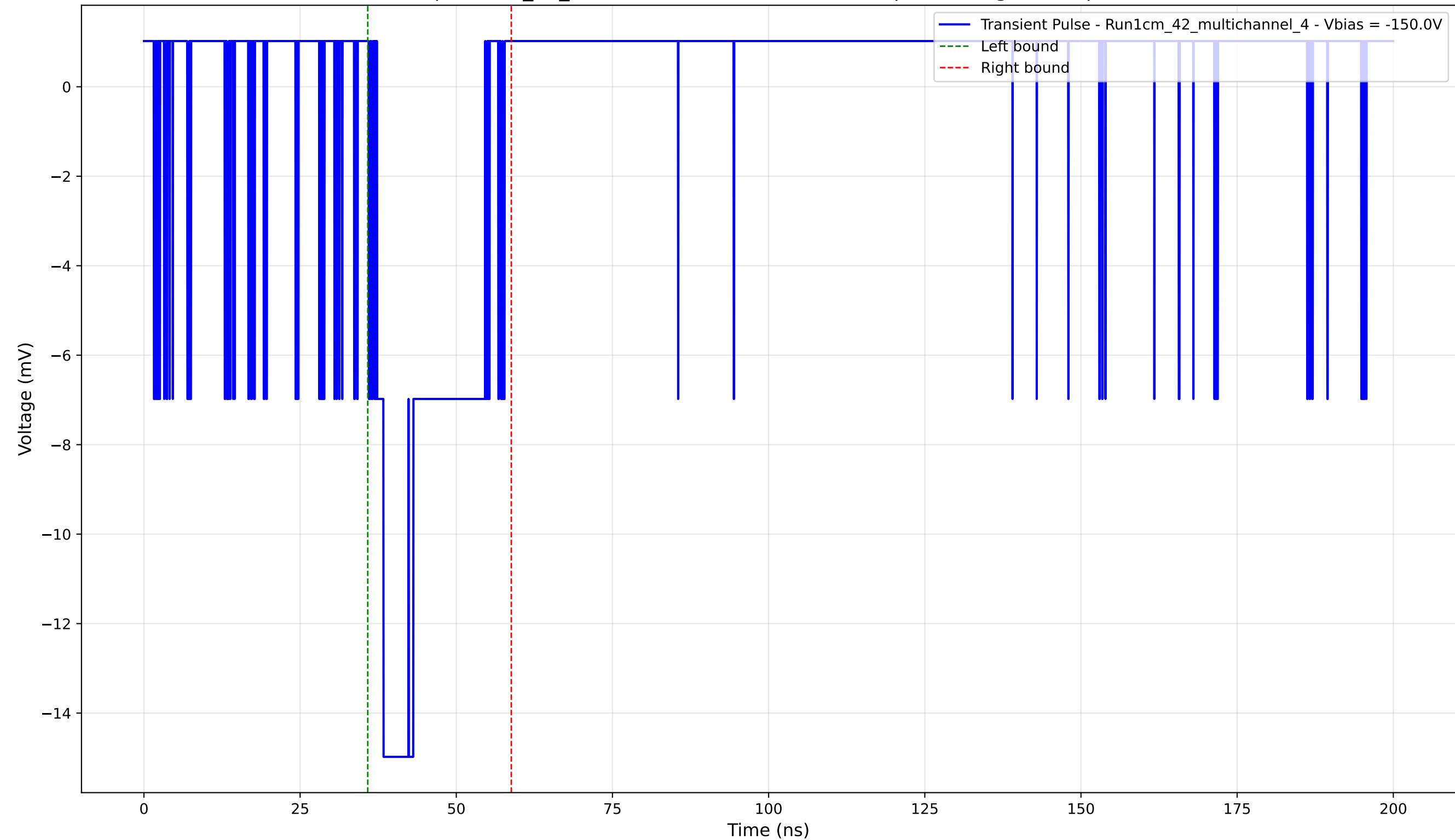
Transient Pulse - Sample: 1cm_42_multichannel - Position: 4520.0 \mu\text{m} - Charge: 3.37 pC - Rise Time: 1.04 ns
