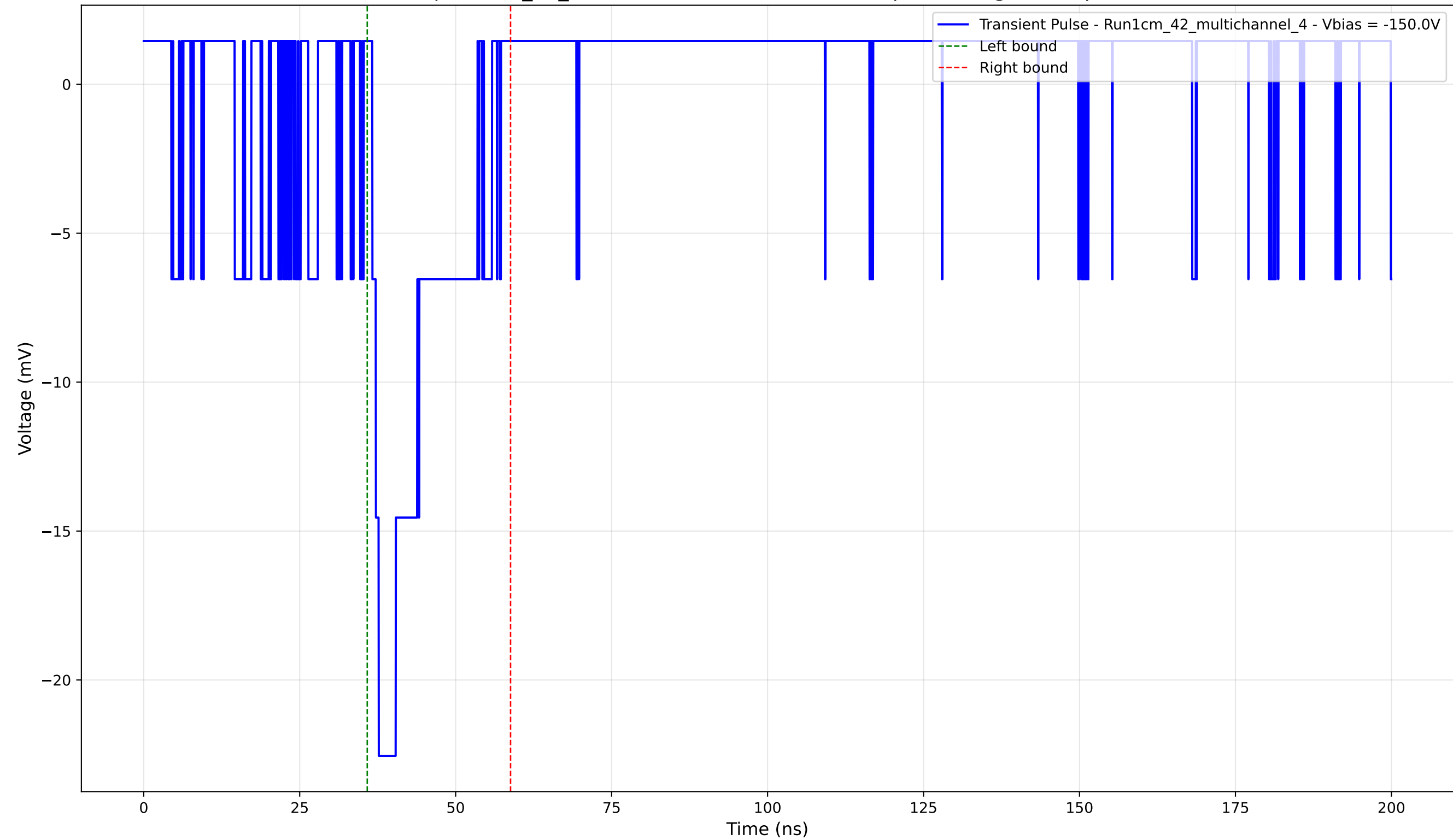
Transient Pulse - Sample: 1cm_42_multichannel - Position: 1240.0 \mu\text{m} - Charge: 3.85 pC - Rise Time: 1.04 ns
