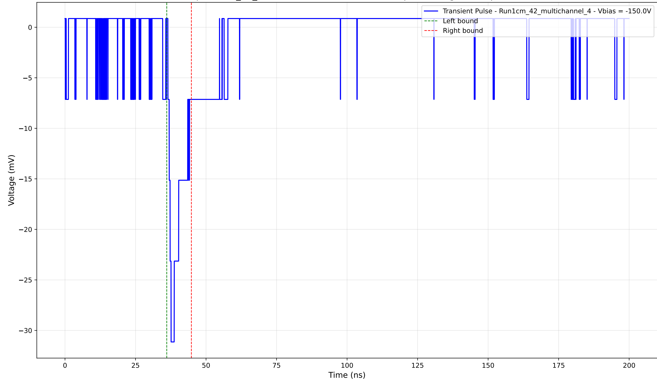
Transient Pulse - Sample: 1cm_42_multichannel - Position: 1480.0 \mu\text{m} - Charge: 2.92 pC - Rise Time: 1.13 ns
