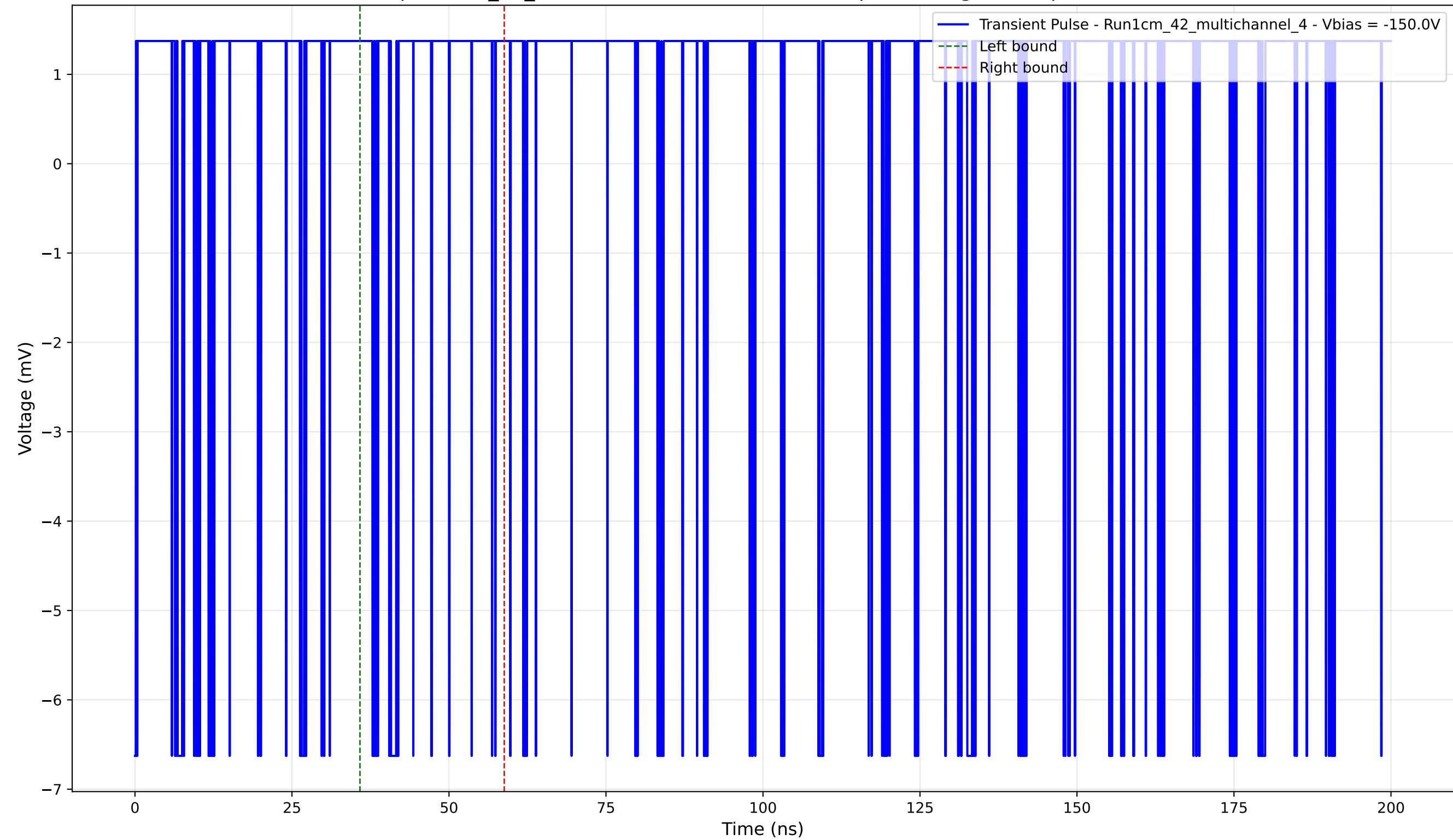
Transient Pulse - Sample: 1cm_42_multichannel - Position: 3910.0 \mu\text{m} - Charge: 0.26 pC - Rise Time: 0.00 ns (N/A)
