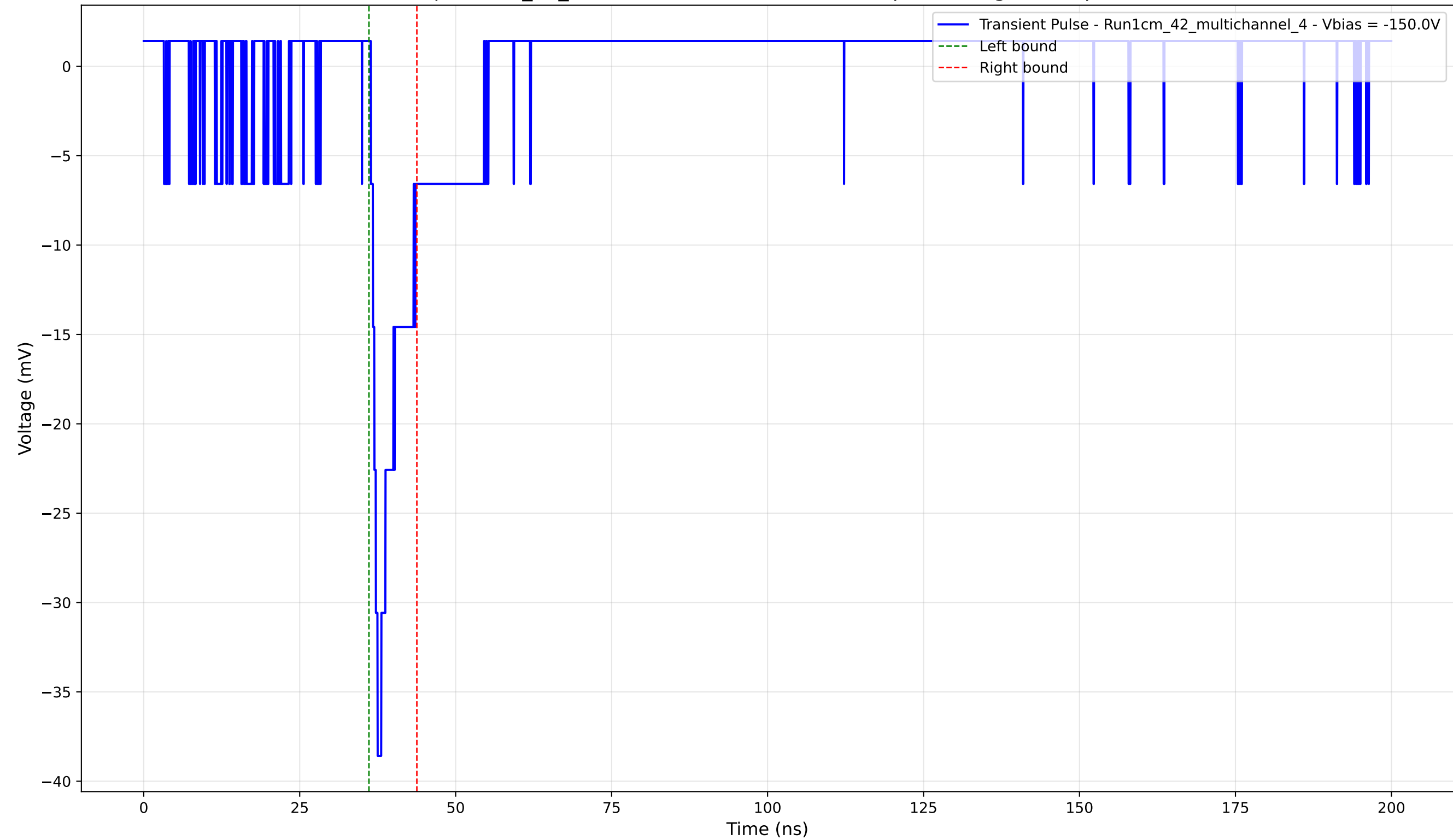
Transient Pulse - Sample: 1cm_42_multichannel - Position: 1690.0 \mu\text{m} - Charge: 2.88 pC - Rise Time: 1.09 ns
