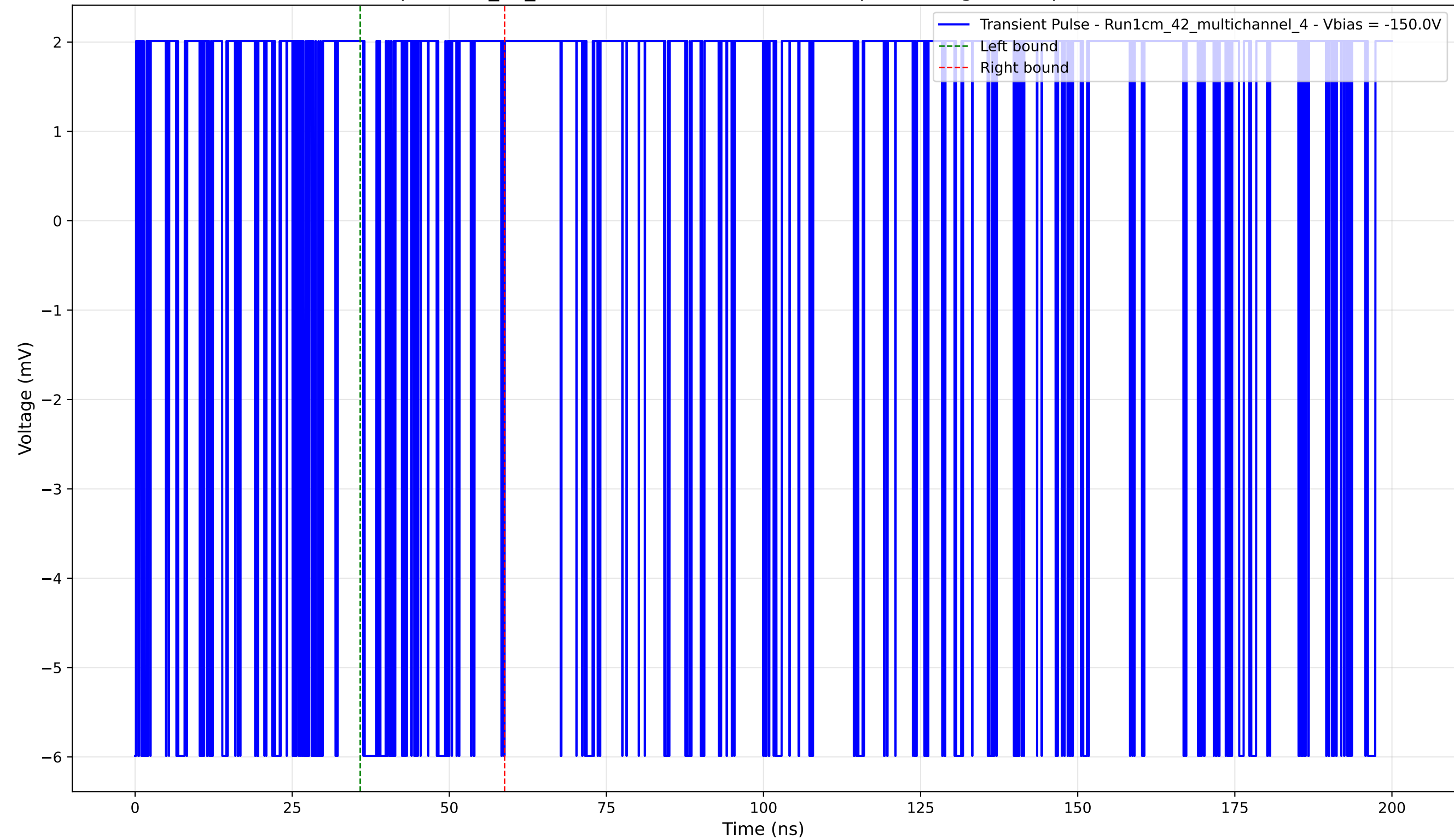
Transient Pulse - Sample: 1cm_42_multichannel - Position: 2380.0 \mu\text{m} - Charge: 0.24 pC - Rise Time: 0.00 ns (N/A)
