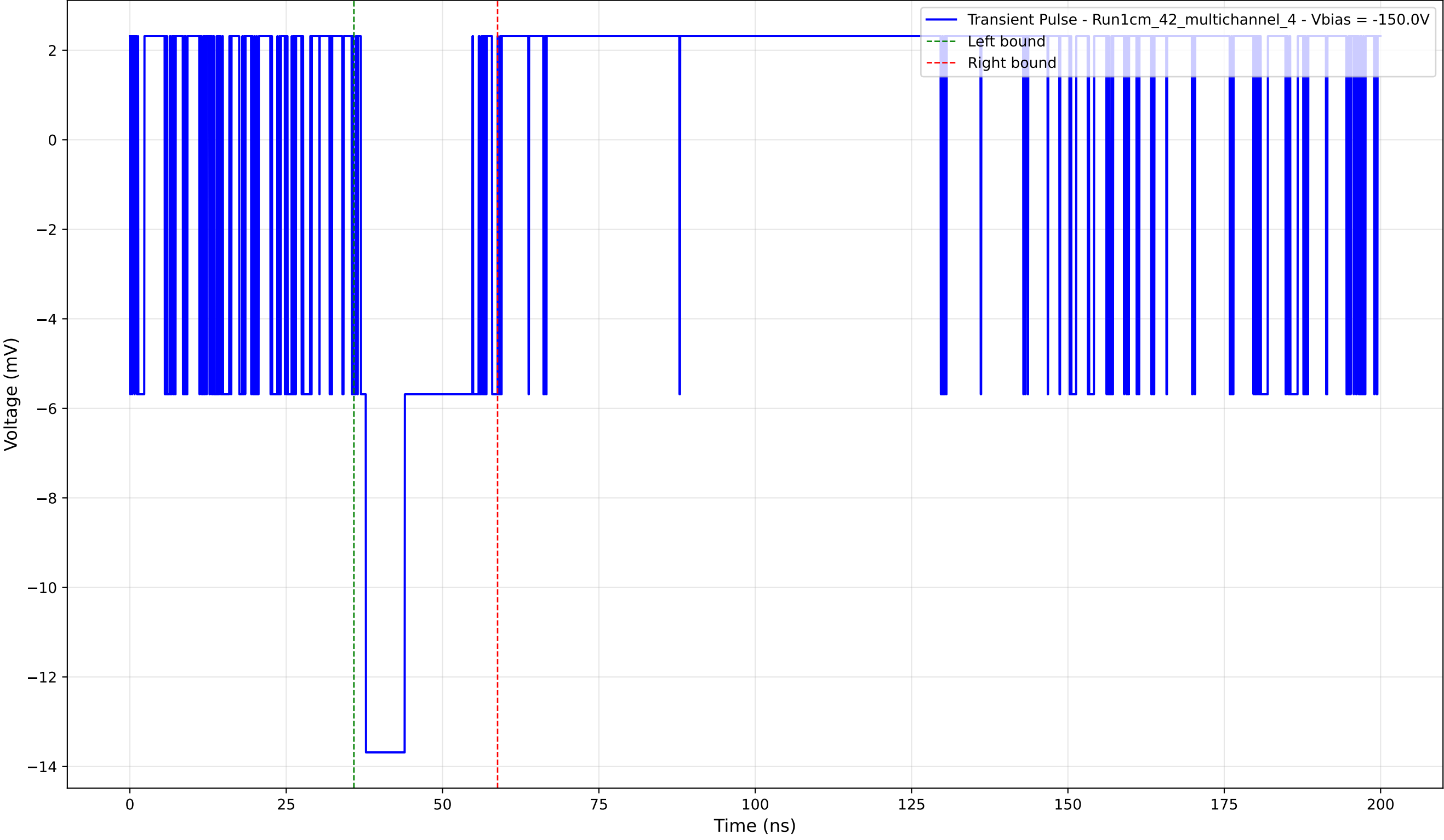
Transient Pulse - Sample: 1cm_42_multichannel - Position: 735.0 \mu\text{m} - Charge: 3.26 pC - Rise Time: 0.00 ns (N/A)
