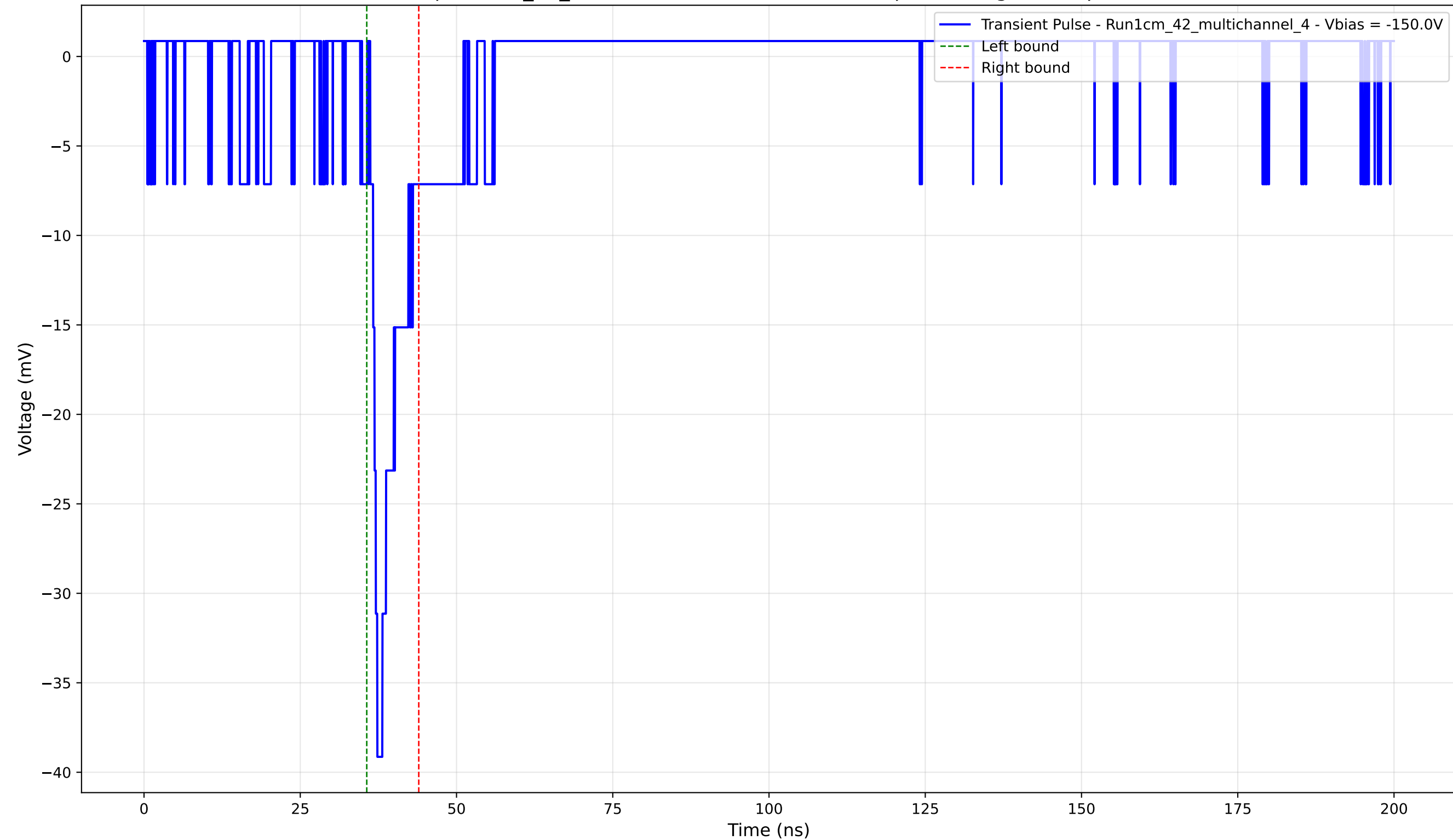
Transient Pulse - Sample: 1cm_42_multichannel - Position: 3000.0 \mu\text{m} - Charge: 2.96 pC - Rise Time: 1.13 ns
