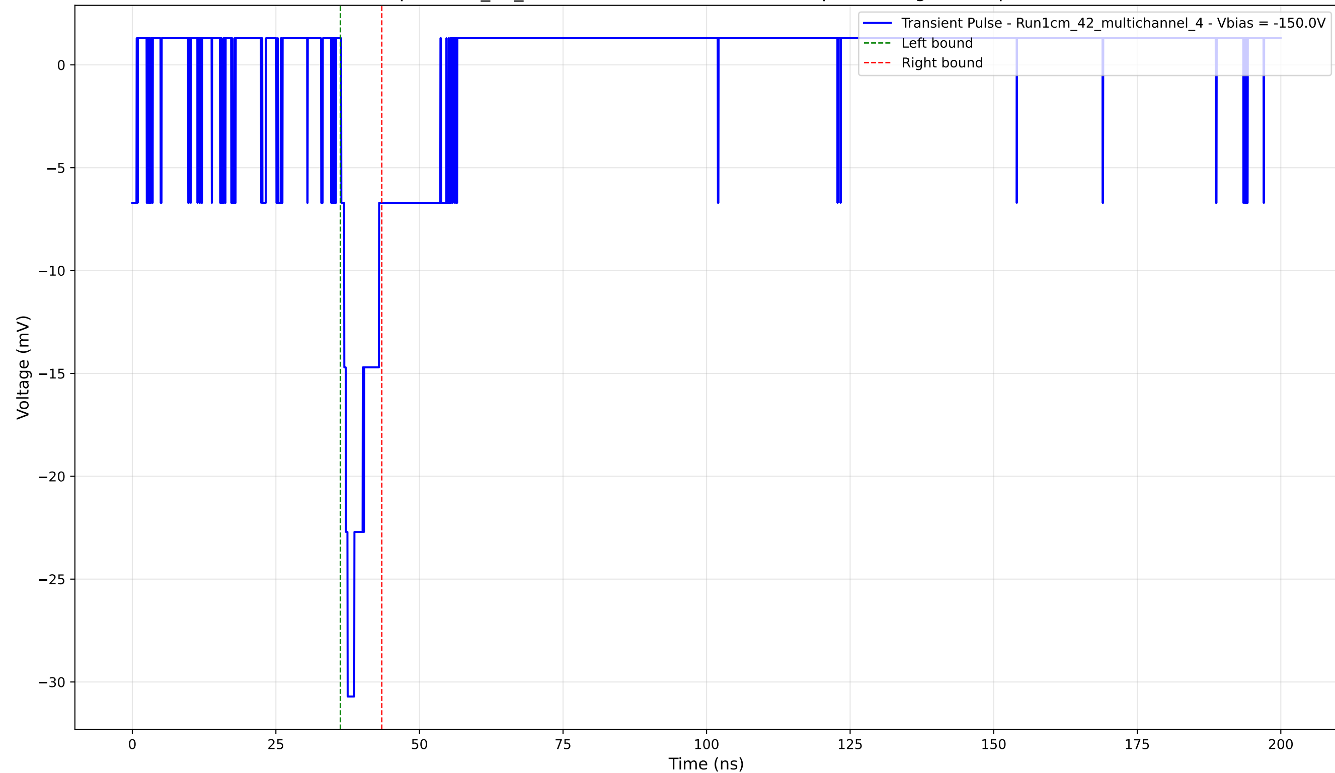
Transient Pulse - Sample: 1cm_42_multichannel - Position: 1530.0 \mu\text{m} - Charge: 2.59 pC - Rise Time: 1.11 ns
