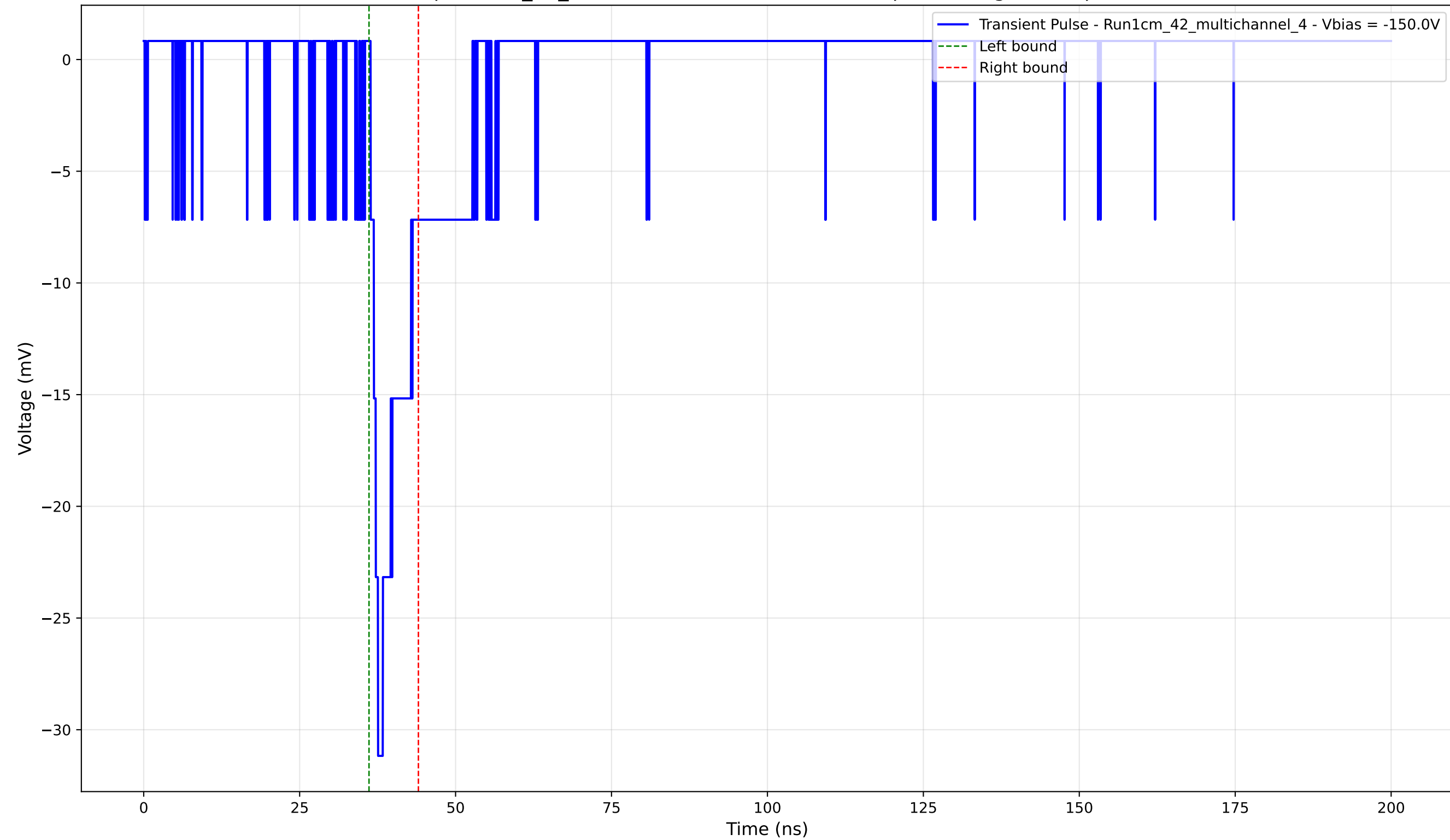
Transient Pulse - Sample: 1cm_42_multichannel - Position: 3220.0 \mu\text{m} - Charge: 2.59 pC - Rise Time: 1.19 ns
