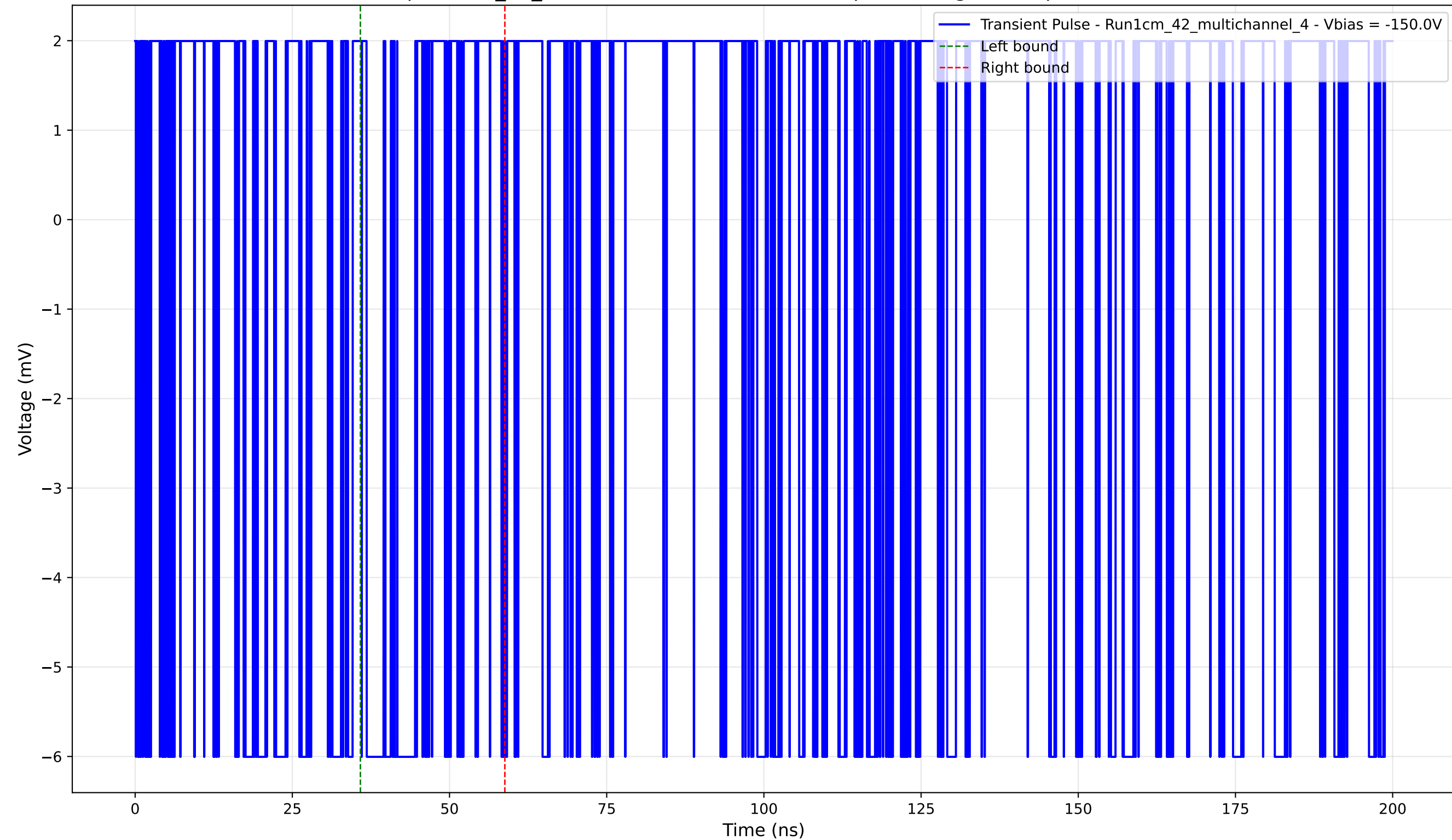
Transient Pulse - Sample: 1cm_42_multichannel - Position: 385.0 \mu\text{m} - Charge: 0.68 pC - Rise Time: 0.00 ns (N/A)
