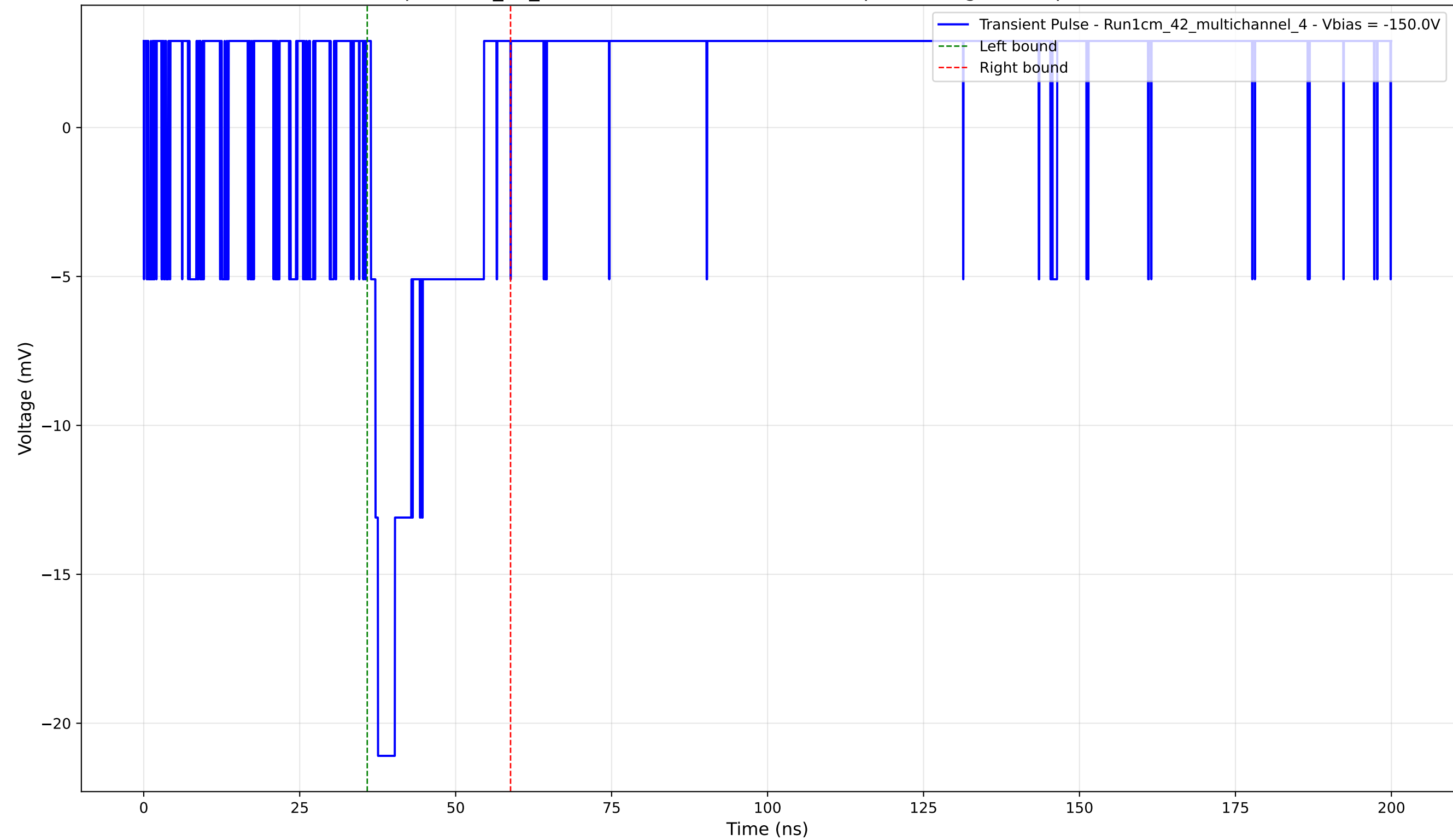
Transient Pulse - Sample: 1cm_42_multichannel - Position: 1280.0 \mu\text{m} - Charge: 2.99 pC - Rise Time: 0.00 ns (N/A)
