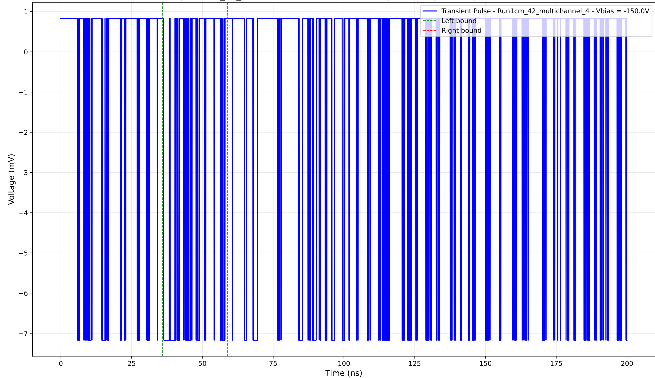
Transient Pulse - Sample: 1cm_42_multichannel - Position: 2385.0 \mu\text{m} - Charge: 1.02 pC - Rise Time: 0.00 ns (N/A)
