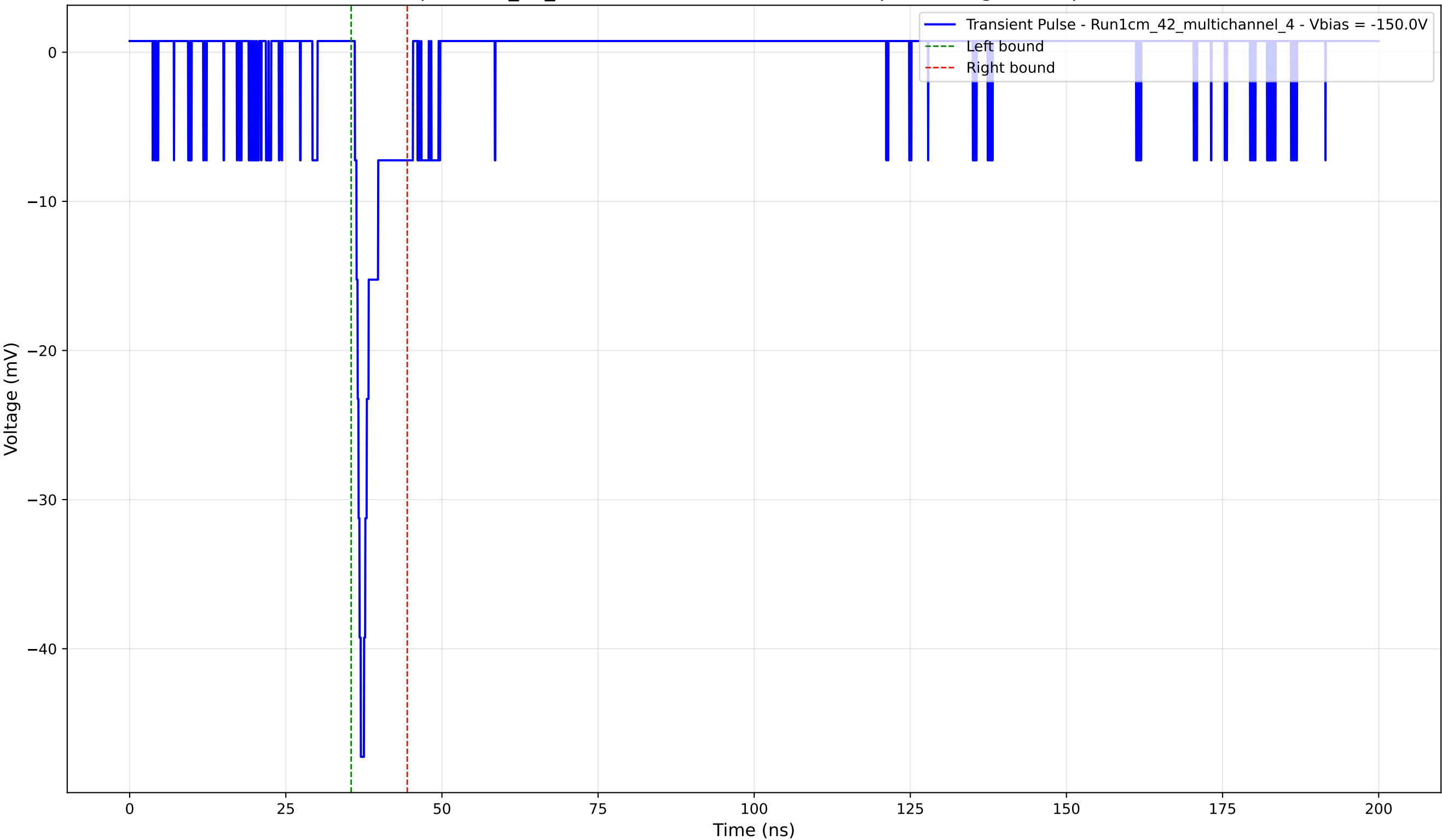
Transient Pulse - Sample: 1cm_42_multichannel - Position: 2440.0 \mu\text{m} - Charge: 2.48 pC - Rise Time: 0.95 ns
