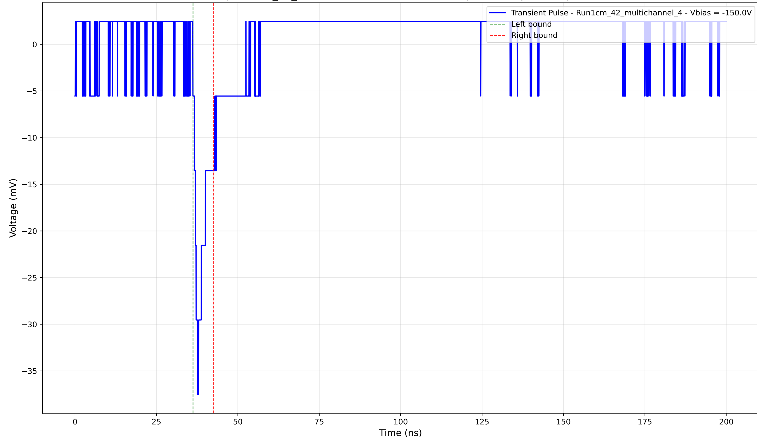
Transient Pulse - Sample: 1cm_42_multichannel - Position: 1675.0 \mu\text{m} - Charge: 2.45 pC - Rise Time: 1.41 ns
