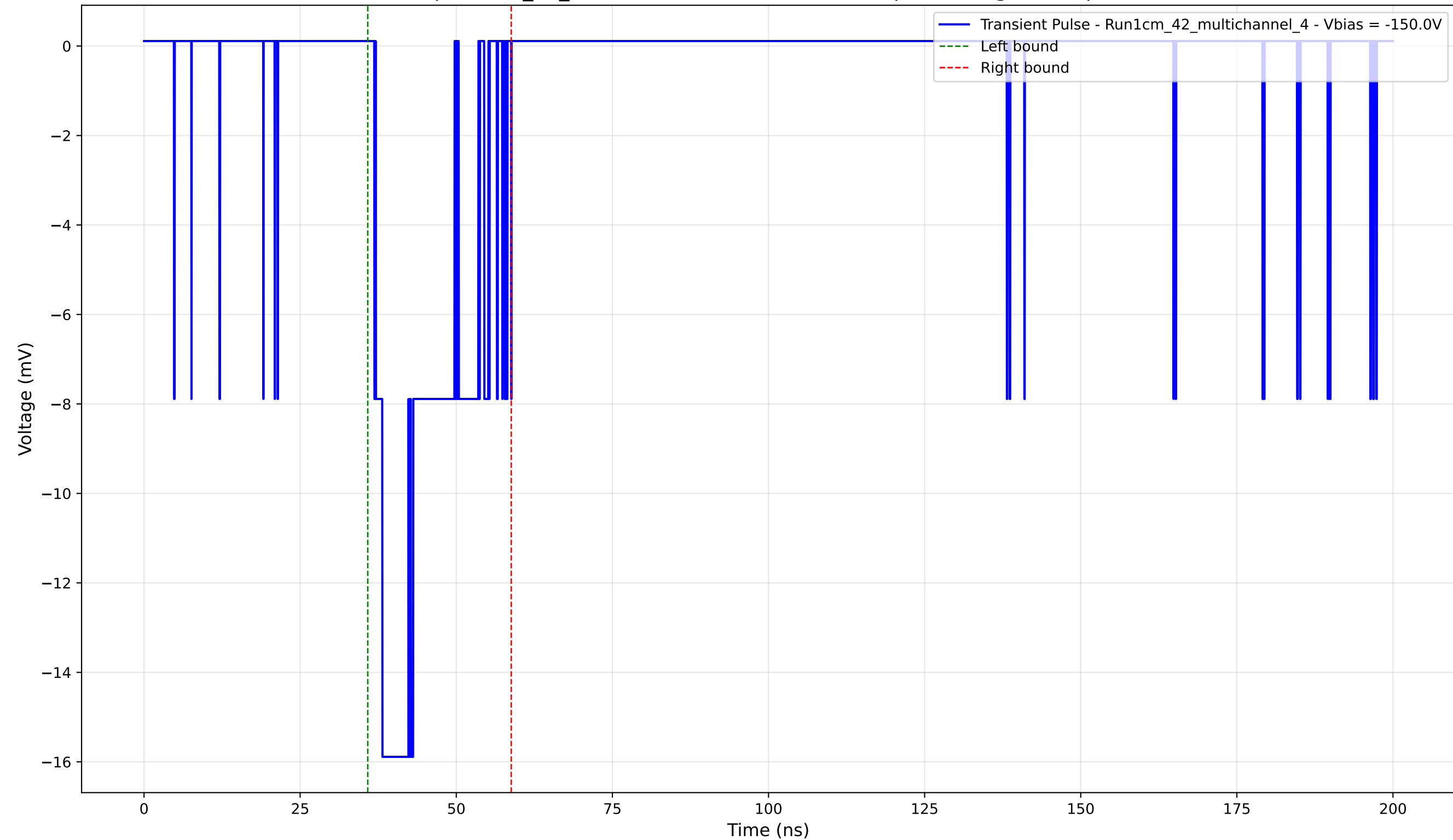
Transient Pulse - Sample: 1cm_42_multichannel - Position: 4060.0 \mu\text{m} - Charge: 3.53 pC - Rise Time: 1.06 ns
