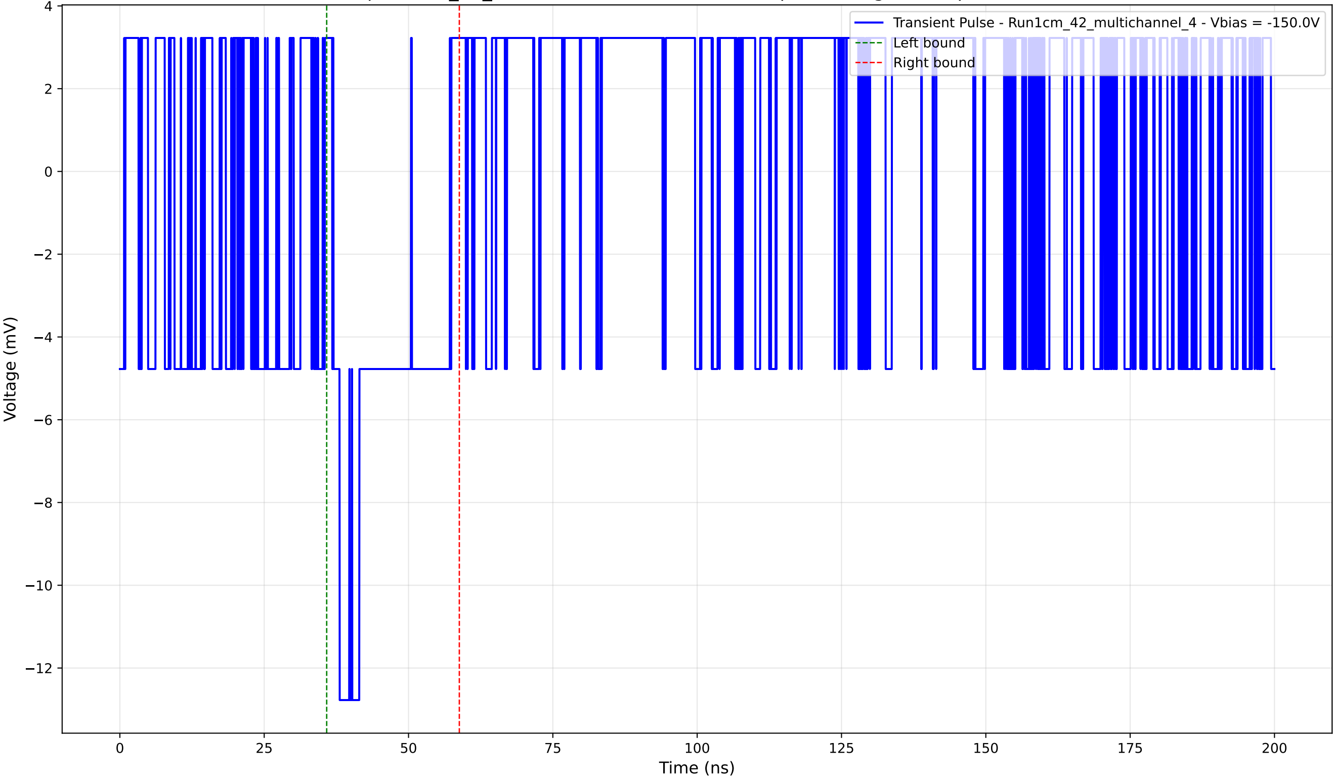
Transient Pulse - Sample: 1cm_42_multichannel - Position: 920.0 \mu\text{m} - Charge: 2.29 pC - Rise Time: 0.00 ns (N/A)
