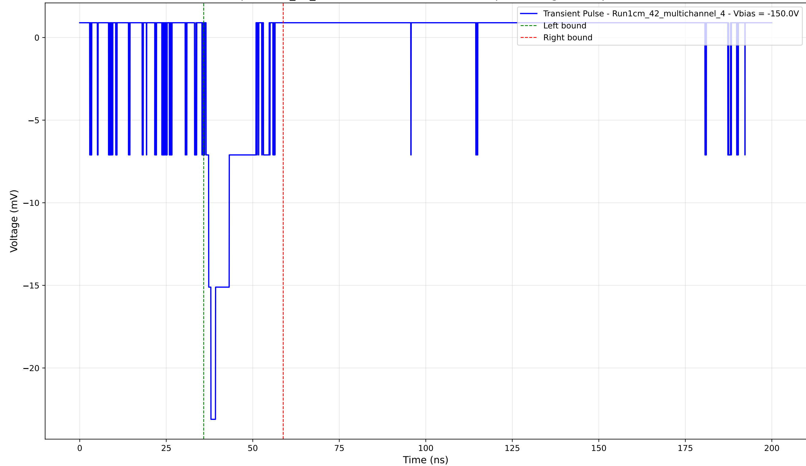
Transient Pulse - Sample: 1cm_42_multichannel - Position: 3525.0 \mu\text{m} - Charge: 3.43 pC - Rise Time: 1.42 ns
