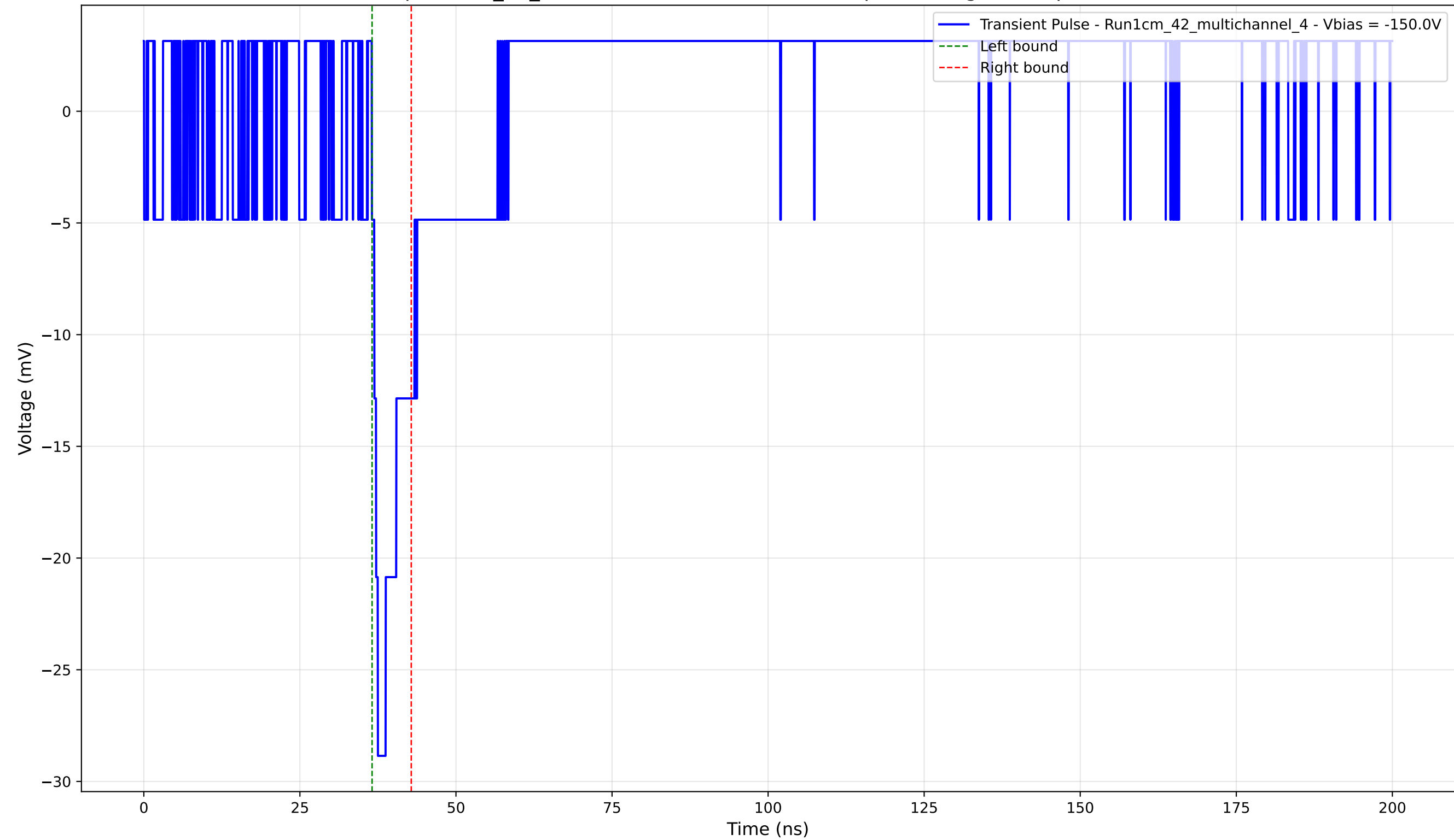
Transient Pulse - Sample: 1cm_42_multichannel - Position: 1505.0 \mu\text{m} - Charge: 2.28 pC - Rise Time: 0.00 ns (N/A)
