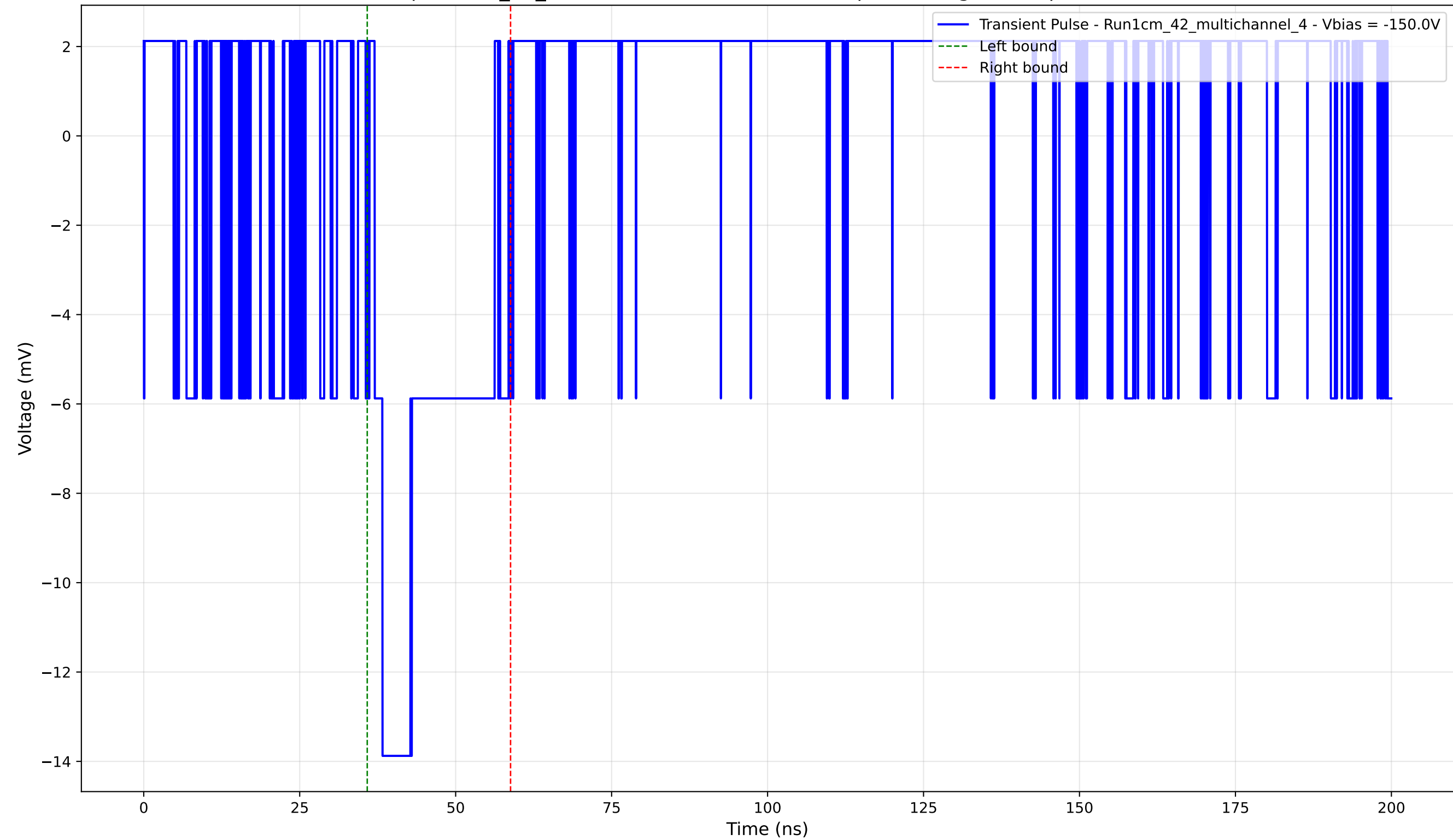
Transient Pulse - Sample: 1cm_42_multichannel - Position: 285.0 \mu\text{m} - Charge: 3.14 pC - Rise Time: 0.00 ns (N/A)
