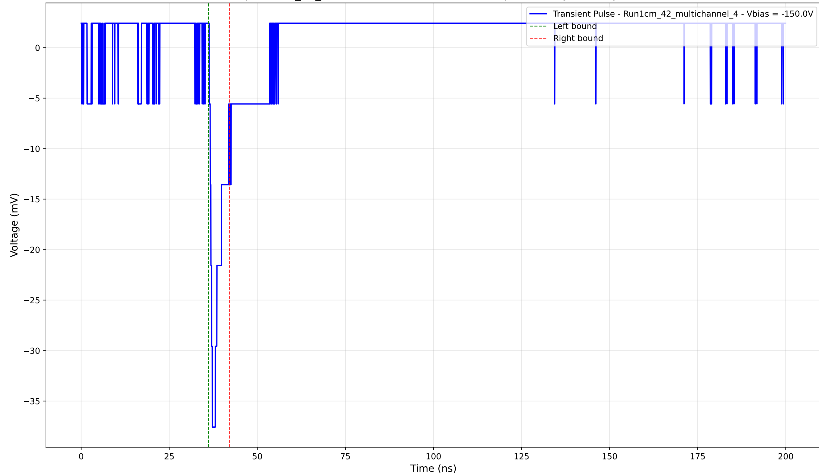
Transient Pulse - Sample: 1cm_42_multichannel - Position: 1805.0 \mu\text{m} - Charge: 2.34 pC - Rise Time: 0.89 ns
