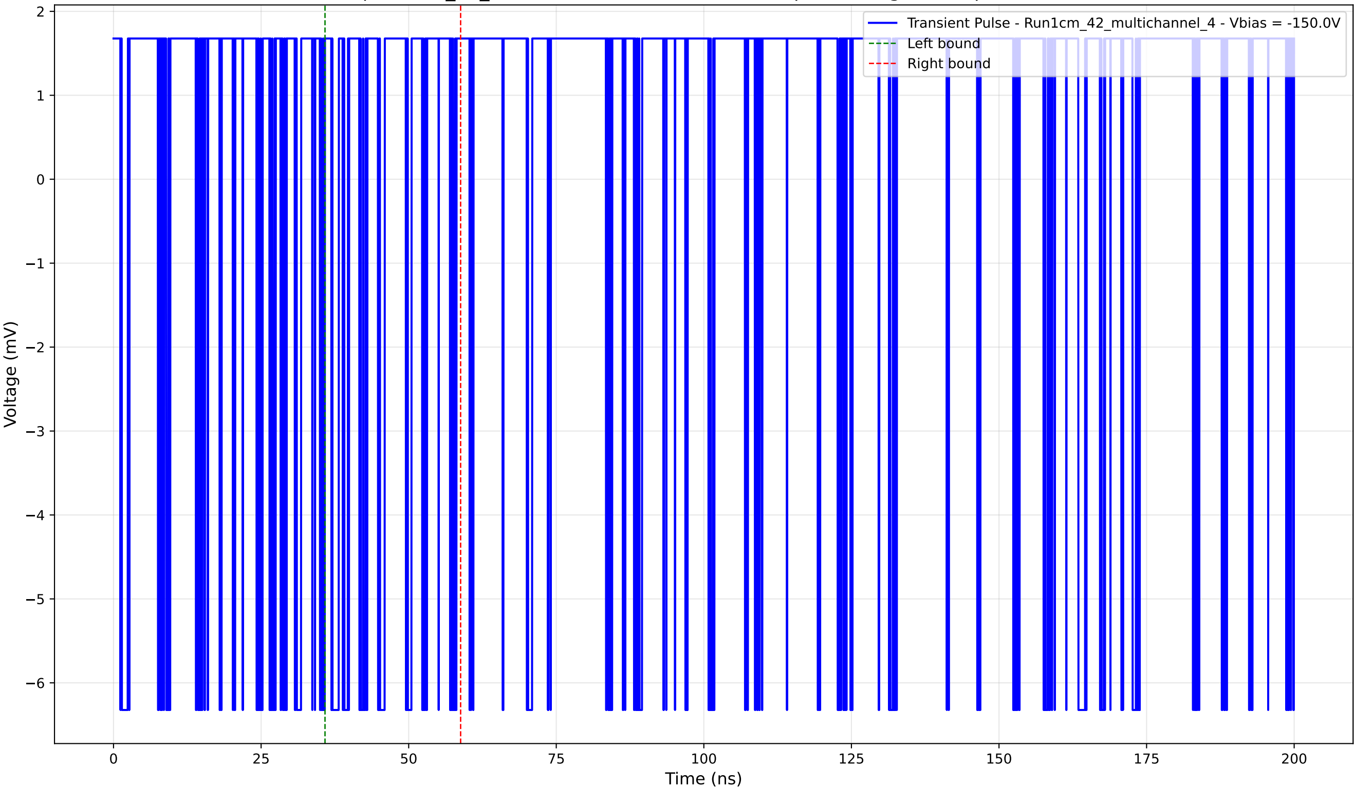
Transient Pulse - Sample: 1cm_42_multichannel - Position: 2900.0 \mu\text{m} - Charge: 0.22 pC - Rise Time: 0.00 ns (N/A)
