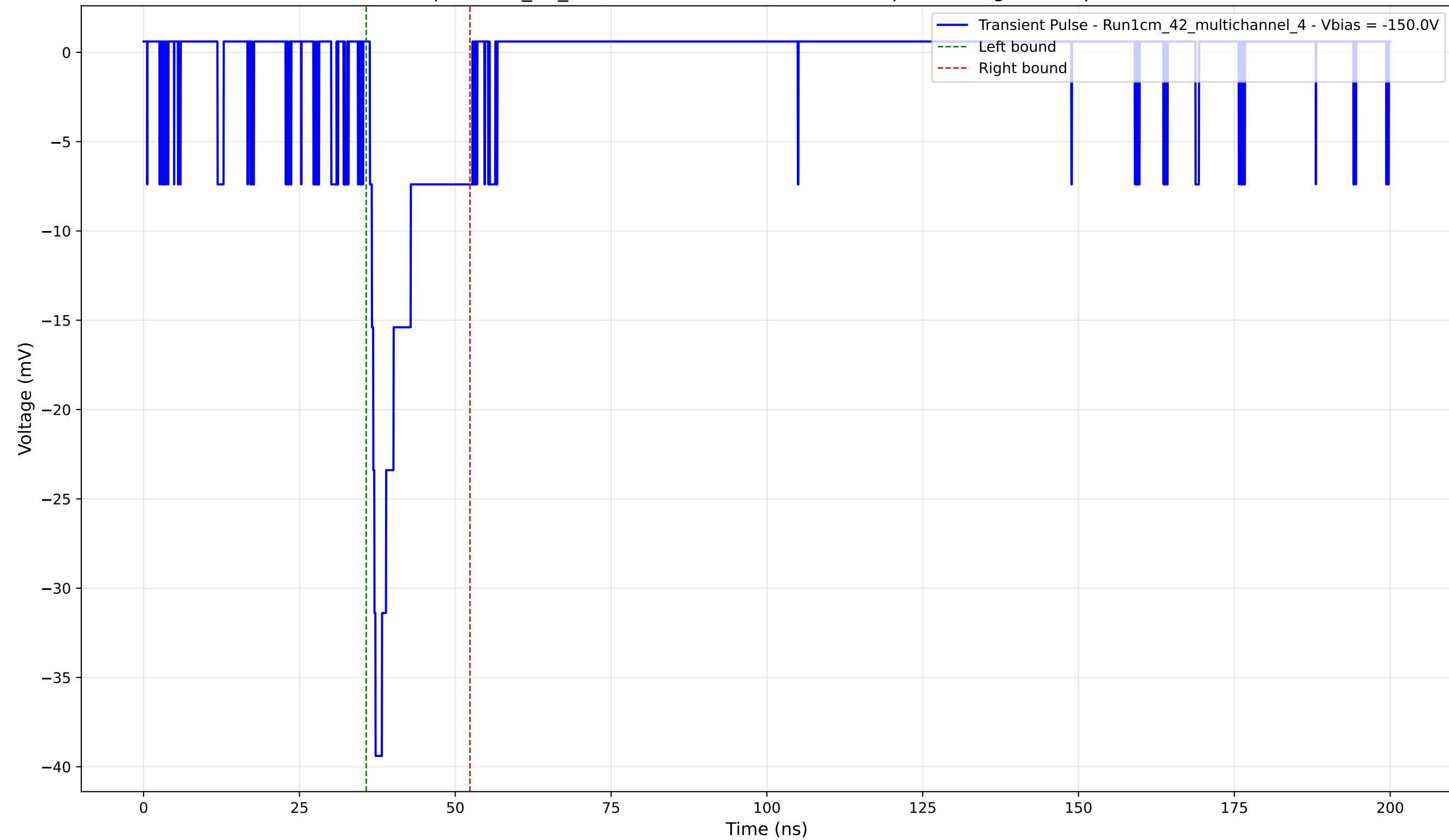
Transient Pulse - Sample: 1cm_42_multichannel - Position: 1770.0 \mu\text{m} - Charge: 4.36 pC - Rise Time: 0.91 ns
