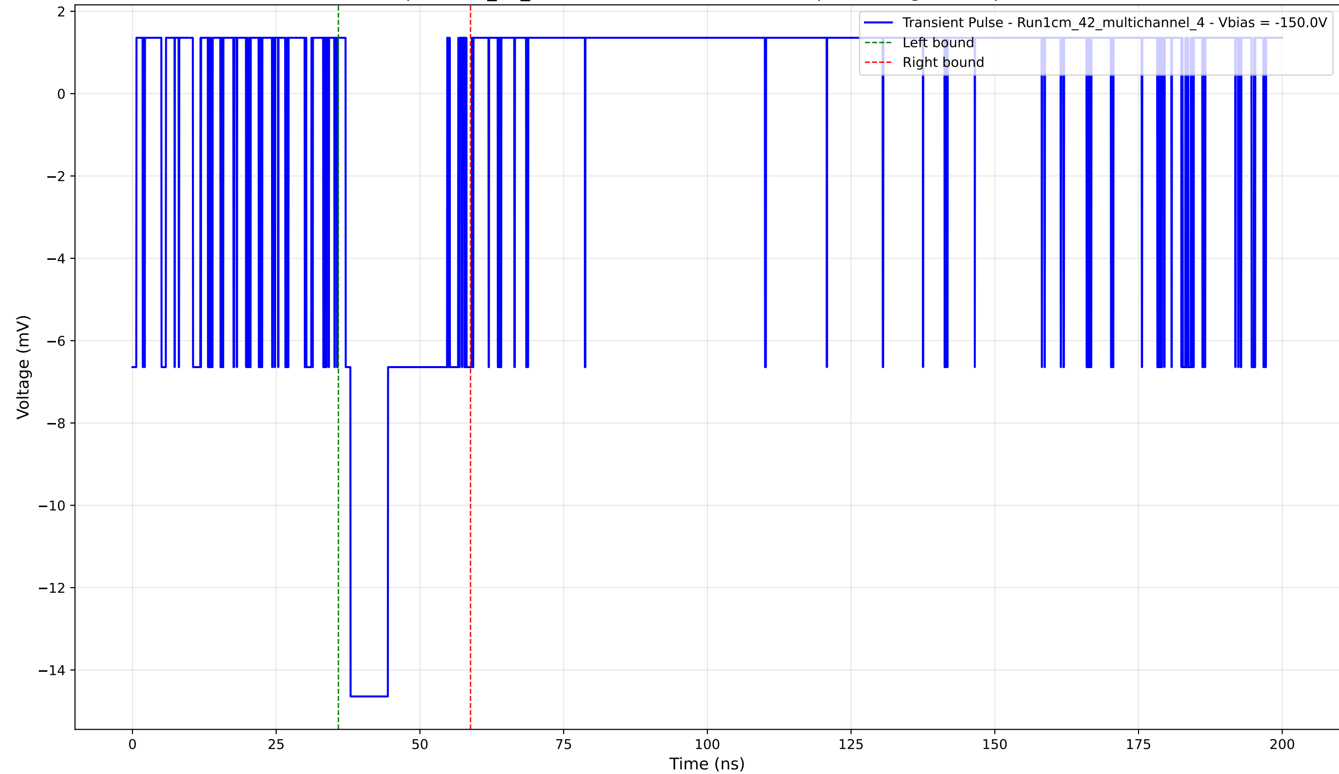
Transient Pulse - Sample: 1cm_42_multichannel - Position: 640.0 \mu\text{m} - Charge: 3.73 pC - Rise Time: 0.86 ns
