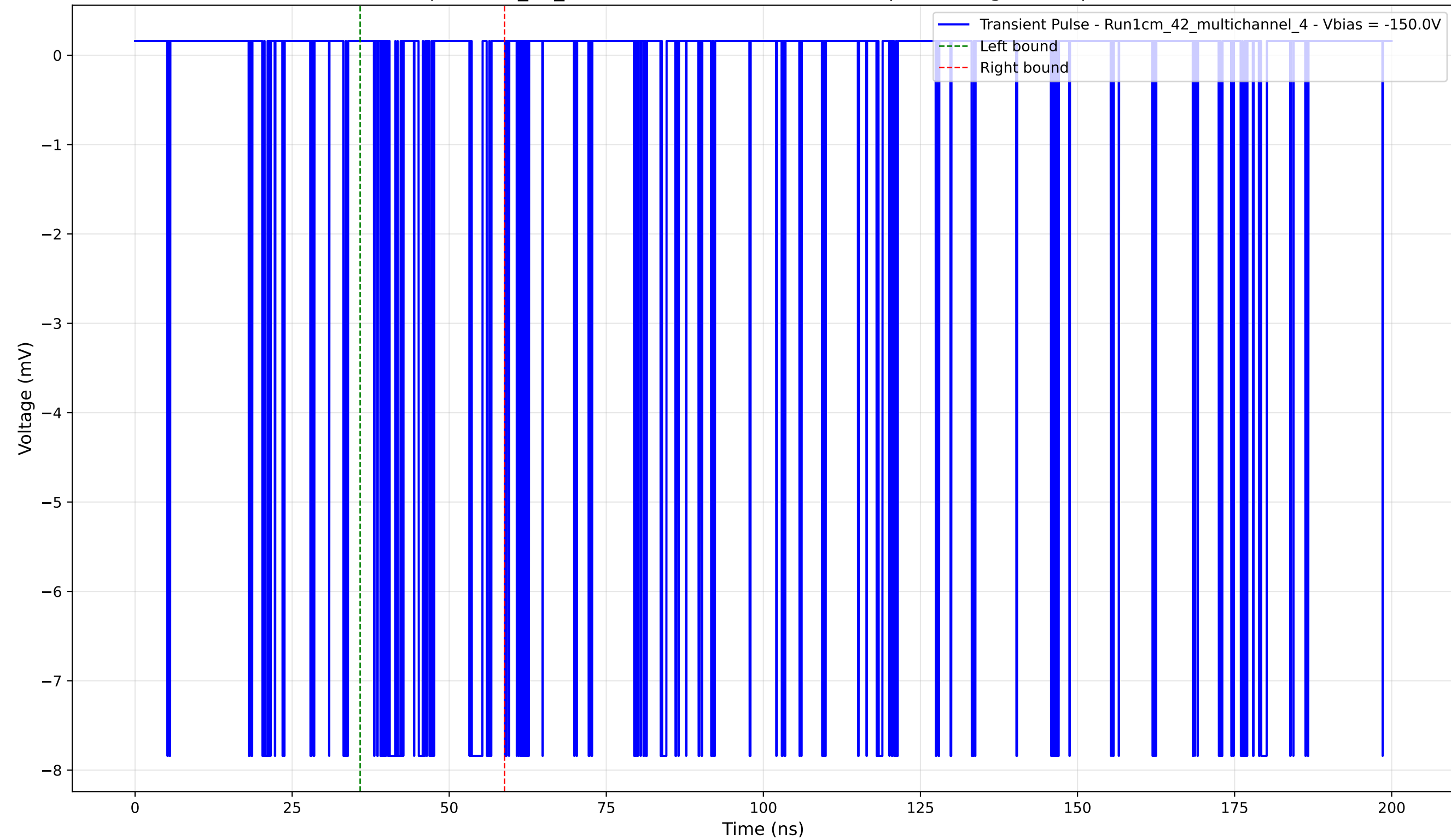
Transient Pulse - Sample: 1cm_42_multichannel - Position: 3925.0 \mu\text{m} - Charge: 1.03 pC - Rise Time: 0.02 ns
