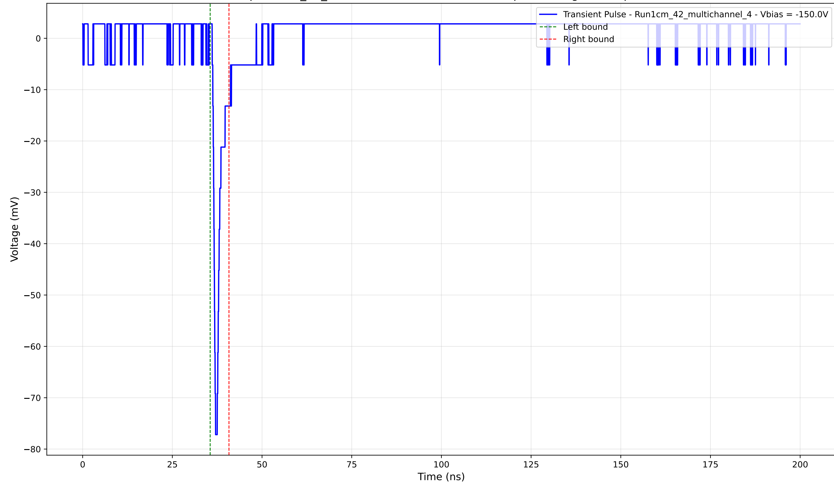
Transient Pulse - Sample: 1cm_42_multichannel - Position: 2270.0 \mu\text{m} - Charge: 3.05 pC - Rise Time: 0.77 ns
