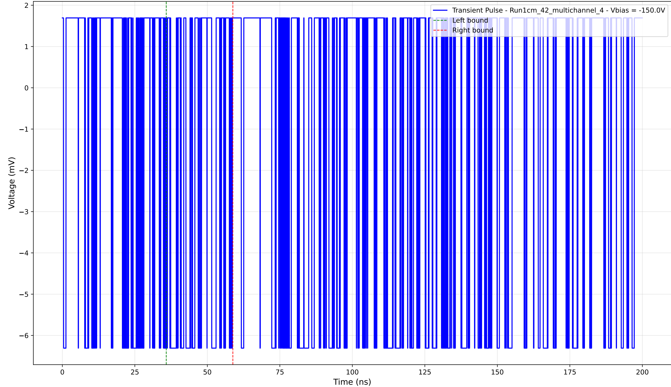
Transient Pulse - Sample: 1cm_42_multichannel - Position: 1370.0 \mu\text{m} - Charge: 0.84 pC - Rise Time: 0.00 ns (N/A)
