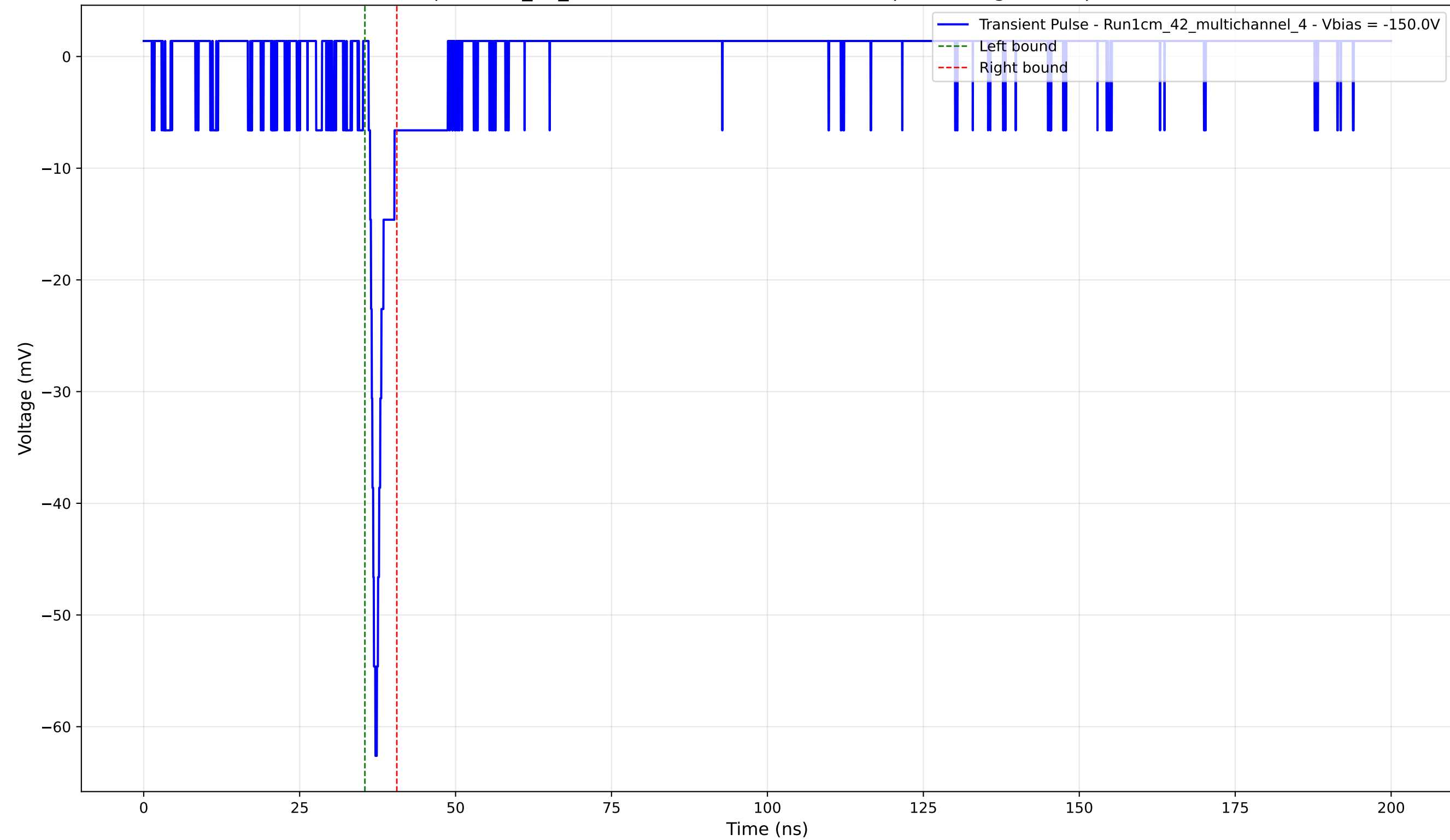
Transient Pulse - Sample: 1cm_42_multichannel - Position: 2445.0 \mu\text{m} - Charge: 2.27 pC - Rise Time: 1.08 ns
