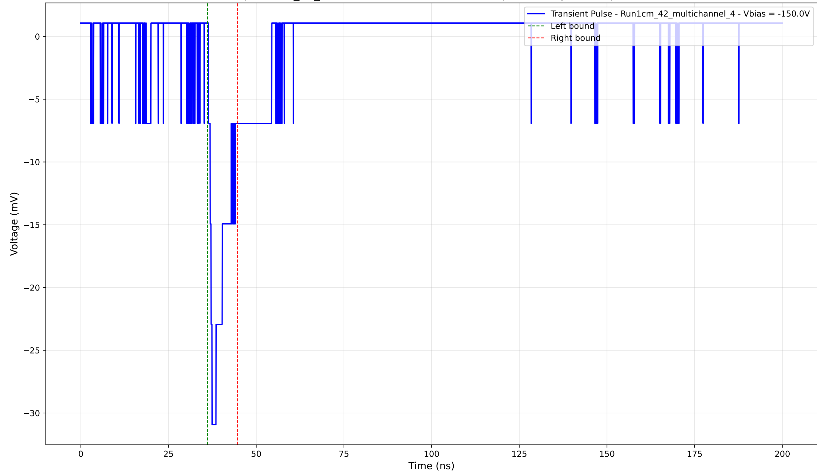
Transient Pulse - Sample: 1cm_42_multichannel - Position: 1565.0 \mu\text{m} - Charge: 2.92 pC - Rise Time: 1.03 ns
