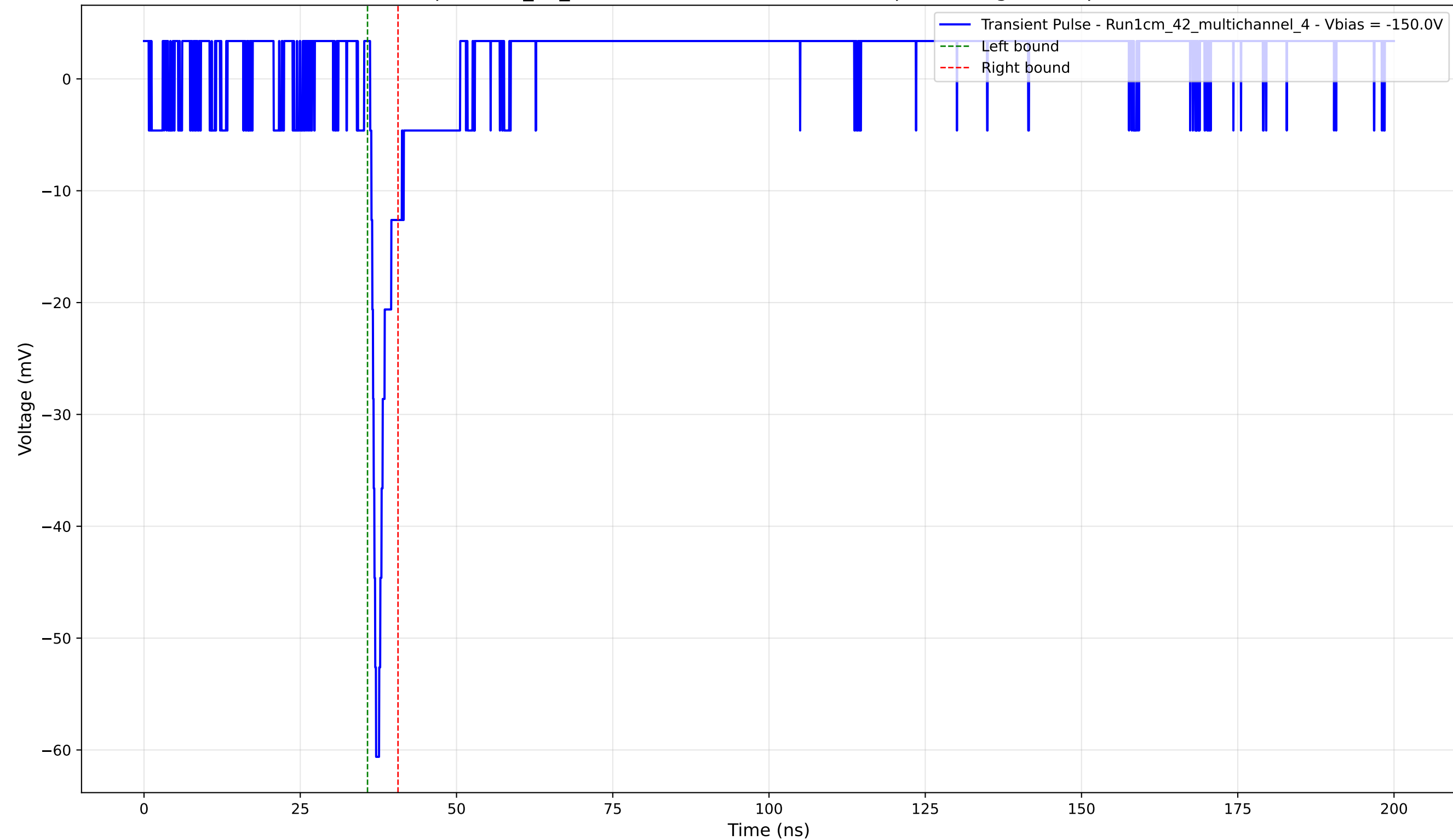
Transient Pulse - Sample: 1cm_42_multichannel - Position: 2620.0 \mu\text{m} - Charge: 2.48 pC - Rise Time: 0.76 ns
