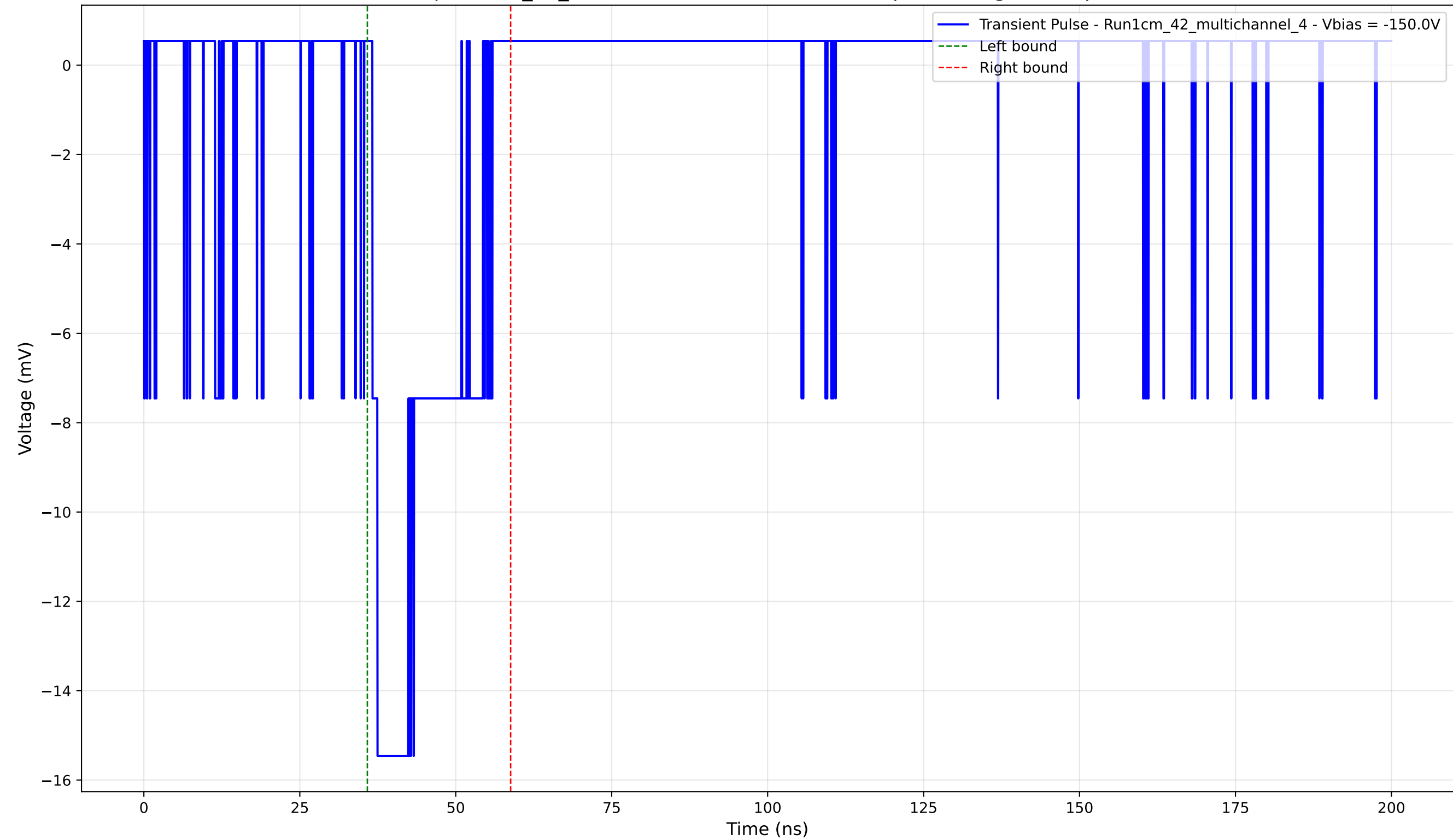
Transient Pulse - Sample: 1cm_42_multichannel - Position: 3640.0 \mu\text{m} - Charge: 3.48 pC - Rise Time: 0.82 ns
