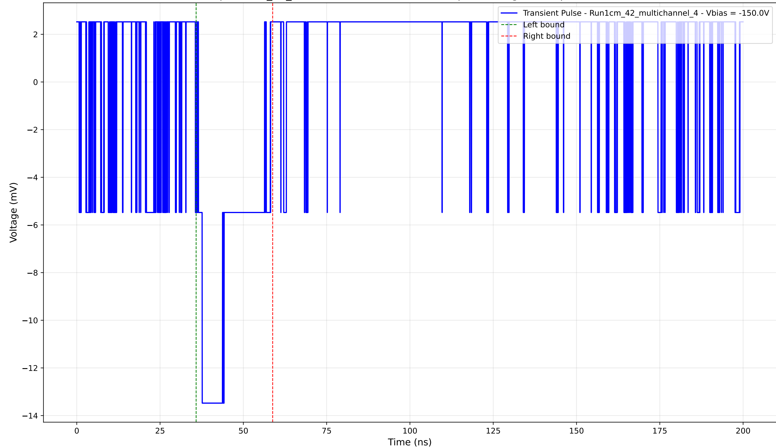
Transient Pulse - Sample: 1cm_42_multichannel - Position: 940.0 \mu\text{m} - Charge: 3.32 pC - Rise Time: 0.00 ns (N/A)
