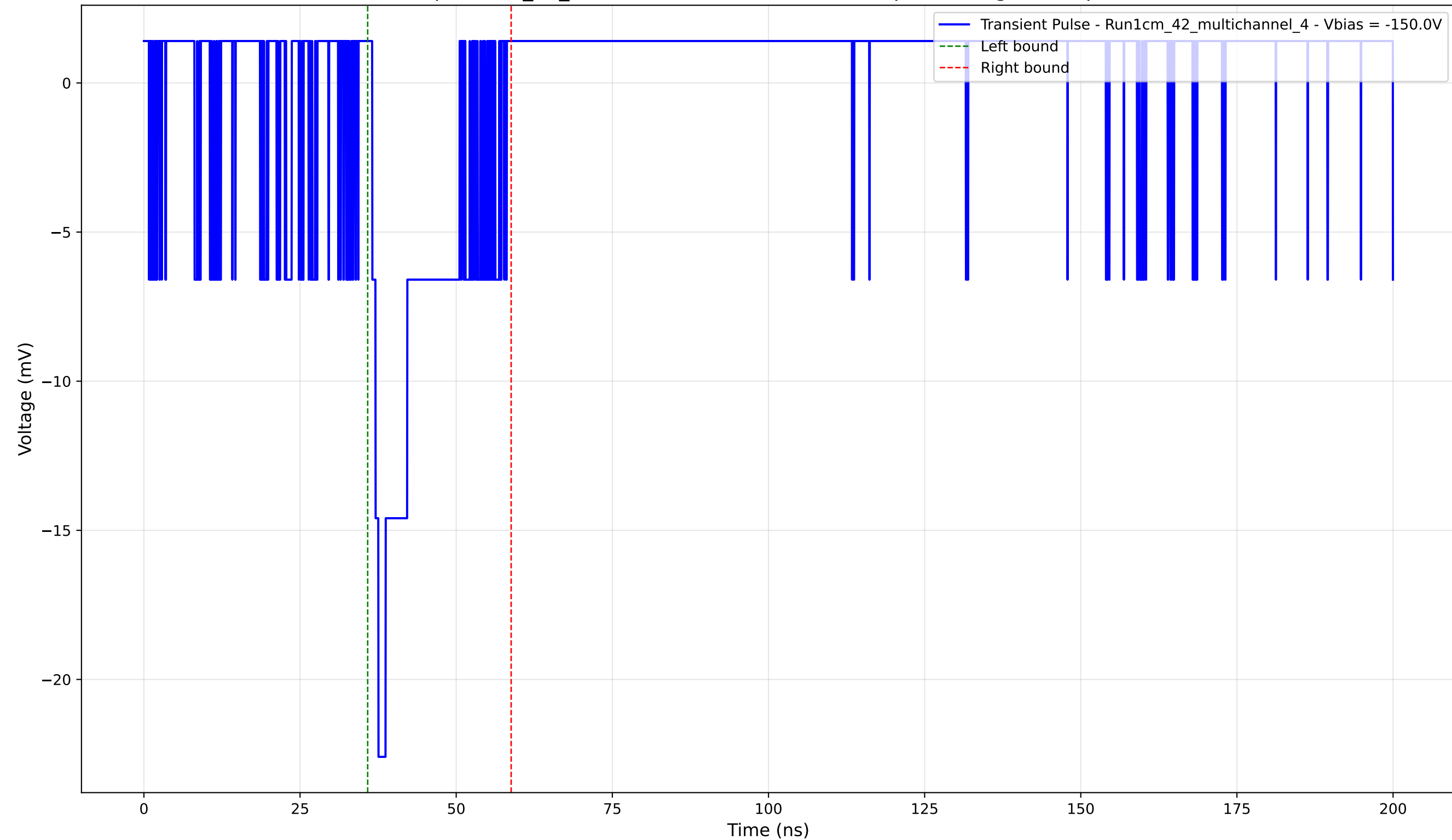
Transient Pulse - Sample: 1cm_42_multichannel - Position: 3330.0 \mu\text{m} - Charge: 3.33 pC - Rise Time: 1.00 ns
