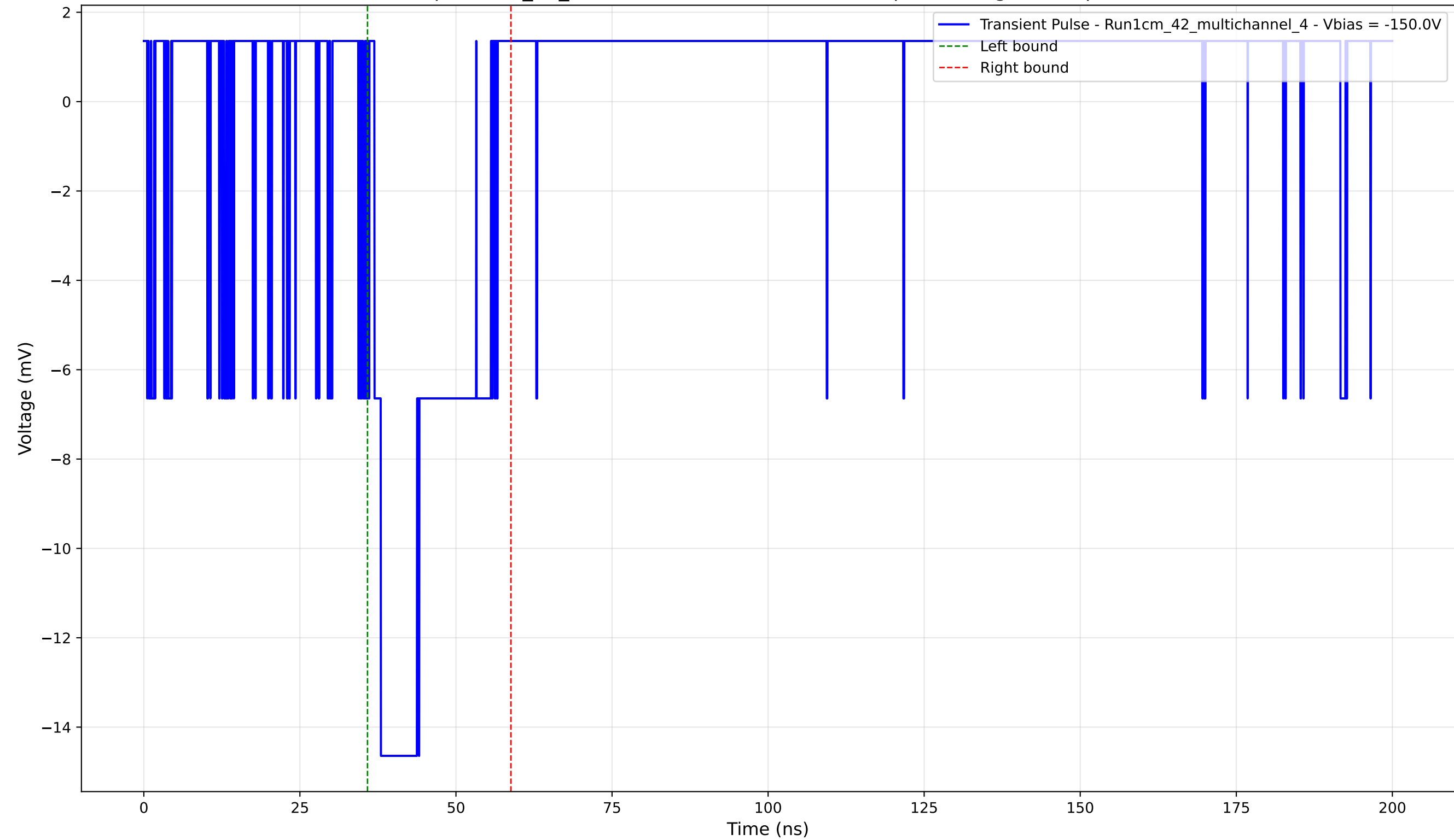
Transient Pulse - Sample: 1cm_42_multichannel - Position: 4055.0 \mu\text{m} - Charge: 3.37 pC - Rise Time: 1.04 ns
