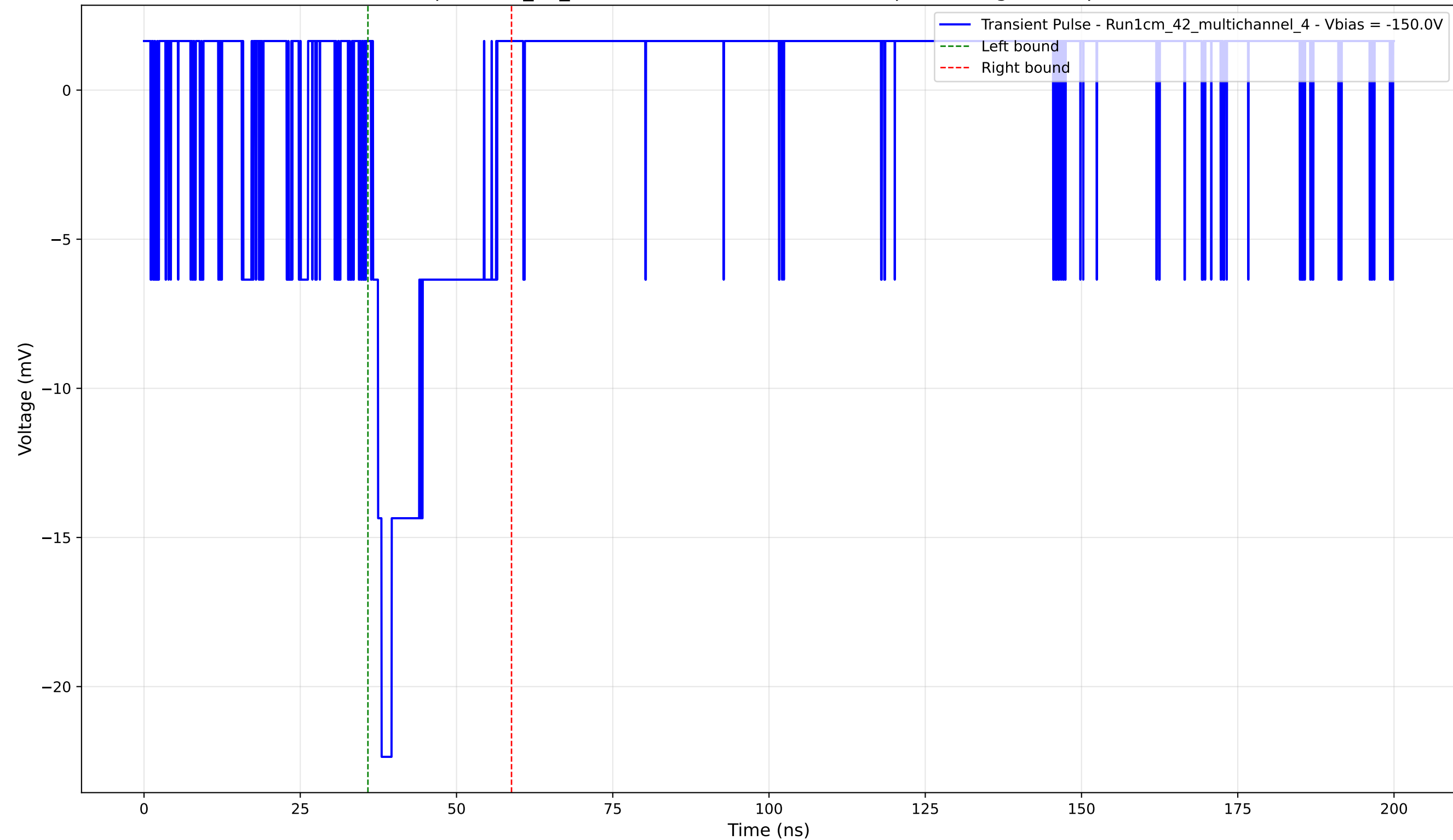
Transient Pulse - Sample: 1cm_42_multichannel - Position: 1070.0 \mu\text{m} - Charge: 3.75 pC - Rise Time: 1.38 ns
