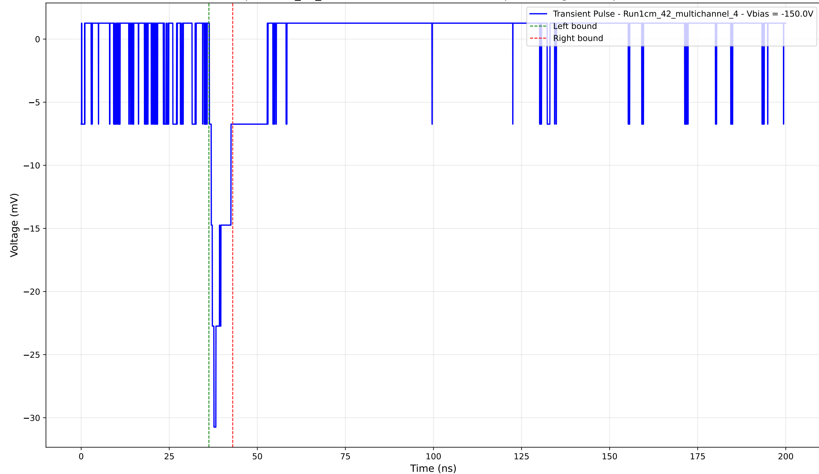
Transient Pulse - Sample: 1cm_42_multichannel - Position: 3230.0 \mu\text{m} - Charge: 2.26 pC - Rise Time: 1.31 ns
