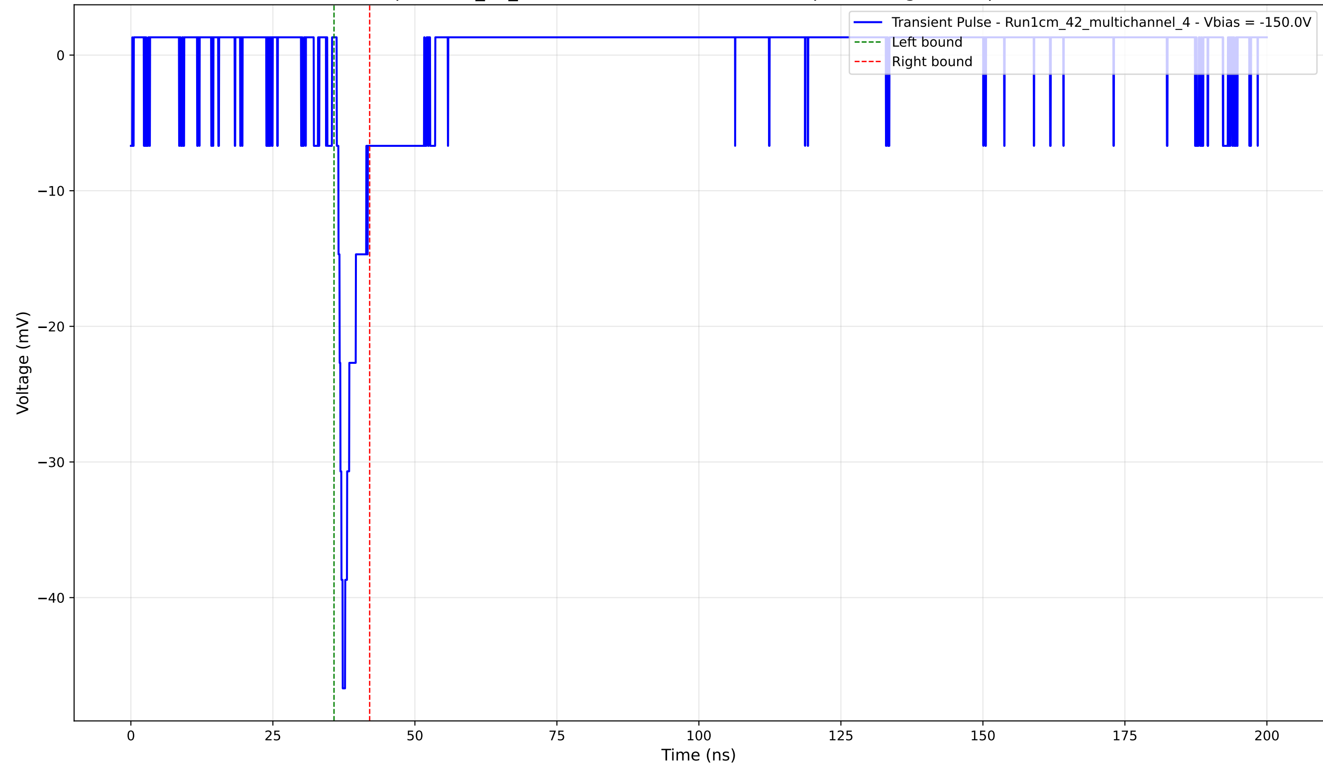
Transient Pulse - Sample: 1cm_42_multichannel - Position: 2815.0 \mu\text{m} - Charge: 2.51 pC - Rise Time: 1.05 ns
