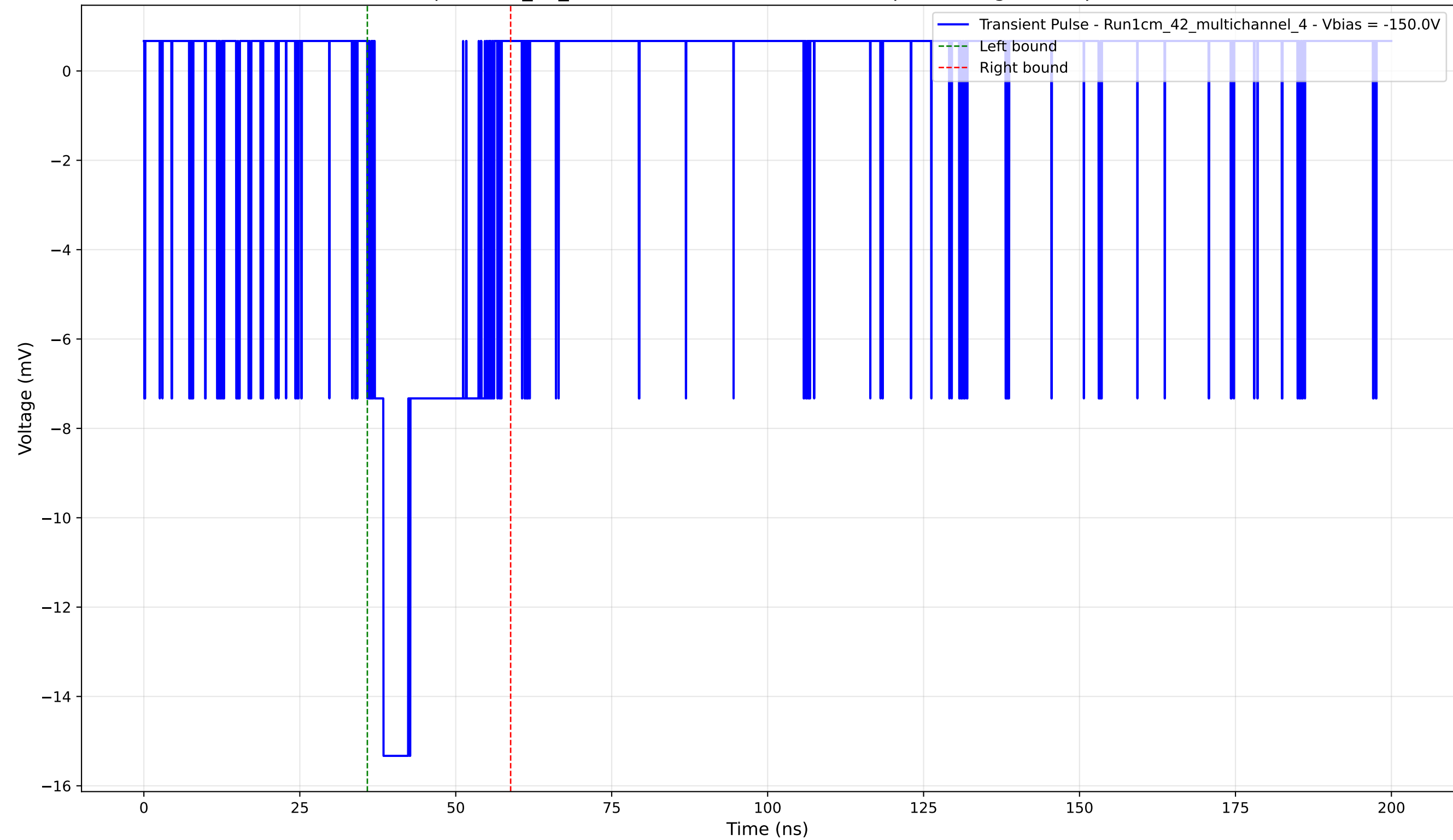
Transient Pulse - Sample: 1cm_42_multichannel - Position: 4605.0 \mu\text{m} - Charge: 3.40 pC - Rise Time: 1.40 ns
