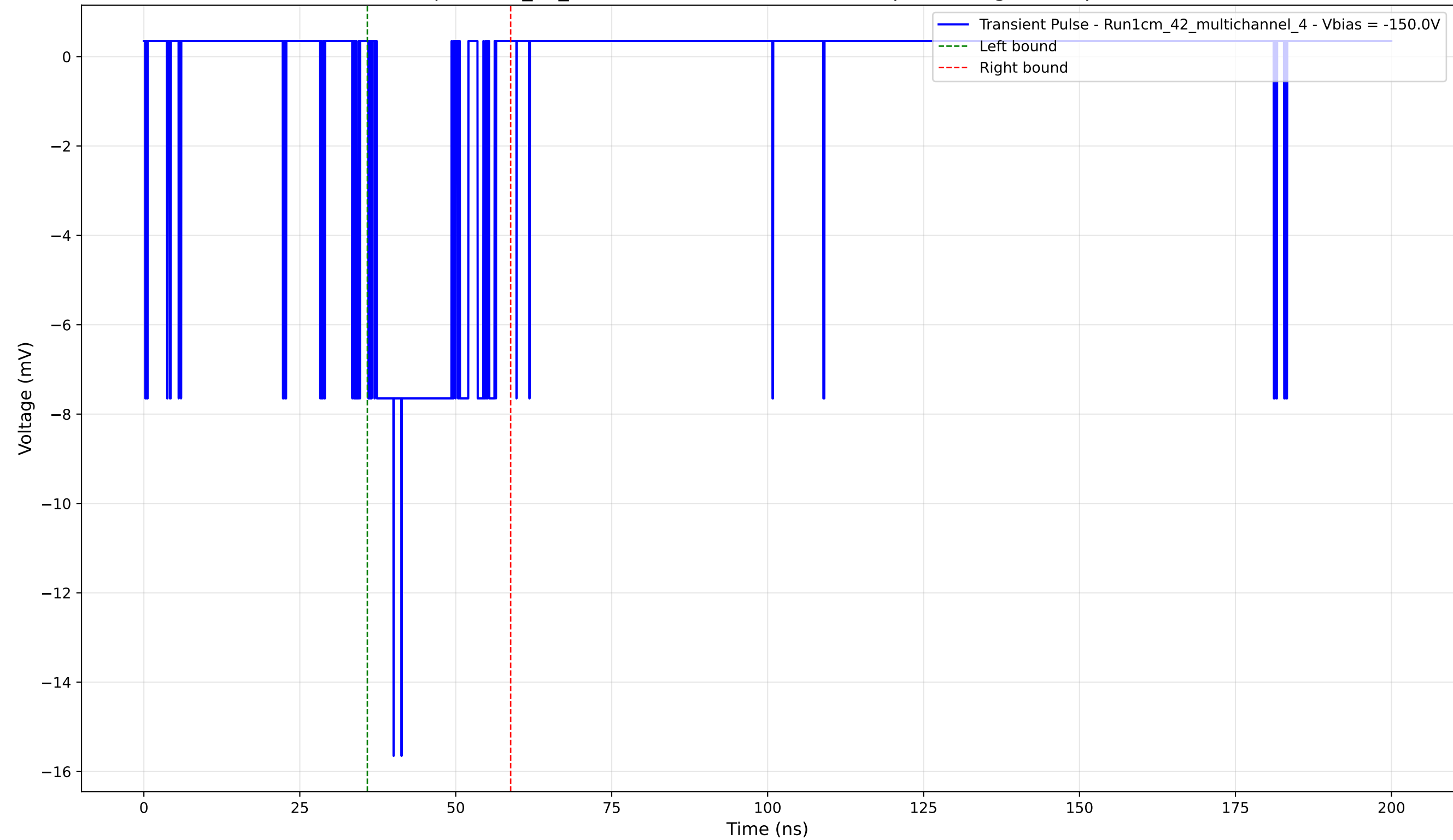
Transient Pulse - Sample: 1cm_42_multichannel - Position: 4830.0 \mu\text{m} - Charge: 2.48 pC - Rise Time: 2.70 ns
