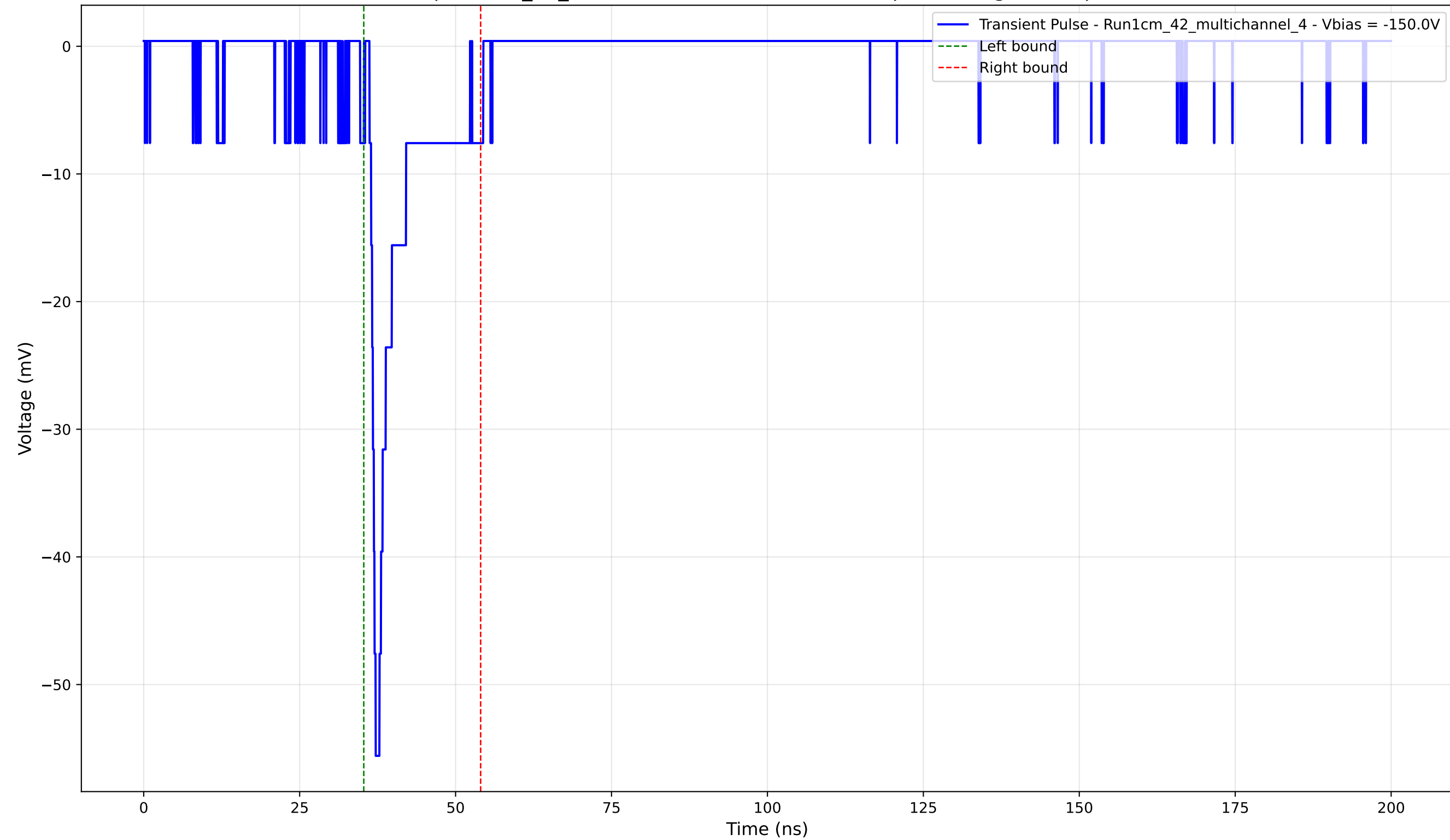
Transient Pulse - Sample: 1cm_42_multichannel - Position: 2025.0 \mu\text{m} - Charge: 4.93 pC - Rise Time: 0.99 ns
