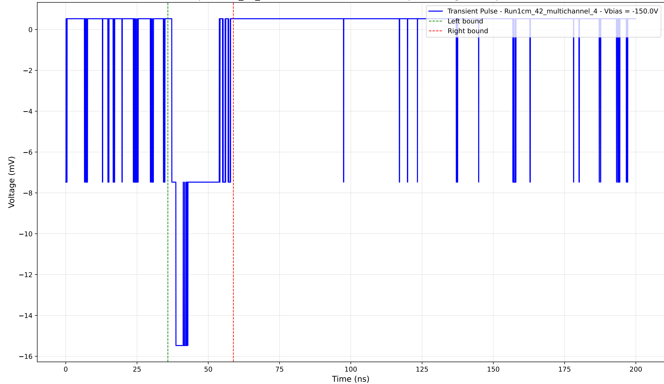
Transient Pulse - Sample: 1cm_42_multichannel - Position: 4715.0 \mu\text{m} - Charge: 3.31 pC - Rise Time: 1.46 ns
