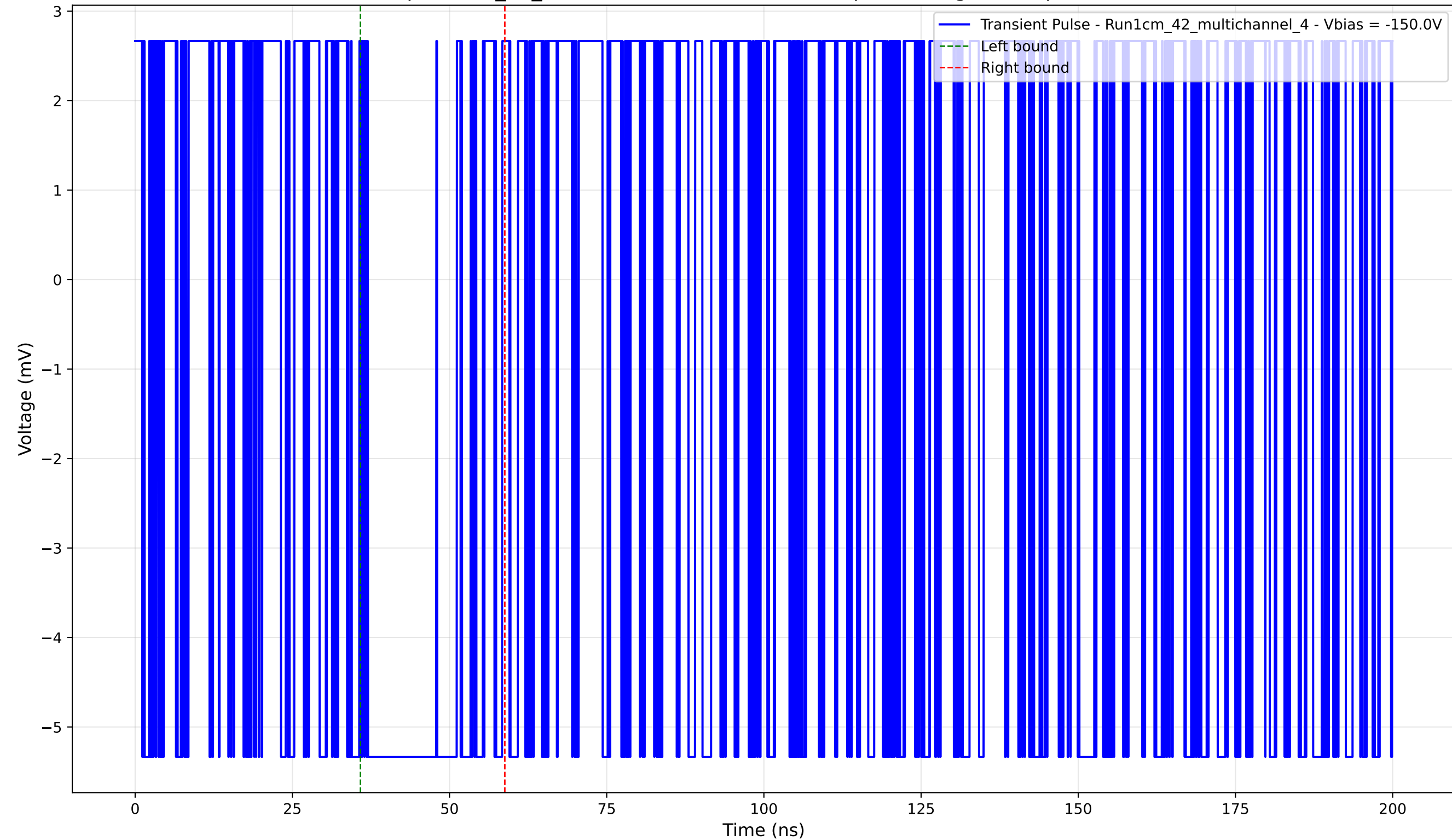
Transient Pulse - Sample: 1cm_42_multichannel - Position: 320.0 \mu\text{m} - Charge: 1.72 pC - Rise Time: 0.00 ns (N/A)
