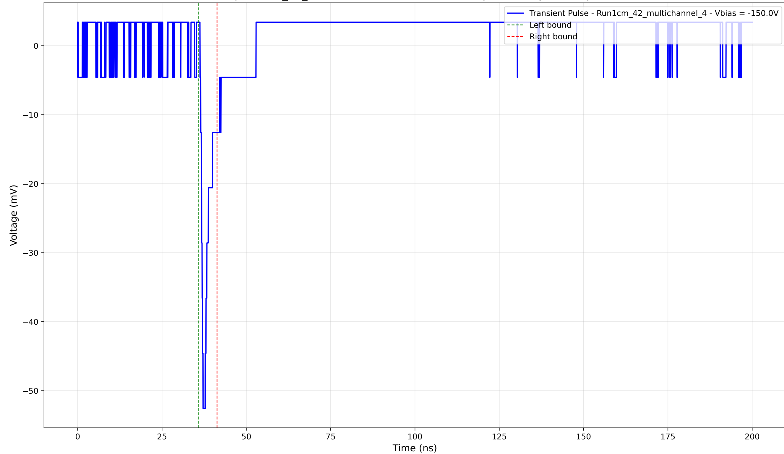
Transient Pulse - Sample: 1cm_42_multichannel - Position: 2015.0 \mu\text{m} - Charge: 2.56 pC - Rise Time: 0.70 ns
