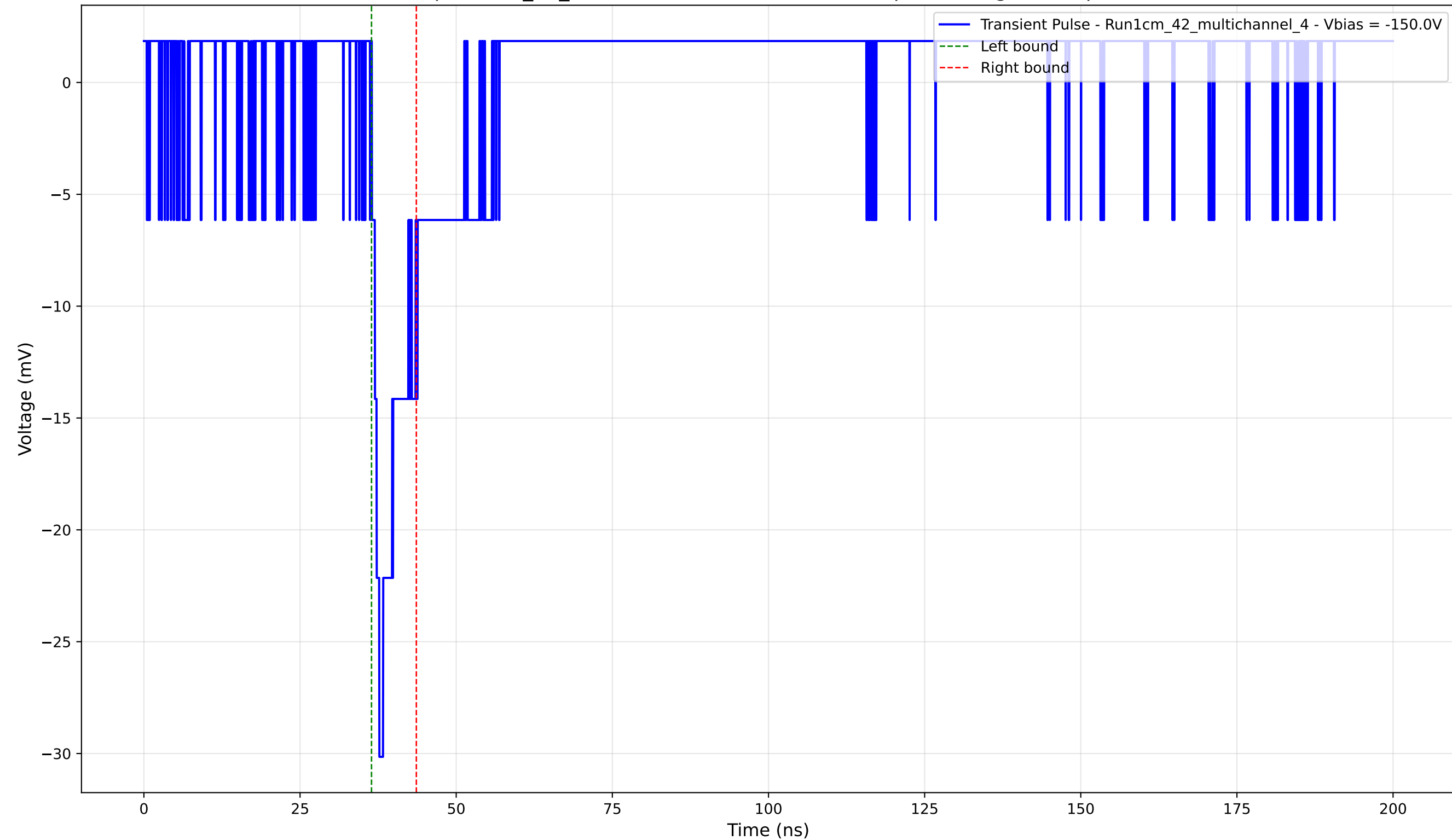
Transient Pulse - Sample: 1cm_42_multichannel - Position: 3275.0 \mu\text{m} - Charge: 2.39 pC - Rise Time: 1.19 ns
