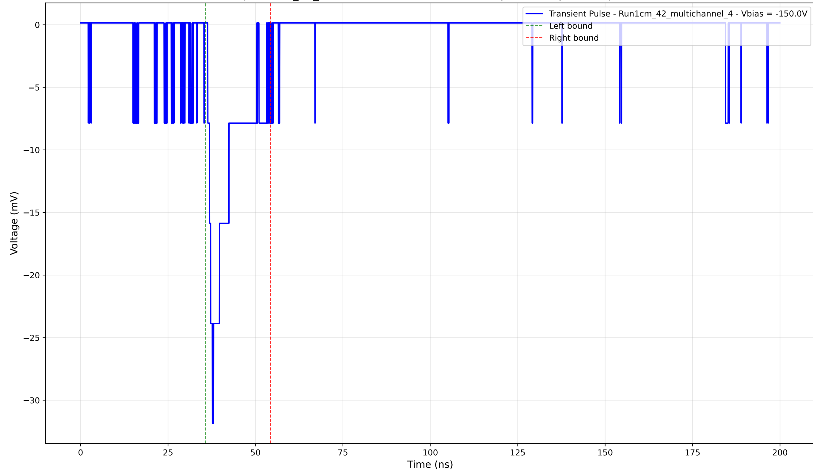
Transient Pulse - Sample: 1cm_42_multichannel - Position: 3210.0 \mu\text{m} - Charge: 3.97 pC - Rise Time: 1.29 ns
