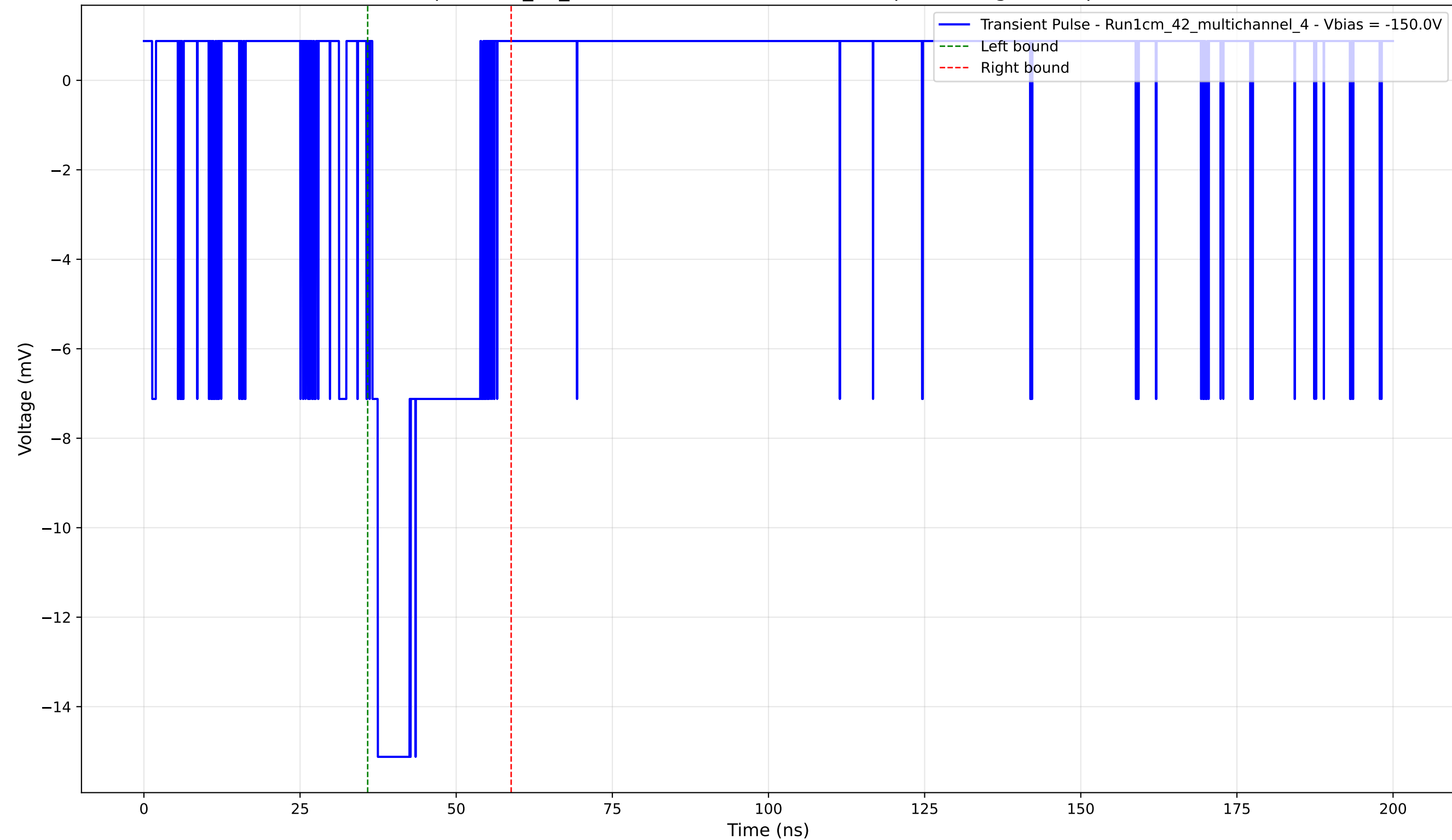
Transient Pulse - Sample: 1cm_42_multichannel - Position: 3700.0 \mu\text{m} - Charge: 3.35 pC - Rise Time: 0.88 ns
