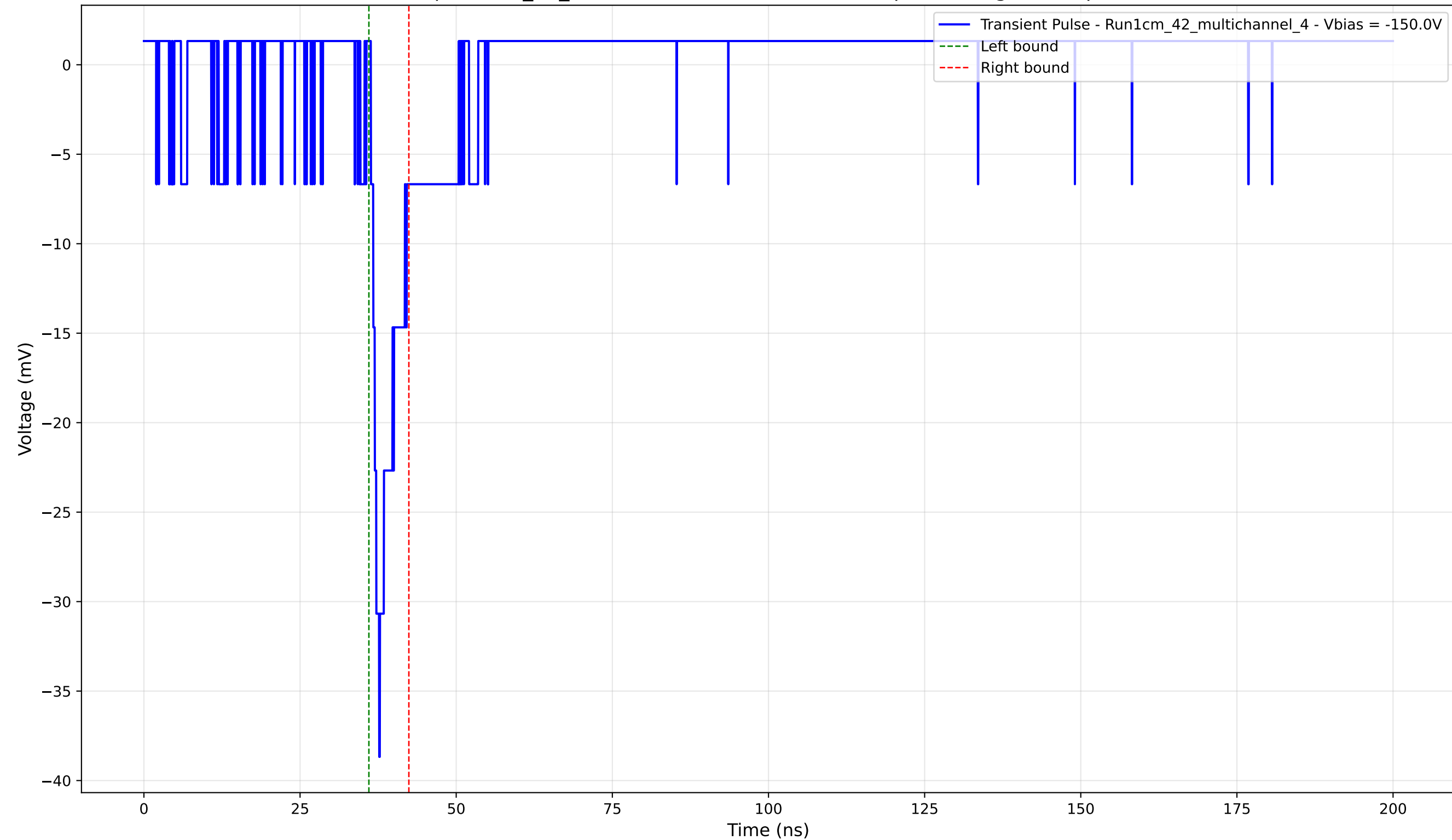
Transient Pulse - Sample: 1cm_42_multichannel - Position: 3055.0 \mu\text{m} - Charge: 2.33 pC - Rise Time: 1.33 ns
