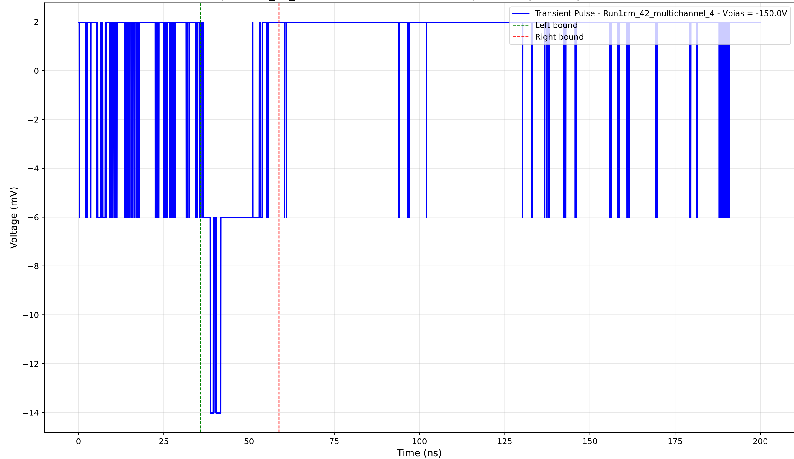
Transient Pulse - Sample: 1cm_42_multichannel - Position: 4820.0 \mu\text{m} - Charge: 2.31 pC - Rise Time: 0.00 ns (N/A)
