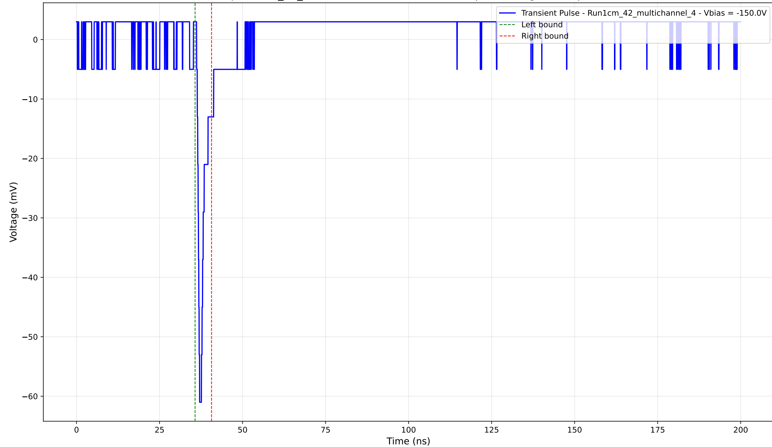
Transient Pulse - Sample: 1cm_42_multichannel - Position: 2600.0 \mu\text{m} - Charge: 2.54 pC - Rise Time: 0.72 ns
