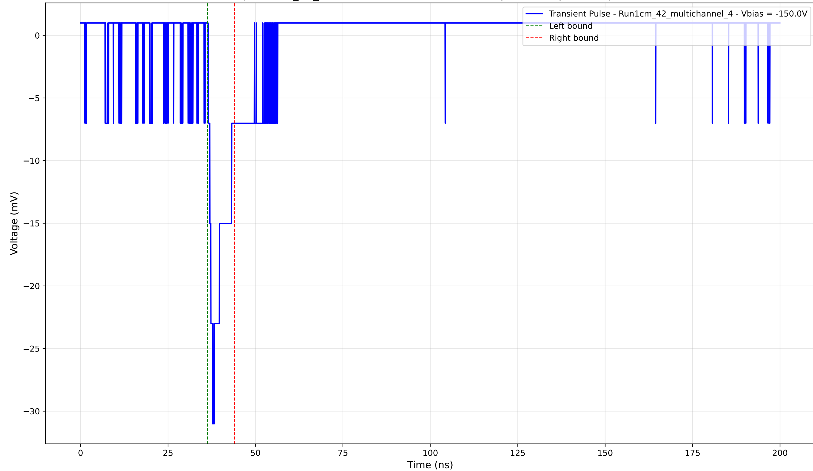
Transient Pulse - Sample: 1cm_42_multichannel - Position: 3250.0 \mu\text{m} - Charge: 2.51 pC - Rise Time: 1.23 ns
