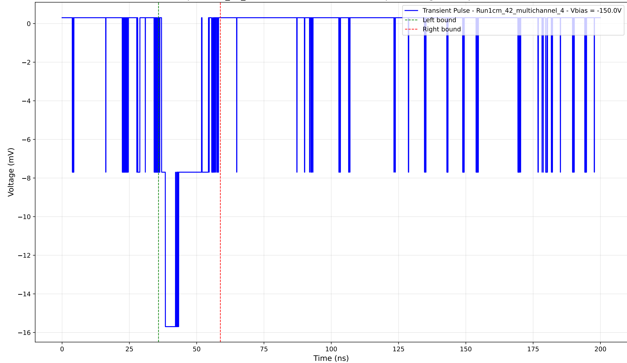
Transient Pulse - Sample: 1cm_42_multichannel - Position: 4755.0 \mu\text{m} - Charge: 3.59 pC - Rise Time: 1.42 ns
