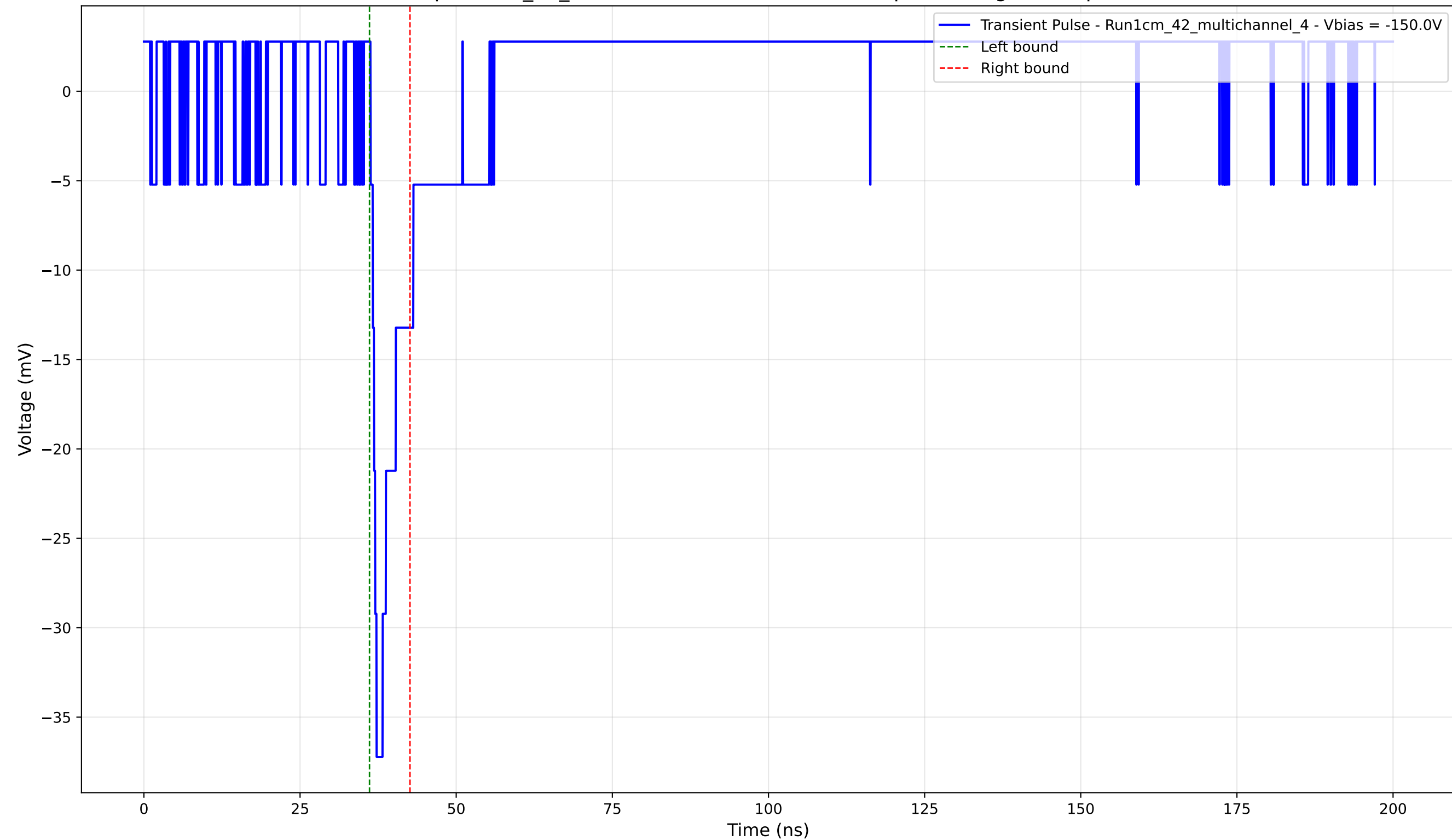
Transient Pulse - Sample: 1cm_42_multichannel - Position: 1755.0 \mu\text{m} - Charge: 2.60 pC - Rise Time: 0.97 ns
