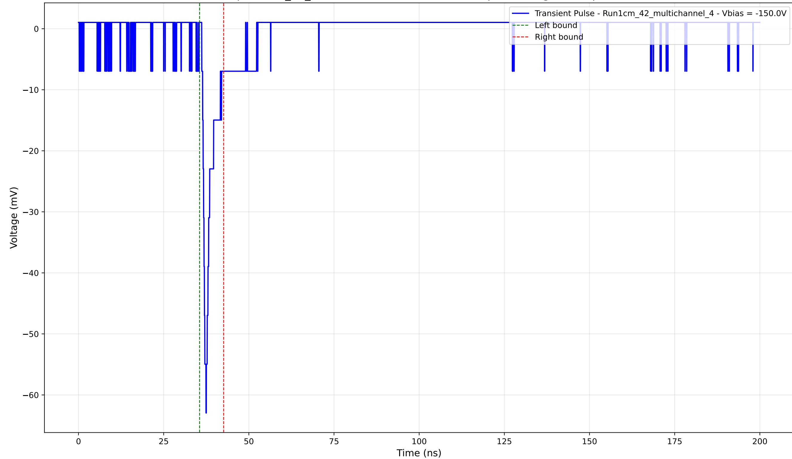
Transient Pulse - Sample: 1cm_42_multichannel - Position: 2690.0 \mu\text{m} - Charge: 3.04 pC - Rise Time: 1.24 ns
