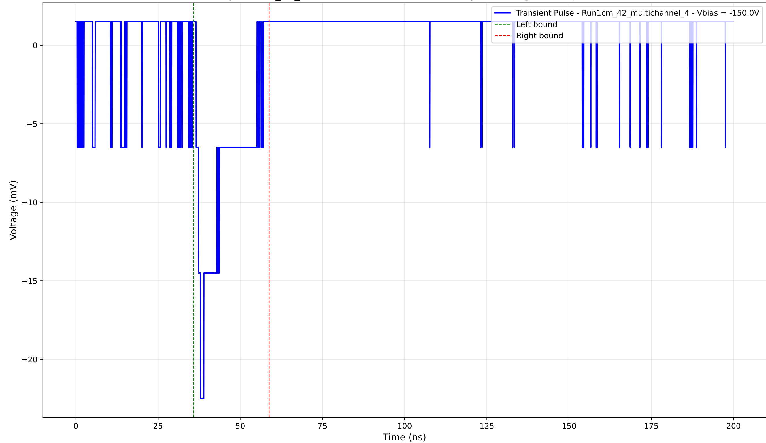
Transient Pulse - Sample: 1cm_42_multichannel - Position: 3540.0 \mu\text{m} - Charge: 3.58 pC - Rise Time: 1.38 ns
