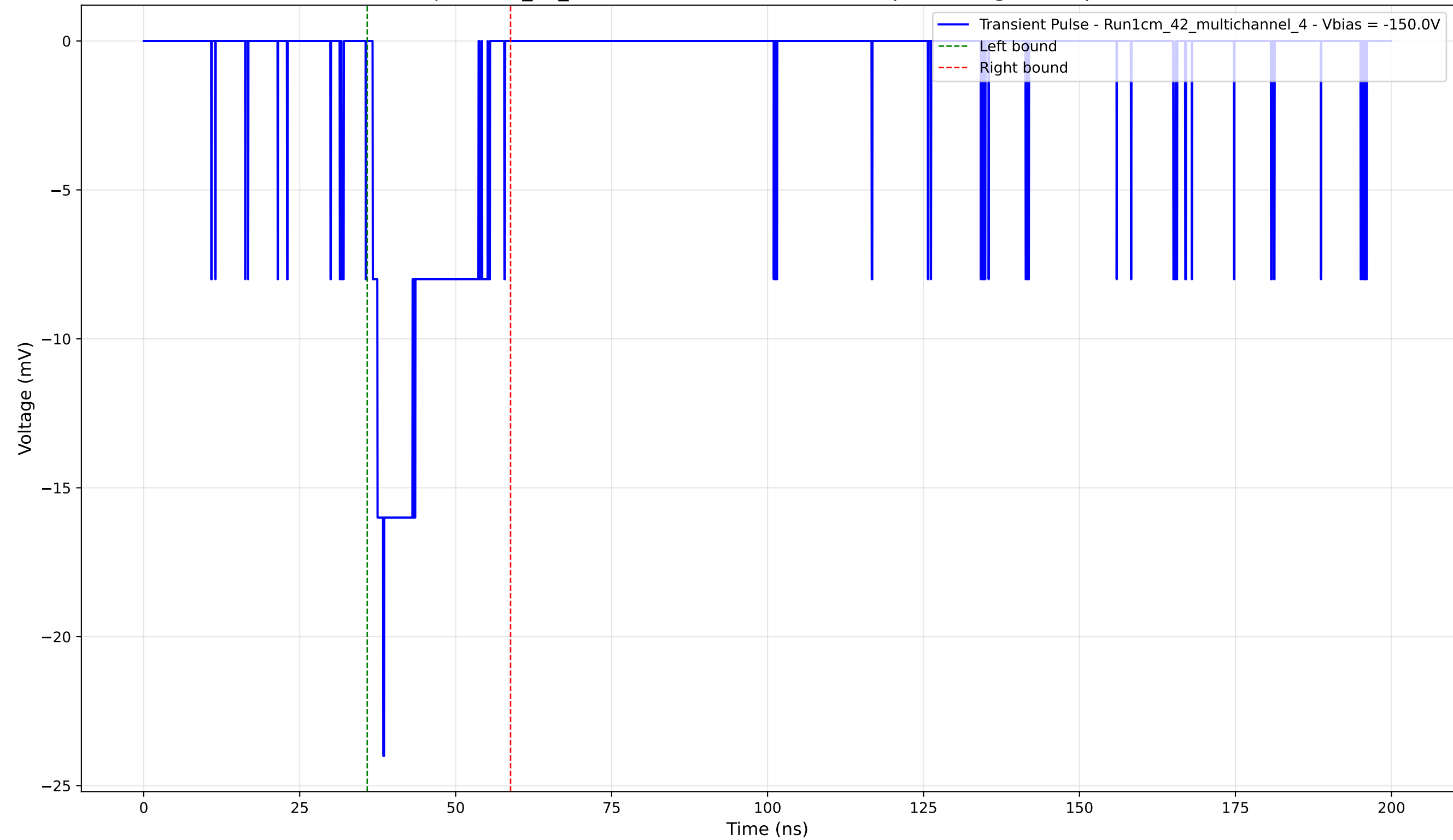
Transient Pulse - Sample: 1cm_42_multichannel - Position: 3660.0 \mu\text{m} - Charge: 3.96 pC - Rise Time: 1.69 ns
