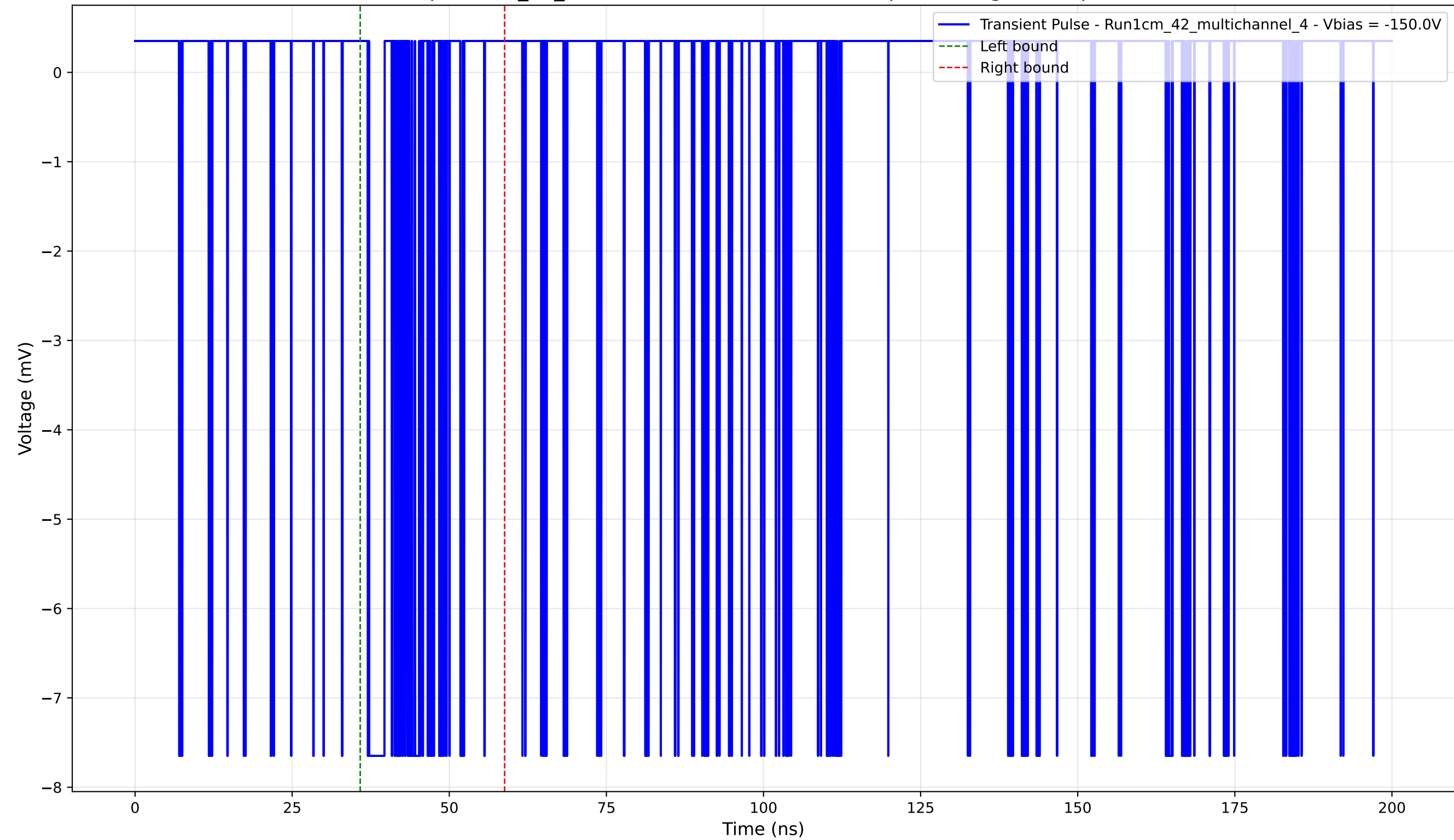
Transient Pulse - Sample: 1cm_42_multichannel - Position: 3375.0 \mu\text{m} - Charge: 1.01 pC - Rise Time: 0.02 ns
