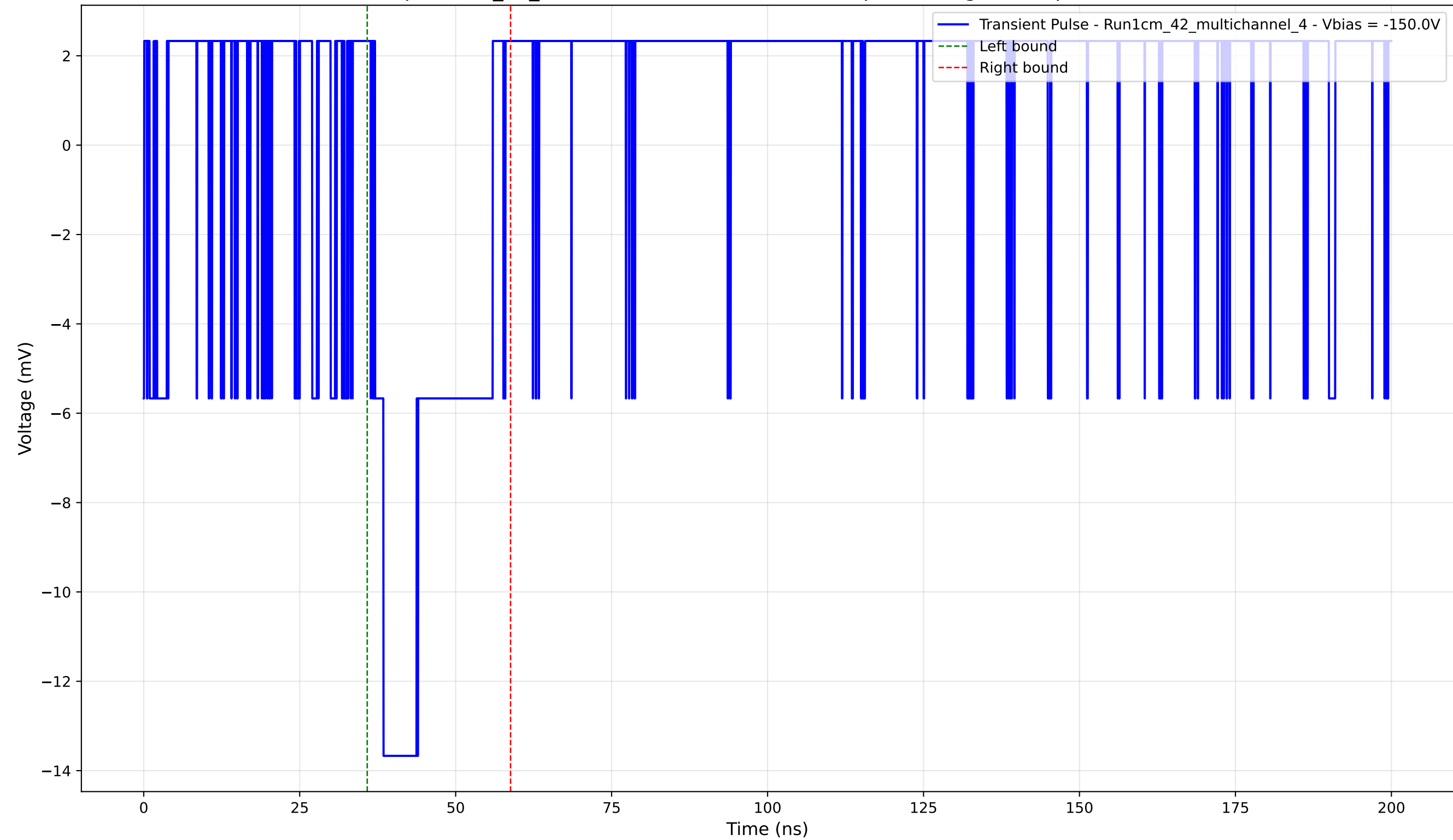
Transient Pulse - Sample: 1cm_42_multichannel - Position: 4495.0 \mu\text{m} - Charge: 2.87 pC - Rise Time: 0.00 ns (N/A)
