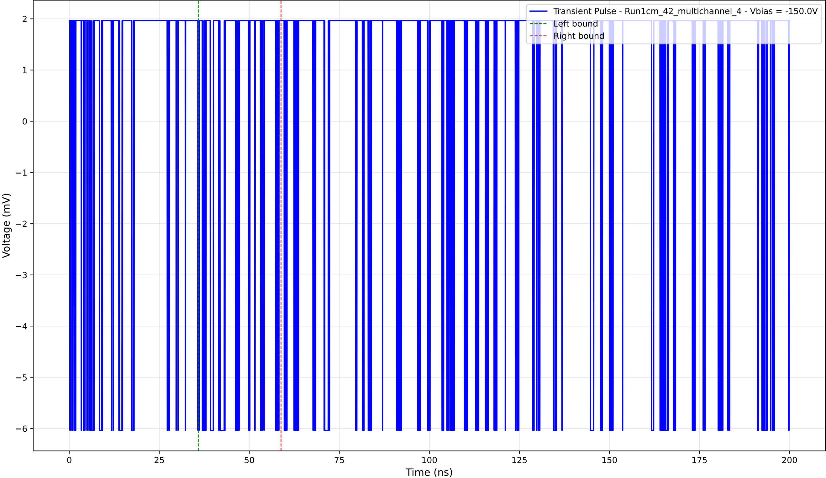
Transient Pulse - Sample: 1cm_42_multichannel - Position: 4410.0 \mu\text{m} - Charge: 0.15 pC - Rise Time: 0.00 ns (N/A)
