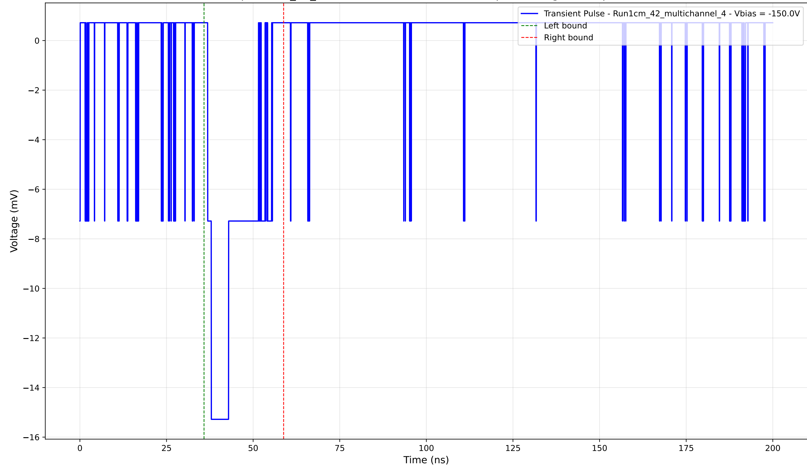
Transient Pulse - Sample: 1cm_42_multichannel - Position: 4050.0 \mu\text{m} - Charge: 3.28 pC - Rise Time: 1.06 ns
