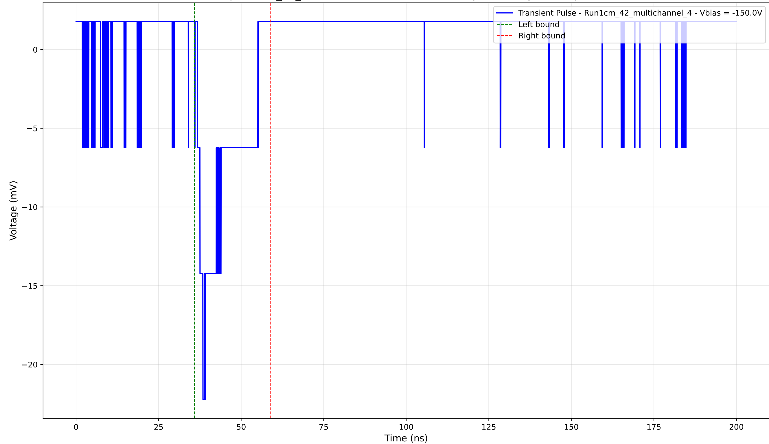
Transient Pulse - Sample: 1cm_42_multichannel - Position: 3715.0 \mu\text{m} - Charge: 3.22 pC - Rise Time: 1.64 ns
