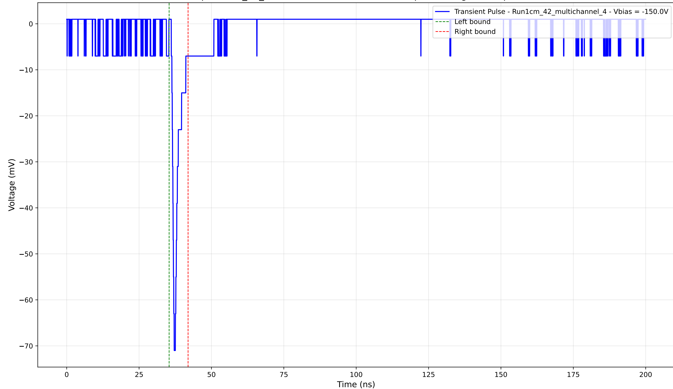
Transient Pulse - Sample: 1cm_42_multichannel - Position: 2190.0 \mu\text{m} - Charge: 3.19 pC - Rise Time: 0.80 ns
