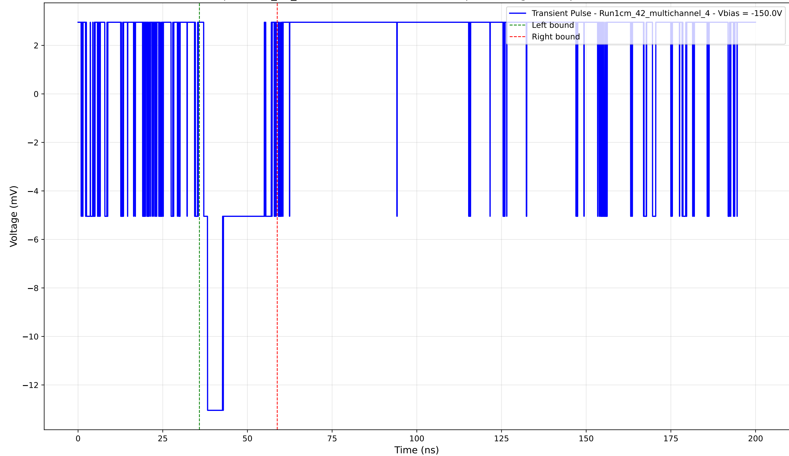
Transient Pulse - Sample: 1cm_42_multichannel - Position: 435.0 \mu\text{m} - Charge: 2.58 pC - Rise Time: 0.00 ns (N/A)
