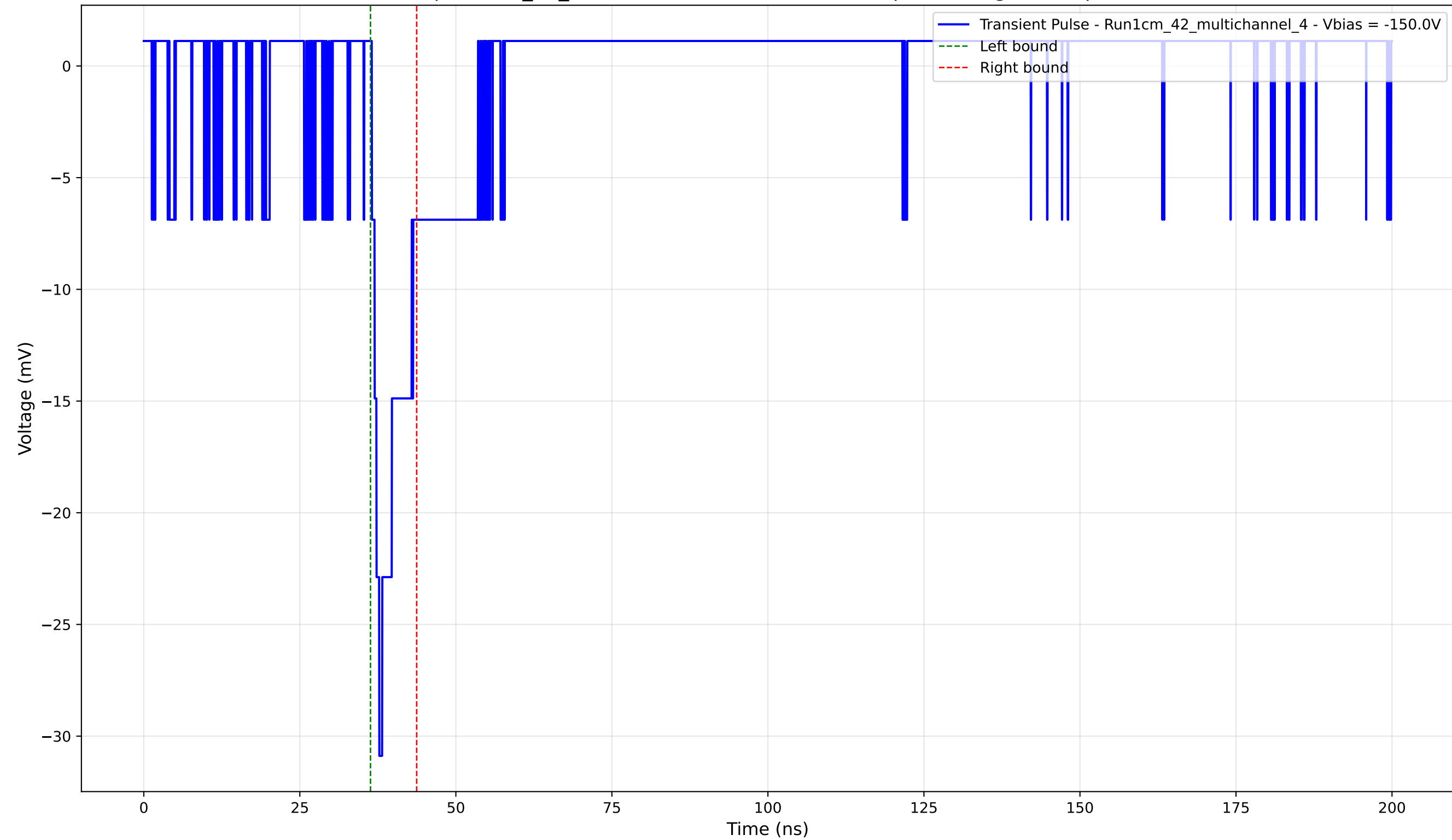
Transient Pulse - Sample: 1cm_42_multichannel - Position: 3255.0 \mu\text{m} - Charge: 2.43 pC - Rise Time: 1.19 ns
