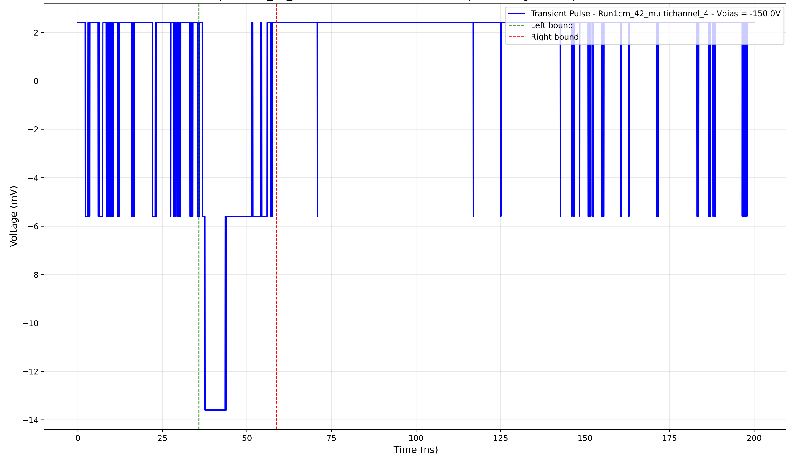
Transient Pulse - Sample: 1cm_42_multichannel - Position: 3770.0 \mu\text{m} - Charge: 2.95 pC - Rise Time: 0.00 ns (N/A)
