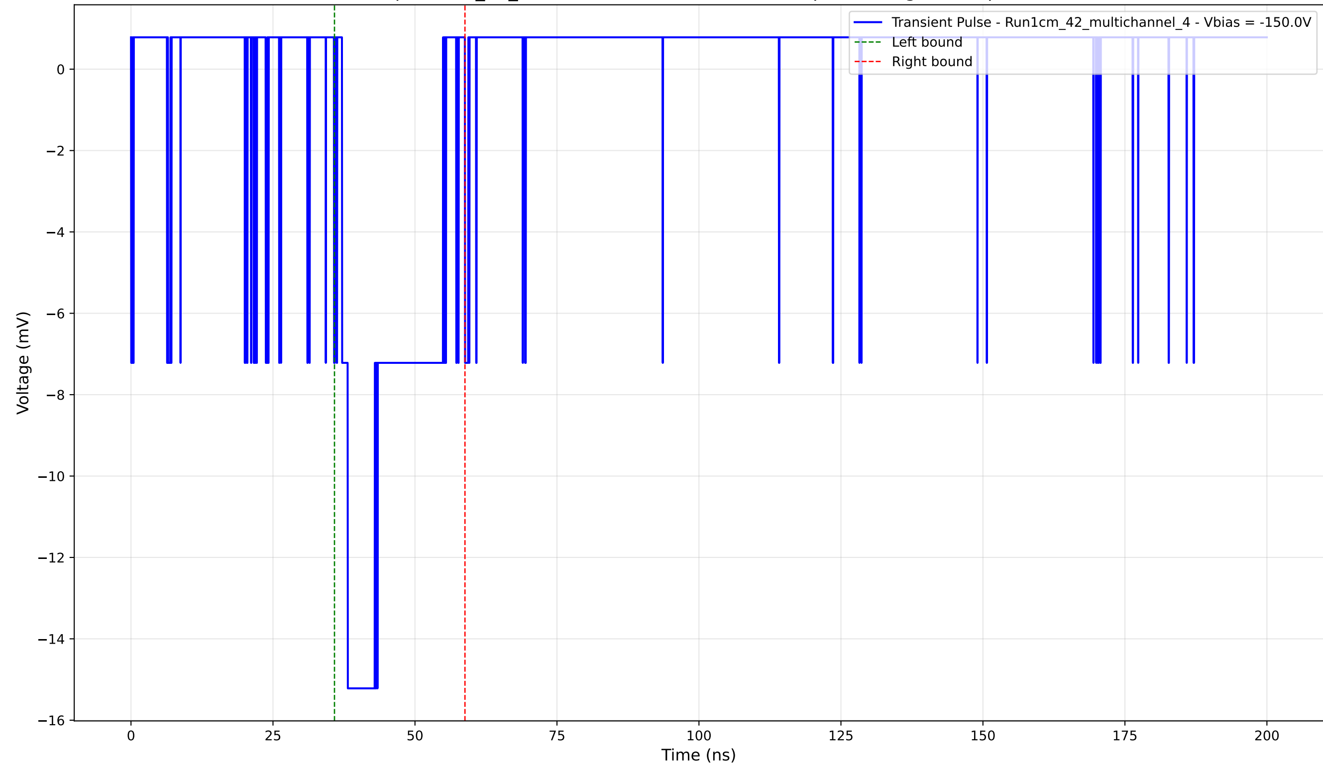
Transient Pulse - Sample: 1cm_42_multichannel - Position: 4130.0 \mu\text{m} - Charge: 3.37 pC - Rise Time: 1.02 ns
