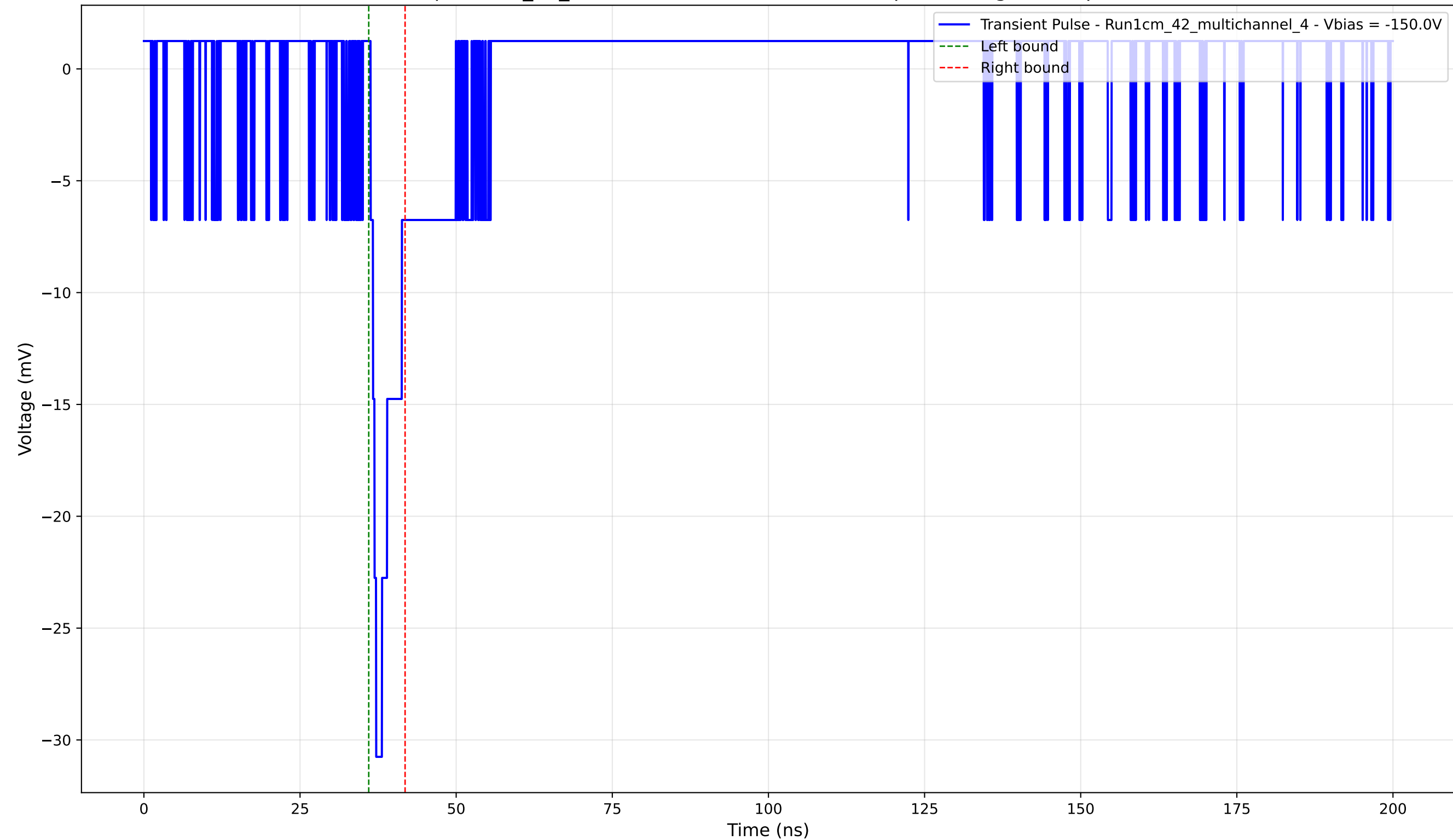
Transient Pulse - Sample: 1cm_42_multichannel - Position: 1820.0 \mu\text{m} - Charge: 1.95 pC - Rise Time: 0.89 ns
