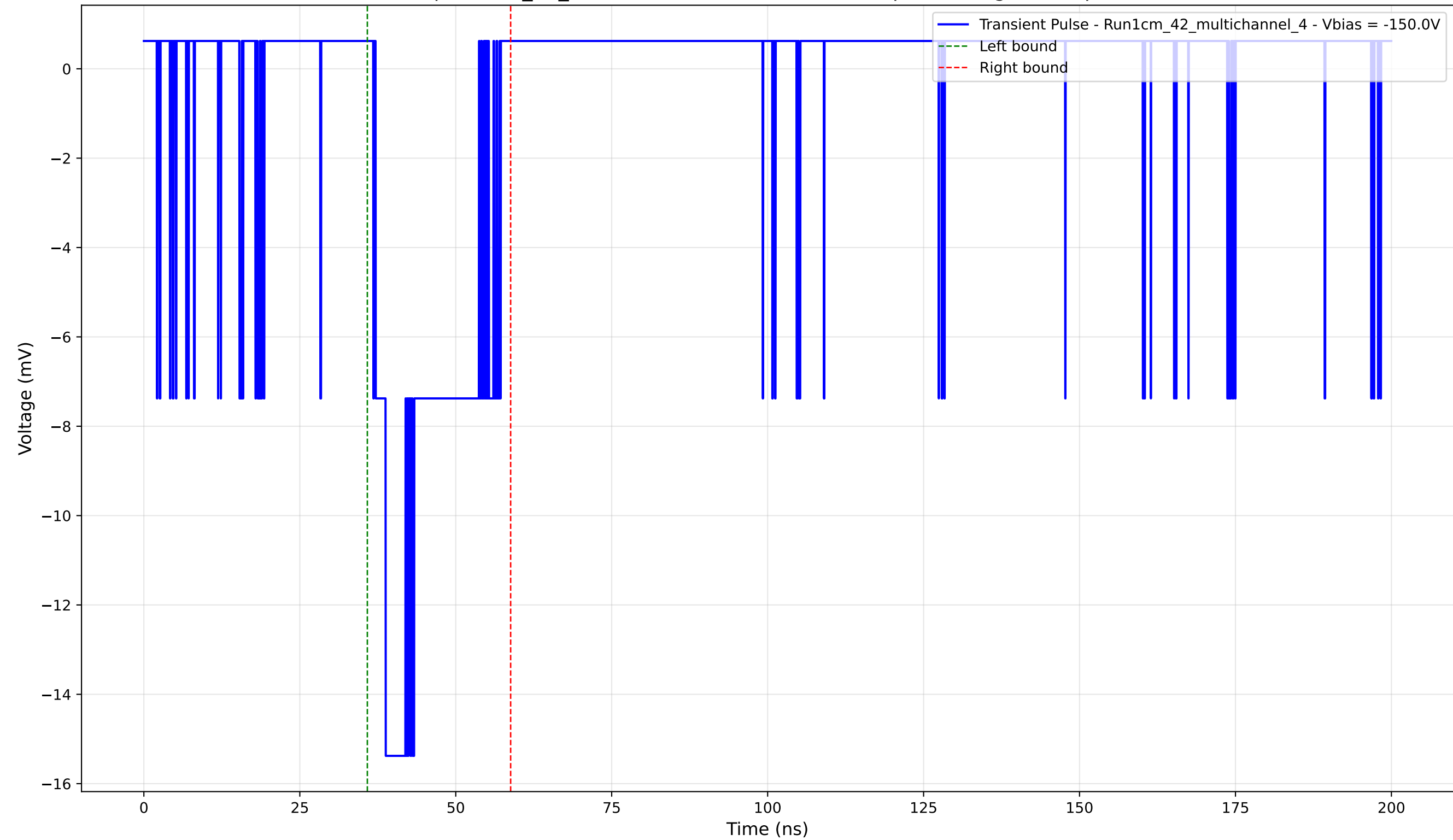
Transient Pulse - Sample: 1cm_42_multichannel - Position: 4645.0 \mu\text{m} - Charge: 3.39 pC - Rise Time: 1.62 ns
