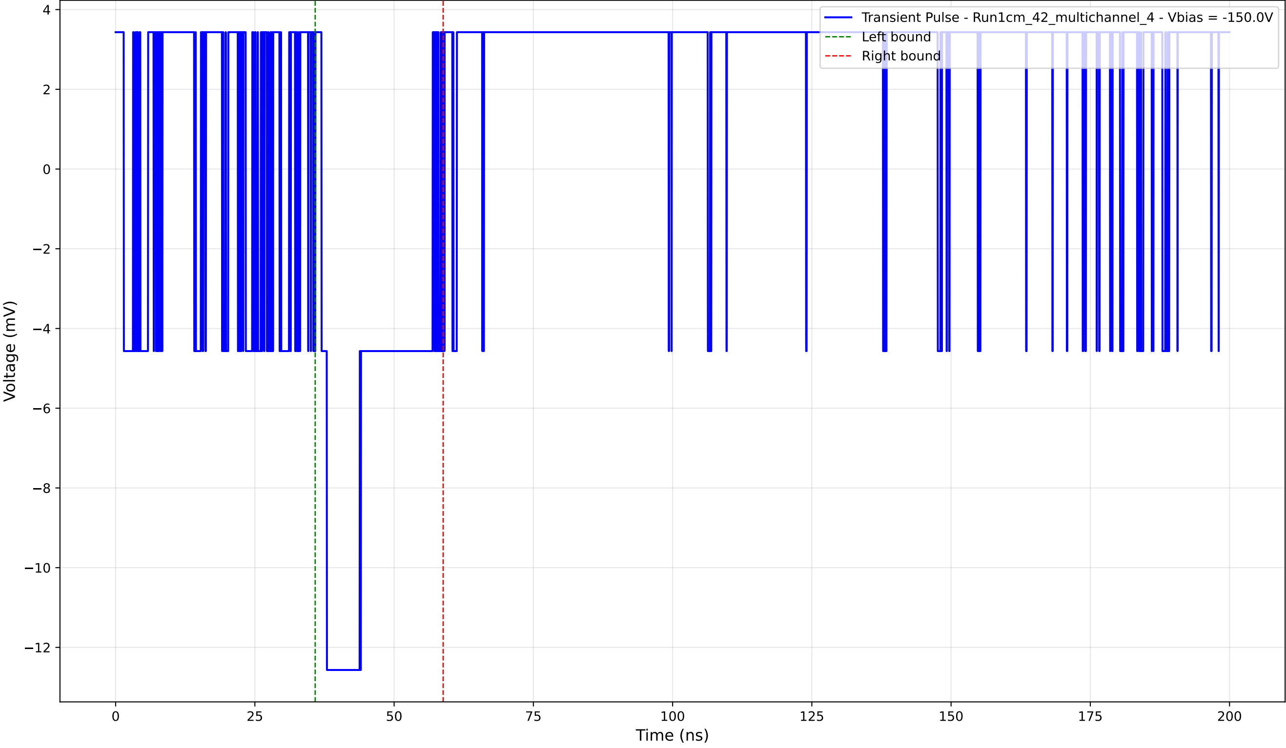
Transient Pulse - Sample: 1cm_42_multichannel - Position: 635.0 \mu\text{m} - Charge: 2.74 pC - Rise Time: 0.00 ns (N/A)
