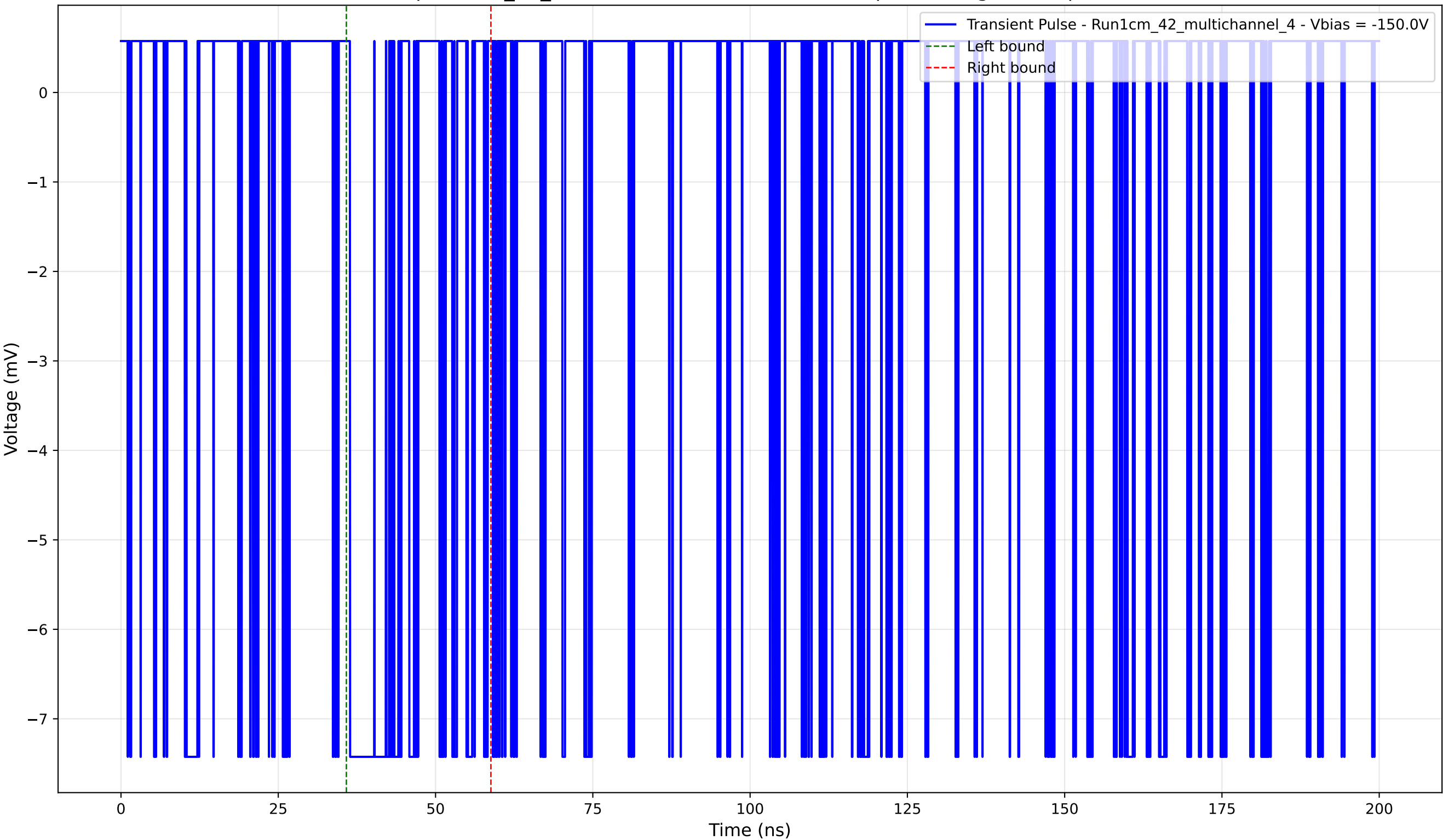
Transient Pulse - Sample: 1cm_42_multichannel - Position: 2865.0 \mu\text{m} - Charge: 1.55 pC - Rise Time: 0.02 ns
