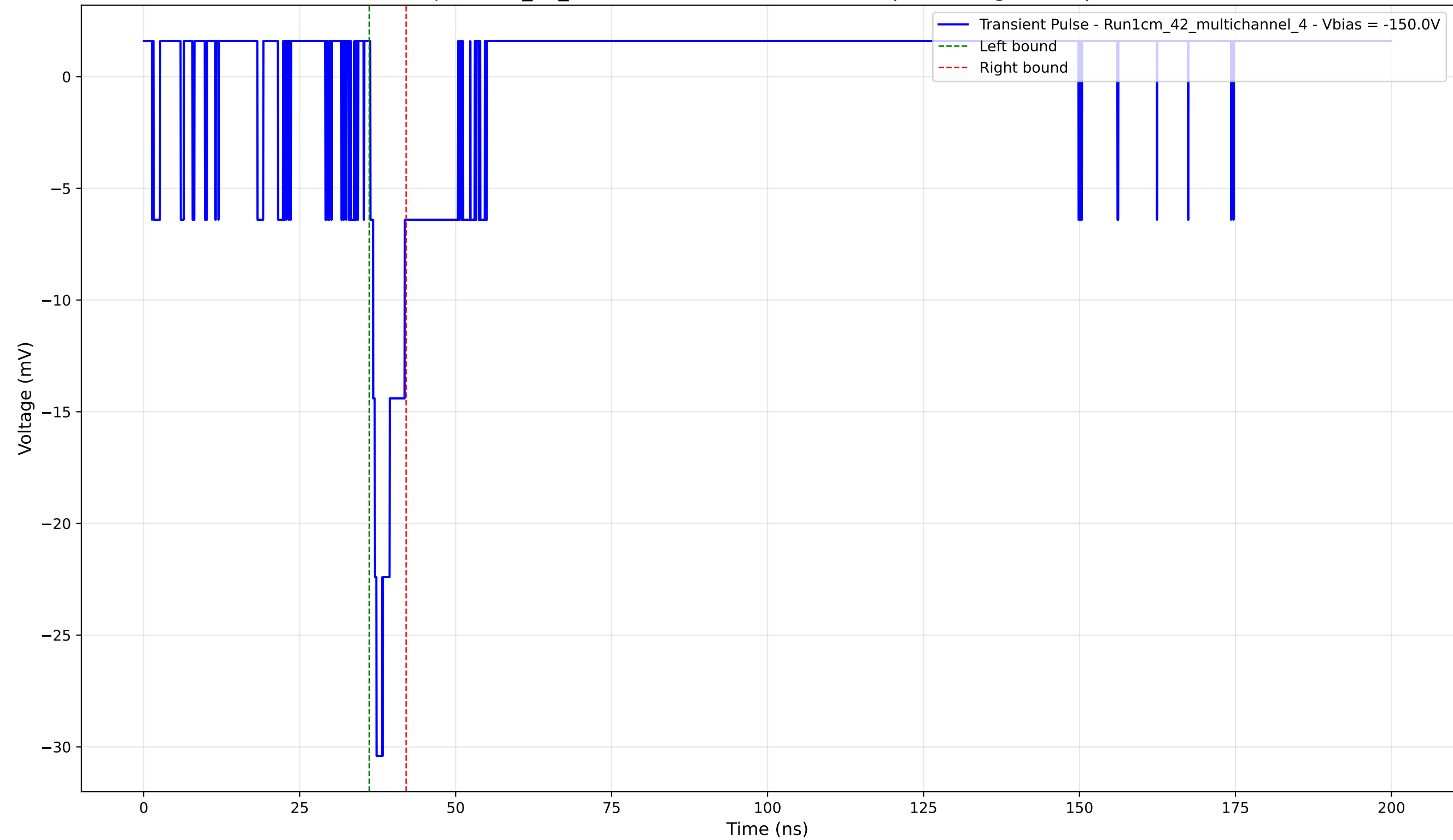
Transient Pulse - Sample: 1cm_42_multichannel - Position: 3080.0 \mu\text{m} - Charge: 2.08 pC - Rise Time: 0.99 ns
