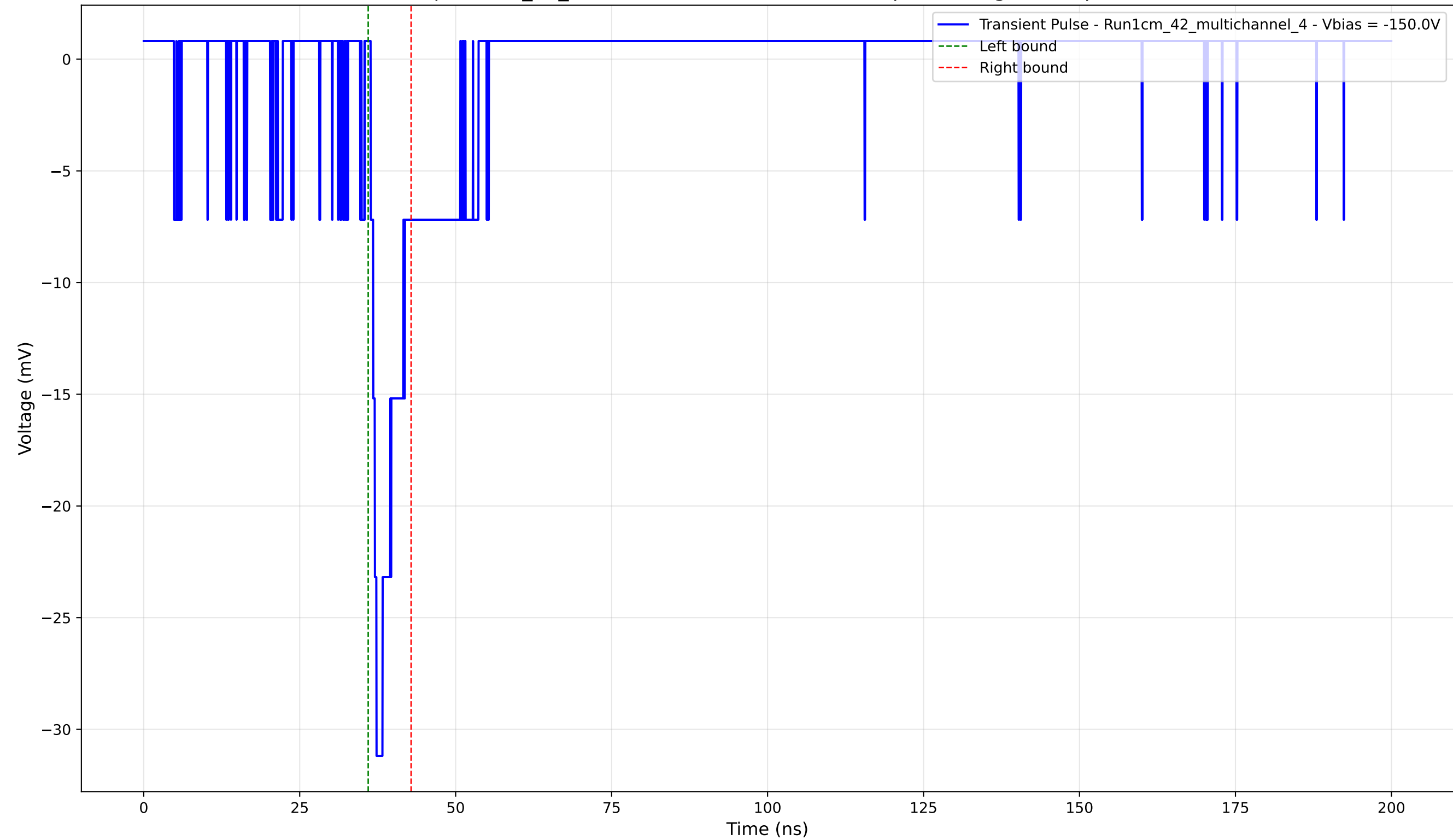
Transient Pulse - Sample: 1cm_42_multichannel - Position: 3100.0 \mu\text{m} - Charge: 2.28 pC - Rise Time: 0.93 ns
