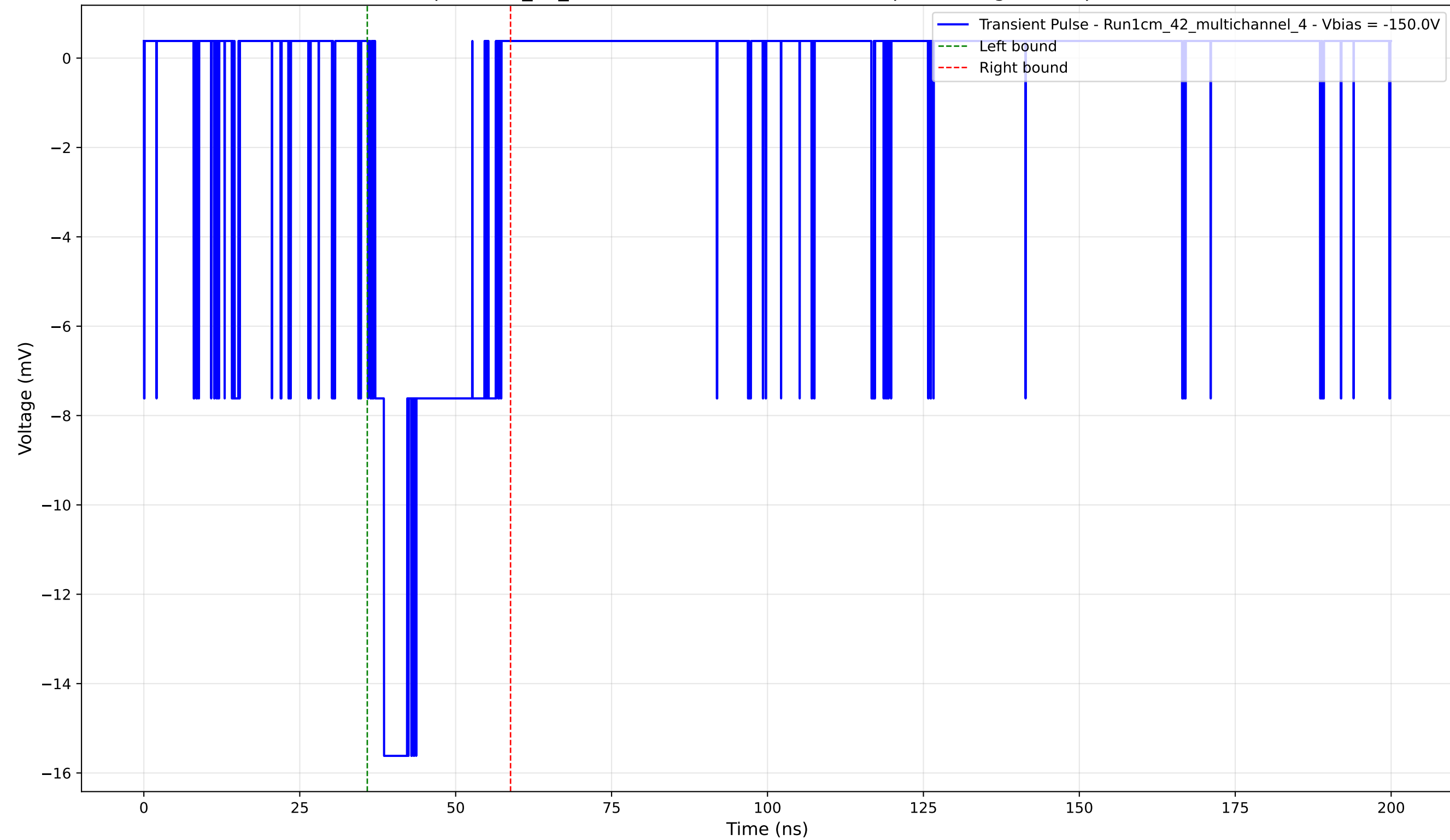
Transient Pulse - Sample: 1cm_42_multichannel - Position: 4590.0 \mu\text{m} - Charge: 3.60 pC - Rise Time: 1.42 ns
