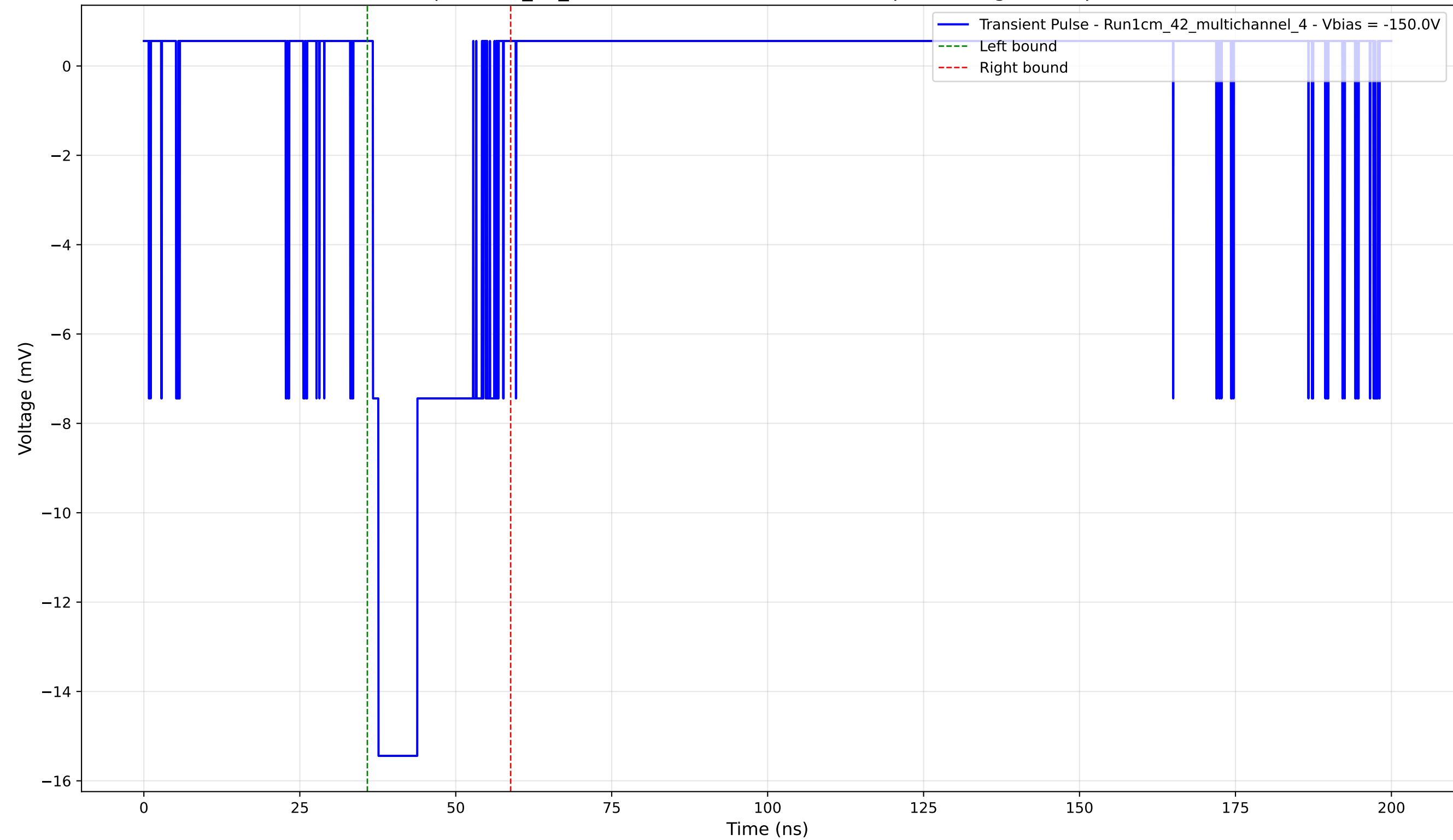
Transient Pulse - Sample: 1cm_42_multichannel - Position: 3775.0 \mu\text{m} - Charge: 3.81 pC - Rise Time: 0.90 ns
