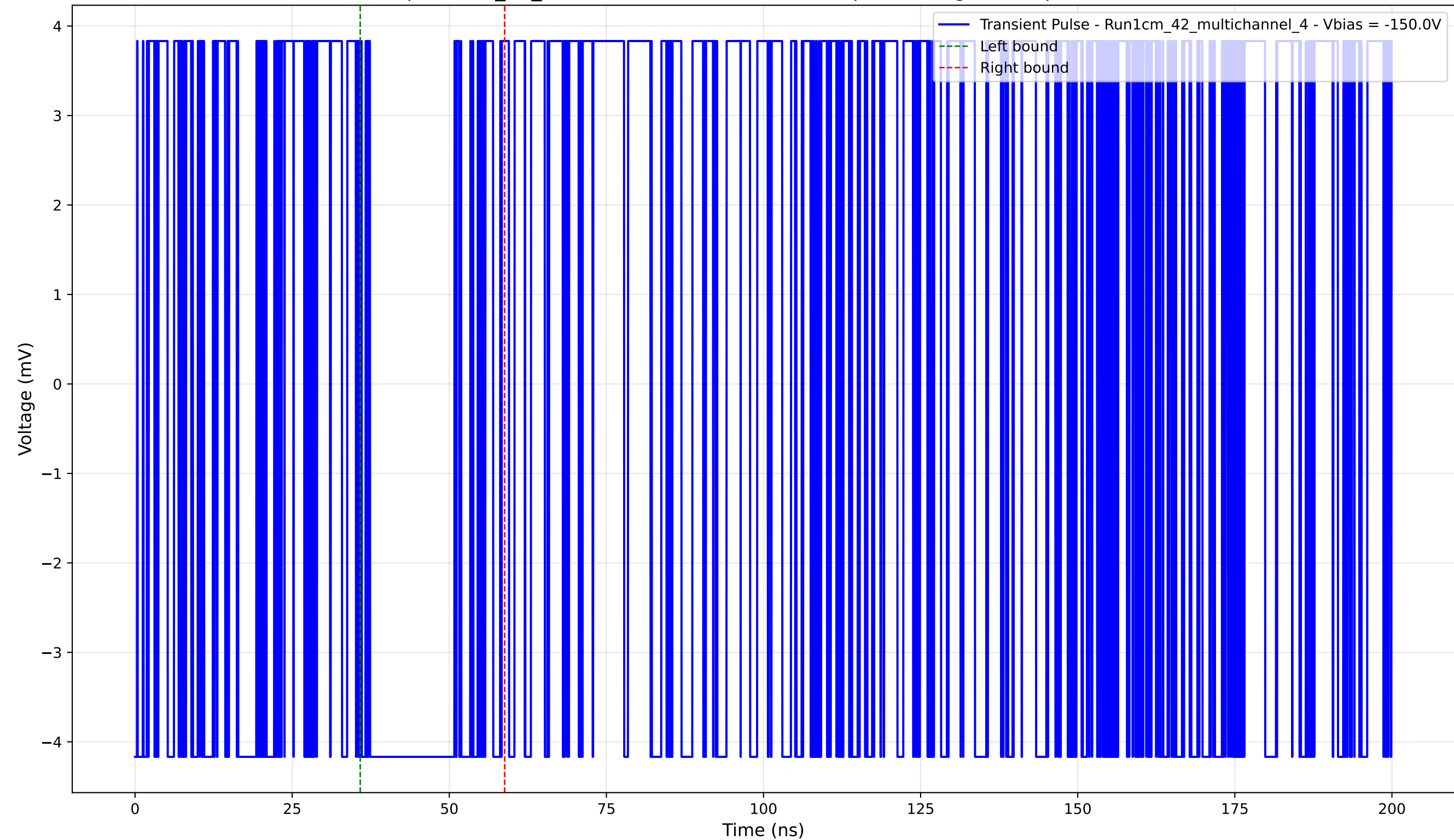
Transient Pulse - Sample: 1cm_42_multichannel - Position: 830.0 \mu\text{m} - Charge: 1.27 pC - Rise Time: 0.00 ns (N/A)
