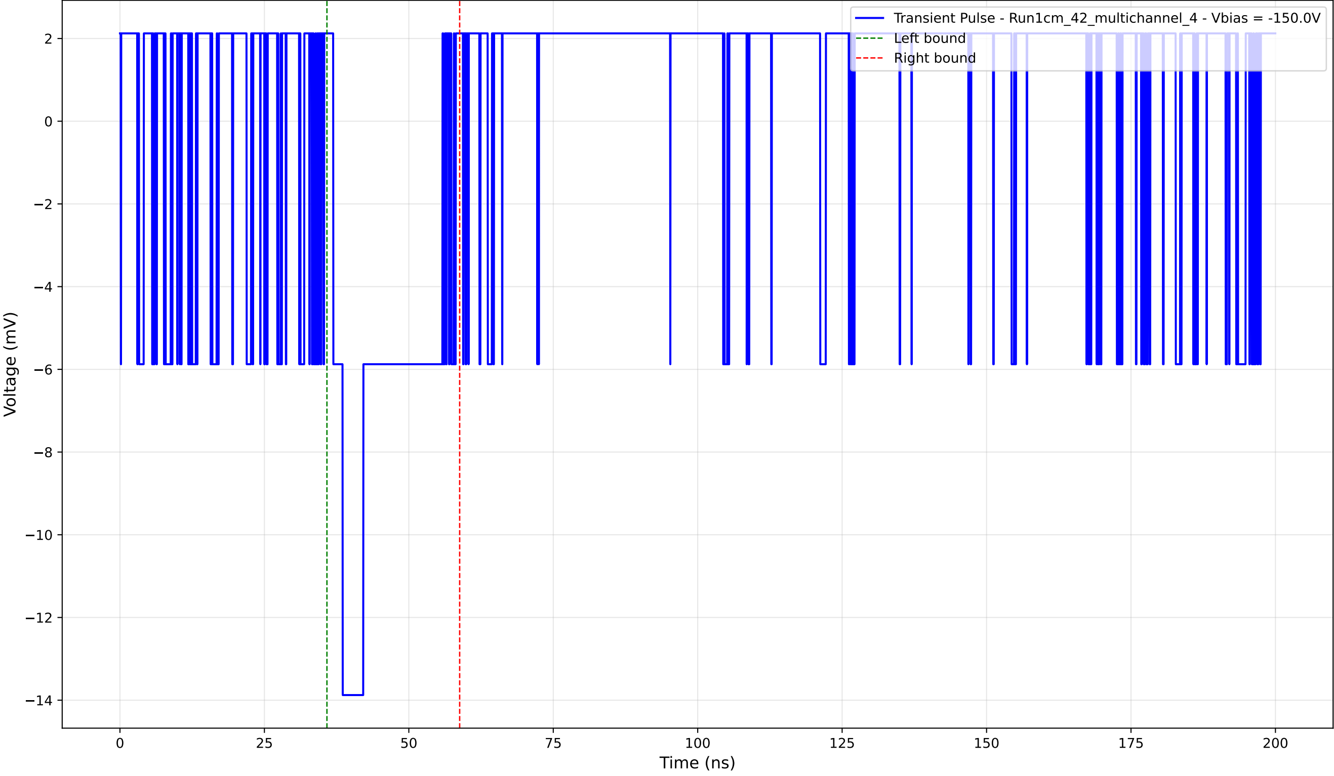
Transient Pulse - Sample: 1cm_42_multichannel - Position: 205.0 \mu\text{m} - Charge: 2.81 pC - Rise Time: 0.00 ns (N/A)
