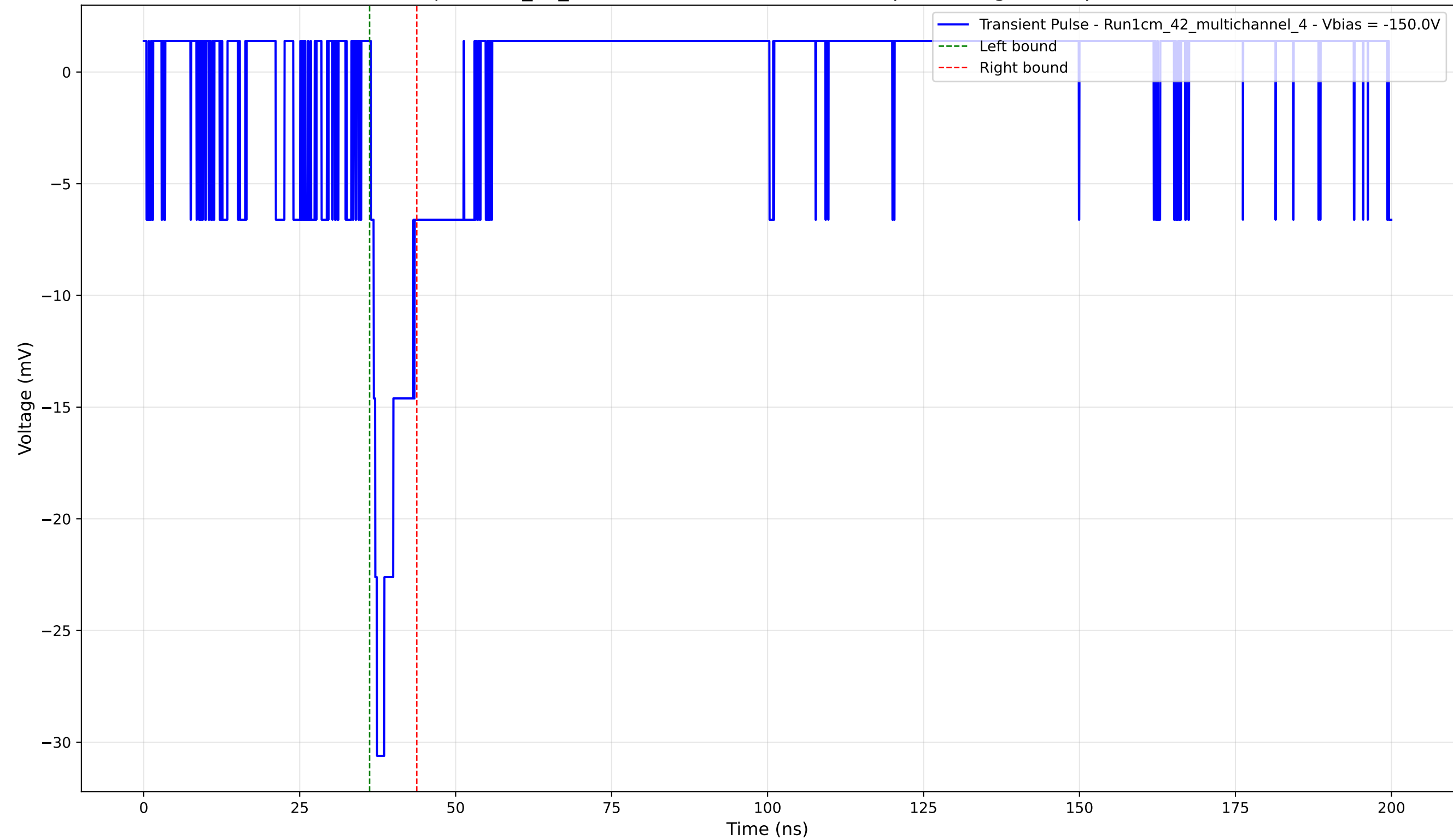
Transient Pulse - Sample: 1cm_42_multichannel - Position: 1595.0 \mu\text{m} - Charge: 2.66 pC - Rise Time: 0.97 ns
