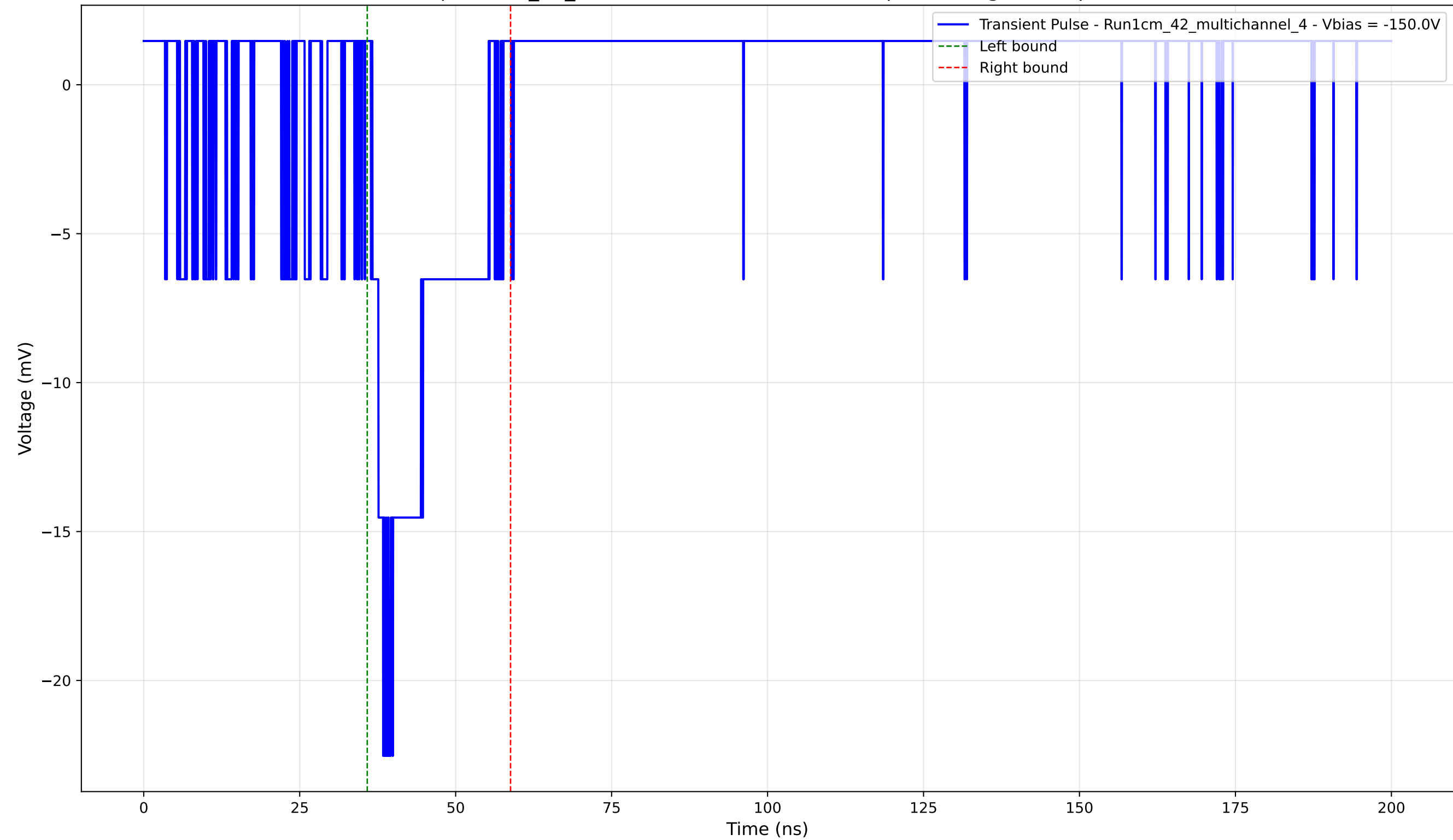
Transient Pulse - Sample: 1cm_42_multichannel - Position: 970.0 \mu\text{m} - Charge: 3.73 pC - Rise Time: 1.74 ns
