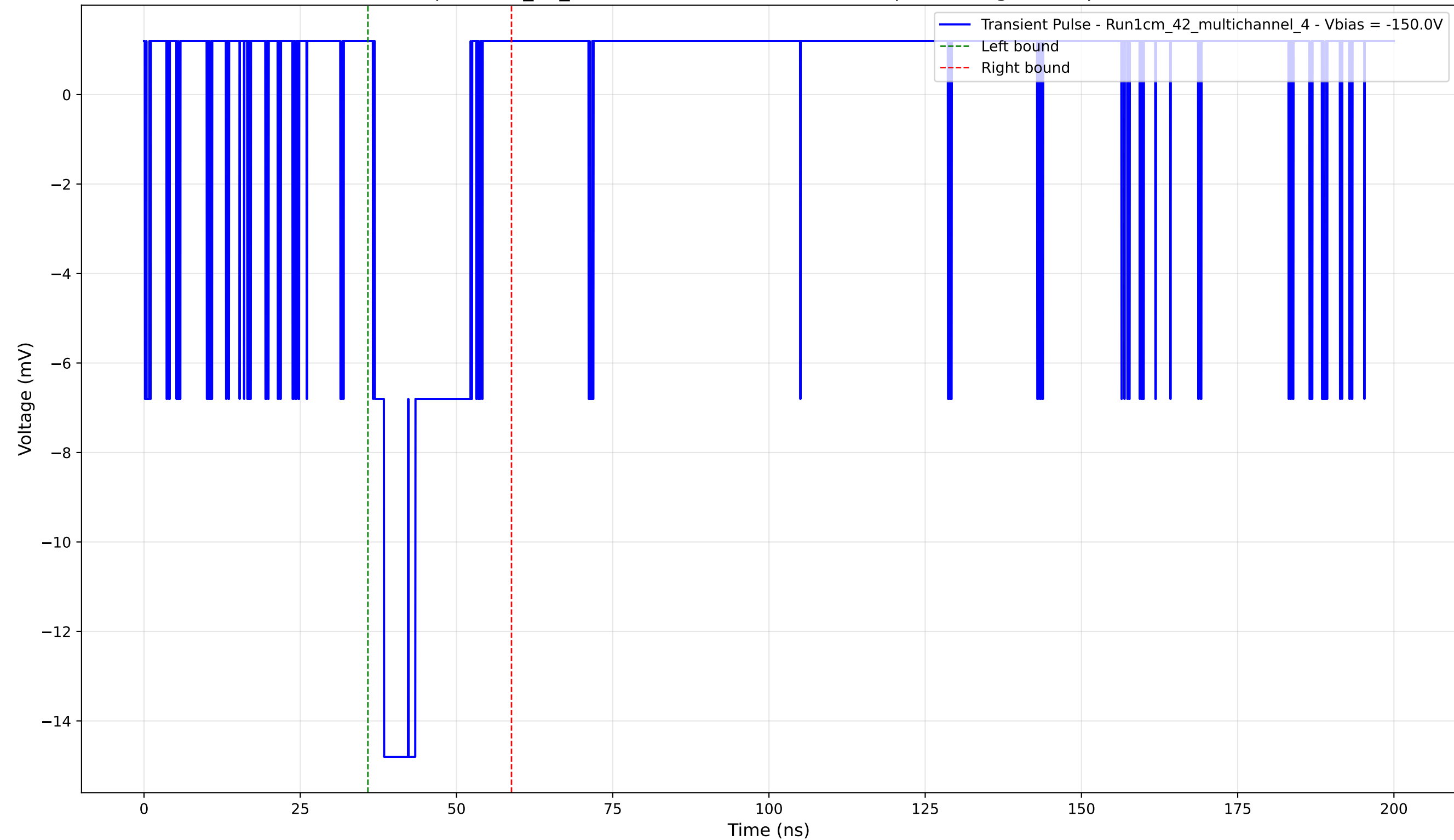
Transient Pulse - Sample: 1cm_42_multichannel - Position: 4225.0 \mu\text{m} - Charge: 2.81 pC - Rise Time: 1.50 ns
