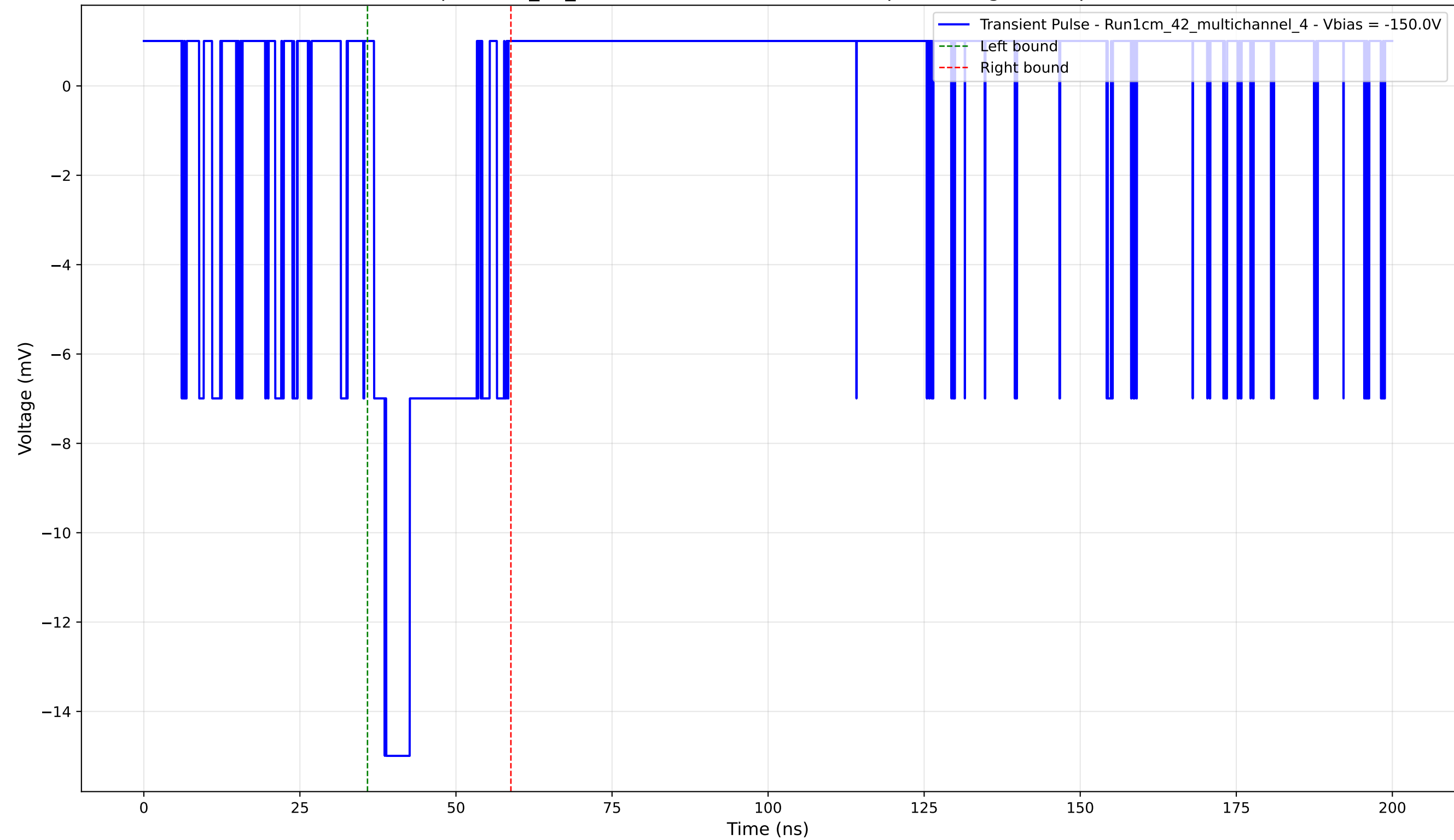
Transient Pulse - Sample: 1cm_42_multichannel - Position: 215.0 \mu\text{m} - Charge: 3.26 pC - Rise Time: 1.74 ns
