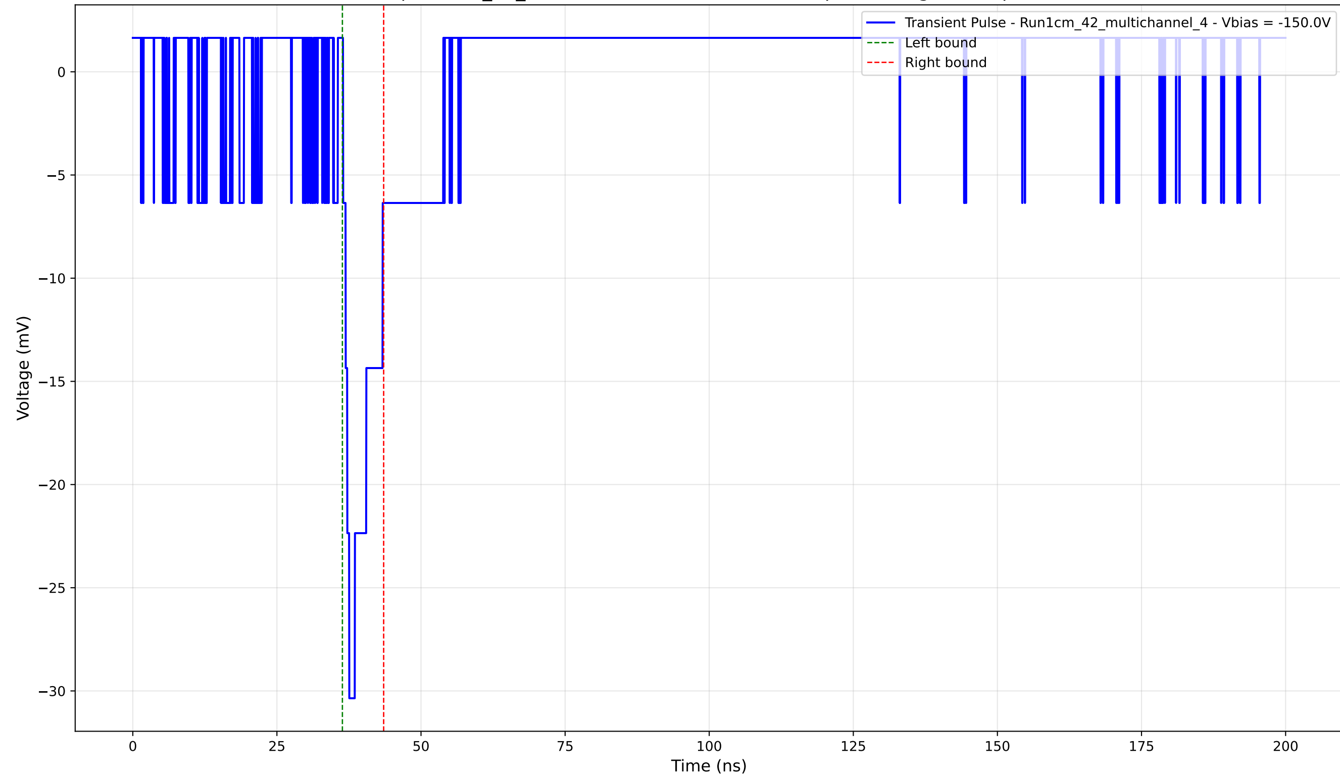
Transient Pulse - Sample: 1cm_42_multichannel - Position: 1490.0 \mu\text{m} - Charge: 2.60 pC - Rise Time: 1.07 ns
