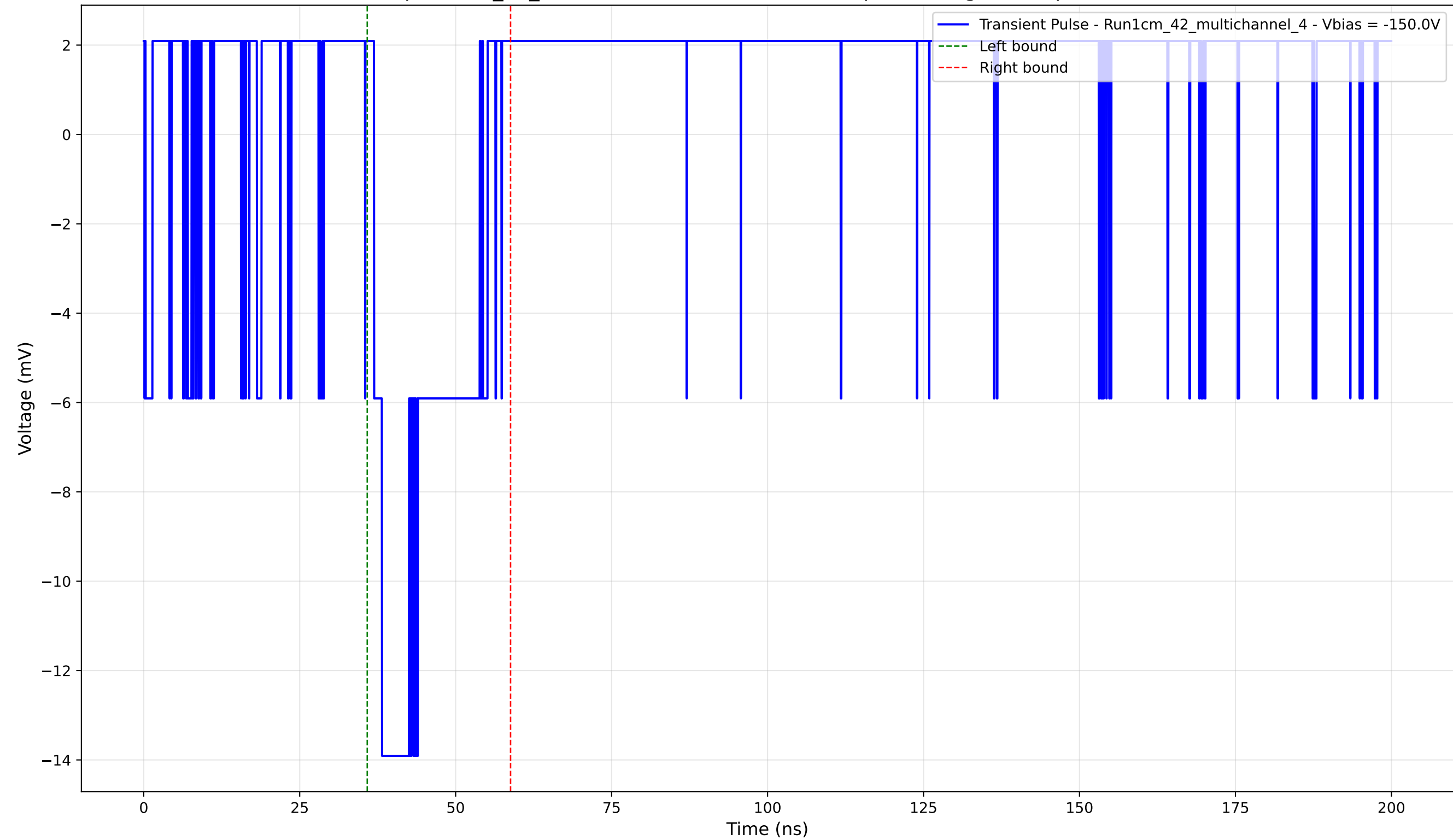
Transient Pulse - Sample: 1cm_42_multichannel - Position: 4090.0 \mu\text{m} - Charge: 2.73 pC - Rise Time: 0.00 ns (N/A)
