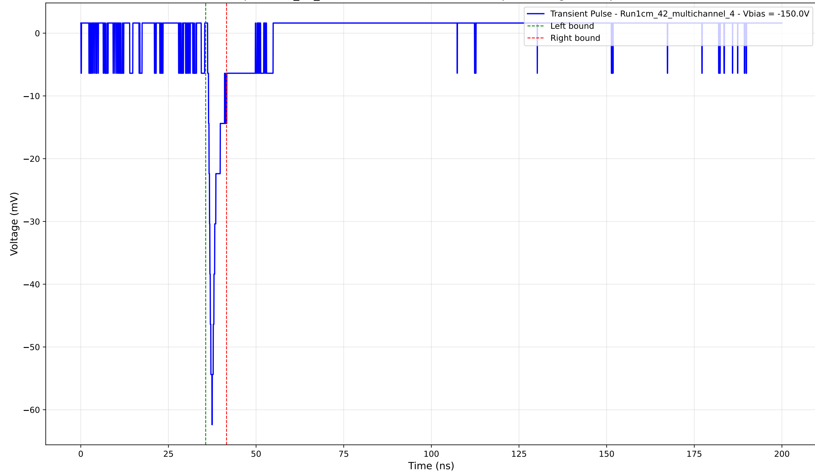
Transient Pulse - Sample: 1cm_42_multichannel - Position: 2075.0 \mu\text{m} - Charge: 2.77 pC - Rise Time: 1.24 ns
