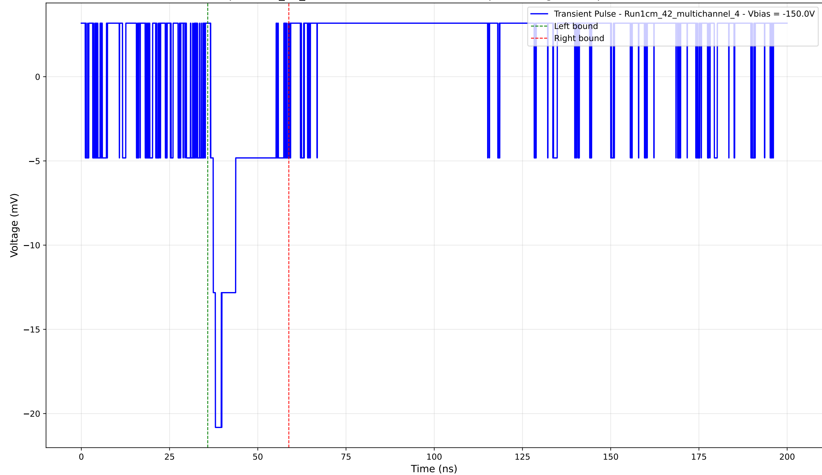
Transient Pulse - Sample: 1cm_42_multichannel - Position: 1075.0 \mu\text{m} - Charge: 3.24 pC - Rise Time: 0.00 ns (N/A)
