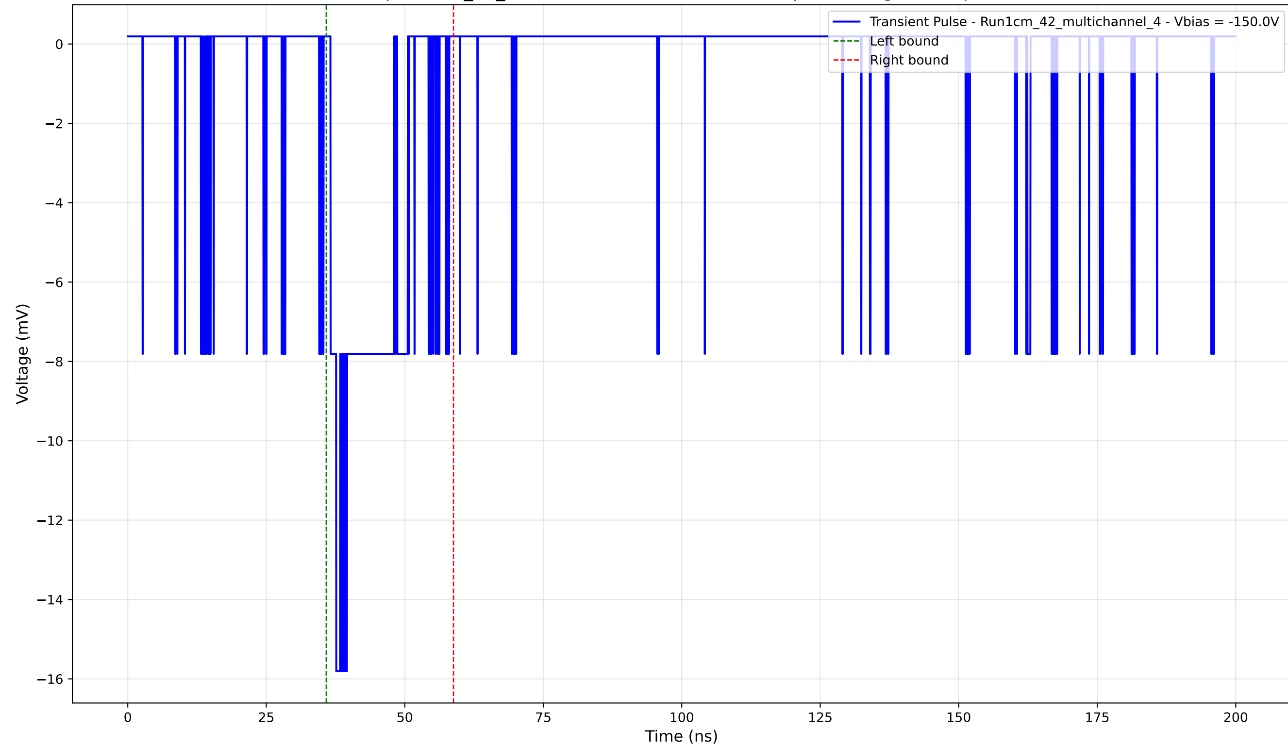
Transient Pulse - Sample: 1cm_42_multichannel - Position: 3350.0 \mu\text{m} - Charge: 2.49 pC - Rise Time: 1.04 ns
