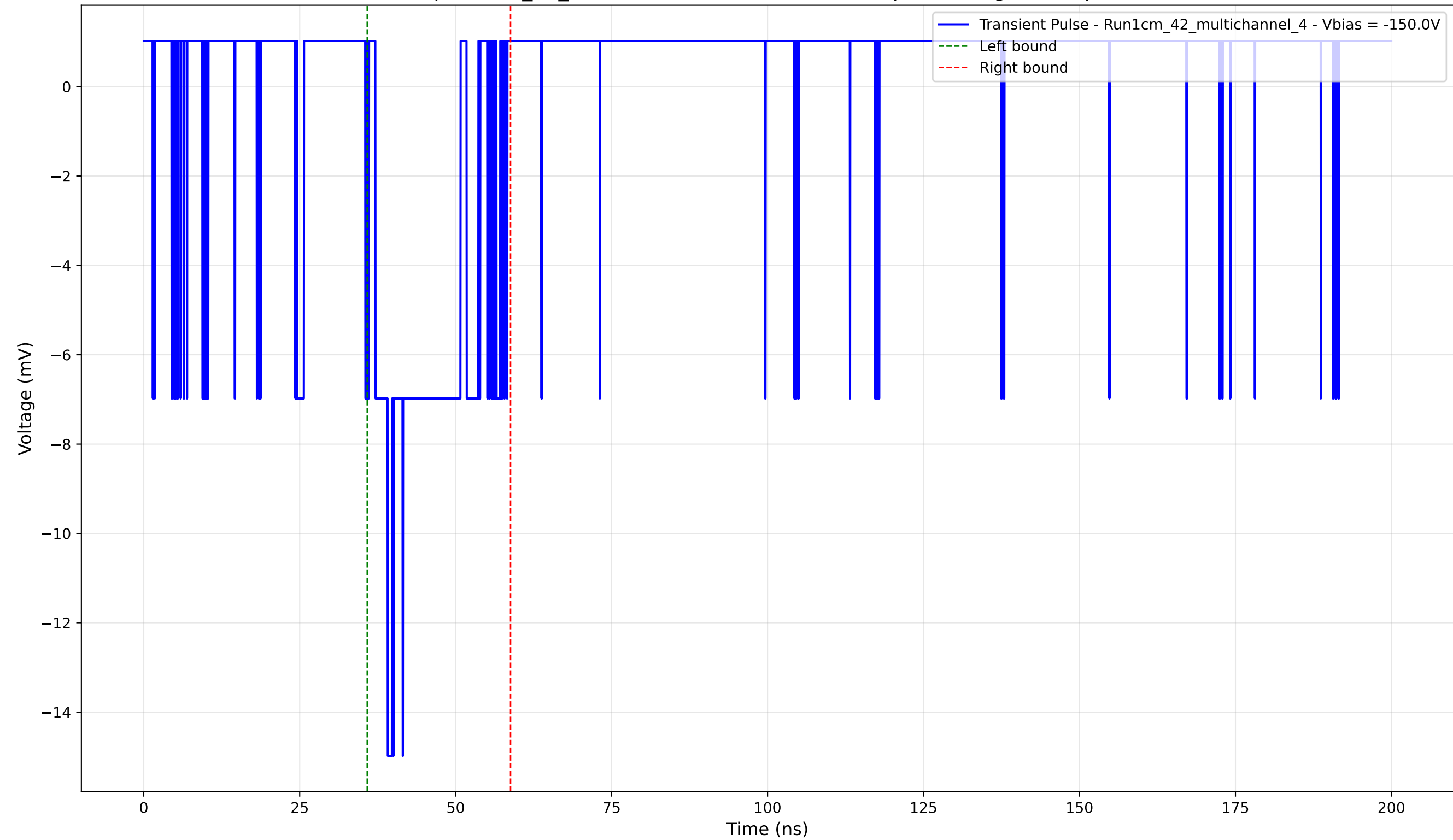
Transient Pulse - Sample: 1cm_42_multichannel - Position: 3960.0 \mu\text{m} - Charge: 2.45 pC - Rise Time: 1.98 ns
