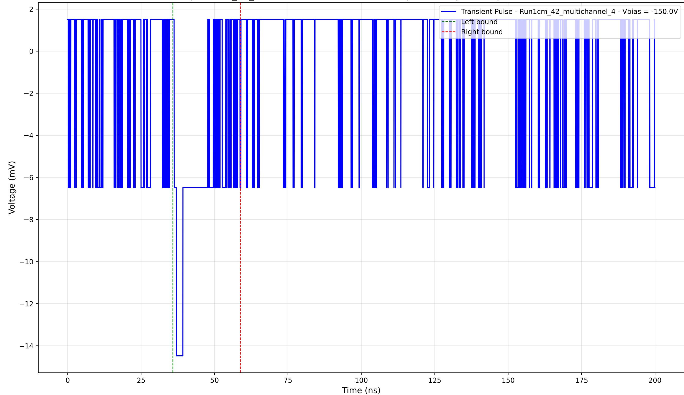
Transient Pulse - Sample: 1cm_42_multichannel - Position: 1835.0 \mu\text{m} - Charge: 2.42 pC - Rise Time: 0.00 ns (N/A)
