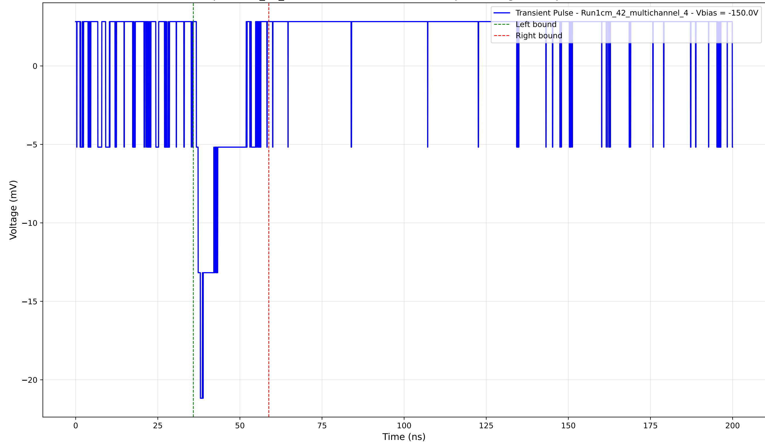
Transient Pulse - Sample: 1cm_42_multichannel - Position: 3555.0 \mu\text{m} - Charge: 2.52 pC - Rise Time: 0.00 ns (N/A)
