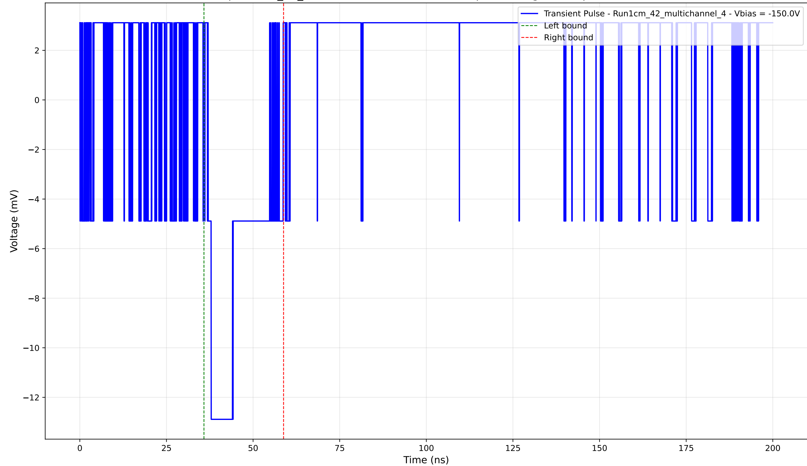
Transient Pulse - Sample: 1cm_42_multichannel - Position: 630.0 \mu\text{m} - Charge: 2.93 pC - Rise Time: 0.00 ns (N/A)
