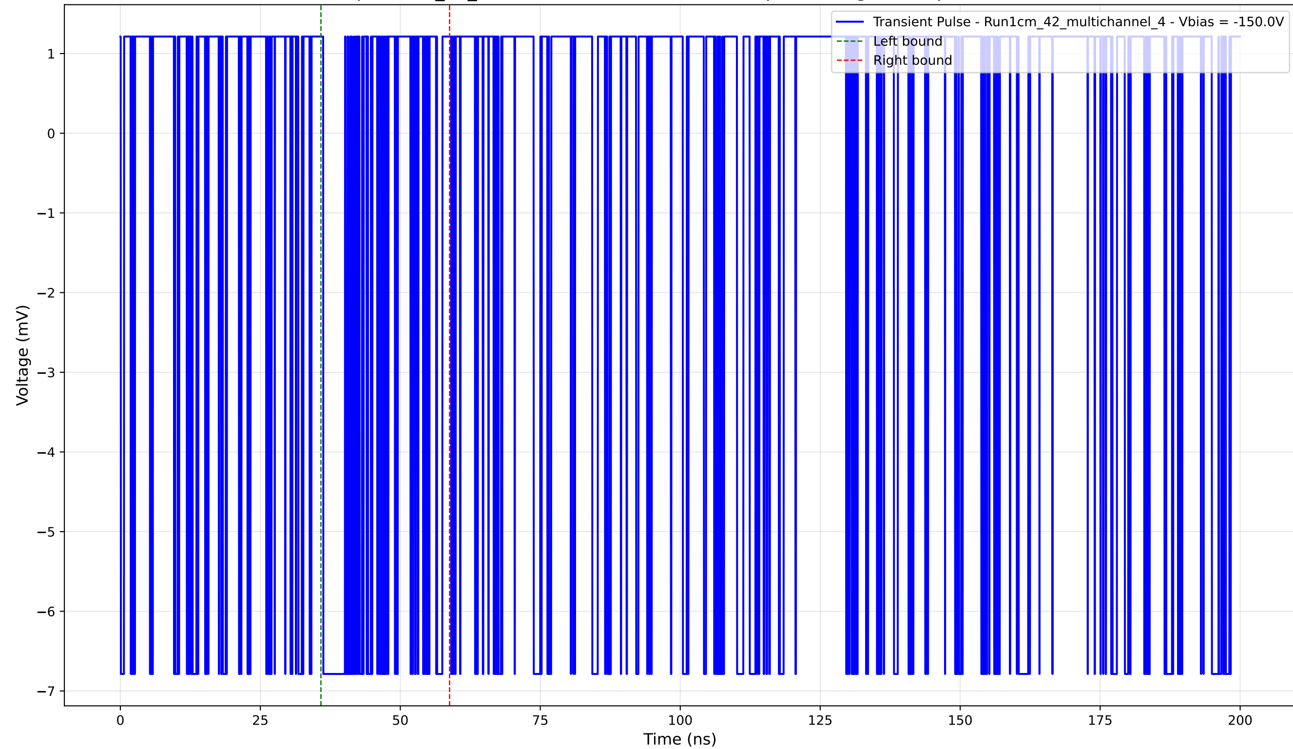
Transient Pulse - Sample: 1cm_42_multichannel - Position: 2360.0 \mu\text{m} - Charge: 1.12 pC - Rise Time: 0.00 ns (N/A)
