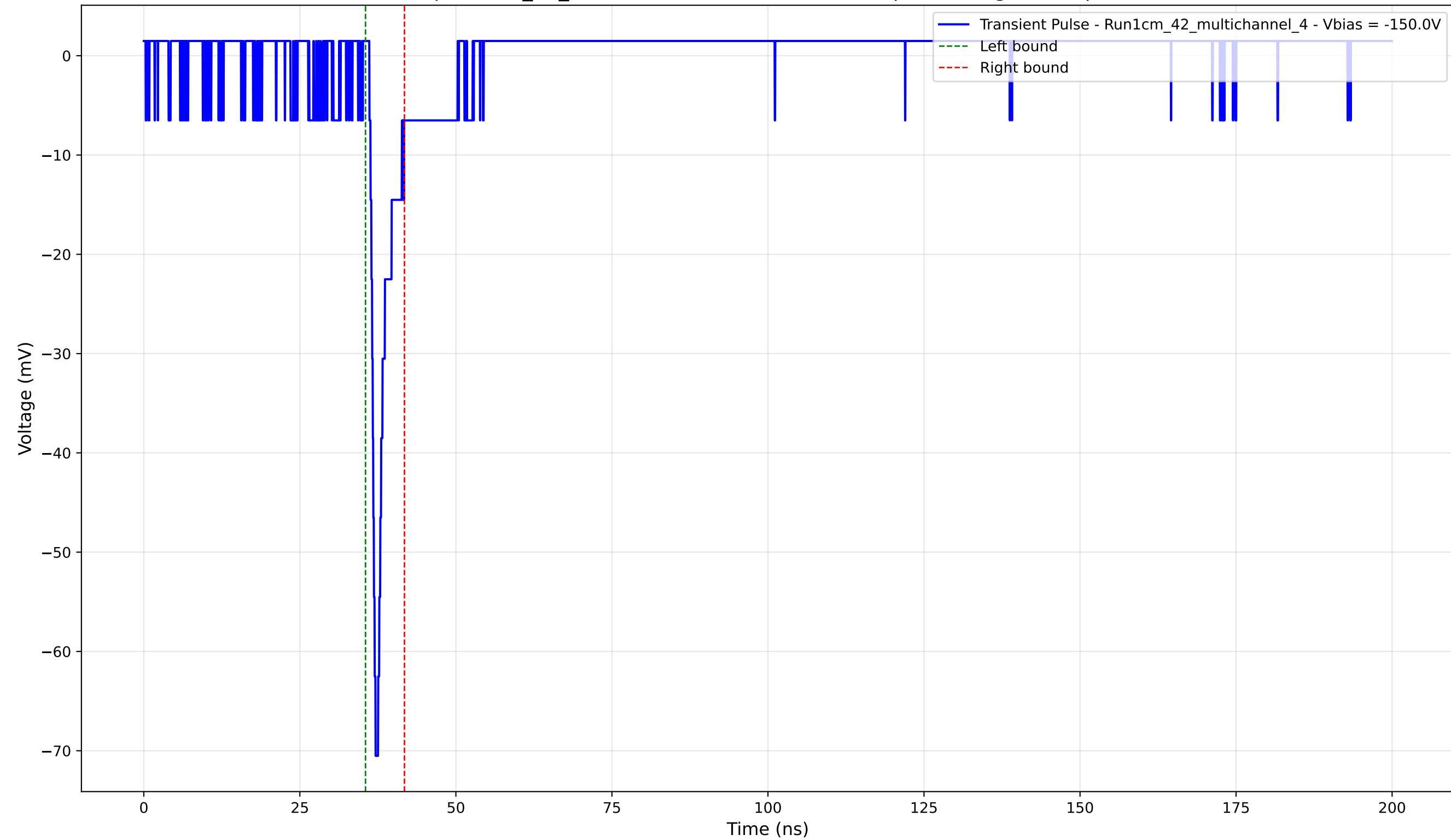
Transient Pulse - Sample: 1cm_42_multichannel - Position: 2180.0 \mu\text{m} - Charge: 3.18 pC - Rise Time: 0.82 ns
