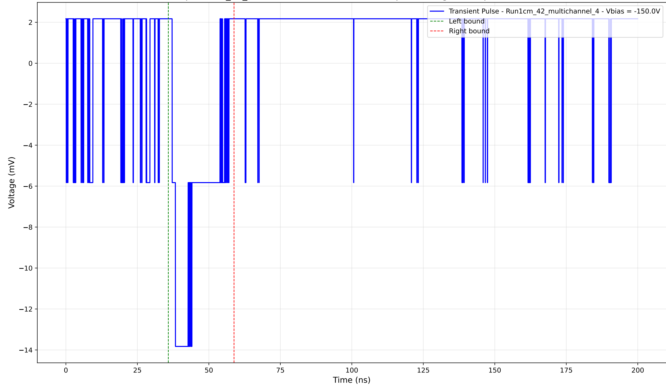
Transient Pulse - Sample: 1cm_42_multichannel - Position: 4295.0 \mu\text{m} - Charge: 2.77 pC - Rise Time: 0.00 ns (N/A)
