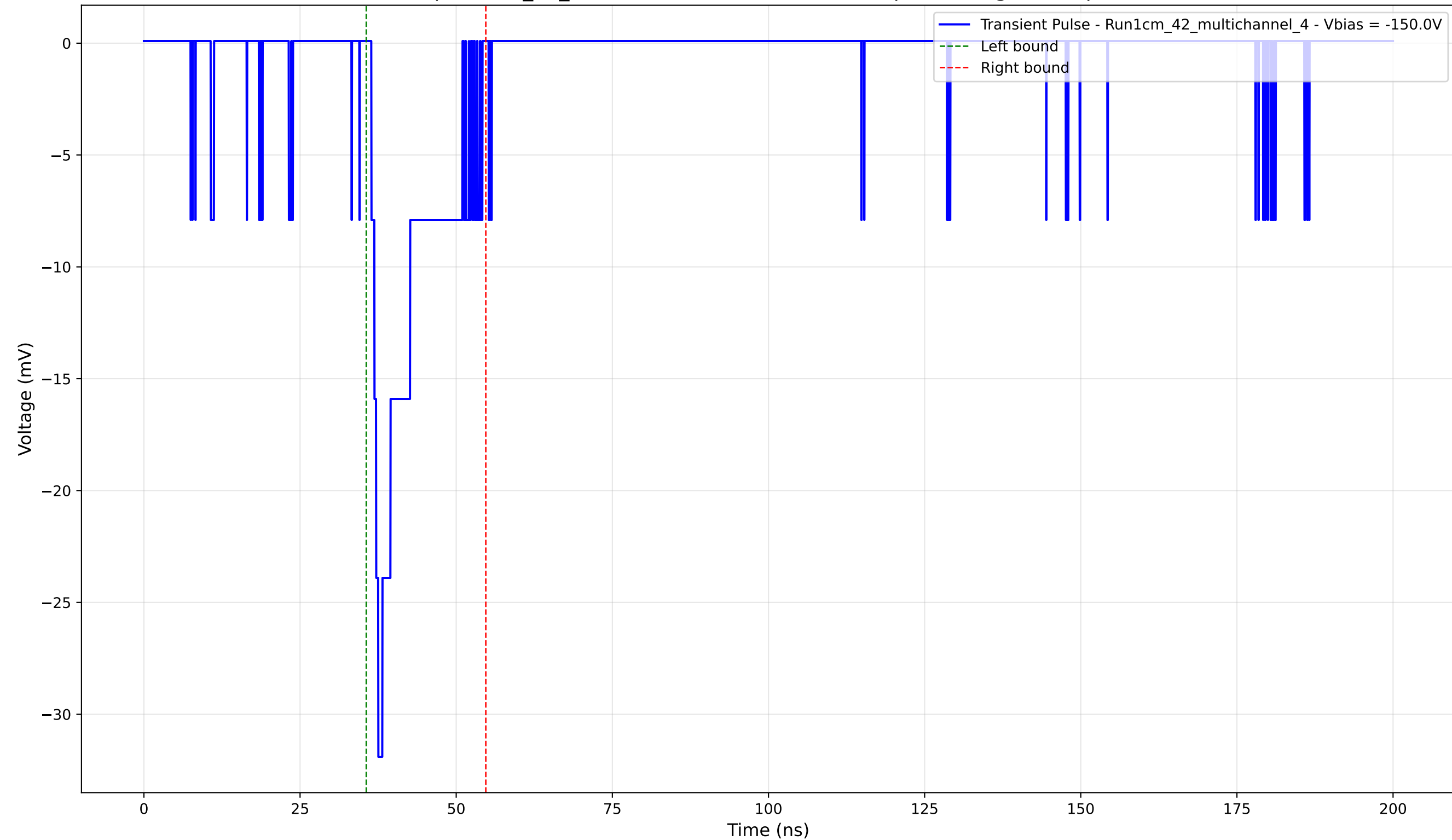
Transient Pulse - Sample: 1cm_42_multichannel - Position: 3205.0 \mu\text{m} - Charge: 4.04 pC - Rise Time: 1.11 ns
