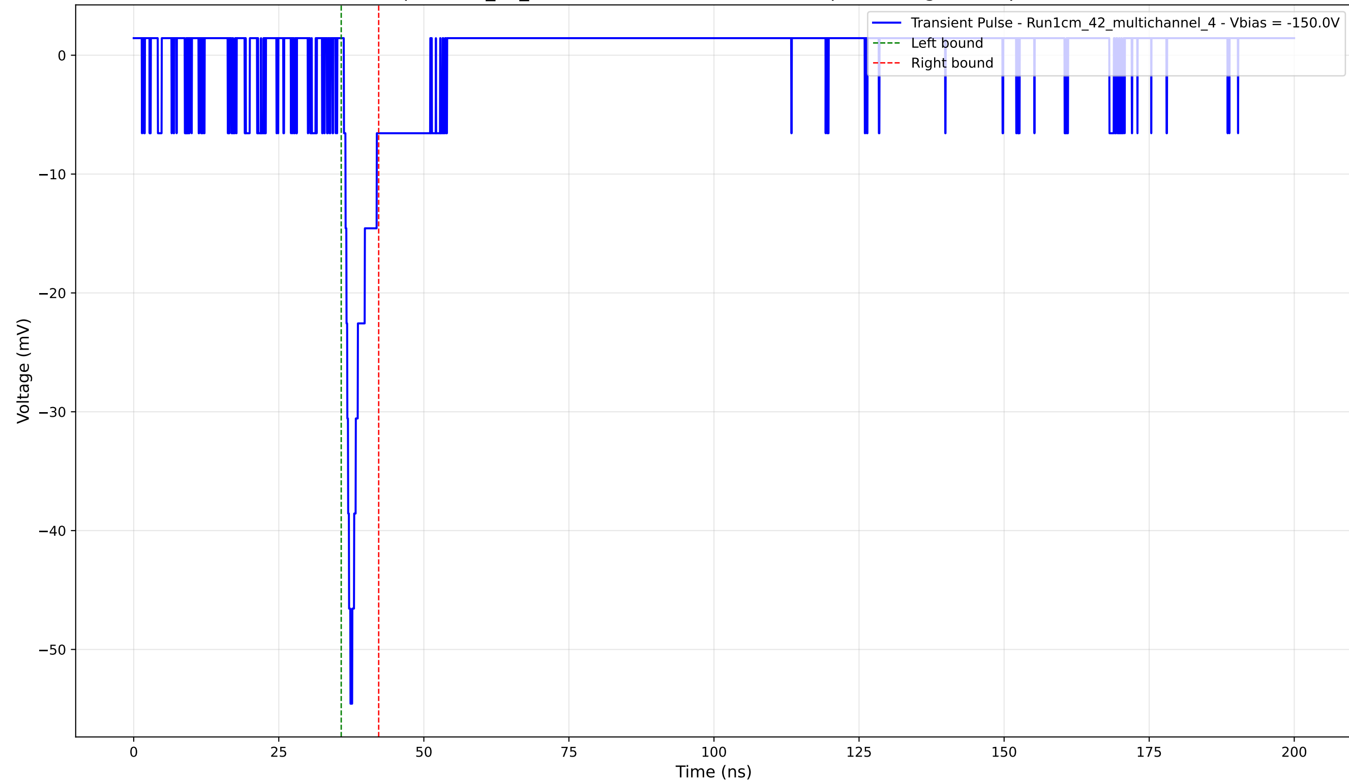
Transient Pulse - Sample: 1cm_42_multichannel - Position: 2790.0 \mu\text{m} - Charge: 2.84 pC - Rise Time: 1.12 ns
