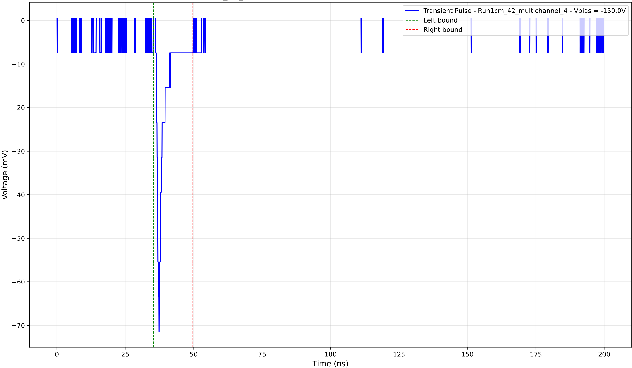
Transient Pulse - Sample: 1cm_42_multichannel - Position: 2585.0 \mu\text{m} - Charge: 4.25 pC - Rise Time: 1.16 ns
