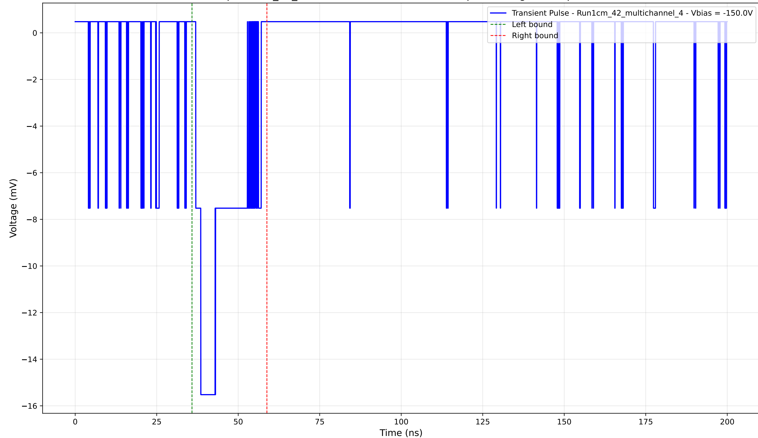
Transient Pulse - Sample: 1cm_42_multichannel - Position: 4260.0 \mu\text{m} - Charge: 3.45 pC - Rise Time: 1.56 ns
