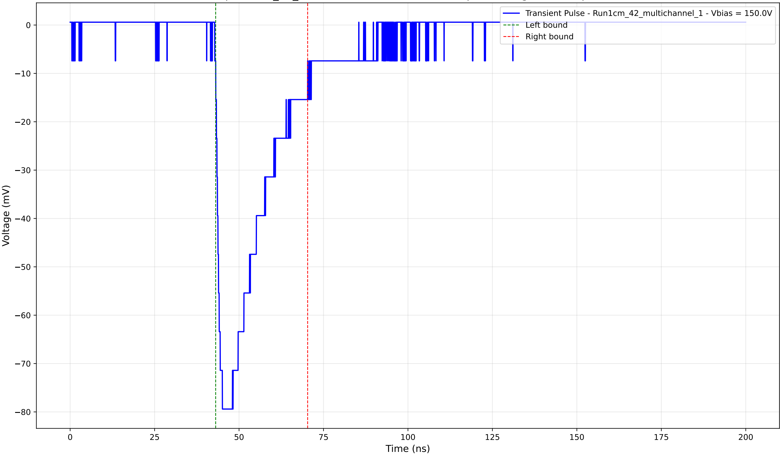
Transient Pulse - Sample: 1cm_42_multichannel - Position: 755.0 \mu\text{m} - Charge: -22.61 pC - Rise Time: 1.98 ns
