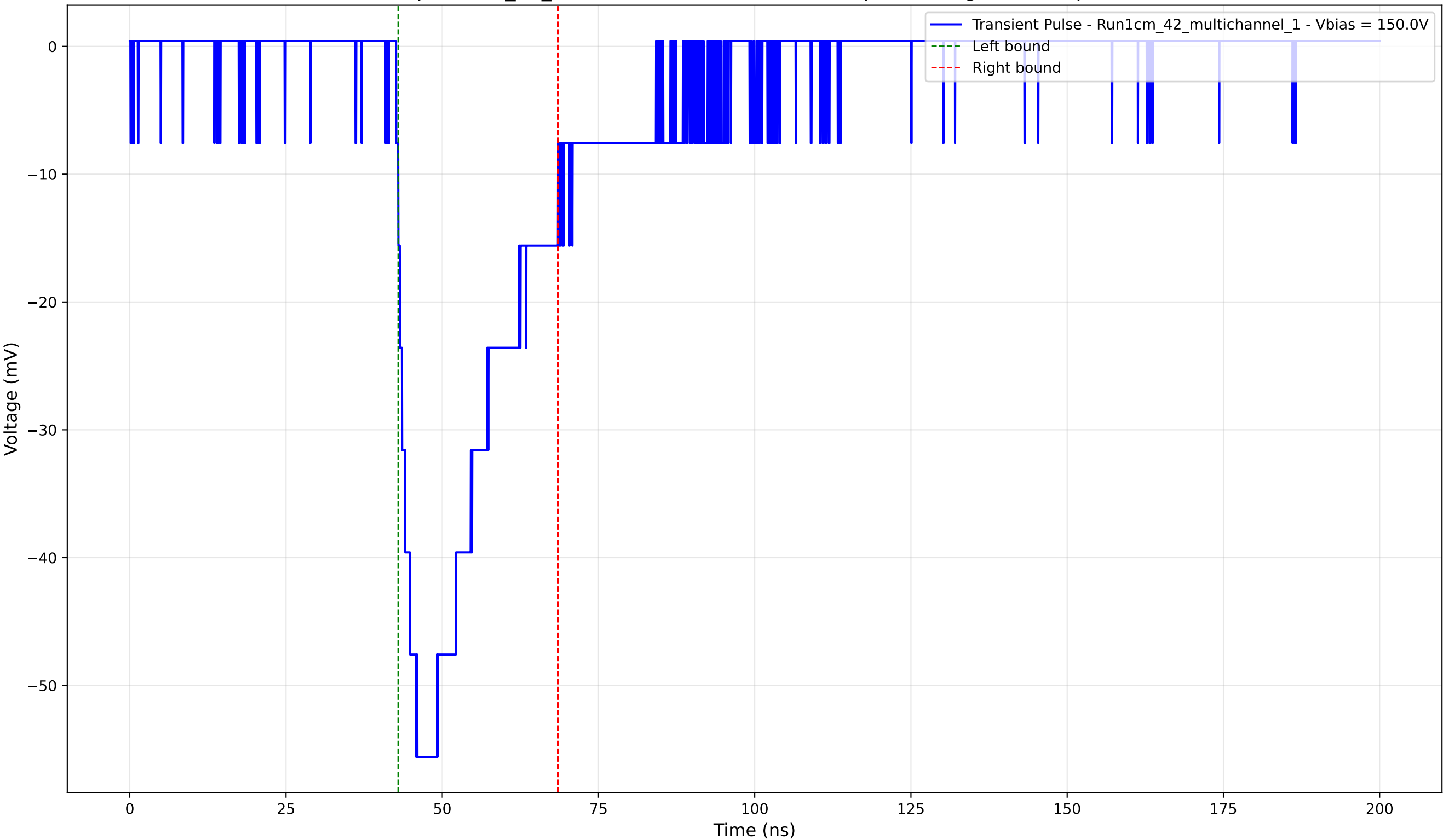
Transient Pulse - Sample: 1cm_42_multichannel - Position: 110.0 \mu\text{m} - Charge: -16.64 pC - Rise Time: 3.19 ns
