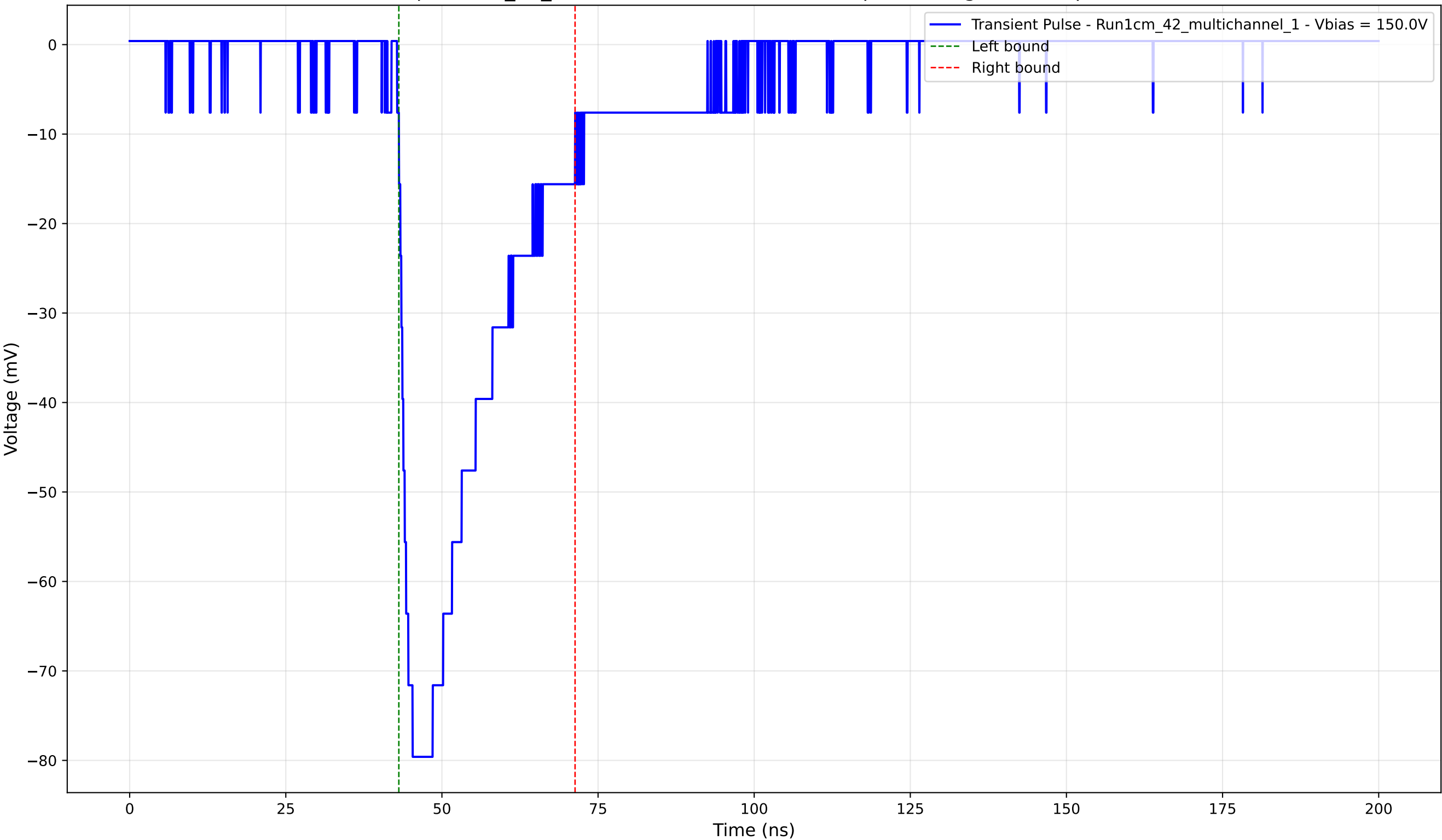
Transient Pulse - Sample: 1cm_42_multichannel - Position: 660.0 \mu\text{m} - Charge: -23.38 pC - Rise Time: 2.20 ns
