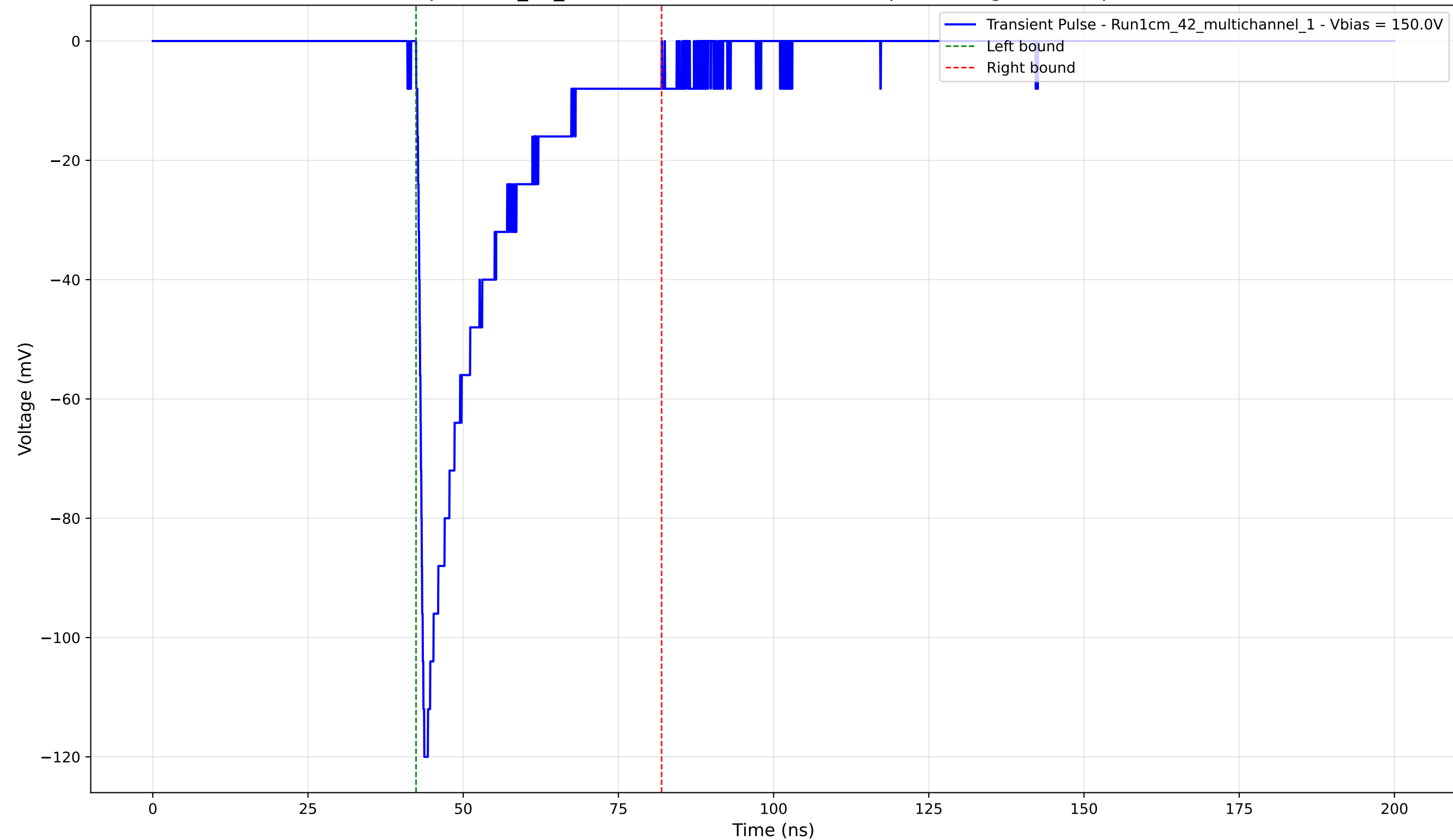
Transient Pulse - Sample: 1cm_42_multichannel - Position: 1465.0 \mu\text{m} - Charge: -24.78 pC - Rise Time: 0.97 ns
