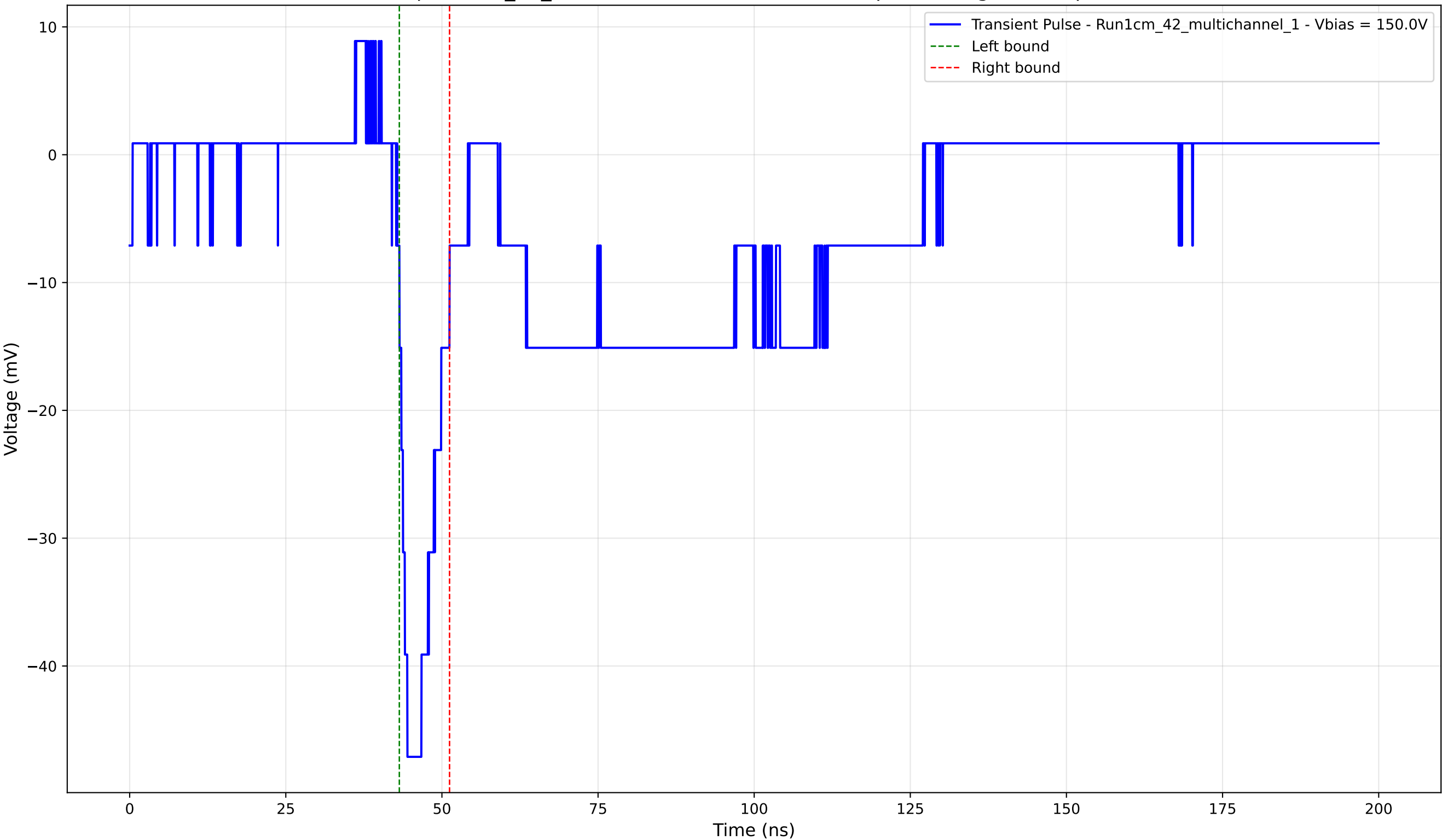
Transient Pulse - Sample: 1cm_42_multichannel - Position: 4190.0 \mu\text{m} - Charge: -5.21 pC - Rise Time: 1.63 ns
