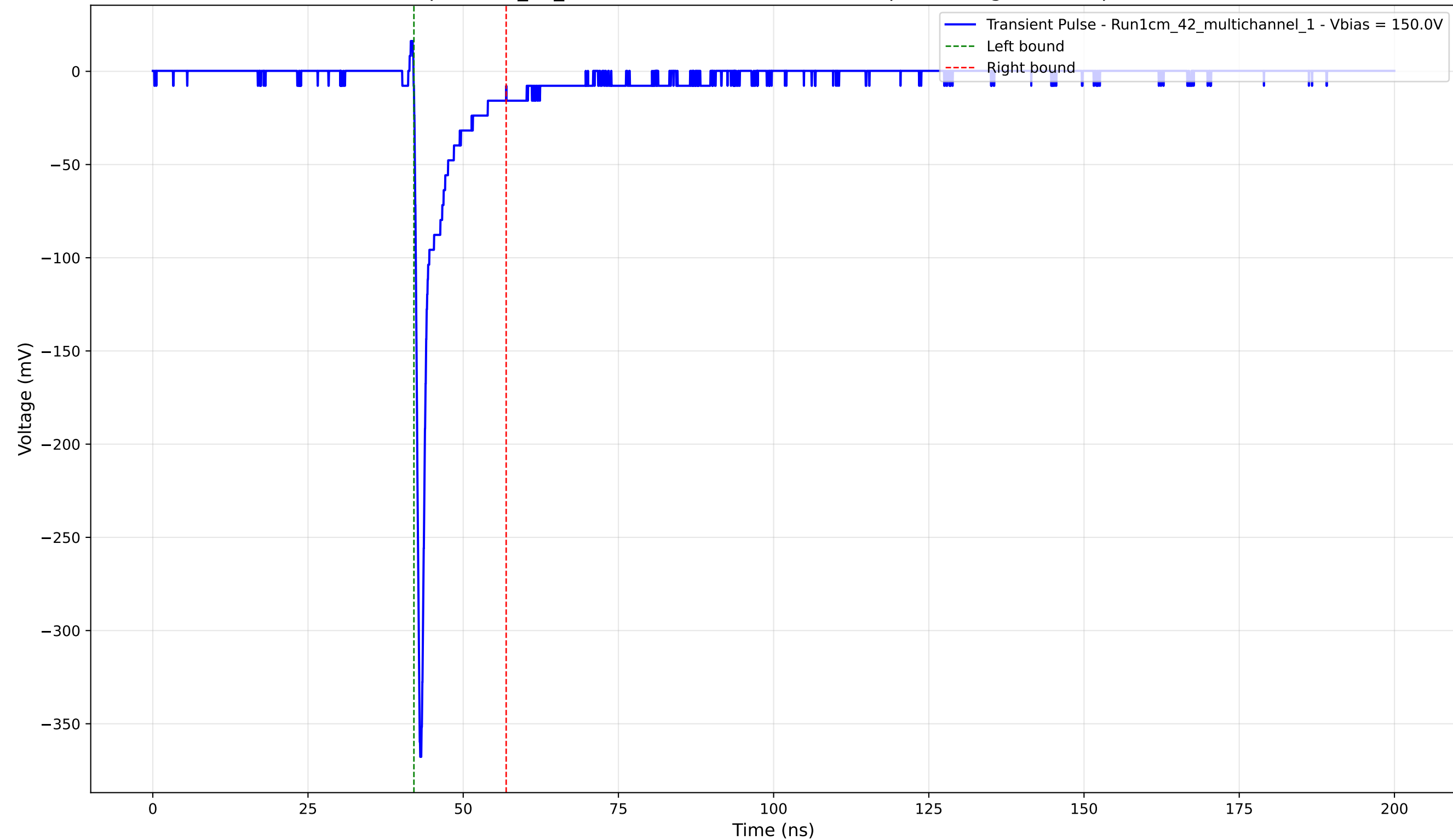
Transient Pulse - Sample: 1cm_42_multichannel - Position: 2460.0 \mu\text{m} - Charge: -20.33 pC - Rise Time: 0.74 ns
