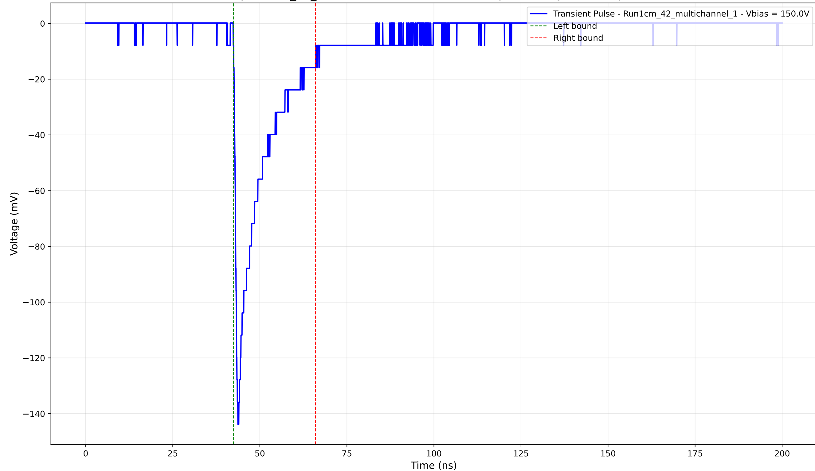
Transient Pulse - Sample: 1cm_42_multichannel - Position: 1585.0 \mu\text{m} - Charge: -22.52 pC - Rise Time: 1.02 ns
