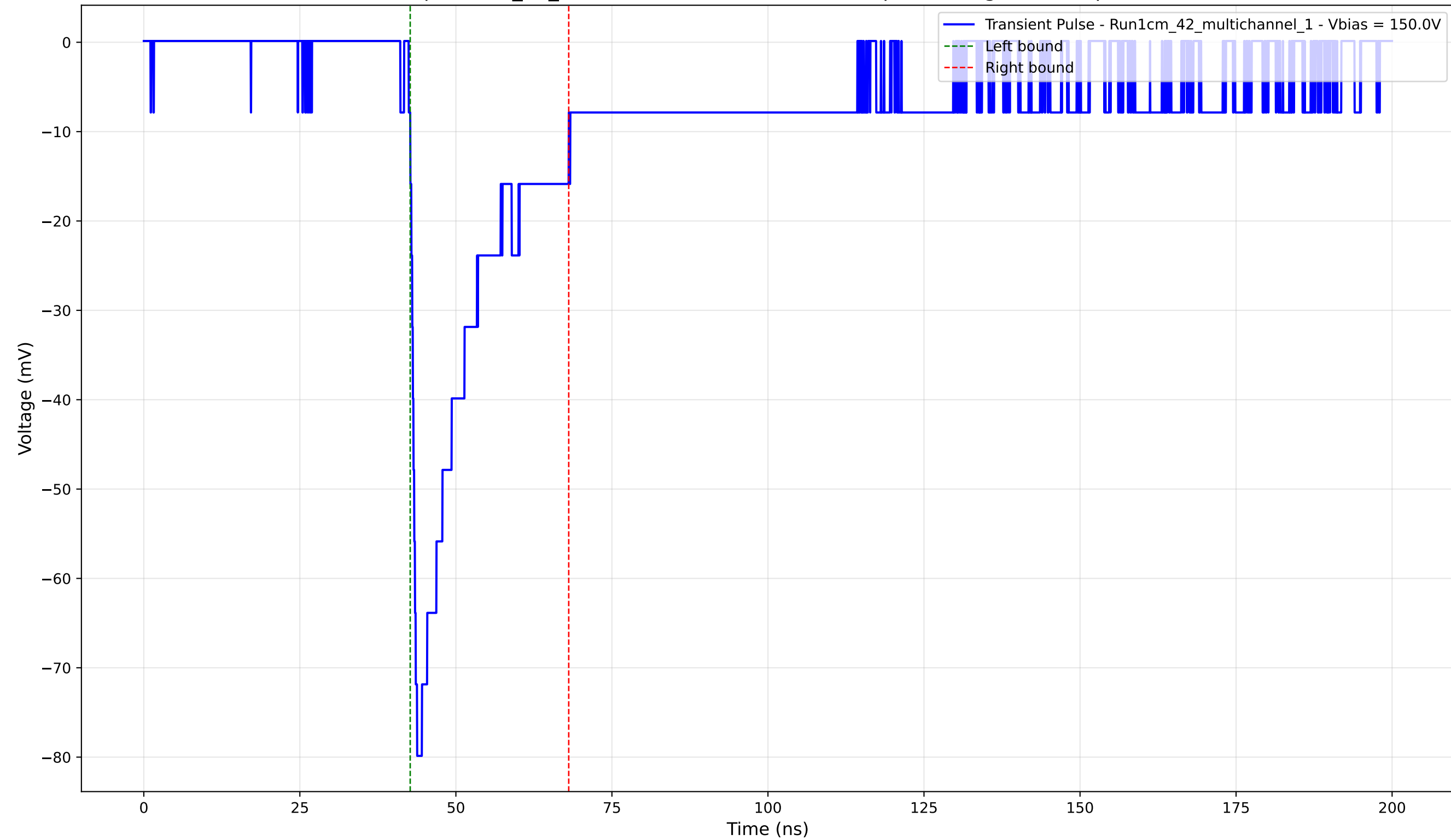
Transient Pulse - Sample: 1cm_42_multichannel - Position: 3500.0 \mu\text{m} - Charge: -16.21 pC - Rise Time: 1.10 ns
