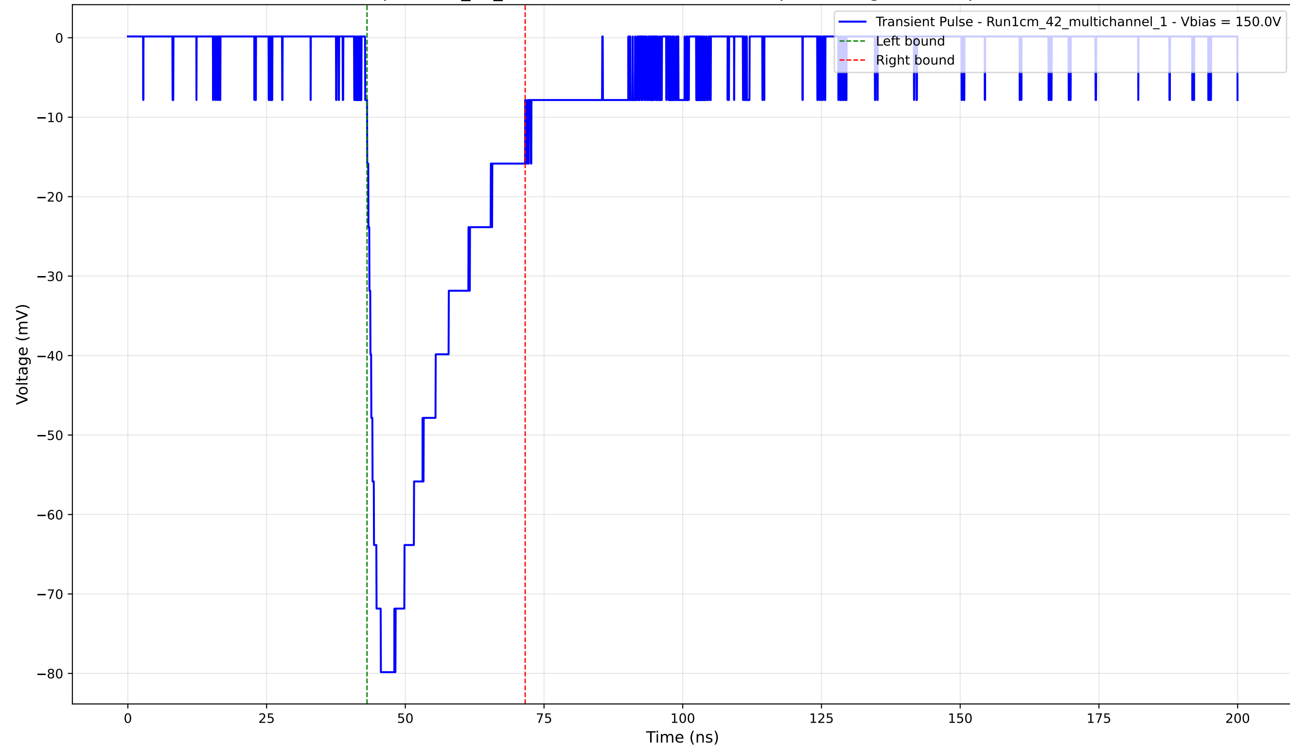
Transient Pulse - Sample: 1cm_42_multichannel - Position: 595.0 \mu\text{m} - Charge: -23.41 pC - Rise Time: 2.48 ns
