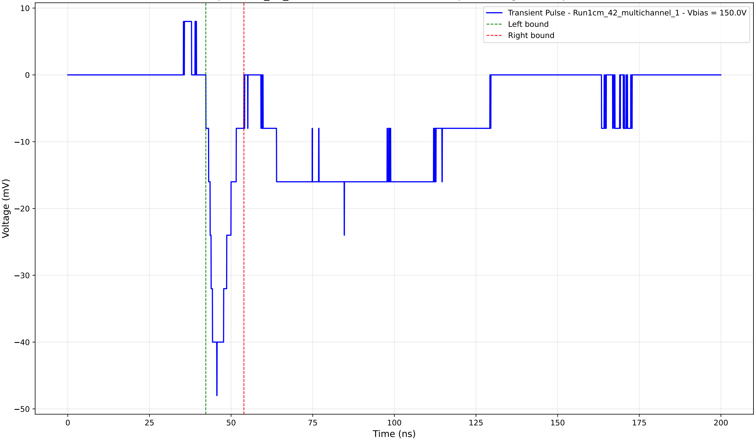
Transient Pulse - Sample: 1cm_42_multichannel - Position: 4710.0 \mu\text{m} - Charge: -5.56 pC - Rise Time: 3.35 ns
