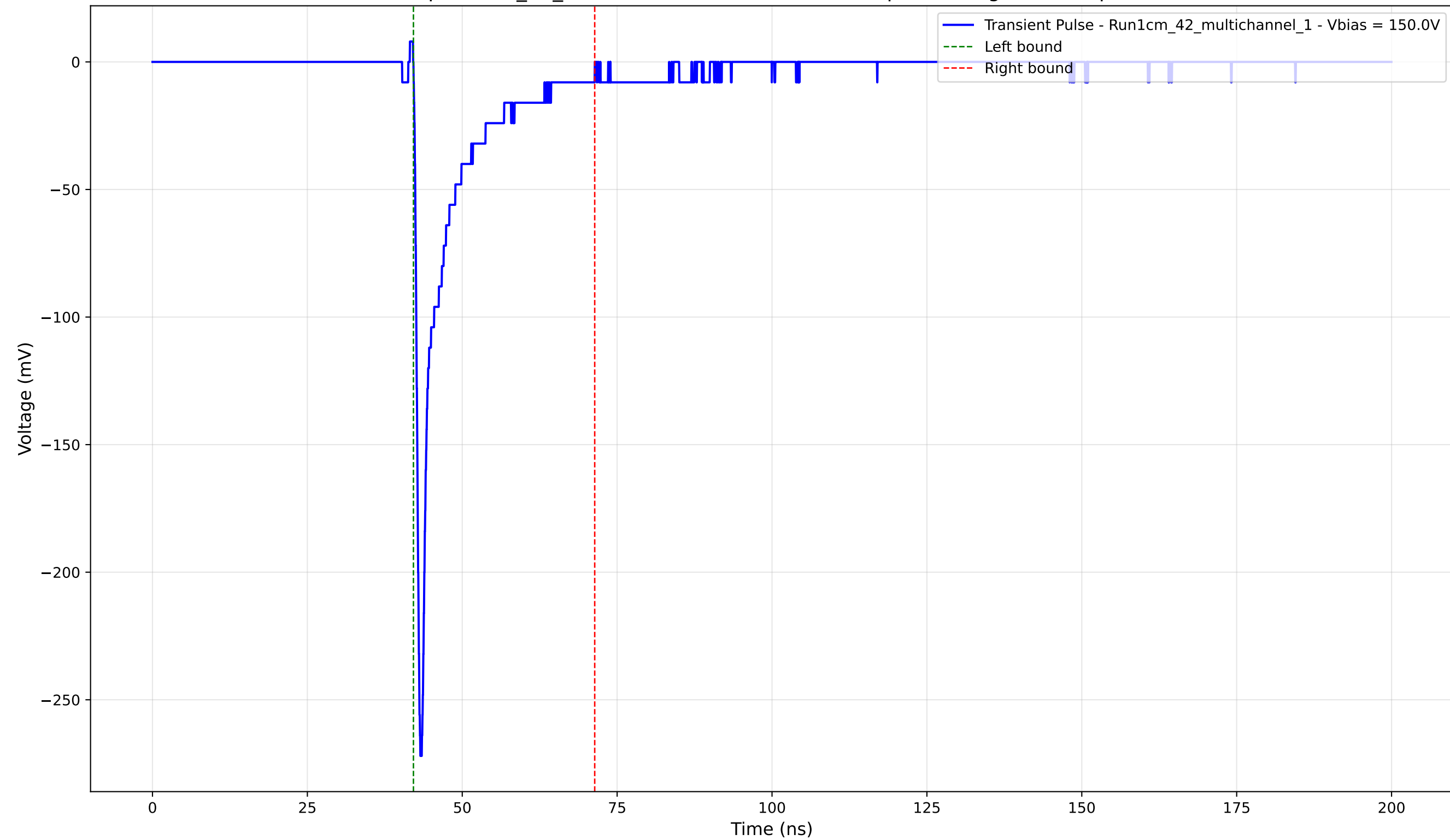
Transient Pulse - Sample: 1cm_42_multichannel - Position: 2715.0 \mu\text{m} - Charge: -23.99 pC - Rise Time: 0.76 ns
