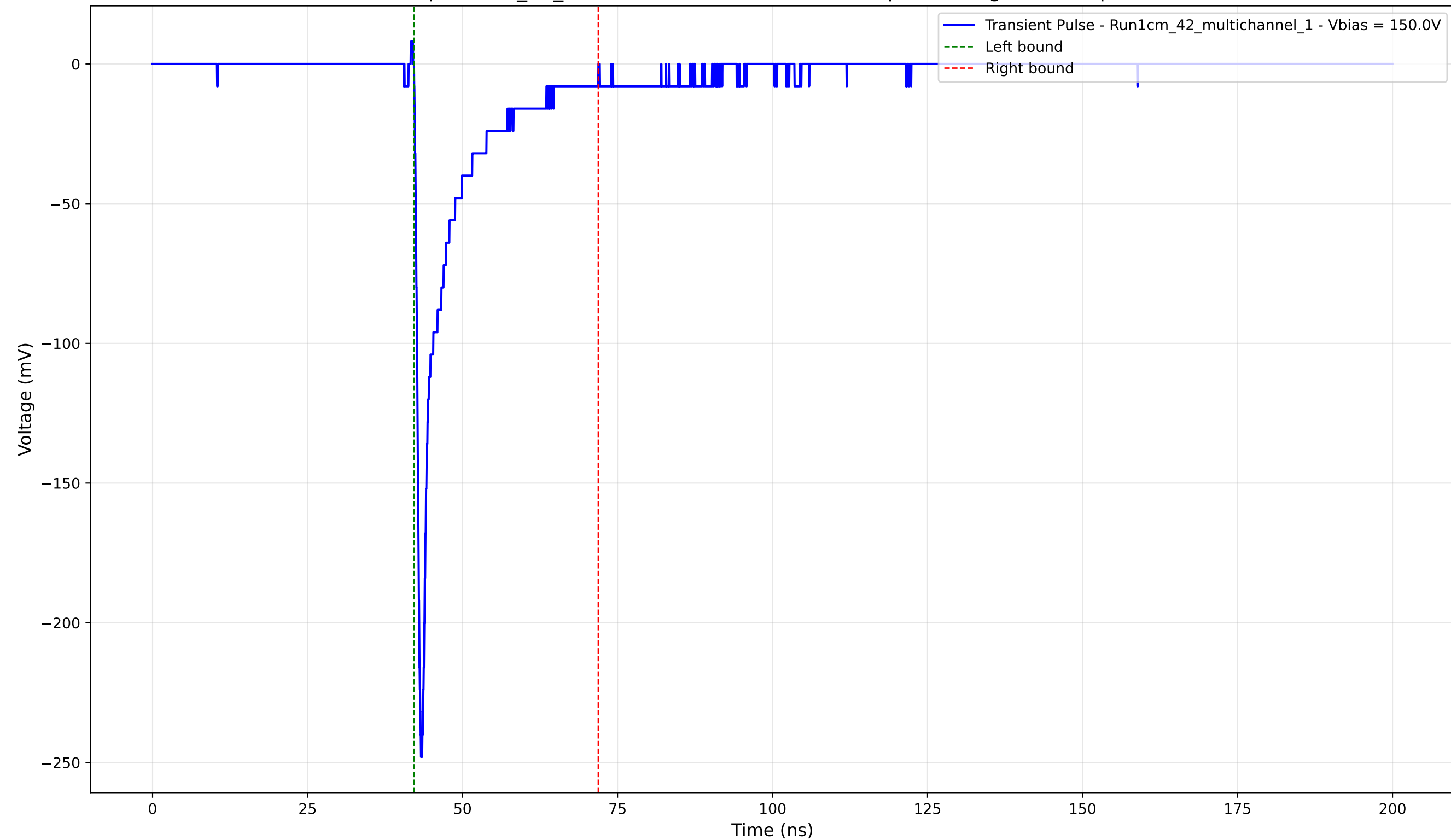
Transient Pulse - Sample: 1cm_42_multichannel - Position: 2765.0 \mu\text{m} - Charge: -23.27 pC - Rise Time: 0.78 ns
