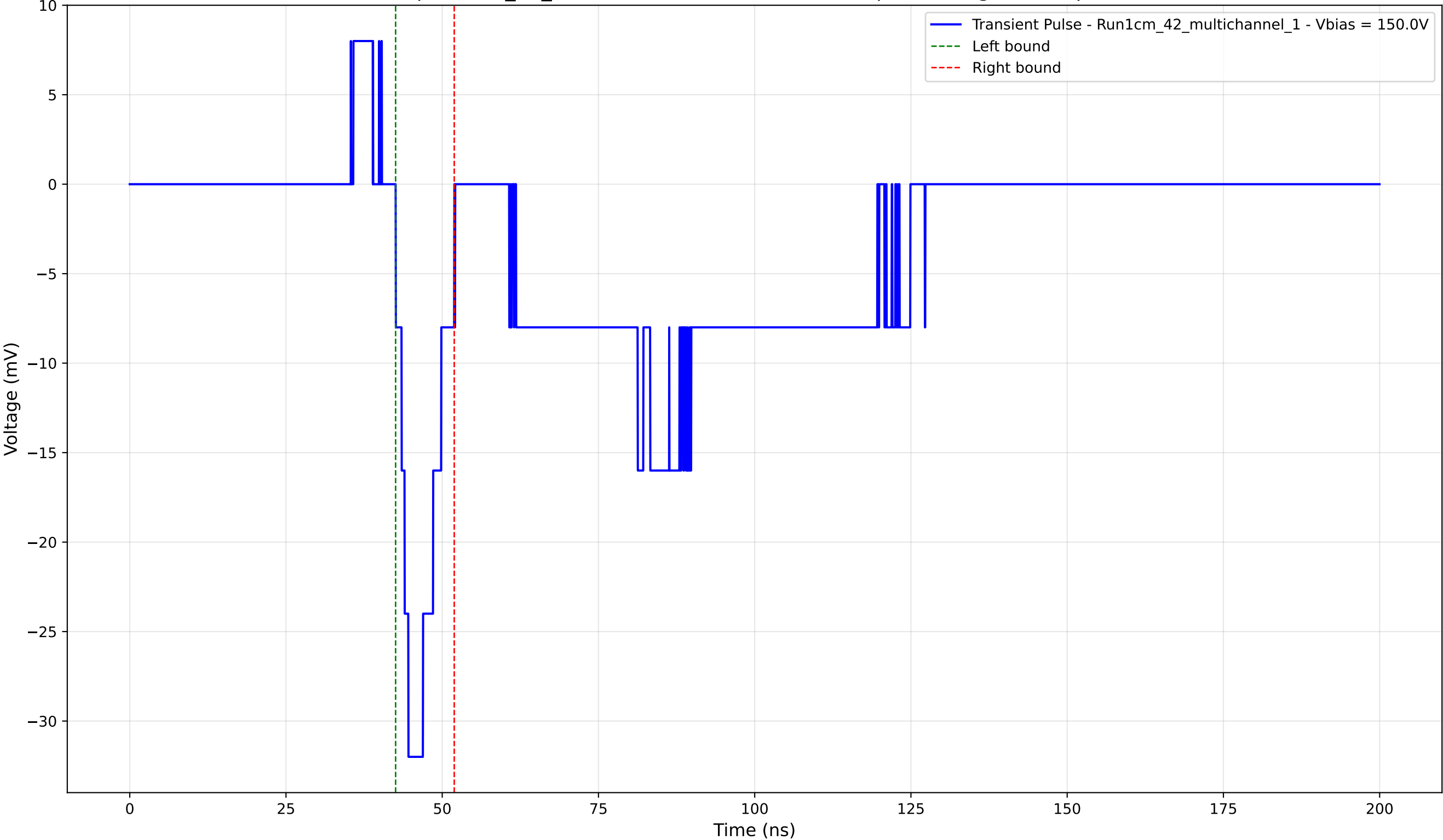
Transient Pulse - Sample: 1cm_42_multichannel - Position: 4350.0 \mu\text{m} - Charge: -3.62 pC - Rise Time: 2.03 ns
