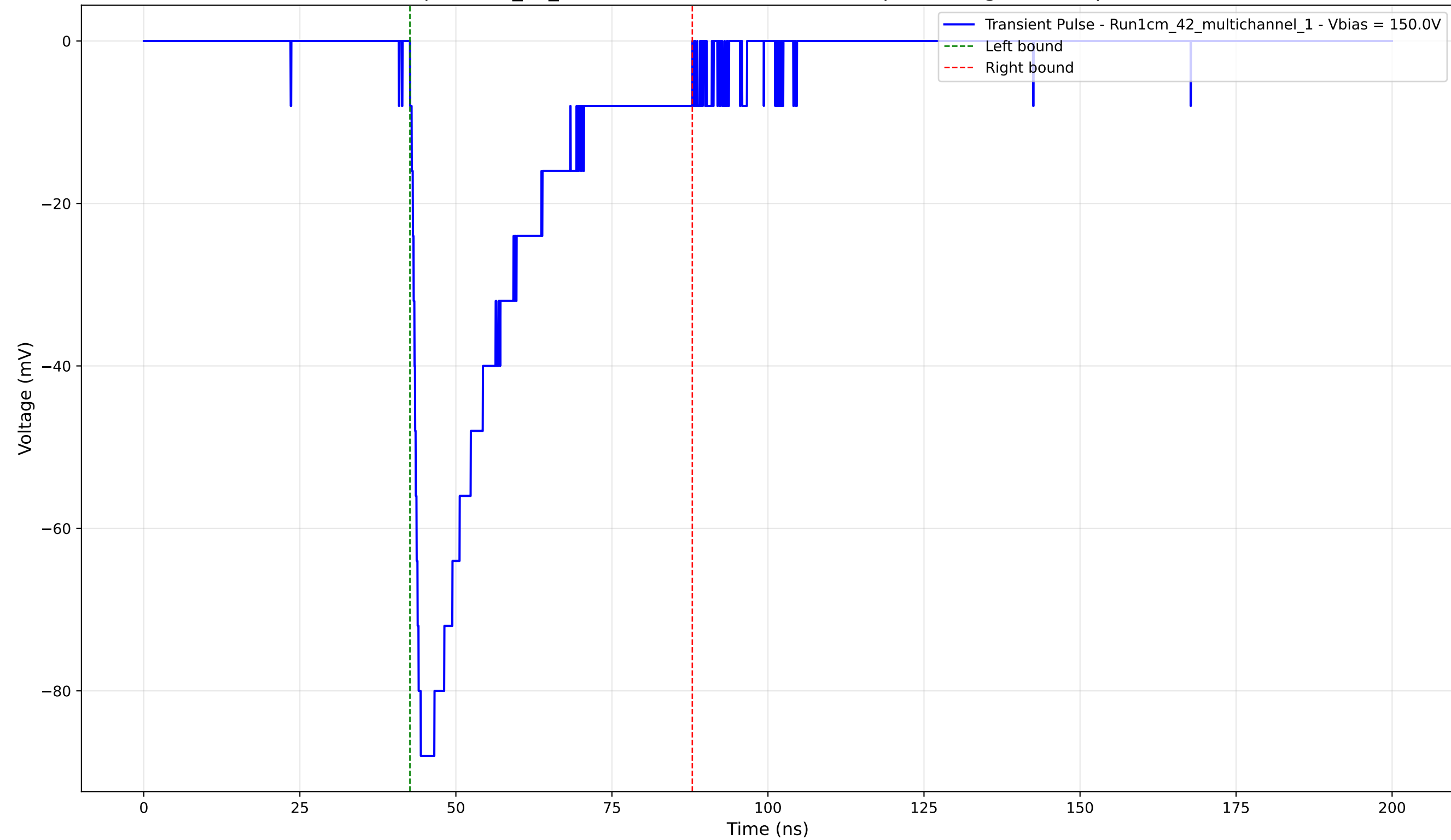
Transient Pulse - Sample: 1cm_42_multichannel - Position: 1050.0 \mu\text{m} - Charge: -25.74 pC - Rise Time: 1.12 ns
