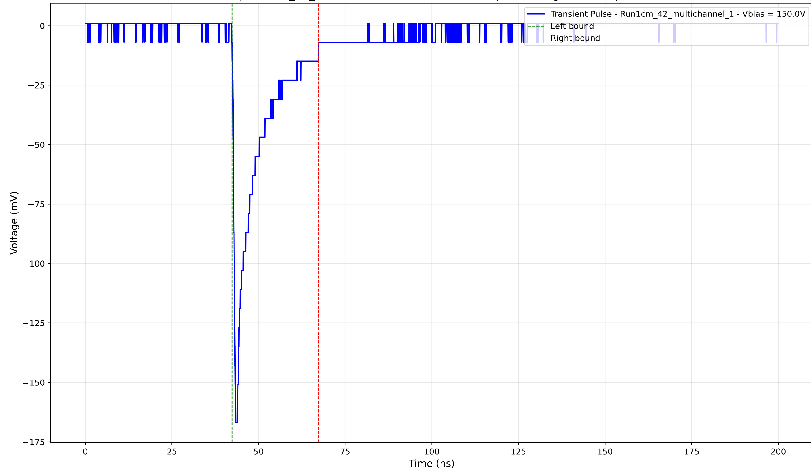
Transient Pulse - Sample: 1cm_42_multichannel - Position: 1735.0 \mu\text{m} - Charge: -22.83 pC - Rise Time: 0.82 ns
