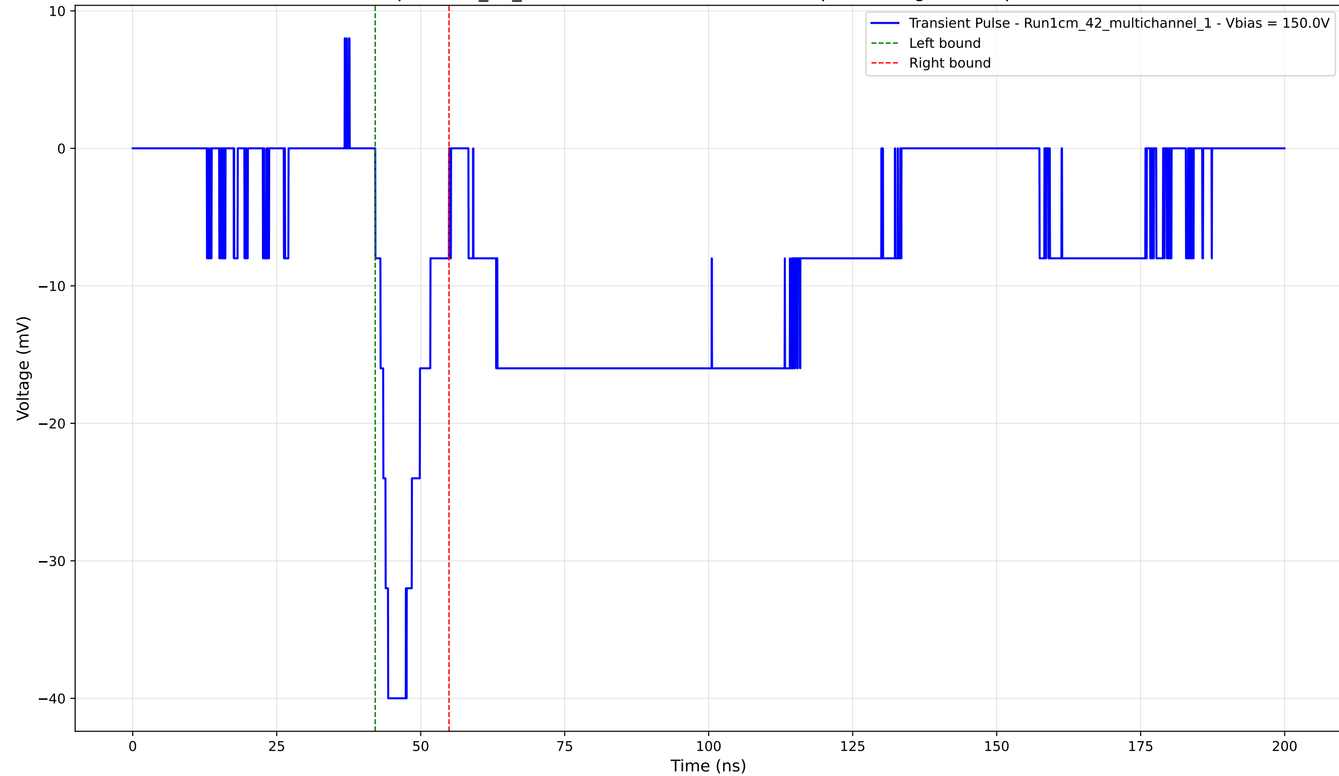
Transient Pulse - Sample: 1cm_42_multichannel - Position: 4795.0 \mu\text{m} - Charge: -5.68 pC - Rise Time: 2.23 ns
