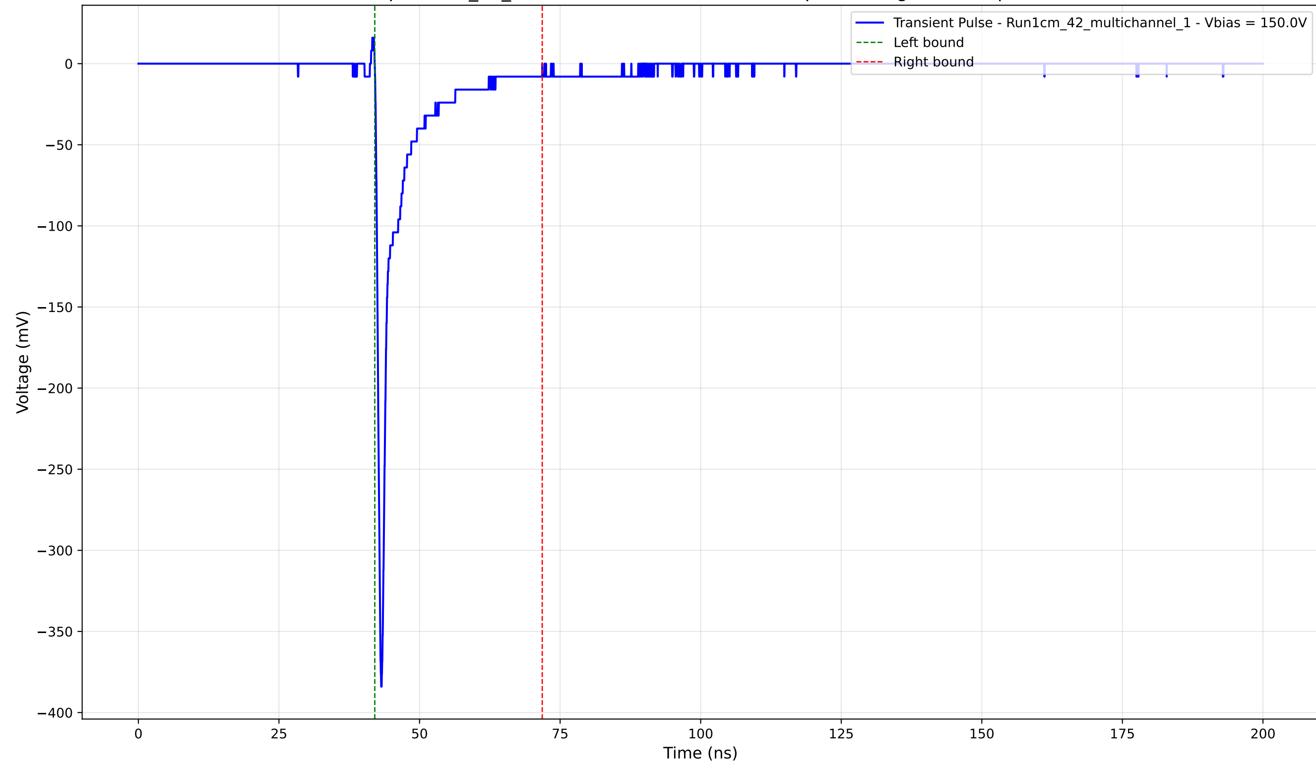
Transient Pulse - Sample: 1cm_42_multichannel - Position: 2235.0 \mu\text{m} - Charge: -26.43 pC - Rise Time: 0.76 ns
