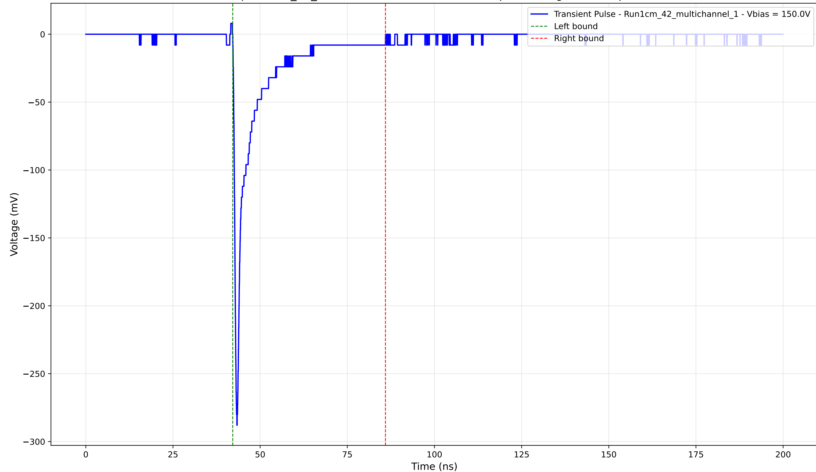
Transient Pulse - Sample: 1cm_42_multichannel - Position: 2050.0 \mu\text{m} - Charge: -27.84 pC - Rise Time: 0.81 ns
