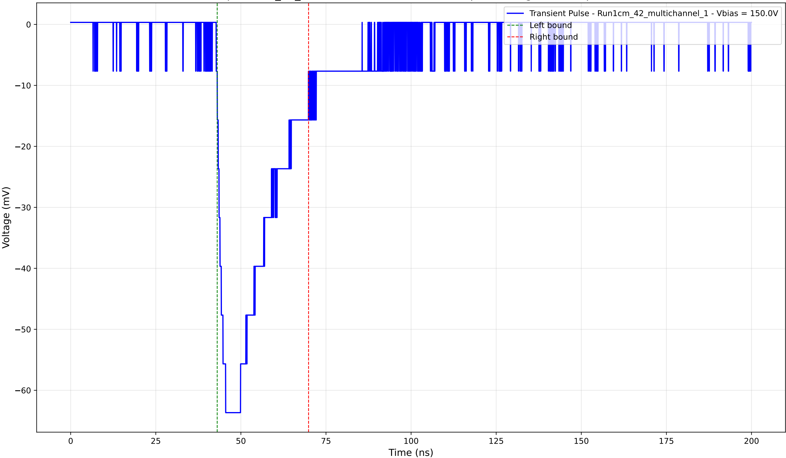
Transient Pulse - Sample: 1cm_42_multichannel - Position: 265.0 \mu\text{m} - Charge: -19.80 pC - Rise Time: 2.78 ns
