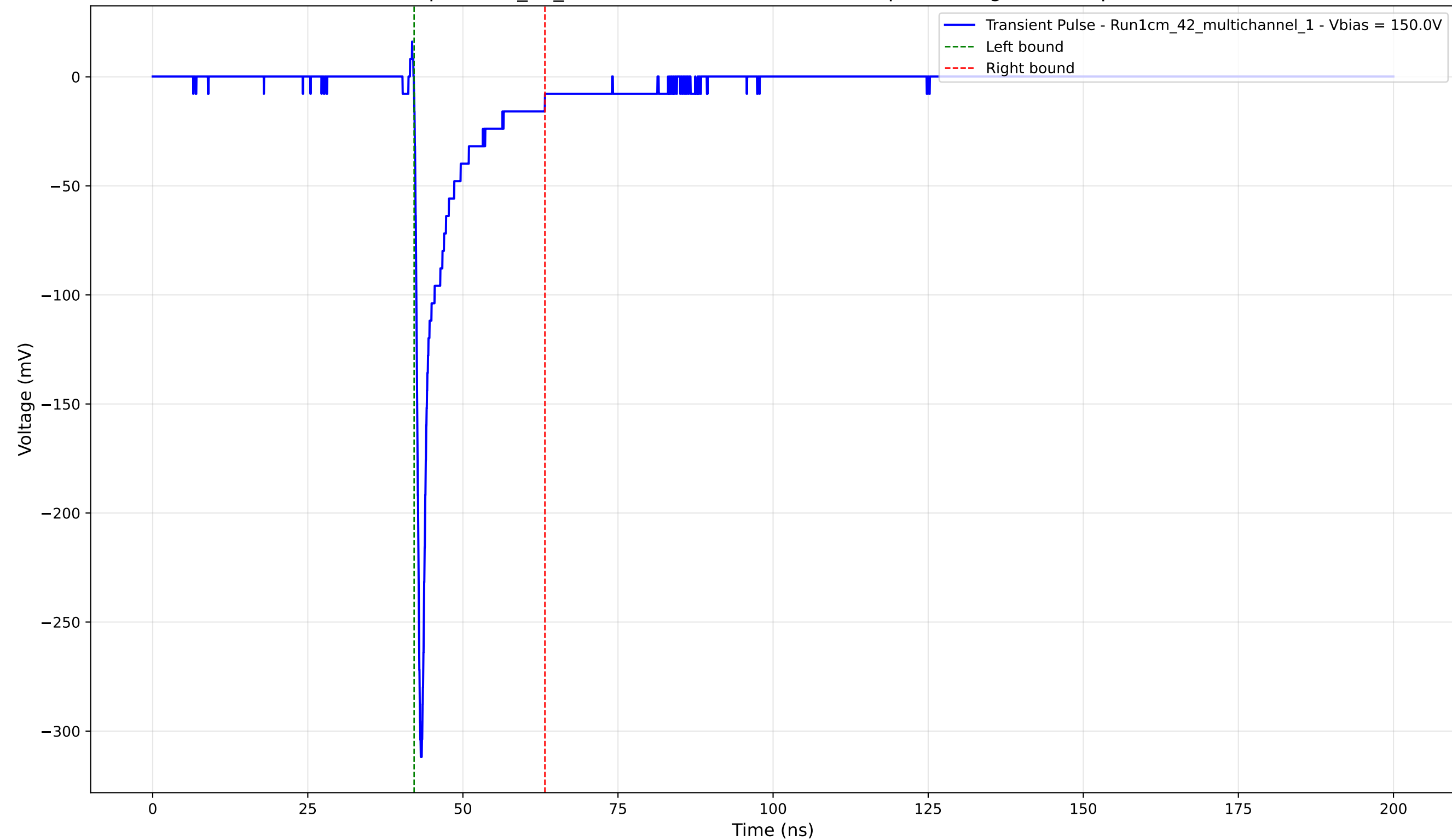
Transient Pulse - Sample: 1cm_42_multichannel - Position: 2635.0 \mu\text{m} - Charge: -23.11 pC - Rise Time: 0.78 ns
