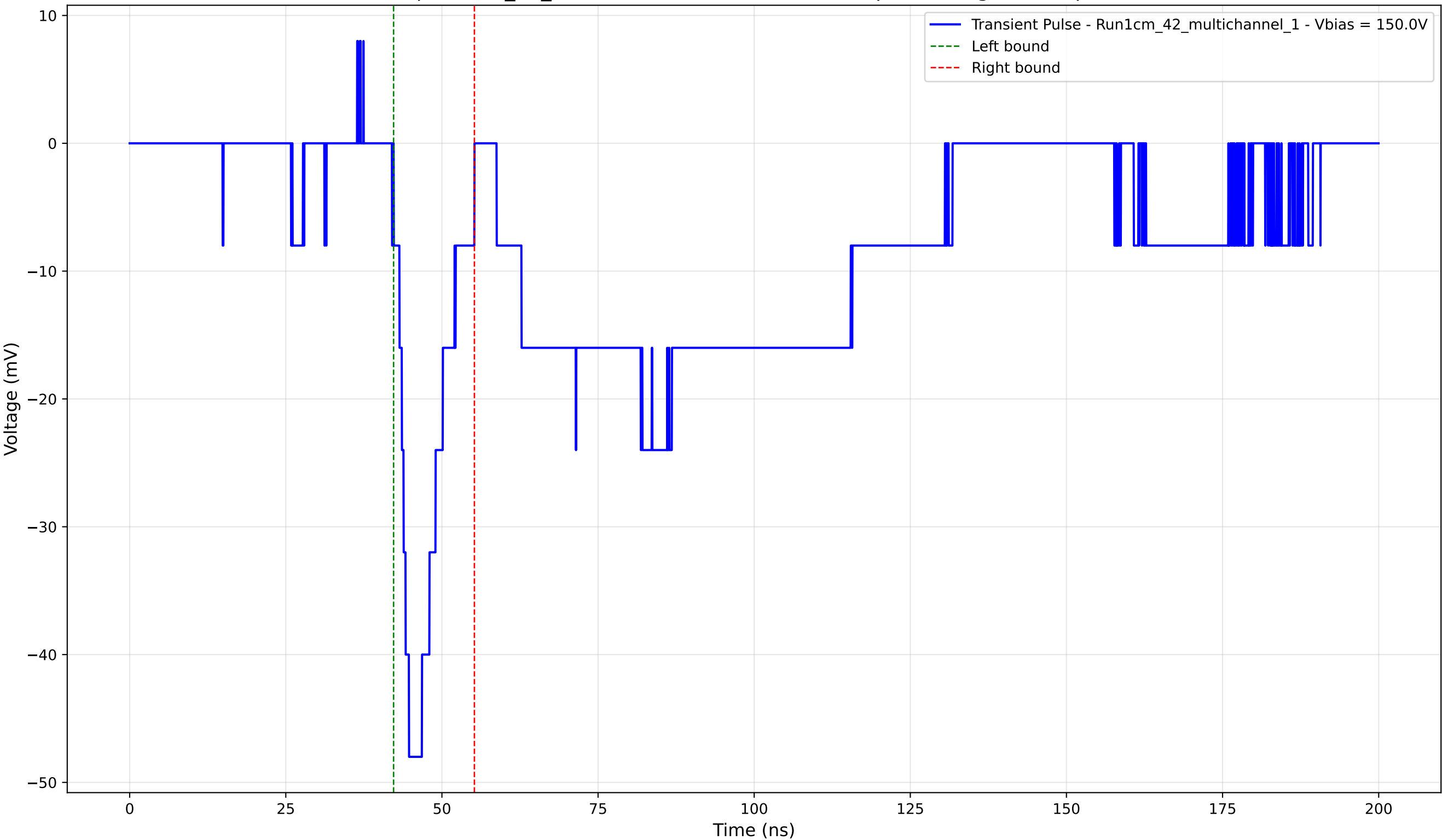
Transient Pulse - Sample: 1cm_42_multichannel - Position: 4510.0 \mu\text{m} - Charge: -6.31 pC - Rise Time: 2.45 ns
