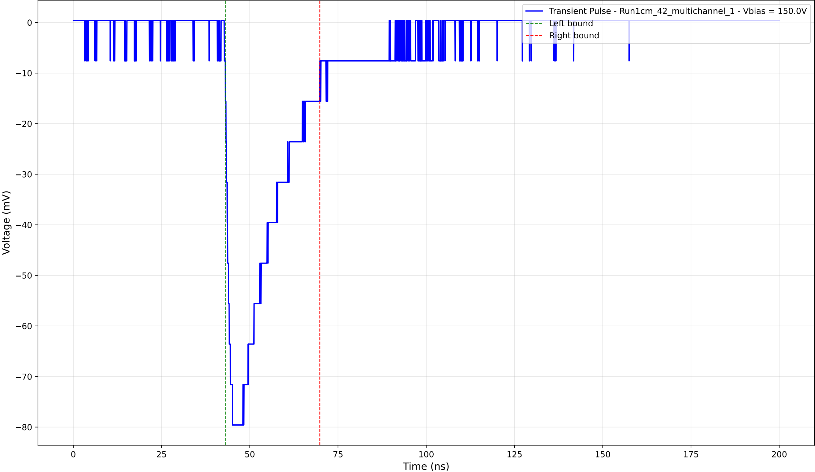
Transient Pulse - Sample: 1cm_42_multichannel - Position: 760.0 \mu\text{m} - Charge: -22.64 pC - Rise Time: 2.02 ns
