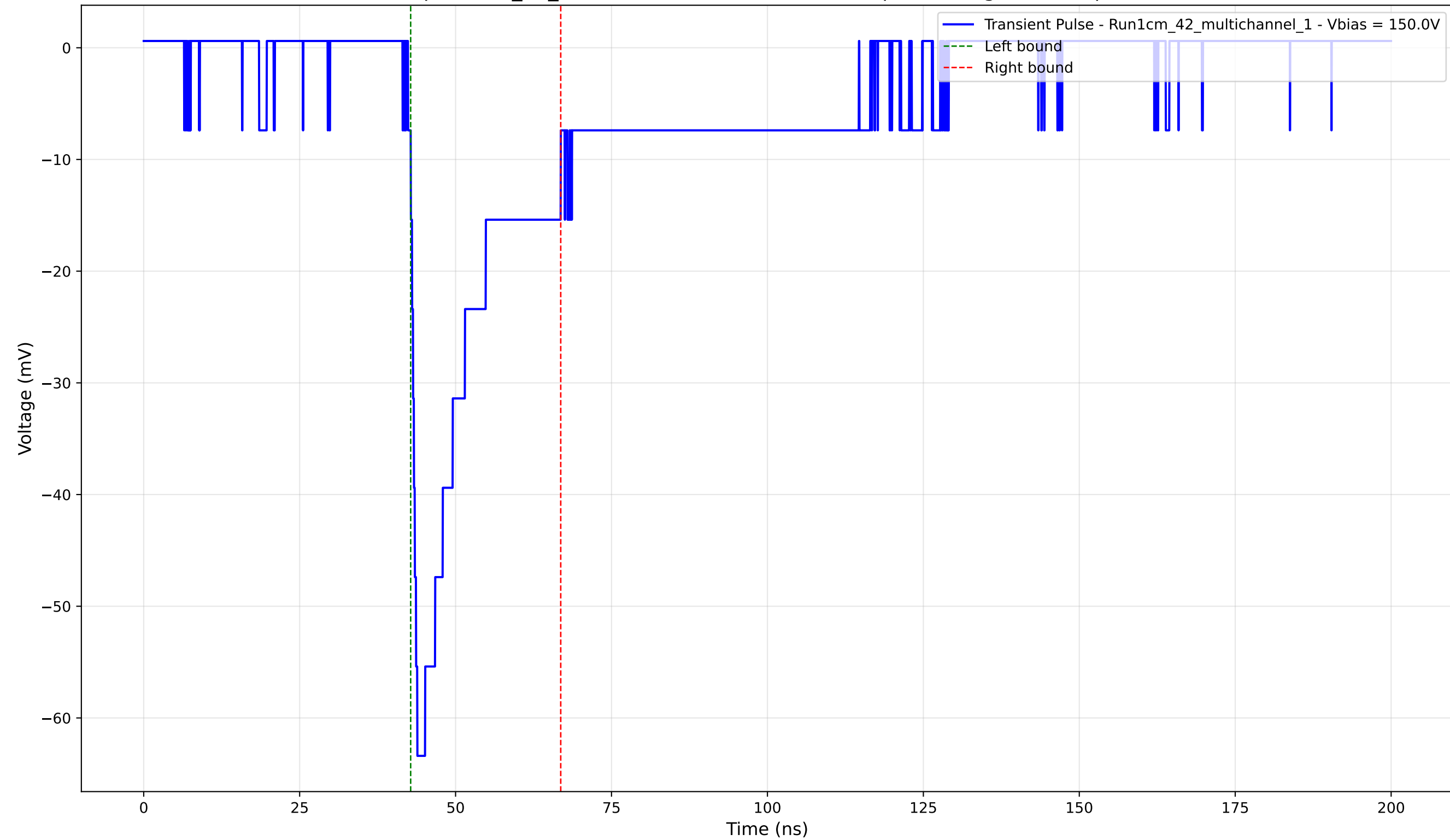
Transient Pulse - Sample: 1cm_42_multichannel - Position: 3650.0 \mu\text{m} - Charge: -13.03 pC - Rise Time: 1.48 ns
