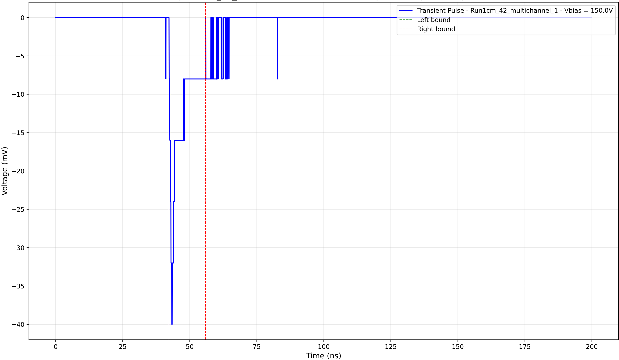
Transient Pulse - Sample: 1cm_42_multichannel - Position: 2860.0 \mu\text{m} - Charge: -3.48 pC - Rise Time: 1.03 ns
