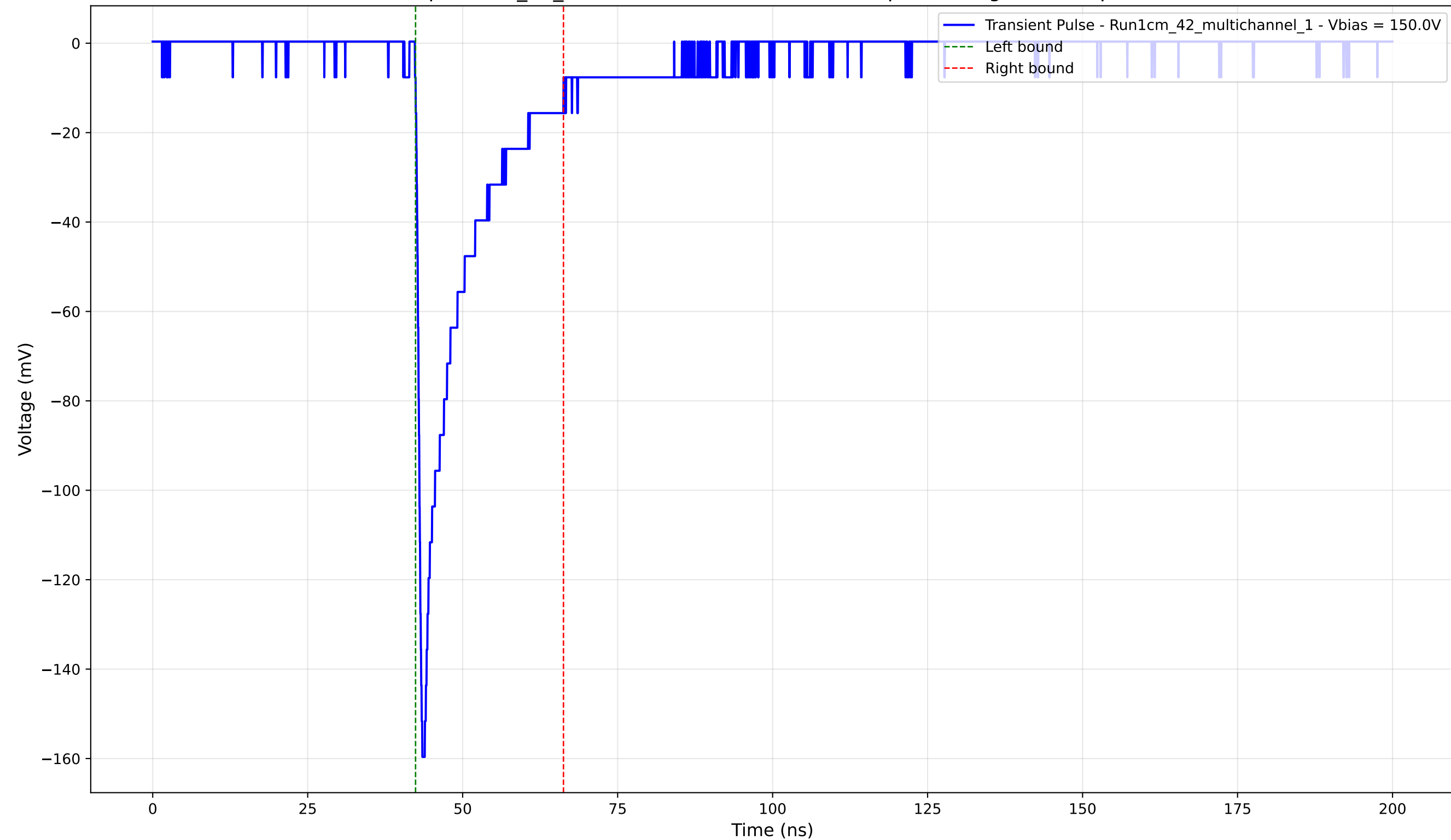
Transient Pulse - Sample: 1cm_42_multichannel - Position: 1695.0 \mu\text{m} - Charge: -22.58 pC - Rise Time: 0.88 ns
