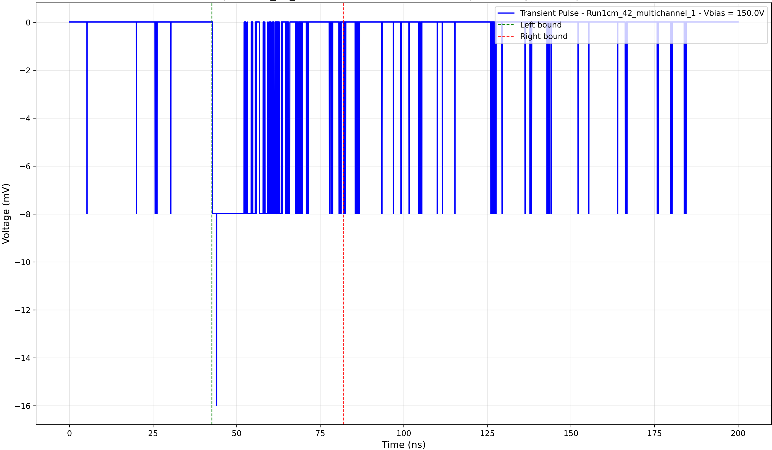
Transient Pulse - Sample: 1cm_42_multichannel - Position: 1395.0 \mu\text{m} - Charge: -3.18 pC - Rise Time: 1.14 ns
