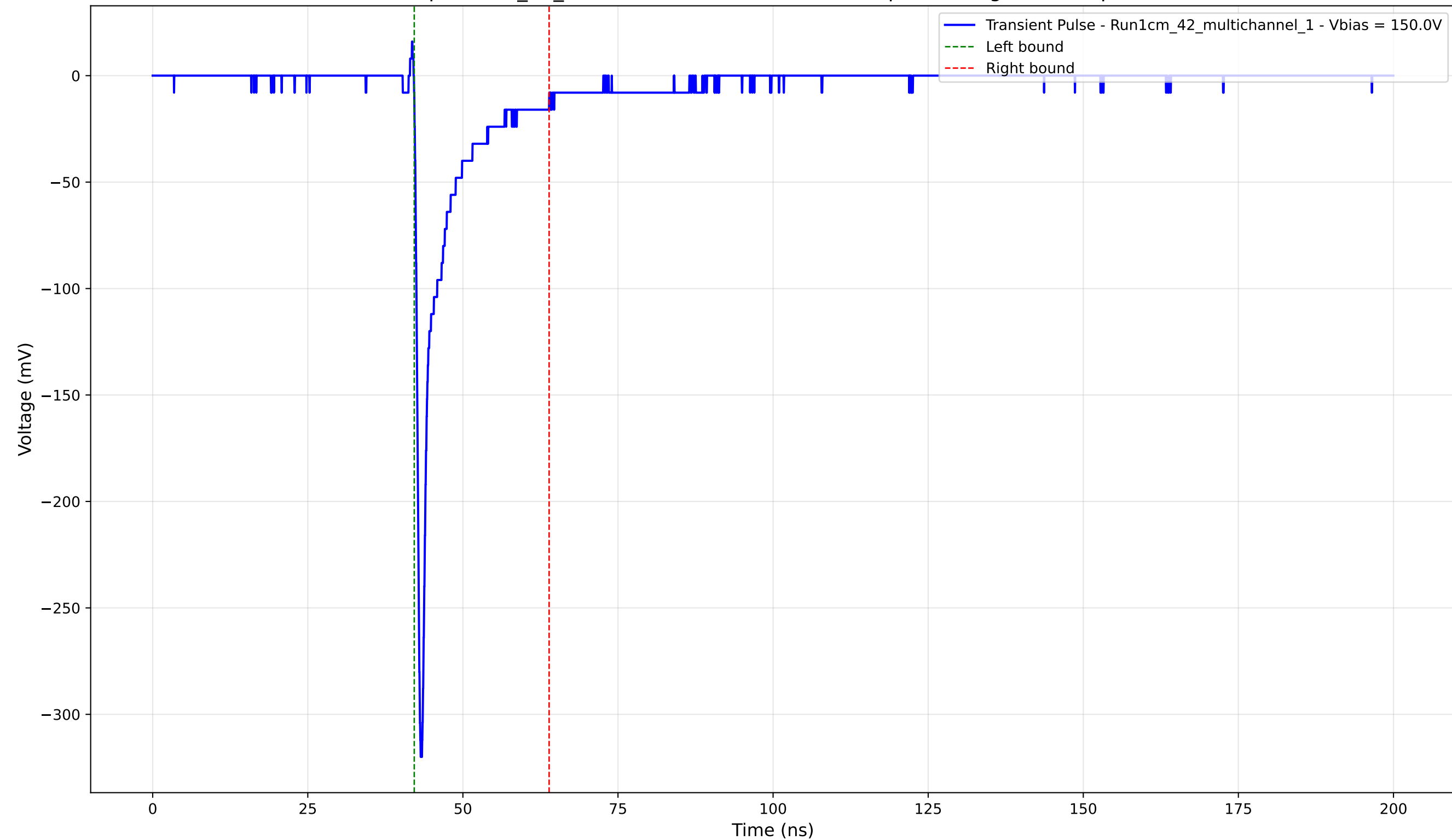
Transient Pulse - Sample: 1cm_42_multichannel - Position: 2135.0 \mu\text{m} - Charge: -24.37 pC - Rise Time: 0.76 ns
