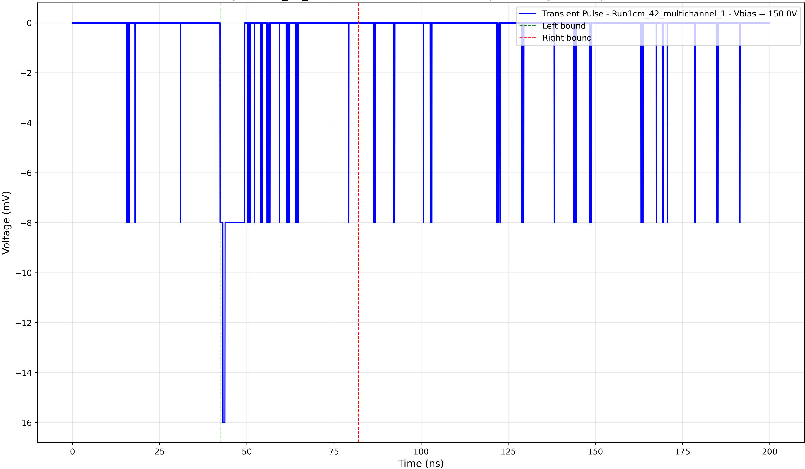
Transient Pulse - Sample: 1cm_42_multichannel - Position: 1895.0 \mu\text{m} - Charge: -1.50 pC - Rise Time: 0.82 ns
