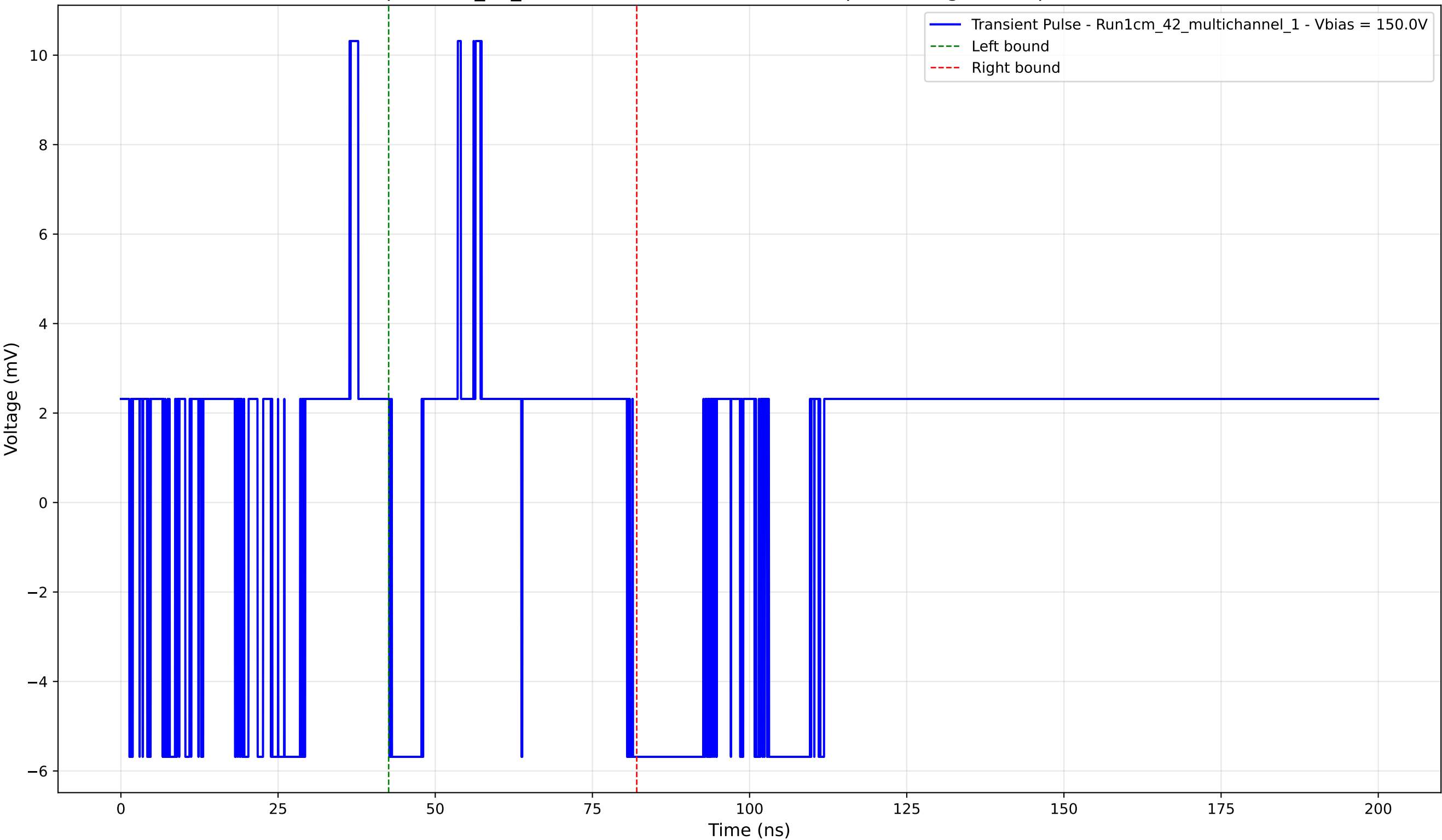
Transient Pulse - Sample: 1cm_42_multichannel - Position: 4420.0 \mu\text{m} - Charge: 0.98 pC - Rise Time: 0.00 ns (N/A)
