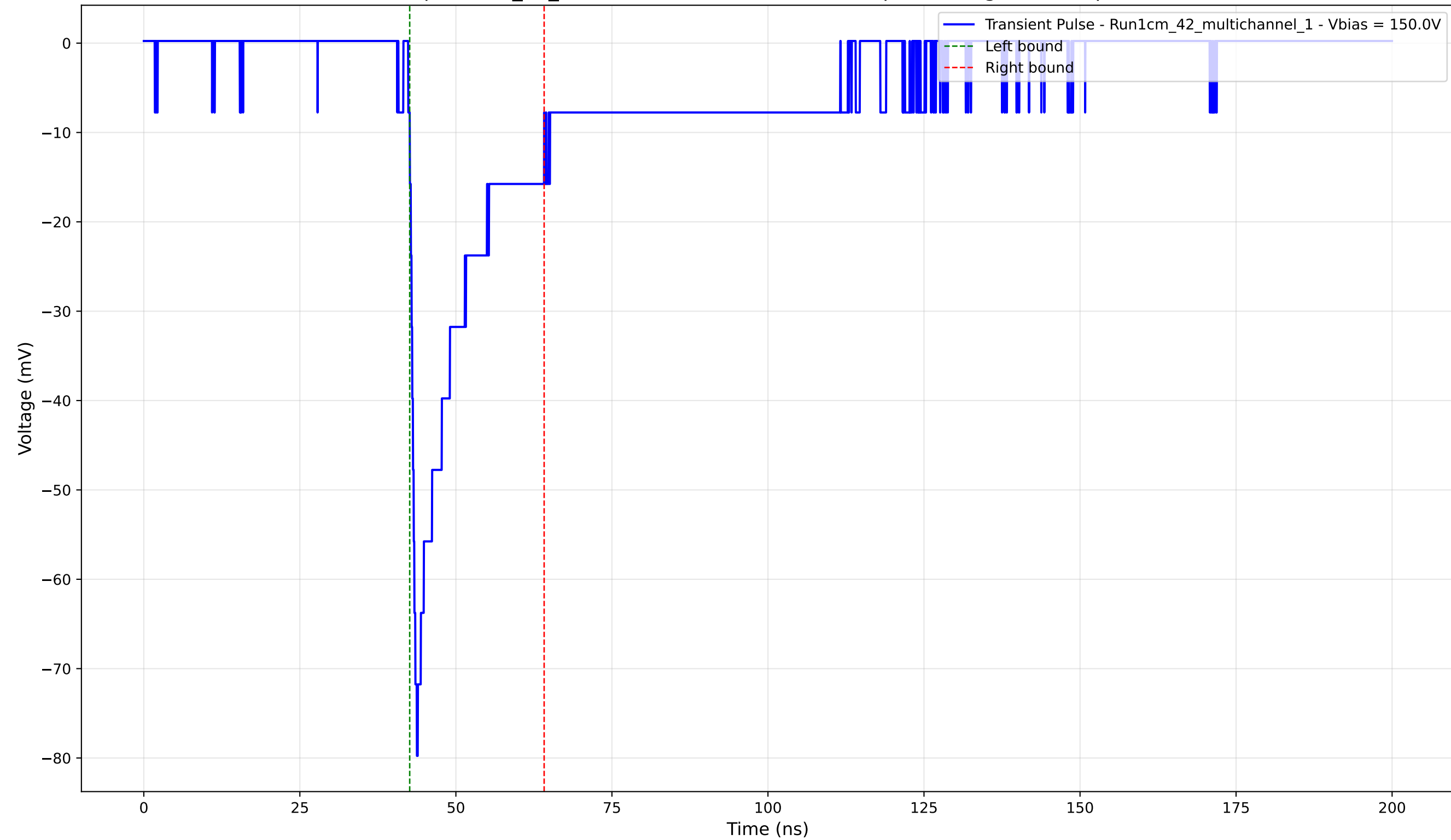
Transient Pulse - Sample: 1cm_42_multichannel - Position: 3335.0 \mu\text{m} - Charge: -12.74 pC - Rise Time: 1.14 ns
