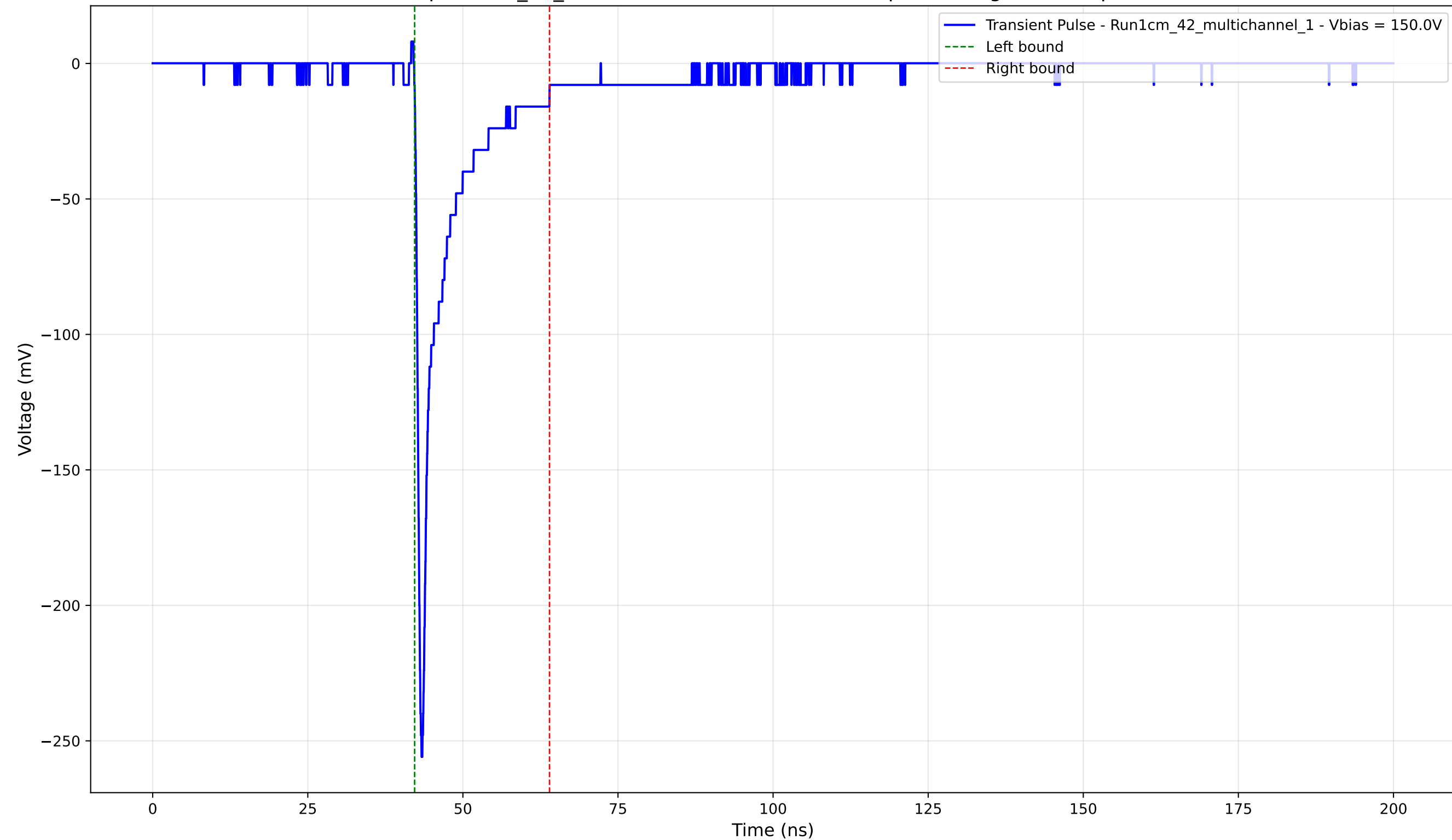
Transient Pulse - Sample: 1cm_42_multichannel - Position: 2755.0 \mu\text{m} - Charge: -22.38 pC - Rise Time: 0.80 ns
