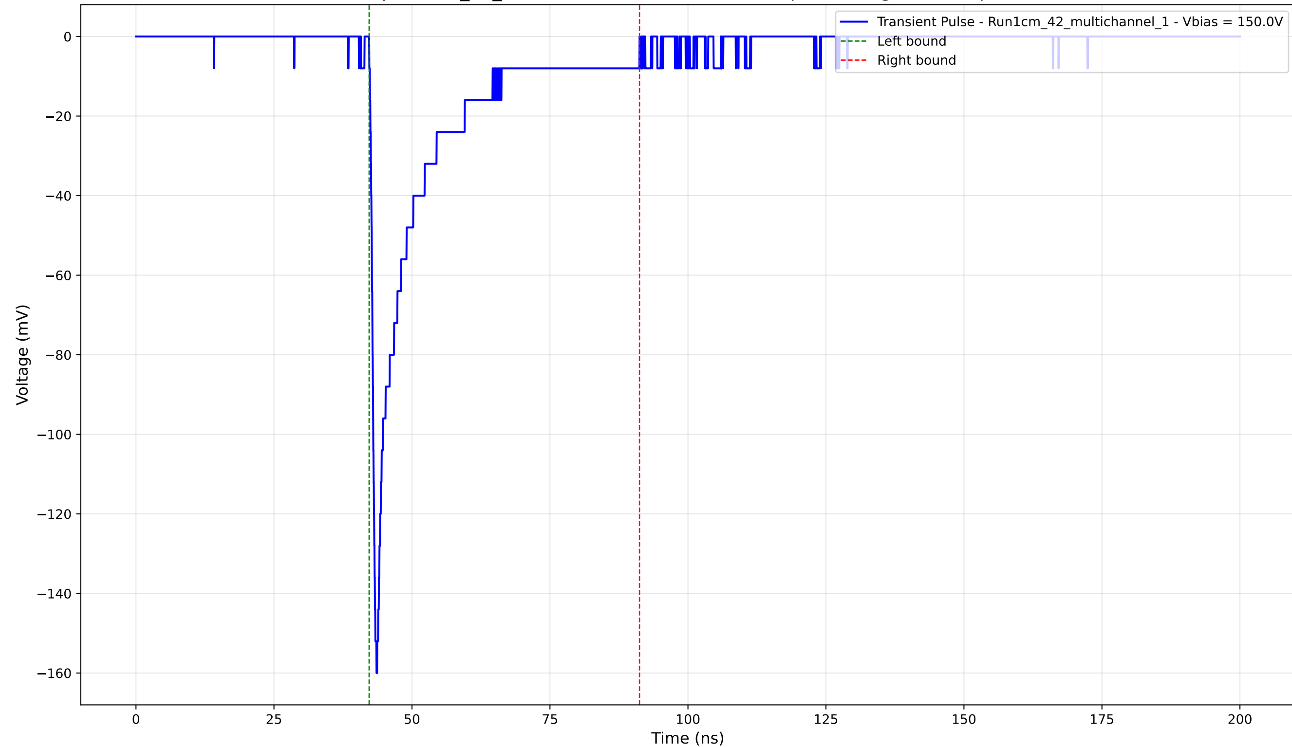
Transient Pulse - Sample: 1cm_42_multichannel - Position: 3040.0 \mu\text{m} - Charge: -24.20 pC - Rise Time: 0.84 ns
