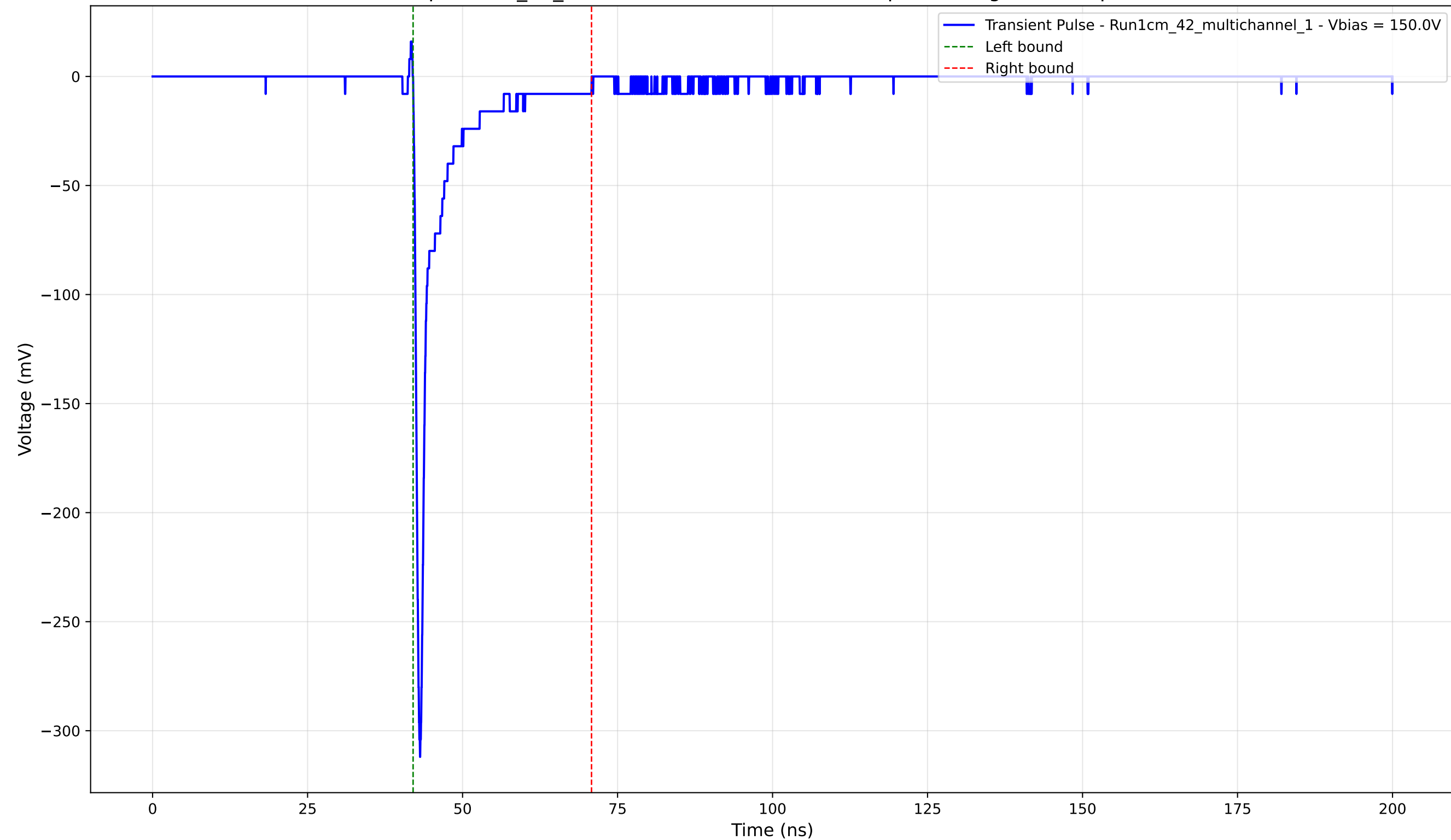
Transient Pulse - Sample: 1cm_42_multichannel - Position: 2325.0 \mu\text{m} - Charge: -19.57 pC - Rise Time: 0.78 ns
