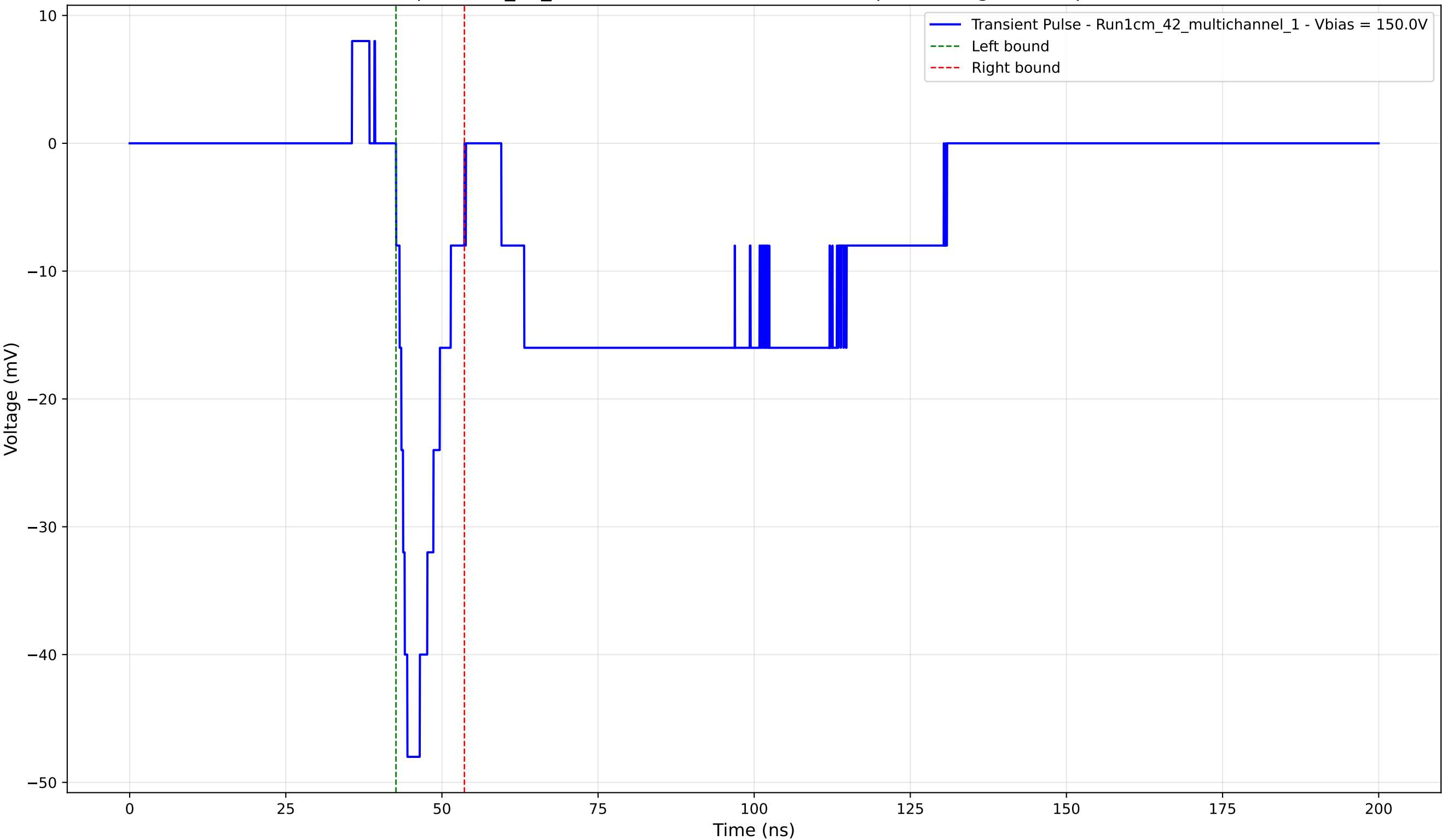
Transient Pulse - Sample: 1cm_42_multichannel - Position: 4150.0 \mu\text{m} - Charge: -5.72 pC - Rise Time: 1.81 ns
