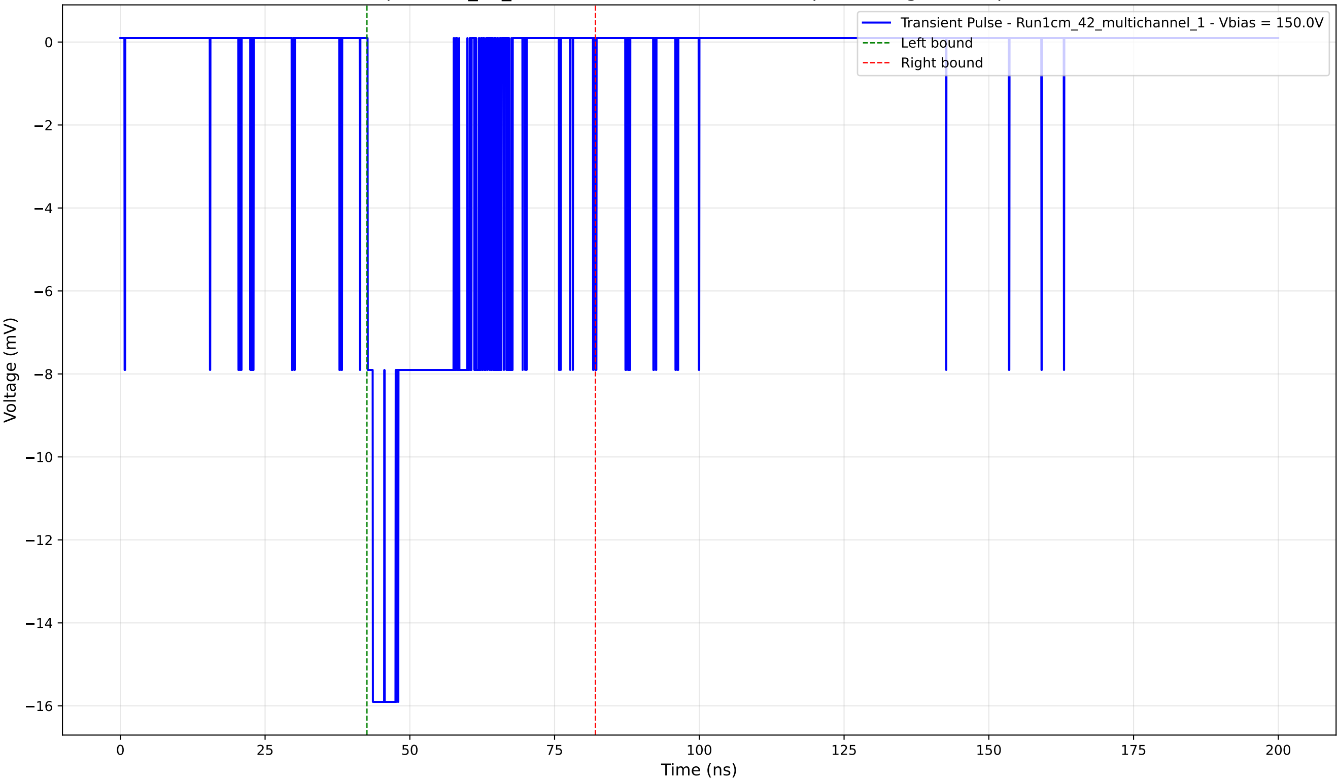
Transient Pulse - Sample: 1cm_42_multichannel - Position: 1345.0 \mu\text{m} - Charge: -3.95 pC - Rise Time: 0.90 ns
