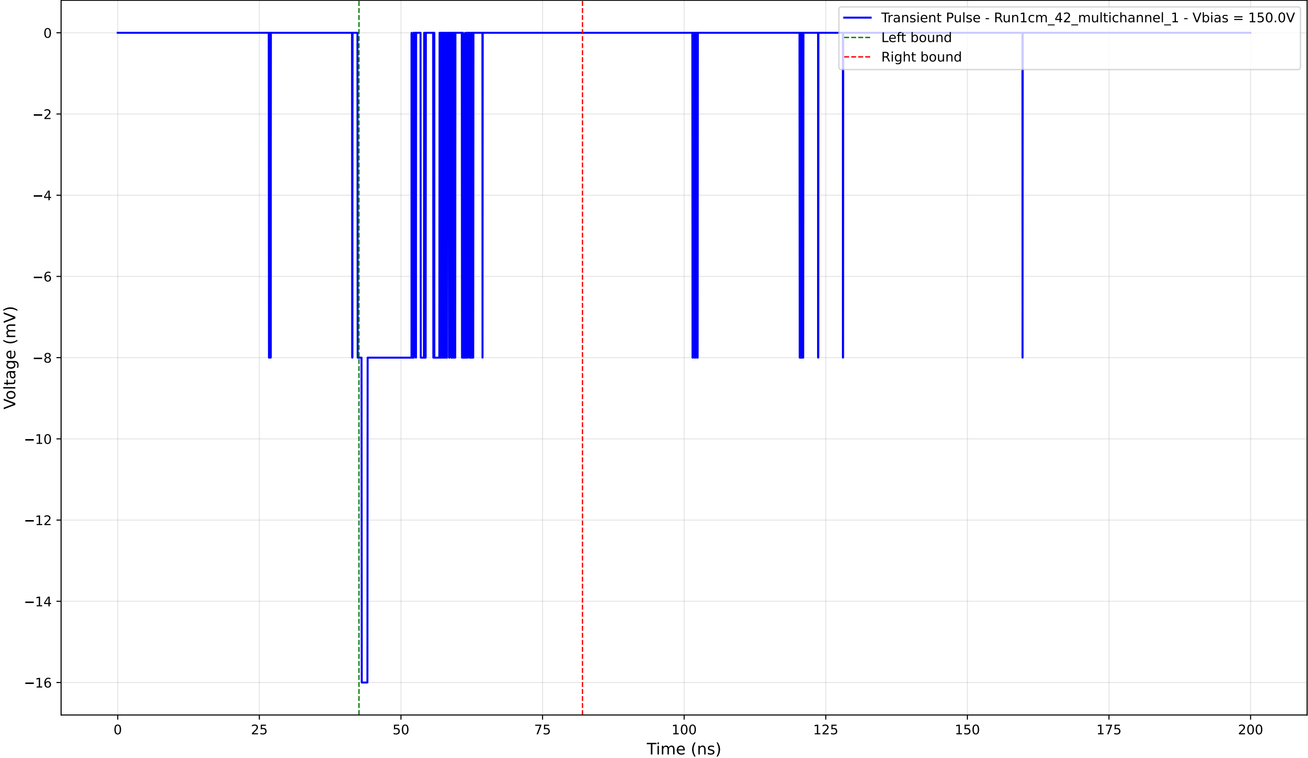
Transient Pulse - Sample: 1cm_42_multichannel - Position: 2915.0 \mu\text{m} - Charge: -2.36 pC - Rise Time: 0.74 ns
