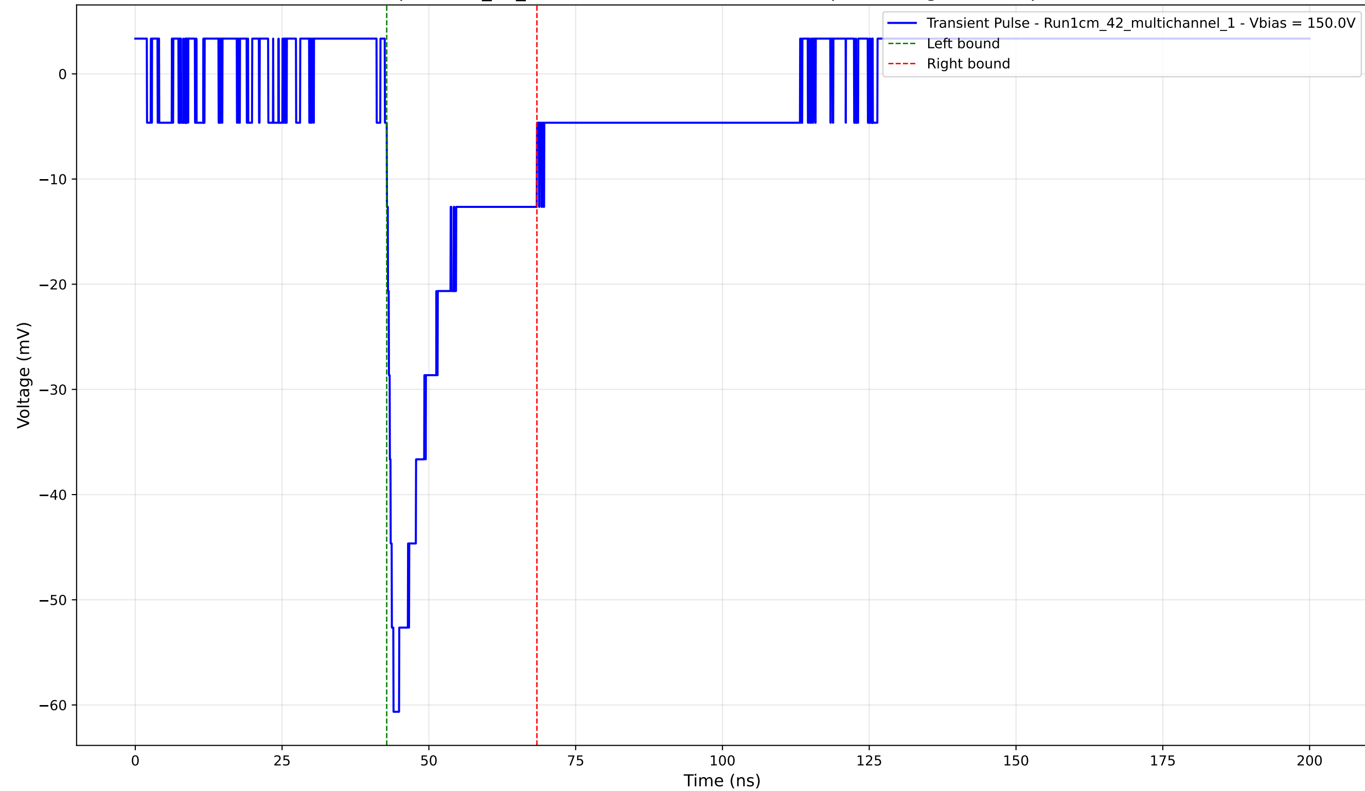
Transient Pulse - Sample: 1cm_42_multichannel - Position: 3660.0 \mu\text{m} - Charge: -11.87 pC - Rise Time: 1.14 ns
