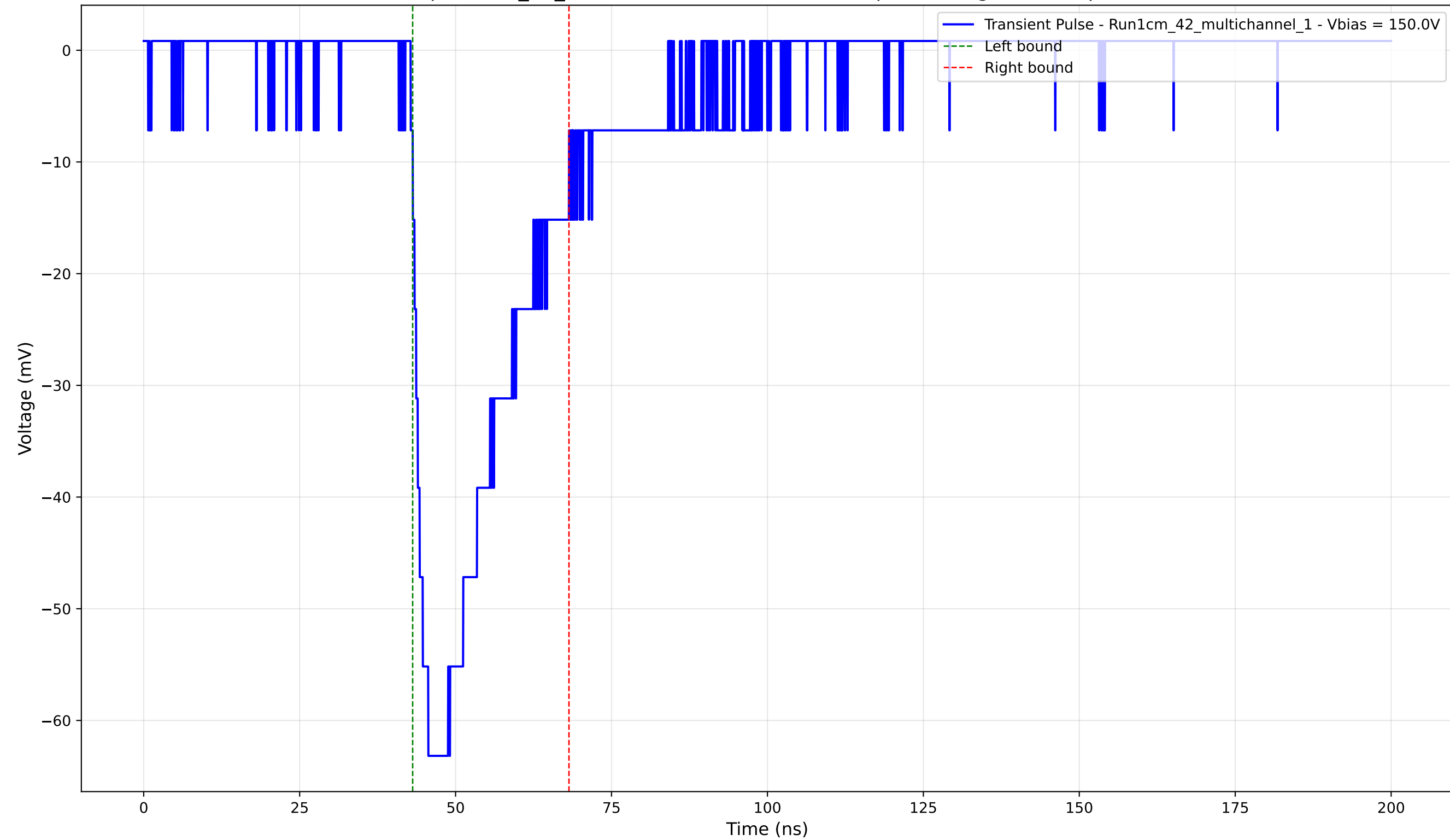
Transient Pulse - Sample: 1cm_42_multichannel - Position: 430.0 \mu\text{m} - Charge: -18.18 pC - Rise Time: 2.82 ns
