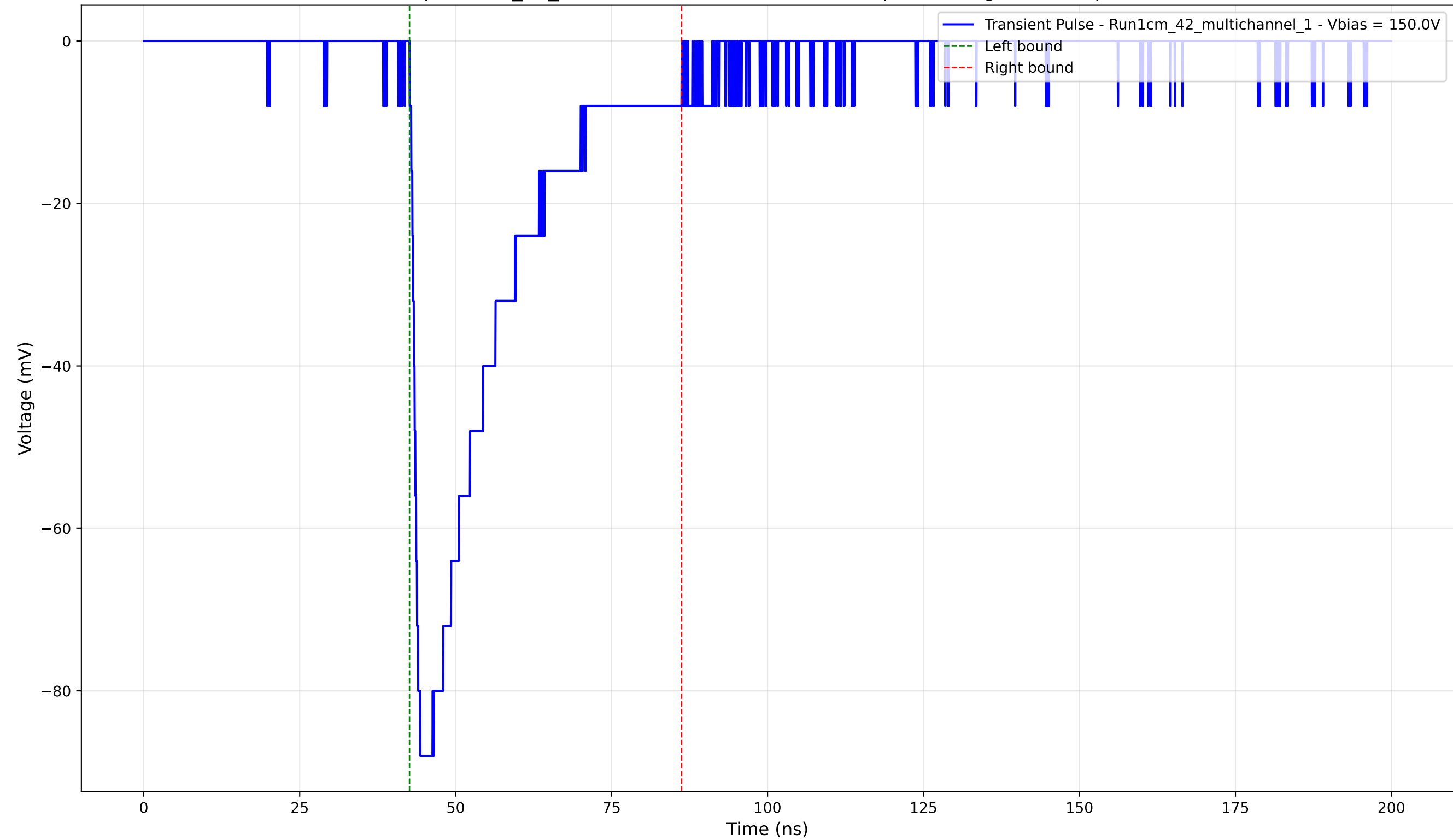
Transient Pulse - Sample: 1cm_42_multichannel - Position: 1085.0 \mu\text{m} - Charge: -25.51 pC - Rise Time: 1.12 ns
