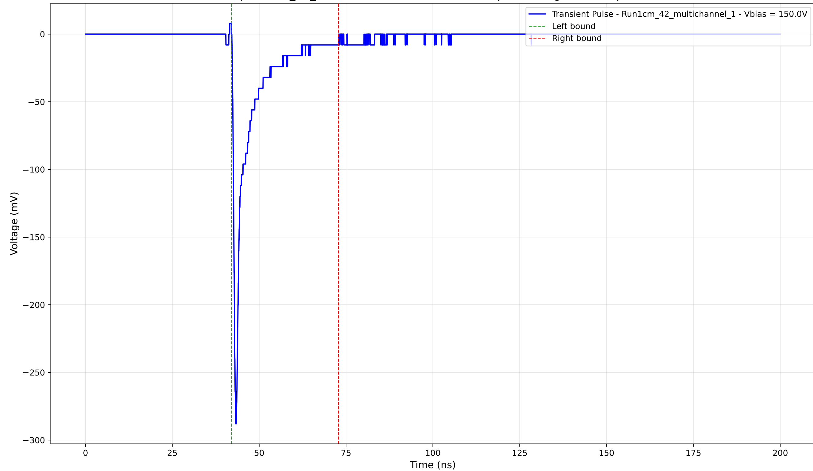
Transient Pulse - Sample: 1cm_42_multichannel - Position: 2690.0 \mu\text{m} - Charge: -24.02 pC - Rise Time: 0.79 ns
