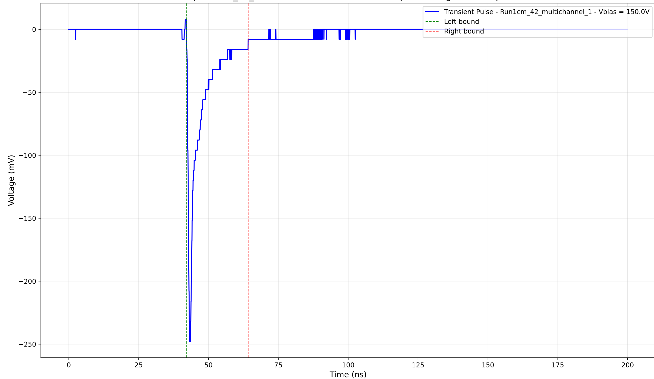
Transient Pulse - Sample: 1cm_42_multichannel - Position: 2760.0 \mu\text{m} - Charge: -22.18 pC - Rise Time: 0.74 ns
