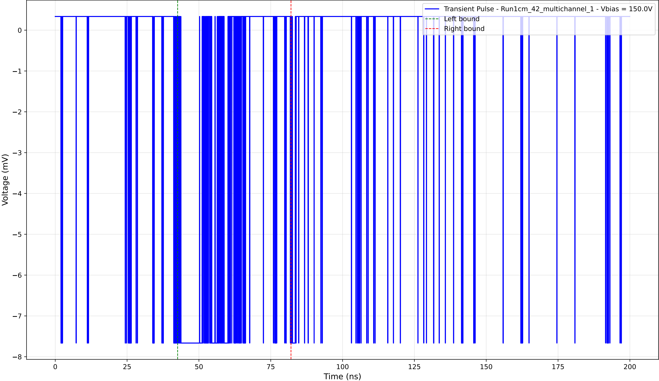
Transient Pulse - Sample: 1cm_42_multichannel - Position: 870.0 \mu\text{m} - Charge: -2.25 pC - Rise Time: 0.02 ns
