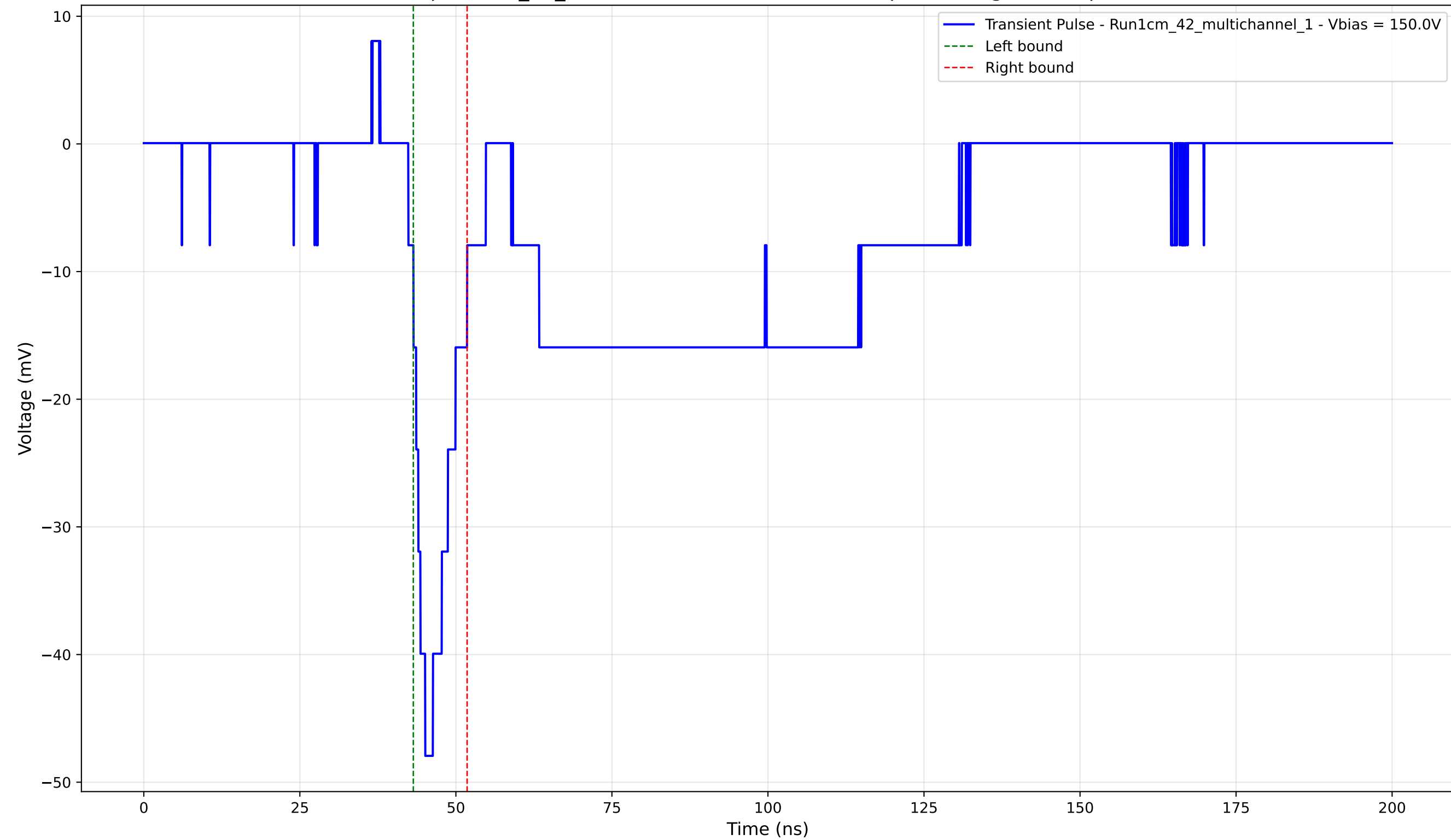
Transient Pulse - Sample: 1cm_42_multichannel - Position: 4490.0 \mu\text{m} - Charge: -5.26 pC - Rise Time: 2.71 ns
