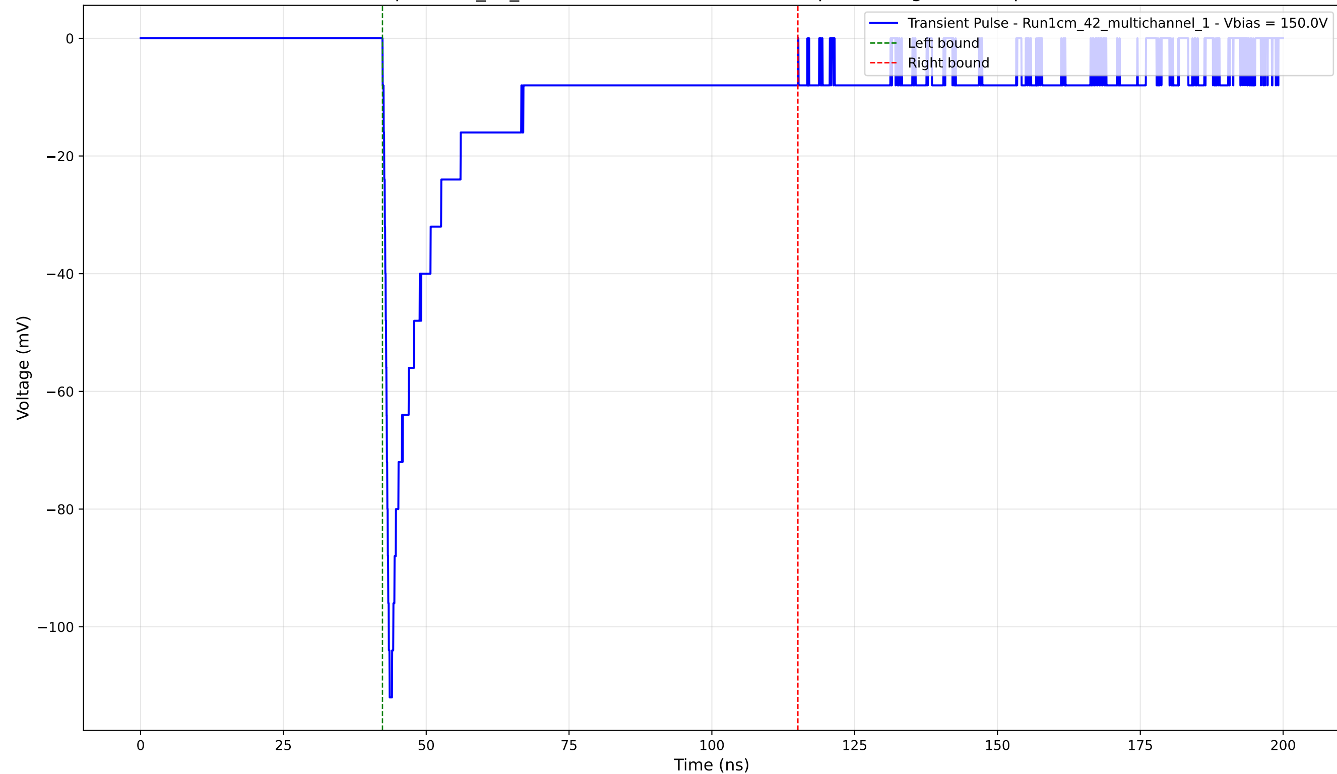
Transient Pulse - Sample: 1cm_42_multichannel - Position: 3235.0 \mu\text{m} - Charge: -24.24 pC - Rise Time: 0.91 ns
