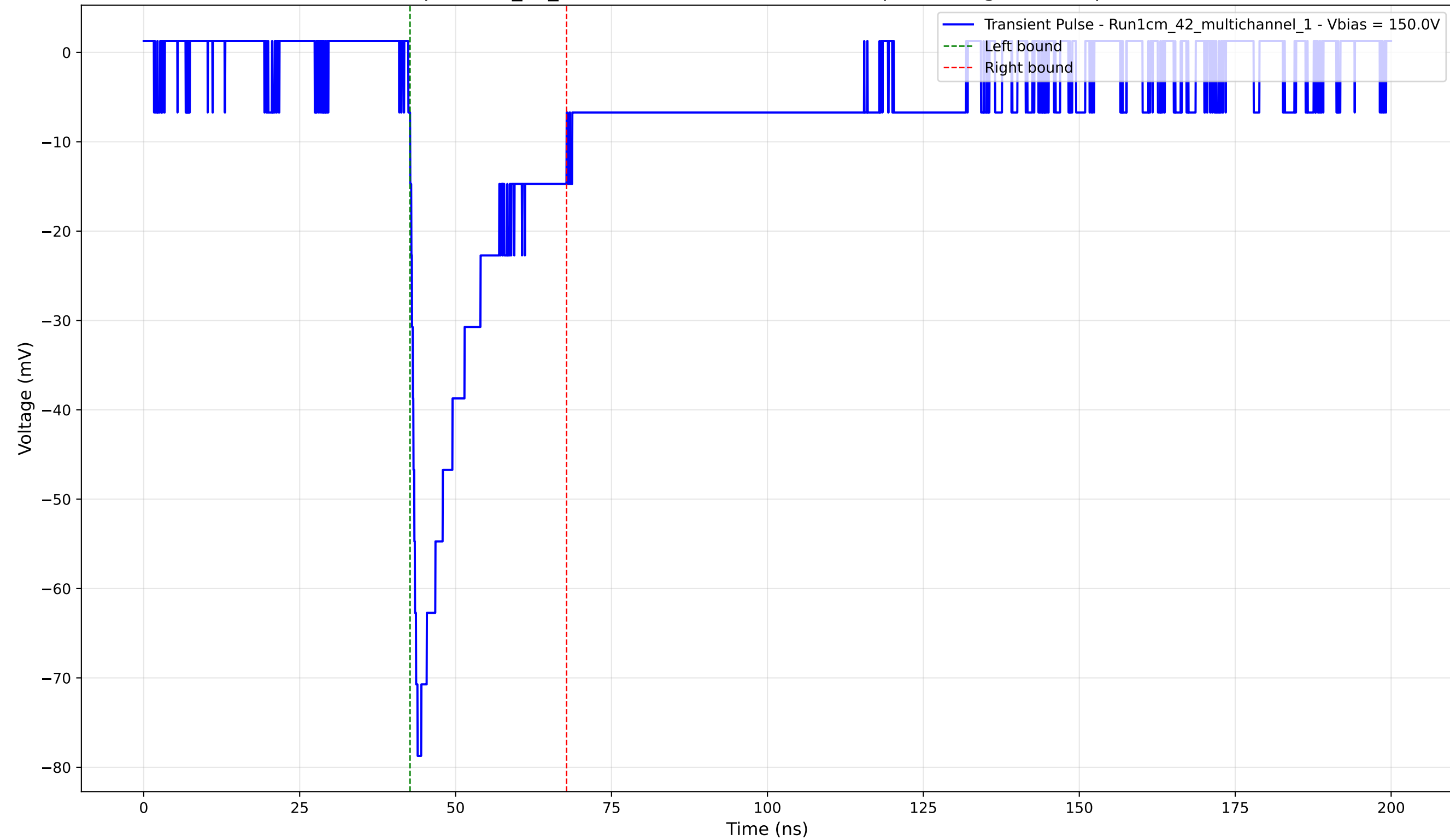
Transient Pulse - Sample: 1cm_42_multichannel - Position: 3530.0 \mu\text{m} - Charge: -15.57 pC - Rise Time: 1.20 ns
