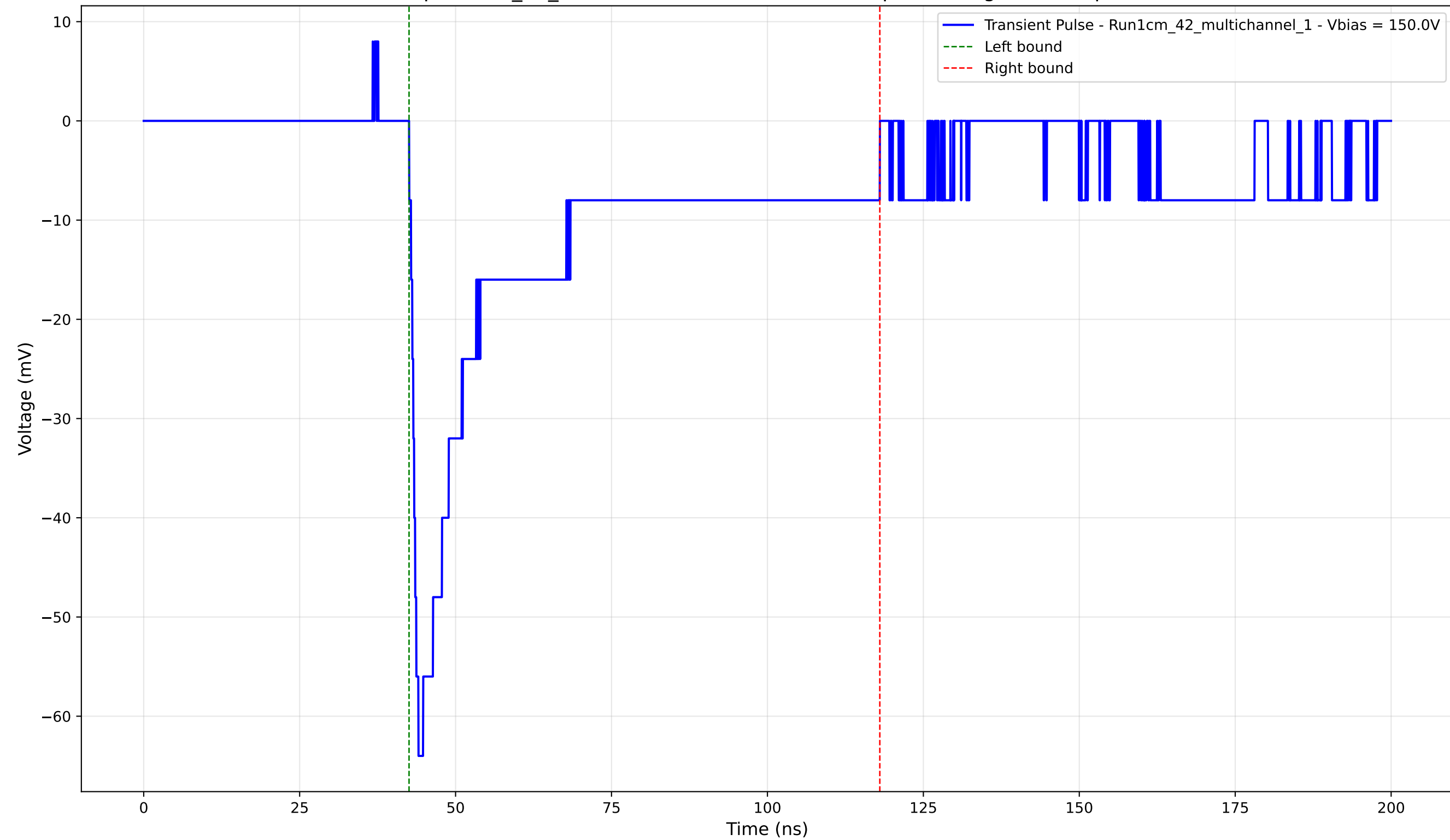
Transient Pulse - Sample: 1cm_42_multichannel - Position: 3665.0 \mu\text{m} - Charge: -21.15 pC - Rise Time: 1.48 ns
