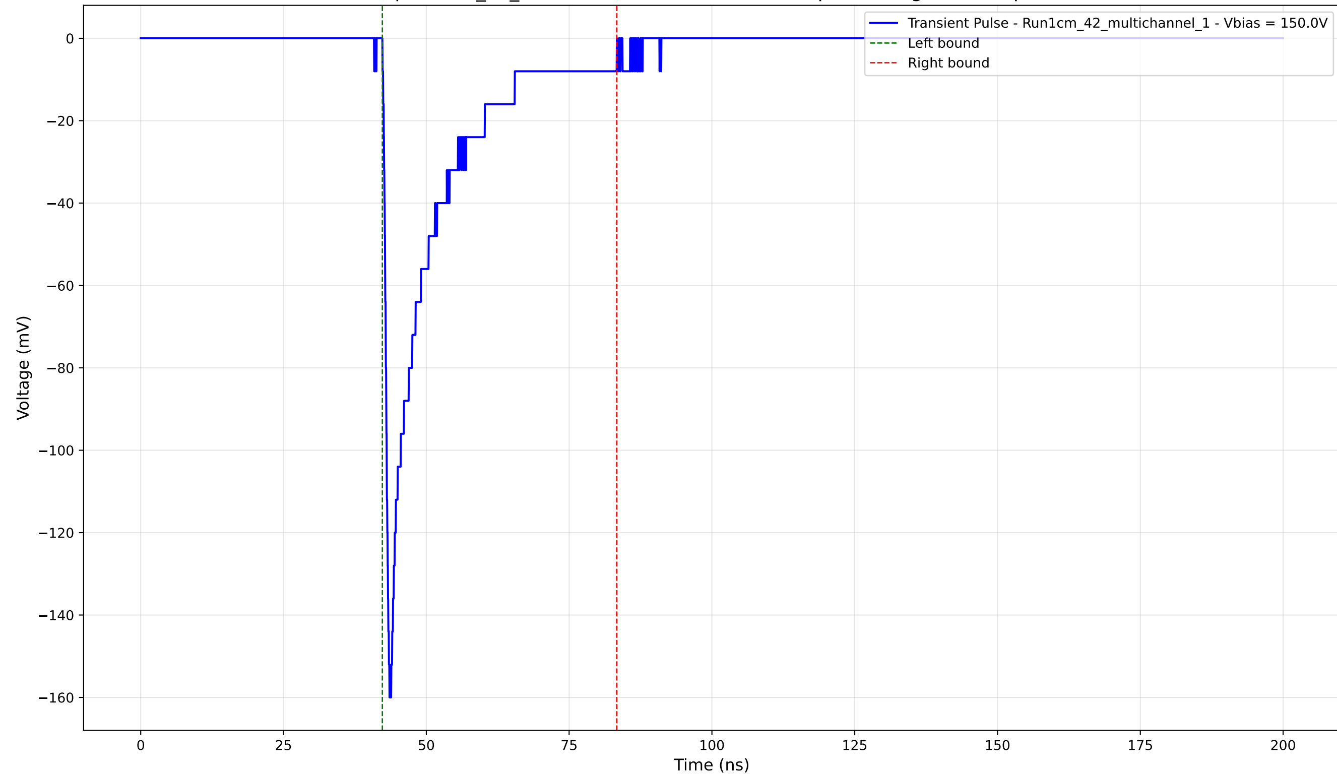
Transient Pulse - Sample: 1cm_42_multichannel - Position: 1680.0 \mu\text{m} - Charge: -24.96 pC - Rise Time: 0.82 ns
