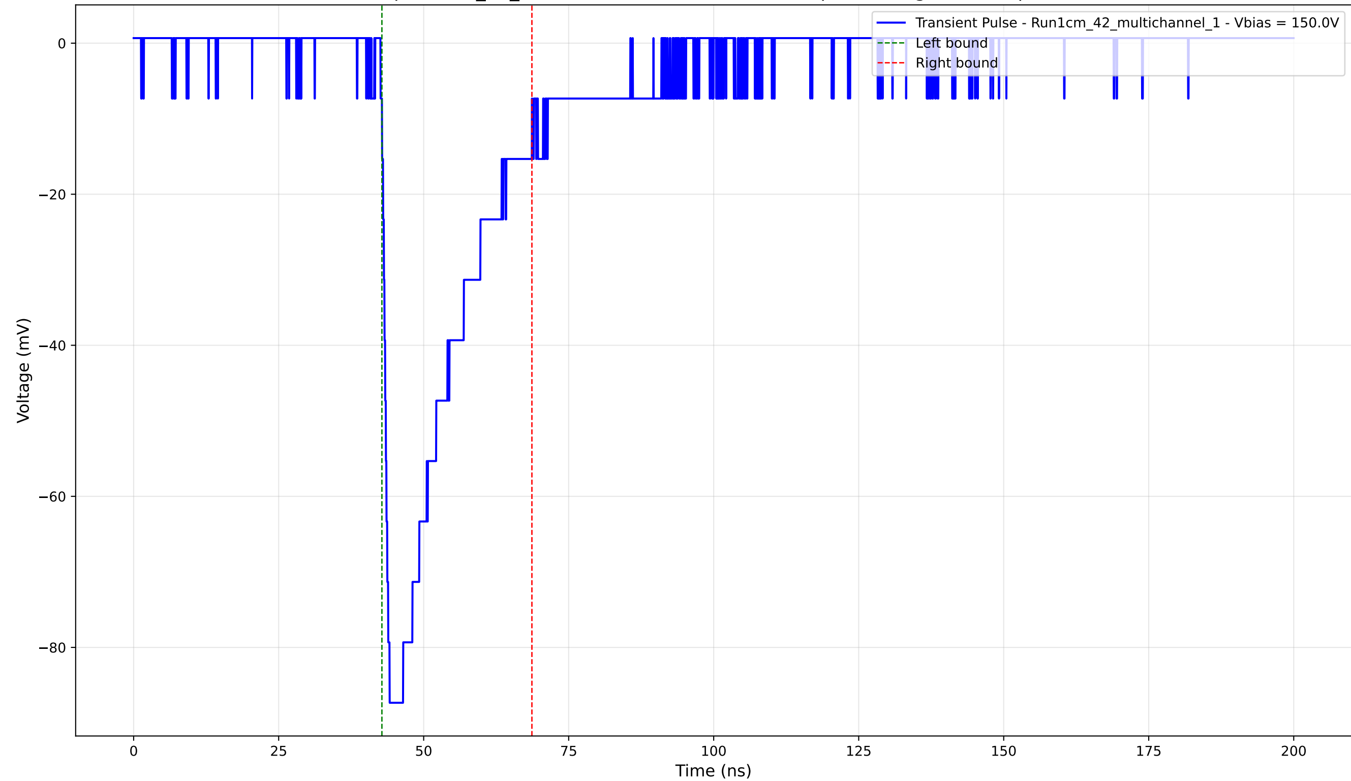
Transient Pulse - Sample: 1cm_42_multichannel - Position: 1120.0 \mu\text{m} - Charge: -22.28 pC - Rise Time: 1.08 ns
