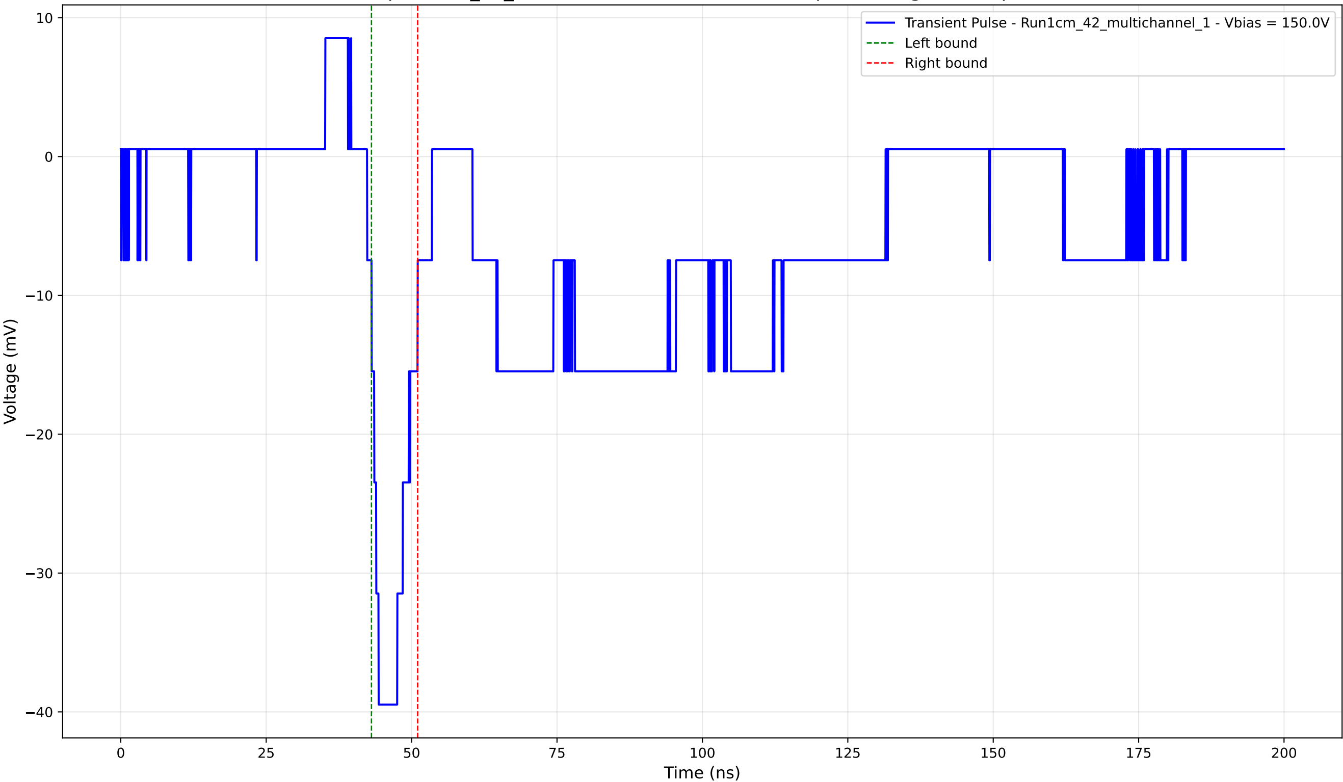
Transient Pulse - Sample: 1cm_42_multichannel - Position: 4740.0 \mu\text{m} - Charge: -4.66 pC - Rise Time: 1.97 ns
