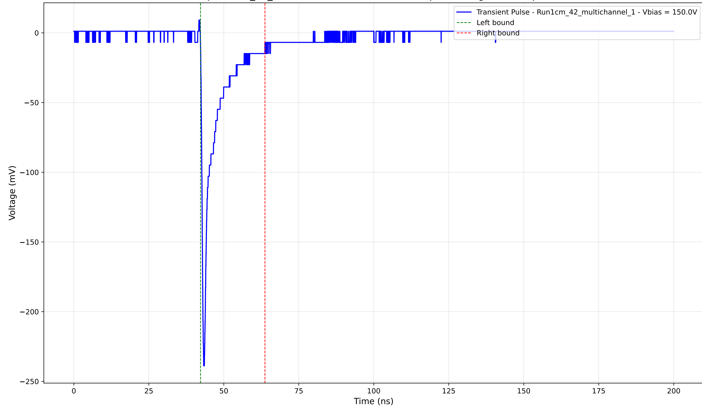
Transient Pulse - Sample: 1cm_42_multichannel - Position: 2775.0 \mu\text{m} - Charge: -21.22 pC - Rise Time: 0.82 ns
