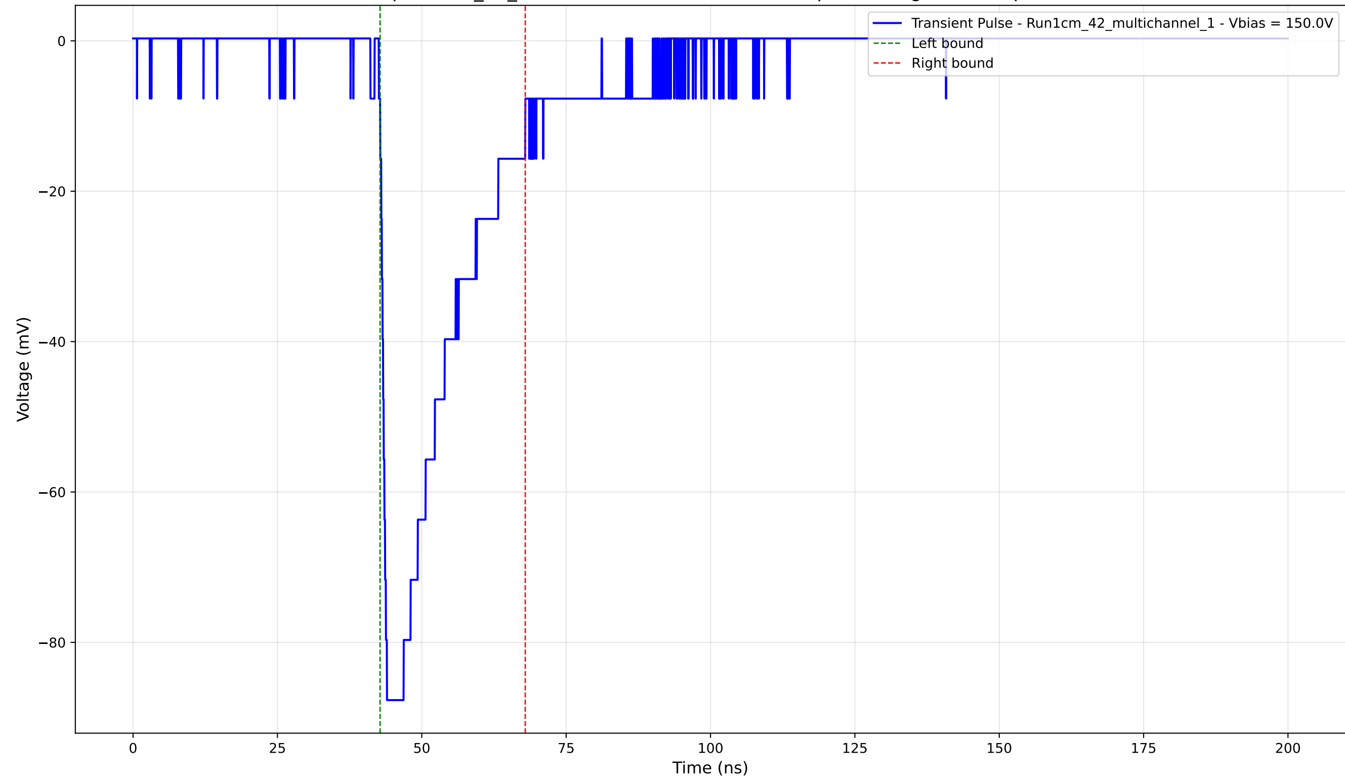
Transient Pulse - Sample: 1cm_42_multichannel - Position: 1160.0 \mu\text{m} - Charge: -22.11 pC - Rise Time: 1.00 ns
