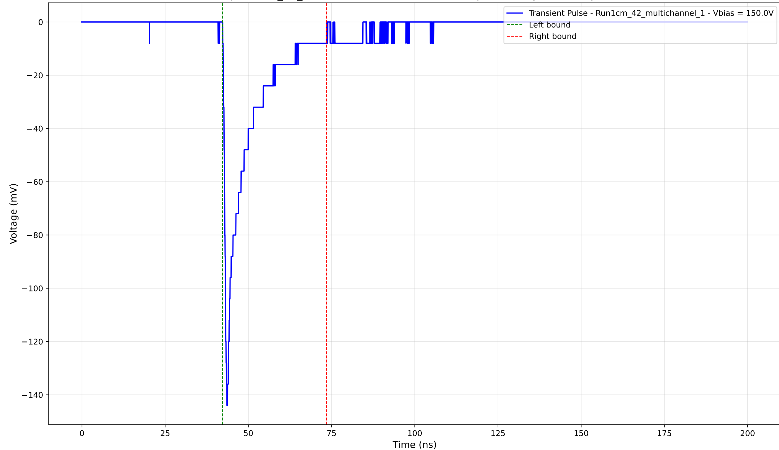
Transient Pulse - Sample: 1cm_42_multichannel - Position: 3075.0 \mu\text{m} - Charge: -19.81 pC - Rise Time: 0.98 ns
