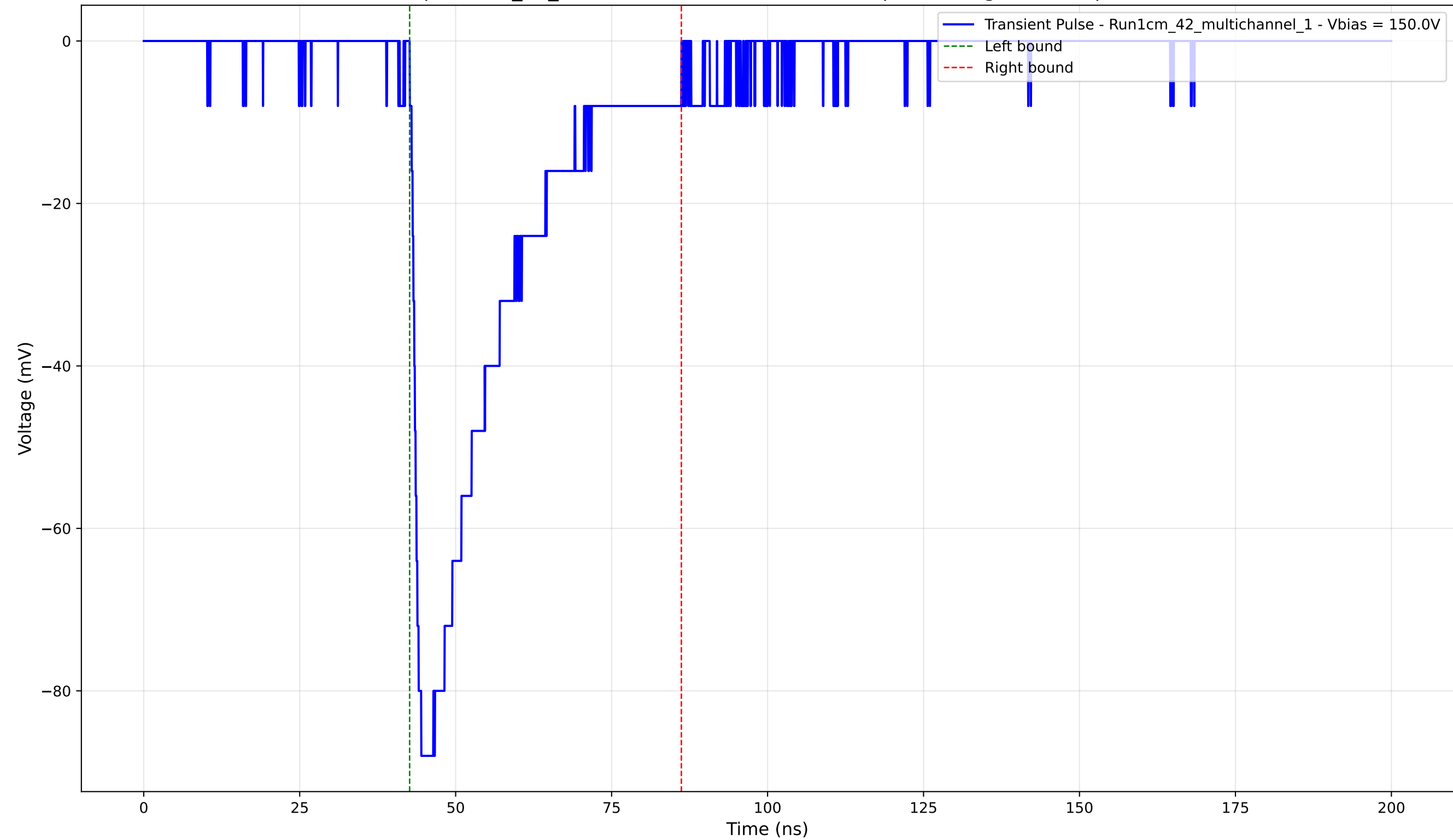
Transient Pulse - Sample: 1cm_42_multichannel - Position: 1035.0 \mu\text{m} - Charge: -25.97 pC - Rise Time: 1.14 ns
