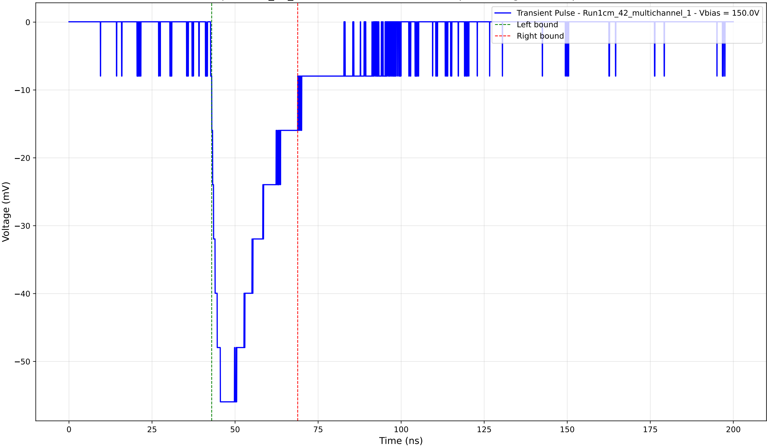
Transient Pulse - Sample: 1cm_42_multichannel - Position: 115.0 \mu\text{m} - Charge: -17.72 pC - Rise Time: 2.93 ns
