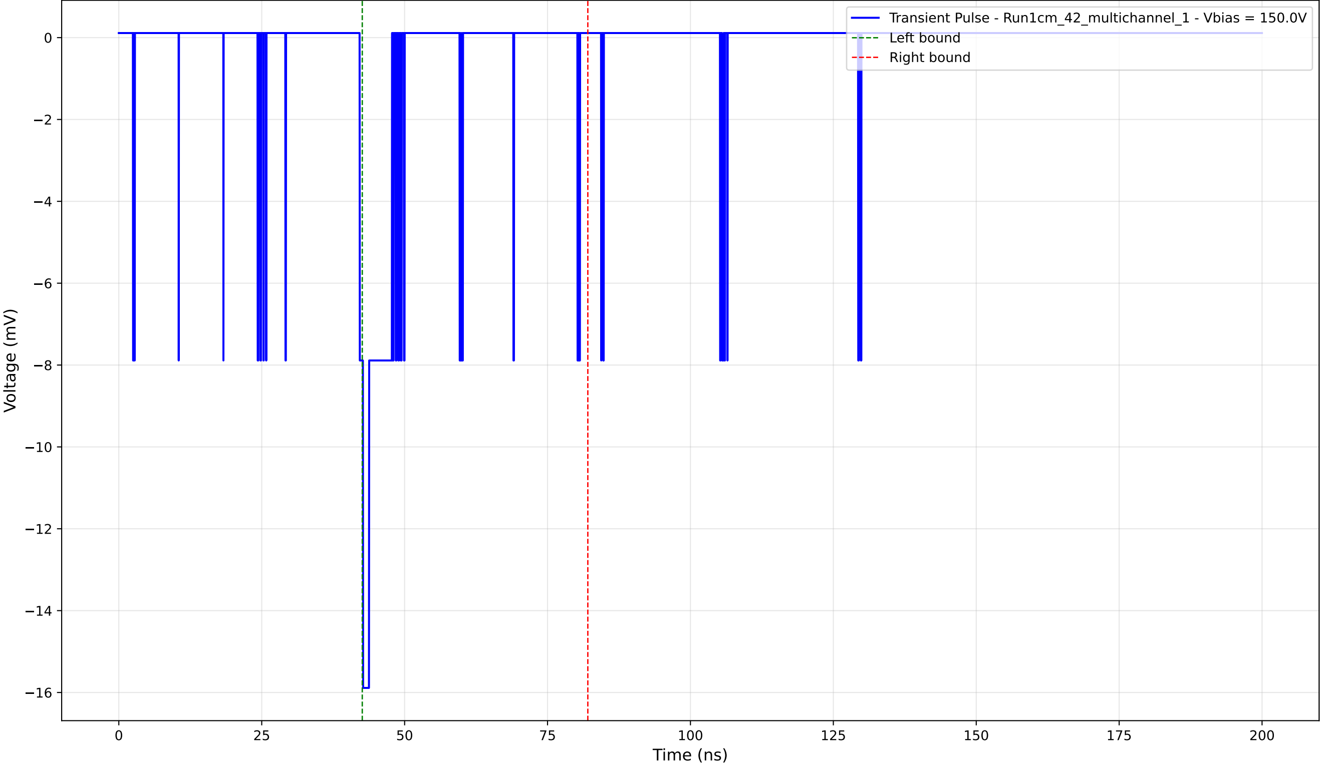
Transient Pulse - Sample: 1cm_42_multichannel - Position: 2385.0 \mu\text{m} - Charge: -1.17 pC - Rise Time: 0.60 ns
