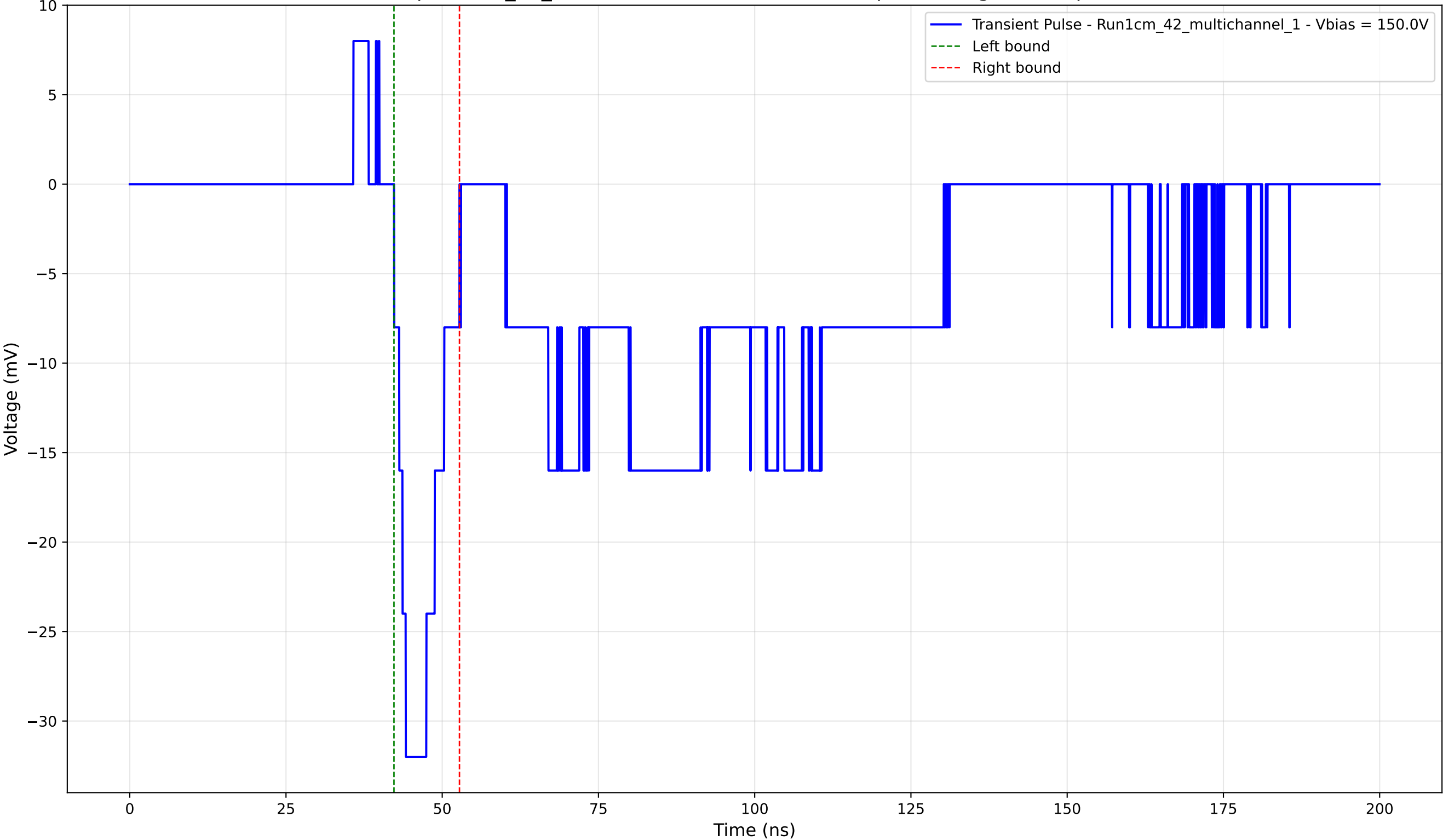
Transient Pulse - Sample: 1cm_42_multichannel - Position: 4835.0 \mu\text{m} - Charge: -4.18 pC - Rise Time: 1.87 ns
