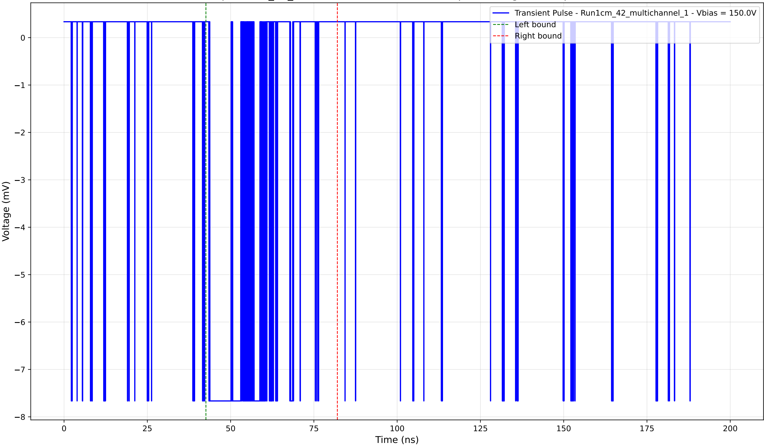
Transient Pulse - Sample: 1cm_42_multichannel - Position: 865.0 \mu\text{m} - Charge: -2.27 pC - Rise Time: 0.02 ns
