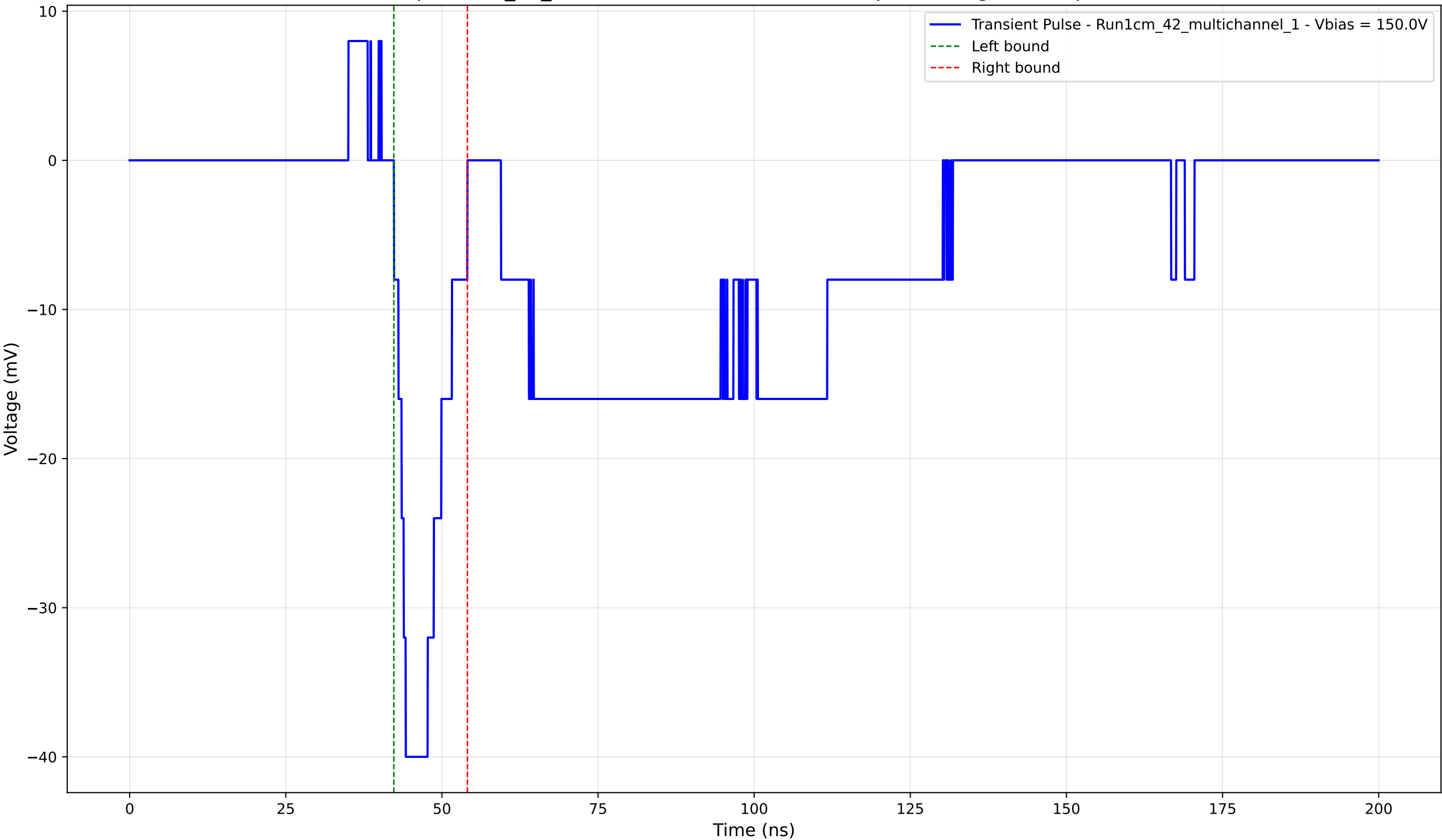
Transient Pulse - Sample: 1cm_42_multichannel - Position: 4680.0 \mu\text{m} - Charge: -5.60 pC - Rise Time: 1.89 ns
