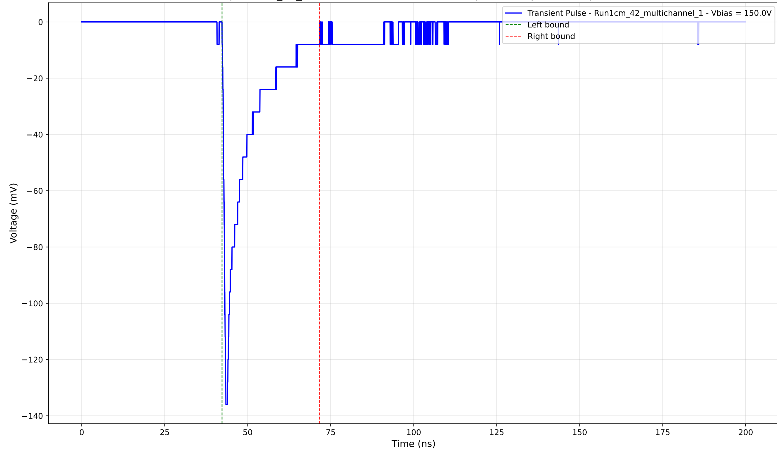
Transient Pulse - Sample: 1cm_42_multichannel - Position: 3080.0 \mu\text{m} - Charge: -19.35 pC - Rise Time: 0.91 ns
