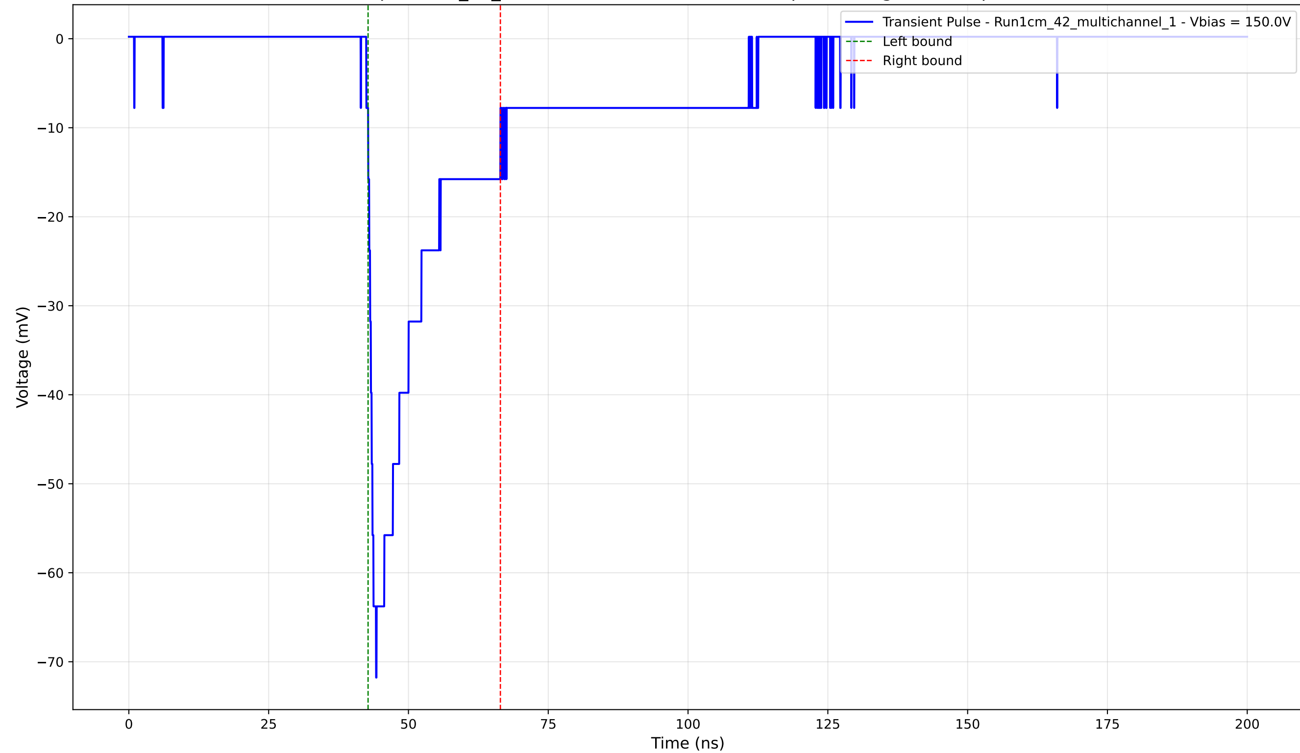
Transient Pulse - Sample: 1cm_42_multichannel - Position: 3620.0 \mu\text{m} - Charge: -13.72 pC - Rise Time: 1.74 ns
