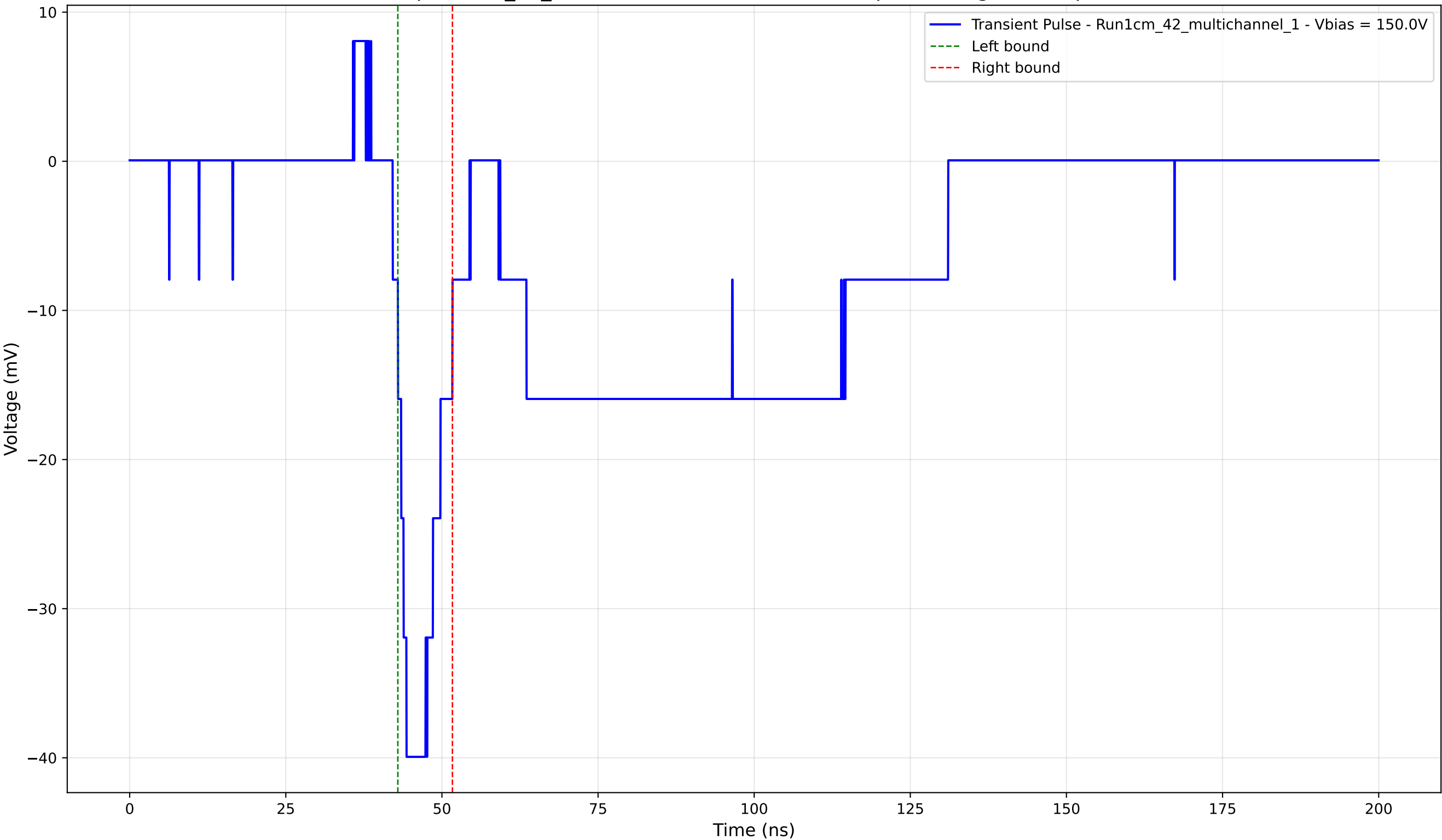
Transient Pulse - Sample: 1cm_42_multichannel - Position: 4785.0 \mu\text{m} - Charge: -5.03 pC - Rise Time: 2.21 ns
