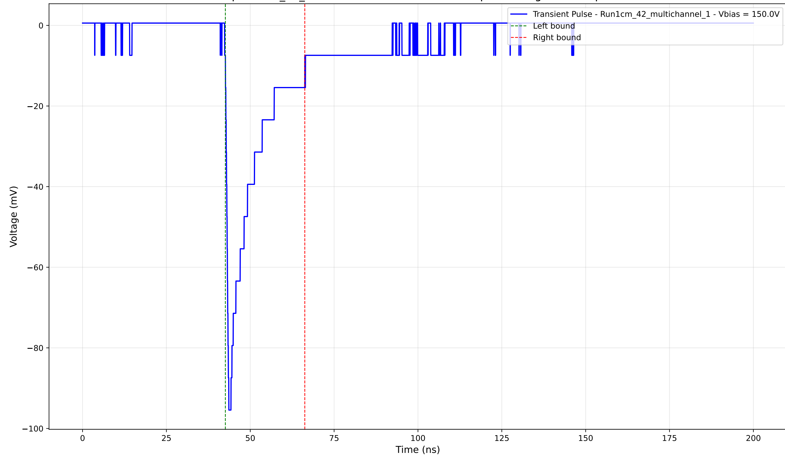
Transient Pulse - Sample: 1cm_42_multichannel - Position: 3310.0 \mu\text{m} - Charge: -15.99 pC - Rise Time: 0.87 ns
