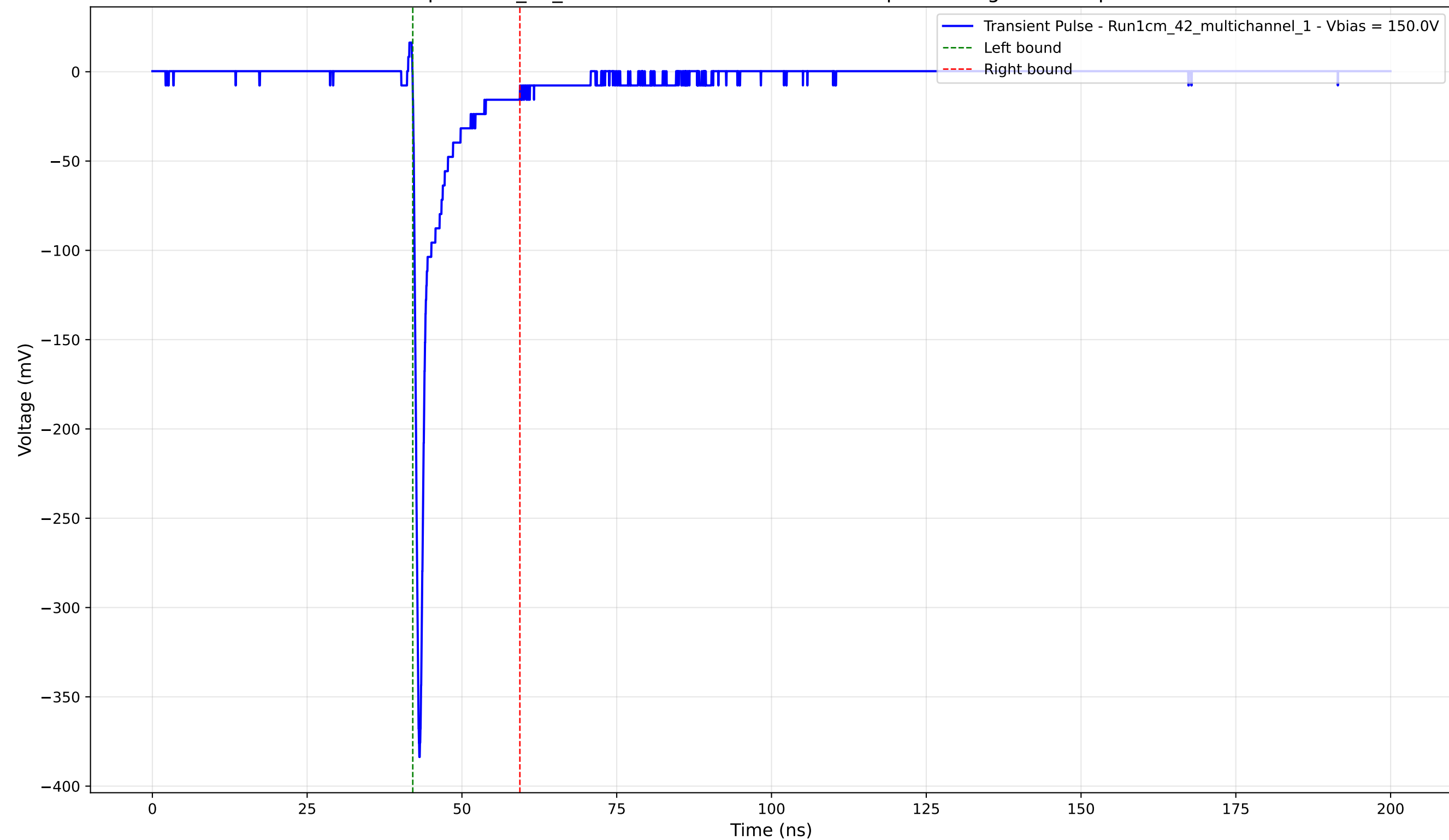
Transient Pulse - Sample: 1cm_42_multichannel - Position: 2310.0 \mu\text{m} - Charge: -21.73 pC - Rise Time: 0.75 ns
