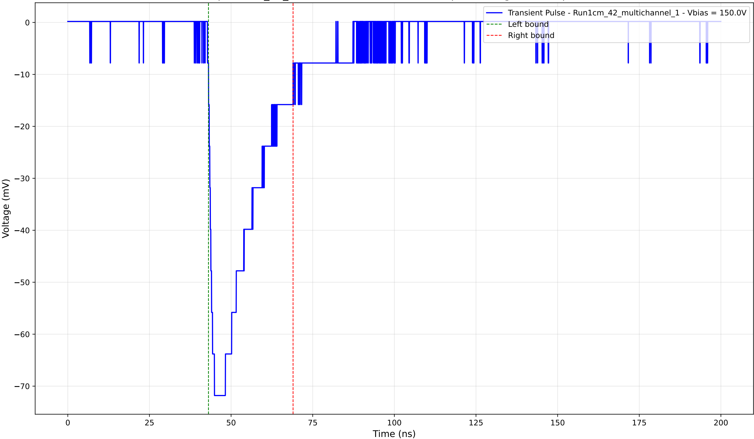
Transient Pulse - Sample: 1cm_42_multichannel - Position: 790.0 \mu\text{m} - Charge: -20.38 pC - Rise Time: 2.14 ns
