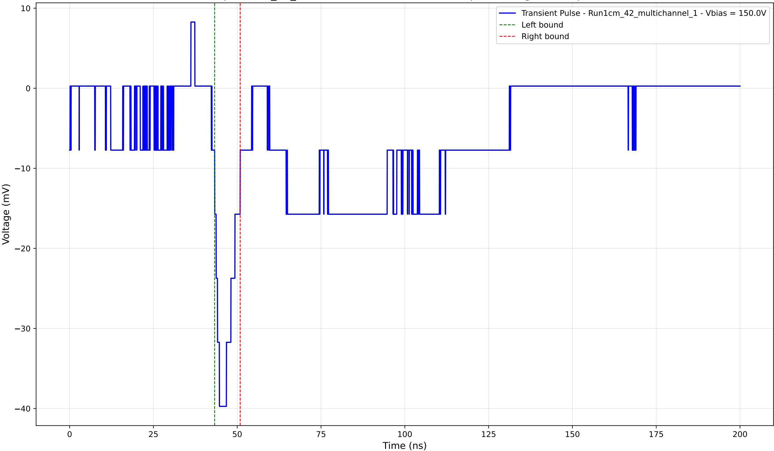
Transient Pulse - Sample: 1cm_42_multichannel - Position: 4340.0 \mu\text{m} - Charge: -4.27 pC - Rise Time: 2.23 ns
