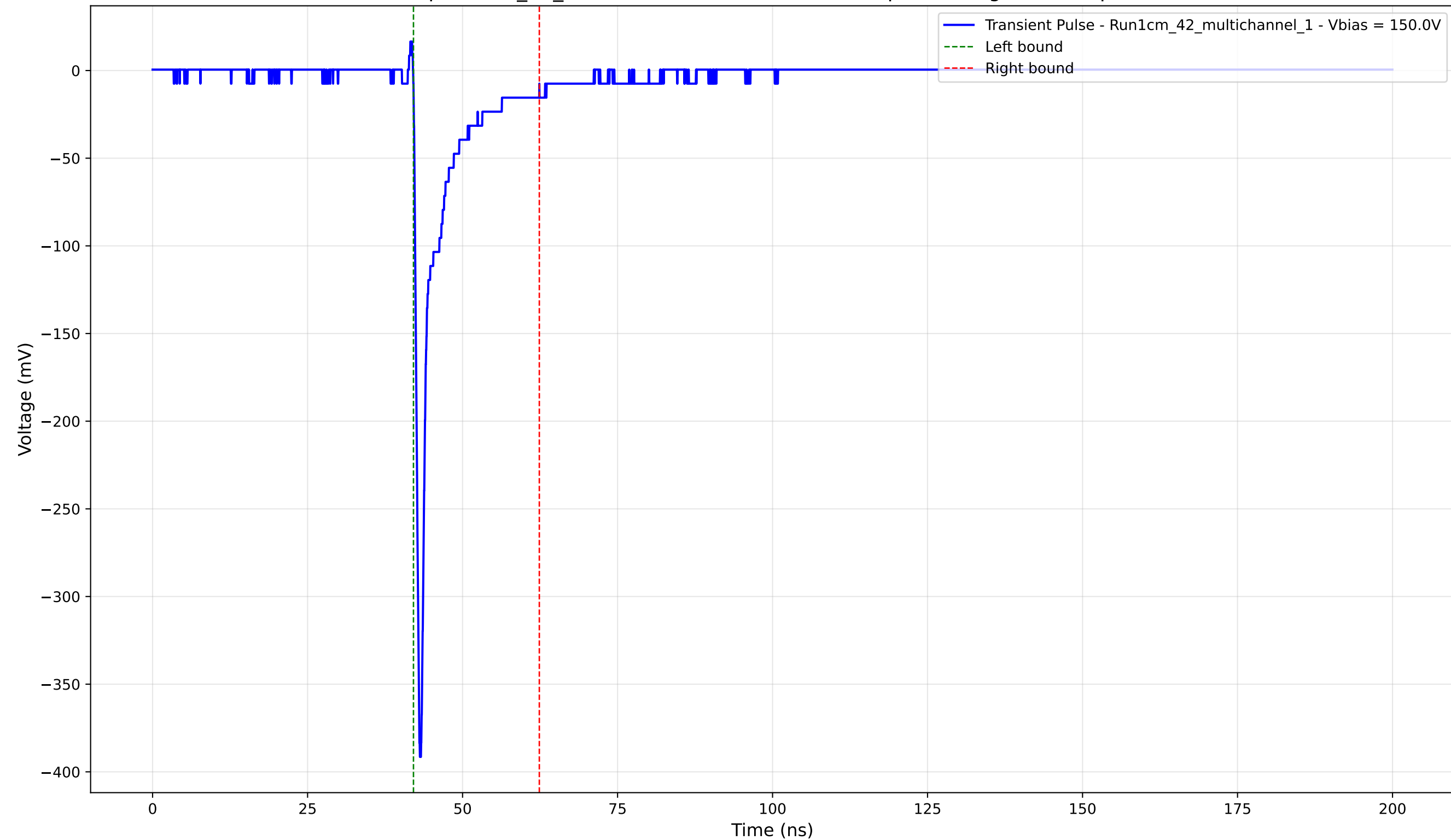
Transient Pulse - Sample: 1cm_42_multichannel - Position: 2260.0 \mu\text{m} - Charge: -24.99 pC - Rise Time: 0.74 ns
