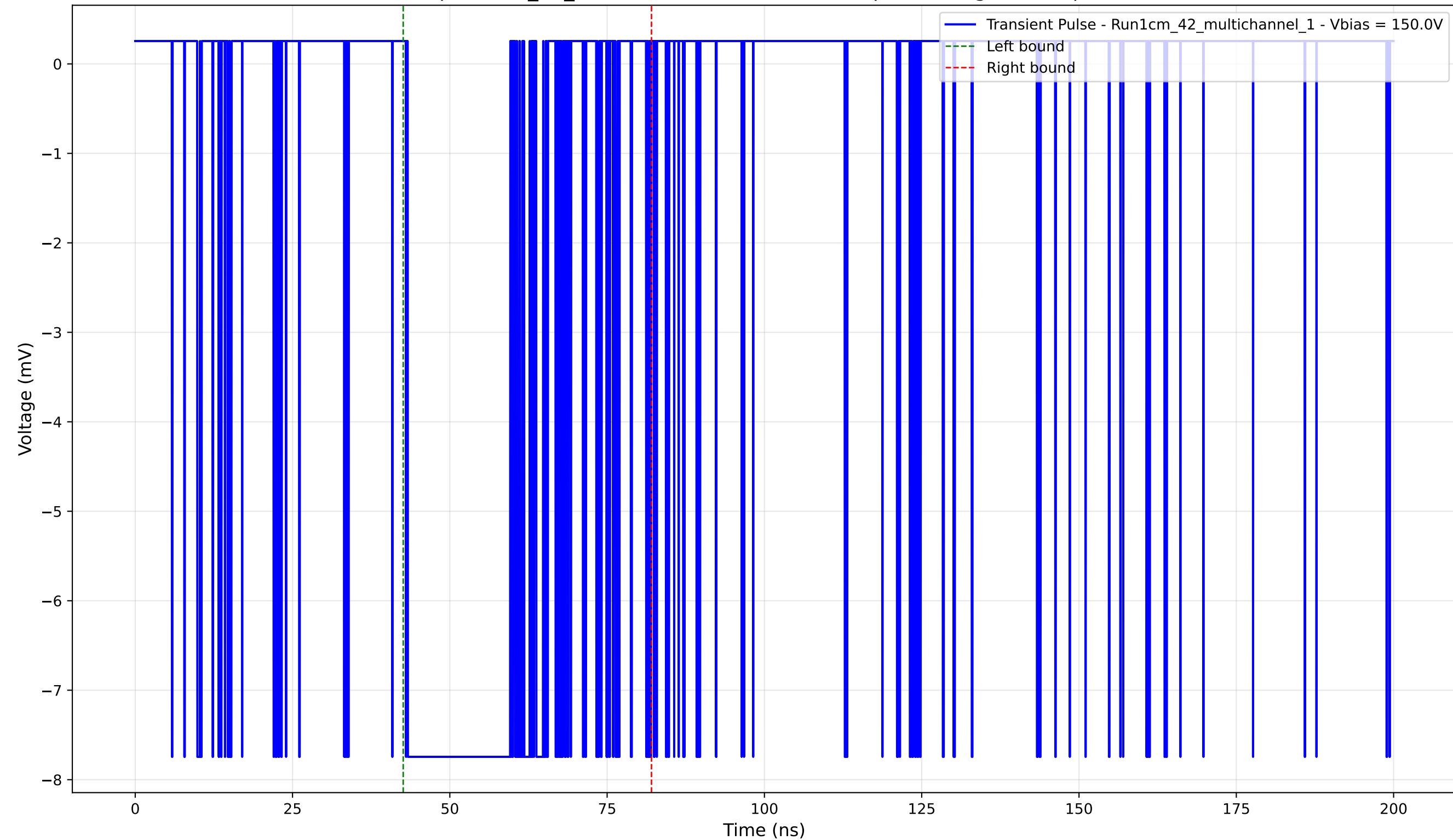
Transient Pulse - Sample: 1cm_42_multichannel - Position: 65.0 \mu\text{m} - Charge: -3.57 pC - Rise Time: 0.02 ns
