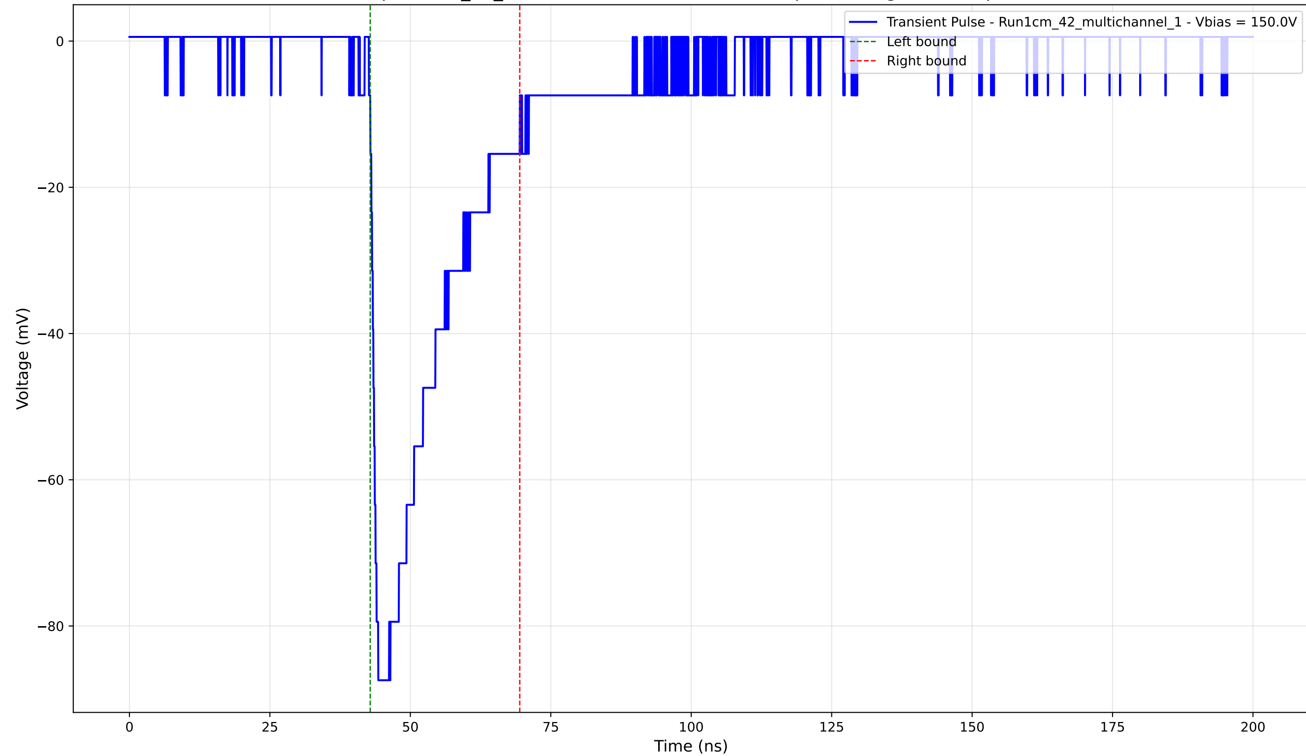
Transient Pulse - Sample: 1cm_42_multichannel - Position: 1080.0 \mu\text{m} - Charge: -22.48 pC - Rise Time: 1.12 ns
