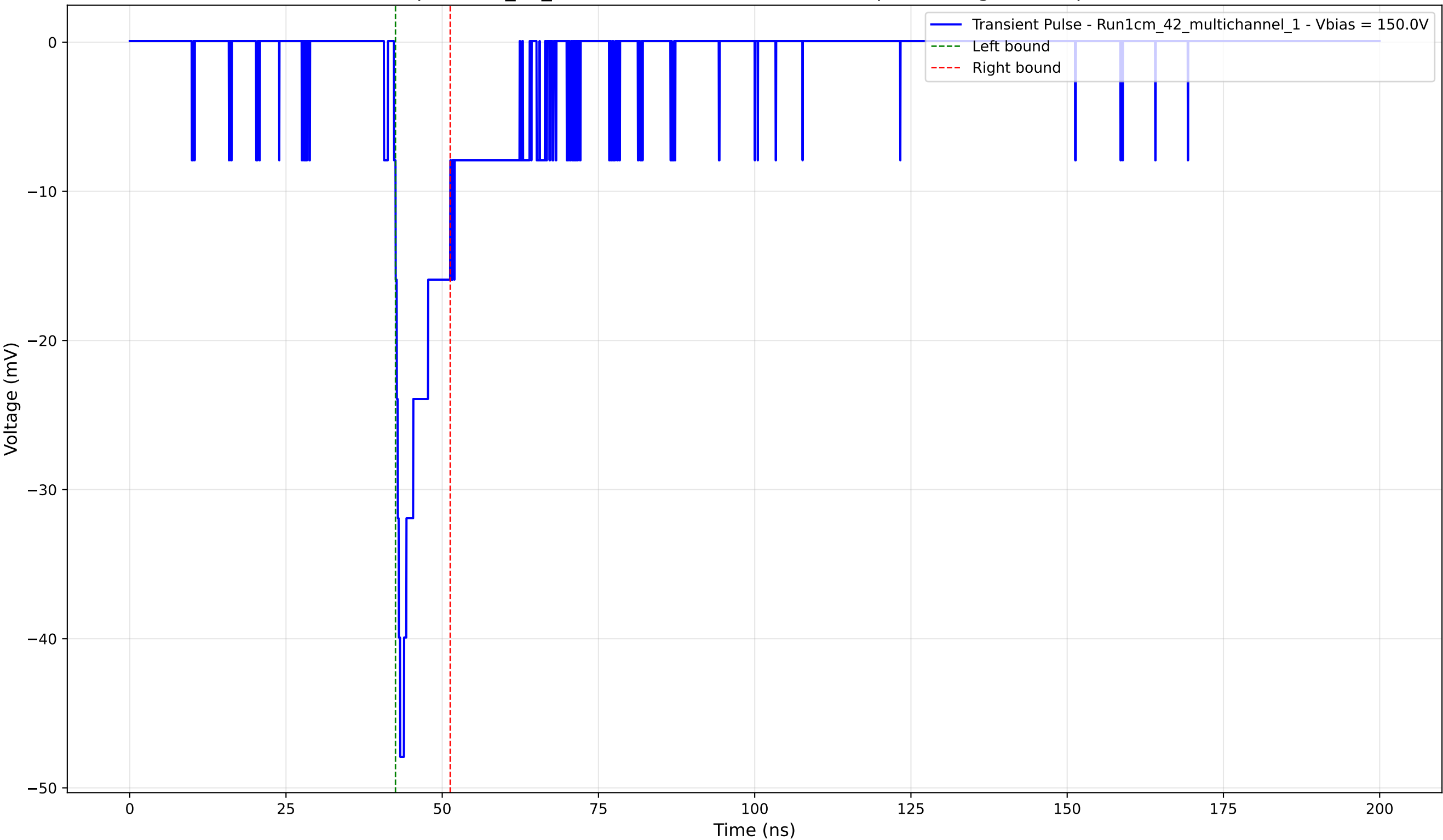
Transient Pulse - Sample: 1cm_42_multichannel - Position: 2935.0 \mu\text{m} - Charge: -4.28 pC - Rise Time: 0.99 ns
