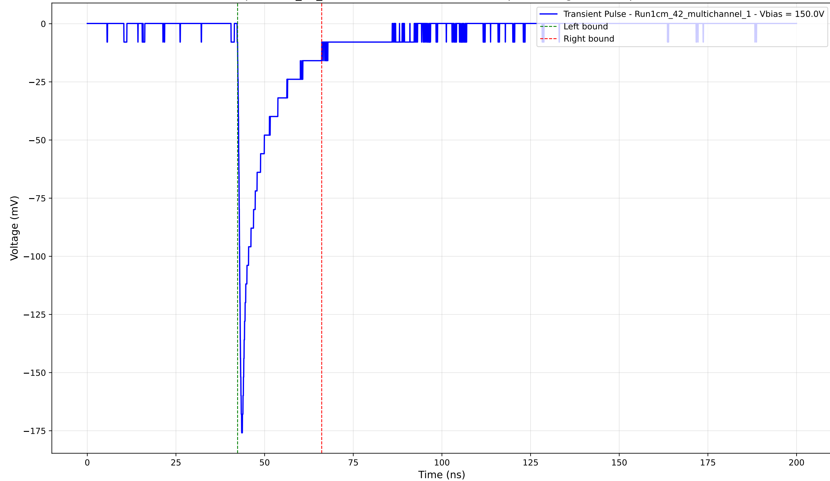
Transient Pulse - Sample: 1cm_42_multichannel - Position: 1755.0 \mu\text{m} - Charge: -22.62 pC - Rise Time: 0.88 ns
