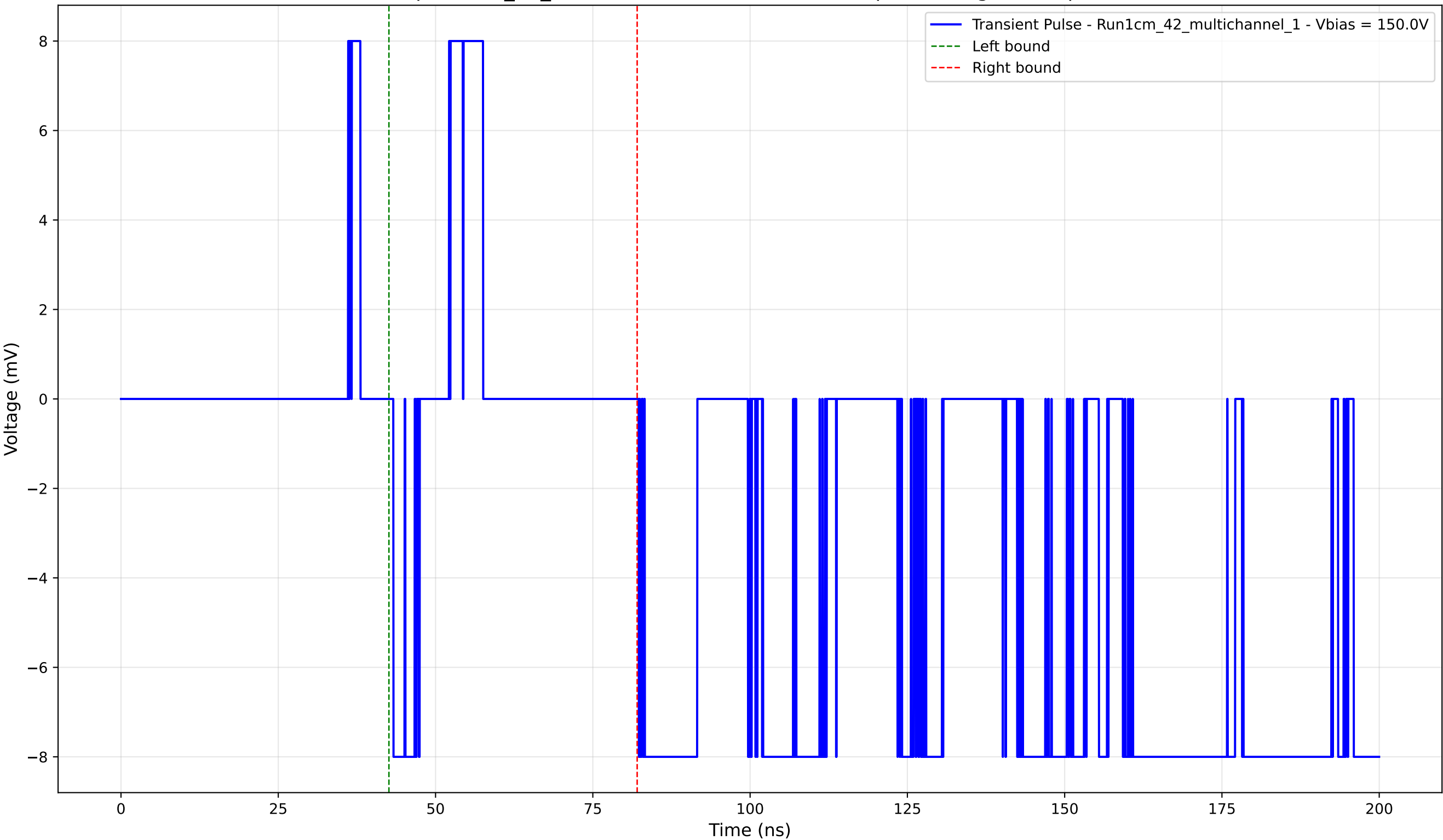
Transient Pulse - Sample: 1cm_42_multichannel - Position: 3890.0 \mu\text{m} - Charge: 0.26 pC - Rise Time: 0.02 ns
