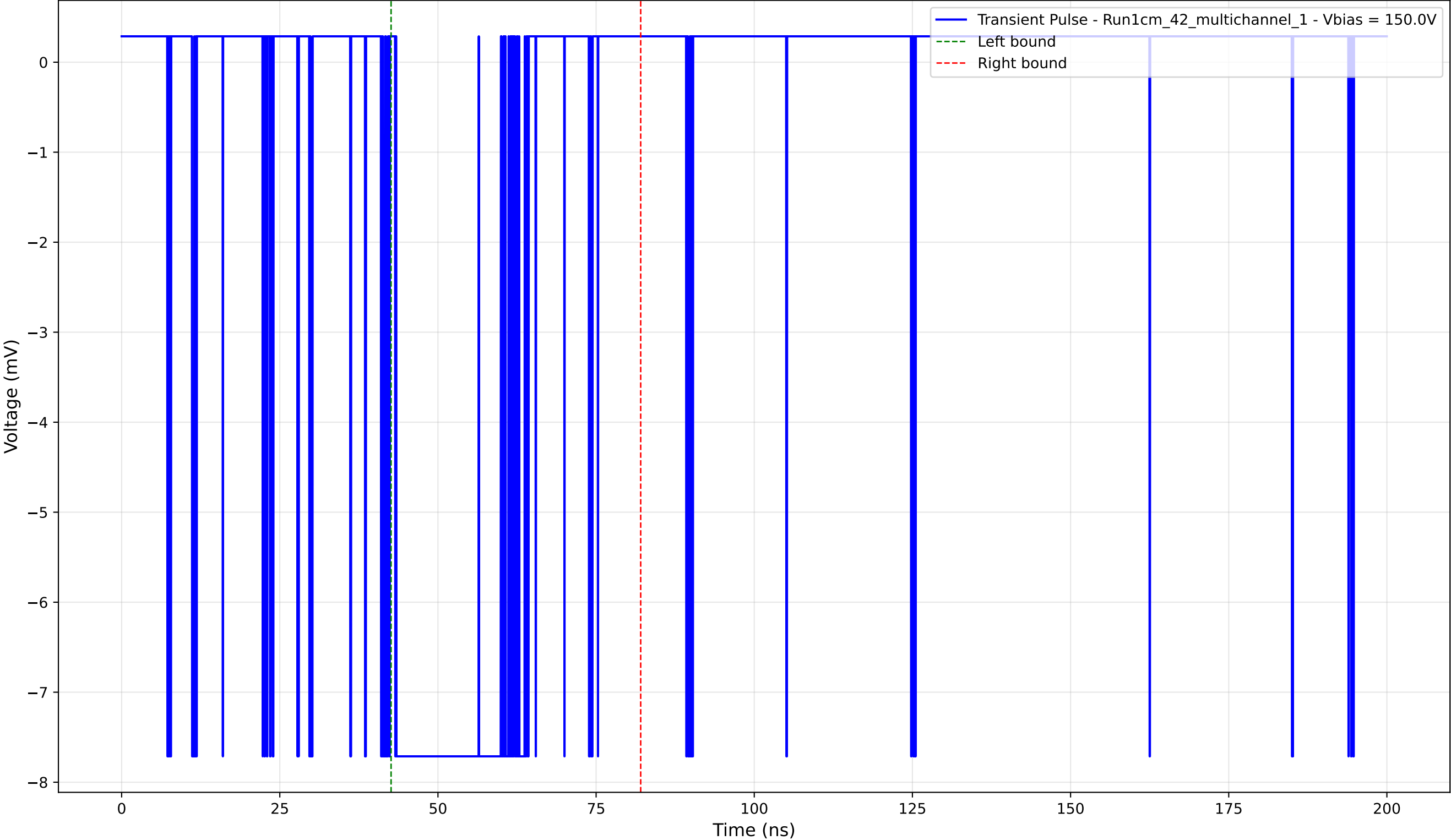
Transient Pulse - Sample: 1cm_42_multichannel - Position: 385.0 \mu\text{m} - Charge: -3.00 pC - Rise Time: 0.02 ns
