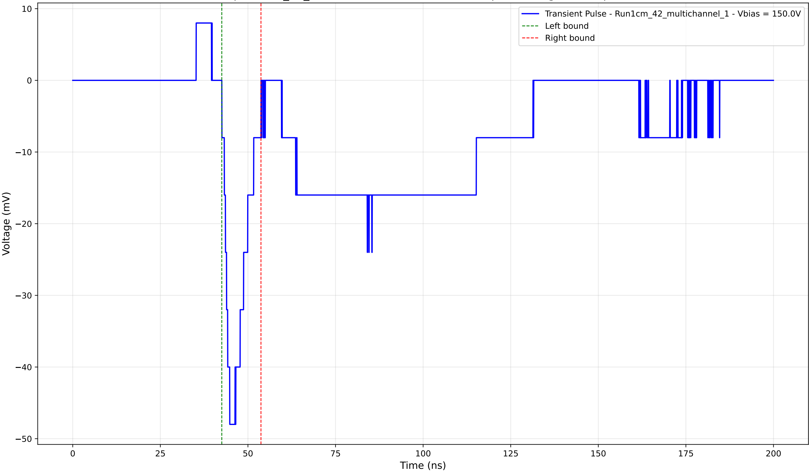
Transient Pulse - Sample: 1cm_42_multichannel - Position: 4580.0 \mu\text{m} - Charge: -5.76 pC - Rise Time: 2.25 ns
