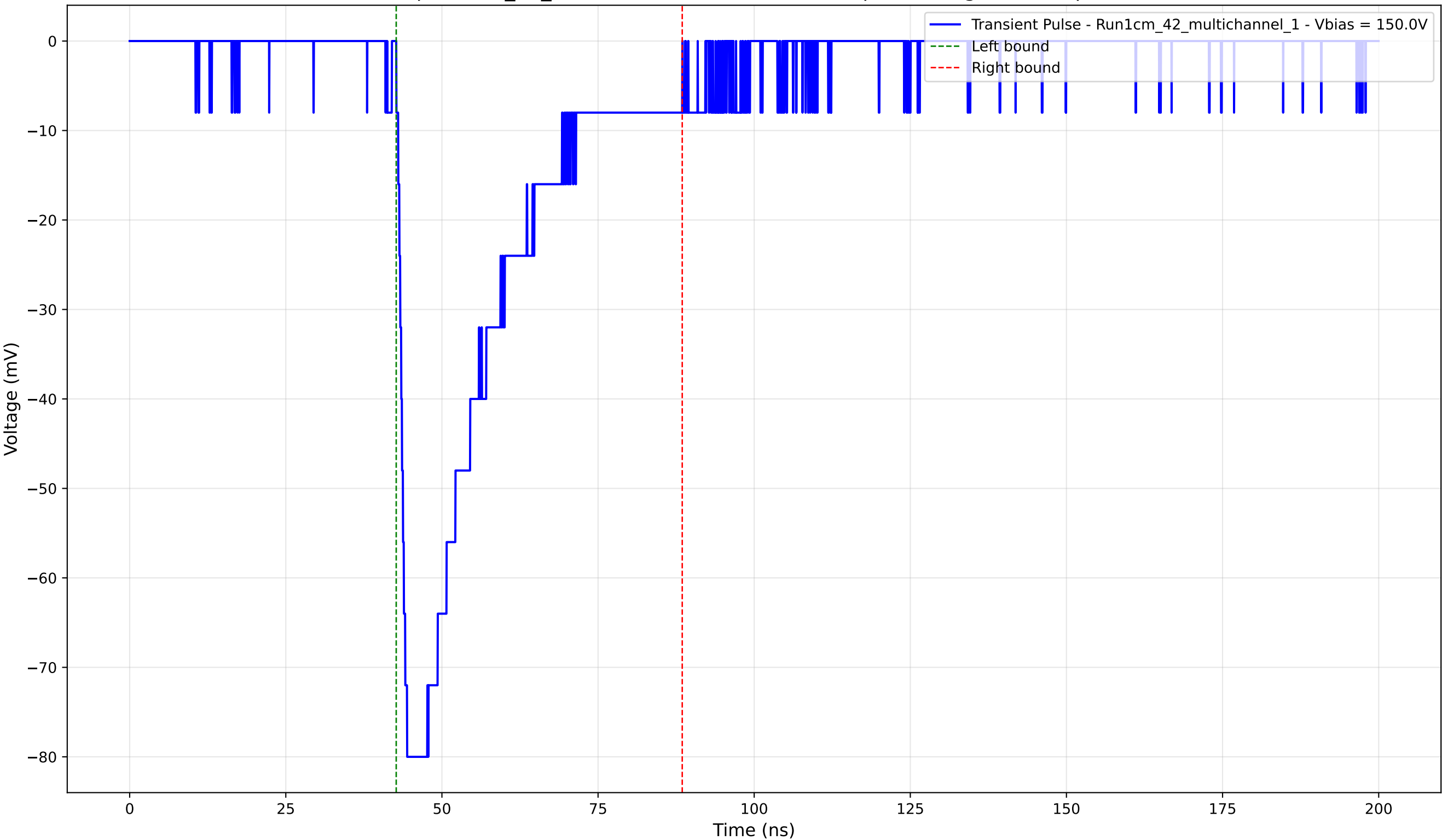
Transient Pulse - Sample: 1cm_42_multichannel - Position: 950.0 \mu\text{m} - Charge: -25.43 pC - Rise Time: 1.14 ns
