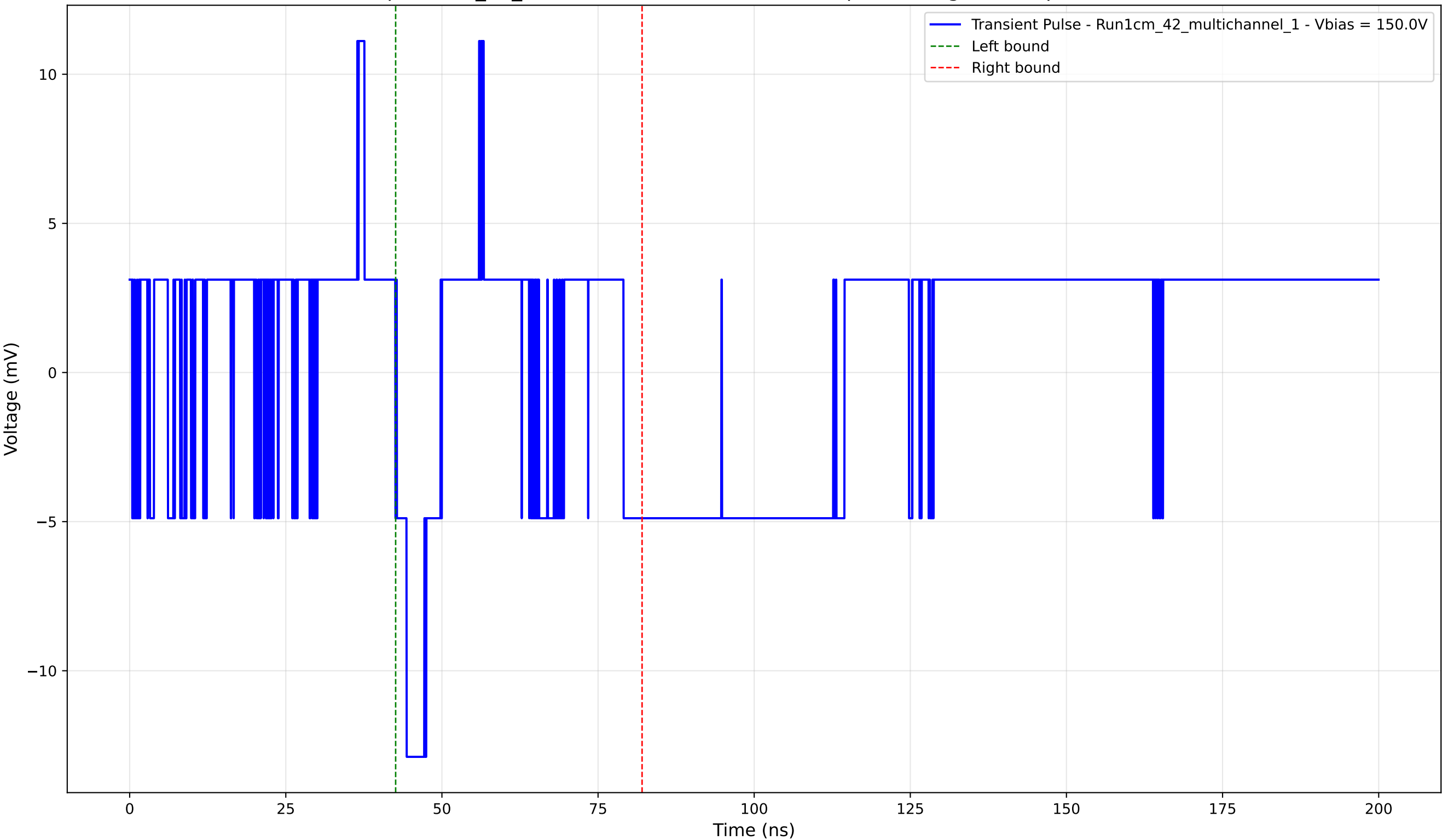
Transient Pulse - Sample: 1cm_42_multichannel - Position: 4370.0 \mu\text{m} - Charge: -0.22 pC - Rise Time: 0.00 ns (N/A)
