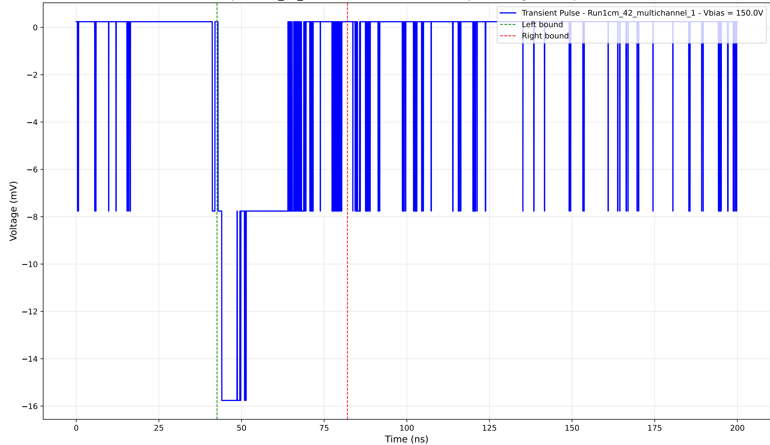
Transient Pulse - Sample: 1cm_42_multichannel - Position: 900.0 \mu\text{m} - Charge: -4.89 pC - Rise Time: 1.16 ns
