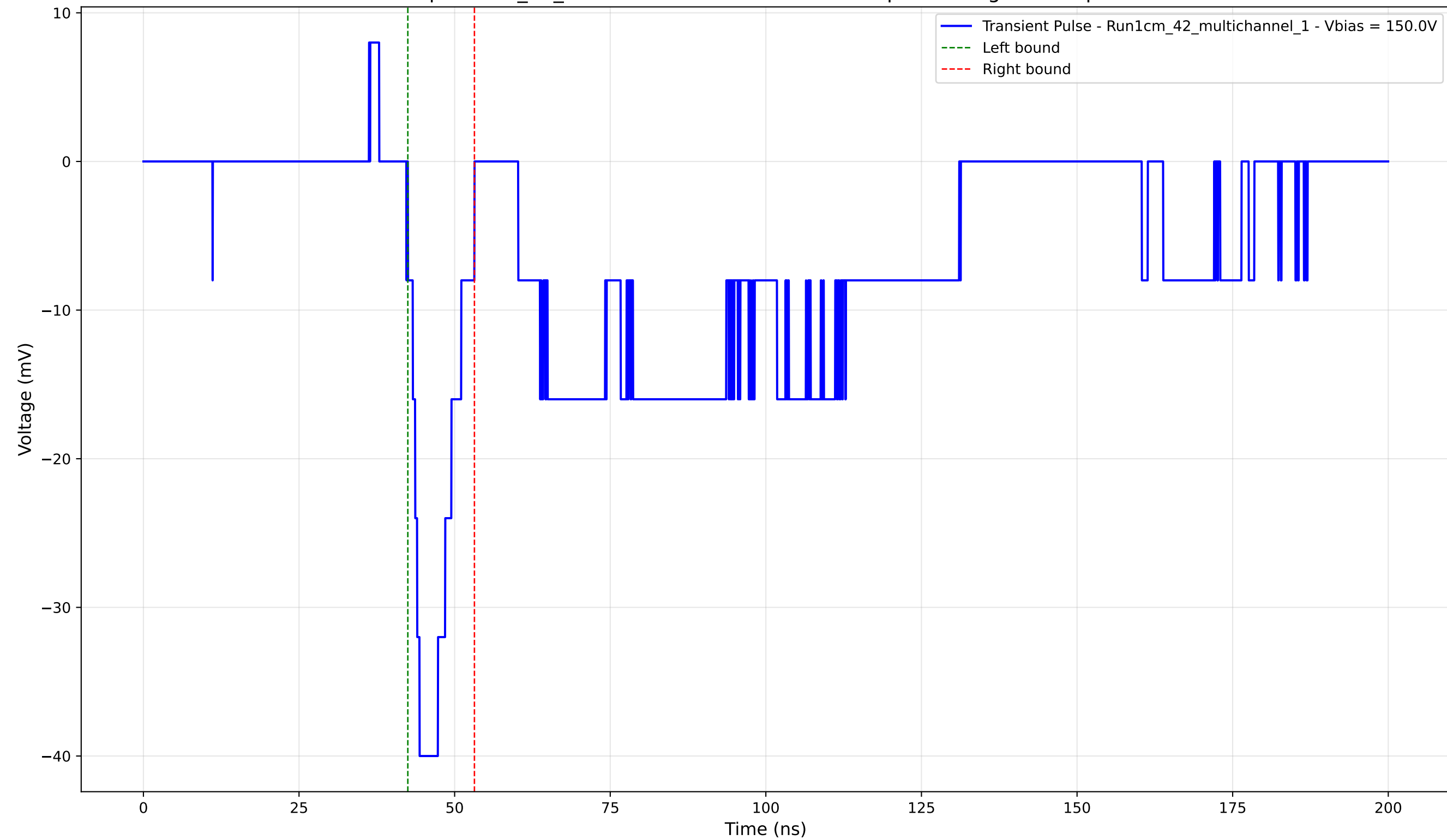
Transient Pulse - Sample: 1cm_42_multichannel - Position: 4330.0 \mu\text{m} - Charge: -5.08 pC - Rise Time: 1.87 ns
