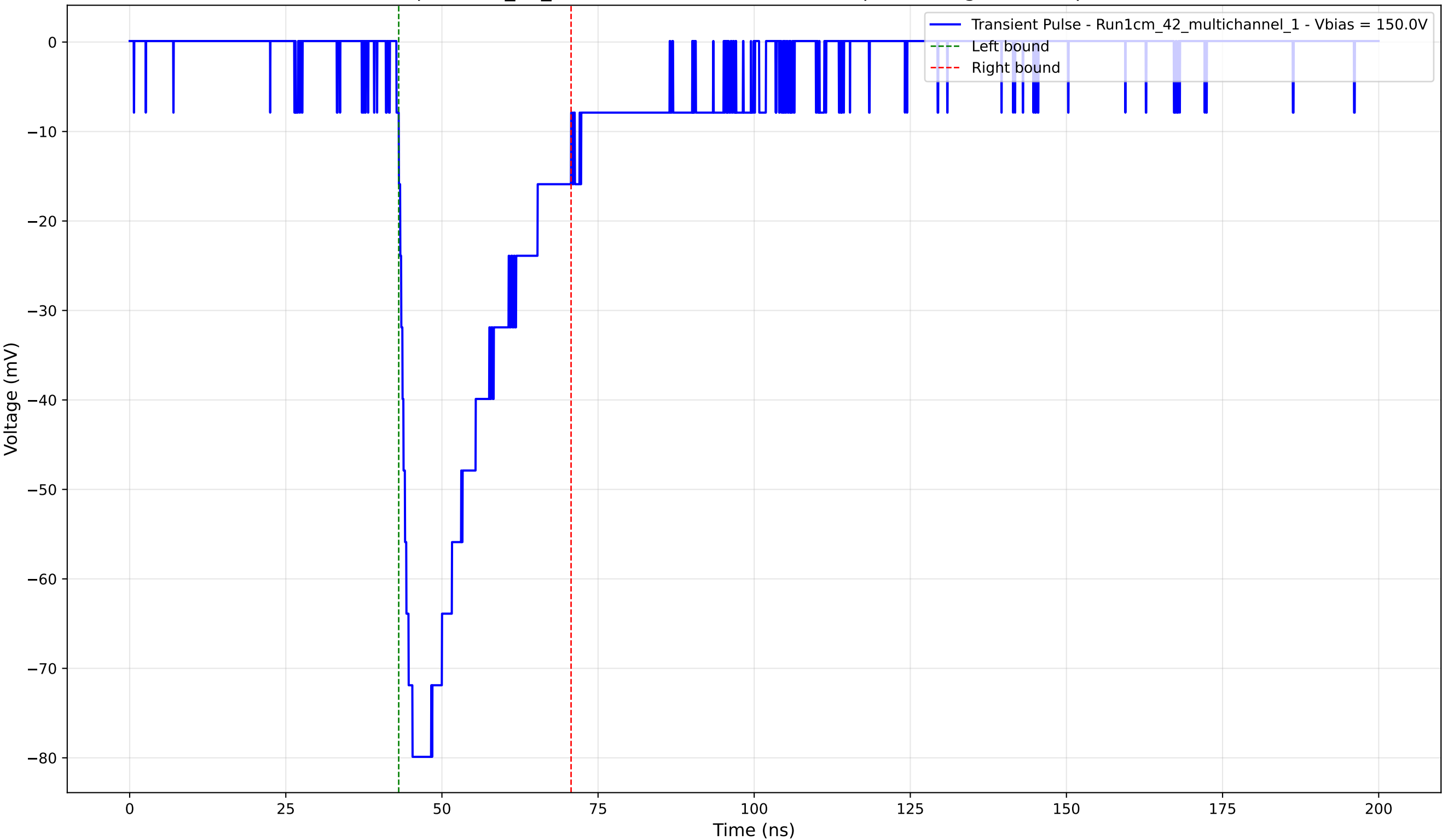
Transient Pulse - Sample: 1cm_42_multichannel - Position: 635.0 \mu\text{m} - Charge: -23.26 pC - Rise Time: 2.20 ns
