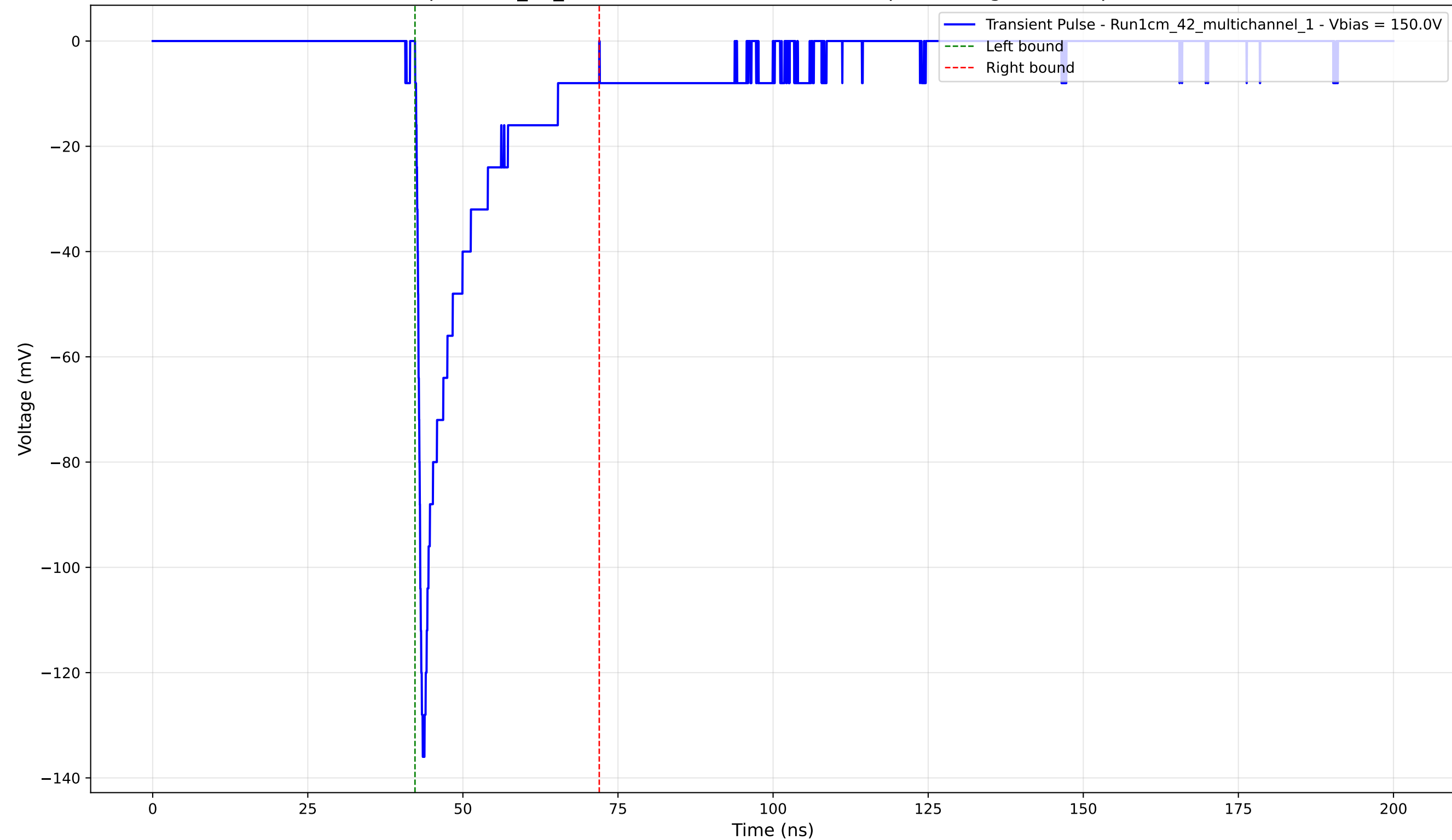
Transient Pulse - Sample: 1cm_42_multichannel - Position: 3100.0 \mu\text{m} - Charge: -19.06 pC - Rise Time: 0.93 ns
