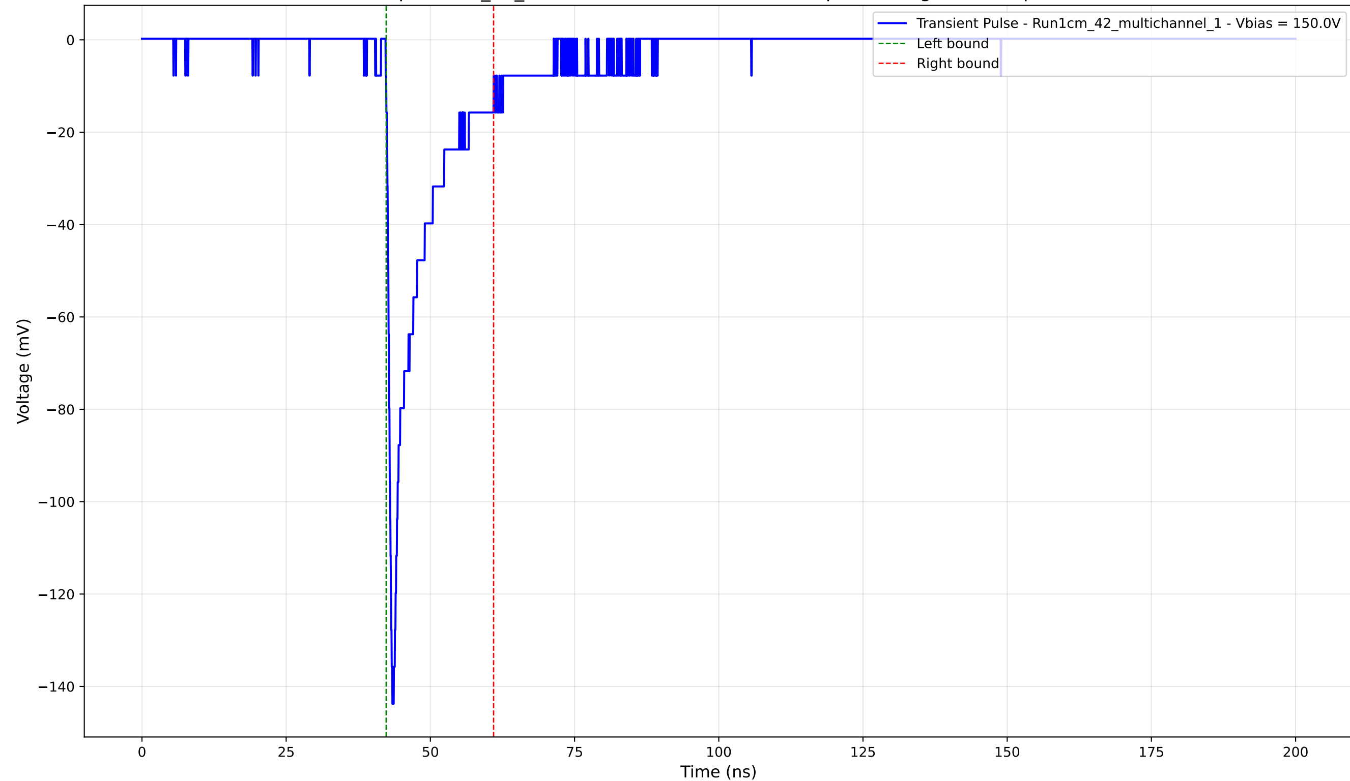
Transient Pulse - Sample: 1cm_42_multichannel - Position: 2960.0 \mu\text{m} - Charge: -15.70 pC - Rise Time: 0.92 ns
