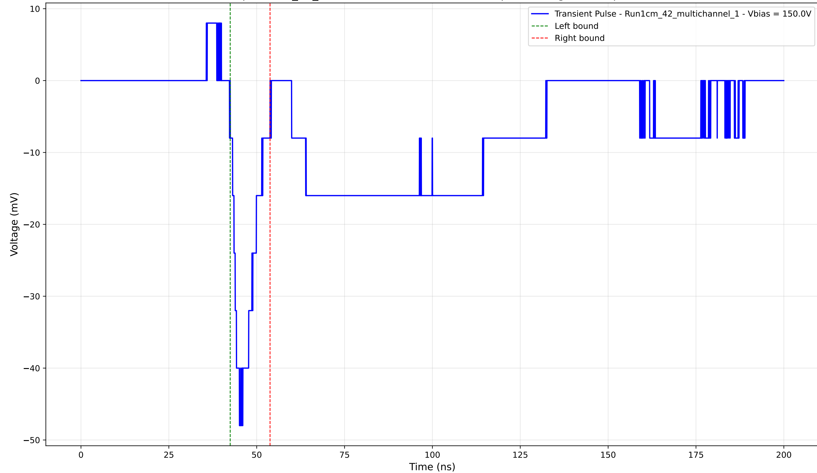
Transient Pulse - Sample: 1cm_42_multichannel - Position: 4700.0 \mu\text{m} - Charge: -5.63 pC - Rise Time: 2.61 ns
