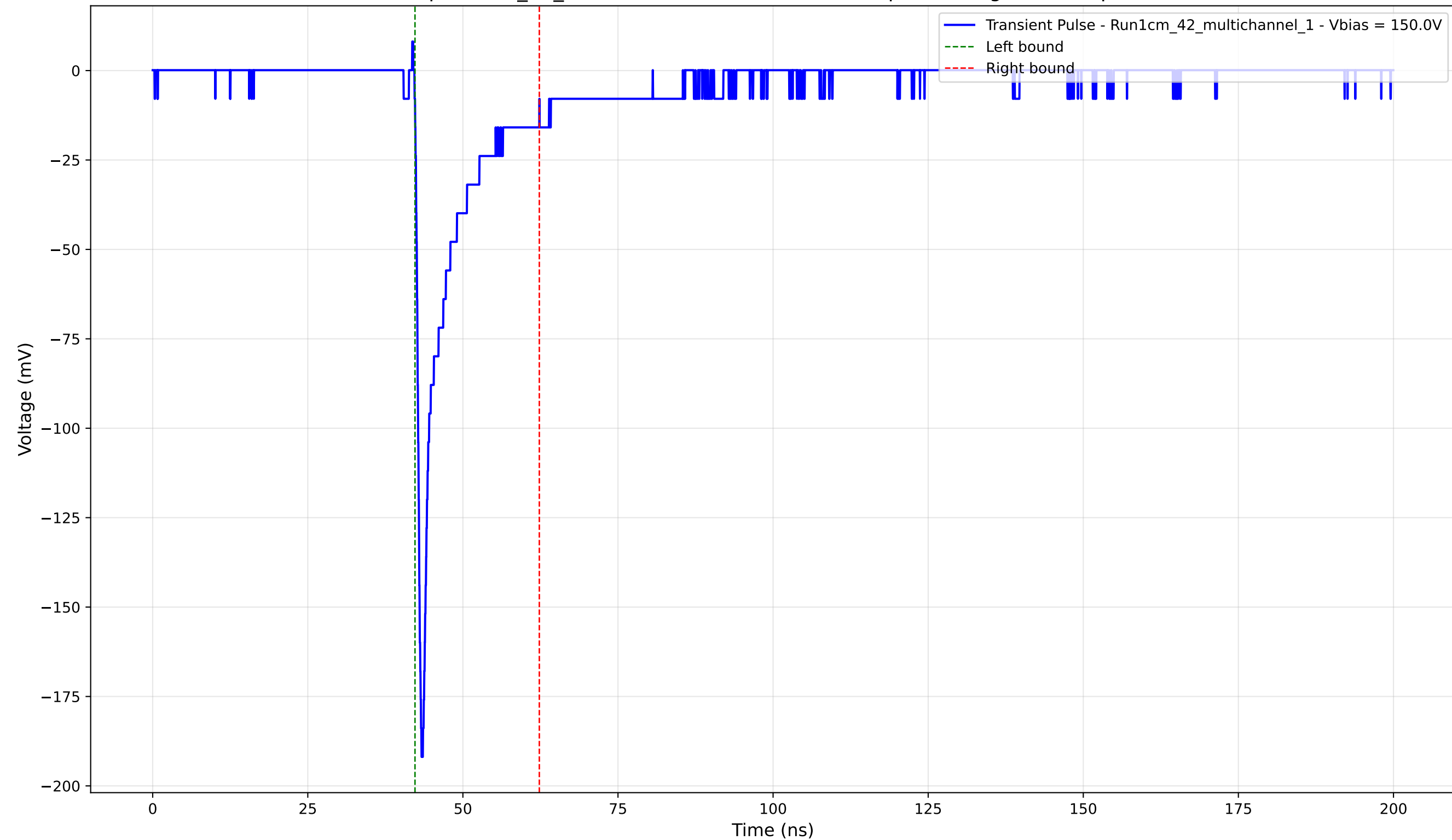
Transient Pulse - Sample: 1cm_42_multichannel - Position: 2820.0 \mu\text{m} - Charge: -18.04 pC - Rise Time: 0.83 ns
