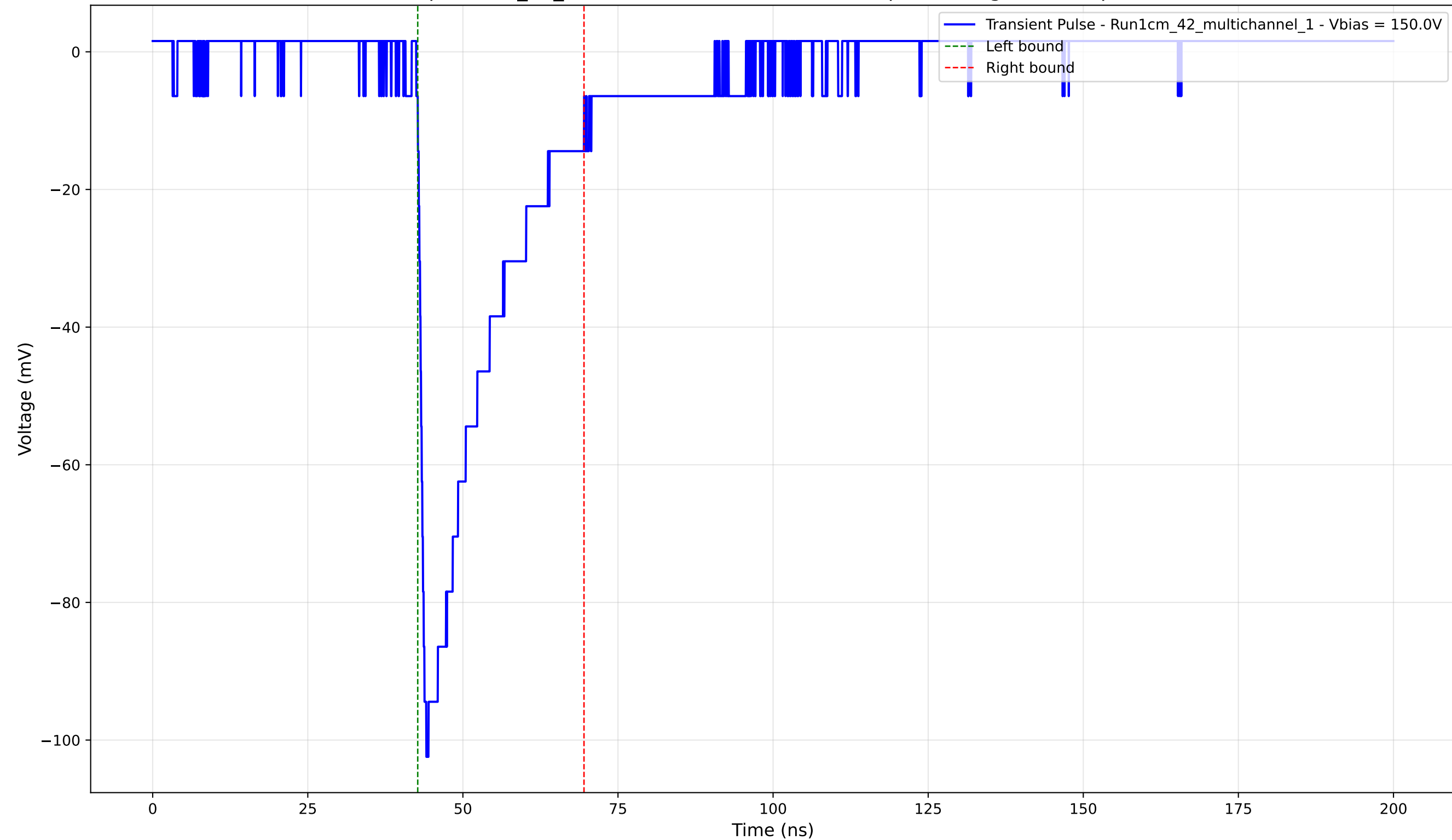
Transient Pulse - Sample: 1cm_42_multichannel - Position: 1255.0 \mu\text{m} - Charge: -23.05 pC - Rise Time: 1.07 ns
