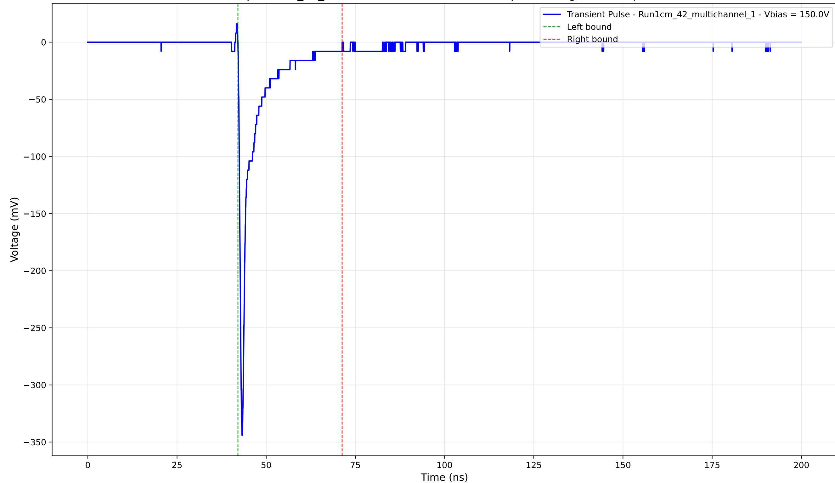
Transient Pulse - Sample: 1cm_42_multichannel - Position: 2170.0 \mu\text{m} - Charge: -25.64 pC - Rise Time: 0.77 ns
