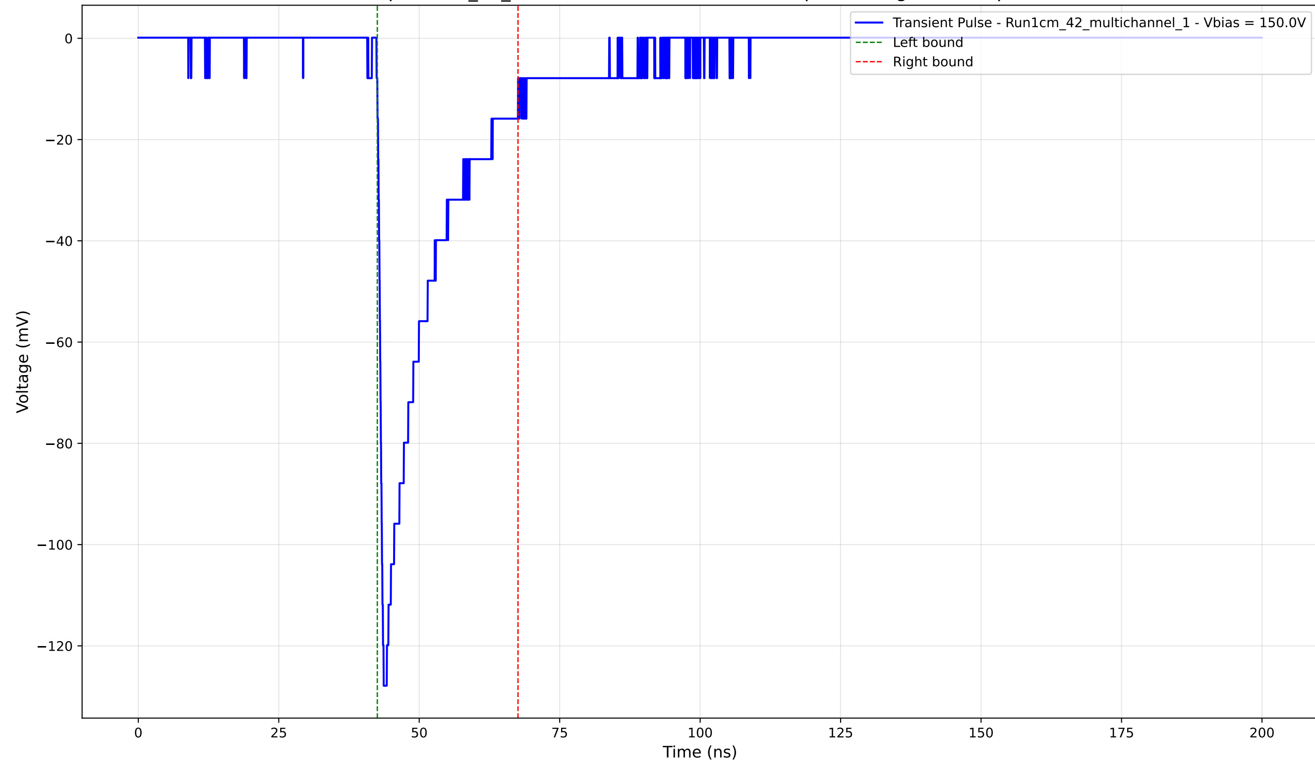
Transient Pulse - Sample: 1cm_42_multichannel - Position: 1495.0 \mu\text{m} - Charge: -23.40 pC - Rise Time: 0.99 ns
