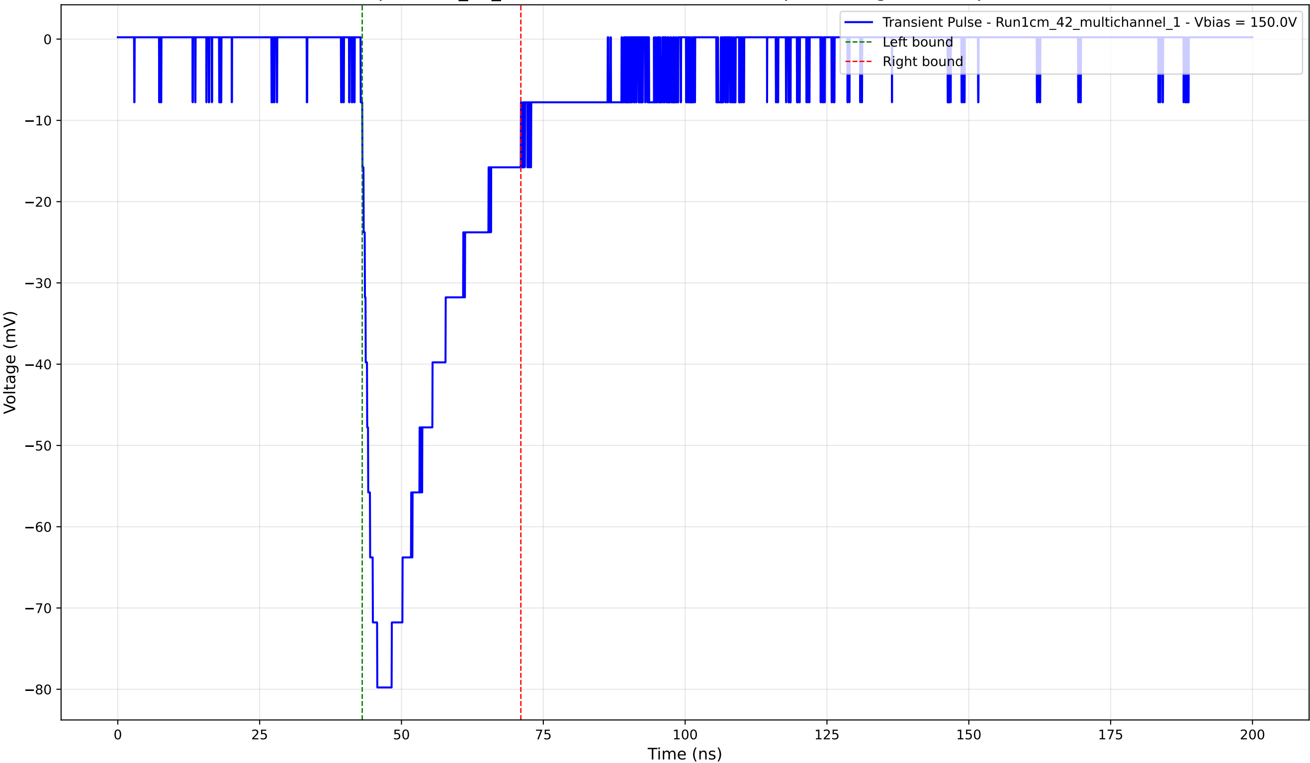
Transient Pulse - Sample: 1cm_42_multichannel - Position: 530.0 \mu\text{m} - Charge: -23.16 pC - Rise Time: 2.64 ns
