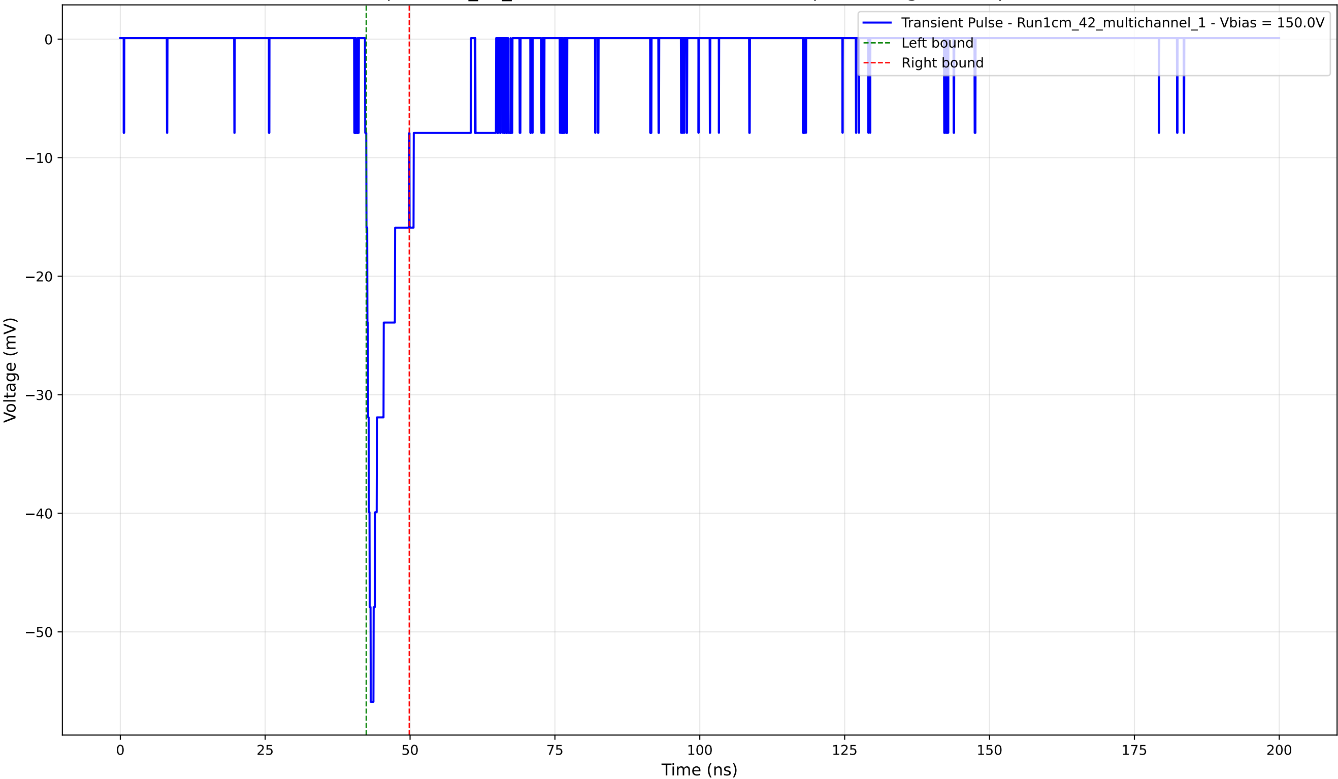
Transient Pulse - Sample: 1cm_42_multichannel - Position: 1920.0 \mu\text{m} - Charge: -4.00 pC - Rise Time: 0.97 ns
