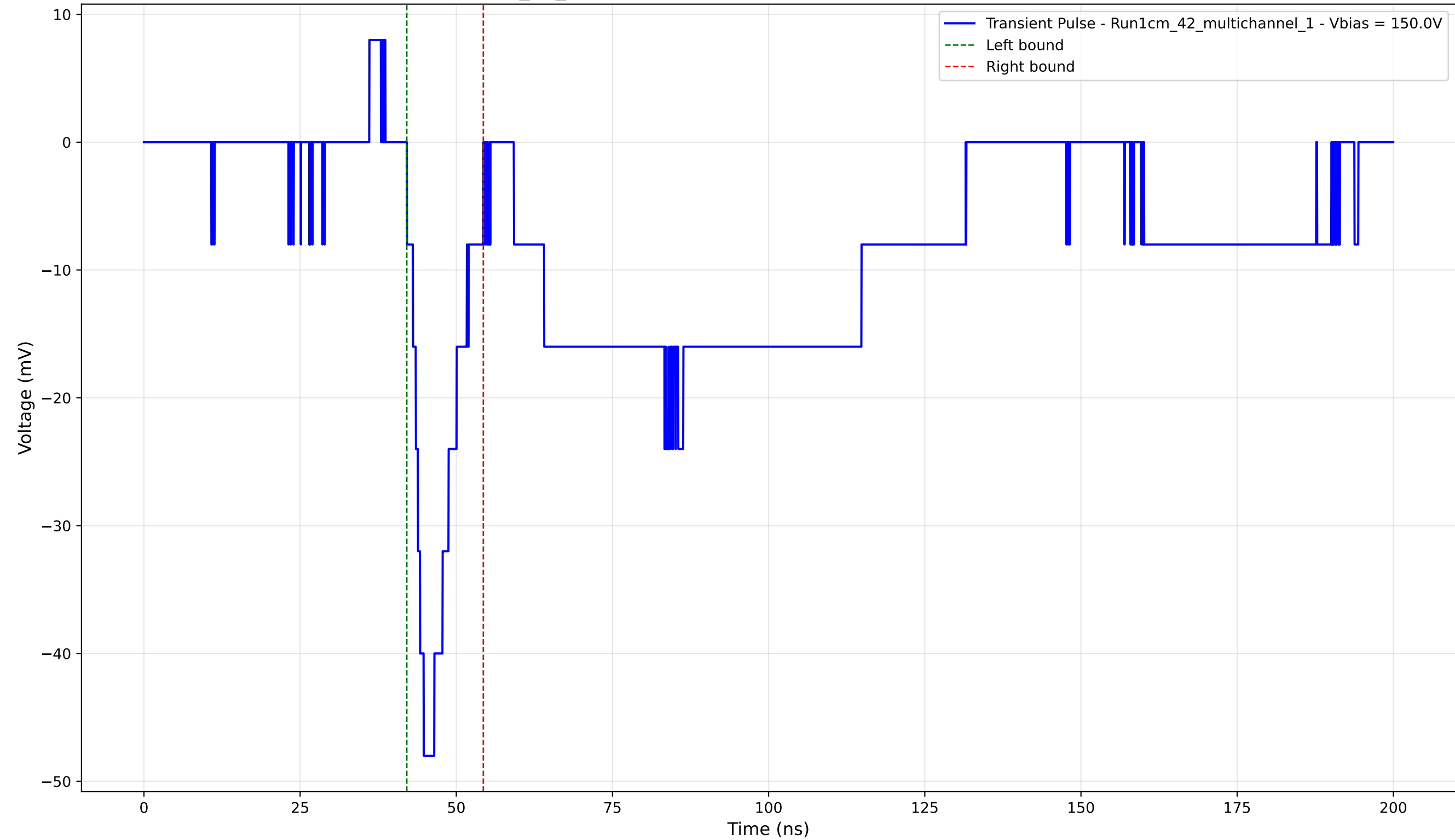
Transient Pulse - Sample: 1cm_42_multichannel - Position: 4625.0 \mu\text{m} - Charge: -6.04 pC - Rise Time: 2.69 ns
