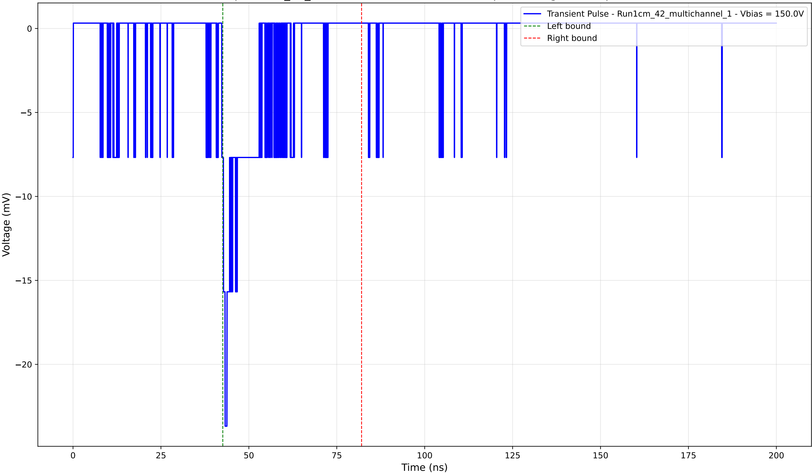
Transient Pulse - Sample: 1cm_42_multichannel - Position: 1905.0 \mu\text{m} - Charge: -2.62 pC - Rise Time: 0.95 ns
