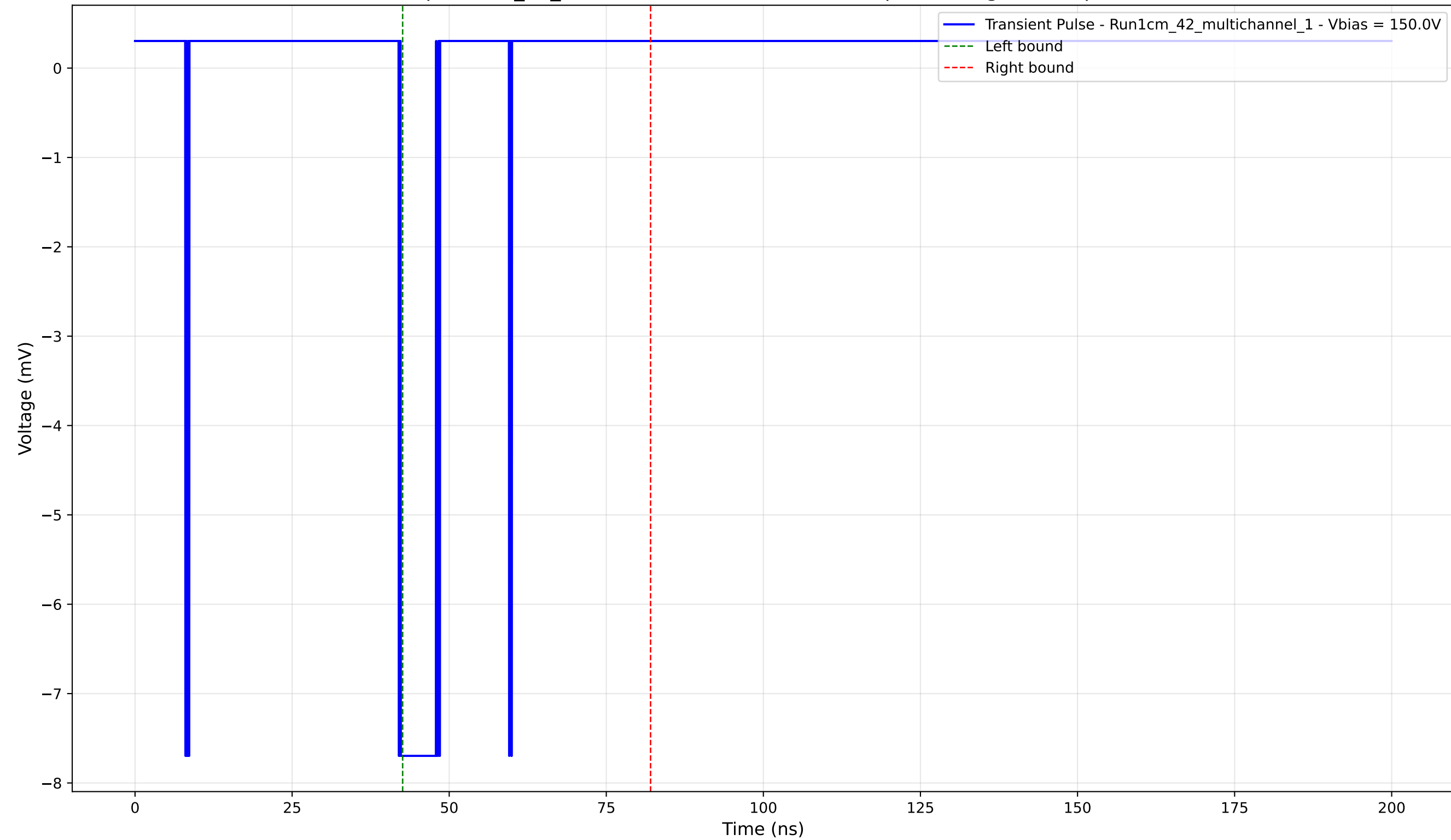
Transient Pulse - Sample: 1cm_42_multichannel - Position: 3390.0 \mu\text{m} - Charge: -0.70 pC - Rise Time: 0.02 ns
