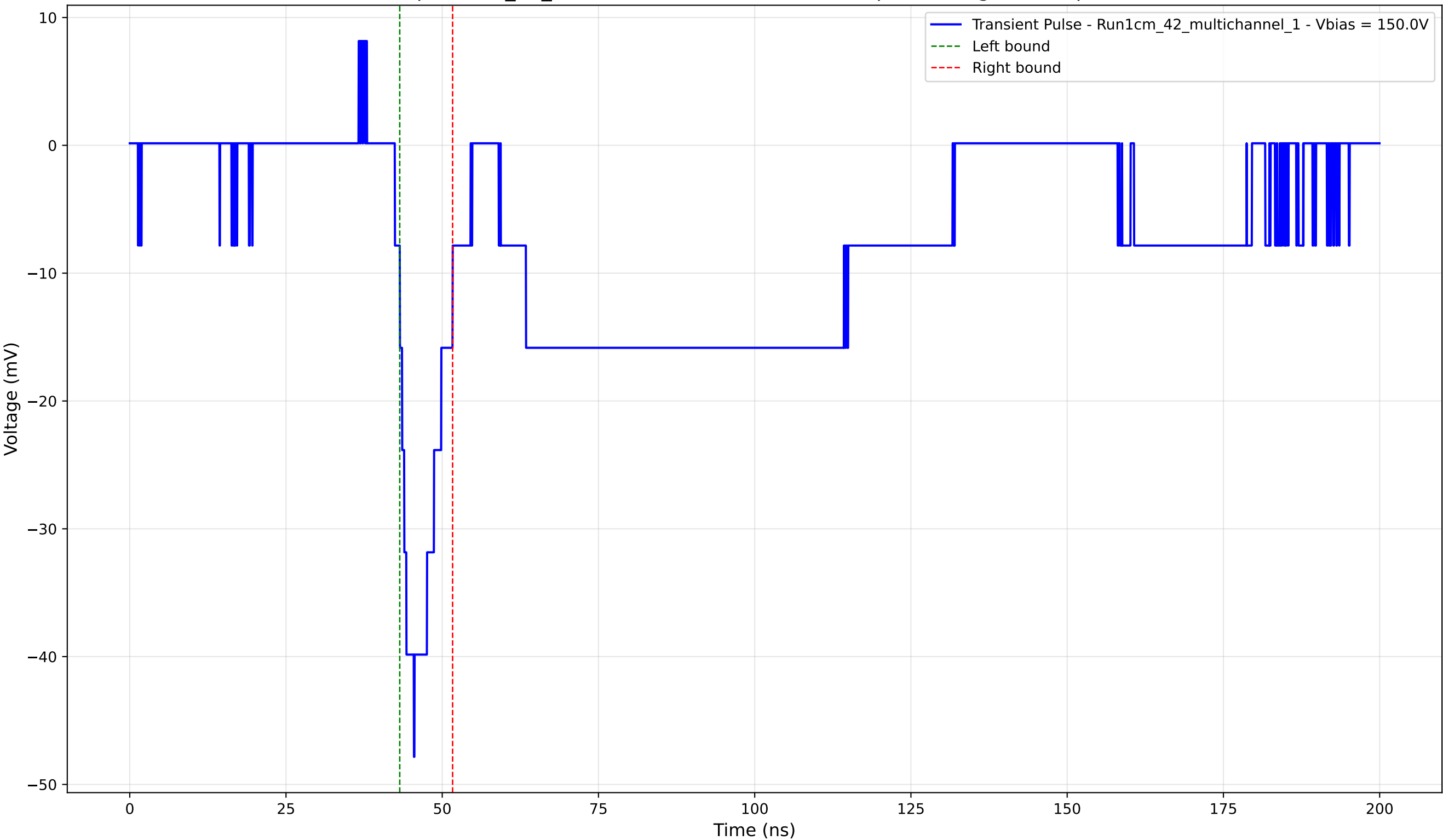
Transient Pulse - Sample: 1cm_42_multichannel - Position: 4325.0 \mu\text{m} - Charge: -4.98 pC - Rise Time: 3.05 ns
