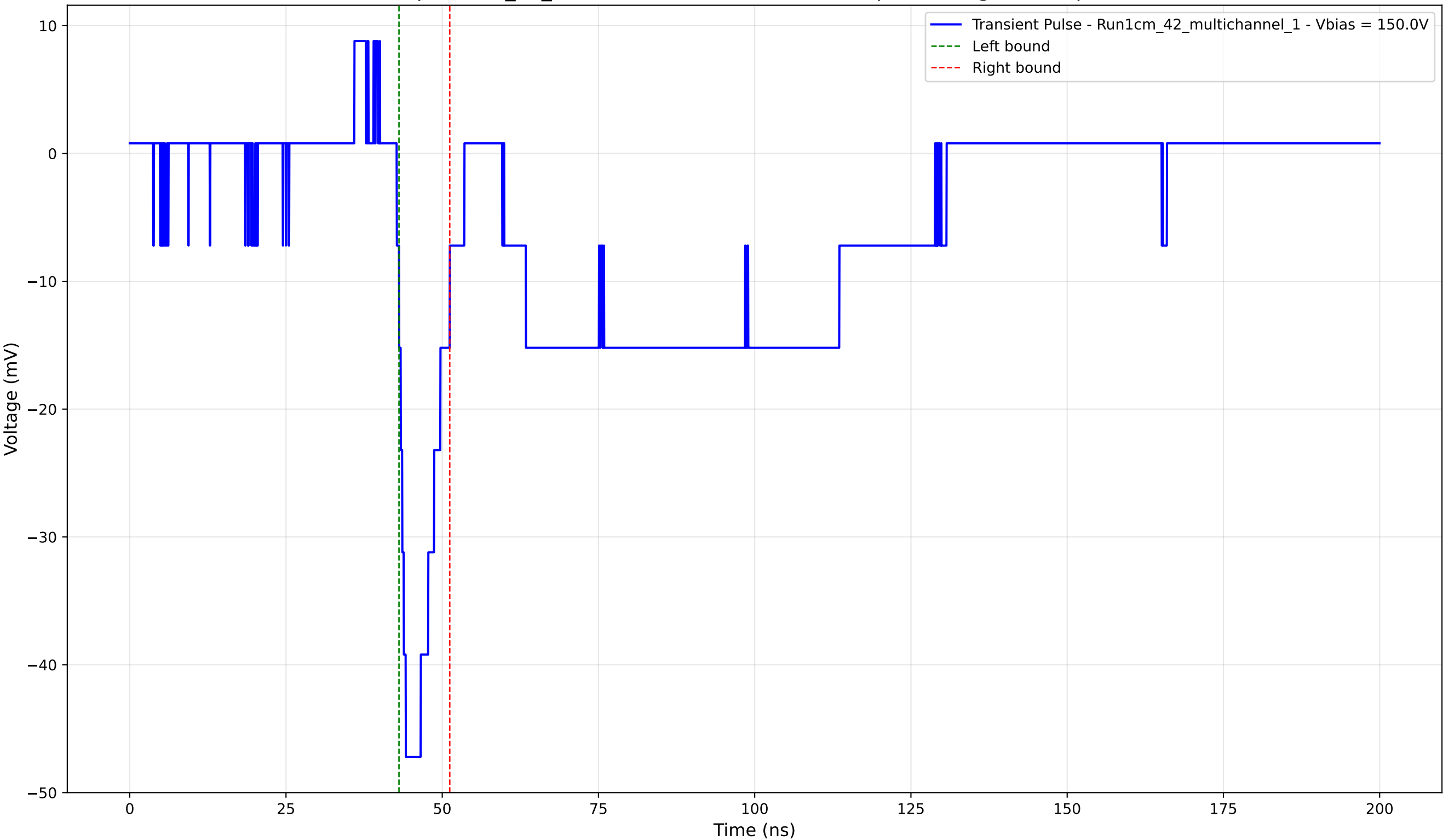
Transient Pulse - Sample: 1cm_42_multichannel - Position: 4005.0 \mu\text{m} - Charge: -5.31 pC - Rise Time: 1.45 ns
