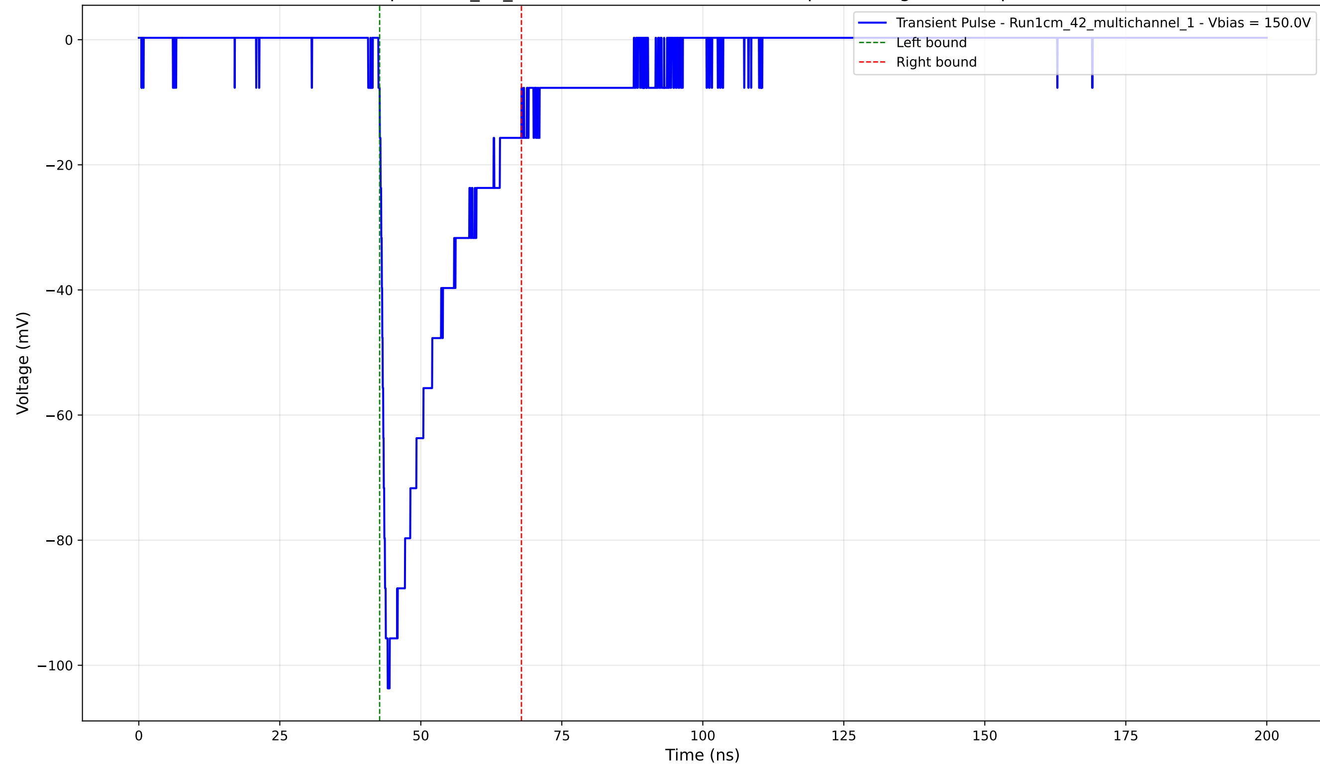
Transient Pulse - Sample: 1cm_42_multichannel - Position: 1270.0 \mu\text{m} - Charge: -22.82 pC - Rise Time: 1.07 ns
