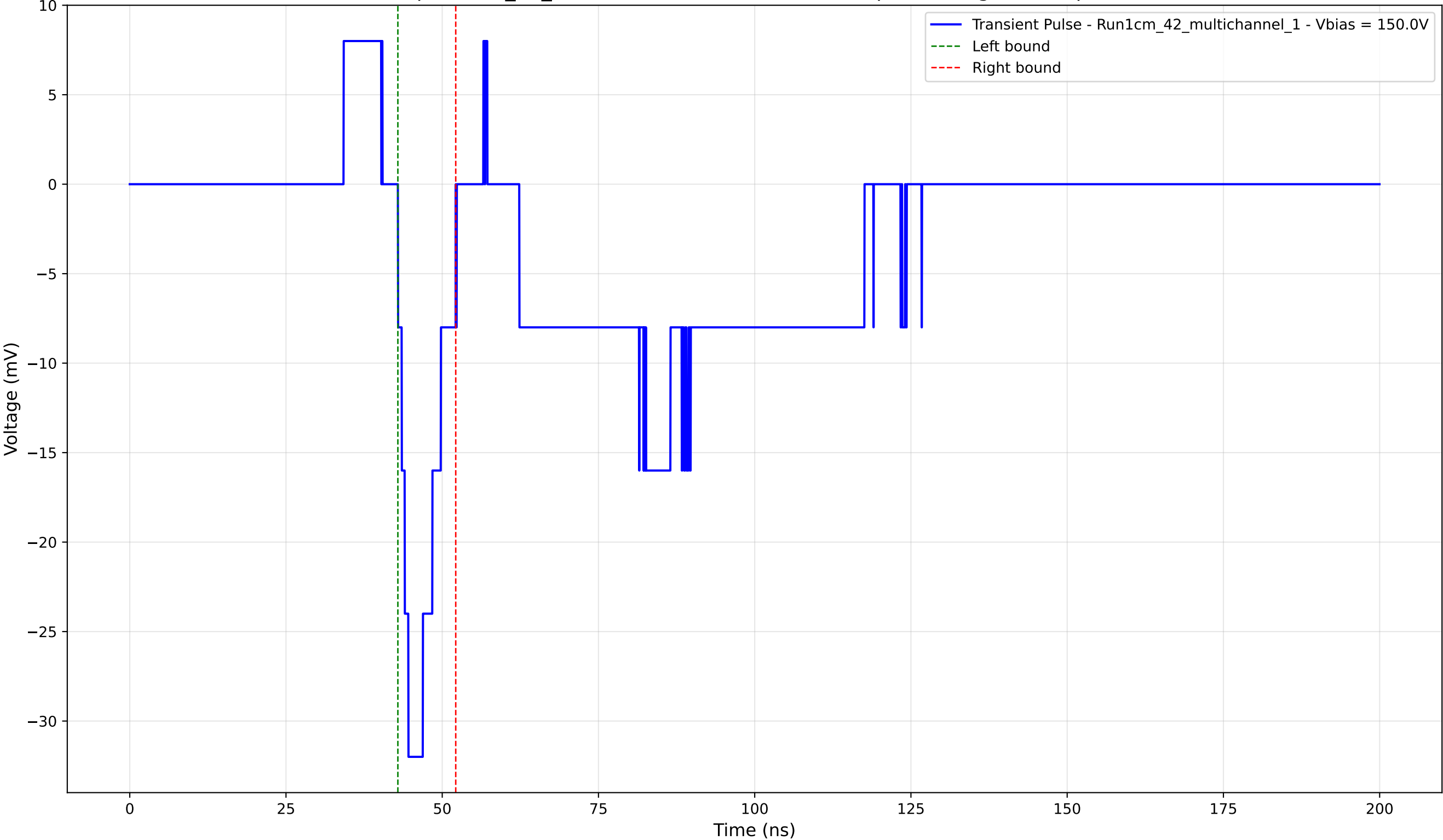
Transient Pulse - Sample: 1cm_42_multichannel - Position: 4465.0 \mu\text{m} - Charge: -3.56 pC - Rise Time: 1.67 ns
