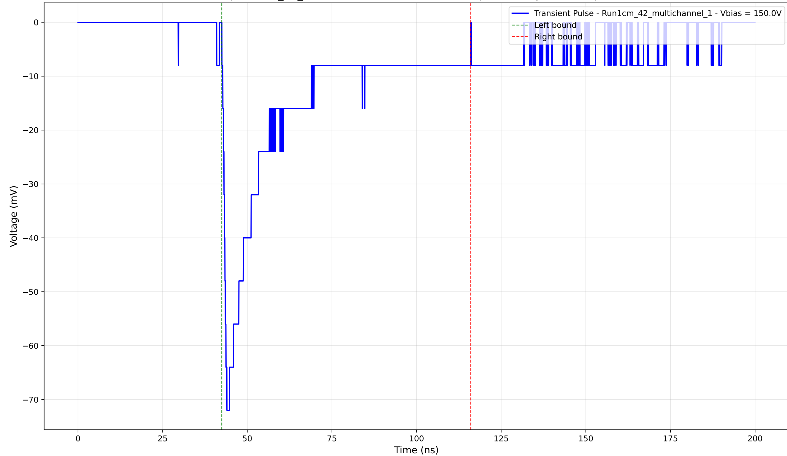
Transient Pulse - Sample: 1cm_42_multichannel - Position: 3605.0 \mu\text{m} - Charge: -23.30 pC - Rise Time: 1.48 ns
