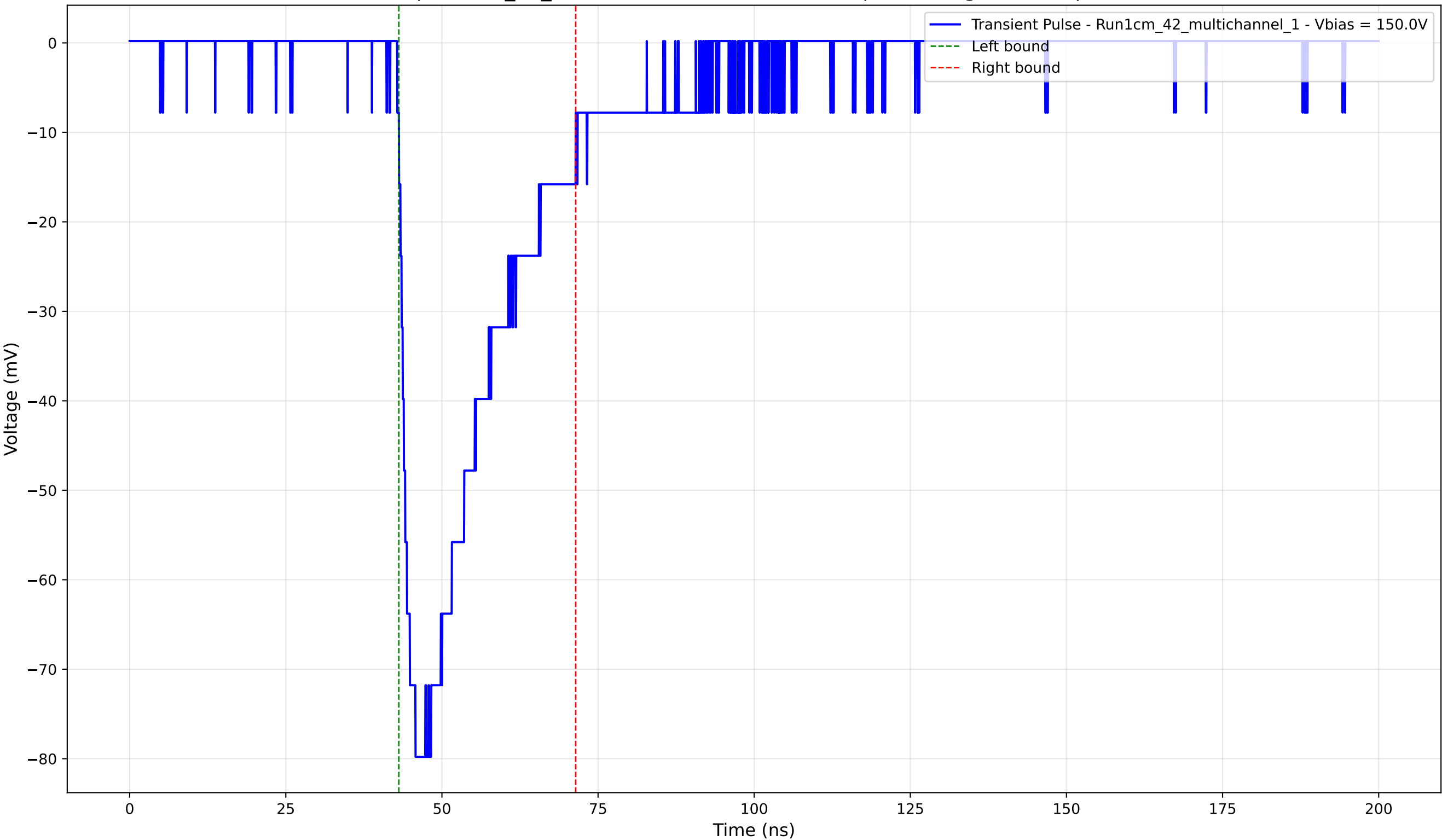
Transient Pulse - Sample: 1cm_42_multichannel - Position: 560.0 \mu\text{m} - Charge: -23.26 pC - Rise Time: 2.66 ns
