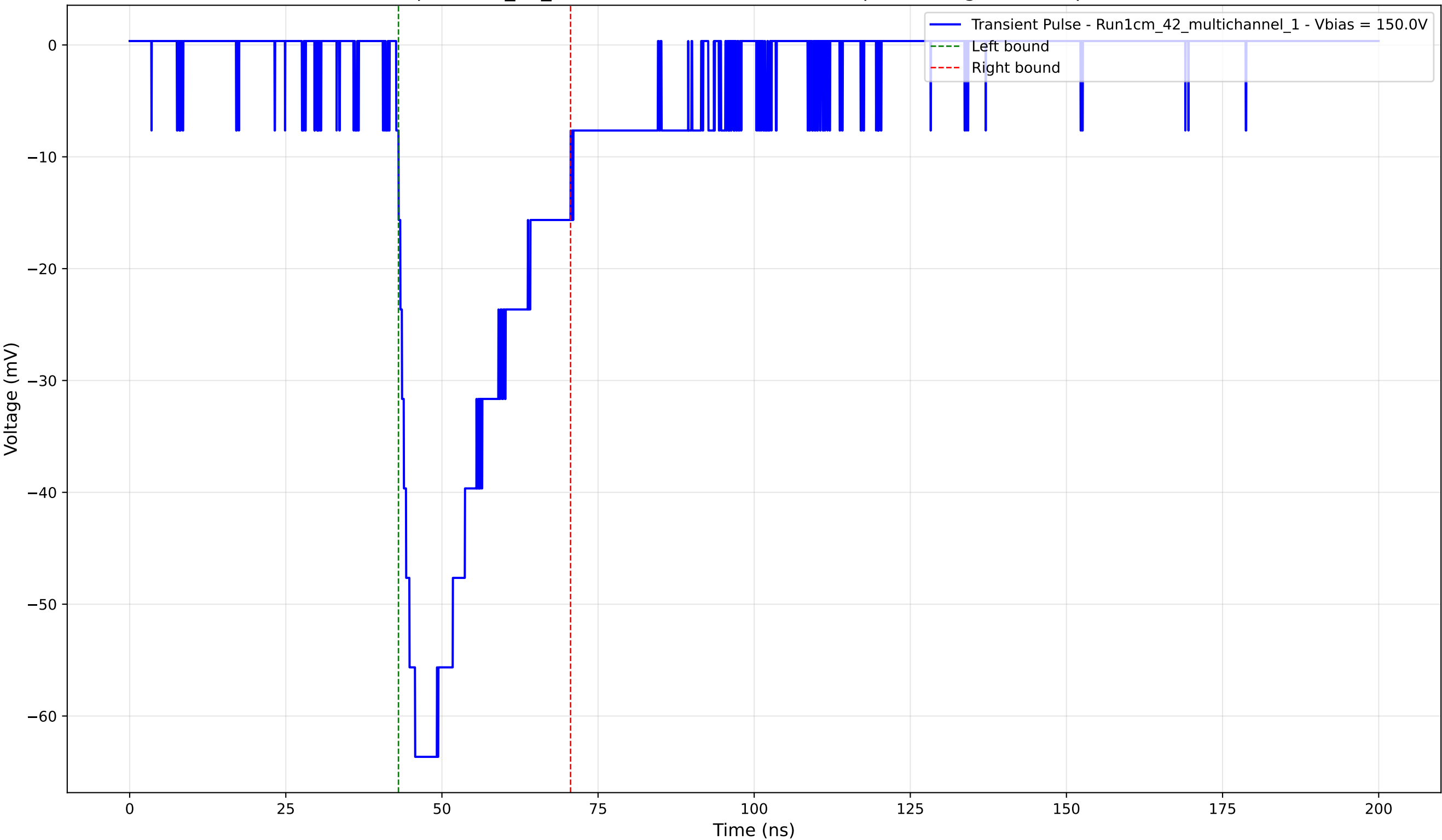
Transient Pulse - Sample: 1cm_42_multichannel - Position: 275.0 \mu\text{m} - Charge: -19.69 pC - Rise Time: 3.02 ns
