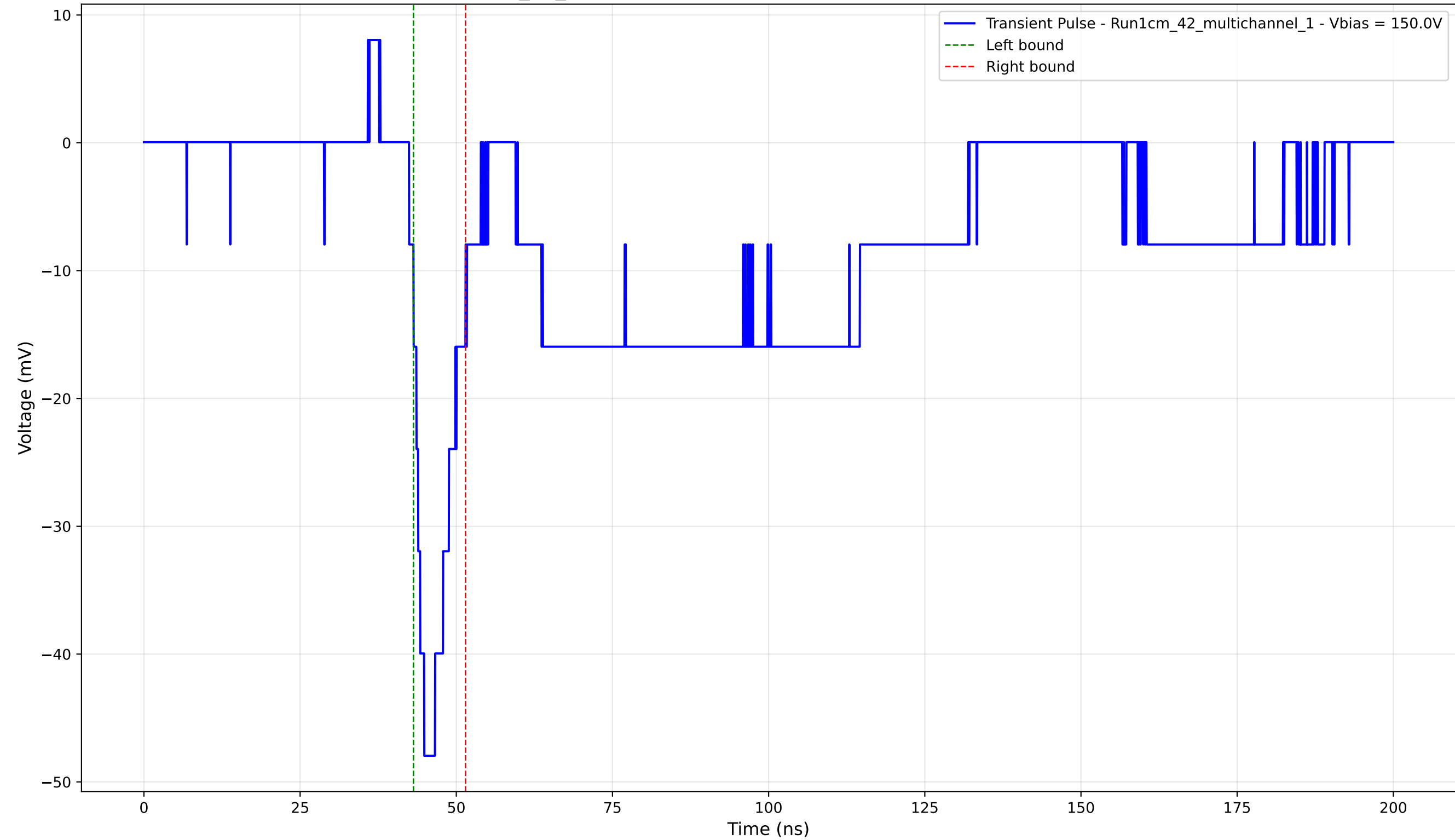
Transient Pulse - Sample: 1cm_42_multichannel - Position: 4505.0 \mu\text{m} - Charge: -5.32 pC - Rise Time: 2.43 ns
