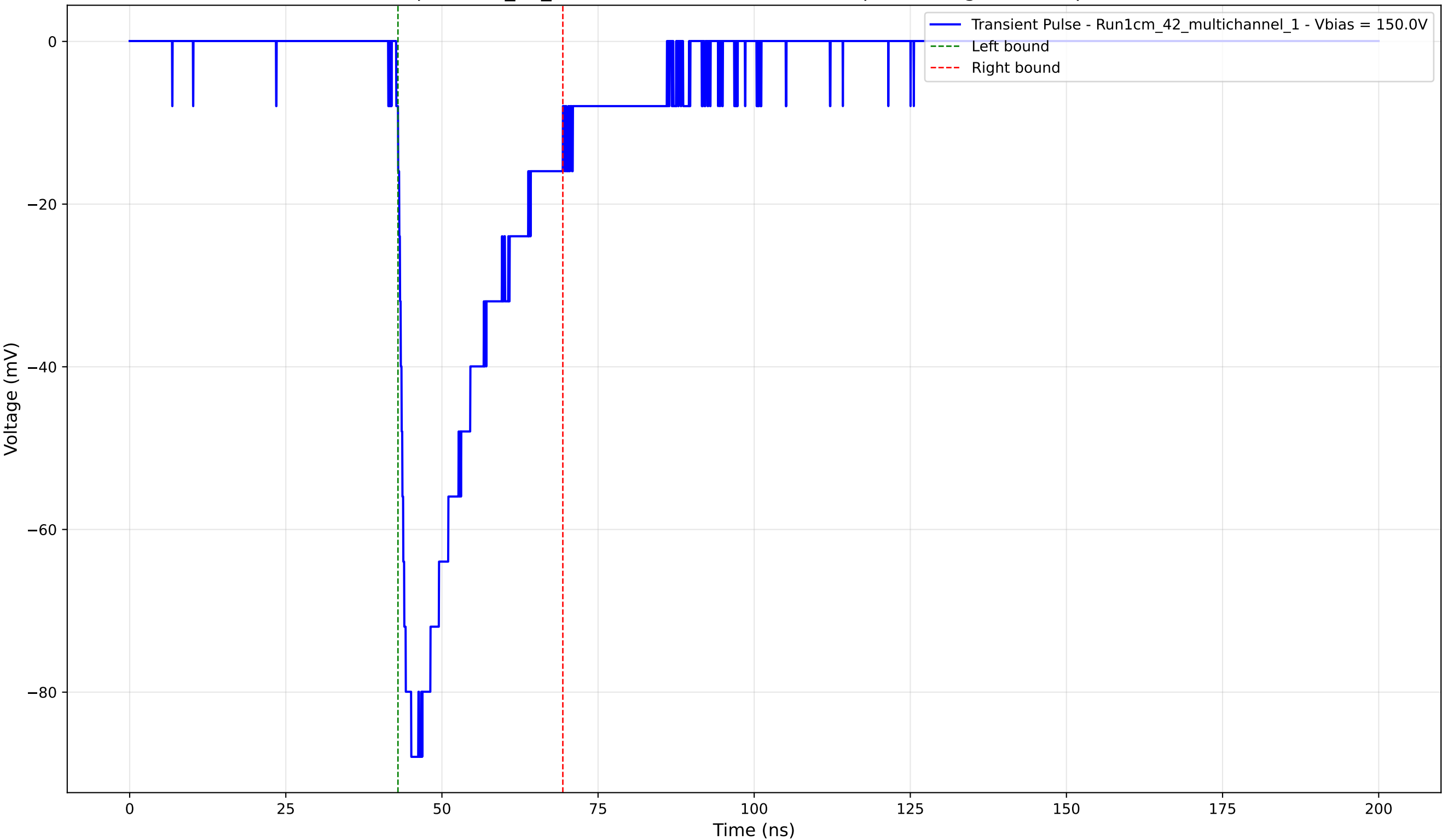
Transient Pulse - Sample: 1cm_42_multichannel - Position: 975.0 \mu\text{m} - Charge: -22.83 pC - Rise Time: 1.24 ns
