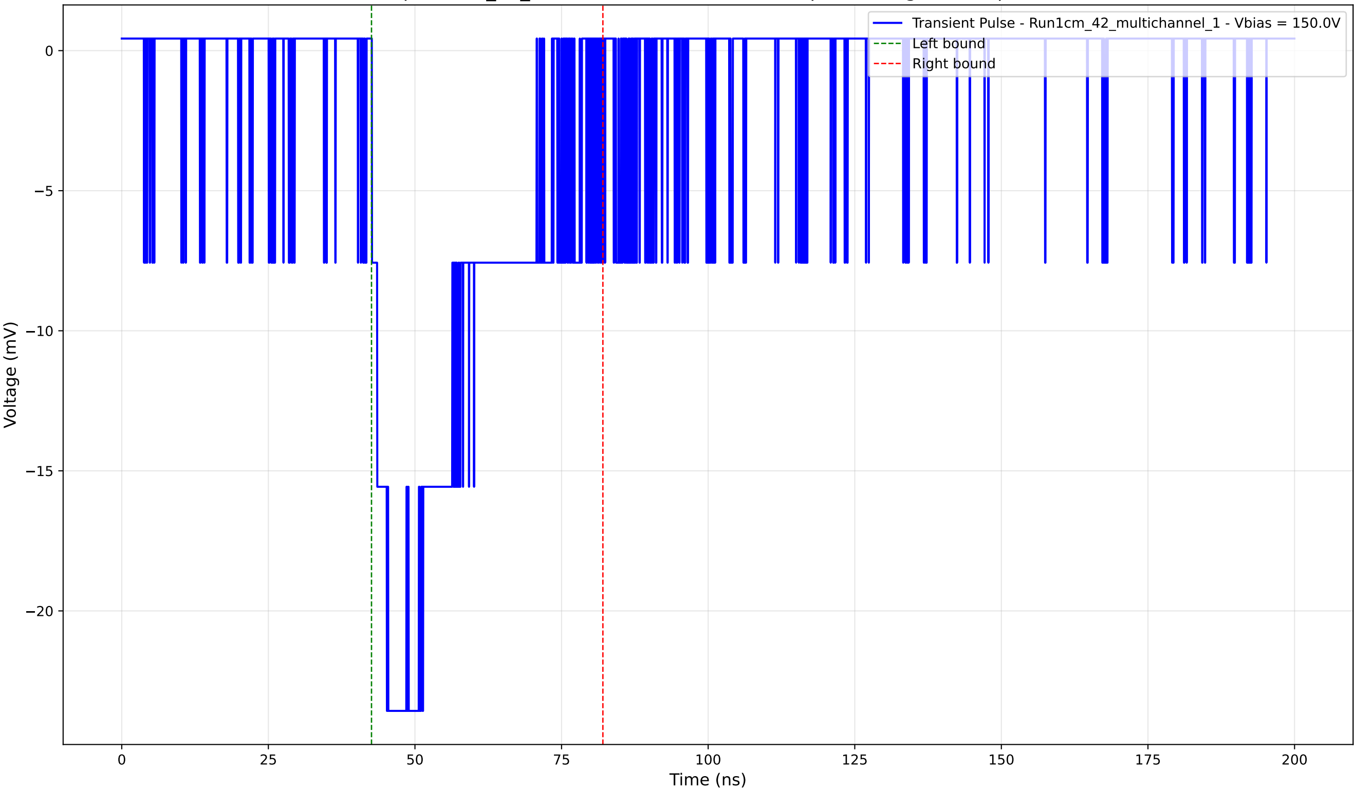
Transient Pulse - Sample: 1cm_42_multichannel - Position: 80.0 \mu\text{m} - Charge: -8.21 pC - Rise Time: 2.55 ns
