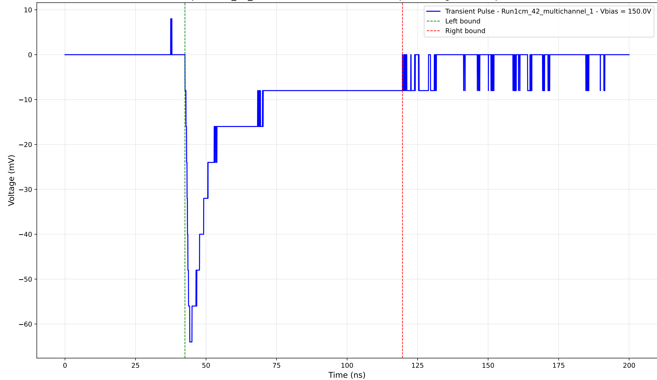
Transient Pulse - Sample: 1cm_42_multichannel - Position: 3710.0 \mu\text{m} - Charge: -21.58 pC - Rise Time: 1.68 ns
