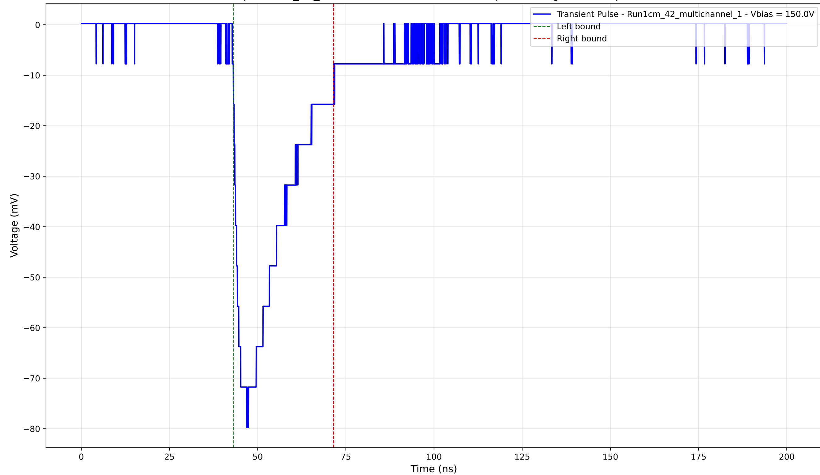
Transient Pulse - Sample: 1cm_42_multichannel - Position: 455.0 \mu\text{m} - Charge: -22.63 pC - Rise Time: 3.80 ns
