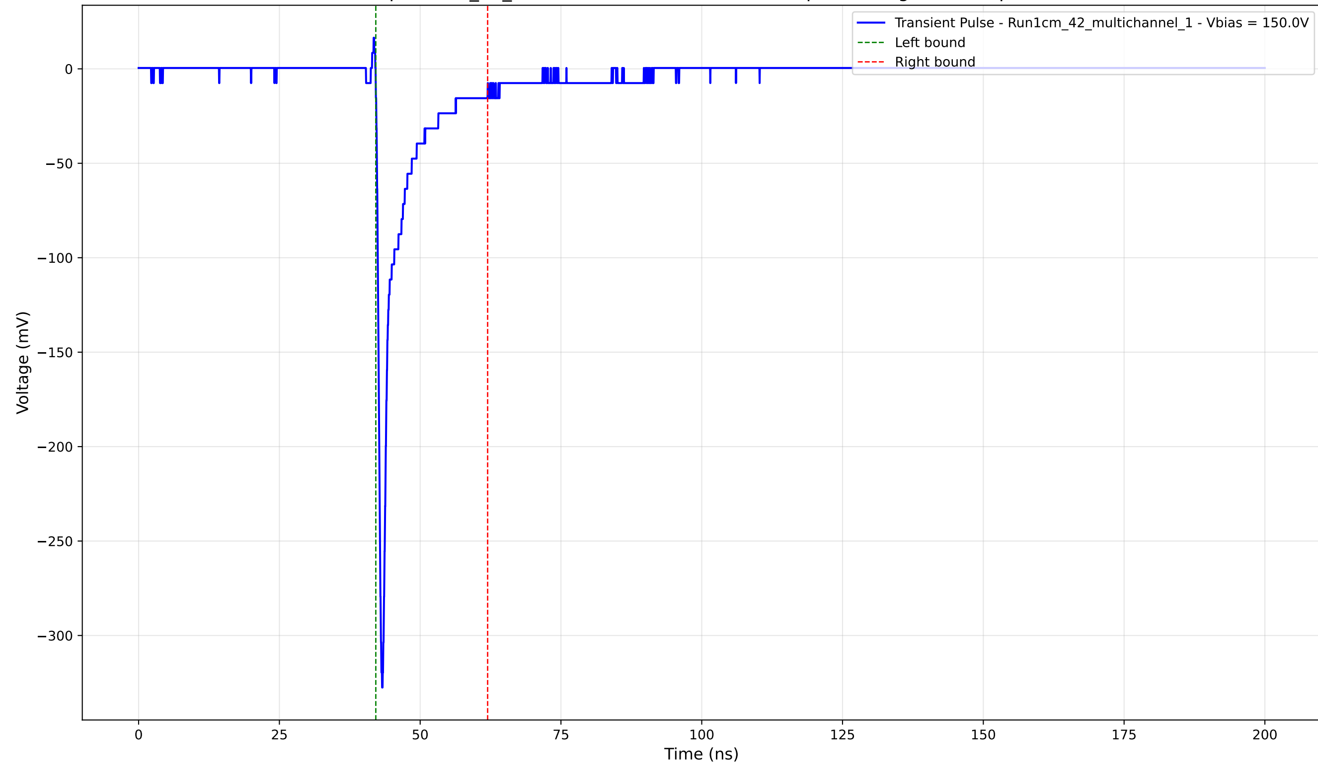
Transient Pulse - Sample: 1cm_42_multichannel - Position: 2610.0 \mu\text{m} - Charge: -22.71 pC - Rise Time: 0.74 ns
