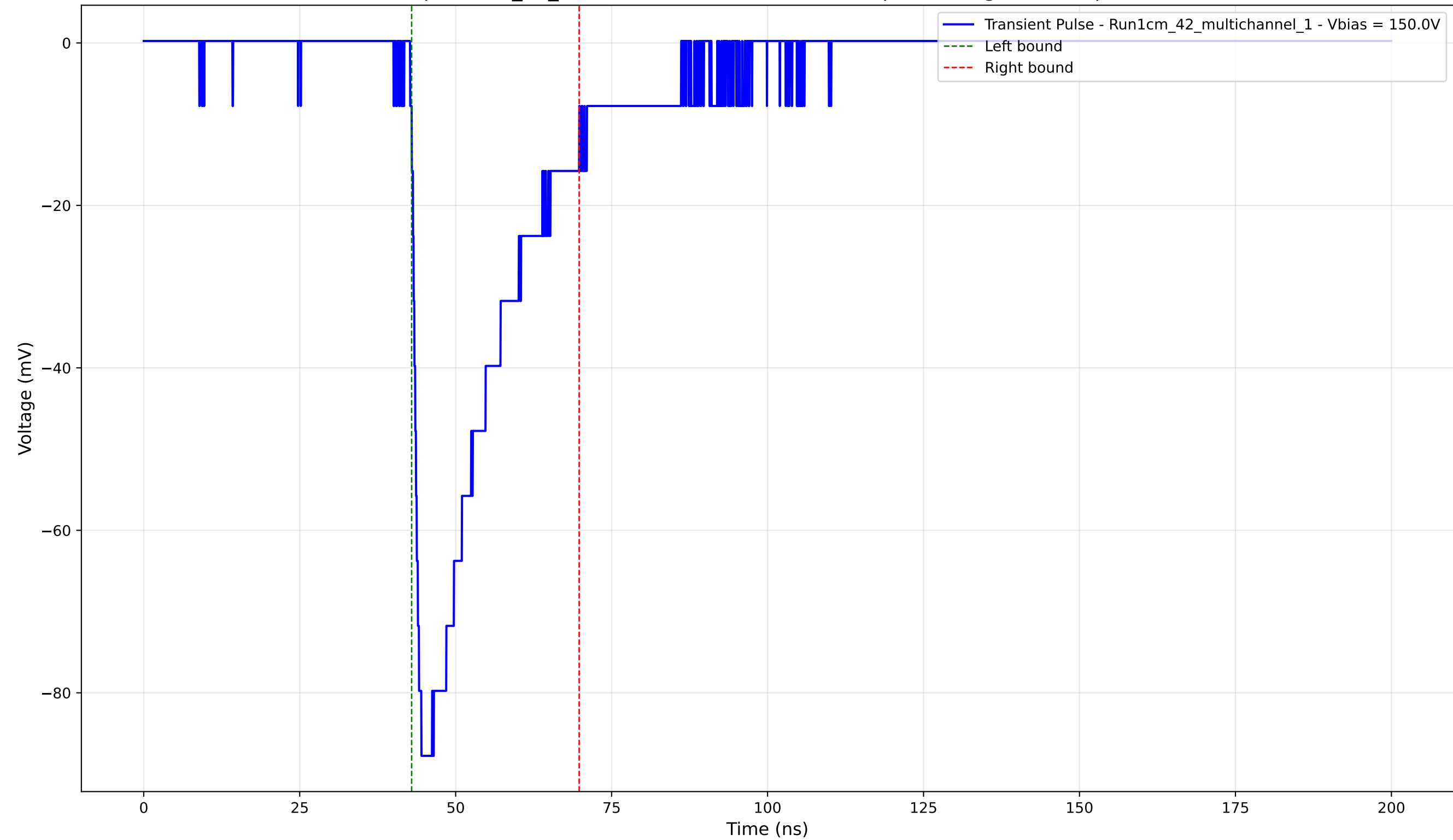
Transient Pulse - Sample: 1cm_42_multichannel - Position: 1000.0 \mu\text{m} - Charge: -23.18 pC - Rise Time: 1.18 ns
