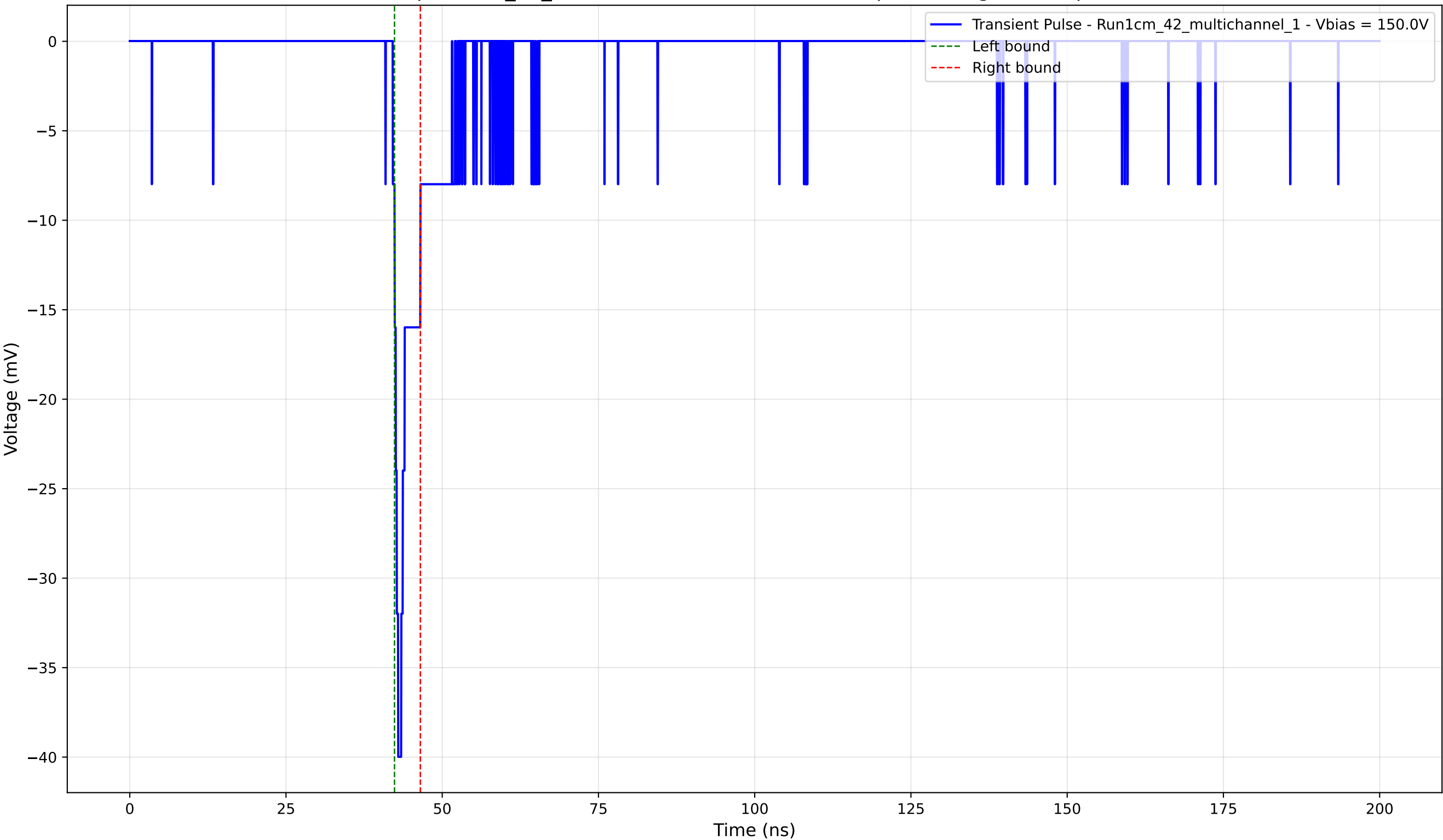
Transient Pulse - Sample: 1cm_42_multichannel - Position: 2360.0 \mu\text{m} - Charge: -1.78 pC - Rise Time: 0.87 ns
