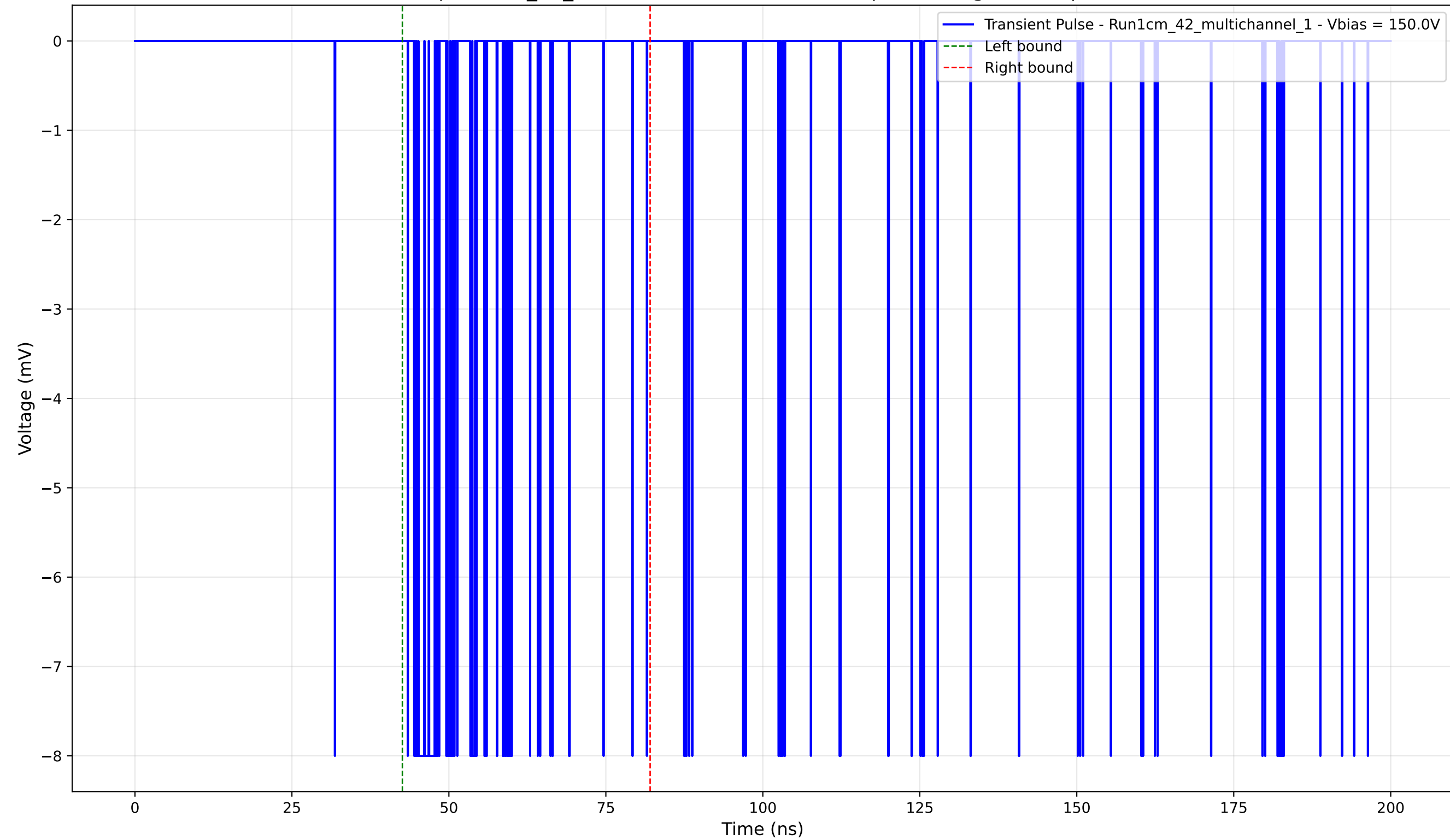
Transient Pulse - Sample: 1cm_42_multichannel - Position: 40.0 \mu\text{m} - Charge: -1.10 pC - Rise Time: 0.02 ns
