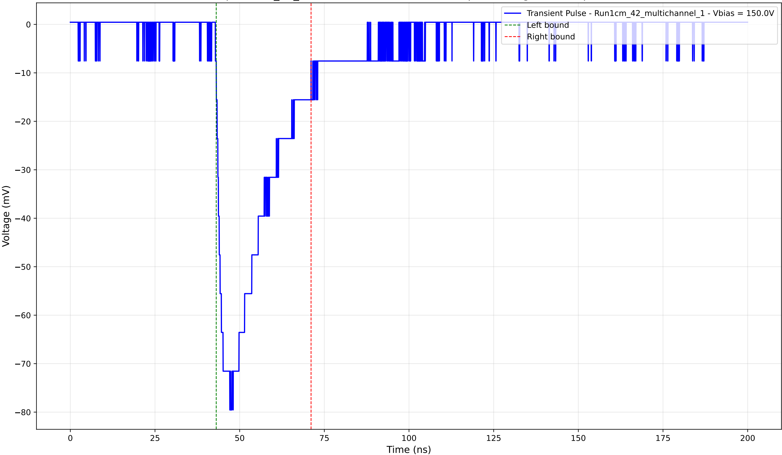
Transient Pulse - Sample: 1cm_42_multichannel - Position: 480.0 \mu\text{m} - Charge: -22.70 pC - Rise Time: 4.00 ns
