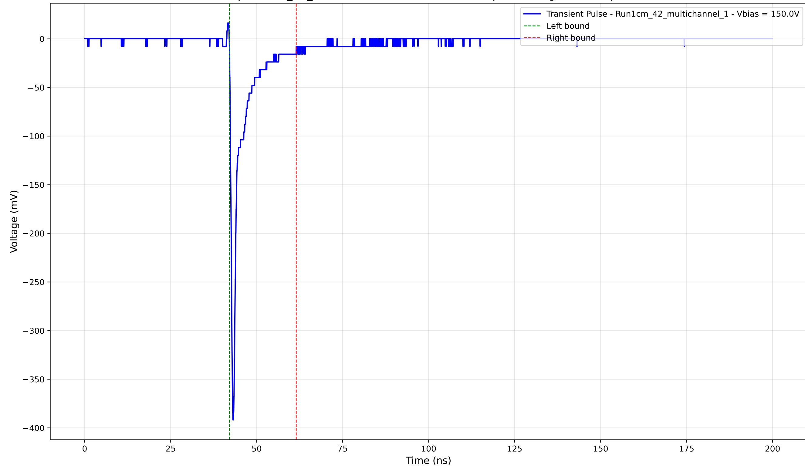
Transient Pulse - Sample: 1cm_42_multichannel - Position: 2255.0 \mu\text{m} - Charge: -24.67 pC - Rise Time: 0.74 ns
