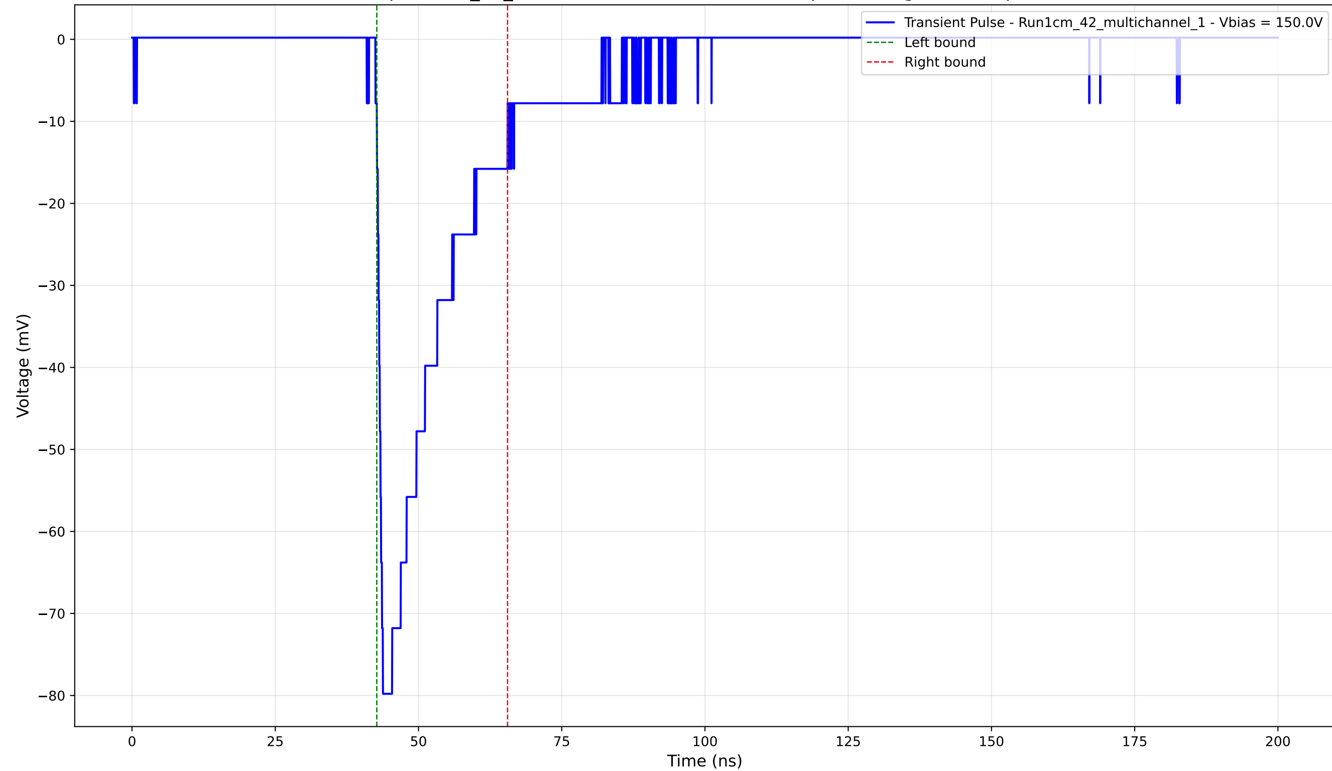
Transient Pulse - Sample: 1cm_42_multichannel - Position: 1305.0 \mu\text{m} - Charge: -17.39 pC - Rise Time: 1.06 ns
