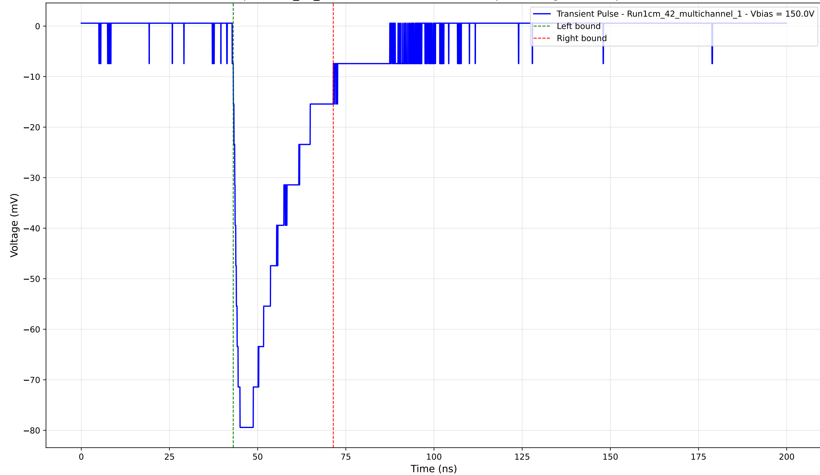
Transient Pulse - Sample: 1cm_42_multichannel - Position: 710.0 \mu\text{m} - Charge: -23.54 pC - Rise Time: 1.92 ns
