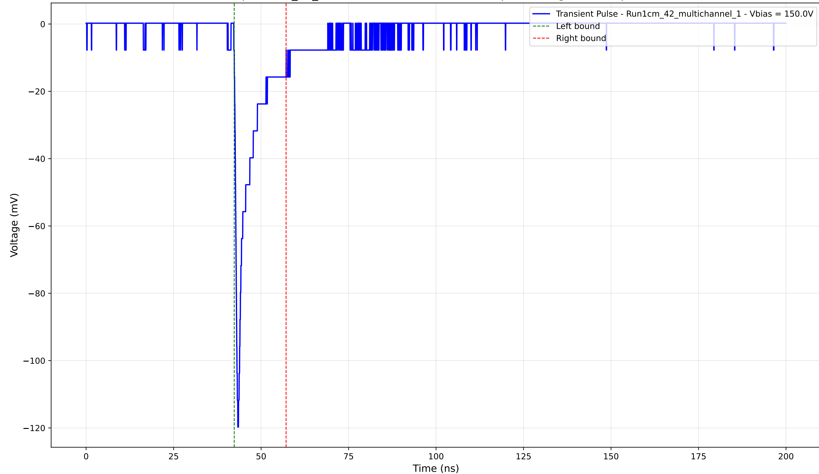
Transient Pulse - Sample: 1cm_42_multichannel - Position: 2840.0 \mu\text{m} - Charge: -10.44 pC - Rise Time: 0.87 ns
