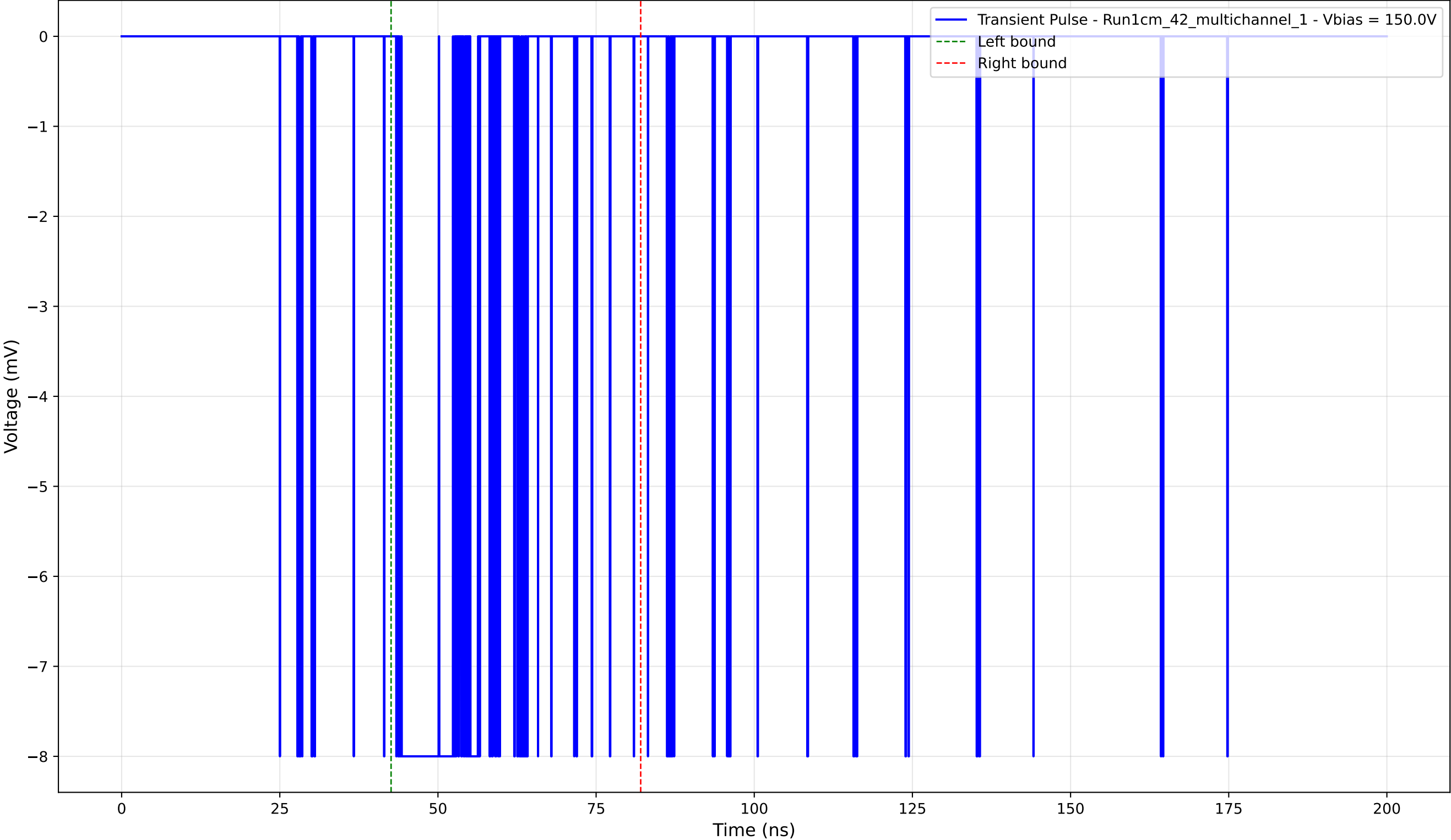
Transient Pulse - Sample: 1cm_42_multichannel - Position: 360.0 \mu\text{m} - Charge: -2.13 pC - Rise Time: 0.02 ns
