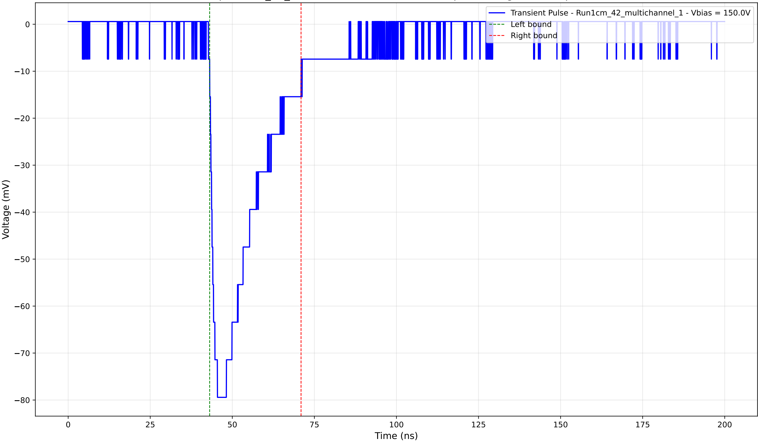
Transient Pulse - Sample: 1cm_42_multichannel - Position: 640.0 \mu\text{m} - Charge: -22.98 pC - Rise Time: 2.36 ns
