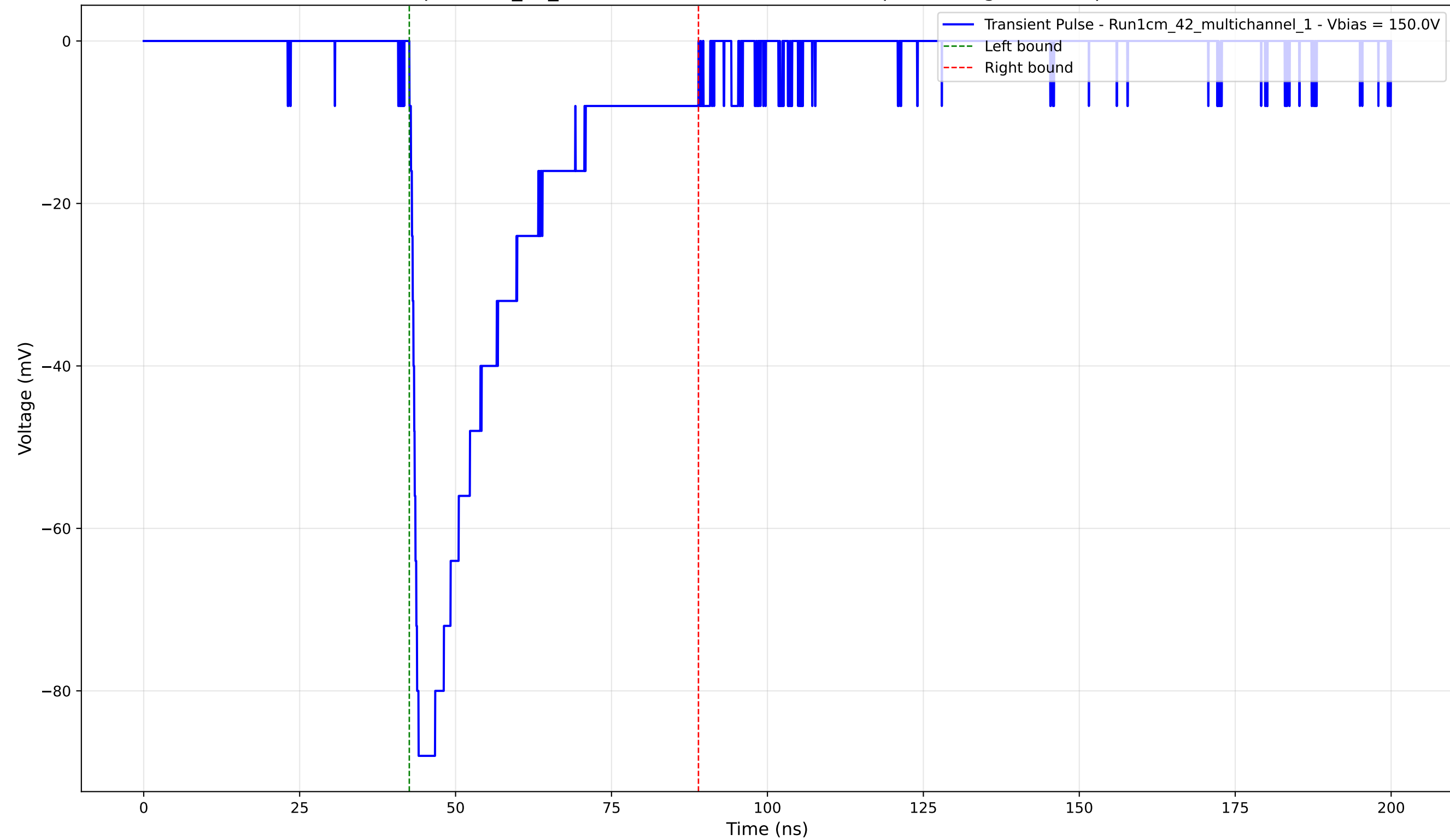
Transient Pulse - Sample: 1cm_42_multichannel - Position: 1130.0 \mu\text{m} - Charge: -26.22 pC - Rise Time: 1.00 ns
