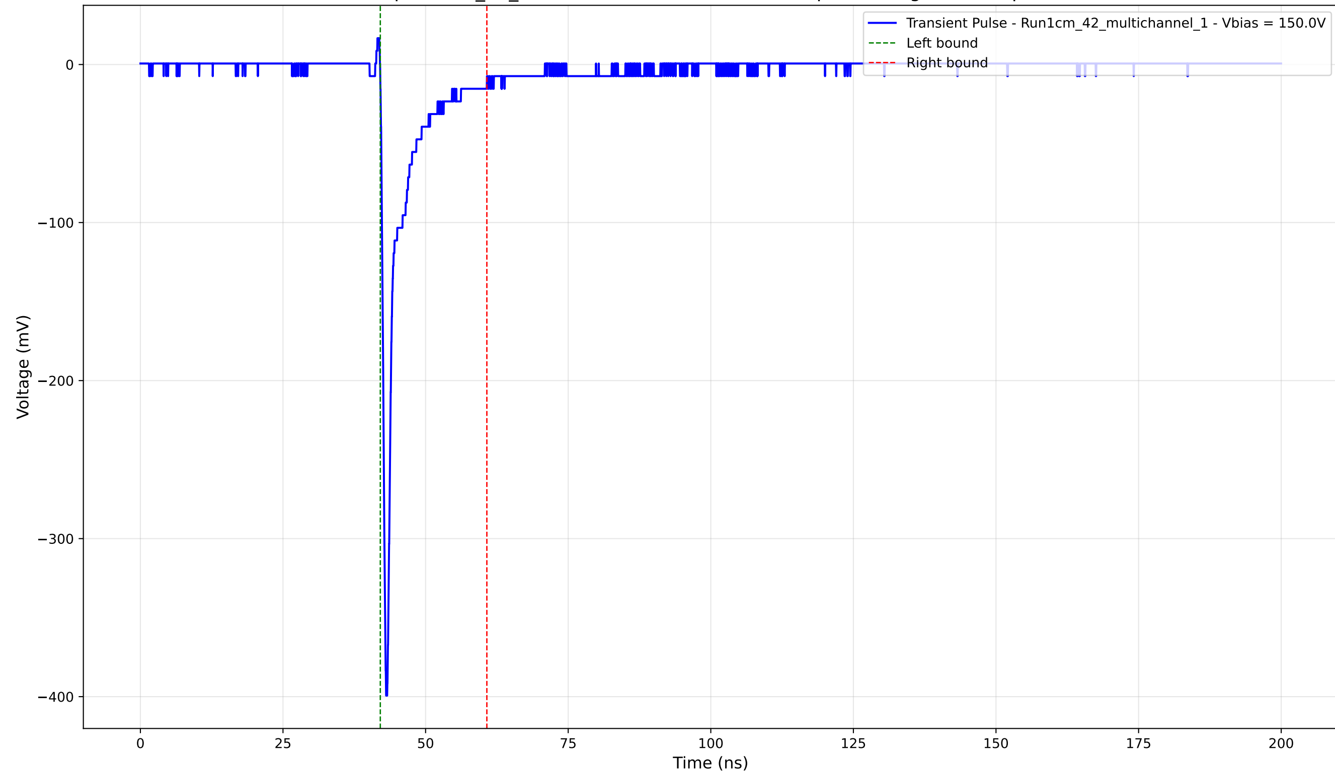
Transient Pulse - Sample: 1cm_42_multichannel - Position: 2285.0 \mu\text{m} - Charge: -24.05 pC - Rise Time: 0.72 ns
