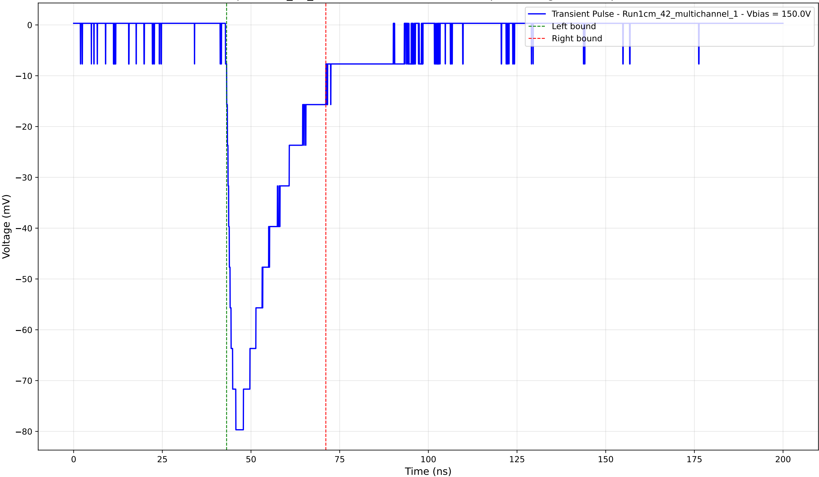
Transient Pulse - Sample: 1cm_42_multichannel - Position: 590.0 \mu\text{m} - Charge: -22.76 pC - Rise Time: 2.60 ns
