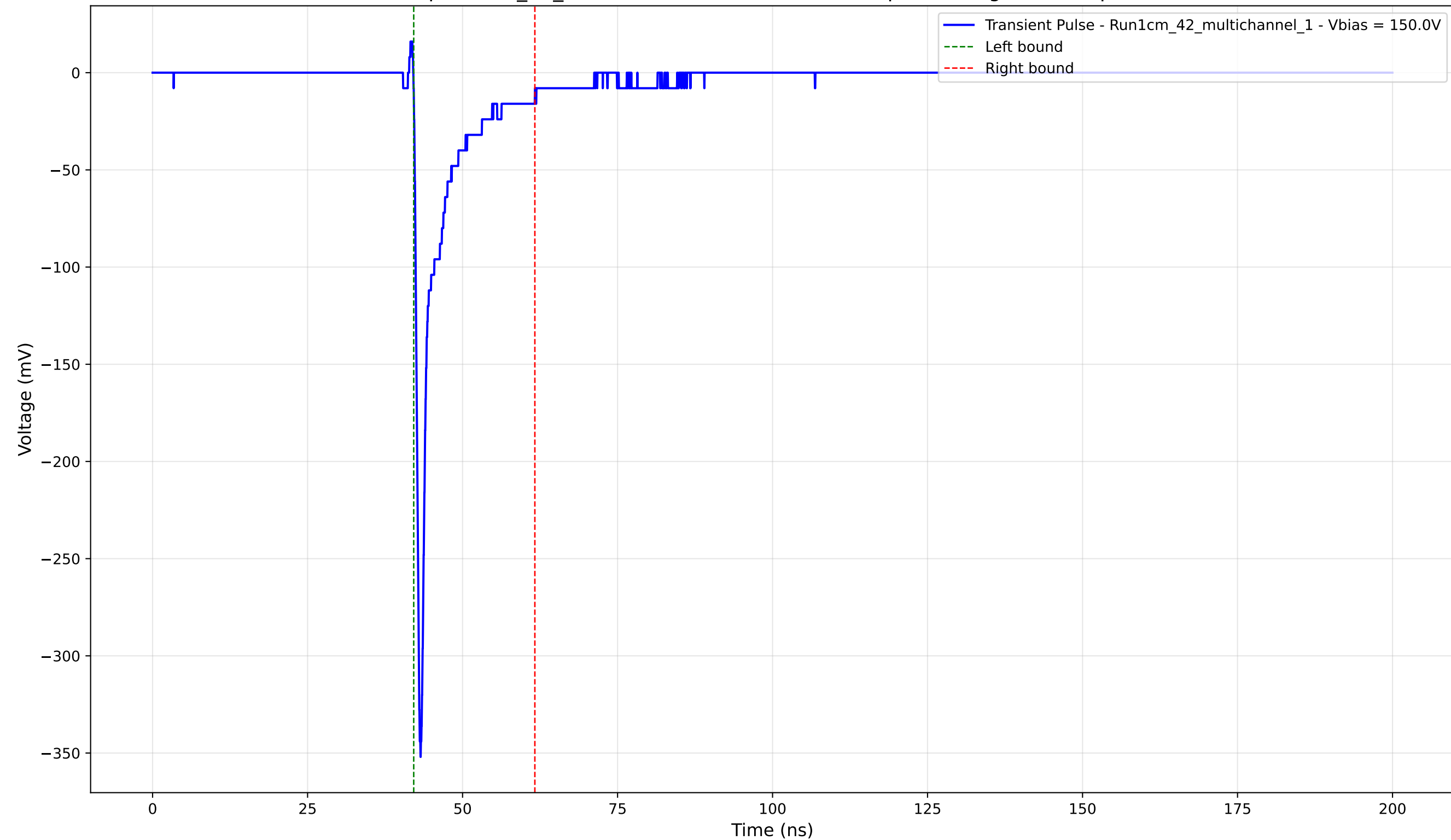
Transient Pulse - Sample: 1cm_42_multichannel - Position: 2570.0 \mu\text{m} - Charge: -23.11 pC - Rise Time: 0.75 ns
