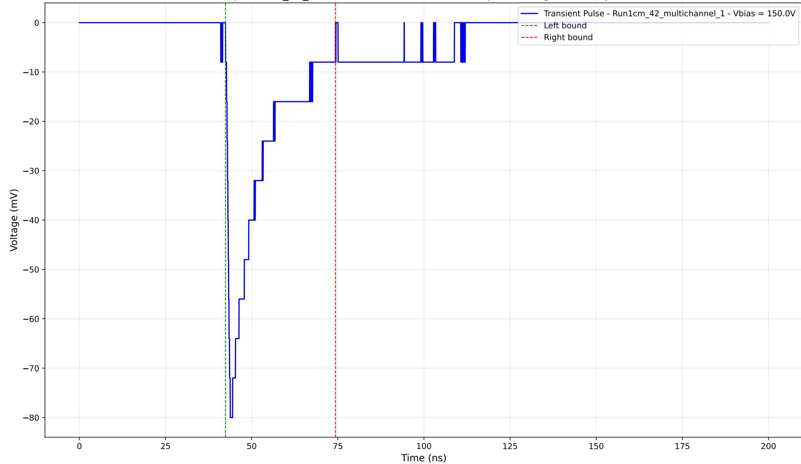
Transient Pulse - Sample: 1cm_42_multichannel - Position: 3495.0 \mu\text{m} - Charge: -16.60 pC - Rise Time: 0.90 ns
