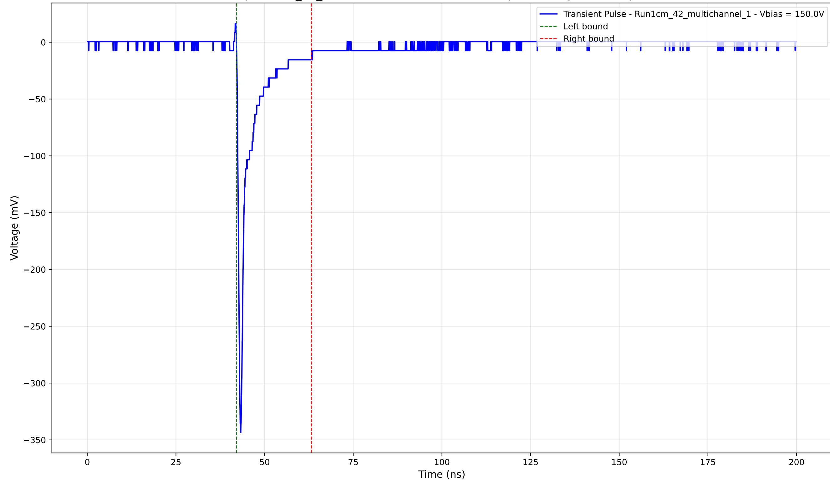
Transient Pulse - Sample: 1cm_42_multichannel - Position: 2595.0 \mu\text{m} - Charge: -23.79 pC - Rise Time: 0.75 ns
