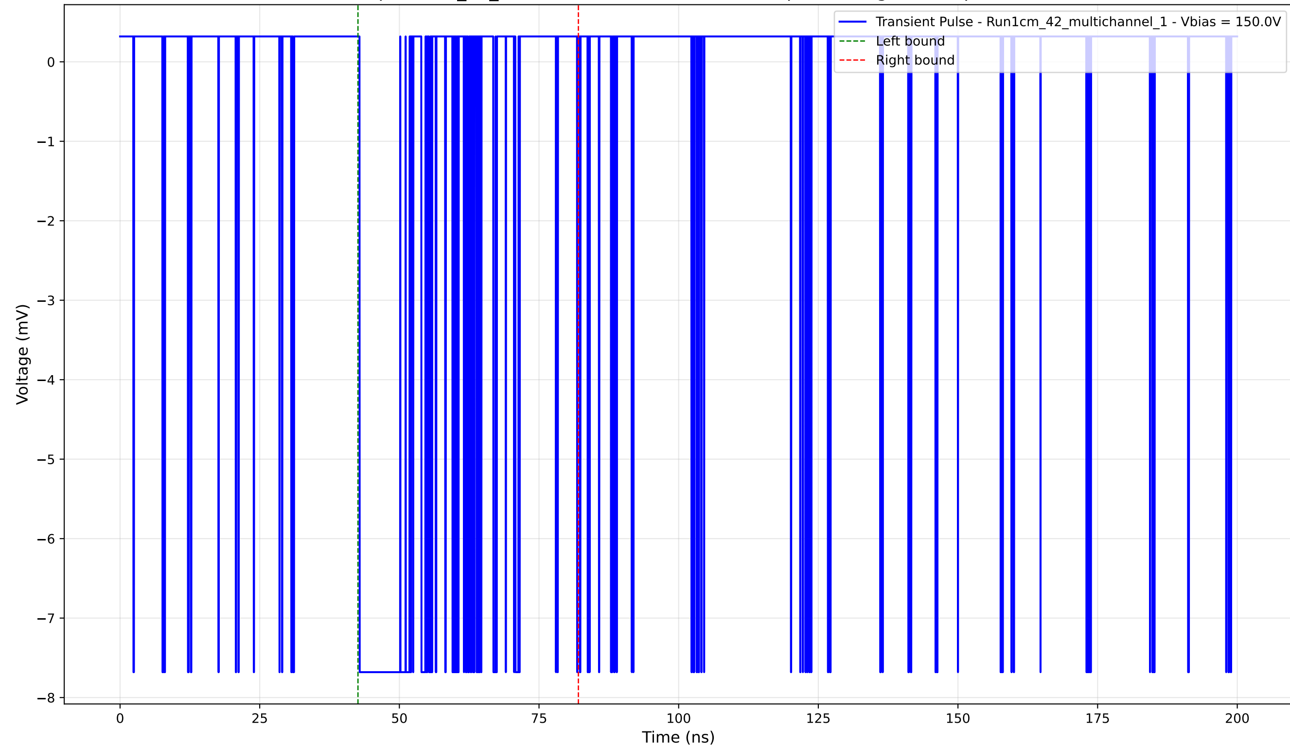
Transient Pulse - Sample: 1cm_42_multichannel - Position: 1370.0 \mu\text{m} - Charge: -1.91 pC - Rise Time: 0.02 ns
