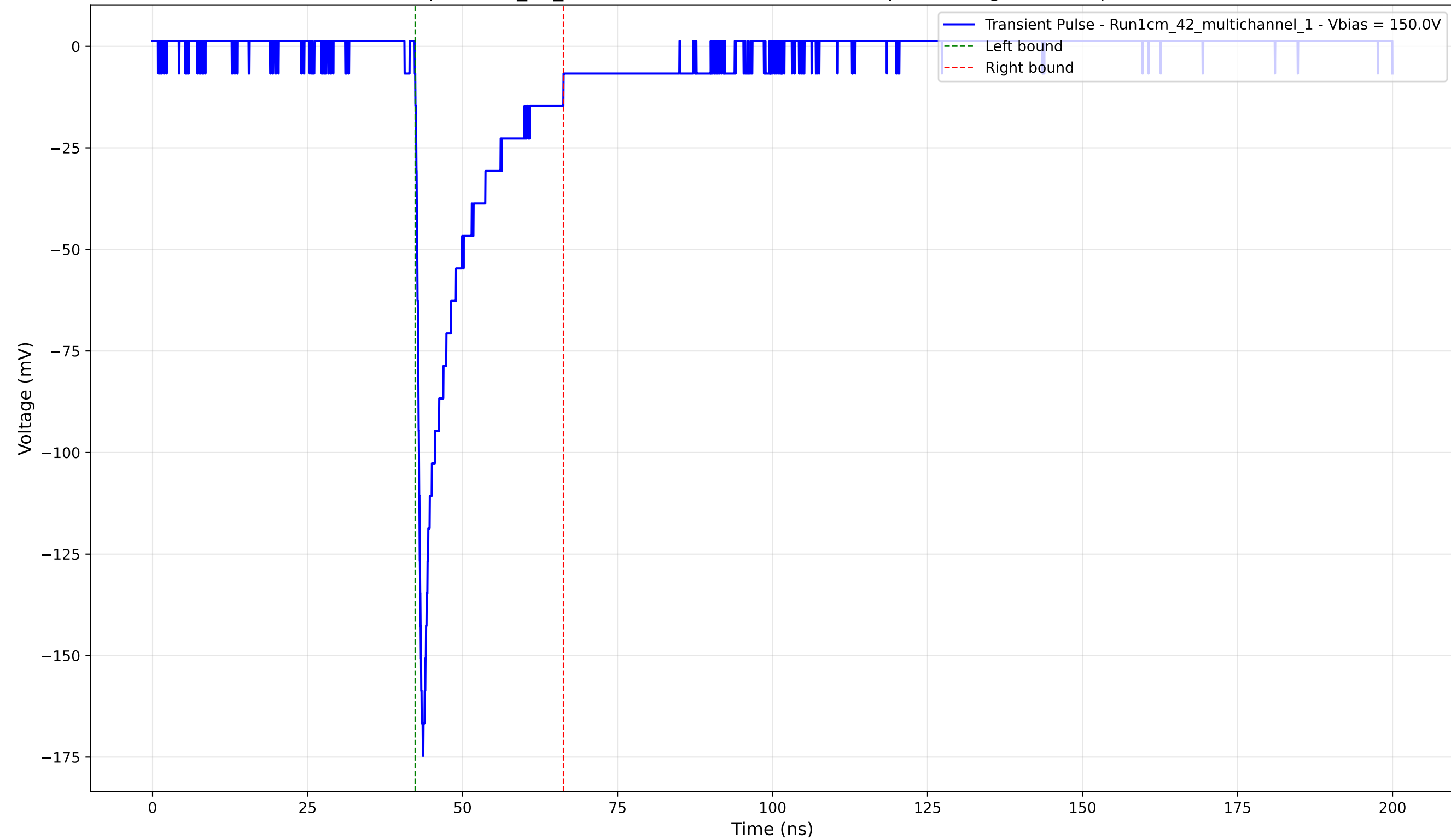
Transient Pulse - Sample: 1cm_42_multichannel - Position: 1745.0 \mu\text{m} - Charge: -22.15 pC - Rise Time: 0.87 ns
