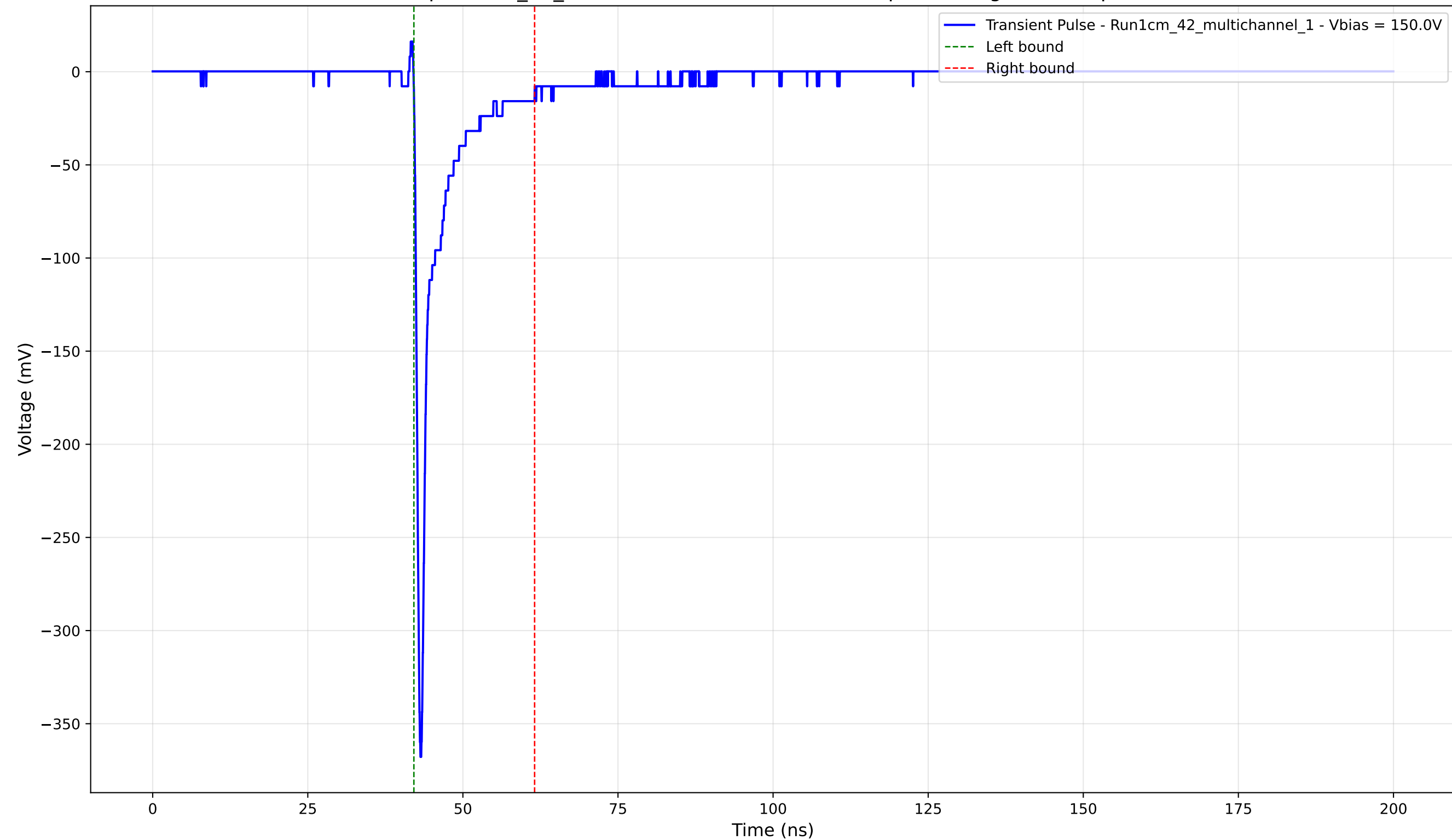
Transient Pulse - Sample: 1cm_42_multichannel - Position: 2545.0 \mu\text{m} - Charge: -23.63 pC - Rise Time: 0.76 ns
