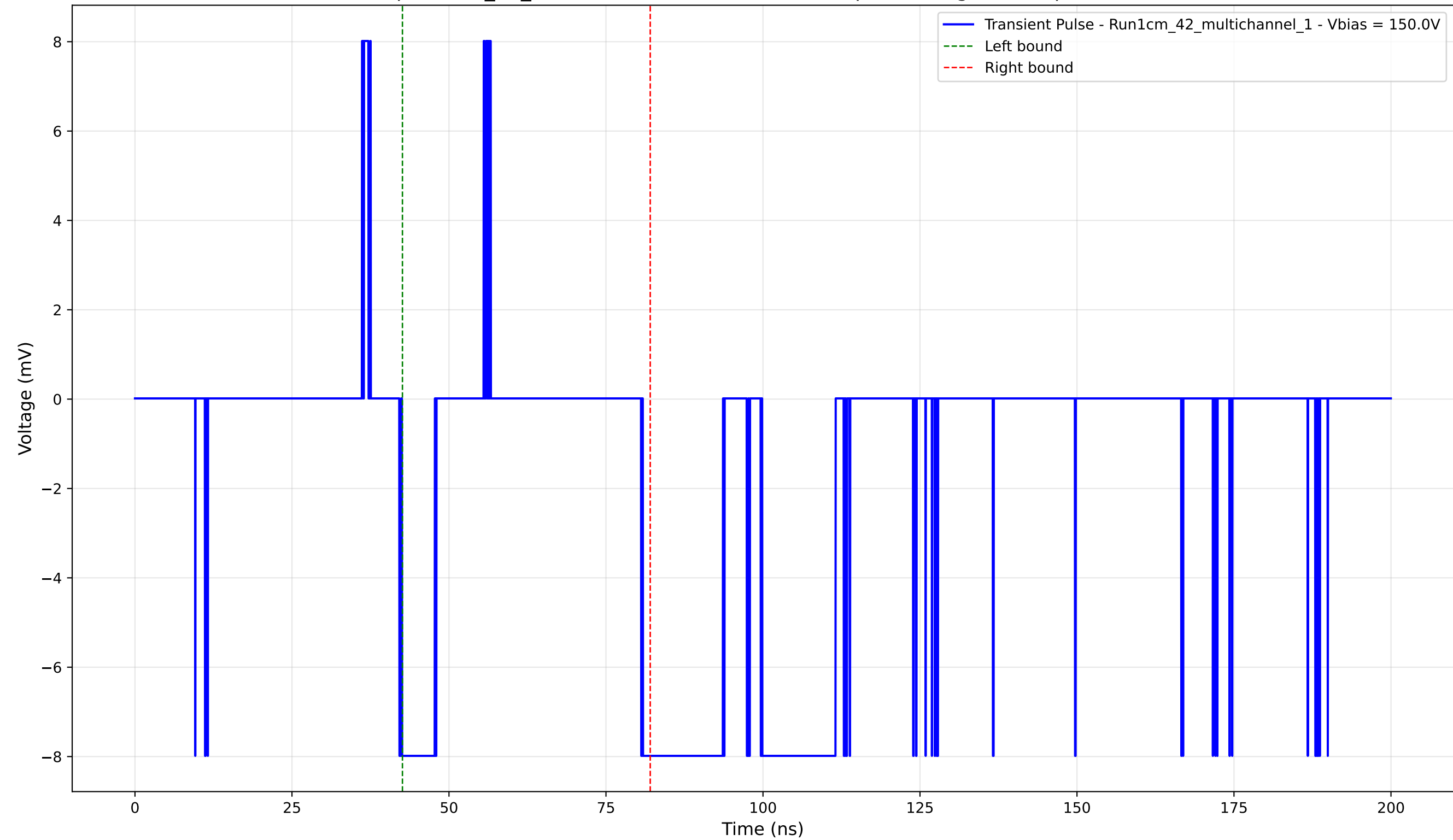
Transient Pulse - Sample: 1cm_42_multichannel - Position: 3920.0 \mu\text{m} - Charge: -0.93 pC - Rise Time: 0.00 ns (N/A)
