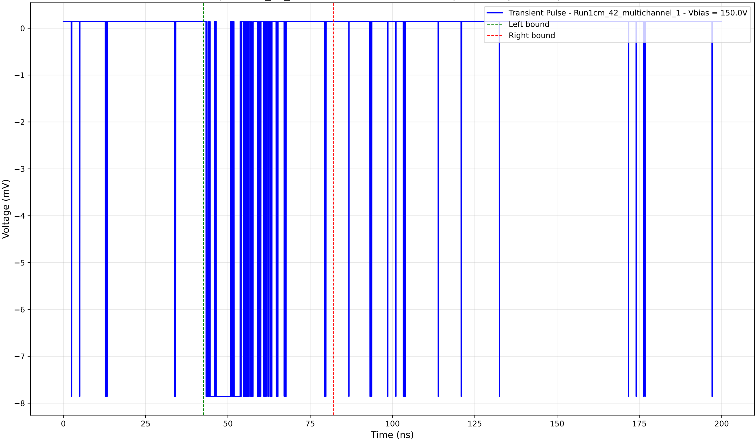
Transient Pulse - Sample: 1cm_42_multichannel - Position: 350.0 \mu\text{m} - Charge: -1.94 pC - Rise Time: 0.02 ns
