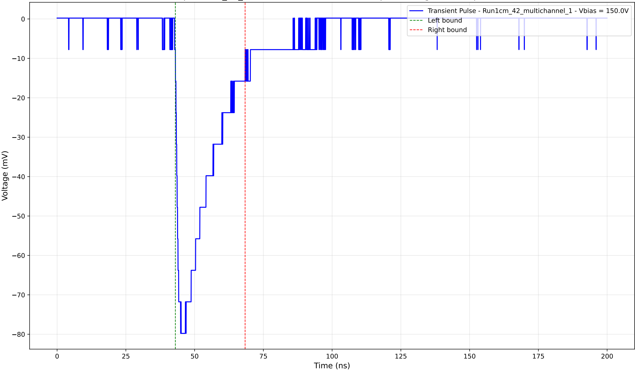
Transient Pulse - Sample: 1cm_42_multichannel - Position: 945.0 \mu\text{m} - Charge: -21.12 pC - Rise Time: 1.90 ns
