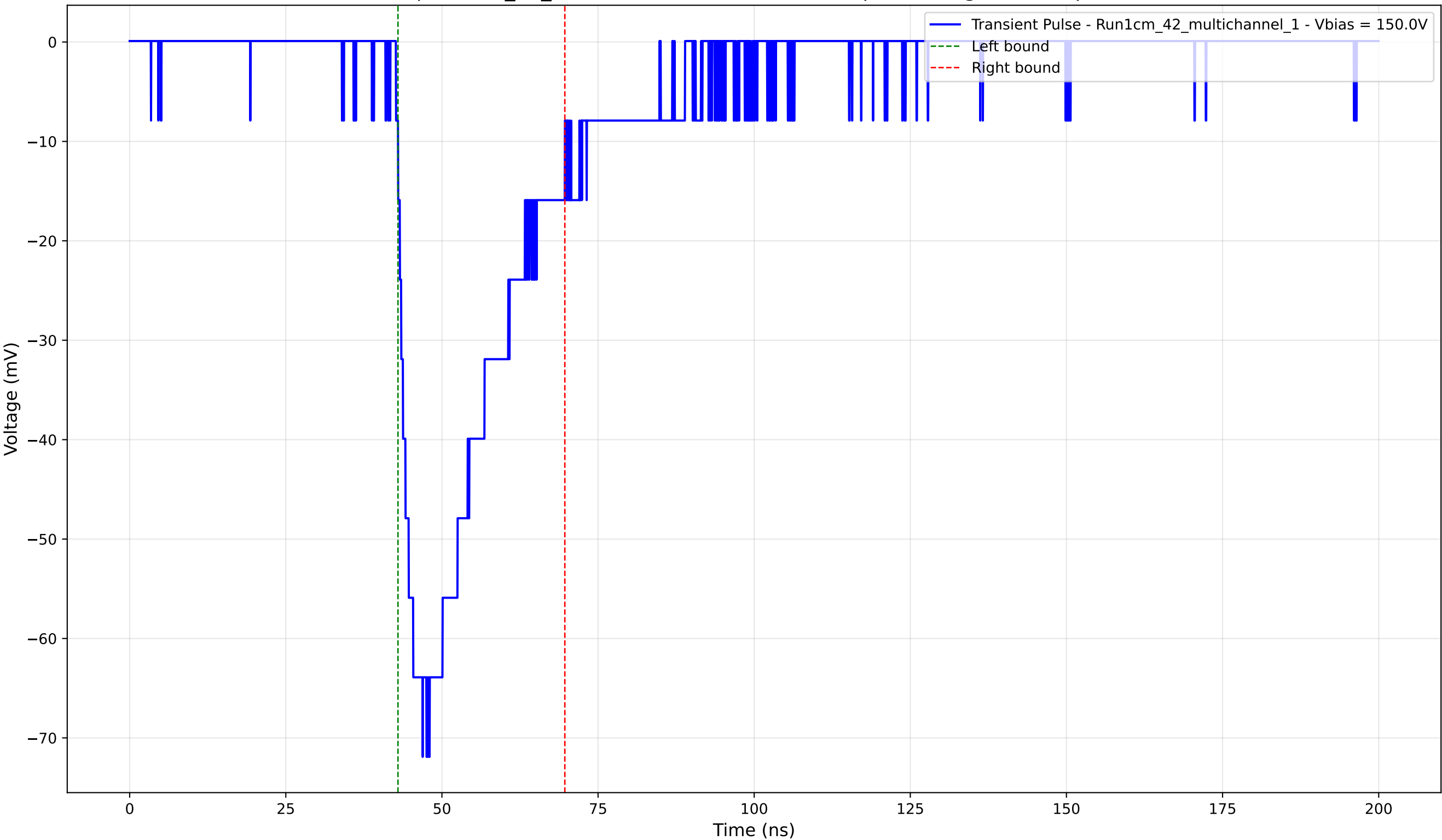
Transient Pulse - Sample: 1cm_42_multichannel - Position: 210.0 \mu\text{m} - Charge: -20.31 pC - Rise Time: 4.26 ns
