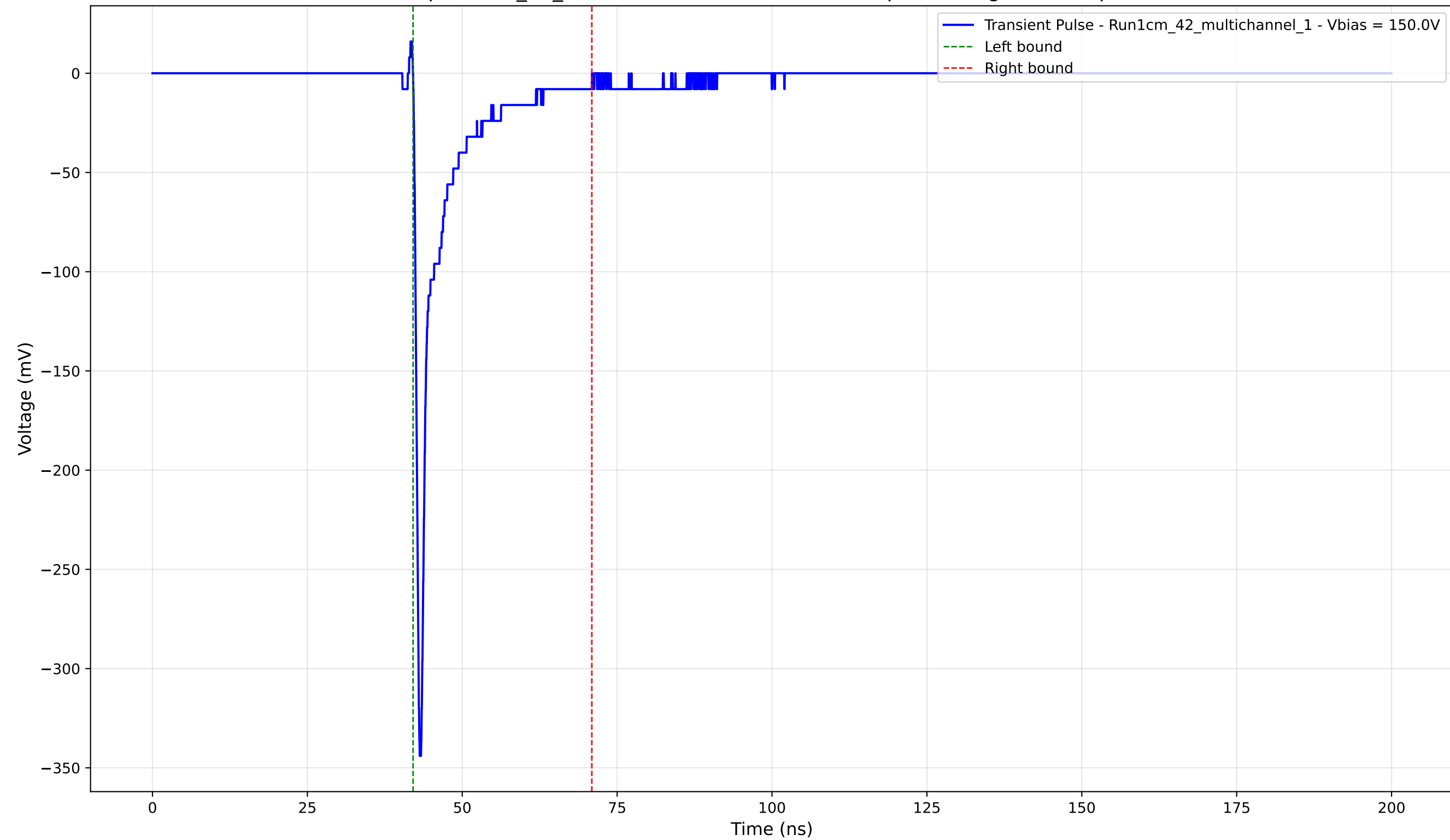
Transient Pulse - Sample: 1cm_42_multichannel - Position: 2575.0 \mu\text{m} - Charge: -24.80 pC - Rise Time: 0.75 ns
