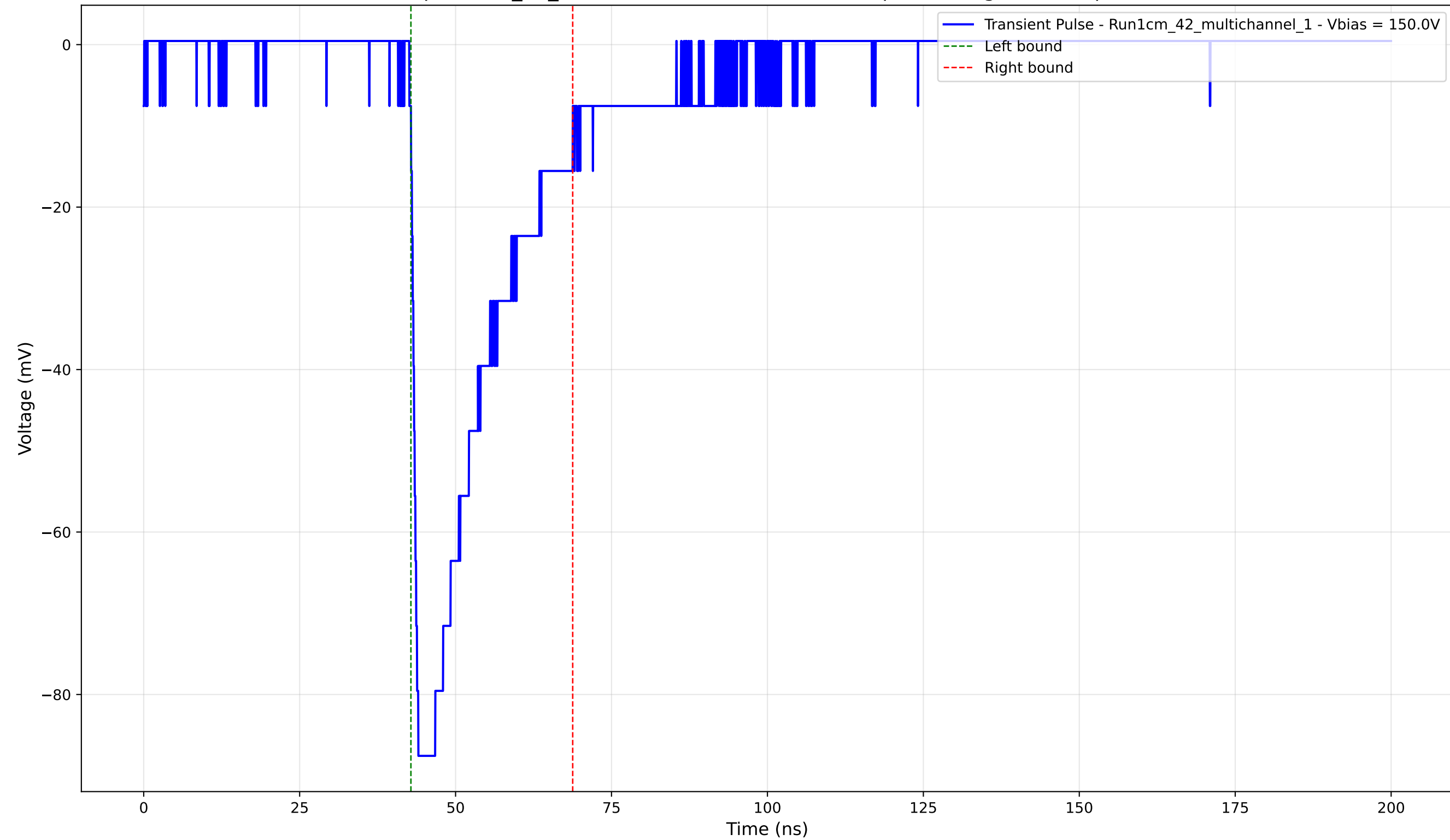
Transient Pulse - Sample: 1cm_42_multichannel - Position: 1145.0 \mu\text{m} - Charge: -22.14 pC - Rise Time: 0.98 ns
