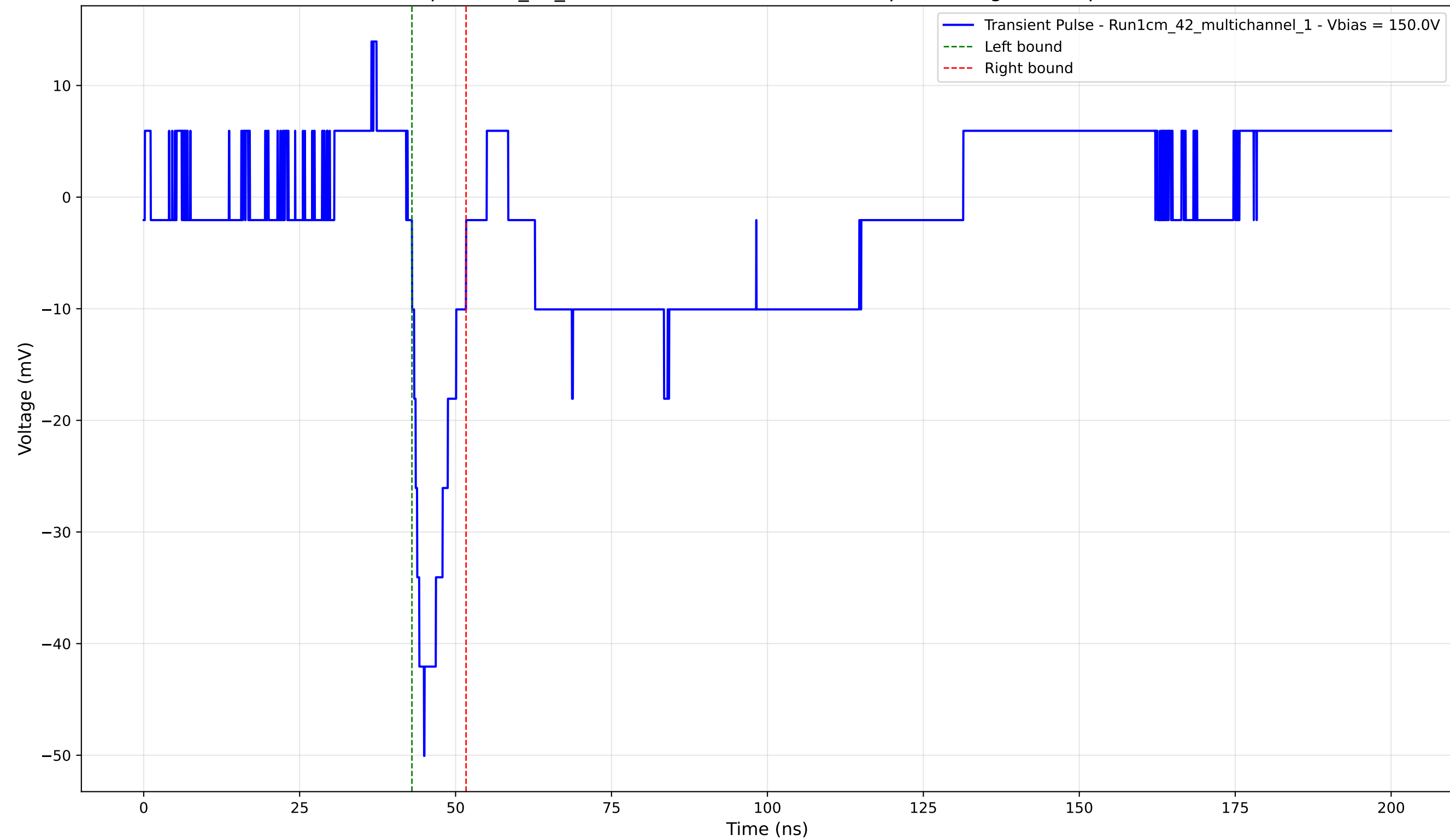
Transient Pulse - Sample: 1cm_42_multichannel - Position: 4055.0 \mu\text{m} - Charge: -4.74 pC - Rise Time: 1.93 ns
