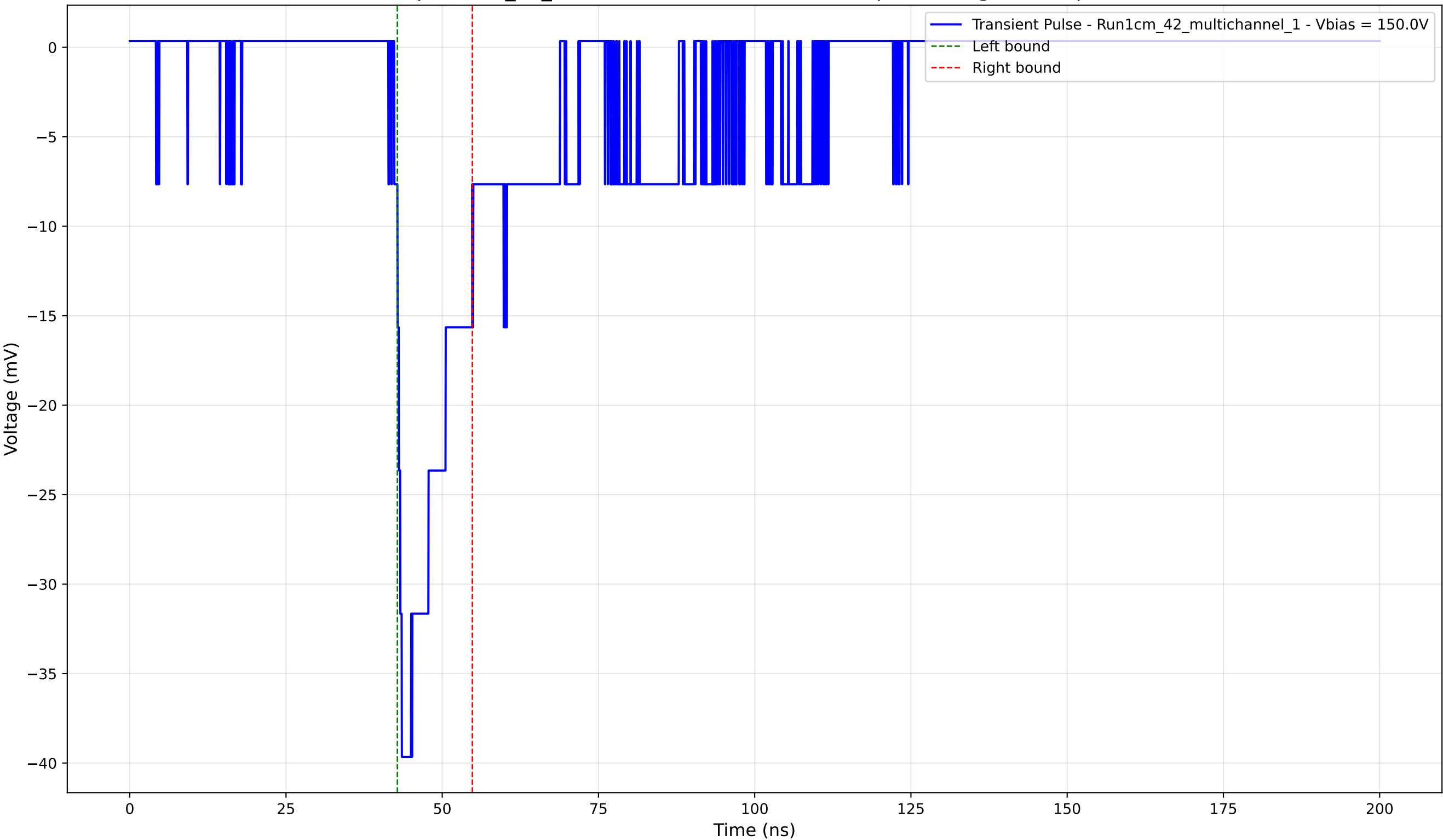
Transient Pulse - Sample: 1cm_42_multichannel - Position: 3450.0 \mu\text{m} - Charge: -5.93 pC - Rise Time: 1.21 ns
