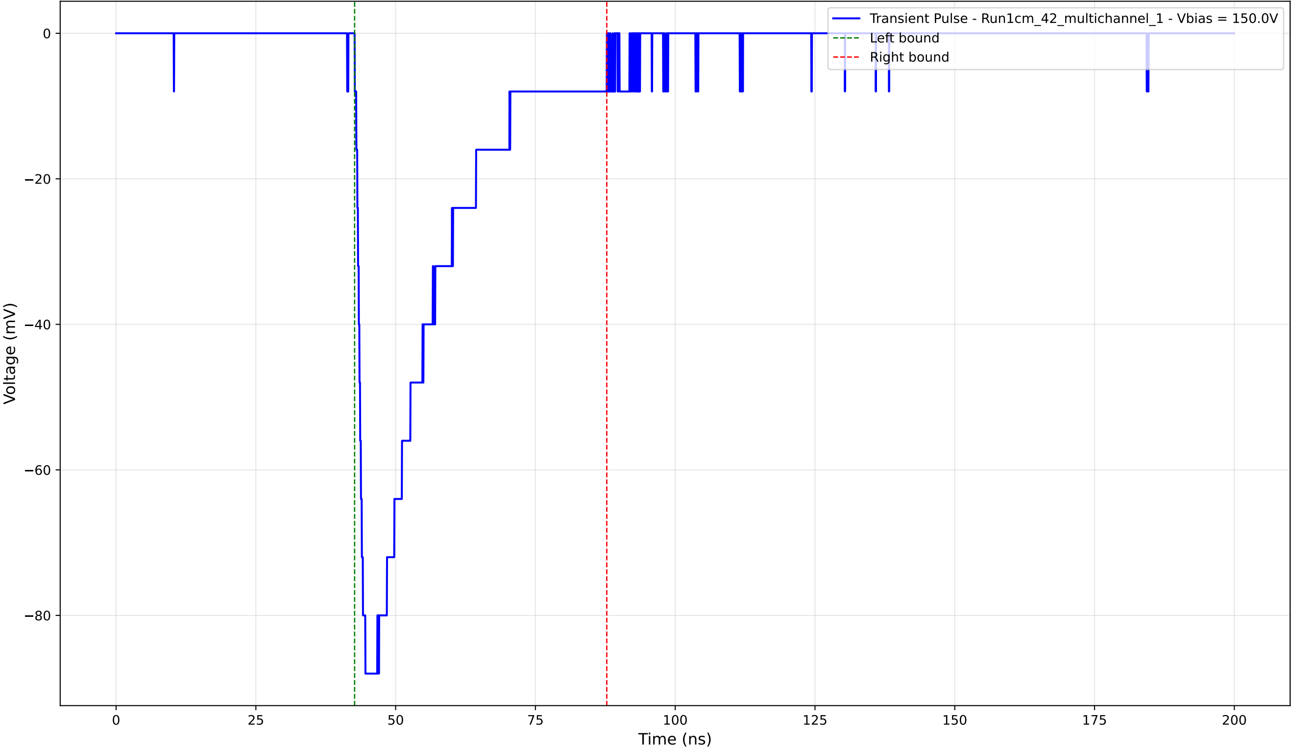
Transient Pulse - Sample: 1cm_42_multichannel - Position: 990.0 \mu\text{m} - Charge: -26.29 pC - Rise Time: 1.20 ns
