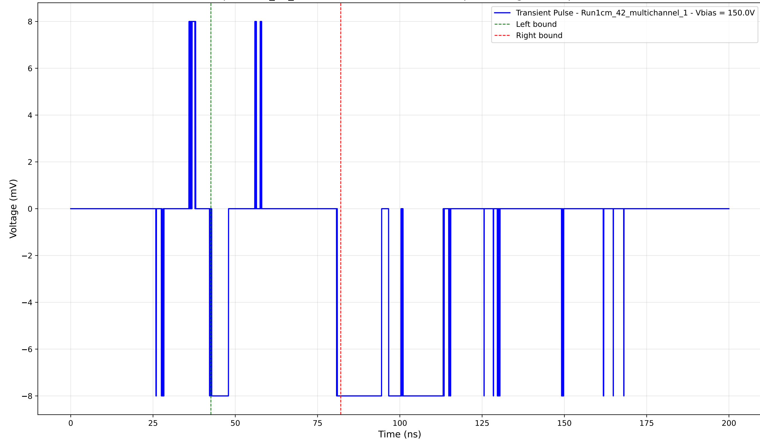
Transient Pulse - Sample: 1cm_42_multichannel - Position: 4390.0 \mu\text{m} - Charge: -0.91 pC - Rise Time: 0.02 ns
