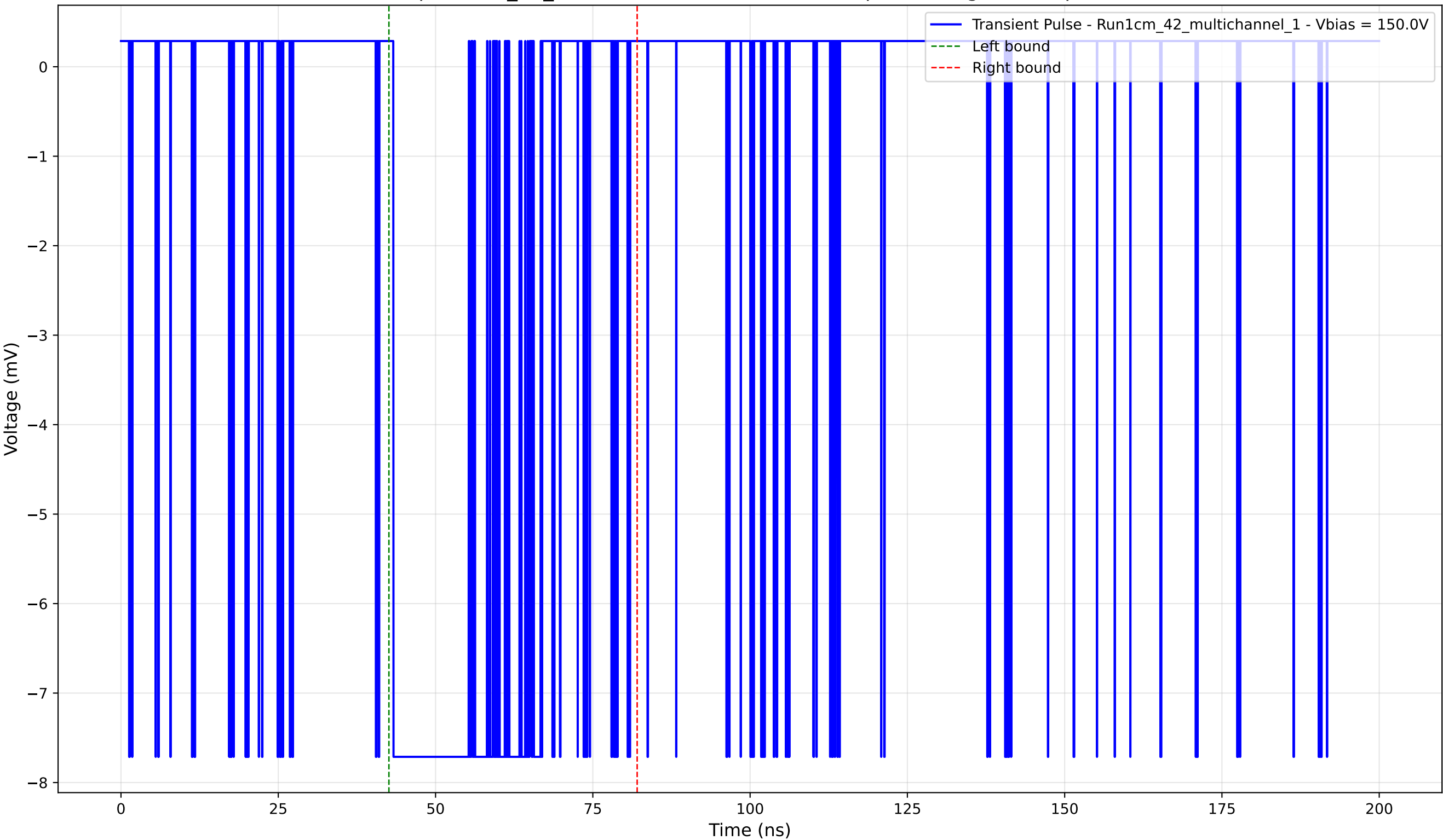
Transient Pulse - Sample: 1cm_42_multichannel - Position: 845.0 \mu\text{m} - Charge: -3.40 pC - Rise Time: 0.02 ns
