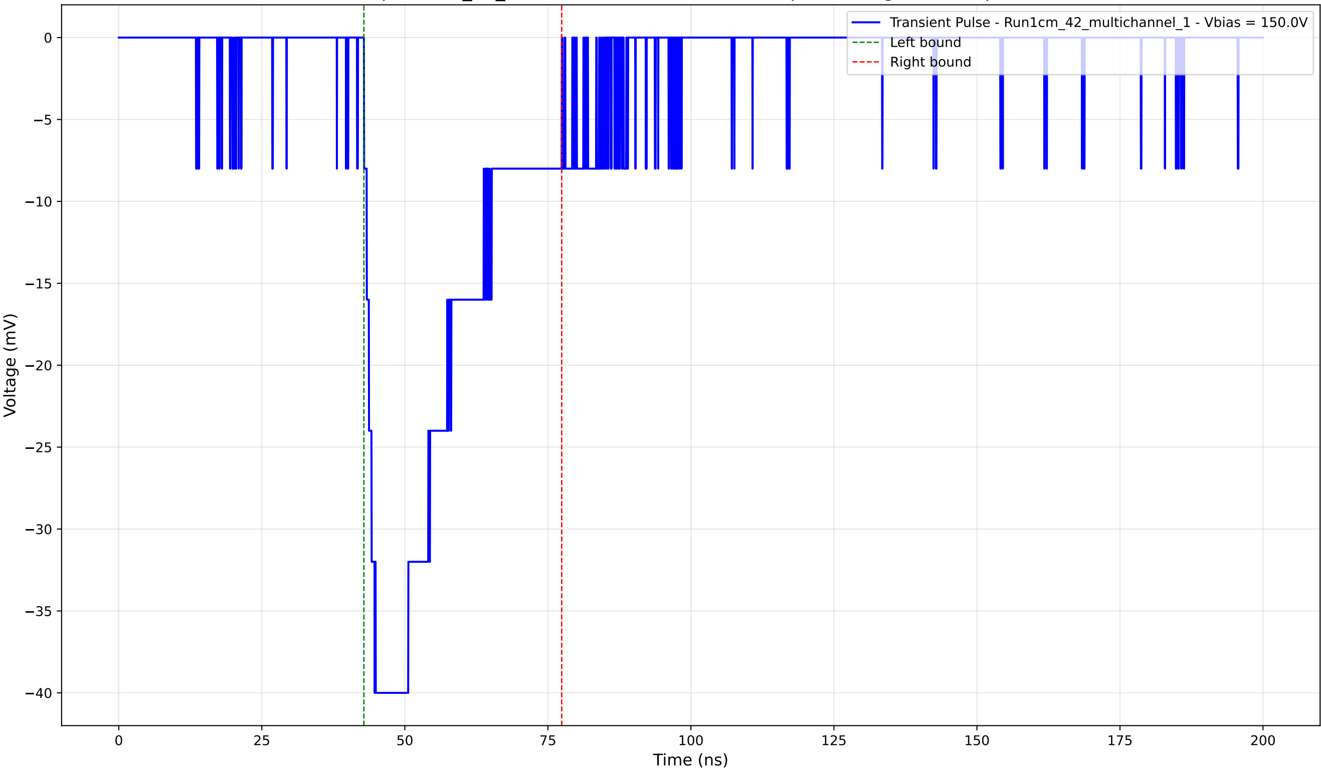
Transient Pulse - Sample: 1cm_42_multichannel - Position: 415.0 \mu\text{m} - Charge: -13.69 pC - Rise Time: 1.87 ns
