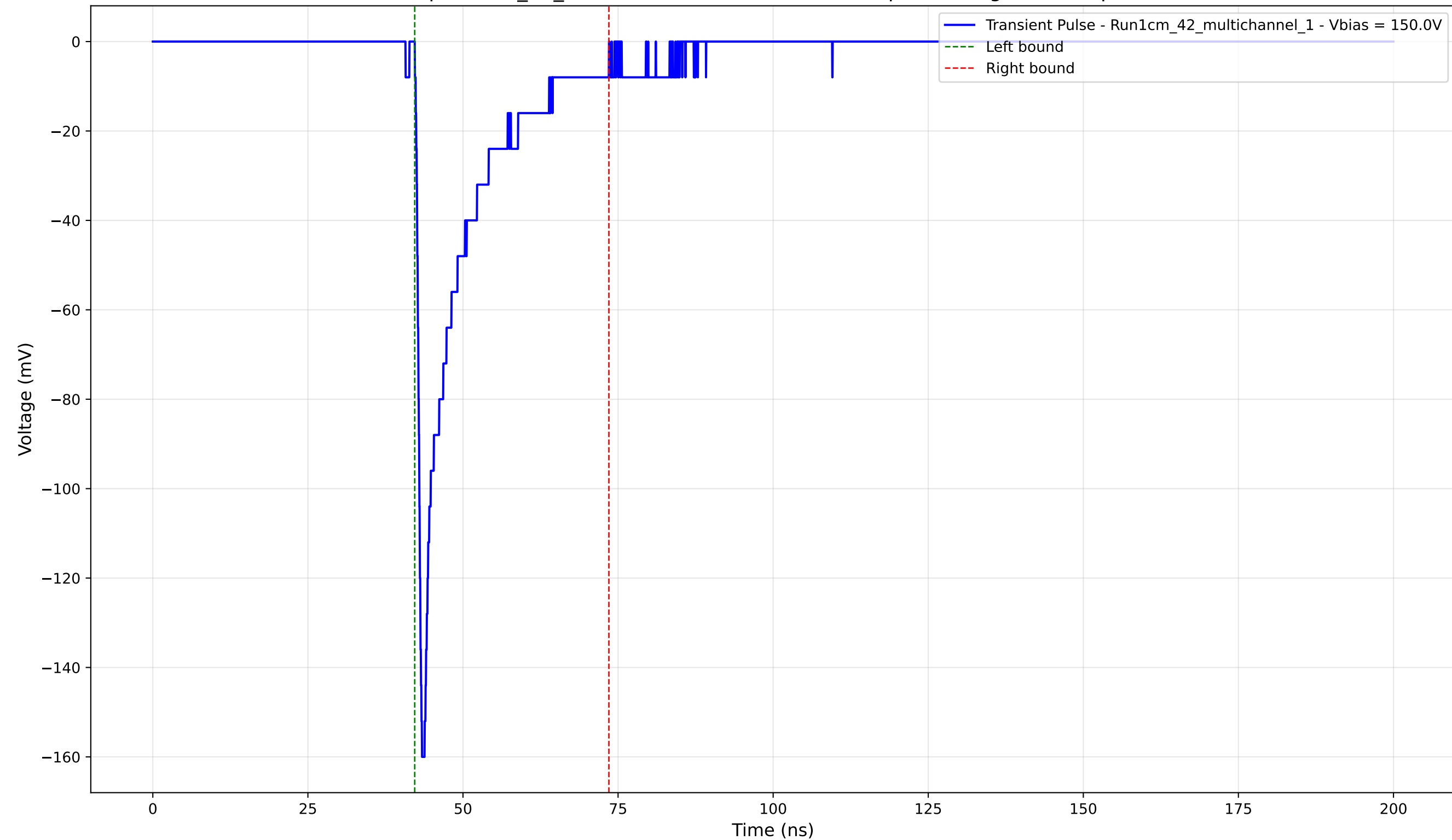
Transient Pulse - Sample: 1cm_42_multichannel - Position: 3020.0 \mu\text{m} - Charge: -21.23 pC - Rise Time: 0.78 ns
