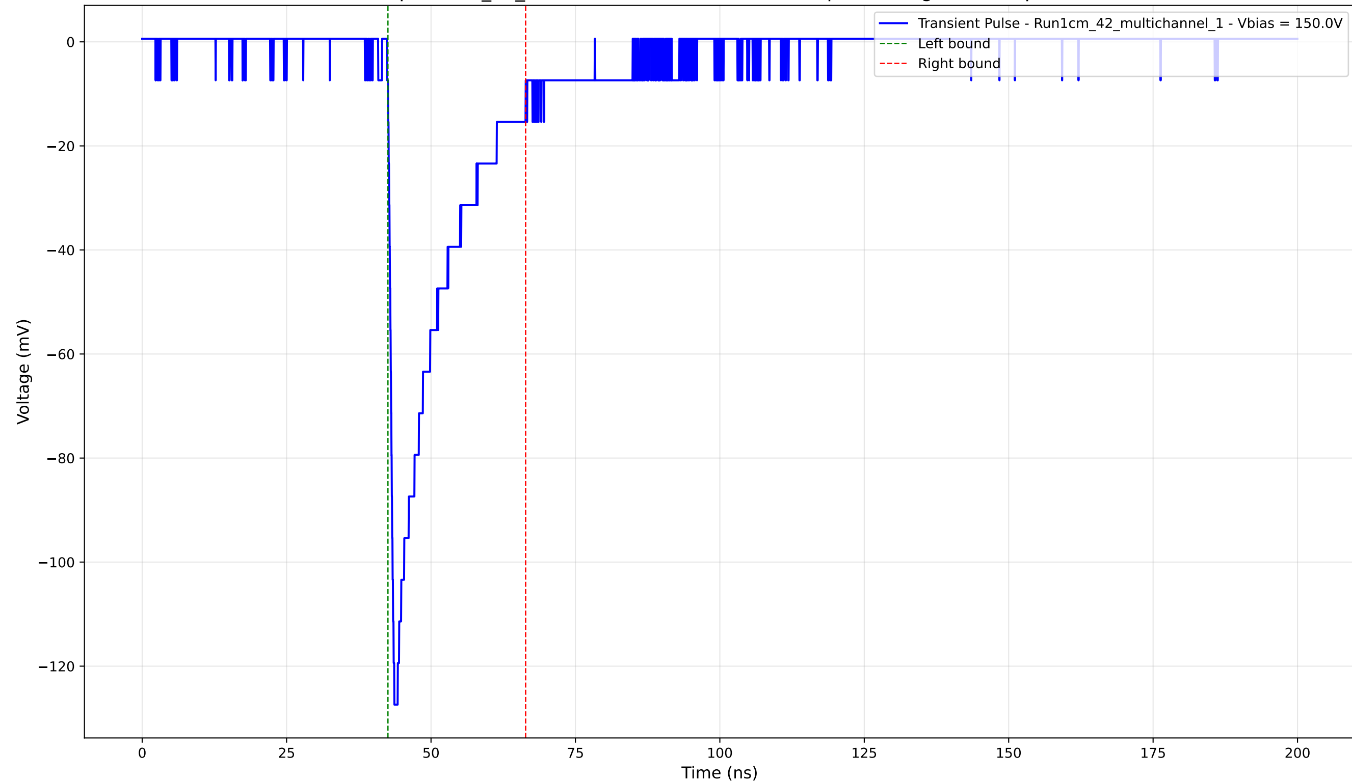
Transient Pulse - Sample: 1cm_42_multichannel - Position: 1510.0 \mu\text{m} - Charge: -22.28 pC - Rise Time: 0.97 ns
