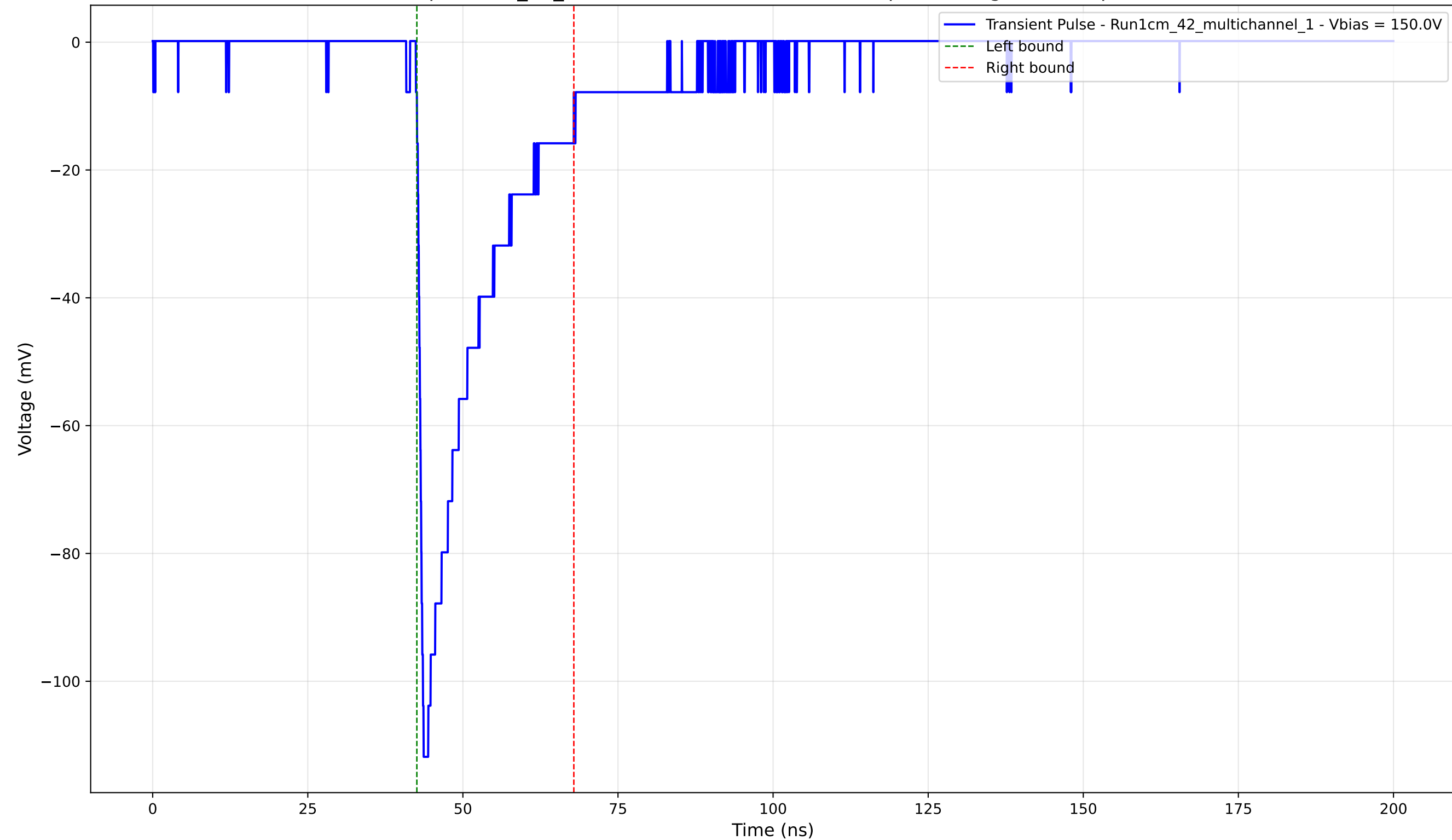
Transient Pulse - Sample: 1cm_42_multichannel - Position: 1455.0 \mu\text{m} - Charge: -21.80 pC - Rise Time: 0.97 ns
