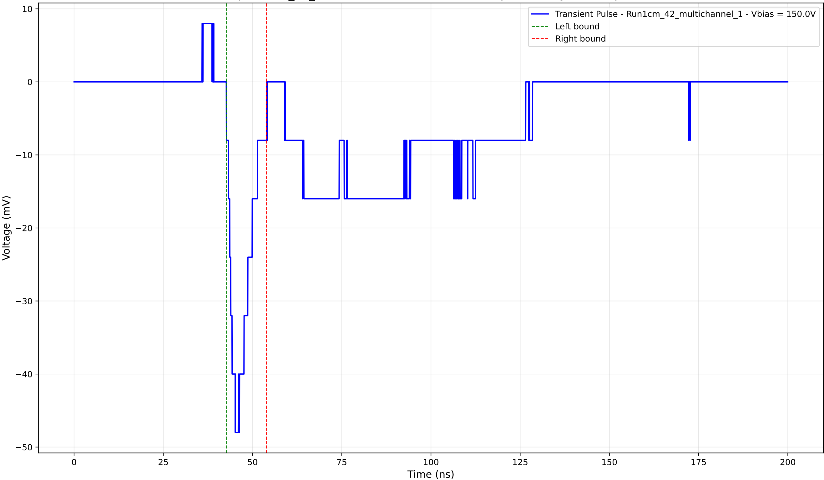
Transient Pulse - Sample: 1cm_42_multichannel - Position: 4315.0 \mu\text{m} - Charge: -5.59 pC - Rise Time: 2.51 ns
