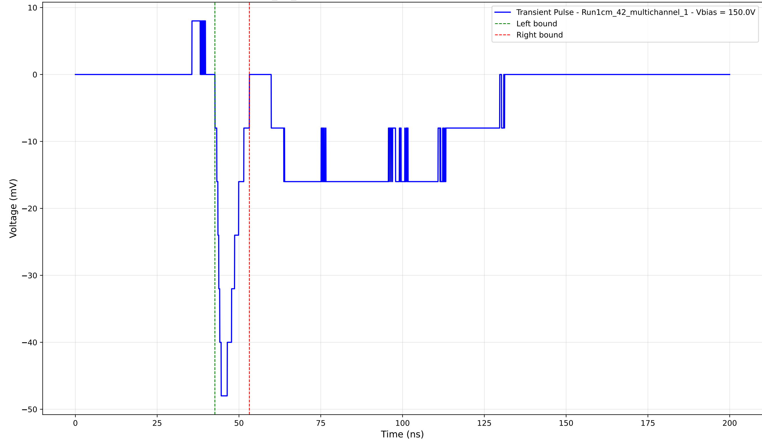
Transient Pulse - Sample: 1cm_42_multichannel - Position: 4185.0 \mu\text{m} - Charge: -5.67 pC - Rise Time: 1.91 ns
