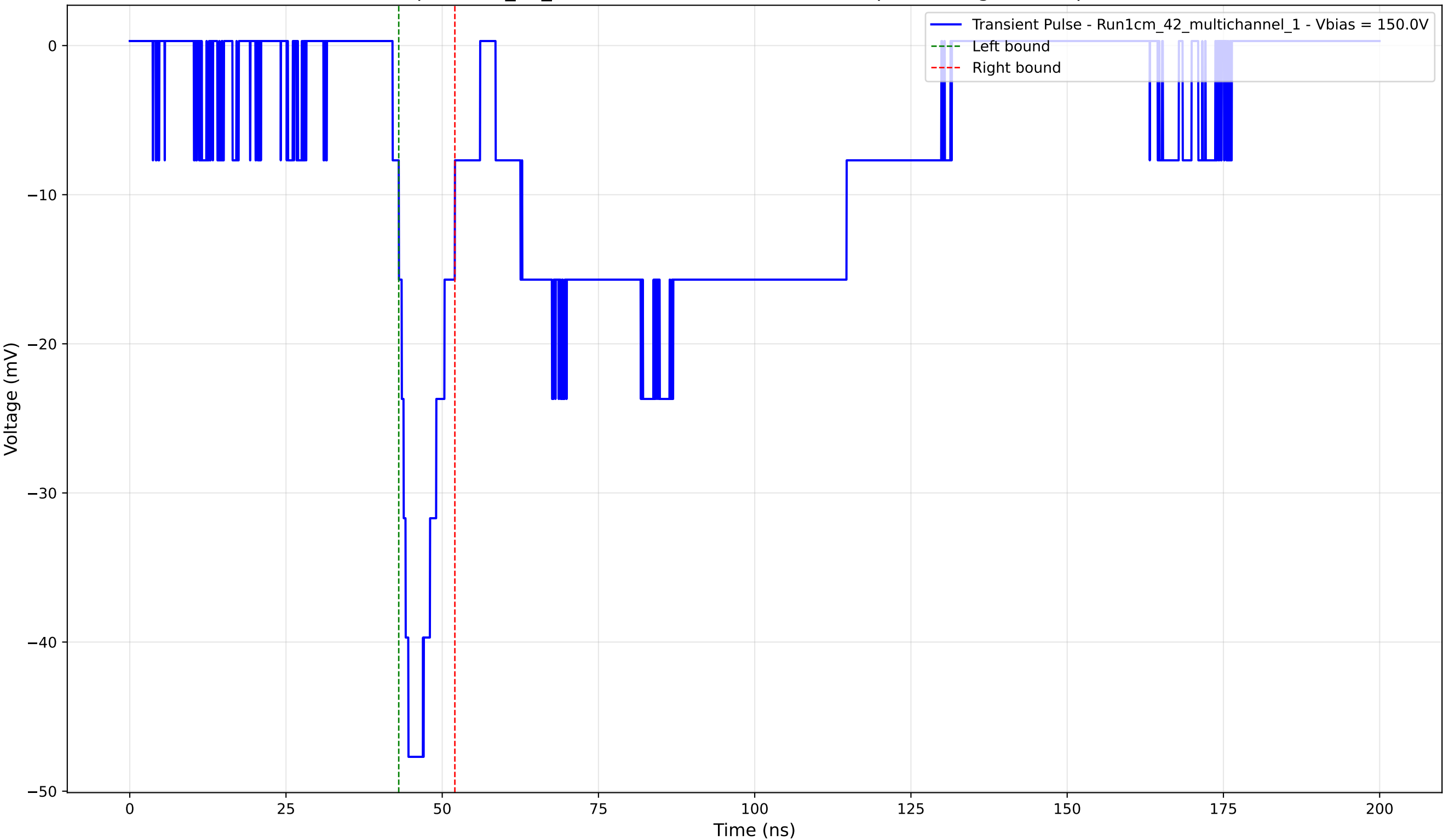
Transient Pulse - Sample: 1cm_42_multichannel - Position: 4545.0 \mu\text{m} - Charge: -5.76 pC - Rise Time: 2.53 ns
