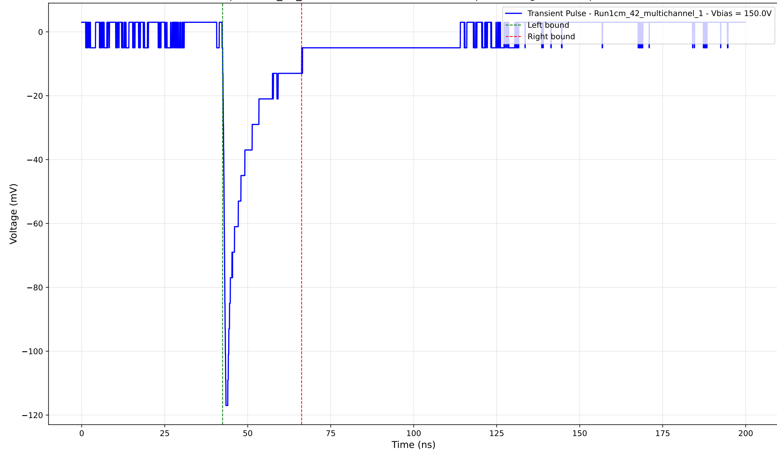
Transient Pulse - Sample: 1cm_42_multichannel - Position: 3155.0 \mu\text{m} - Charge: -15.97 pC - Rise Time: 0.88 ns
