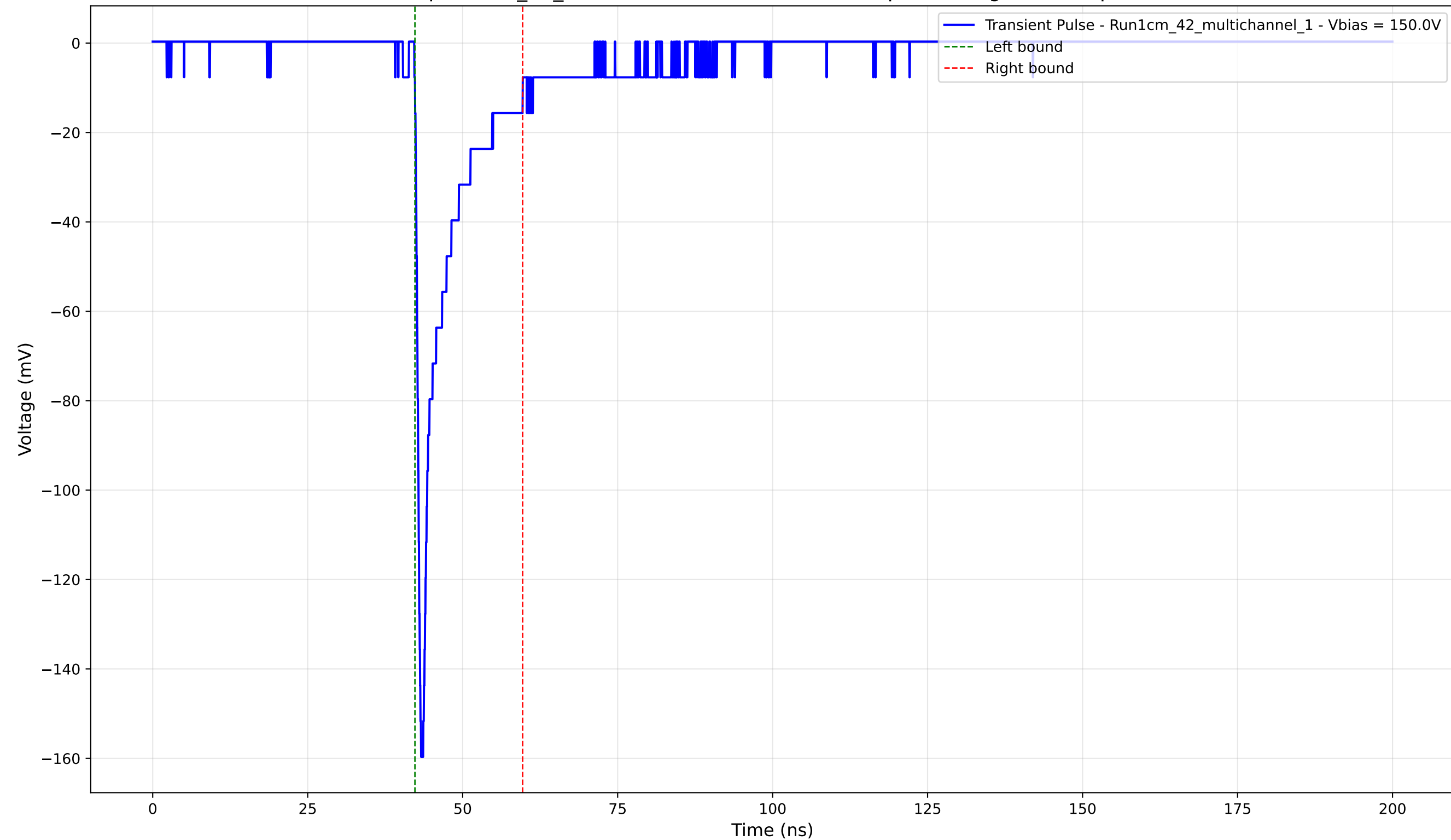
Transient Pulse - Sample: 1cm_42_multichannel - Position: 2830.0 \mu\text{m} - Charge: -14.81 pC - Rise Time: 0.80 ns
