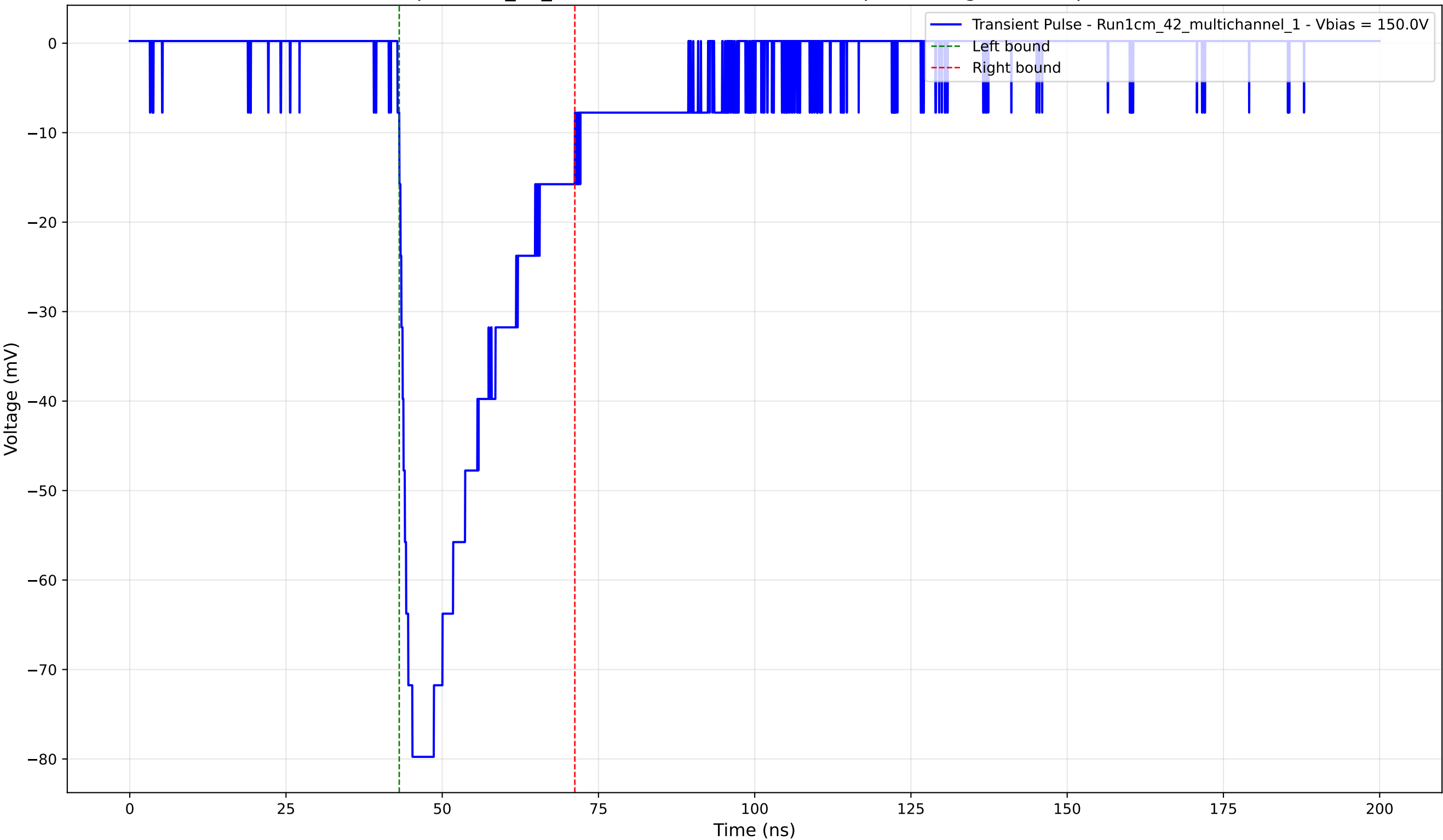
Transient Pulse - Sample: 1cm_42_multichannel - Position: 670.0 \mu\text{m} - Charge: -23.73 pC - Rise Time: 2.10 ns
