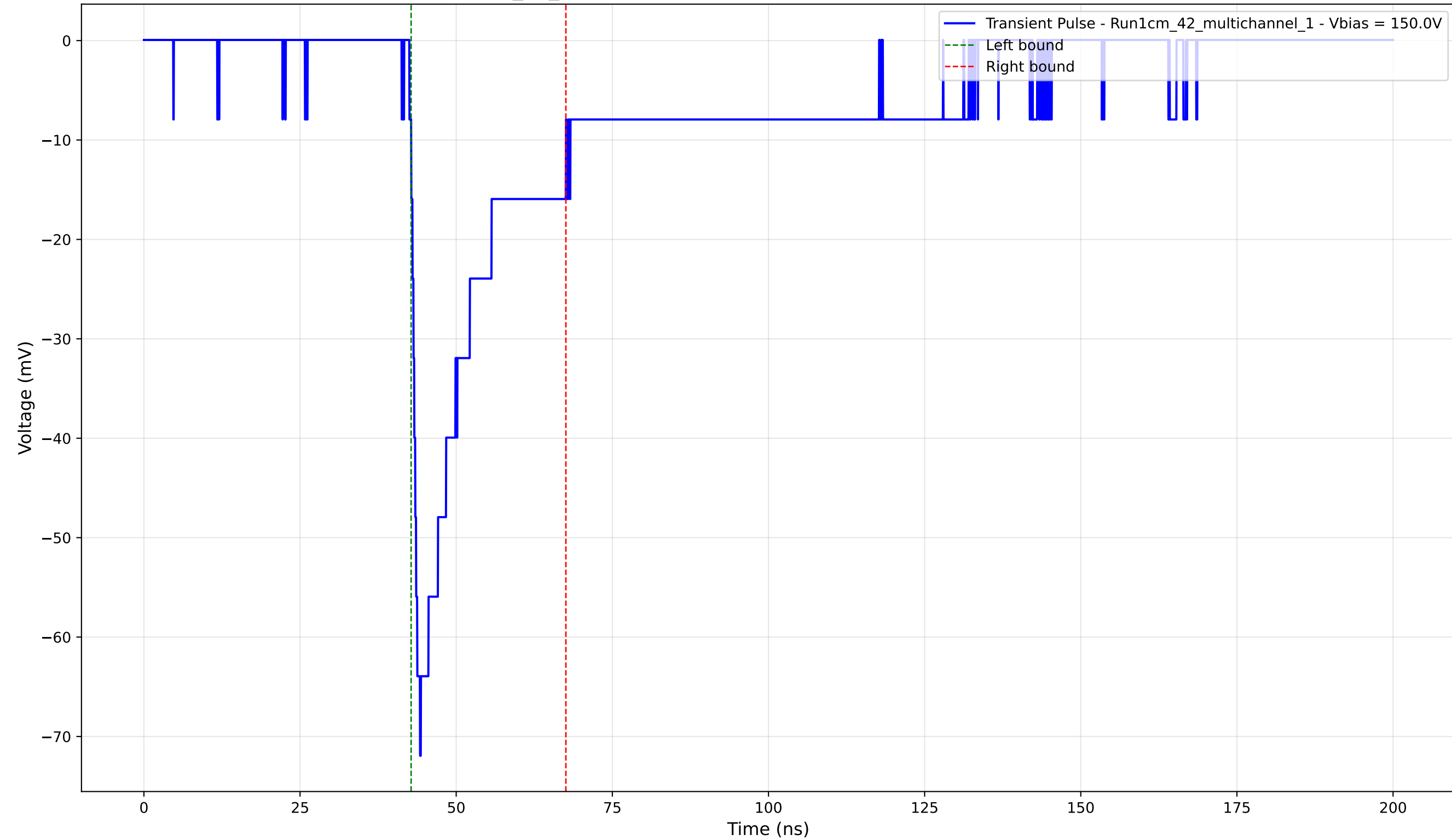
Transient Pulse - Sample: 1cm_42_multichannel - Position: 3635.0 \mu\text{m} - Charge: -14.09 pC - Rise Time: 1.70 ns
