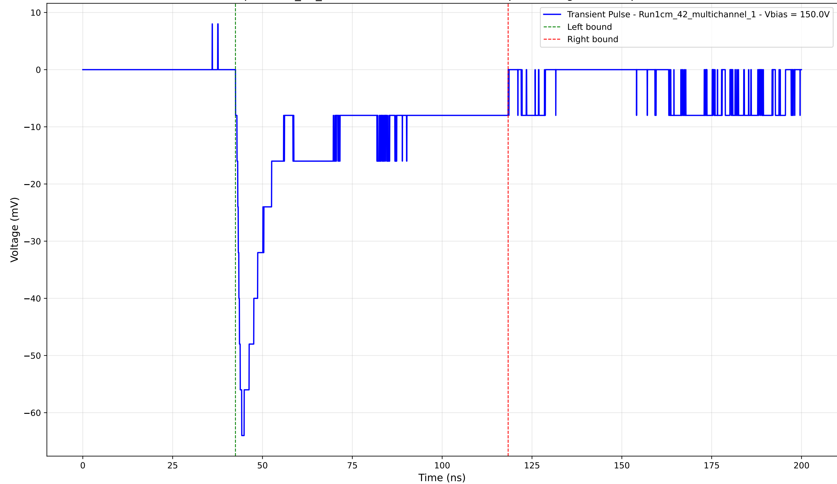
Transient Pulse - Sample: 1cm_42_multichannel - Position: 3735.0 \mu\text{m} - Charge: -21.16 pC - Rise Time: 1.72 ns
