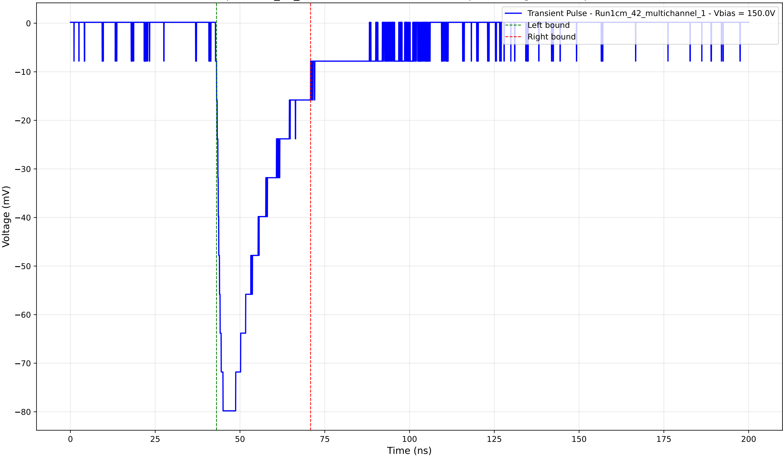
Transient Pulse - Sample: 1cm_42_multichannel - Position: 735.0 \mu\text{m} - Charge: -23.41 pC - Rise Time: 1.92 ns
