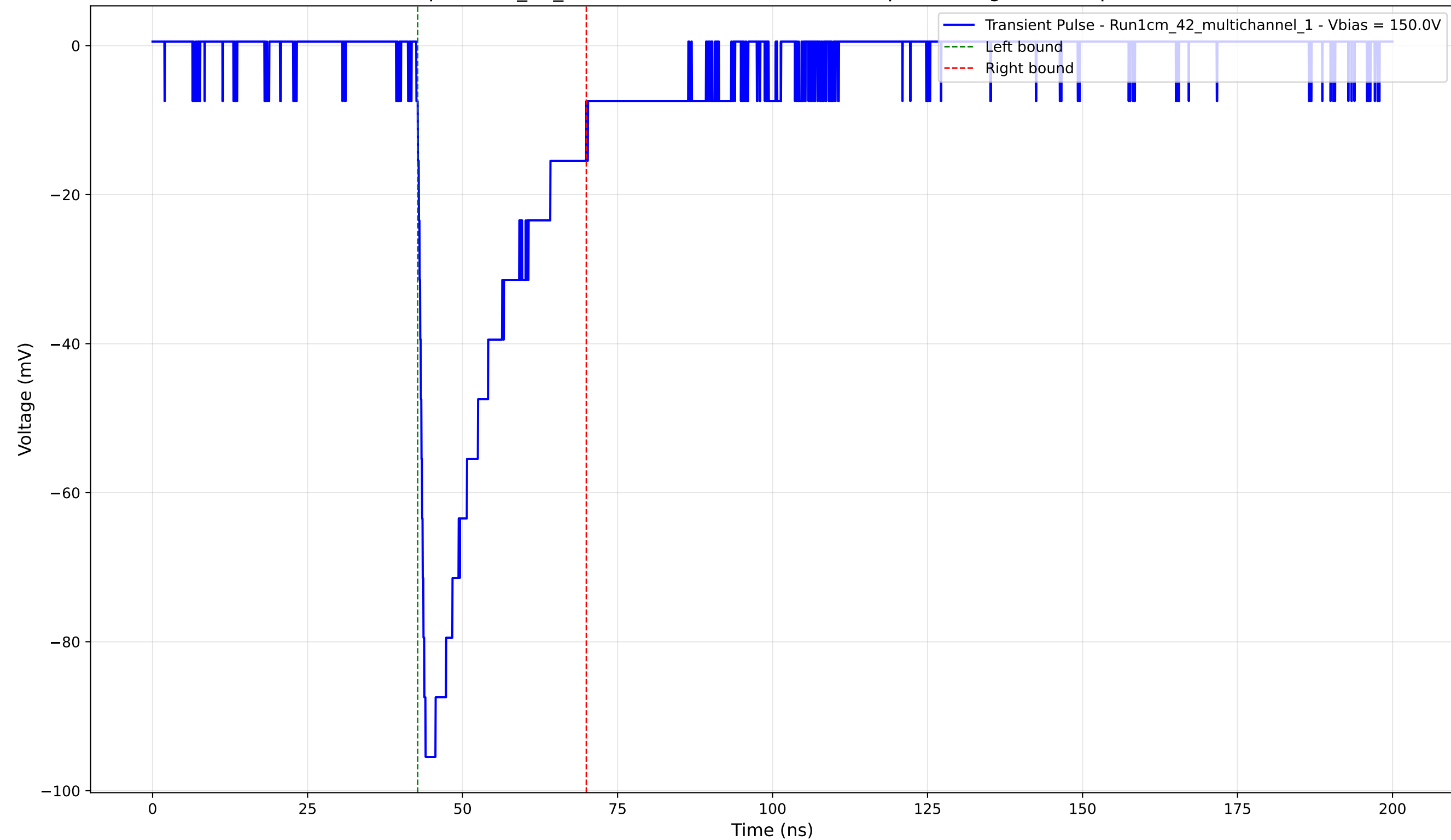
Transient Pulse - Sample: 1cm_42_multichannel - Position: 1190.0 \mu\text{m} - Charge: -23.52 pC - Rise Time: 1.05 ns
