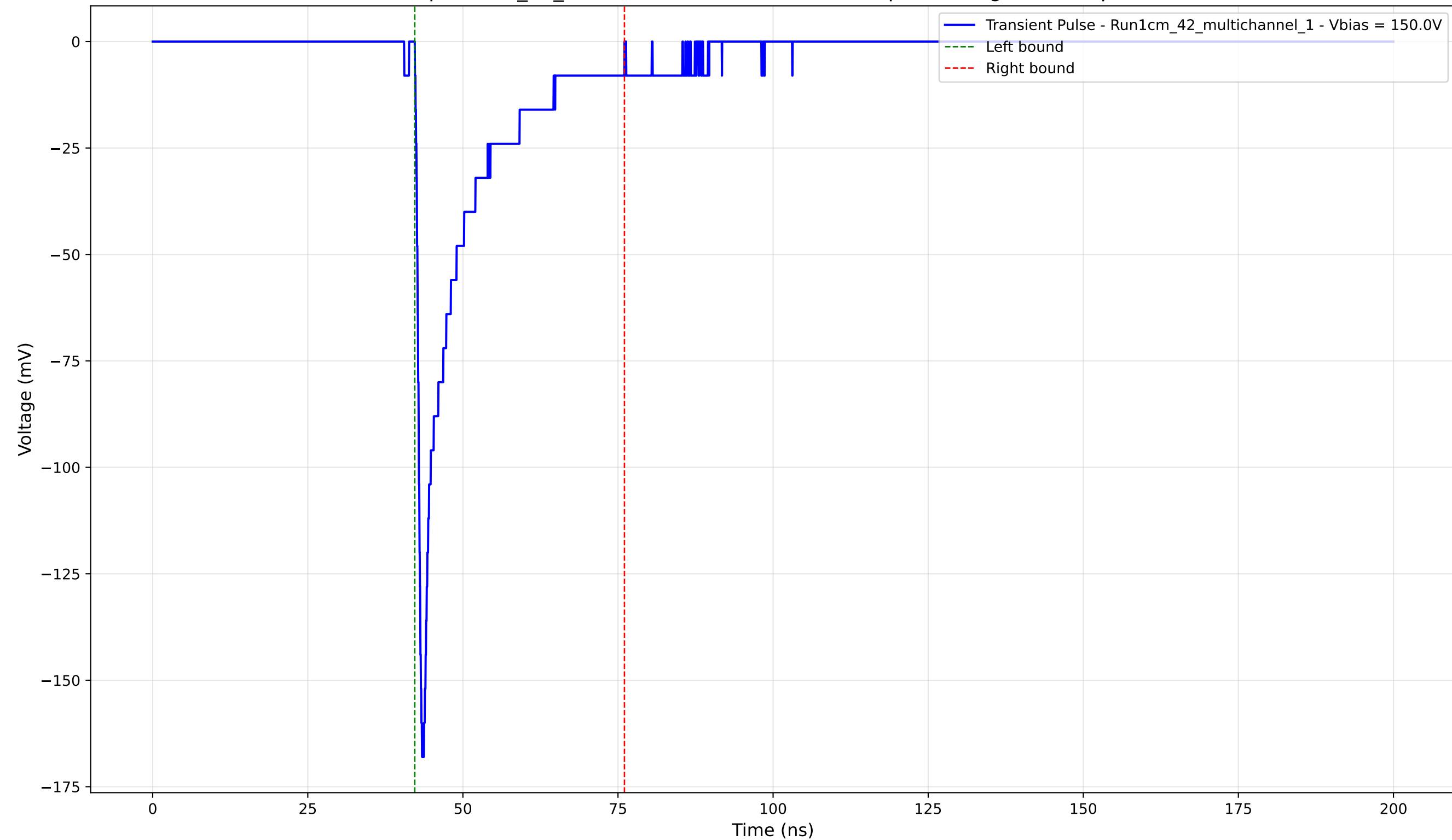
Transient Pulse - Sample: 1cm_42_multichannel - Position: 2985.0 \mu\text{m} - Charge: -21.92 pC - Rise Time: 0.80 ns
