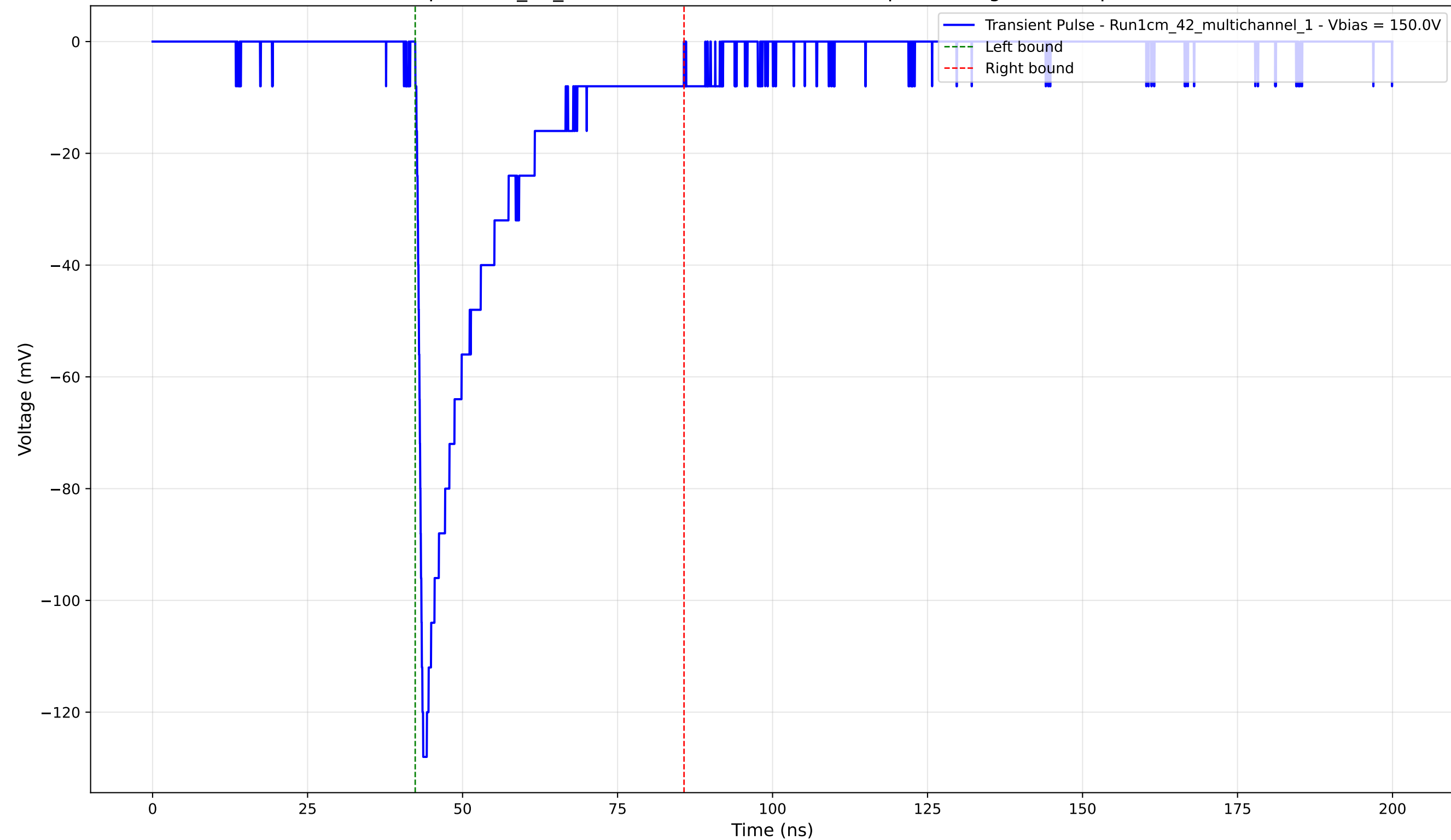
Transient Pulse - Sample: 1cm_42_multichannel - Position: 1515.0 \mu\text{m} - Charge: -26.02 pC - Rise Time: 0.97 ns
