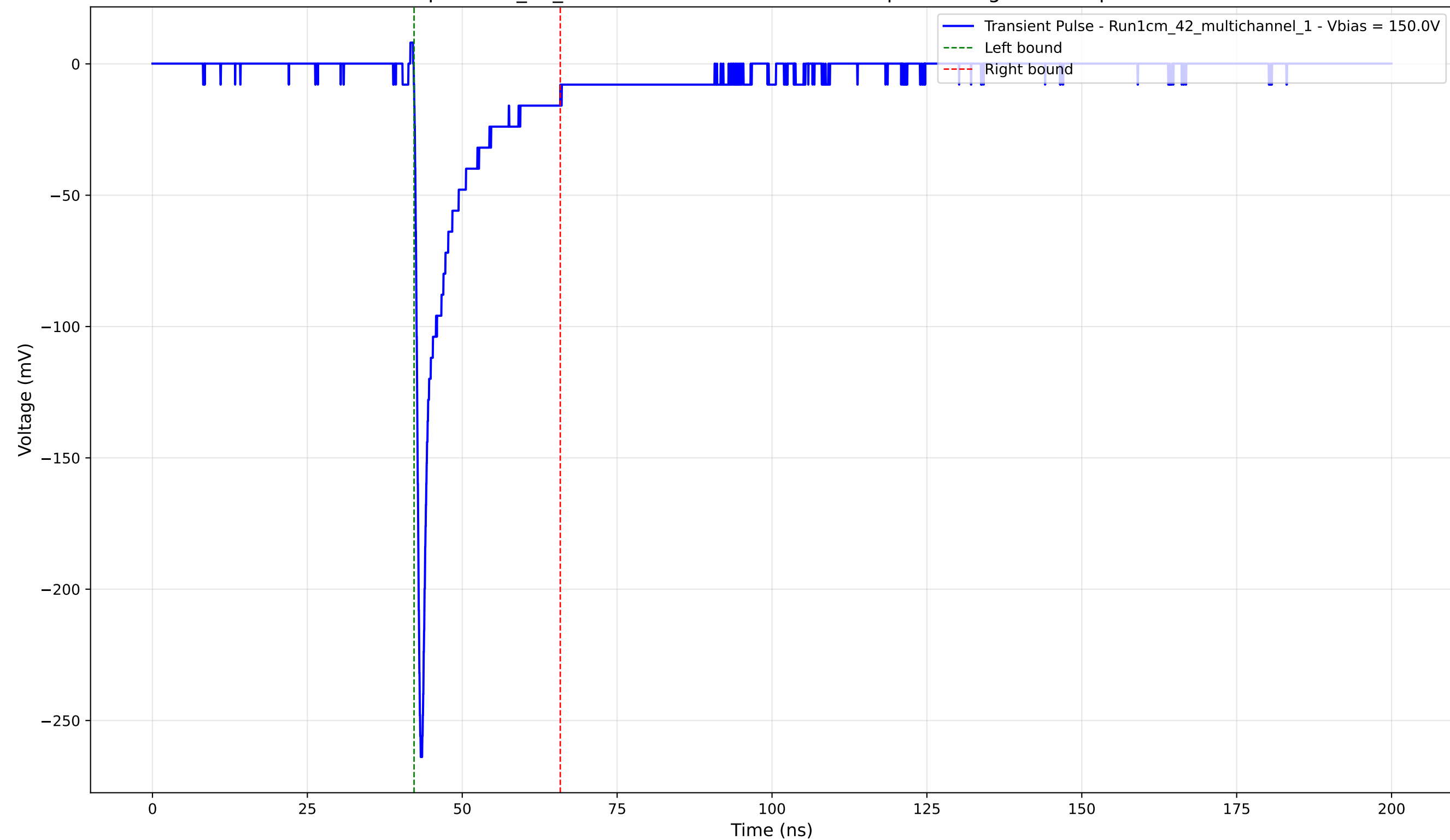
Transient Pulse - Sample: 1cm_42_multichannel - Position: 2015.0 \mu\text{m} - Charge: -24.39 pC - Rise Time: 0.77 ns
