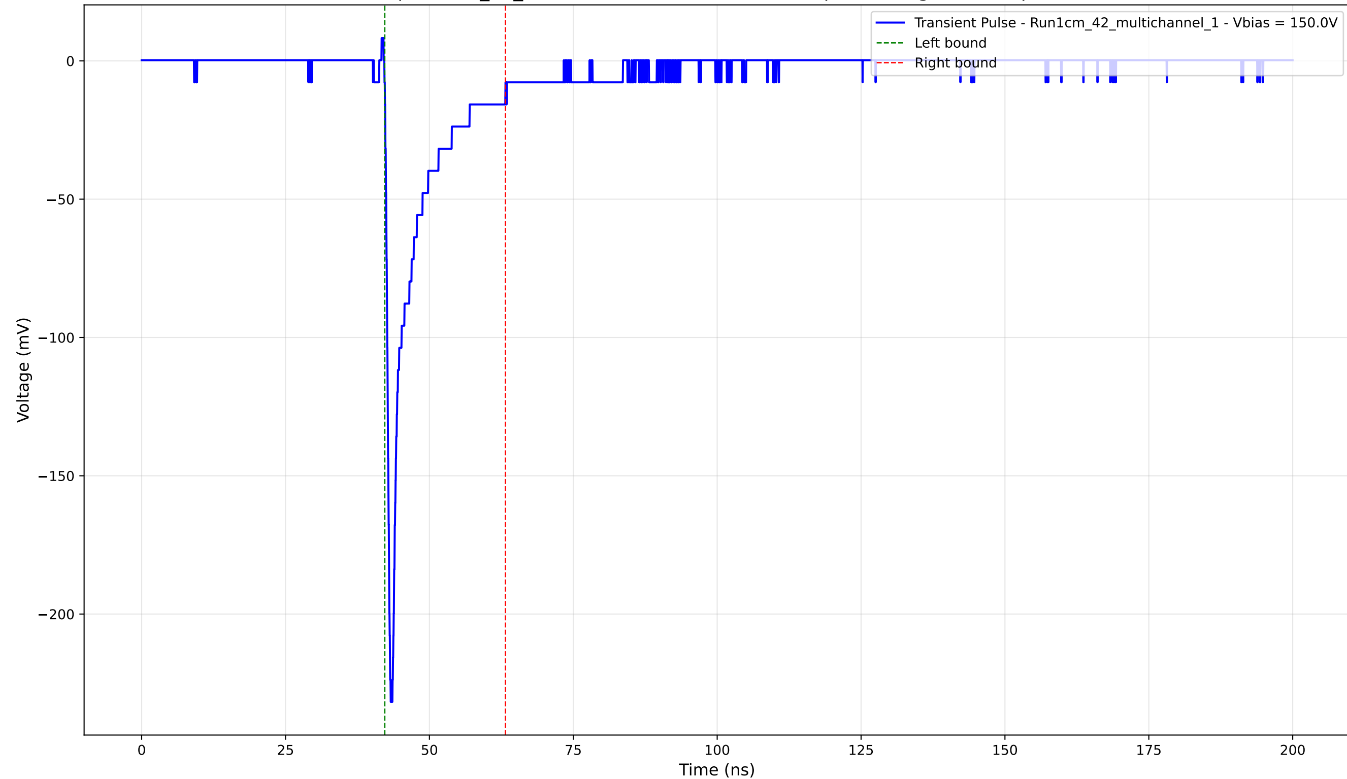
Transient Pulse - Sample: 1cm_42_multichannel - Position: 2780.0 \mu\text{m} - Charge: -21.05 pC - Rise Time: 0.82 ns
