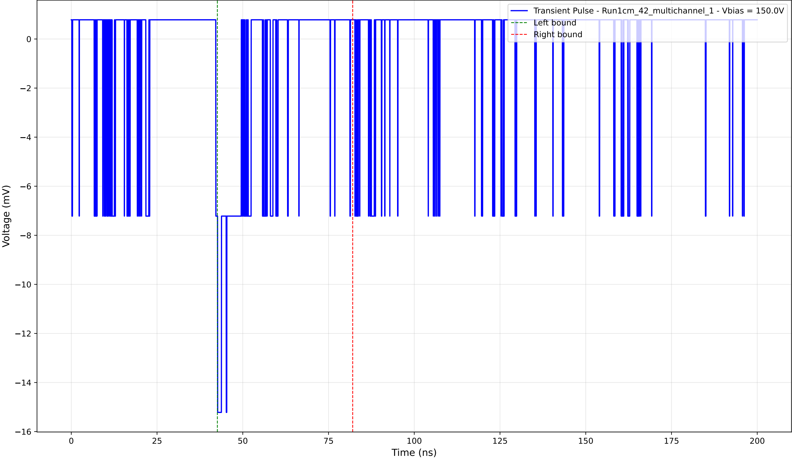
Transient Pulse - Sample: 1cm_42_multichannel - Position: 2395.0 \mu\text{m} - Charge: -1.43 pC - Rise Time: 0.54 ns
