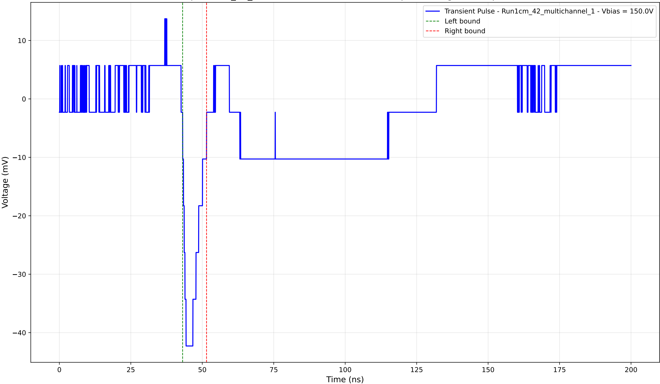
Transient Pulse - Sample: 1cm_42_multichannel - Position: 4090.0 \mu\text{m} - Charge: -4.60 pC - Rise Time: 1.20 ns
