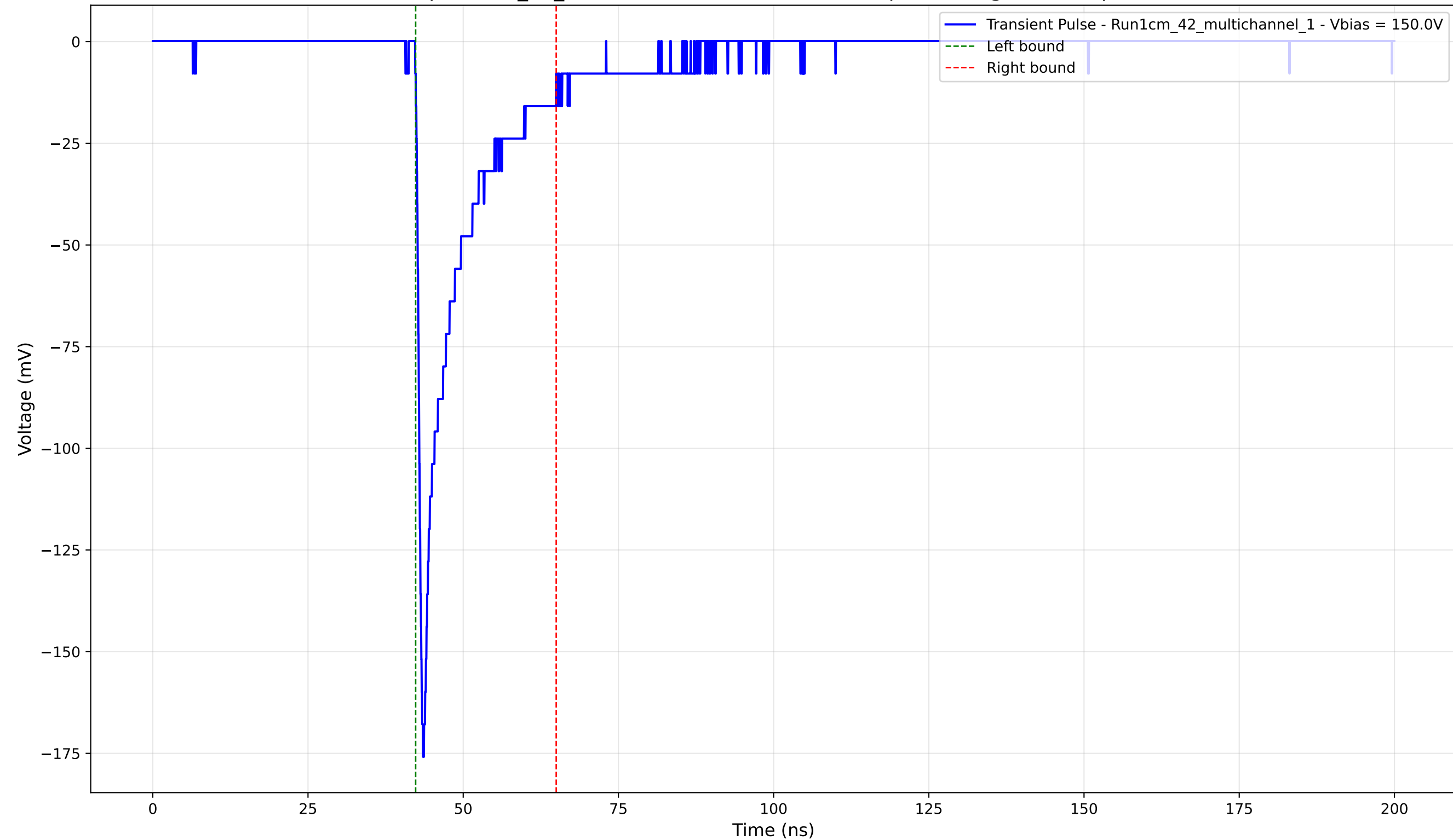
Transient Pulse - Sample: 1cm_42_multichannel - Position: 1770.0 \mu\text{m} - Charge: -21.58 pC - Rise Time: 0.86 ns
