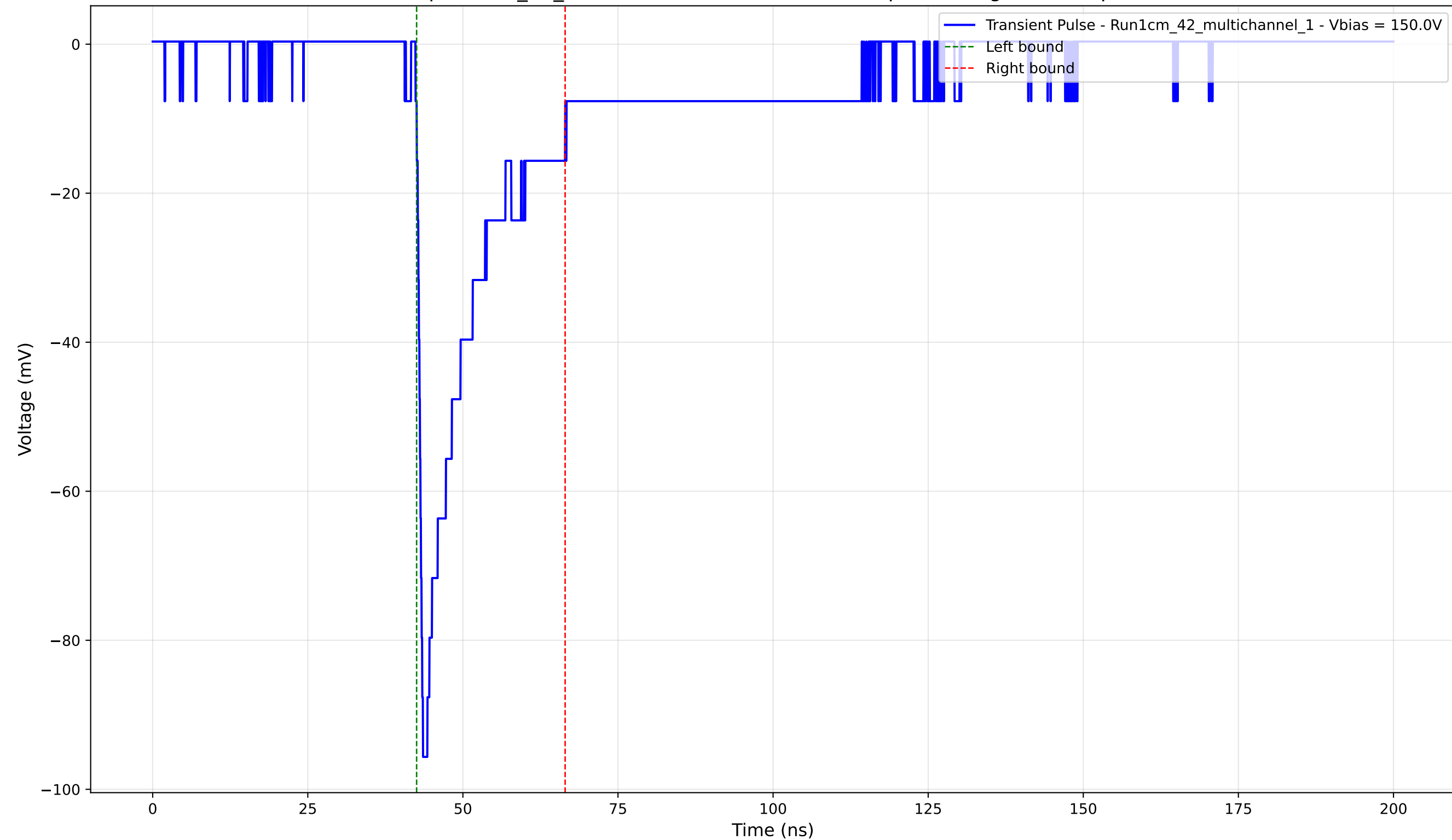
Transient Pulse - Sample: 1cm_42_multichannel - Position: 3305.0 \mu\text{m} - Charge: -16.77 pC - Rise Time: 0.90 ns
