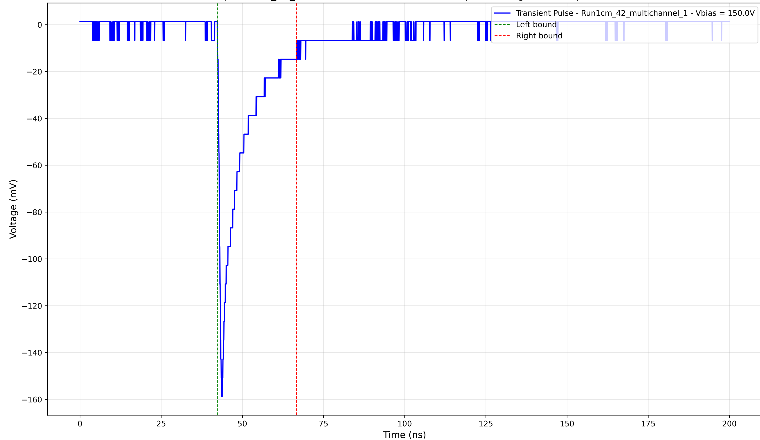
Transient Pulse - Sample: 1cm_42_multichannel - Position: 1665.0 \mu\text{m} - Charge: -22.42 pC - Rise Time: 0.96 ns
