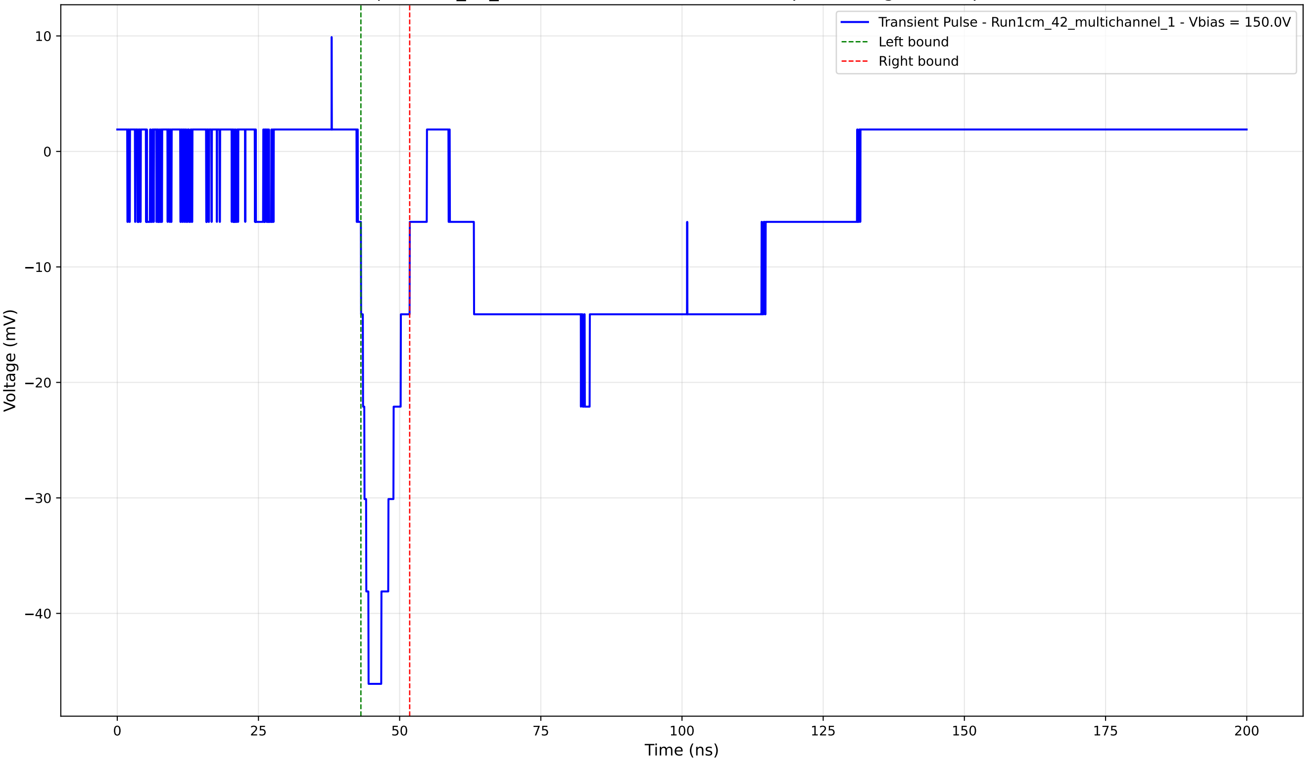
Transient Pulse - Sample: 1cm_42_multichannel - Position: 4235.0 \mu\text{m} - Charge: -5.32 pC - Rise Time: 1.89 ns
