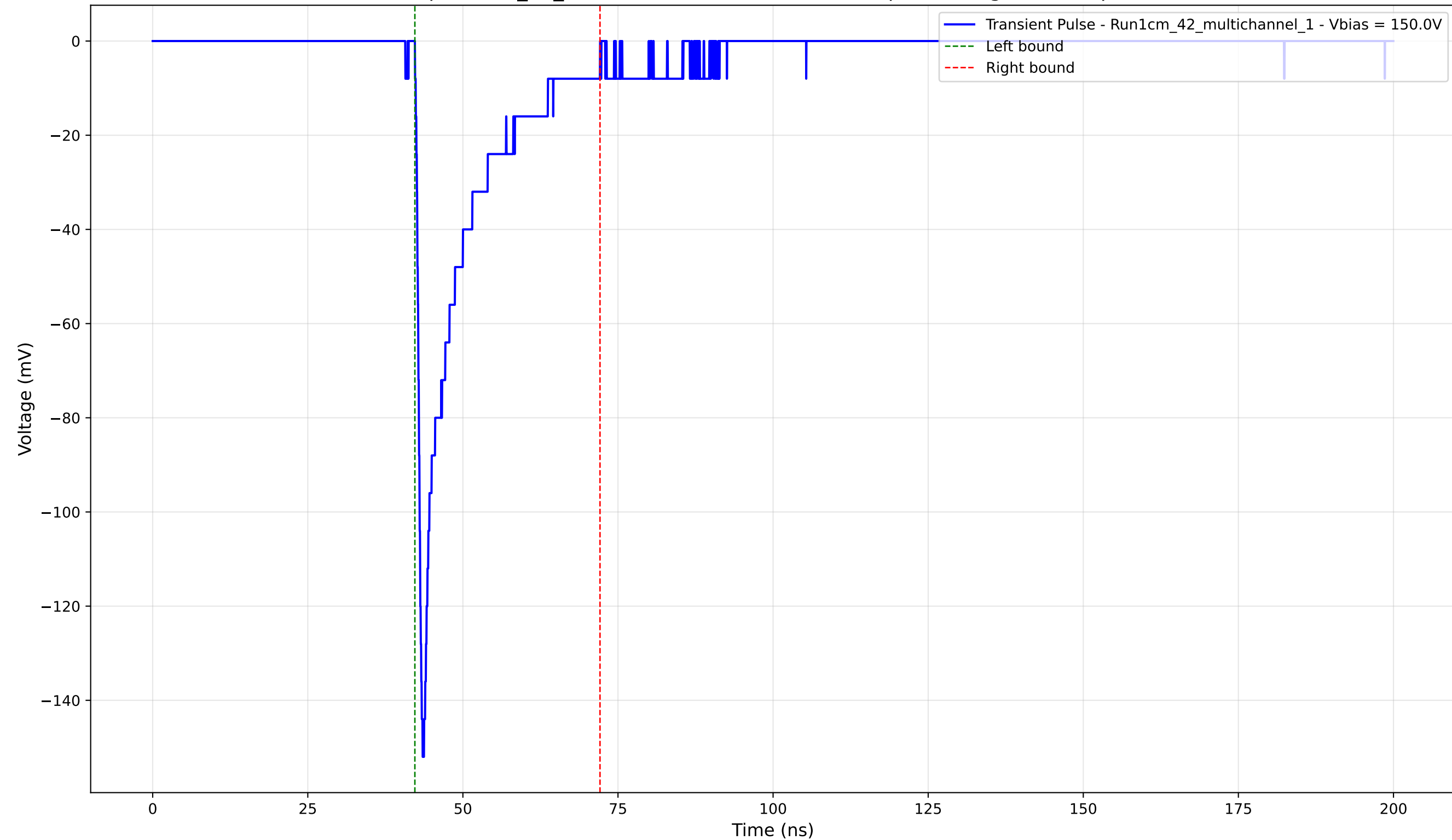
Transient Pulse - Sample: 1cm_42_multichannel - Position: 3050.0 \mu\text{m} - Charge: -19.92 pC - Rise Time: 0.96 ns
