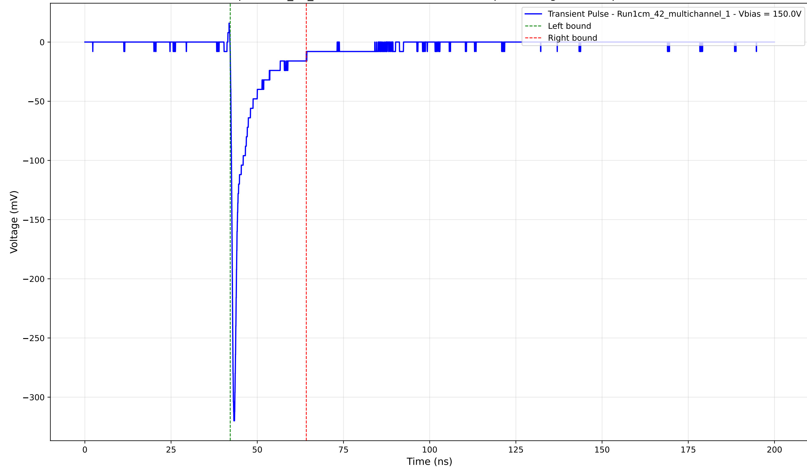
Transient Pulse - Sample: 1cm_42_multichannel - Position: 2130.0 \mu\text{m} - Charge: -24.41 pC - Rise Time: 0.76 ns
