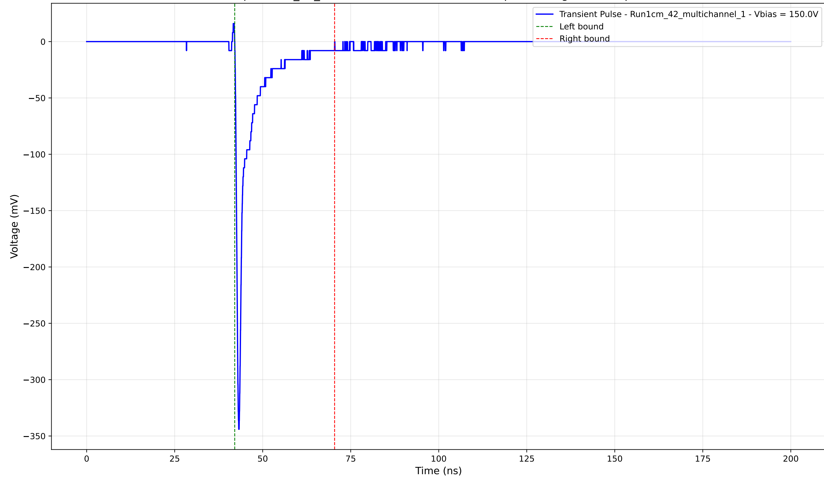
Transient Pulse - Sample: 1cm_42_multichannel - Position: 2580.0 \mu\text{m} - Charge: -24.57 pC - Rise Time: 0.75 ns
