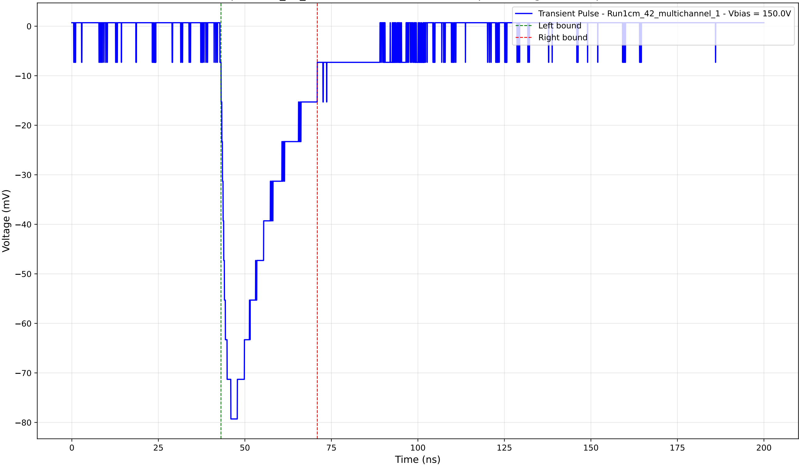
Transient Pulse - Sample: 1cm_42_multichannel - Position: 600.0 \mu\text{m} - Charge: -22.72 pC - Rise Time: 2.84 ns
