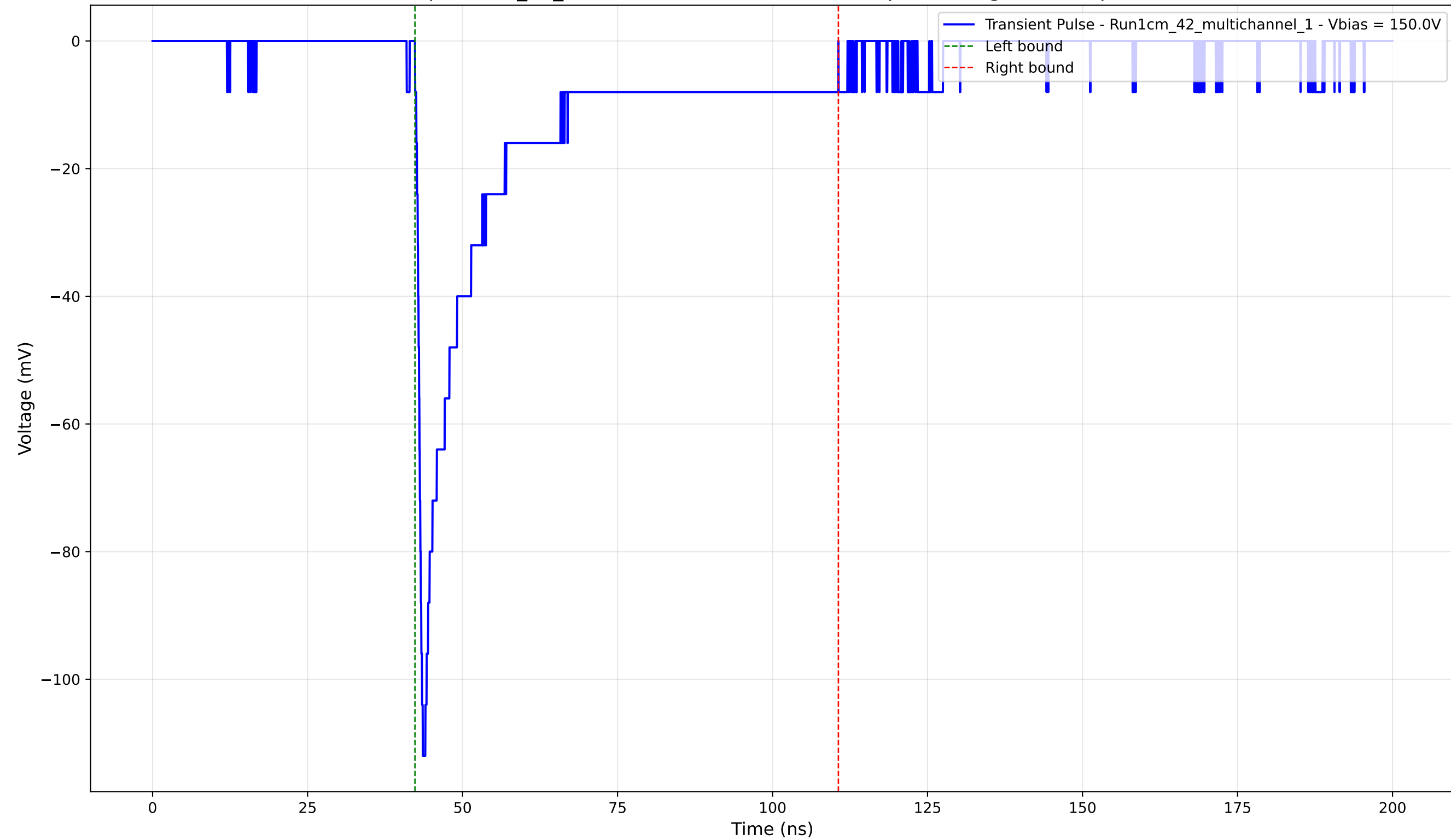
Transient Pulse - Sample: 1cm_42_multichannel - Position: 3250.0 \mu\text{m} - Charge: -23.89 pC - Rise Time: 0.93 ns
