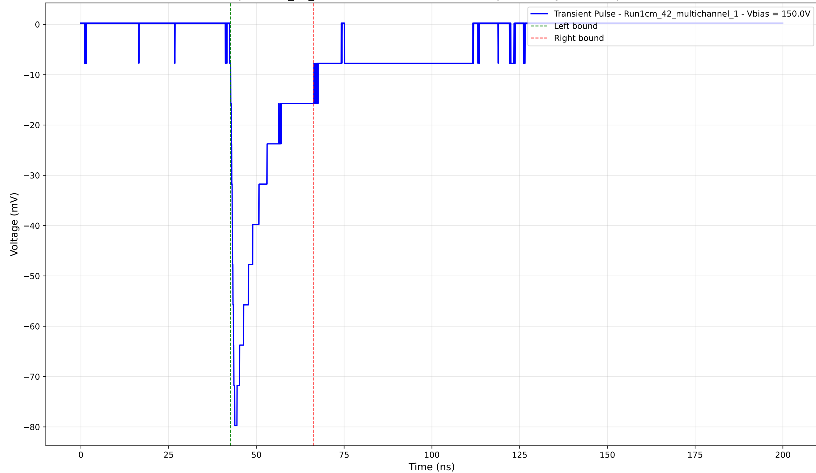
Transient Pulse - Sample: 1cm_42_multichannel - Position: 3490.0 \mu\text{m} - Charge: -15.00 pC - Rise Time: 1.16 ns
