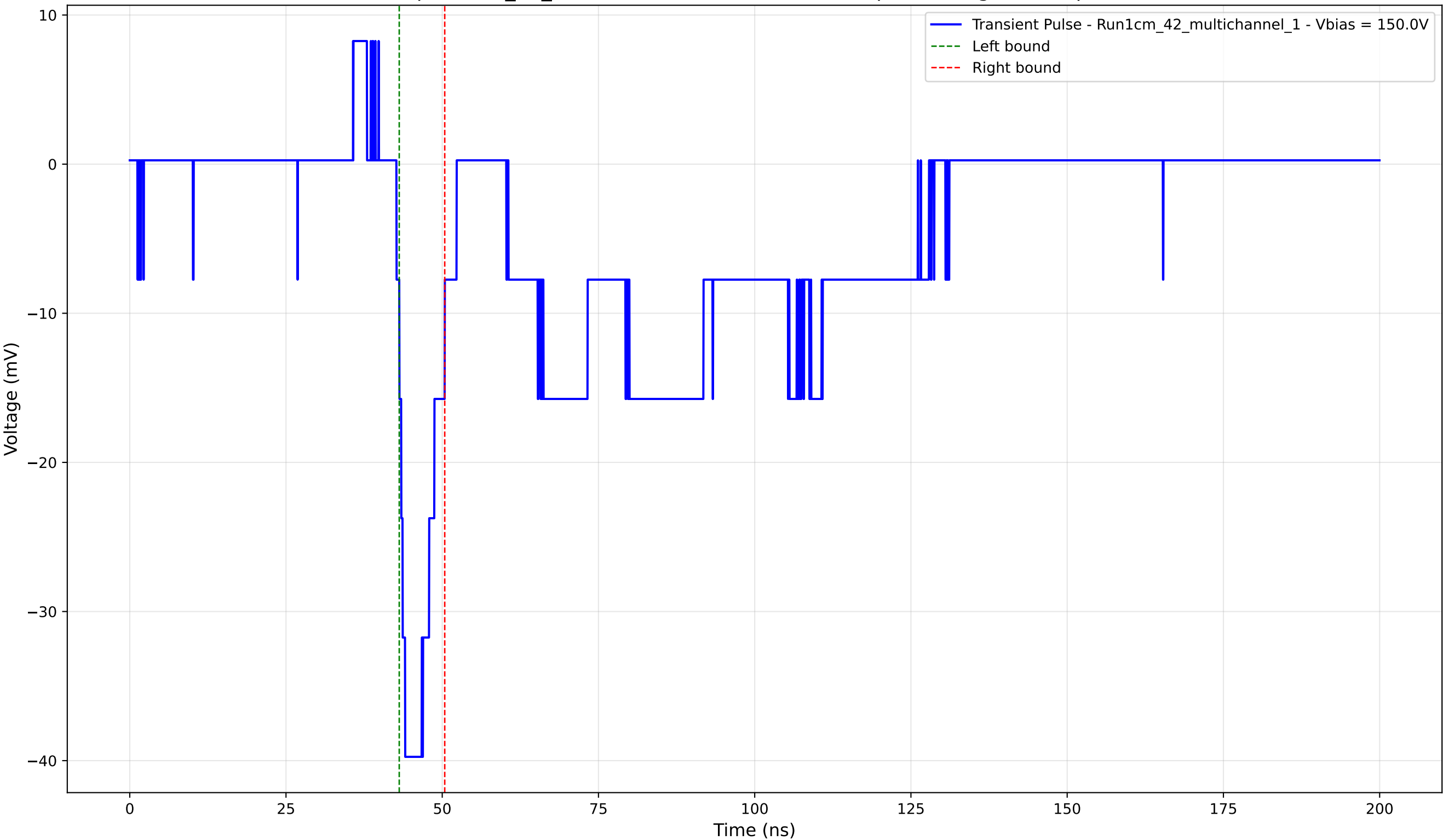
Transient Pulse - Sample: 1cm_42_multichannel - Position: 3970.0 \mu\text{m} - Charge: -4.26 pC - Rise Time: 1.39 ns
