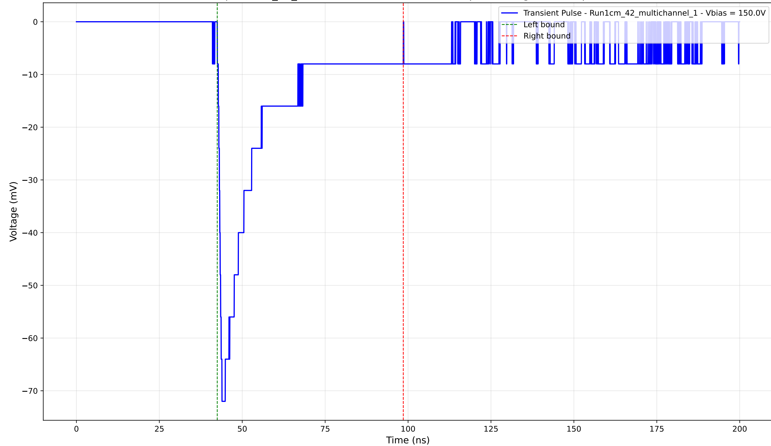
Transient Pulse - Sample: 1cm_42_multichannel - Position: 3585.0 \mu\text{m} - Charge: -19.82 pC - Rise Time: 1.40 ns
