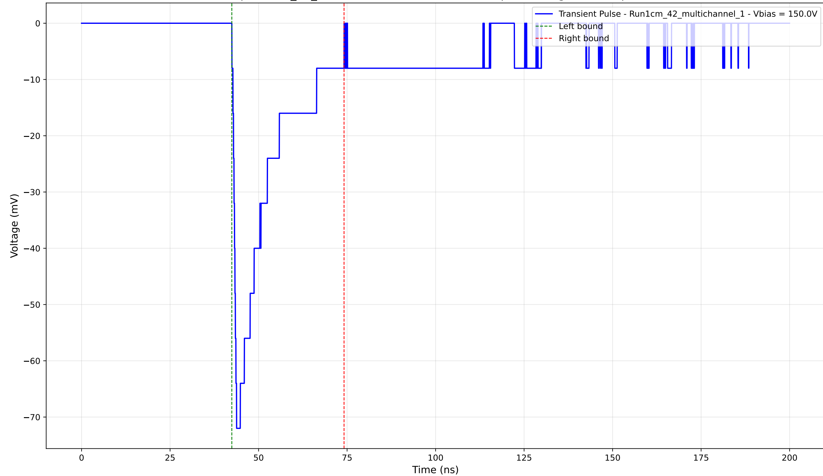
Transient Pulse - Sample: 1cm_42_multichannel - Position: 3570.0 \mu\text{m} - Charge: -15.68 pC - Rise Time: 1.32 ns
