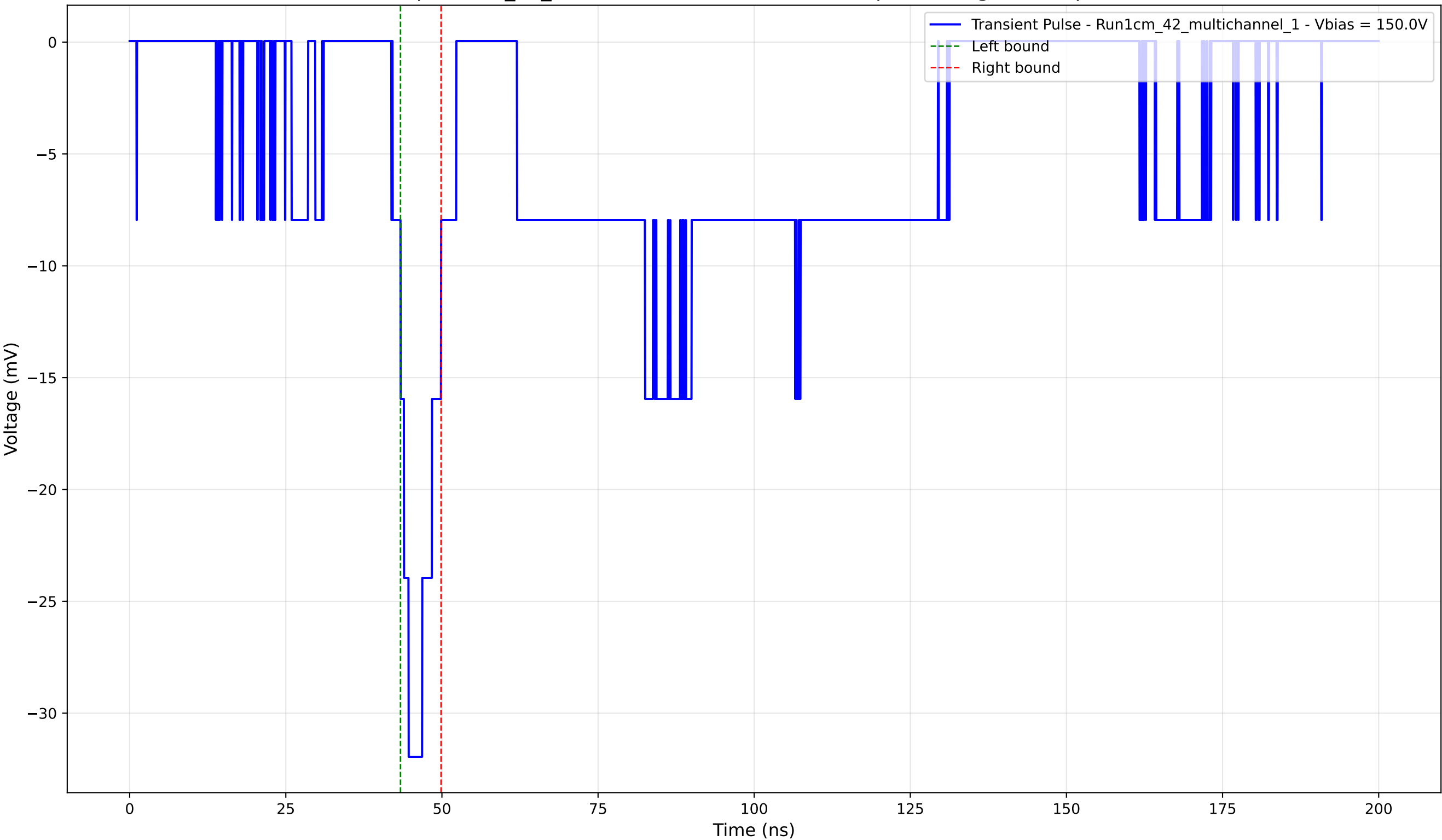
Transient Pulse - Sample: 1cm_42_multichannel - Position: 4460.0 \mu\text{m} - Charge: -3.14 pC - Rise Time: 2.57 ns
