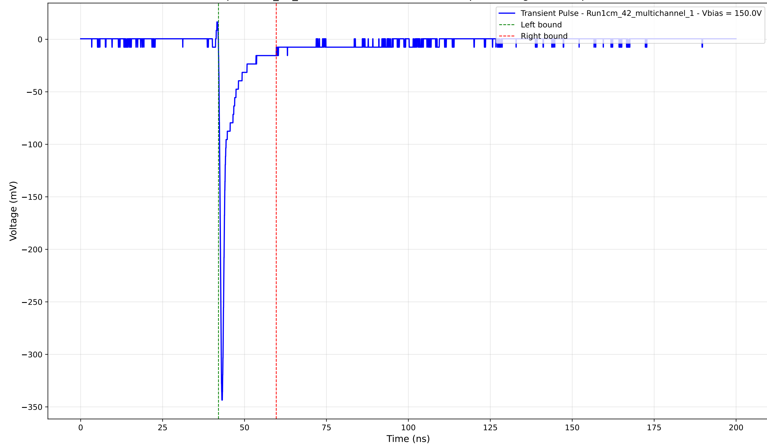
Transient Pulse - Sample: 1cm_42_multichannel - Position: 2455.0 \mu\text{m} - Charge: -19.79 pC - Rise Time: 0.73 ns
