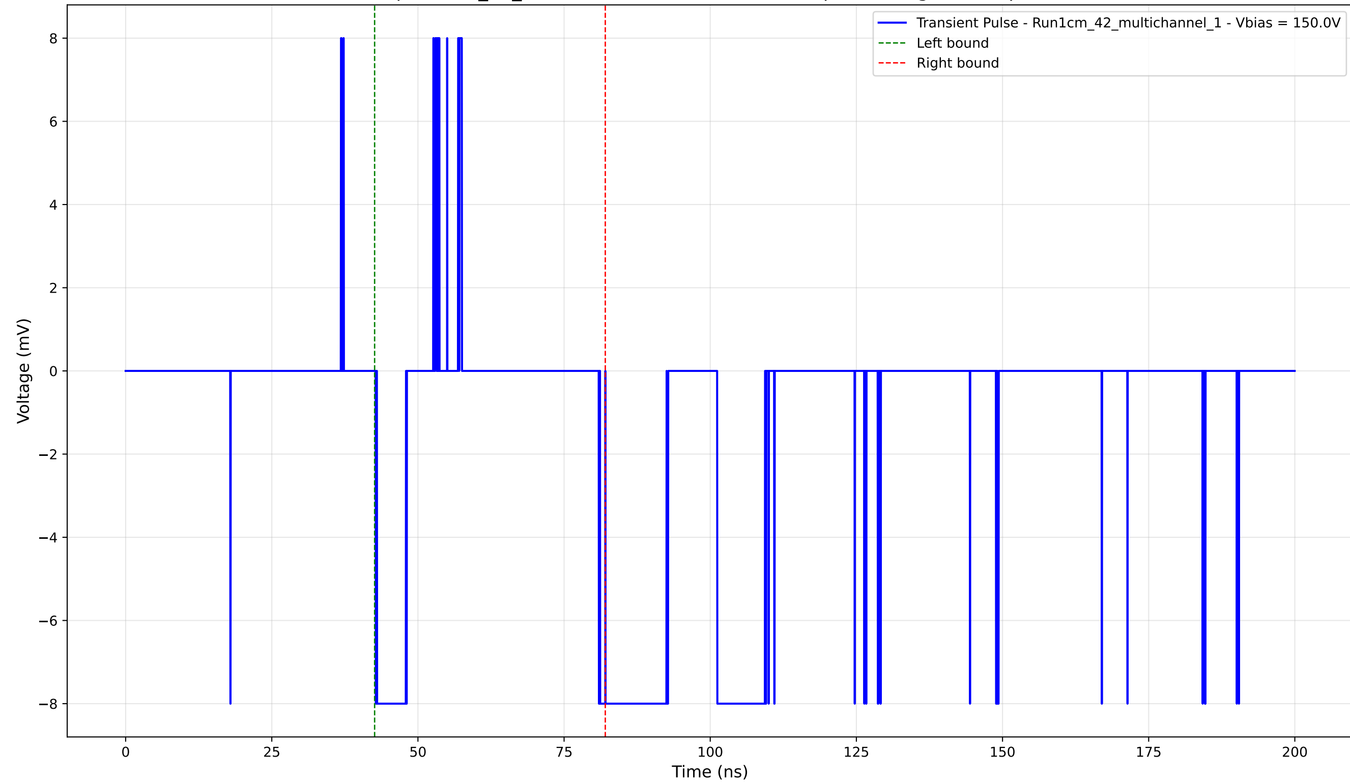
Transient Pulse - Sample: 1cm_42_multichannel - Position: 3885.0 \mu\text{m} - Charge: -0.80 pC - Rise Time: 0.02 ns
