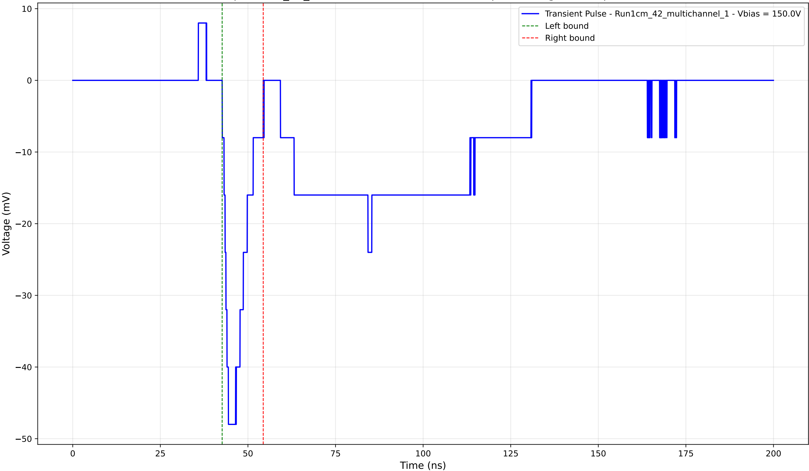
Transient Pulse - Sample: 1cm_42_multichannel - Position: 4125.0 \mu\text{m} - Charge: -5.95 pC - Rise Time: 1.77 ns
