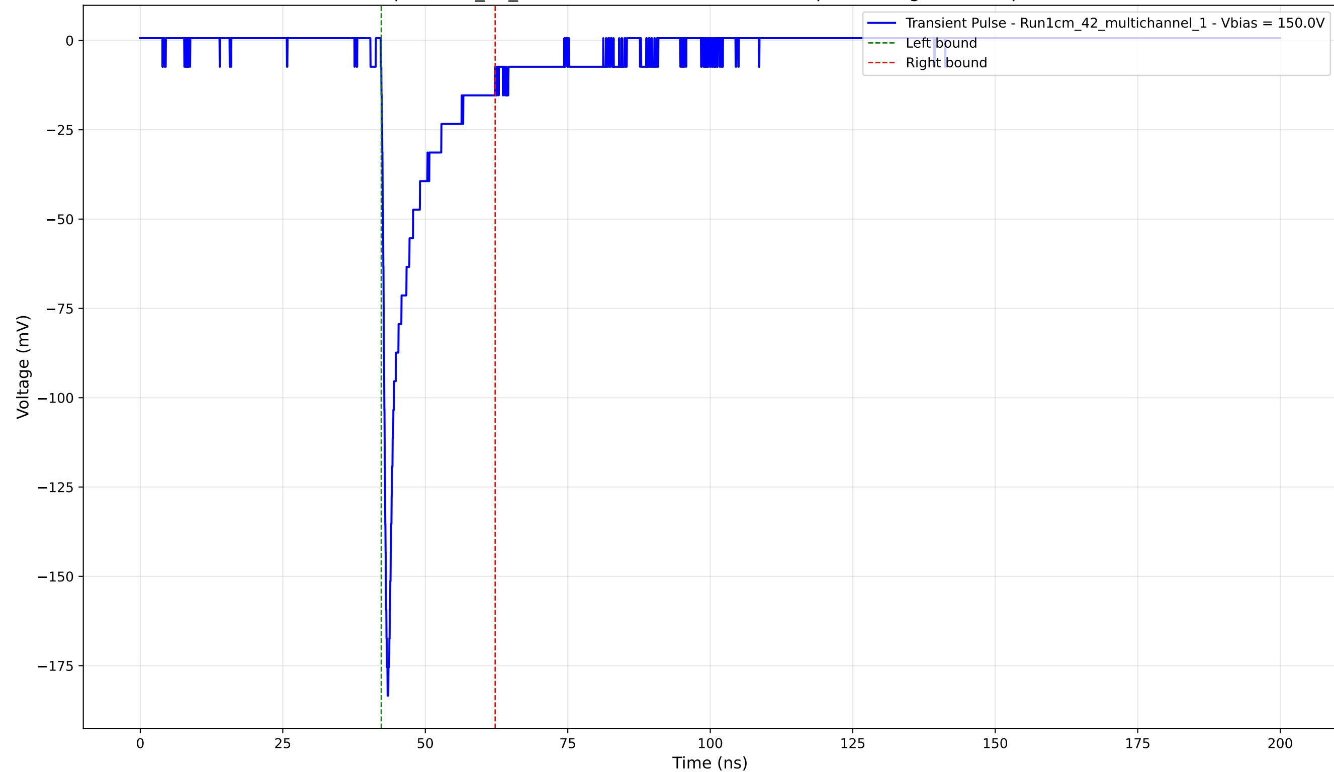
Transient Pulse - Sample: 1cm_42_multichannel - Position: 1945.0 \mu\text{m} - Charge: -17.55 pC - Rise Time: 0.83 ns
