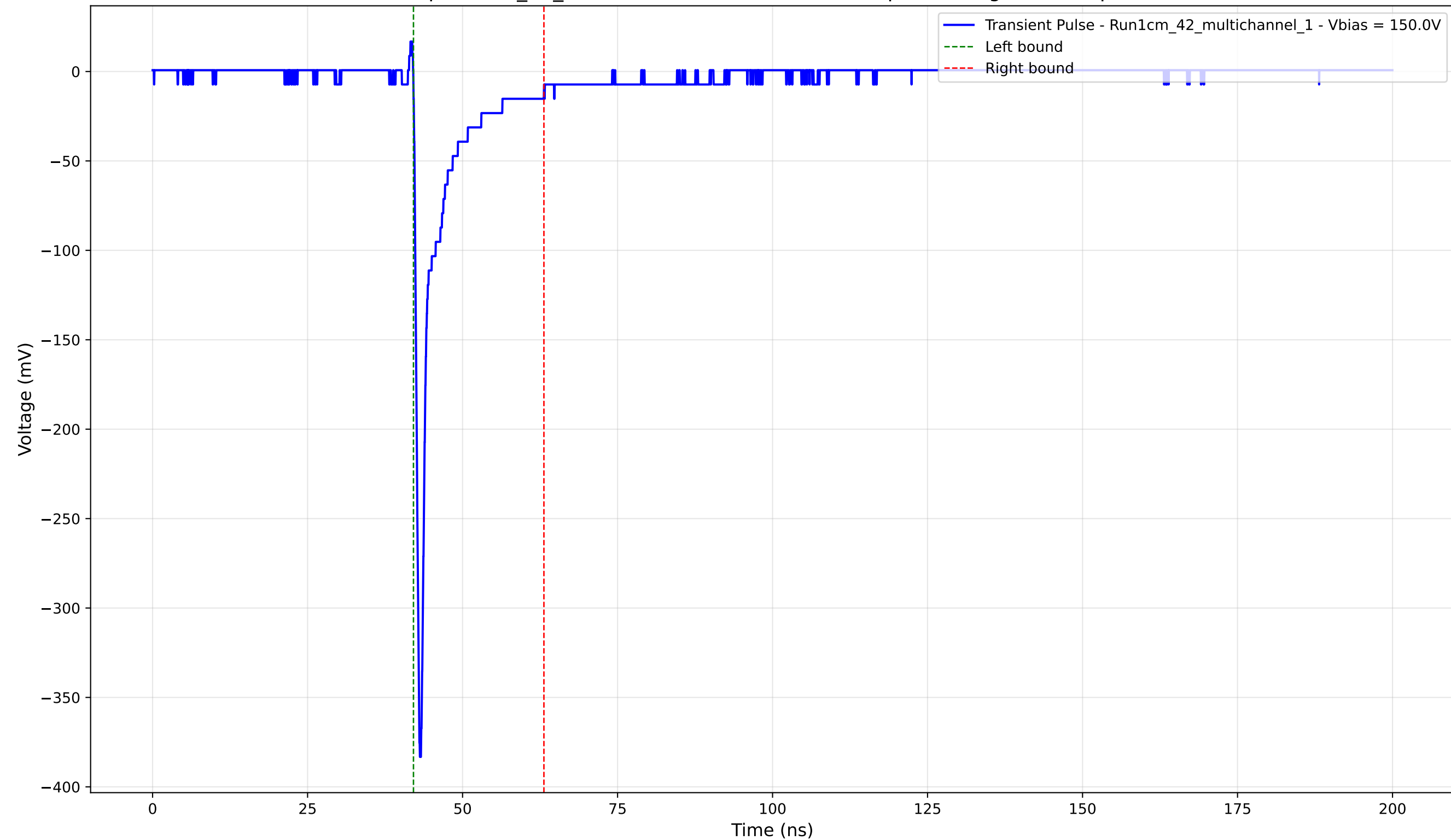
Transient Pulse - Sample: 1cm_42_multichannel - Position: 2515.0 \mu\text{m} - Charge: -24.42 pC - Rise Time: 0.75 ns
