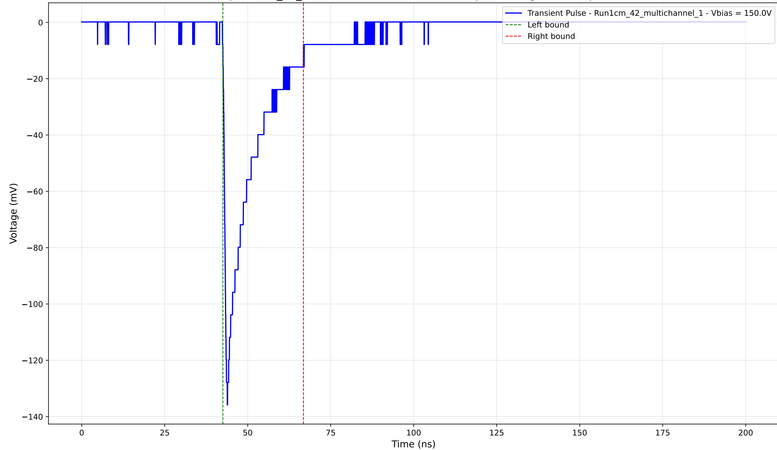
Transient Pulse - Sample: 1cm_42_multichannel - Position: 1525.0 \mu\text{m} - Charge: -22.68 pC - Rise Time: 1.07 ns
