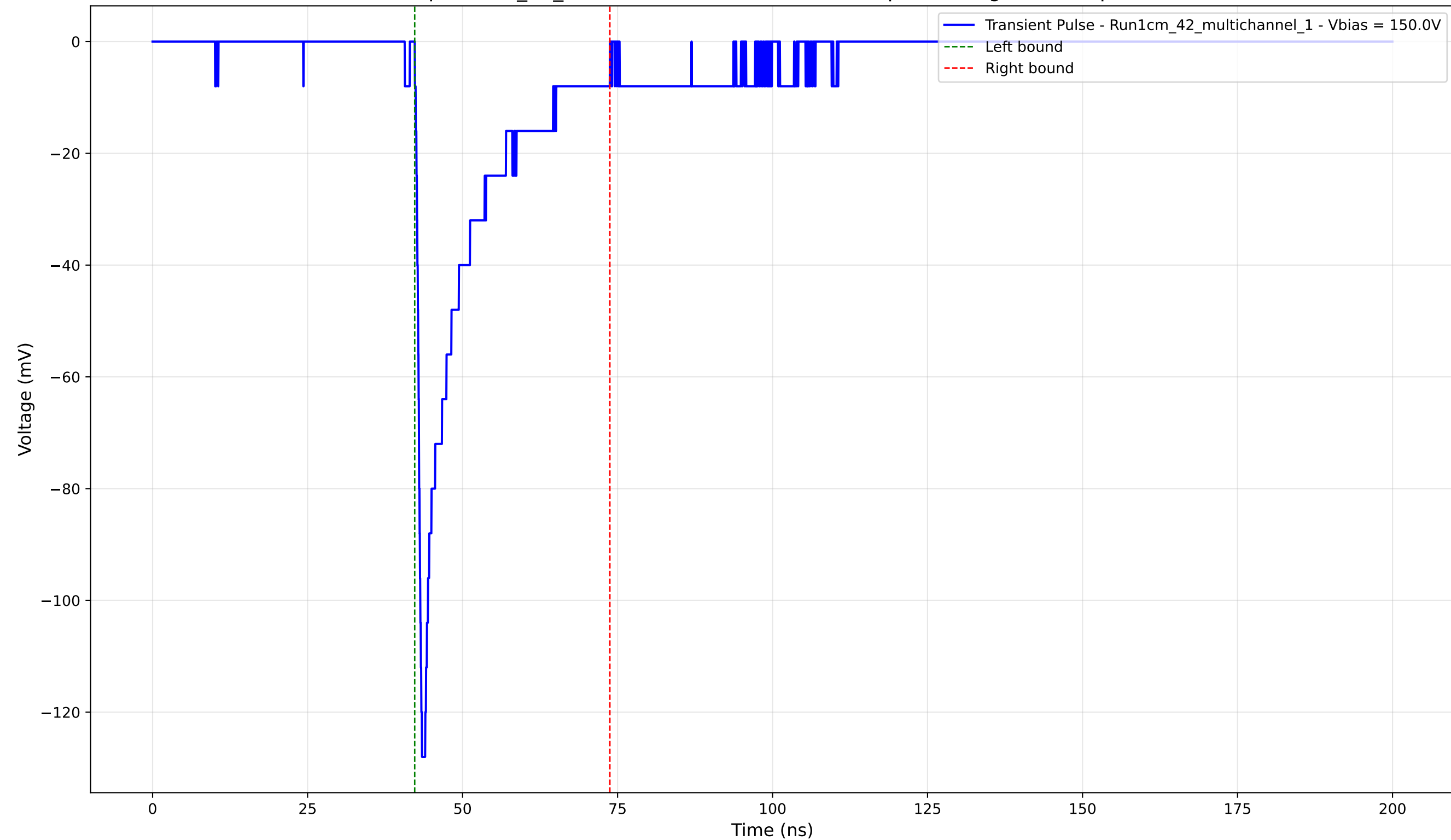
Transient Pulse - Sample: 1cm_42_multichannel - Position: 3120.0 \mu\text{m} - Charge: -18.89 pC - Rise Time: 0.91 ns
