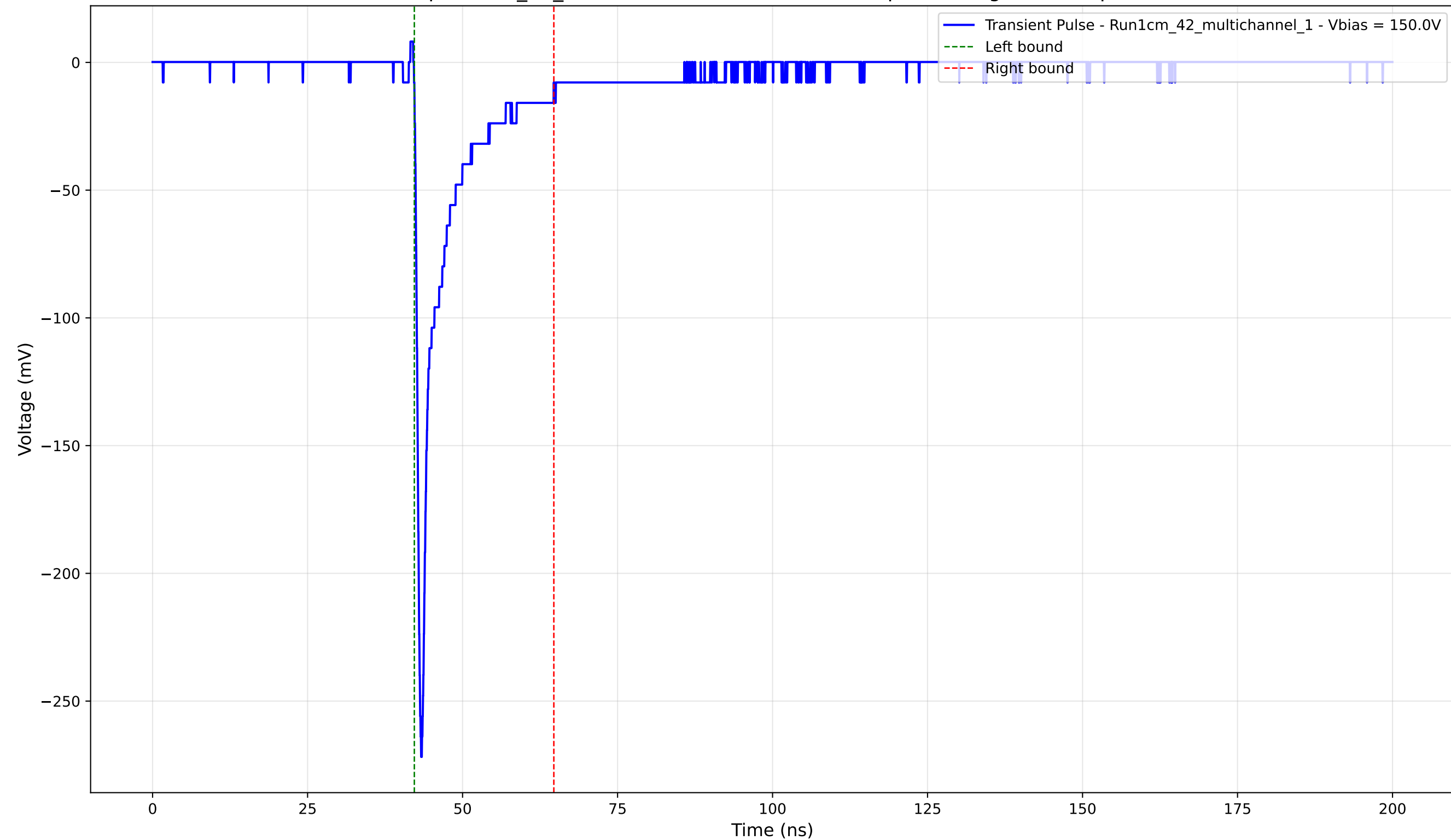
Transient Pulse - Sample: 1cm_42_multichannel - Position: 2730.0 \mu\text{m} - Charge: -23.04 pC - Rise Time: 0.79 ns
