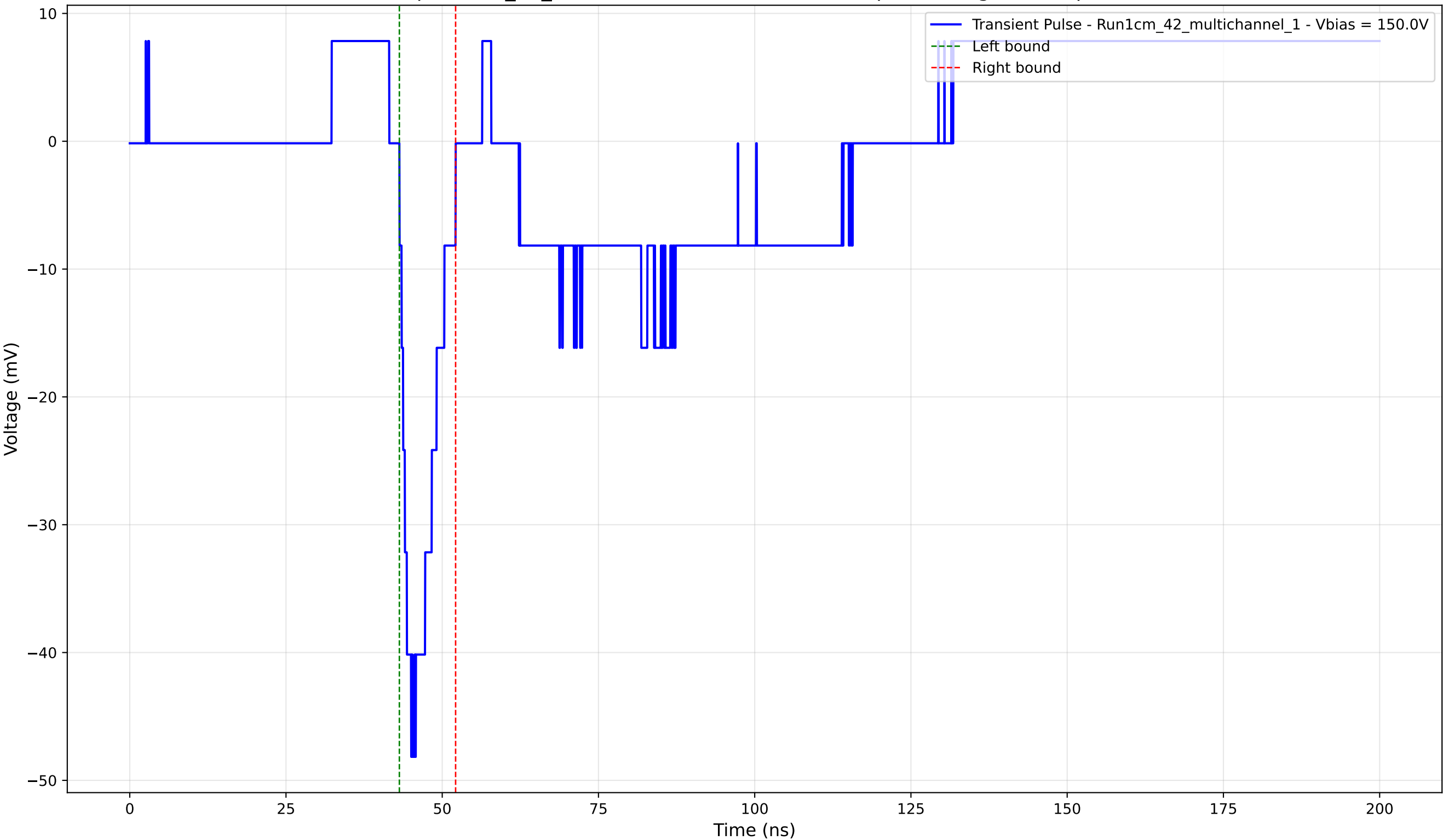
Transient Pulse - Sample: 1cm_42_multichannel - Position: 4265.0 \mu\text{m} - Charge: -4.65 pC - Rise Time: 1.87 ns
