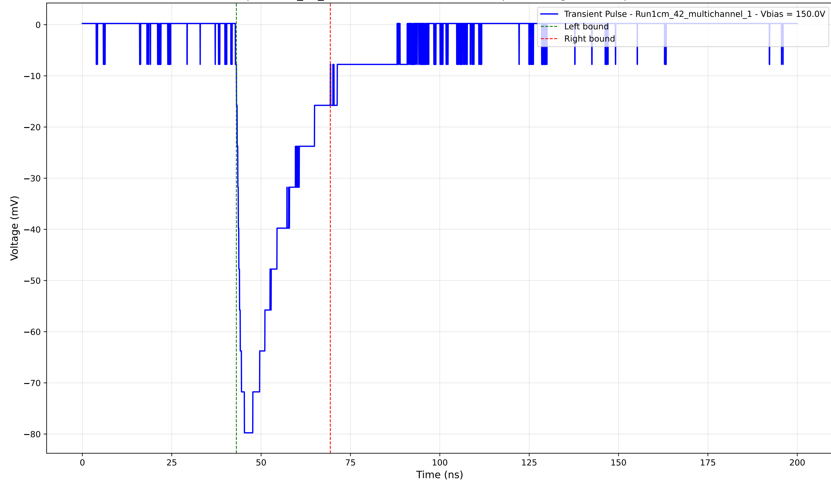
Transient Pulse - Sample: 1cm_42_multichannel - Position: 765.0 \mu\text{m} - Charge: -22.11 pC - Rise Time: 2.24 ns
