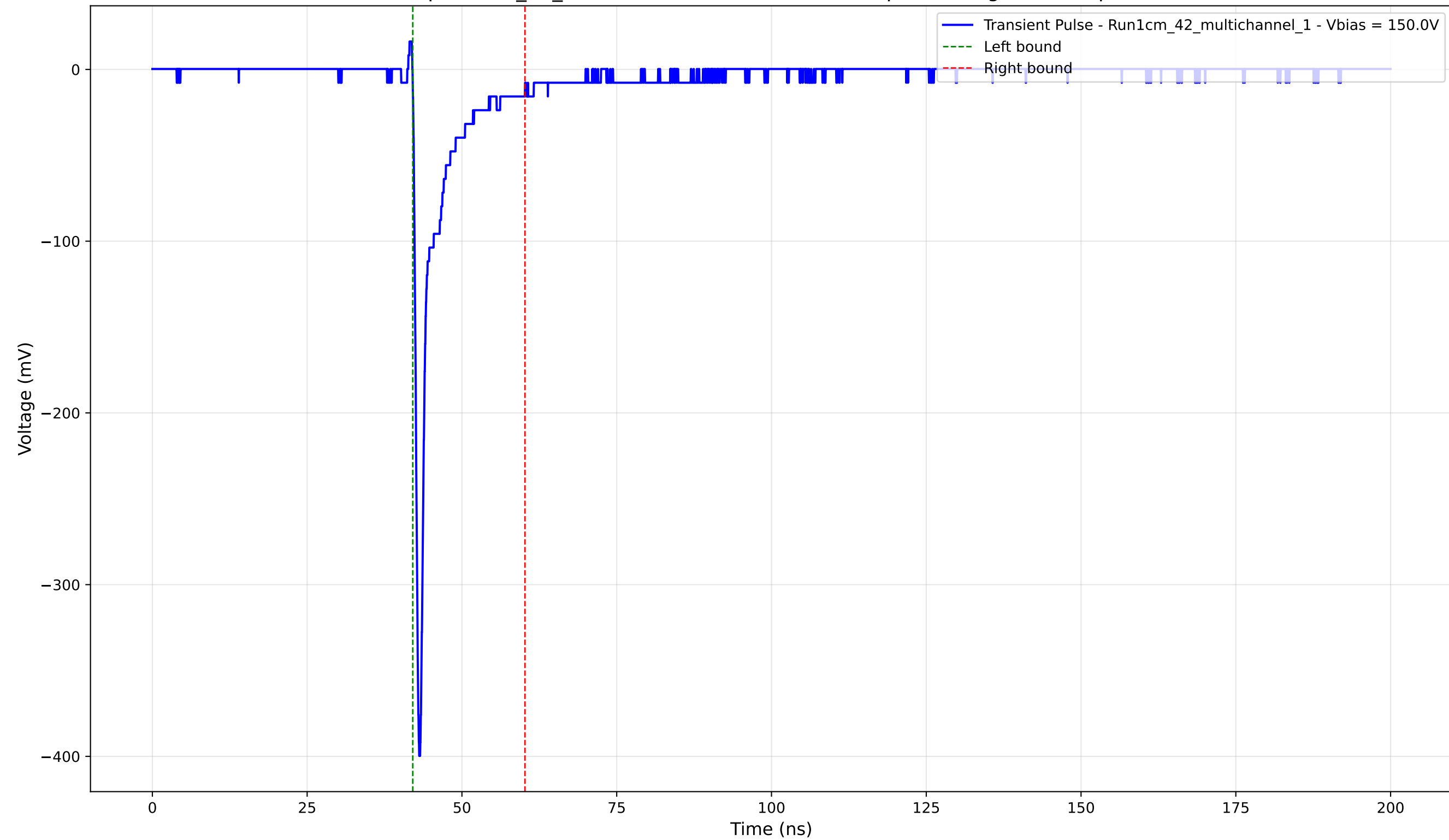
Transient Pulse - Sample: 1cm_42_multichannel - Position: 2480.0 \mu\text{m} - Charge: -23.36 pC - Rise Time: 0.72 ns
