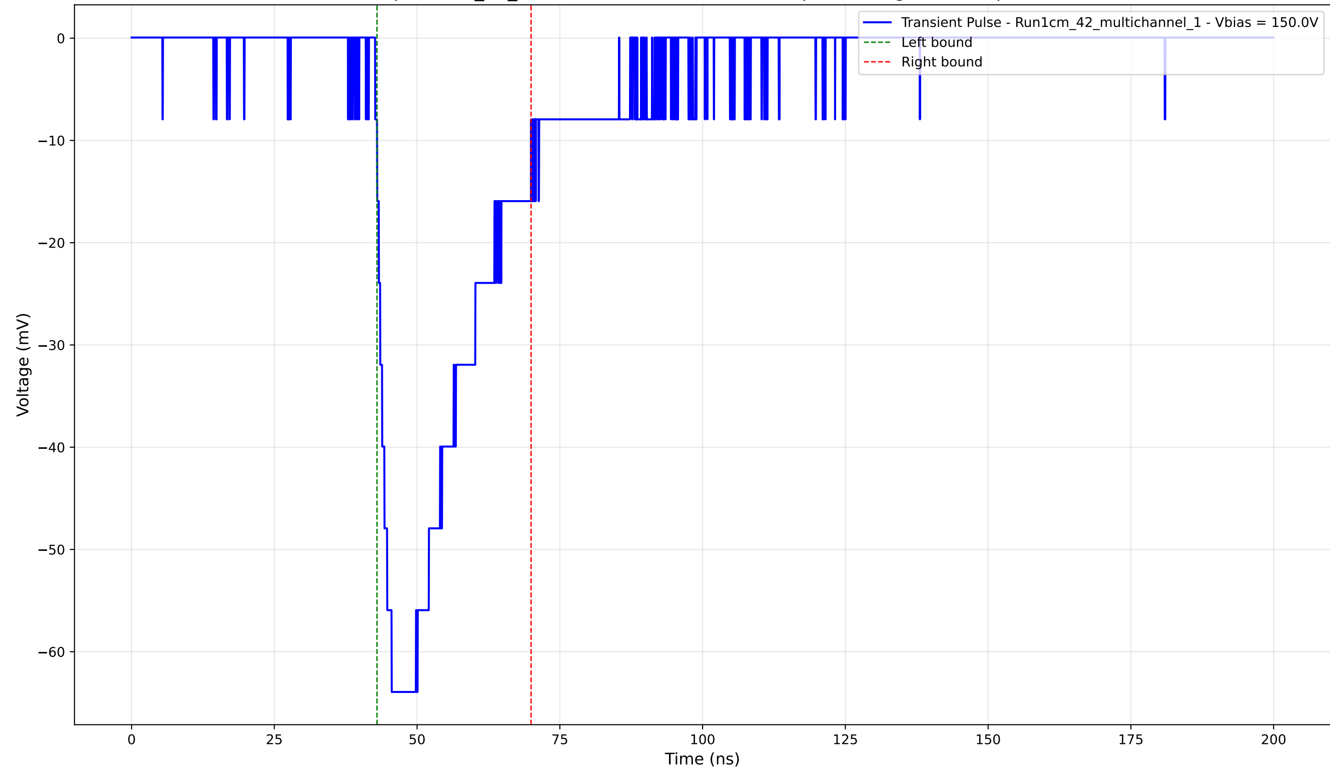
Transient Pulse - Sample: 1cm_42_multichannel - Position: 250.0 \mu\text{m} - Charge: -20.09 pC - Rise Time: 2.88 ns
