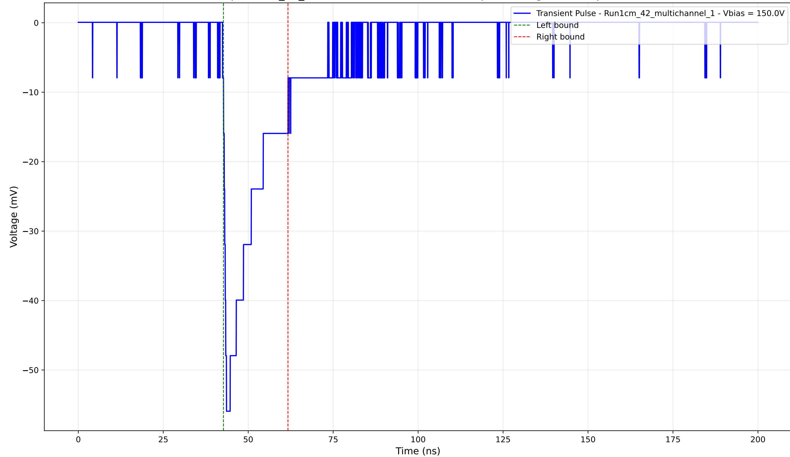
Transient Pulse - Sample: 1cm_42_multichannel - Position: 1425.0 \mu\text{m} - Charge: -10.66 pC - Rise Time: 1.17 ns
