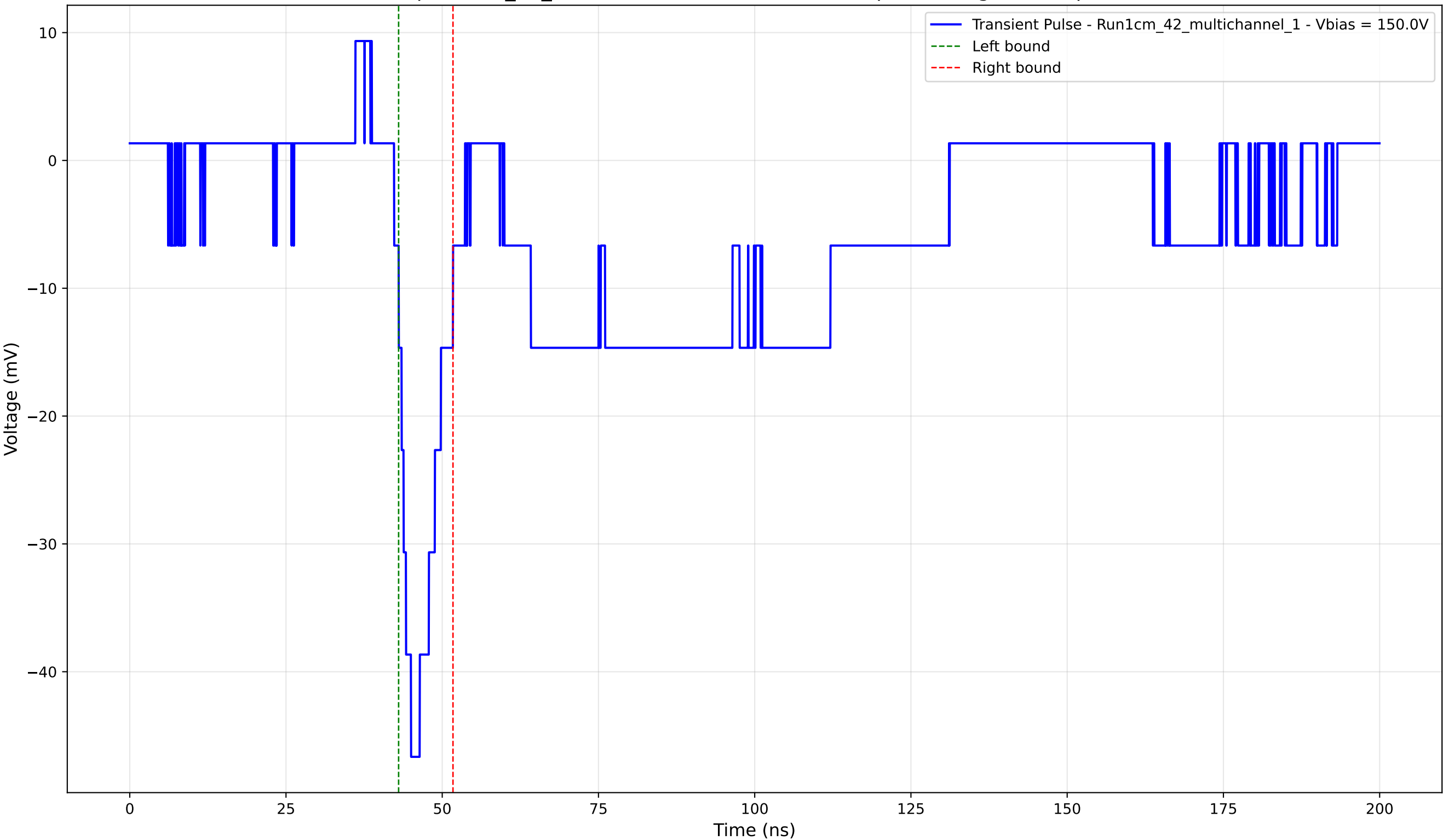
Transient Pulse - Sample: 1cm_42_multichannel - Position: 4615.0 \mu\text{m} - Charge: -5.16 pC - Rise Time: 2.71 ns
