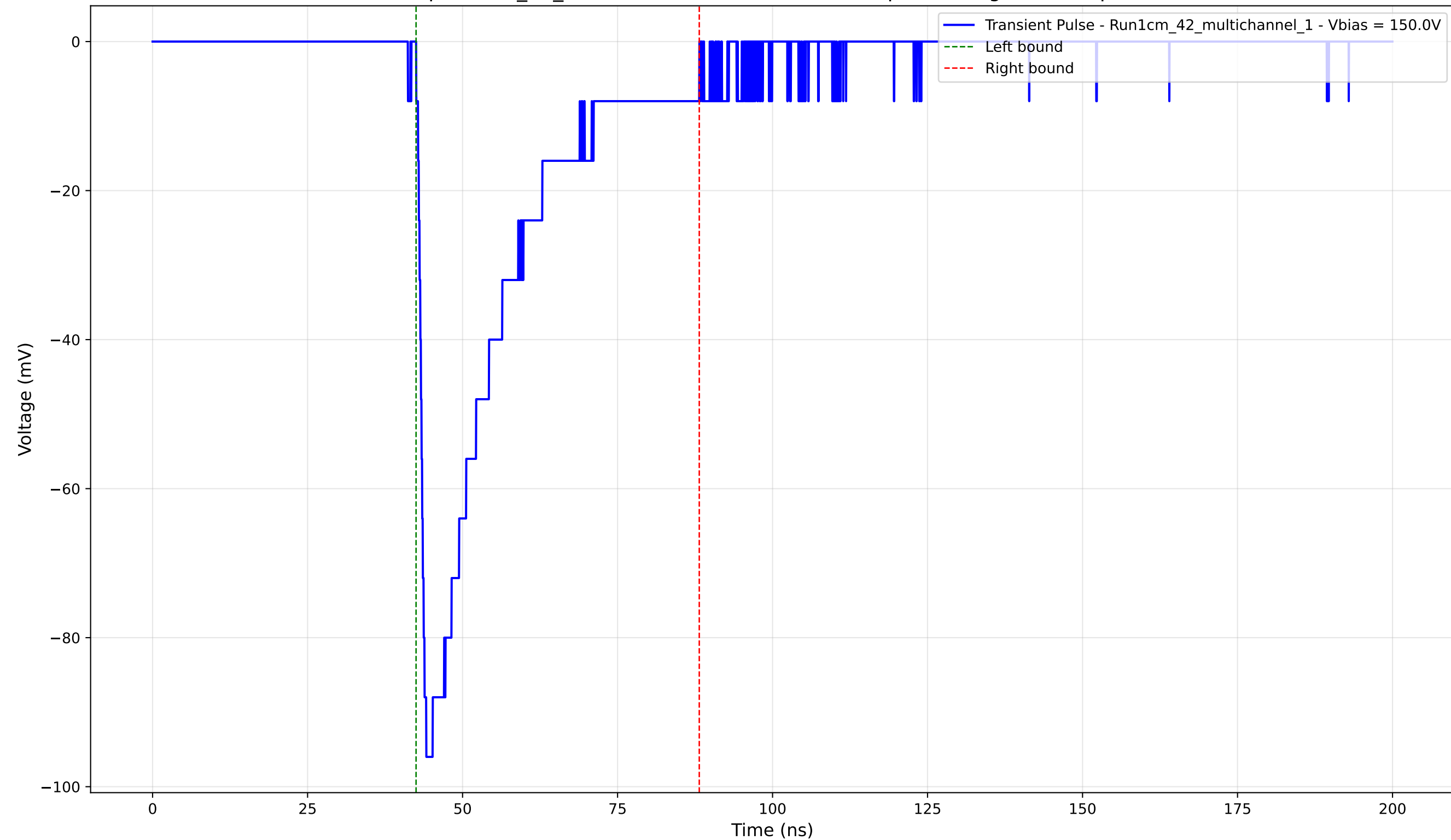
Transient Pulse - Sample: 1cm_42_multichannel - Position: 1175.0 \mu\text{m} - Charge: -26.35 pC - Rise Time: 1.06 ns
