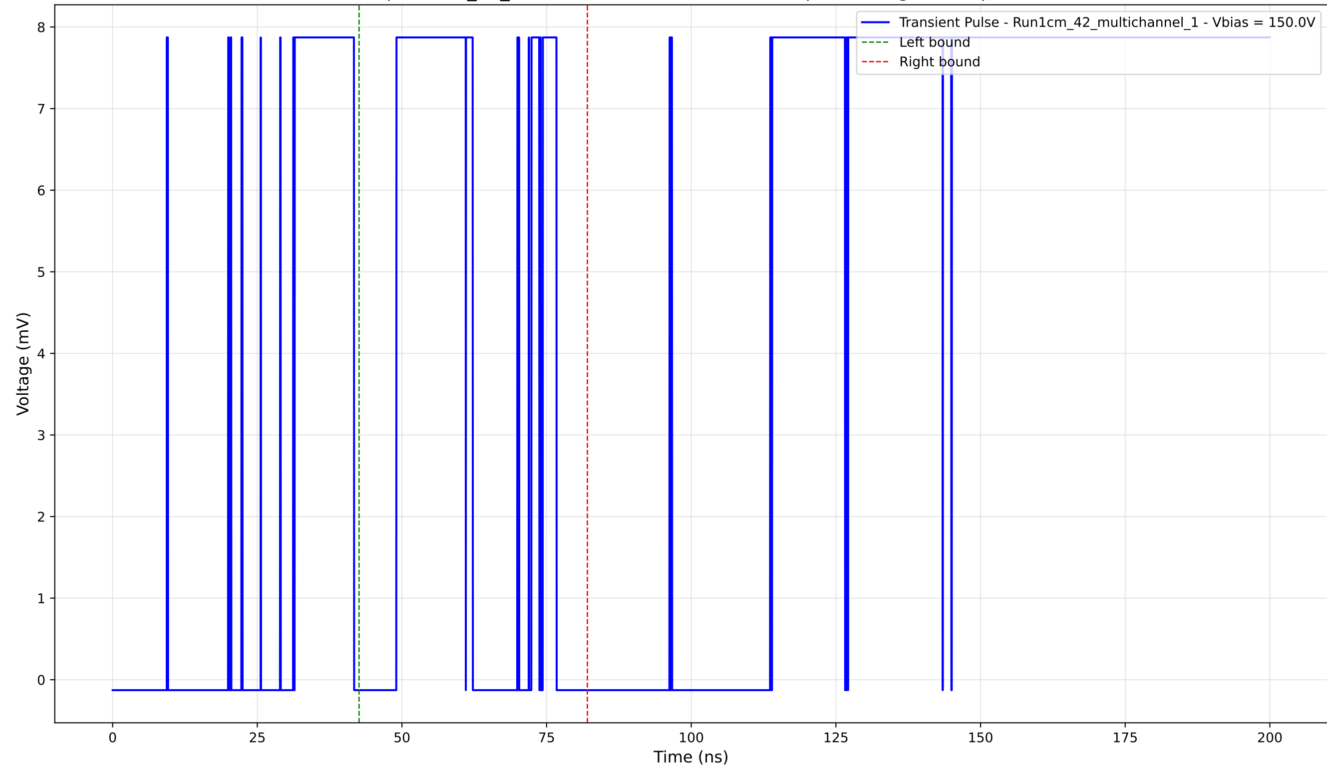
Transient Pulse - Sample: 1cm_42_multichannel - Position: 3925.0 \mu\text{m} - Charge: 2.66 pC - Rise Time: 0.02 ns
