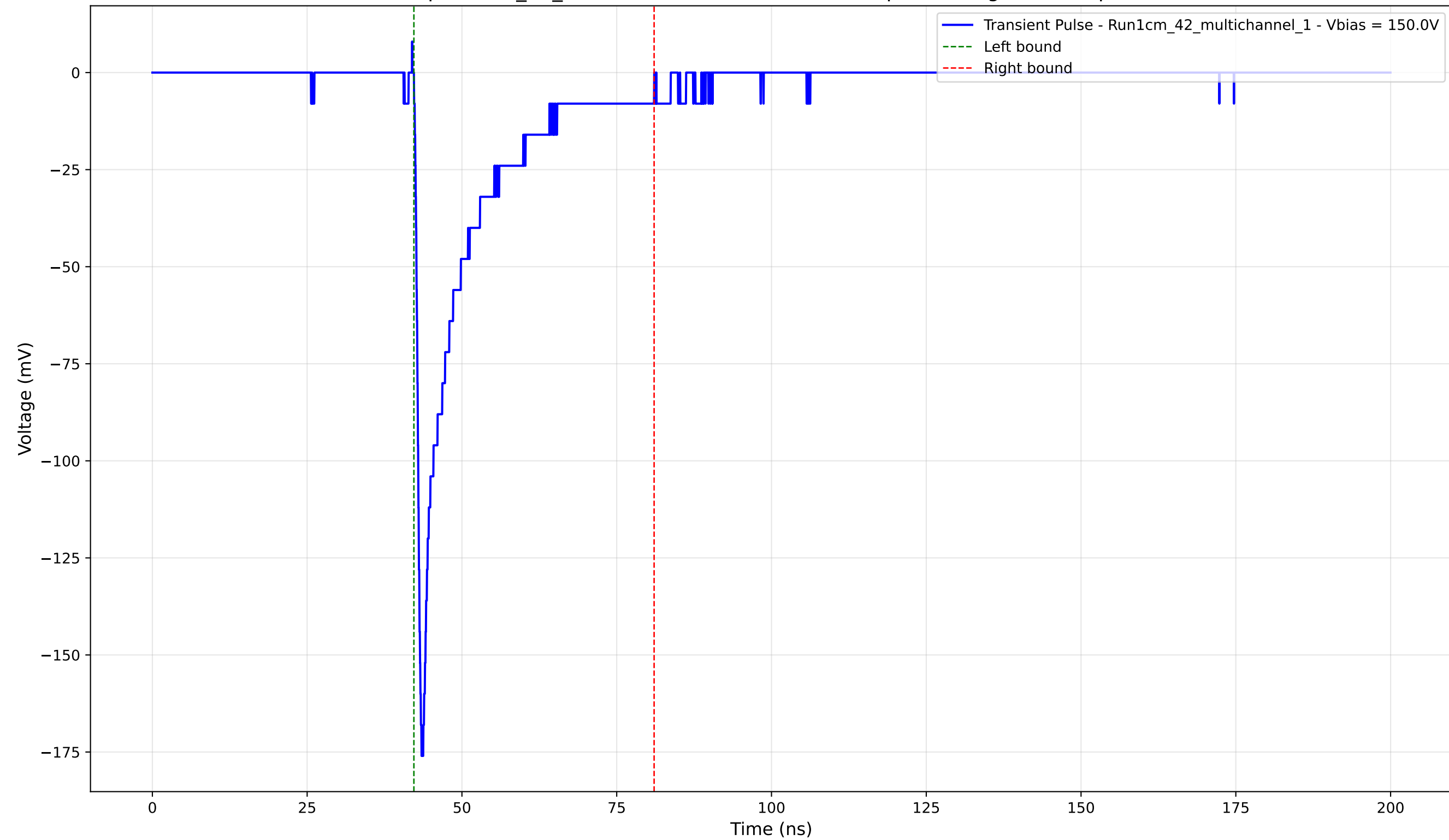
Transient Pulse - Sample: 1cm_42_multichannel - Position: 1765.0 \mu\text{m} - Charge: -24.44 pC - Rise Time: 0.84 ns
