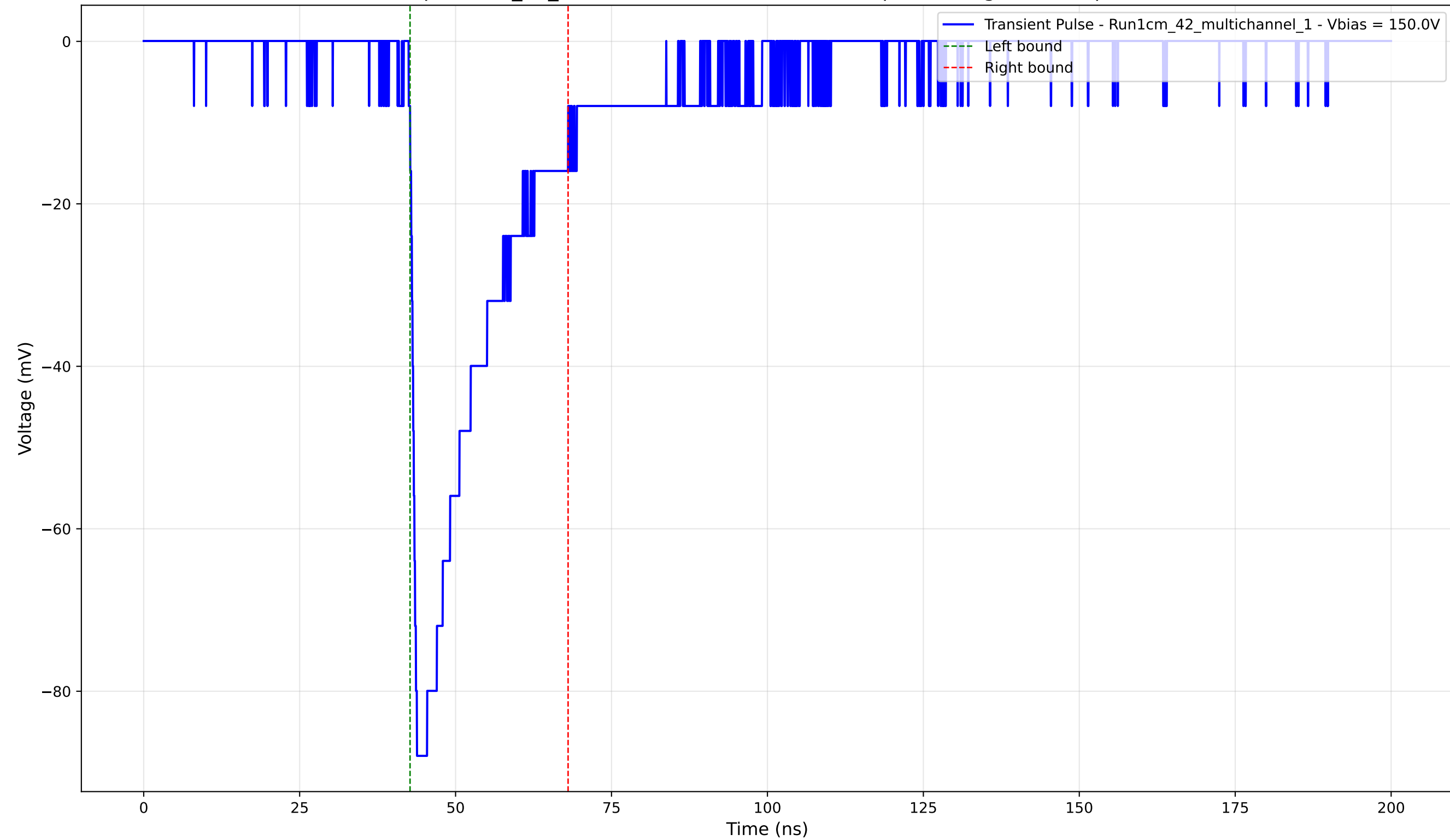
Transient Pulse - Sample: 1cm_42_multichannel - Position: 1295.0 \mu\text{m} - Charge: -20.52 pC - Rise Time: 0.94 ns
