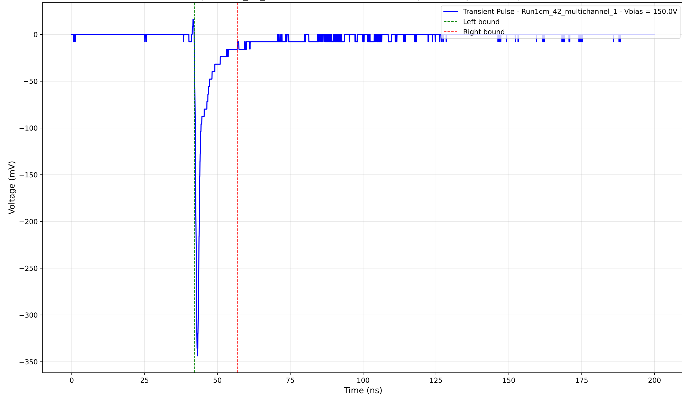
Transient Pulse - Sample: 1cm_42_multichannel - Position: 2320.0 \mu\text{m} - Charge: -18.86 pC - Rise Time: 0.75 ns
