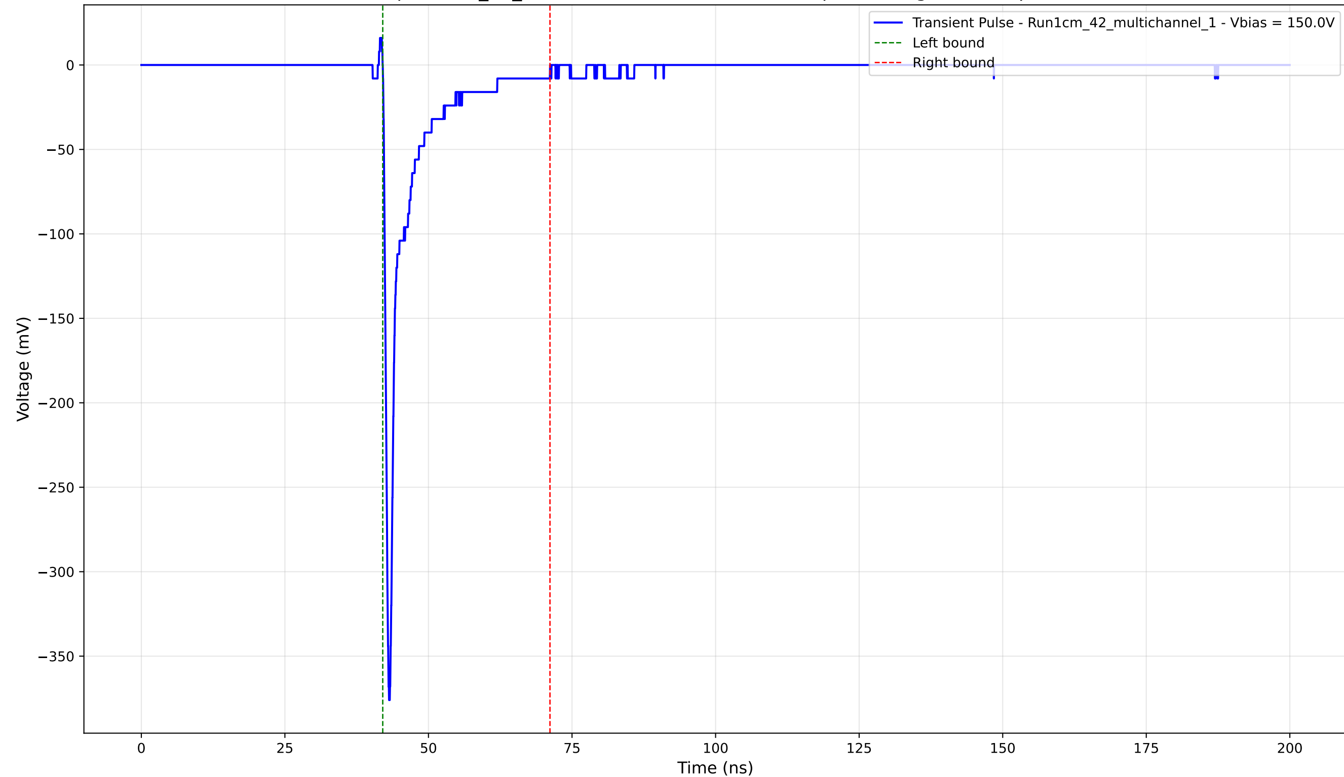
Transient Pulse - Sample: 1cm_42_multichannel - Position: 2530.0 \mu\text{m} - Charge: -25.31 pC - Rise Time: 0.75 ns
