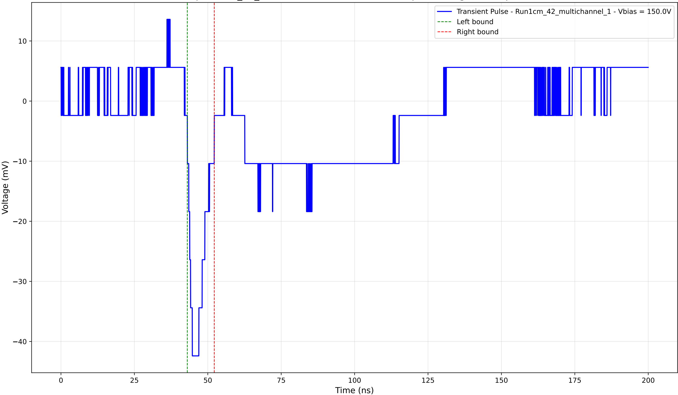
Transient Pulse - Sample: 1cm_42_multichannel - Position: 4550.0 \mu\text{m} - Charge: -4.82 pC - Rise Time: 1.70 ns
