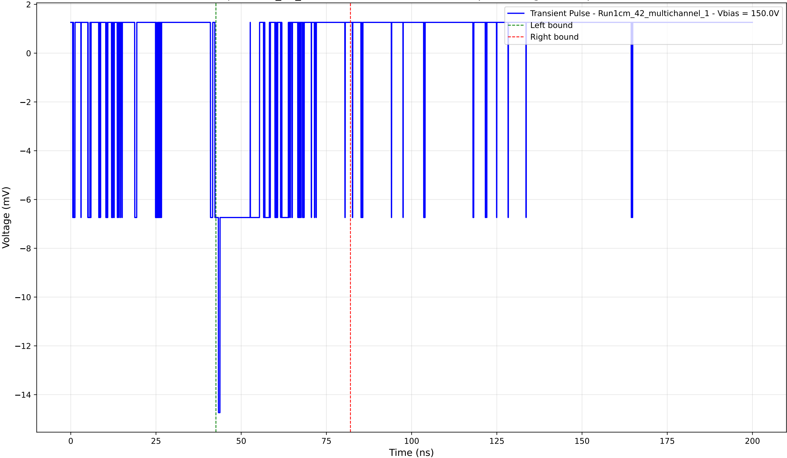
Transient Pulse - Sample: 1cm_42_multichannel - Position: 1865.0 \mu\text{m} - Charge: -2.00 pC - Rise Time: 1.06 ns
