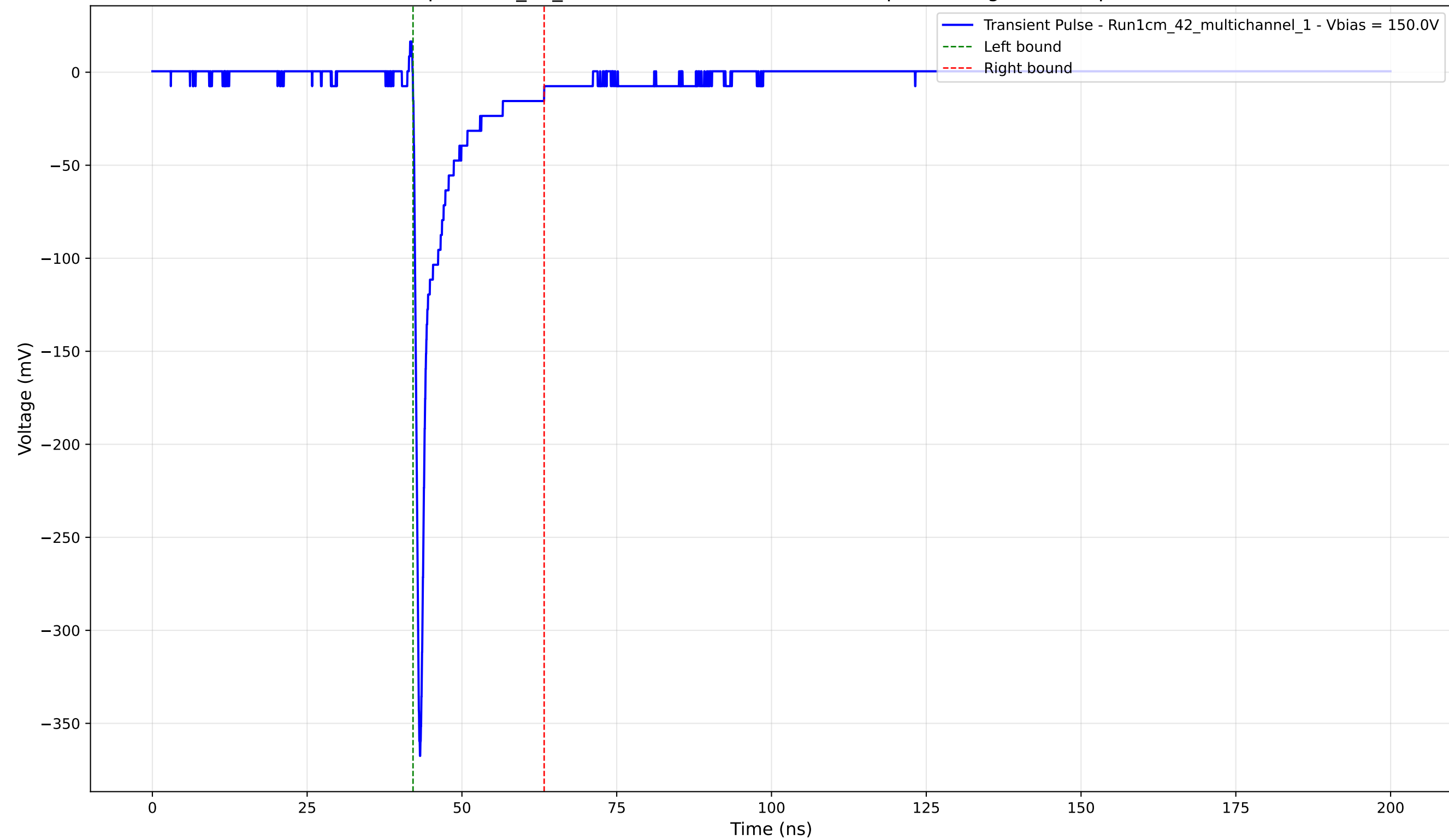
Transient Pulse - Sample: 1cm_42_multichannel - Position: 2205.0 \mu\text{m} - Charge: -24.61 pC - Rise Time: 0.77 ns
