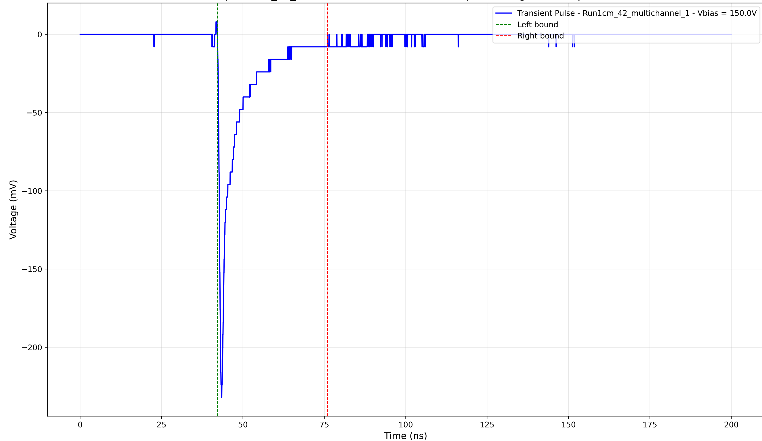
Transient Pulse - Sample: 1cm_42_multichannel - Position: 1965.0 \mu\text{m} - Charge: -23.88 pC - Rise Time: 0.86 ns
