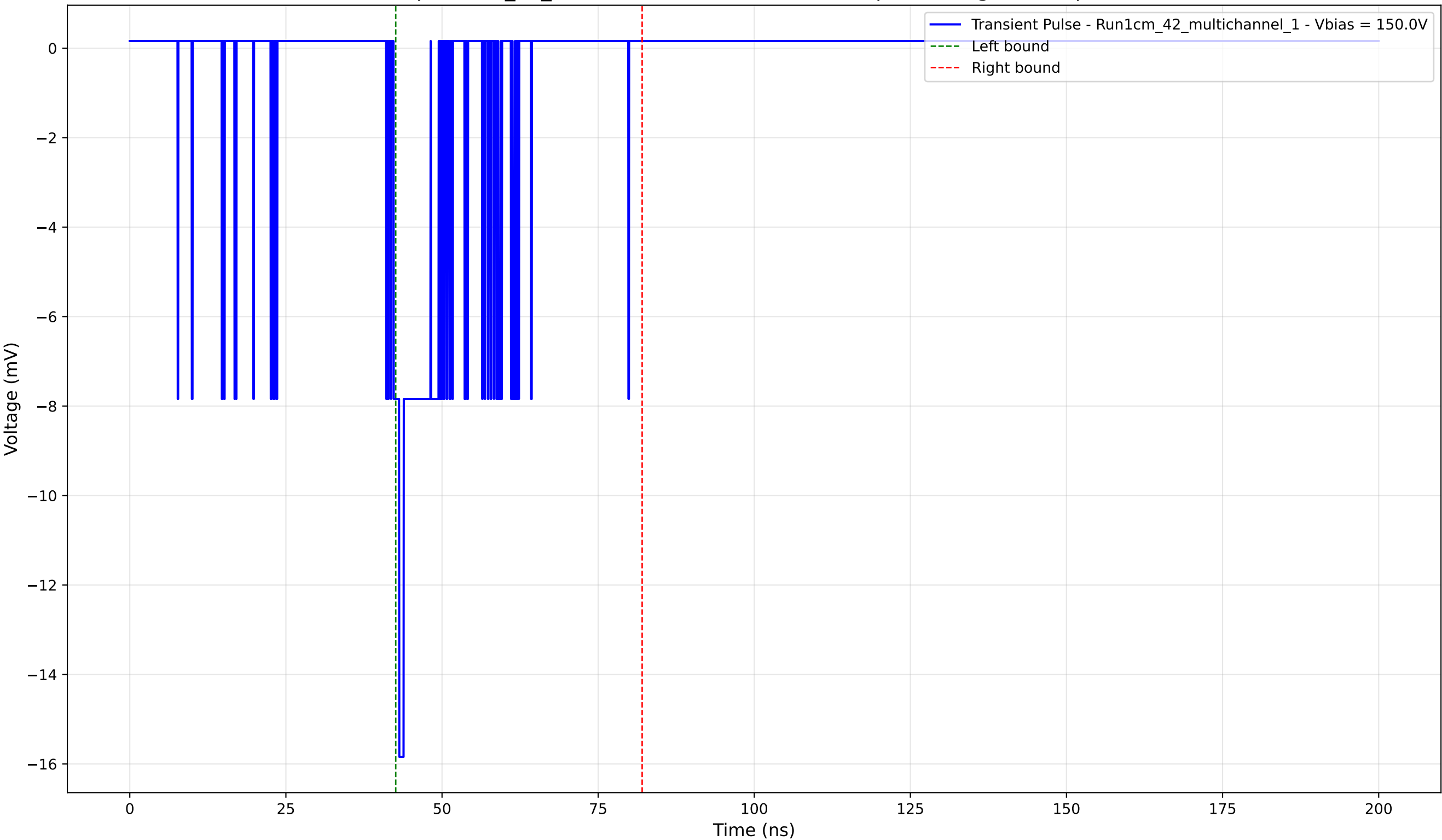
Transient Pulse - Sample: 1cm_42_multichannel - Position: 2880.0 \mu\text{m} - Charge: -1.60 pC - Rise Time: 0.92 ns
