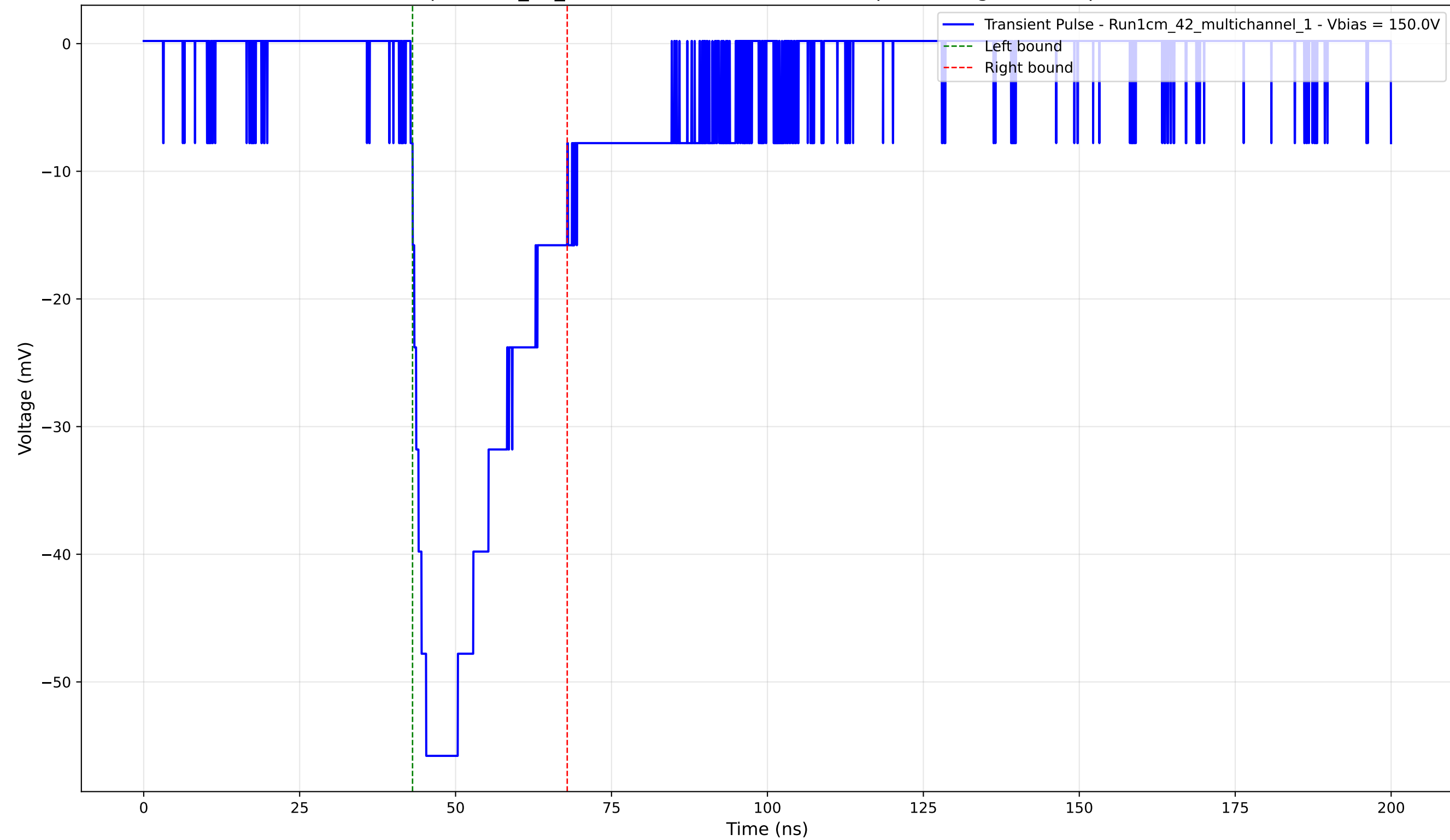
Transient Pulse - Sample: 1cm_42_multichannel - Position: 290.0 \mu\text{m} - Charge: -17.28 pC - Rise Time: 2.51 ns
