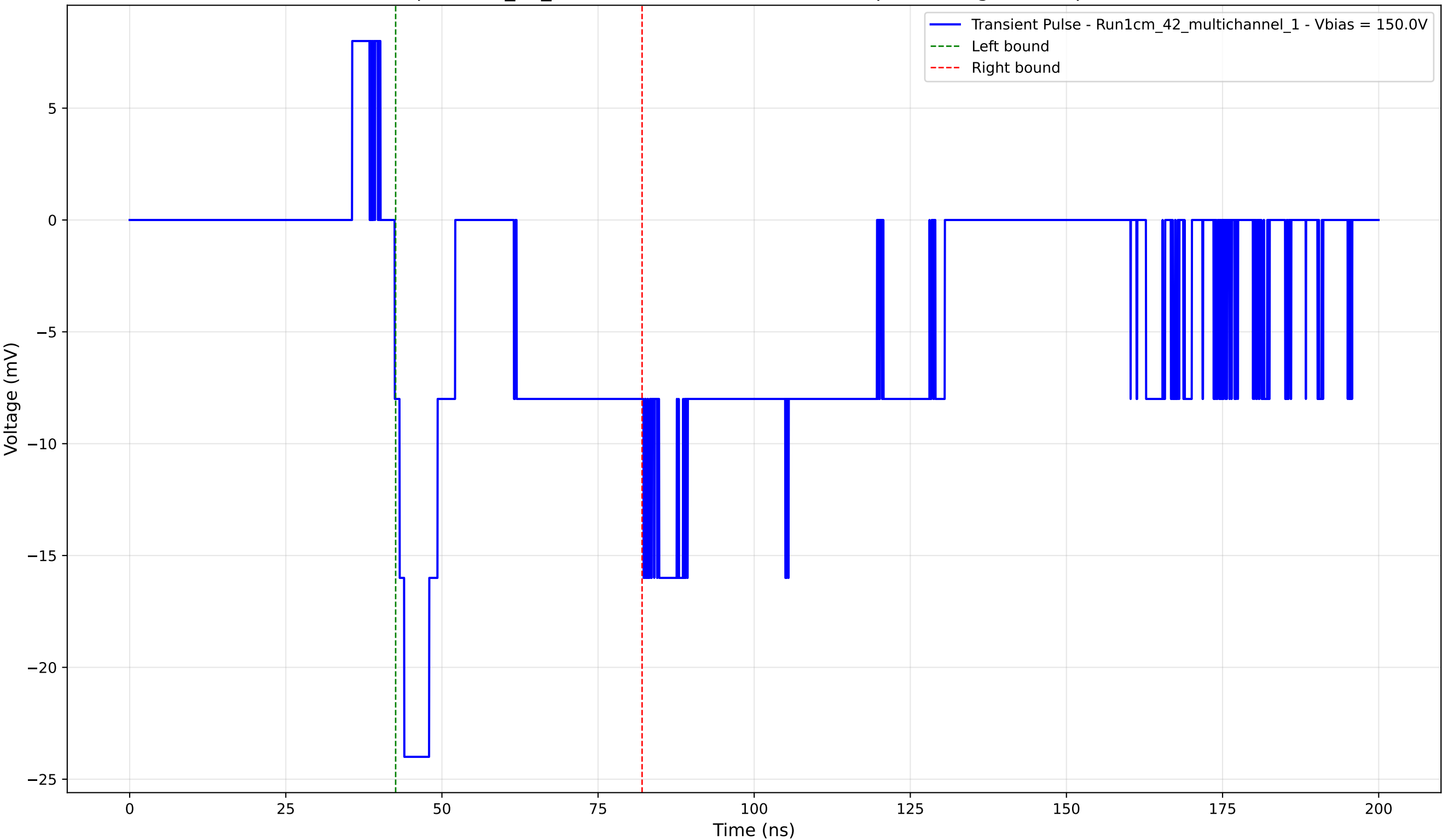
Transient Pulse - Sample: 1cm_42_multichannel - Position: 4850.0 \mu\text{m} - Charge: -6.38 pC - Rise Time: 1.53 ns
