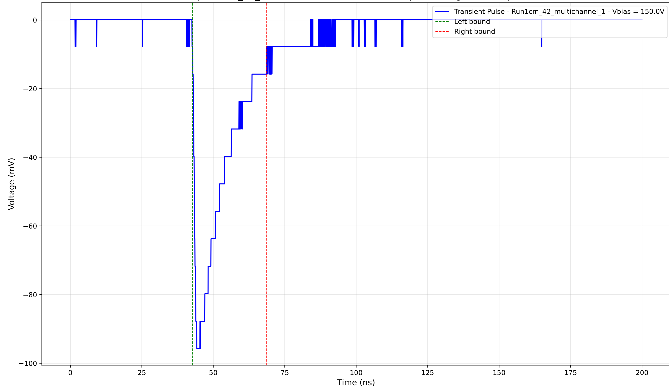
Transient Pulse - Sample: 1cm_42_multichannel - Position: 1180.0 \mu\text{m} - Charge: -22.70 pC - Rise Time: 1.08 ns
