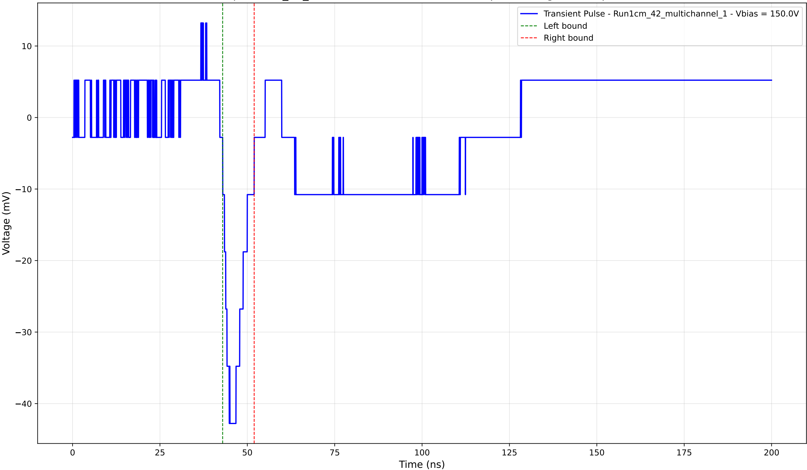
Transient Pulse - Sample: 1cm_42_multichannel - Position: 4690.0 \mu\text{m} - Charge: -4.66 pC - Rise Time: 1.88 ns
