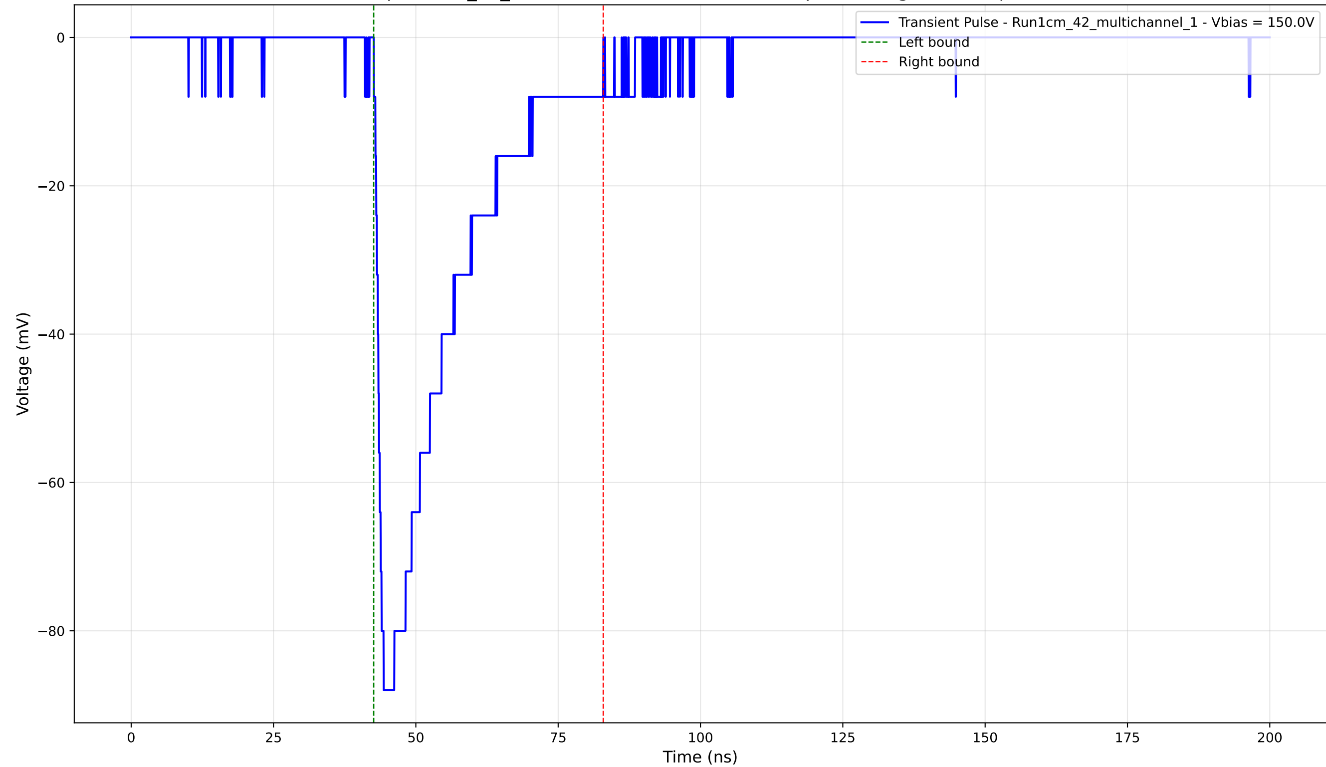
Transient Pulse - Sample: 1cm_42_multichannel - Position: 1065.0 \mu\text{m} - Charge: -25.18 pC - Rise Time: 1.10 ns
