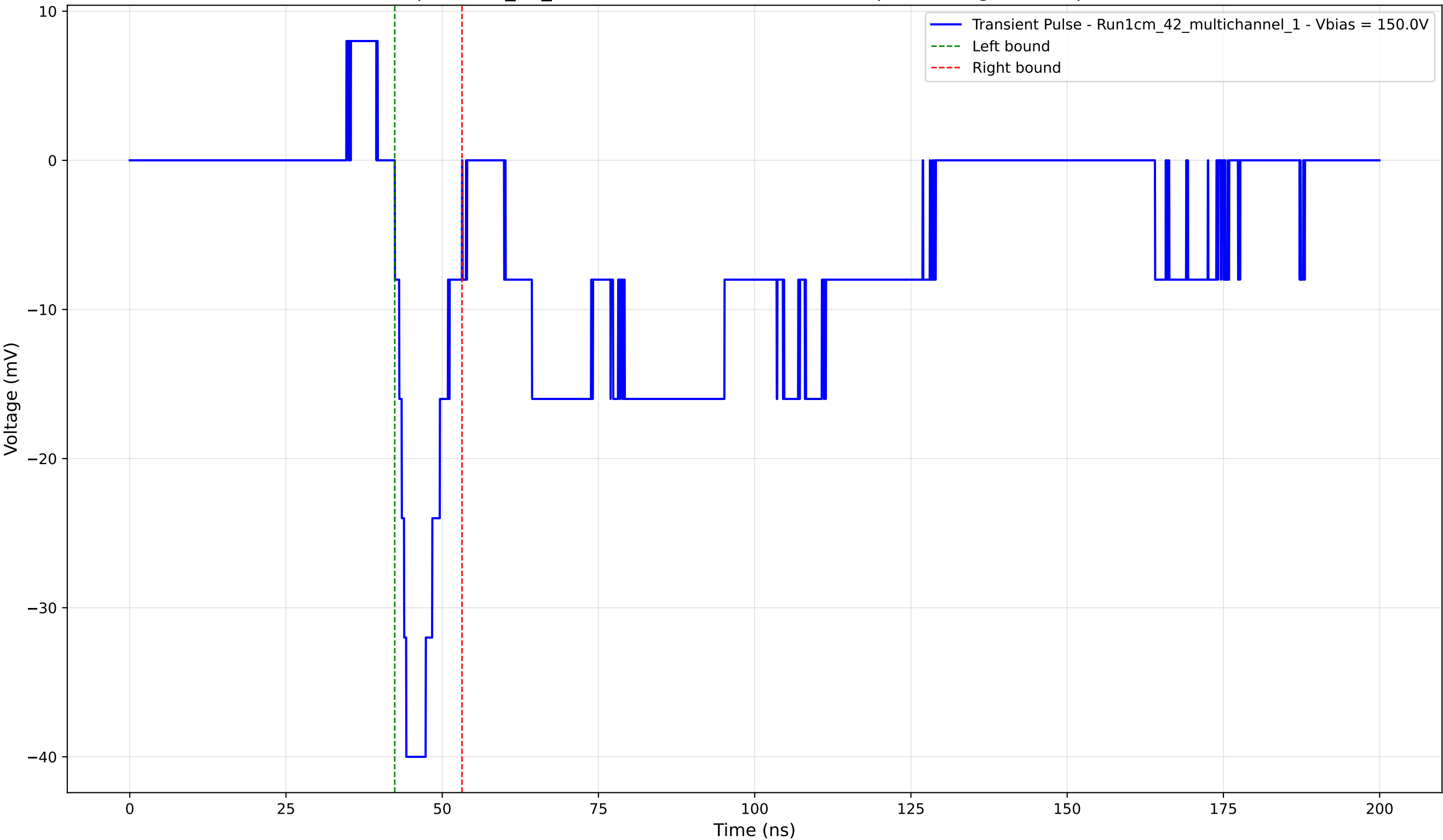
Transient Pulse - Sample: 1cm_42_multichannel - Position: 4770.0 \mu\text{m} - Charge: -5.19 pC - Rise Time: 1.83 ns
