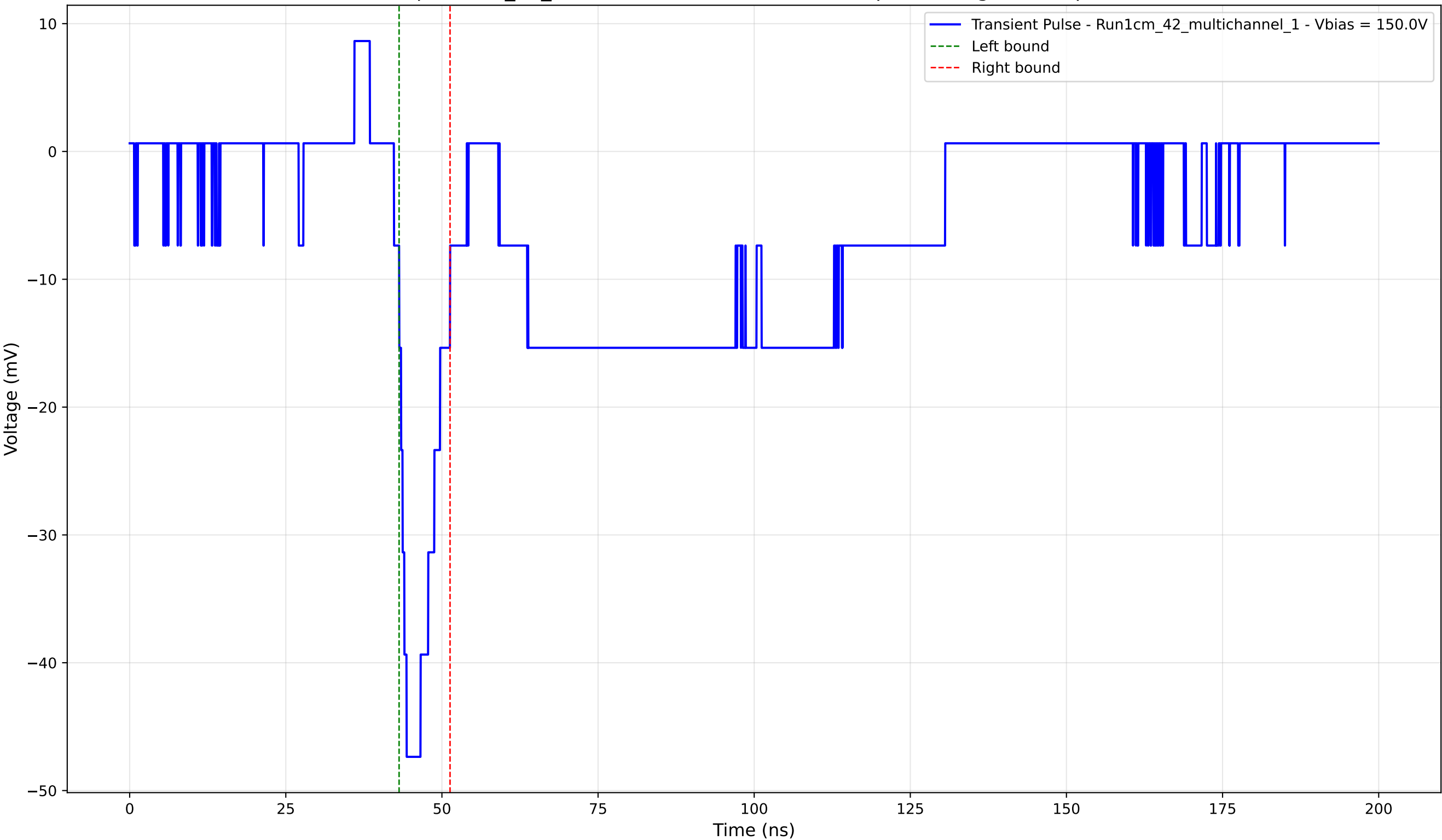
Transient Pulse - Sample: 1cm_42_multichannel - Position: 4095.0 \mu\text{m} - Charge: -5.28 pC - Rise Time: 2.03 ns
