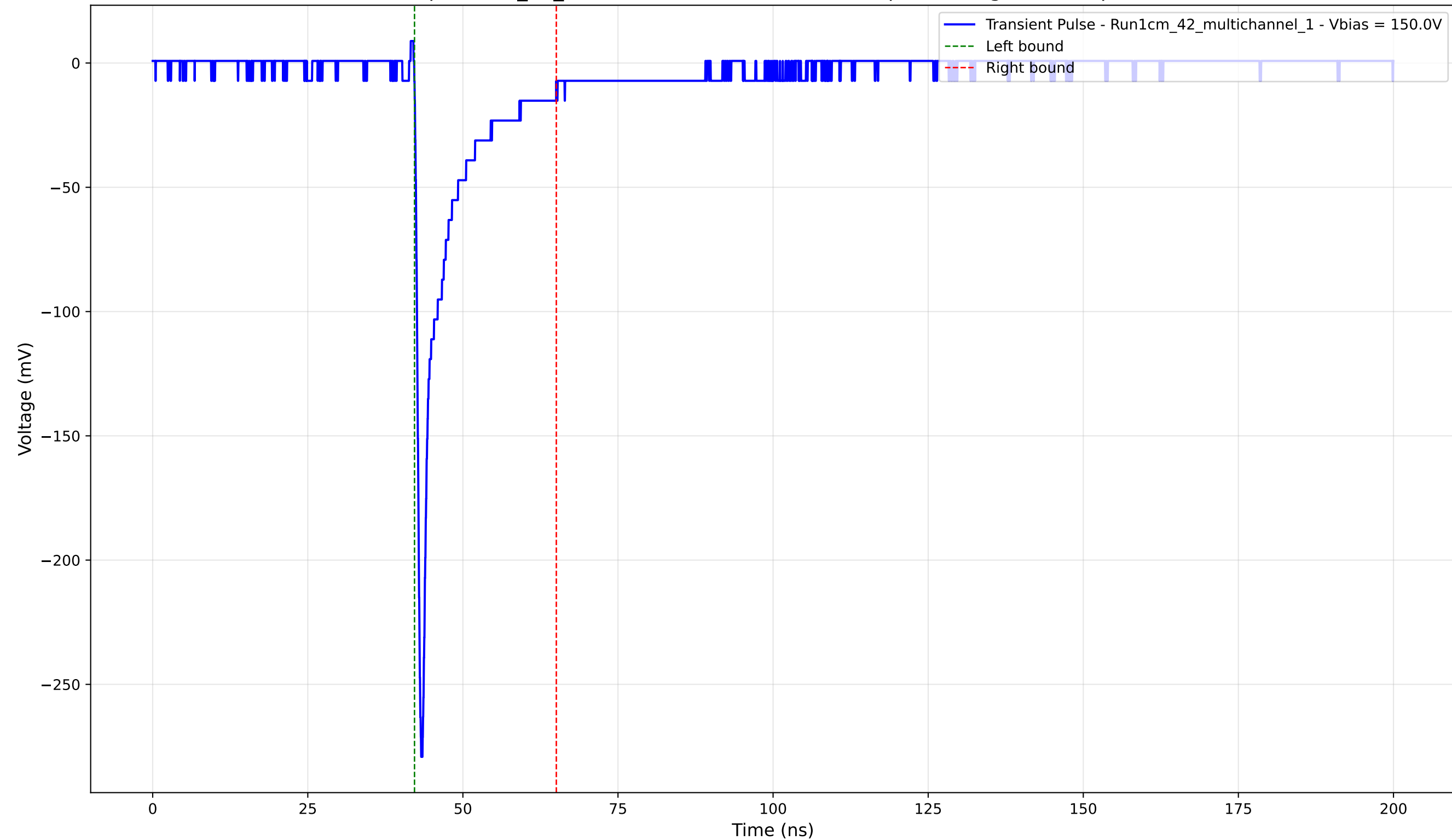
Transient Pulse - Sample: 1cm_42_multichannel - Position: 2045.0 \mu\text{m} - Charge: -24.09 pC - Rise Time: 0.79 ns
