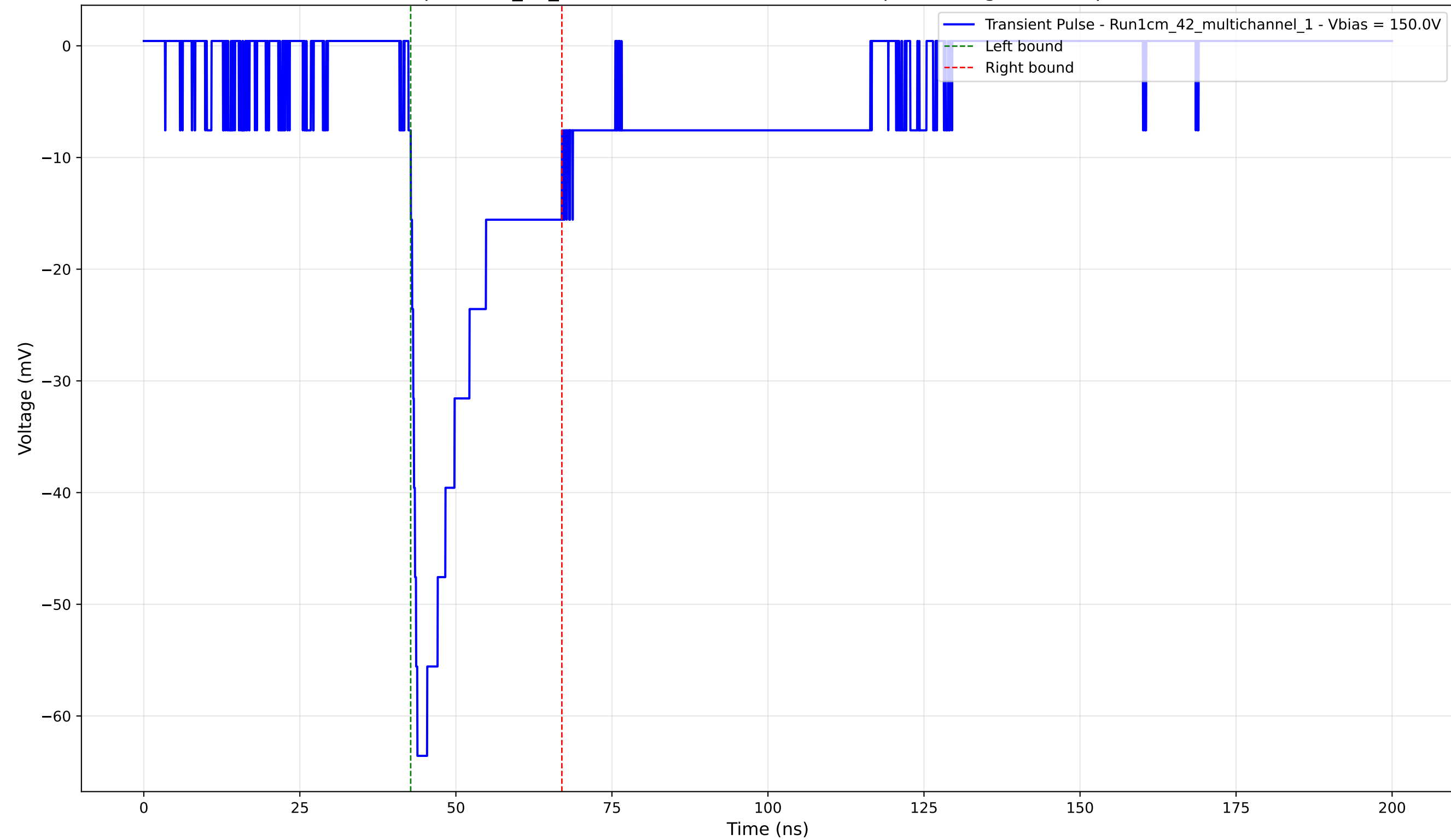
Transient Pulse - Sample: 1cm_42_multichannel - Position: 3640.0 \mu\text{m} - Charge: -13.50 pC - Rise Time: 1.42 ns
