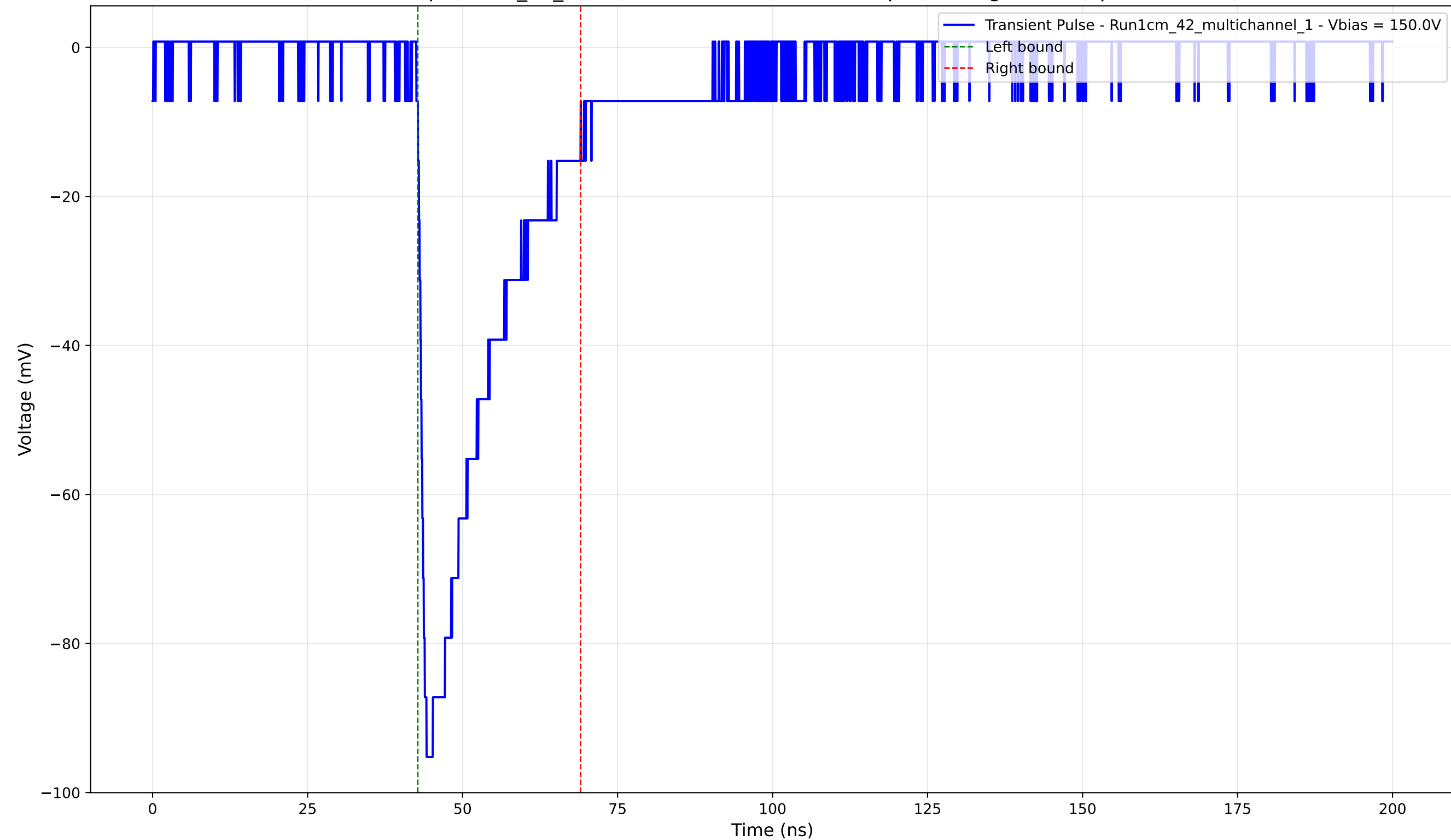
Transient Pulse - Sample: 1cm_42_multichannel - Position: 1170.0 \mu\text{m} - Charge: -23.12 pC - Rise Time: 1.11 ns
