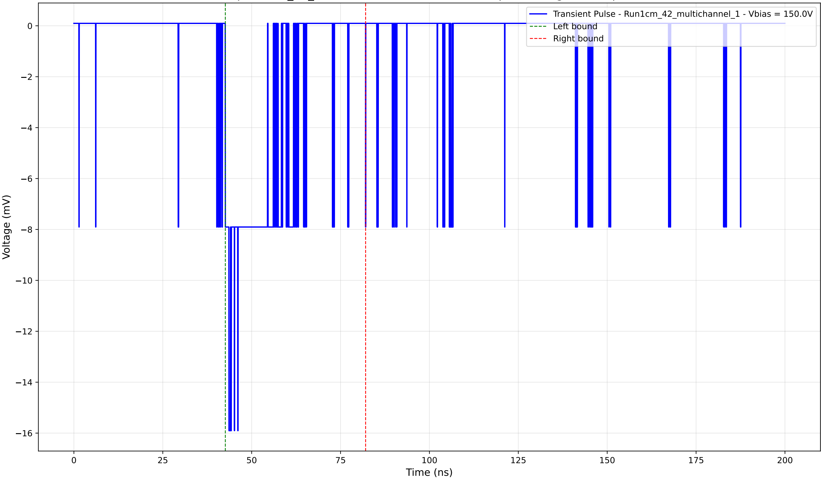
Transient Pulse - Sample: 1cm_42_multichannel - Position: 1400.0 \mu\text{m} - Charge: -2.95 pC - Rise Time: 1.04 ns
