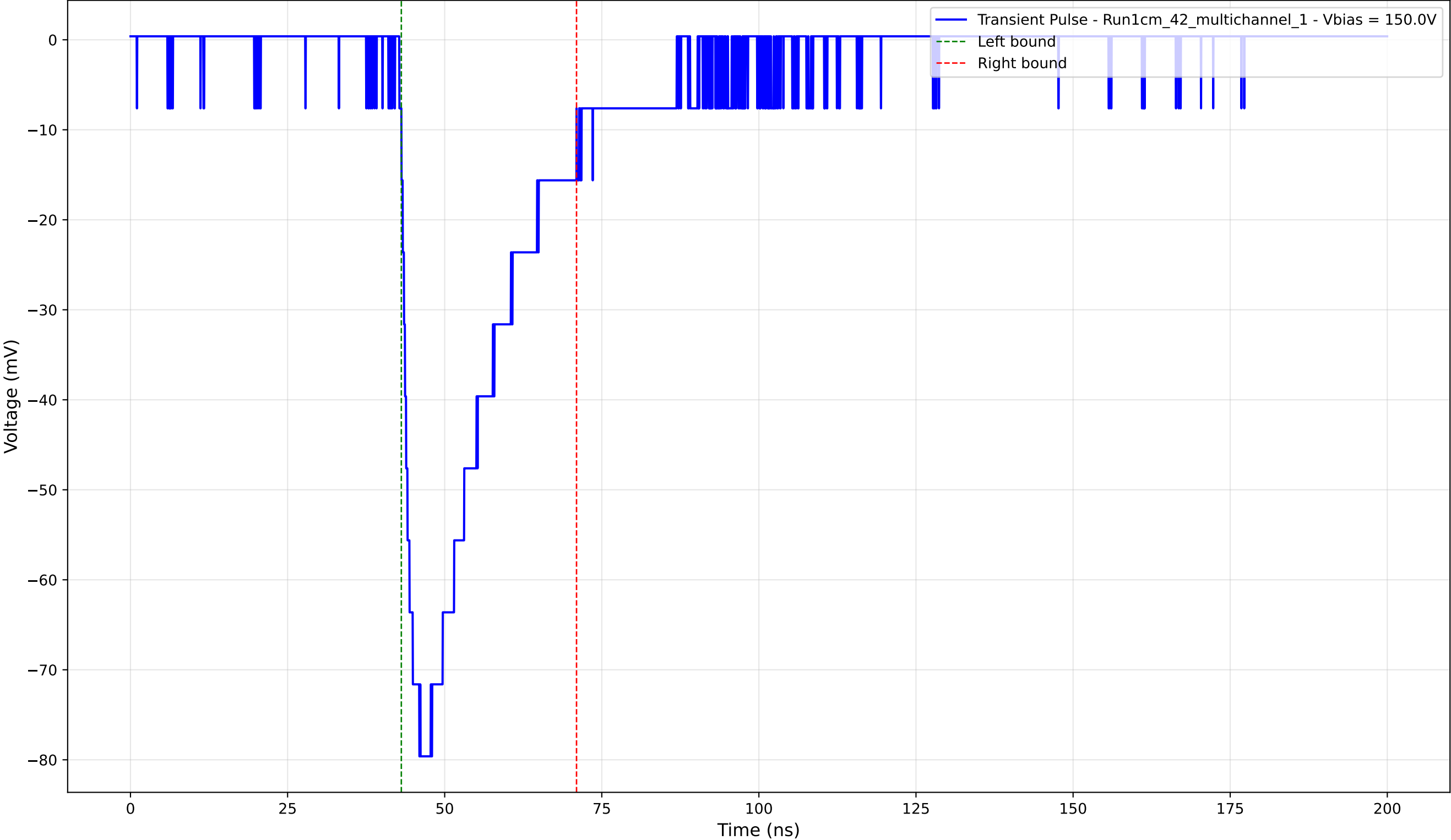
Transient Pulse - Sample: 1cm_42_multichannel - Position: 620.0 \mu\text{m} - Charge: -22.60 pC - Rise Time: 2.86 ns
