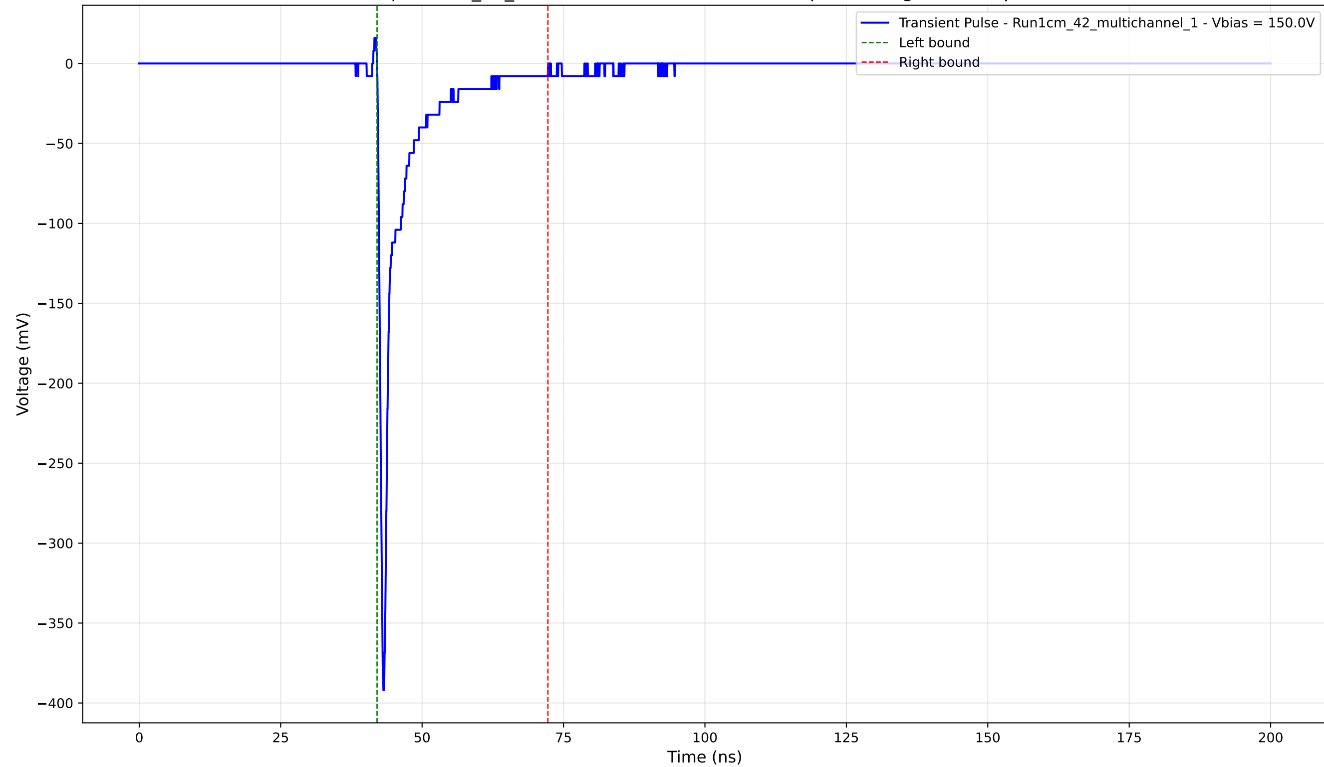
Transient Pulse - Sample: 1cm_42_multichannel - Position: 2250.0 \mu\text{m} - Charge: -26.60 pC - Rise Time: 0.76 ns
