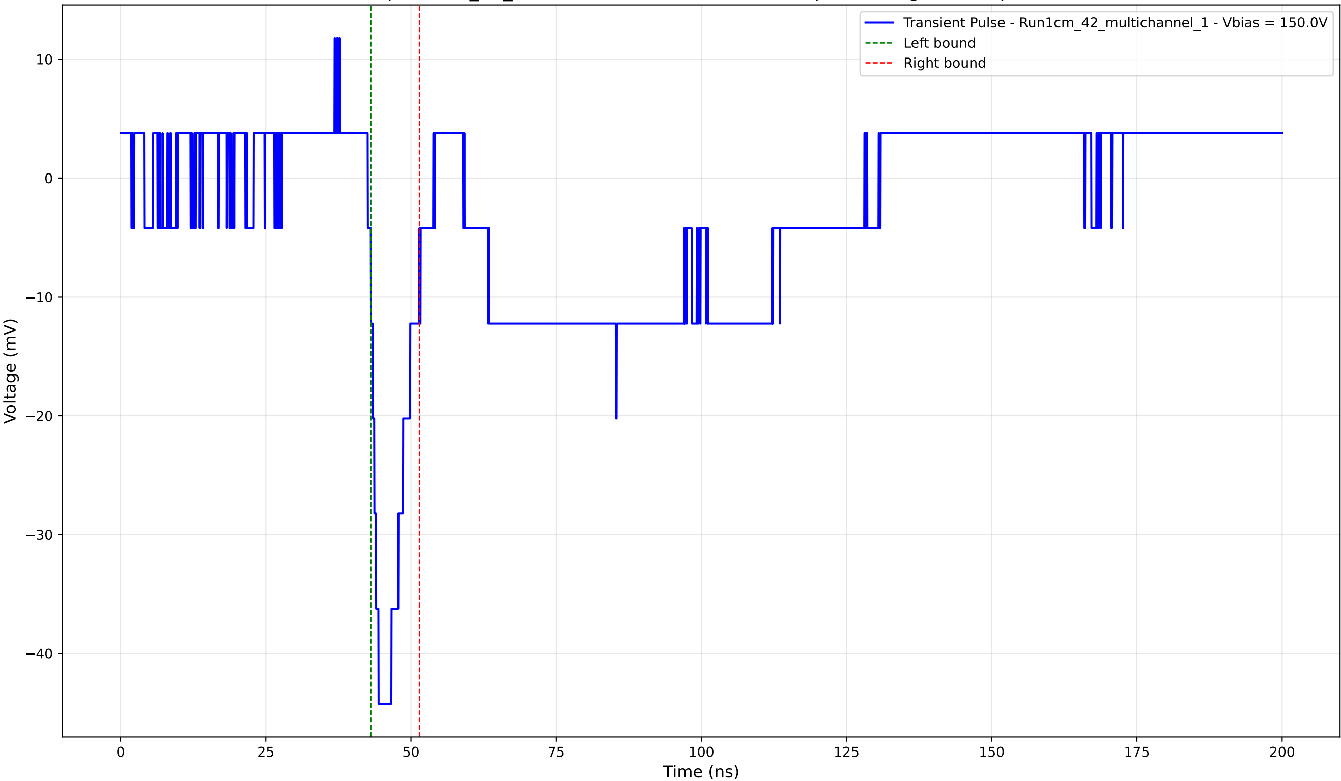
Transient Pulse - Sample: 1cm_42_multichannel - Position: 4120.0 \mu\text{m} - Charge: -4.84 pC - Rise Time: 1.32 ns
