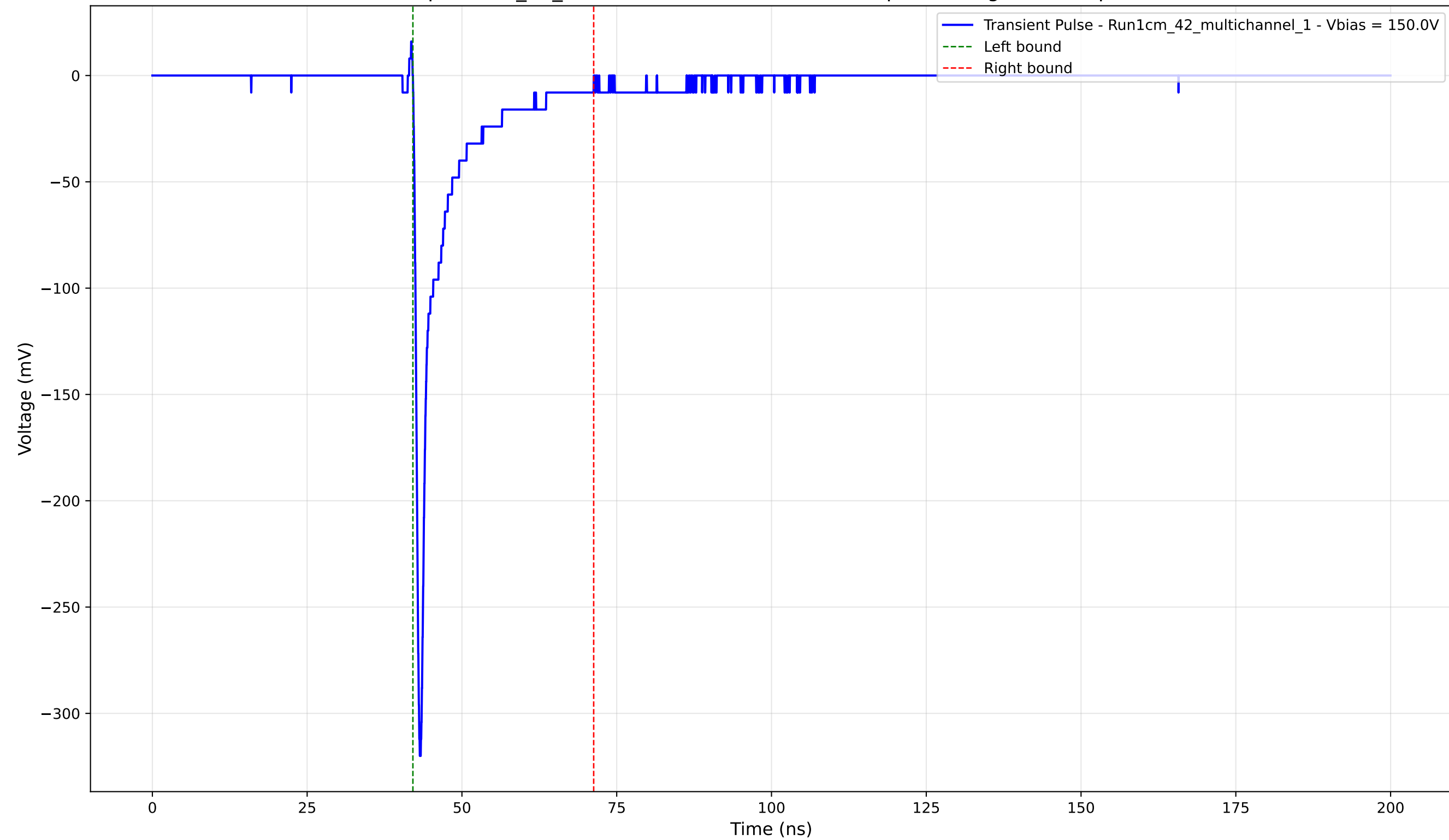
Transient Pulse - Sample: 1cm_42_multichannel - Position: 2620.0 \mu\text{m} - Charge: -24.55 pC - Rise Time: 0.74 ns
