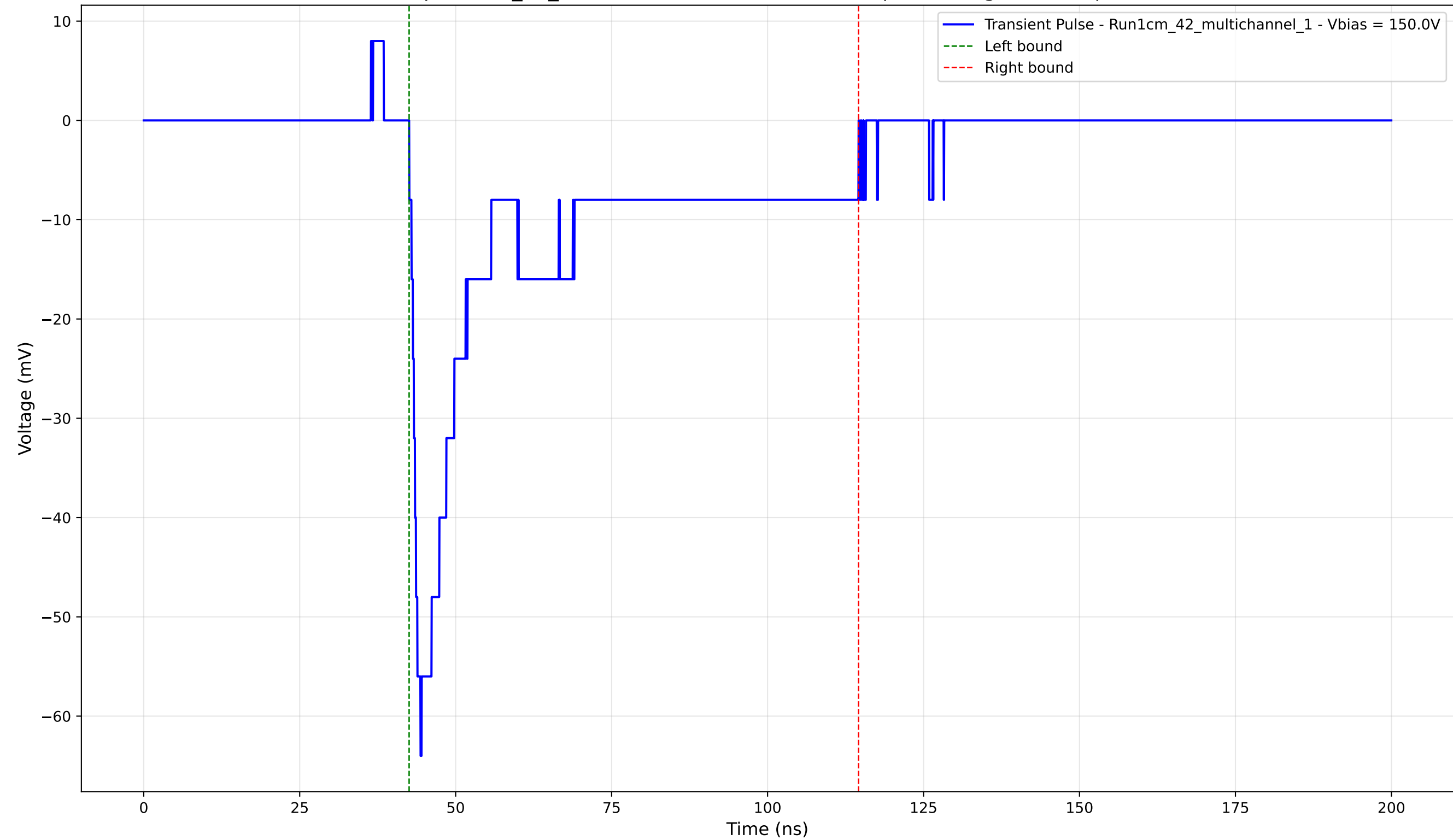
Transient Pulse - Sample: 1cm_42_multichannel - Position: 3740.0 \mu\text{m} - Charge: -19.18 pC - Rise Time: 1.80 ns
