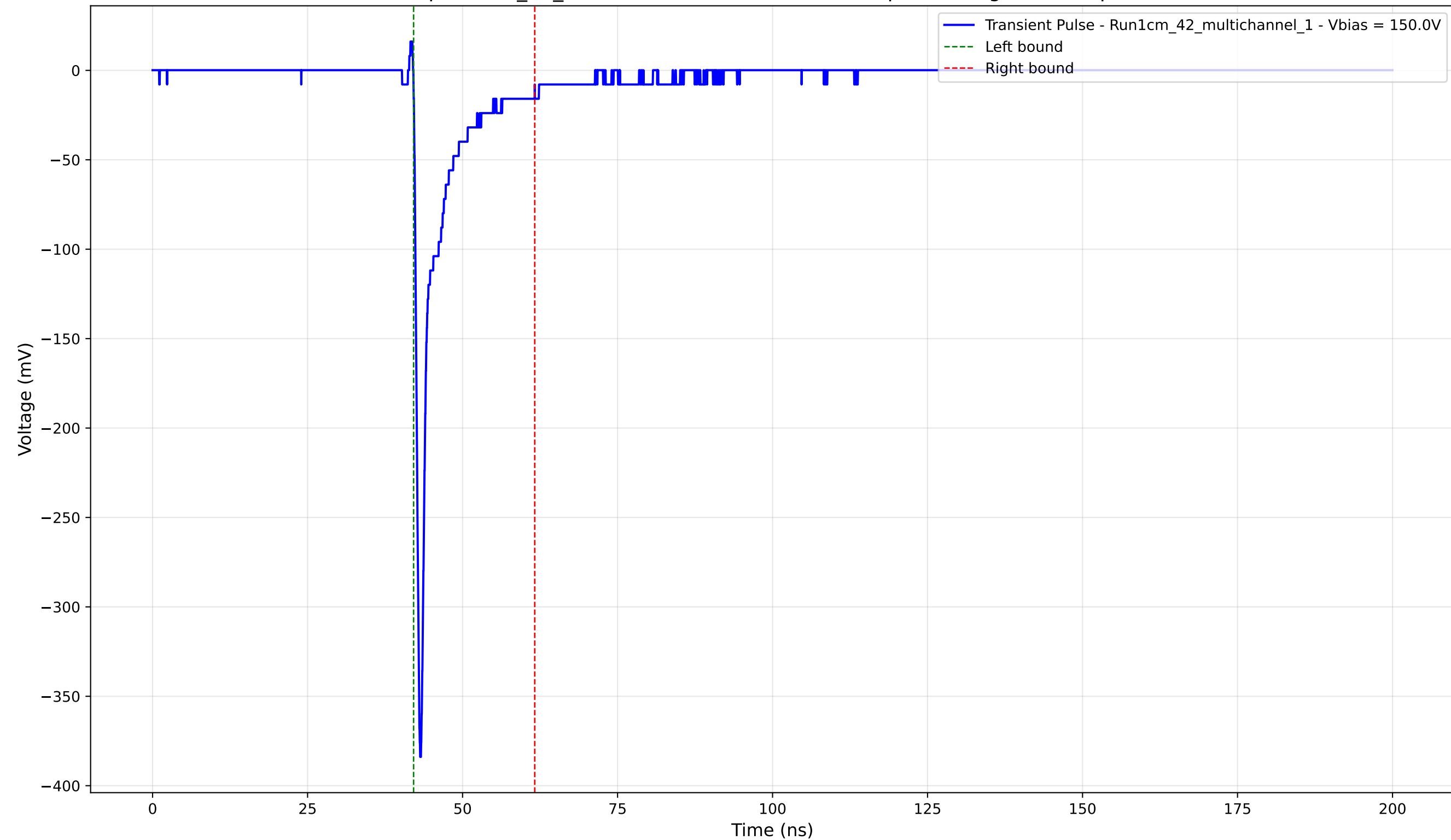
Transient Pulse - Sample: 1cm_42_multichannel - Position: 2240.0 \mu\text{m} - Charge: -24.40 pC - Rise Time: 0.75 ns
