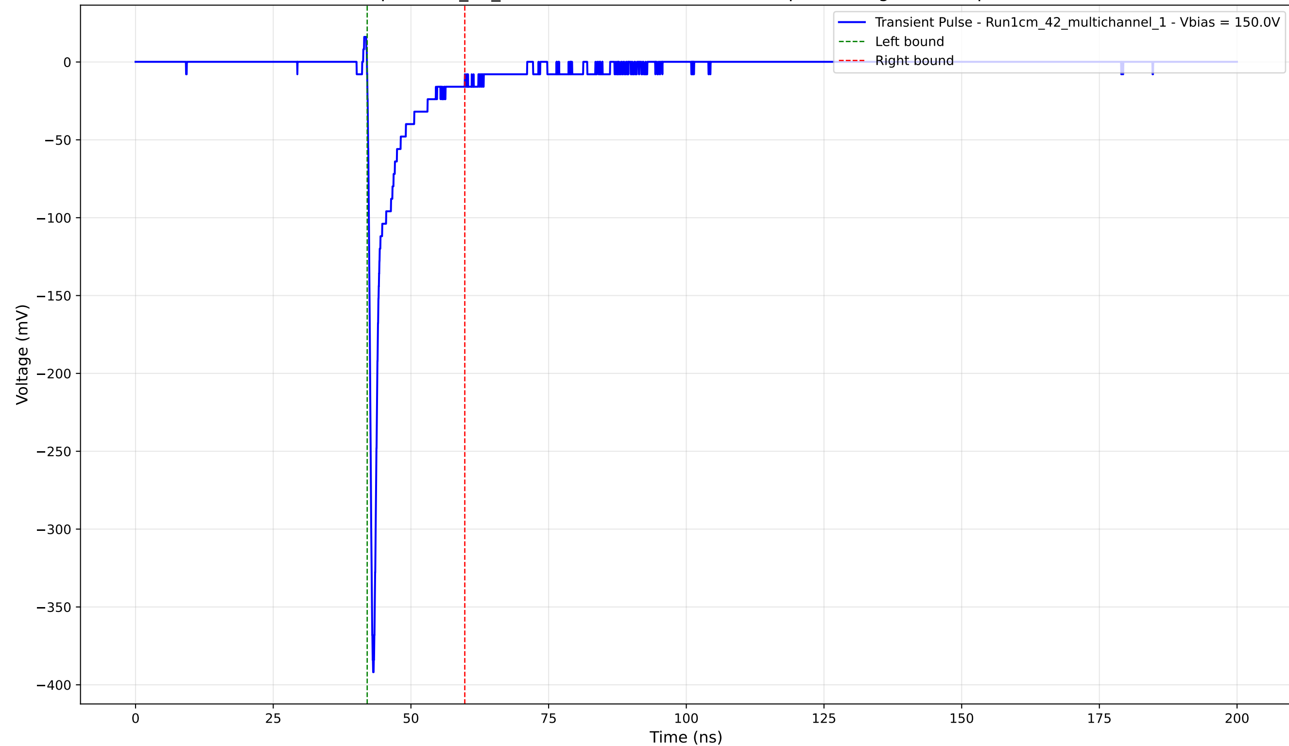
Transient Pulse - Sample: 1cm_42_multichannel - Position: 2505.0 \mu\text{m} - Charge: -23.30 pC - Rise Time: 0.74 ns
