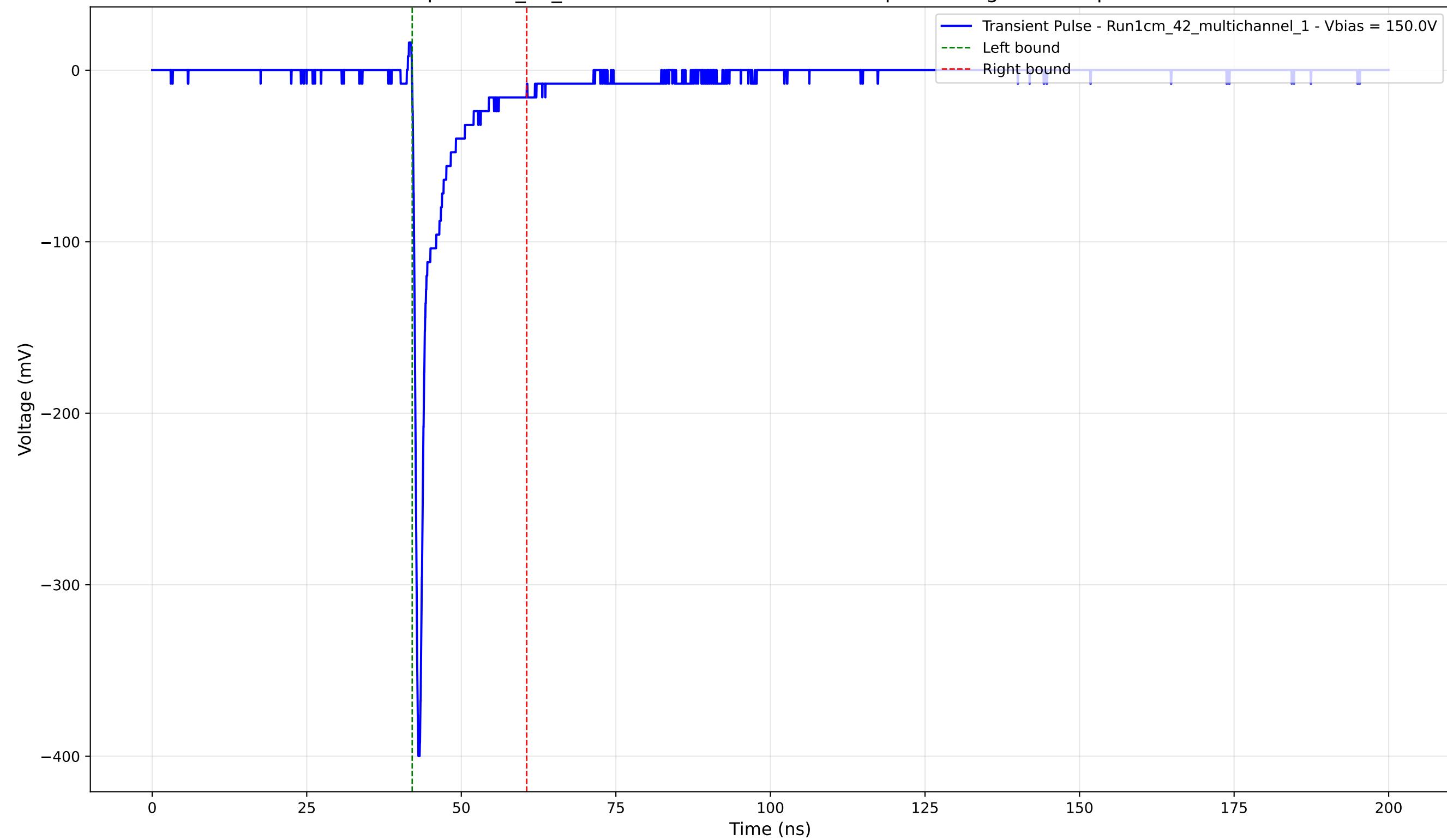
Transient Pulse - Sample: 1cm_42_multichannel - Position: 2290.0 \mu\text{m} - Charge: -23.85 pC - Rise Time: 0.72 ns
