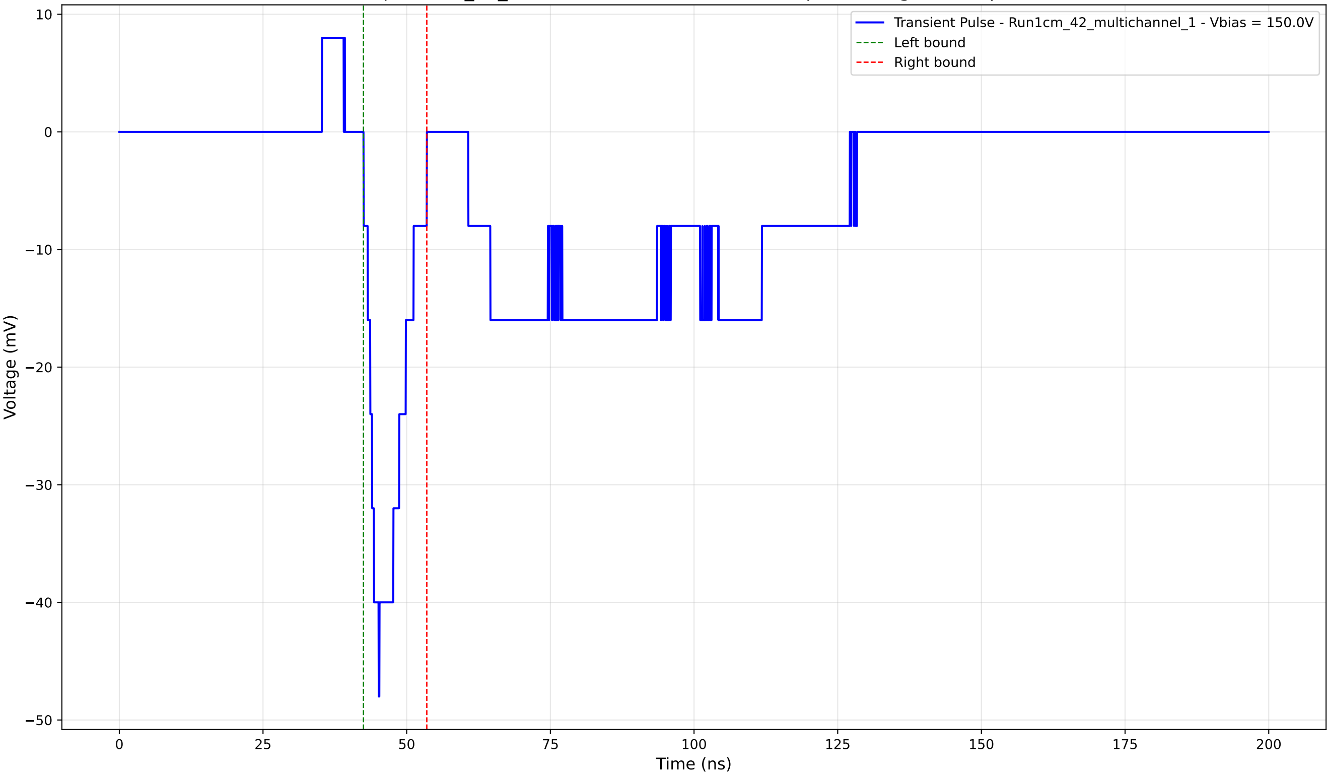
Transient Pulse - Sample: 1cm_42_multichannel - Position: 4560.0 \mu\text{m} - Charge: -5.34 pC - Rise Time: 2.63 ns
