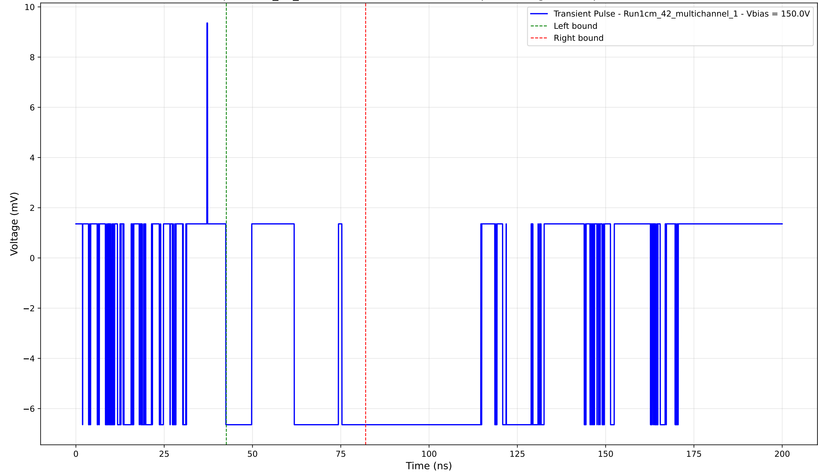
Transient Pulse - Sample: 1cm_42_multichannel - Position: 4435.0 \mu\text{m} - Charge: -3.16 pC - Rise Time: 0.00 ns (N/A)
