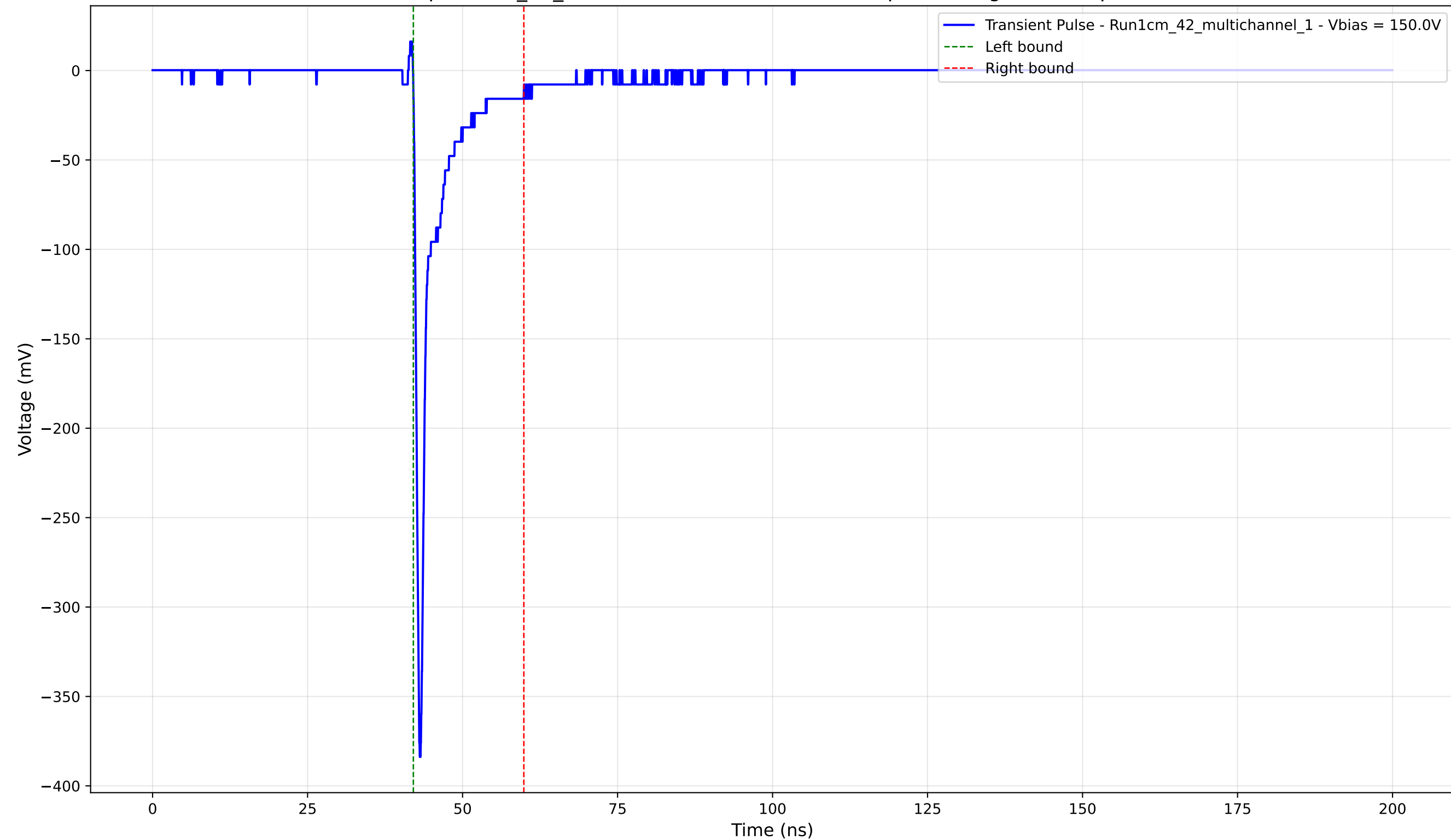
Transient Pulse - Sample: 1cm_42_multichannel - Position: 2465.0 \mu\text{m} - Charge: -21.94 pC - Rise Time: 0.75 ns
