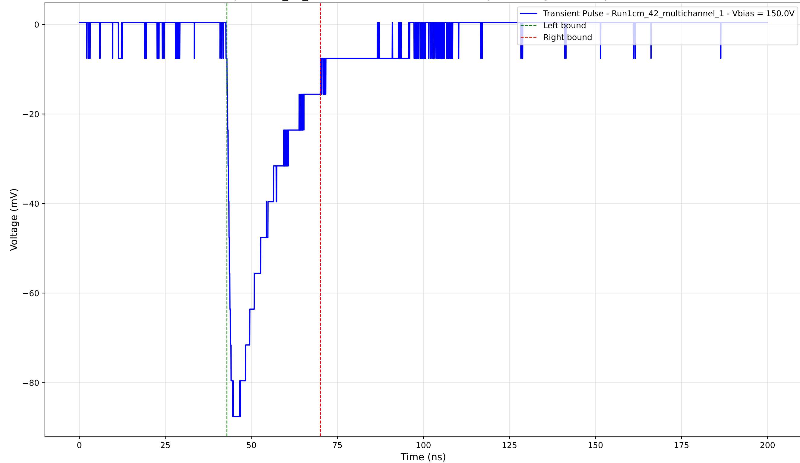
Transient Pulse - Sample: 1cm_42_multichannel - Position: 1020.0 \mu\text{m} - Charge: -23.08 pC - Rise Time: 1.20 ns
