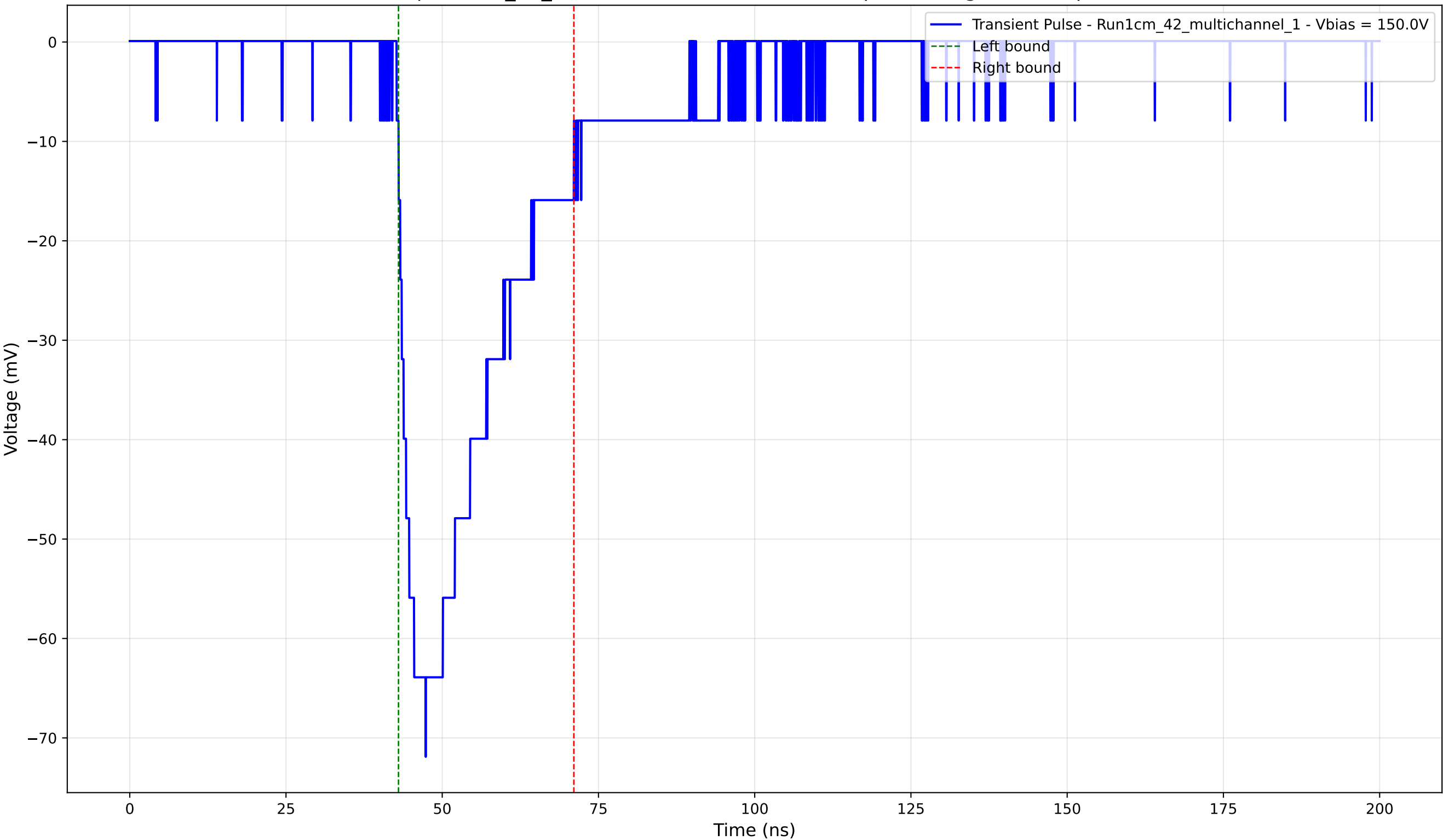
Transient Pulse - Sample: 1cm_42_multichannel - Position: 245.0 \mu\text{m} - Charge: -20.63 pC - Rise Time: 4.64 ns
