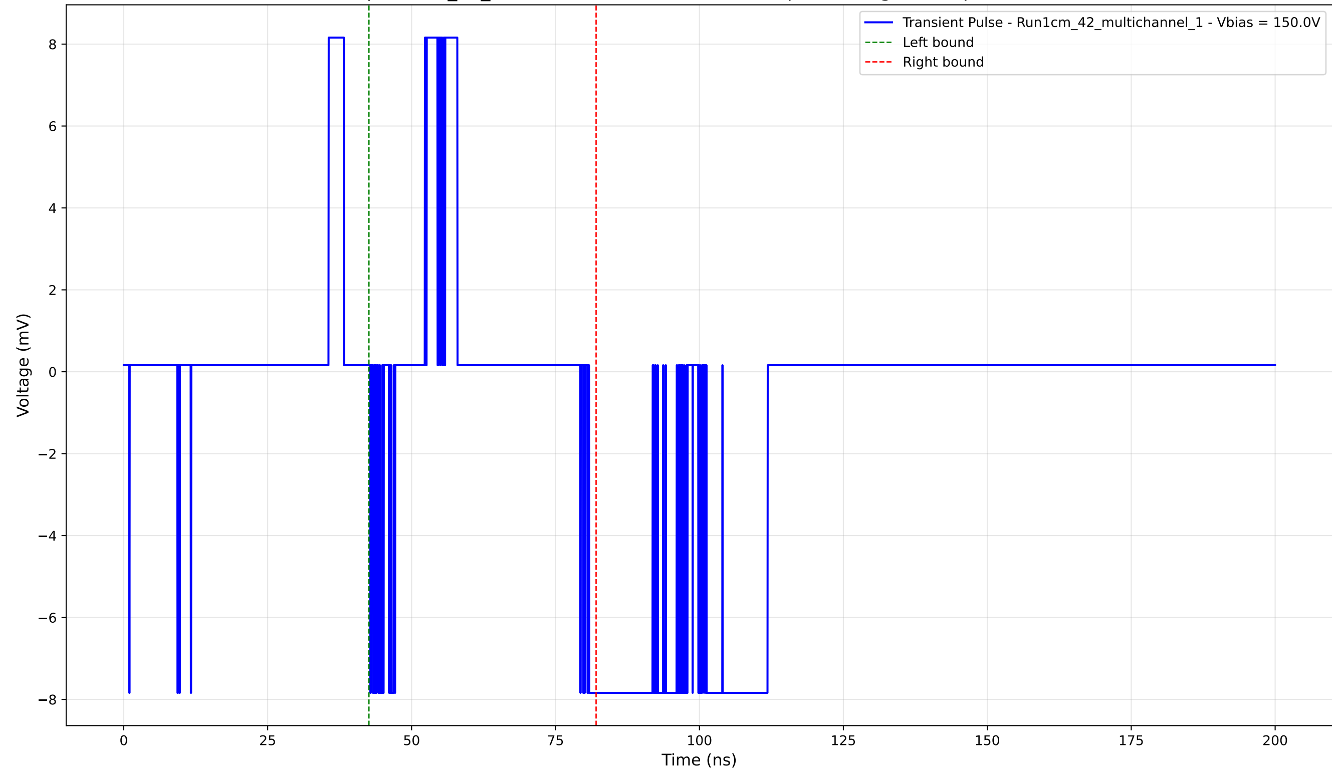
Transient Pulse - Sample: 1cm_42_multichannel - Position: 4410.0 \mu\text{m} - Charge: 0.40 pC - Rise Time: 0.00 ns (N/A)
