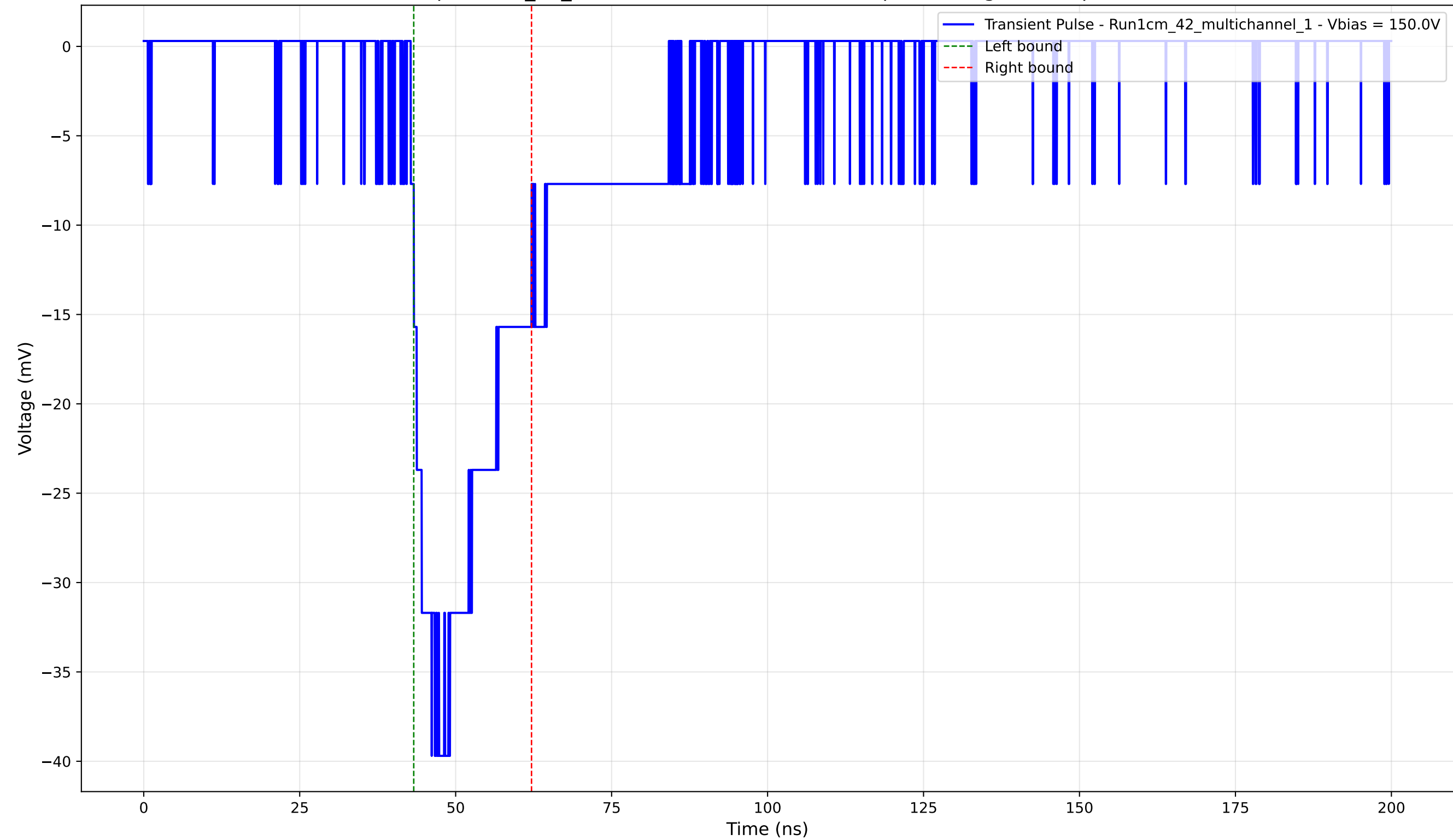
Transient Pulse - Sample: 1cm_42_multichannel - Position: 310.0 \mu\text{m} - Charge: -9.58 pC - Rise Time: 3.35 ns
