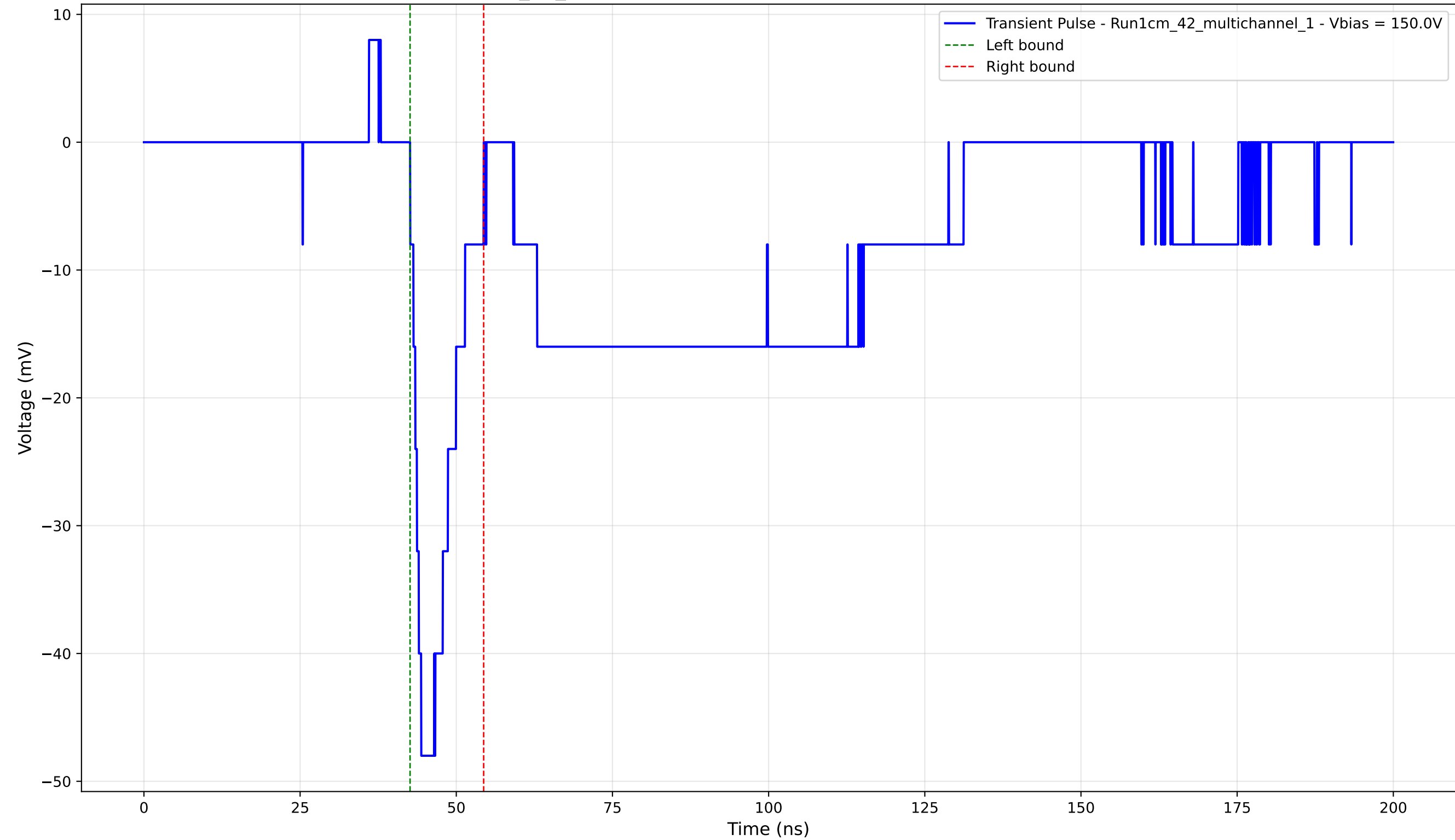
Transient Pulse - Sample: 1cm_42_multichannel - Position: 4105.0 \mu\text{m} - Charge: -6.01 pC - Rise Time: 1.77 ns
