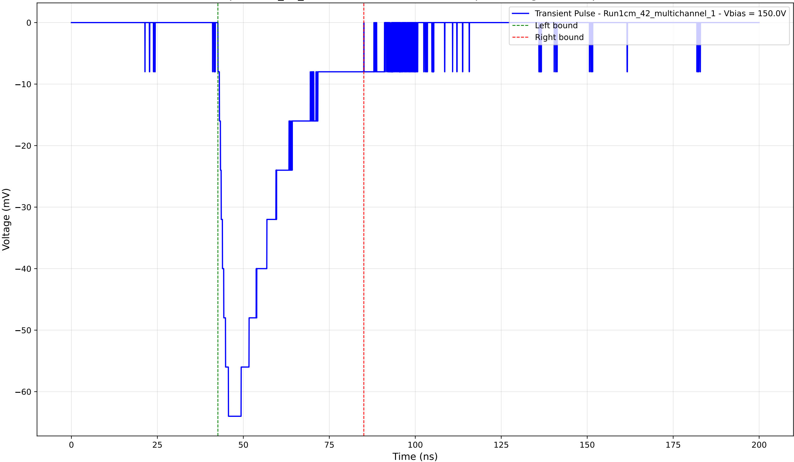
Transient Pulse - Sample: 1cm_42_multichannel - Position: 270.0 \mu\text{m} - Charge: -22.38 pC - Rise Time: 3.04 ns
