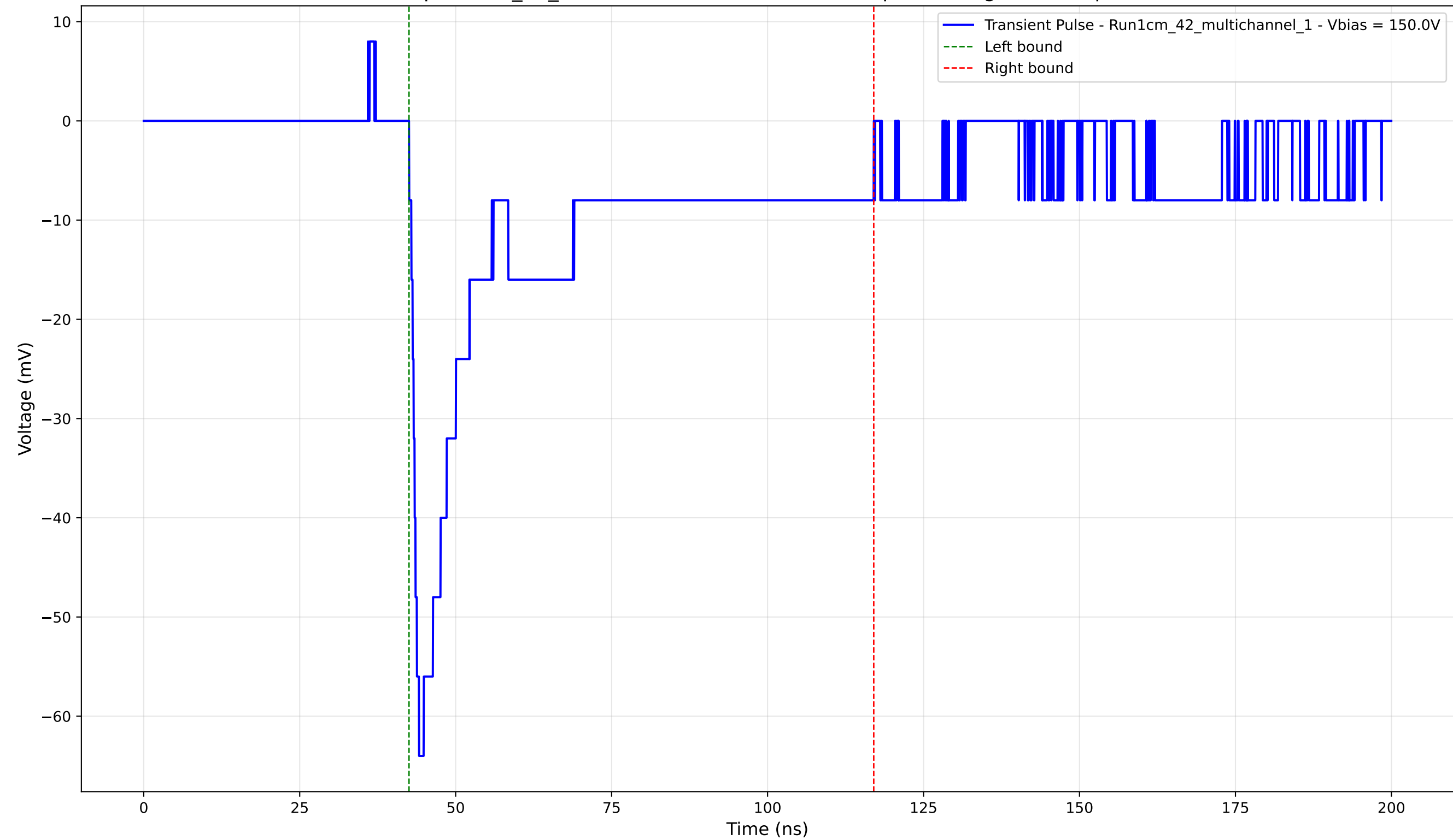
Transient Pulse - Sample: 1cm_42_multichannel - Position: 3720.0 \mu\text{m} - Charge: -20.23 pC - Rise Time: 1.58 ns
