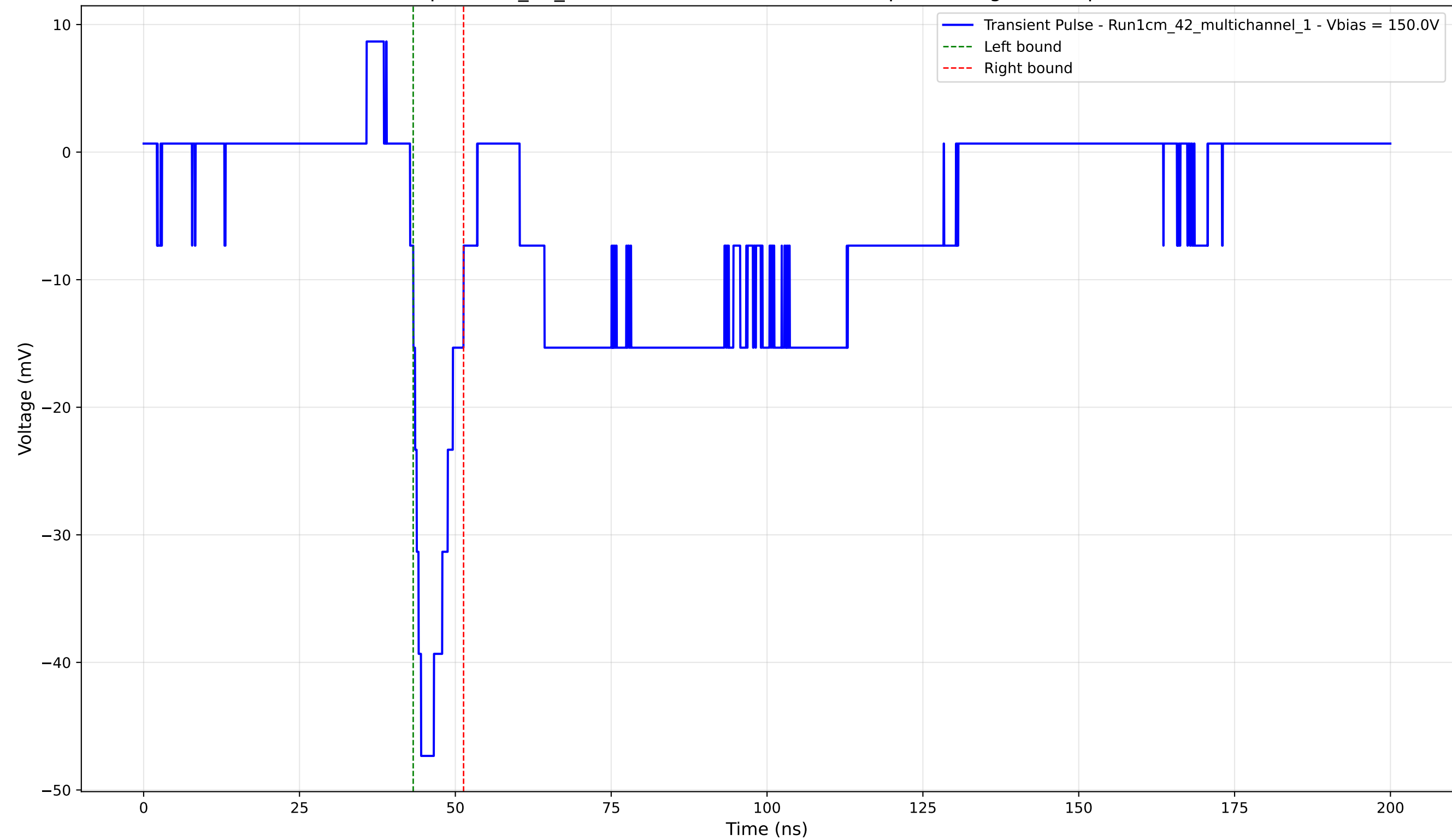
Transient Pulse - Sample: 1cm_42_multichannel - Position: 4230.0 \mu\text{m} - Charge: -5.18 pC - Rise Time: 1.77 ns
