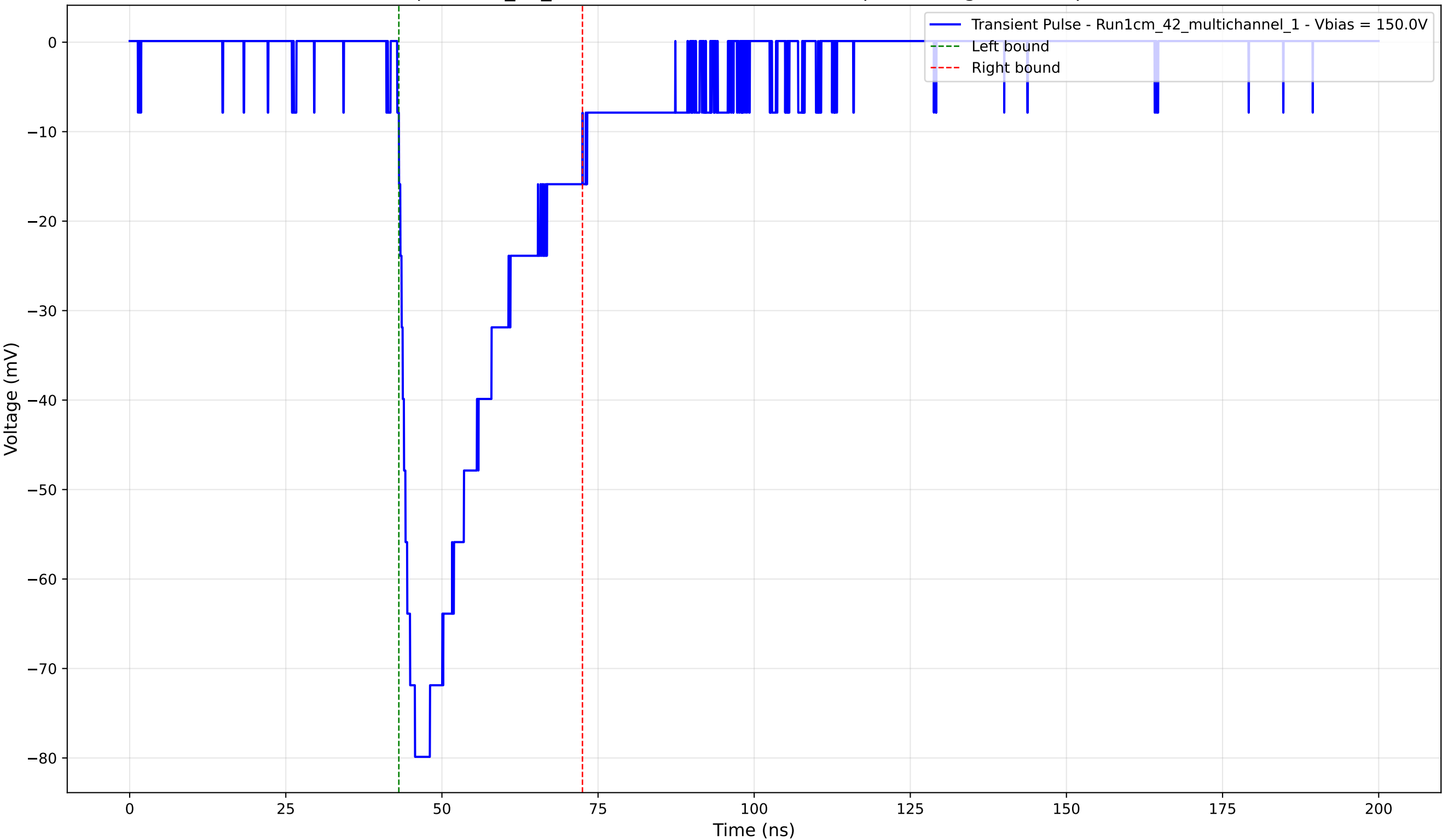
Transient Pulse - Sample: 1cm_42_multichannel - Position: 540.0 \mu\text{m} - Charge: -23.85 pC - Rise Time: 2.58 ns
