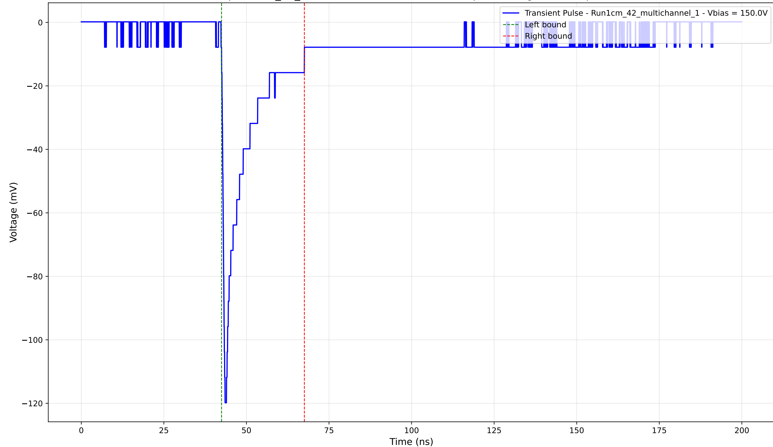
Transient Pulse - Sample: 1cm_42_multichannel - Position: 3180.0 \mu\text{m} - Charge: -17.39 pC - Rise Time: 0.93 ns
