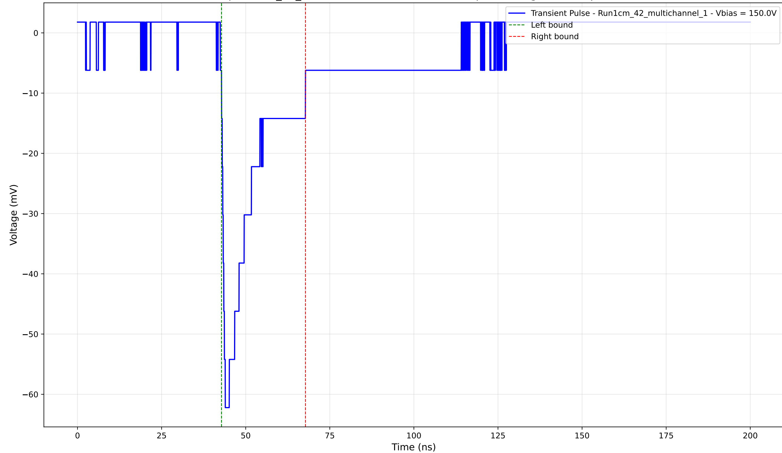
Transient Pulse - Sample: 1cm_42_multichannel - Position: 3645.0 \mu\text{m} - Charge: -12.68 pC - Rise Time: 1.12 ns
