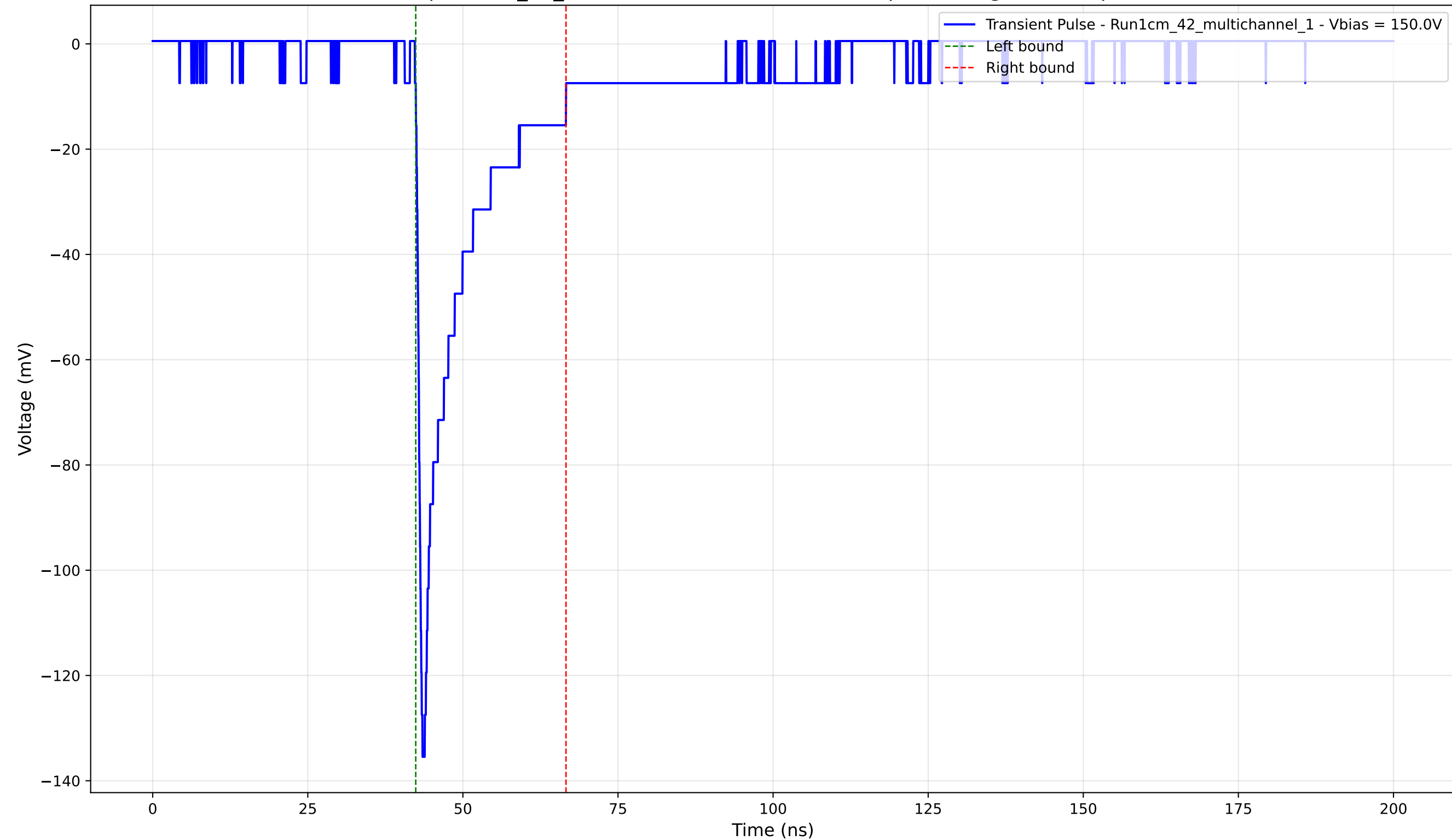
Transient Pulse - Sample: 1cm_42_multichannel - Position: 3095.0 \mu\text{m} - Charge: -18.78 pC - Rise Time: 0.94 ns
