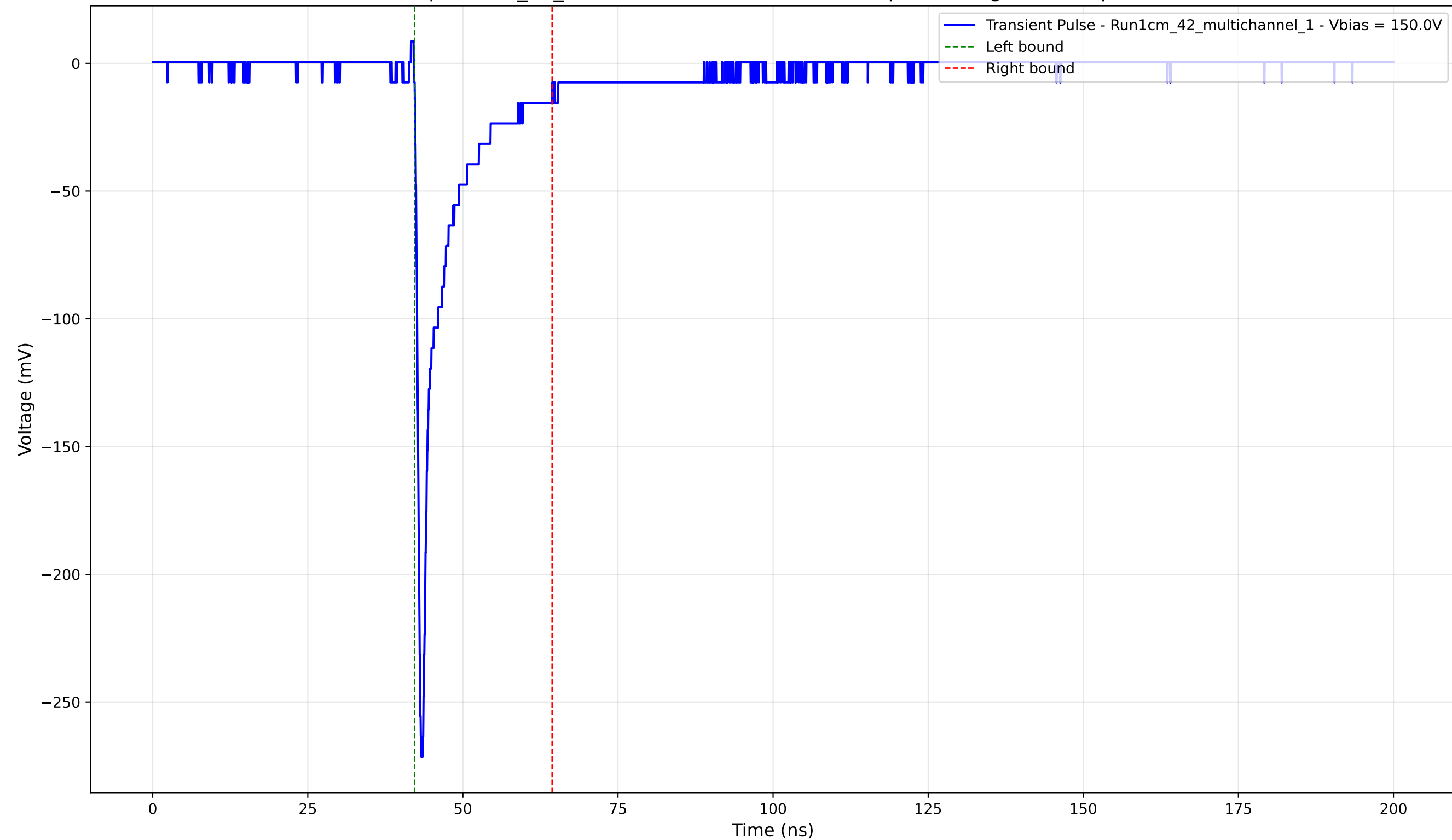
Transient Pulse - Sample: 1cm_42_multichannel - Position: 2025.0 \mu\text{m} - Charge: -24.04 pC - Rise Time: 0.77 ns
