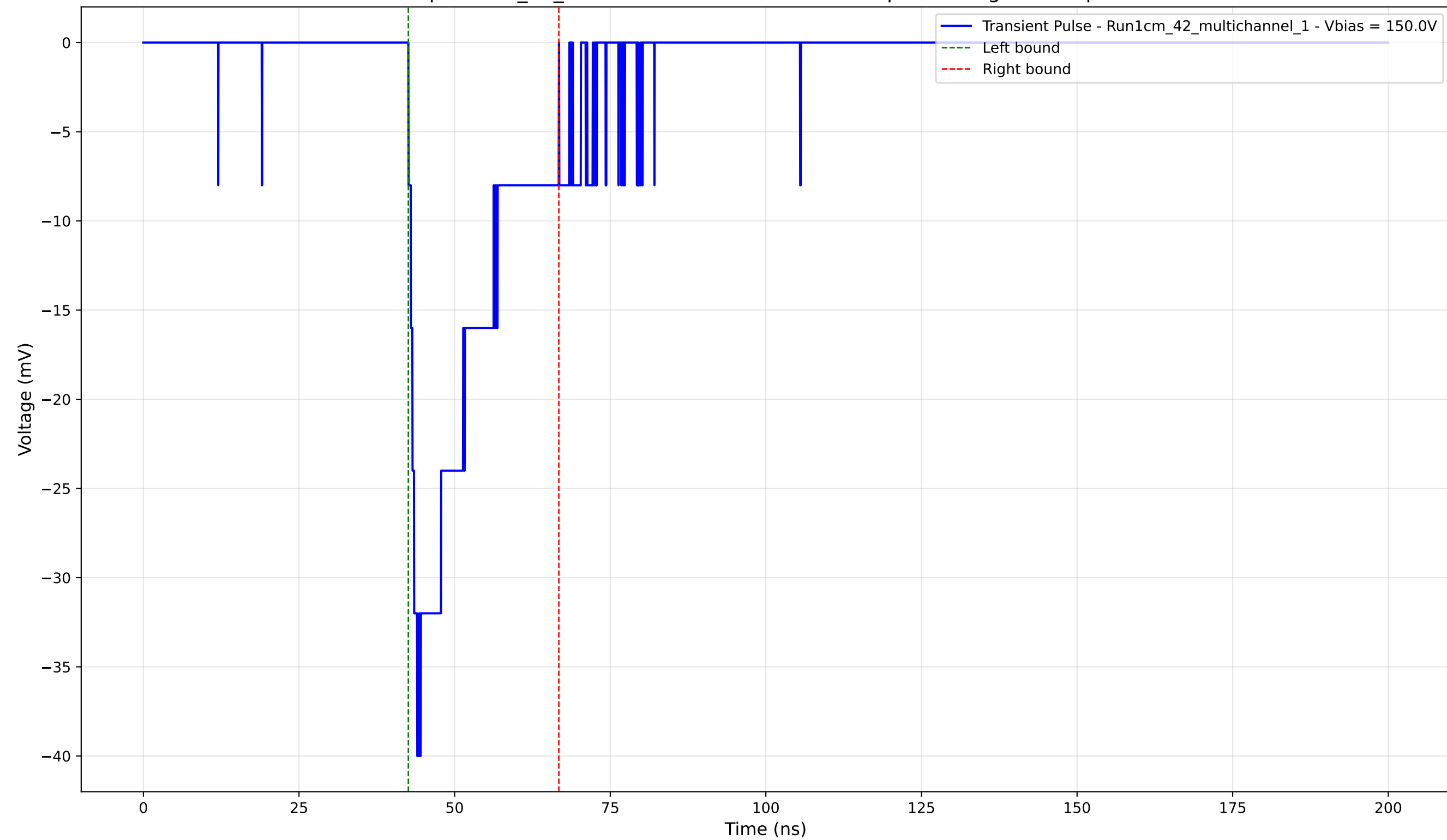
Transient Pulse - Sample: 1cm_42_multichannel - Position: 1330.0 \mu\text{m} - Charge: -8.16 pC - Rise Time: 1.41 ns
