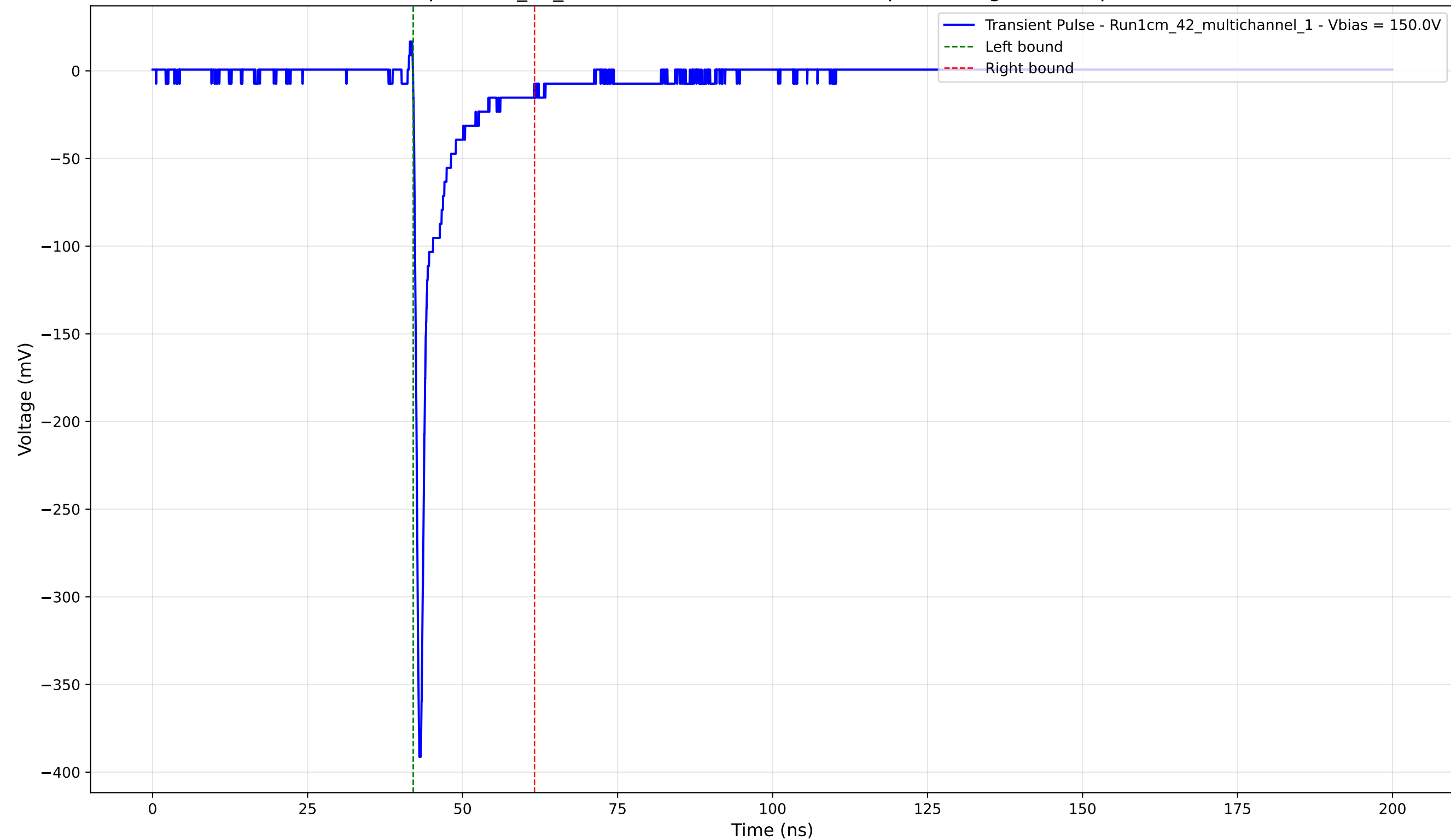
Transient Pulse - Sample: 1cm_42_multichannel - Position: 2475.0 \mu\text{m} - Charge: -23.46 pC - Rise Time: 0.74 ns
