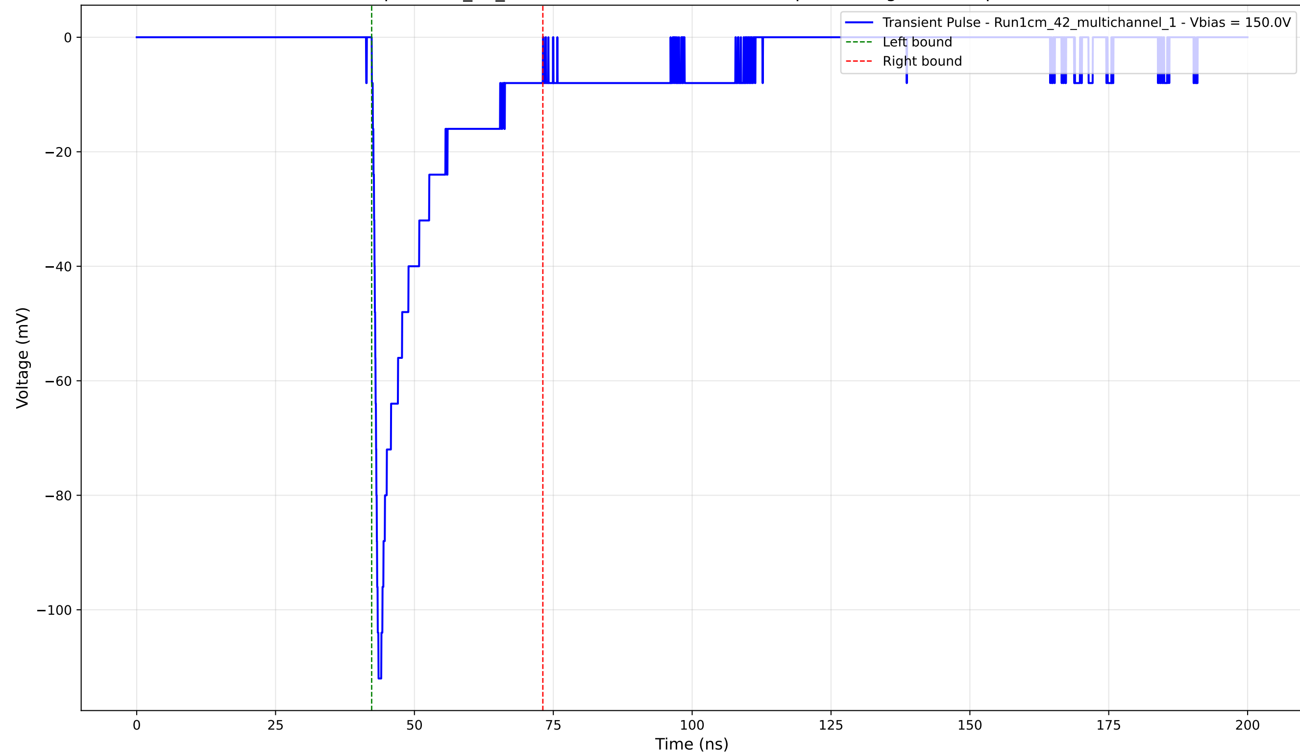
Transient Pulse - Sample: 1cm_42_multichannel - Position: 3210.0 \mu\text{m} - Charge: -17.38 pC - Rise Time: 0.89 ns
