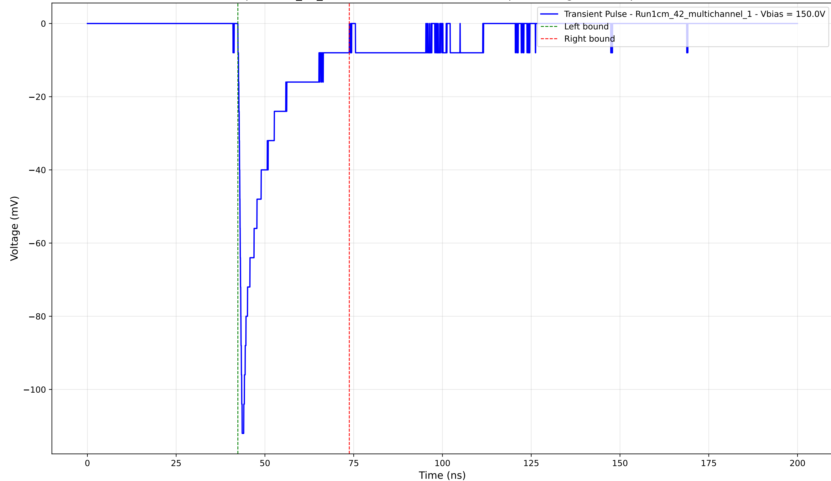
Transient Pulse - Sample: 1cm_42_multichannel - Position: 3240.0 \mu\text{m} - Charge: -17.39 pC - Rise Time: 0.91 ns
