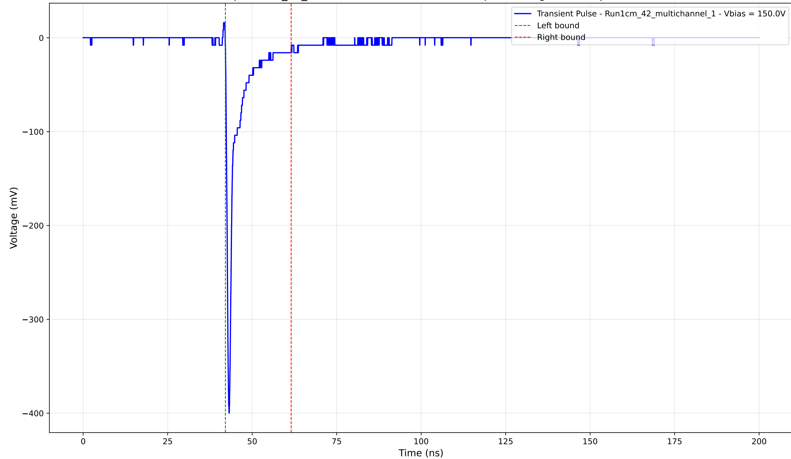
Transient Pulse - Sample: 1cm_42_multichannel - Position: 2490.0 \mu\text{m} - Charge: -23.98 pC - Rise Time: 0.74 ns
