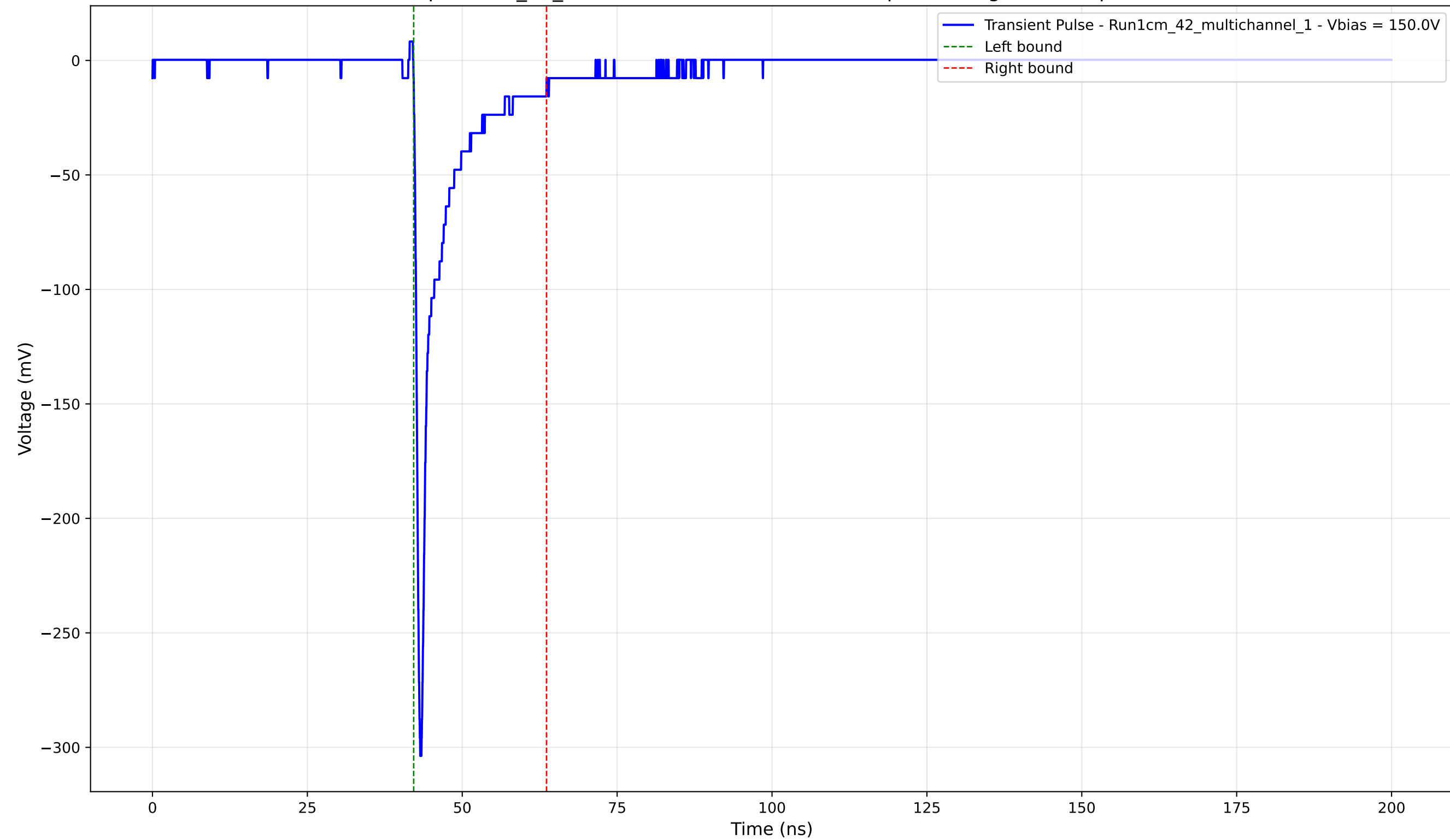
Transient Pulse - Sample: 1cm_42_multichannel - Position: 2660.0 \mu\text{m} - Charge: -23.32 pC - Rise Time: 0.78 ns
