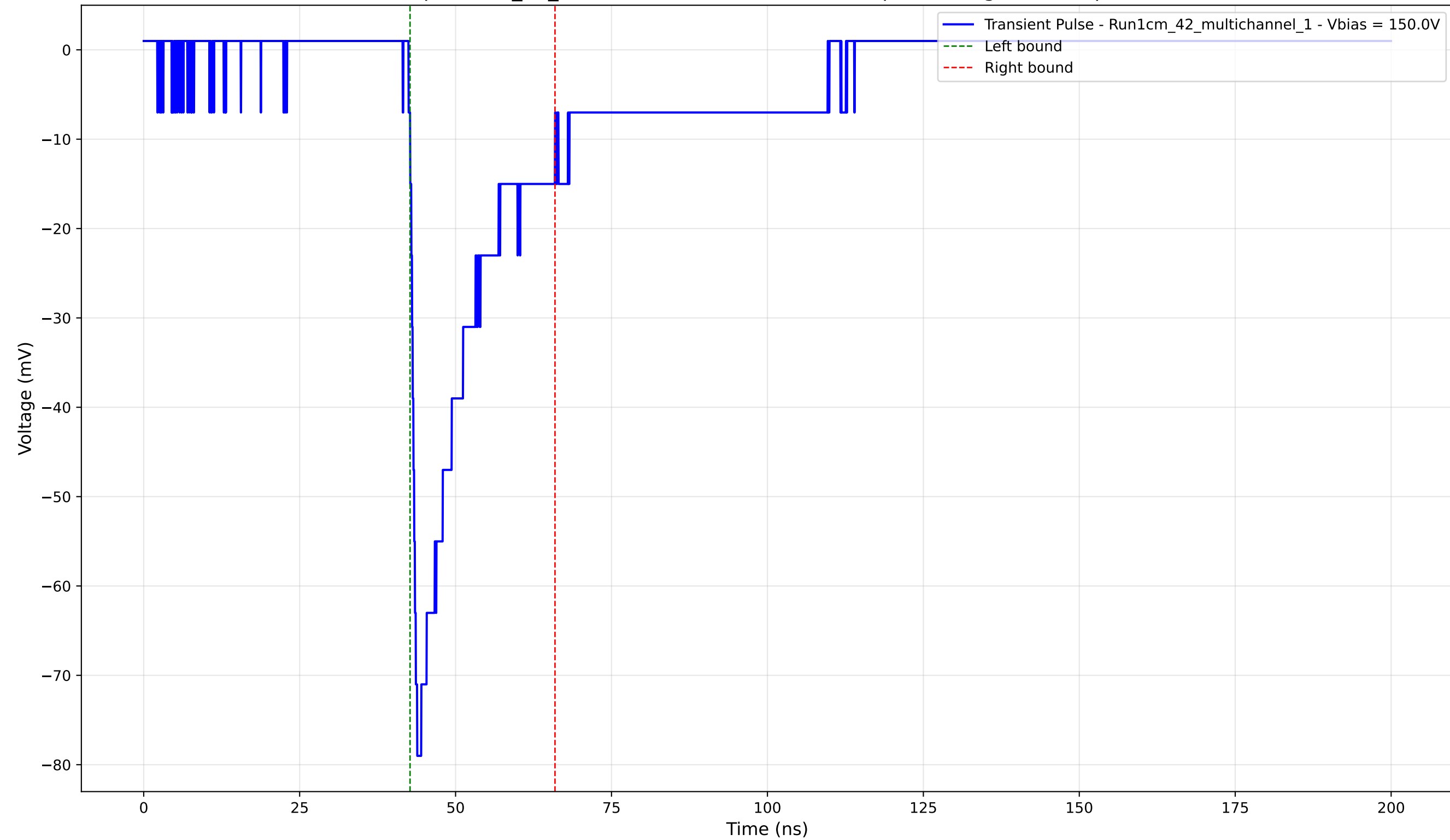
Transient Pulse - Sample: 1cm_42_multichannel - Position: 3525.0 \mu\text{m} - Charge: -14.84 pC - Rise Time: 1.14 ns
