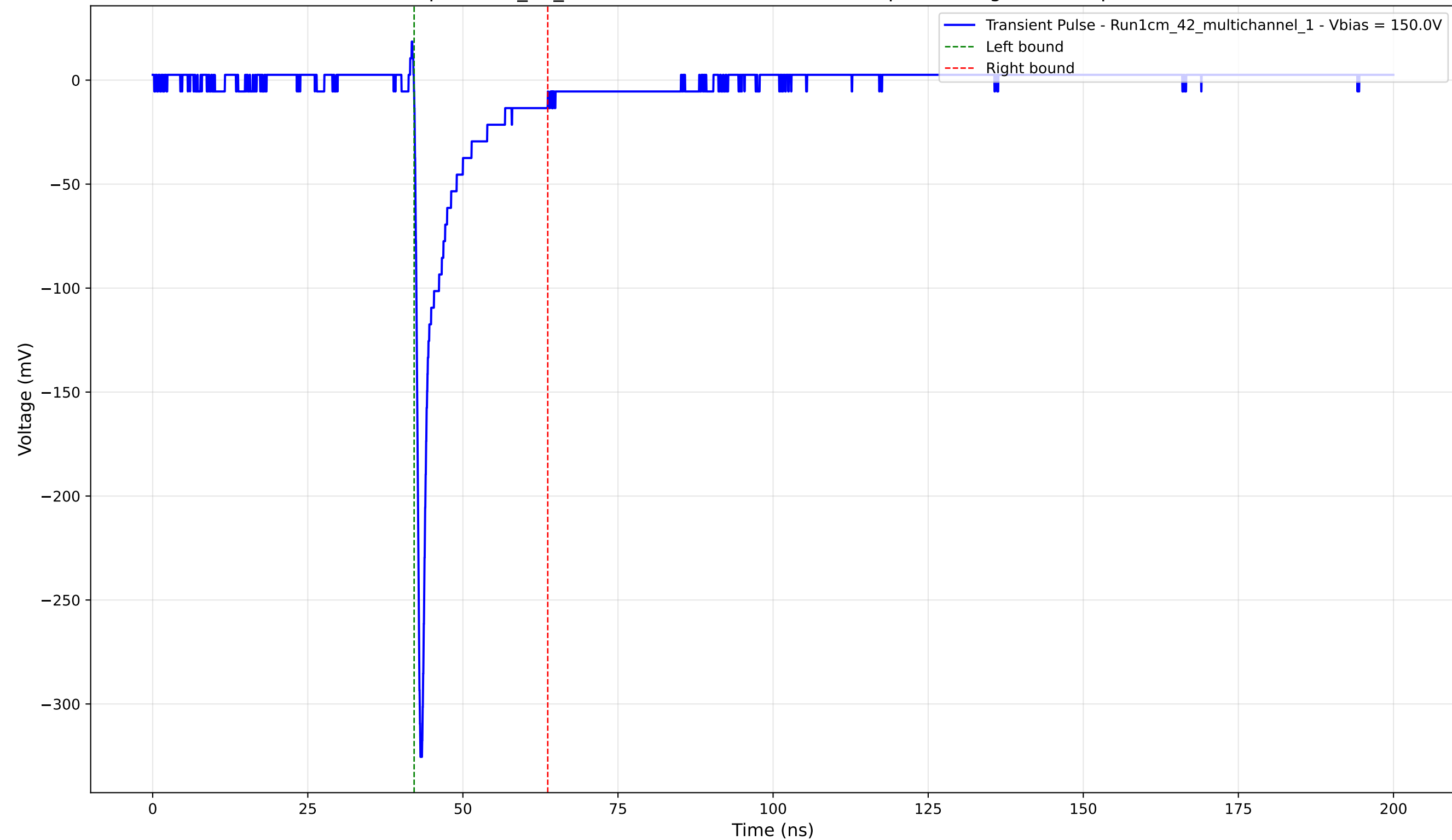
Transient Pulse - Sample: 1cm_42_multichannel - Position: 2145.0 \mu\text{m} - Charge: -23.52 pC - Rise Time: 0.73 ns
