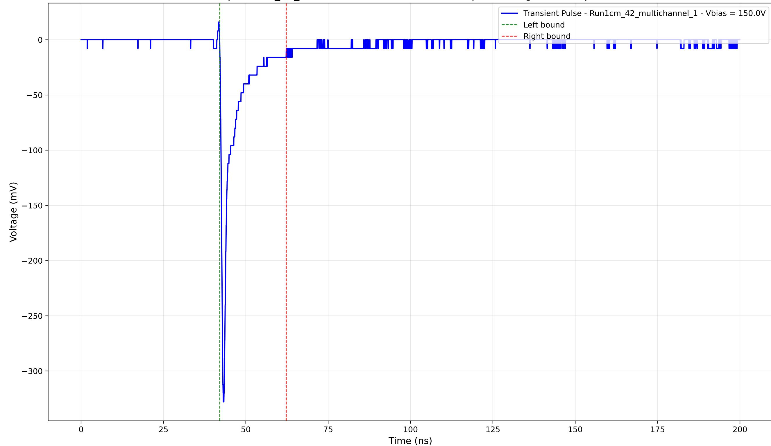
Transient Pulse - Sample: 1cm_42_multichannel - Position: 2605.0 \mu\text{m} - Charge: -23.13 pC - Rise Time: 0.74 ns
