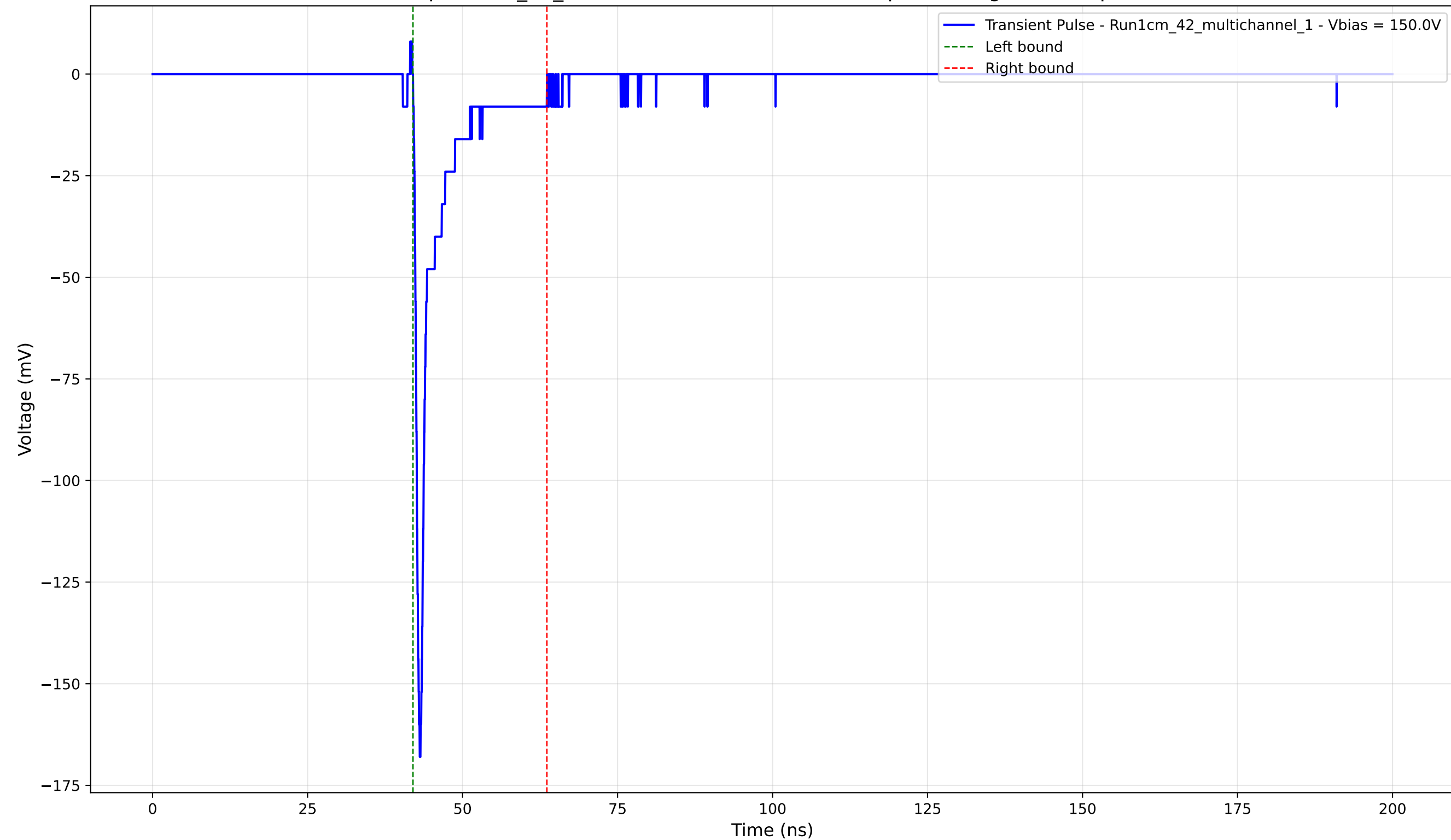
Transient Pulse - Sample: 1cm_42_multichannel - Position: 2435.0 \mu\text{m} - Charge: -10.44 pC - Rise Time: 0.72 ns
