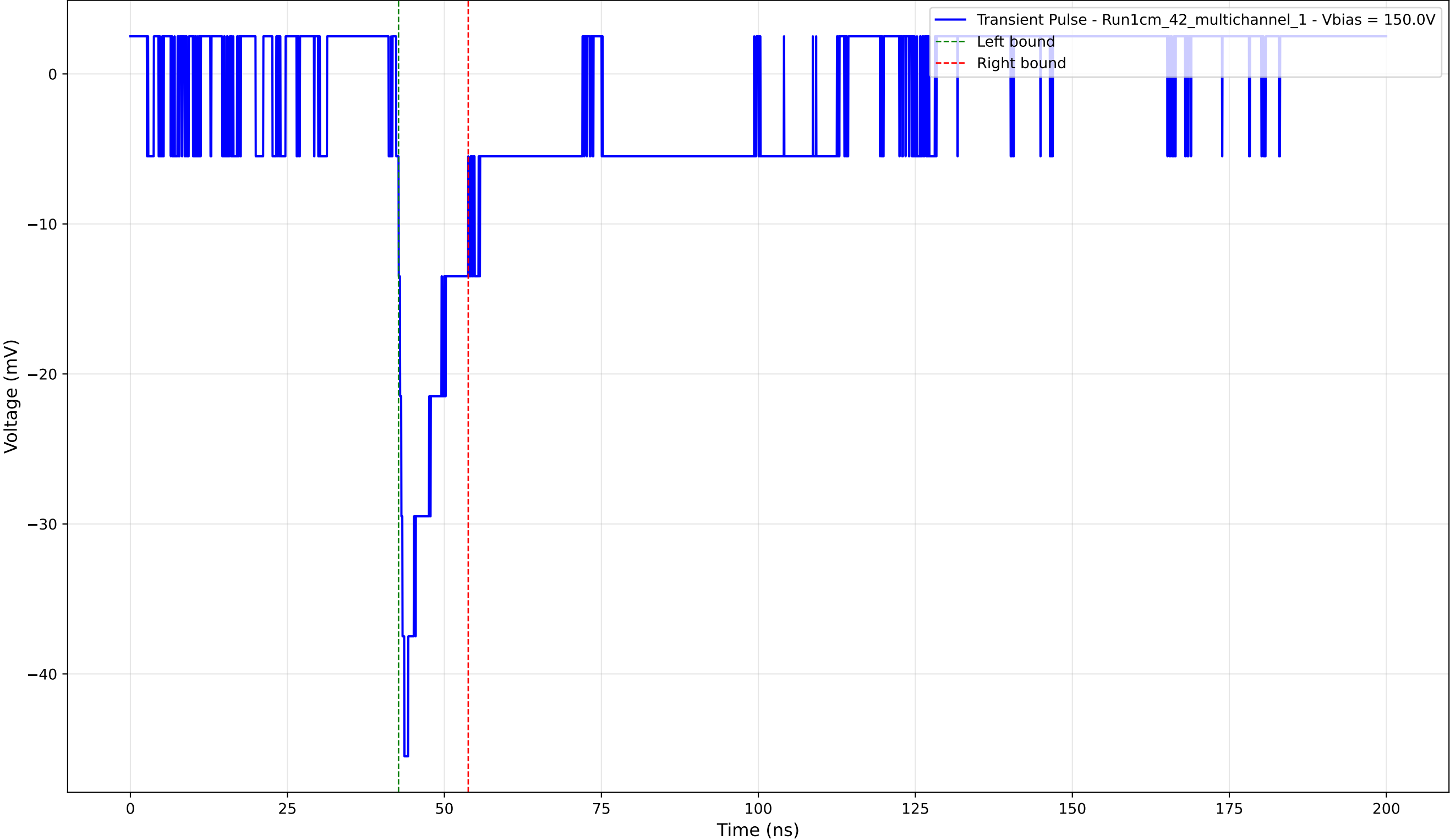
Transient Pulse - Sample: 1cm_42_multichannel - Position: 3350.0 \mu\text{m} - Charge: -5.23 pC - Rise Time: 1.31 ns
