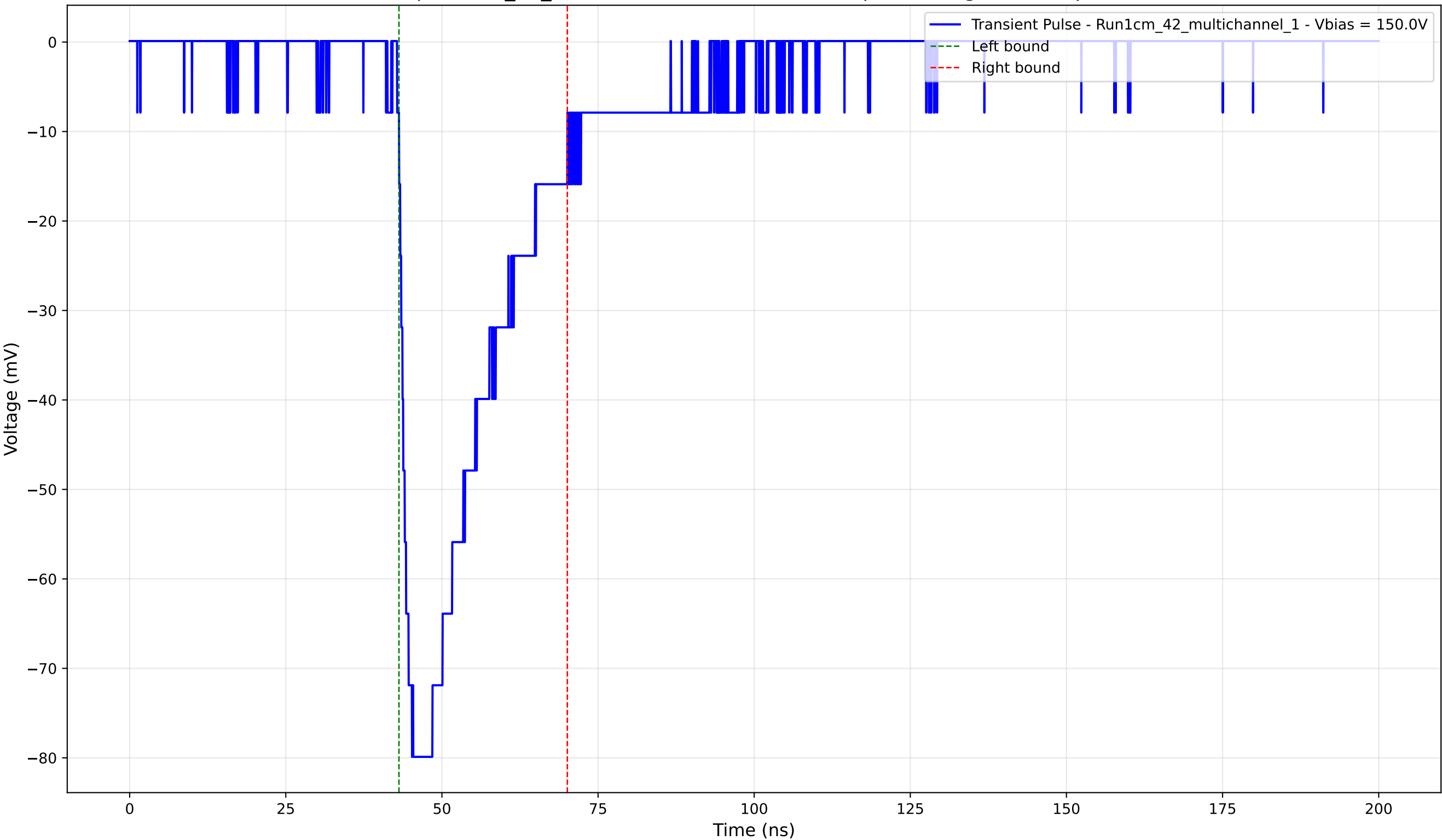
Transient Pulse - Sample: 1cm_42_multichannel - Position: 650.0 \mu\text{m} - Charge: -23.11 pC - Rise Time: 2.08 ns
