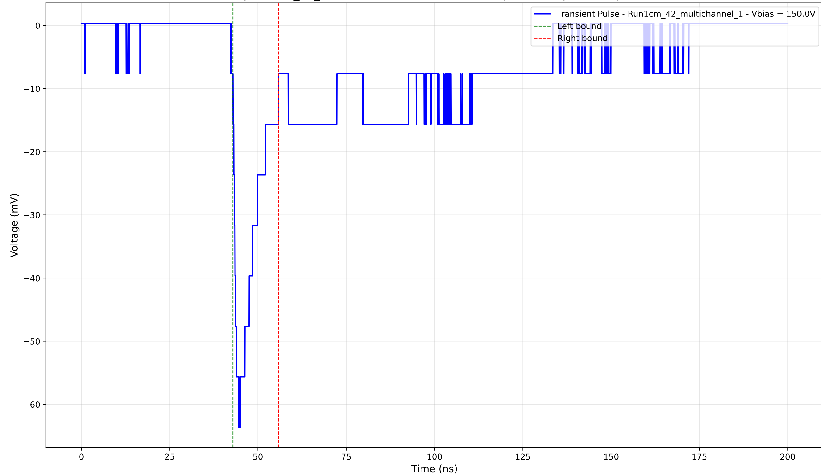
Transient Pulse - Sample: 1cm_42_multichannel - Position: 3795.0 \mu\text{m} - Charge: -8.37 pC - Rise Time: 2.00 ns
