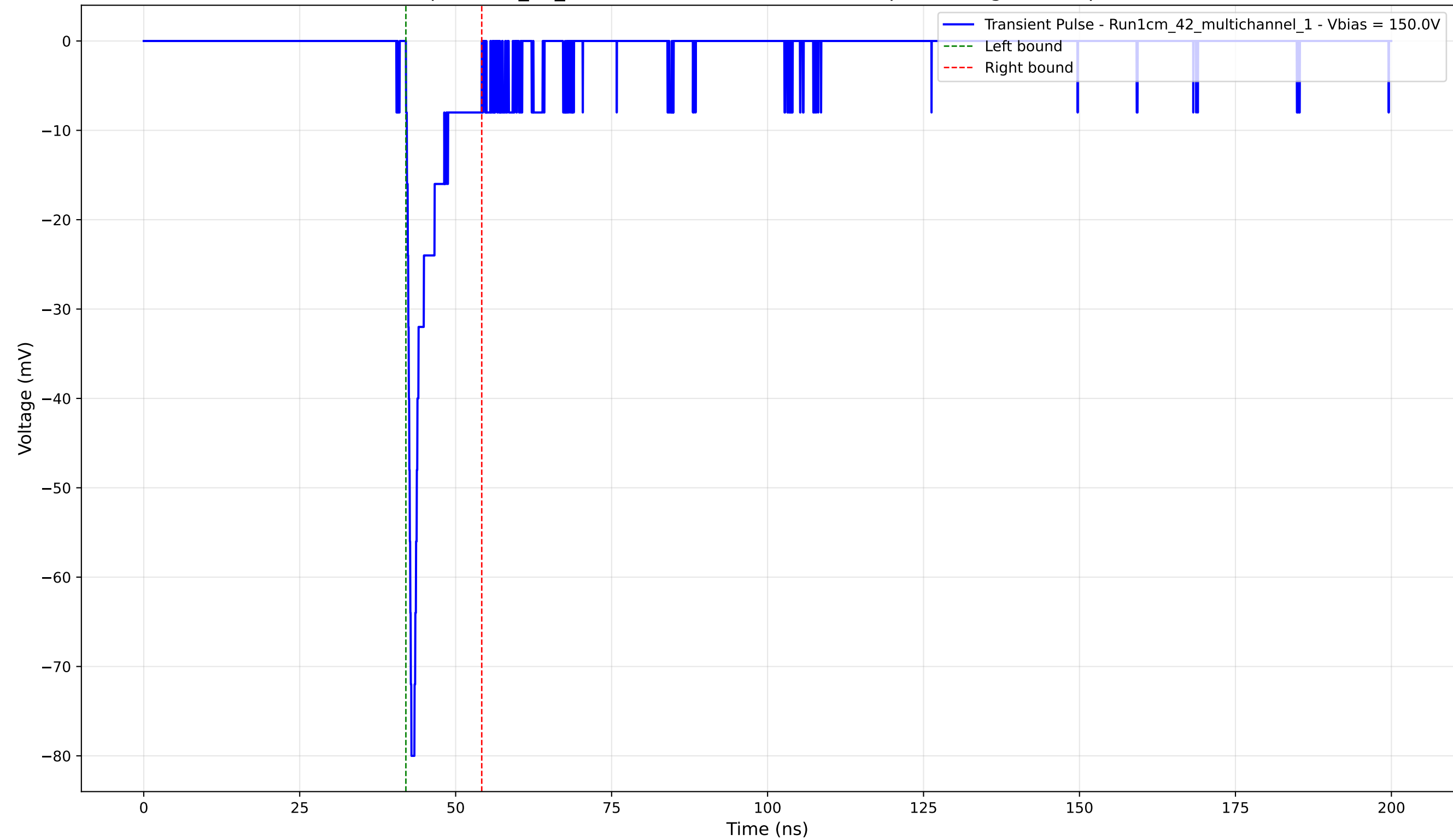
Transient Pulse - Sample: 1cm_42_multichannel - Position: 2425.0 \mu\text{m} - Charge: -5.03 pC - Rise Time: 0.64 ns
