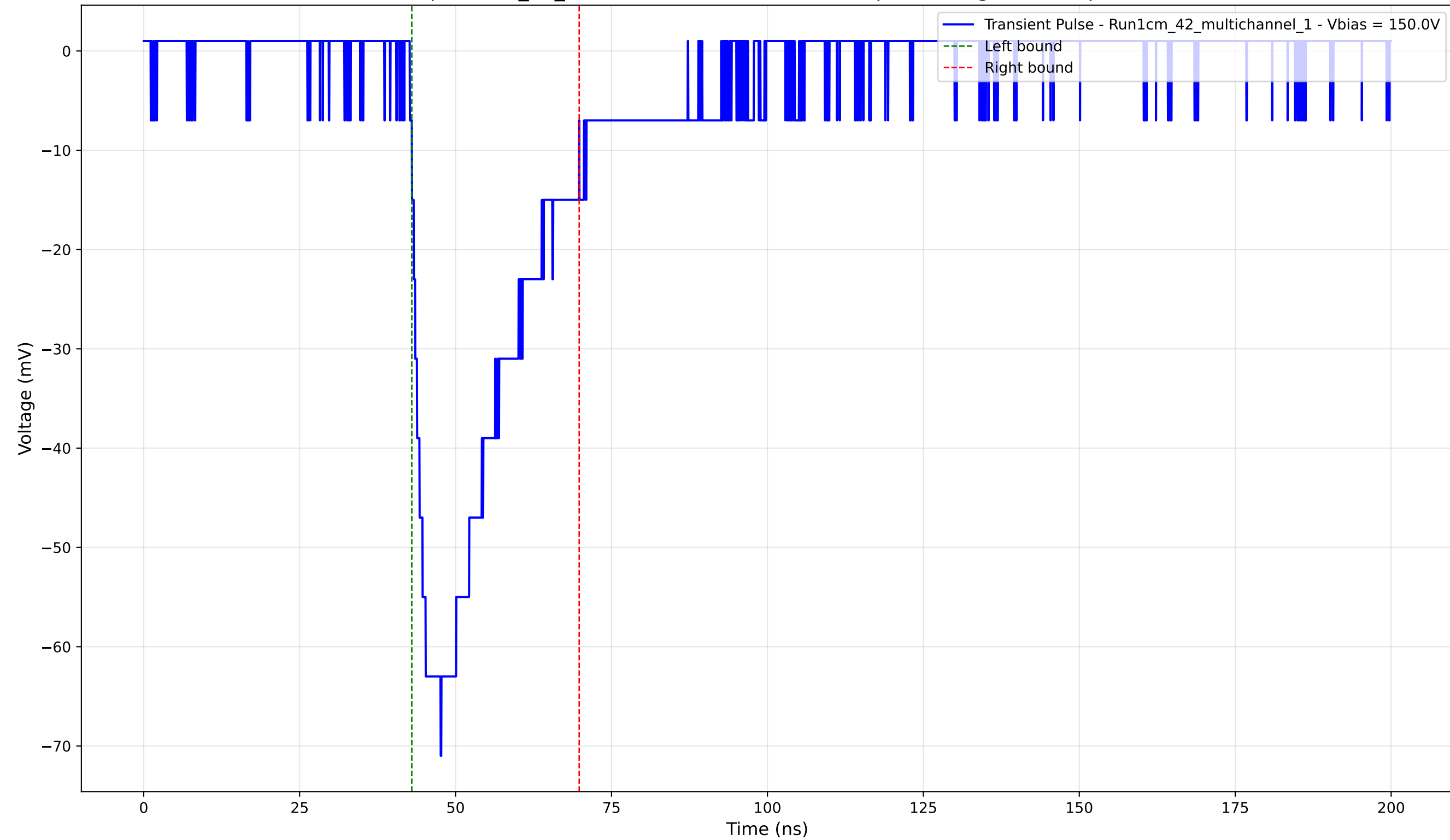
Transient Pulse - Sample: 1cm_42_multichannel - Position: 255.0 \mu\text{m} - Charge: -19.76 pC - Rise Time: 4.62 ns
