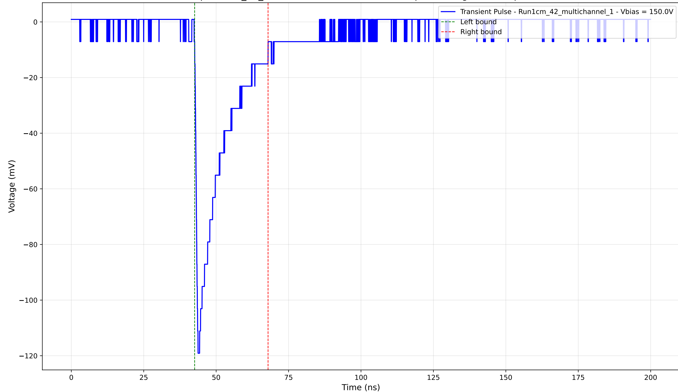
Transient Pulse - Sample: 1cm_42_multichannel - Position: 1460.0 \mu\text{m} - Charge: -22.33 pC - Rise Time: 1.01 ns
