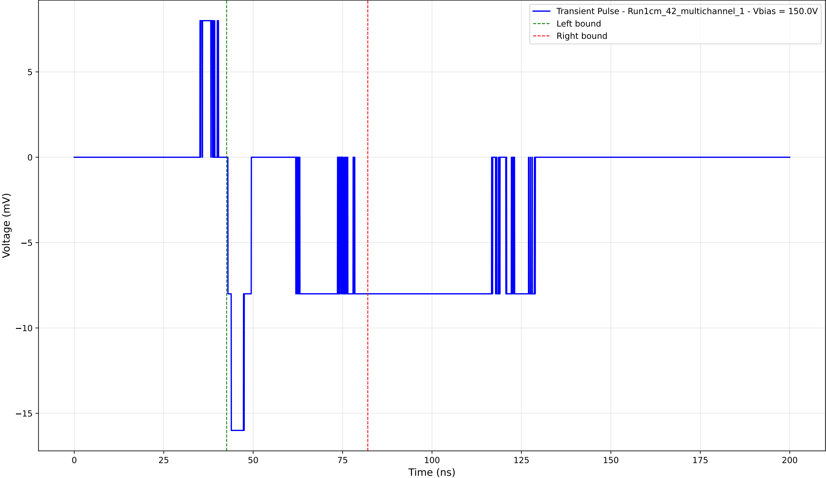
Transient Pulse - Sample: 1cm_42_multichannel - Position: 3945.0 \mu\text{m} - Charge: -4.45 pC - Rise Time: 0.96 ns
