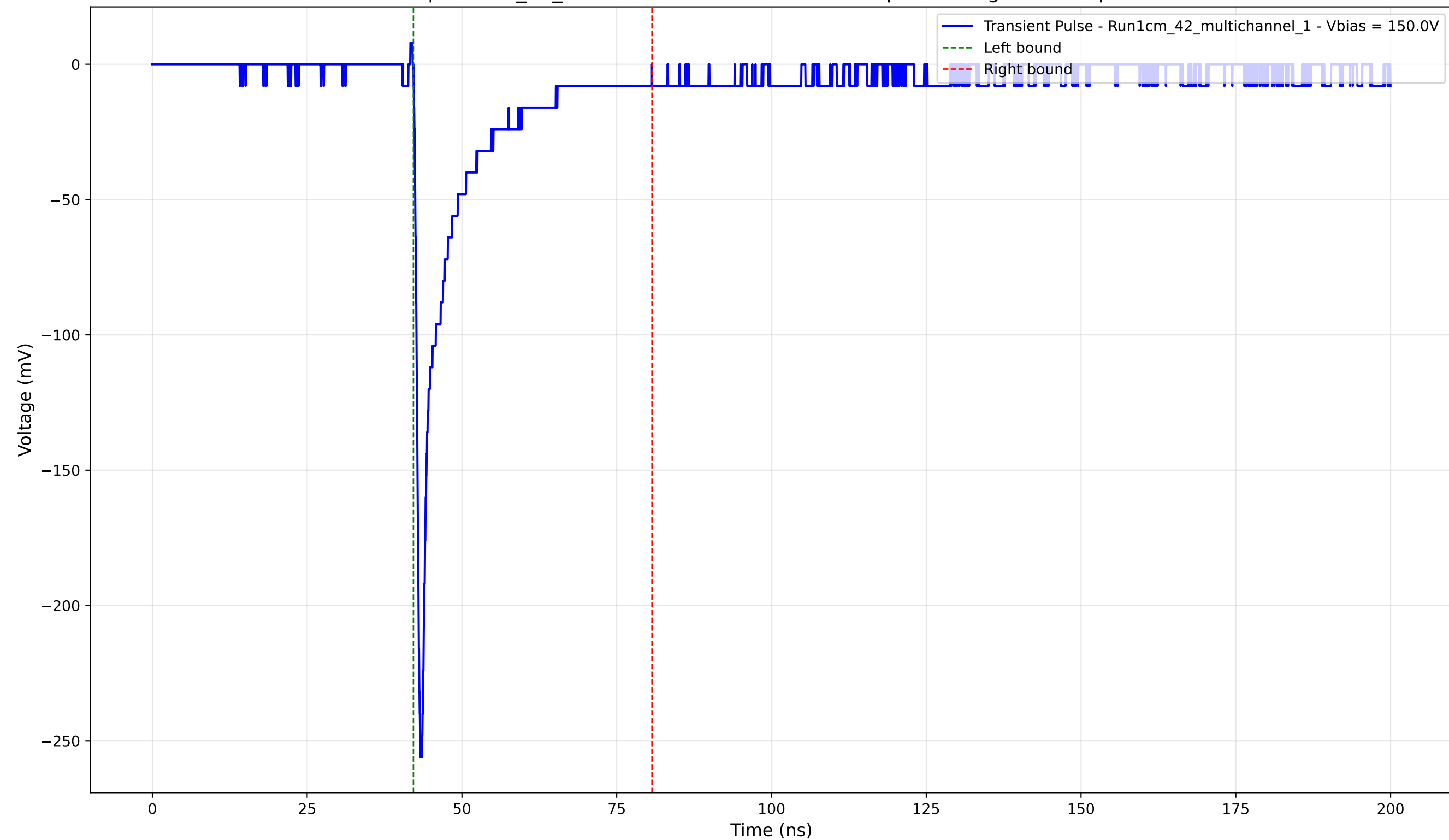
Transient Pulse - Sample: 1cm_42_multichannel - Position: 1995.0 \mu\text{m} - Charge: -26.54 pC - Rise Time: 0.78 ns
