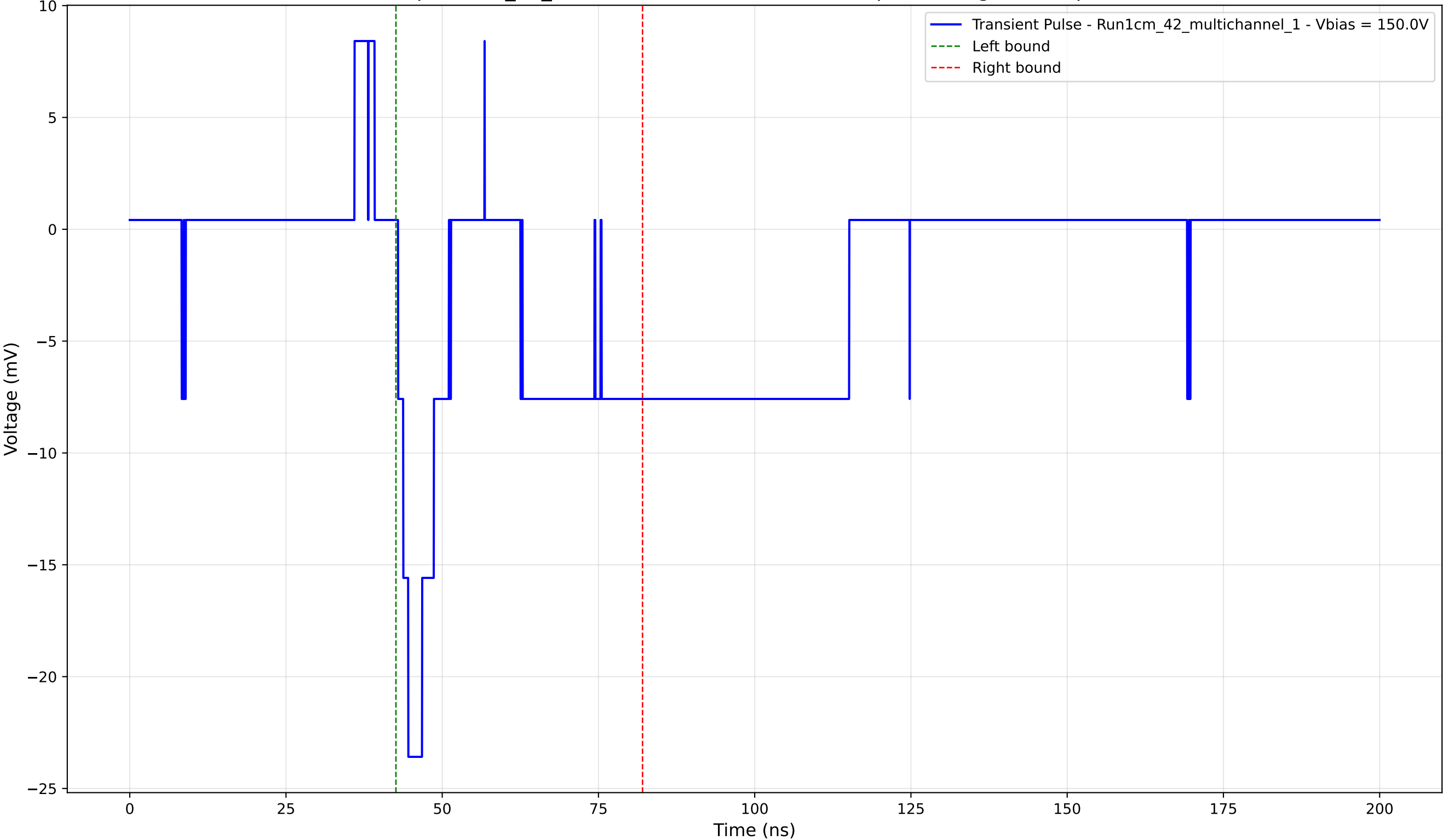
Transient Pulse - Sample: 1cm_42_multichannel - Position: 4360.0 \mu\text{m} - Charge: -5.19 pC - Rise Time: 1.63 ns
