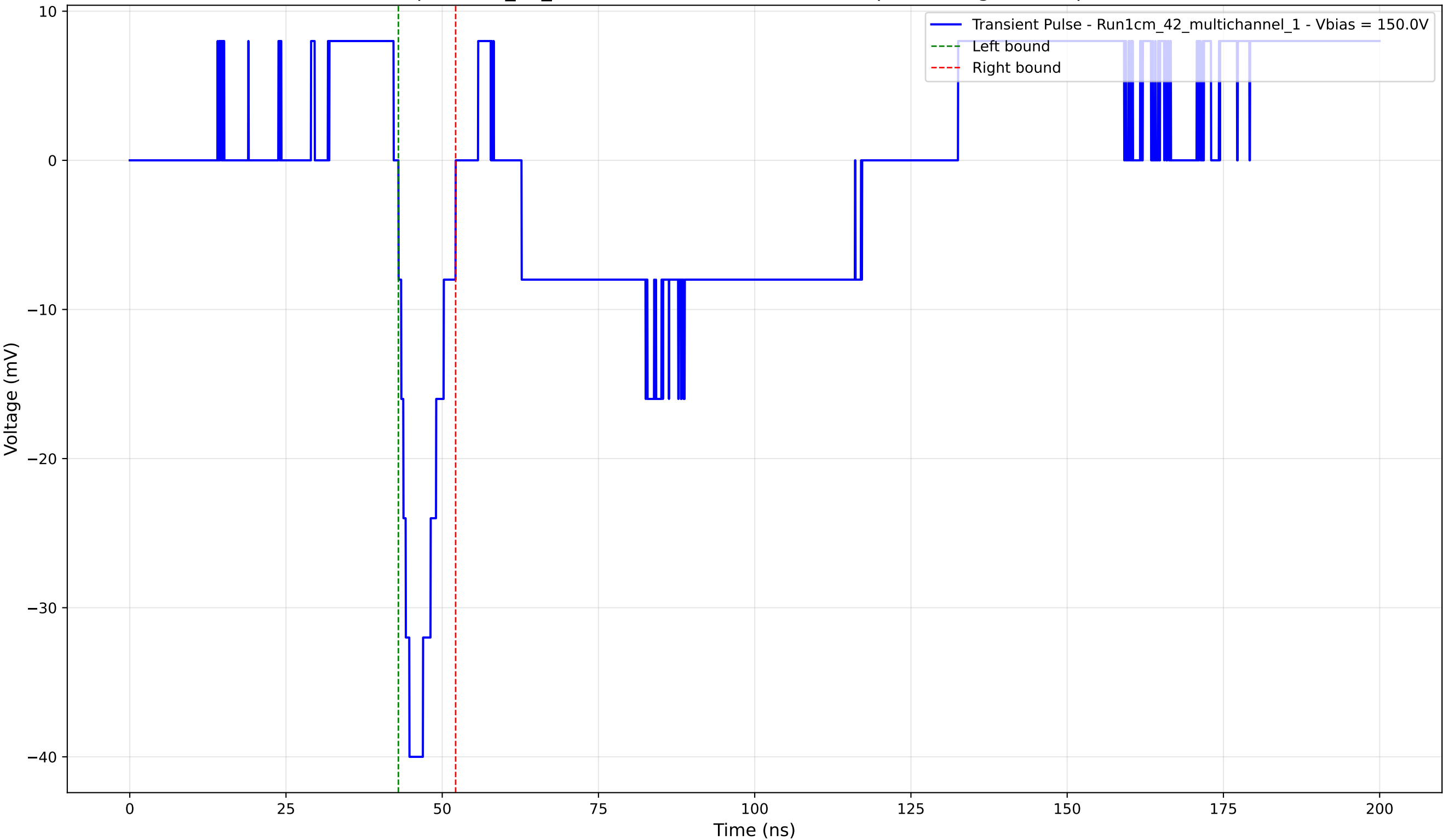
Transient Pulse - Sample: 1cm_42_multichannel - Position: 4565.0 \mu\text{m} - Charge: -4.37 pC - Rise Time: 1.75 ns
