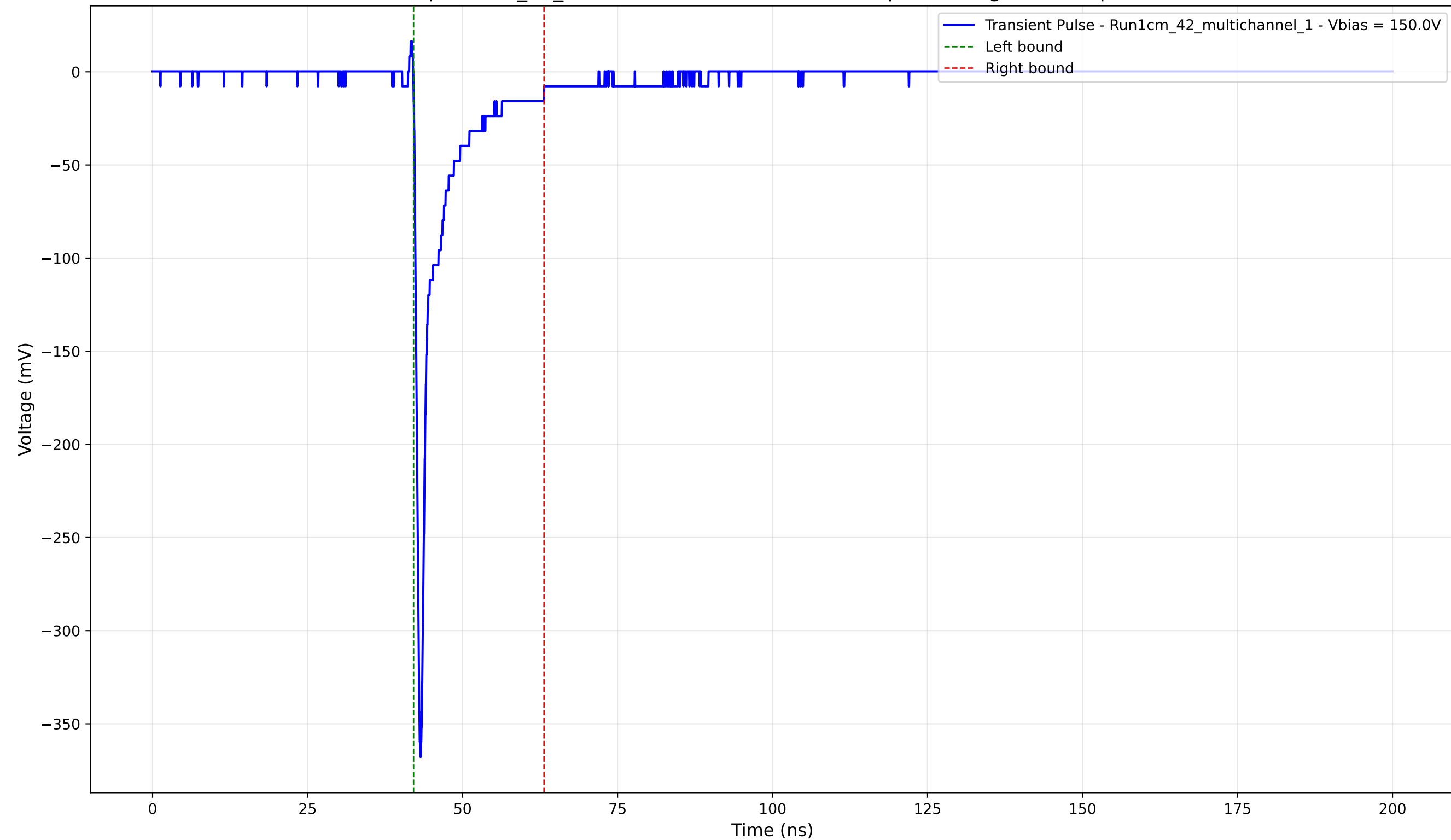
Transient Pulse - Sample: 1cm_42_multichannel - Position: 2210.0 \mu\text{m} - Charge: -24.62 pC - Rise Time: 0.75 ns
