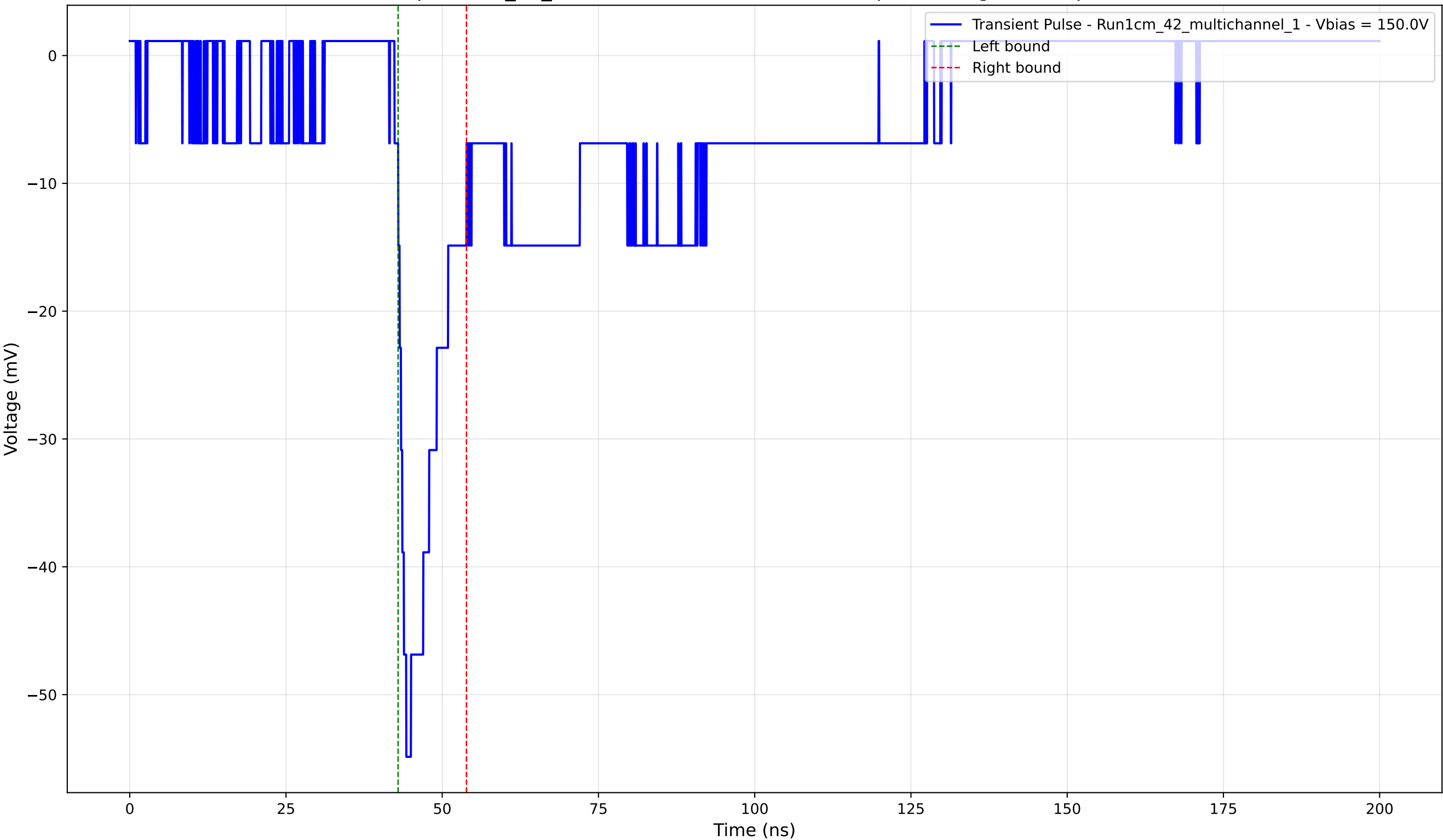
Transient Pulse - Sample: 1cm_42_multichannel - Position: 3830.0 \mu\text{m} - Charge: -6.71 pC - Rise Time: 1.88 ns
