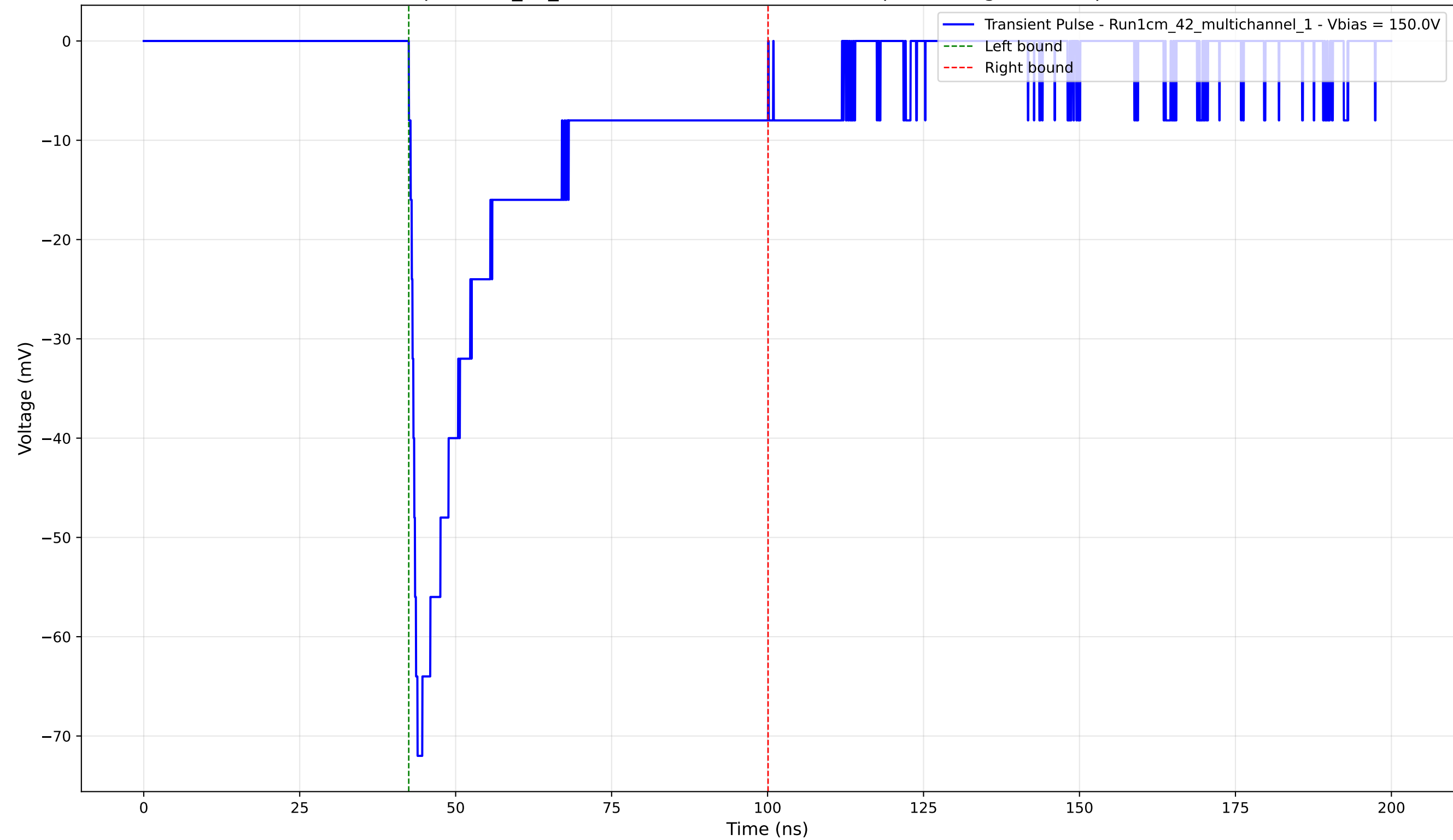
Transient Pulse - Sample: 1cm_42_multichannel - Position: 3590.0 \mu\text{m} - Charge: -19.89 pC - Rise Time: 1.38 ns
