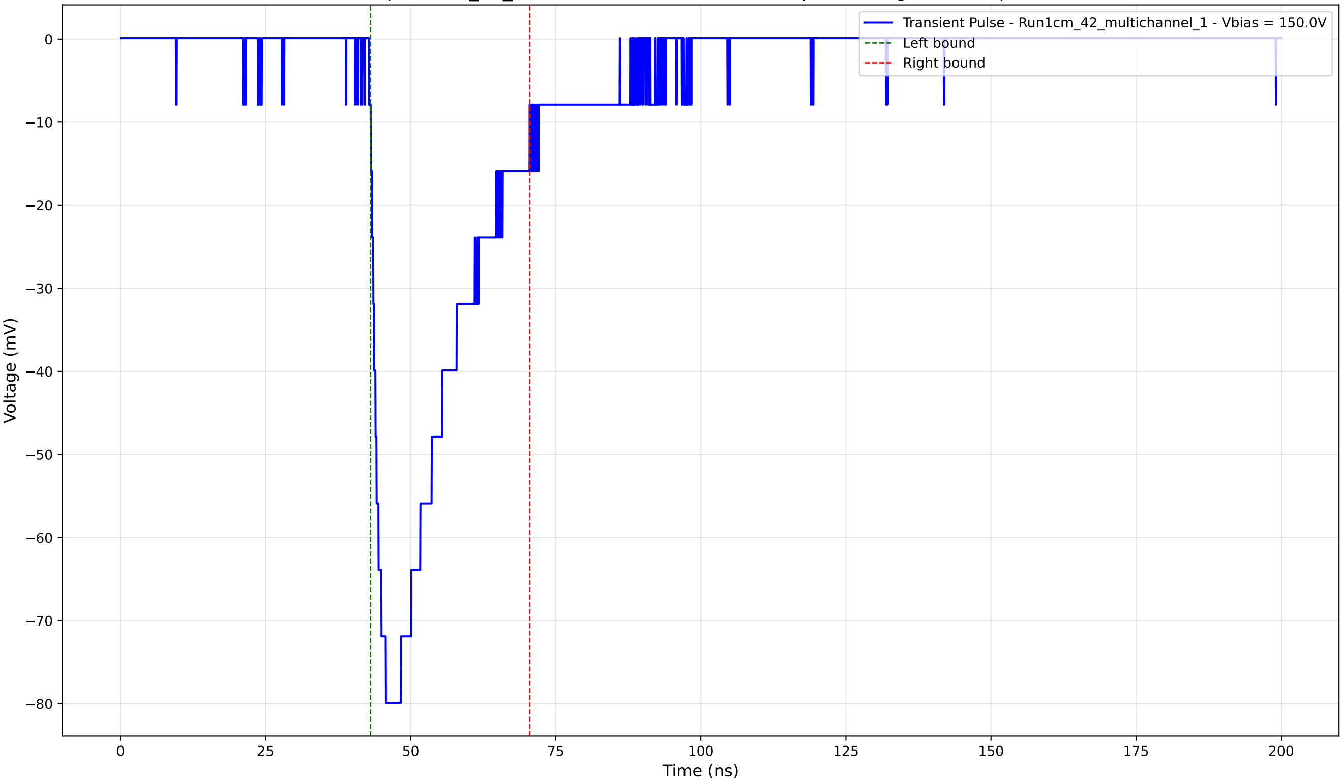
Transient Pulse - Sample: 1cm_42_multichannel - Position: 535.0 \mu\text{m} - Charge: -23.11 pC - Rise Time: 2.62 ns
