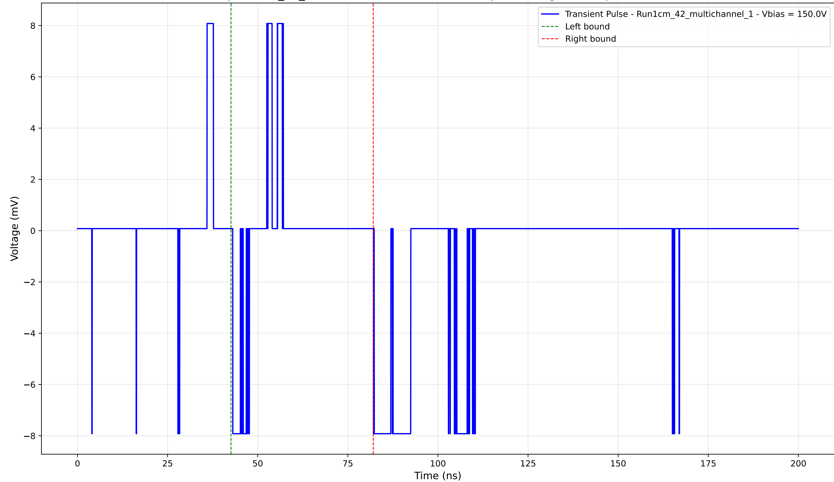
Transient Pulse - Sample: 1cm_42_multichannel - Position: 3905.0 \mu\text{m} - Charge: -0.10 pC - Rise Time: 0.00 ns (N/A)
