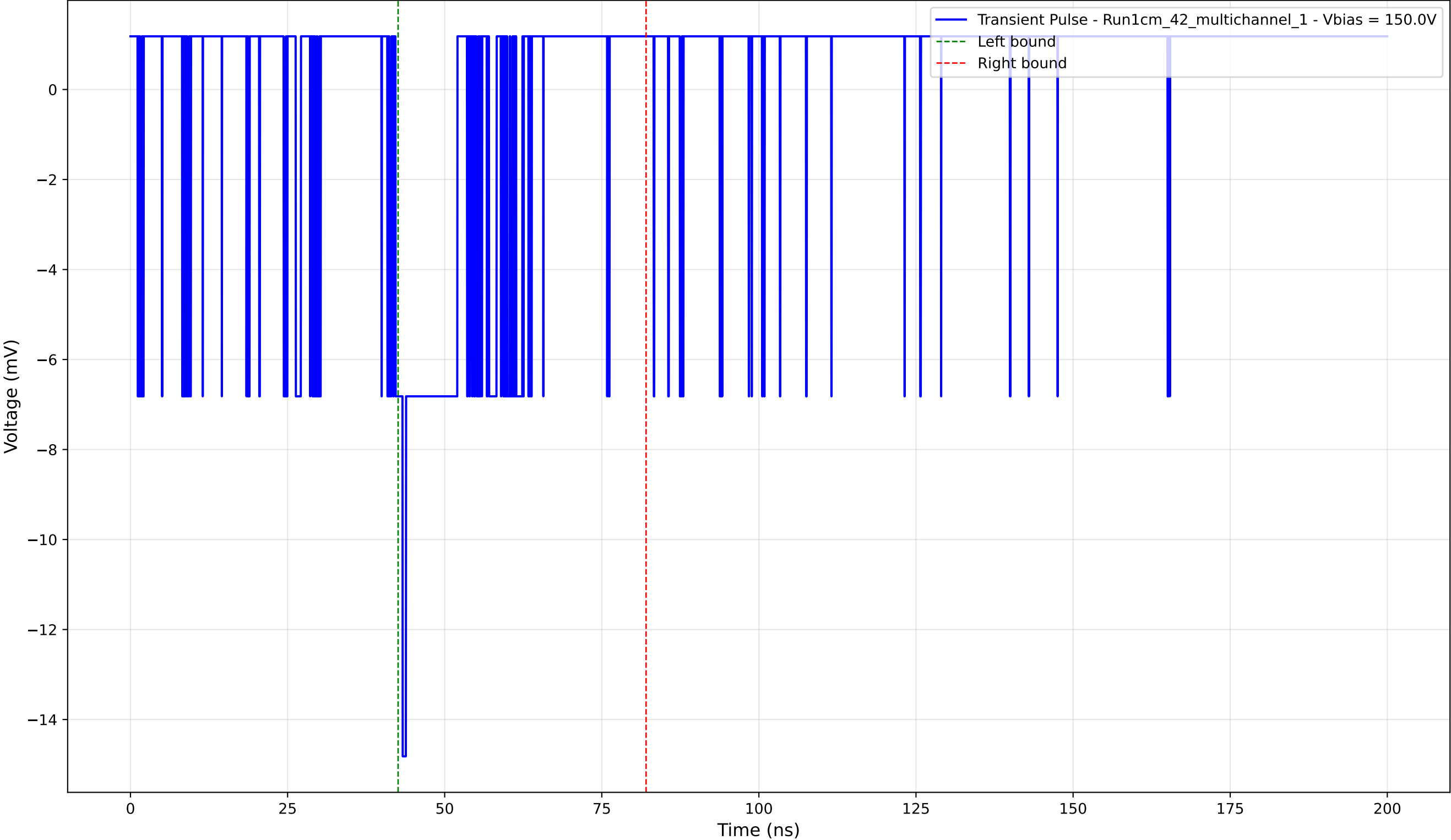
Transient Pulse - Sample: 1cm_42_multichannel - Position: 2910.0 \mu\text{m} - Charge: -1.53 pC - Rise Time: 1.14 ns
