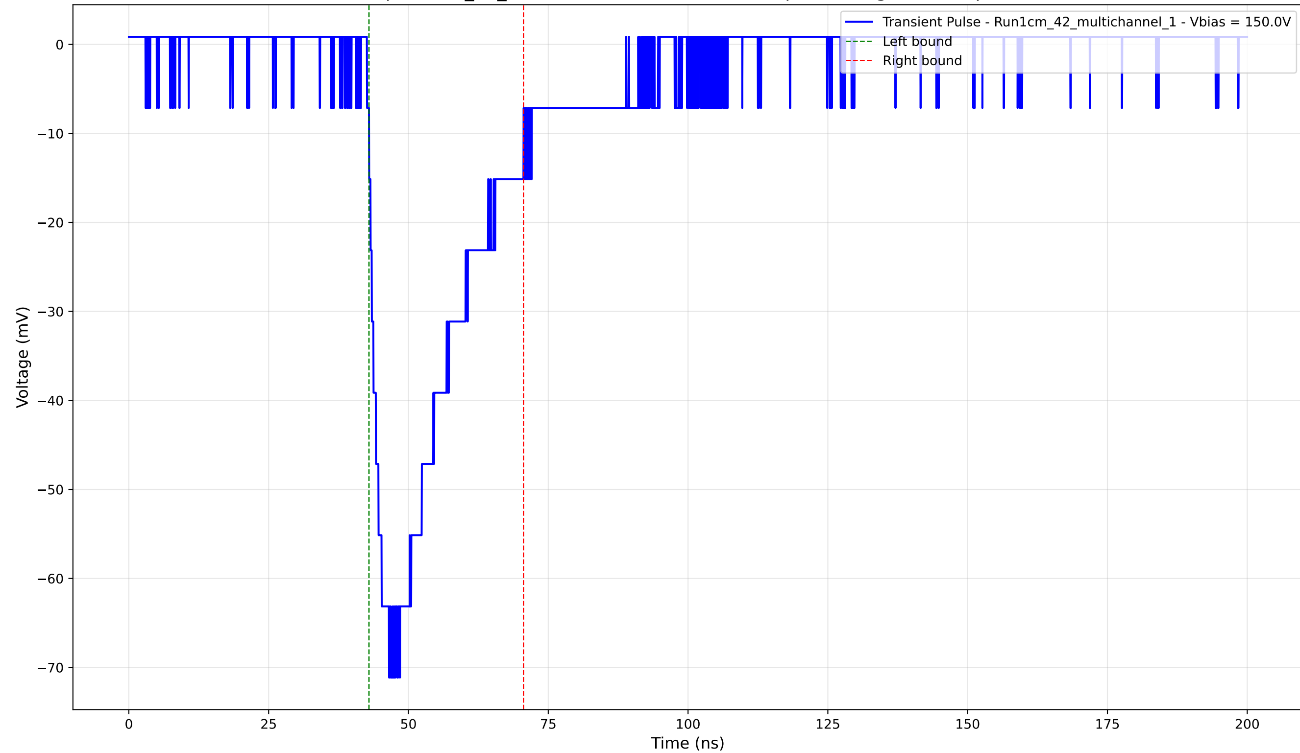
Transient Pulse - Sample: 1cm_42_multichannel - Position: 190.0 \mu\text{m} - Charge: -20.62 pC - Rise Time: 3.94 ns
