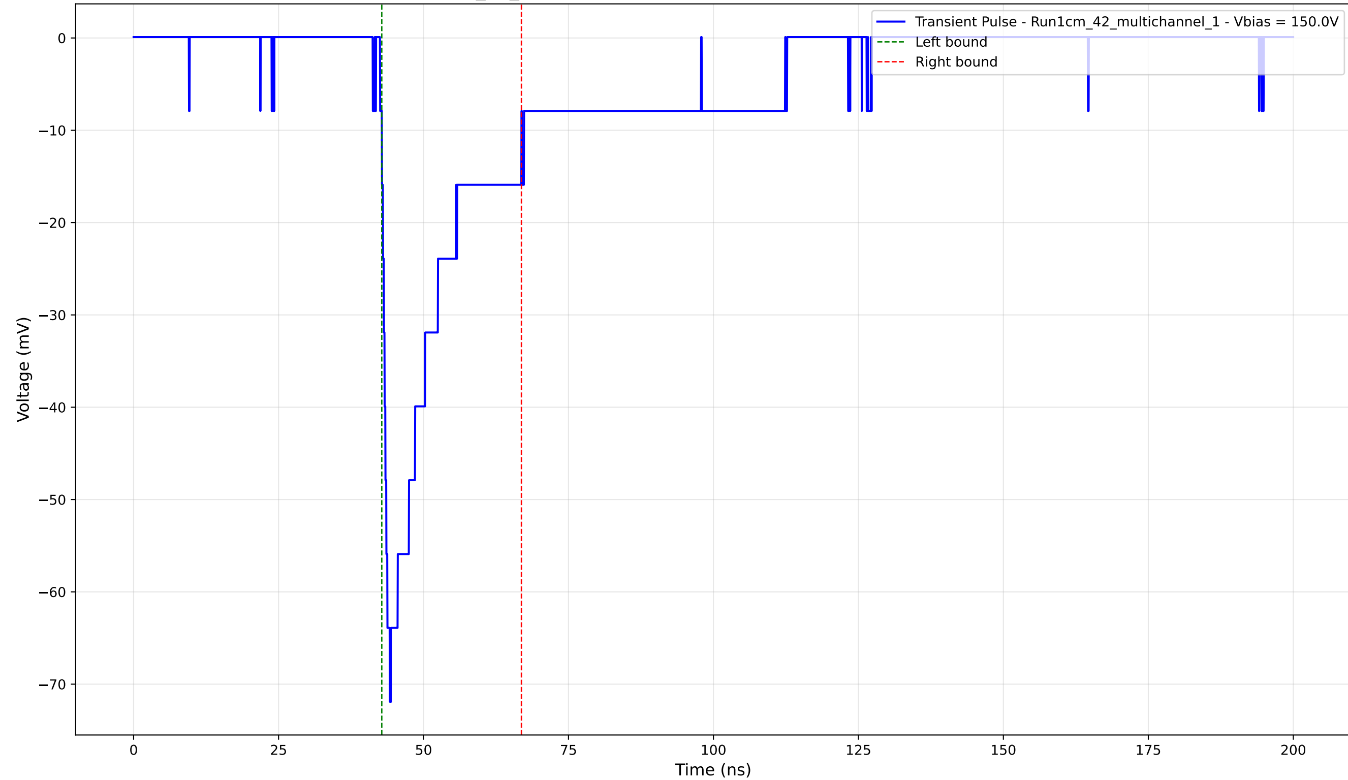
Transient Pulse - Sample: 1cm_42_multichannel - Position: 3615.0 \mu\text{m} - Charge: -14.07 pC - Rise Time: 1.68 ns
