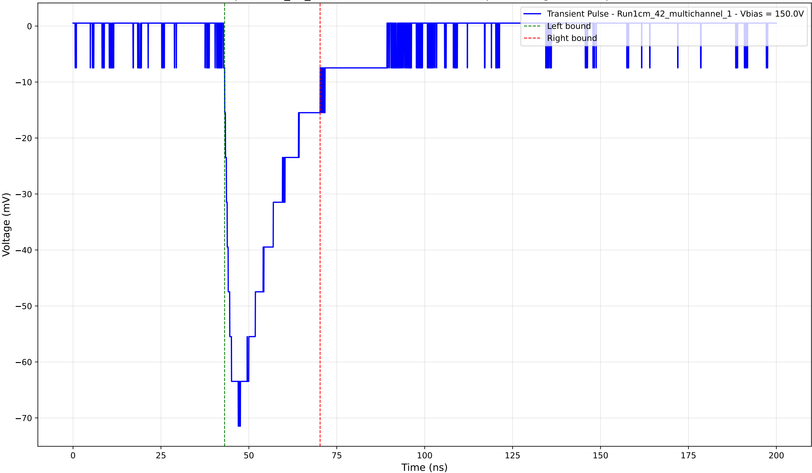
Transient Pulse - Sample: 1cm_42_multichannel - Position: 435.0 \mu\text{m} - Charge: -20.07 pC - Rise Time: 4.20 ns
