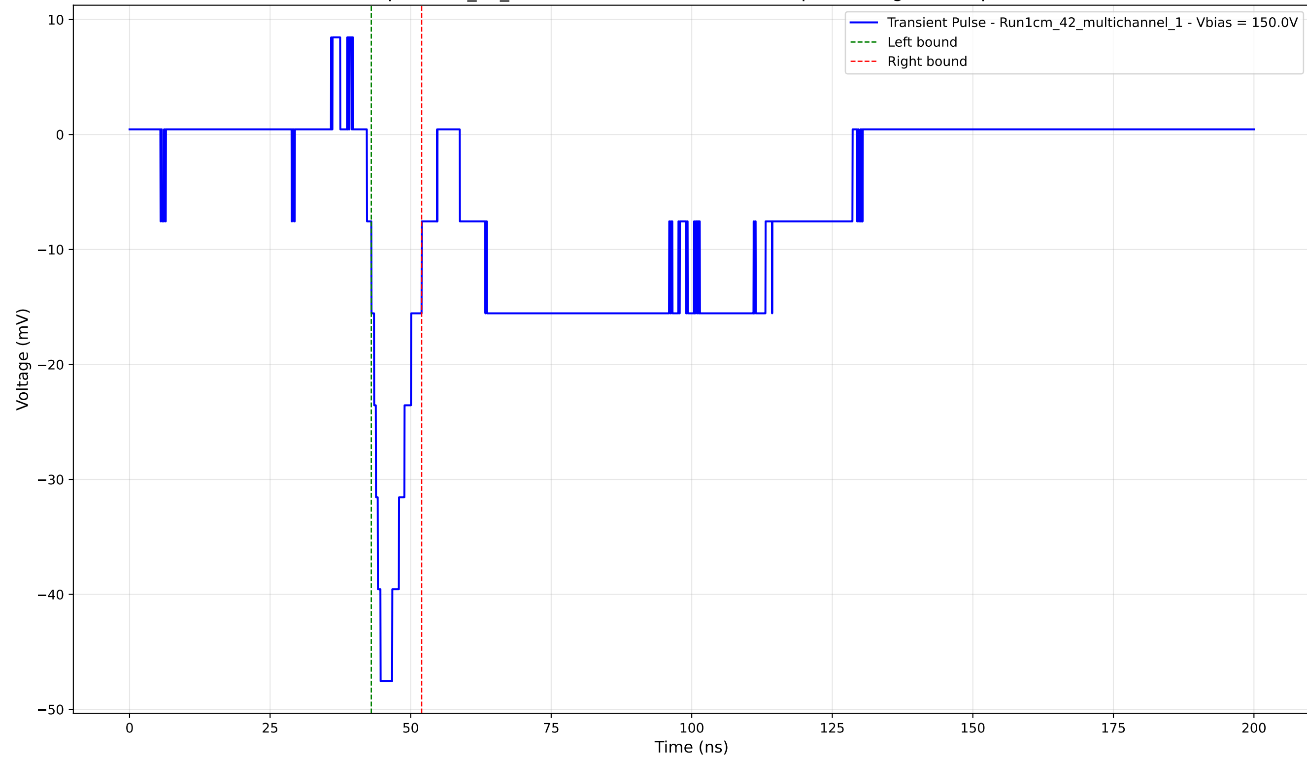
Transient Pulse - Sample: 1cm_42_multichannel - Position: 4650.0 \mu\text{m} - Charge: -5.58 pC - Rise Time: 2.43 ns
