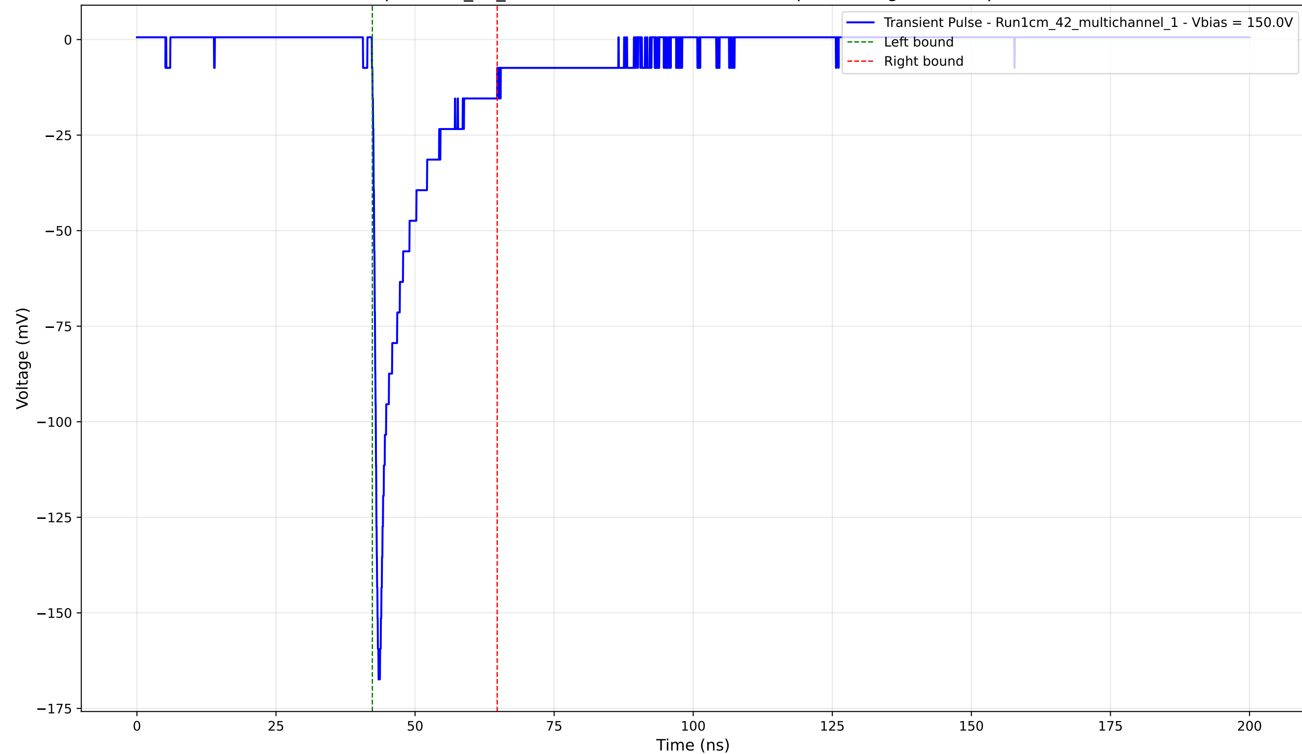
Transient Pulse - Sample: 1cm_42_multichannel - Position: 2980.0 \mu\text{m} - Charge: -19.71 pC - Rise Time: 0.82 ns
