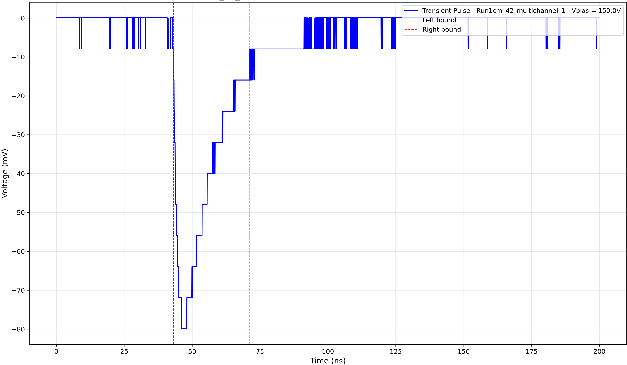
Transient Pulse - Sample: 1cm_42_multichannel - Position: 515.0 \mu\text{m} - Charge: -23.29 pC - Rise Time: 2.86 ns
