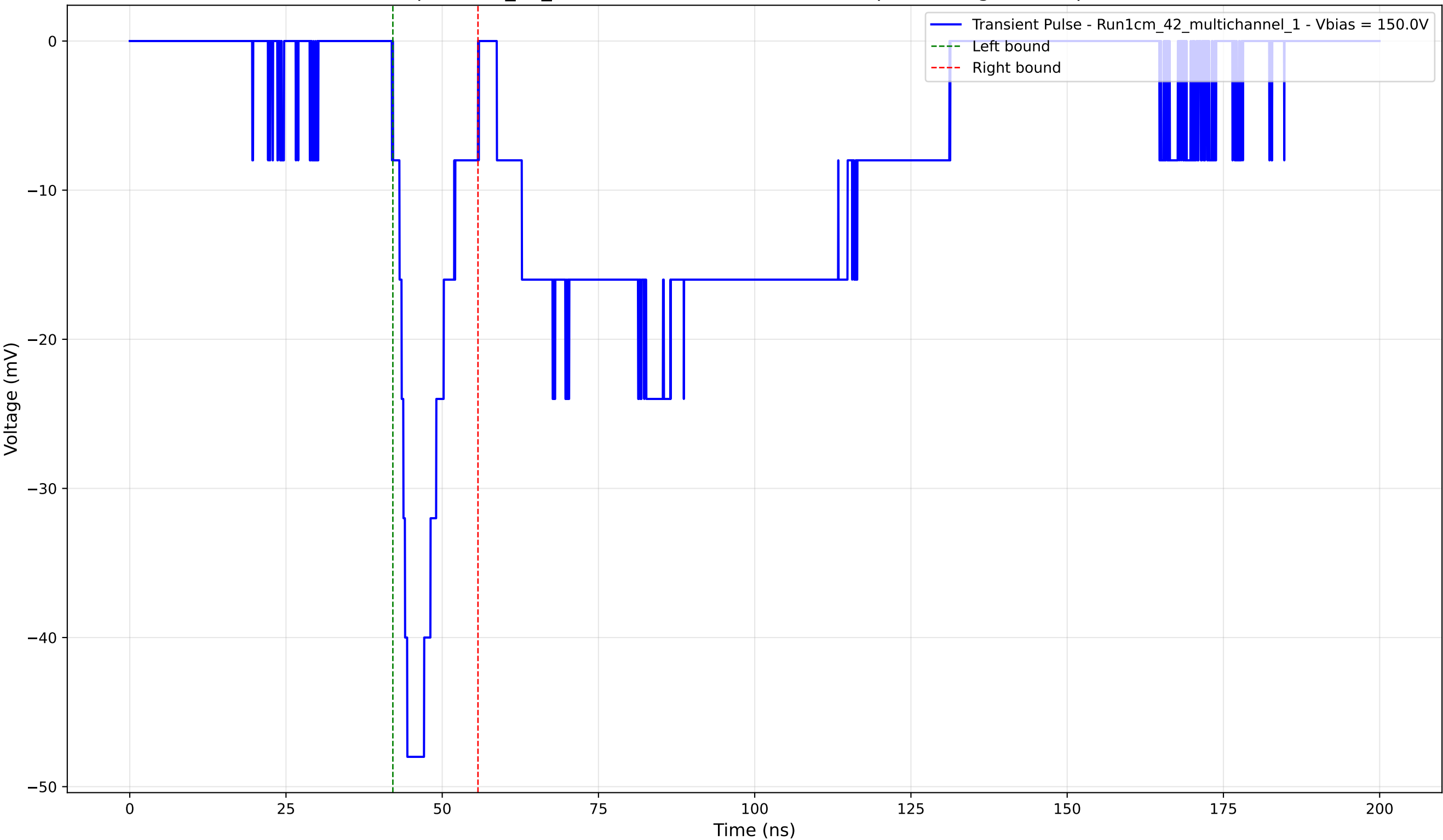
Transient Pulse - Sample: 1cm_42_multichannel - Position: 4275.0 \mu\text{m} - Charge: -6.60 pC - Rise Time: 2.29 ns
