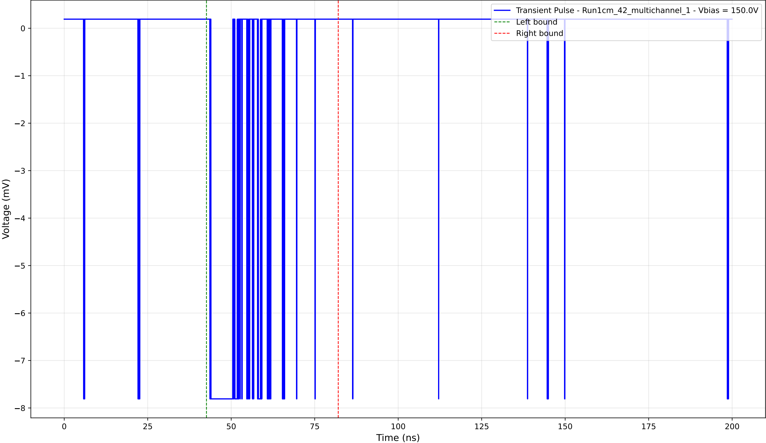
Transient Pulse - Sample: 1cm_42_multichannel - Position: 860.0 \mu\text{m} - Charge: -1.58 pC - Rise Time: 0.02 ns
