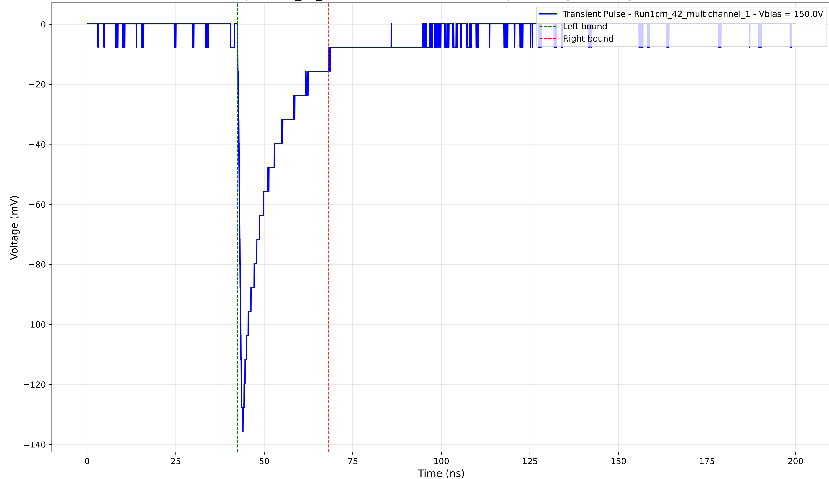
Transient Pulse - Sample: 1cm_42_multichannel - Position: 1530.0 \mu\text{m} - Charge: -23.36 pC - Rise Time: 1.05 ns
