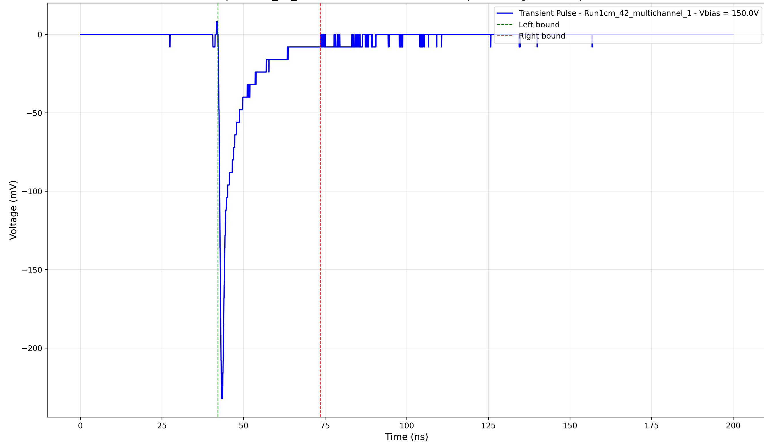
Transient Pulse - Sample: 1cm_42_multichannel - Position: 2785.0 \mu\text{m} - Charge: -22.81 pC - Rise Time: 0.82 ns
