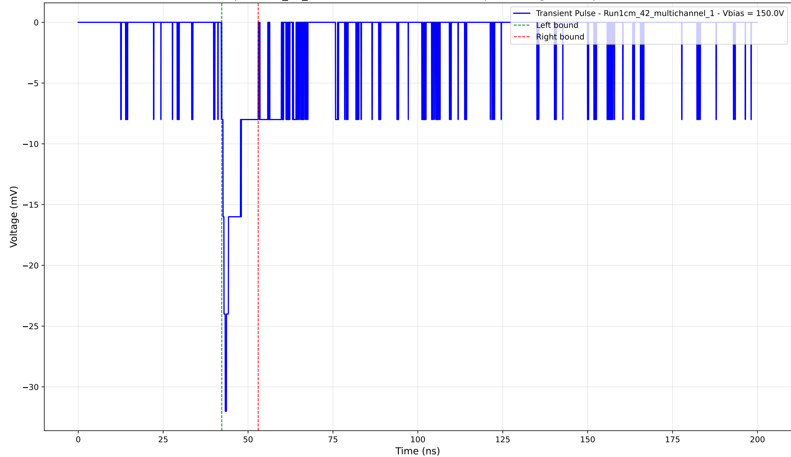
Transient Pulse - Sample: 1cm_42_multichannel - Position: 1910.0 \mu\text{m} - Charge: -2.82 pC - Rise Time: 1.01 ns
