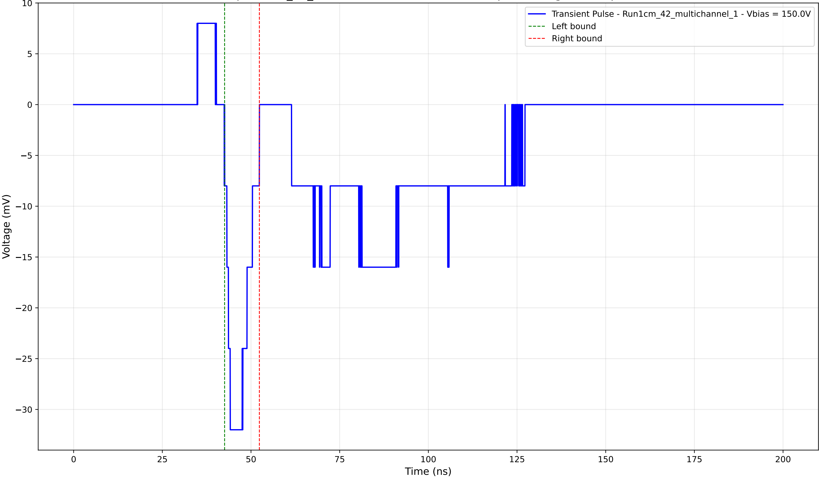
Transient Pulse - Sample: 1cm_42_multichannel - Position: 4825.0 \mu\text{m} - Charge: -4.12 pC - Rise Time: 1.57 ns
