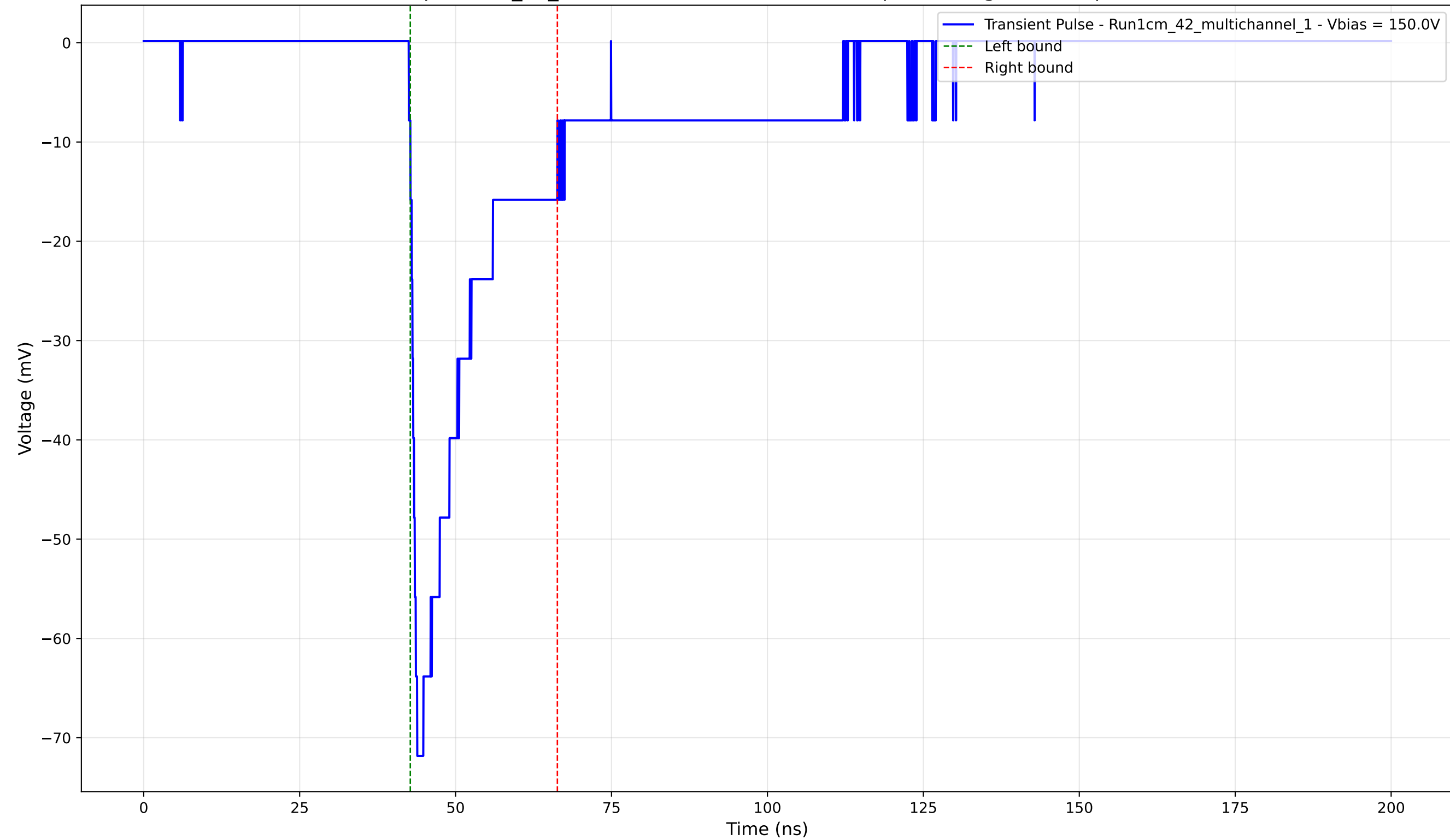
Transient Pulse - Sample: 1cm_42_multichannel - Position: 3565.0 \mu\text{m} - Charge: -14.32 pC - Rise Time: 1.34 ns
