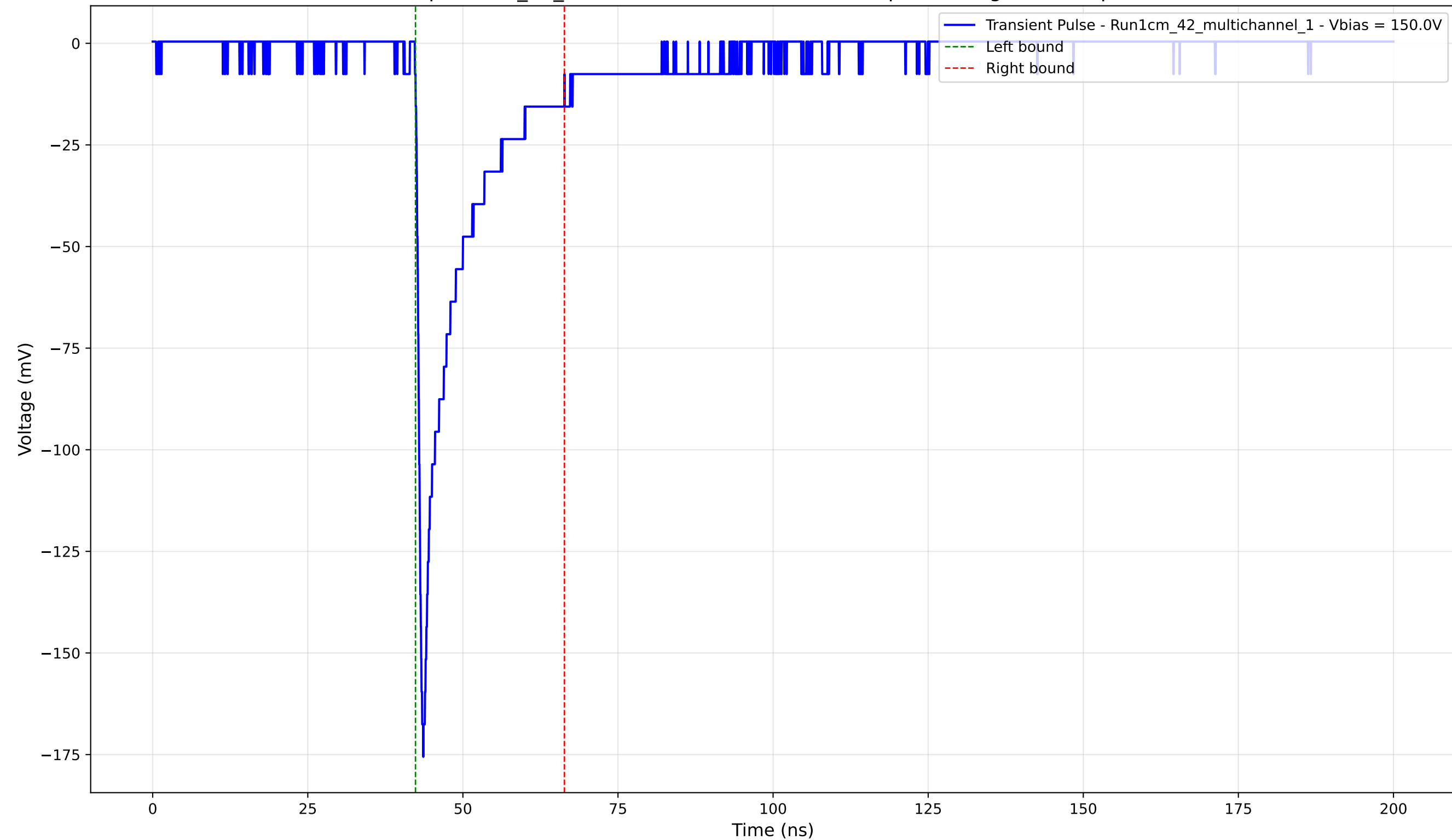
Transient Pulse - Sample: 1cm_42_multichannel - Position: 1750.0 \mu\text{m} - Charge: -22.37 pC - Rise Time: 0.86 ns
