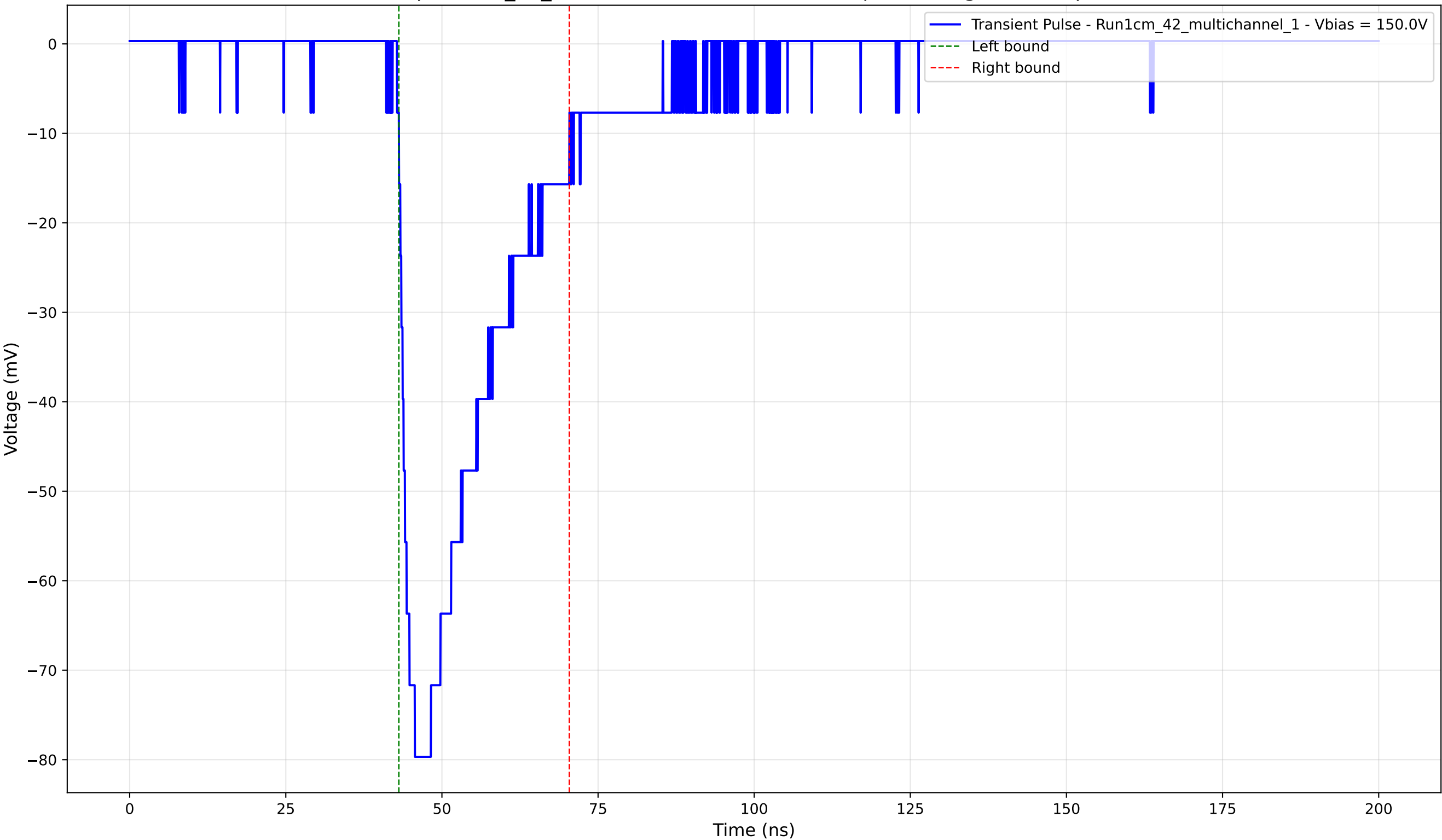
Transient Pulse - Sample: 1cm_42_multichannel - Position: 630.0 \mu\text{m} - Charge: -22.91 pC - Rise Time: 2.56 ns
