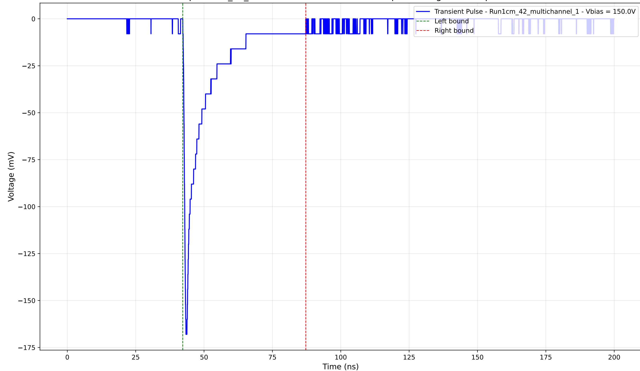
Transient Pulse - Sample: 1cm_42_multichannel - Position: 2995.0 \mu\text{m} - Charge: -24.30 pC - Rise Time: 0.80 ns
