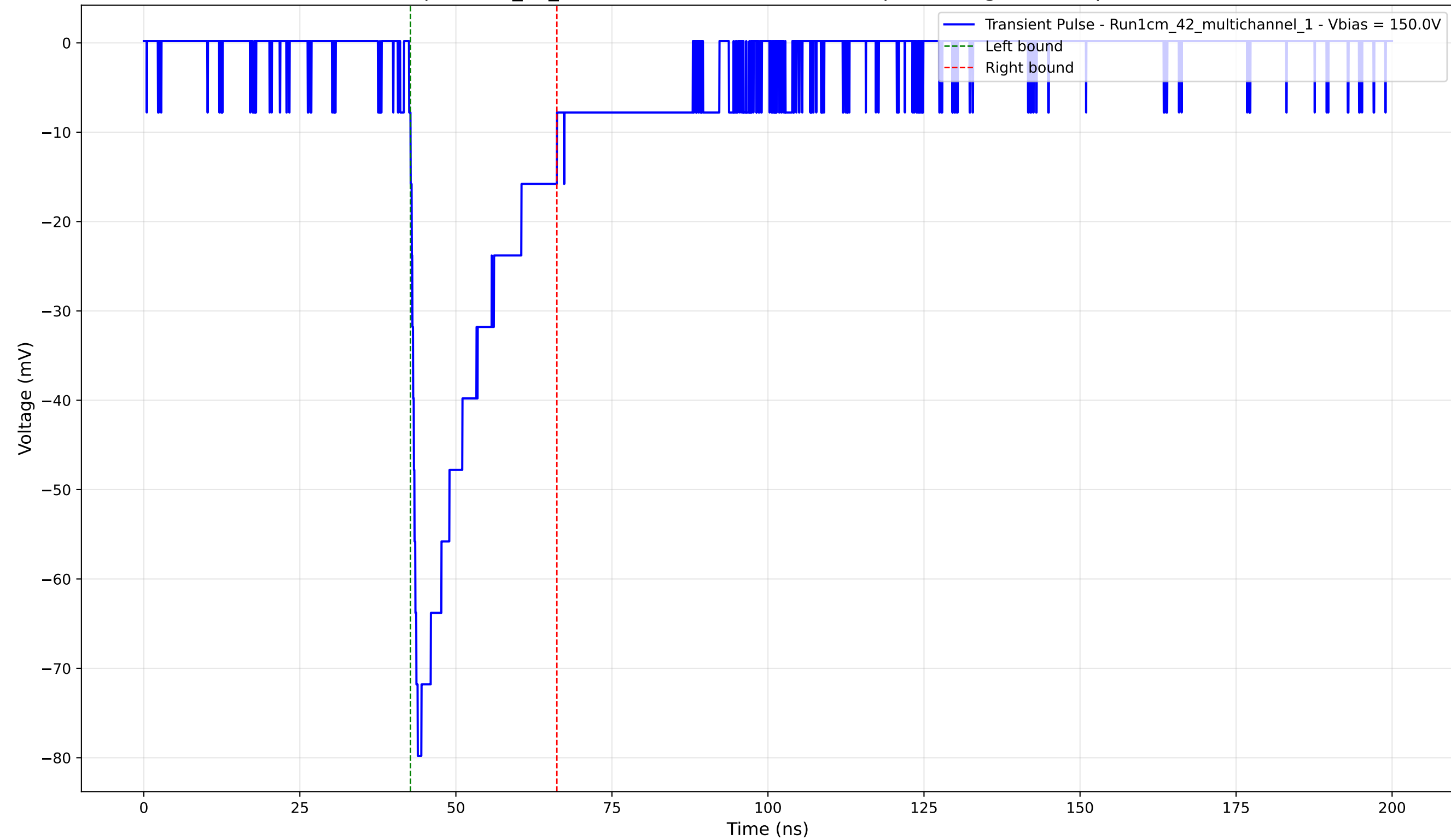
Transient Pulse - Sample: 1cm_42_multichannel - Position: 1310.0 \mu\text{m} - Charge: -17.21 pC - Rise Time: 1.16 ns
