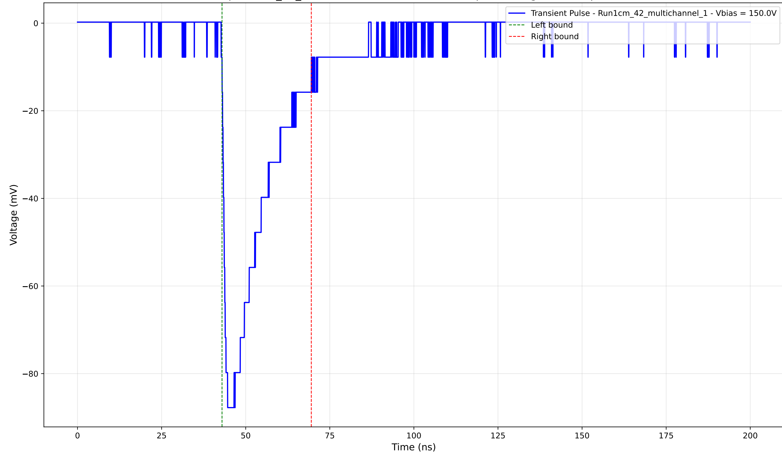
Transient Pulse - Sample: 1cm_42_multichannel - Position: 1015.0 \mu\text{m} - Charge: -23.00 pC - Rise Time: 1.18 ns
