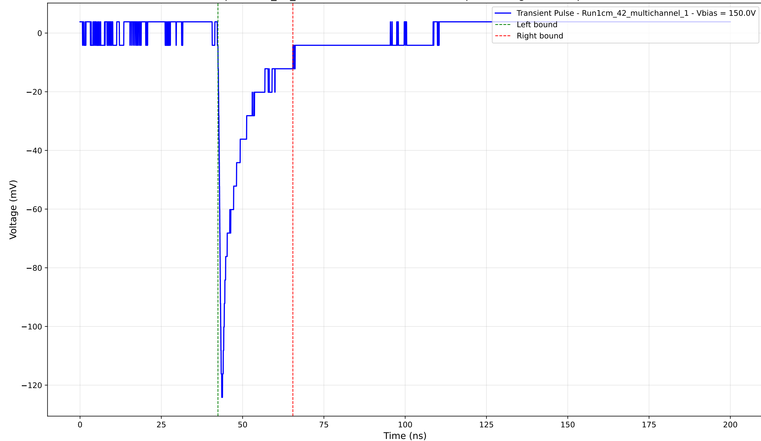
Transient Pulse - Sample: 1cm_42_multichannel - Position: 3145.0 \mu\text{m} - Charge: -15.58 pC - Rise Time: 0.86 ns
