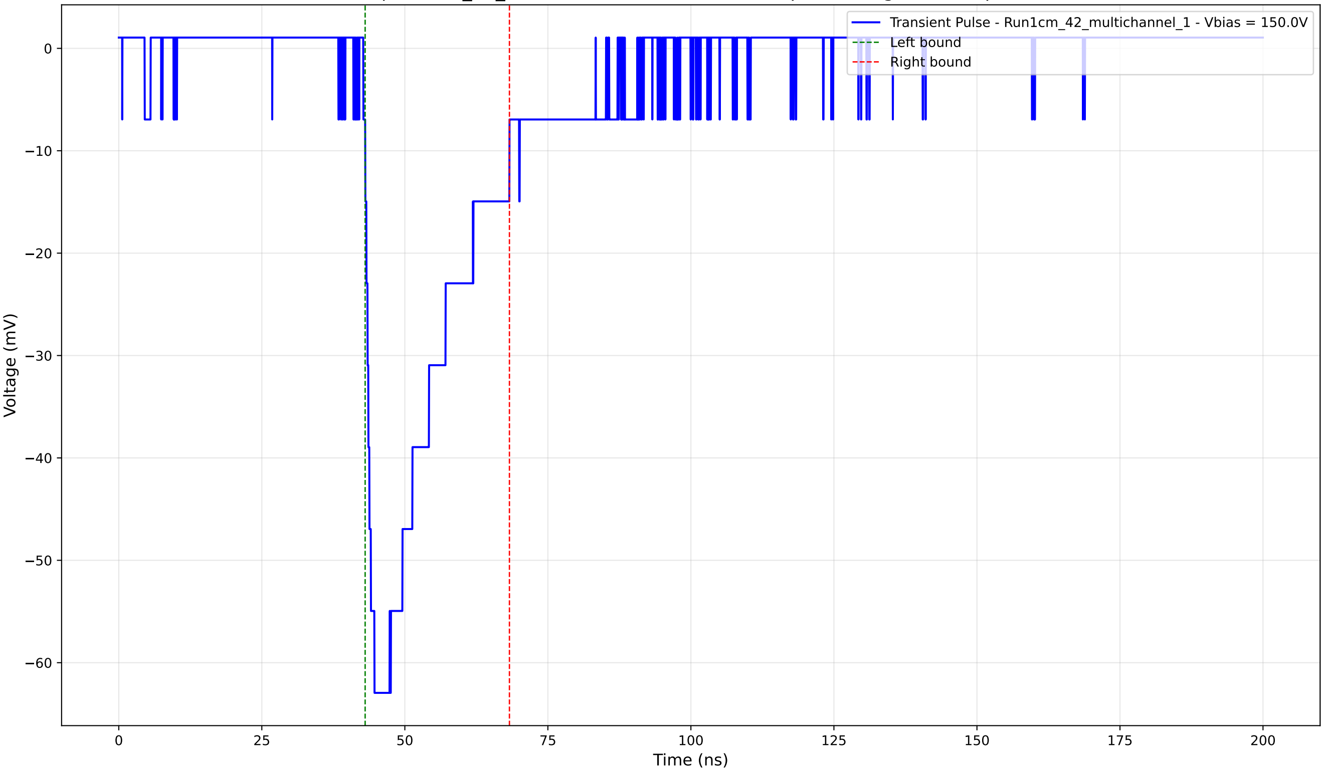
Transient Pulse - Sample: 1cm_42_multichannel - Position: 930.0 \mu\text{m} - Charge: -16.94 pC - Rise Time: 1.94 ns
