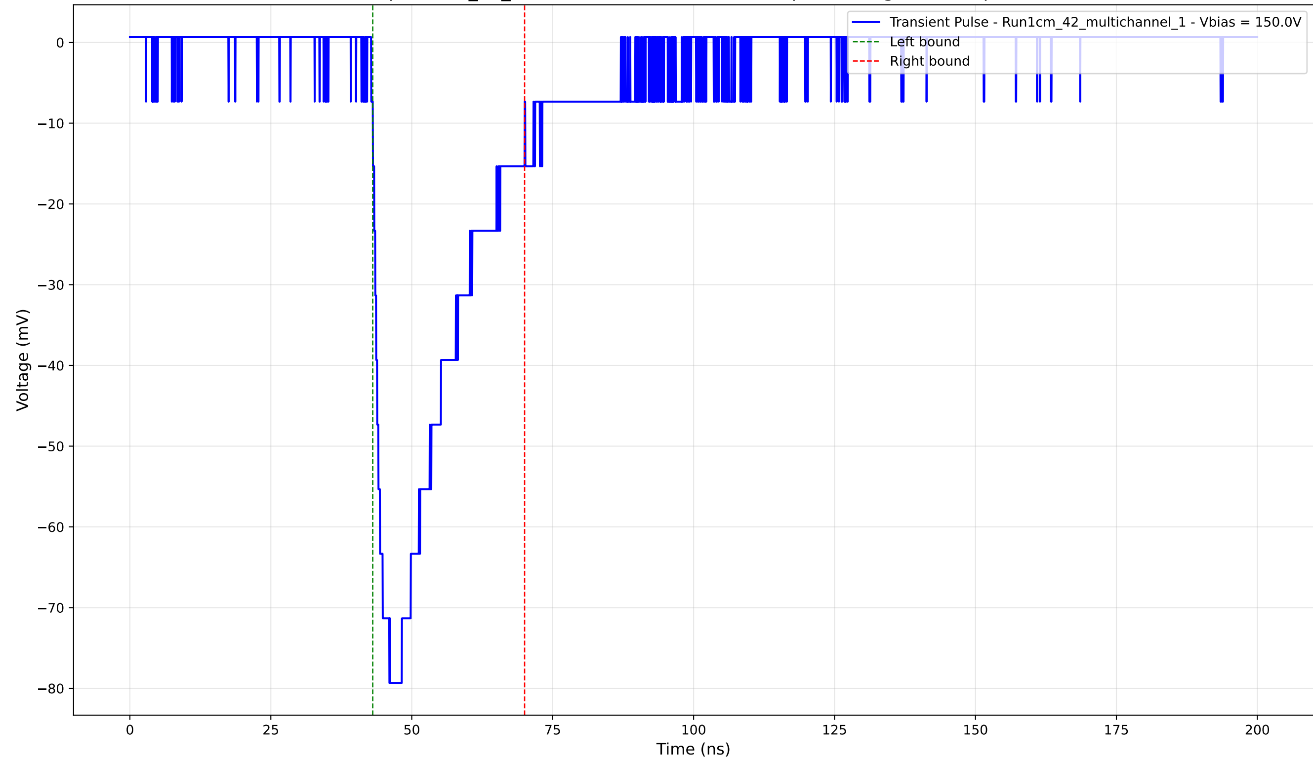
Transient Pulse - Sample: 1cm_42_multichannel - Position: 605.0 \mu\text{m} - Charge: -22.40 pC - Rise Time: 2.94 ns
