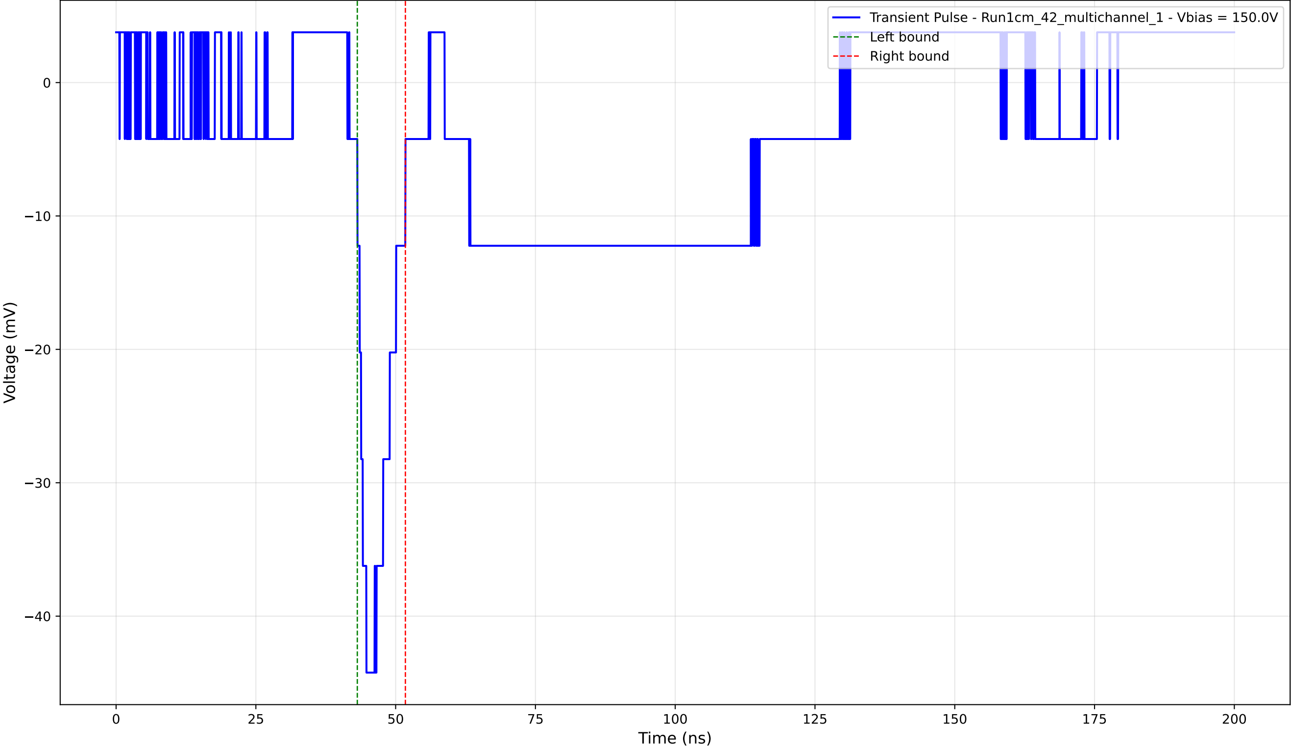
Transient Pulse - Sample: 1cm_42_multichannel - Position: 4320.0 \mu\text{m} - Charge: -4.82 pC - Rise Time: 1.62 ns
