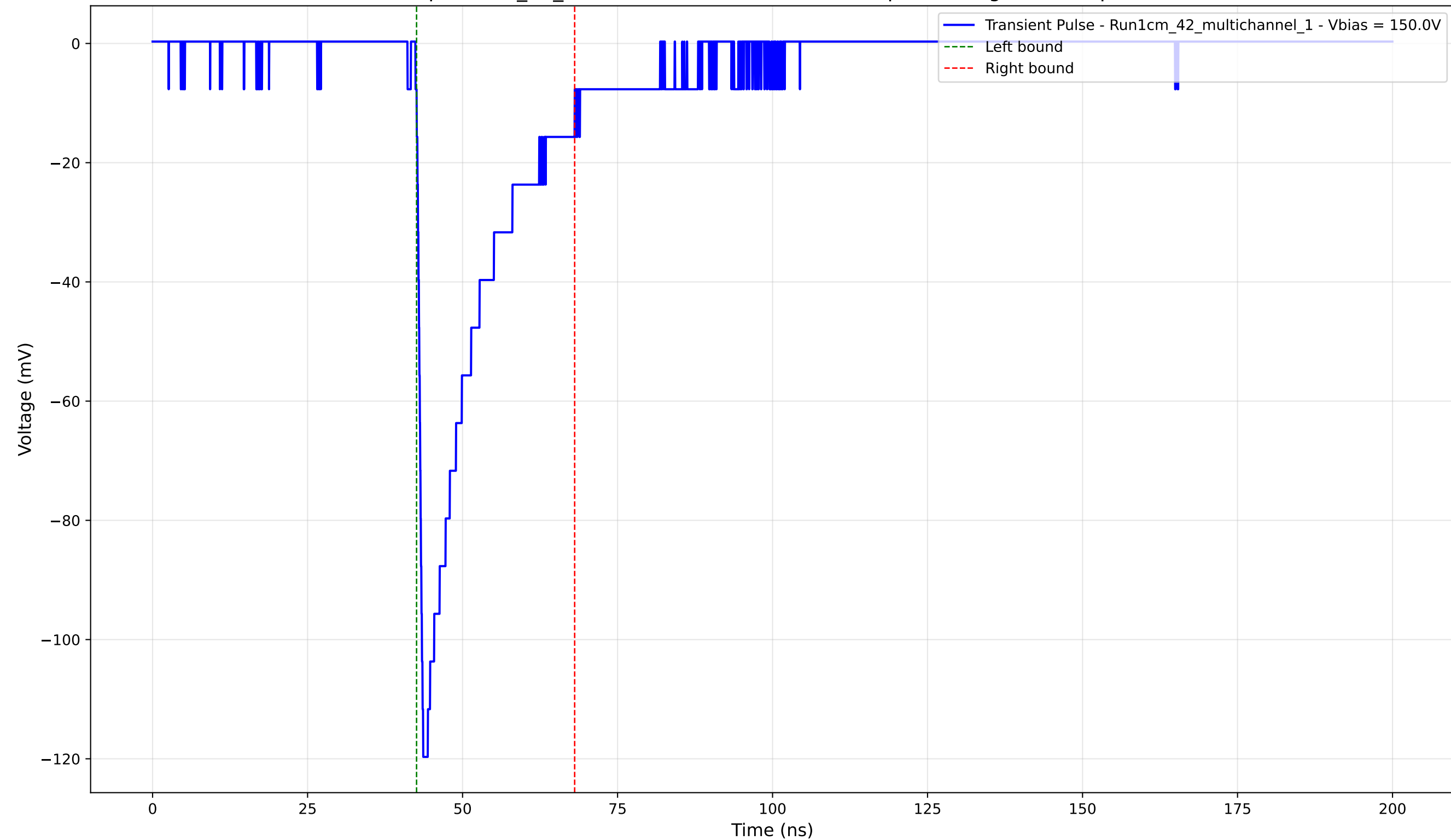
Transient Pulse - Sample: 1cm_42_multichannel - Position: 1470.0 \mu\text{m} - Charge: -23.02 pC - Rise Time: 0.95 ns
