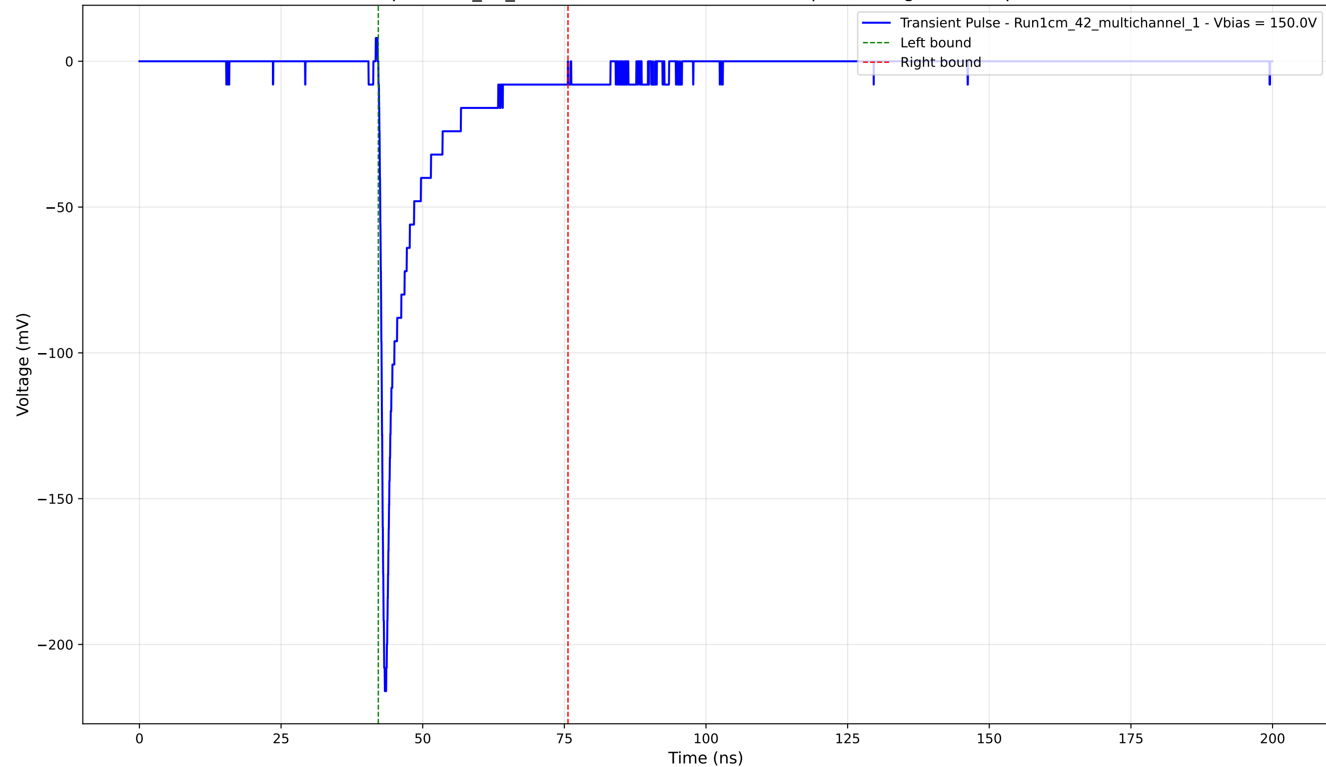
Transient Pulse - Sample: 1cm_42_multichannel - Position: 2805.0 \mu\text{m} - Charge: -22.35 pC - Rise Time: 0.83 ns
