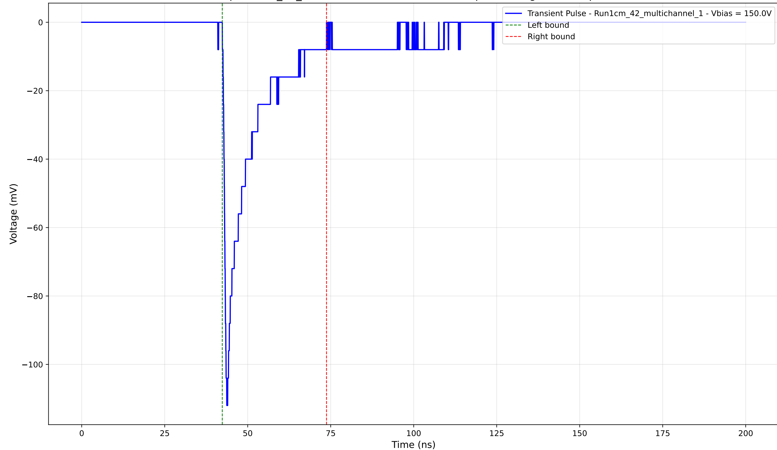
Transient Pulse - Sample: 1cm_42_multichannel - Position: 3260.0 \mu\text{m} - Charge: -17.85 pC - Rise Time: 0.93 ns
