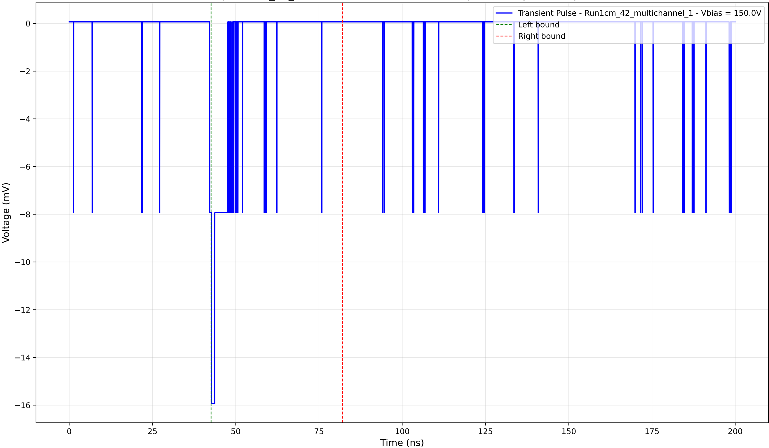
Transient Pulse - Sample: 1cm_42_multichannel - Position: 2390.0 \mu\text{m} - Charge: -1.21 pC - Rise Time: 0.58 ns
