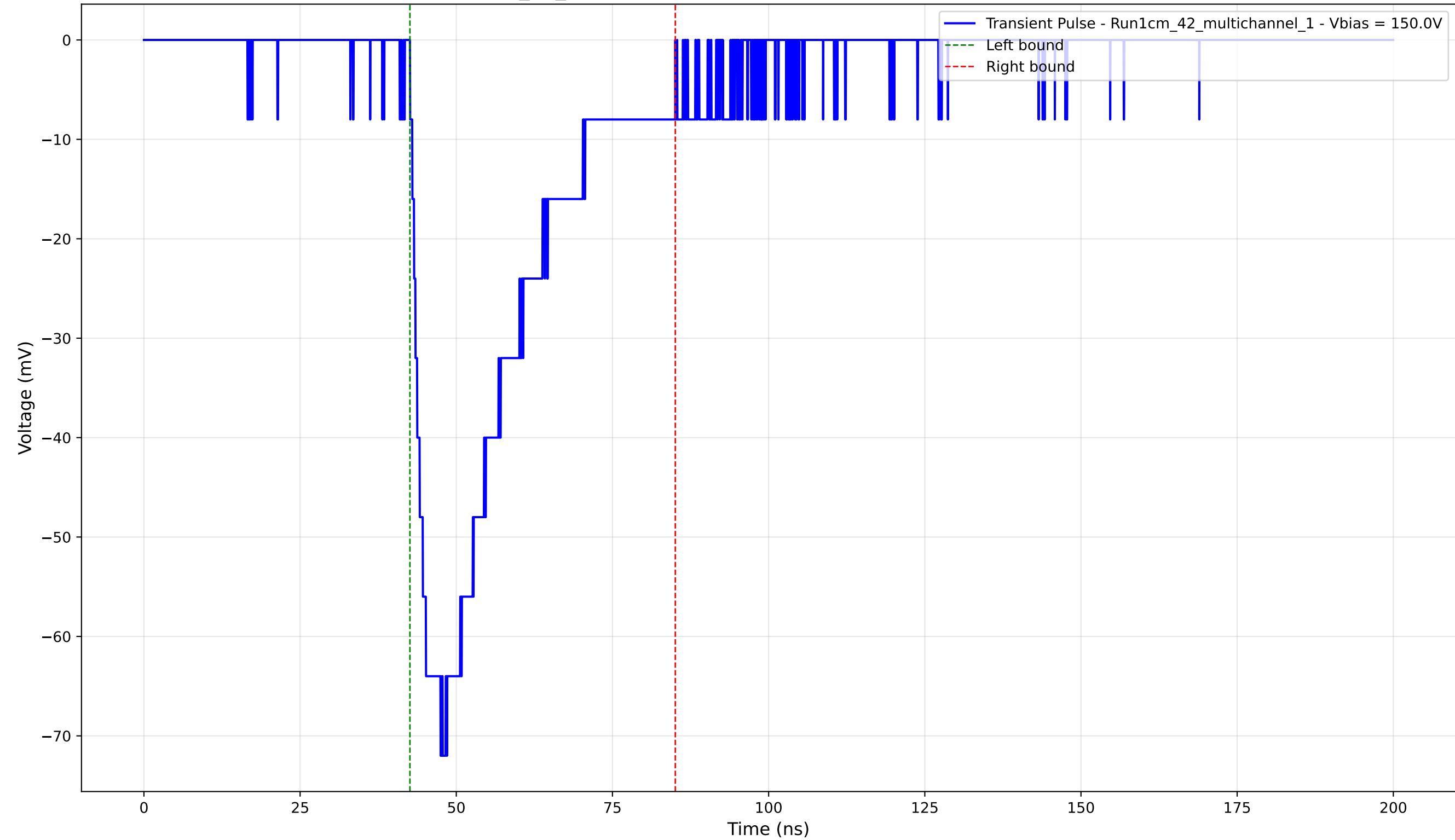
Transient Pulse - Sample: 1cm_42_multichannel - Position: 175.0 \mu\text{m} - Charge: -23.29 pC - Rise Time: 4.88 ns
