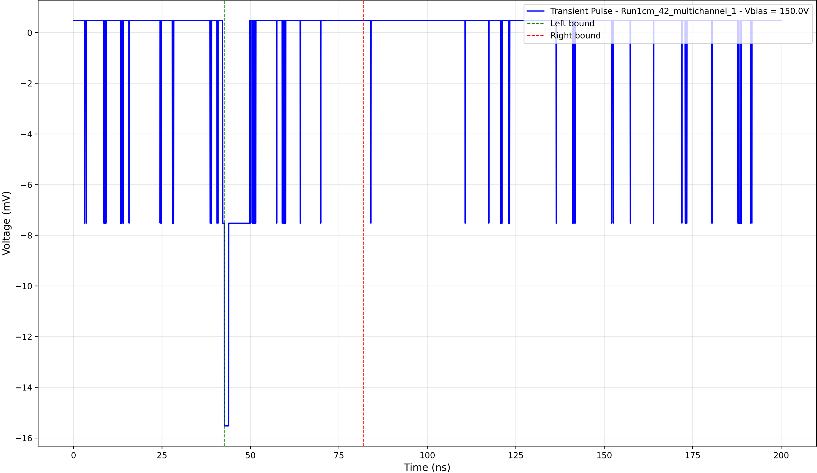
Transient Pulse - Sample: 1cm_42_multichannel - Position: 2375.0 \mu\text{m} - Charge: -1.14 pC - Rise Time: 0.50 ns
