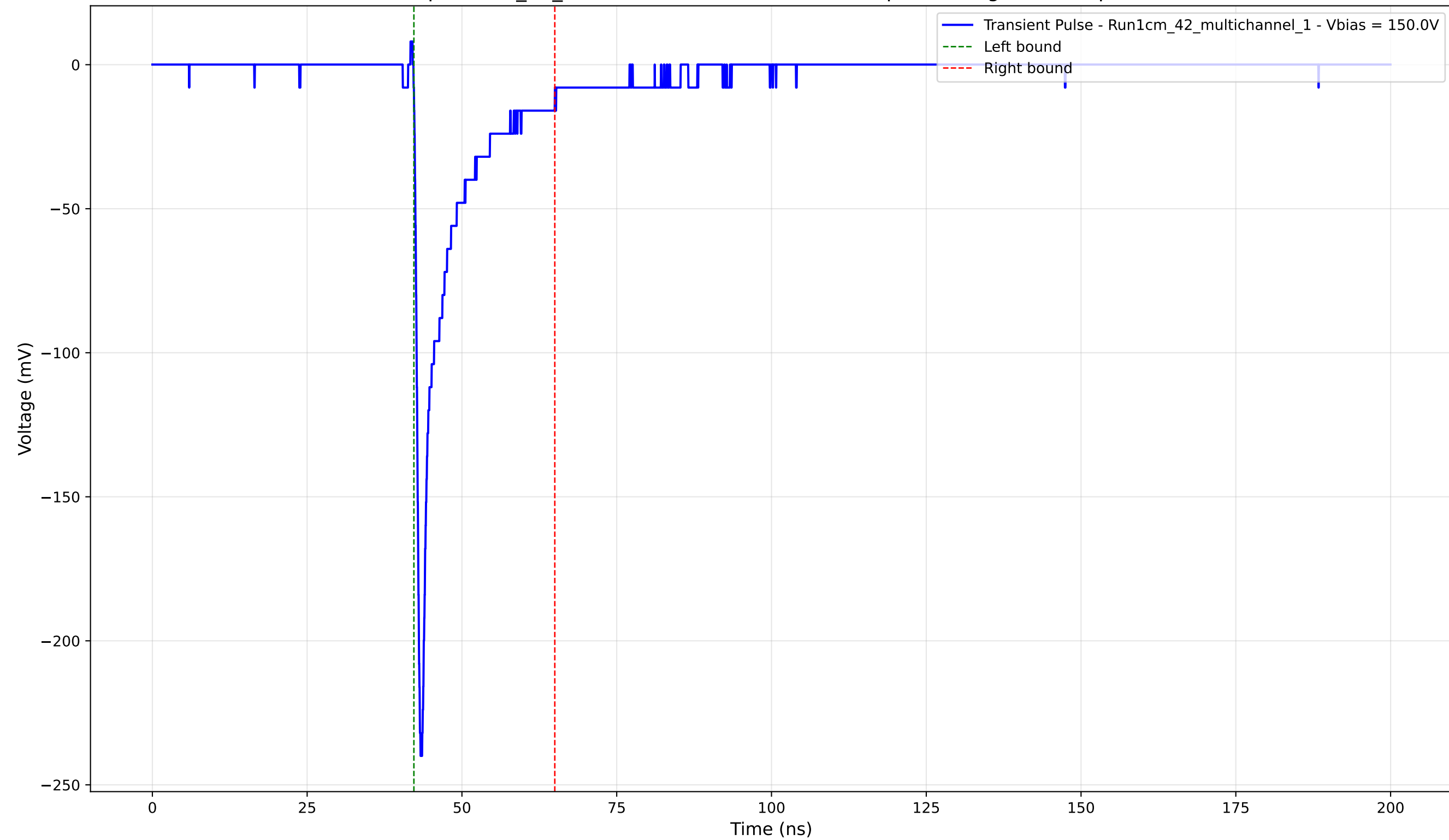
Transient Pulse - Sample: 1cm_42_multichannel - Position: 1975.0 \mu\text{m} - Charge: -23.04 pC - Rise Time: 0.82 ns
