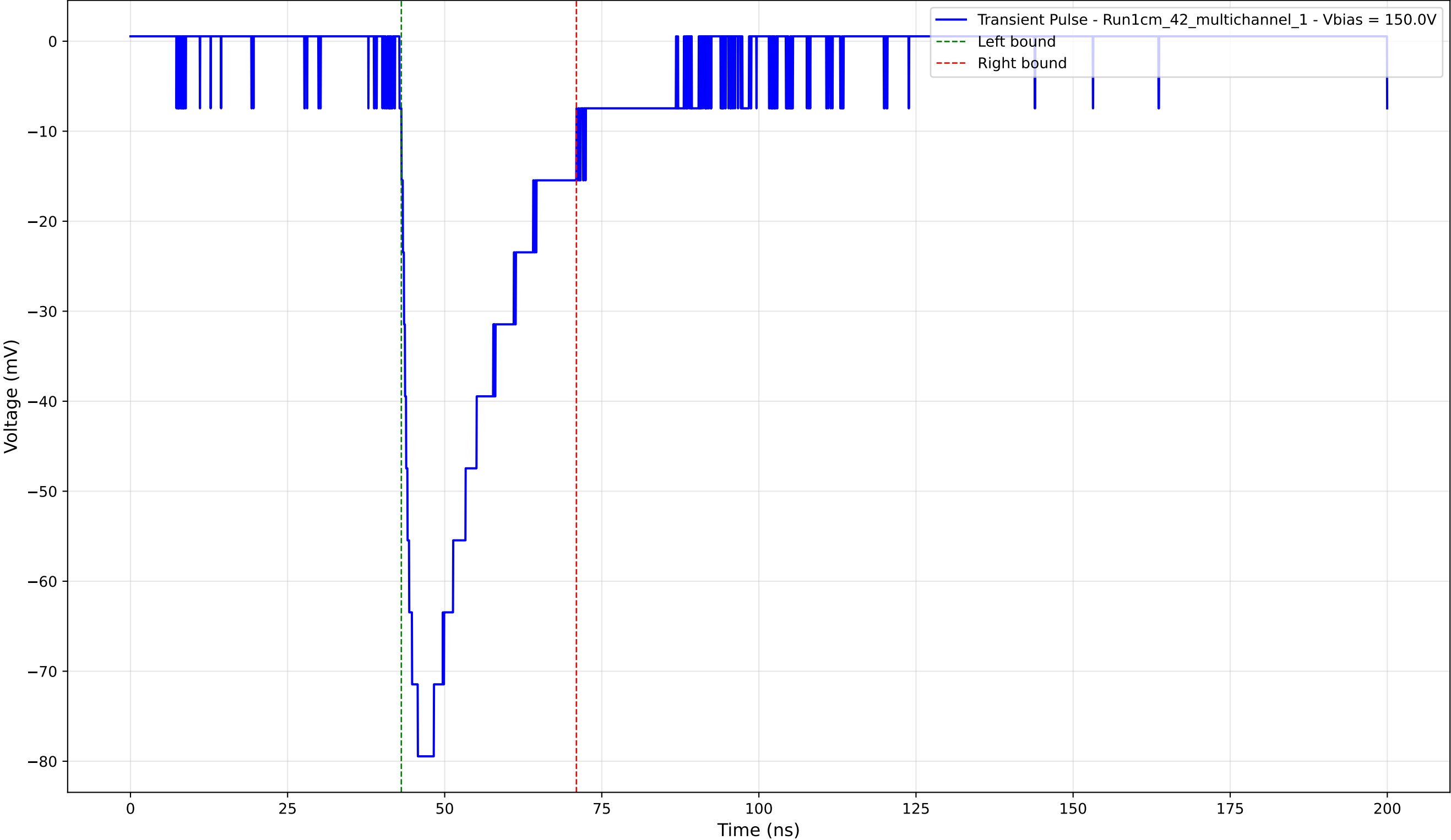
Transient Pulse - Sample: 1cm_42_multichannel - Position: 625.0 \mu\text{m} - Charge: -22.68 pC - Rise Time: 2.62 ns
