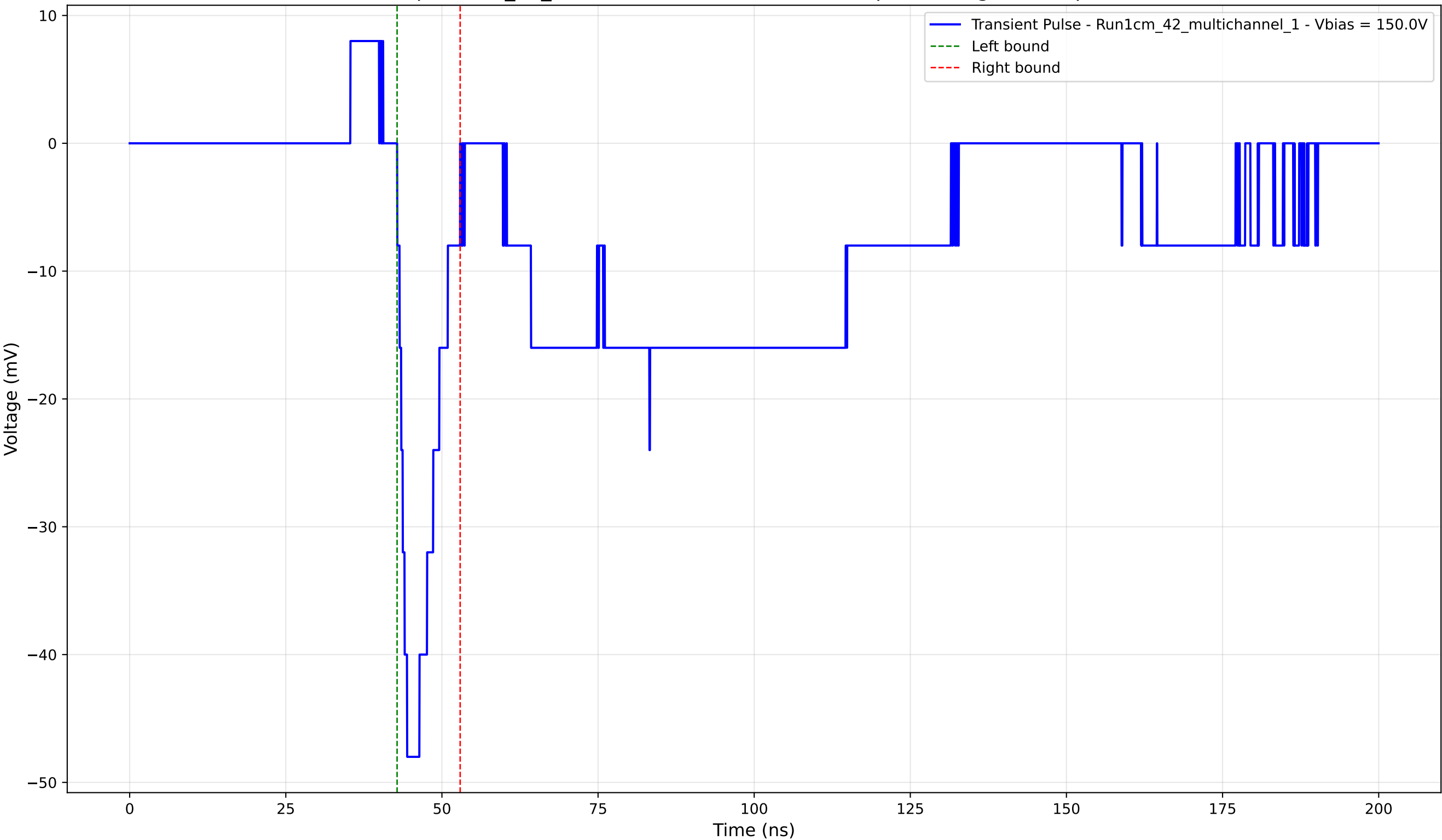
Transient Pulse - Sample: 1cm_42_multichannel - Position: 4110.0 \mu\text{m} - Charge: -5.50 pC - Rise Time: 1.59 ns
