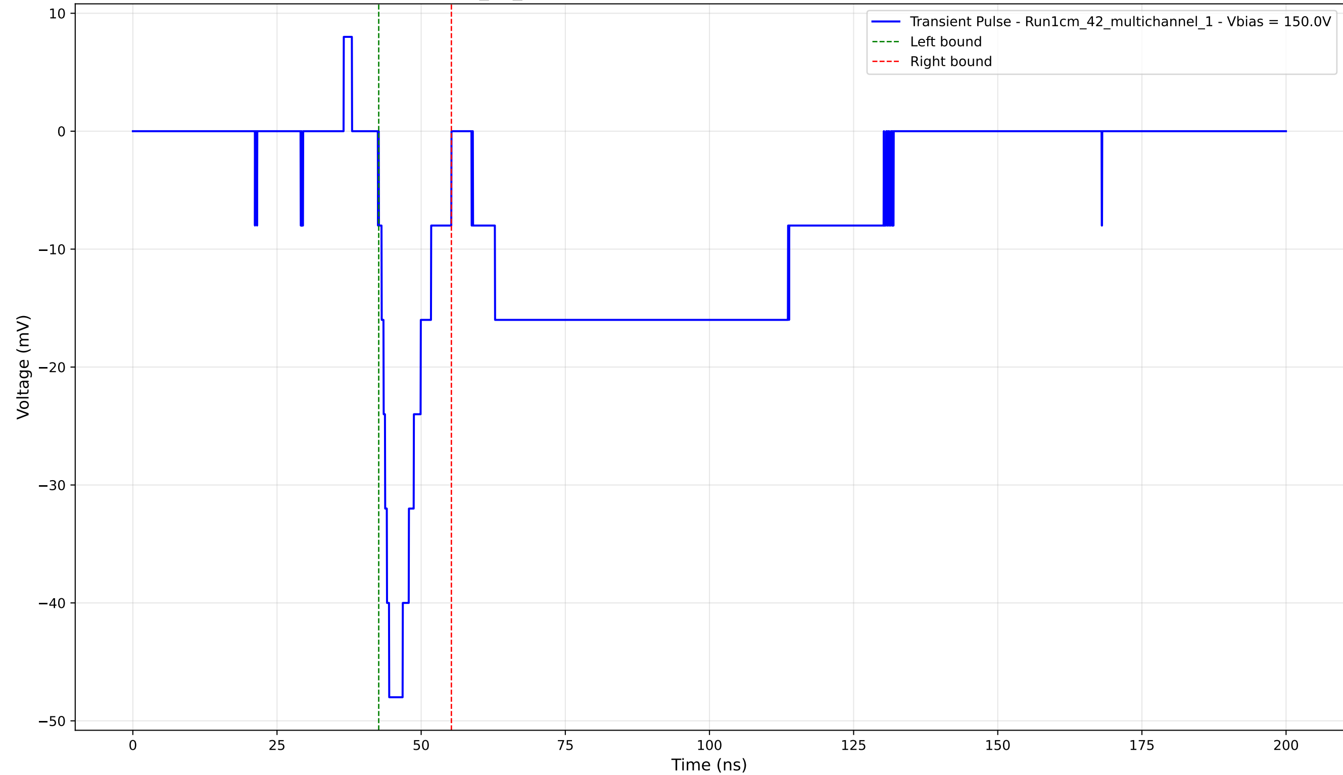
Transient Pulse - Sample: 1cm_42_multichannel - Position: 4180.0 \mu\text{m} - Charge: -6.20 pC - Rise Time: 1.79 ns
