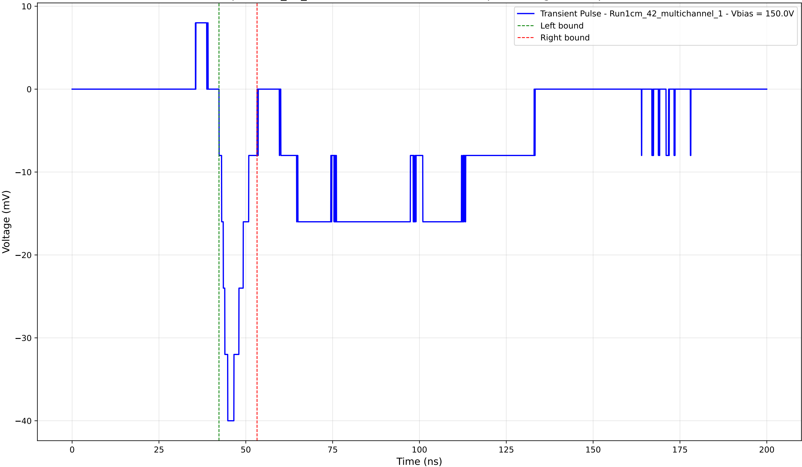
Transient Pulse - Sample: 1cm_42_multichannel - Position: 4815.0 \mu\text{m} - Charge: -4.85 pC - Rise Time: 2.51 ns
