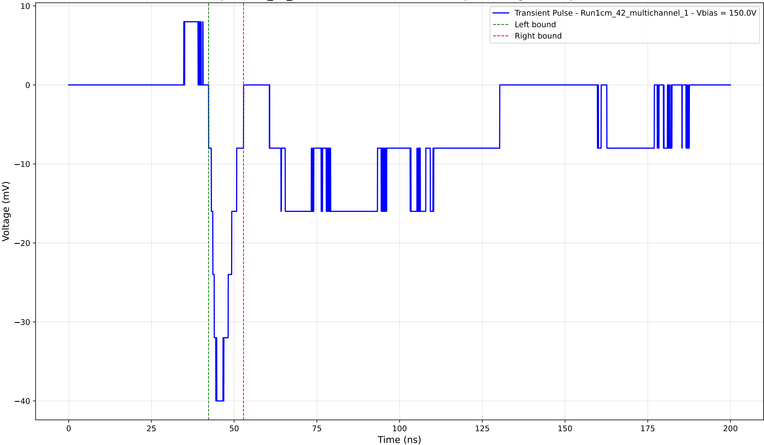
Transient Pulse - Sample: 1cm_42_multichannel - Position: 4800.0 \mu\text{m} - Charge: -4.86 pC - Rise Time: 2.19 ns
