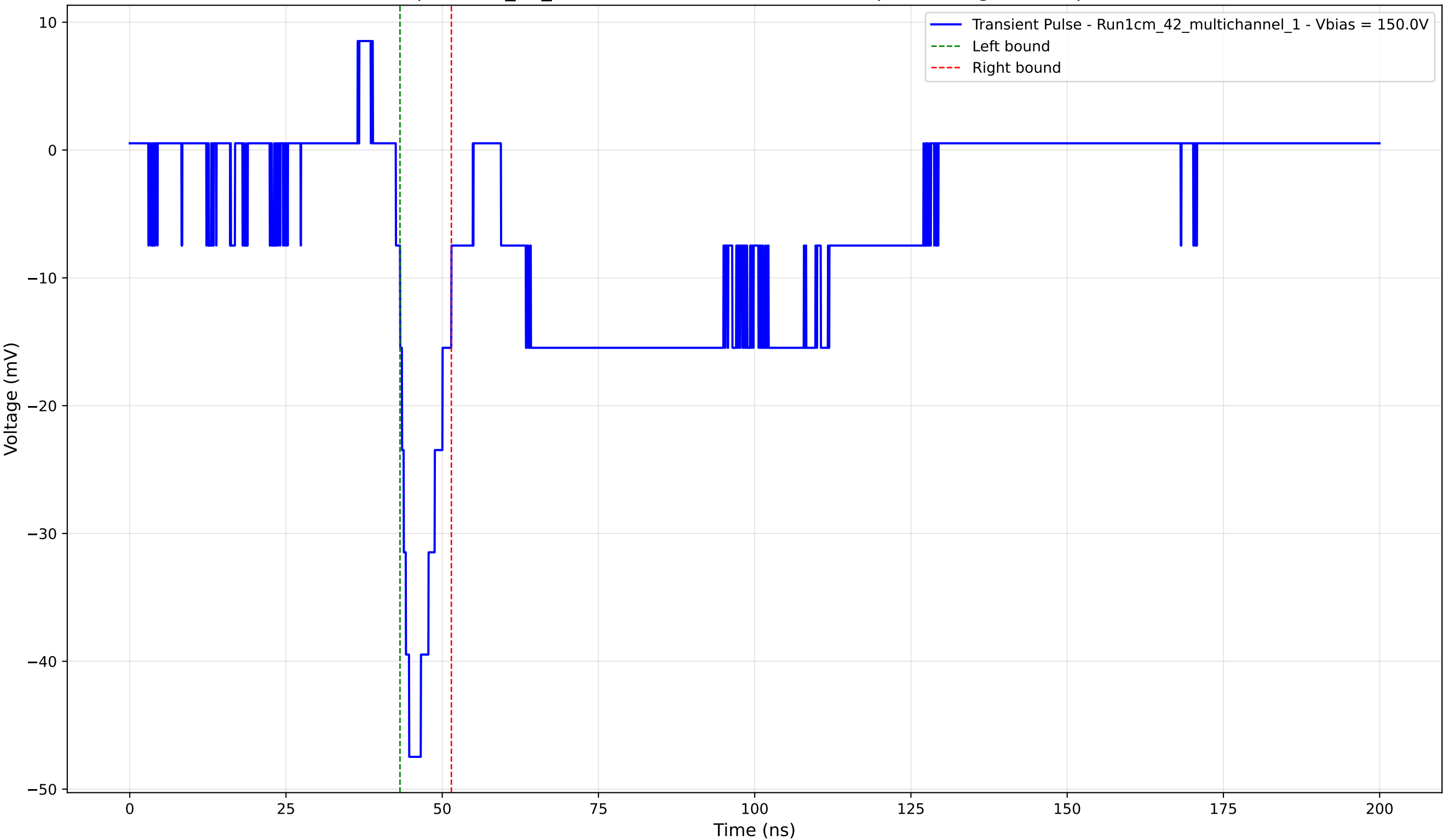
Transient Pulse - Sample: 1cm_42_multichannel - Position: 4305.0 \mu\text{m} - Charge: -5.25 pC - Rise Time: 2.13 ns
