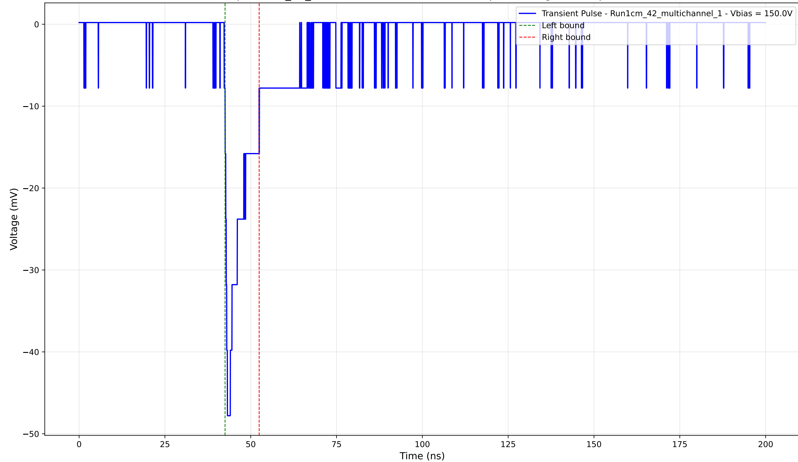
Transient Pulse - Sample: 1cm_42_multichannel - Position: 1840.0 \mu\text{m} - Charge: -4.93 pC - Rise Time: 0.95 ns
