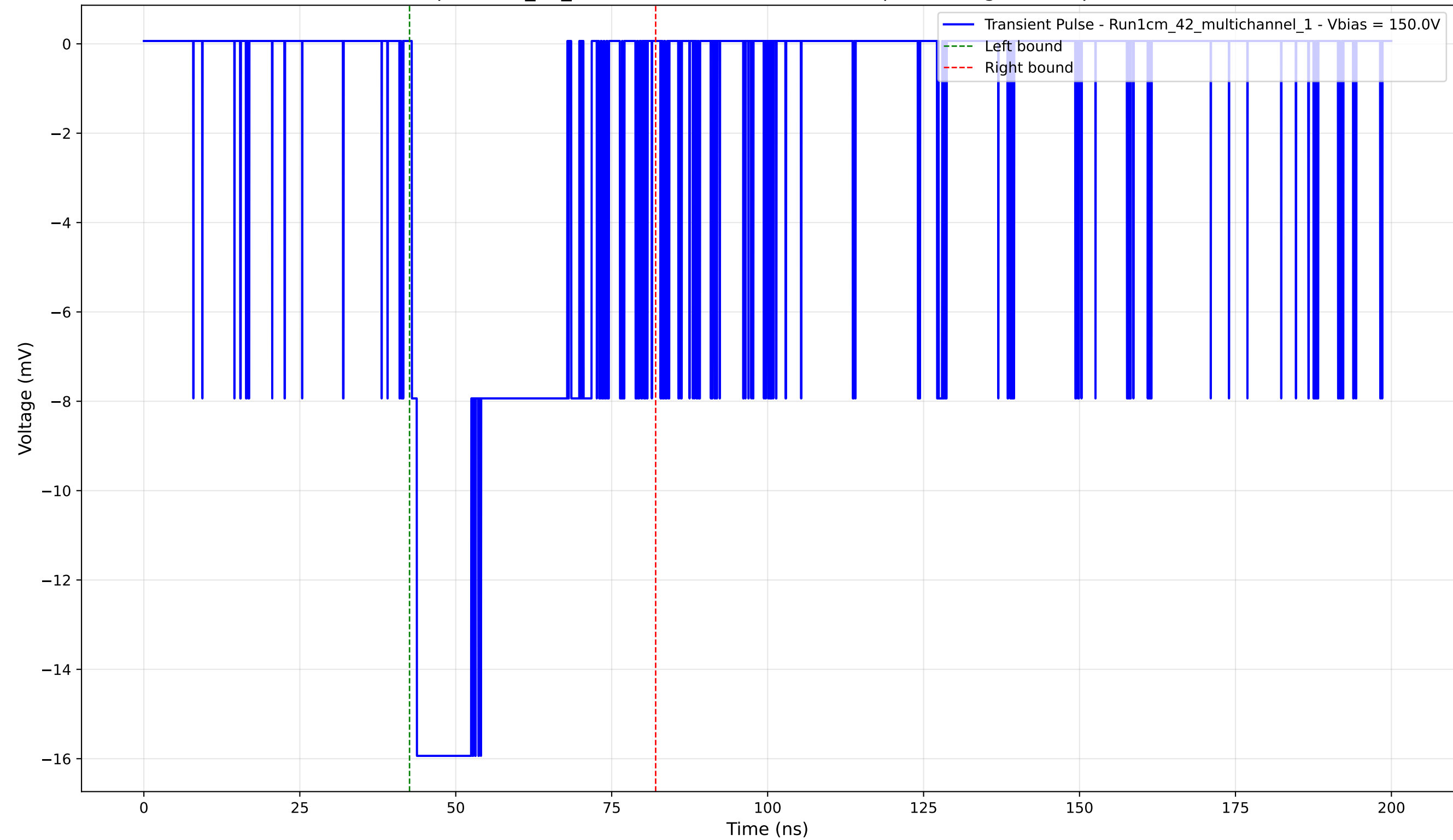
Transient Pulse - Sample: 1cm_42_multichannel - Position: 830.0 \mu\text{m} - Charge: -6.27 pC - Rise Time: 0.82 ns
