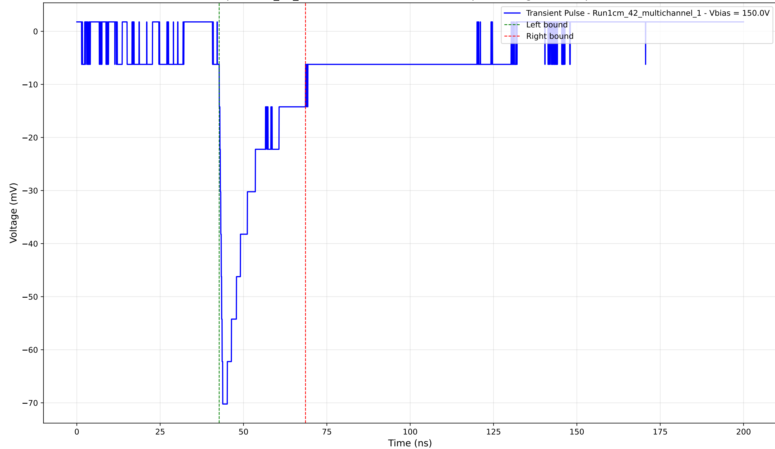
Transient Pulse - Sample: 1cm_42_multichannel - Position: 3580.0 \mu\text{m} - Charge: -15.34 pC - Rise Time: 1.06 ns
