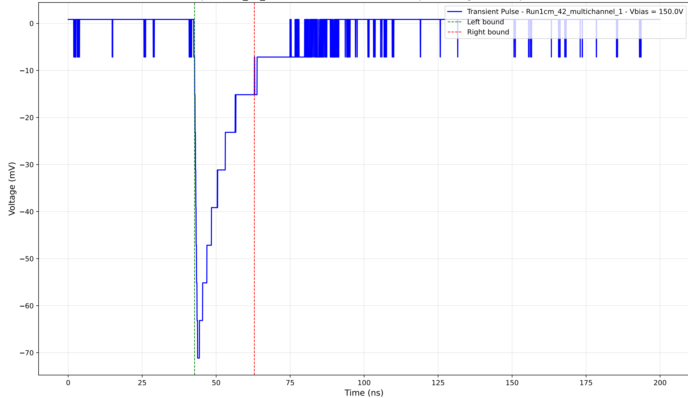
Transient Pulse - Sample: 1cm_42_multichannel - Position: 1430.0 \mu\text{m} - Charge: -12.89 pC - Rise Time: 1.28 ns
