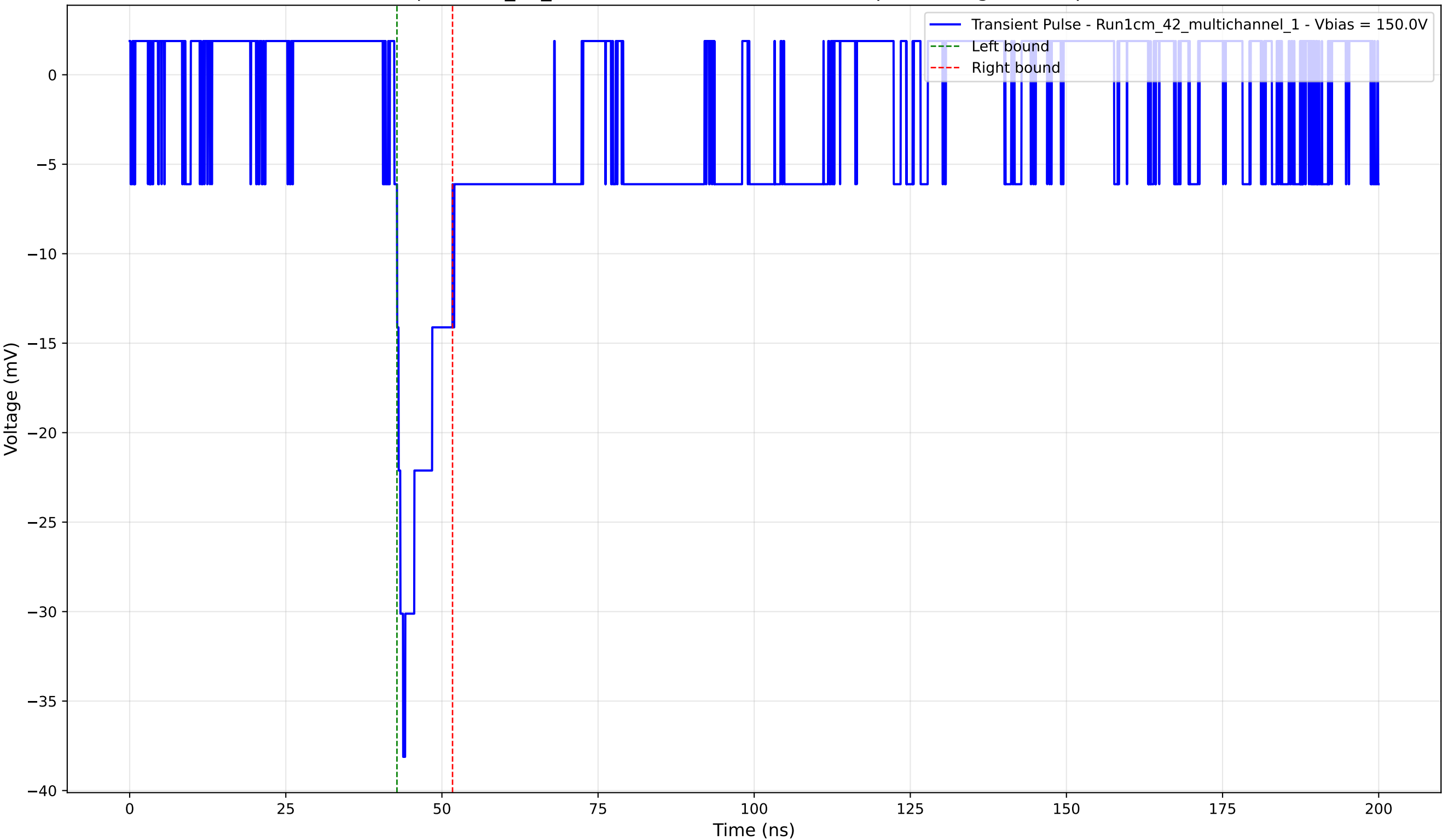
Transient Pulse - Sample: 1cm_42_multichannel - Position: 3355.0 \mu\text{m} - Charge: -3.78 pC - Rise Time: 1.41 ns
