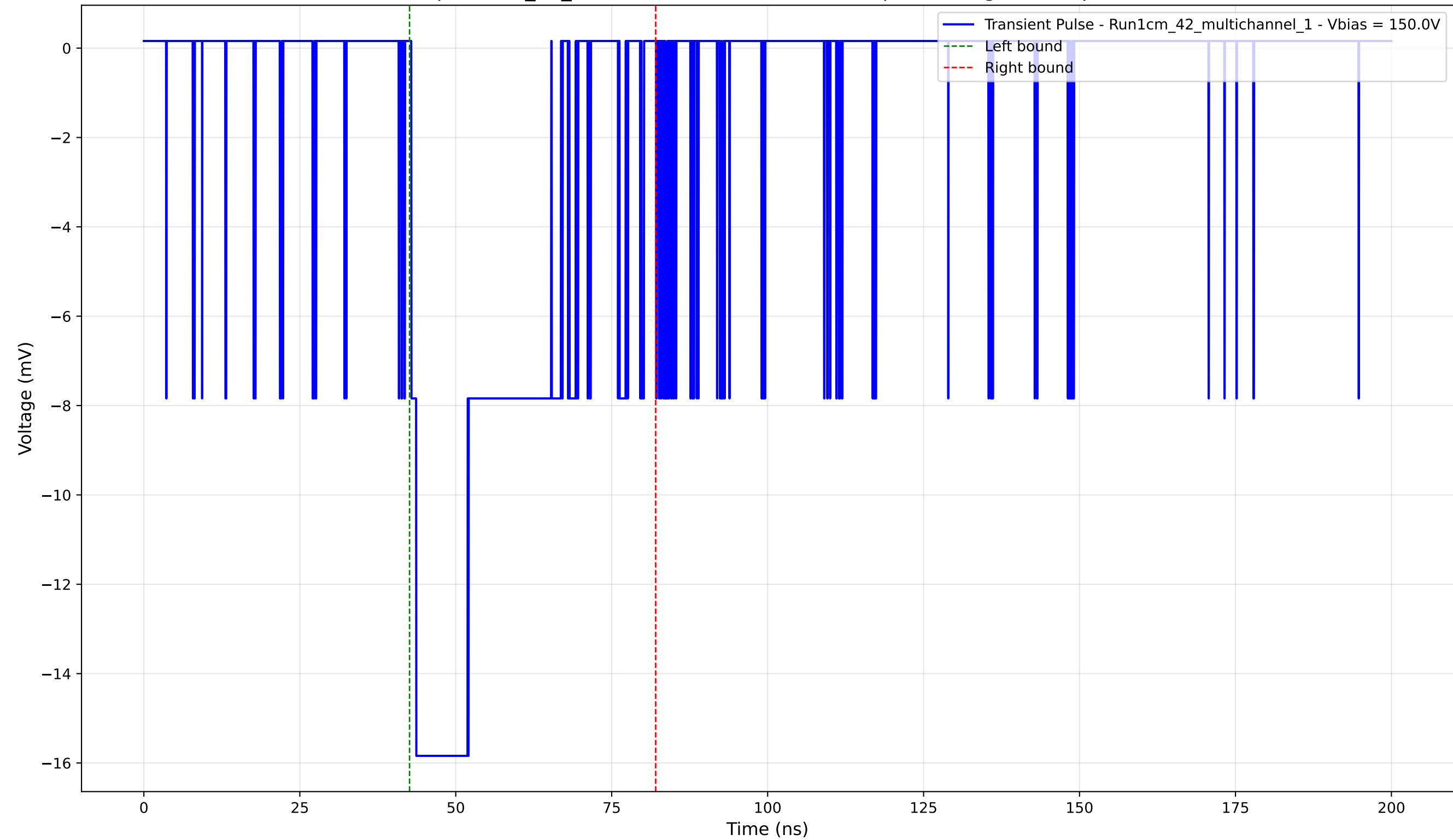
Transient Pulse - Sample: 1cm_42_multichannel - Position: 905.0 \mu\text{m} - Charge: -5.54 pC - Rise Time: 0.80 ns
