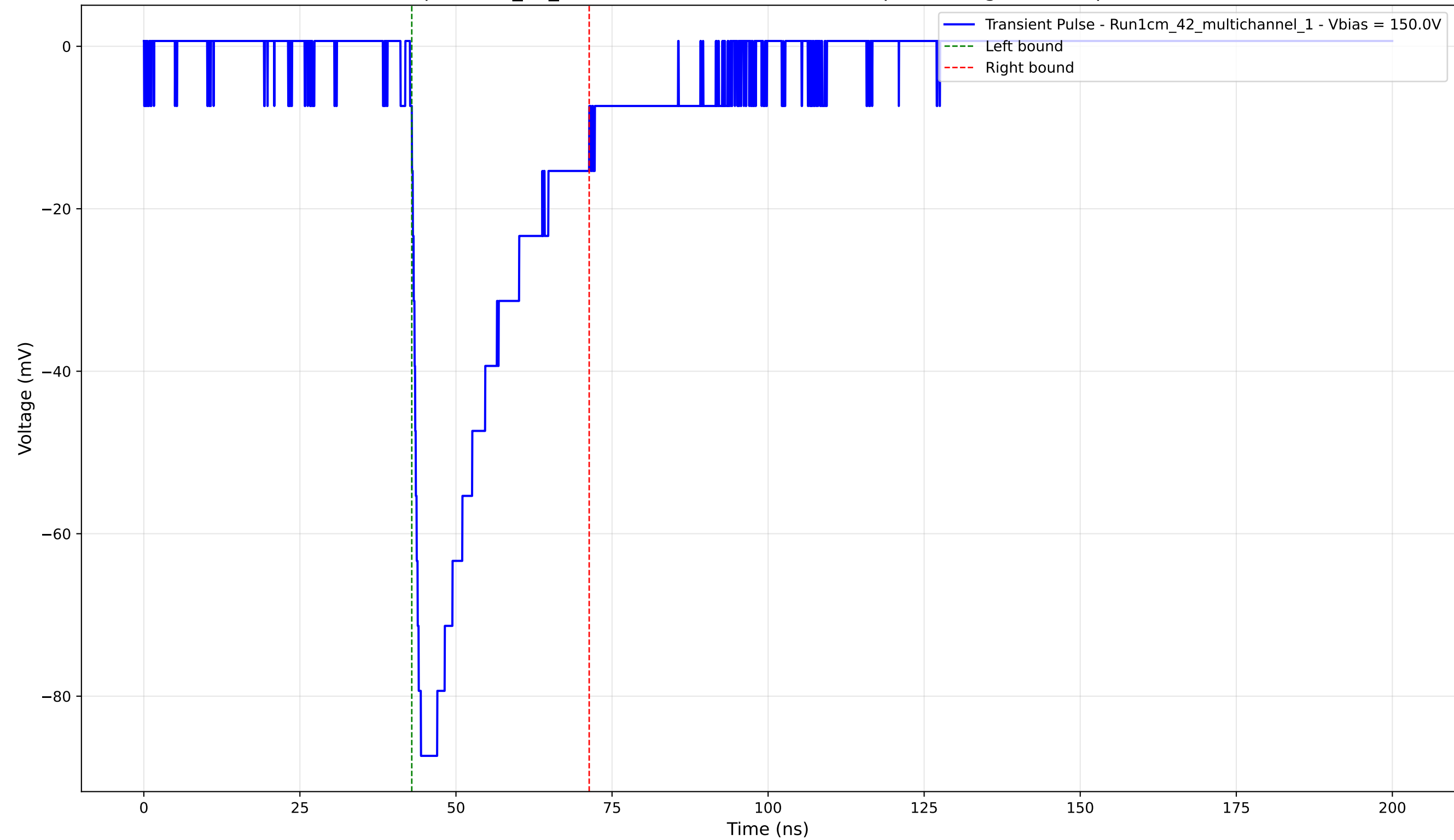
Transient Pulse - Sample: 1cm_42_multichannel - Position: 1040.0 \mu\text{m} - Charge: -23.40 pC - Rise Time: 1.10 ns
