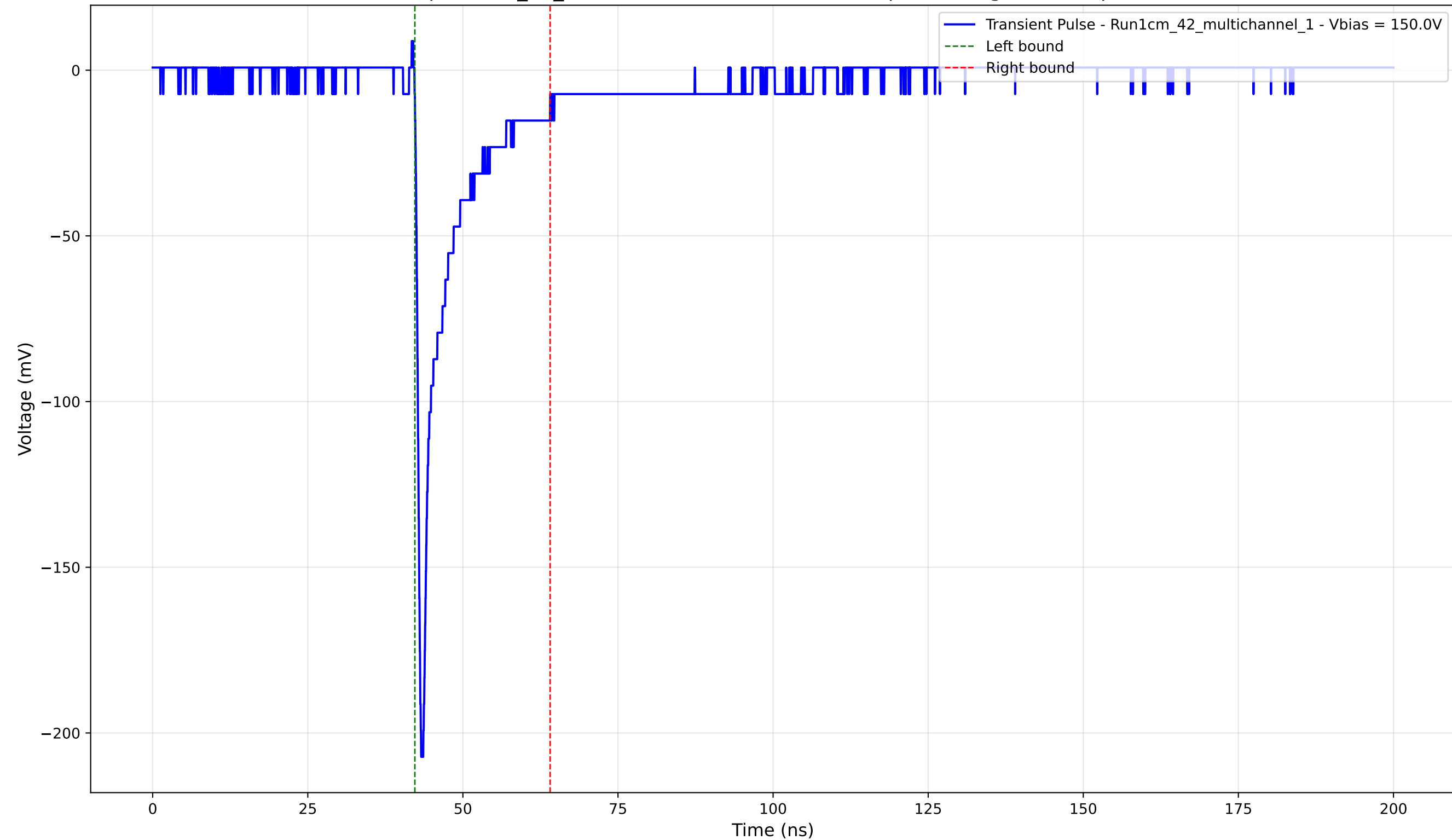
Transient Pulse - Sample: 1cm_42_multichannel - Position: 2810.0 \mu\text{m} - Charge: -20.07 pC - Rise Time: 0.81 ns
