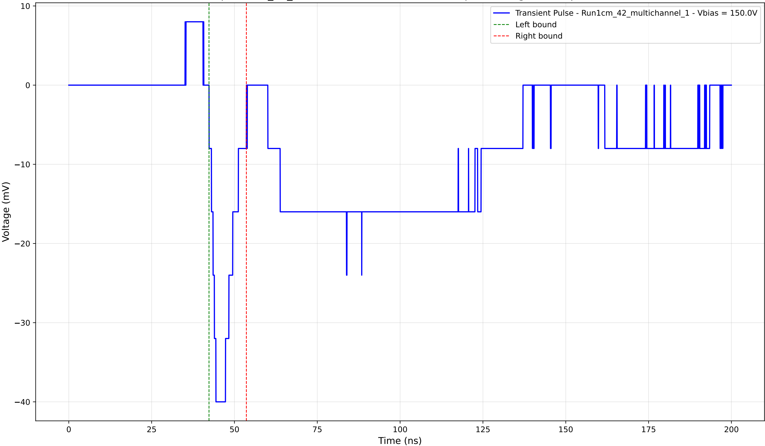
Transient Pulse - Sample: 1cm_42_multichannel - Position: 4775.0 \mu\text{m} - Charge: -5.22 pC - Rise Time: 2.07 ns
