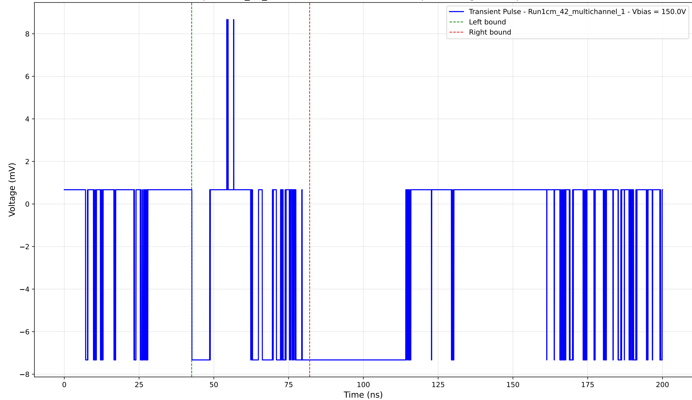
Transient Pulse - Sample: 1cm_42_multichannel - Position: 3930.0 \mu\text{m} - Charge: -2.59 pC - Rise Time: 0.02 ns
