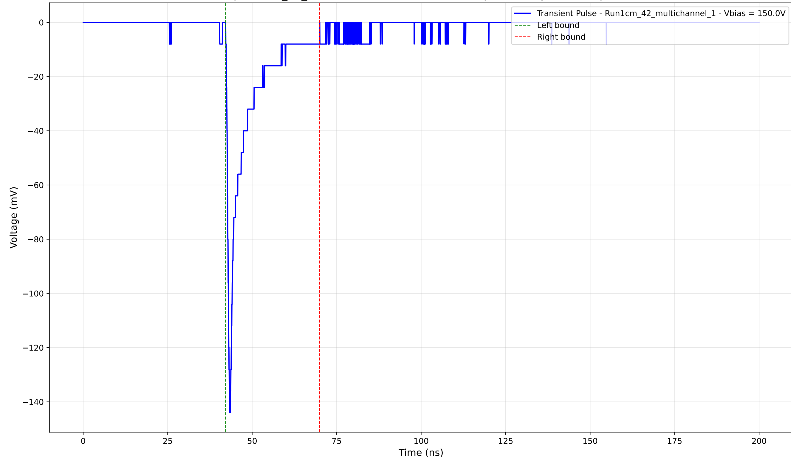
Transient Pulse - Sample: 1cm_42_multichannel - Position: 2835.0 \mu\text{m} - Charge: -14.81 pC - Rise Time: 0.90 ns
