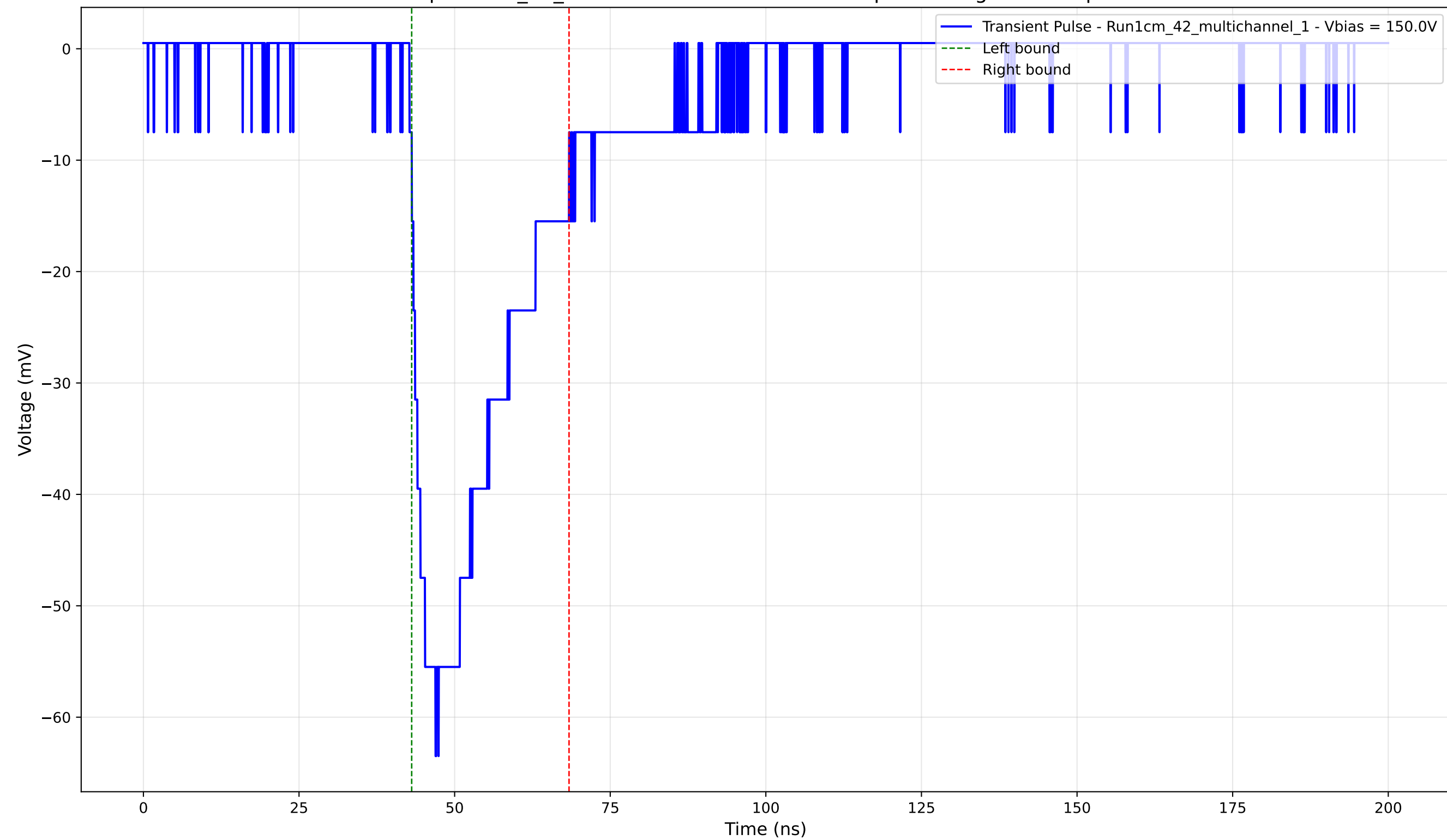
Transient Pulse - Sample: 1cm_42_multichannel - Position: 285.0 \mu\text{m} - Charge: -17.43 pC - Rise Time: 4.18 ns
