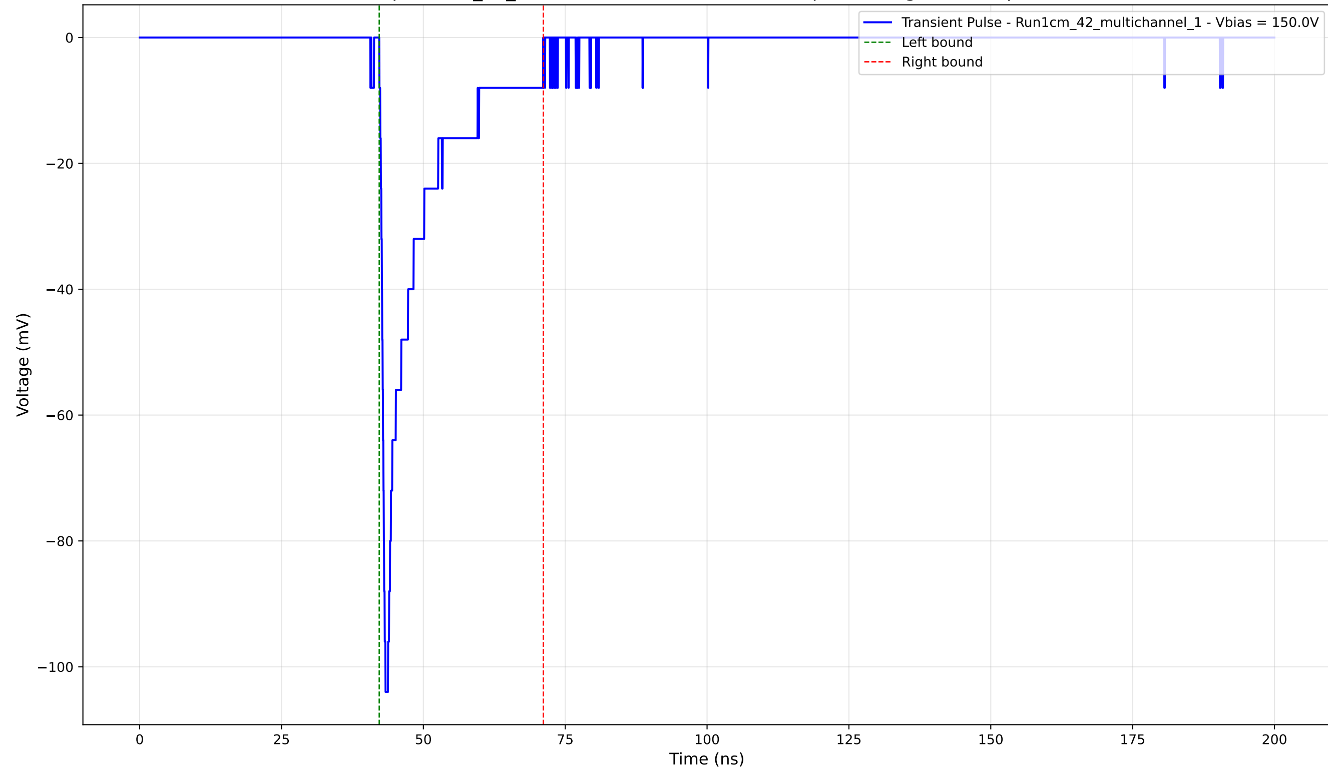
Transient Pulse - Sample: 1cm_42_multichannel - Position: 2950.0 \mu\text{m} - Charge: -13.57 pC - Rise Time: 0.79 ns
