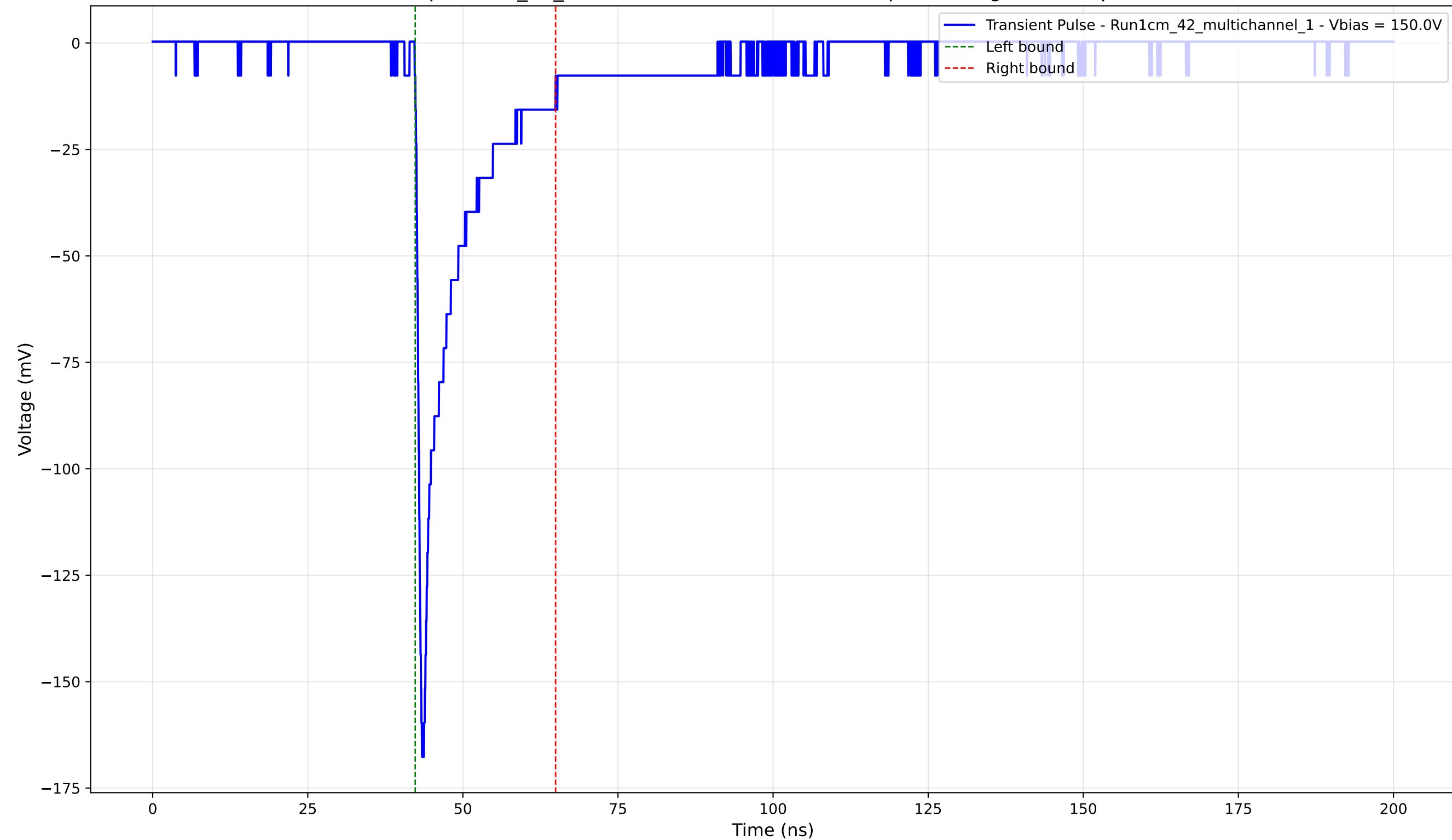
Transient Pulse - Sample: 1cm_42_multichannel - Position: 2990.0 \mu\text{m} - Charge: -20.27 pC - Rise Time: 0.82 ns
