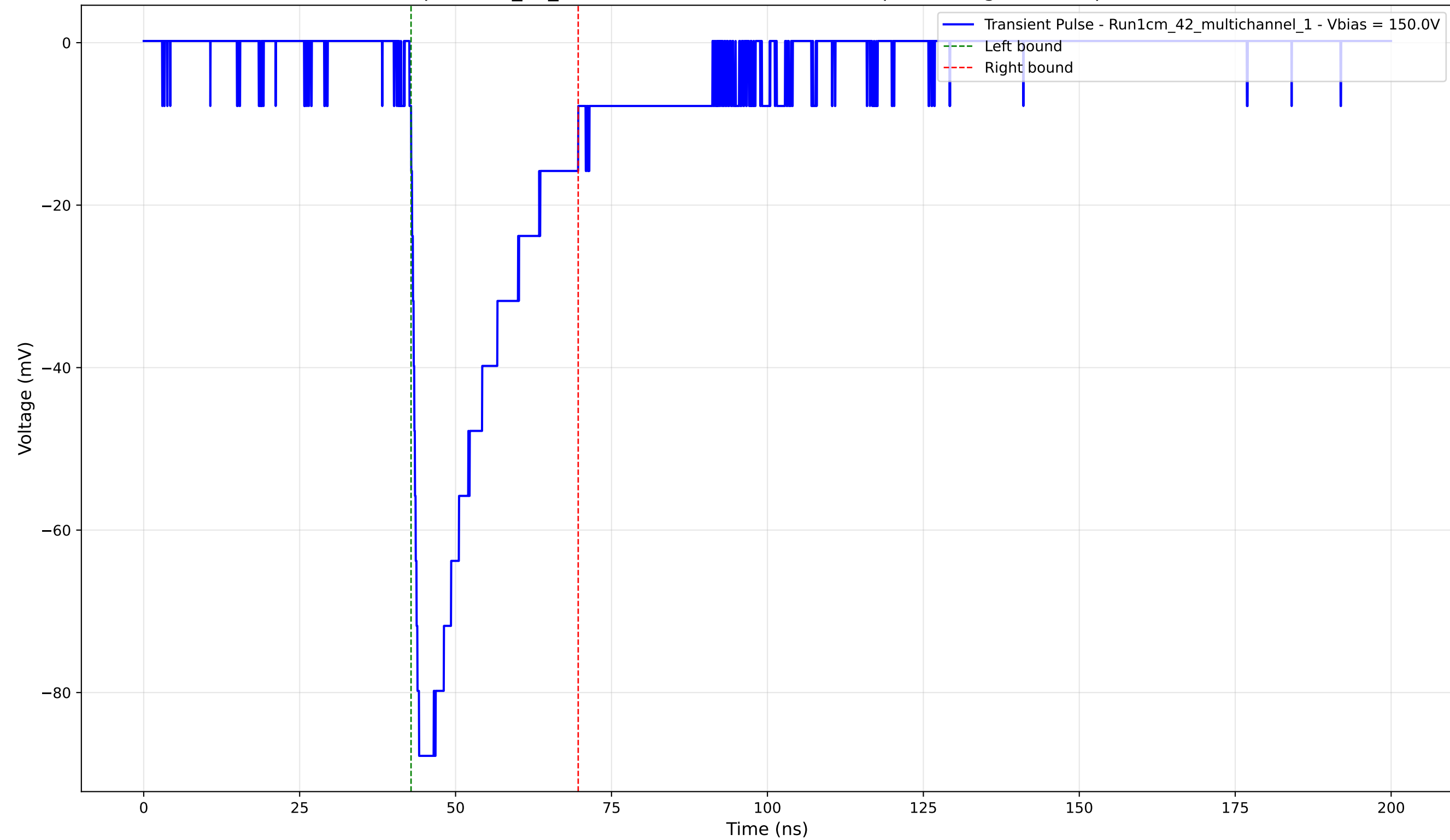
Transient Pulse - Sample: 1cm_42_multichannel - Position: 1110.0 \mu\text{m} - Charge: -22.82 pC - Rise Time: 1.02 ns
