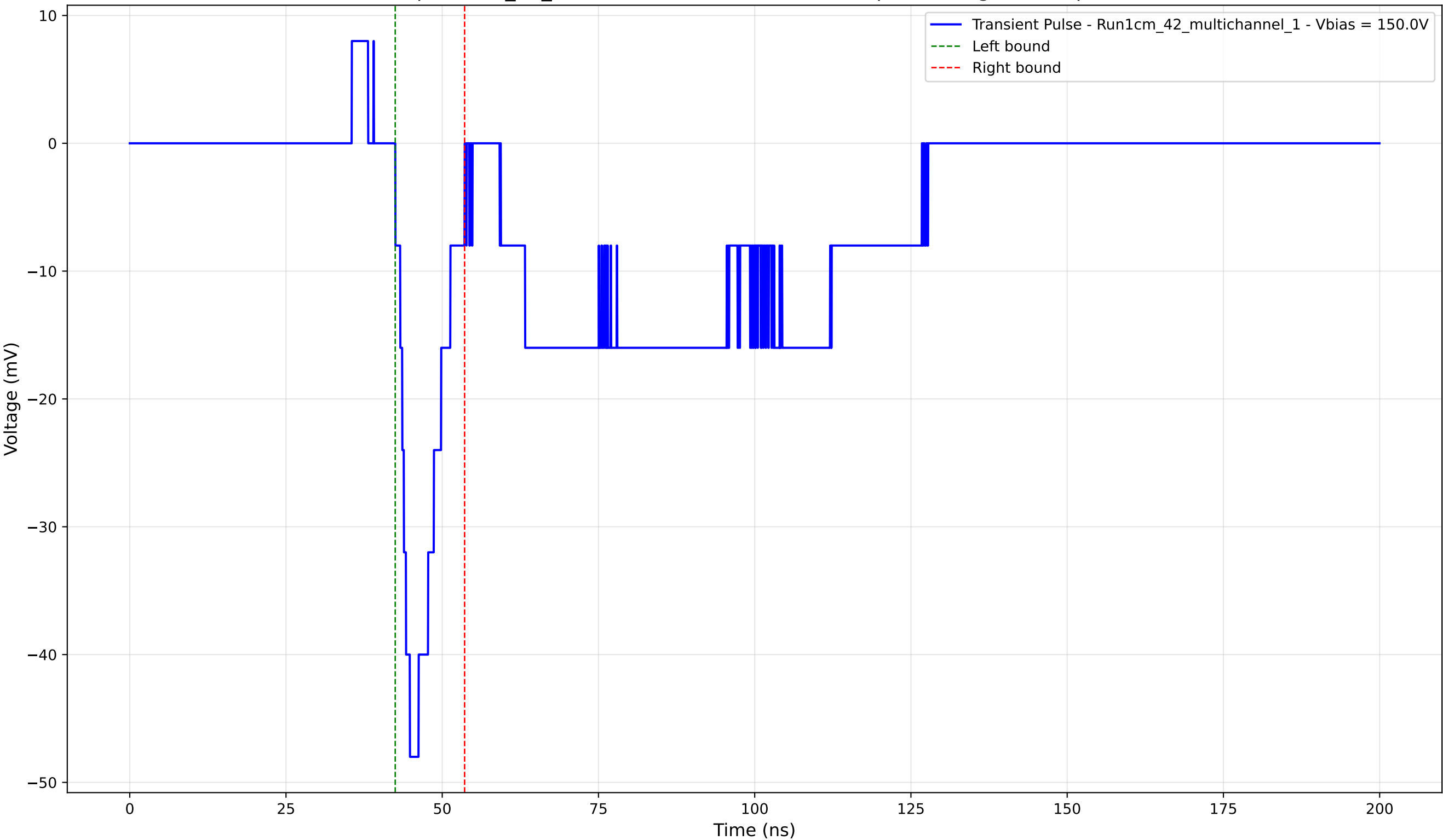
Transient Pulse - Sample: 1cm_42_multichannel - Position: 4300.0 \mu\text{m} - Charge: -5.61 pC - Rise Time: 2.33 ns
