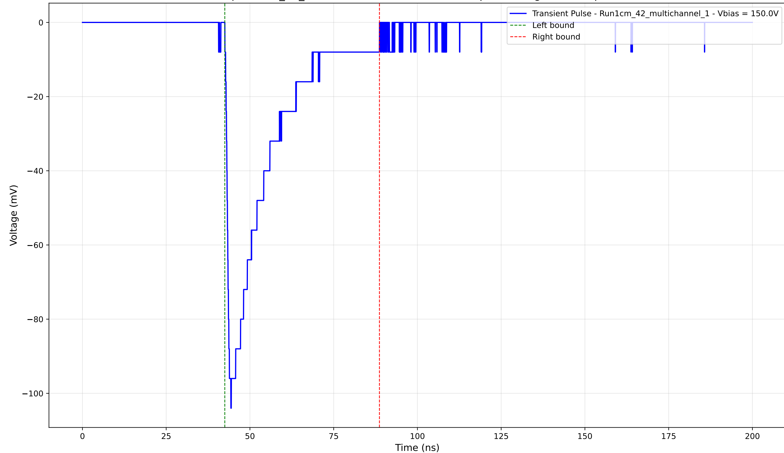
Transient Pulse - Sample: 1cm_42_multichannel - Position: 1245.0 \mu\text{m} - Charge: -26.34 pC - Rise Time: 1.13 ns
