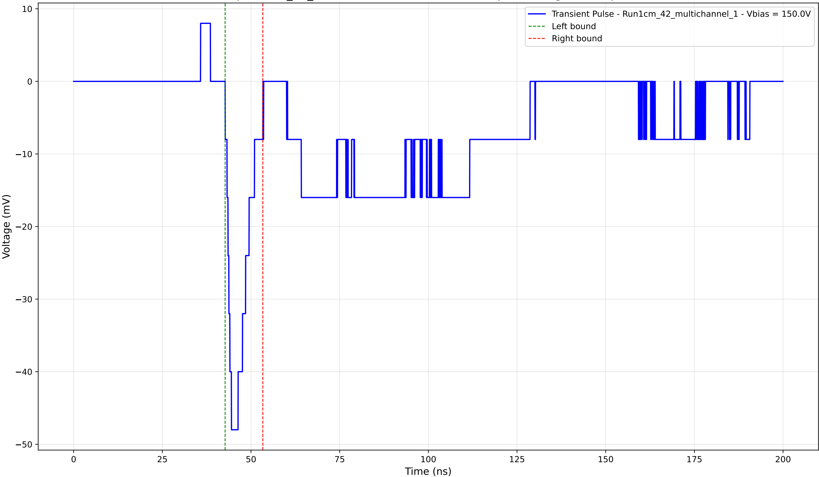
Transient Pulse - Sample: 1cm_42_multichannel - Position: 4100.0 \mu\text{m} - Charge: -5.51 pC - Rise Time: 1.77 ns
