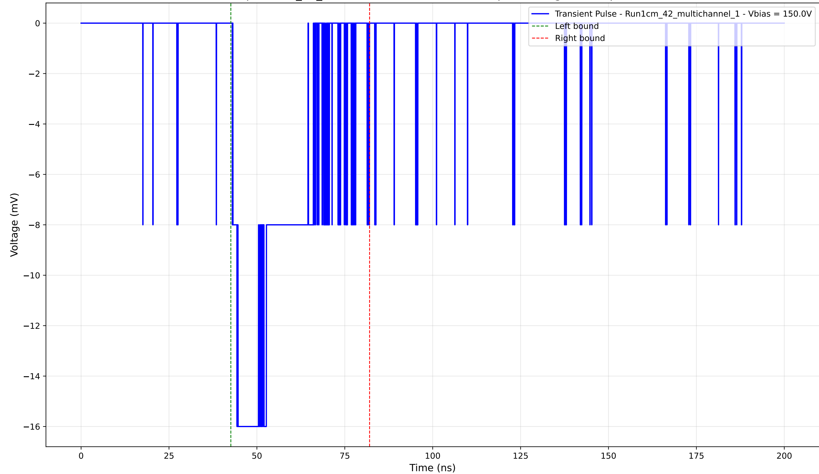
Transient Pulse - Sample: 1cm_42_multichannel - Position: 395.0 \mu\text{m} - Charge: -5.40 pC - Rise Time: 1.20 ns
