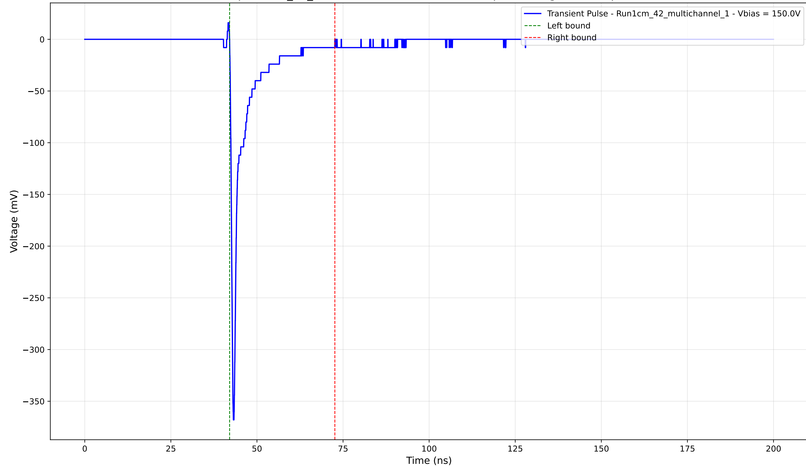
Transient Pulse - Sample: 1cm_42_multichannel - Position: 2215.0 \mu\text{m} - Charge: -26.43 pC - Rise Time: 0.74 ns
