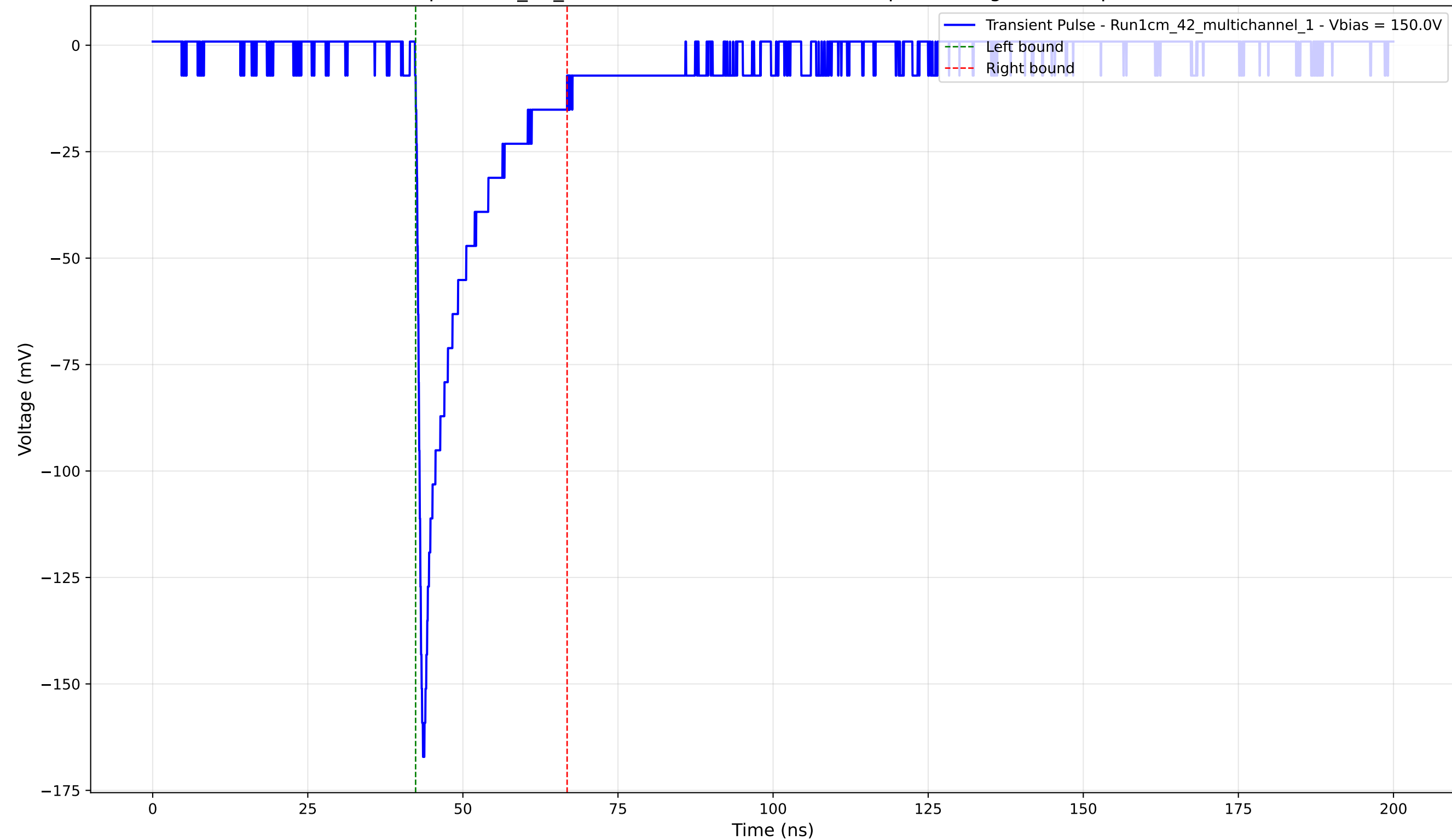
Transient Pulse - Sample: 1cm_42_multichannel - Position: 1705.0 \mu\text{m} - Charge: -22.80 pC - Rise Time: 0.86 ns
