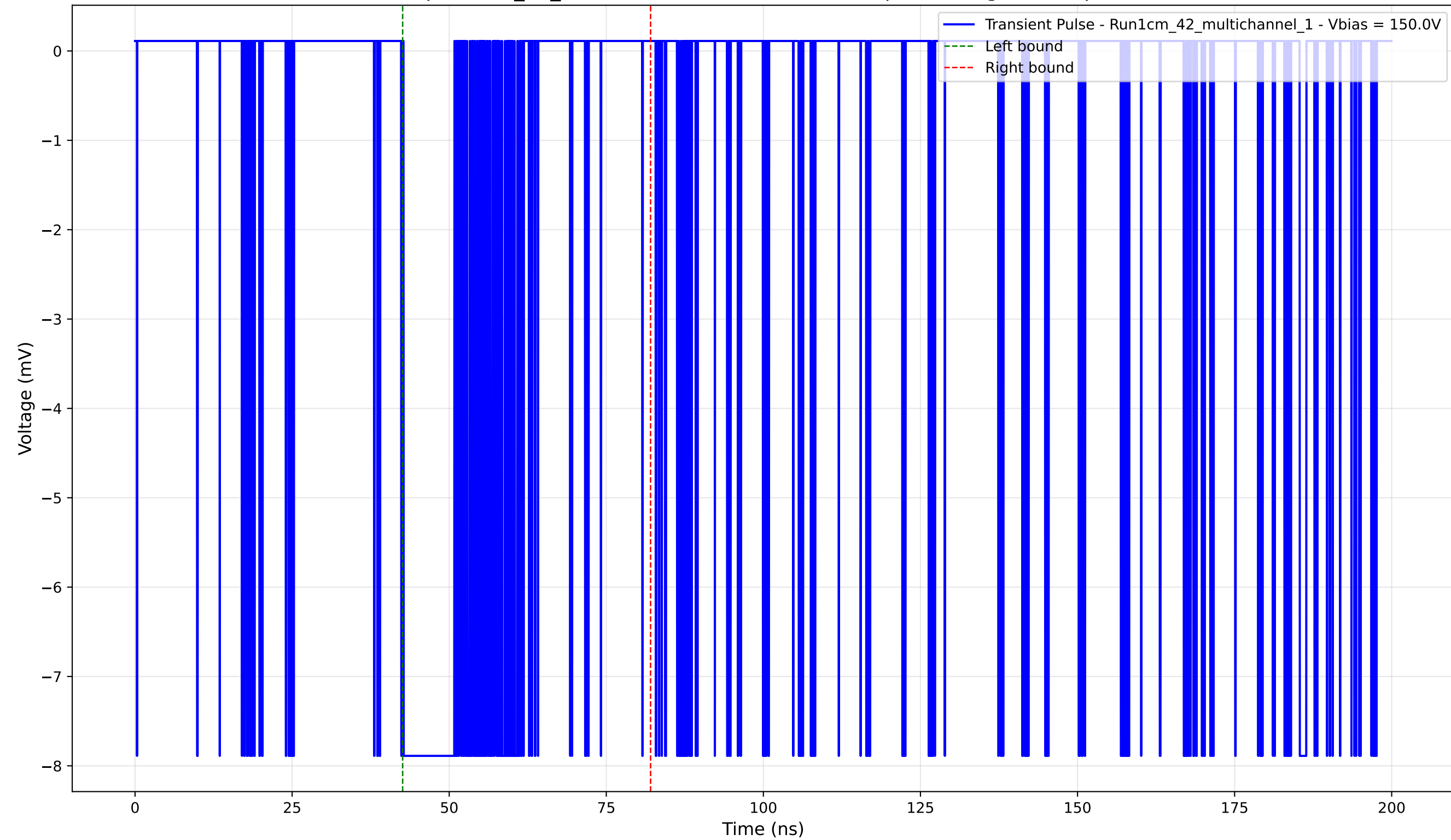
Transient Pulse - Sample: 1cm_42_multichannel - Position: 1380.0 \mu\text{m} - Charge: -2.41 pC - Rise Time: 0.02 ns
