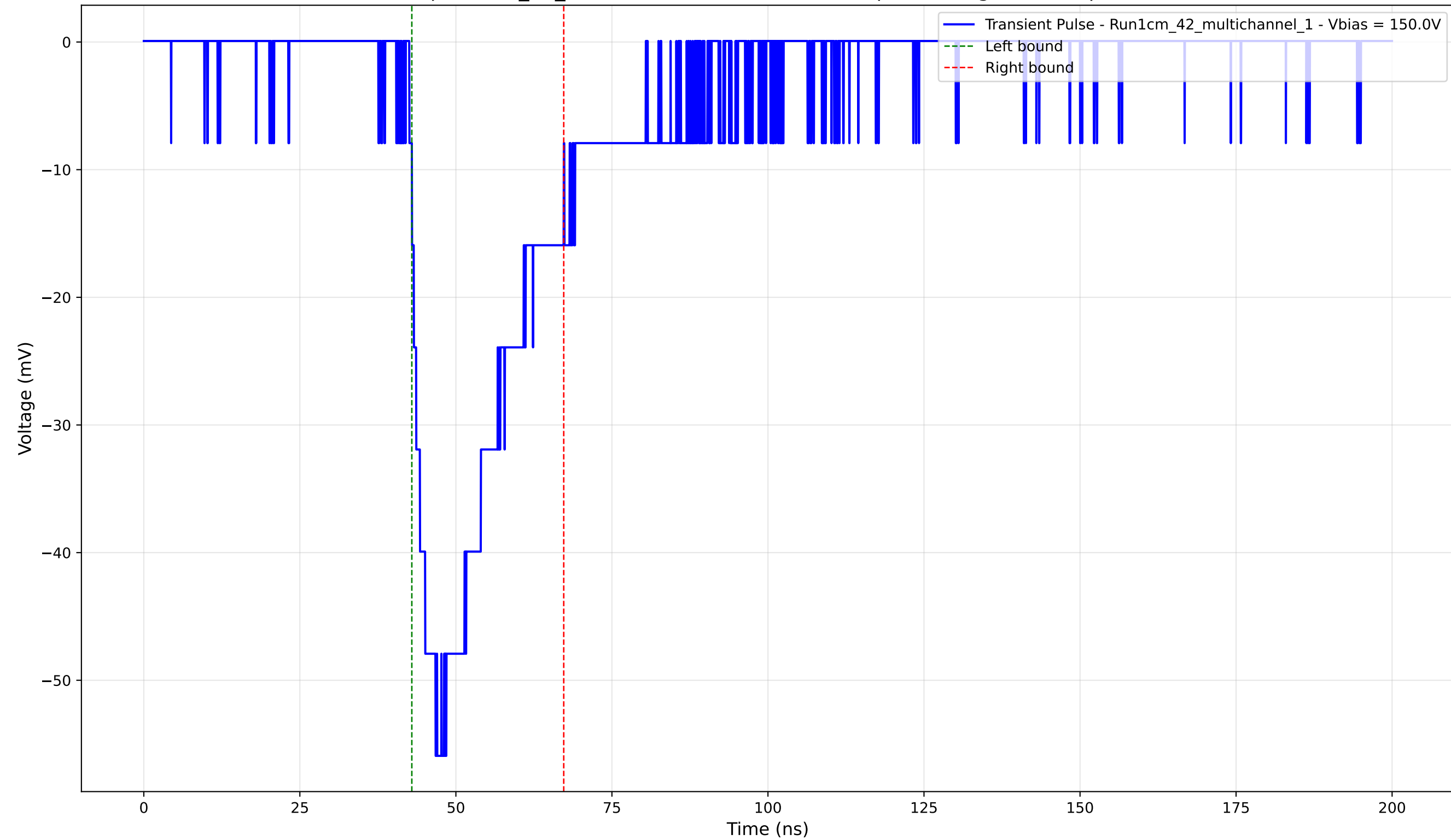
Transient Pulse - Sample: 1cm_42_multichannel - Position: 105.0 \mu\text{m} - Charge: -15.57 pC - Rise Time: 4.21 ns
