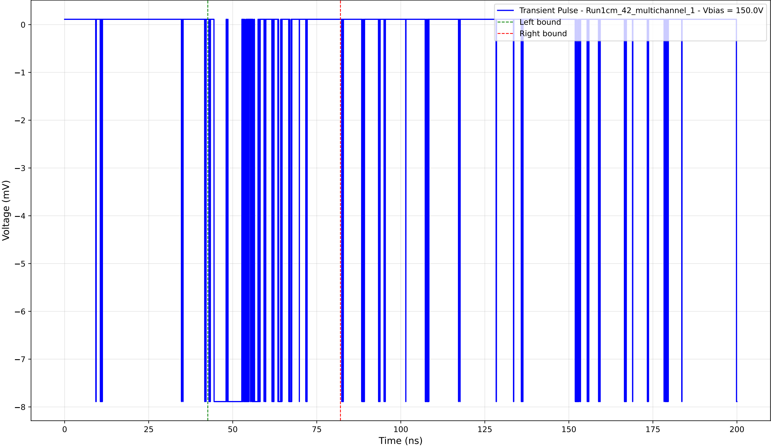
Transient Pulse - Sample: 1cm_42_multichannel - Position: 370.0 \mu\text{m} - Charge: -2.10 pC - Rise Time: 0.02 ns
