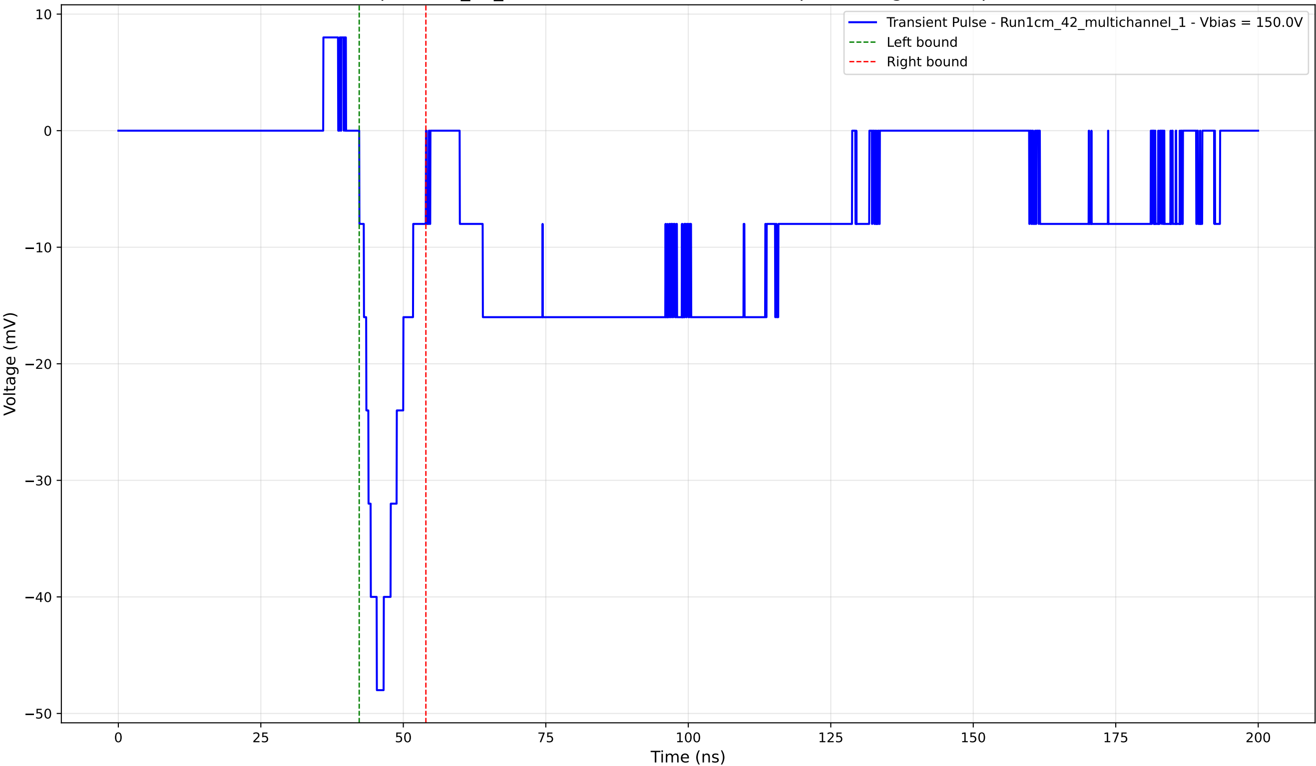
Transient Pulse - Sample: 1cm_42_multichannel - Position: 4655.0 \mu\text{m} - Charge: -5.84 pC - Rise Time: 3.07 ns
