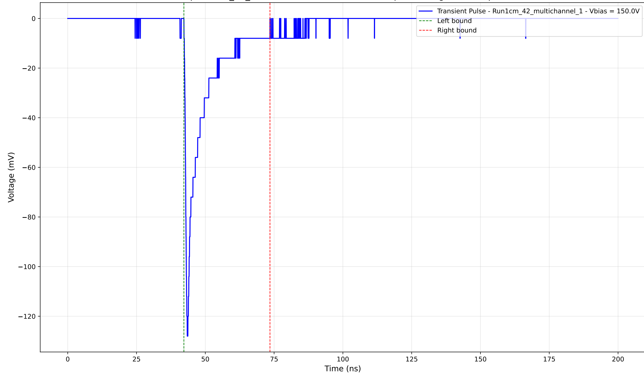
Transient Pulse - Sample: 1cm_42_multichannel - Position: 2955.0 \mu\text{m} - Charge: -16.23 pC - Rise Time: 0.91 ns
