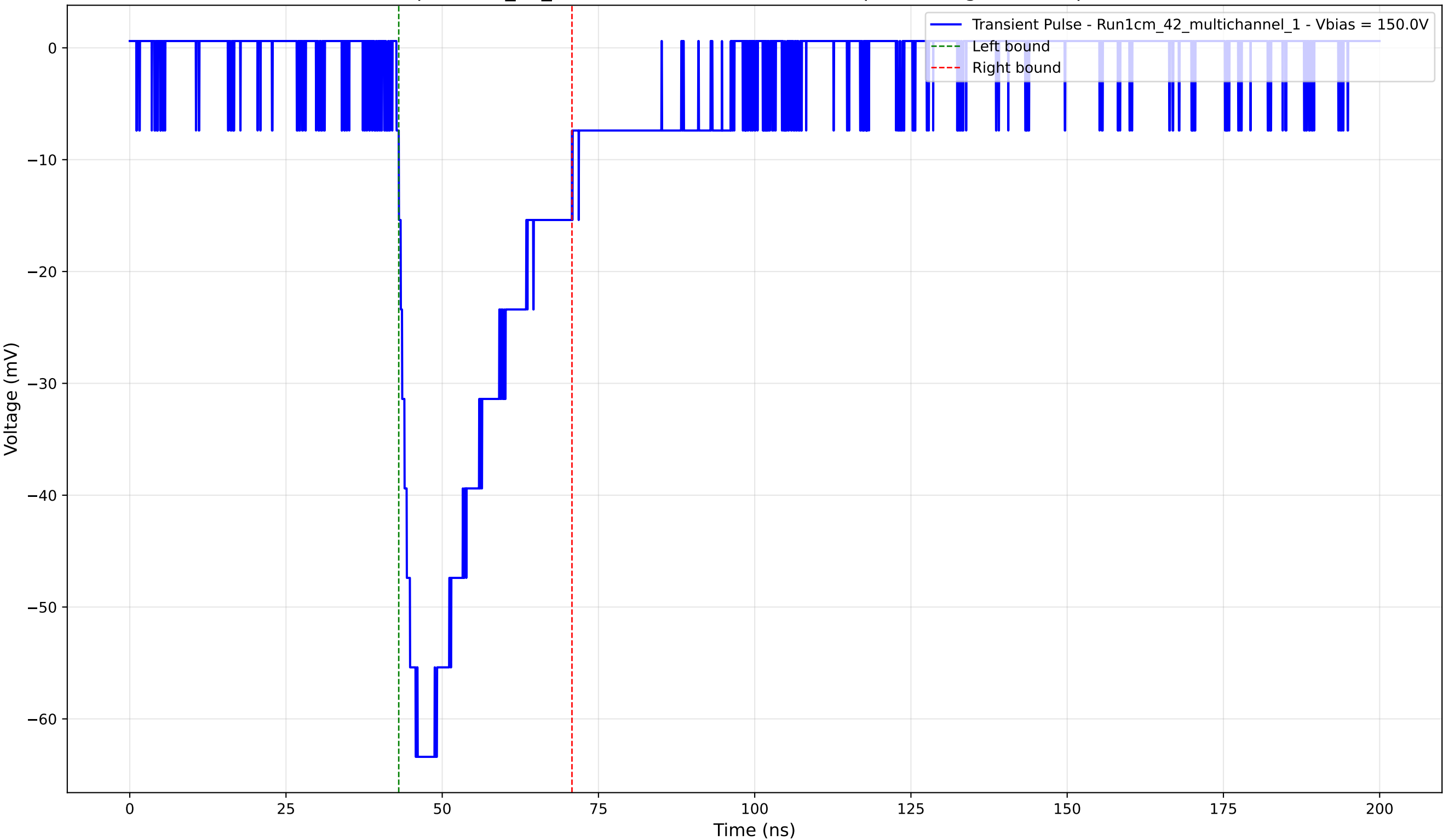
Transient Pulse - Sample: 1cm_42_multichannel - Position: 280.0 \mu\text{m} - Charge: -19.31 pC - Rise Time: 3.06 ns
