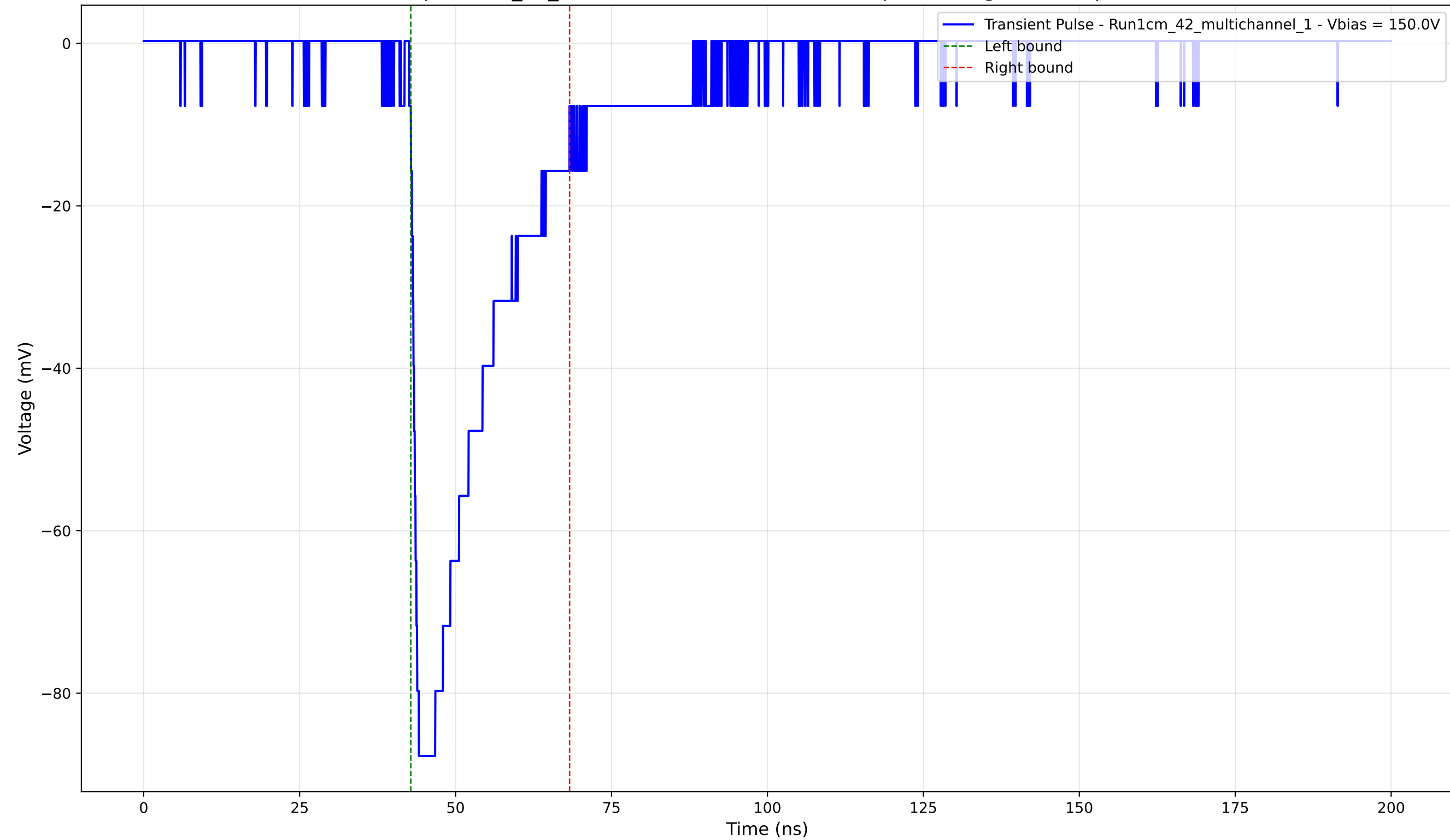
Transient Pulse - Sample: 1cm_42_multichannel - Position: 1135.0 \mu\text{m} - Charge: -22.30 pC - Rise Time: 1.02 ns
