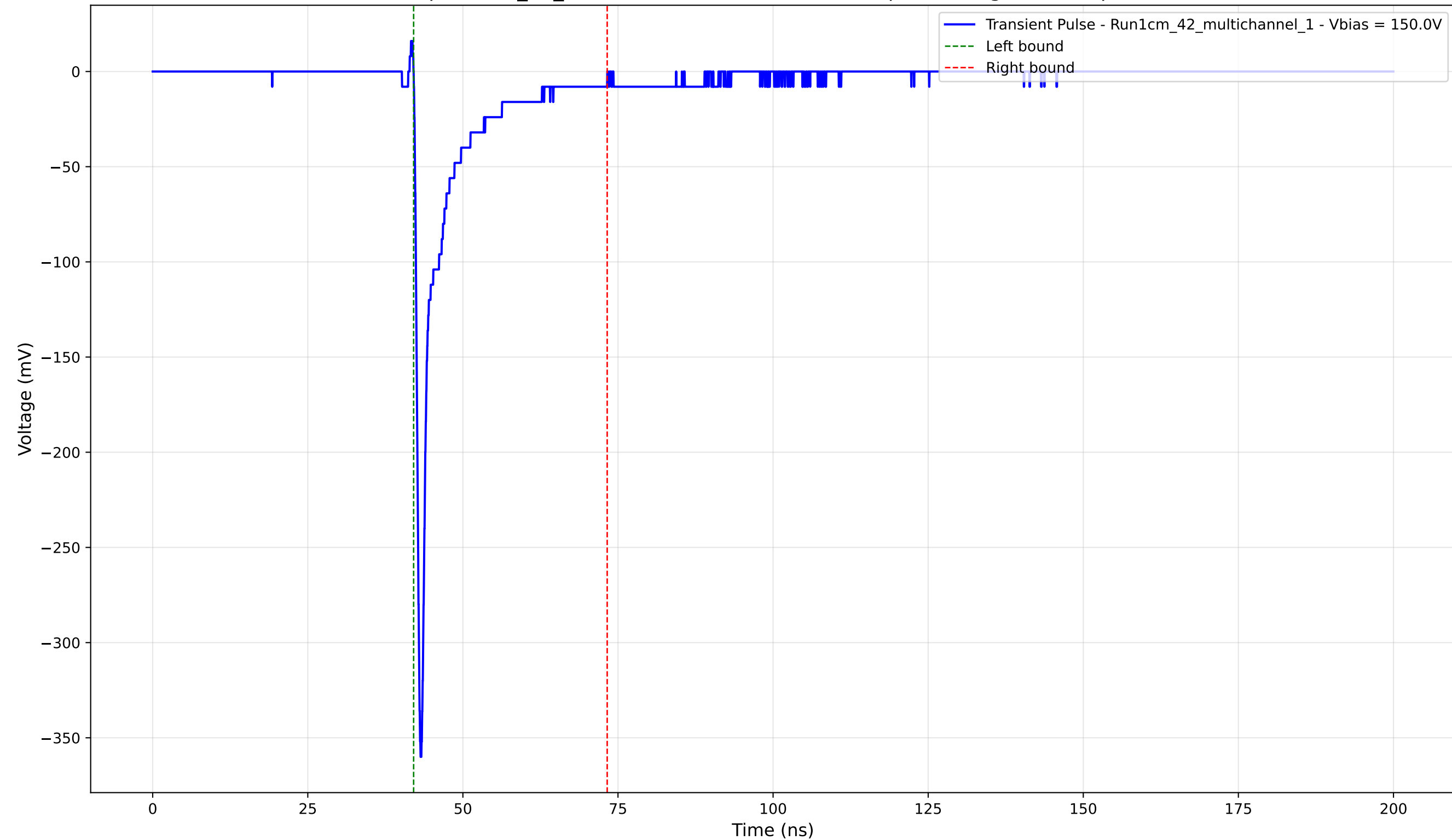
Transient Pulse - Sample: 1cm_42_multichannel - Position: 2200.0 \mu\text{m} - Charge: -26.31 pC - Rise Time: 0.76 ns
