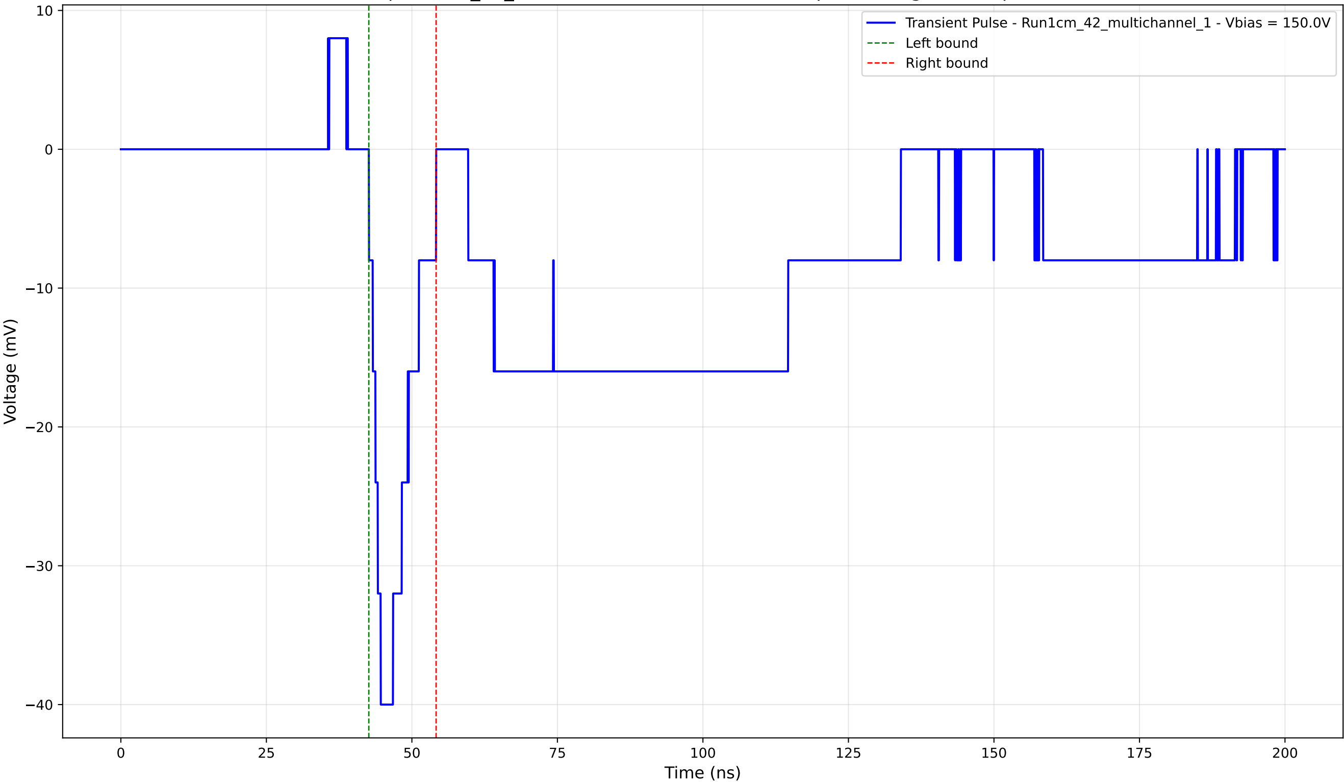
Transient Pulse - Sample: 1cm_42_multichannel - Position: 4475.0 \mu\text{m} - Charge: -5.00 pC - Rise Time: 2.03 ns
