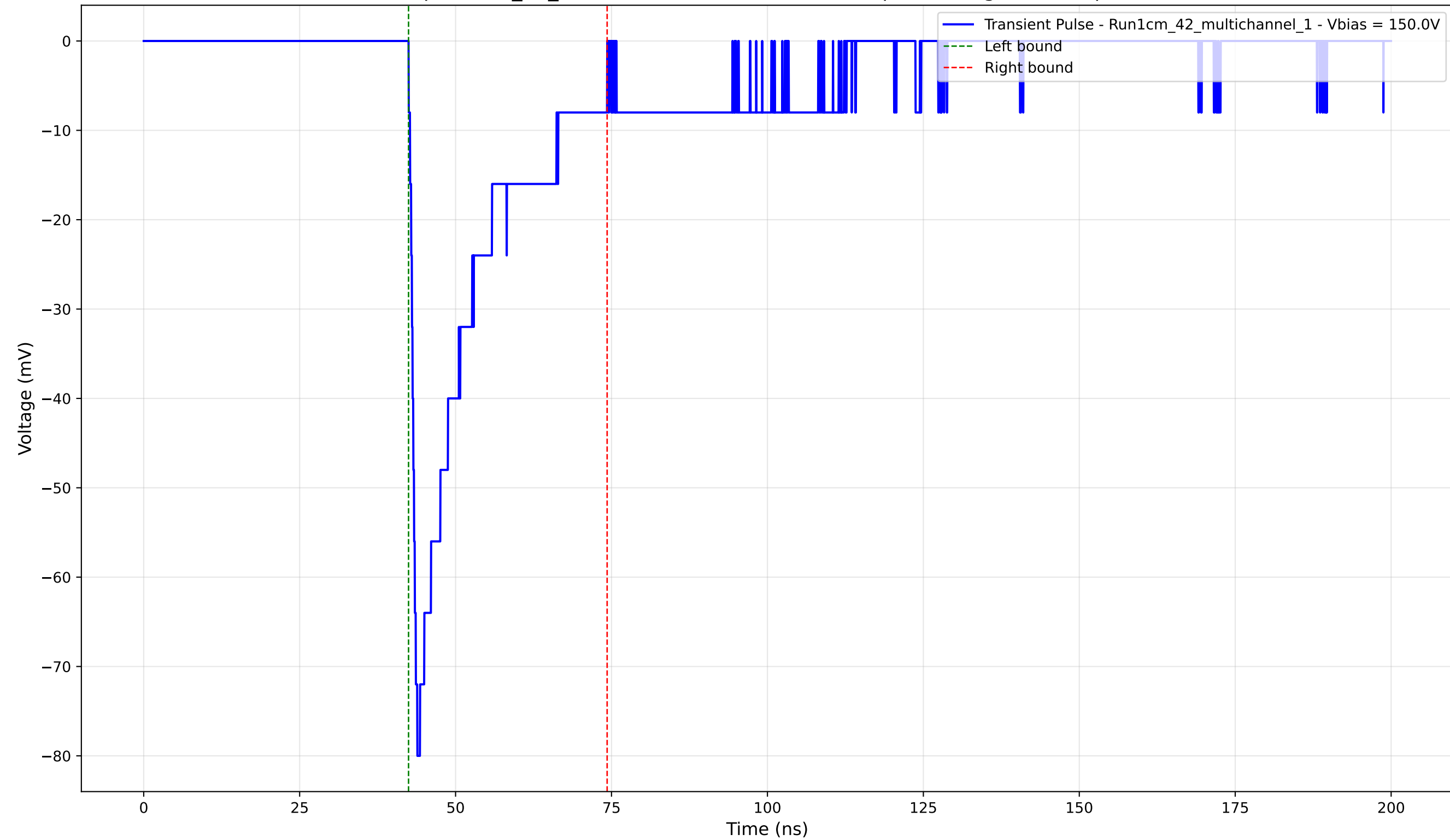
Transient Pulse - Sample: 1cm_42_multichannel - Position: 3485.0 \mu\text{m} - Charge: -15.99 pC - Rise Time: 0.94 ns
