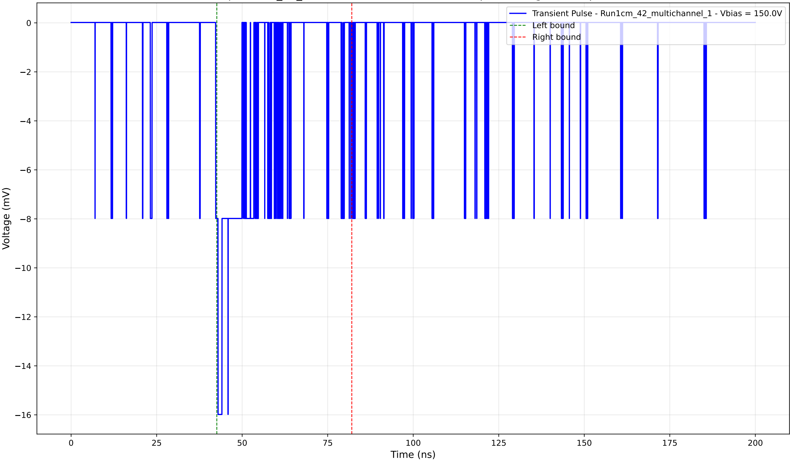
Transient Pulse - Sample: 1cm_42_multichannel - Position: 1900.0 \mu\text{m} - Charge: -2.32 pC - Rise Time: 0.70 ns
