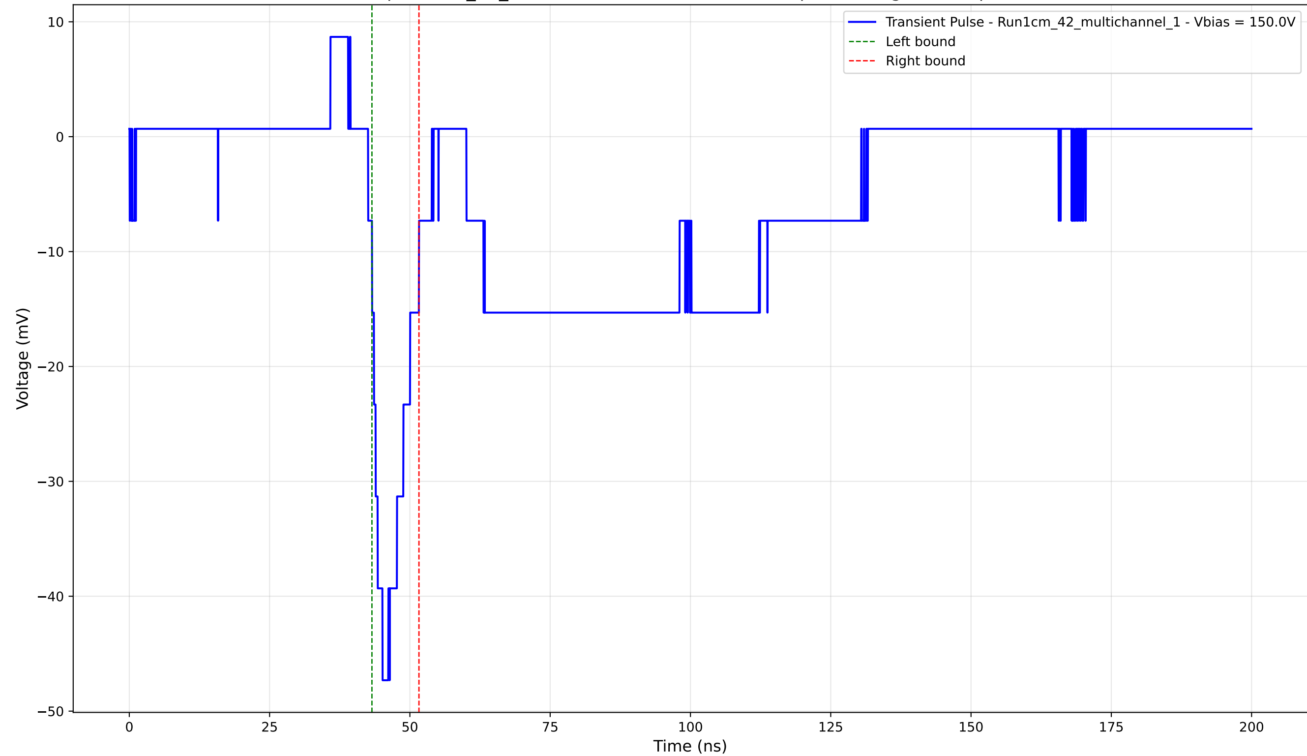
Transient Pulse - Sample: 1cm_42_multichannel - Position: 4605.0 \mu\text{m} - Charge: -5.11 pC - Rise Time: 2.57 ns
