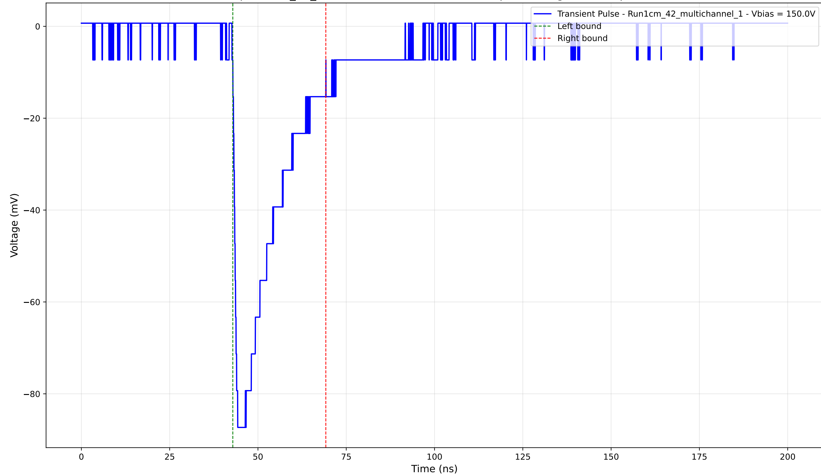
Transient Pulse - Sample: 1cm_42_multichannel - Position: 1070.0 \mu\text{m} - Charge: -22.44 pC - Rise Time: 1.08 ns
