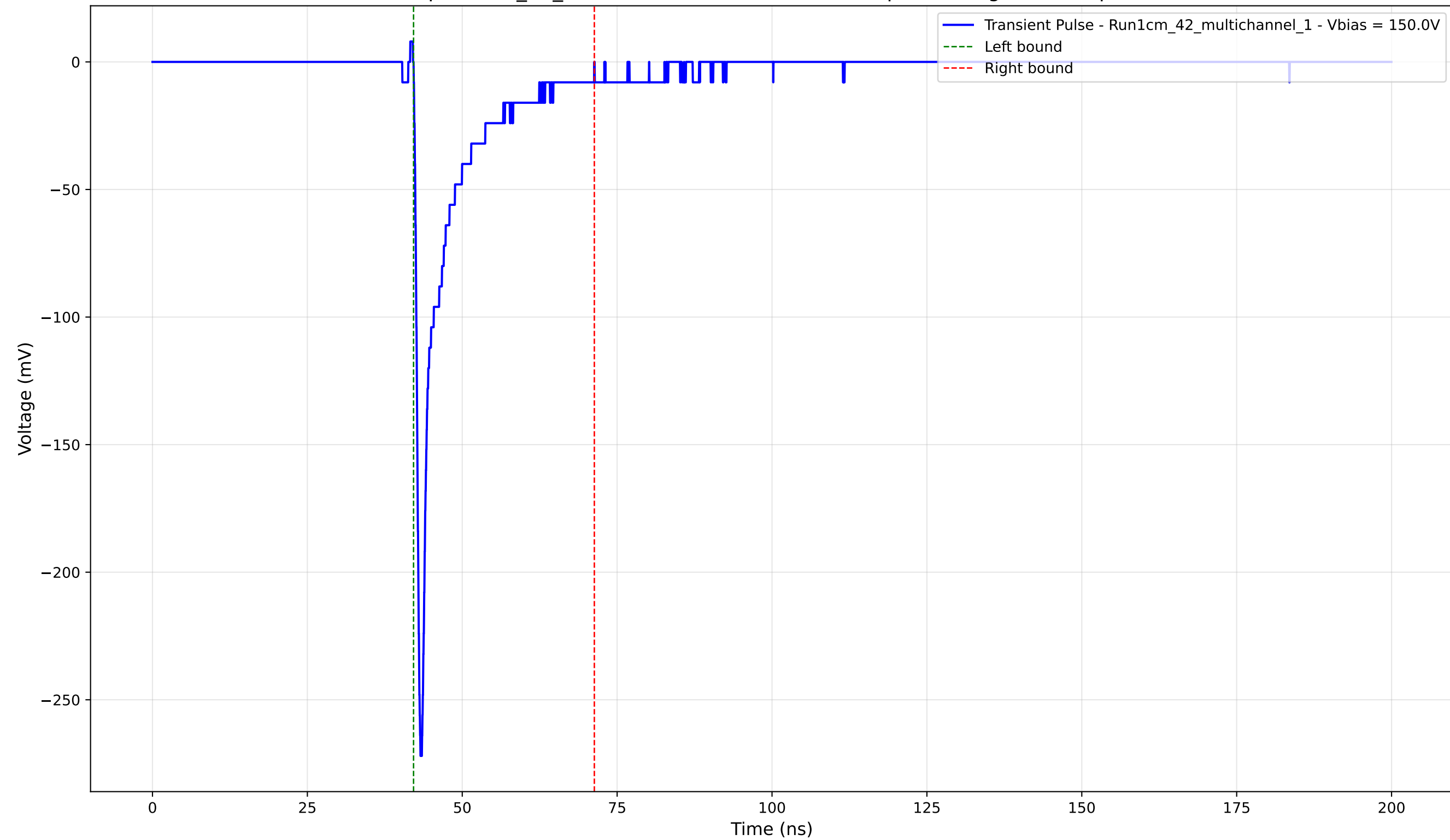
Transient Pulse - Sample: 1cm_42_multichannel - Position: 2720.0 \mu\text{m} - Charge: -23.84 pC - Rise Time: 0.77 ns
