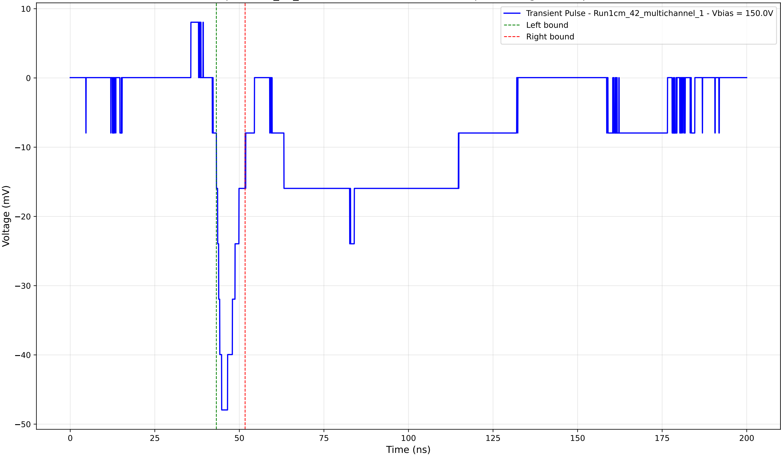
Transient Pulse - Sample: 1cm_42_multichannel - Position: 4310.0 \mu\text{m} - Charge: -5.37 pC - Rise Time: 2.53 ns
