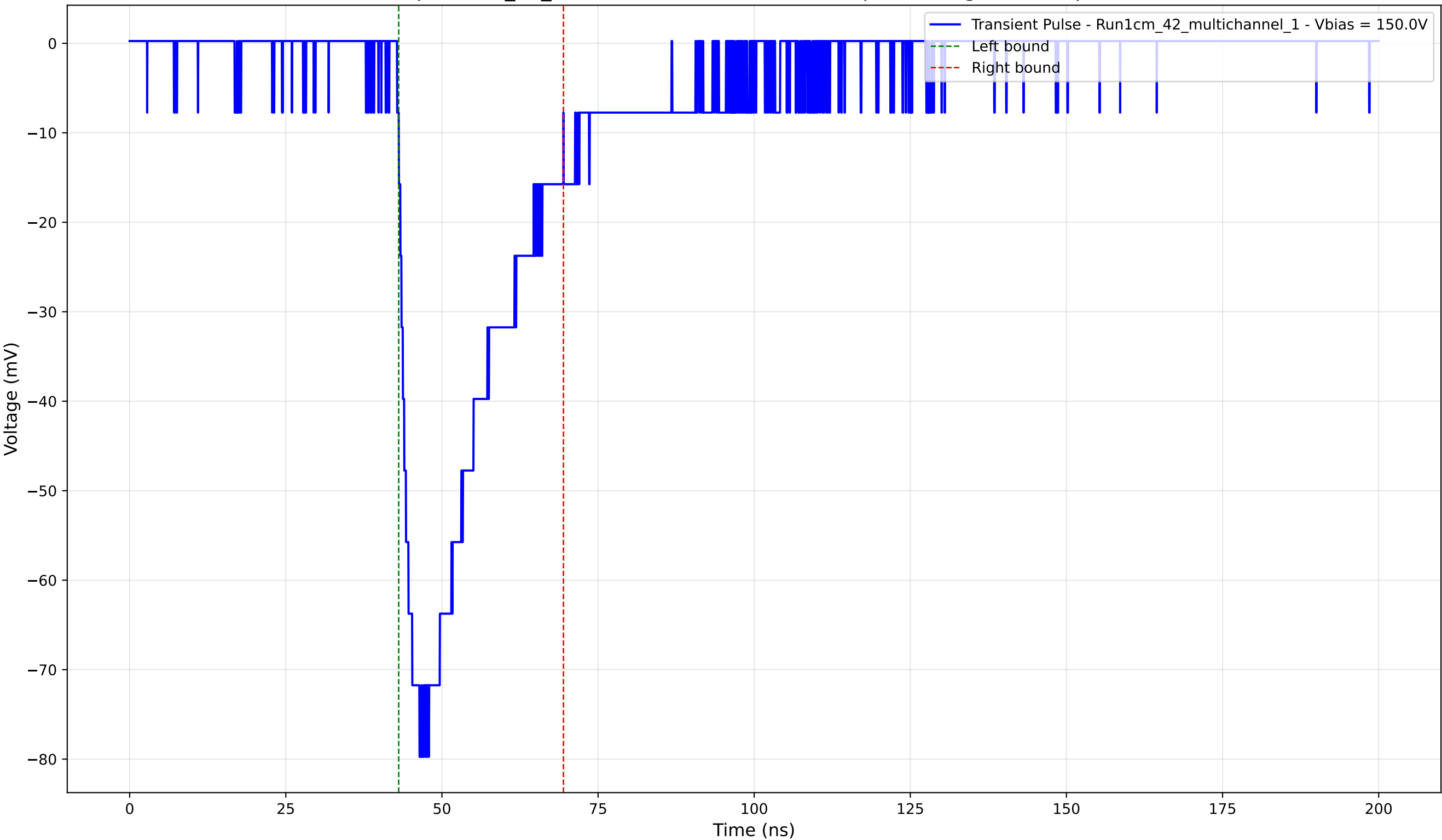
Transient Pulse - Sample: 1cm_42_multichannel - Position: 485.0 \mu\text{m} - Charge: -22.09 pC - Rise Time: 3.32 ns
