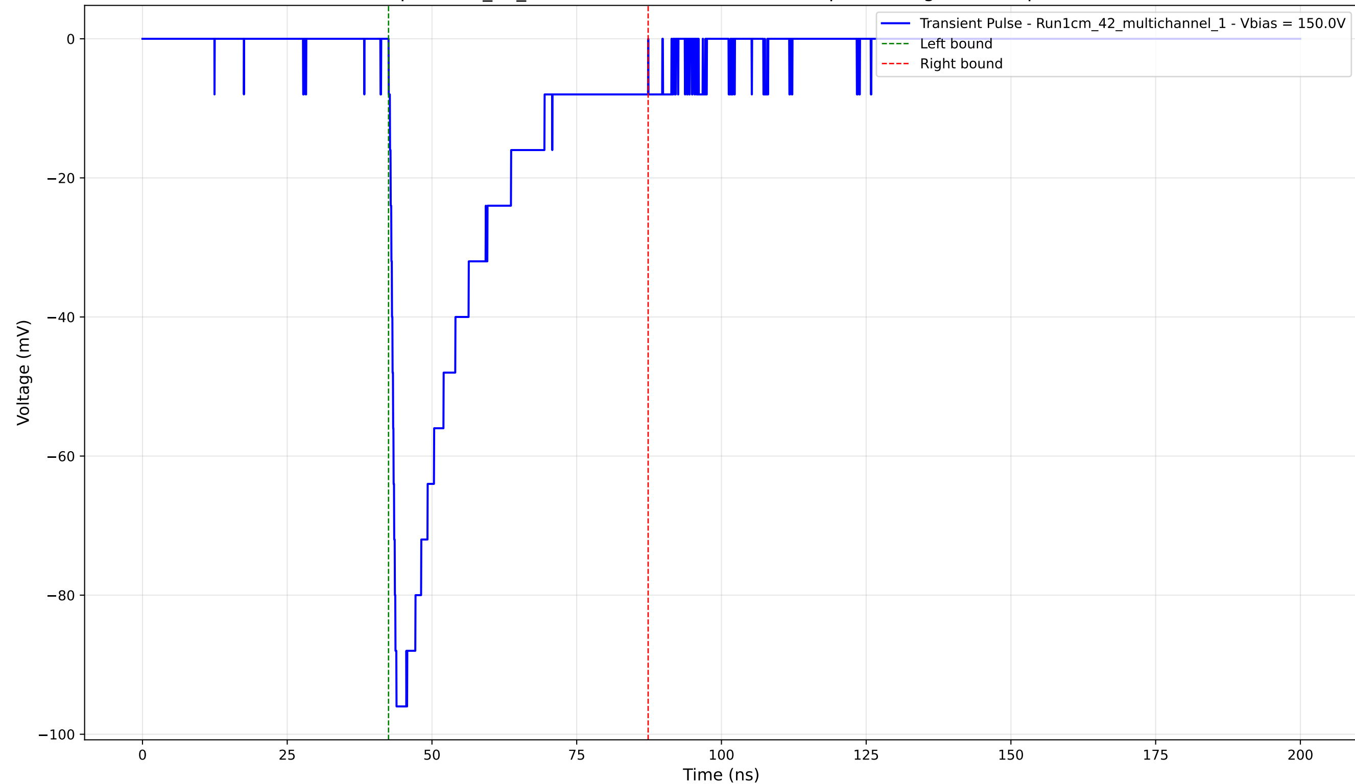
Transient Pulse - Sample: 1cm_42_multichannel - Position: 1240.0 \mu\text{m} - Charge: -26.30 pC - Rise Time: 0.96 ns
