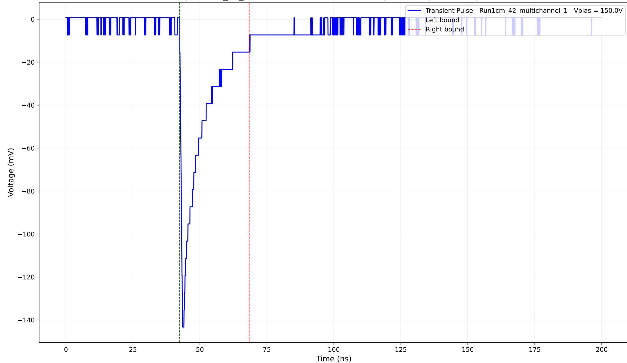
Transient Pulse - Sample: 1cm_42_multichannel - Position: 1605.0 \mu\text{m} - Charge: -23.27 pC - Rise Time: 1.00 ns
