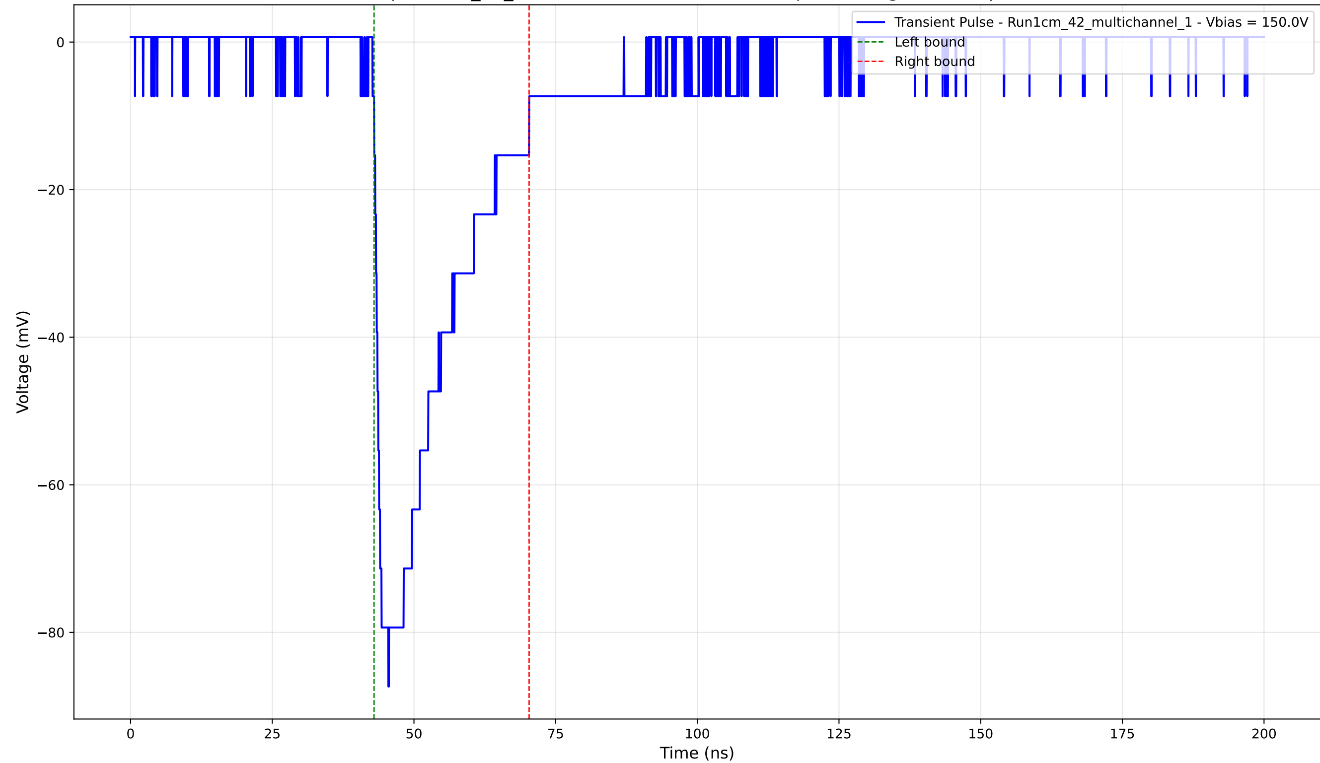
Transient Pulse - Sample: 1cm_42_multichannel - Position: 960.0 \mu\text{m} - Charge: -22.61 pC - Rise Time: 1.32 ns
