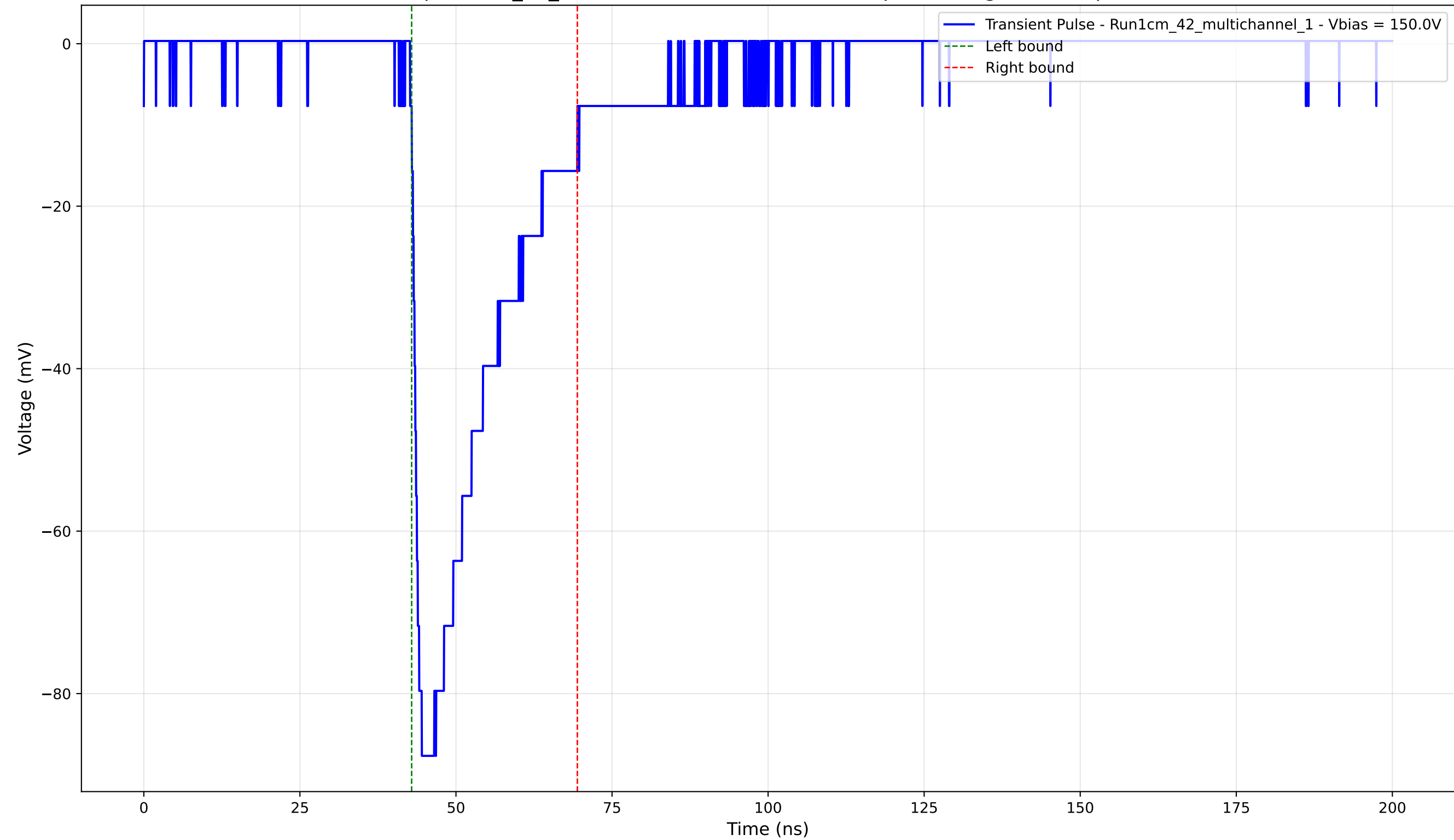
Transient Pulse - Sample: 1cm_42_multichannel - Position: 1030.0 \mu\text{m} - Charge: -22.76 pC - Rise Time: 1.20 ns
