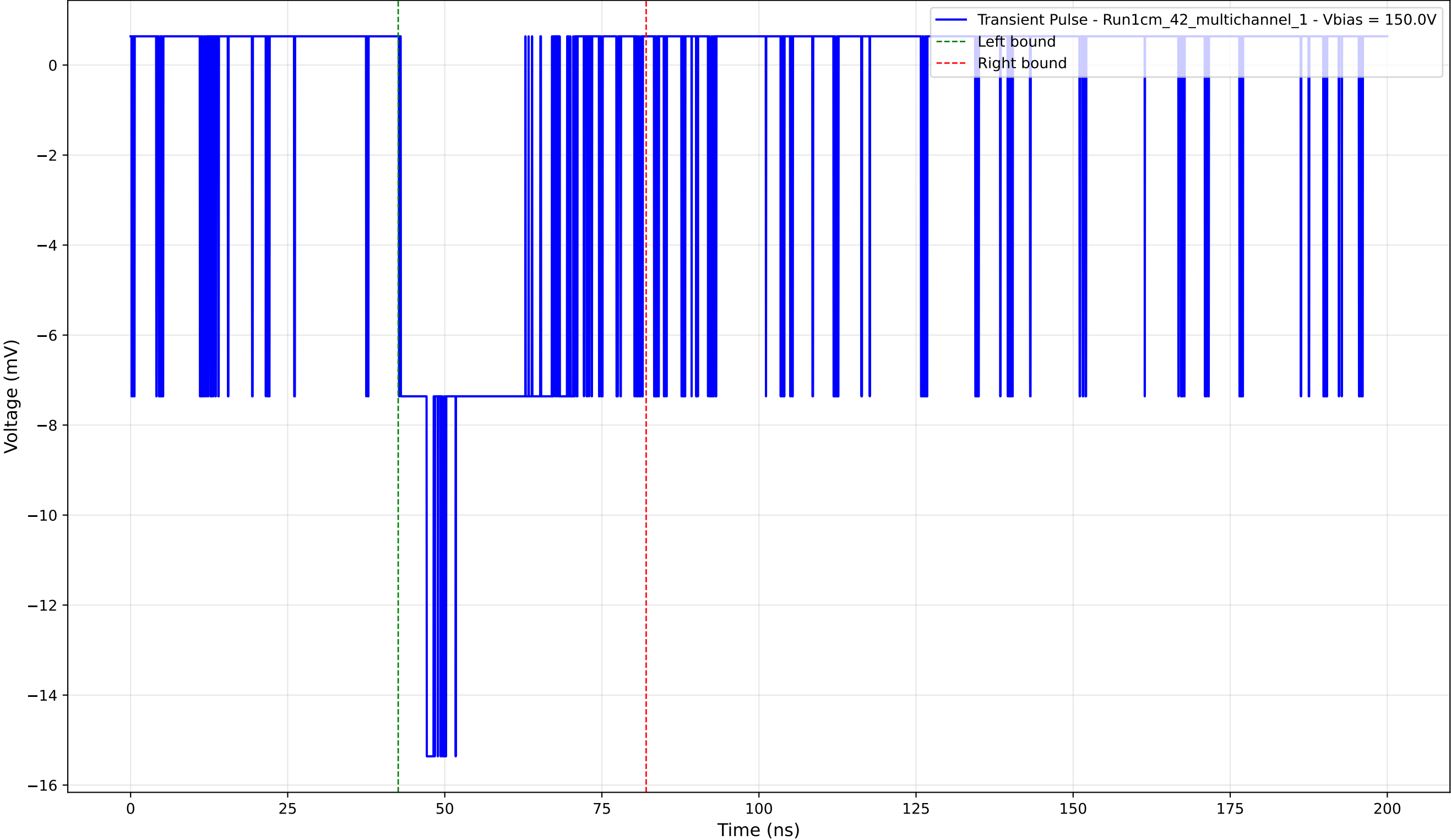
Transient Pulse - Sample: 1cm_42_multichannel - Position: 70.0 \mu\text{m} - Charge: -4.29 pC - Rise Time: 4.14 ns
