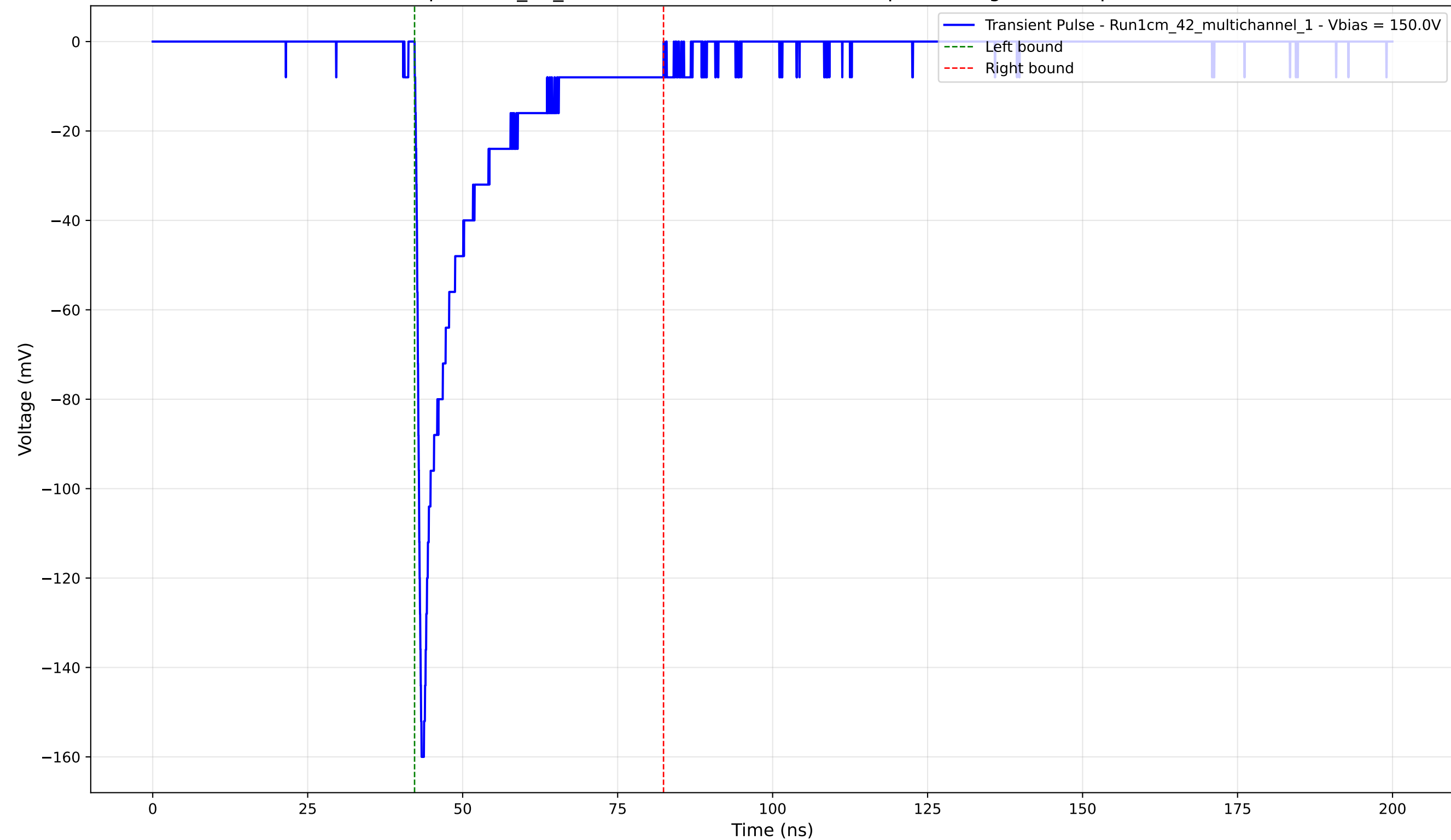
Transient Pulse - Sample: 1cm_42_multichannel - Position: 1805.0 \mu\text{m} - Charge: -22.57 pC - Rise Time: 0.80 ns
