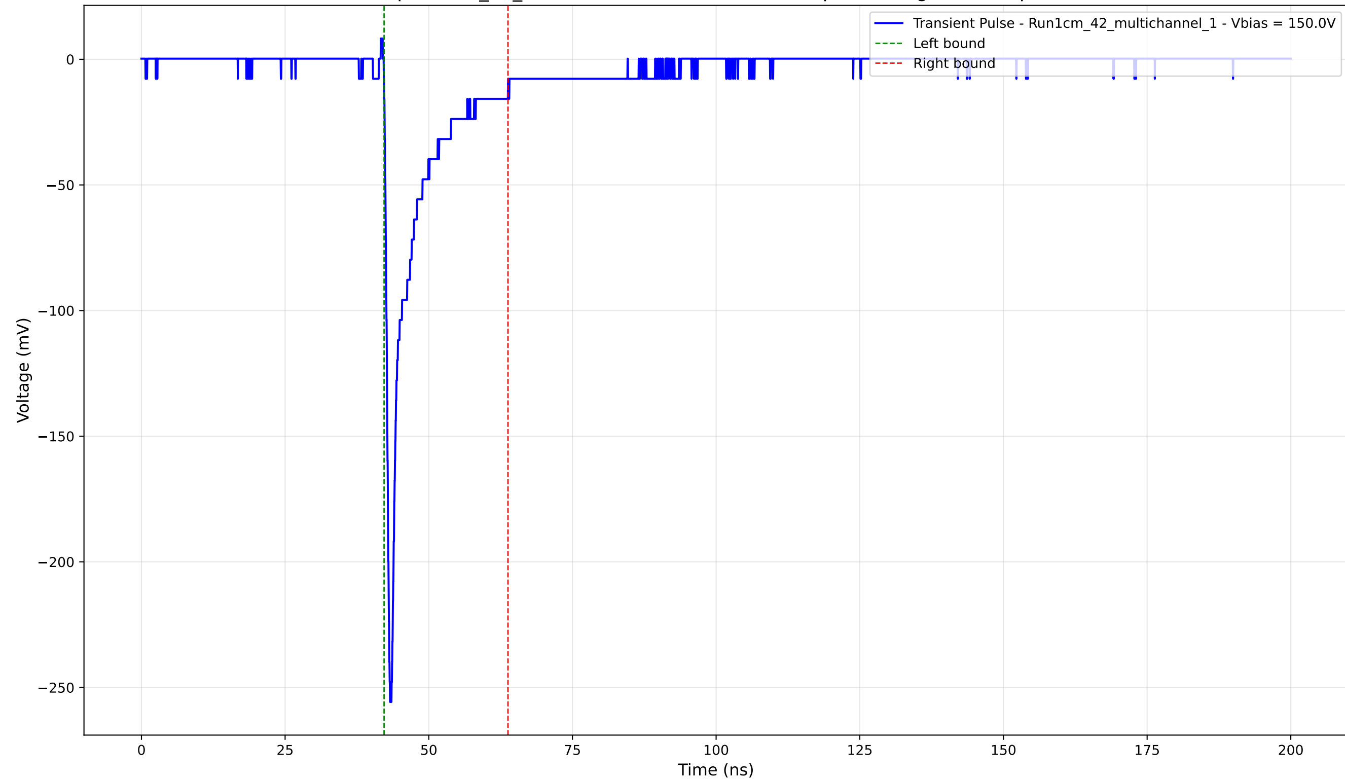
Transient Pulse - Sample: 1cm_42_multichannel - Position: 2750.0 \mu\text{m} - Charge: -22.31 pC - Rise Time: 0.78 ns
