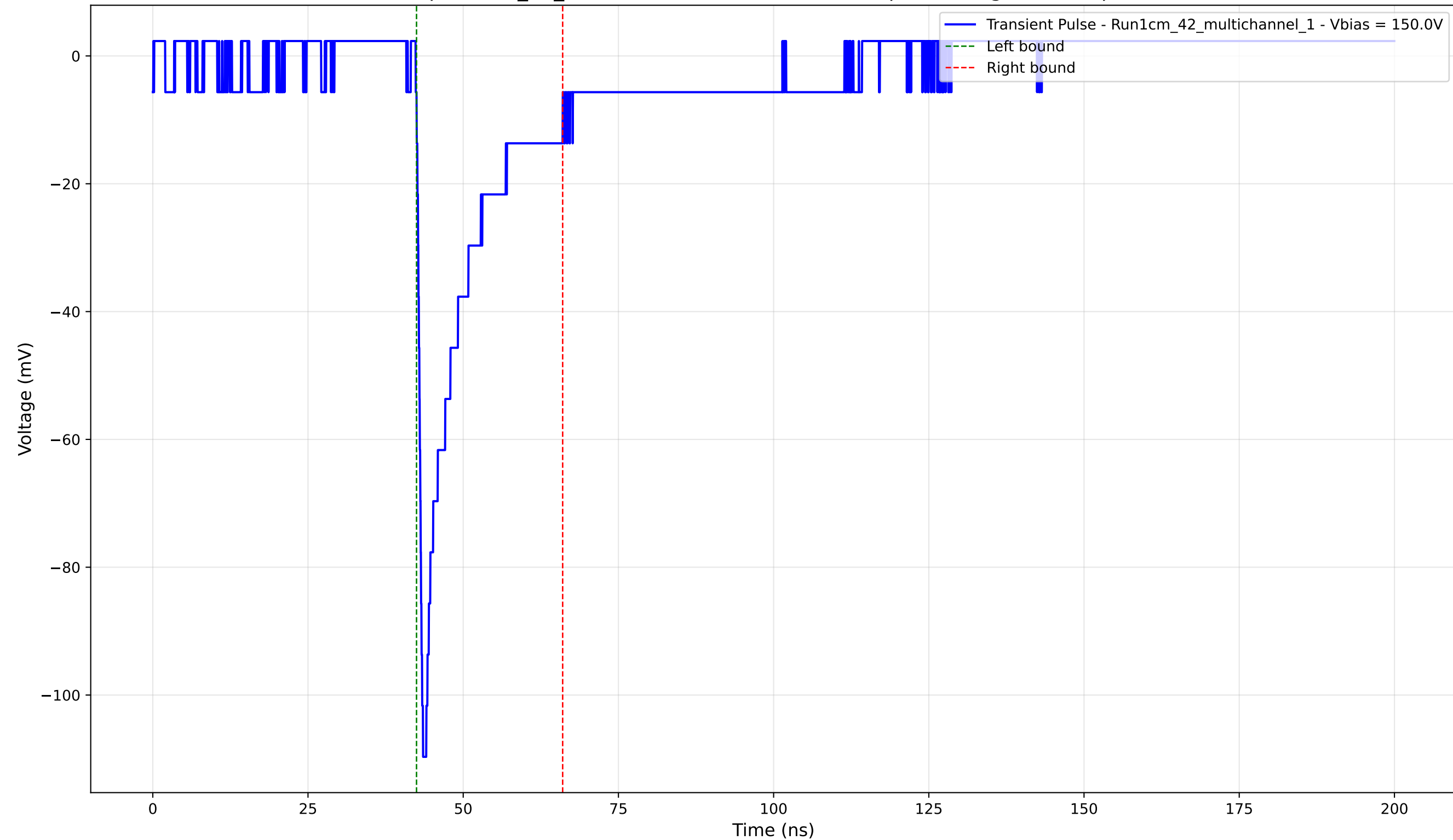
Transient Pulse - Sample: 1cm_42_multichannel - Position: 3220.0 \mu\text{m} - Charge: -15.54 pC - Rise Time: 0.89 ns
