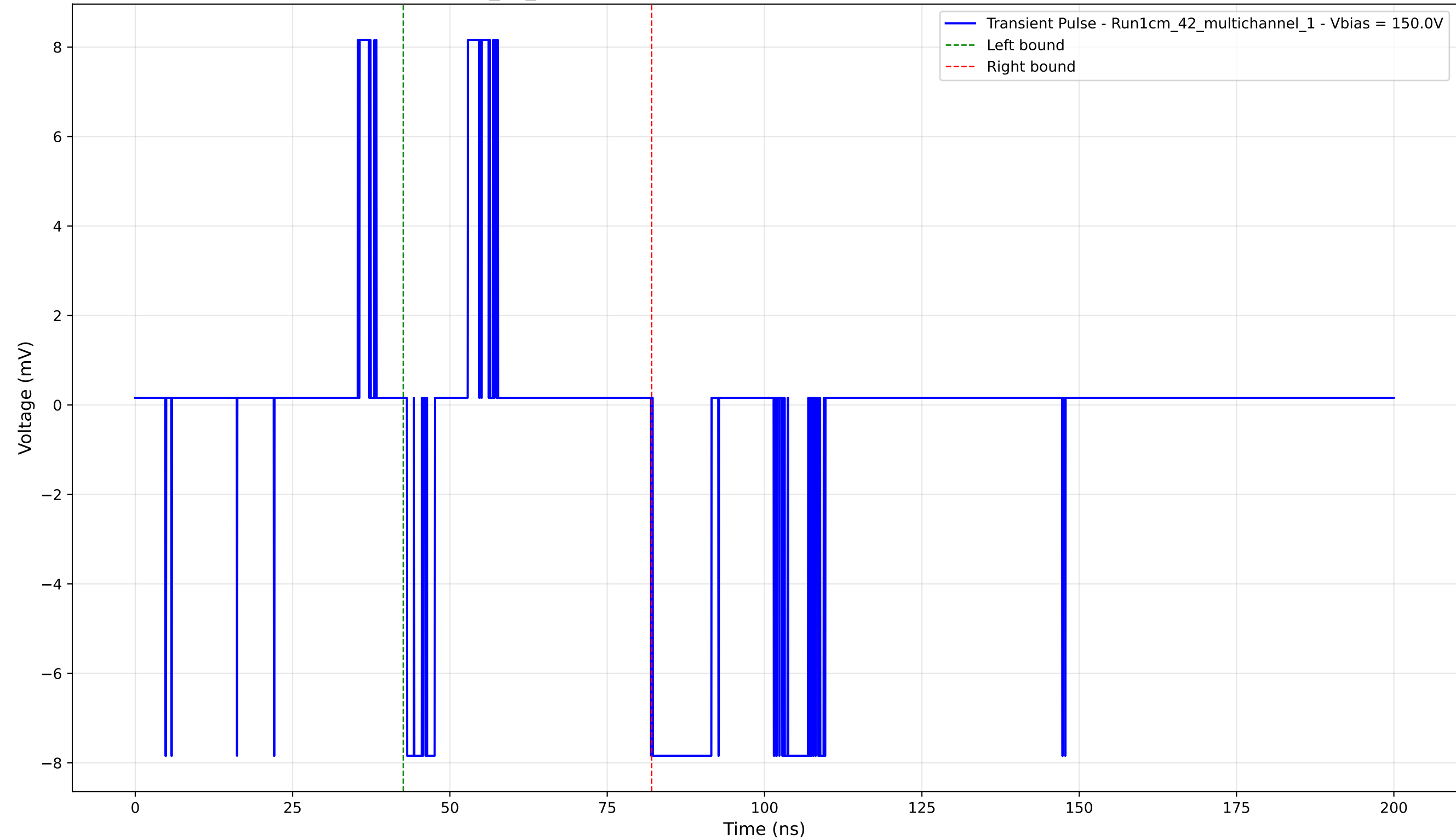
Transient Pulse - Sample: 1cm_42_multichannel - Position: 4415.0 \mu\text{m} - Charge: 0.14 pC - Rise Time: 0.00 ns (N/A)
