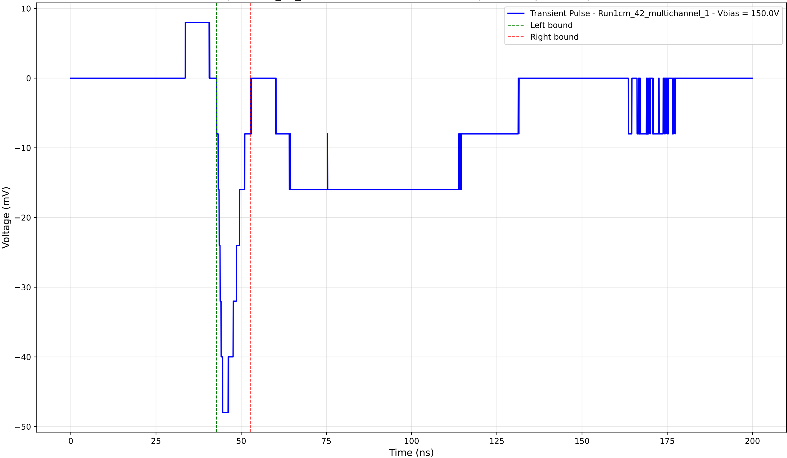
Transient Pulse - Sample: 1cm_42_multichannel - Position: 4140.0 \mu\text{m} - Charge: -5.40 pC - Rise Time: 1.77 ns
