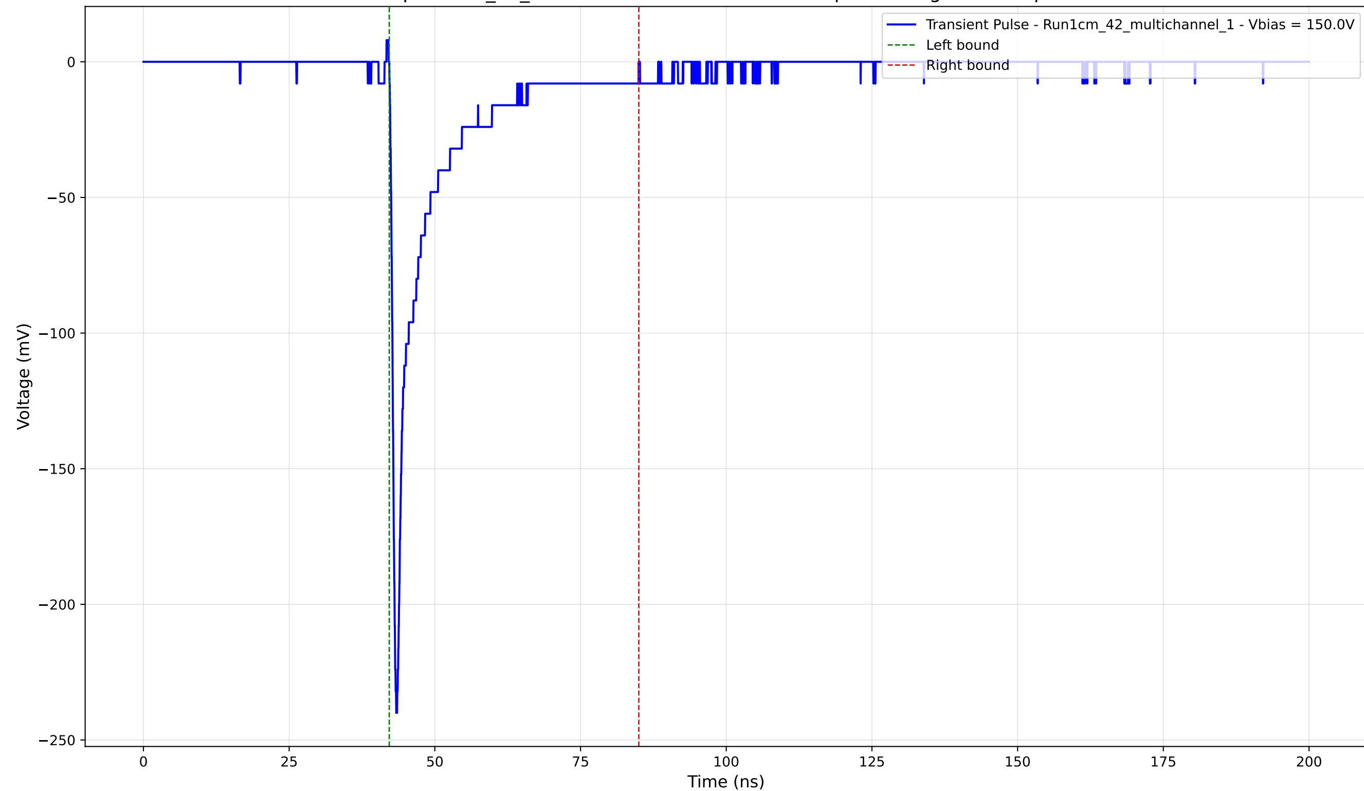
Transient Pulse - Sample: 1cm_42_multichannel - Position: 1970.0 \mu\text{m} - Charge: -26.53 pC - Rise Time: 0.80 ns
