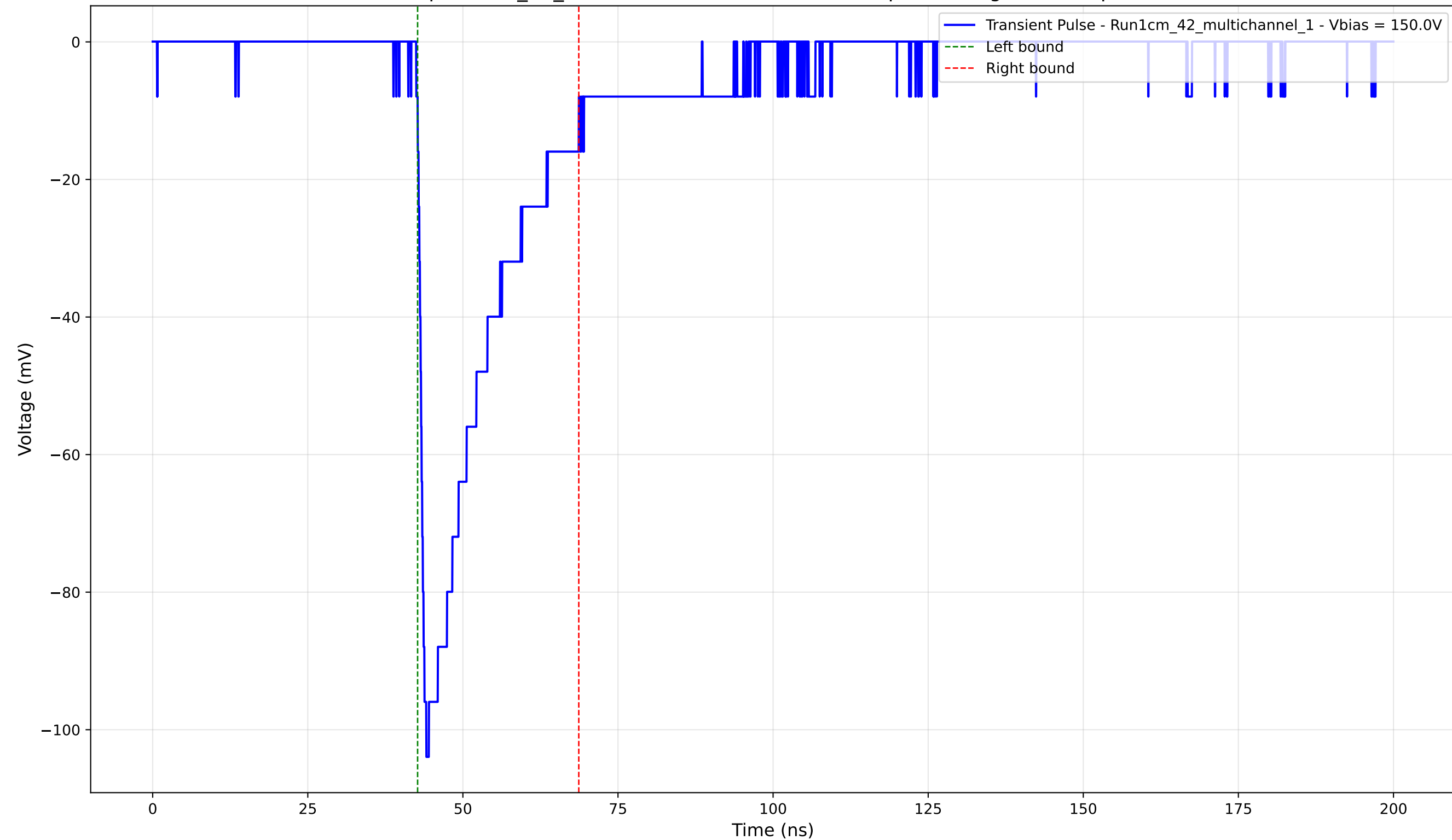
Transient Pulse - Sample: 1cm_42_multichannel - Position: 1265.0 \mu\text{m} - Charge: -23.37 pC - Rise Time: 1.09 ns
