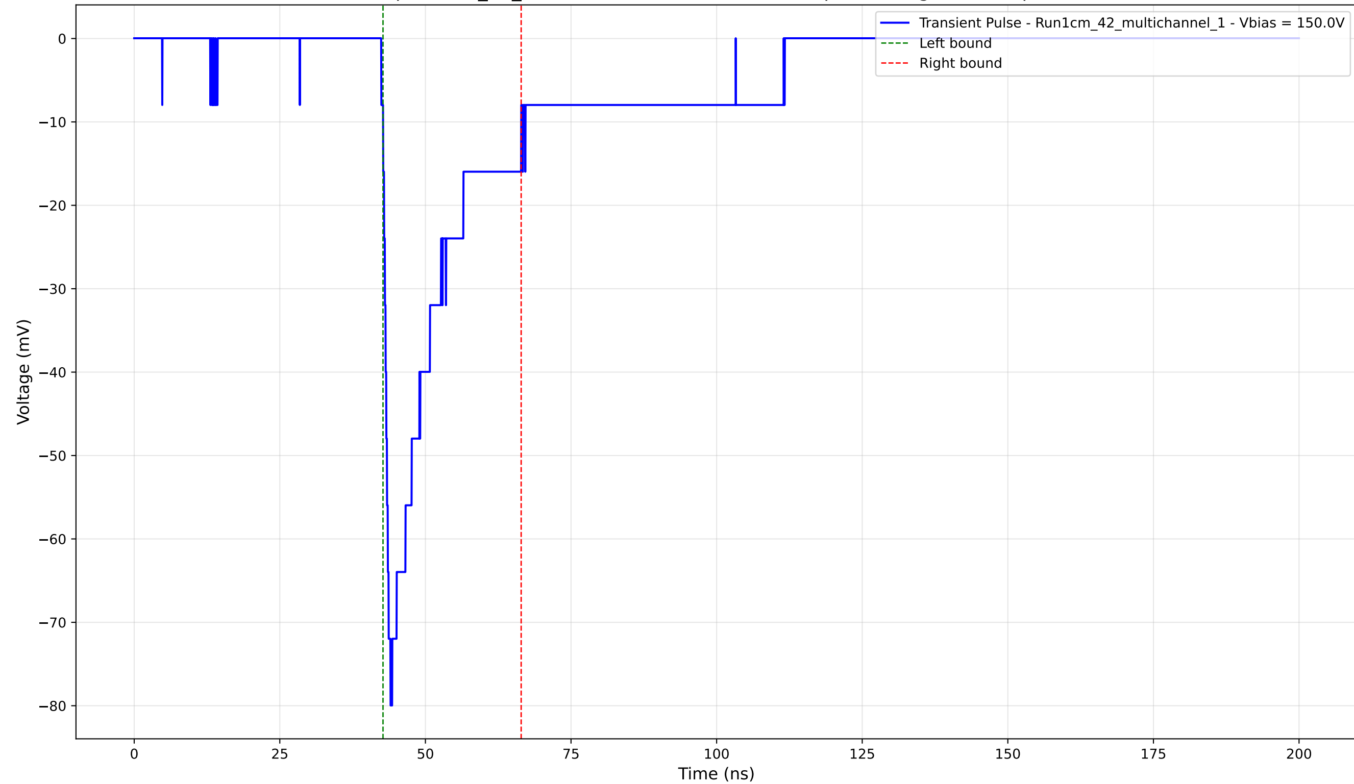
Transient Pulse - Sample: 1cm_42_multichannel - Position: 3540.0 \mu\text{m} - Charge: -14.89 pC - Rise Time: 1.28 ns
