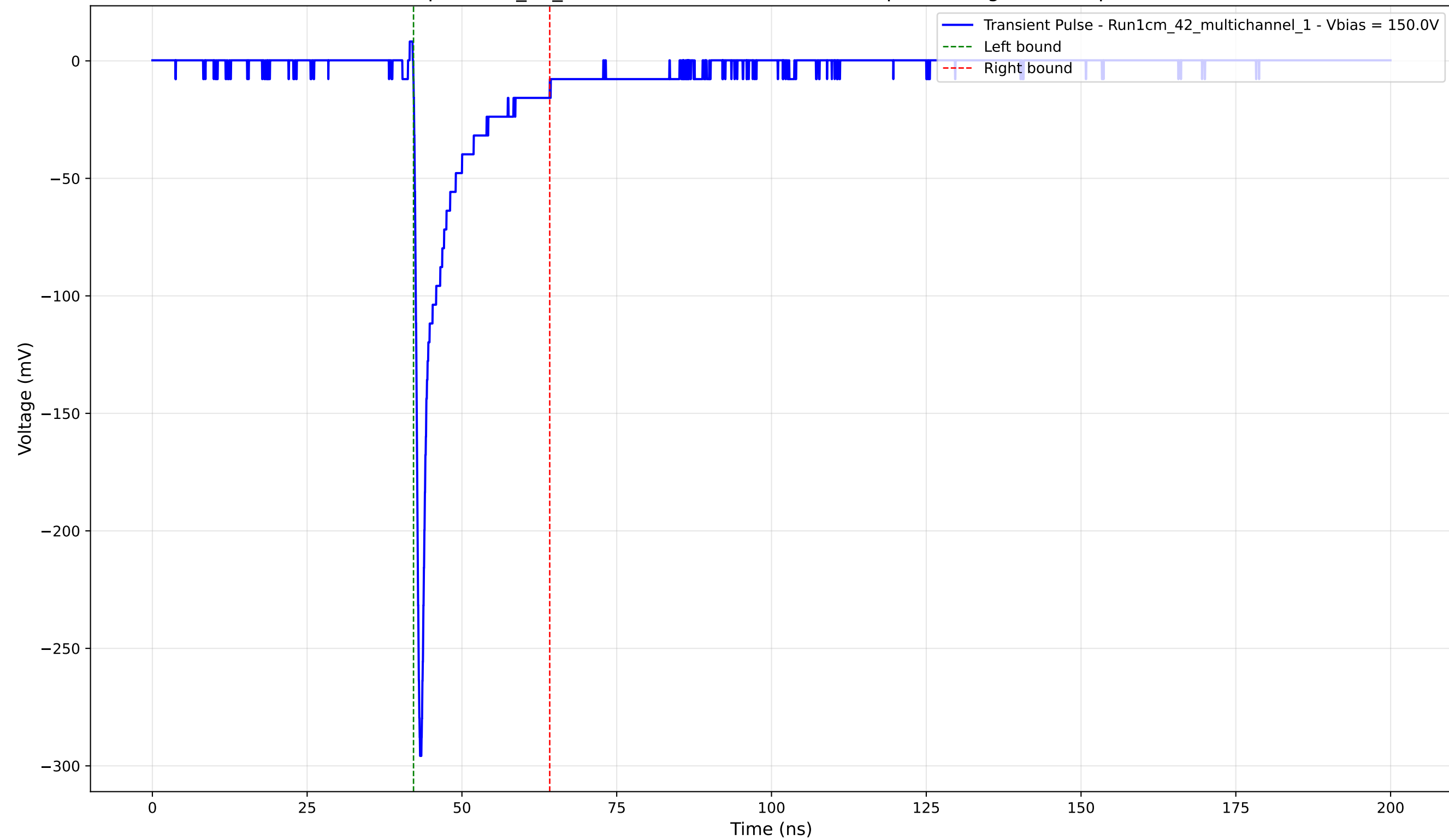
Transient Pulse - Sample: 1cm_42_multichannel - Position: 2085.0 \mu\text{m} - Charge: -24.00 pC - Rise Time: 0.79 ns
