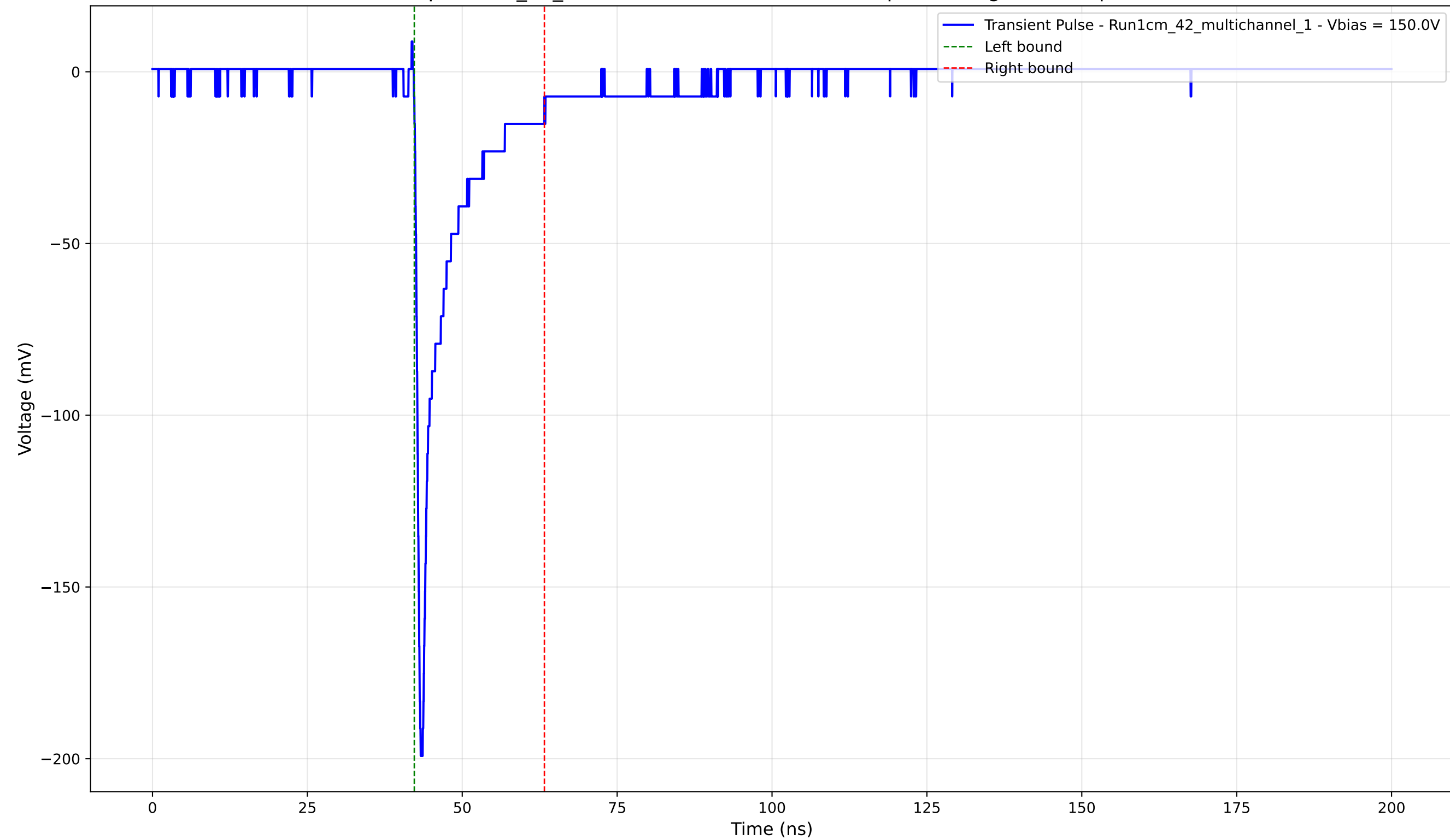
Transient Pulse - Sample: 1cm_42_multichannel - Position: 2815.0 \mu\text{m} - Charge: -19.01 pC - Rise Time: 0.79 ns
