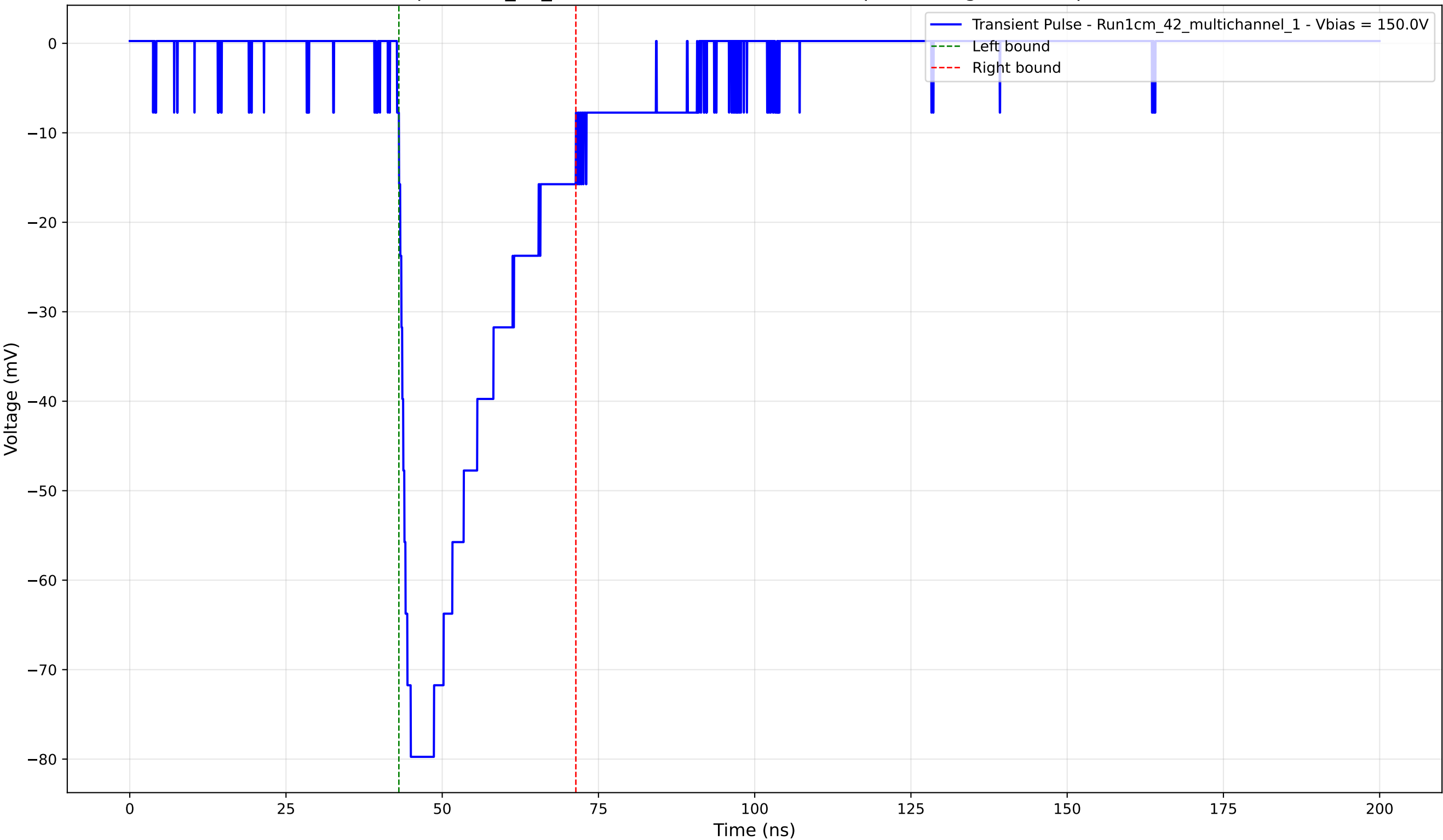
Transient Pulse - Sample: 1cm_42_multichannel - Position: 725.0 \mu\text{m} - Charge: -23.83 pC - Rise Time: 1.90 ns
