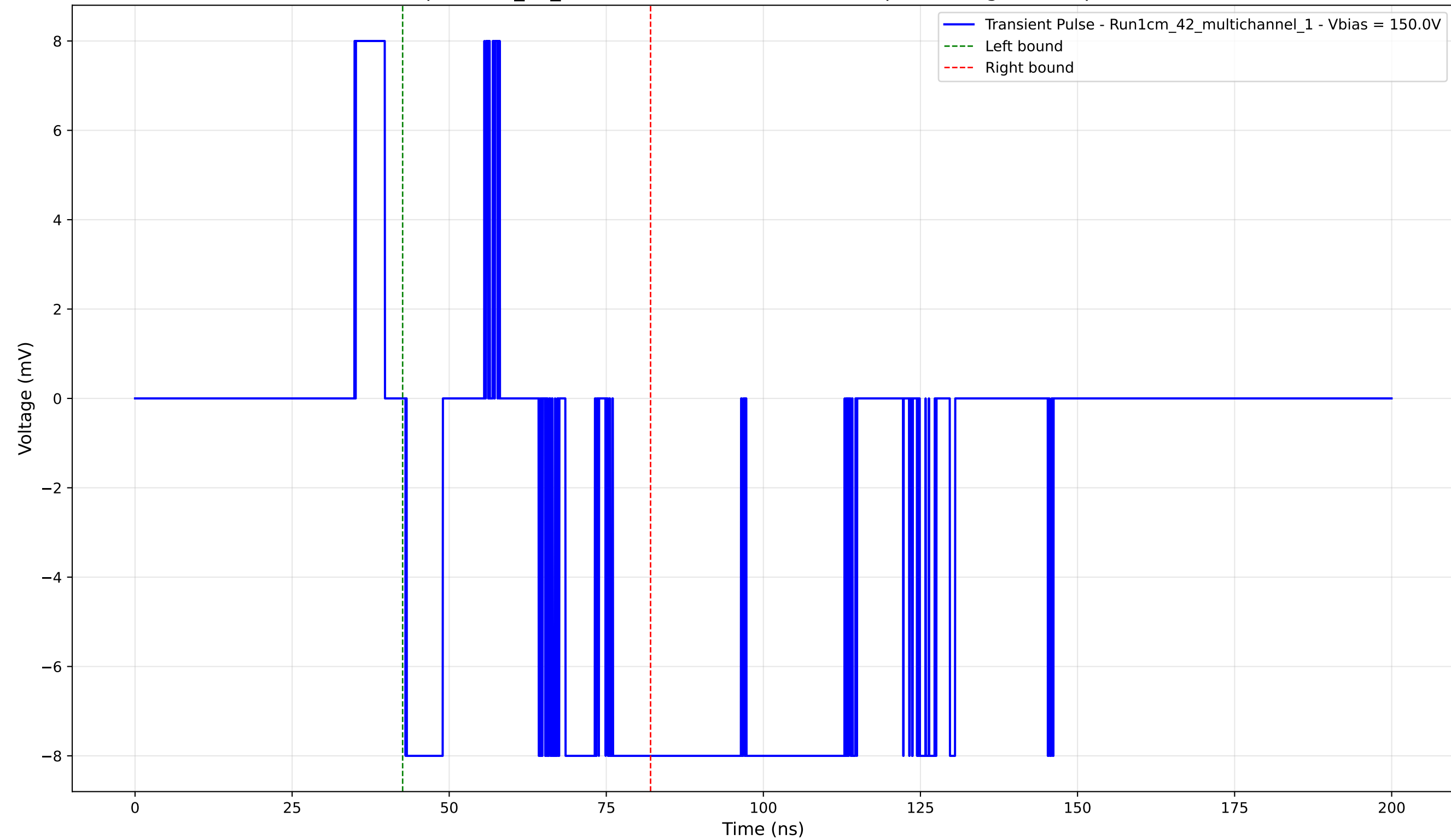
Transient Pulse - Sample: 1cm_42_multichannel - Position: 4440.0 \mu\text{m} - Charge: -2.83 pC - Rise Time: 0.02 ns
