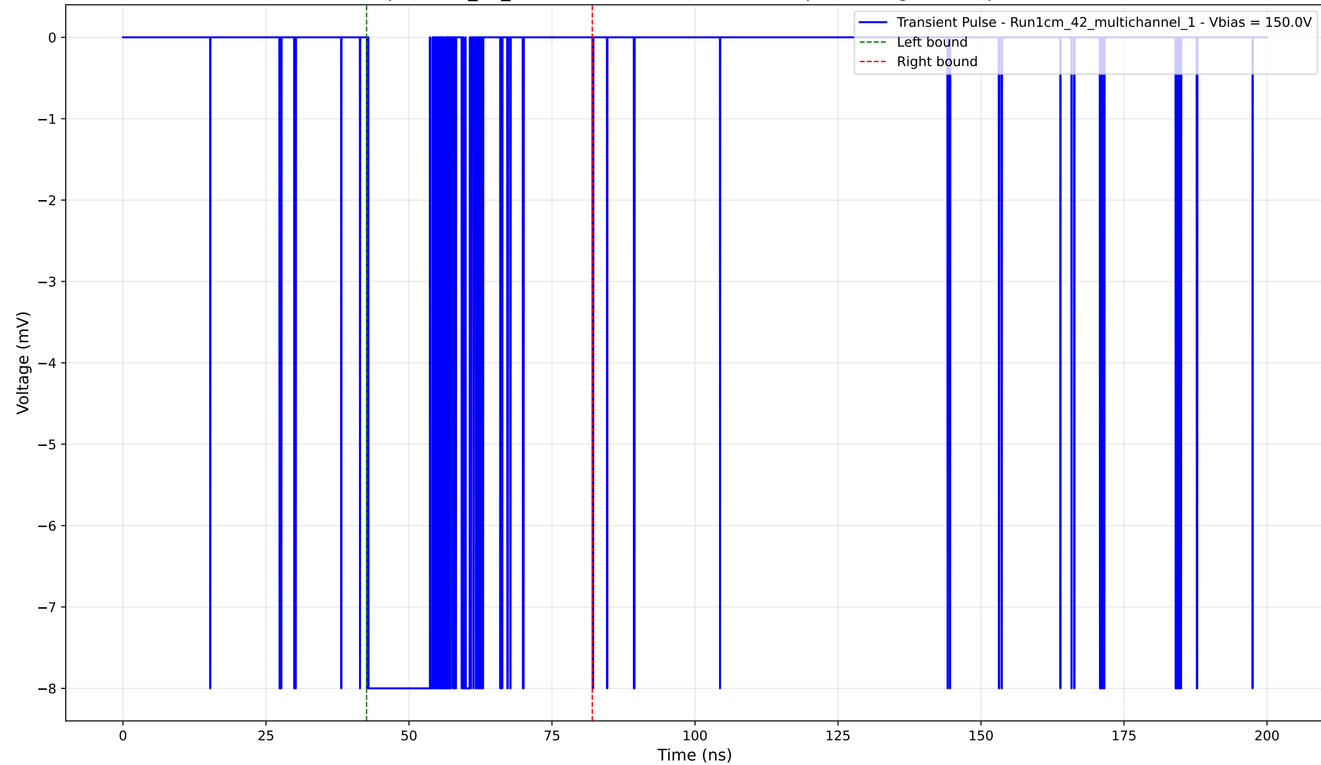
Transient Pulse - Sample: 1cm_42_multichannel - Position: 1355.0 \mu\text{m} - Charge: -2.48 pC - Rise Time: 0.02 ns
