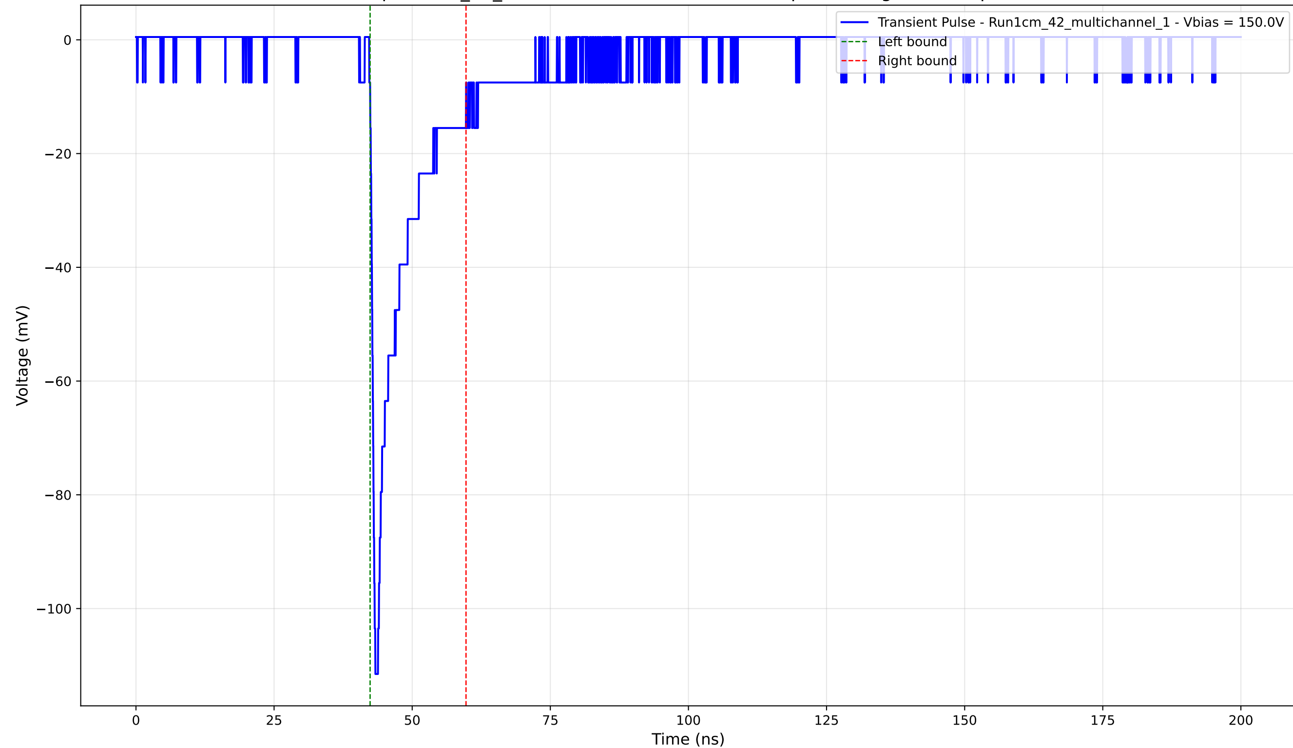
Transient Pulse - Sample: 1cm_42_multichannel - Position: 1825.0 \mu\text{m} - Charge: -12.70 pC - Rise Time: 0.81 ns
