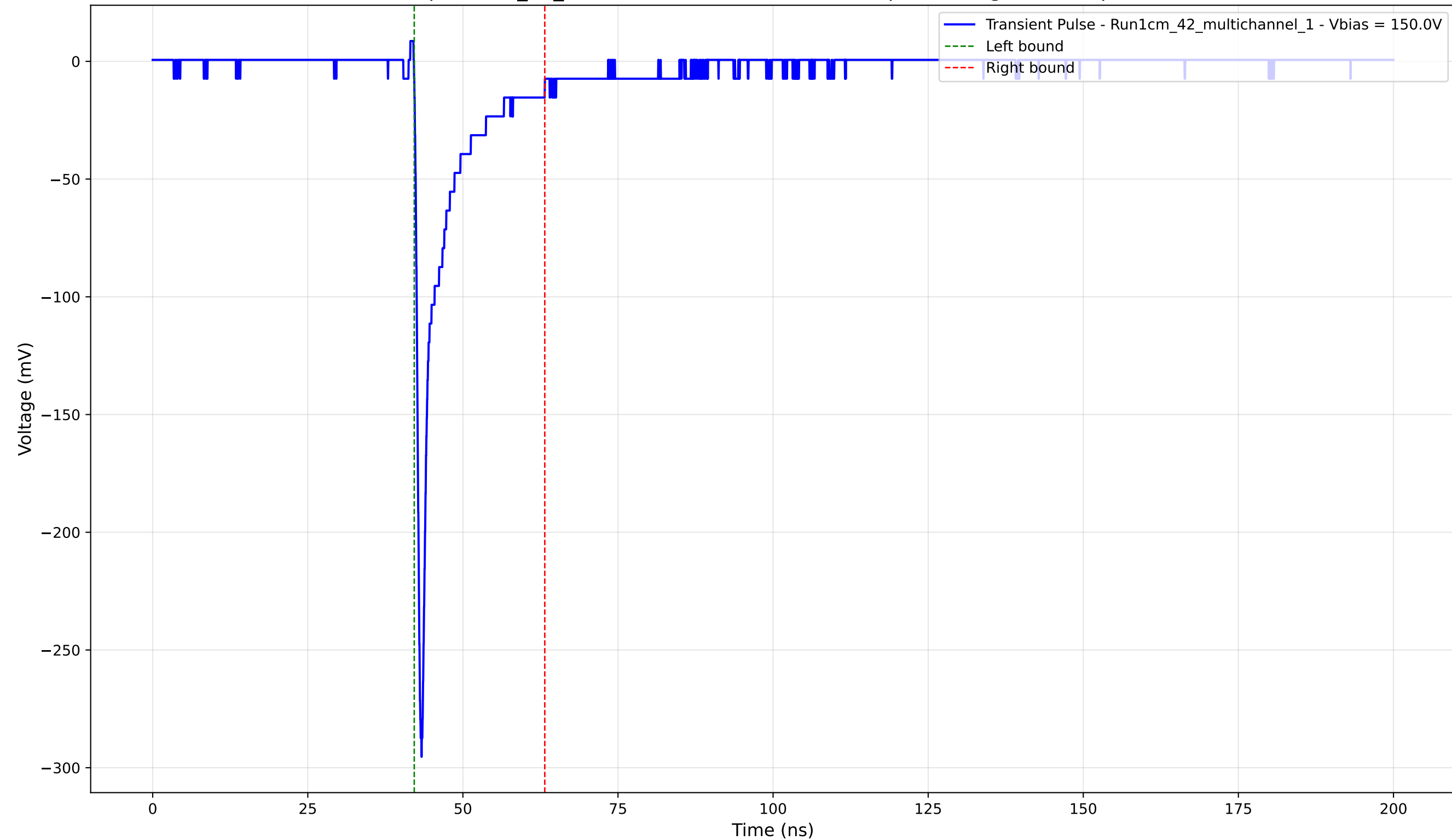
Transient Pulse - Sample: 1cm_42_multichannel - Position: 2675.0 \mu\text{m} - Charge: -22.54 pC - Rise Time: 0.80 ns
