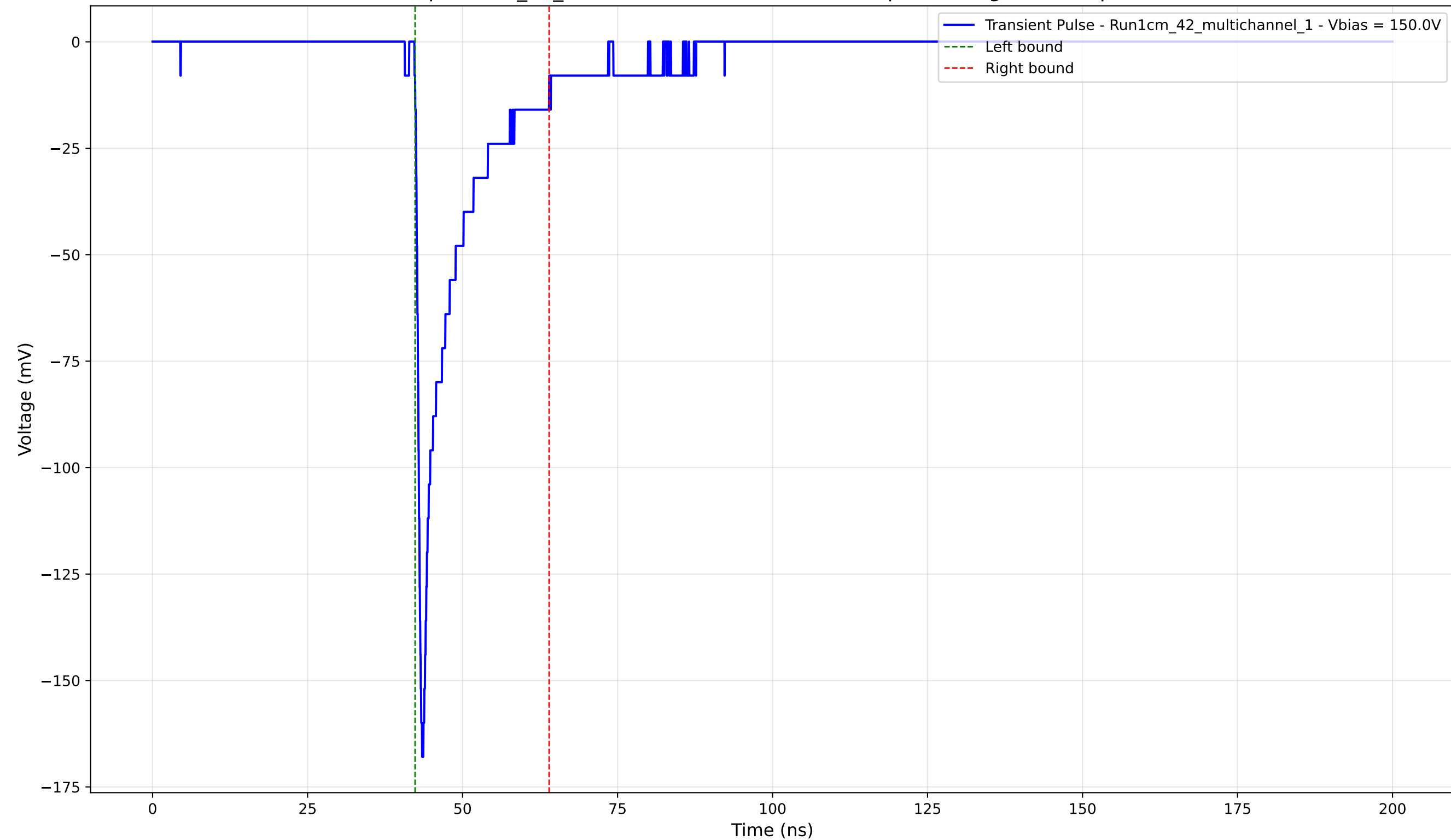
Transient Pulse - Sample: 1cm_42_multichannel - Position: 2975.0 \mu\text{m} - Charge: -19.36 pC - Rise Time: 0.80 ns
