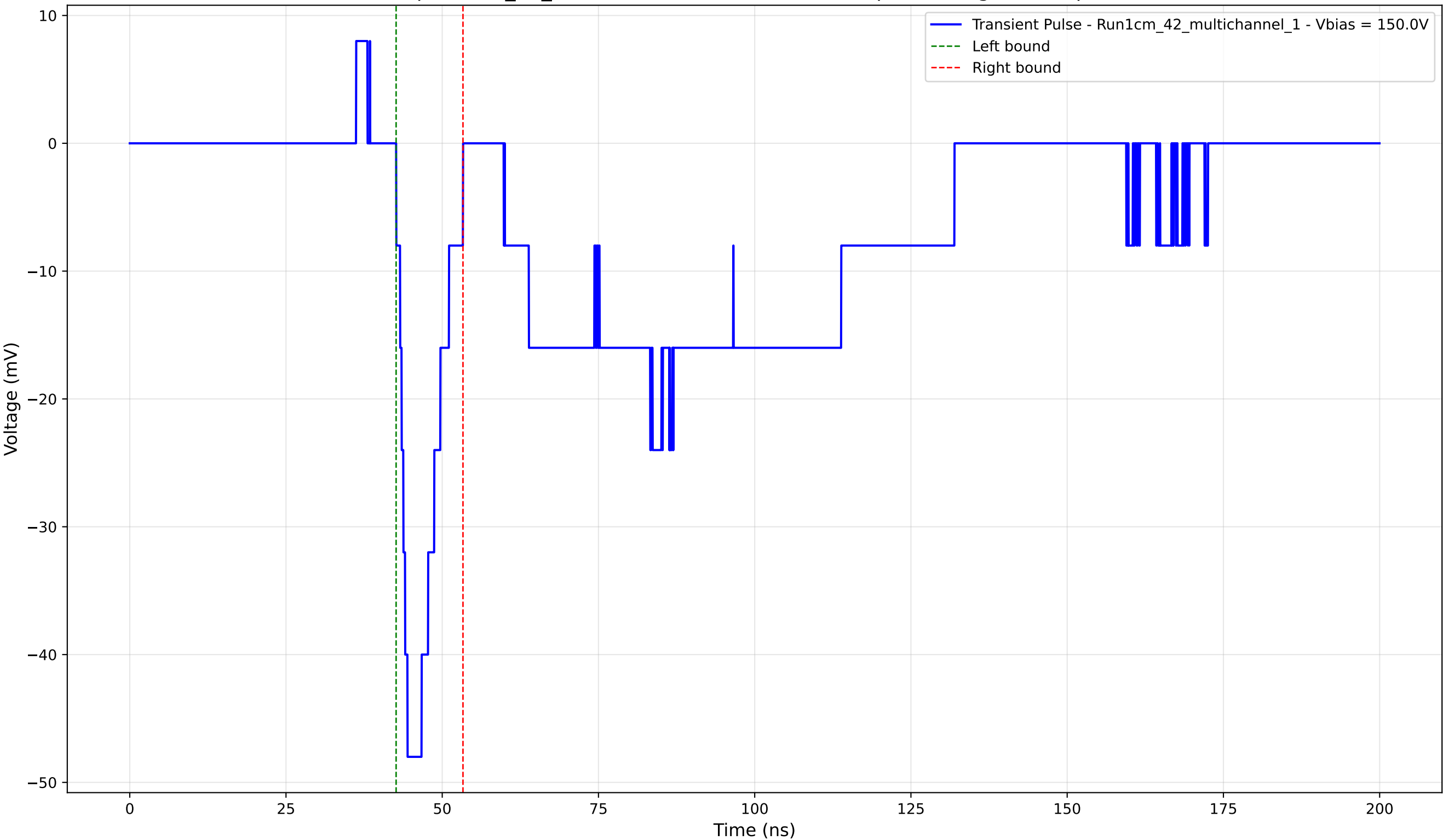
Transient Pulse - Sample: 1cm_42_multichannel - Position: 4200.0 \mu\text{m} - Charge: -5.69 pC - Rise Time: 1.81 ns
