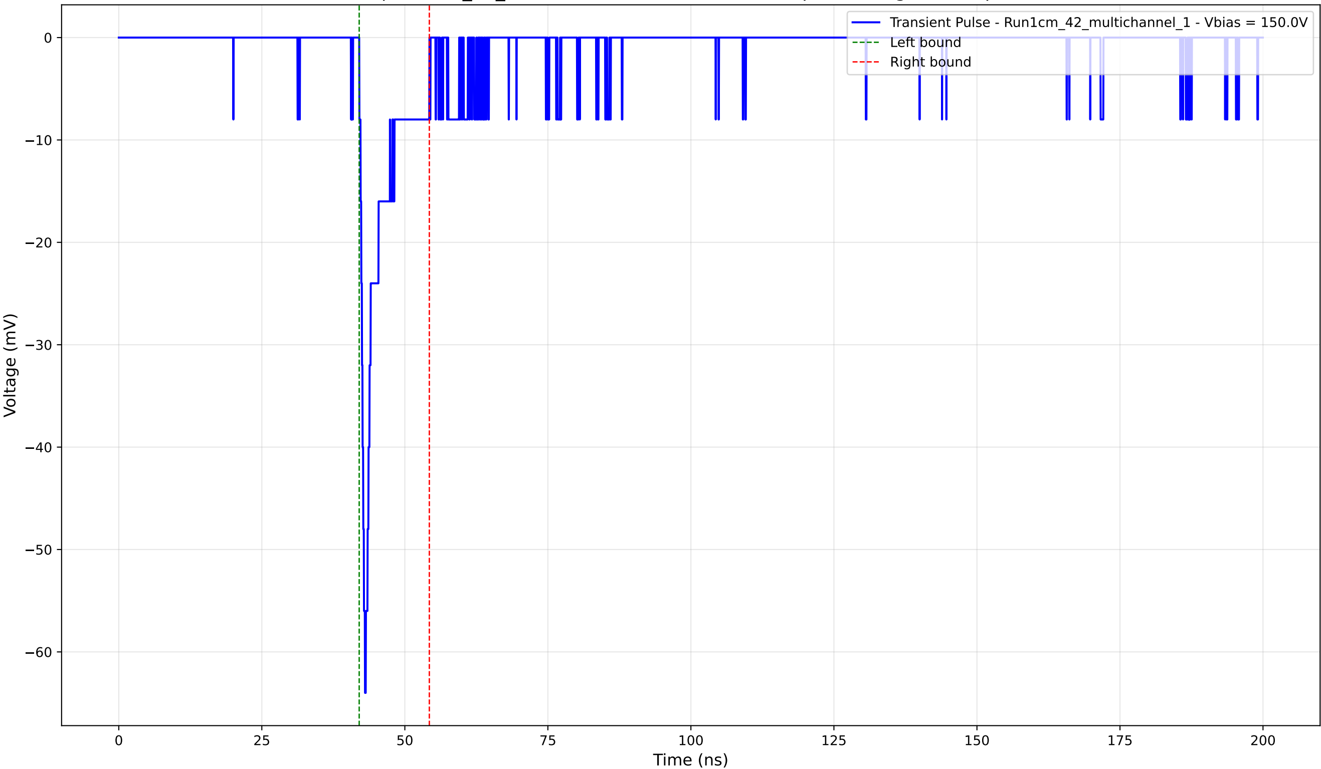
Transient Pulse - Sample: 1cm_42_multichannel - Position: 2420.0 \mu\text{m} - Charge: -4.07 pC - Rise Time: 0.98 ns
