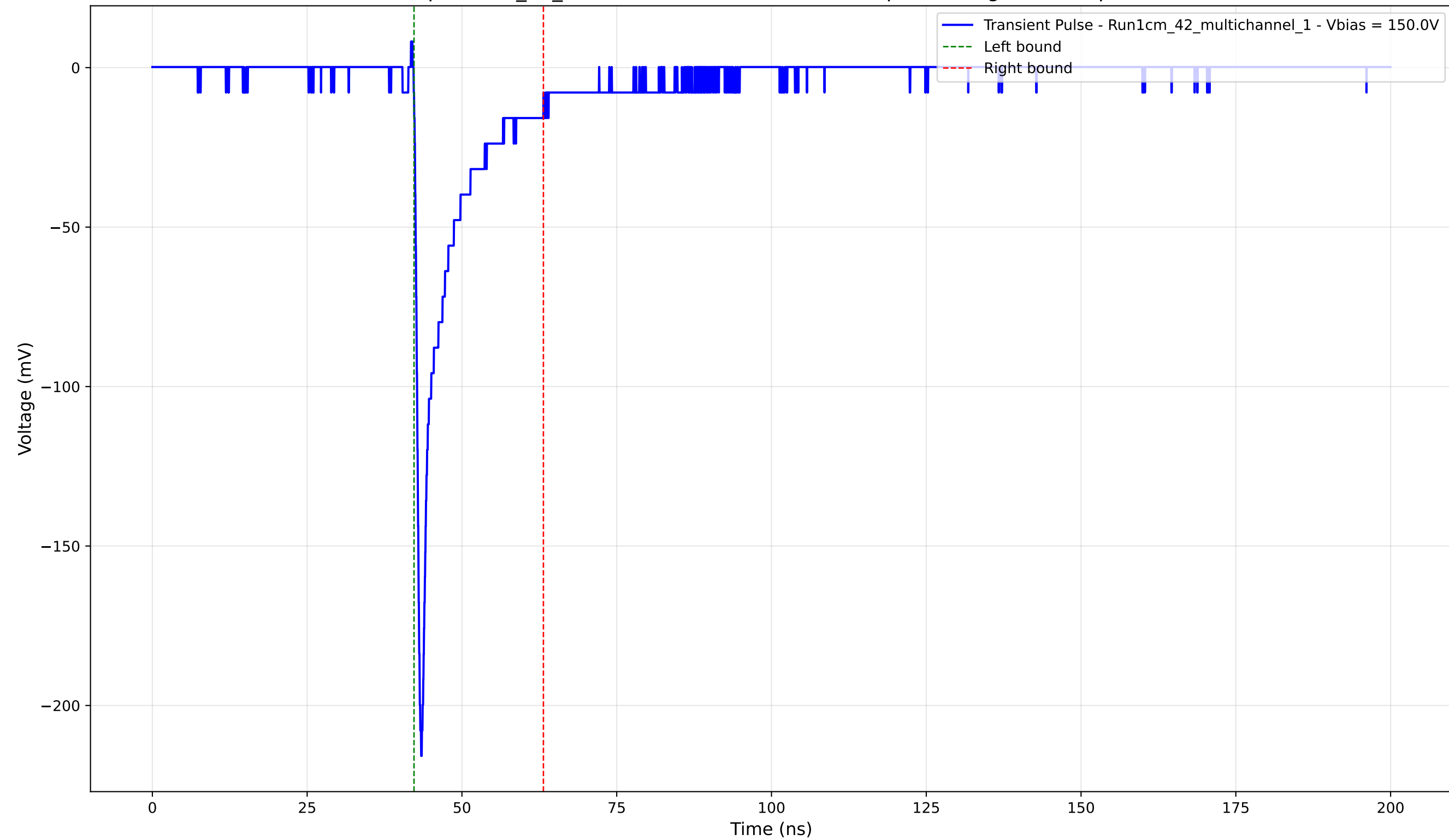
Transient Pulse - Sample: 1cm_42_multichannel - Position: 1955.0 \mu\text{m} - Charge: -20.22 pC - Rise Time: 0.85 ns
