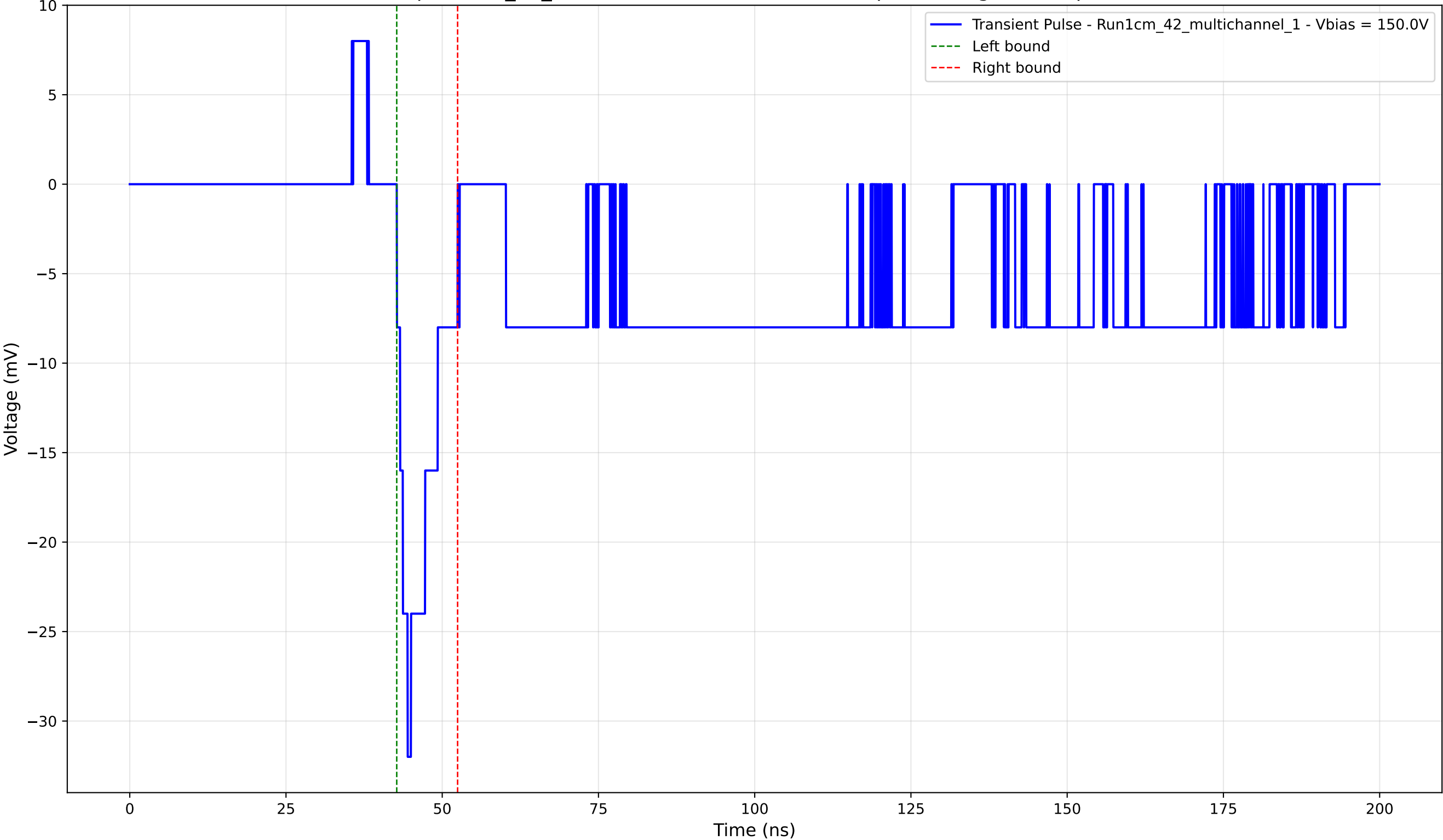
Transient Pulse - Sample: 1cm_42_multichannel - Position: 3855.0 \mu\text{m} - Charge: -3.17 pC - Rise Time: 1.73 ns
