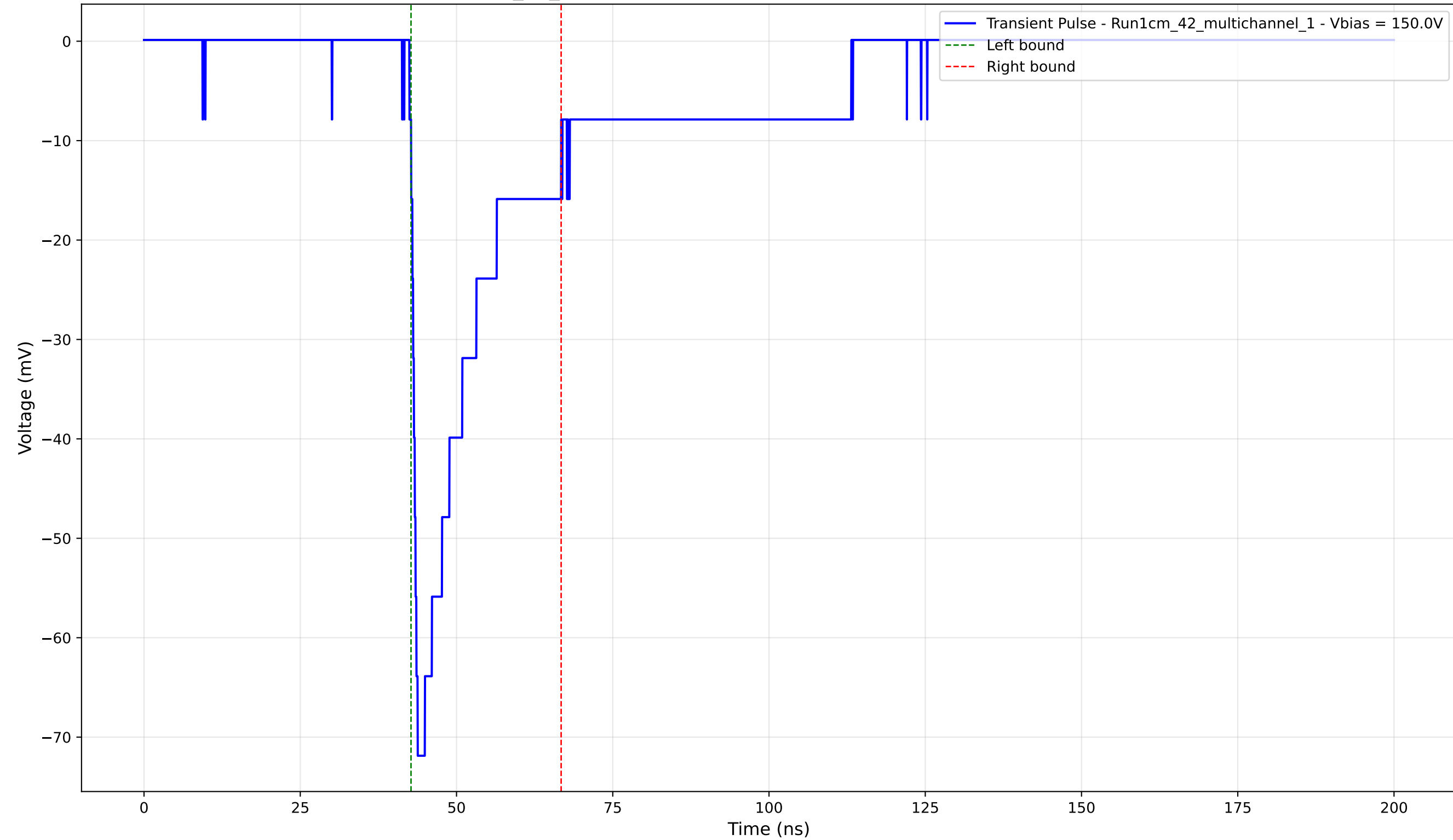
Transient Pulse - Sample: 1cm_42_multichannel - Position: 3560.0 \mu\text{m} - Charge: -14.79 pC - Rise Time: 1.32 ns
