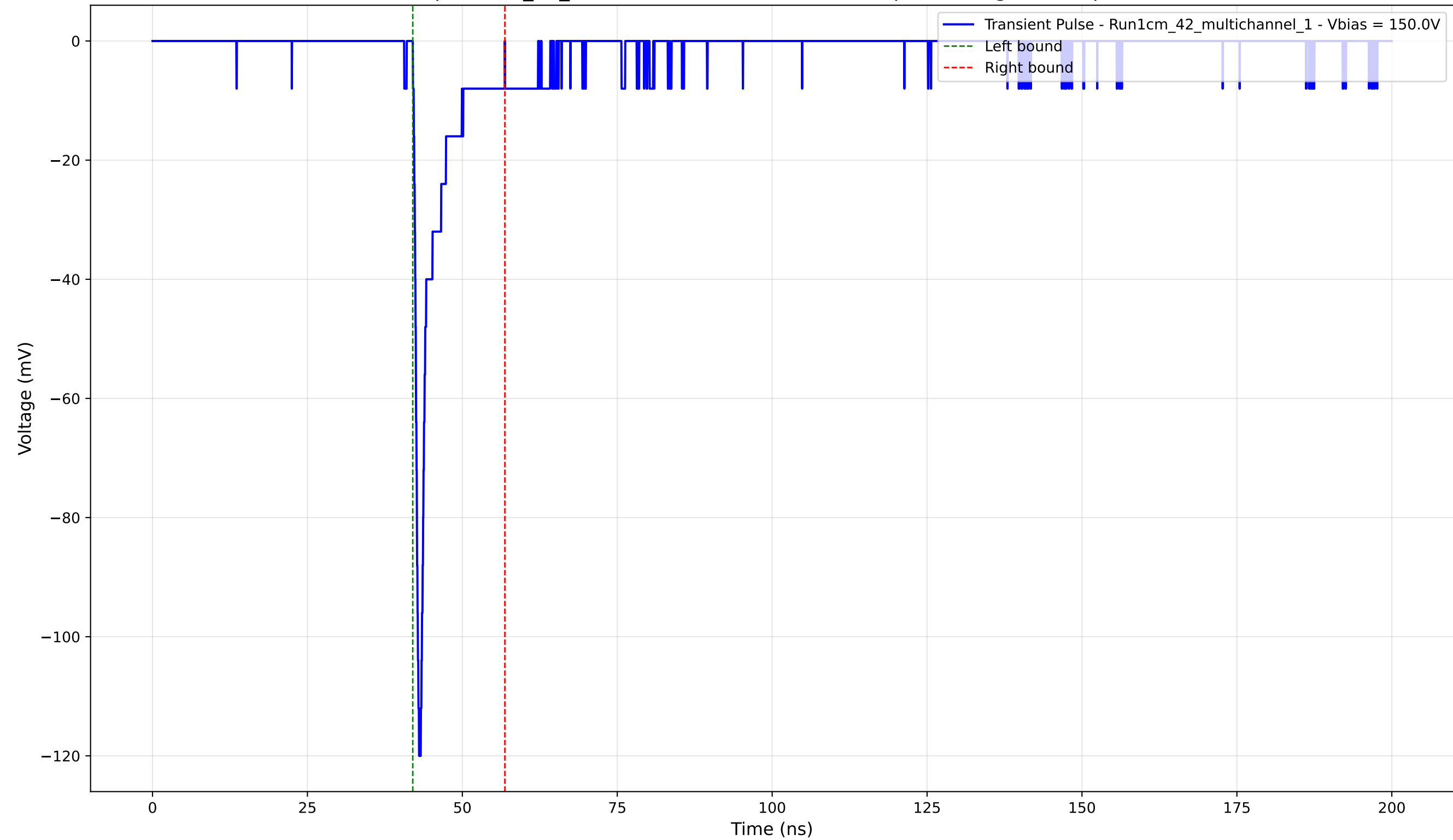
Transient Pulse - Sample: 1cm_42_multichannel - Position: 2430.0 \mu\text{m} - Charge: -7.21 pC - Rise Time: 0.75 ns
