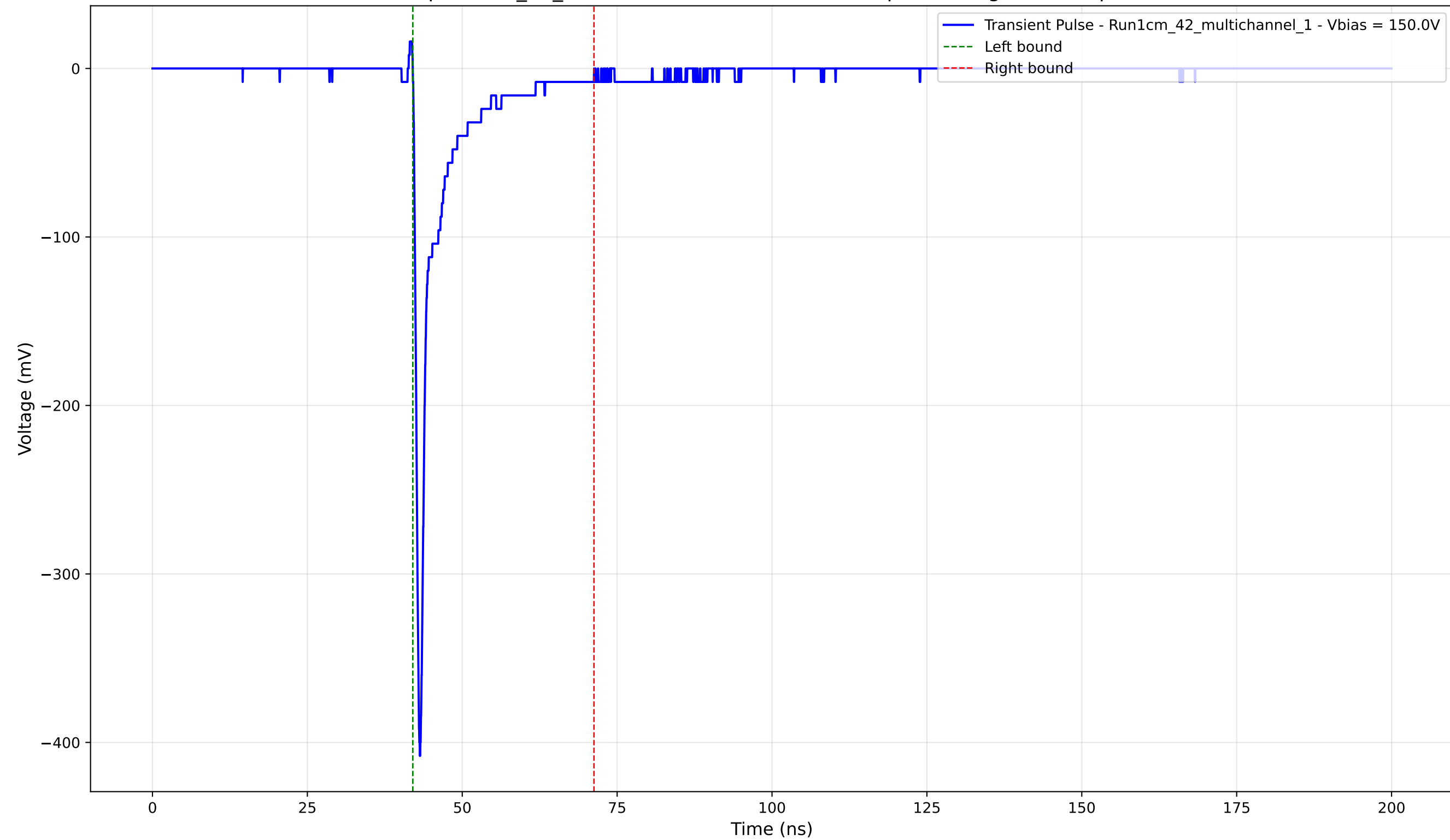
Transient Pulse - Sample: 1cm_42_multichannel - Position: 2280.0 \mu\text{m} - Charge: -26.33 pC - Rise Time: 0.74 ns
