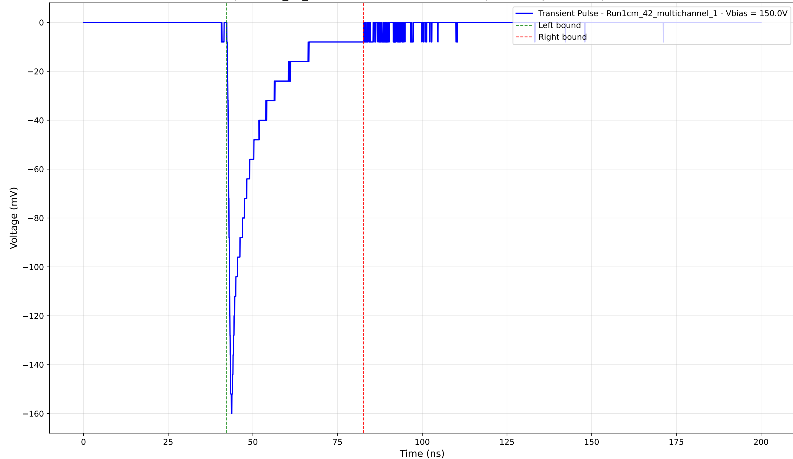
Transient Pulse - Sample: 1cm_42_multichannel - Position: 1670.0 \mu\text{m} - Charge: -25.15 pC - Rise Time: 0.86 ns
