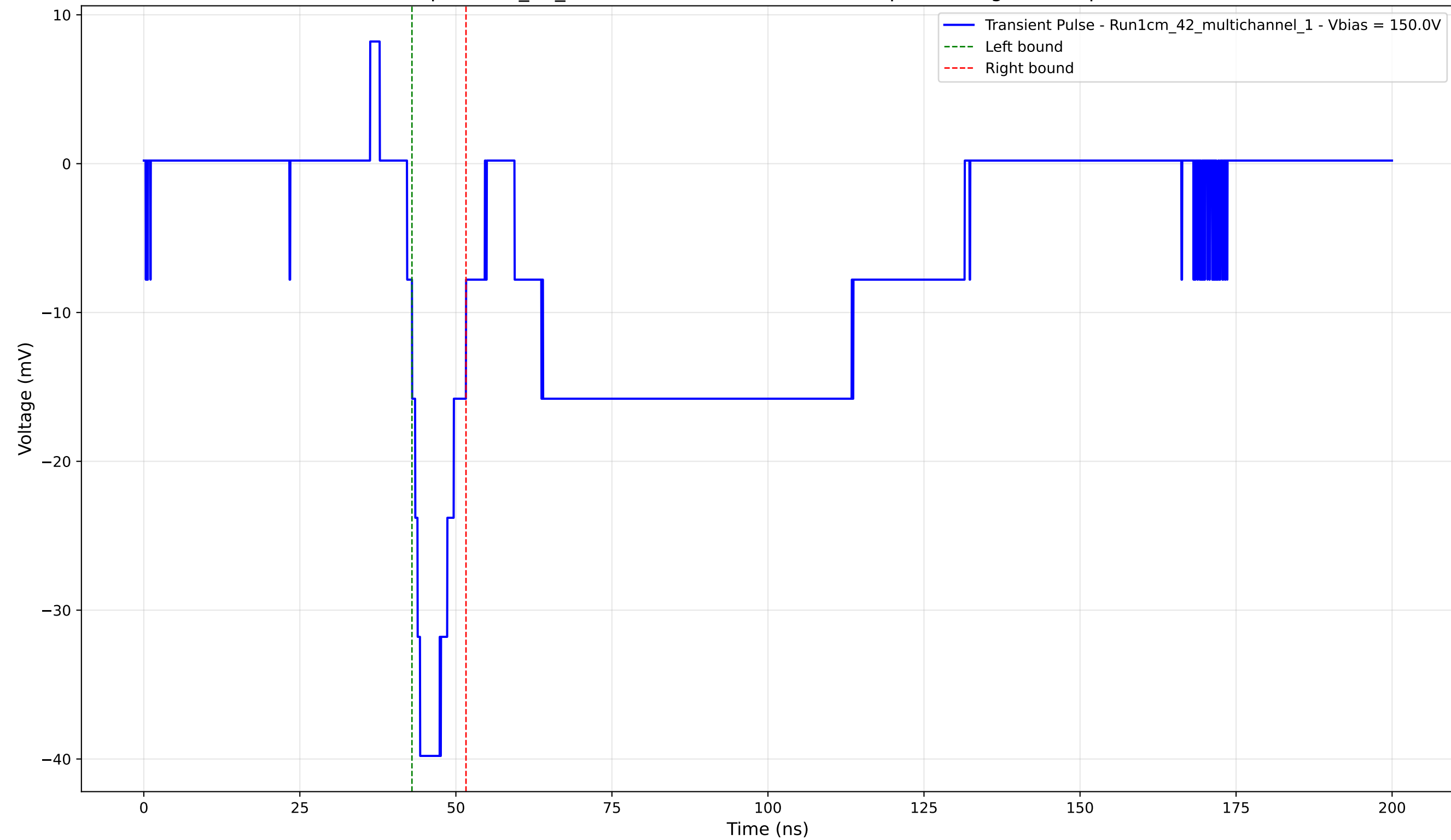
Transient Pulse - Sample: 1cm_42_multichannel - Position: 4735.0 \mu\text{m} - Charge: -5.01 pC - Rise Time: 2.09 ns
