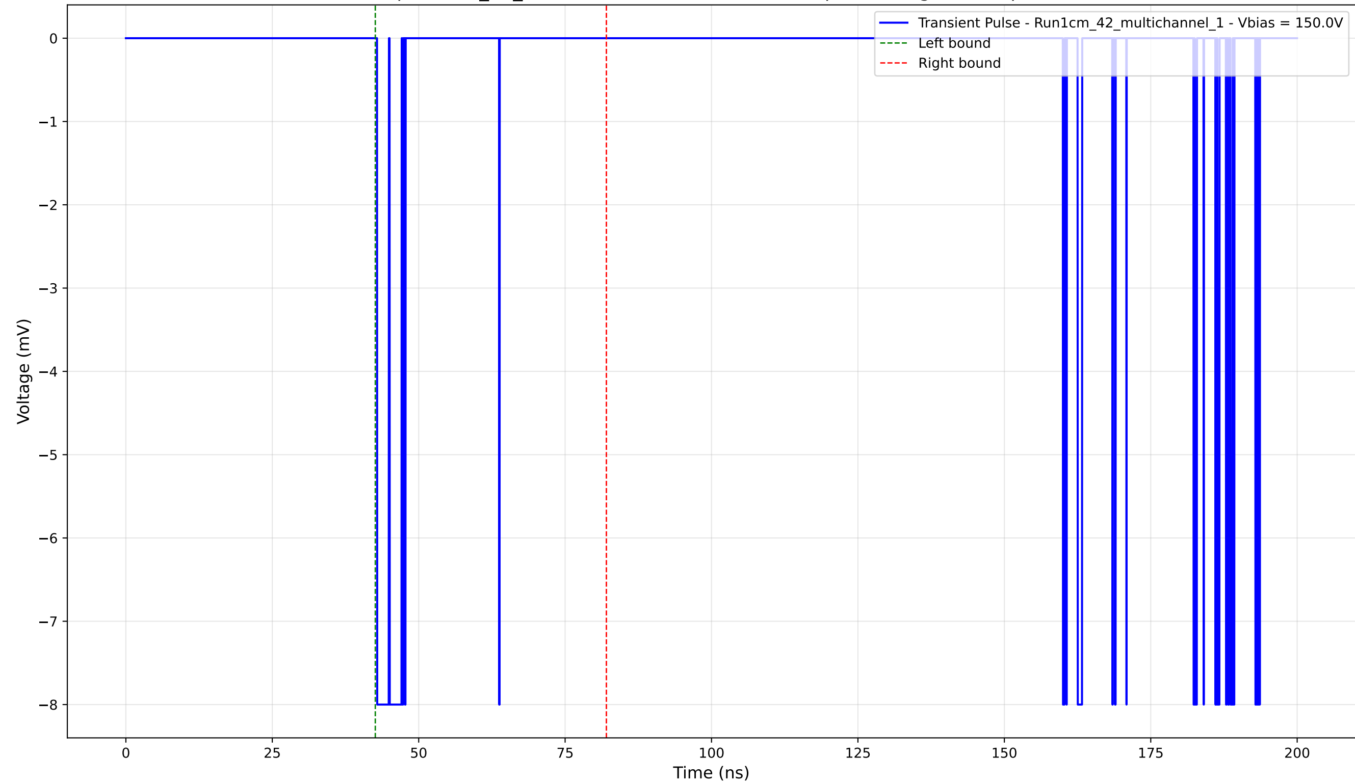
Transient Pulse - Sample: 1cm_42_multichannel - Position: 3410.0 \mu\text{m} - Charge: -0.70 pC - Rise Time: 0.02 ns
