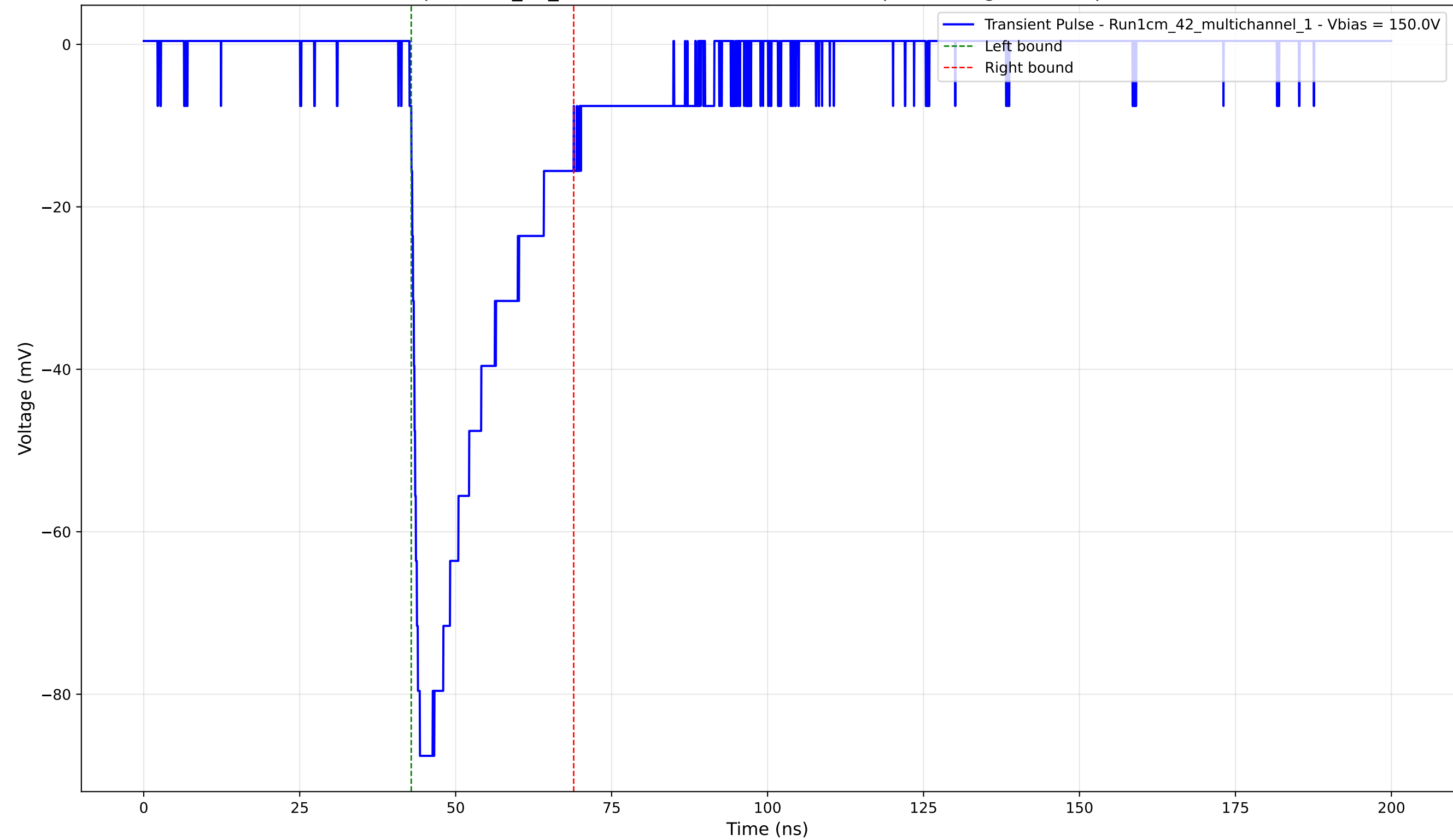
Transient Pulse - Sample: 1cm_42_multichannel - Position: 1095.0 \mu\text{m} - Charge: -22.31 pC - Rise Time: 1.06 ns
