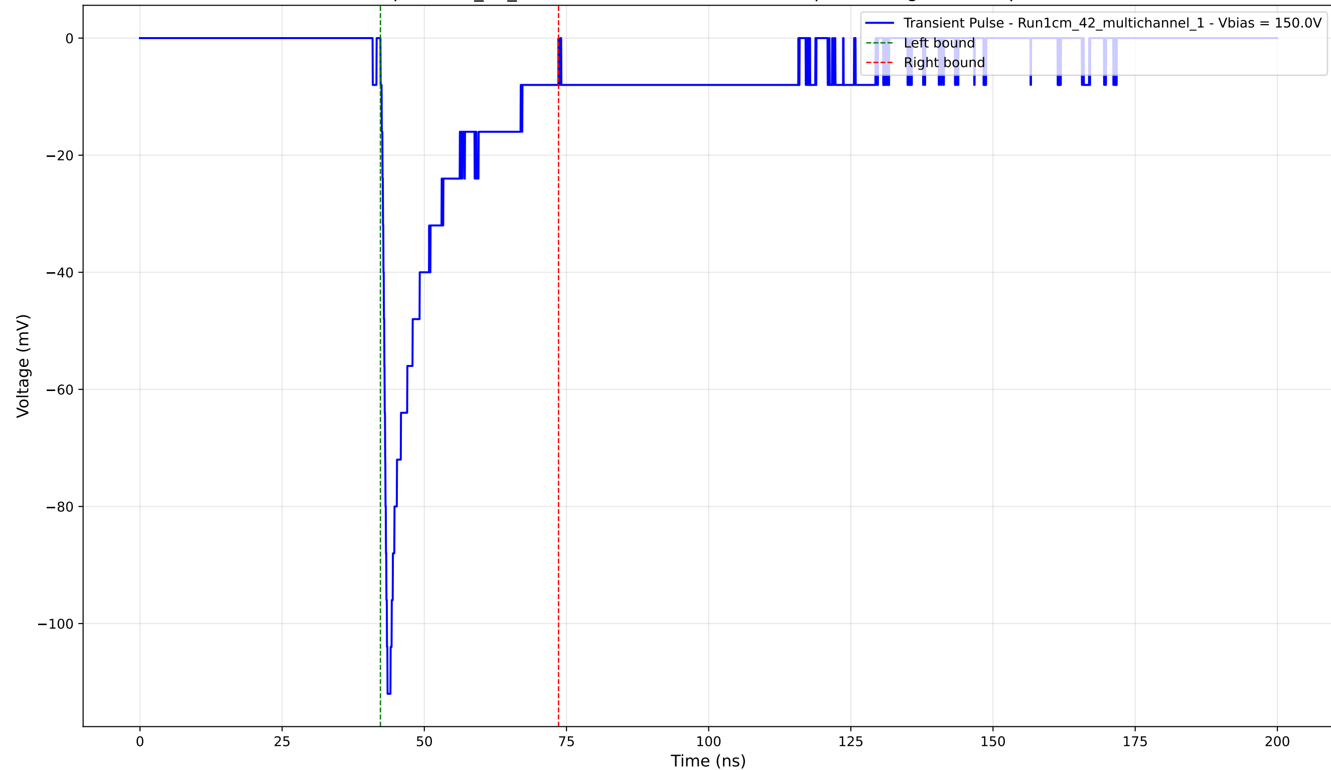
Transient Pulse - Sample: 1cm_42_multichannel - Position: 3225.0 \mu\text{m} - Charge: -18.09 pC - Rise Time: 0.93 ns
