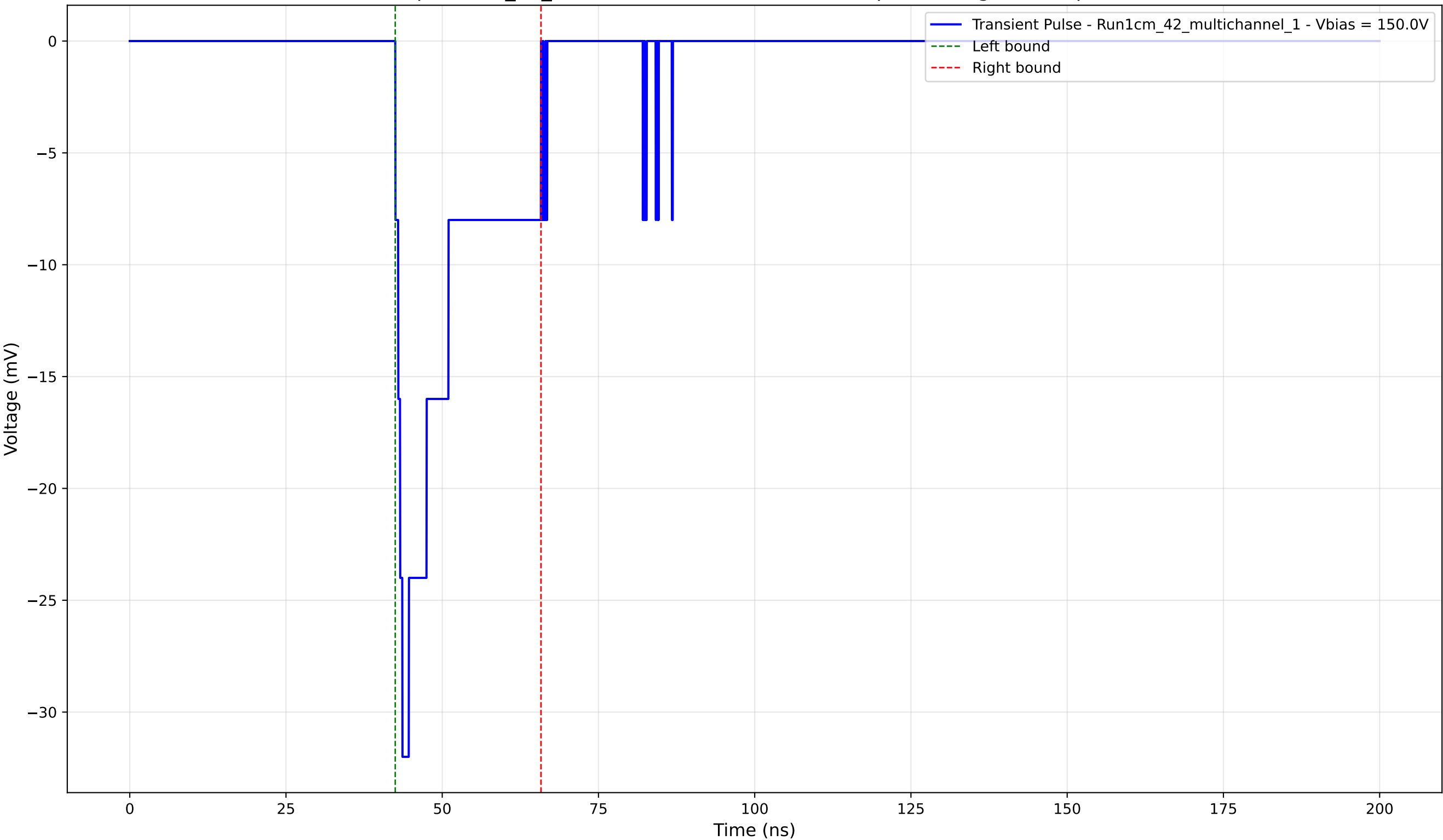
Transient Pulse - Sample: 1cm_42_multichannel - Position: 3445.0 \mu\text{m} - Charge: -5.86 pC - Rise Time: 1.13 ns
