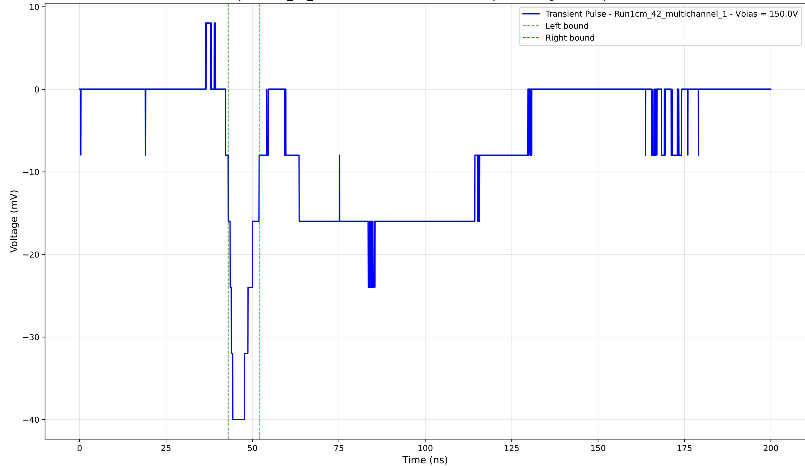
Transient Pulse - Sample: 1cm_42_multichannel - Position: 4705.0 \mu\text{m} - Charge: -5.21 pC - Rise Time: 2.11 ns
