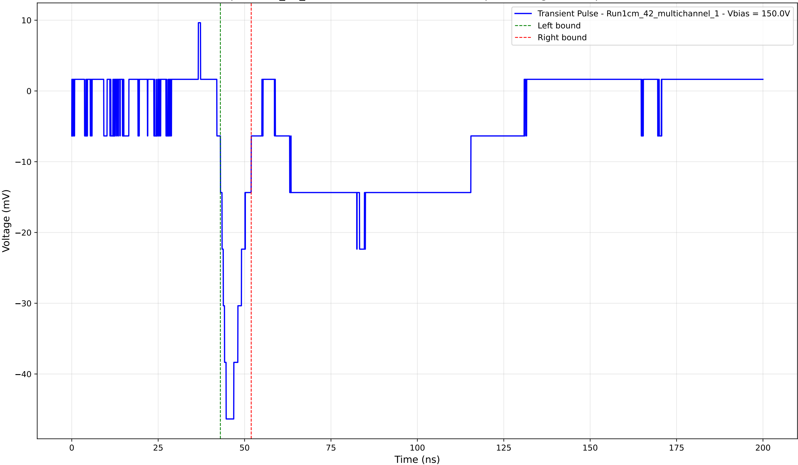
Transient Pulse - Sample: 1cm_42_multichannel - Position: 4540.0 \mu\text{m} - Charge: -5.44 pC - Rise Time: 2.69 ns
