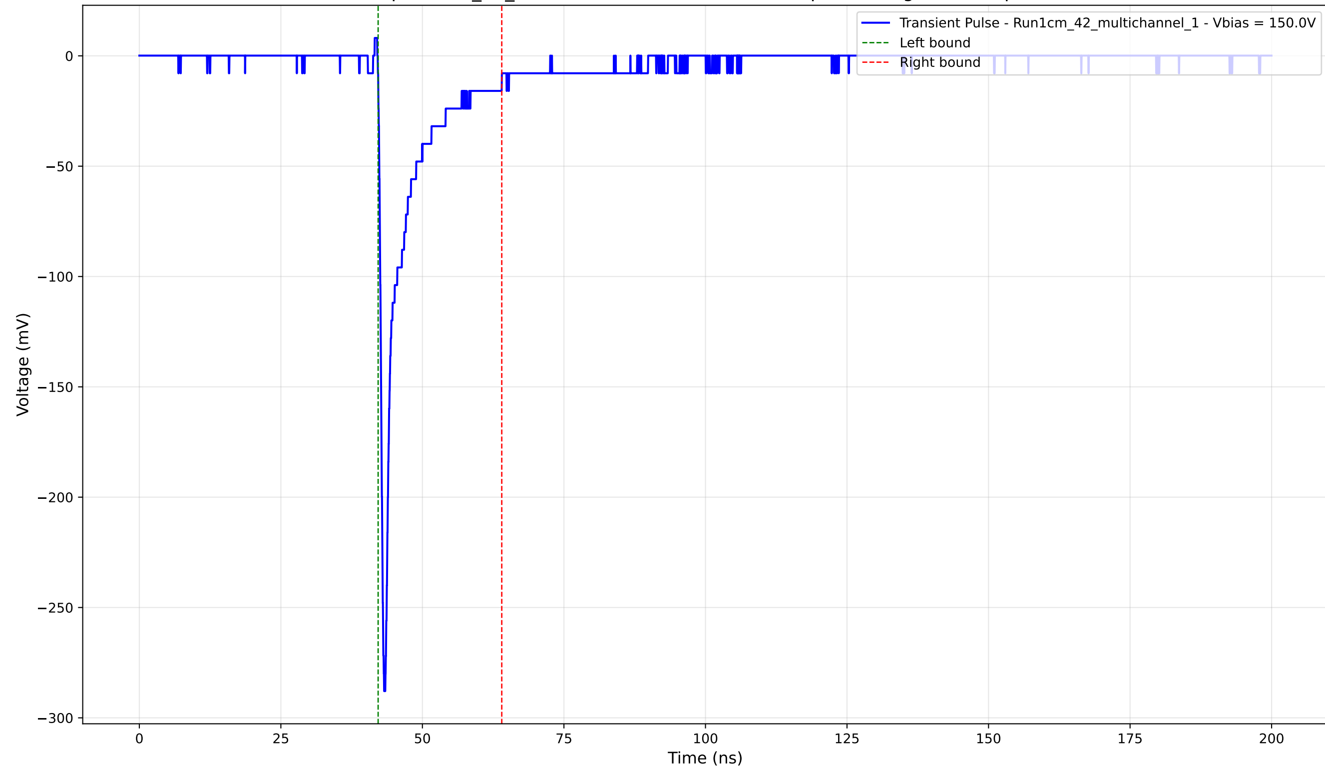
Transient Pulse - Sample: 1cm_42_multichannel - Position: 2695.0 \mu\text{m} - Charge: -23.49 pC - Rise Time: 0.79 ns
