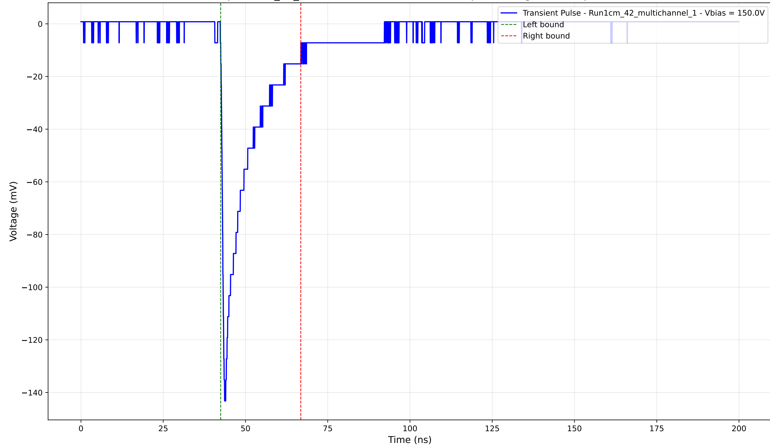
Transient Pulse - Sample: 1cm_42_multichannel - Position: 1595.0 \mu\text{m} - Charge: -22.63 pC - Rise Time: 1.02 ns
