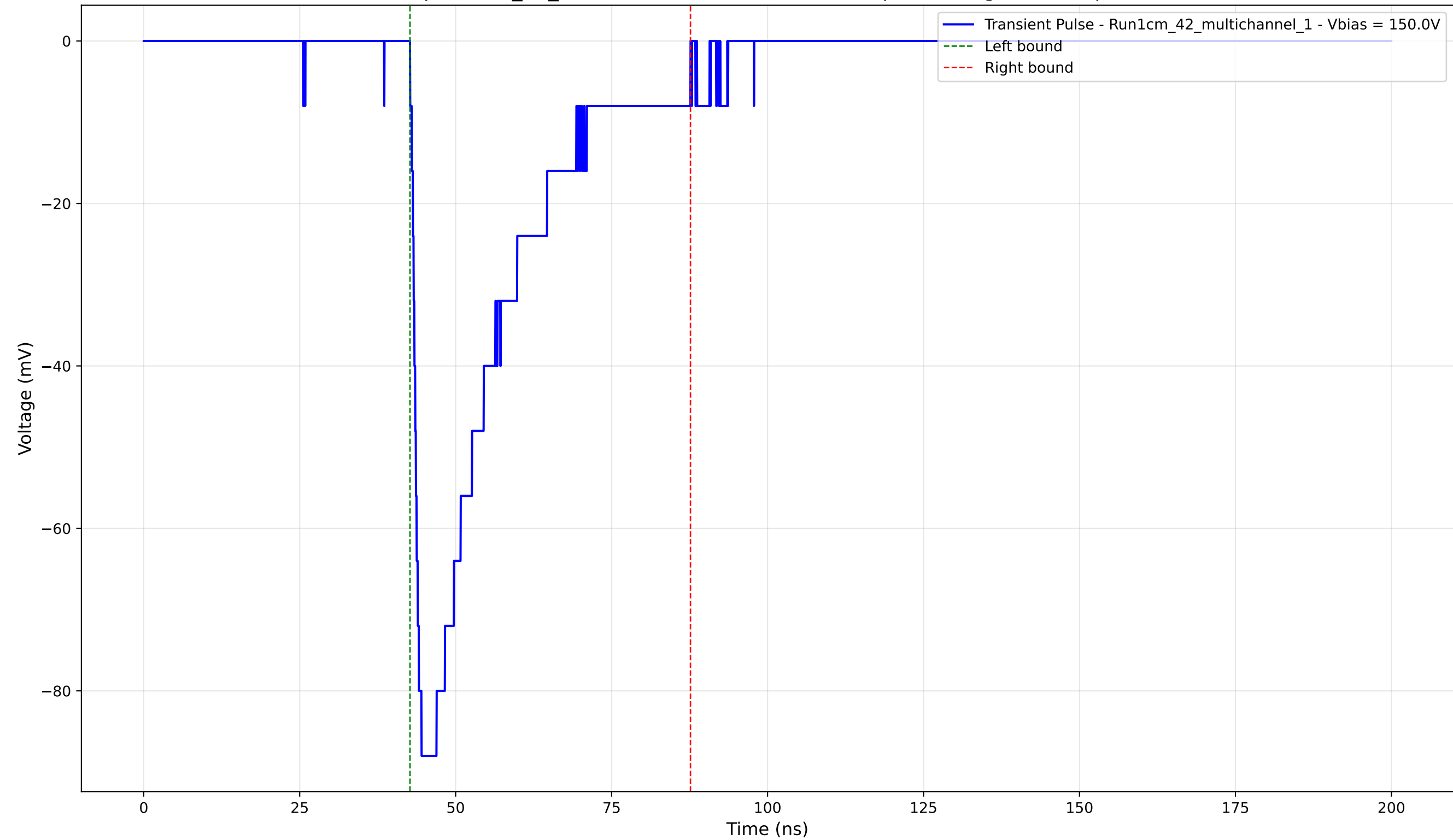
Transient Pulse - Sample: 1cm_42_multichannel - Position: 1010.0 \mu\text{m} - Charge: -26.10 pC - Rise Time: 1.16 ns
