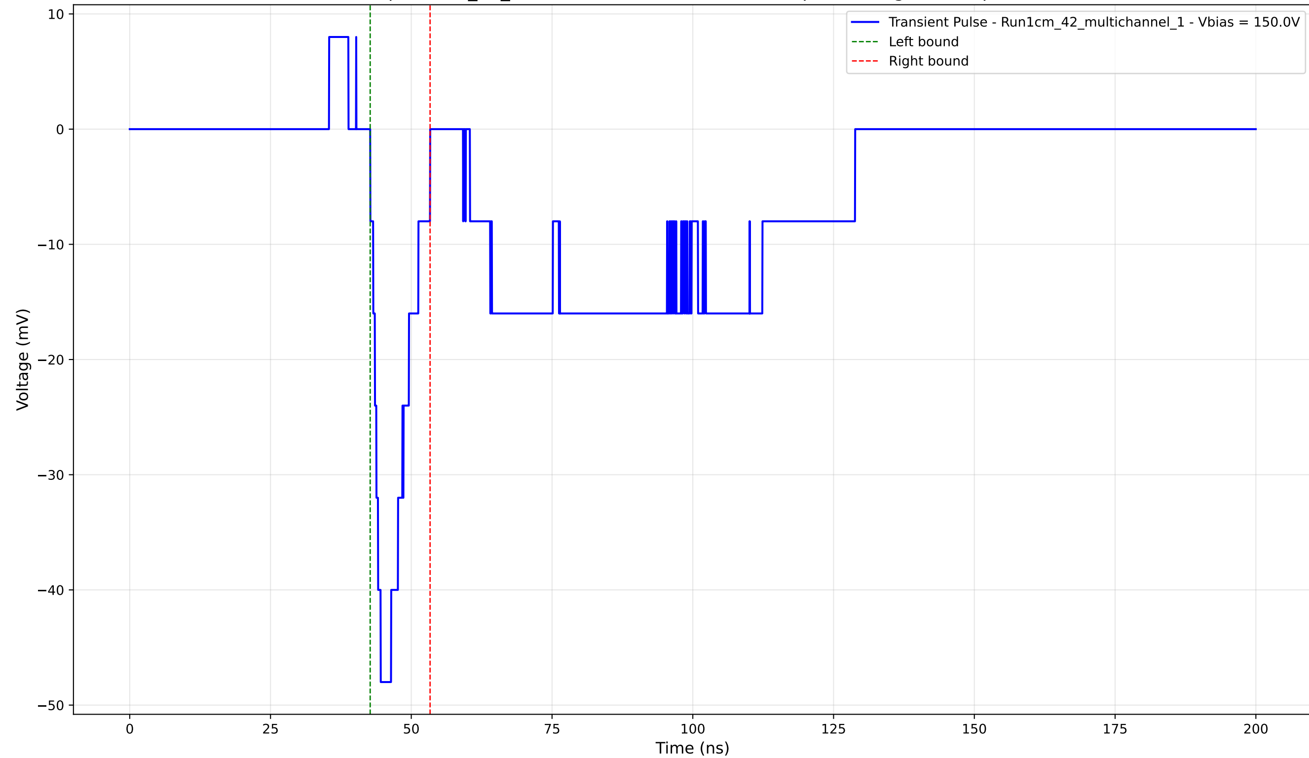
Transient Pulse - Sample: 1cm_42_multichannel - Position: 4170.0 \mu\text{m} - Charge: -5.57 pC - Rise Time: 1.85 ns
