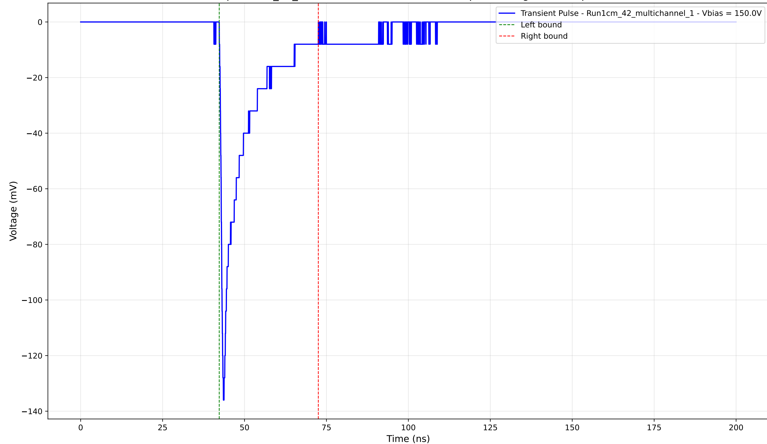
Transient Pulse - Sample: 1cm_42_multichannel - Position: 3105.0 \mu\text{m} - Charge: -19.08 pC - Rise Time: 0.99 ns
