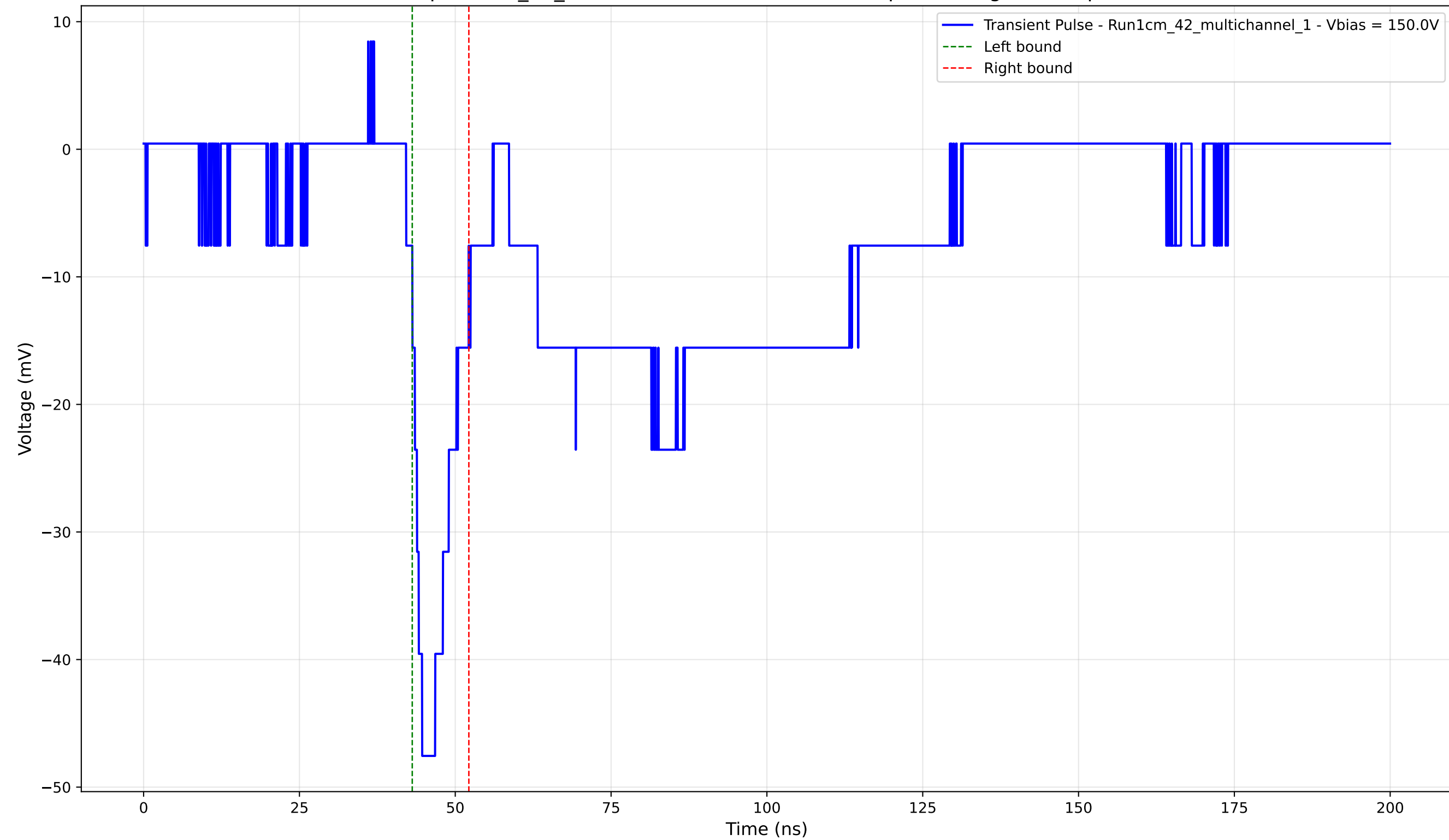
Transient Pulse - Sample: 1cm_42_multichannel - Position: 4570.0 \mu\text{m} - Charge: -5.69 pC - Rise Time: 2.57 ns
