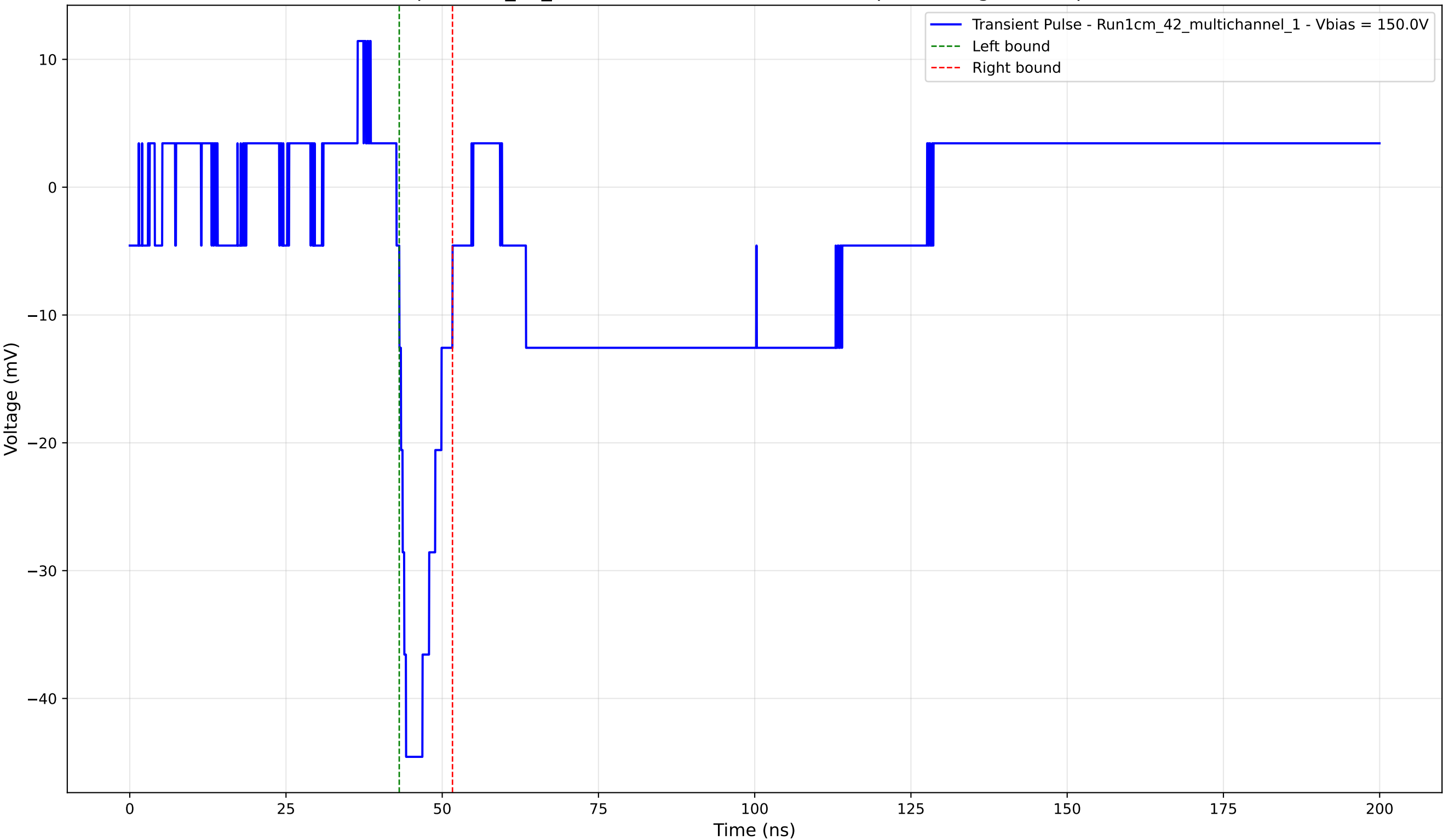
Transient Pulse - Sample: 1cm_42_multichannel - Position: 4050.0 \mu\text{m} - Charge: -5.07 pC - Rise Time: 1.52 ns
