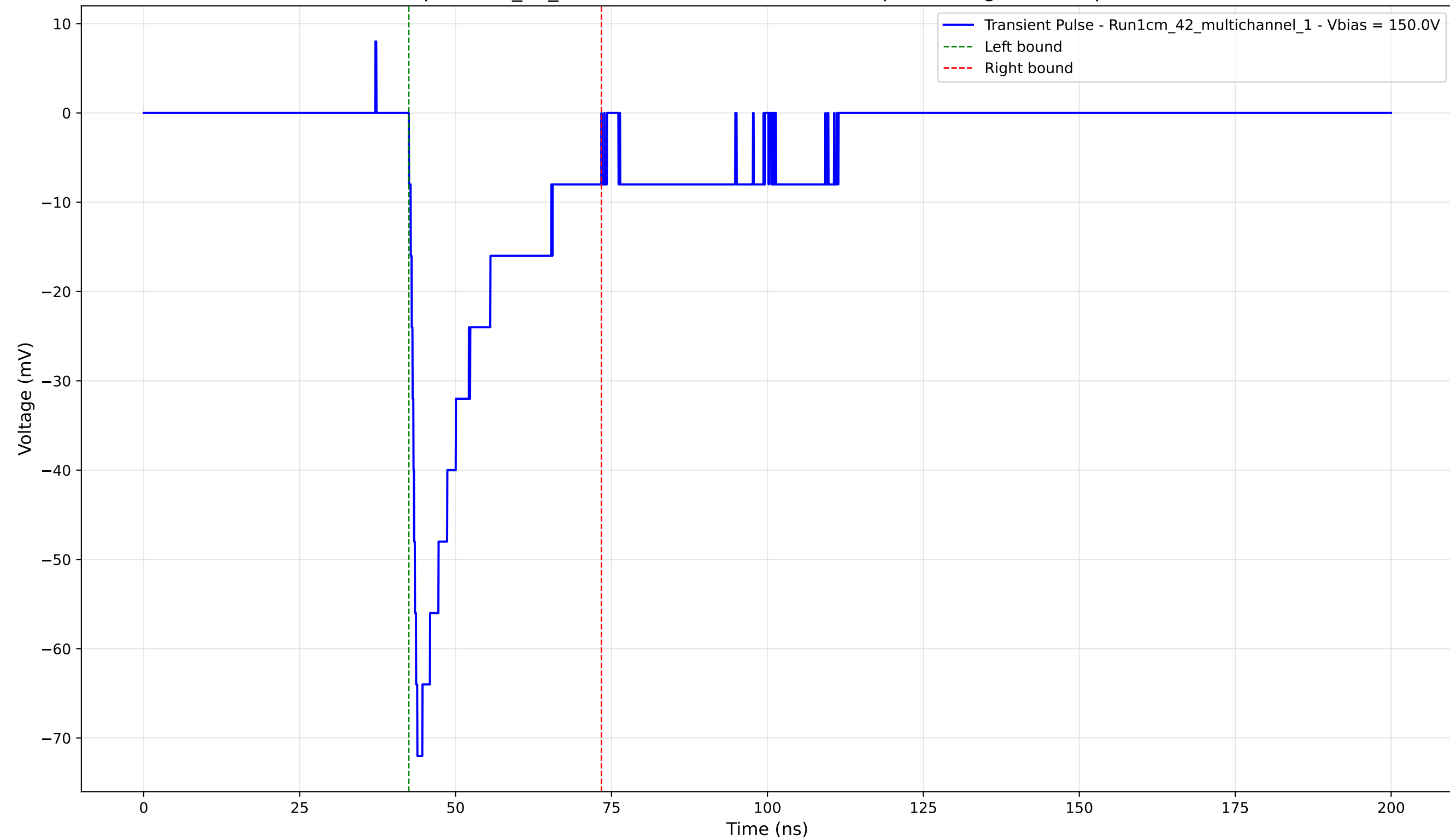
Transient Pulse - Sample: 1cm_42_multichannel - Position: 3575.0 \mu\text{m} - Charge: -15.08 pC - Rise Time: 1.34 ns
