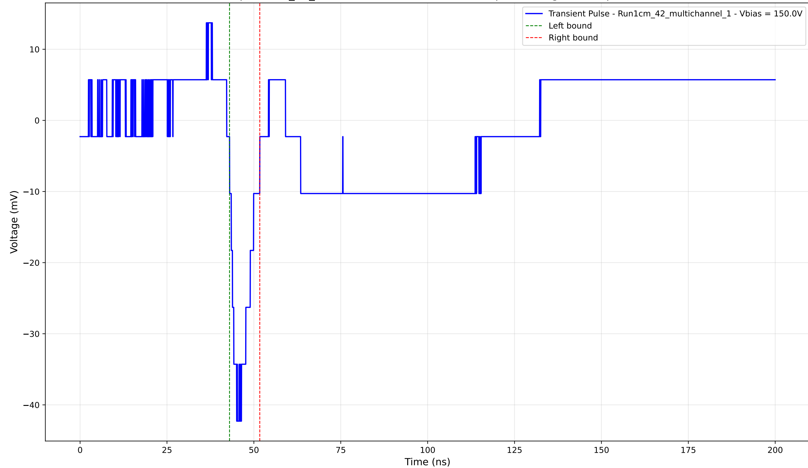
Transient Pulse - Sample: 1cm_42_multichannel - Position: 4685.0 \mu\text{m} - Charge: -4.37 pC - Rise Time: 2.04 ns
