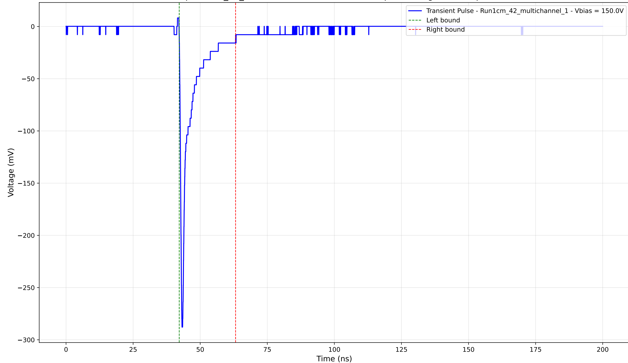
Transient Pulse - Sample: 1cm_42_multichannel - Position: 2680.0 \mu\text{m} - Charge: -22.64 pC - Rise Time: 0.77 ns
