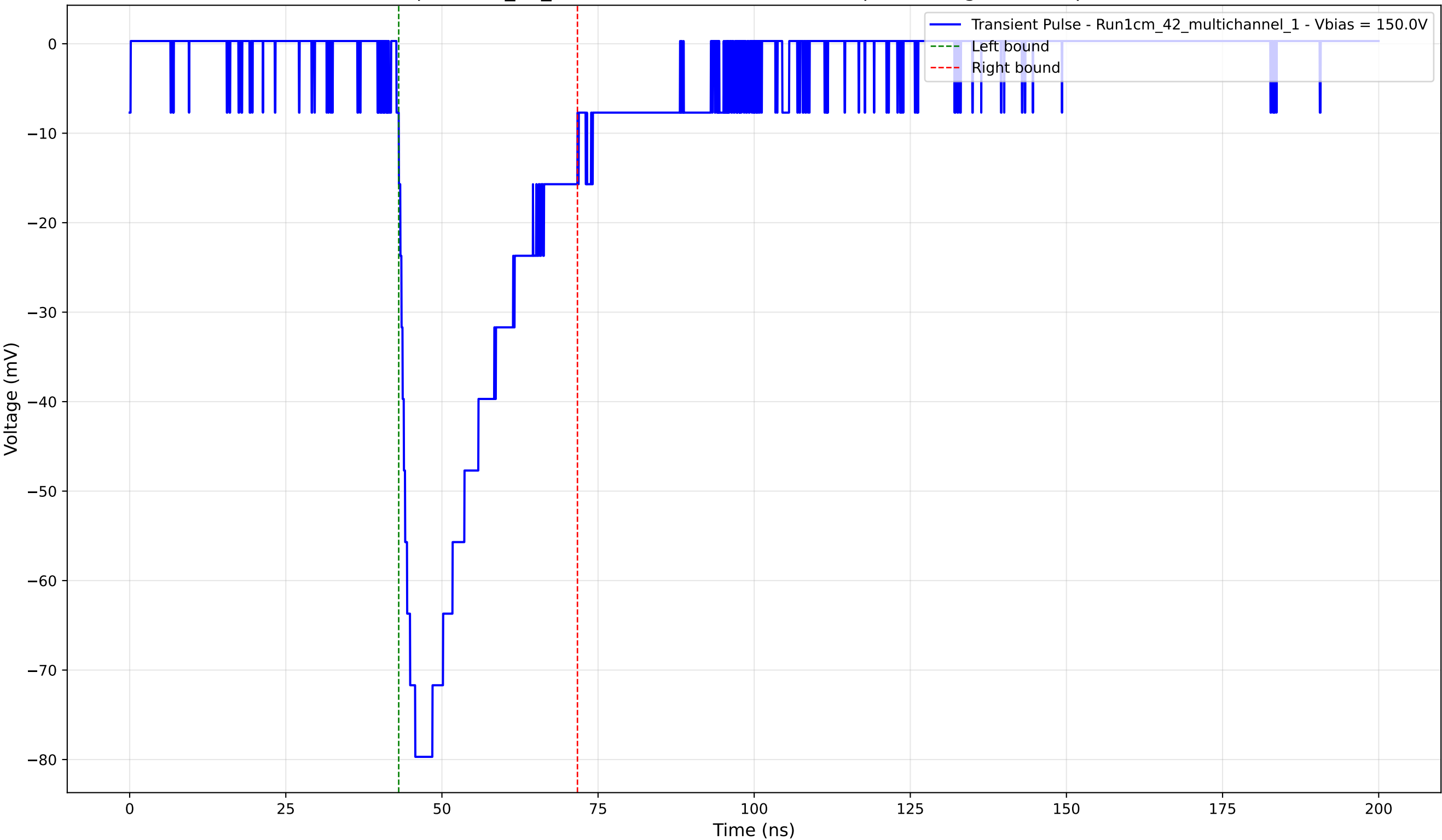
Transient Pulse - Sample: 1cm_42_multichannel - Position: 545.0 \mu\text{m} - Charge: -23.71 pC - Rise Time: 2.64 ns
