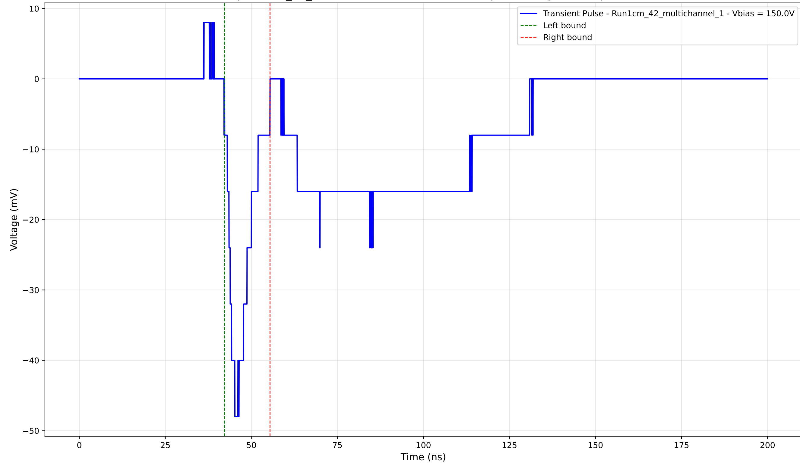
Transient Pulse - Sample: 1cm_42_multichannel - Position: 4695.0 \mu\text{m} - Charge: -6.10 pC - Rise Time: 2.97 ns
