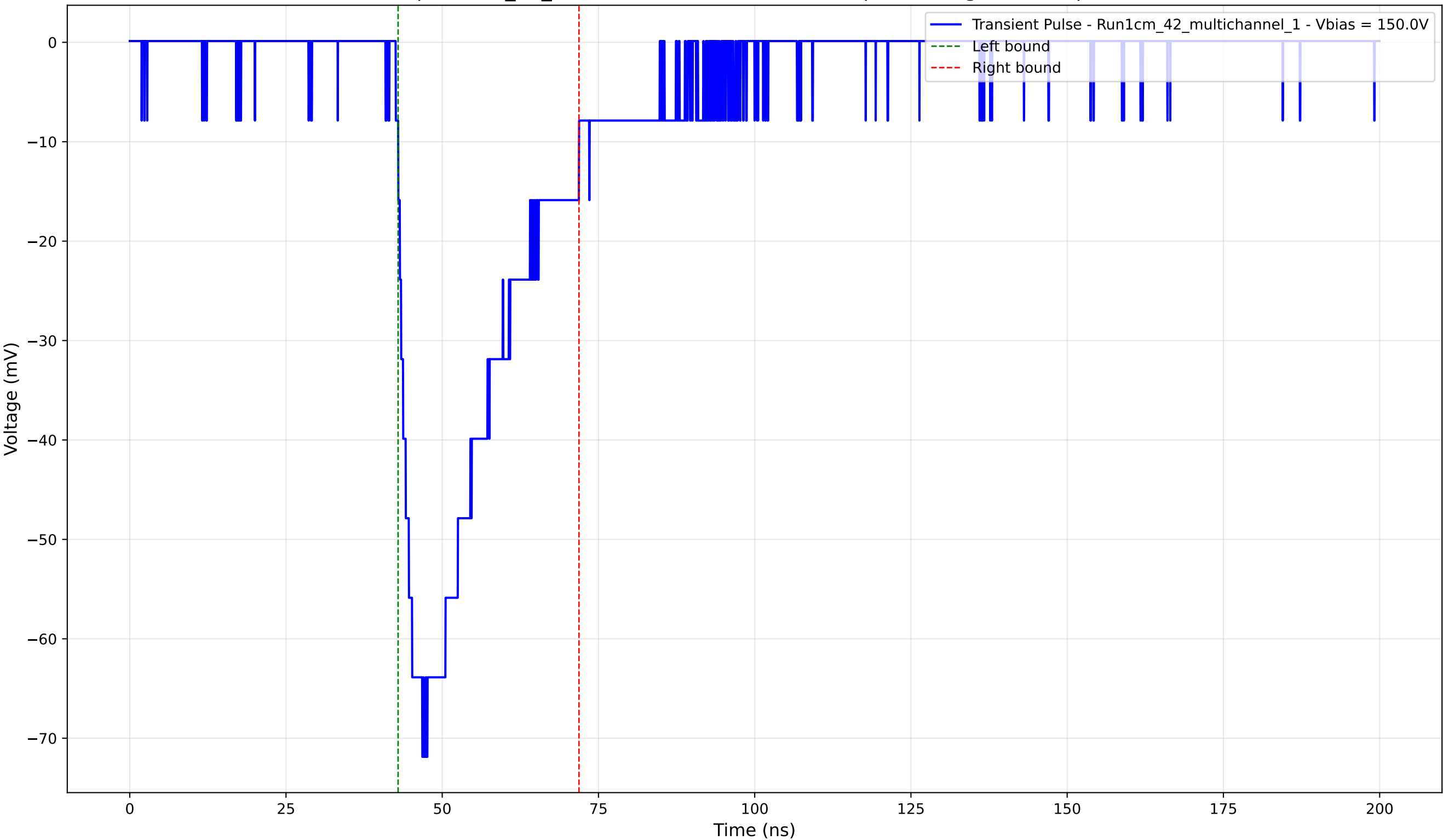
Transient Pulse - Sample: 1cm_42_multichannel - Position: 170.0 \mu\text{m} - Charge: -21.45 pC - Rise Time: 4.24 ns
