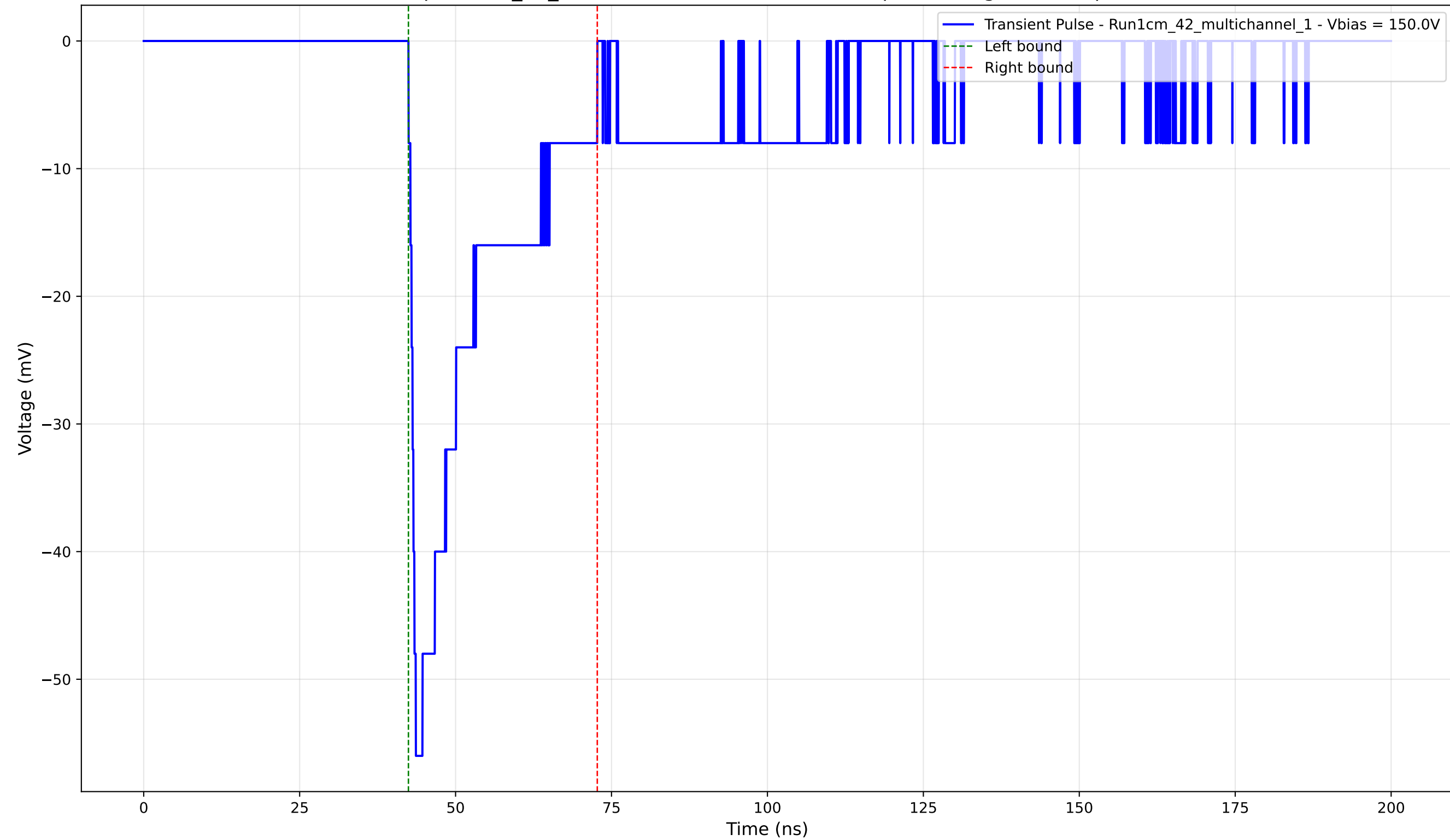
Transient Pulse - Sample: 1cm_42_multichannel - Position: 3460.0 \mu\text{m} - Charge: -12.58 pC - Rise Time: 1.17 ns
