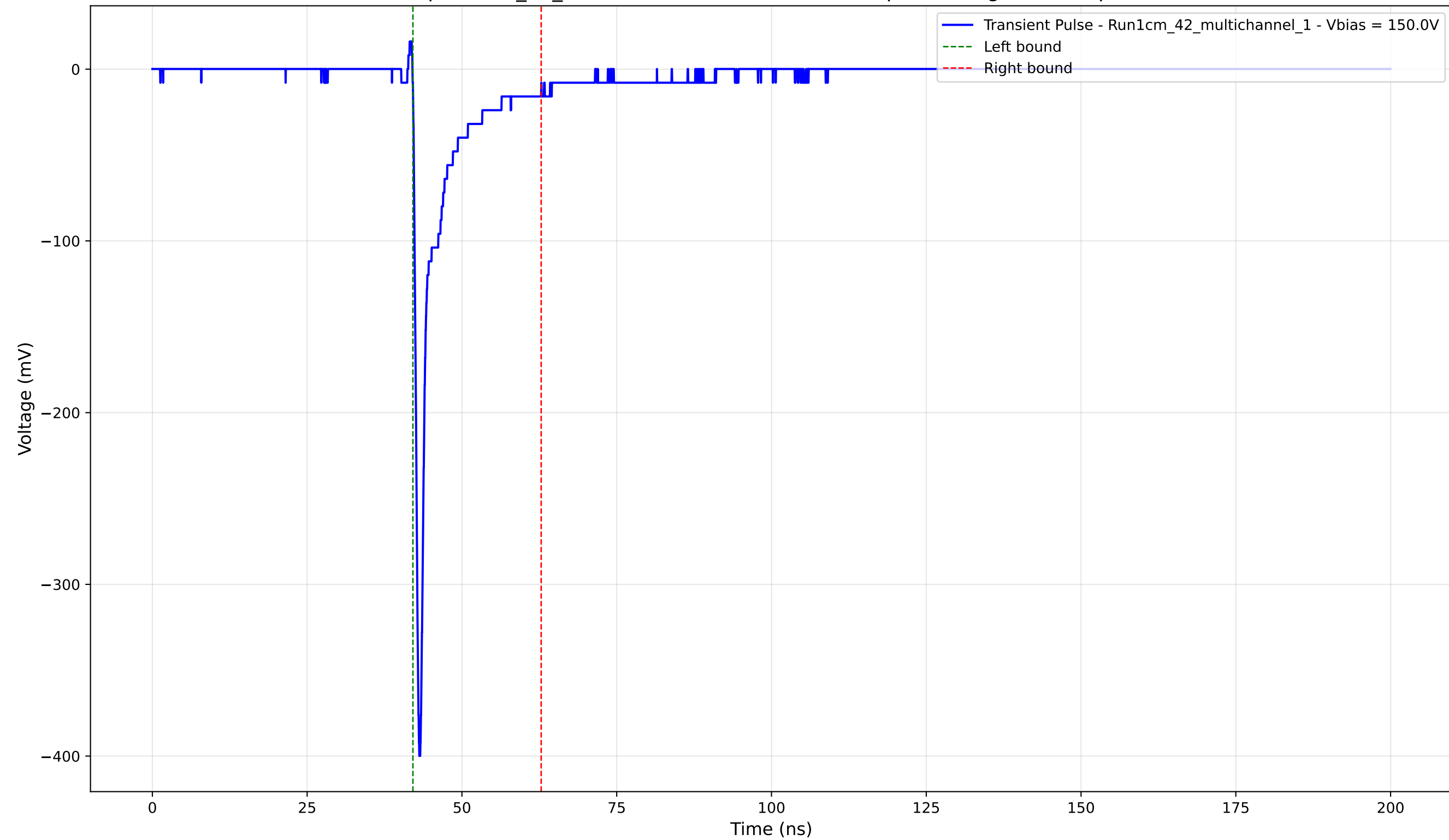
Transient Pulse - Sample: 1cm_42_multichannel - Position: 2275.0 \mu\text{m} - Charge: -25.26 pC - Rise Time: 0.74 ns
