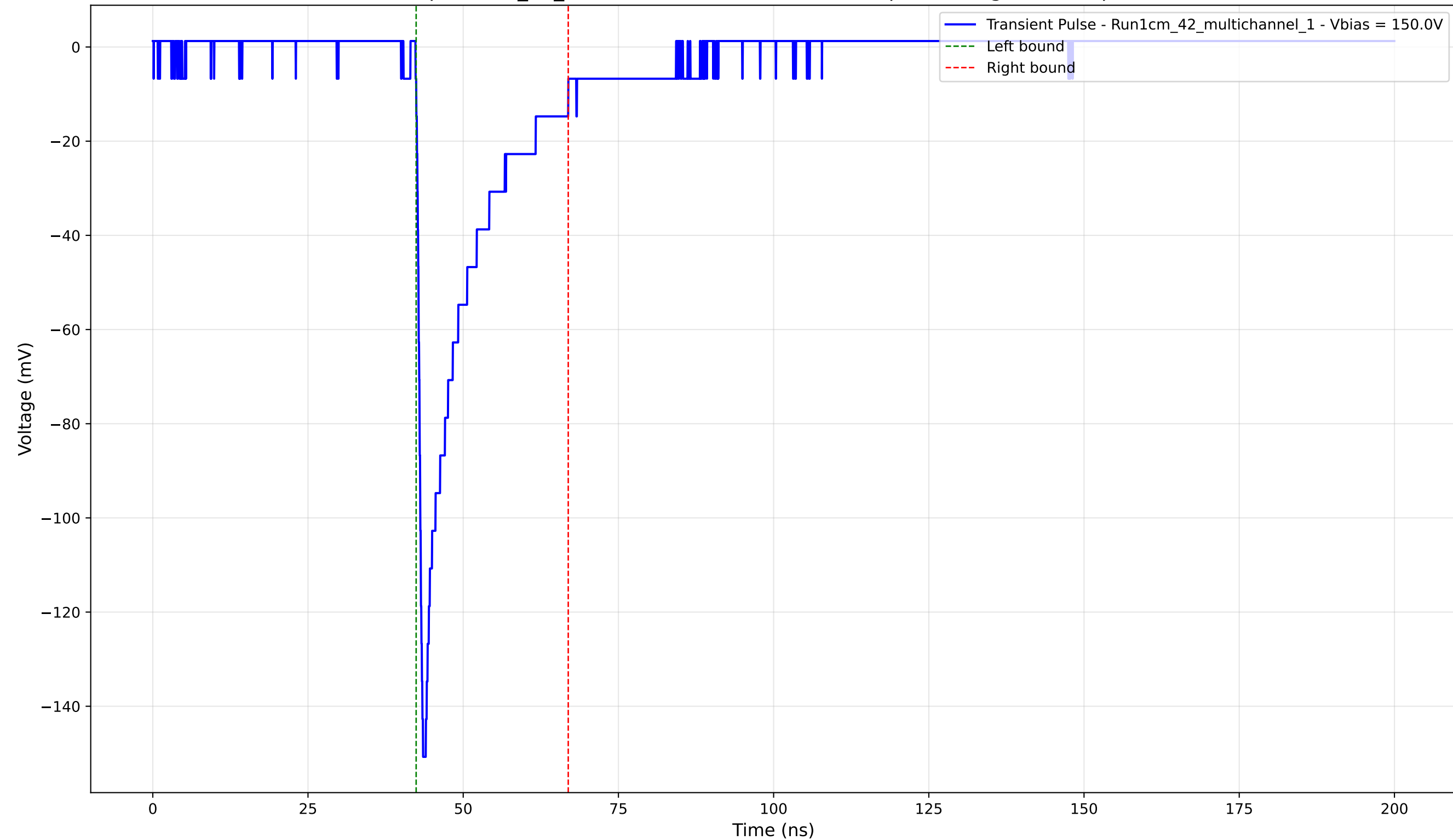
Transient Pulse - Sample: 1cm_42_multichannel - Position: 1645.0 \mu\text{m} - Charge: -22.37 pC - Rise Time: 0.90 ns
