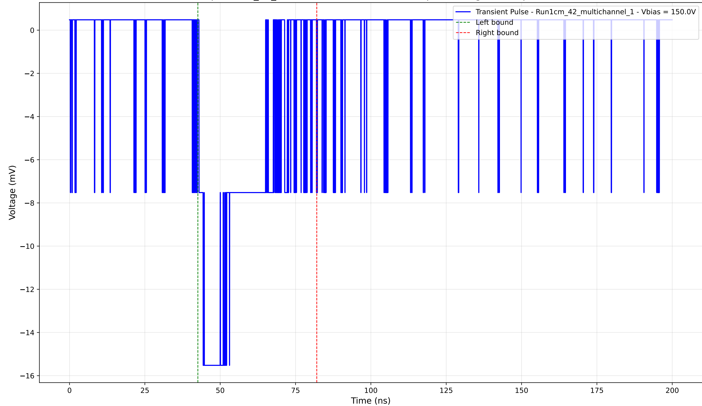
Transient Pulse - Sample: 1cm_42_multichannel - Position: 325.0 \mu\text{m} - Charge: -5.25 pC - Rise Time: 1.40 ns
