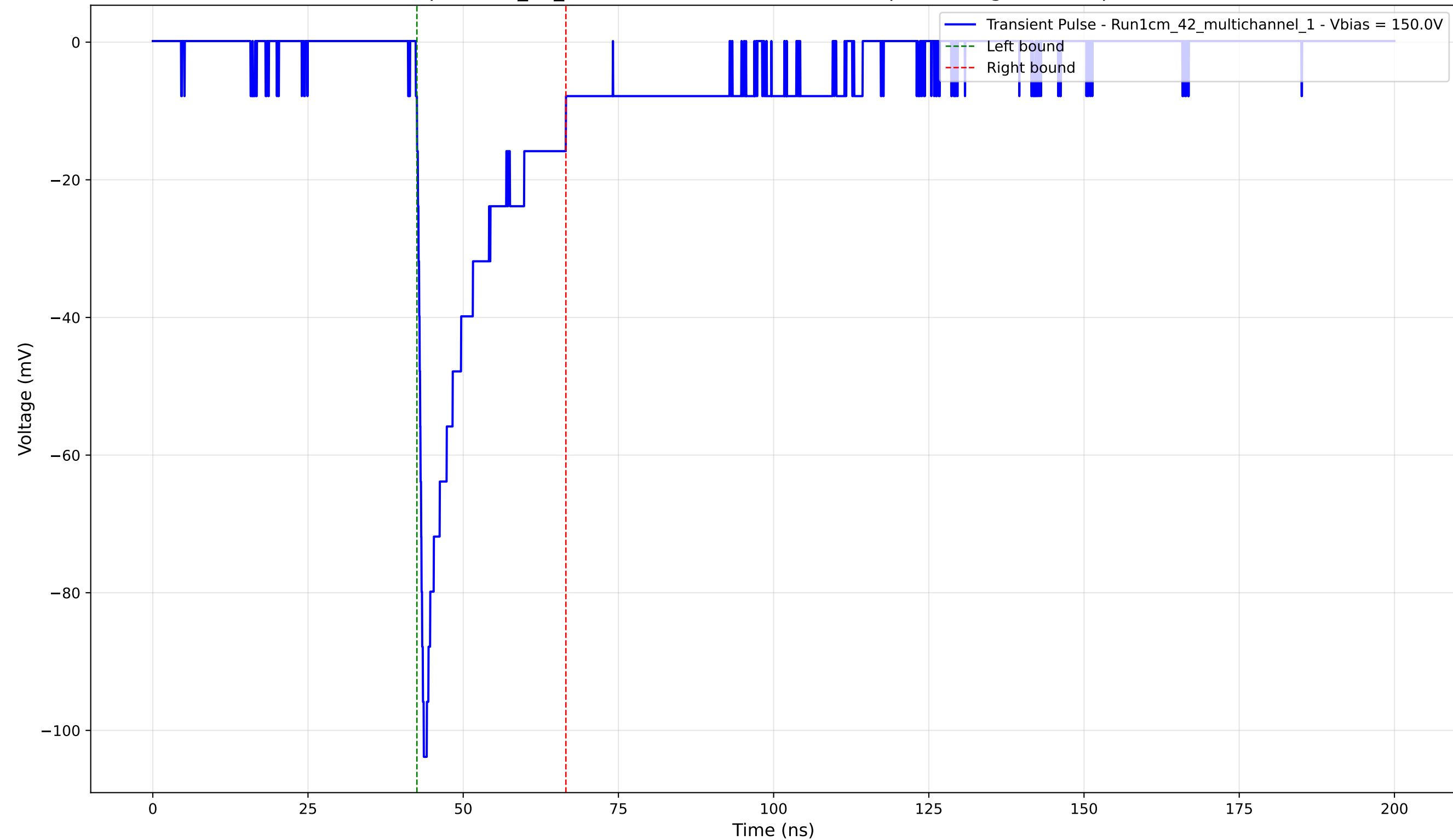
Transient Pulse - Sample: 1cm_42_multichannel - Position: 3295.0 \mu\text{m} - Charge: -17.30 pC - Rise Time: 0.95 ns
