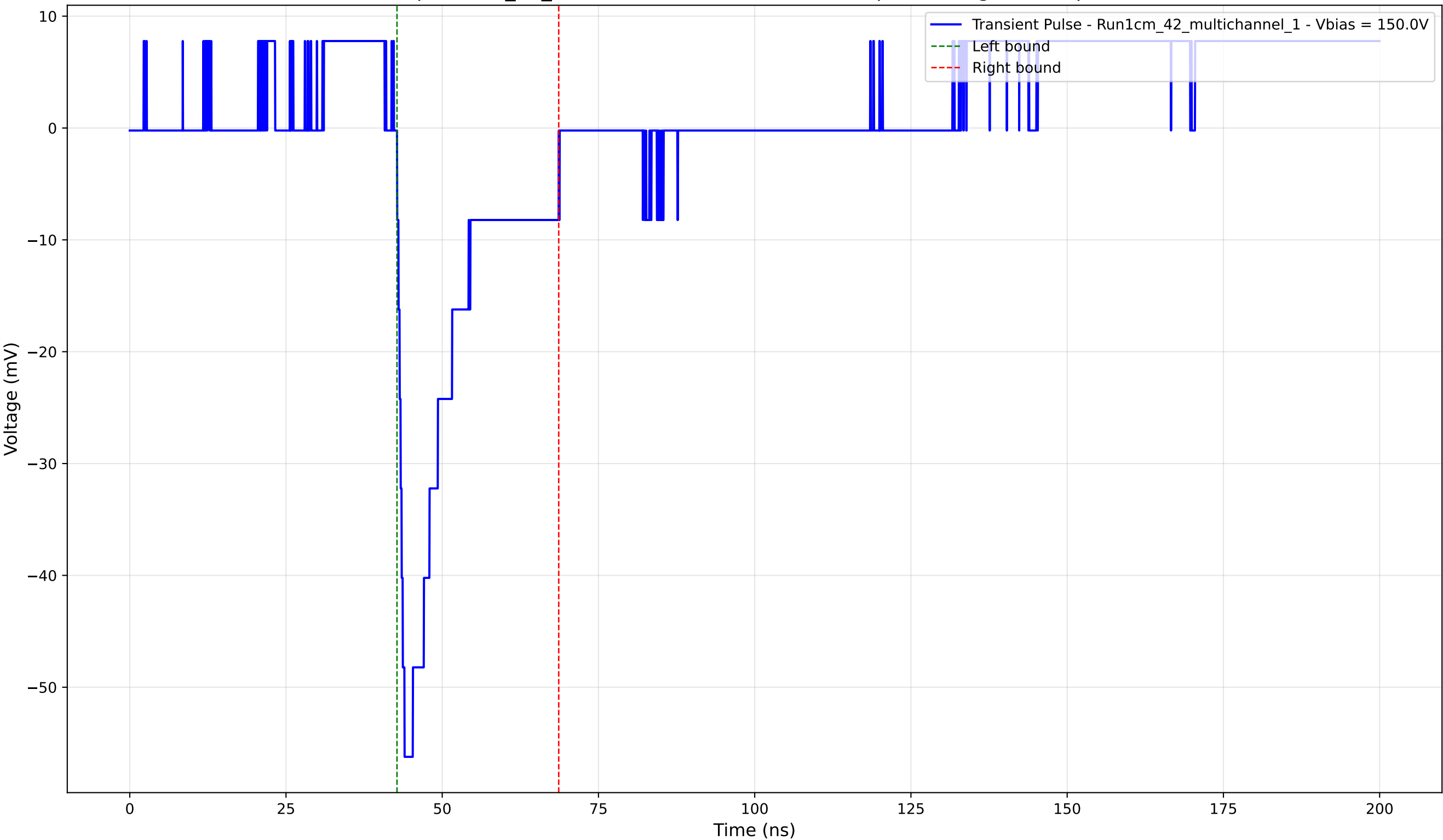
Transient Pulse - Sample: 1cm_42_multichannel - Position: 3690.0 \mu\text{m} - Charge: -9.85 pC - Rise Time: 1.19 ns
