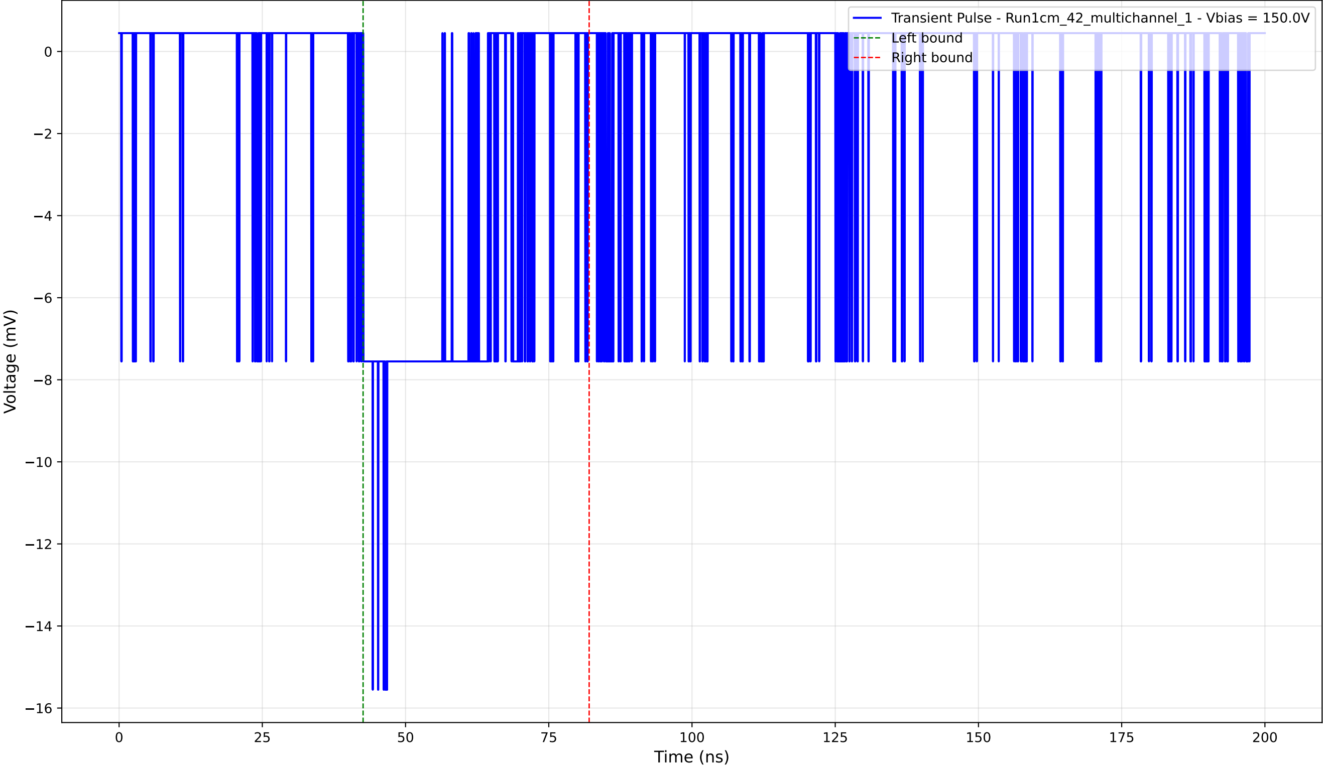
Transient Pulse - Sample: 1cm_42_multichannel - Position: 1350.0 \mu\text{m} - Charge: -3.51 pC - Rise Time: 1.64 ns
