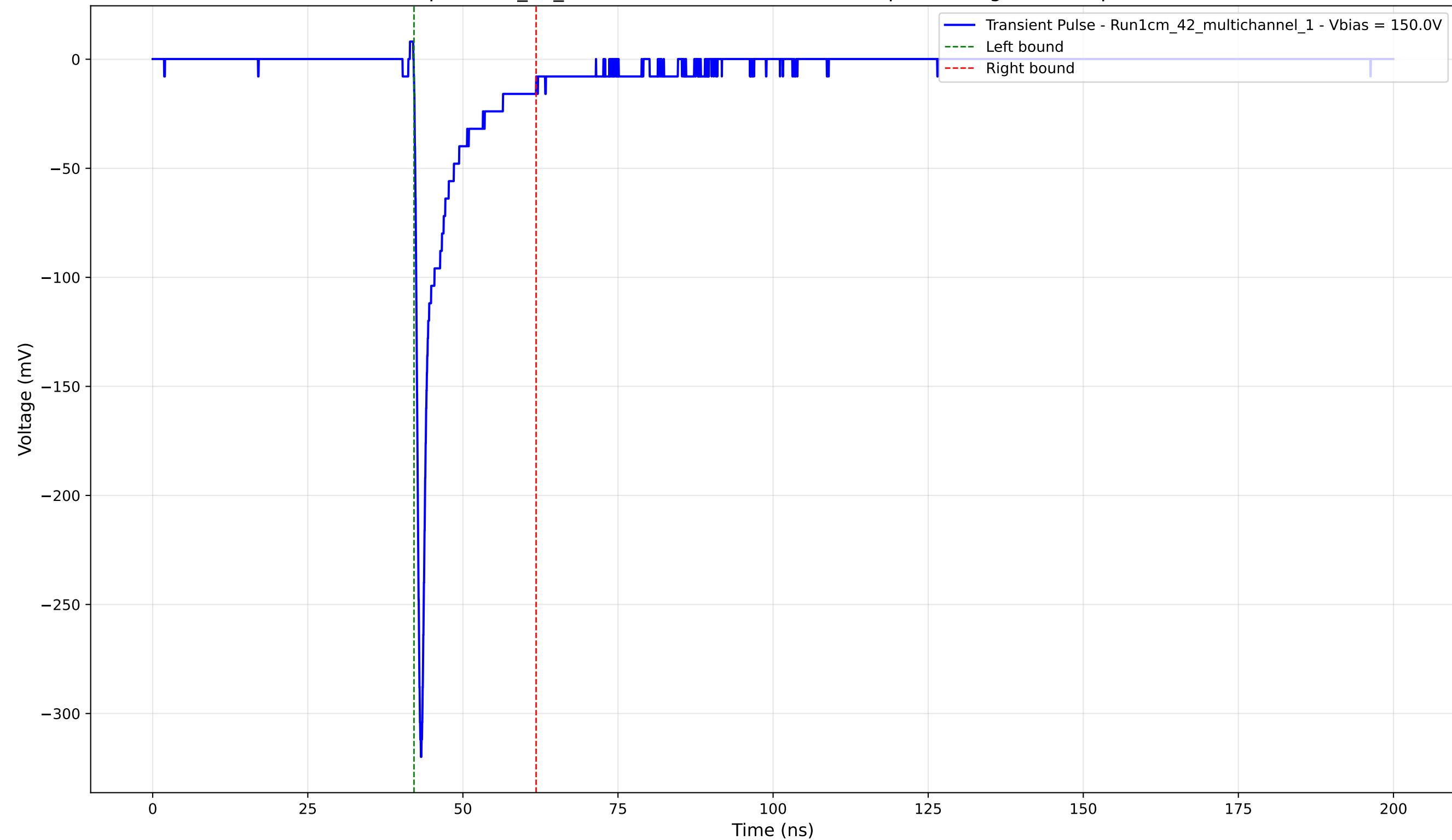
Transient Pulse - Sample: 1cm_42_multichannel - Position: 2625.0 \mu\text{m} - Charge: -22.68 pC - Rise Time: 0.80 ns
