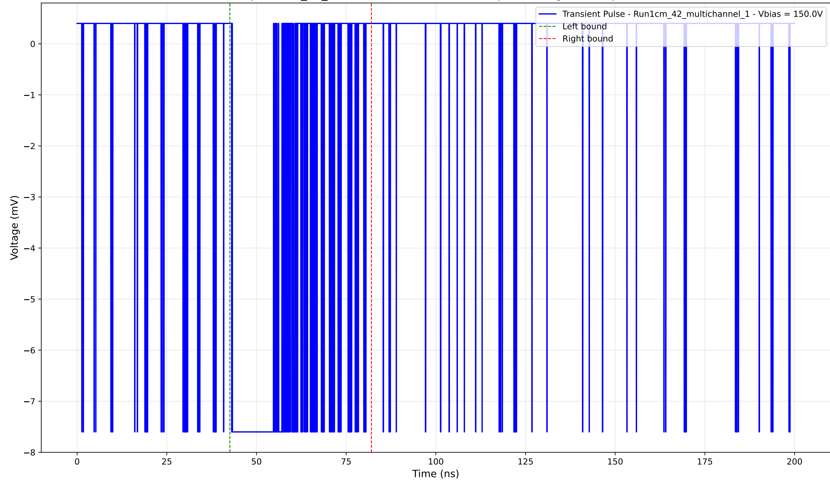
Transient Pulse - Sample: 1cm_42_multichannel - Position: 60.0 \mu\text{m} - Charge: -2.88 pC - Rise Time: 0.02 ns
