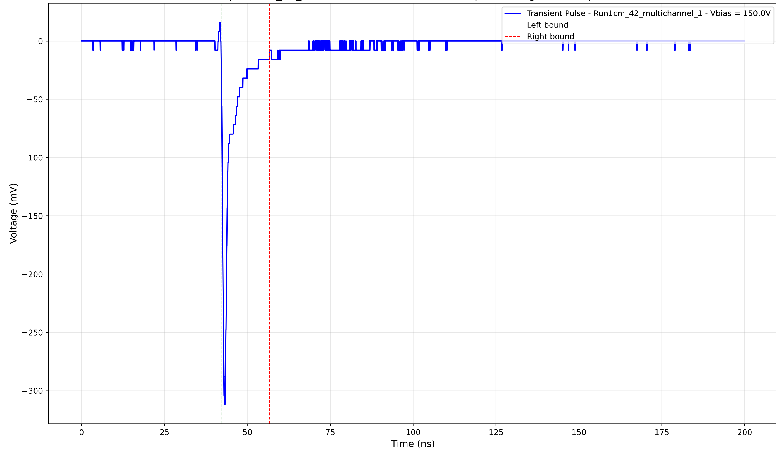
Transient Pulse - Sample: 1cm_42_multichannel - Position: 2450.0 \mu\text{m} - Charge: -17.30 pC - Rise Time: 0.76 ns
