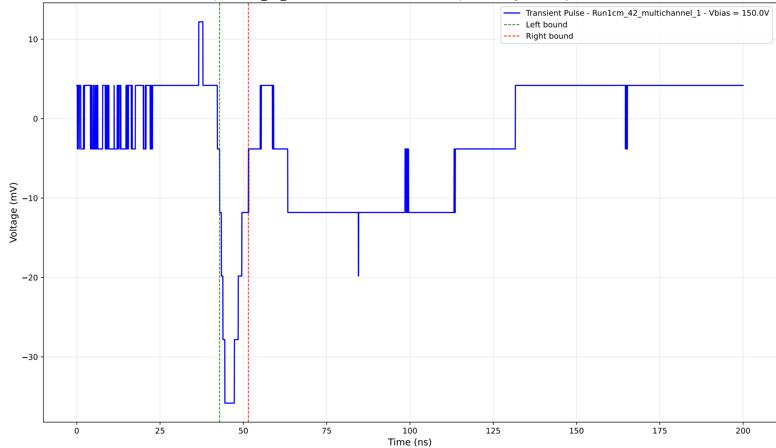
Transient Pulse - Sample: 1cm_42_multichannel - Position: 4805.0 \mu\text{m} - Charge: -4.21 pC - Rise Time: 0.00 ns (N/A)
