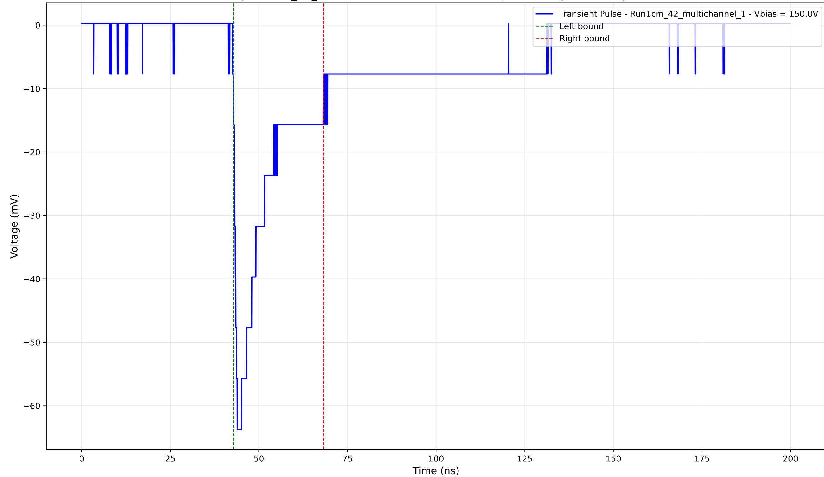
Transient Pulse - Sample: 1cm_42_multichannel - Position: 3655.0 \mu\text{m} - Charge: -13.46 pC - Rise Time: 1.34 ns
