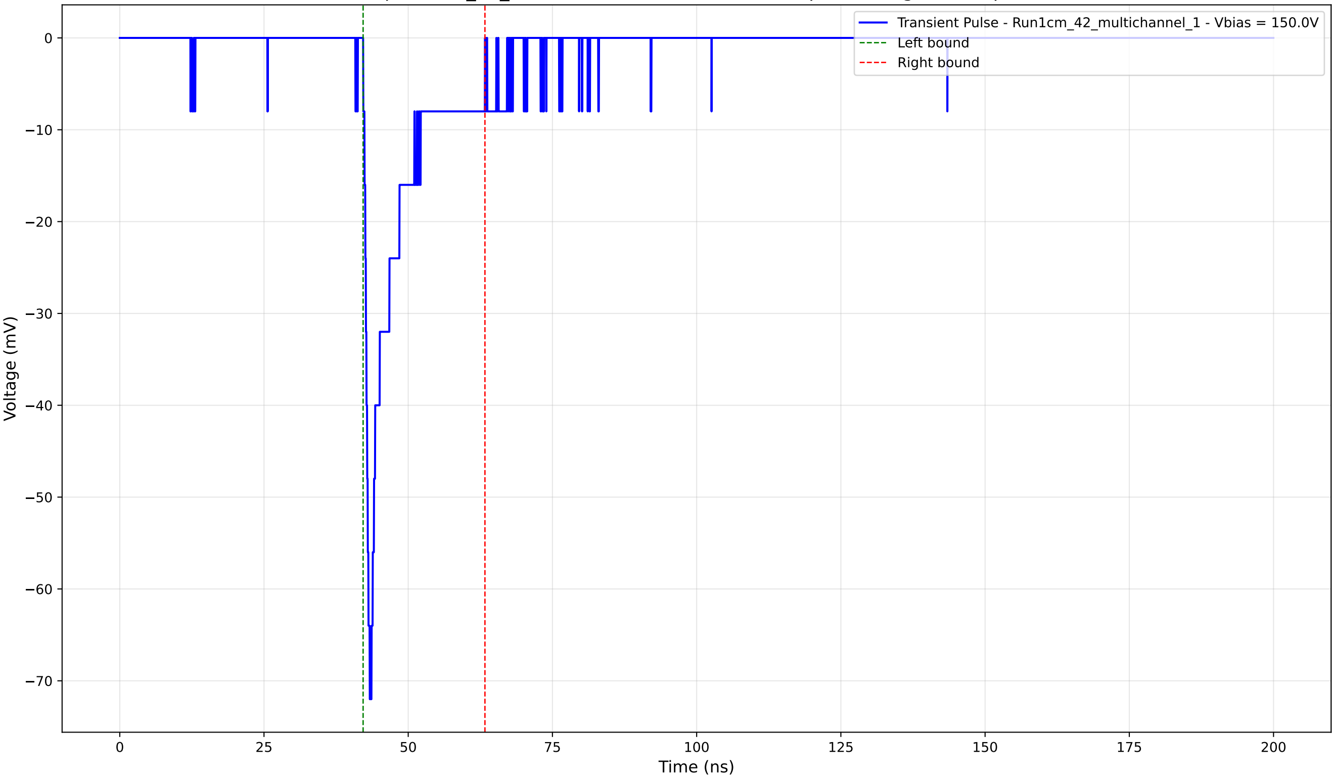
Transient Pulse - Sample: 1cm_42_multichannel - Position: 2850.0 \mu\text{m} - Charge: -7.41 pC - Rise Time: 1.12 ns
