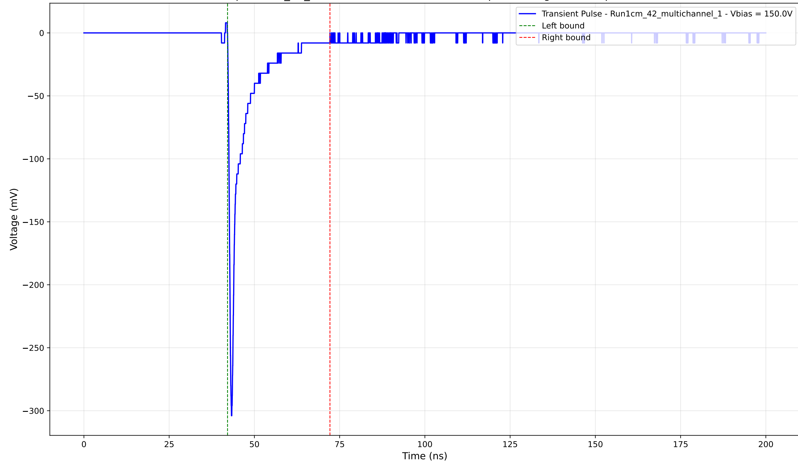
Transient Pulse - Sample: 1cm_42_multichannel - Position: 2095.0 \mu\text{m} - Charge: -25.13 pC - Rise Time: 0.80 ns
