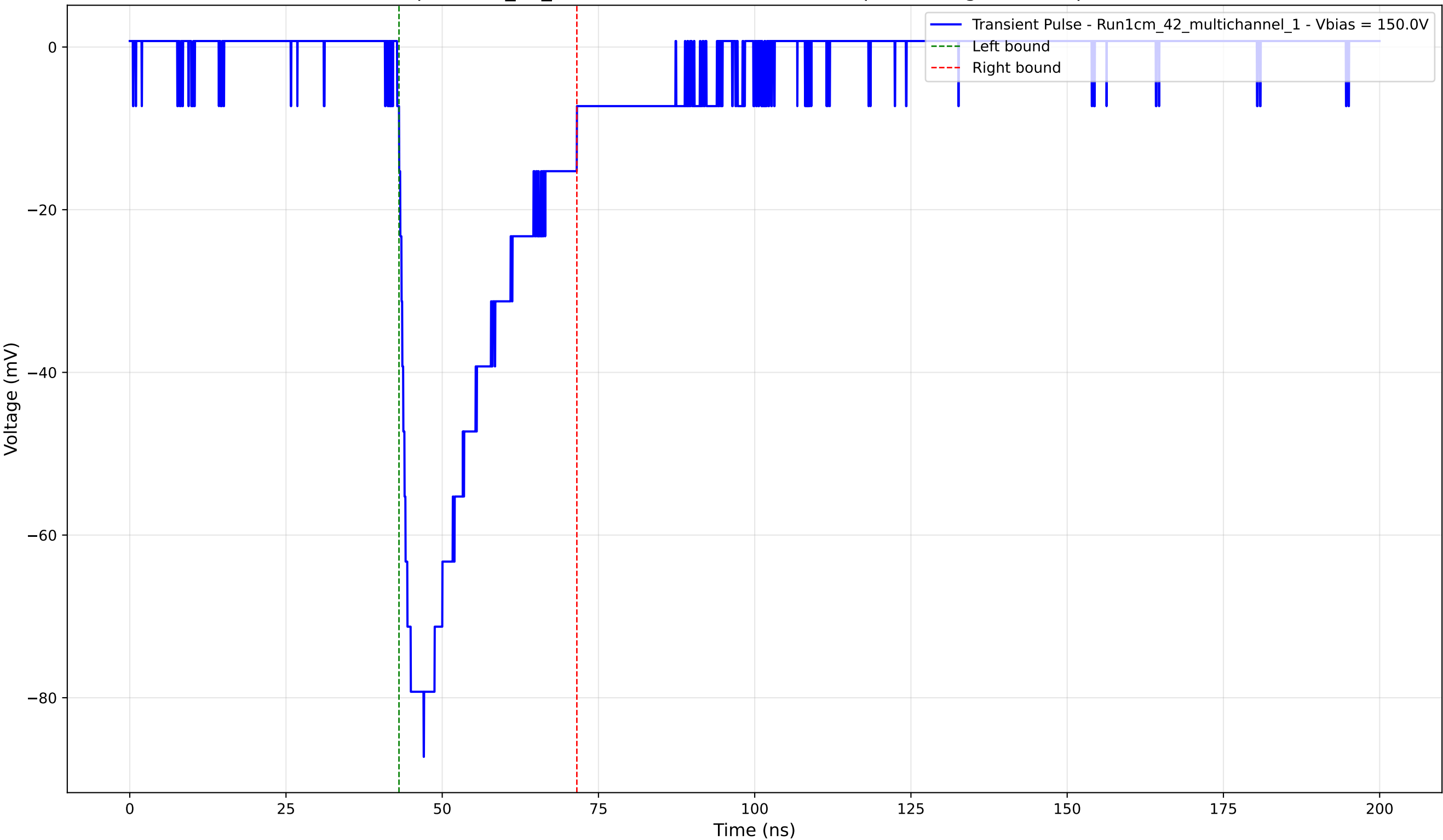
Transient Pulse - Sample: 1cm_42_multichannel - Position: 730.0 \mu\text{m} - Charge: -23.52 pC - Rise Time: 1.88 ns
