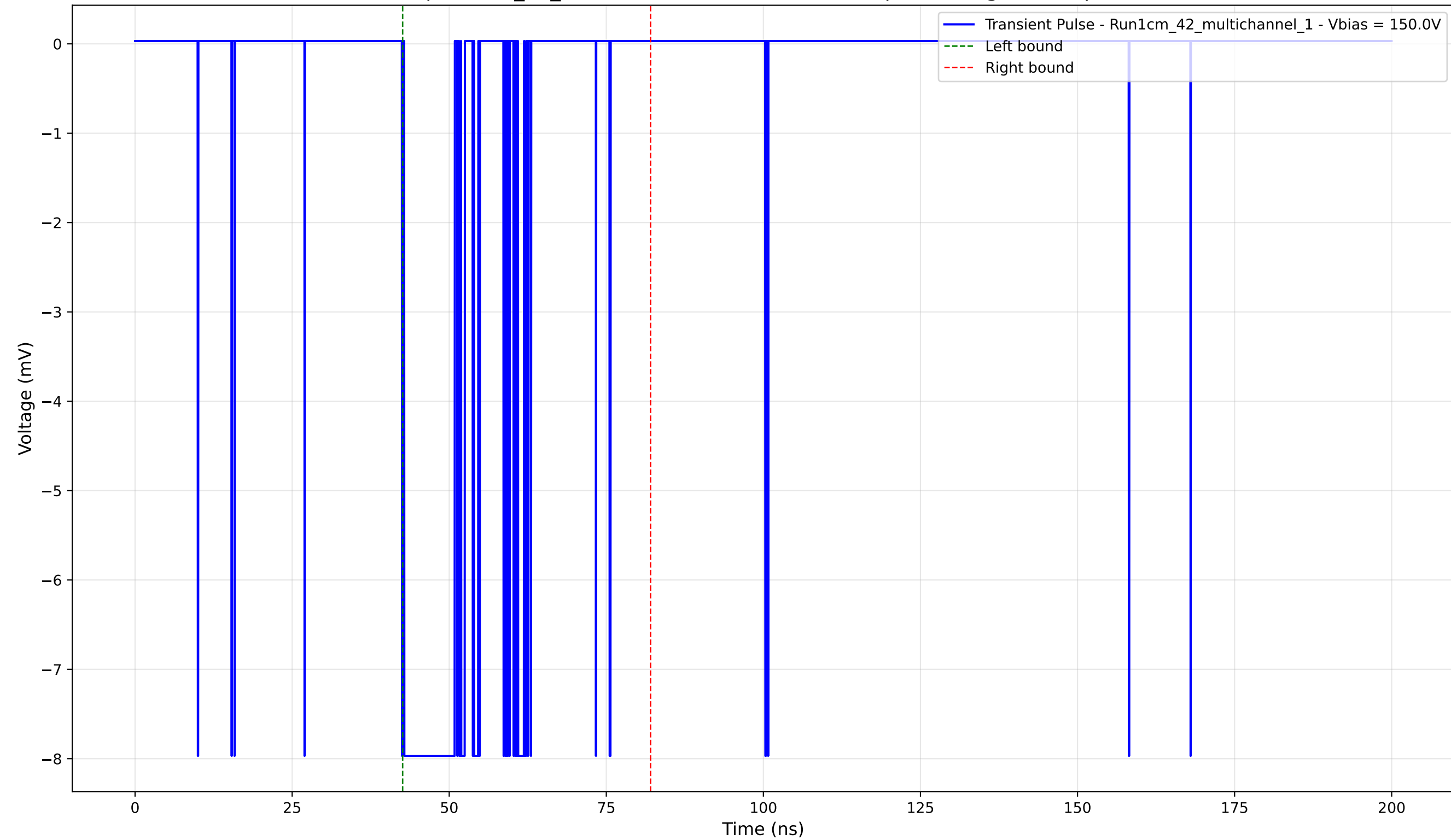
Transient Pulse - Sample: 1cm_42_multichannel - Position: 1375.0 \mu\text{m} - Charge: -1.92 pC - Rise Time: 0.02 ns
