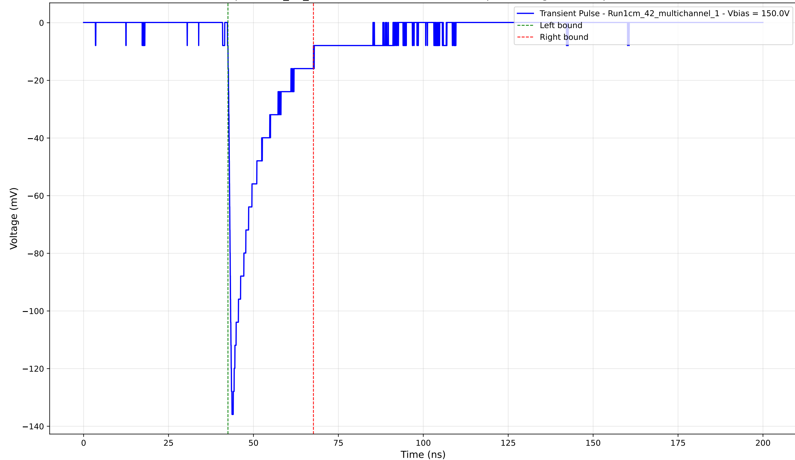
Transient Pulse - Sample: 1cm_42_multichannel - Position: 1545.0 \mu\text{m} - Charge: -22.98 pC - Rise Time: 1.01 ns
