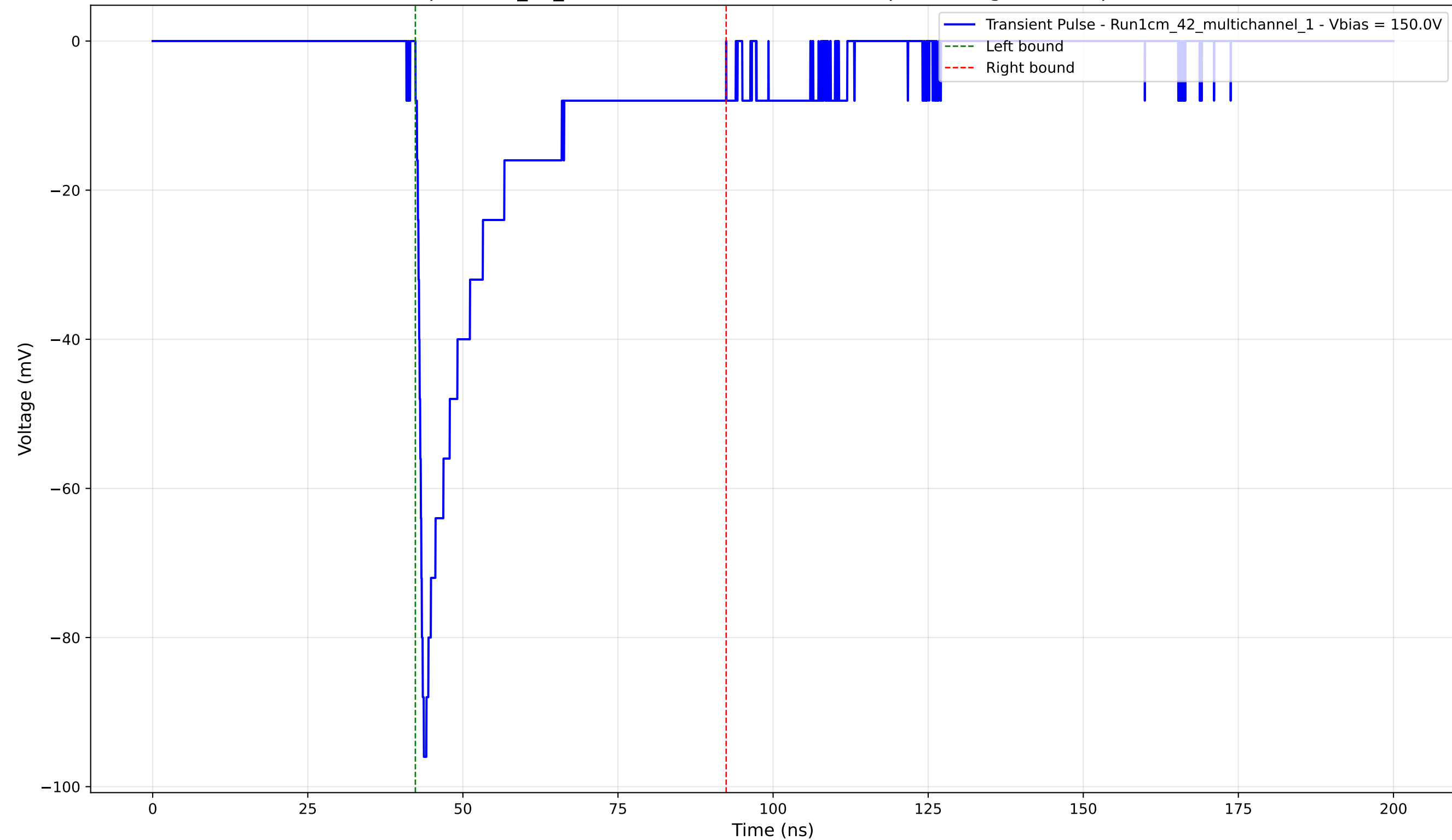
Transient Pulse - Sample: 1cm_42_multichannel - Position: 3315.0 \mu\text{m} - Charge: -20.10 pC - Rise Time: 0.94 ns
