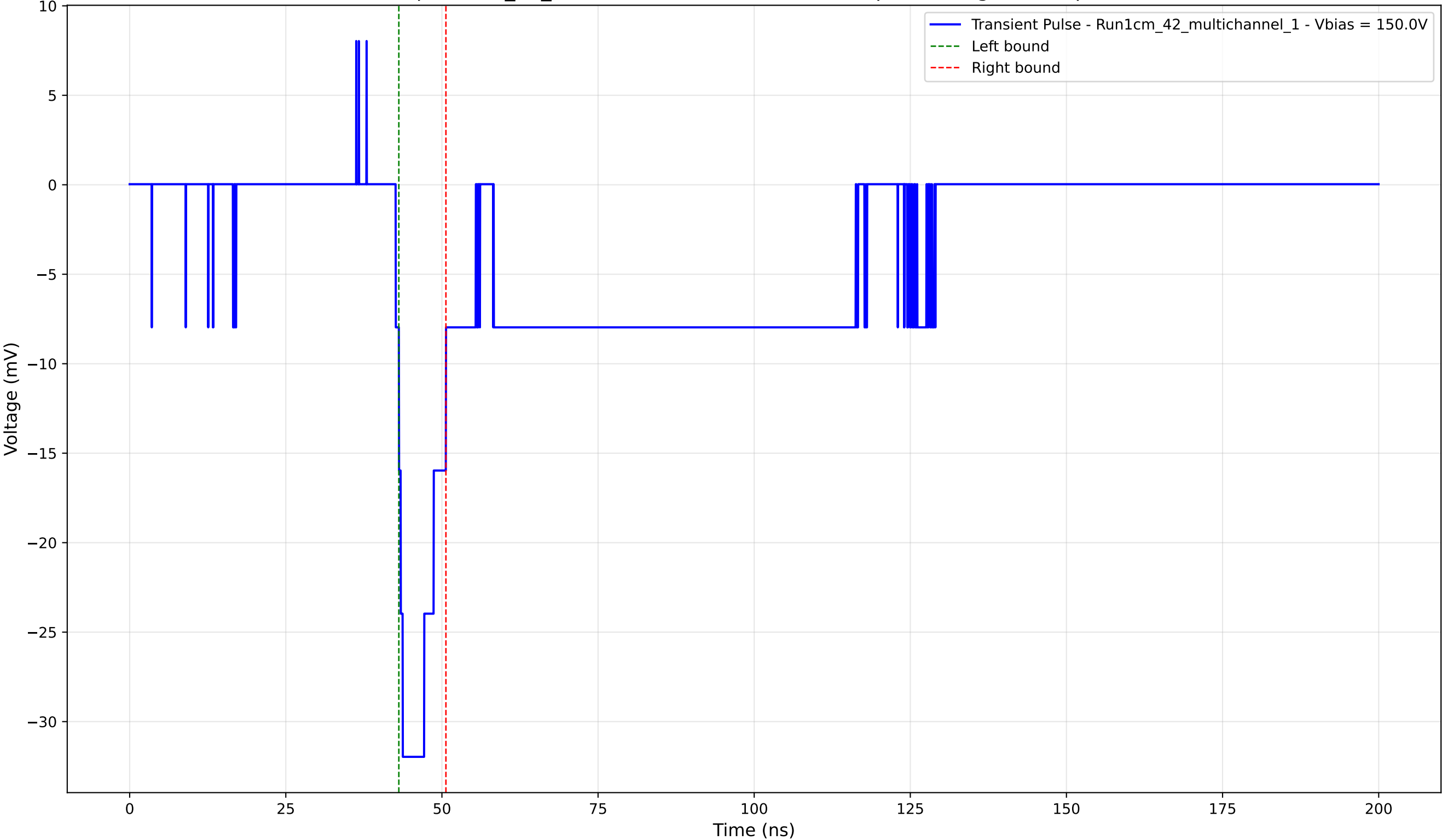
Transient Pulse - Sample: 1cm_42_multichannel - Position: 3850.0 \mu\text{m} - Charge: -3.80 pC - Rise Time: 1.13 ns
