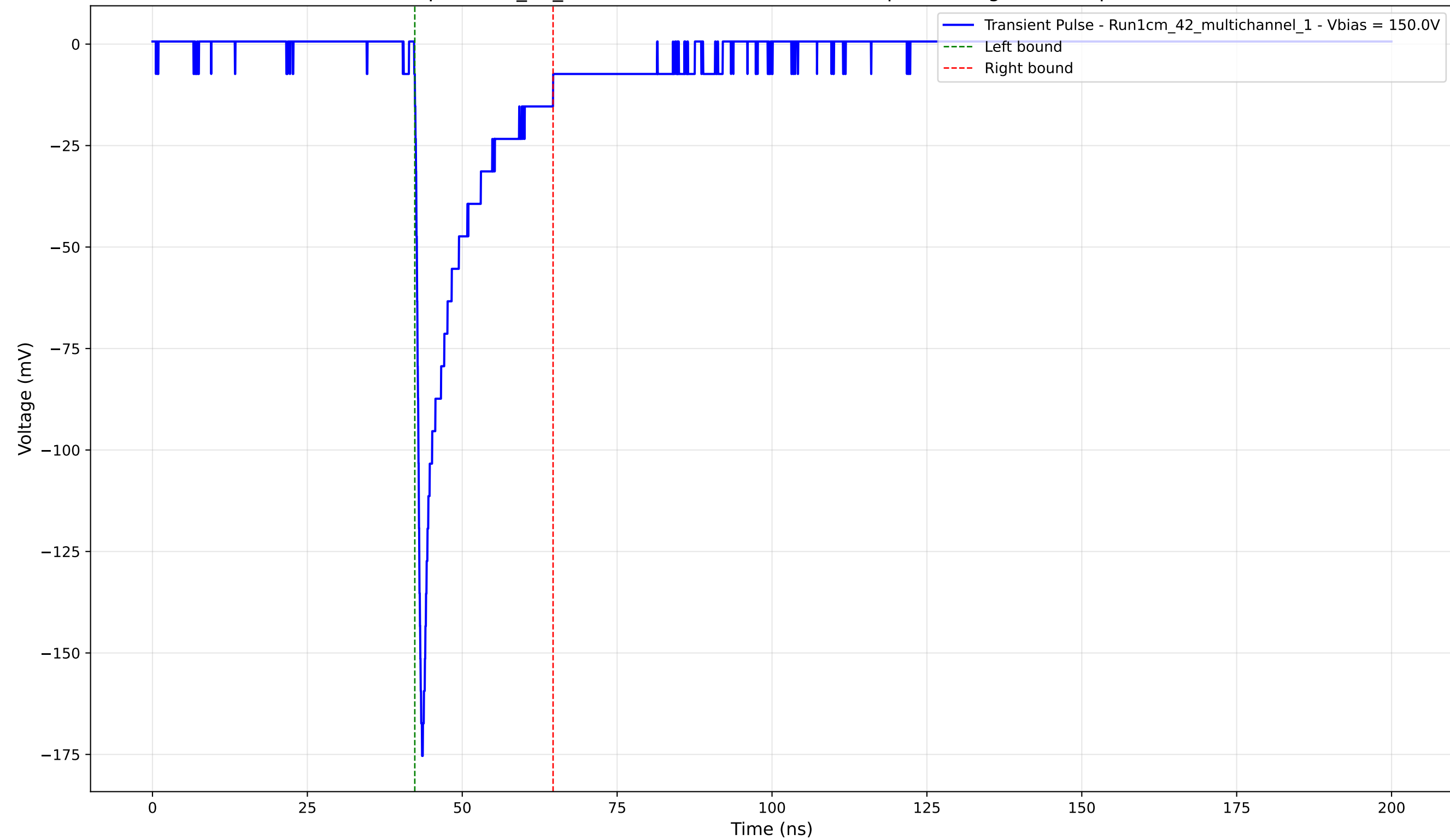
Transient Pulse - Sample: 1cm_42_multichannel - Position: 1795.0 \mu\text{m} - Charge: -20.84 pC - Rise Time: 0.85 ns
