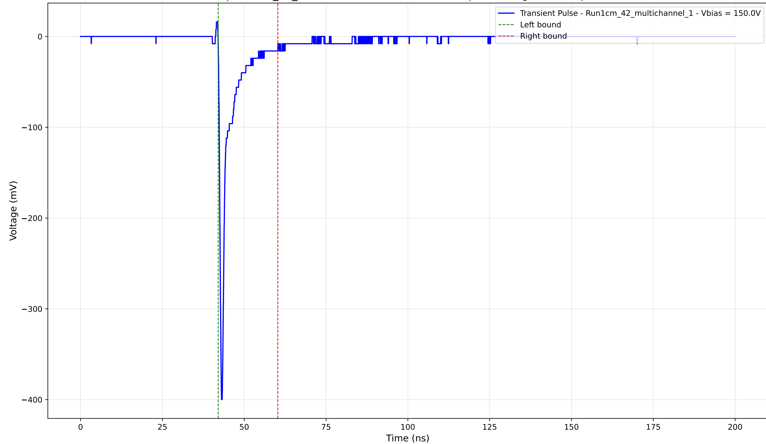
Transient Pulse - Sample: 1cm_42_multichannel - Position: 2295.0 \mu\text{m} - Charge: -23.84 pC - Rise Time: 0.72 ns
