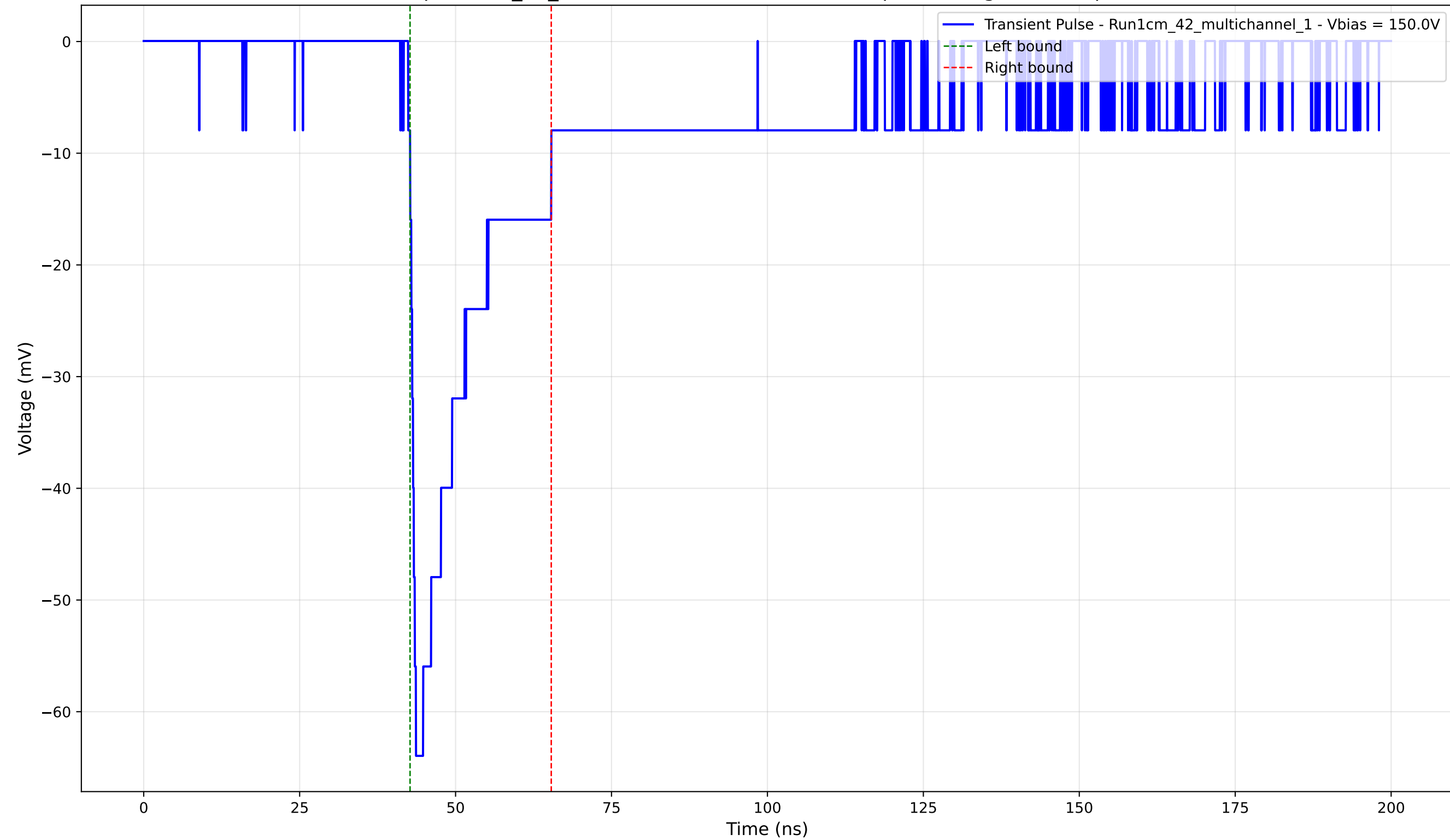
Transient Pulse - Sample: 1cm_42_multichannel - Position: 3465.0 \mu\text{m} - Charge: -12.84 pC - Rise Time: 1.24 ns
