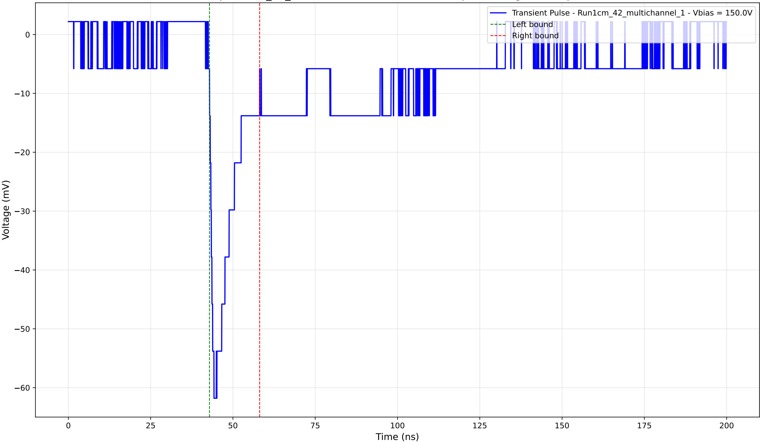
Transient Pulse - Sample: 1cm_42_multichannel - Position: 3775.0 \mu\text{m} - Charge: -8.91 pC - Rise Time: 1.36 ns
