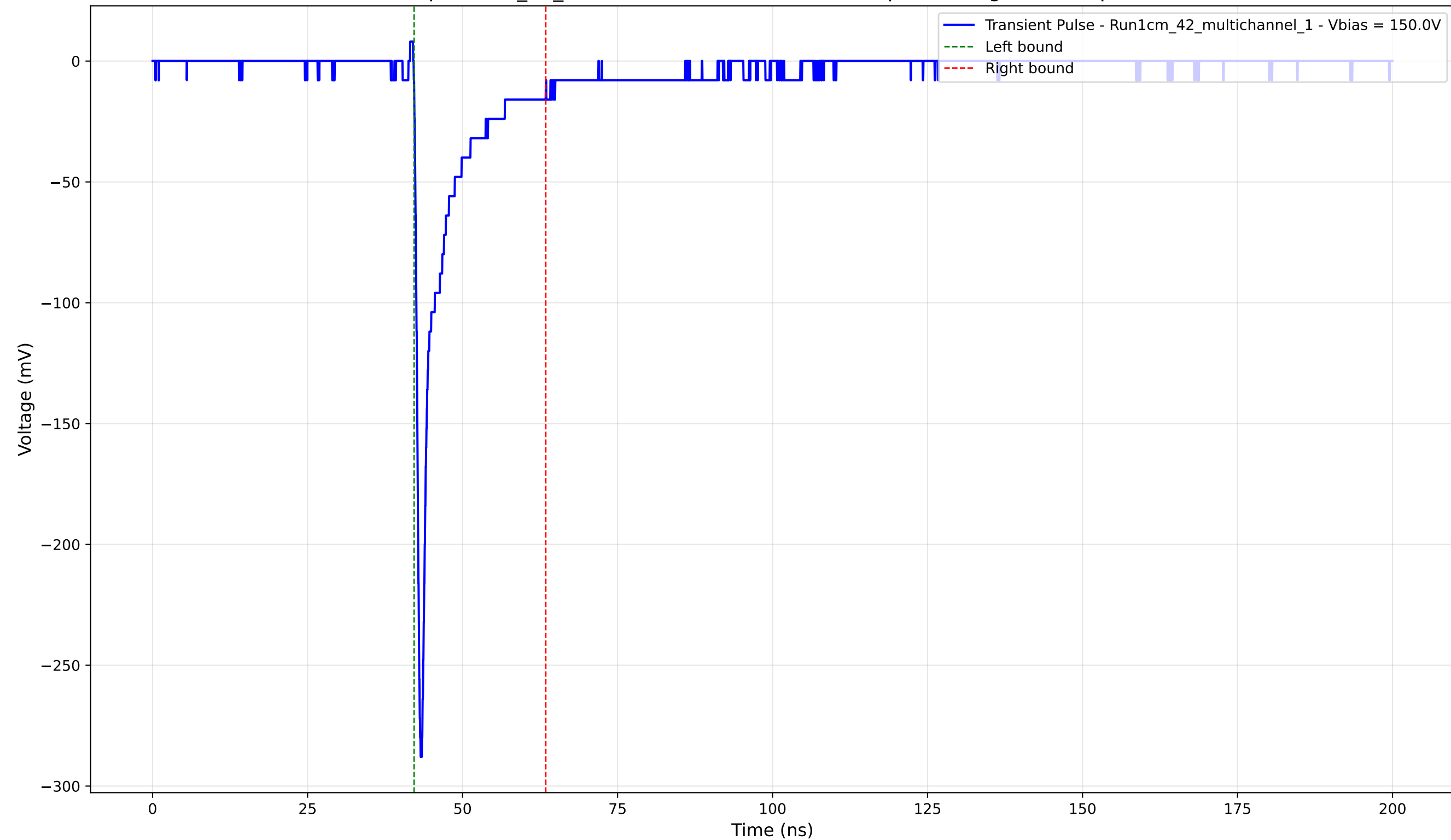
Transient Pulse - Sample: 1cm_42_multichannel - Position: 2685.0 \mu\text{m} - Charge: -22.89 pC - Rise Time: 0.79 ns
