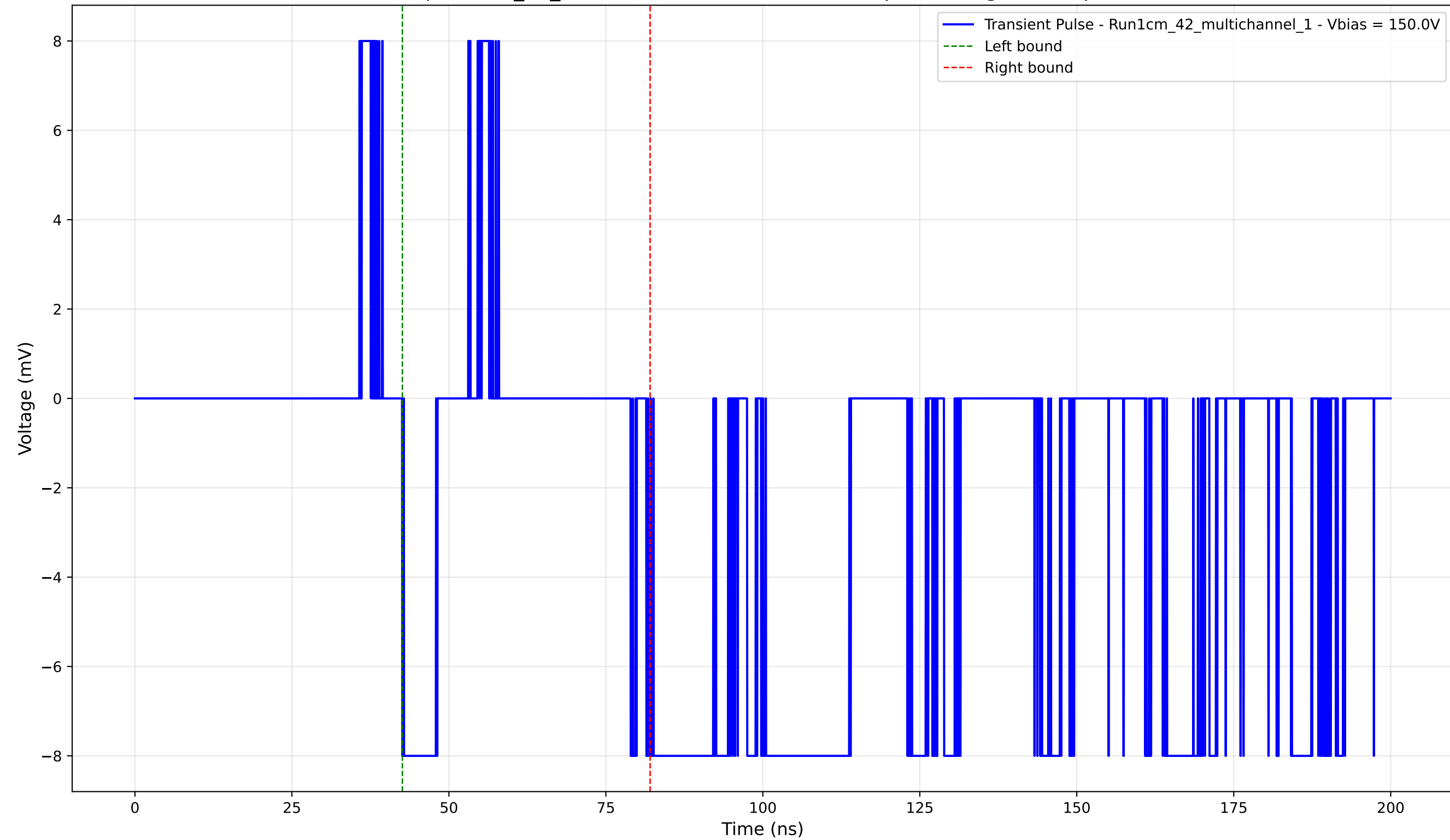
Transient Pulse - Sample: 1cm_42_multichannel - Position: 4385.0 \mu\text{m} - Charge: -0.68 pC - Rise Time: 0.02 ns
