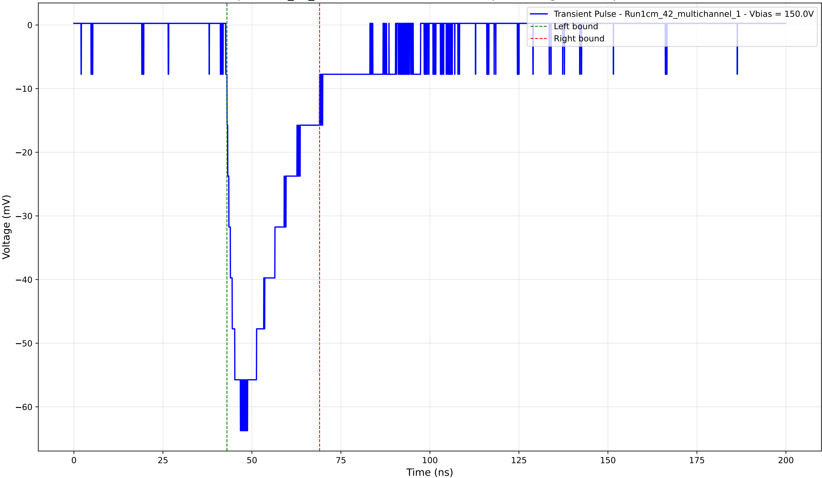
Transient Pulse - Sample: 1cm_42_multichannel - Position: 125.0 \mu\text{m} - Charge: -18.59 pC - Rise Time: 4.12 ns
