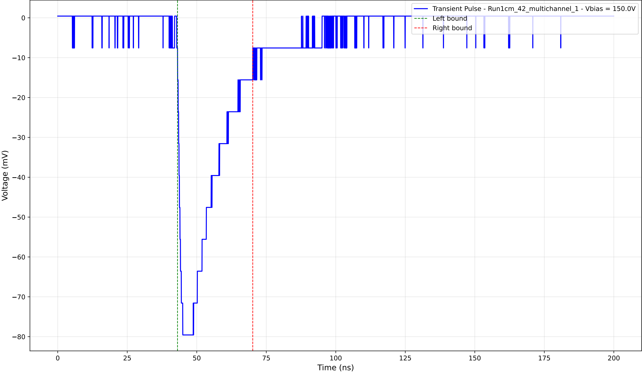
Transient Pulse - Sample: 1cm_42_multichannel - Position: 715.0 \mu\text{m} - Charge: -23.23 pC - Rise Time: 1.88 ns
