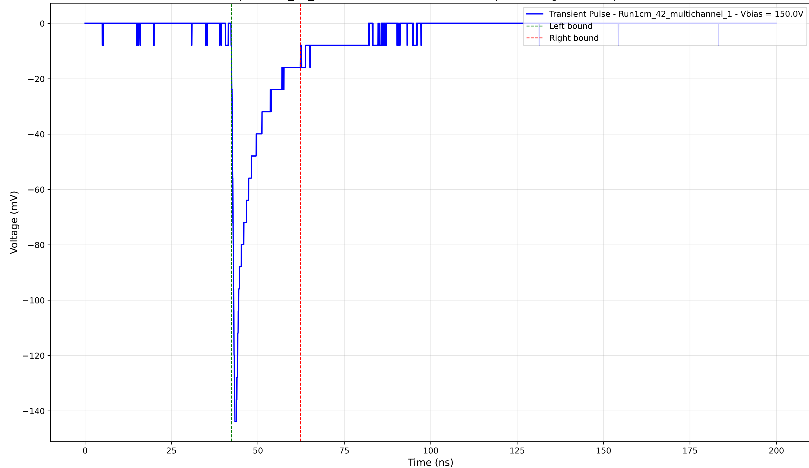
Transient Pulse - Sample: 1cm_42_multichannel - Position: 1815.0 \mu\text{m} - Charge: -17.22 pC - Rise Time: 0.88 ns
