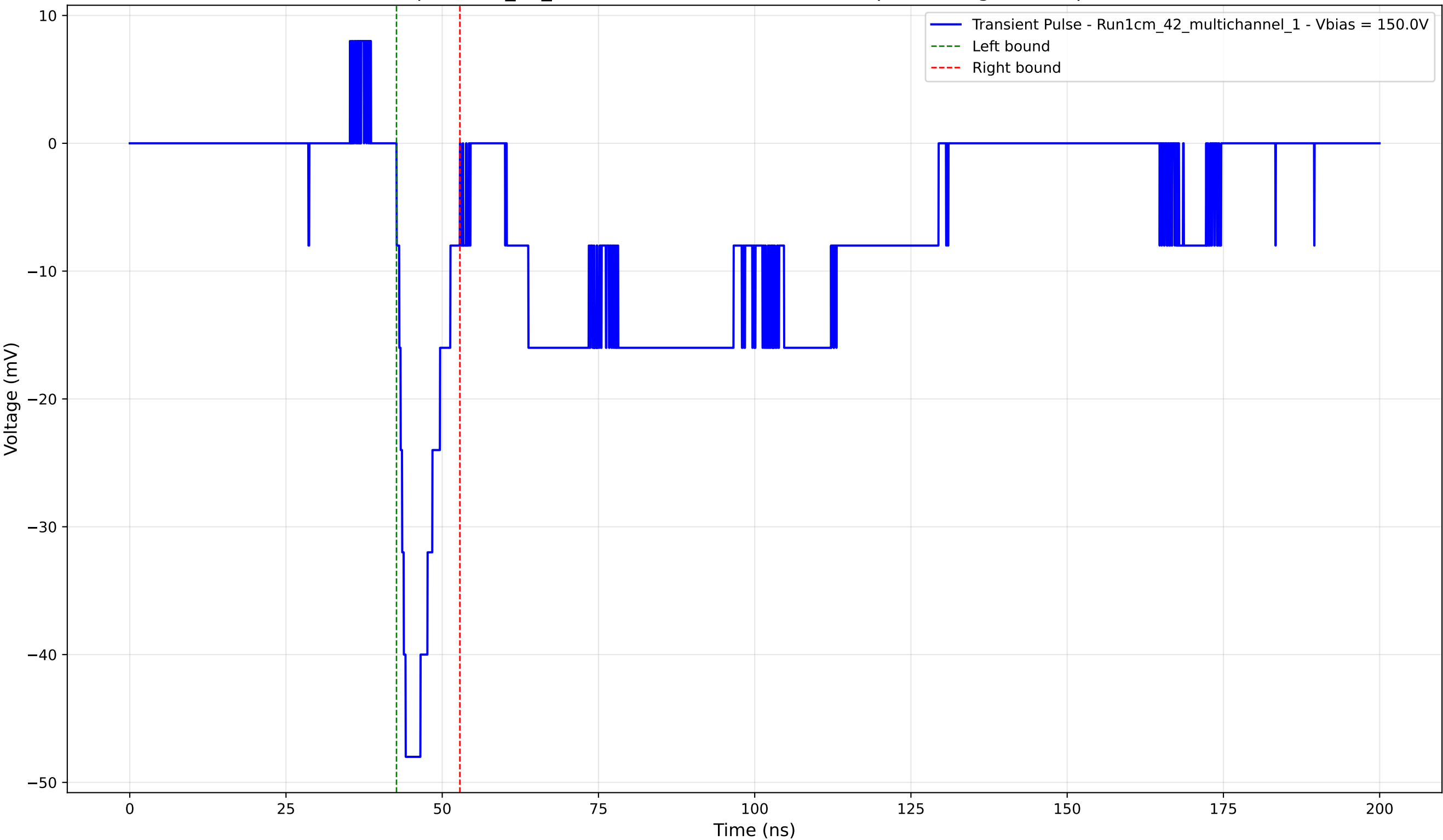
Transient Pulse - Sample: 1cm_42_multichannel - Position: 3990.0 \mu\text{m} - Charge: -5.70 pC - Rise Time: 1.45 ns
