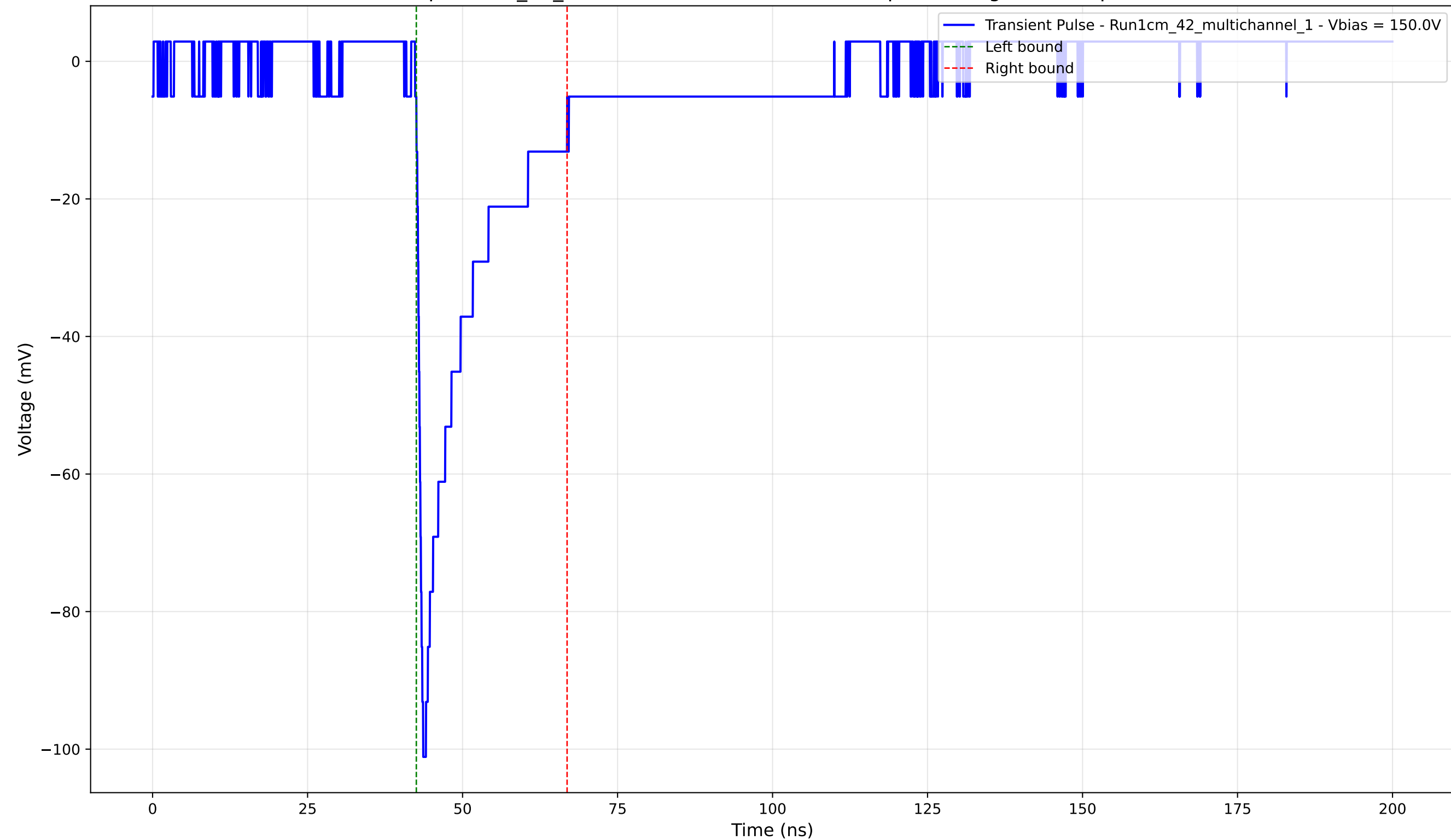
Transient Pulse - Sample: 1cm_42_multichannel - Position: 3300.0 \mu\text{m} - Charge: -16.22 pC - Rise Time: 0.95 ns
