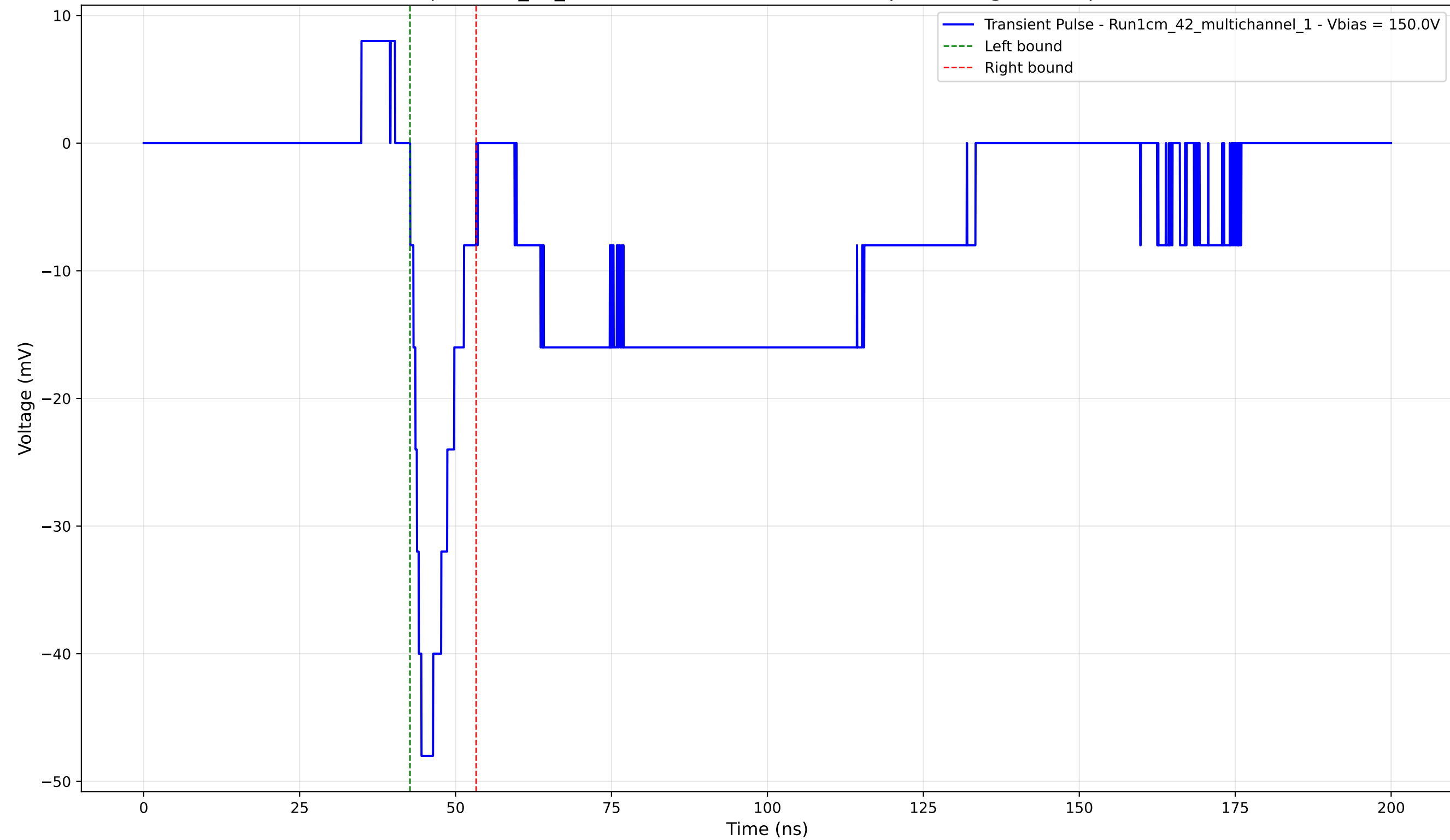
Transient Pulse - Sample: 1cm_42_multichannel - Position: 4195.0 \mu\text{m} - Charge: -5.64 pC - Rise Time: 1.81 ns
