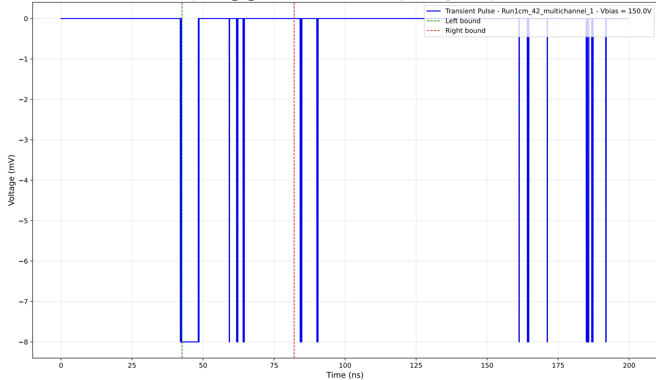
Transient Pulse - Sample: 1cm_42_multichannel - Position: 3385.0 \mu\text{m} - Charge: -1.01 pC - Rise Time: 0.02 ns
