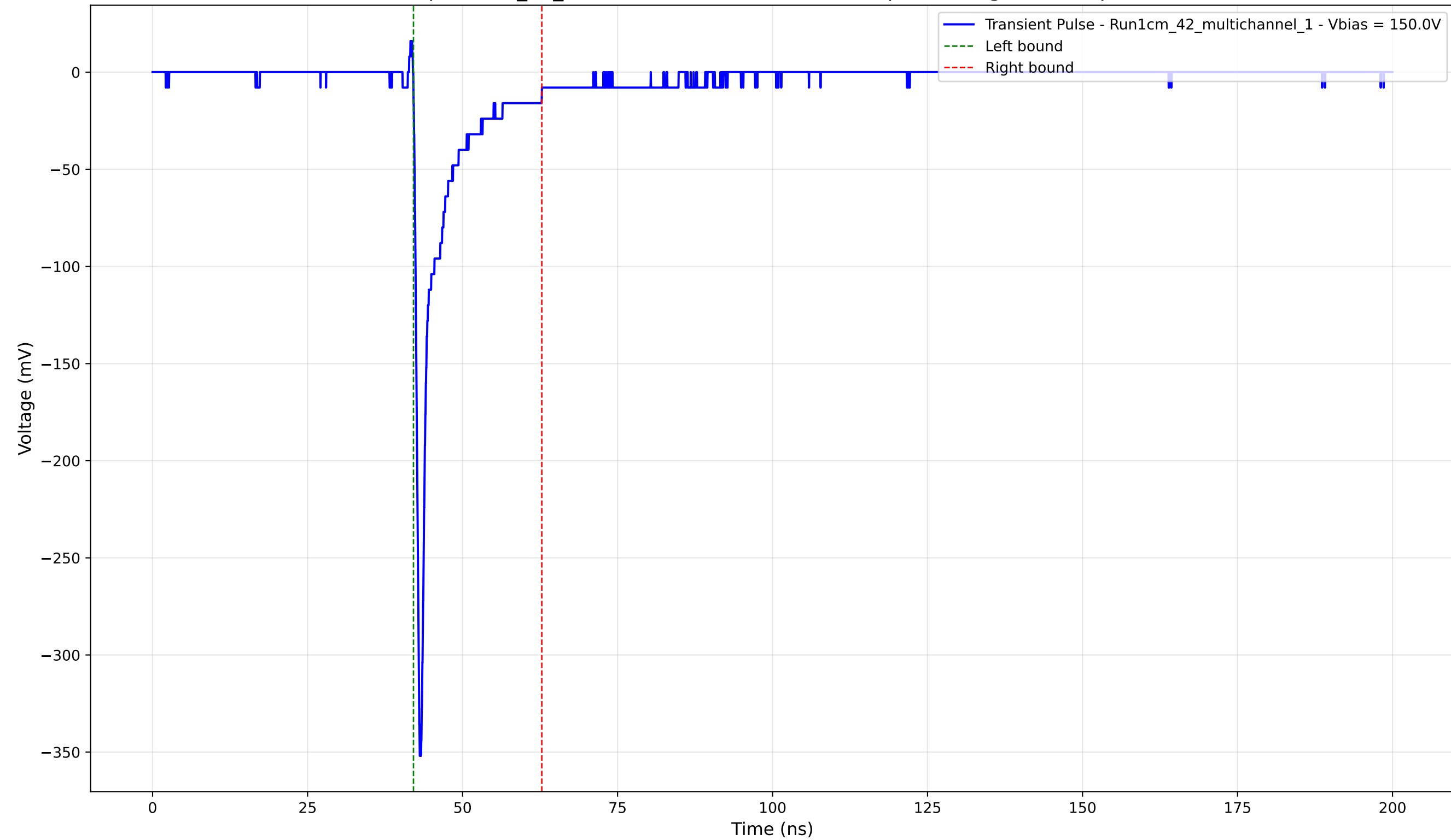
Transient Pulse - Sample: 1cm_42_multichannel - Position: 2565.0 \mu\text{m} - Charge: -23.89 pC - Rise Time: 0.74 ns
