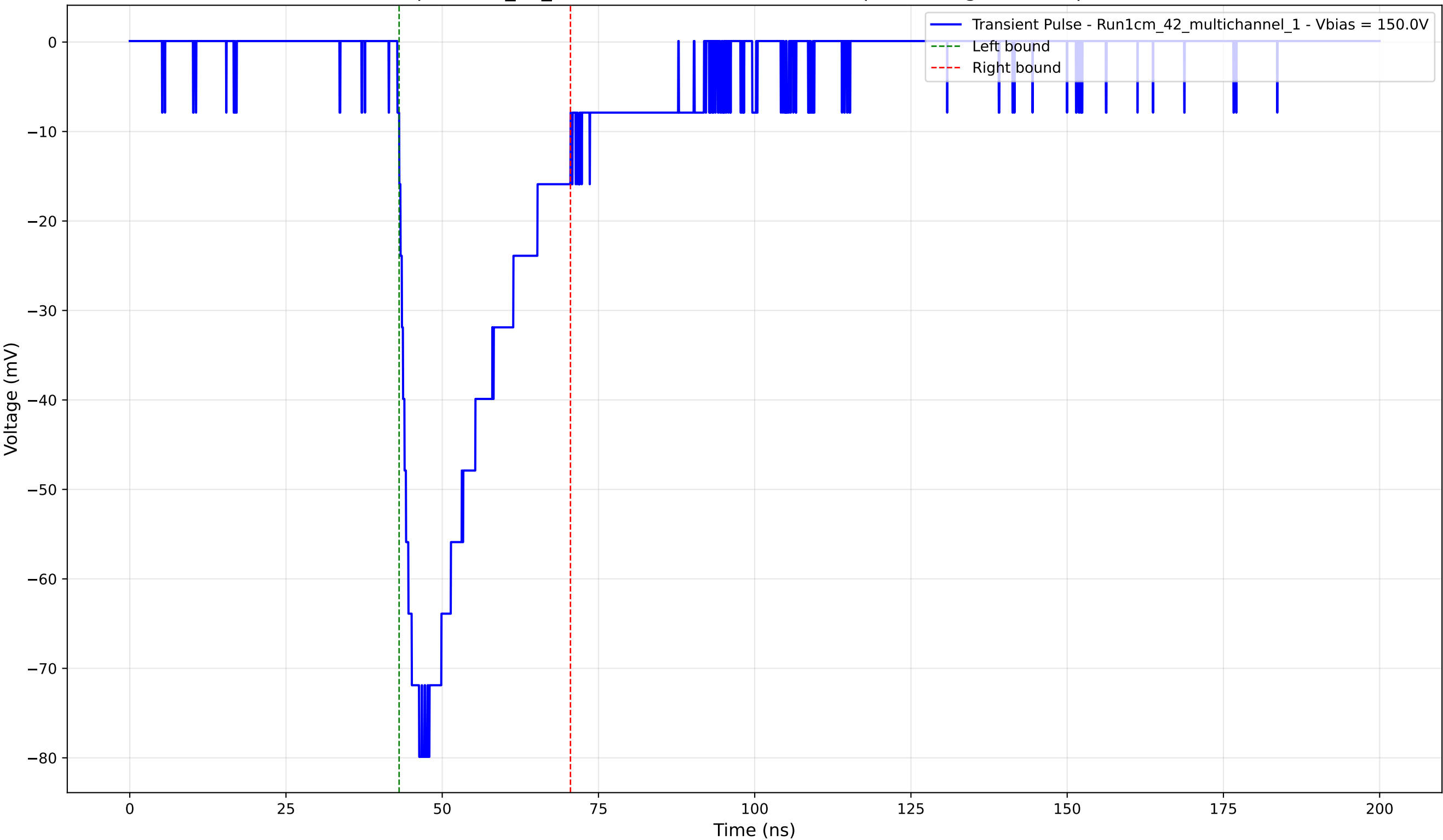
Transient Pulse - Sample: 1cm_42_multichannel - Position: 470.0 \mu\text{m} - Charge: -22.71 pC - Rise Time: 3.20 ns
