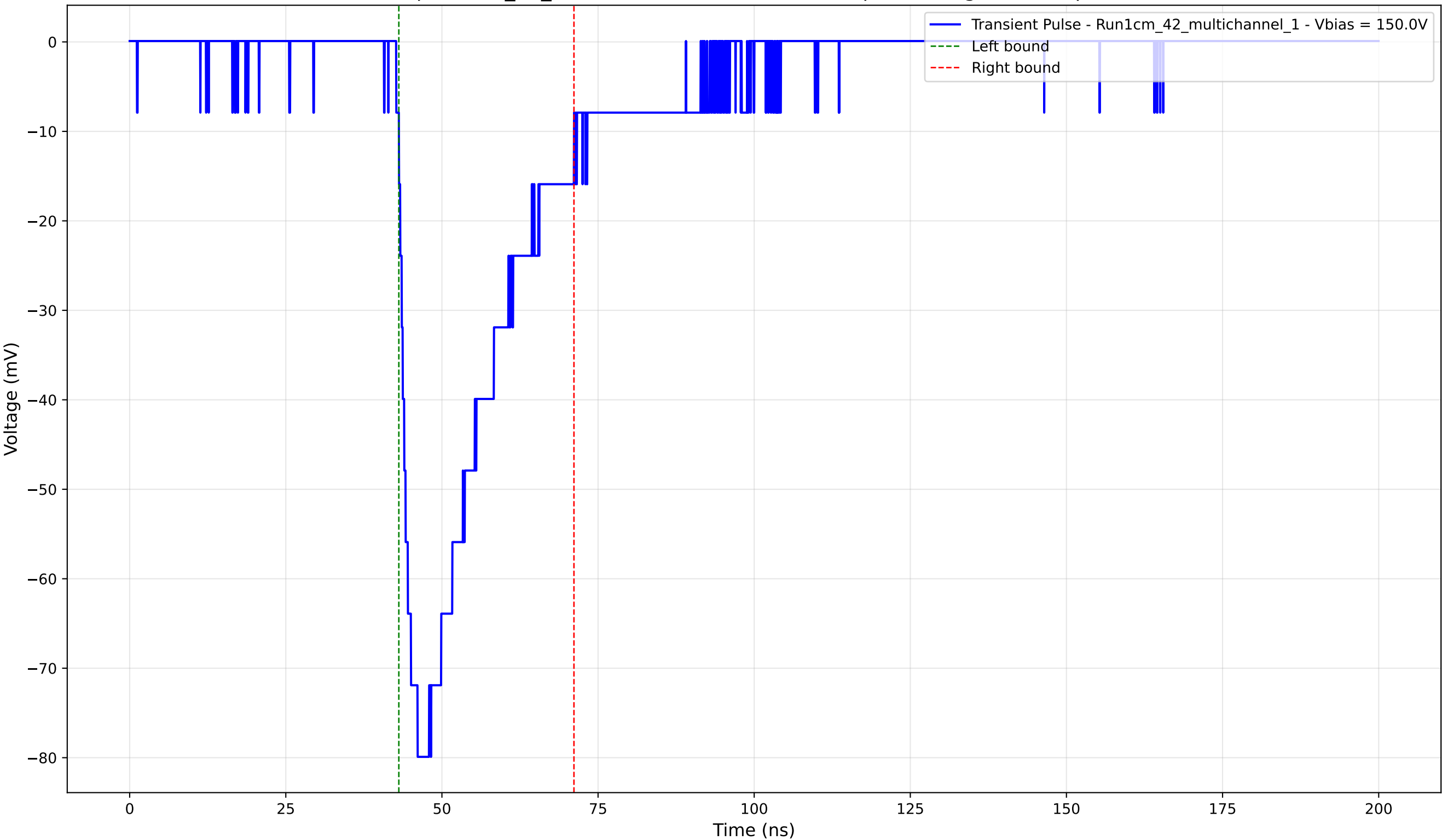
Transient Pulse - Sample: 1cm_42_multichannel - Position: 500.0 \mu\text{m} - Charge: -23.11 pC - Rise Time: 3.00 ns
