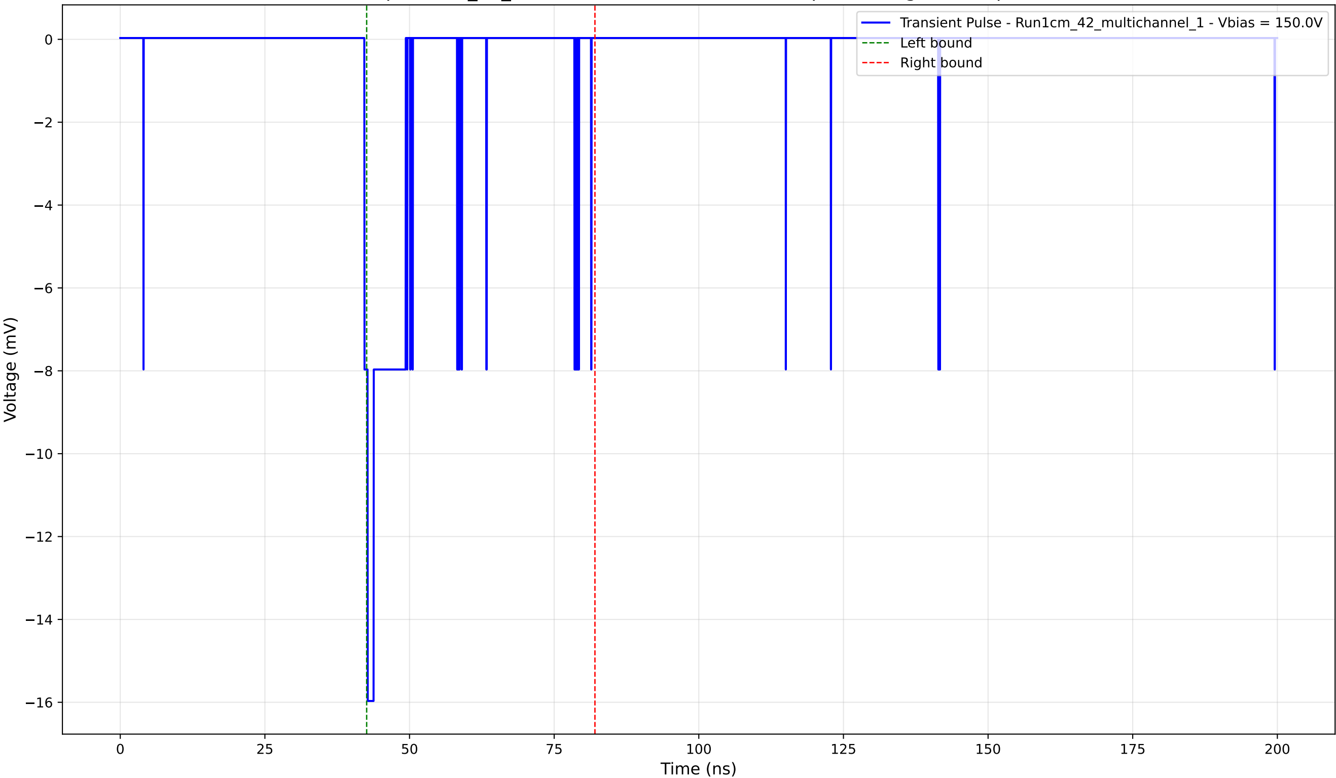
Transient Pulse - Sample: 1cm_42_multichannel - Position: 2380.0 \mu\text{m} - Charge: -1.41 pC - Rise Time: 0.58 ns
