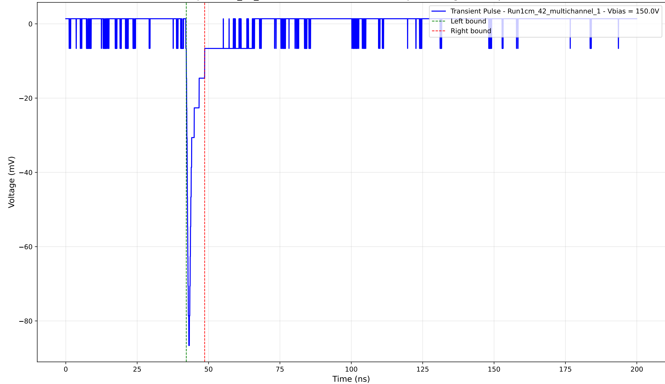
Transient Pulse - Sample: 1cm_42_multichannel - Position: 2350.0 \mu\text{m} - Charge: -4.04 pC - Rise Time: 0.69 ns
