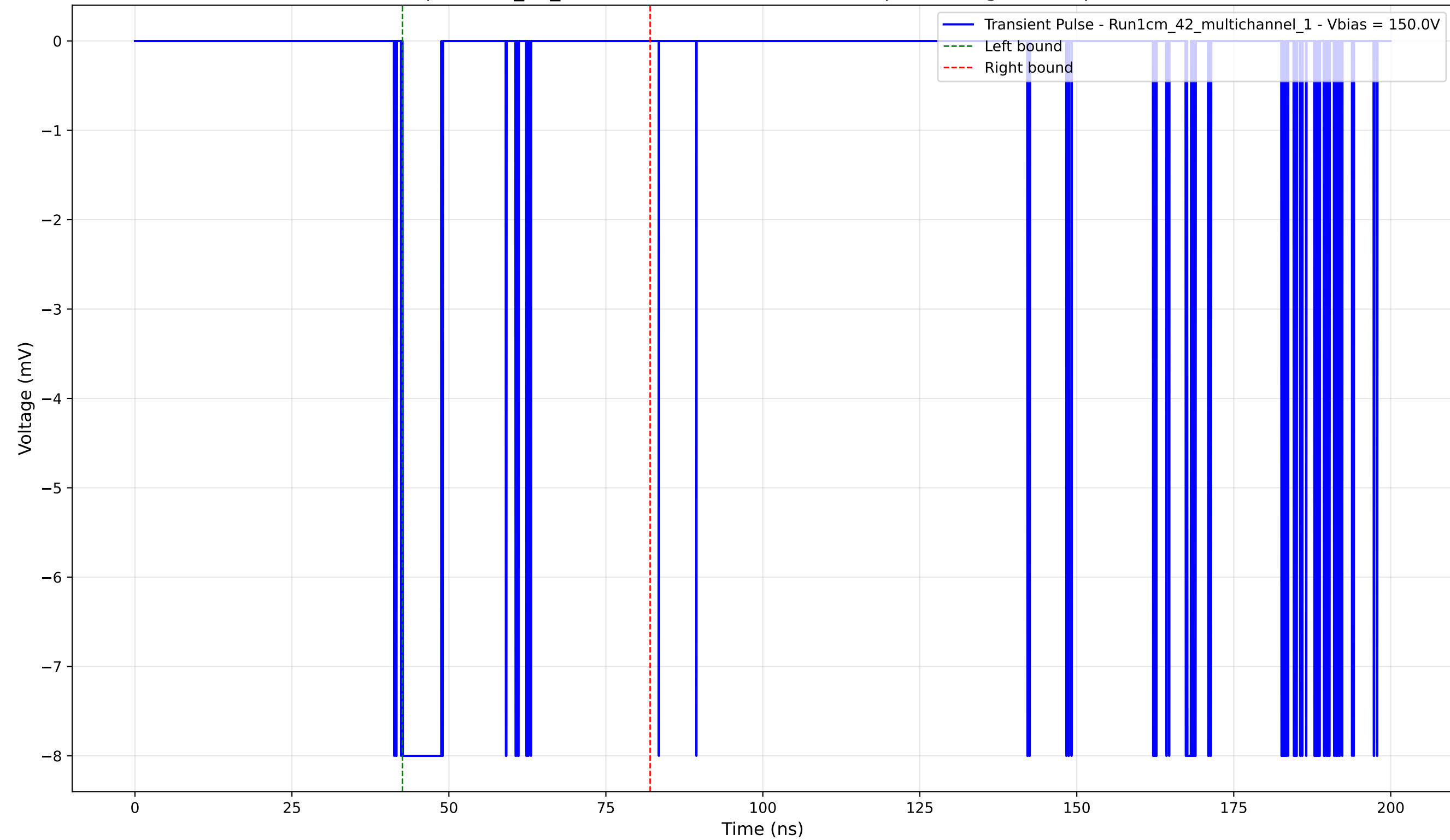
Transient Pulse - Sample: 1cm_42_multichannel - Position: 3420.0 \mu\text{m} - Charge: -1.13 pC - Rise Time: 0.02 ns
