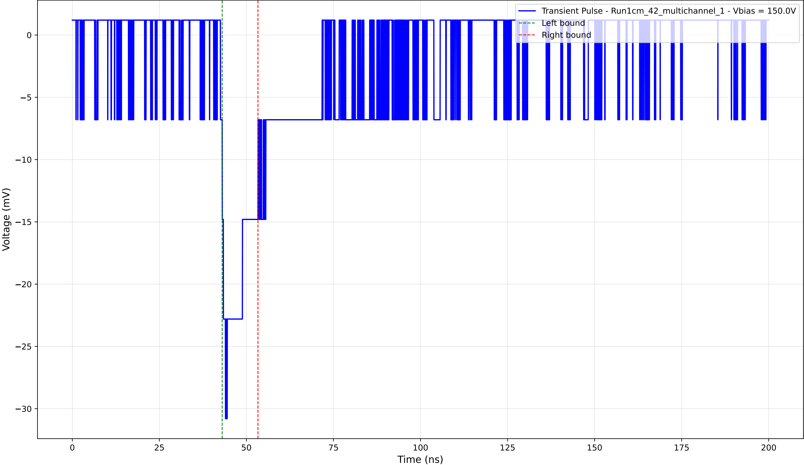
Transient Pulse - Sample: 1cm_42_multichannel - Position: 1335.0 \mu\text{m} - Charge: -3.97 pC - Rise Time: 1.45 ns
