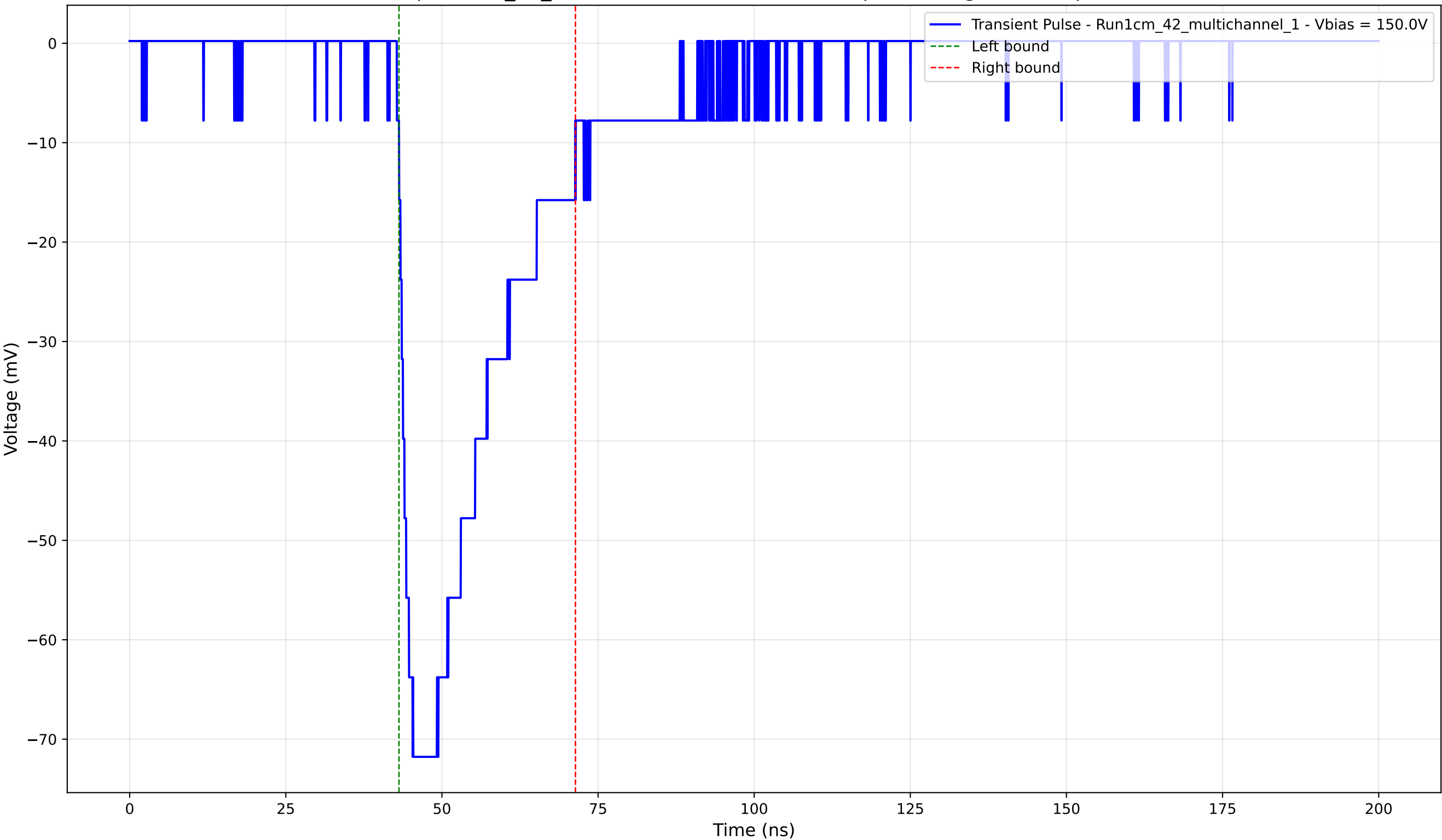
Transient Pulse - Sample: 1cm_42_multichannel - Position: 450.0 \mu\text{m} - Charge: -22.11 pC - Rise Time: 2.52 ns
