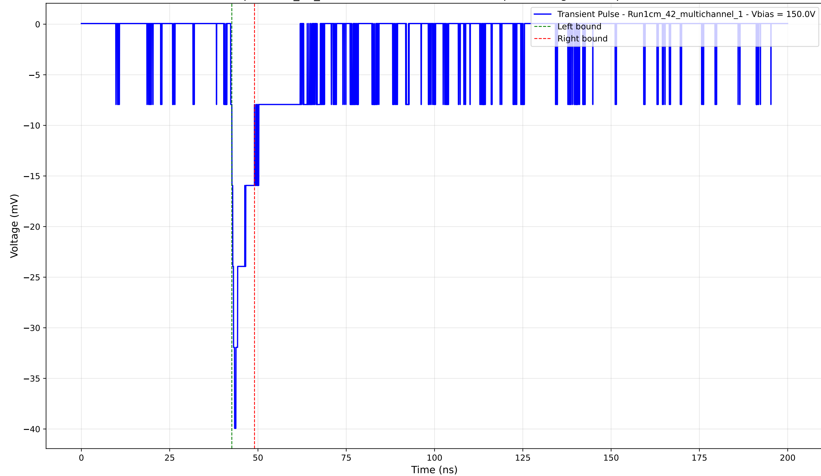
Transient Pulse - Sample: 1cm_42_multichannel - Position: 1845.0 \mu\text{m} - Charge: -2.87 pC - Rise Time: 1.11 ns
