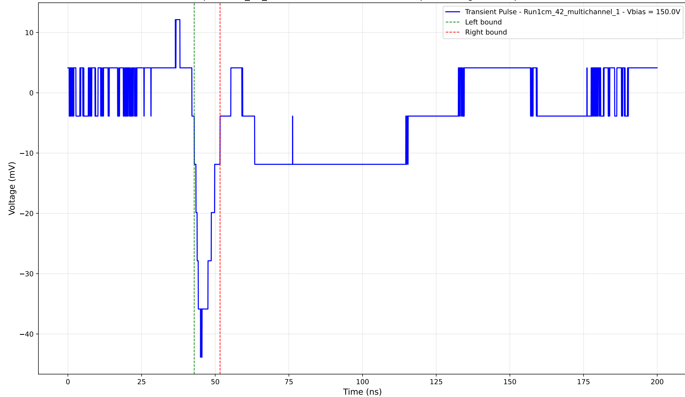
Transient Pulse - Sample: 1cm_42_multichannel - Position: 4750.0 \mu\text{m} - Charge: -4.41 pC - Rise Time: 2.16 ns
