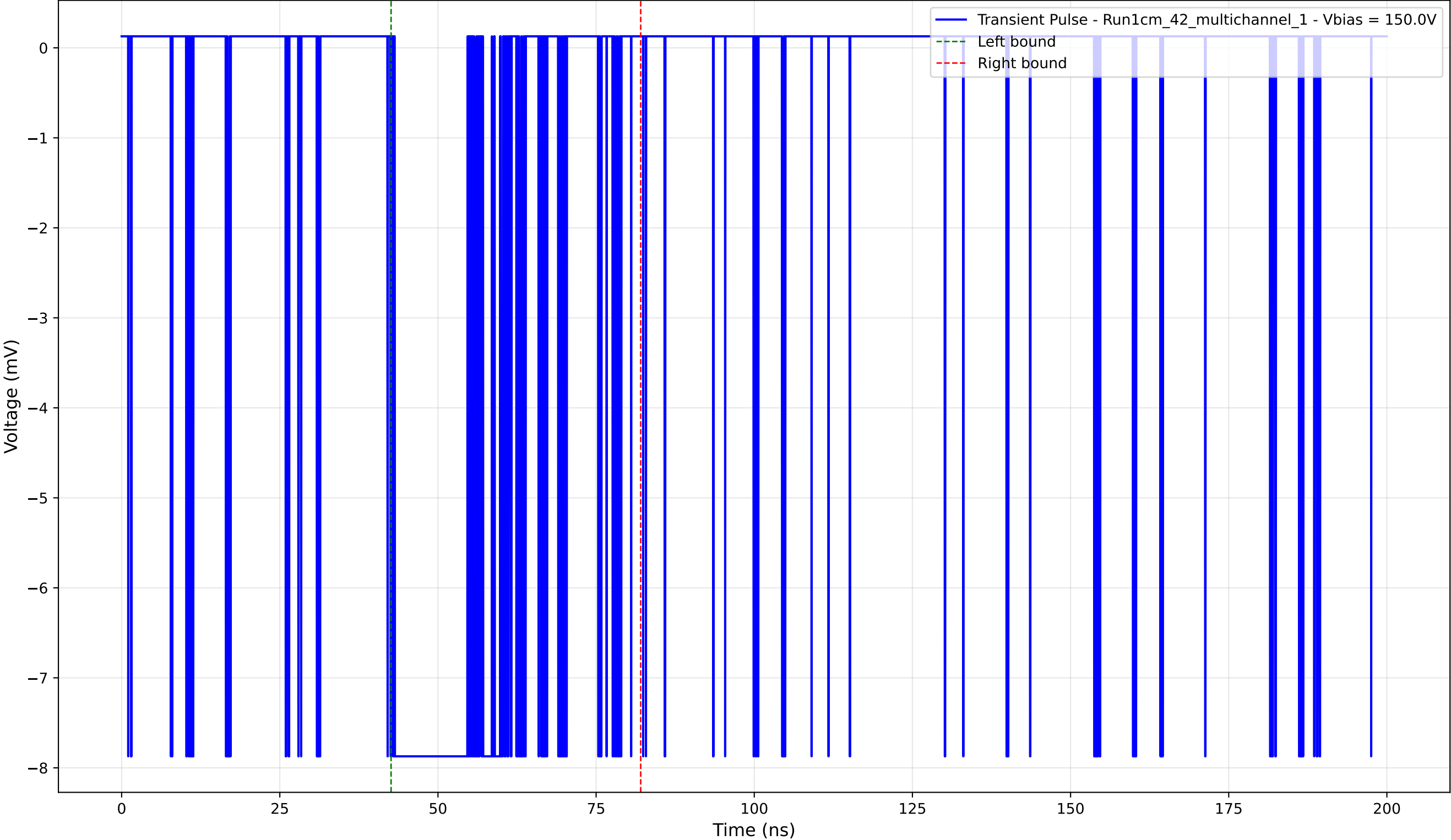
Transient Pulse - Sample: 1cm_42_multichannel - Position: 340.0 \mu\text{m} - Charge: -3.07 pC - Rise Time: 0.02 ns
