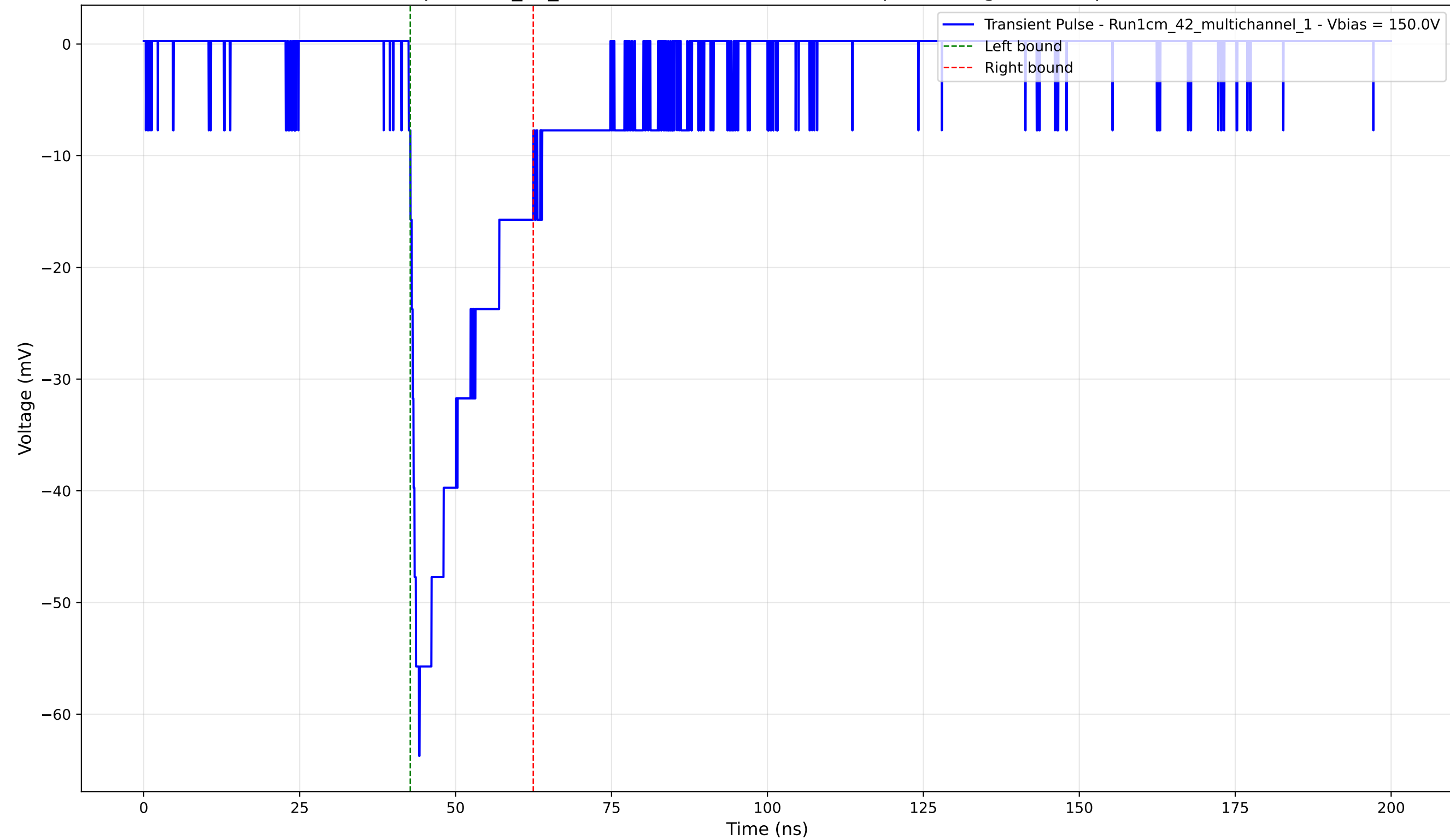
Transient Pulse - Sample: 1cm_42_multichannel - Position: 1320.0 \mu\text{m} - Charge: -12.27 pC - Rise Time: 1.66 ns
