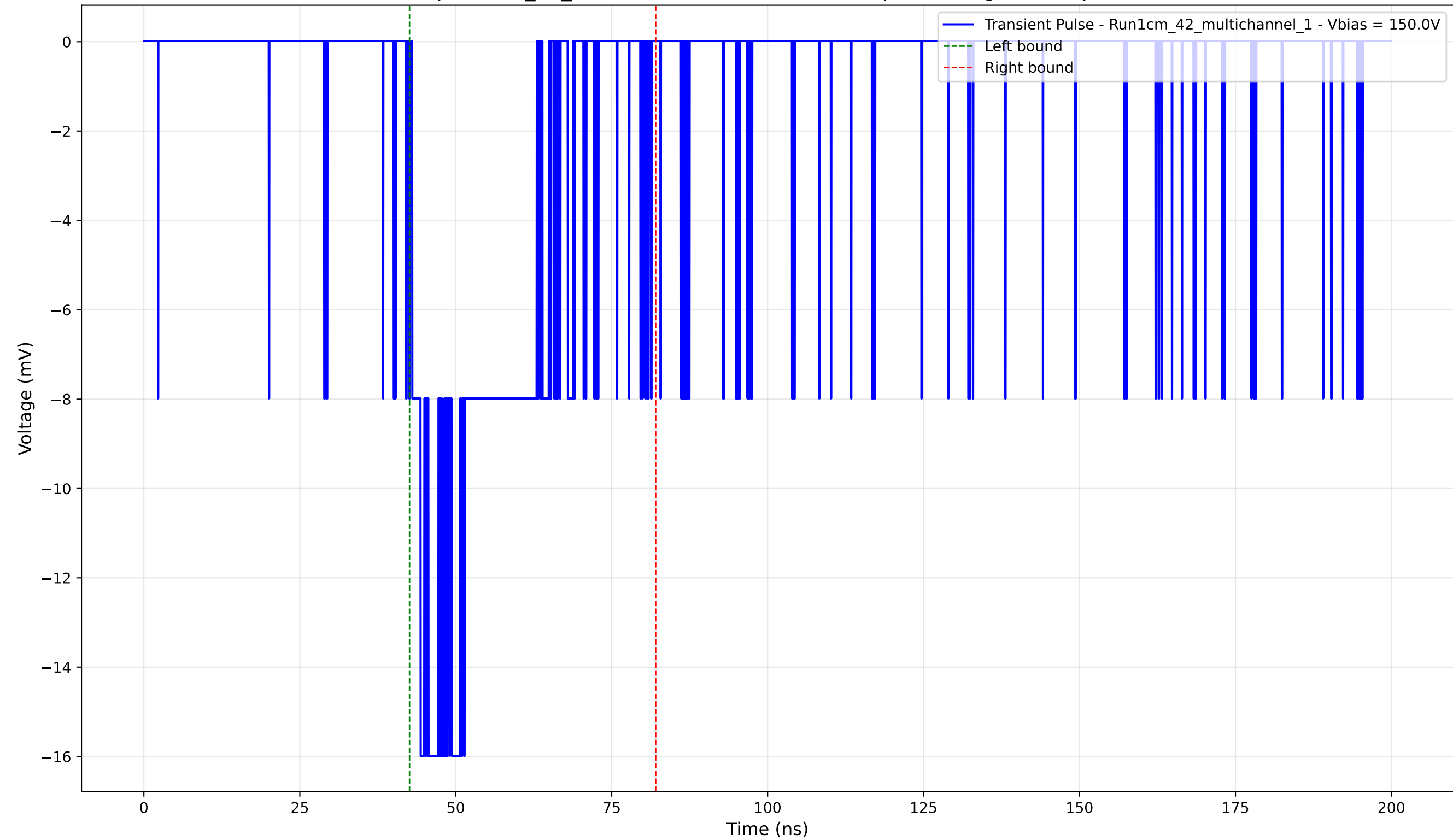
Transient Pulse - Sample: 1cm_42_multichannel - Position: 835.0 \mu\text{m} - Charge: -4.63 pC - Rise Time: 1.36 ns
