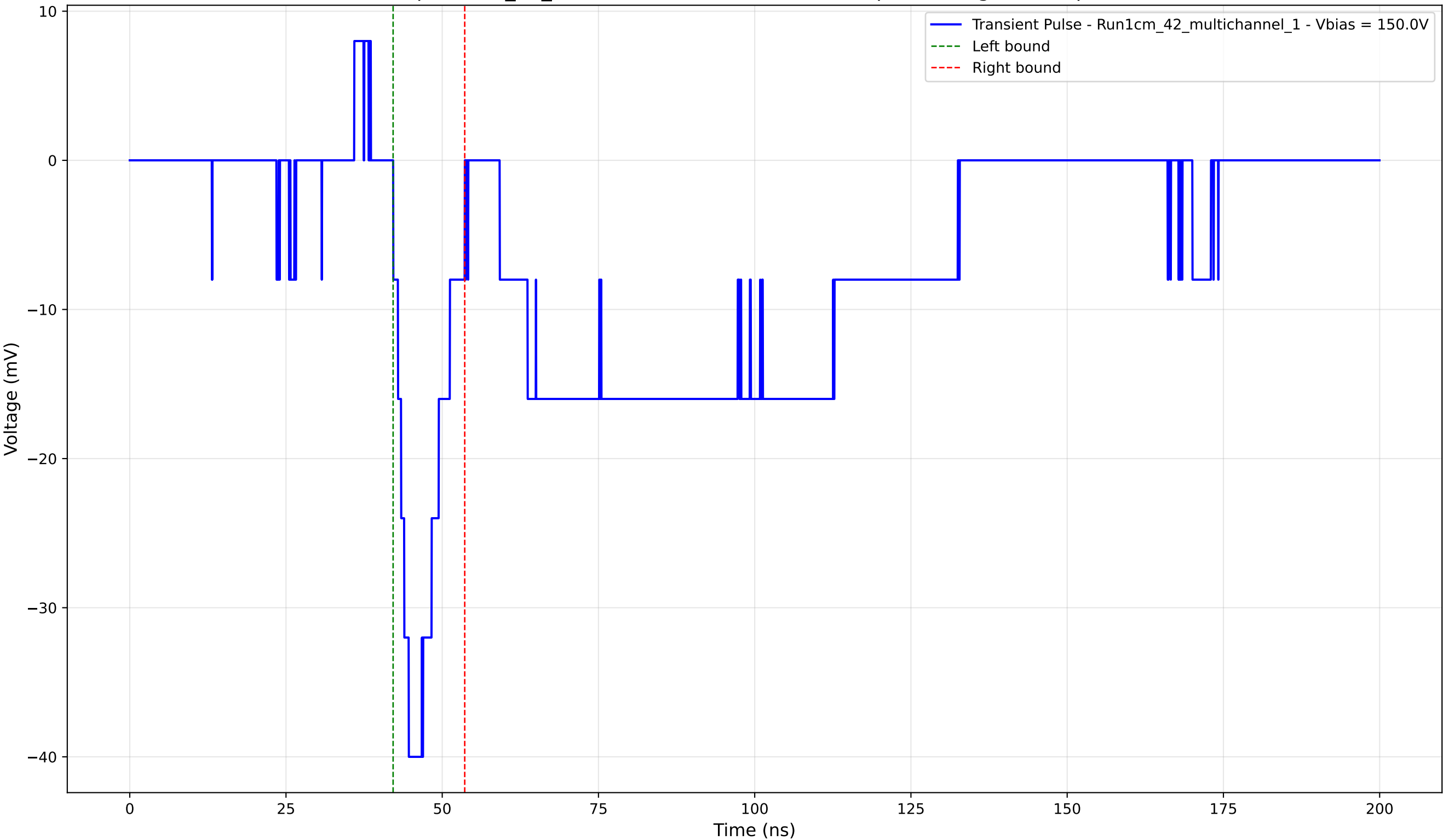
Transient Pulse - Sample: 1cm_42_multichannel - Position: 4810.0 \mu\text{m} - Charge: -5.18 pC - Rise Time: 2.49 ns
