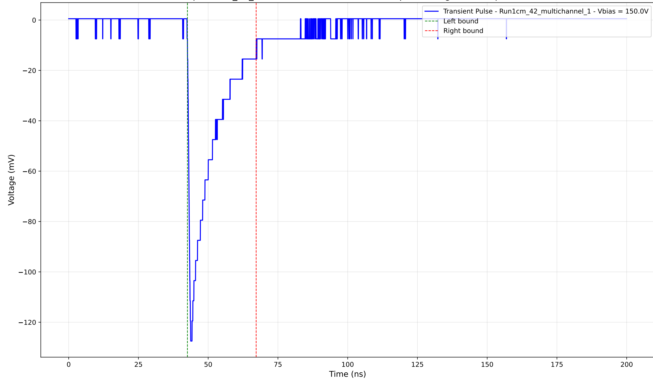
Transient Pulse - Sample: 1cm_42_multichannel - Position: 1485.0 \mu\text{m} - Charge: -22.76 pC - Rise Time: 1.03 ns
