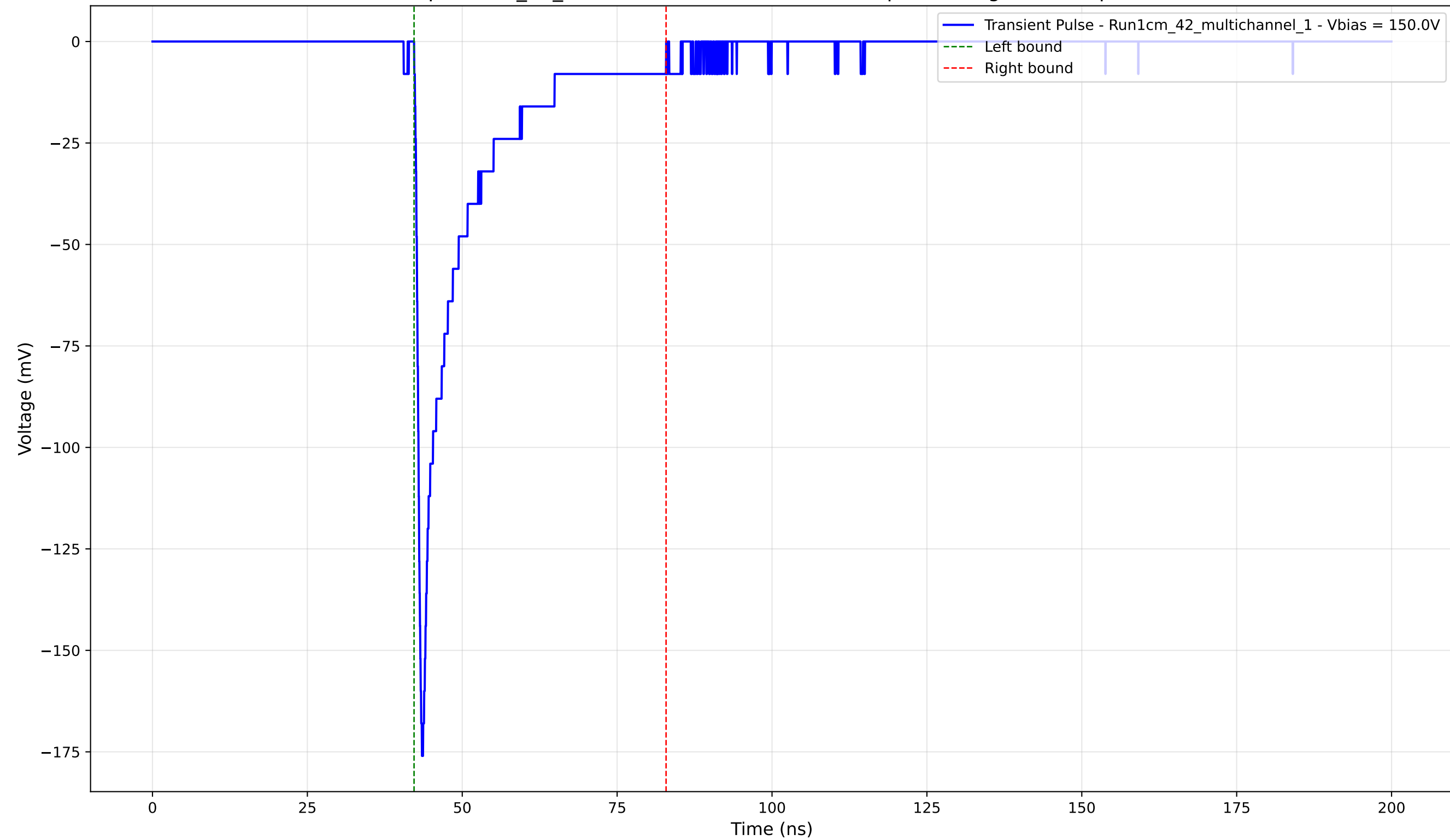
Transient Pulse - Sample: 1cm_42_multichannel - Position: 1785.0 \mu\text{m} - Charge: -24.18 pC - Rise Time: 0.86 ns
