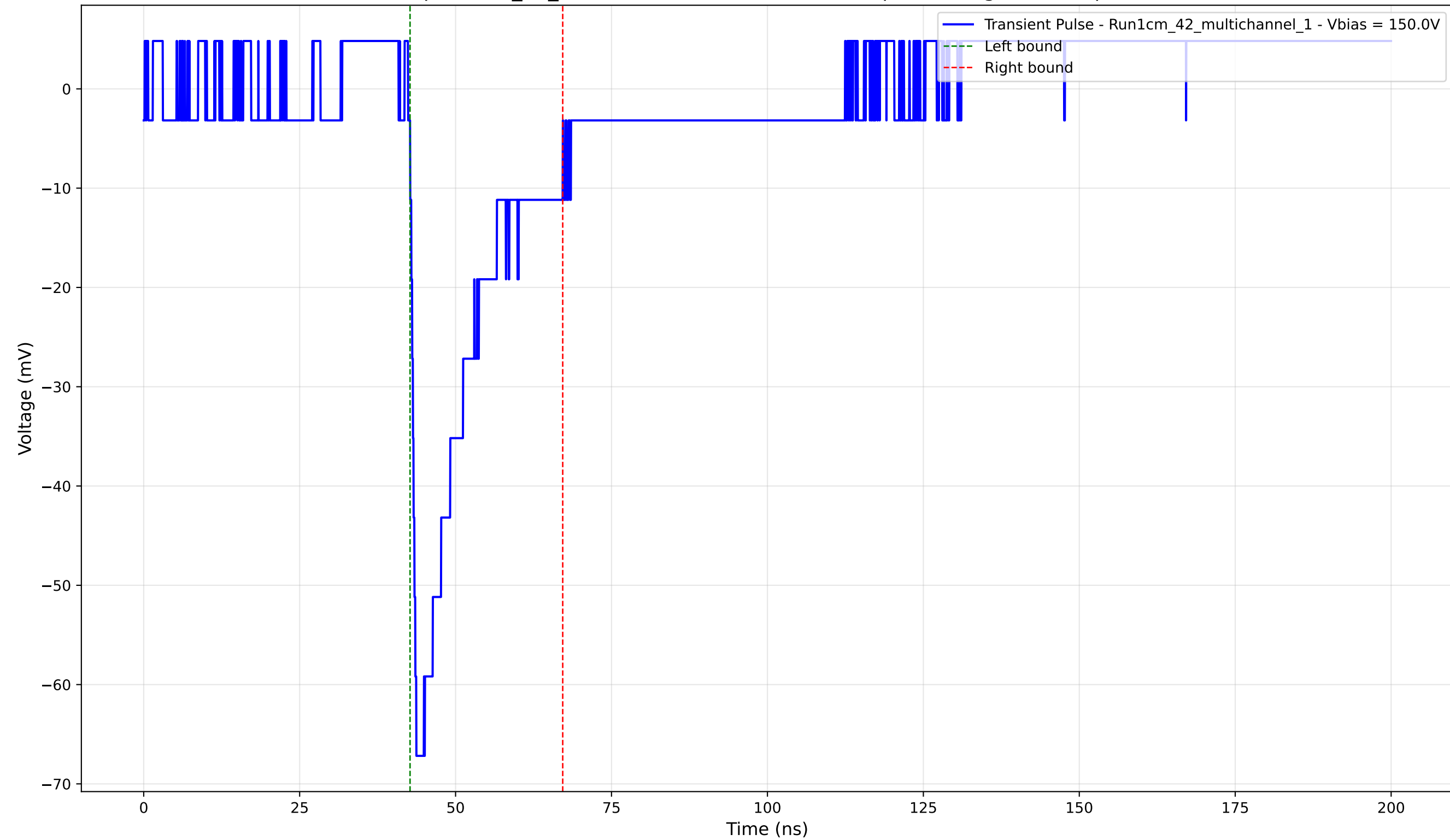
Transient Pulse - Sample: 1cm_42_multichannel - Position: 3550.0 \mu\text{m} - Charge: -12.97 pC - Rise Time: 0.99 ns
