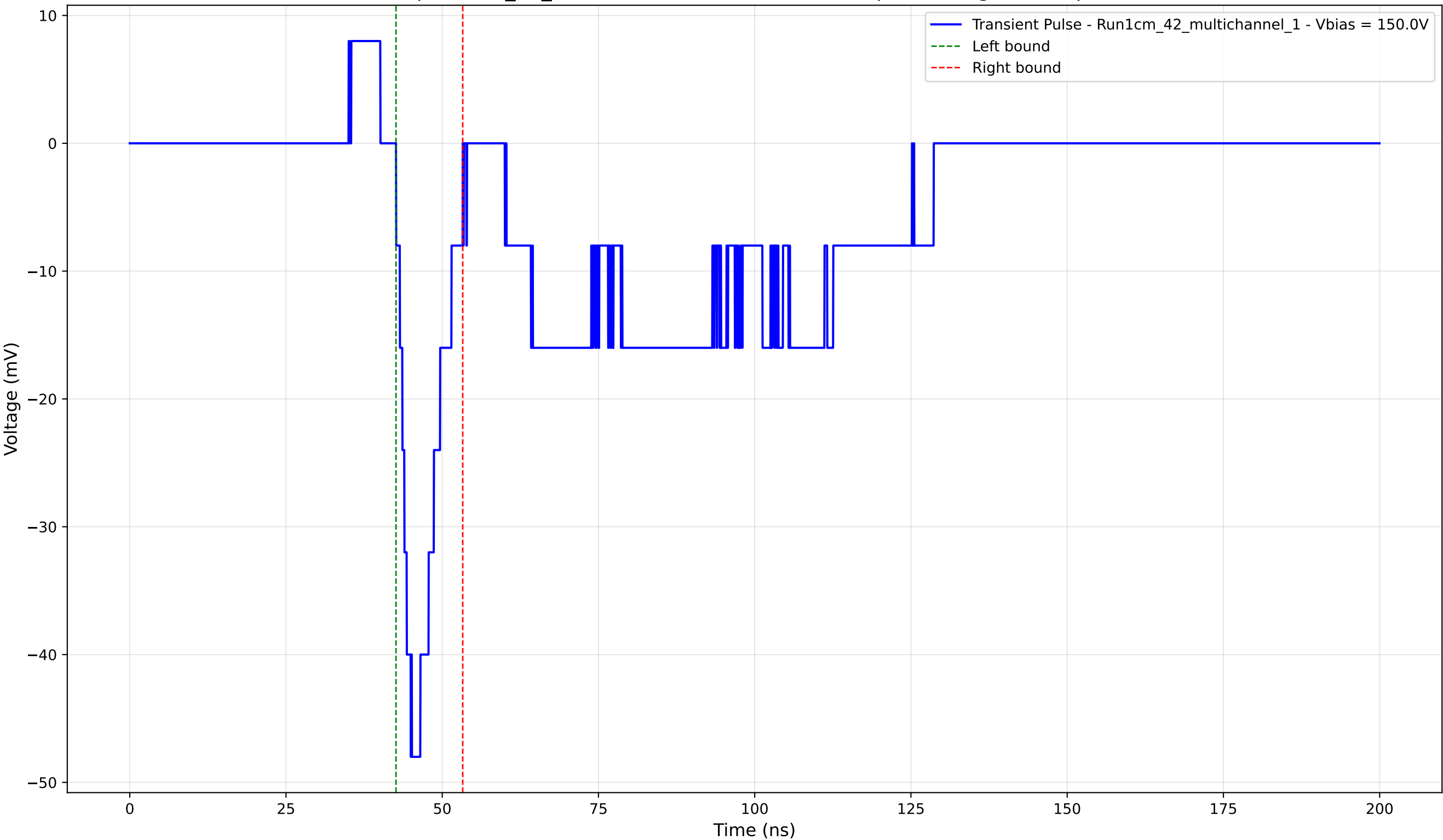
Transient Pulse - Sample: 1cm_42_multichannel - Position: 4530.0 \mu\text{m} - Charge: -5.54 pC - Rise Time: 2.35 ns
