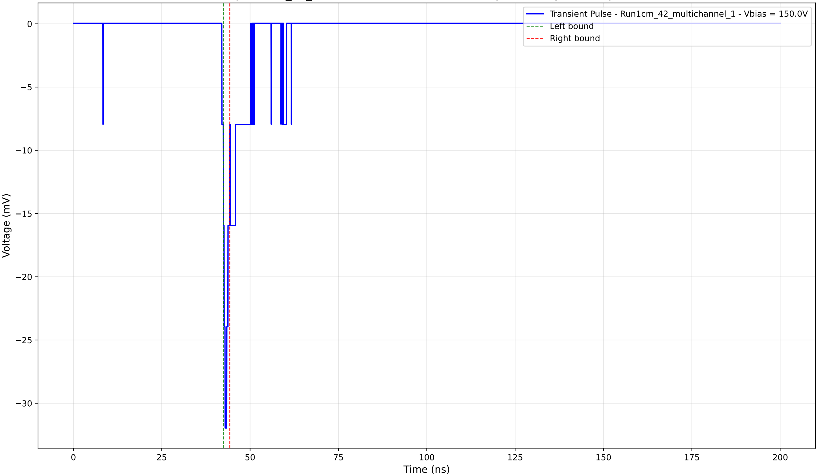
Transient Pulse - Sample: 1cm_42_multichannel - Position: 2410.0 \mu\text{m} - Charge: -0.84 pC - Rise Time: 0.91 ns
