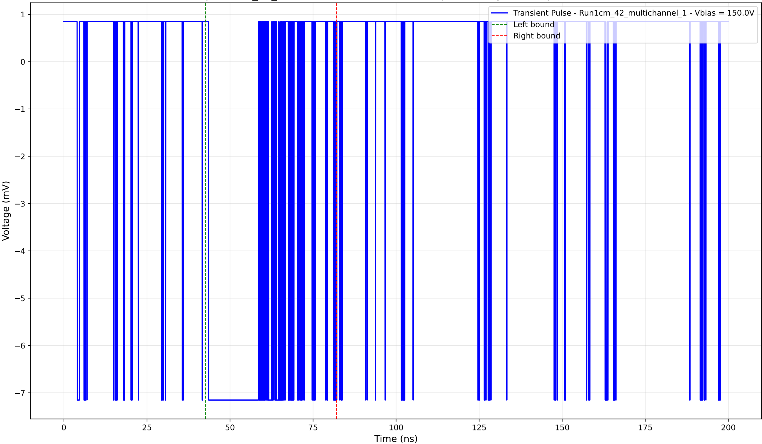
Transient Pulse - Sample: 1cm_42_multichannel - Position: 335.0 \mu\text{m} - Charge: -2.84 pC - Rise Time: 0.00 ns (N/A)
