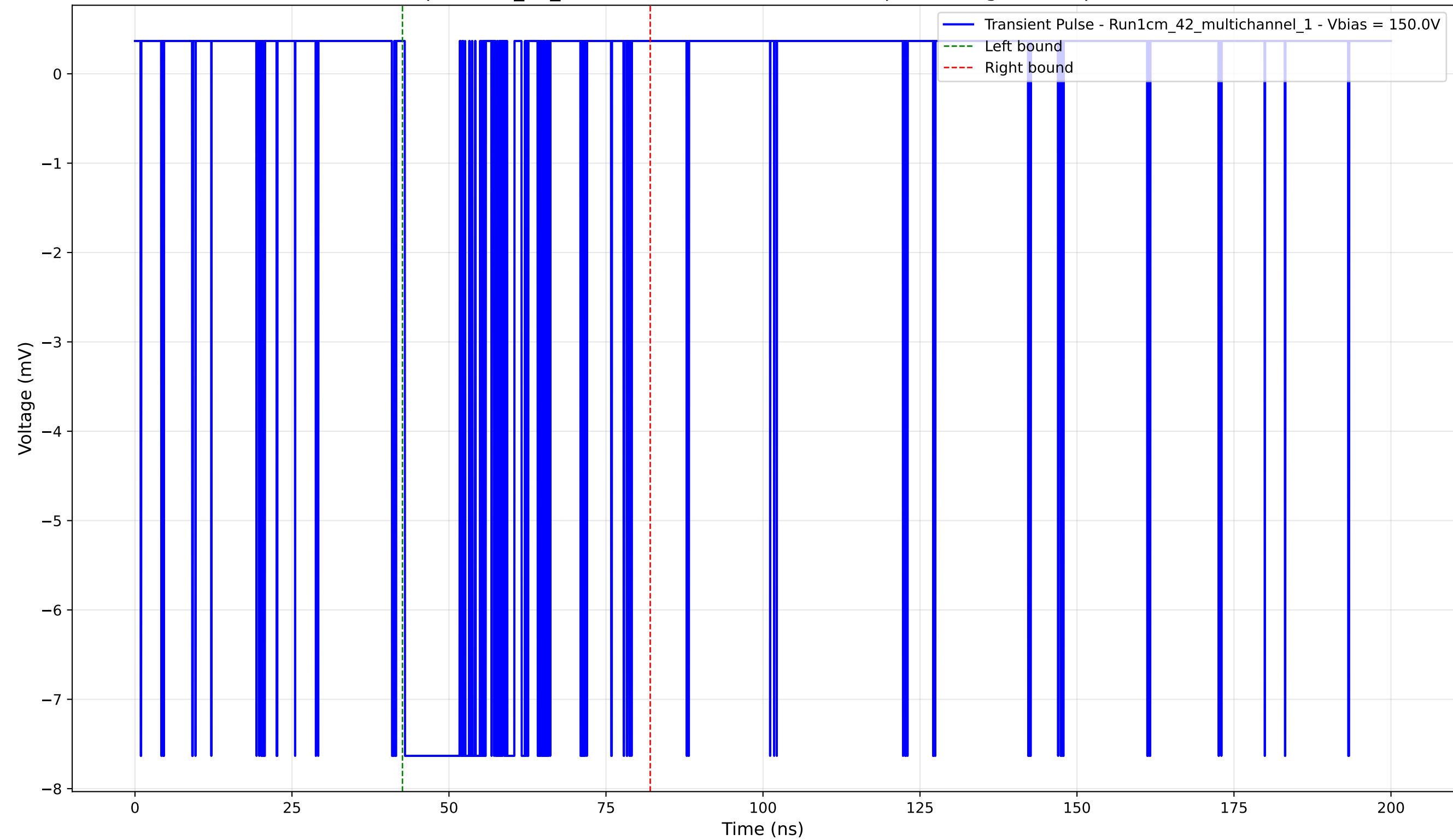
Transient Pulse - Sample: 1cm_42_multichannel - Position: 1390.0 \mu\text{m} - Charge: -2.38 pC - Rise Time: 0.02 ns
