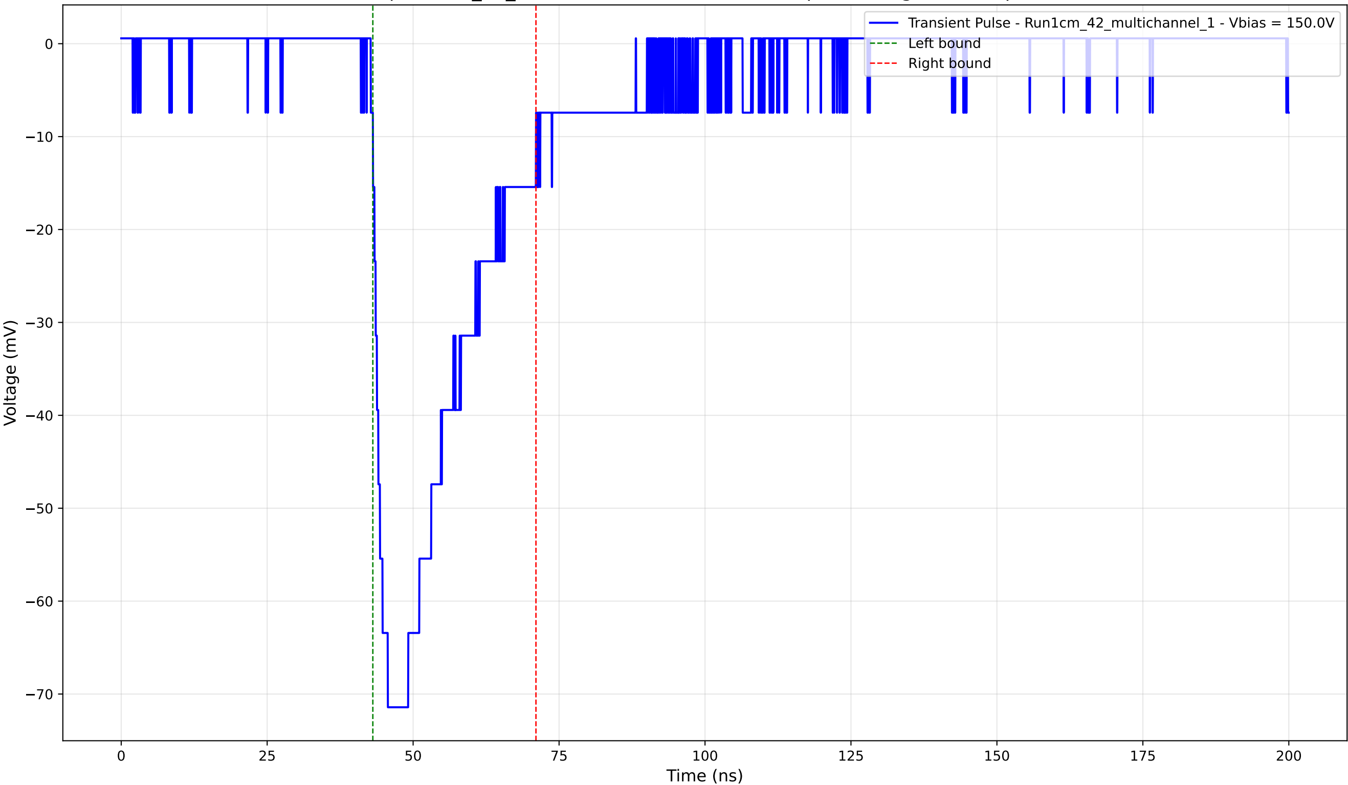
Transient Pulse - Sample: 1cm_42_multichannel - Position: 445.0 \mu\text{m} - Charge: -21.91 pC - Rise Time: 2.92 ns
