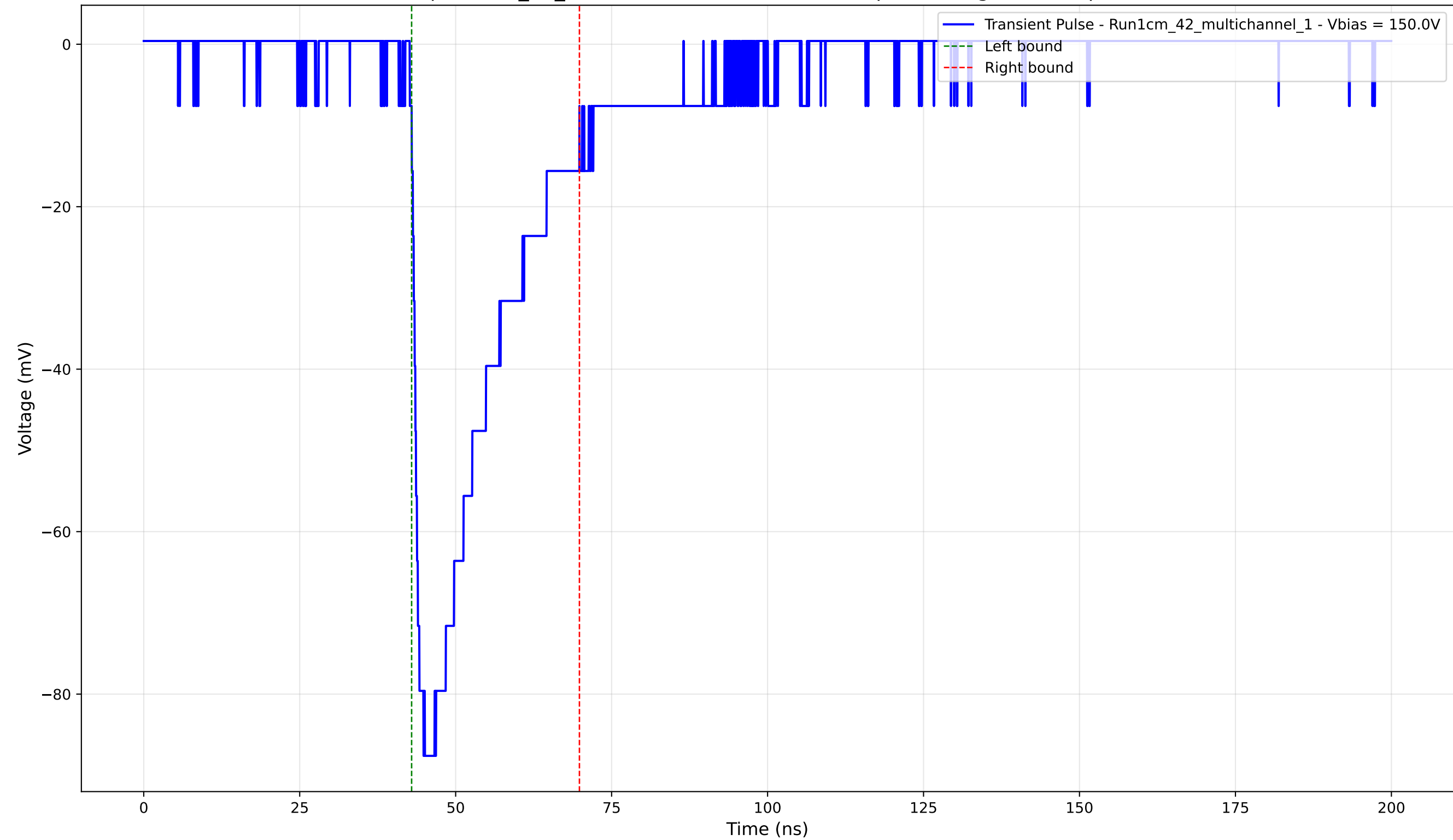
Transient Pulse - Sample: 1cm_42_multichannel - Position: 980.0 \mu\text{m} - Charge: -23.14 pC - Rise Time: 1.24 ns
