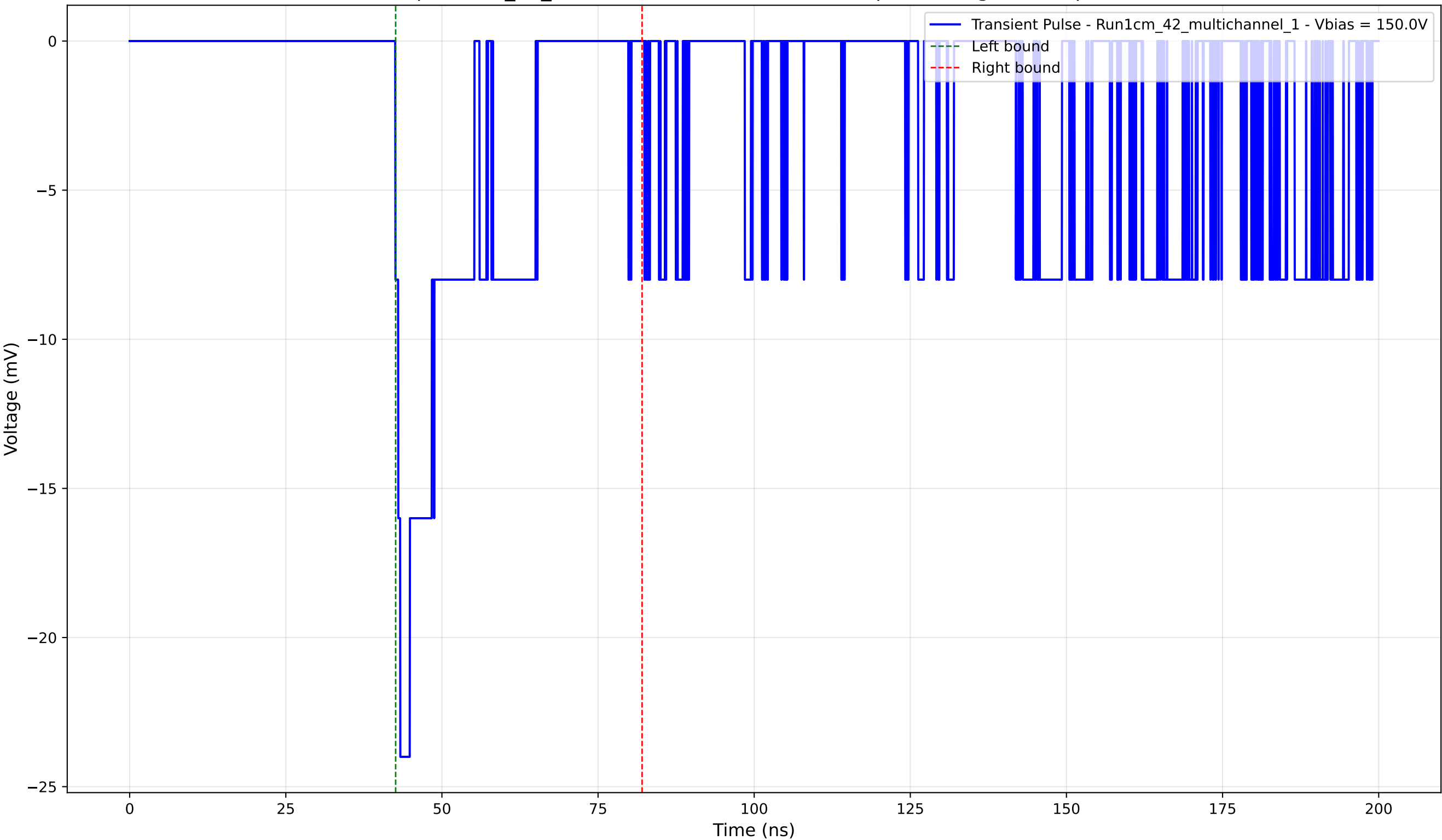
Transient Pulse - Sample: 1cm_42_multichannel - Position: 3360.0 \mu\text{m} - Charge: -4.51 pC - Rise Time: 0.79 ns
