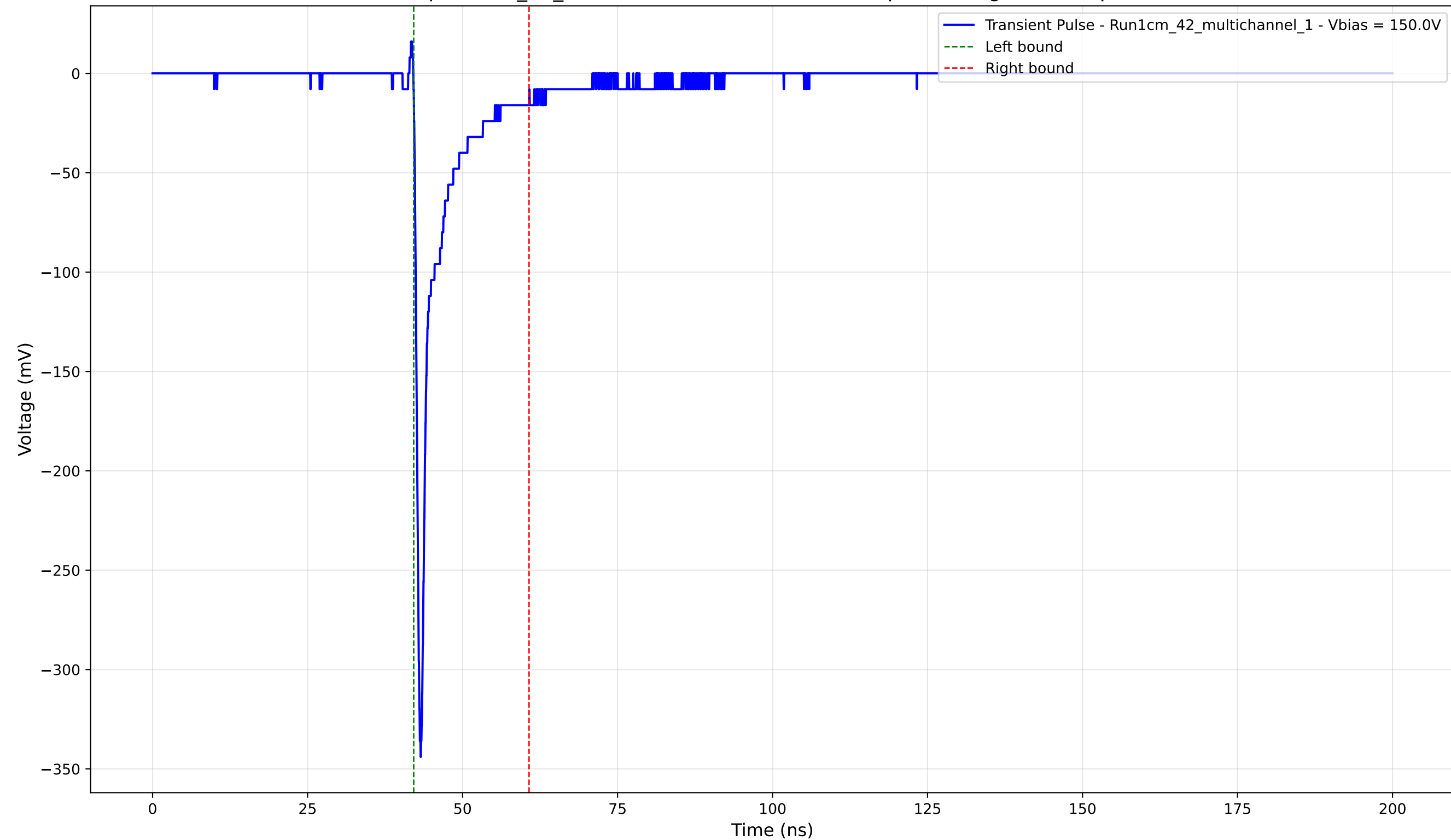
Transient Pulse - Sample: 1cm_42_multichannel - Position: 2585.0 \mu\text{m} - Charge: -22.79 pC - Rise Time: 0.75 ns
