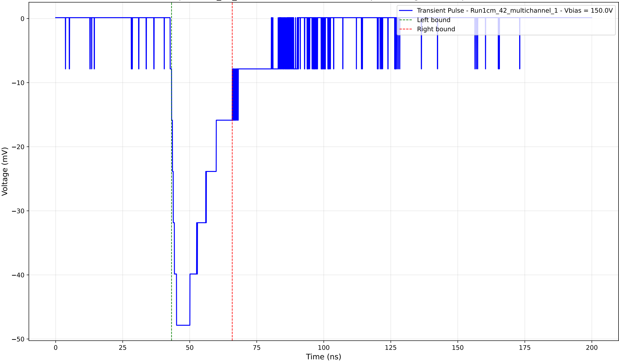
Transient Pulse - Sample: 1cm_42_multichannel - Position: 420.0 \mu\text{m} - Charge: -13.92 pC - Rise Time: 2.39 ns
