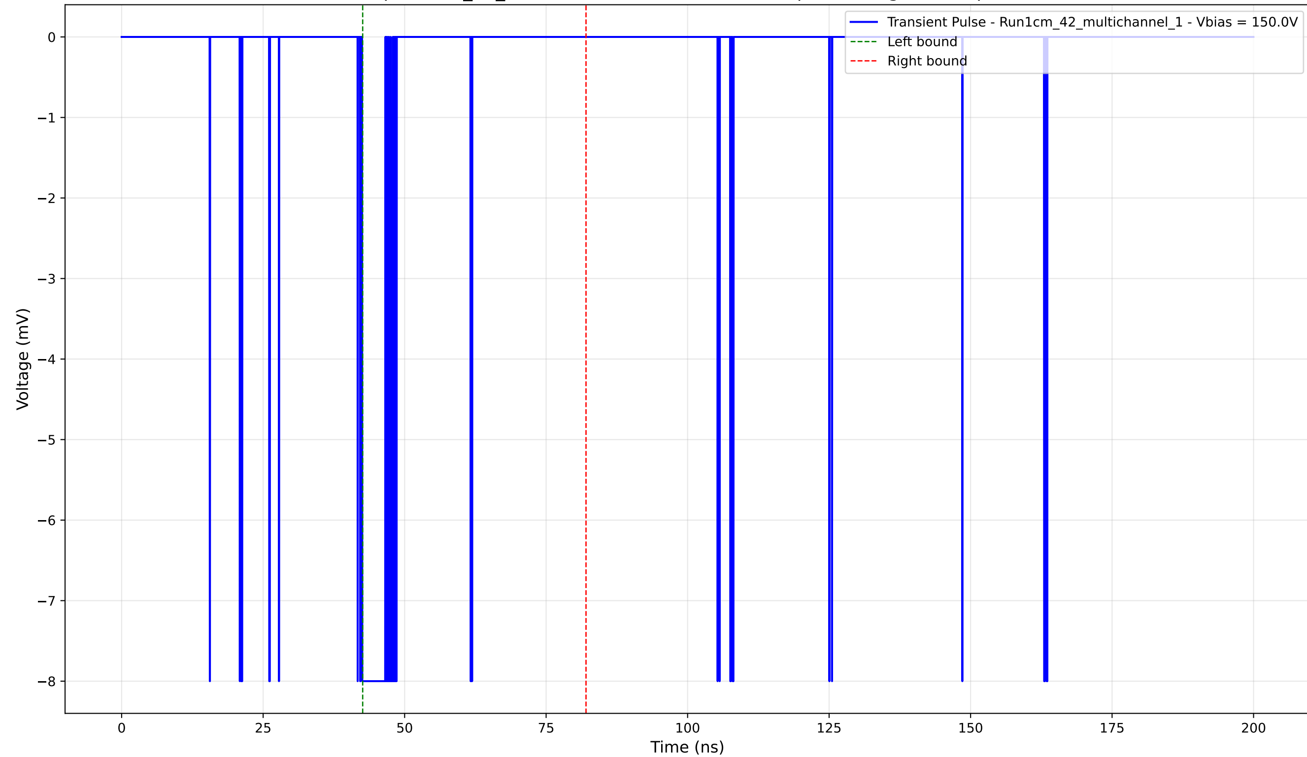
Transient Pulse - Sample: 1cm_42_multichannel - Position: 3395.0 \mu\text{m} - Charge: -0.85 pC - Rise Time: 0.02 ns
