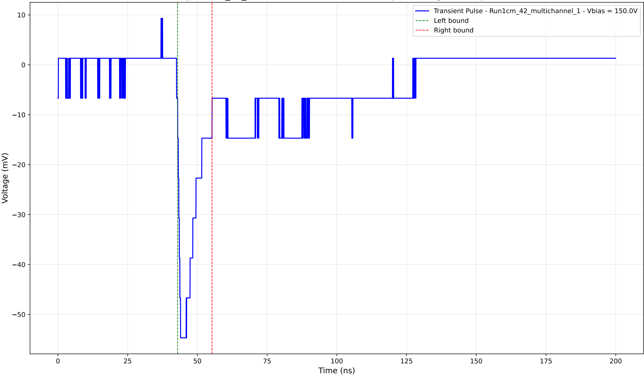
Transient Pulse - Sample: 1cm_42_multichannel - Position: 3810.0 \mu\text{m} - Charge: -7.65 pC - Rise Time: 1.42 ns
