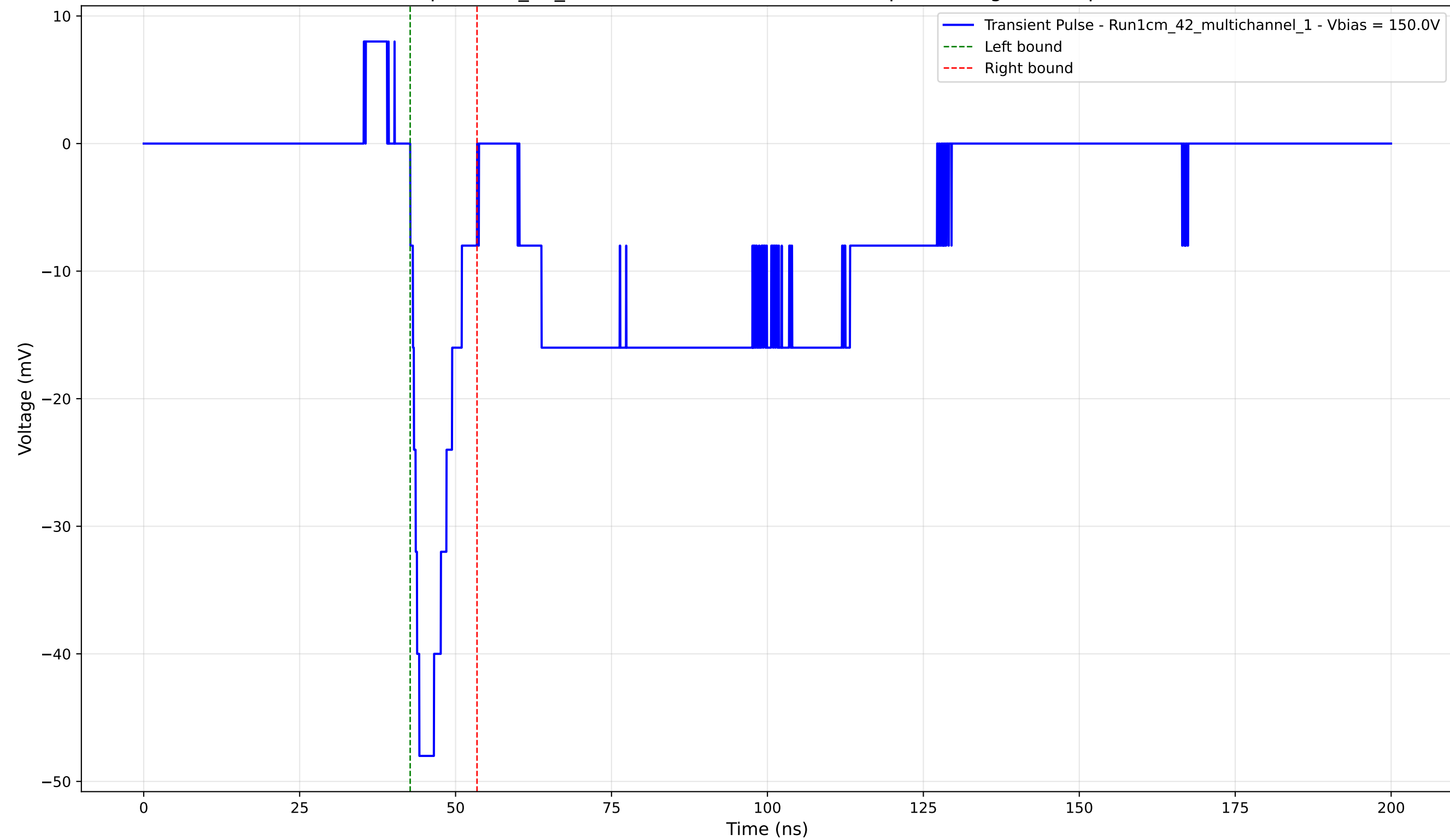
Transient Pulse - Sample: 1cm_42_multichannel - Position: 4000.0 \mu\text{m} - Charge: -5.72 pC - Rise Time: 1.45 ns
