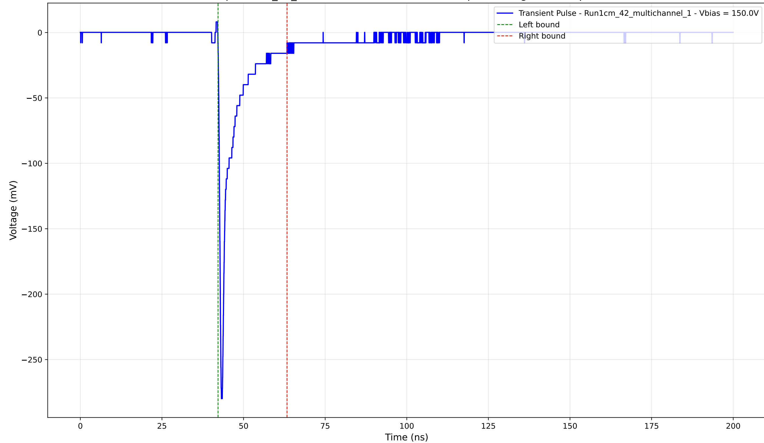
Transient Pulse - Sample: 1cm_42_multichannel - Position: 2700.0 \mu\text{m} - Charge: -22.91 pC - Rise Time: 0.77 ns
