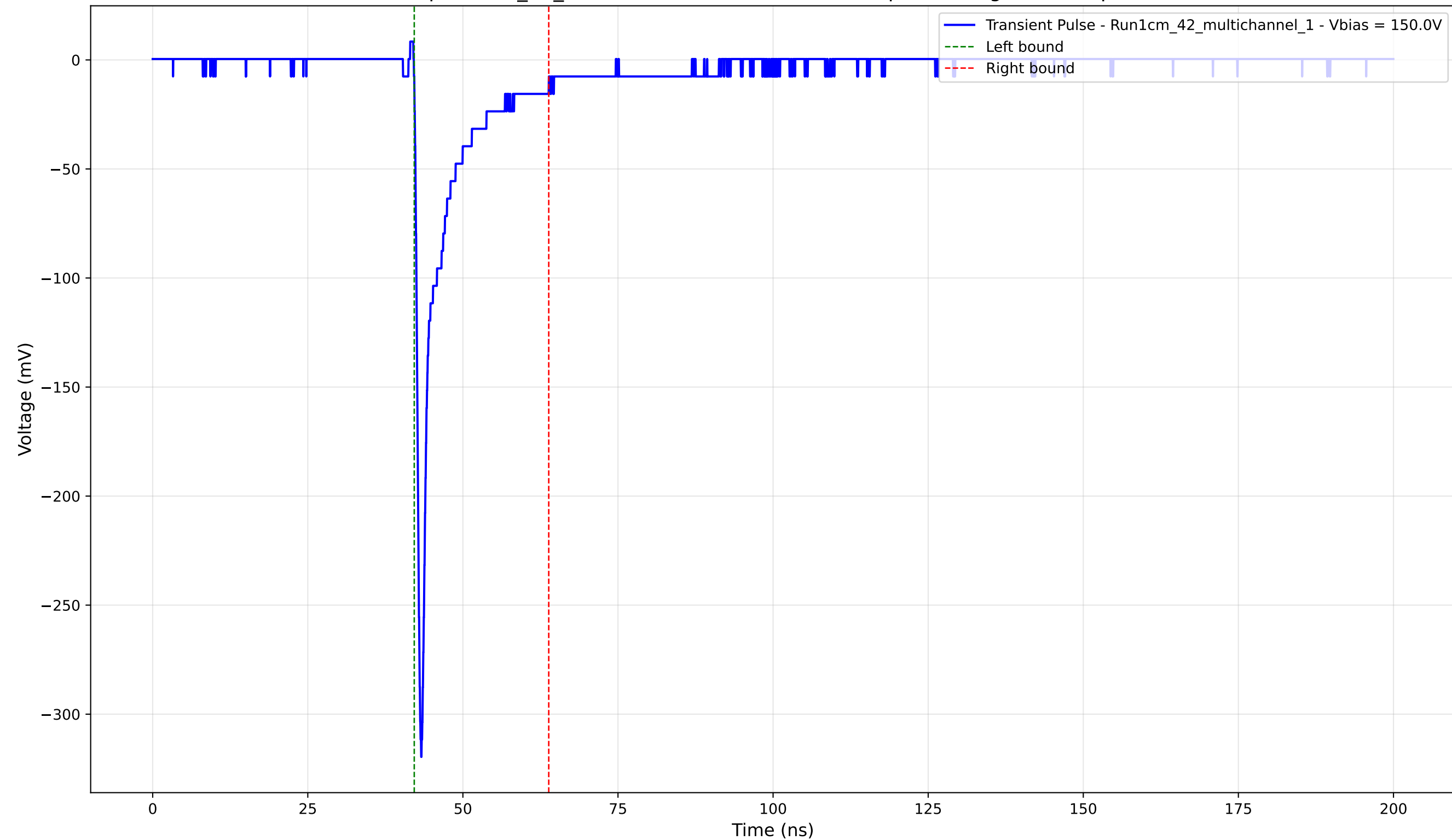
Transient Pulse - Sample: 1cm_42_multichannel - Position: 2125.0 \mu\text{m} - Charge: -23.97 pC - Rise Time: 0.80 ns
