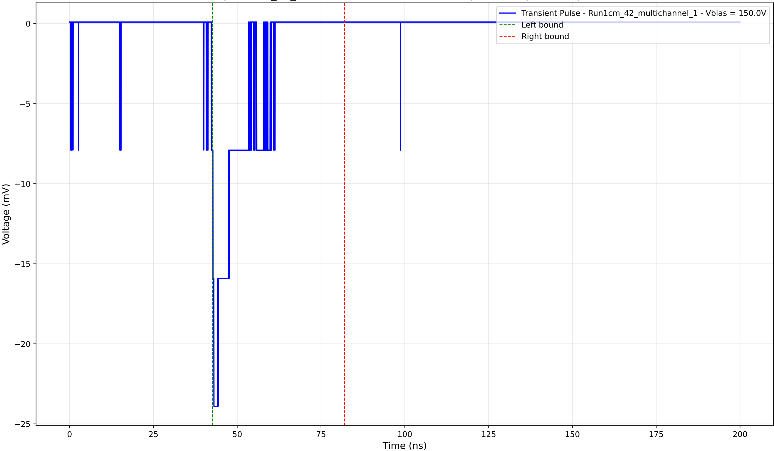
Transient Pulse - Sample: 1cm_42_multichannel - Position: 1850.0 \mu\text{m} - Charge: -3.30 pC - Rise Time: 0.63 ns
