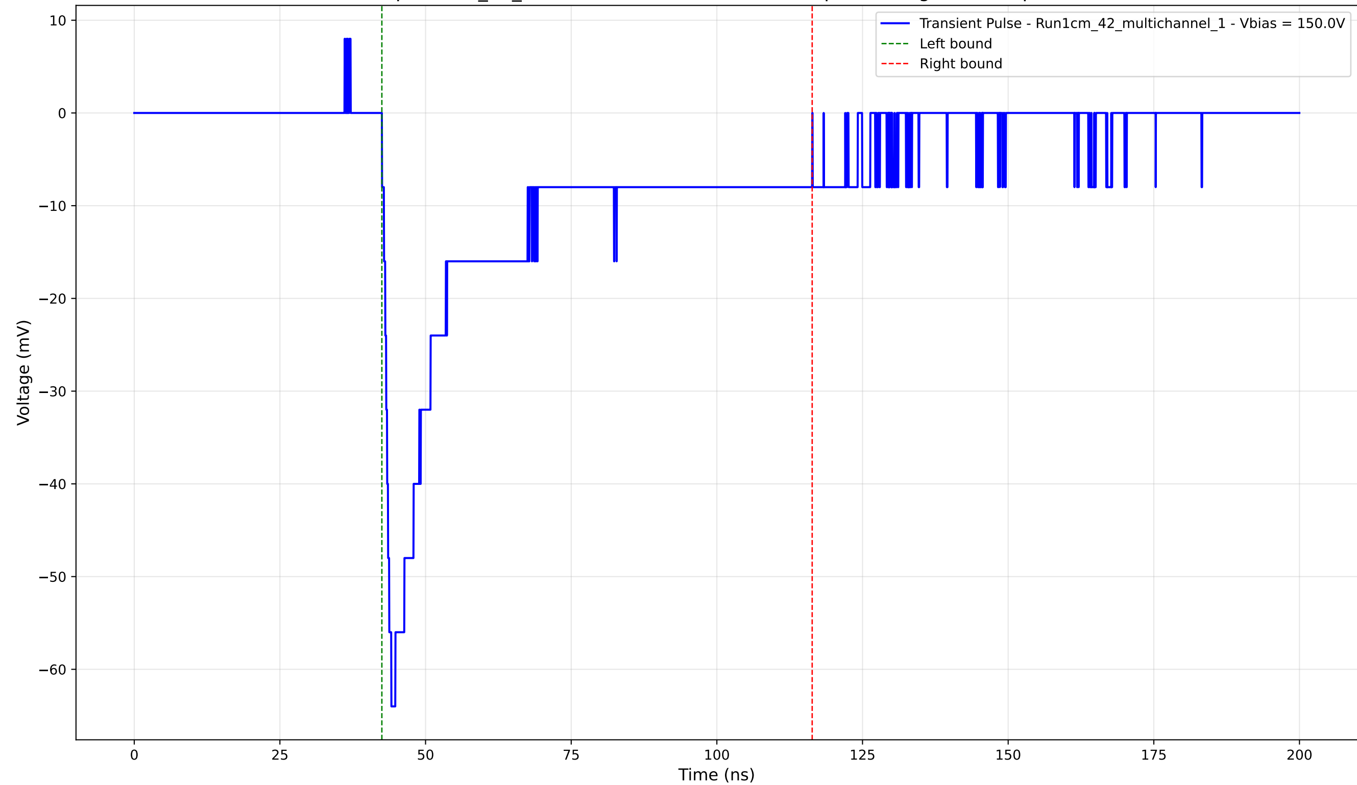
Transient Pulse - Sample: 1cm_42_multichannel - Position: 3695.0 \mu\text{m} - Charge: -20.89 pC - Rise Time: 1.60 ns
