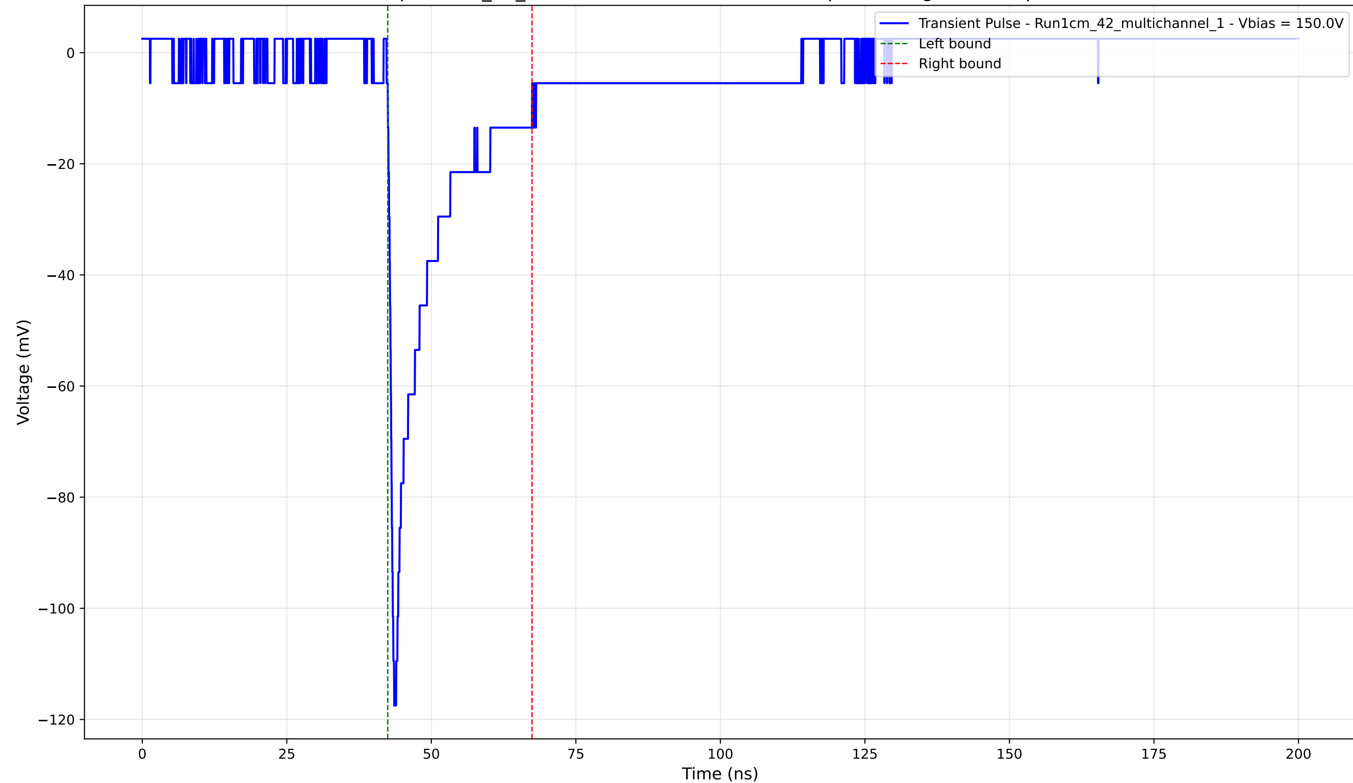
Transient Pulse - Sample: 1cm_42_multichannel - Position: 3190.0 \mu\text{m} - Charge: -16.65 pC - Rise Time: 0.94 ns
