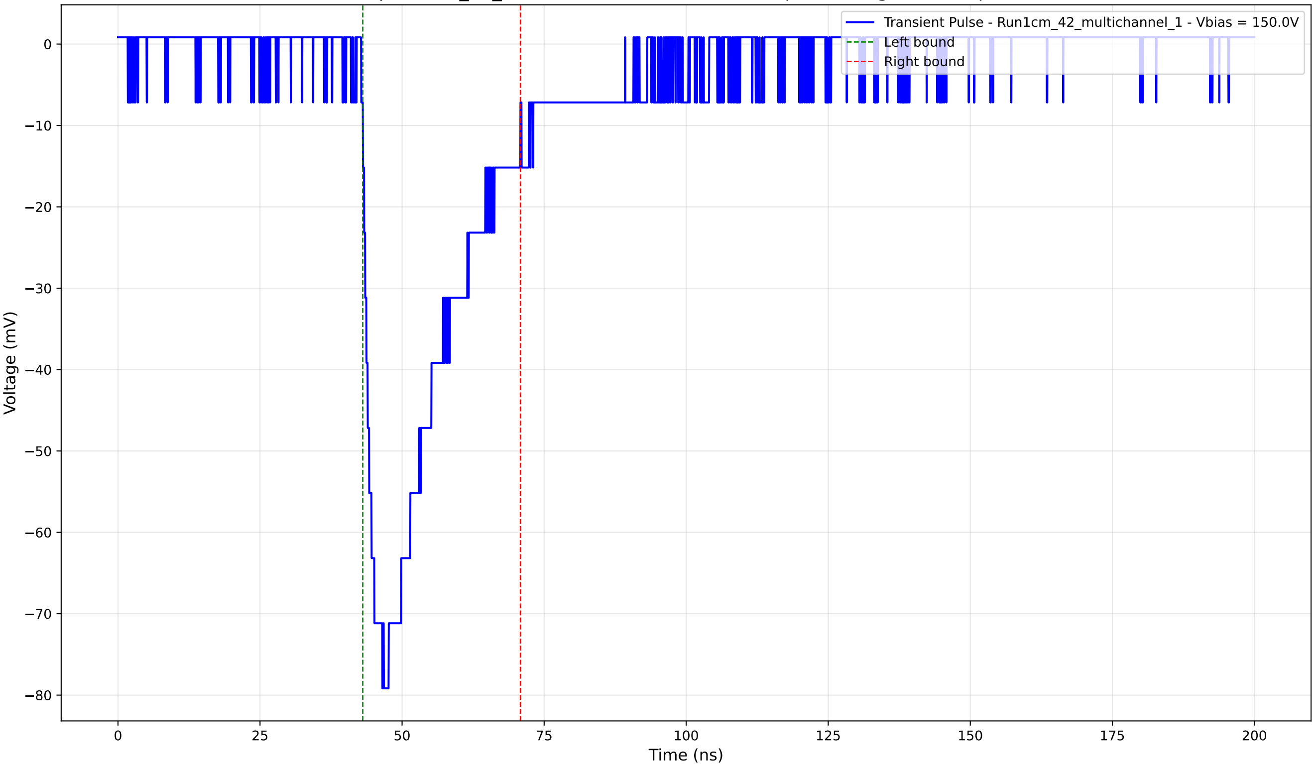
Transient Pulse - Sample: 1cm_42_multichannel - Position: 465.0 \mu\text{m} - Charge: -22.34 pC - Rise Time: 3.44 ns
