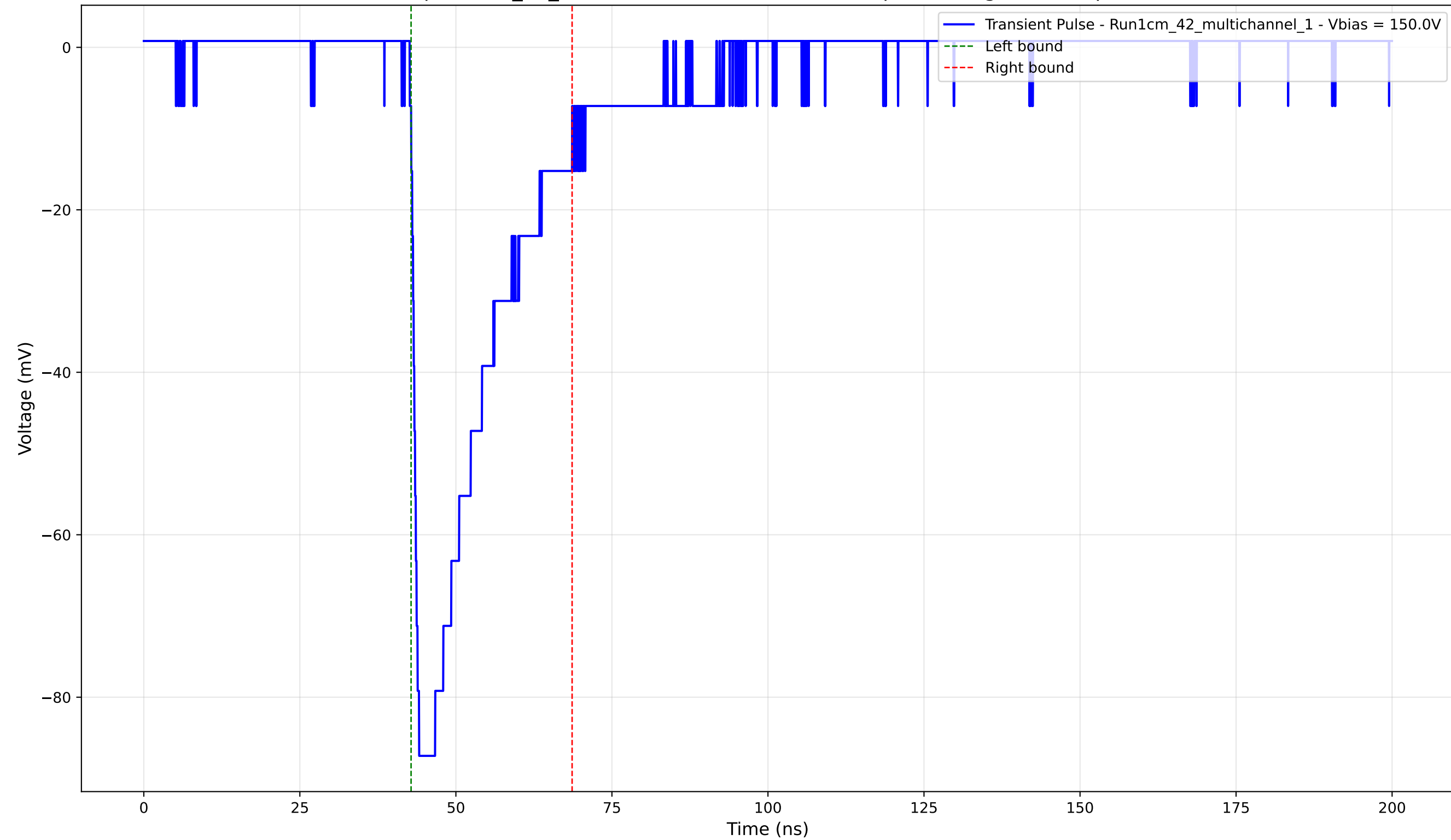
Transient Pulse - Sample: 1cm_42_multichannel - Position: 1125.0 \mu\text{m} - Charge: -22.09 pC - Rise Time: 1.04 ns
