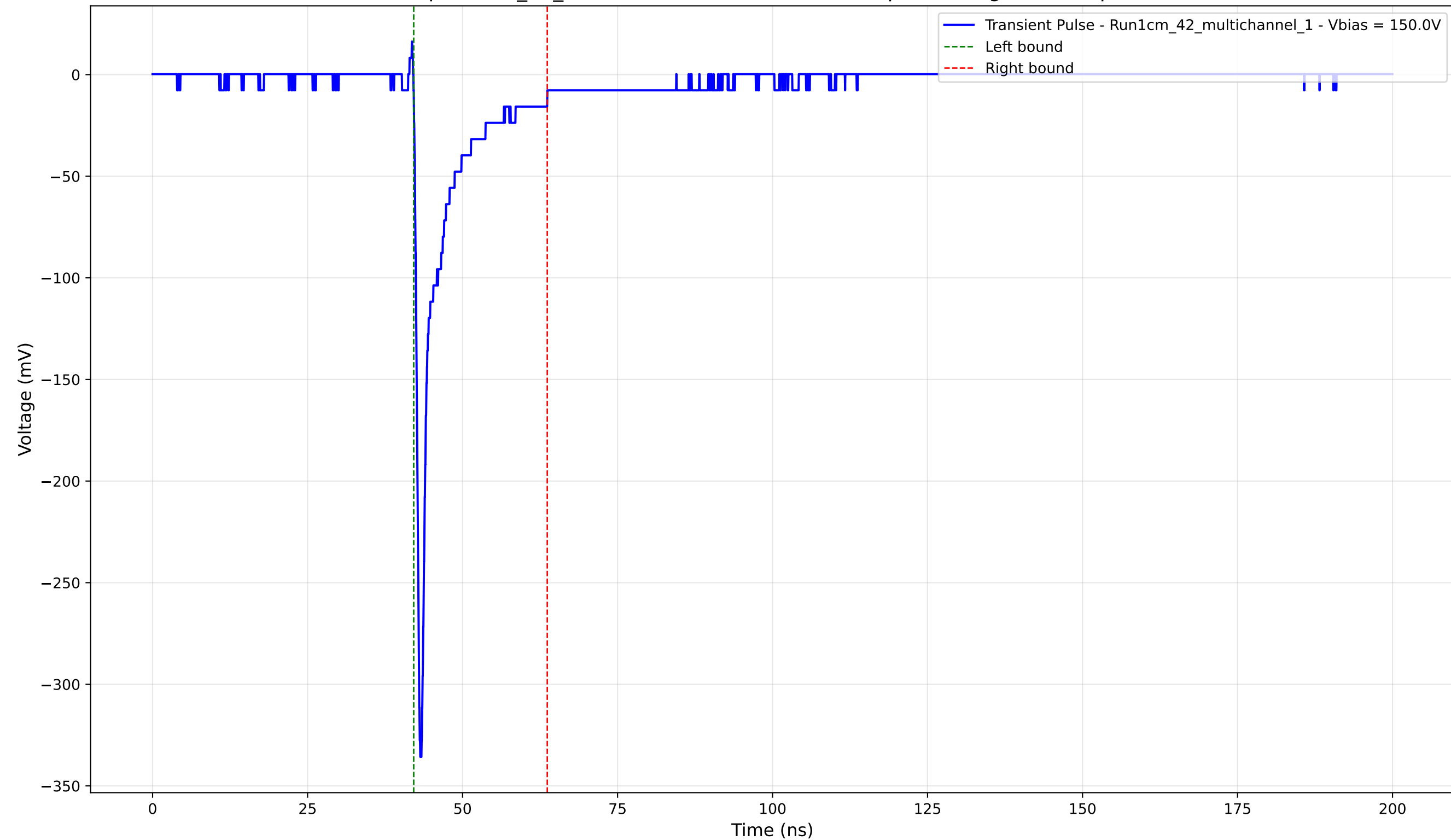
Transient Pulse - Sample: 1cm_42_multichannel - Position: 2165.0 \mu\text{m} - Charge: -24.51 pC - Rise Time: 0.75 ns
