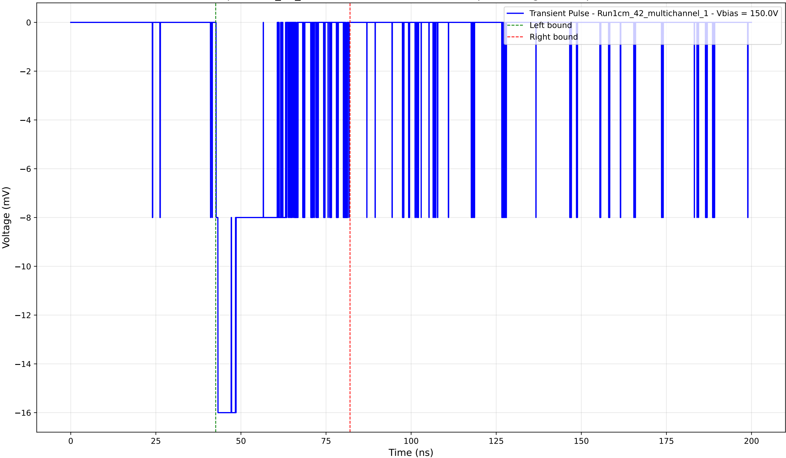
Transient Pulse - Sample: 1cm_42_multichannel - Position: 1405.0 \mu\text{m} - Charge: -4.62 pC - Rise Time: 0.56 ns
