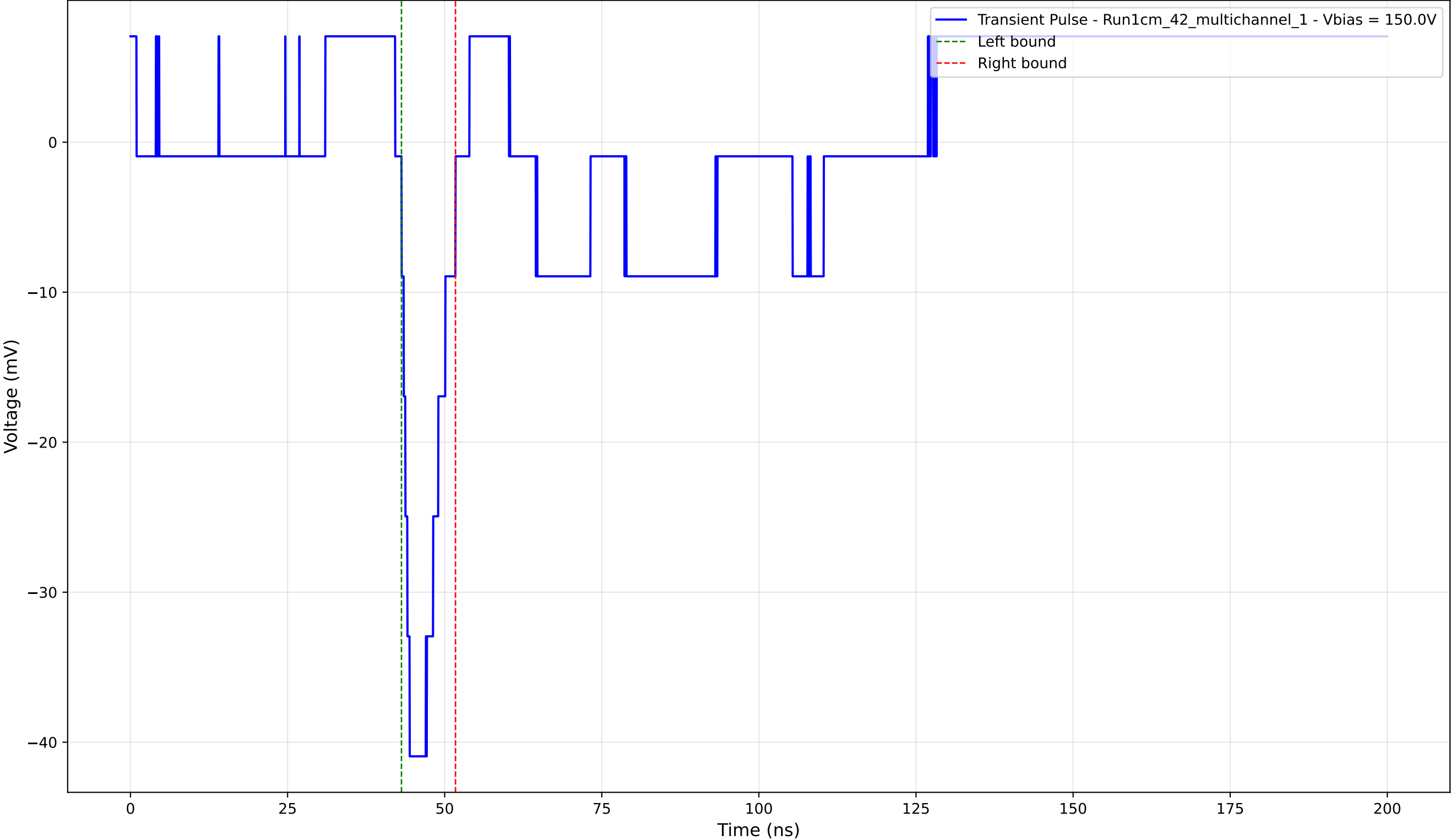
Transient Pulse - Sample: 1cm_42_multichannel - Position: 4260.0 \mu\text{m} - Charge: -4.51 pC - Rise Time: 1.29 ns
