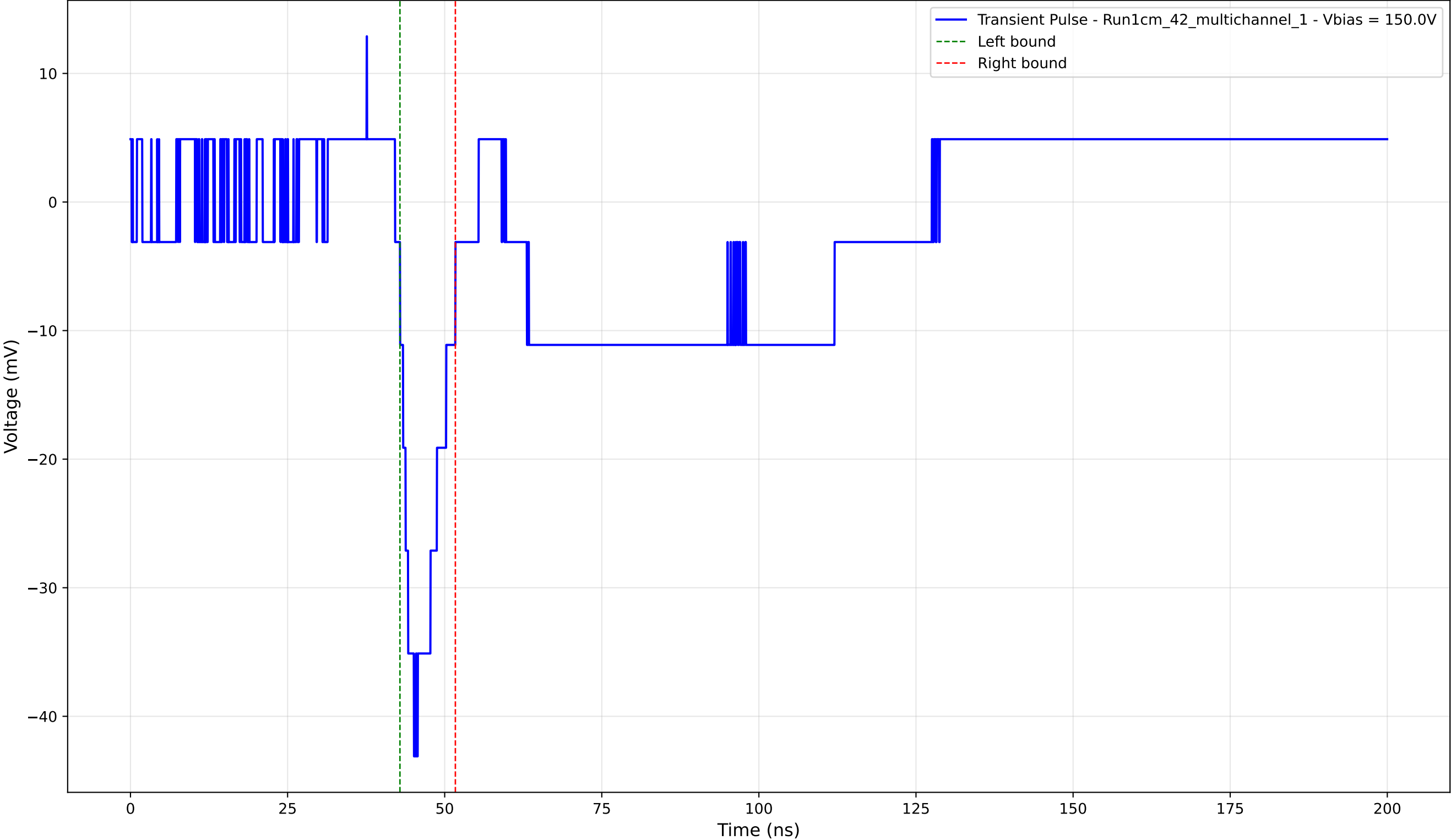
Transient Pulse - Sample: 1cm_42_multichannel - Position: 4765.0 \mu\text{m} - Charge: -4.50 pC - Rise Time: 2.22 ns
