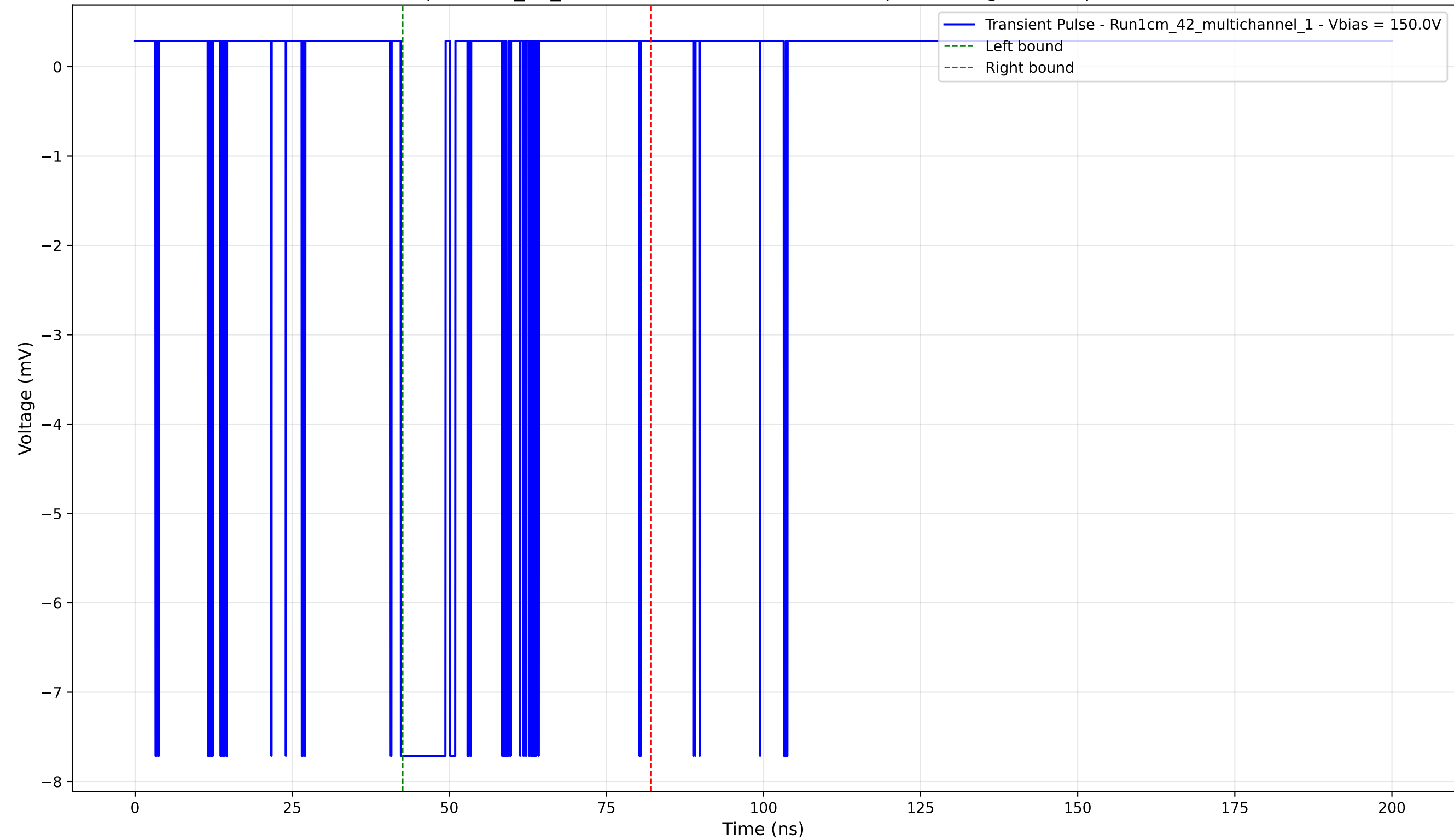
Transient Pulse - Sample: 1cm_42_multichannel - Position: 2895.0 \mu\text{m} - Charge: -1.35 pC - Rise Time: 0.02 ns
