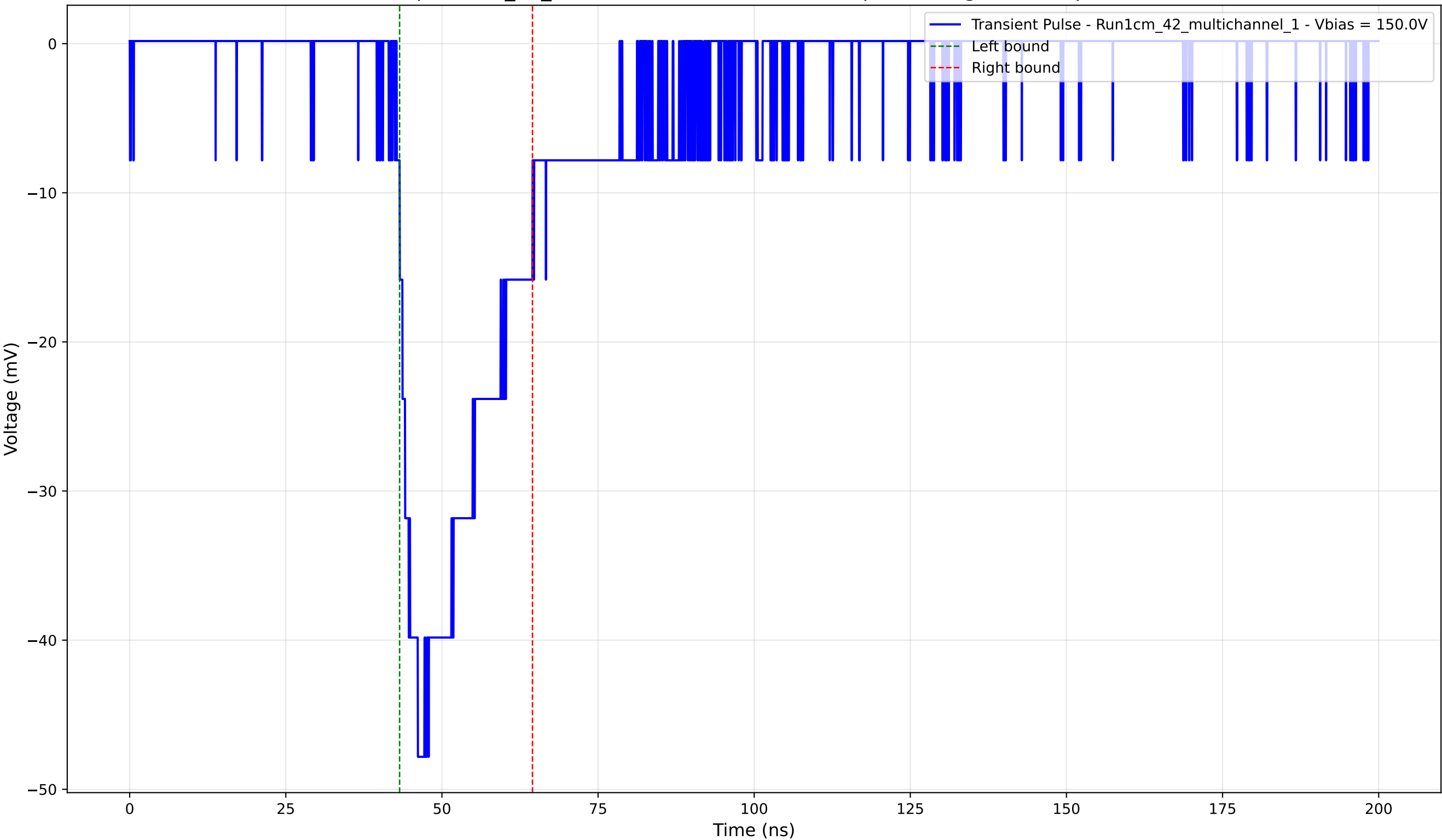
Transient Pulse - Sample: 1cm_42_multichannel - Position: 305.0 \mu\text{m} - Charge: -12.43 pC - Rise Time: 3.39 ns
