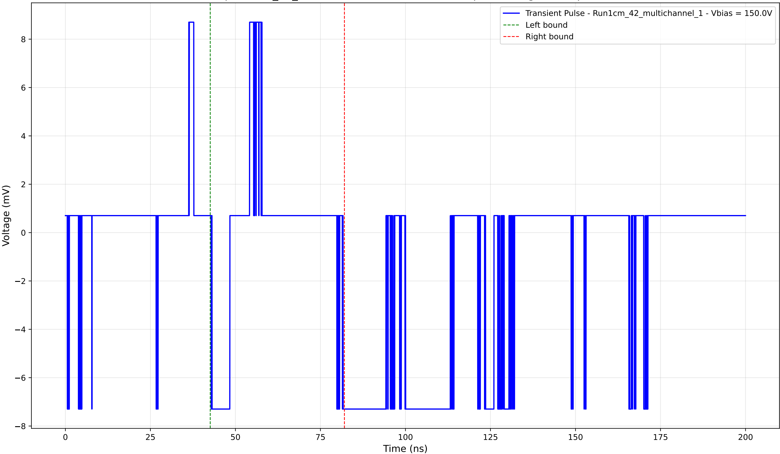
Transient Pulse - Sample: 1cm_42_multichannel - Position: 3935.0 \mu\text{m} - Charge: 0.06 pC - Rise Time: 0.02 ns
