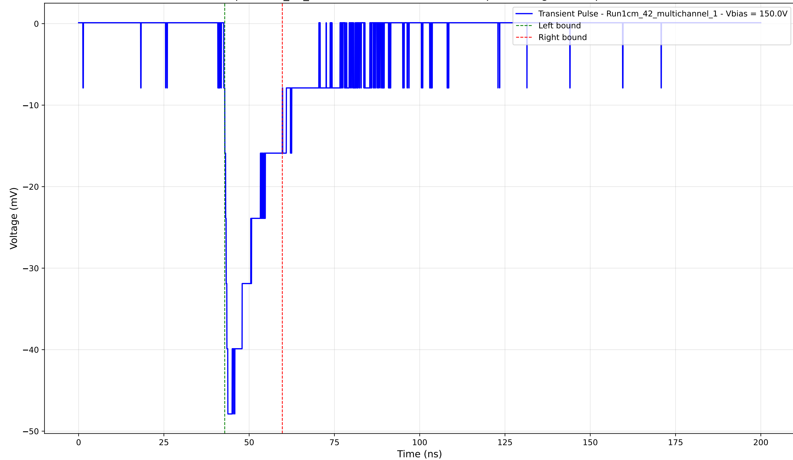
Transient Pulse - Sample: 1cm_42_multichannel - Position: 1325.0 \mu\text{m} - Charge: -9.27 pC - Rise Time: 1.19 ns
