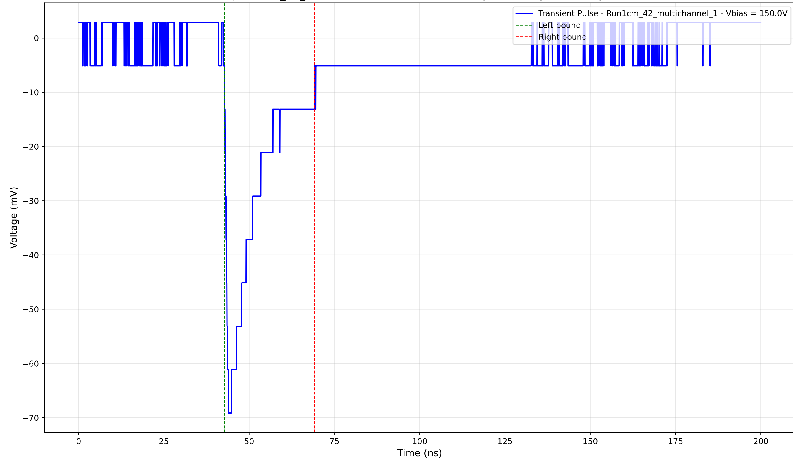
Transient Pulse - Sample: 1cm_42_multichannel - Position: 3600.0 \mu\text{m} - Charge: -14.30 pC - Rise Time: 1.18 ns
