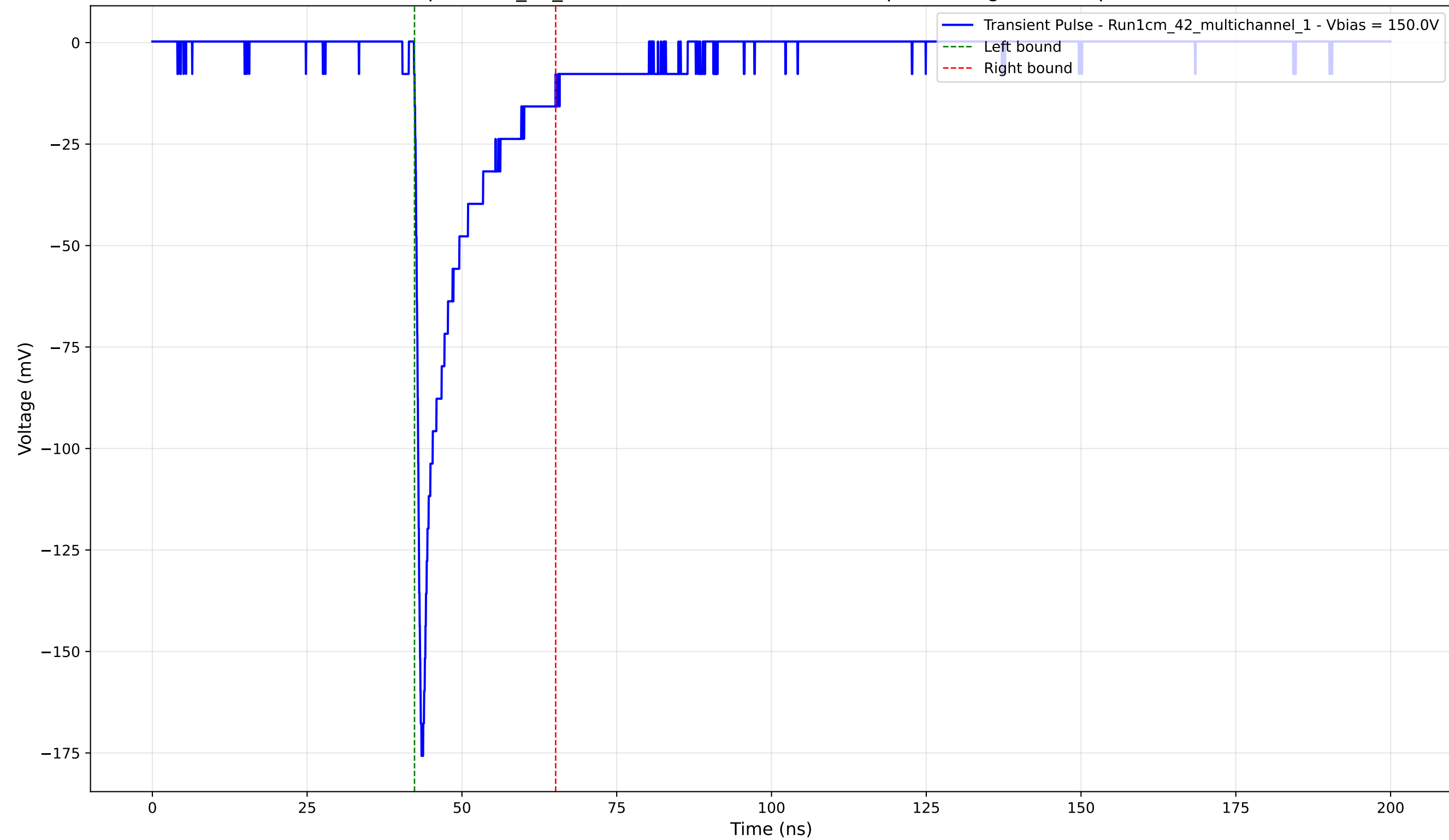
Transient Pulse - Sample: 1cm_42_multichannel - Position: 1790.0 \mu\text{m} - Charge: -21.69 pC - Rise Time: 0.86 ns
