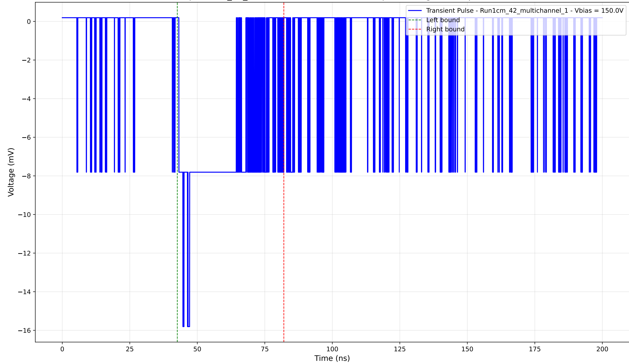
Transient Pulse - Sample: 1cm_42_multichannel - Position: 330.0 \mu\text{m} - Charge: -4.81 pC - Rise Time: 1.50 ns
