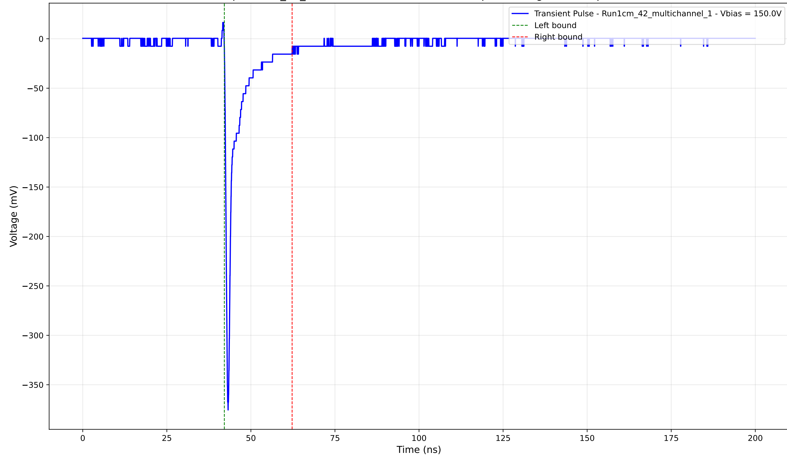
Transient Pulse - Sample: 1cm_42_multichannel - Position: 2540.0 \mu\text{m} - Charge: -24.06 pC - Rise Time: 0.76 ns
