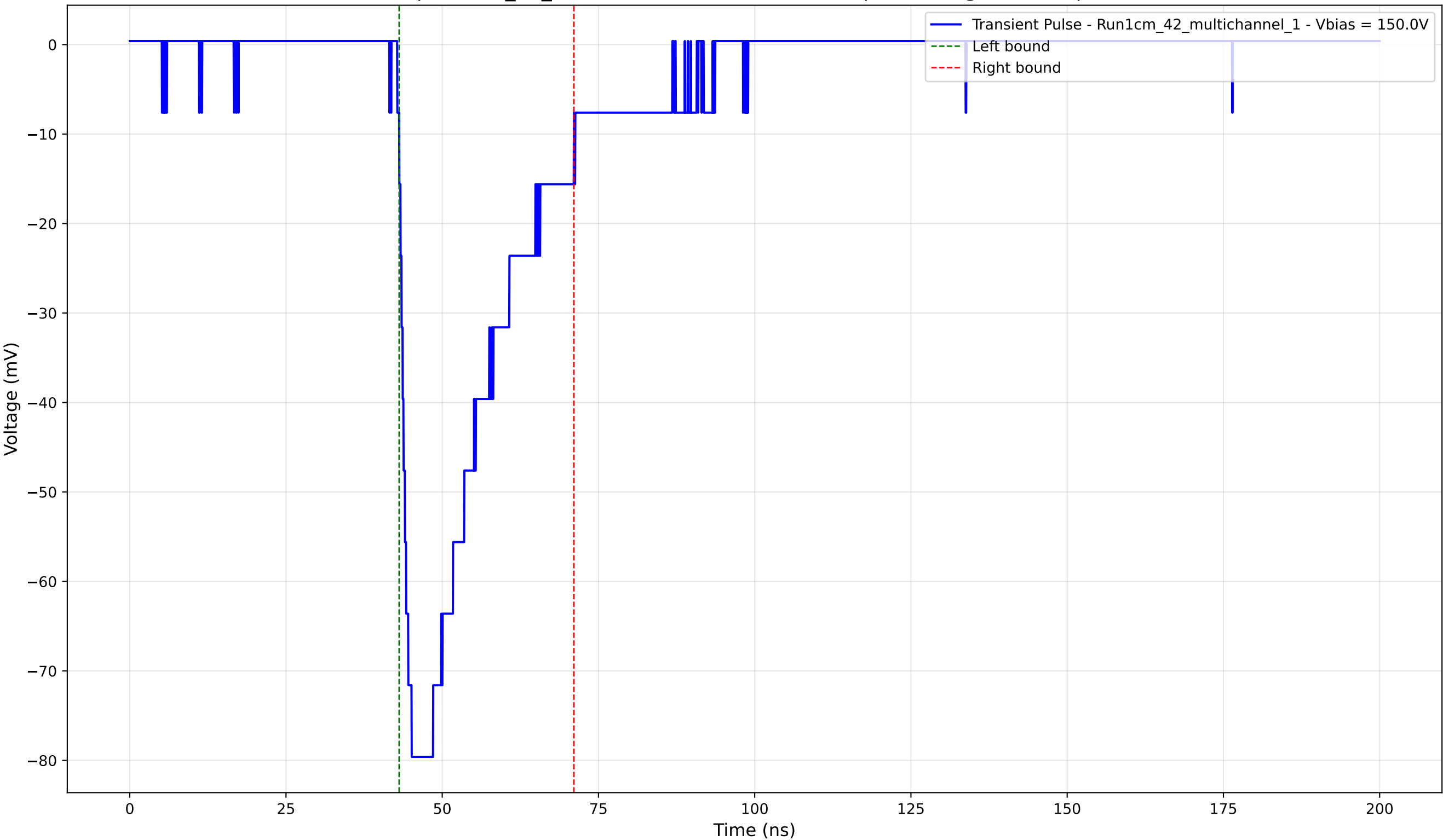
Transient Pulse - Sample: 1cm_42_multichannel - Position: 685.0 \mu\text{m} - Charge: -23.26 pC - Rise Time: 2.00 ns
