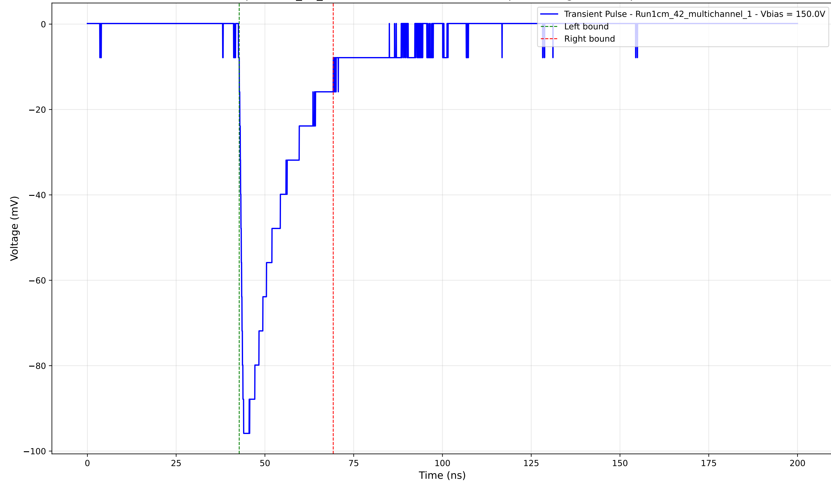
Transient Pulse - Sample: 1cm_42_multichannel - Position: 1200.0 \mu\text{m} - Charge: -23.27 pC - Rise Time: 1.04 ns
