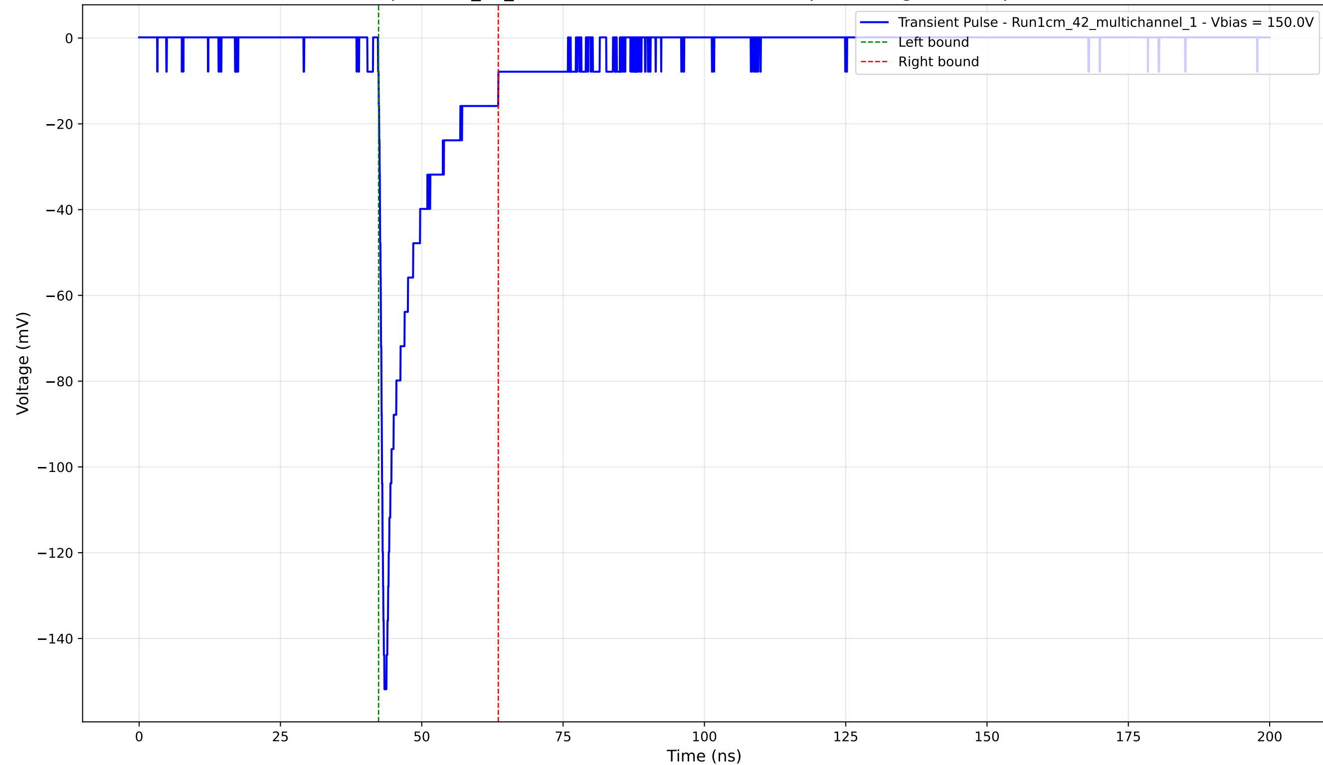
Transient Pulse - Sample: 1cm_42_multichannel - Position: 1810.0 \mu\text{m} - Charge: -18.15 pC - Rise Time: 0.90 ns
