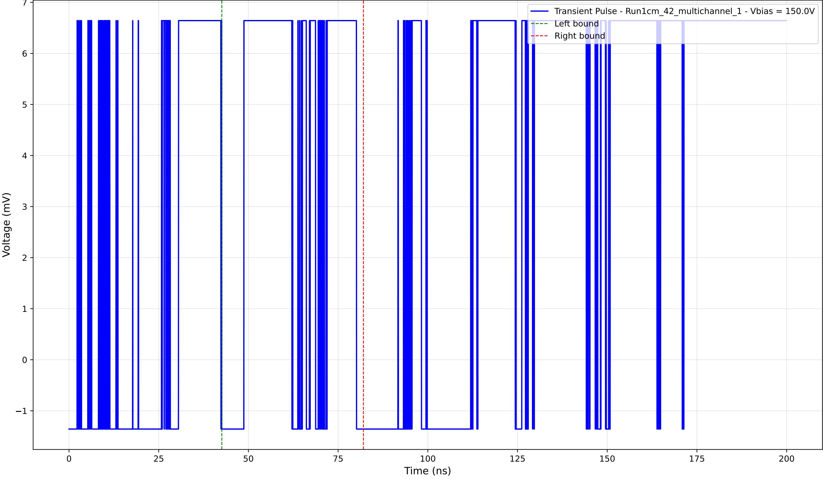
Transient Pulse - Sample: 1cm_42_multichannel - Position: 3880.0 \mu\text{m} - Charge: 3.07 pC - Rise Time: 0.00 ns (N/A)
