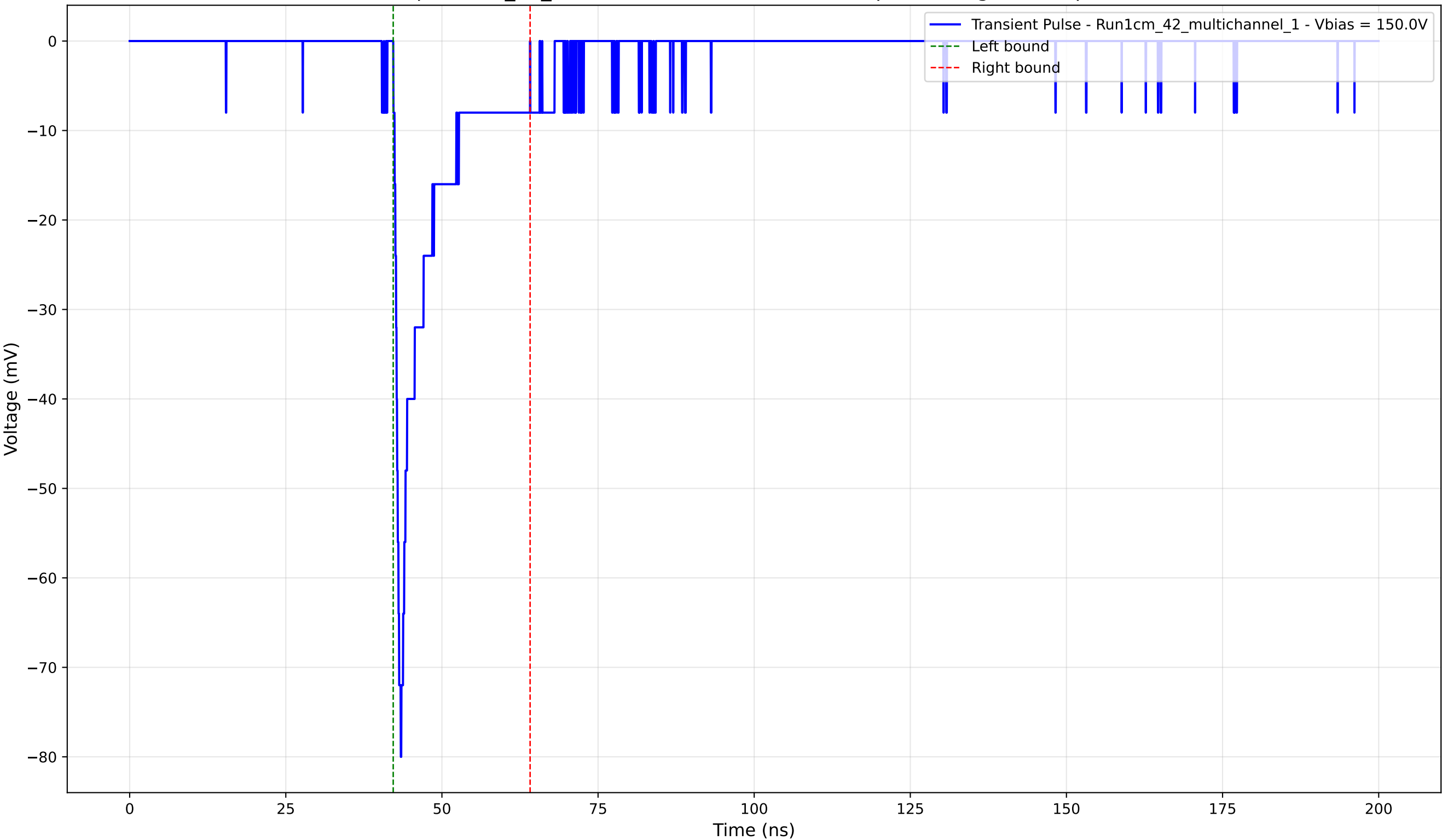
Transient Pulse - Sample: 1cm_42_multichannel - Position: 1925.0 \mu\text{m} - Charge: -7.97 pC - Rise Time: 0.74 ns
