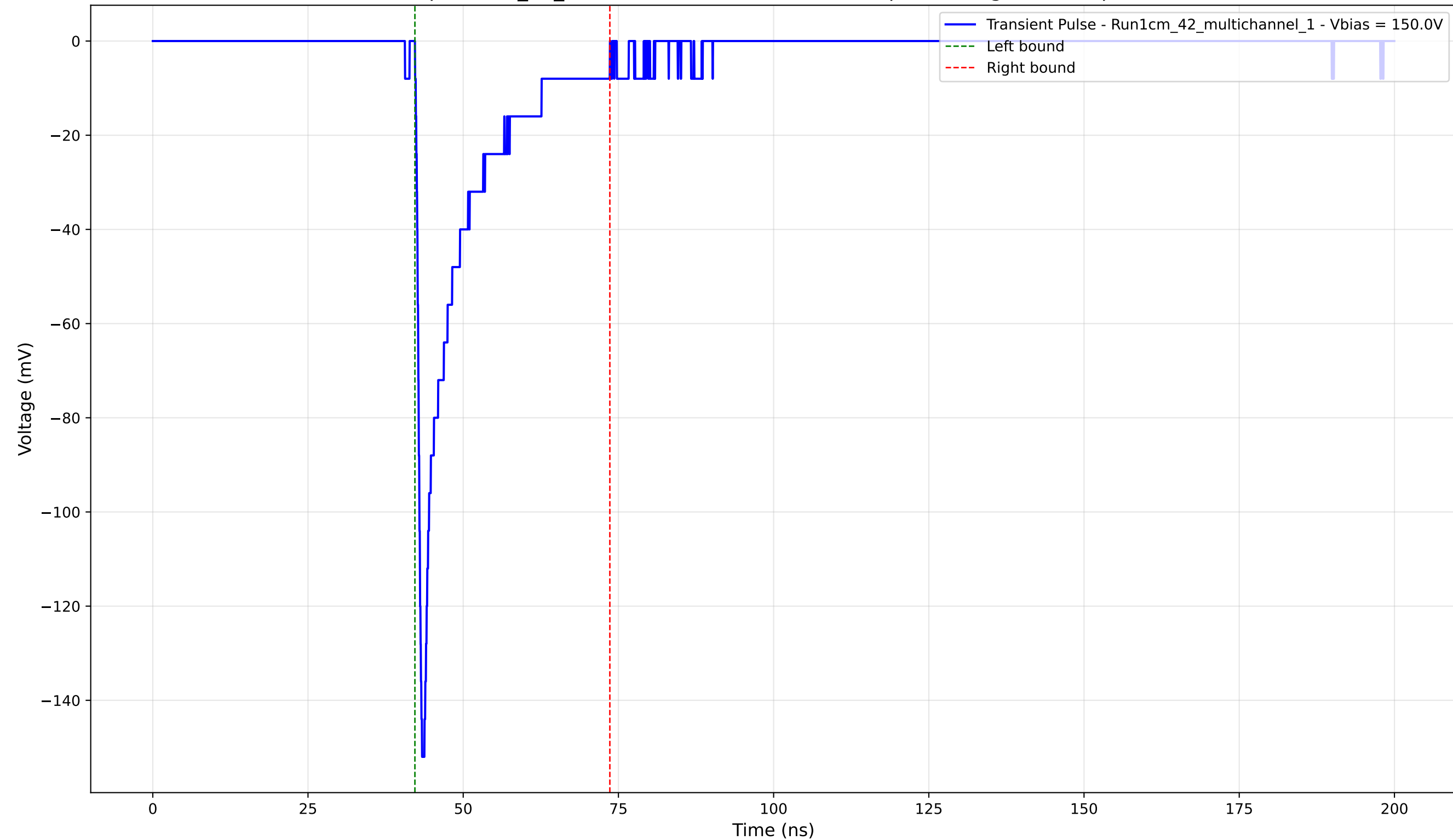
Transient Pulse - Sample: 1cm_42_multichannel - Position: 2965.0 \mu\text{m} - Charge: -19.34 pC - Rise Time: 0.90 ns
