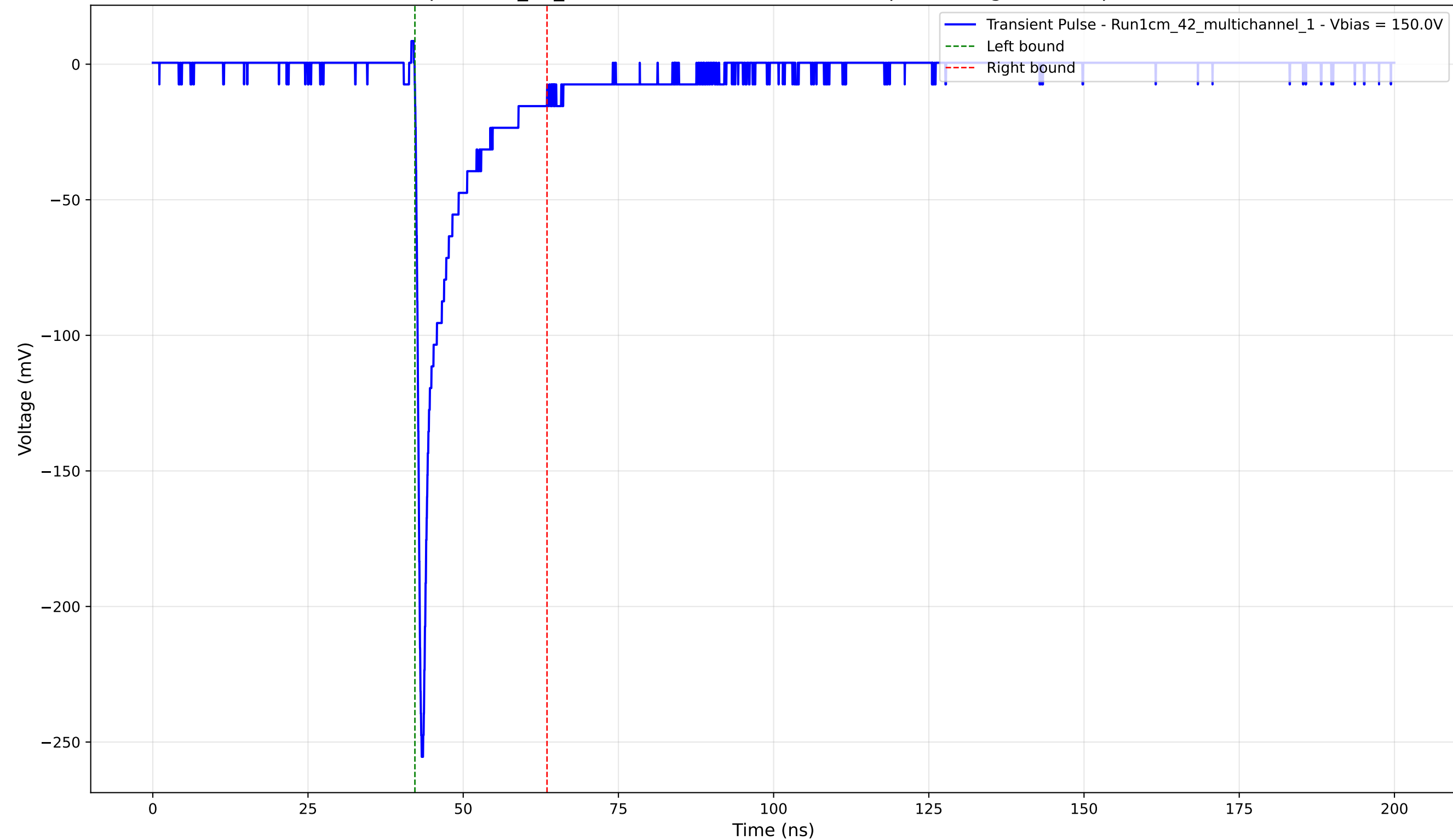
Transient Pulse - Sample: 1cm_42_multichannel - Position: 2000.0 \mu\text{m} - Charge: -23.13 pC - Rise Time: 0.77 ns
