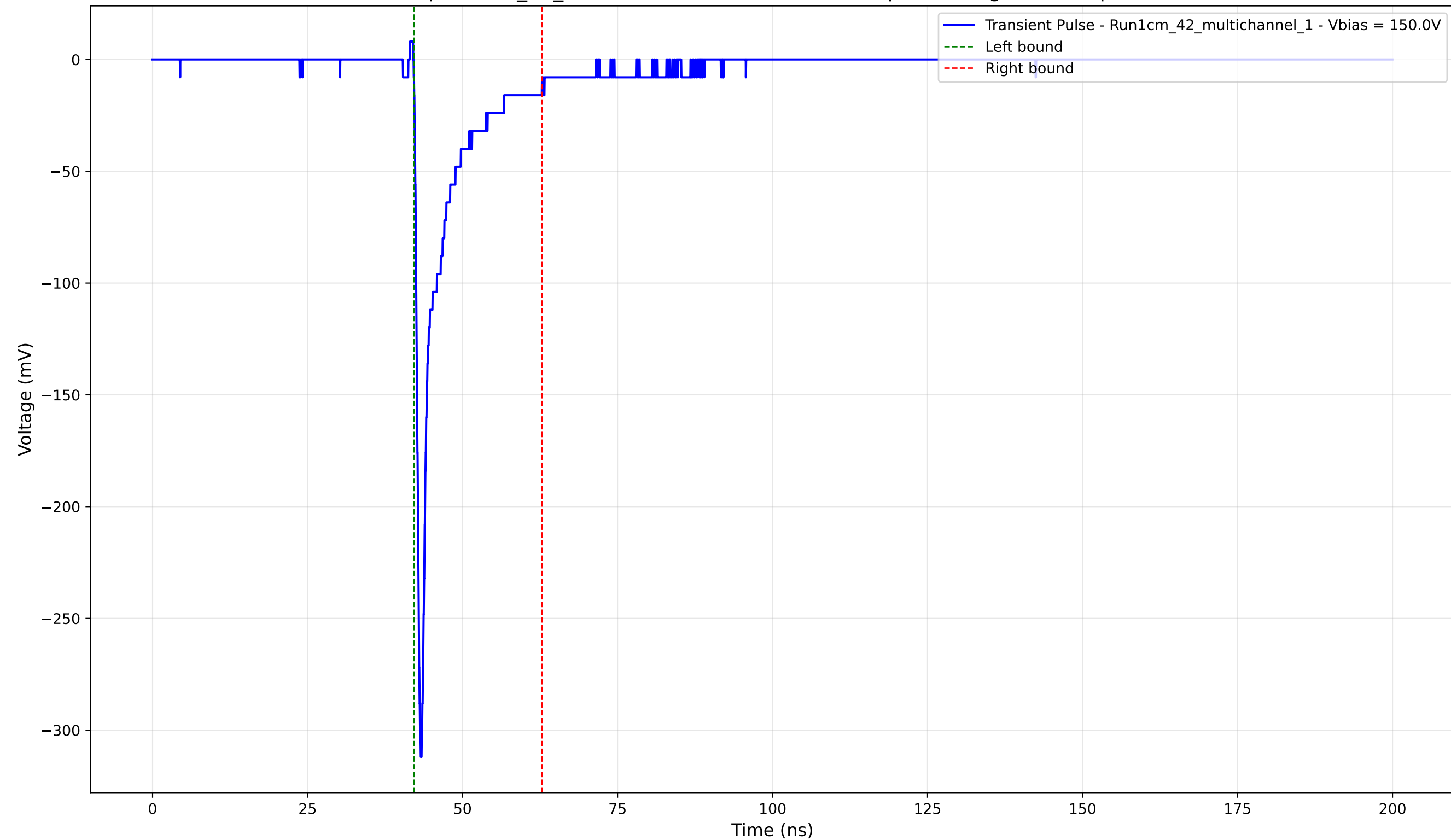
Transient Pulse - Sample: 1cm_42_multichannel - Position: 2115.0 \mu\text{m} - Charge: -23.46 pC - Rise Time: 0.80 ns
