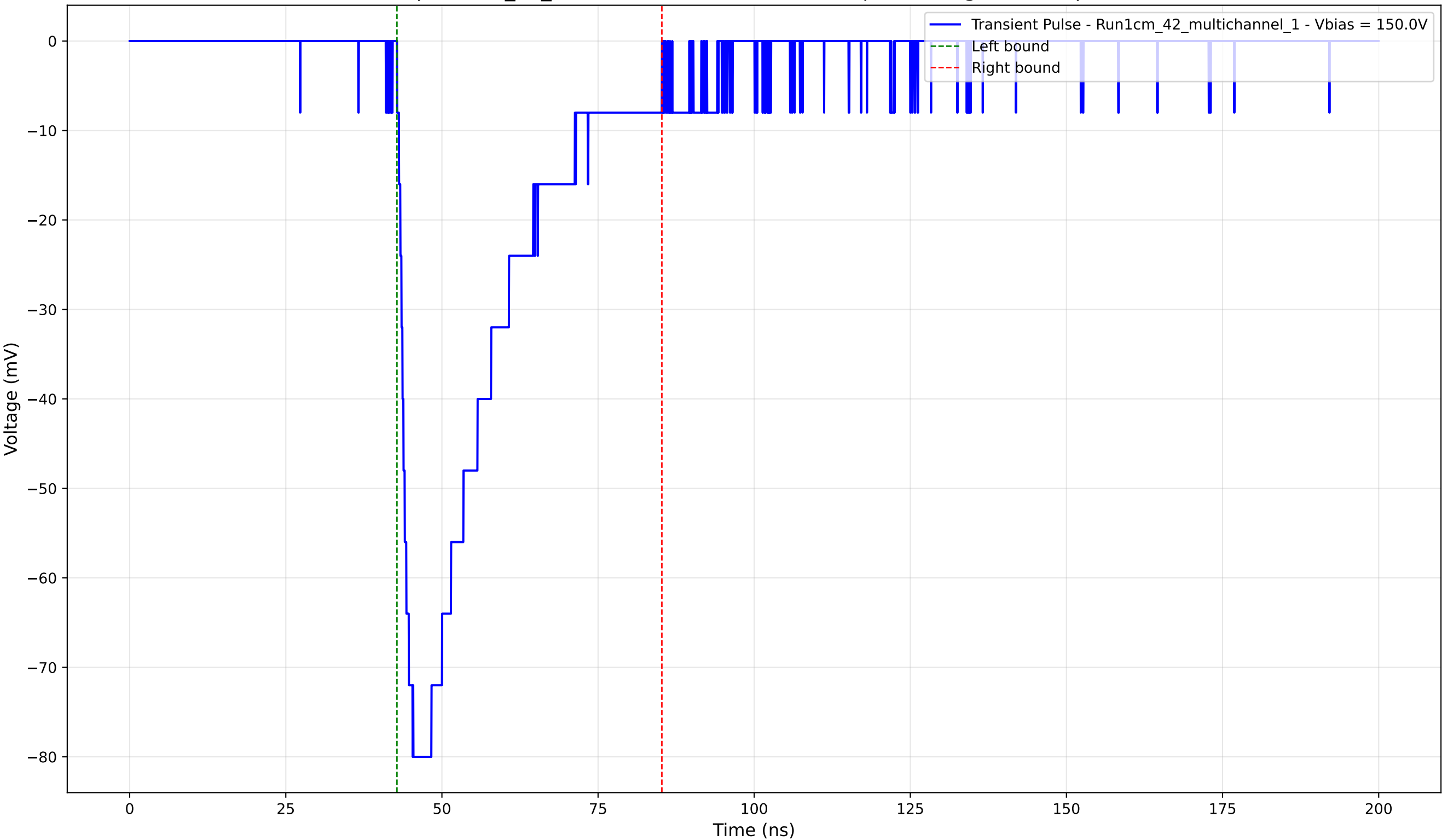
Transient Pulse - Sample: 1cm_42_multichannel - Position: 645.0 \mu\text{m} - Charge: -25.64 pC - Rise Time: 1.60 ns
