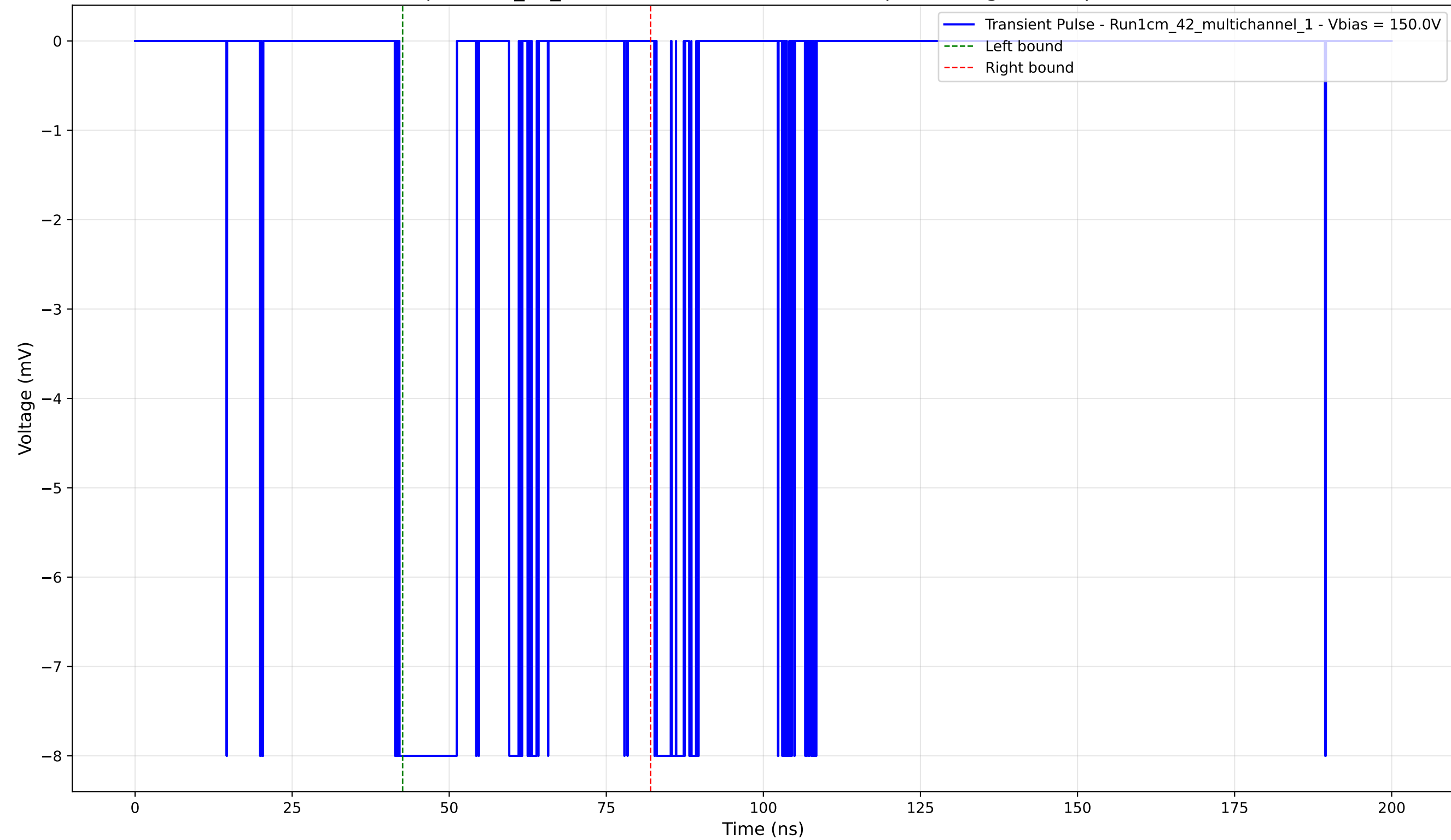
Transient Pulse - Sample: 1cm_42_multichannel - Position: 3425.0 \mu\text{m} - Charge: -1.92 pC - Rise Time: 0.02 ns
