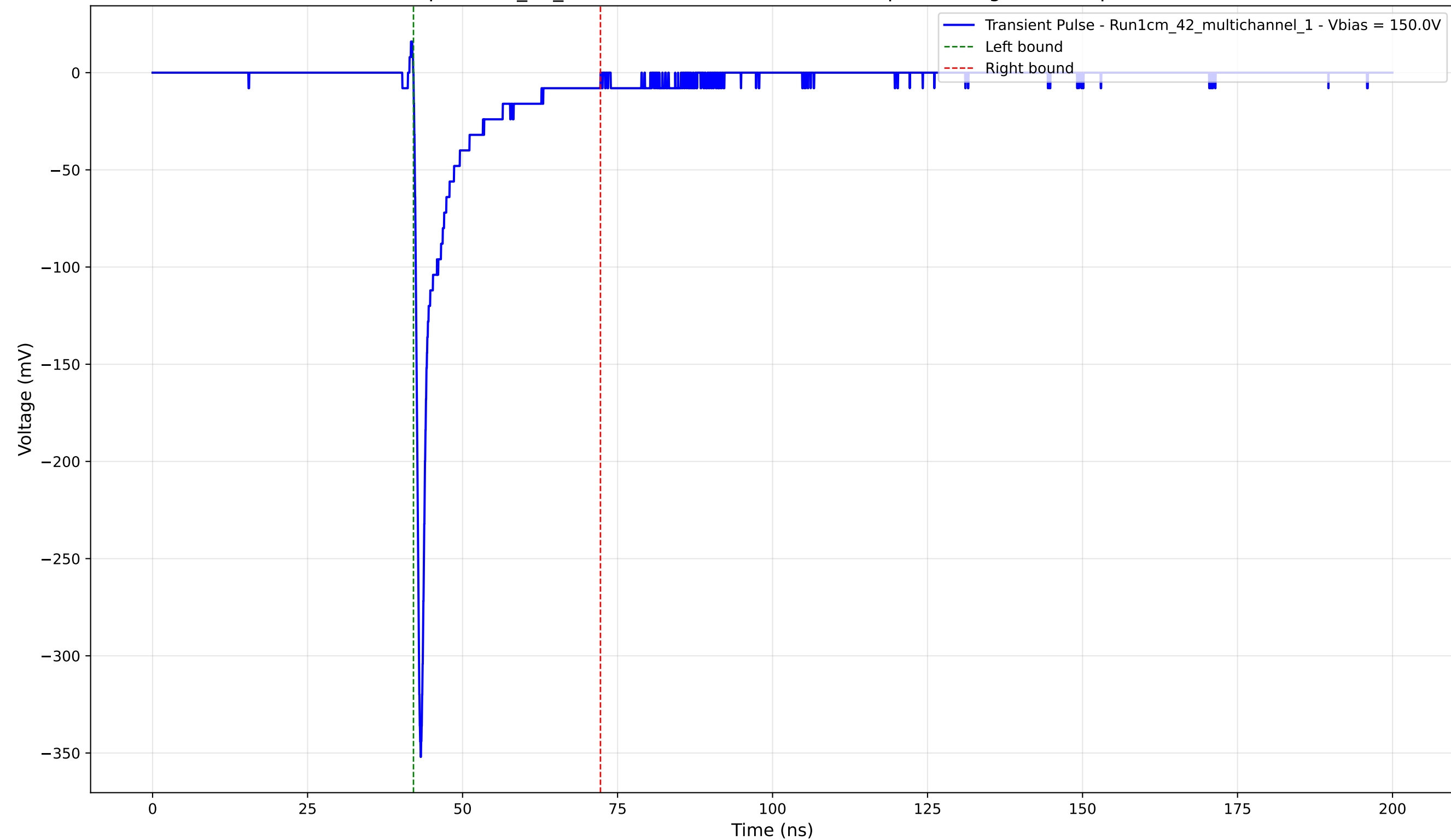
Transient Pulse - Sample: 1cm_42_multichannel - Position: 2185.0 \mu\text{m} - Charge: -25.84 pC - Rise Time: 0.77 ns
