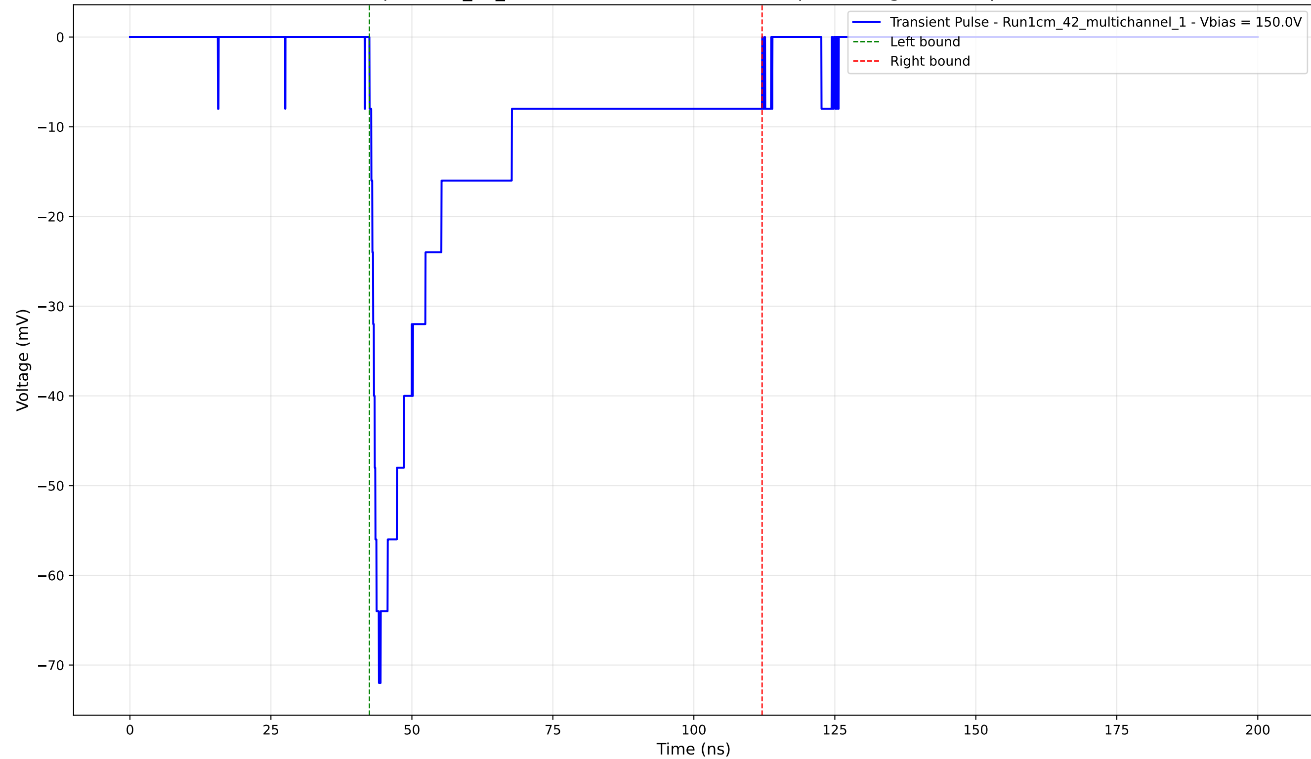
Transient Pulse - Sample: 1cm_42_multichannel - Position: 3610.0 \mu\text{m} - Charge: -21.48 pC - Rise Time: 1.66 ns
