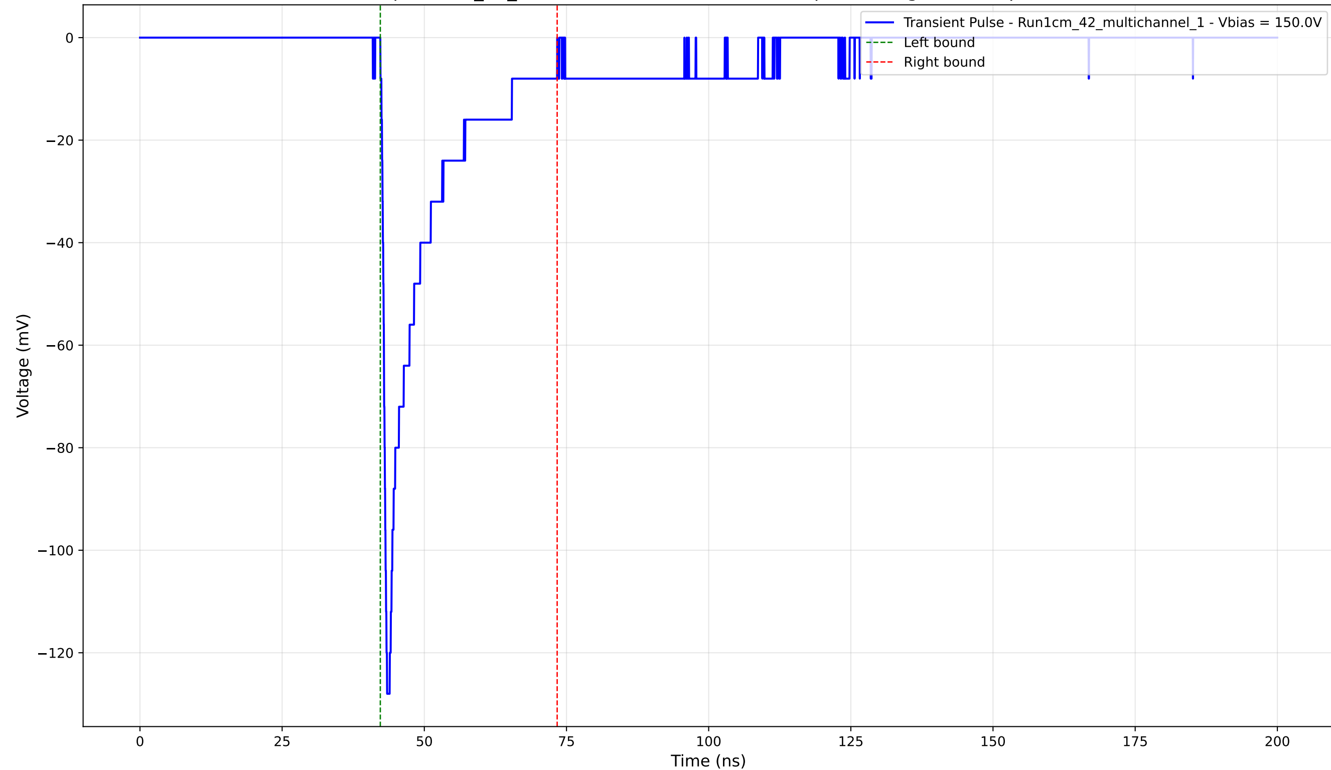
Transient Pulse - Sample: 1cm_42_multichannel - Position: 3125.0 \mu\text{m} - Charge: -18.68 pC - Rise Time: 0.89 ns
