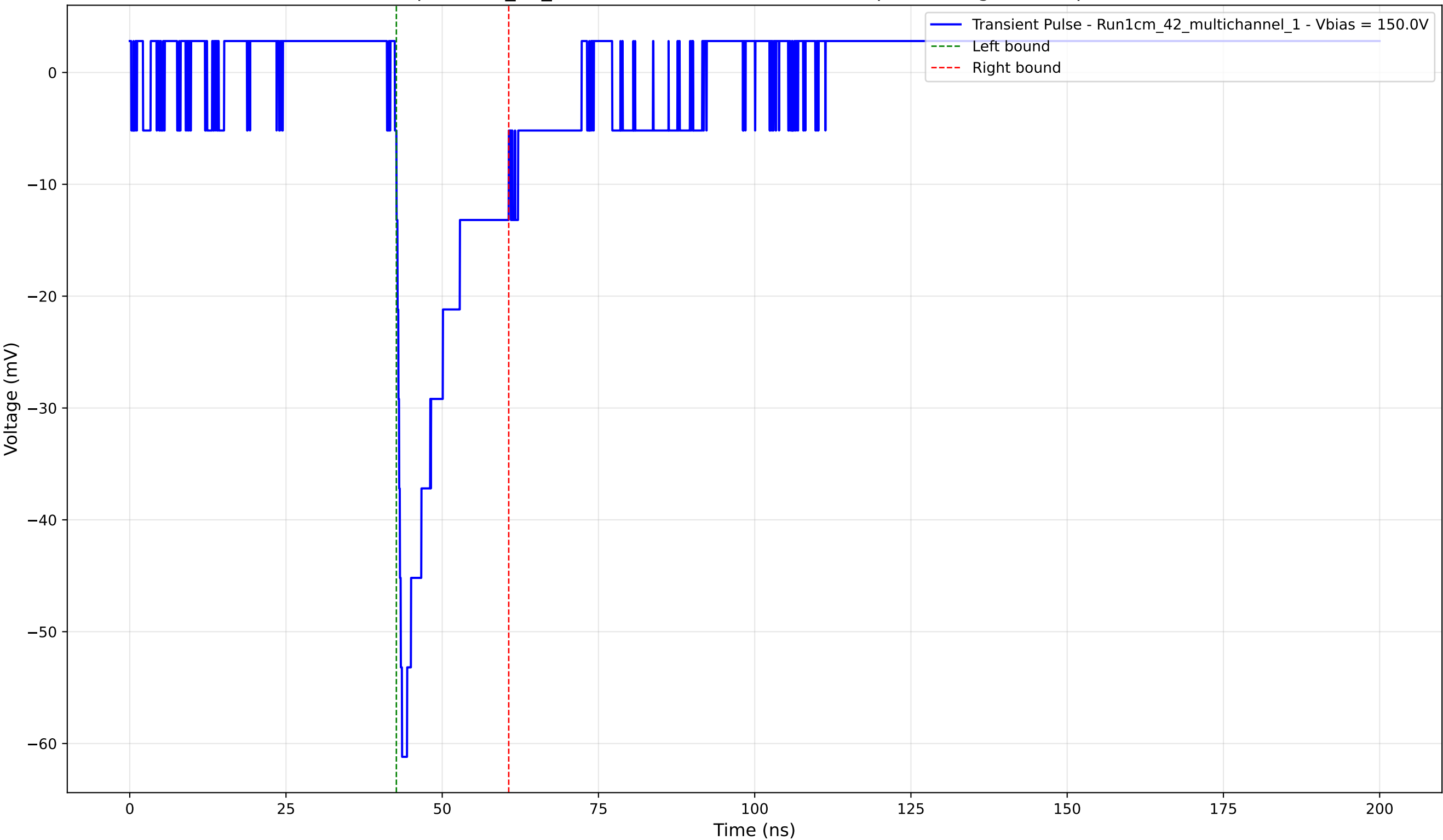
Transient Pulse - Sample: 1cm_42_multichannel - Position: 3340.0 \mu\text{m} - Charge: -9.23 pC - Rise Time: 0.90 ns
