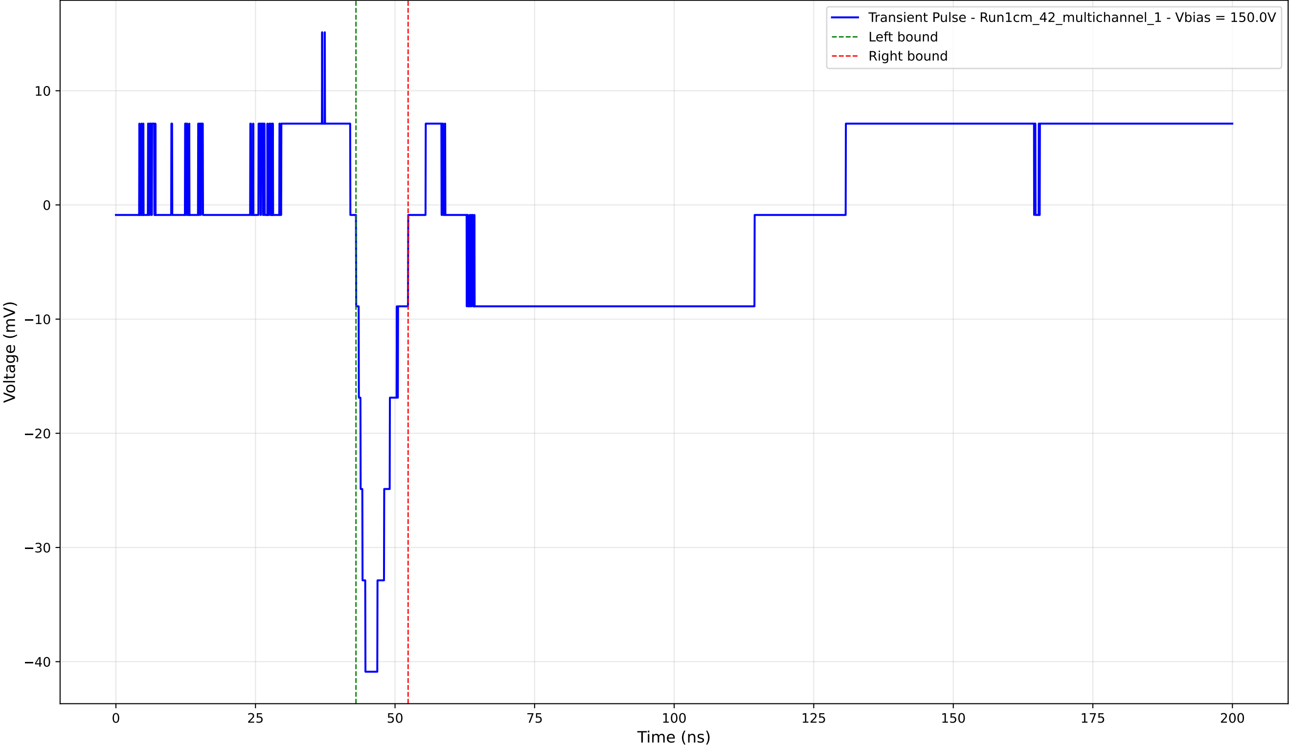
Transient Pulse - Sample: 1cm_42_multichannel - Position: 4585.0 \mu\text{m} - Charge: -4.57 pC - Rise Time: 1.67 ns
