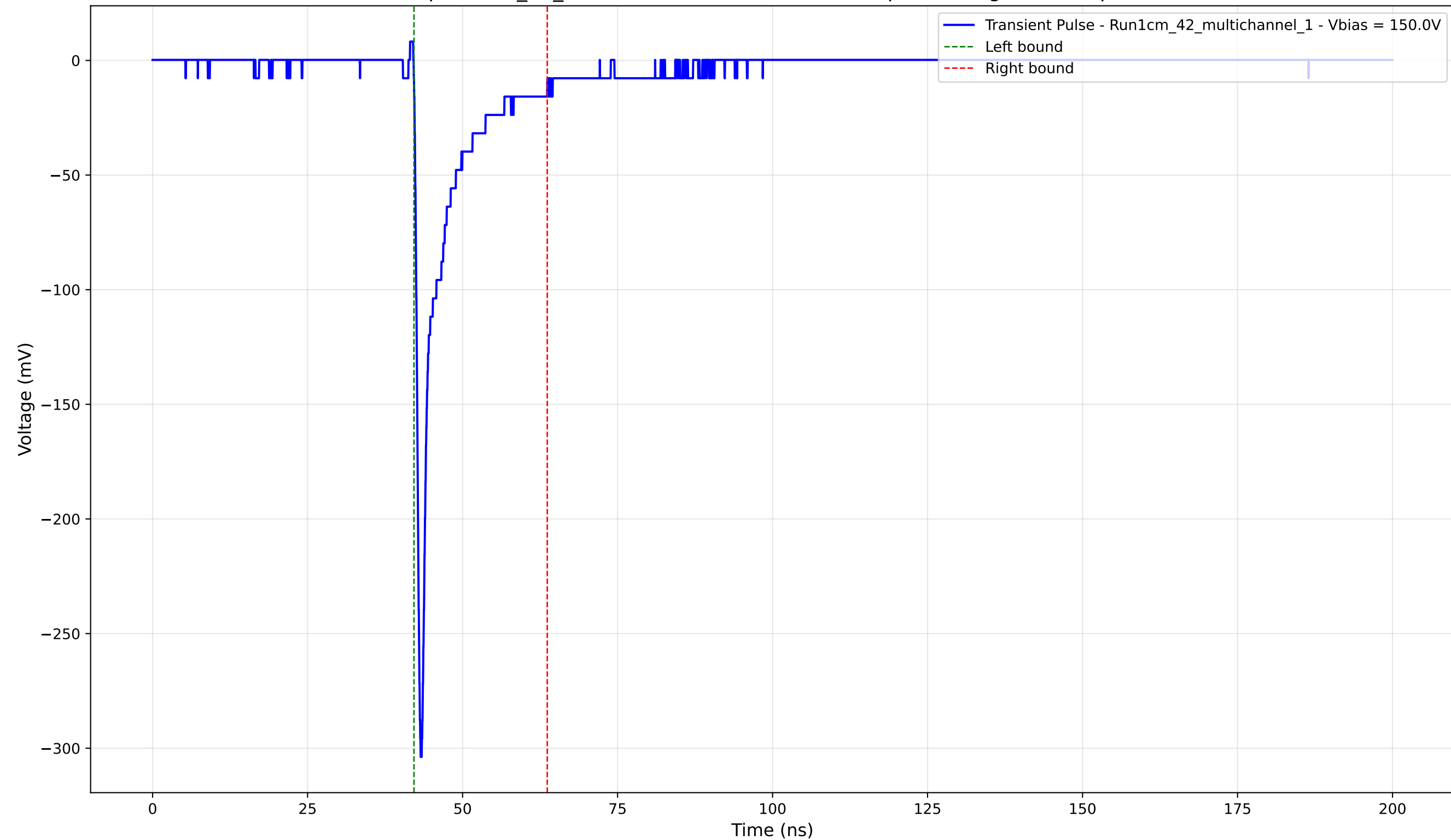
Transient Pulse - Sample: 1cm_42_multichannel - Position: 2100.0 \mu\text{m} - Charge: -23.65 pC - Rise Time: 0.80 ns
