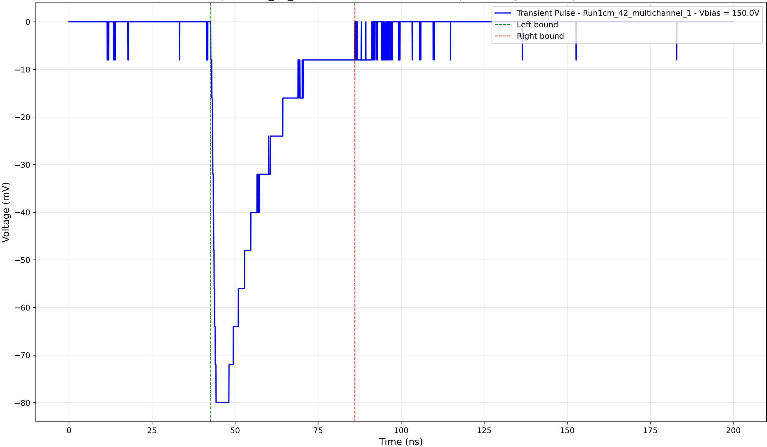
Transient Pulse - Sample: 1cm_42_multichannel - Position: 965.0 \mu\text{m} - Charge: -25.48 pC - Rise Time: 1.02 ns
