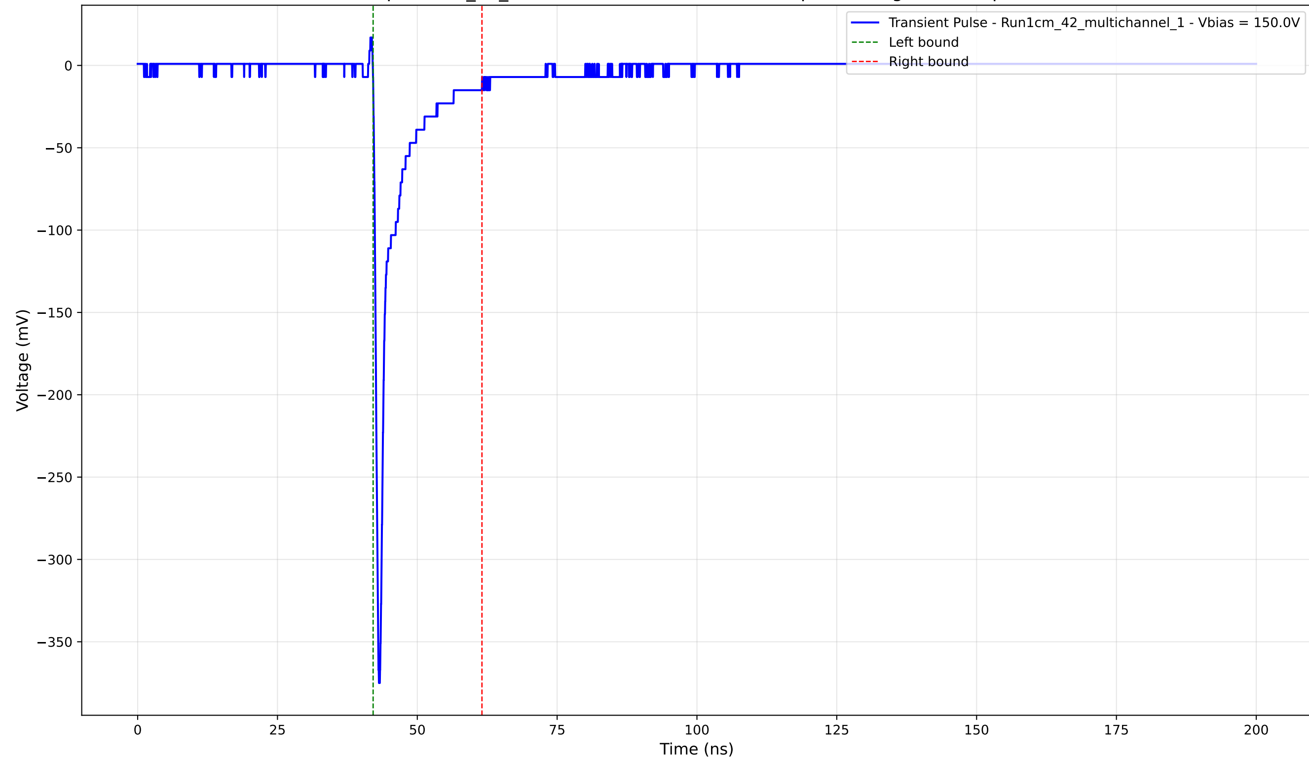
Transient Pulse - Sample: 1cm_42_multichannel - Position: 2225.0 \mu\text{m} - Charge: -24.37 pC - Rise Time: 0.75 ns
