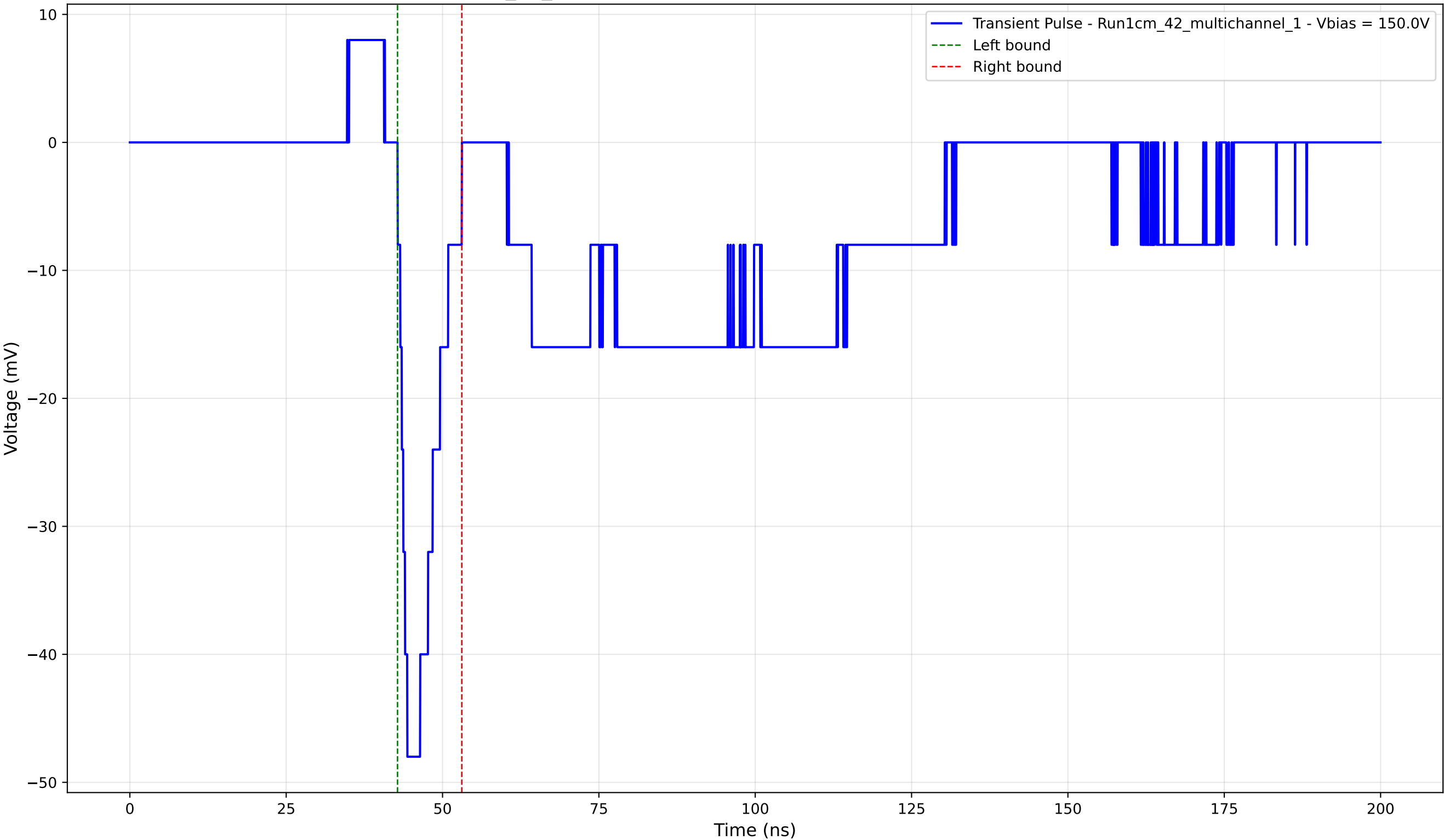
Transient Pulse - Sample: 1cm_42_multichannel - Position: 4060.0 \mu\text{m} - Charge: -5.52 pC - Rise Time: 1.55 ns
