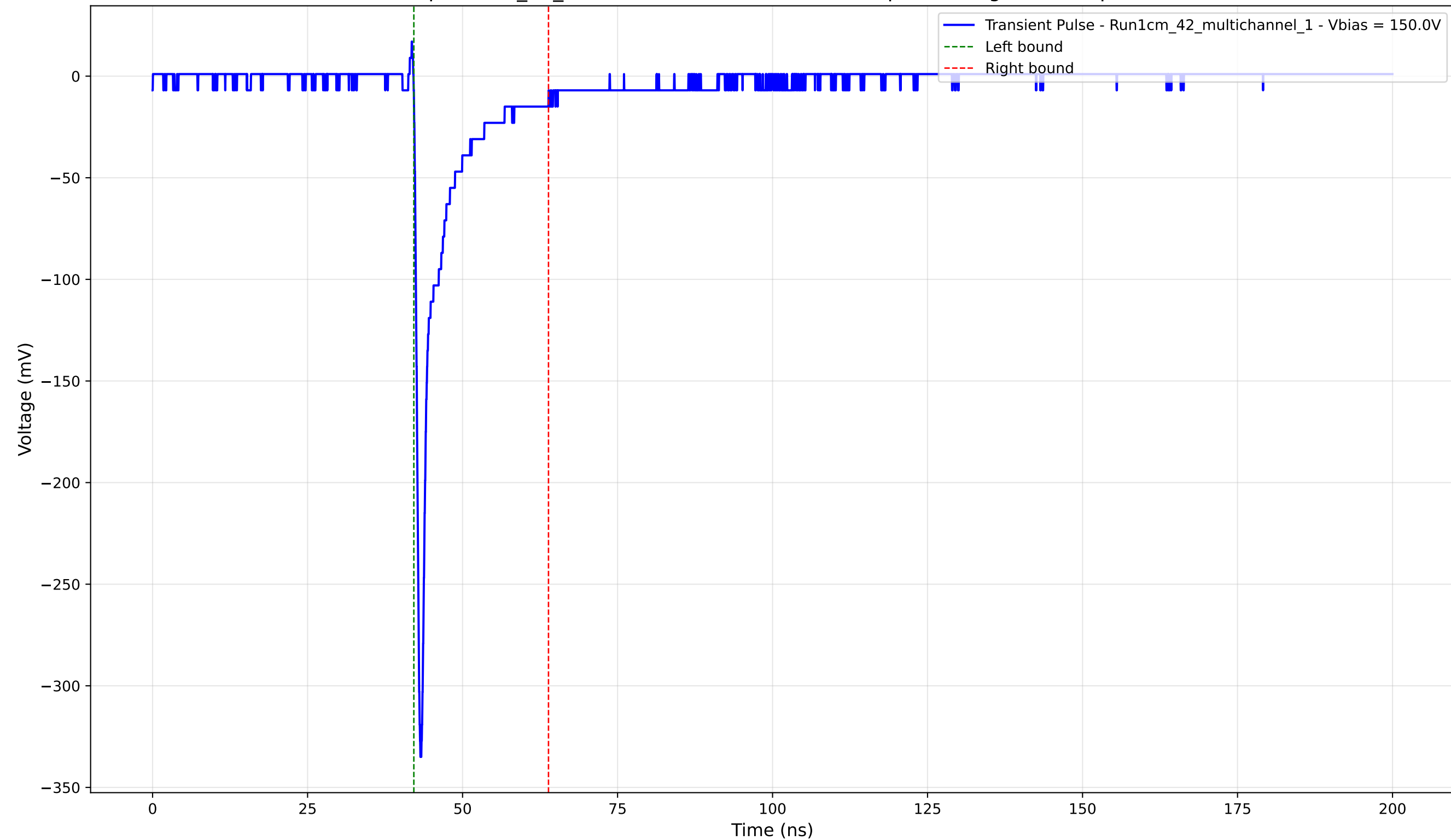
Transient Pulse - Sample: 1cm_42_multichannel - Position: 2160.0 \mu\text{m} - Charge: -24.20 pC - Rise Time: 0.73 ns
