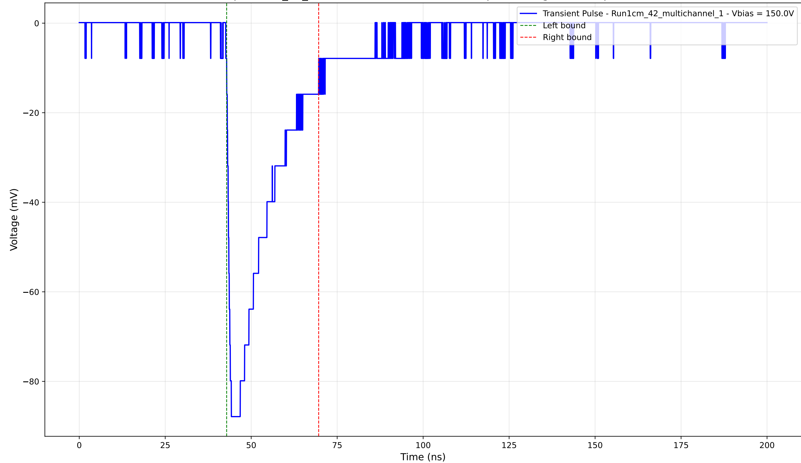
Transient Pulse - Sample: 1cm_42_multichannel - Position: 1090.0 \mu\text{m} - Charge: -23.00 pC - Rise Time: 1.06 ns
