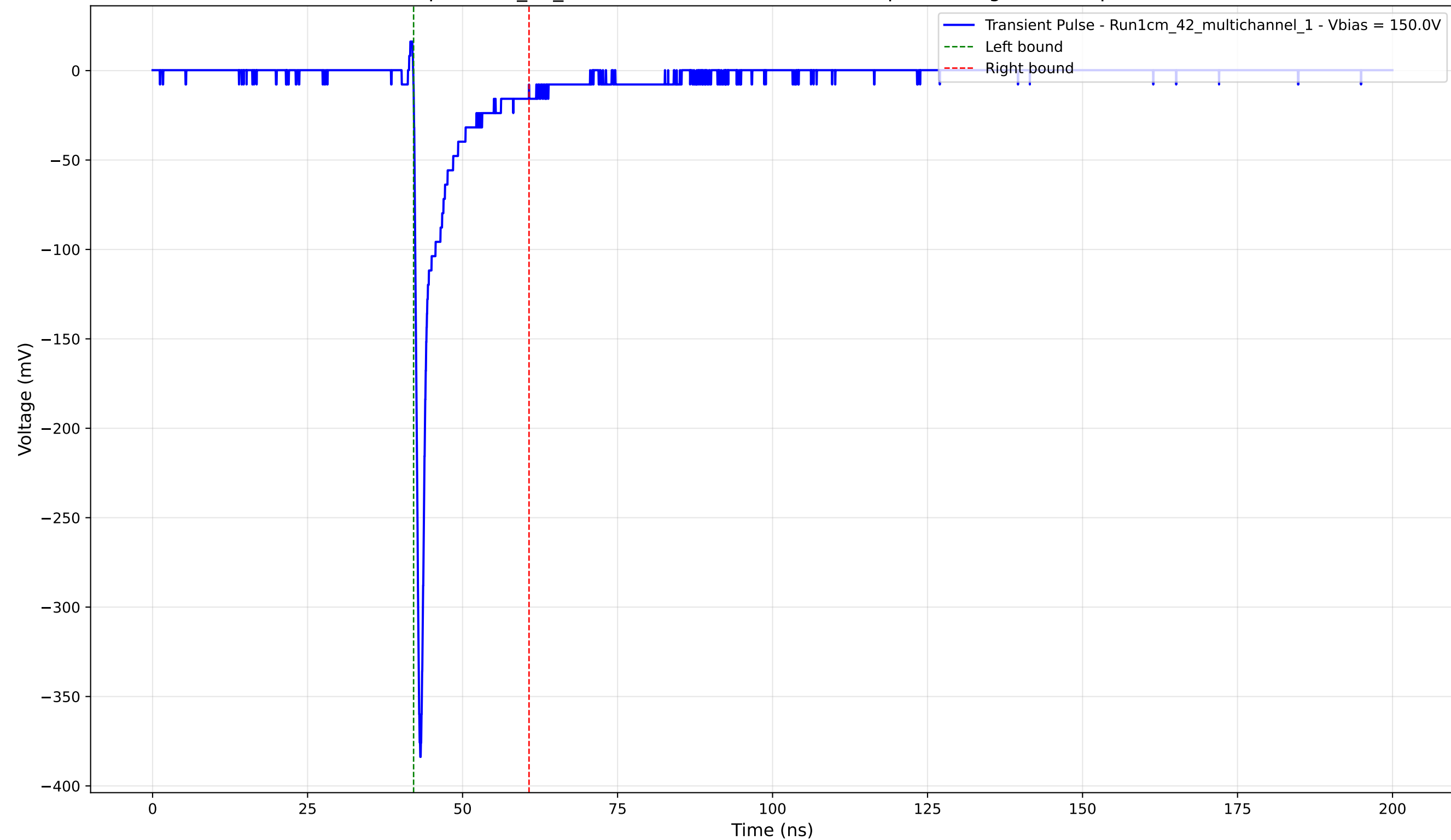
Transient Pulse - Sample: 1cm_42_multichannel - Position: 2525.0 \mu\text{m} - Charge: -23.68 pC - Rise Time: 0.75 ns
