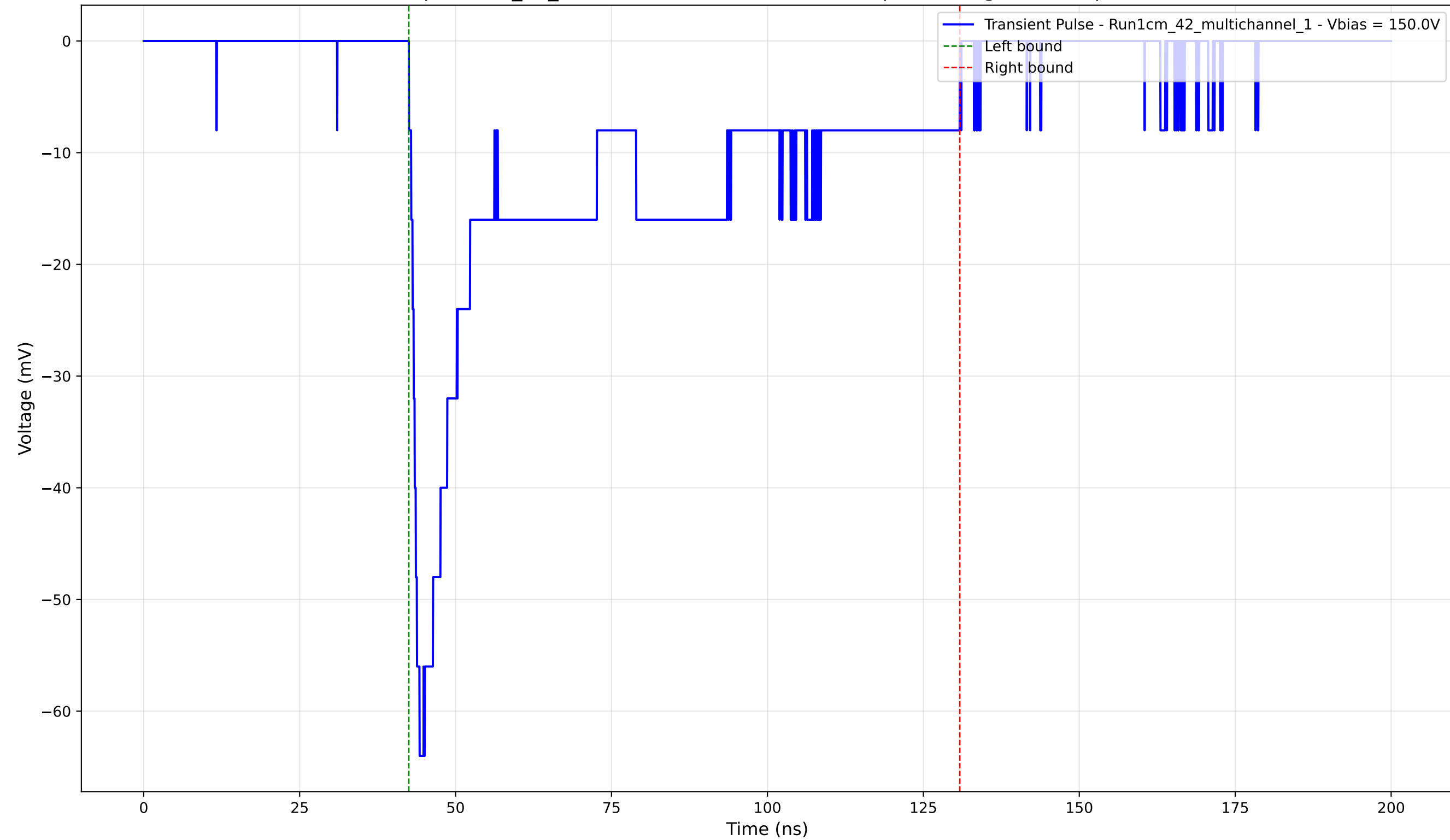
Transient Pulse - Sample: 1cm_42_multichannel - Position: 3755.0 \mu\text{m} - Charge: -26.19 pC - Rise Time: 1.70 ns
