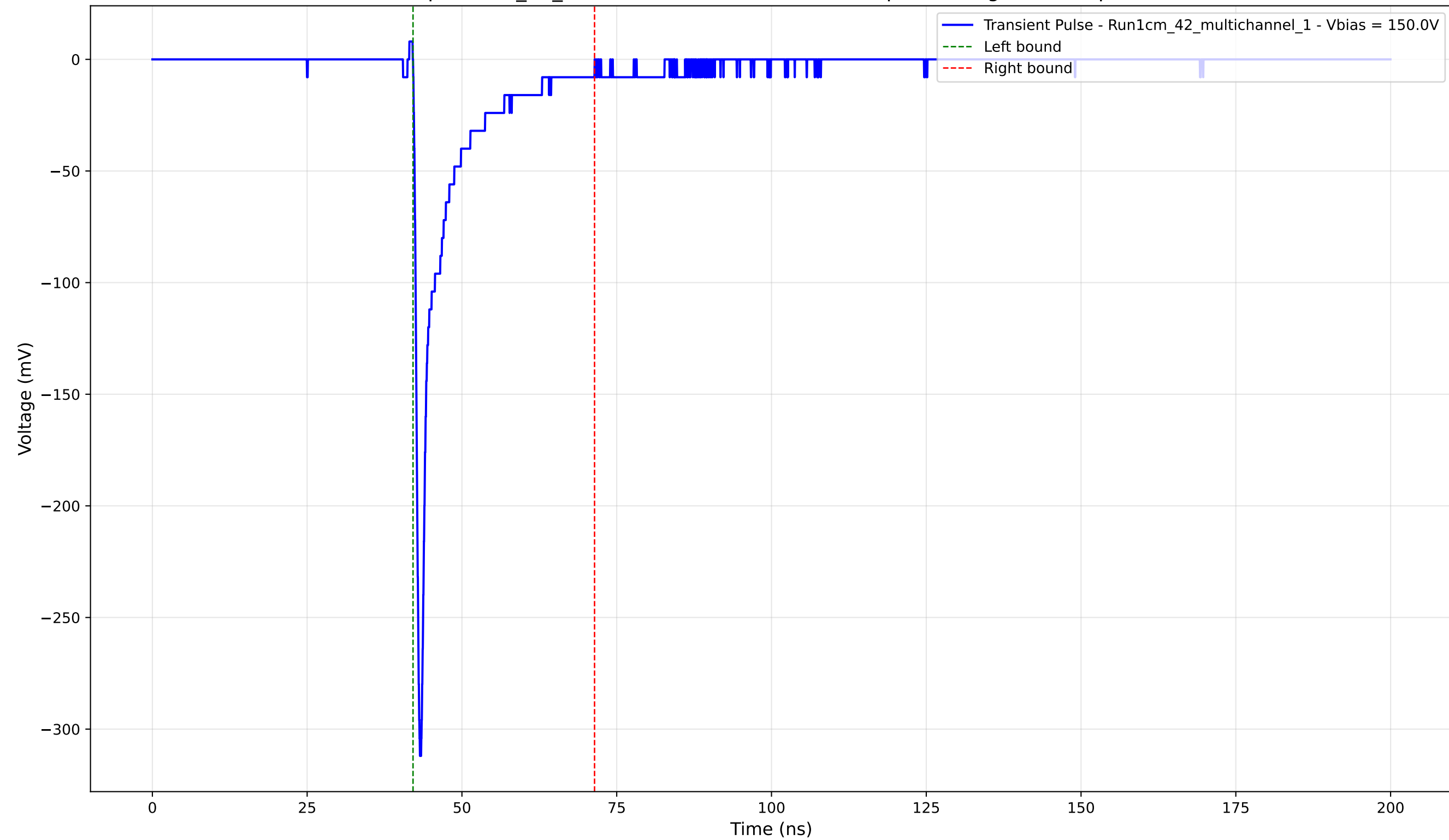
Transient Pulse - Sample: 1cm_42_multichannel - Position: 2120.0 \mu\text{m} - Charge: -24.94 pC - Rise Time: 0.80 ns
