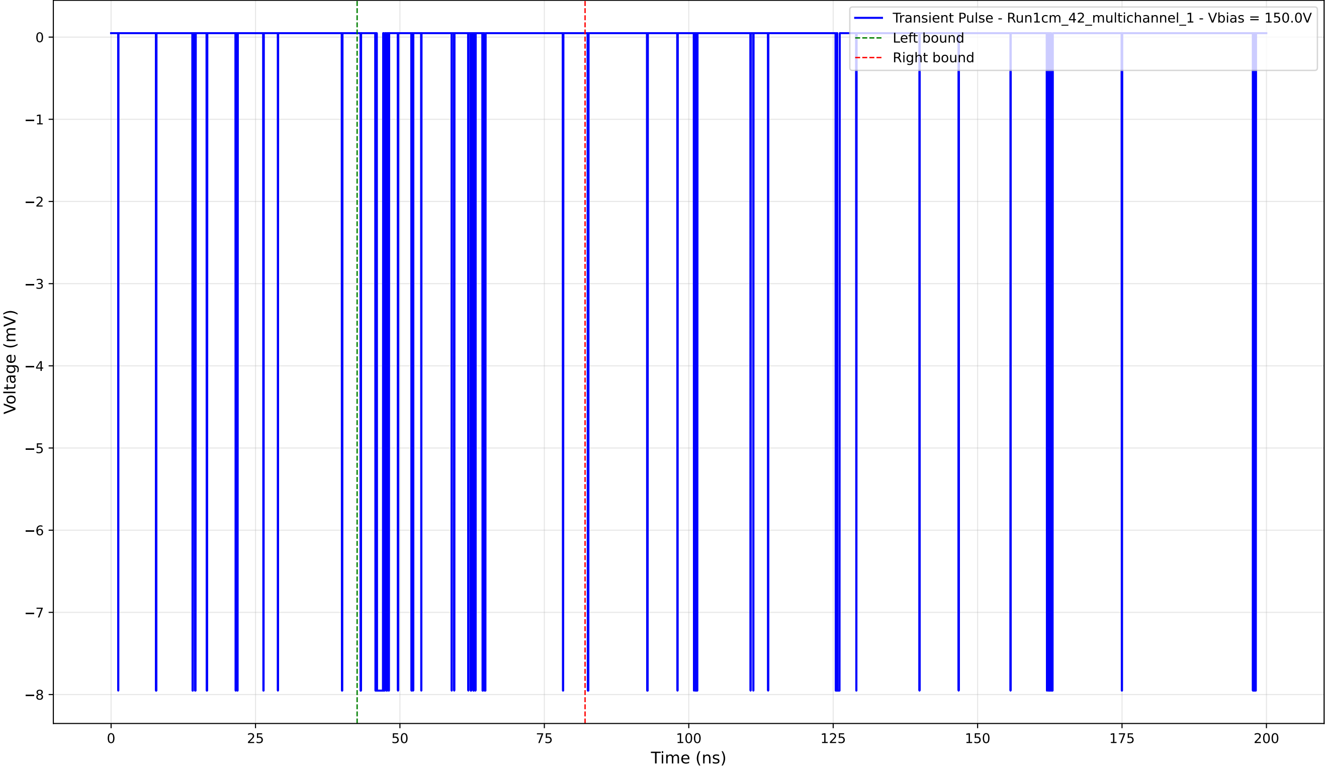
Transient Pulse - Sample: 1cm_42_multichannel - Position: 5.0 \mu\text{m} - Charge: -0.37 pC - Rise Time: 0.02 ns
