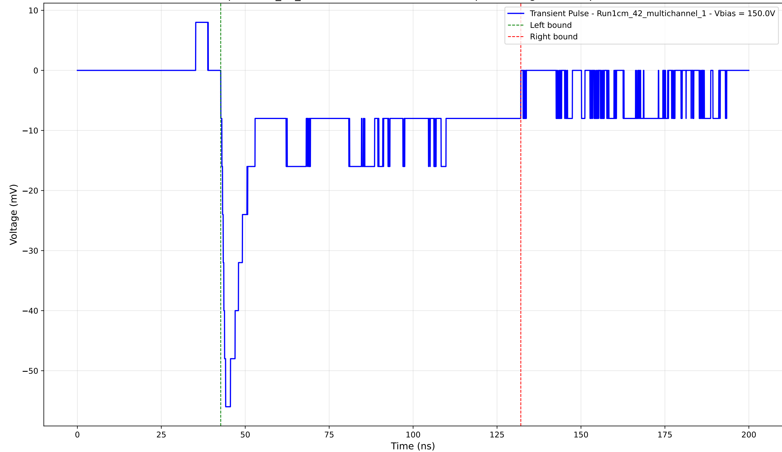
Transient Pulse - Sample: 1cm_42_multichannel - Position: 3815.0 \mu\text{m} - Charge: -22.34 pC - Rise Time: 1.45 ns
