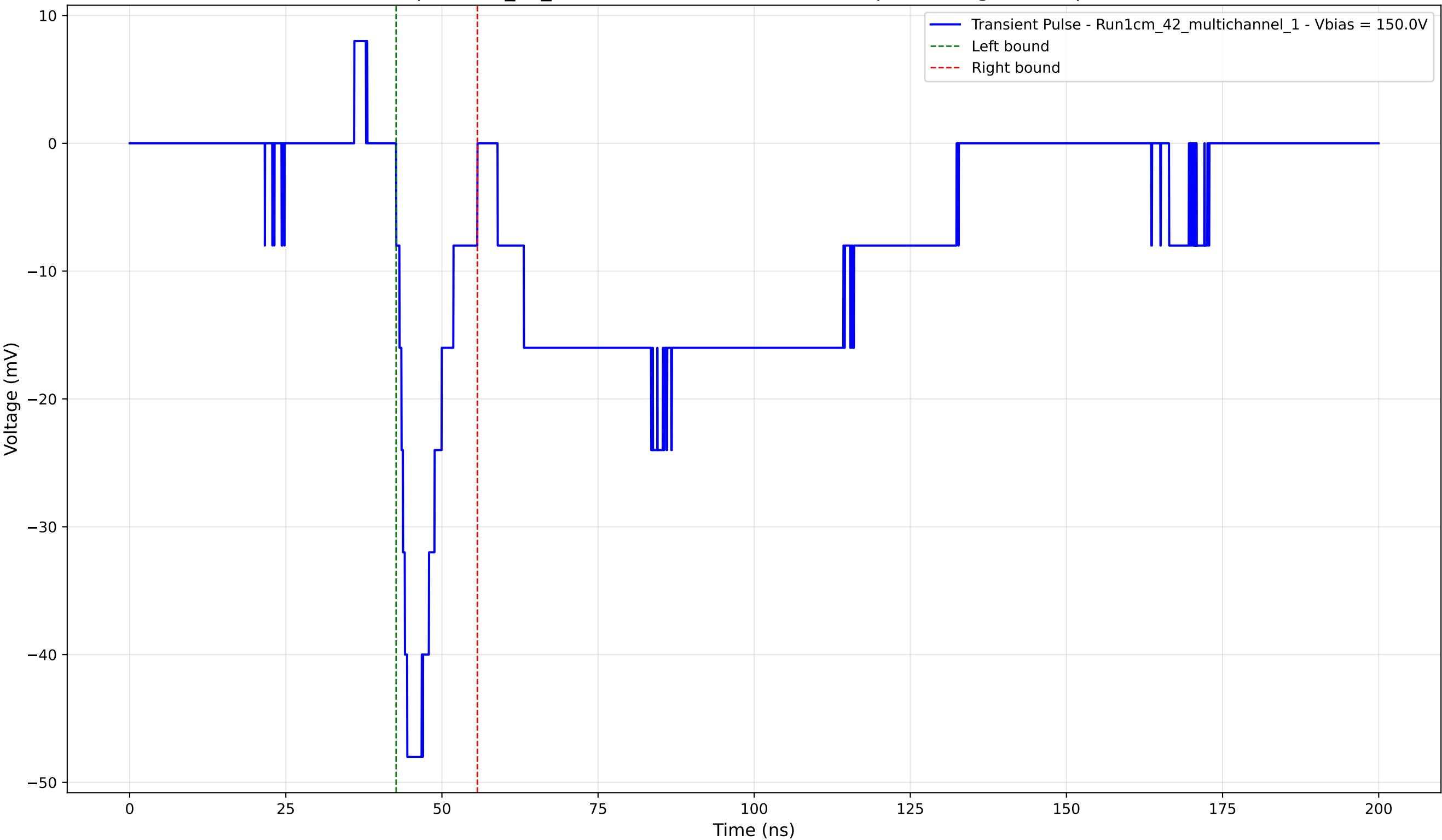
Transient Pulse - Sample: 1cm_42_multichannel - Position: 4220.0 \mu\text{m} - Charge: -6.30 pC - Rise Time: 1.77 ns
