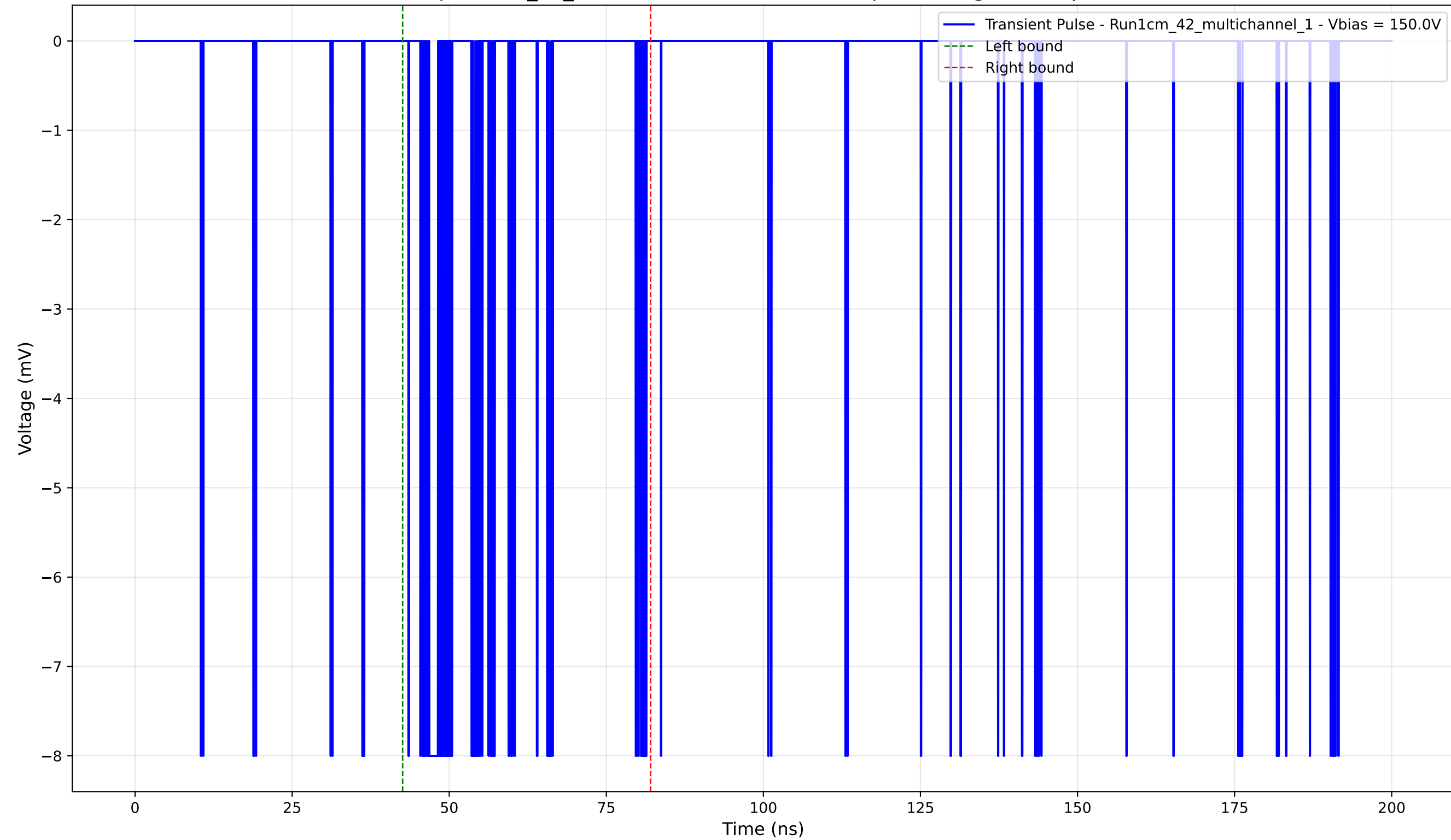
Transient Pulse - Sample: 1cm_42_multichannel - Position: 35.0 \mu\text{m} - Charge: -1.05 pC - Rise Time: 0.02 ns
