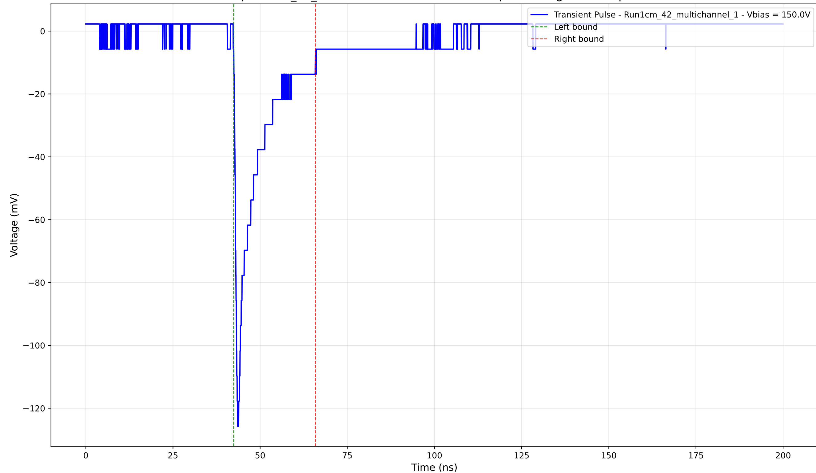
Transient Pulse - Sample: 1cm_42_multichannel - Position: 3135.0 \mu\text{m} - Charge: -16.48 pC - Rise Time: 0.94 ns
