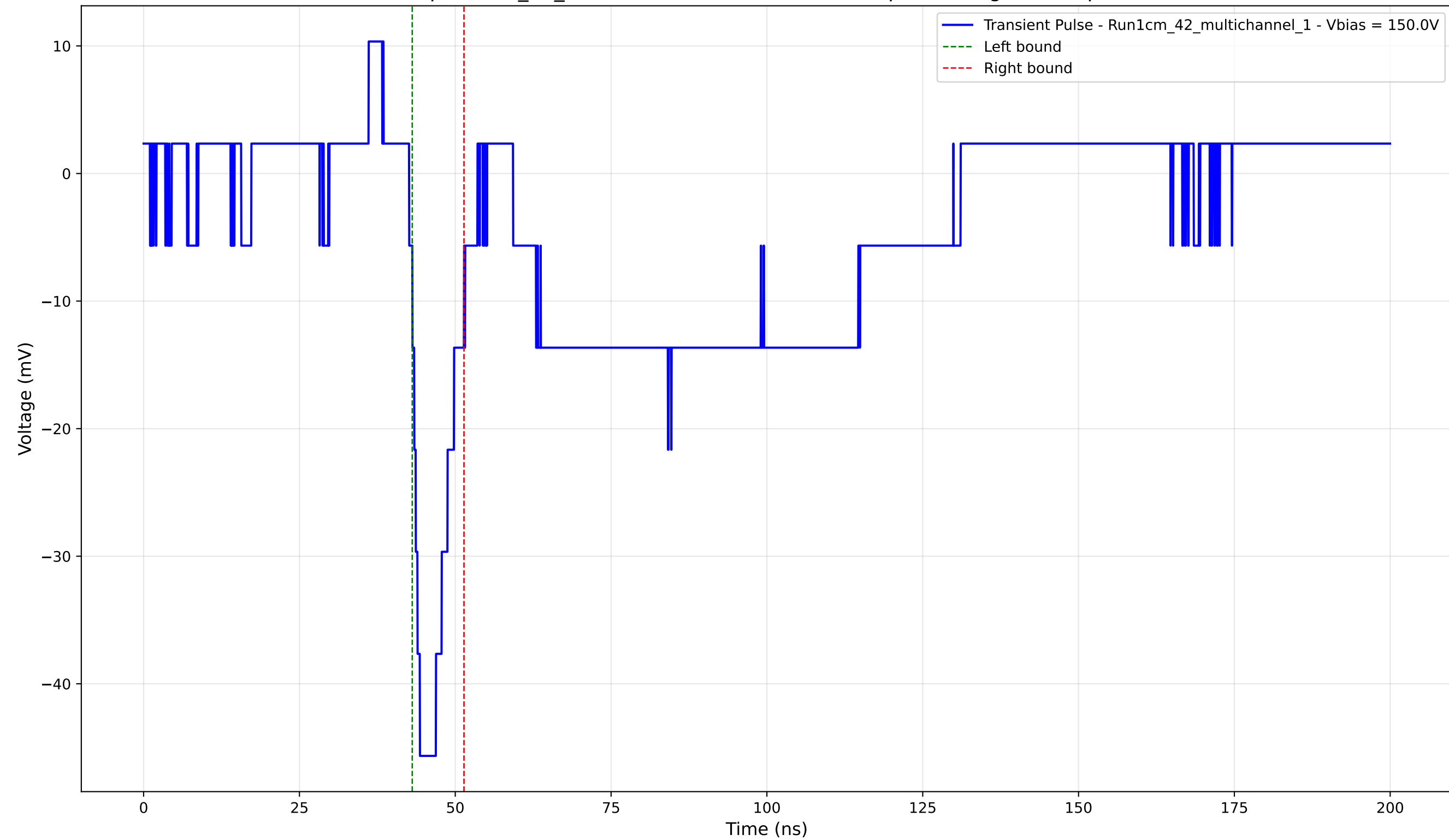
Transient Pulse - Sample: 1cm_42_multichannel - Position: 4085.0 \mu\text{m} - Charge: -5.13 pC - Rise Time: 1.73 ns
