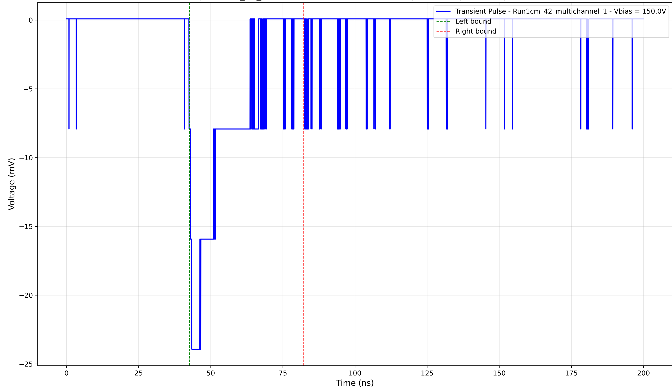
Transient Pulse - Sample: 1cm_42_multichannel - Position: 1410.0 \mu\text{m} - Charge: -5.60 pC - Rise Time: 0.95 ns
