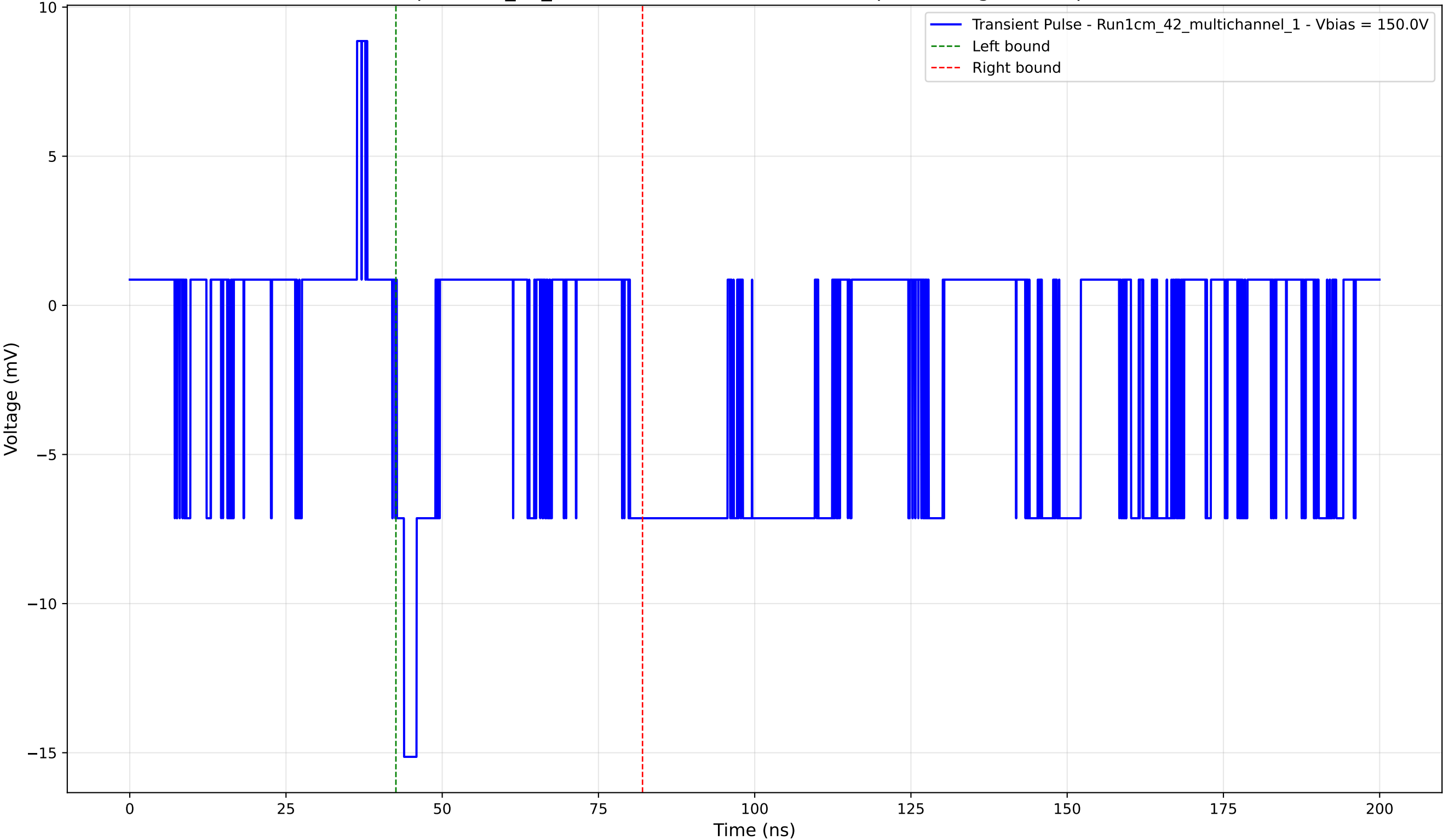
Transient Pulse - Sample: 1cm_42_multichannel - Position: 3870.0 \mu\text{m} - Charge: -1.48 pC - Rise Time: 1.16 ns
