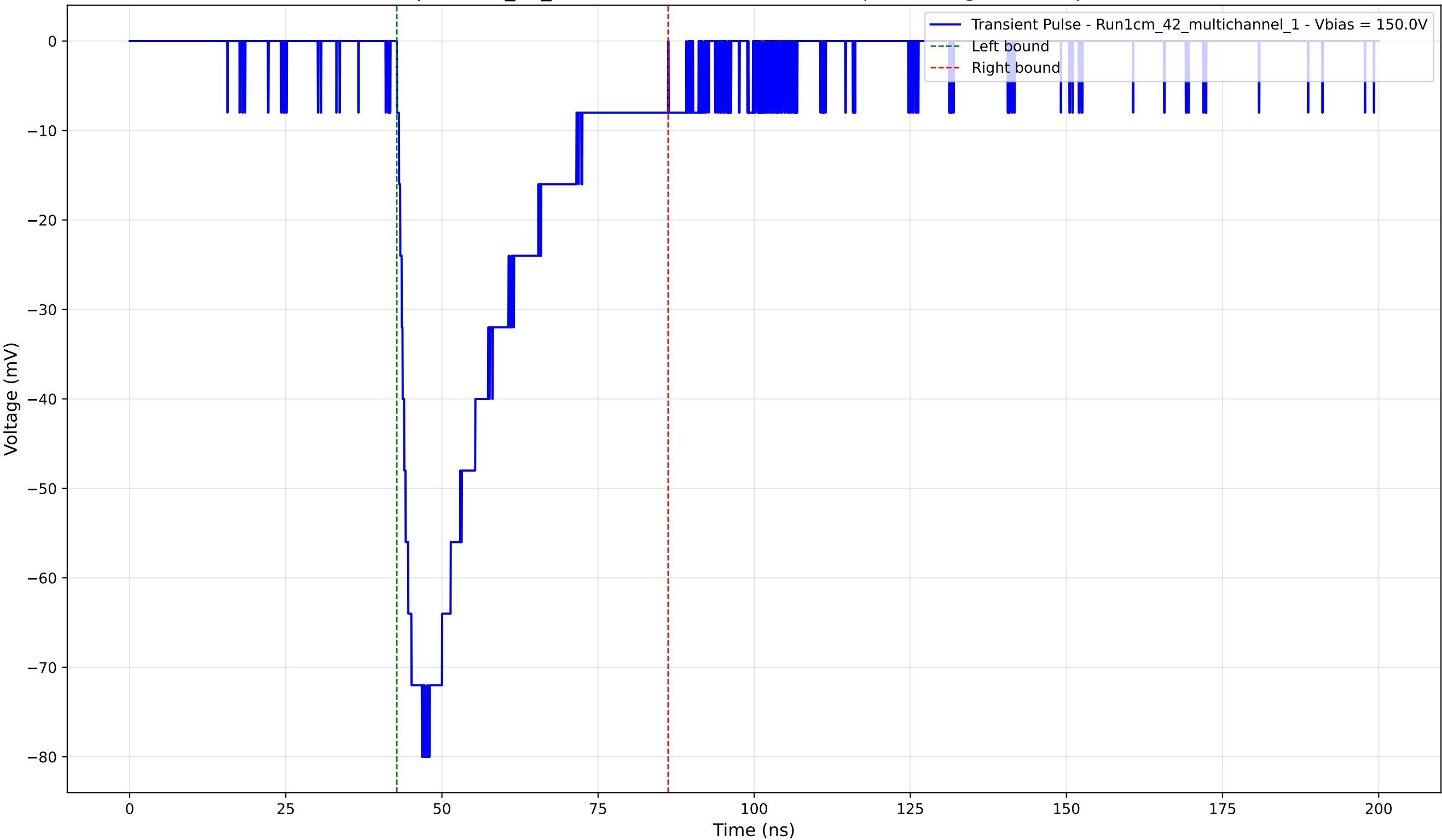
Transient Pulse - Sample: 1cm_42_multichannel - Position: 475.0 \mu\text{m} - Charge: -25.41 pC - Rise Time: 2.02 ns
