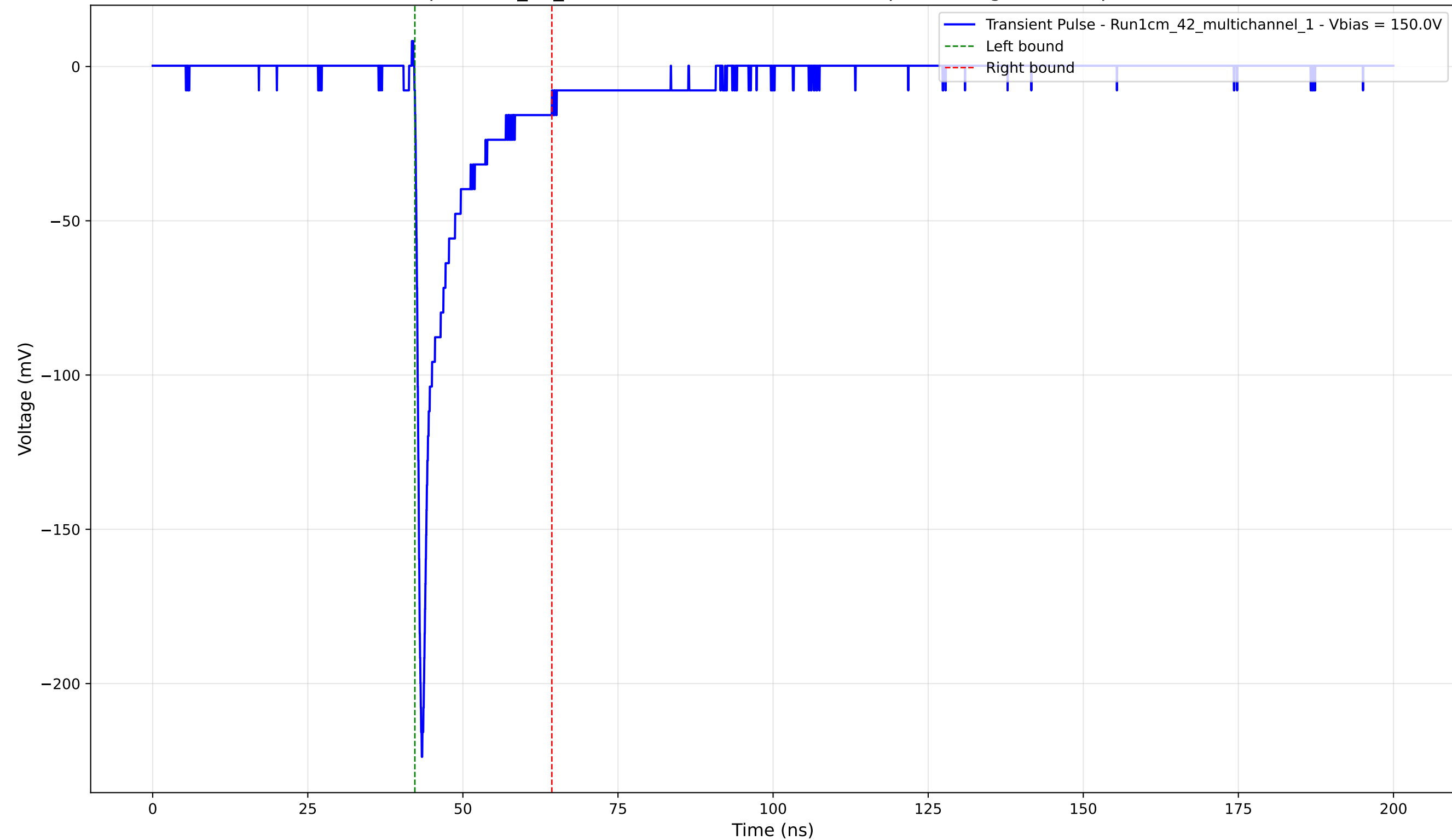
Transient Pulse - Sample: 1cm_42_multichannel - Position: 2800.0 \mu\text{m} - Charge: -20.93 pC - Rise Time: 0.86 ns
