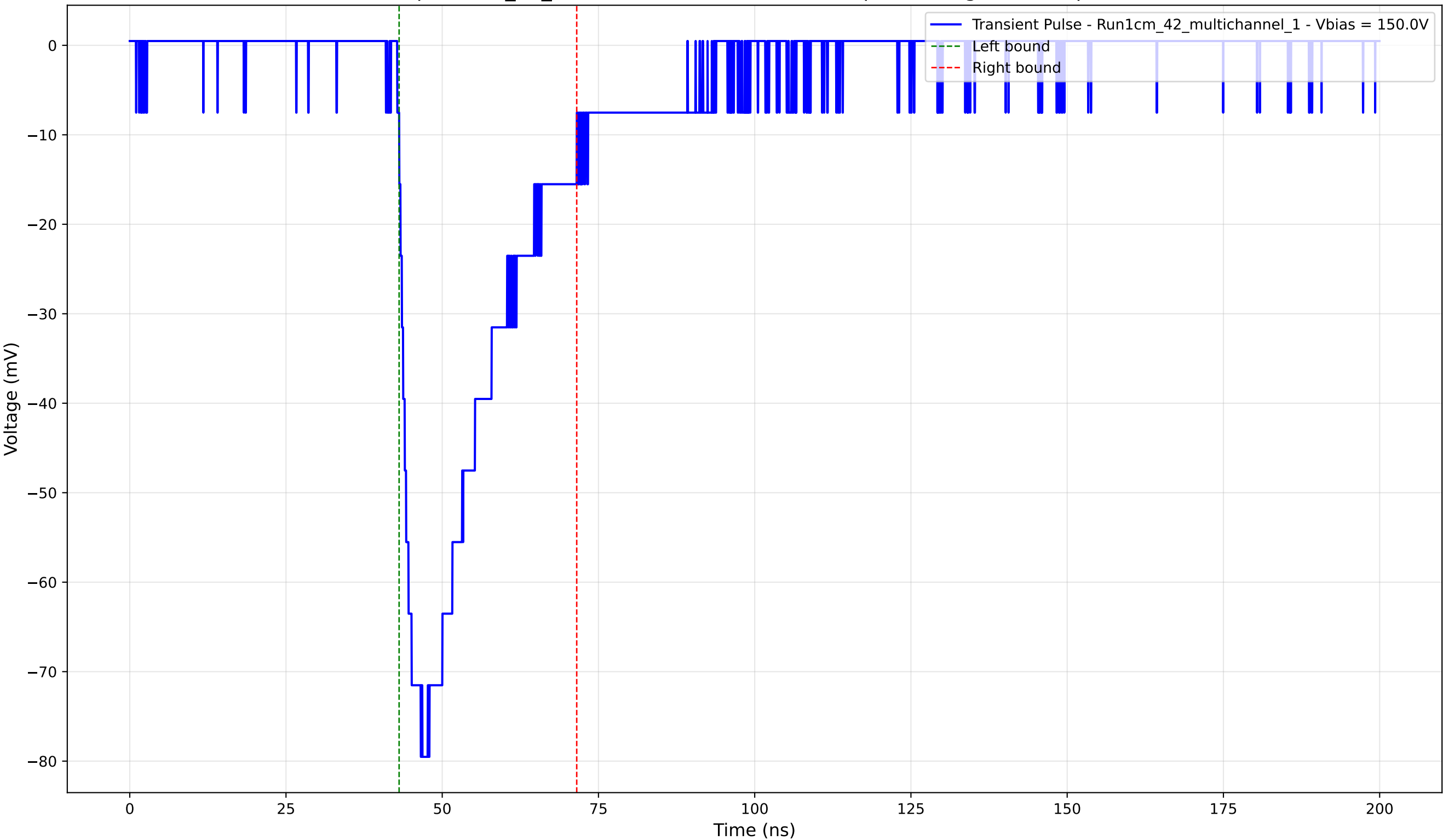
Transient Pulse - Sample: 1cm_42_multichannel - Position: 490.0 \mu\text{m} - Charge: -22.68 pC - Rise Time: 3.46 ns
