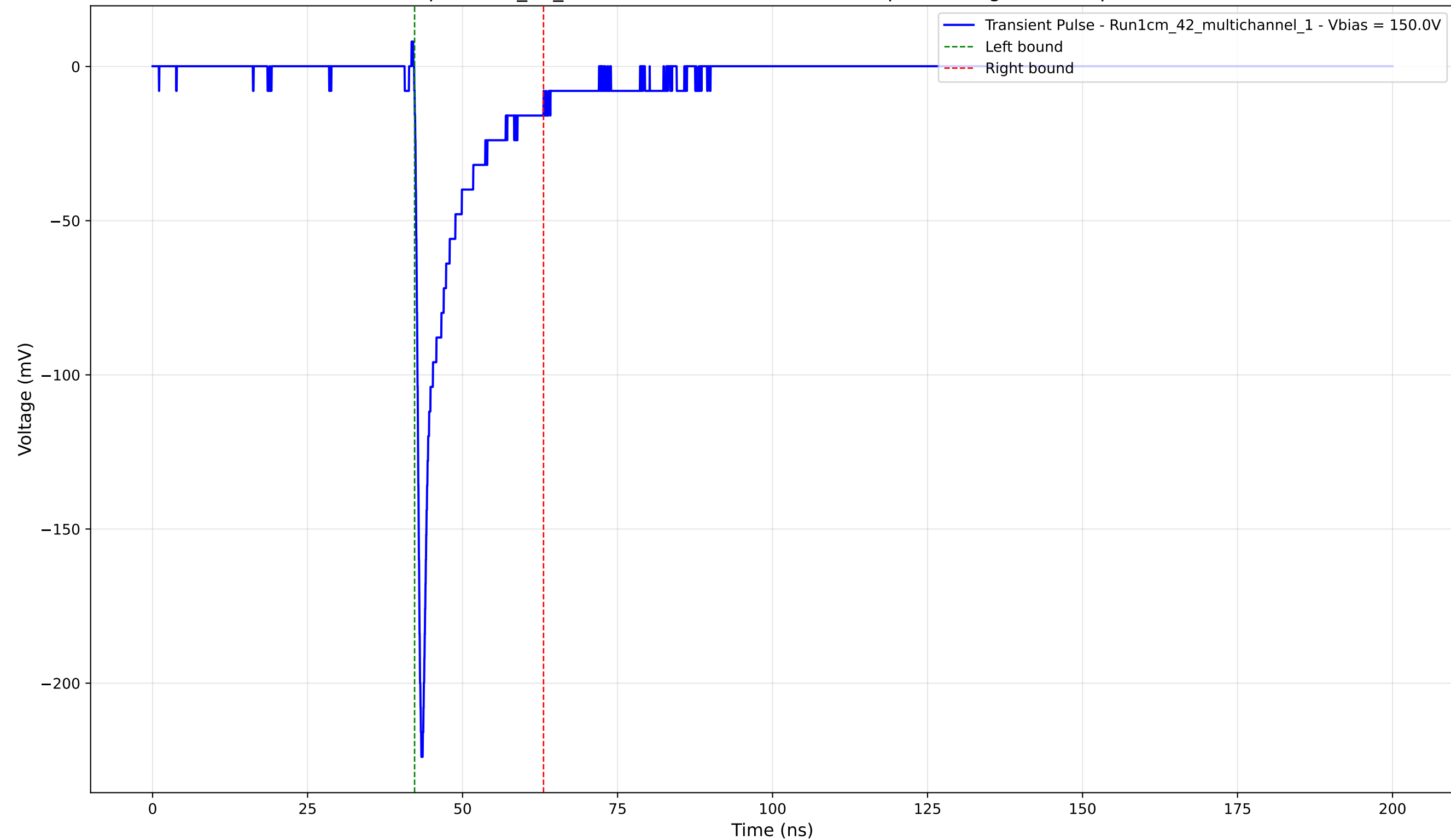
Transient Pulse - Sample: 1cm_42_multichannel - Position: 1960.0 \mu\text{m} - Charge: -20.92 pC - Rise Time: 0.84 ns
