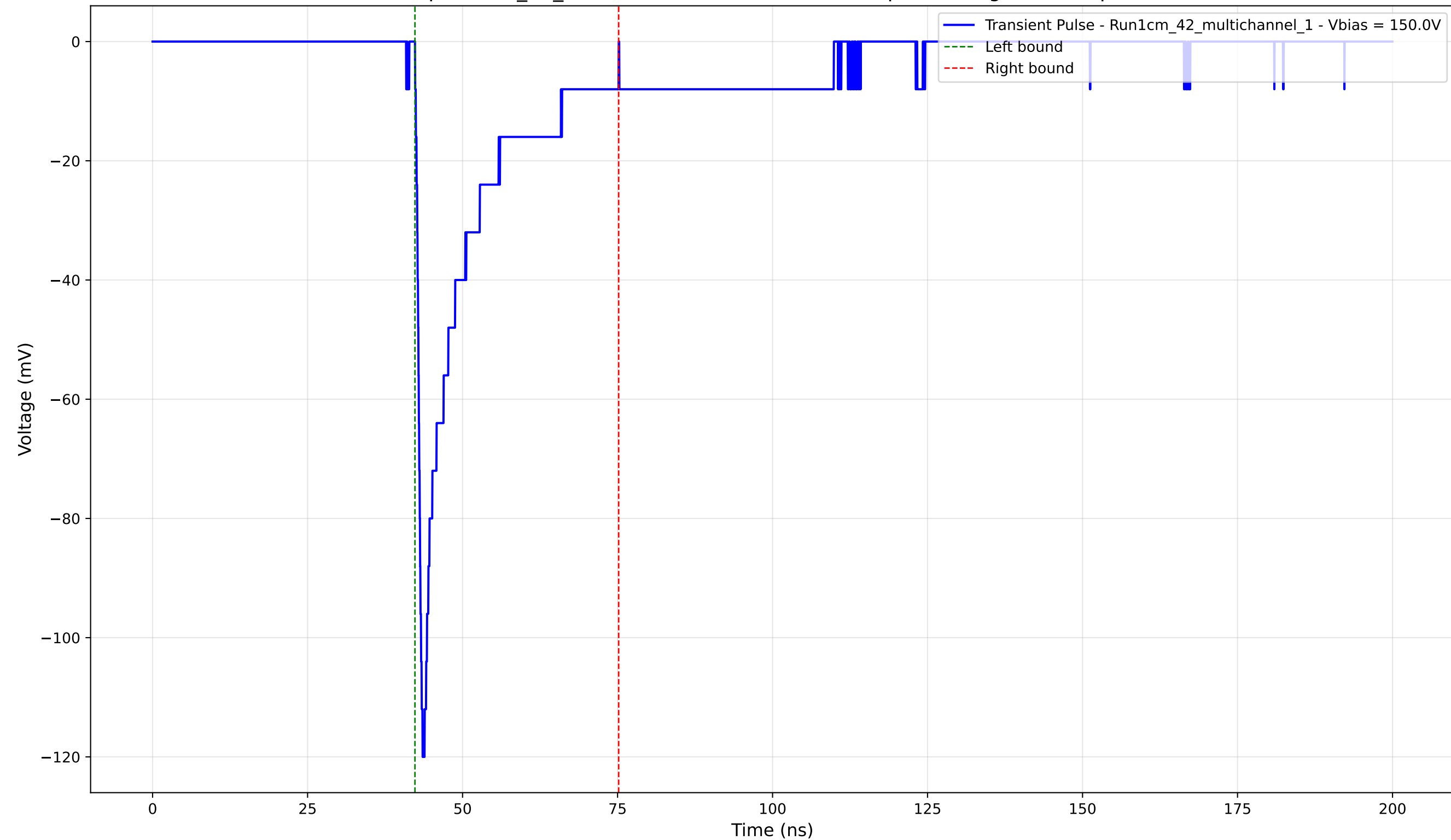
Transient Pulse - Sample: 1cm_42_multichannel - Position: 3175.0 \mu\text{m} - Charge: -17.93 pC - Rise Time: 0.95 ns
