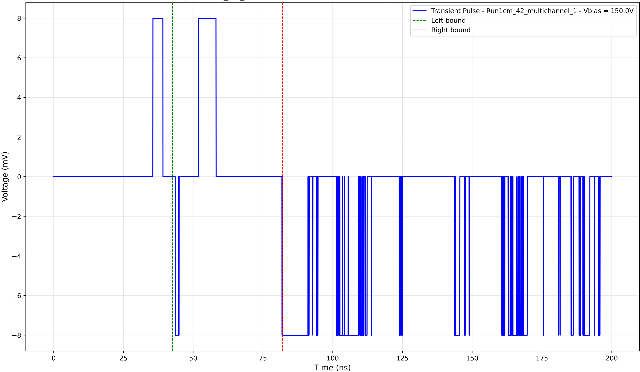
Transient Pulse - Sample: 1cm_42_multichannel - Position: 3895.0 \mu\text{m} - Charge: 0.78 pC - Rise Time: 0.02 ns
