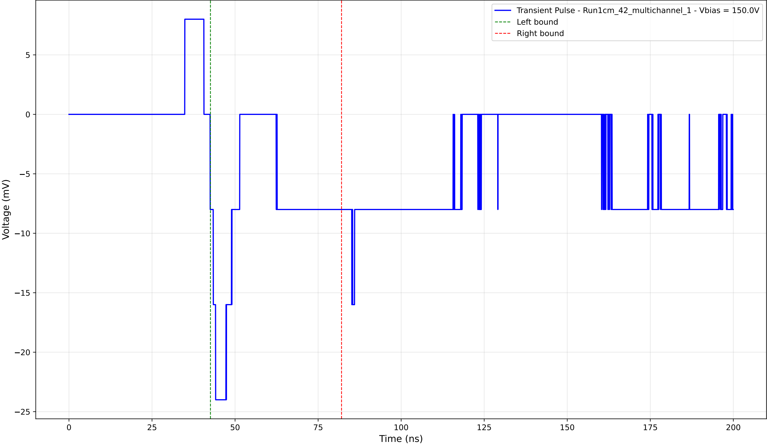
Transient Pulse - Sample: 1cm_42_multichannel - Position: 4855.0 \mu\text{m} - Charge: -5.92 pC - Rise Time: 1.65 ns
