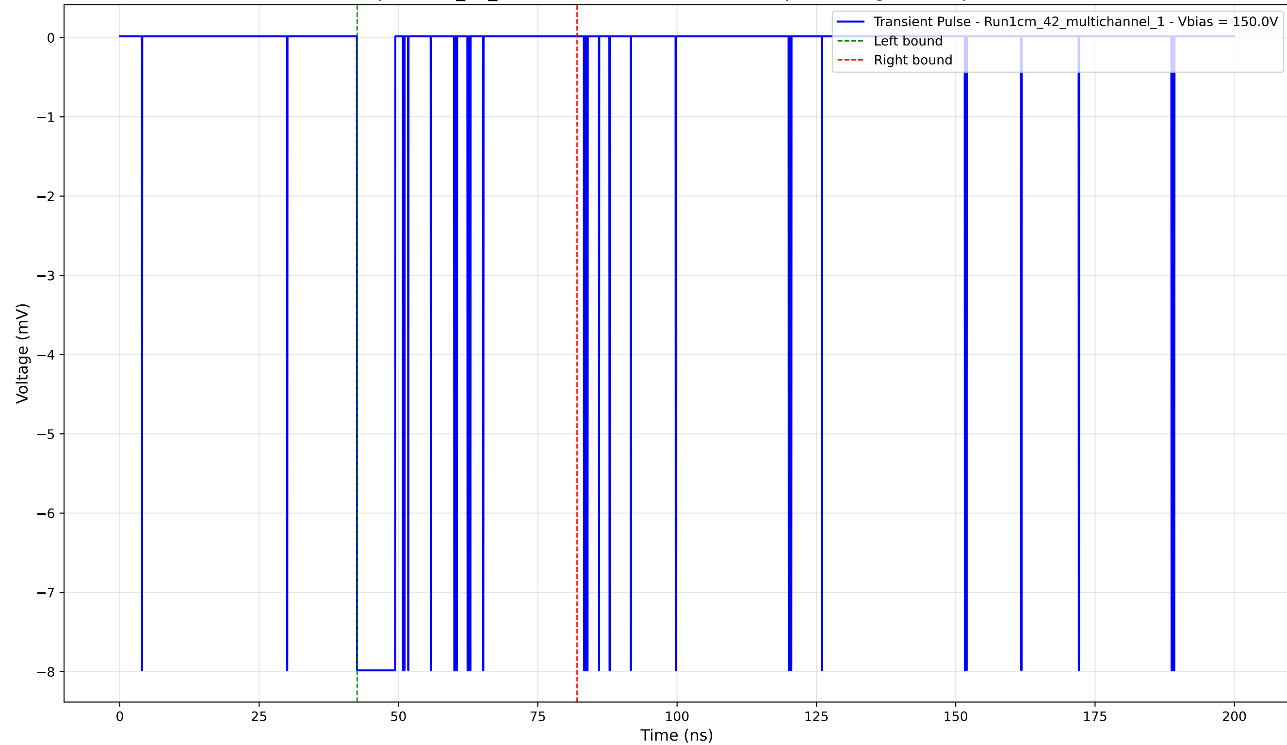
Transient Pulse - Sample: 1cm_42_multichannel - Position: 2900.0 \mu\text{m} - Charge: -1.21 pC - Rise Time: 0.02 ns
