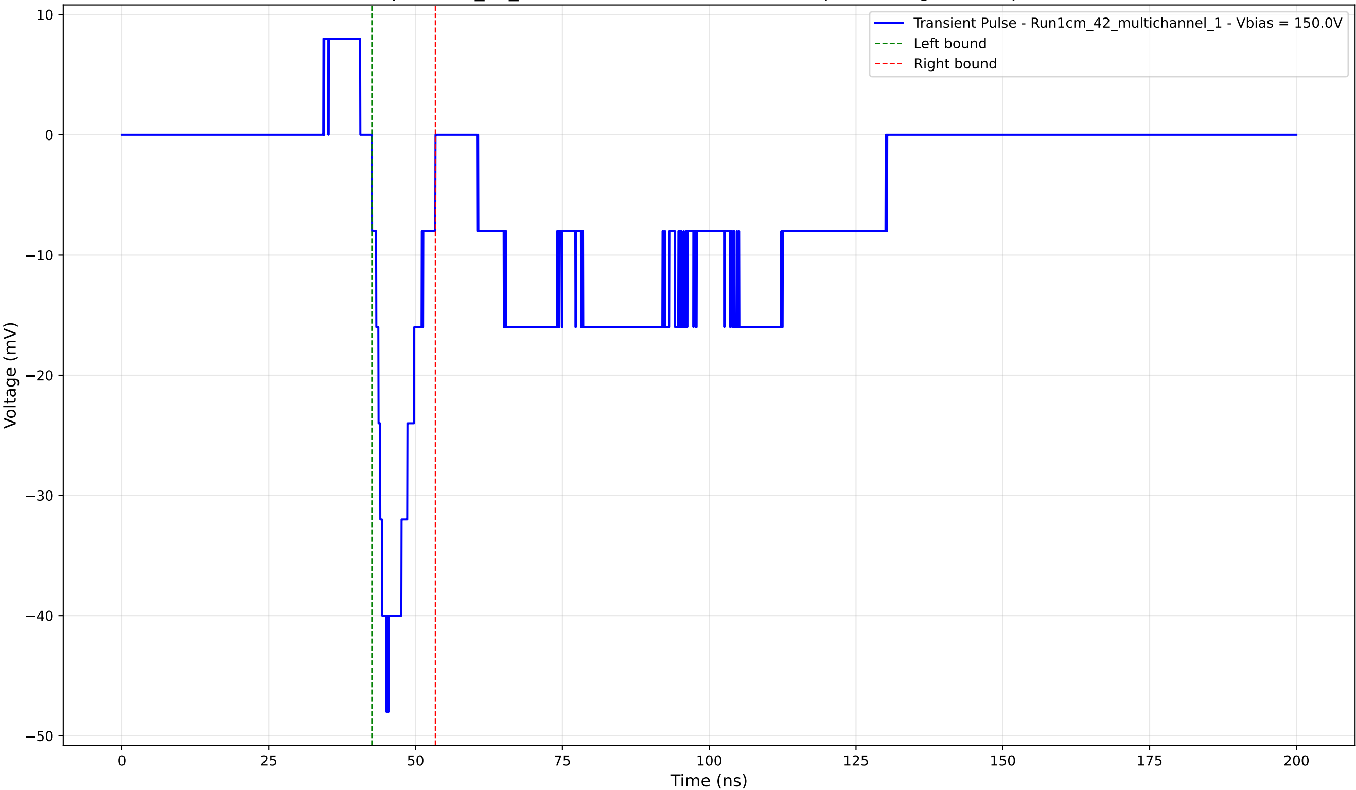
Transient Pulse - Sample: 1cm_42_multichannel - Position: 4590.0 \mu\text{m} - Charge: -5.27 pC - Rise Time: 2.47 ns
