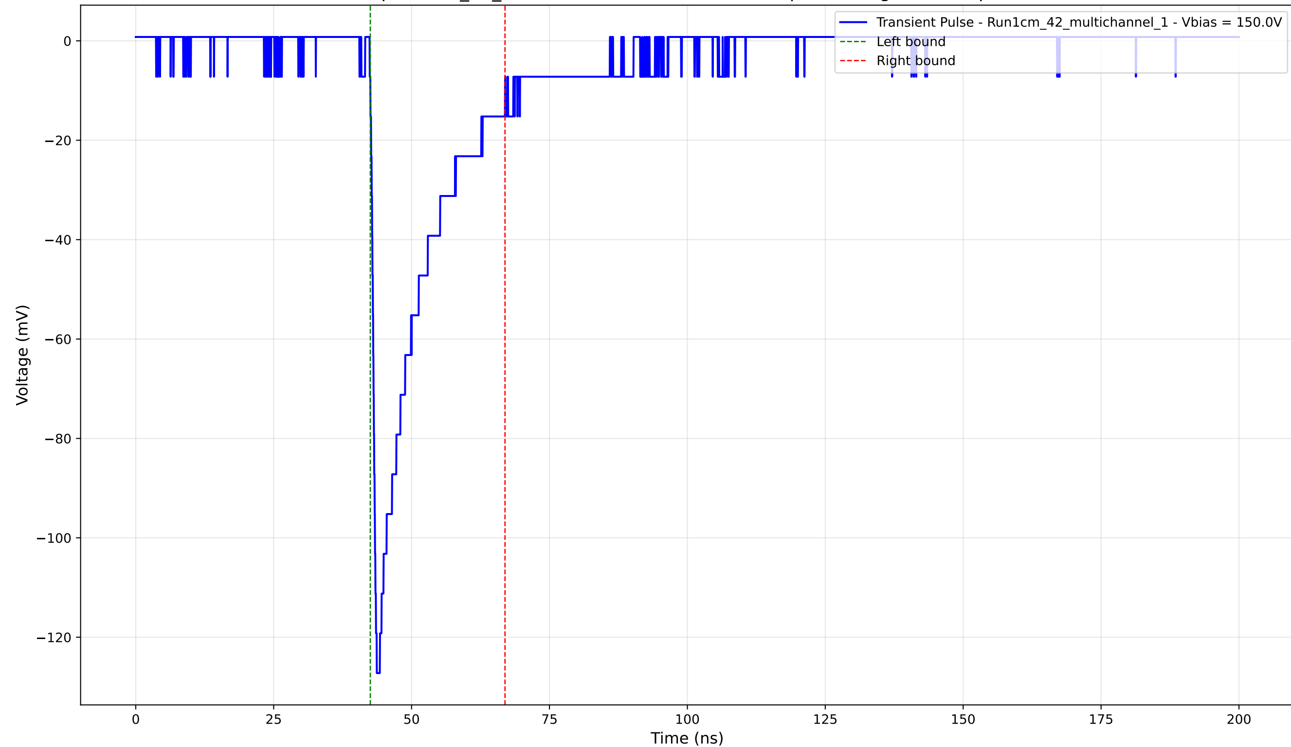
Transient Pulse - Sample: 1cm_42_multichannel - Position: 1500.0 \mu\text{m} - Charge: -22.77 pC - Rise Time: 1.01 ns
