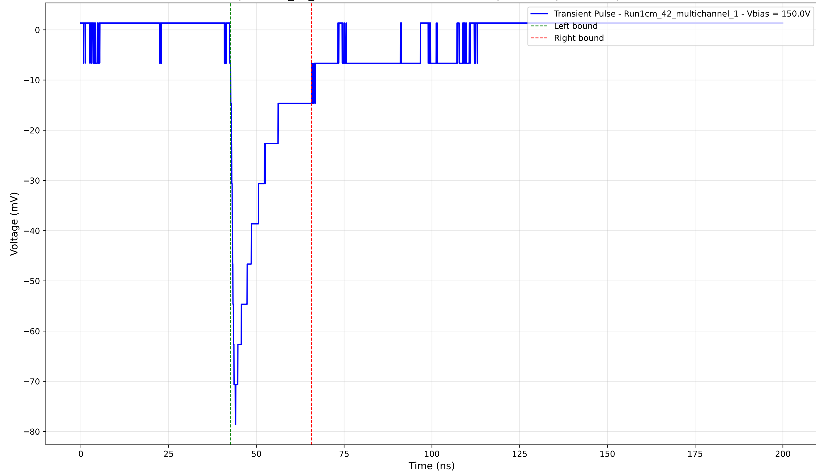
Transient Pulse - Sample: 1cm_42_multichannel - Position: 3475.0 \mu\text{m} - Charge: -13.64 pC - Rise Time: 1.30 ns
