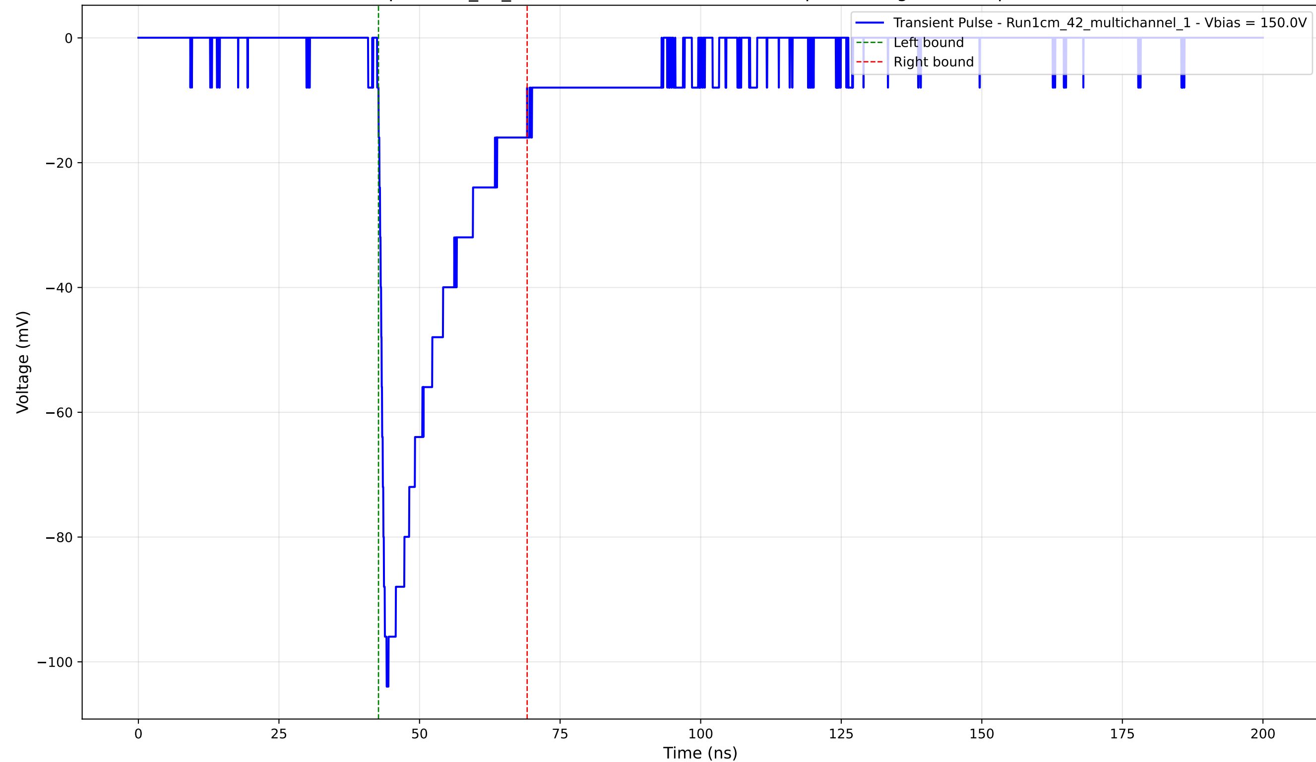
Transient Pulse - Sample: 1cm_42_multichannel - Position: 1250.0 \mu\text{m} - Charge: -23.49 pC - Rise Time: 1.11 ns
