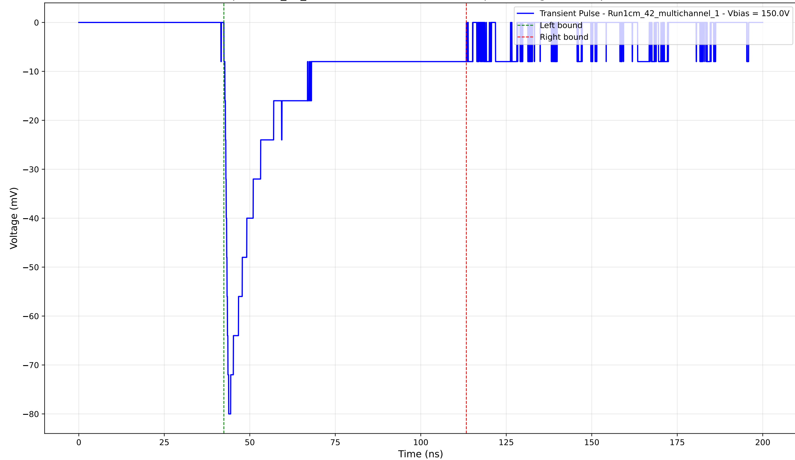
Transient Pulse - Sample: 1cm_42_multichannel - Position: 3505.0 \mu\text{m} - Charge: -23.02 pC - Rise Time: 0.90 ns
