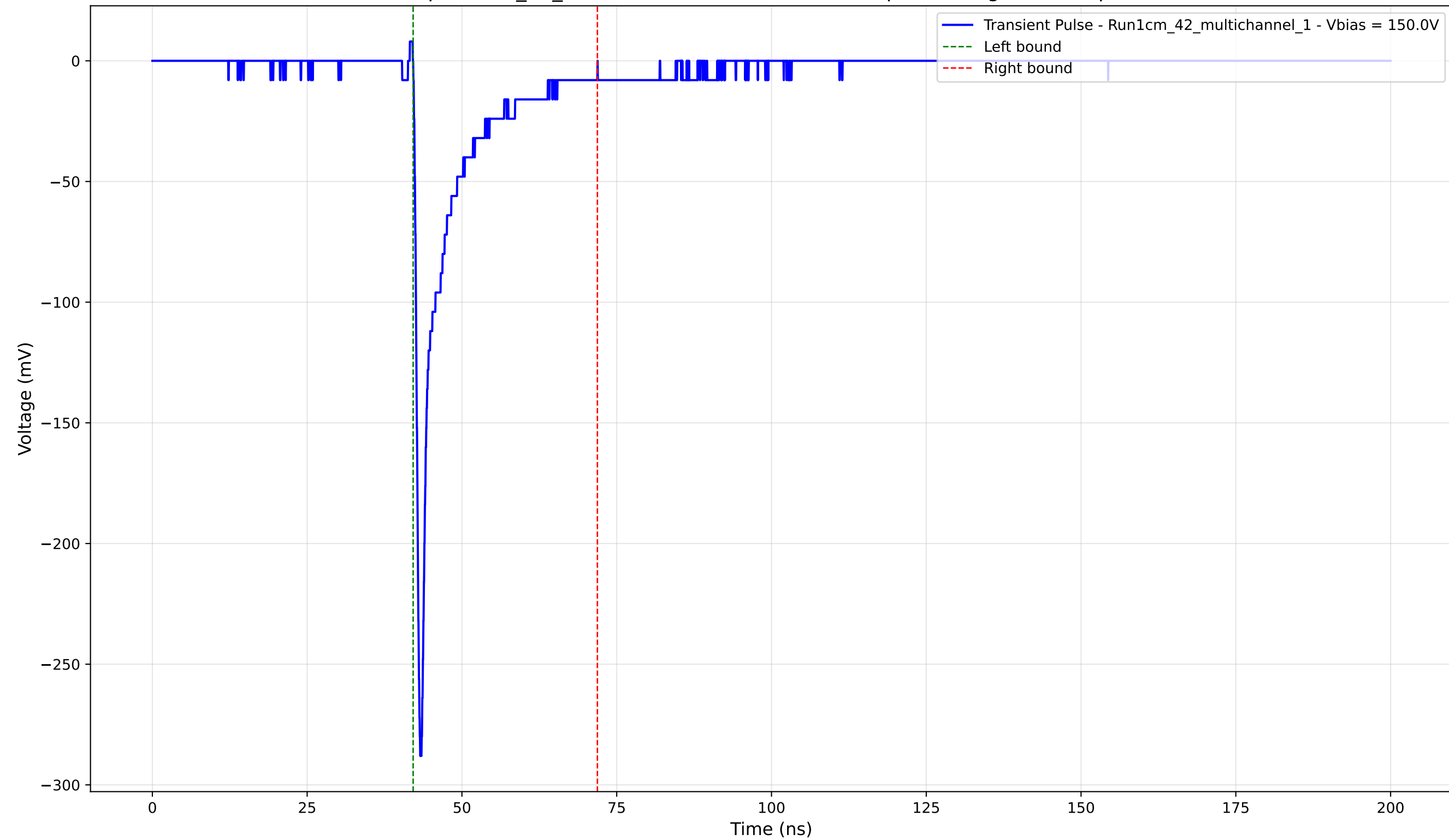
Transient Pulse - Sample: 1cm_42_multichannel - Position: 2065.0 \mu\text{m} - Charge: -25.16 pC - Rise Time: 0.78 ns
