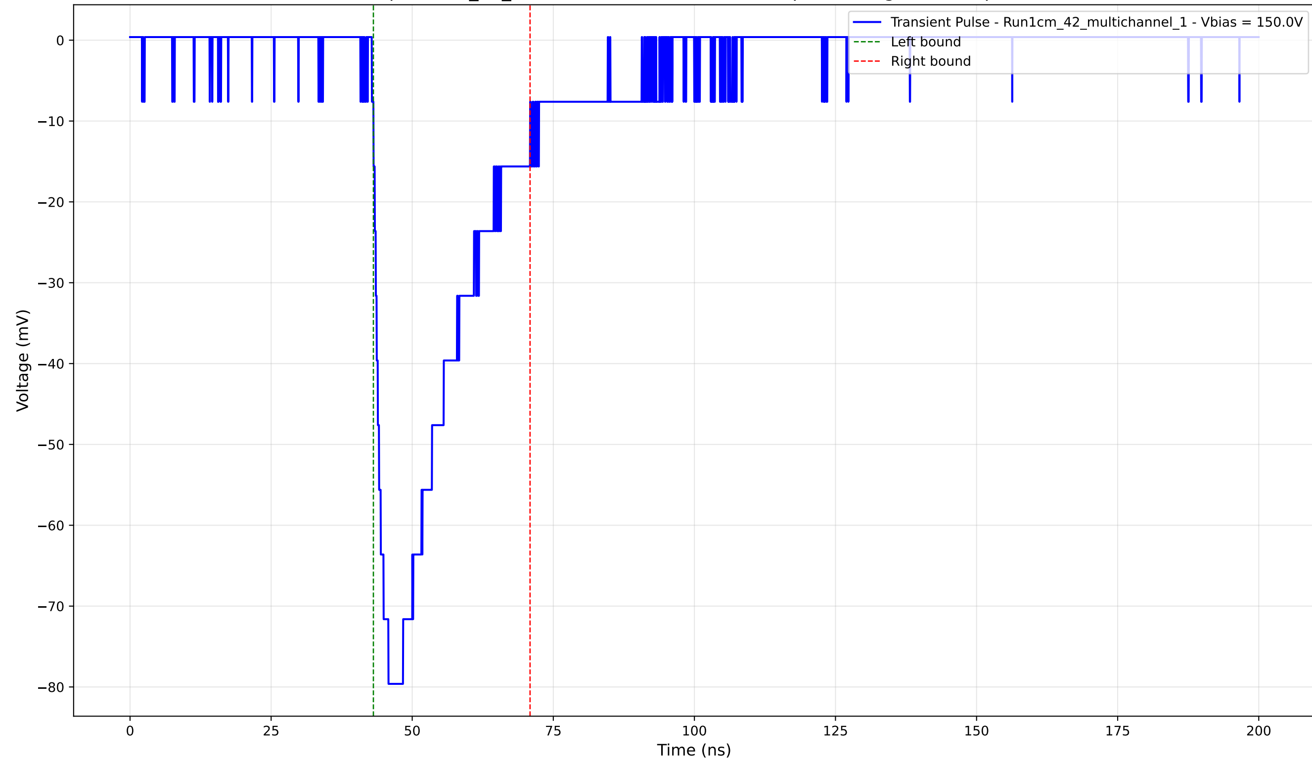
Transient Pulse - Sample: 1cm_42_multichannel - Position: 580.0 \mu\text{m} - Charge: -23.08 pC - Rise Time: 2.66 ns
