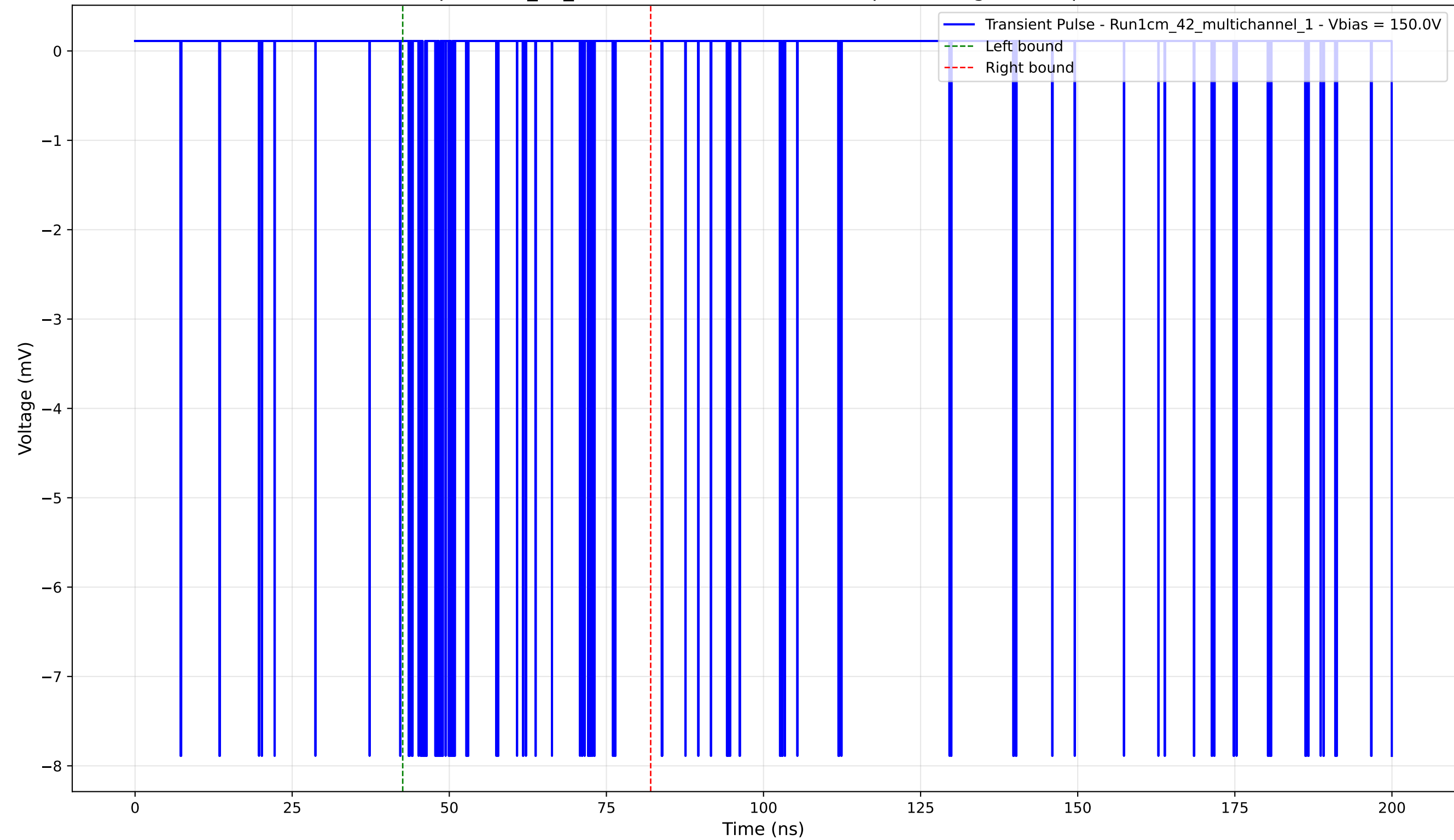
Transient Pulse - Sample: 1cm_42_multichannel - Position: 15.0 \mu\text{m} - Charge: -0.54 pC - Rise Time: 0.02 ns
