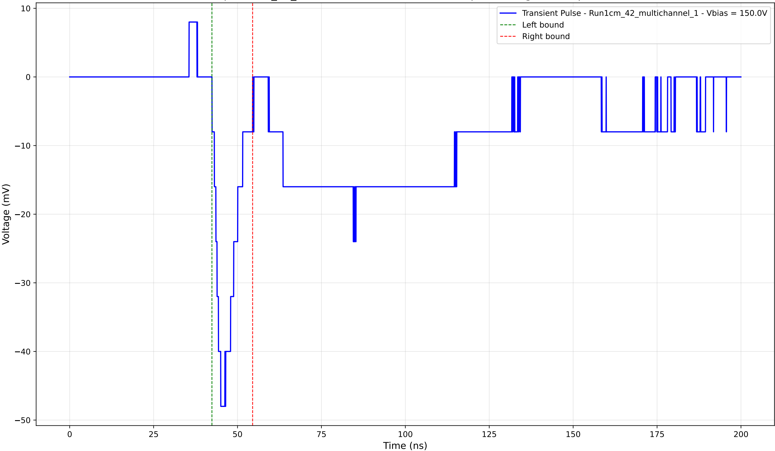
Transient Pulse - Sample: 1cm_42_multichannel - Position: 4610.0 \mu\text{m} - Charge: -5.93 pC - Rise Time: 2.61 ns
