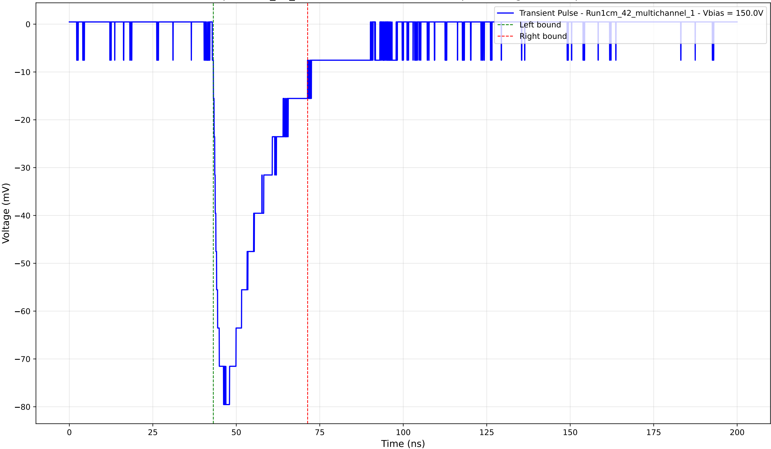
Transient Pulse - Sample: 1cm_42_multichannel - Position: 610.0 \mu\text{m} - Charge: -22.85 pC - Rise Time: 3.06 ns
