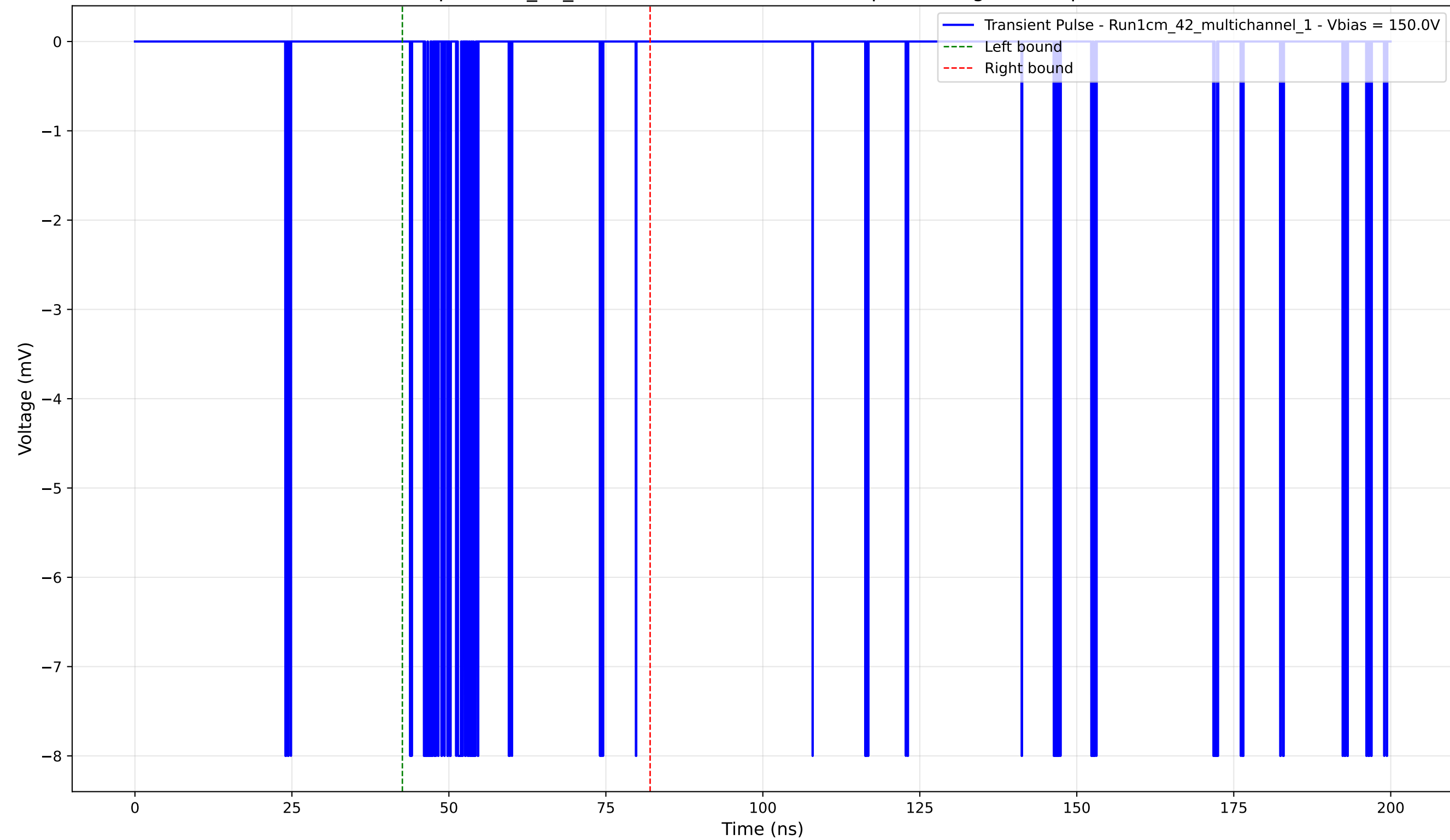
Transient Pulse - Sample: 1cm_42_multichannel - Position: 30.0 \mu\text{m} - Charge: -0.66 pC - Rise Time: 0.02 ns
