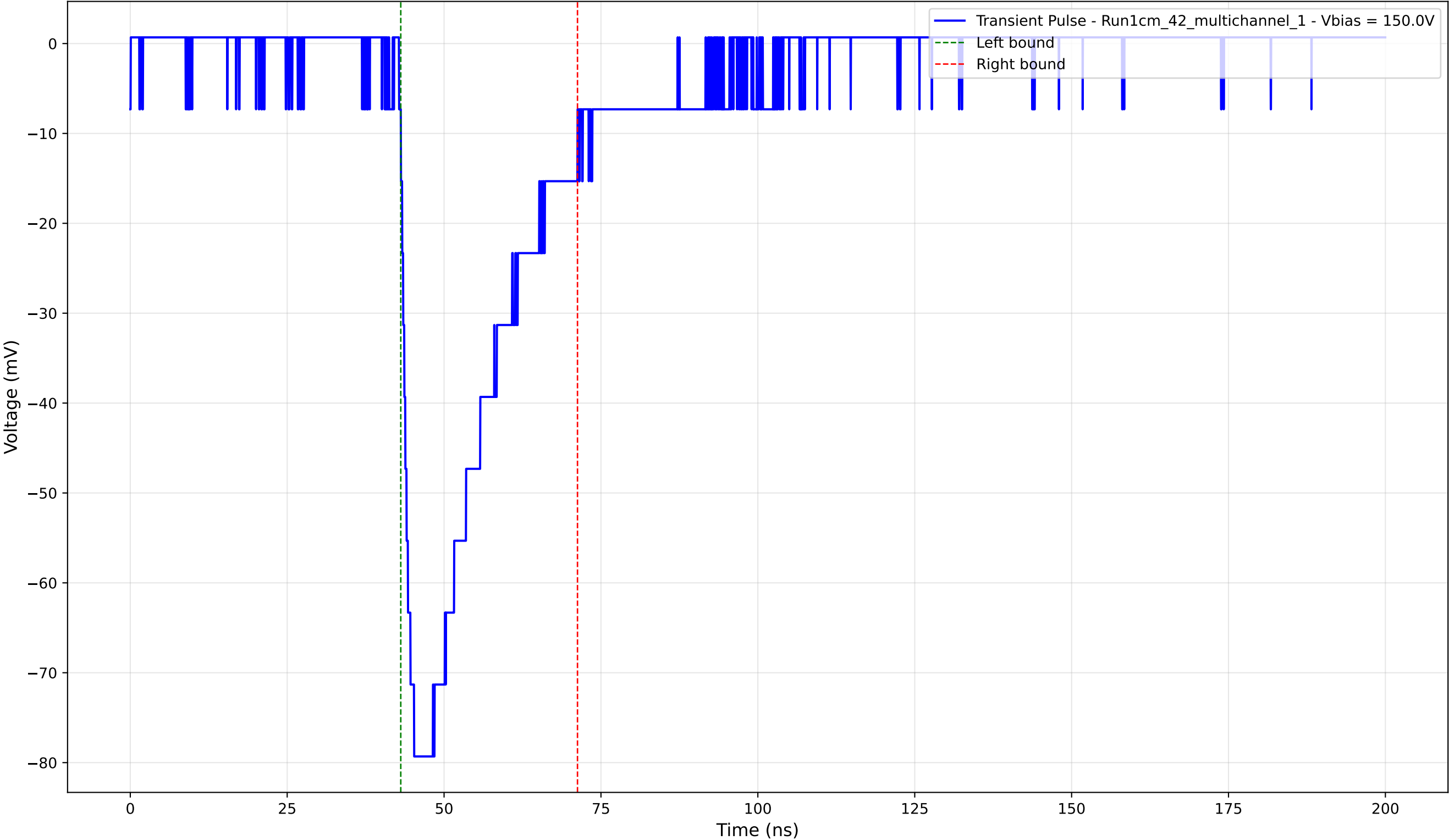
Transient Pulse - Sample: 1cm_42_multichannel - Position: 655.0 \mu\text{m} - Charge: -23.44 pC - Rise Time: 2.12 ns
