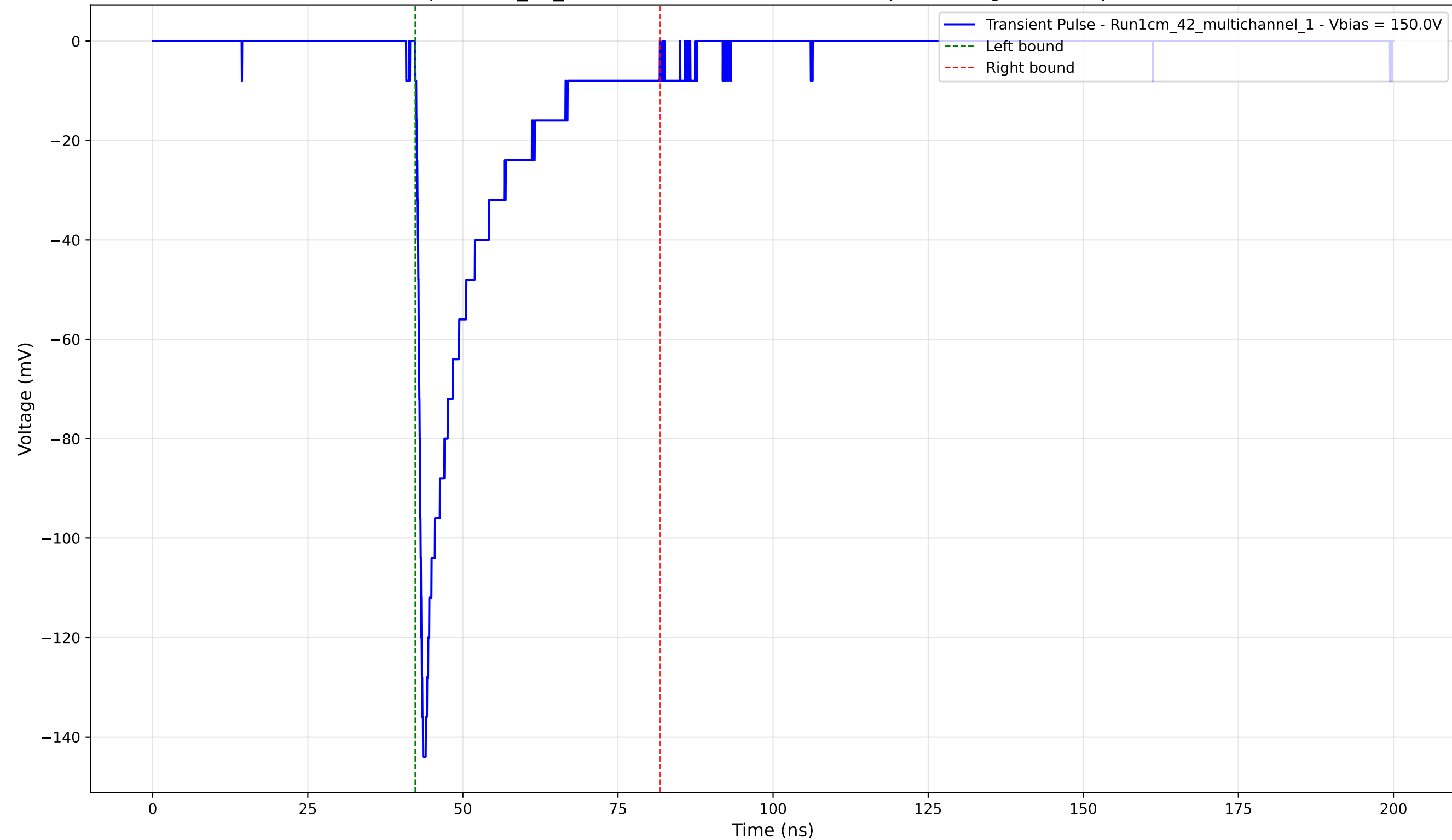
Transient Pulse - Sample: 1cm_42_multichannel - Position: 1610.0 \mu\text{m} - Charge: -24.97 pC - Rise Time: 0.98 ns
