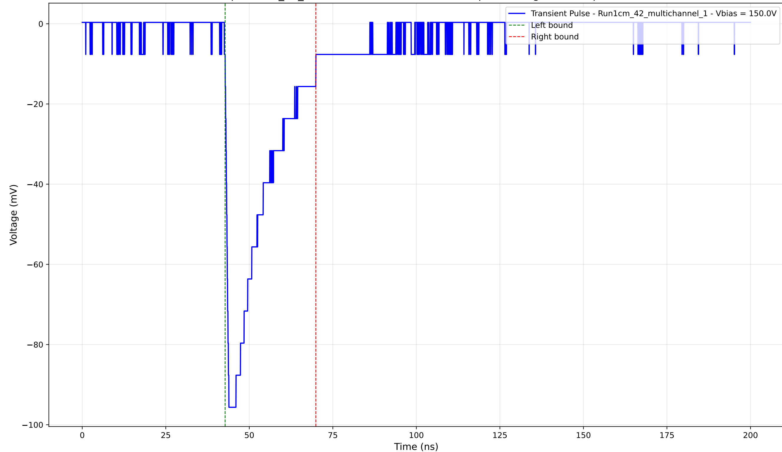
Transient Pulse - Sample: 1cm_42_multichannel - Position: 1220.0 \mu\text{m} - Charge: -23.84 pC - Rise Time: 0.98 ns
