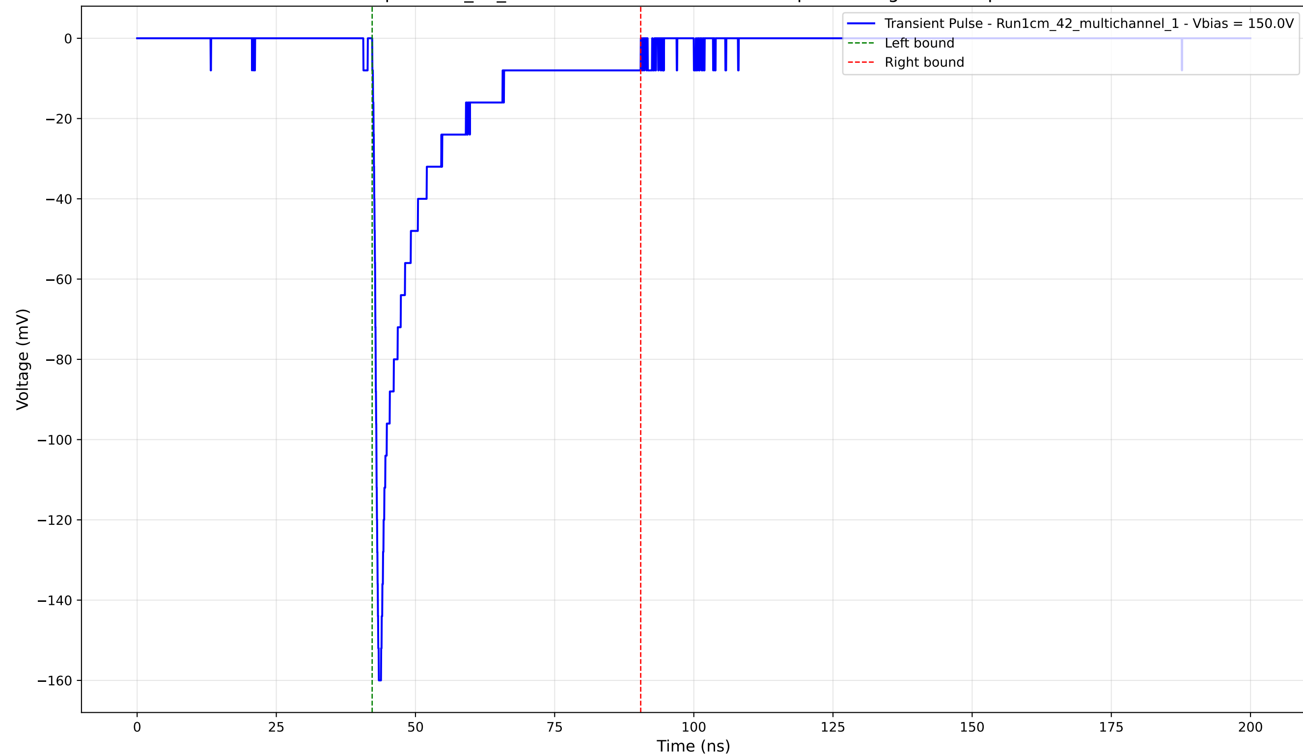
Transient Pulse - Sample: 1cm_42_multichannel - Position: 3025.0 \mu\text{m} - Charge: -24.42 pC - Rise Time: 0.80 ns
