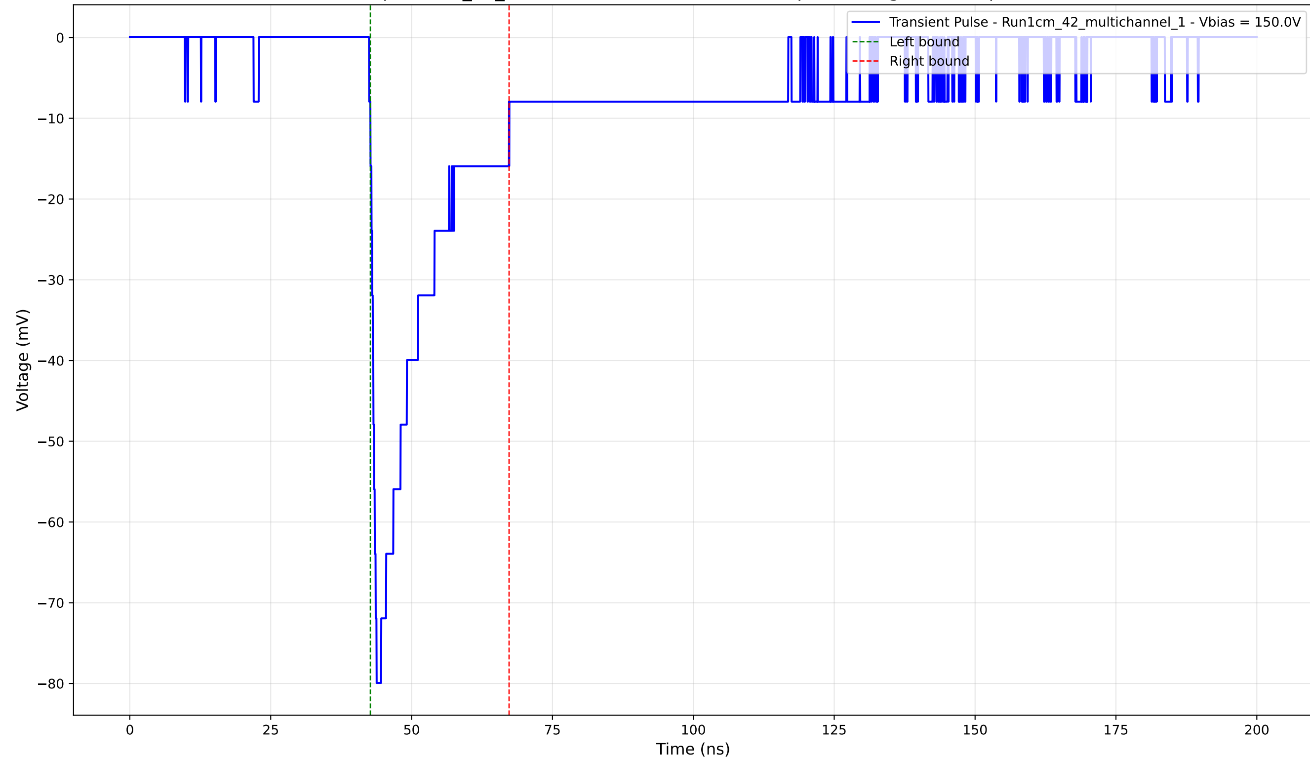
Transient Pulse - Sample: 1cm_42_multichannel - Position: 3510.0 \mu\text{m} - Charge: -15.84 pC - Rise Time: 1.10 ns
