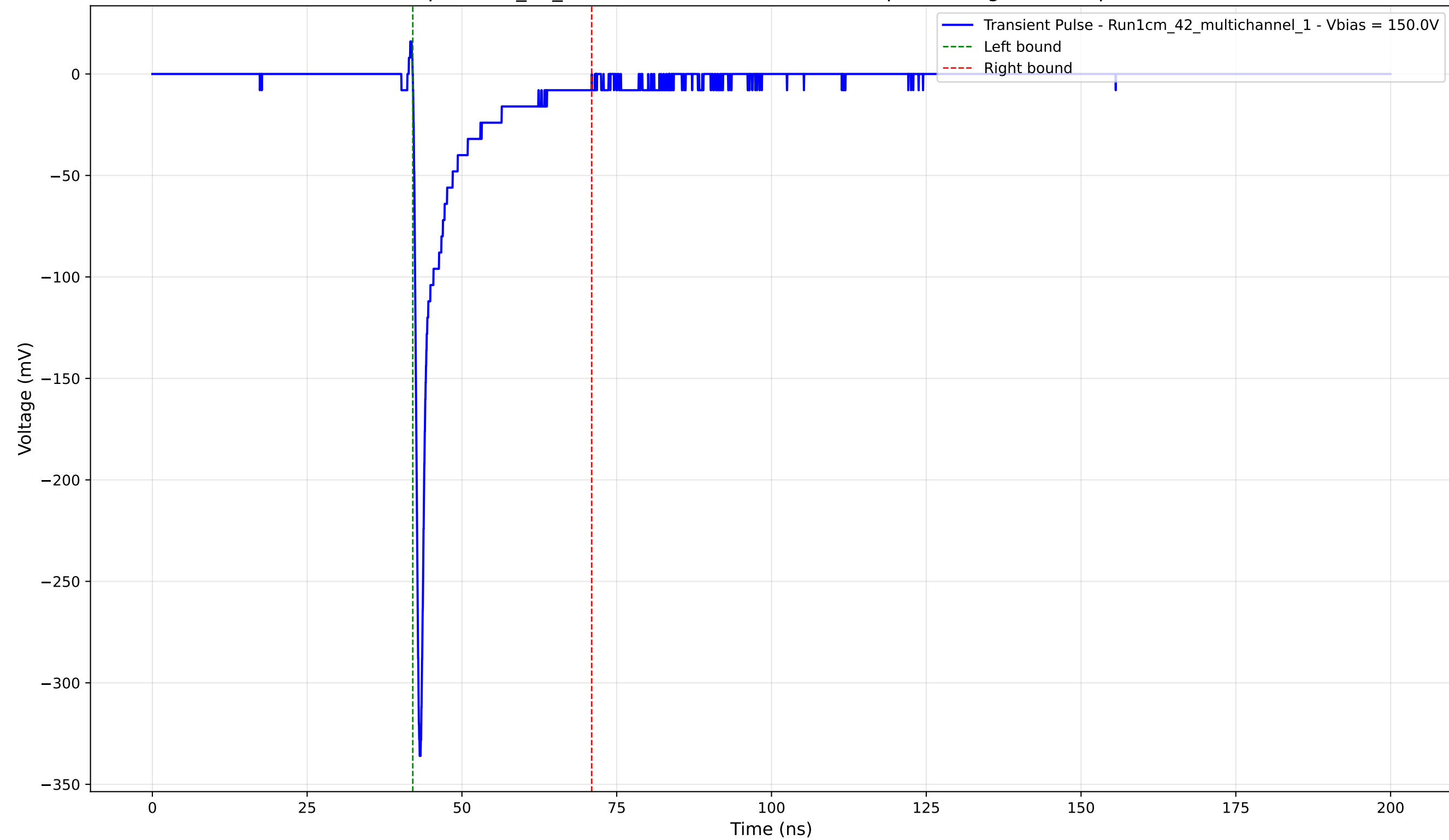
Transient Pulse - Sample: 1cm_42_multichannel - Position: 2590.0 \mu\text{m} - Charge: -24.84 pC - Rise Time: 0.73 ns
