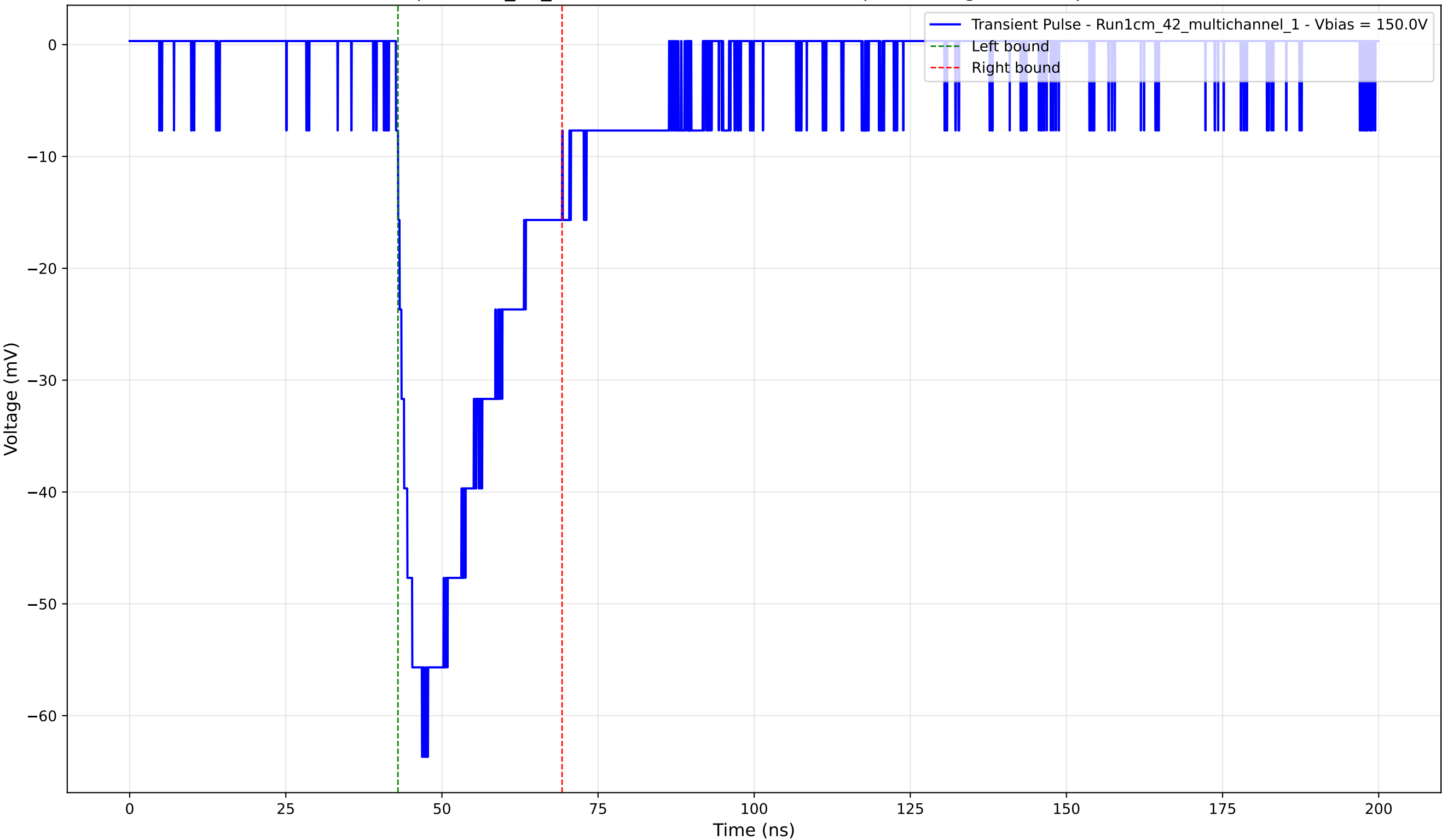
Transient Pulse - Sample: 1cm_42_multichannel - Position: 120.0 \mu\text{m} - Charge: -18.19 pC - Rise Time: 4.16 ns
