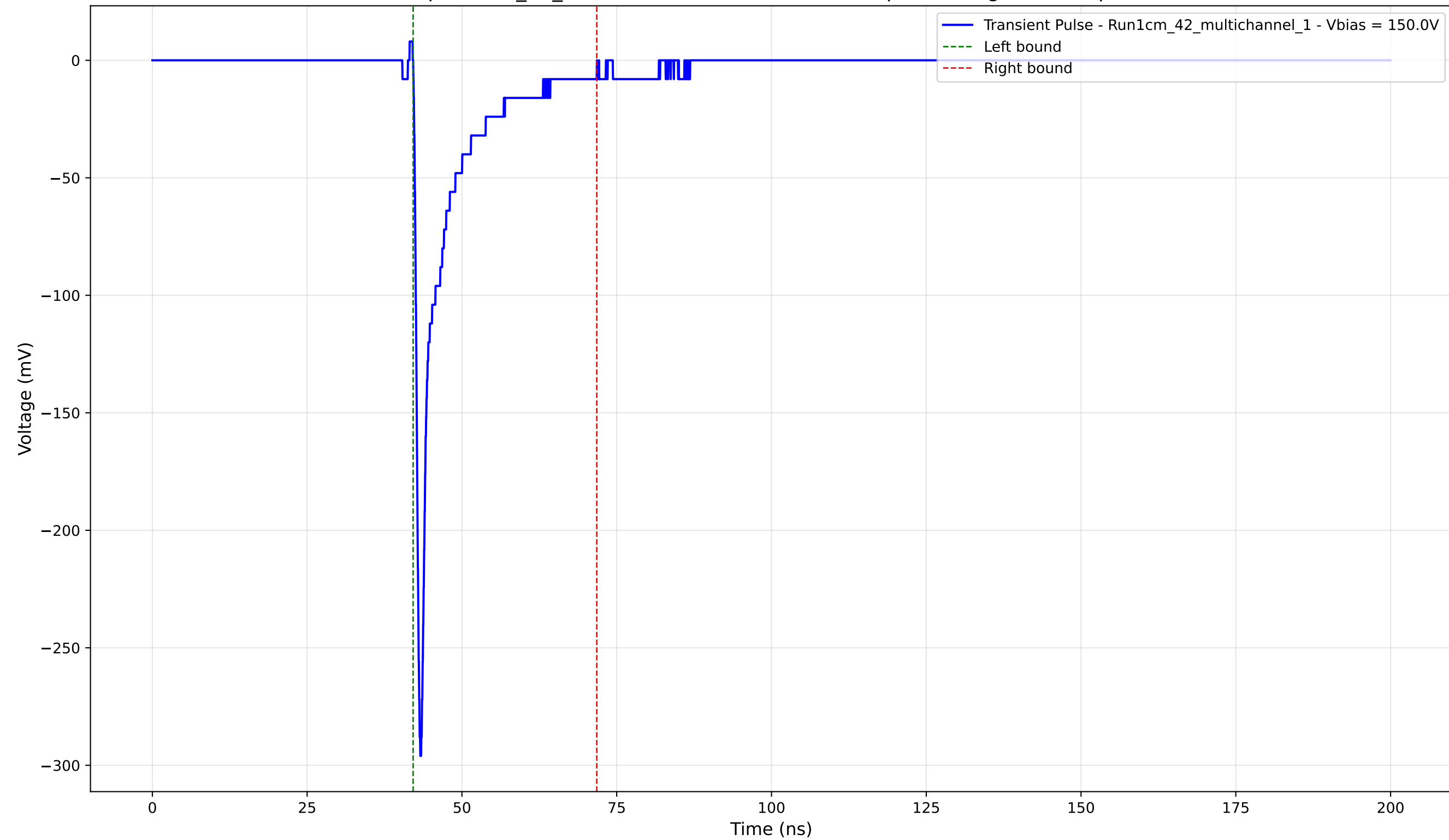
Transient Pulse - Sample: 1cm_42_multichannel - Position: 2080.0 \mu\text{m} - Charge: -24.77 pC - Rise Time: 0.79 ns
