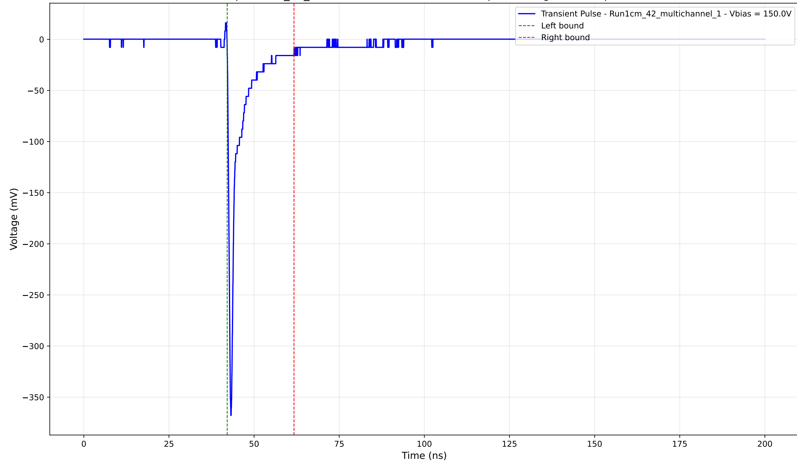
Transient Pulse - Sample: 1cm_42_multichannel - Position: 2550.0 \mu\text{m} - Charge: -23.72 pC - Rise Time: 0.75 ns
