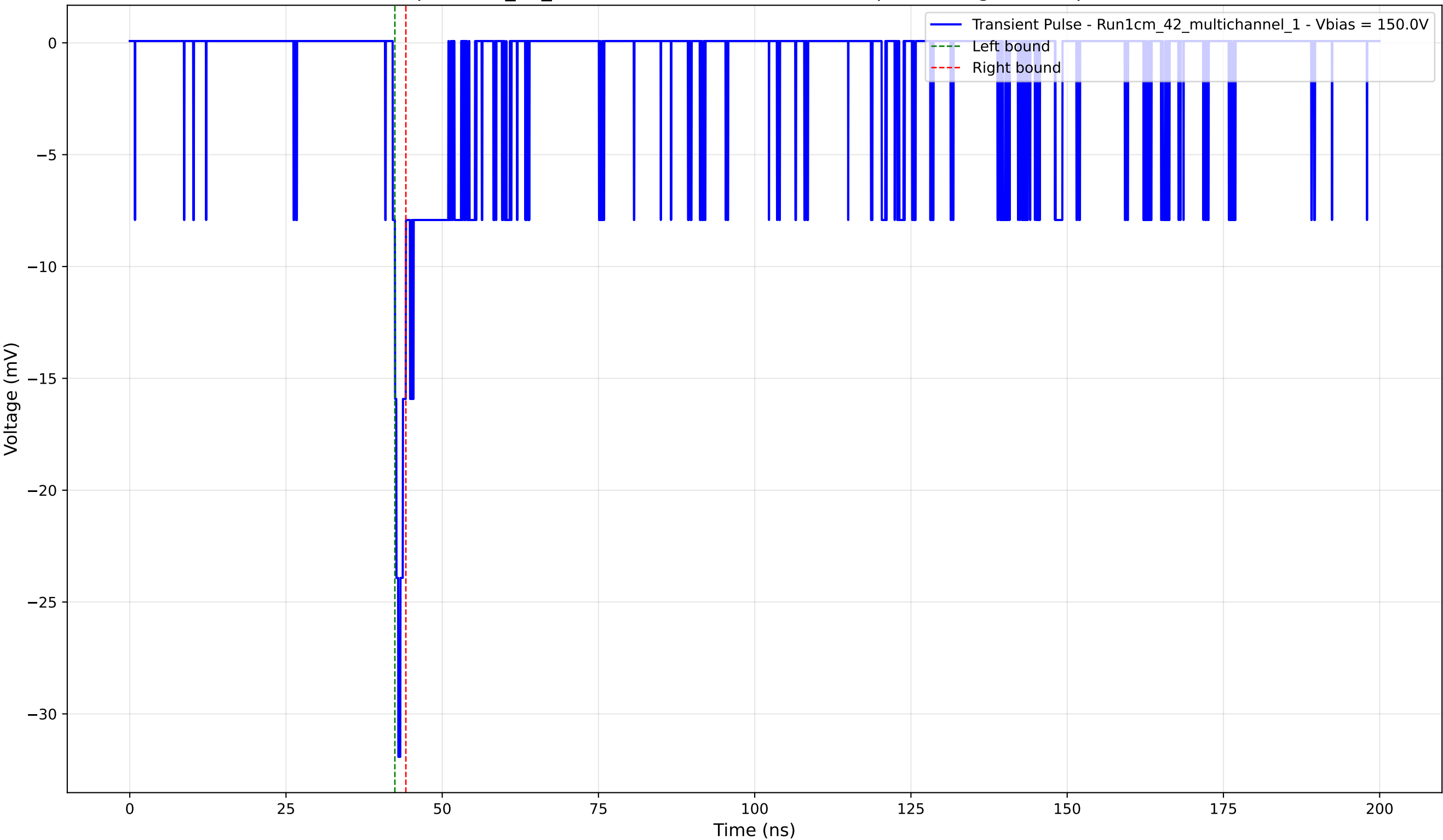
Transient Pulse - Sample: 1cm_42_multichannel - Position: 2365.0 \mu\text{m} - Charge: -0.78 pC - Rise Time: 0.89 ns
