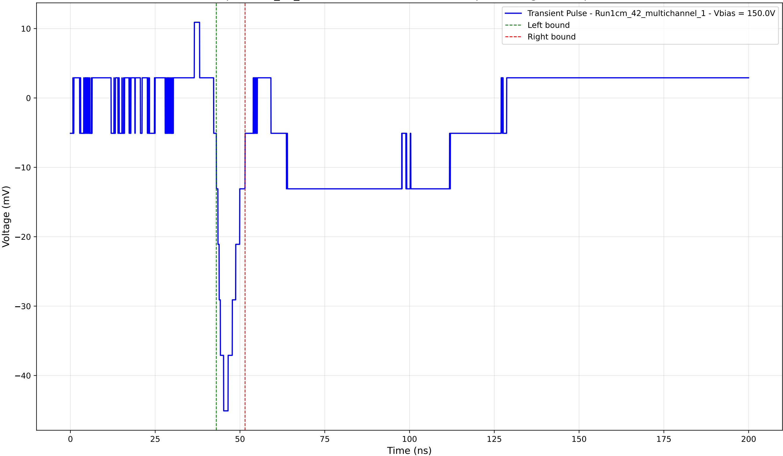
Transient Pulse - Sample: 1cm_42_multichannel - Position: 4715.0 \mu\text{m} - Charge: -4.80 pC - Rise Time: 2.95 ns
