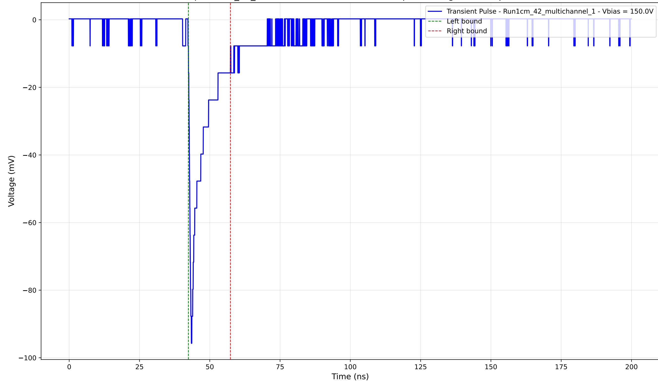
Transient Pulse - Sample: 1cm_42_multichannel - Position: 1830.0 \mu\text{m} - Charge: -10.06 pC - Rise Time: 0.86 ns
