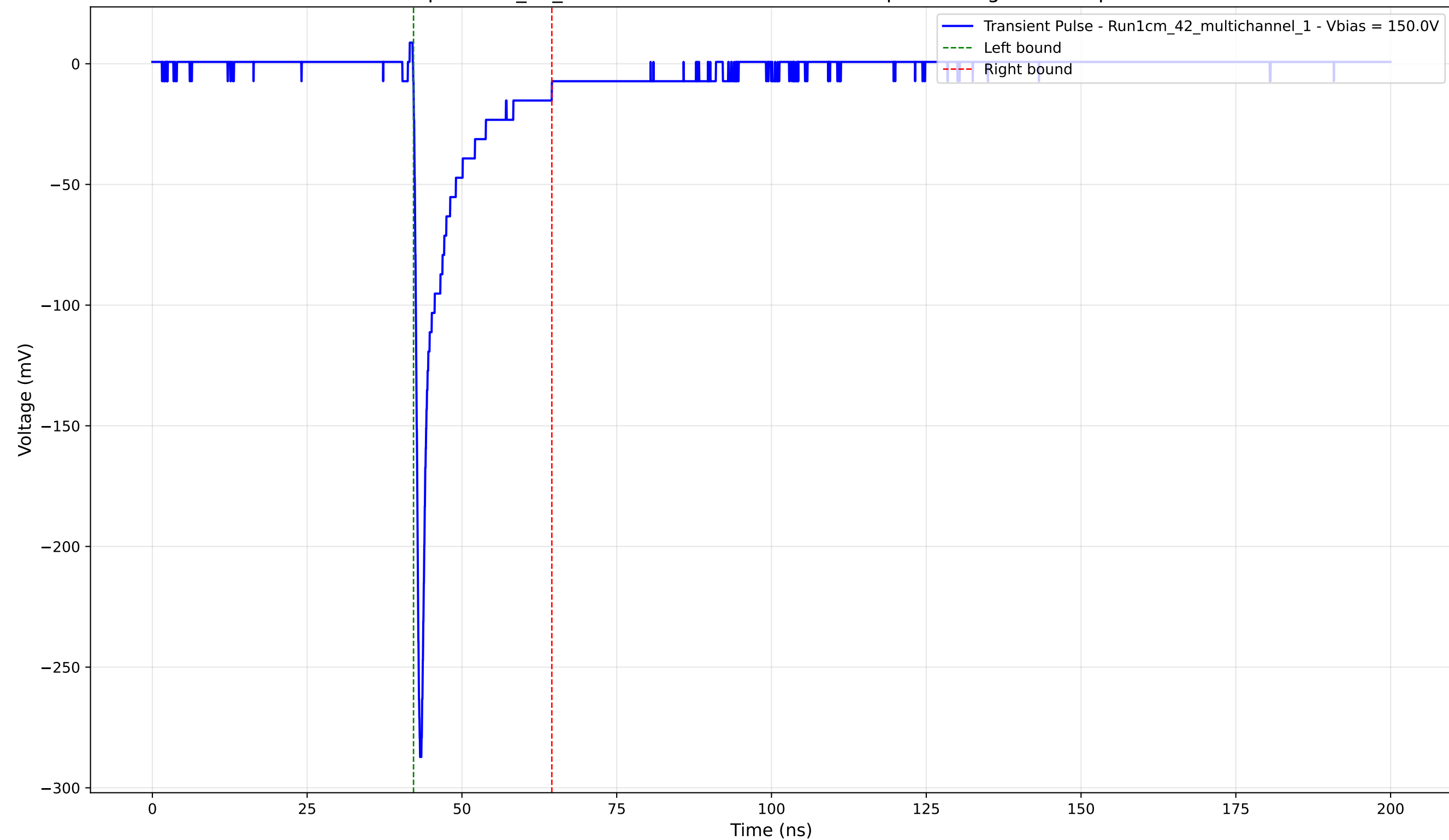
Transient Pulse - Sample: 1cm_42_multichannel - Position: 2075.0 \mu\text{m} - Charge: -23.65 pC - Rise Time: 0.77 ns
