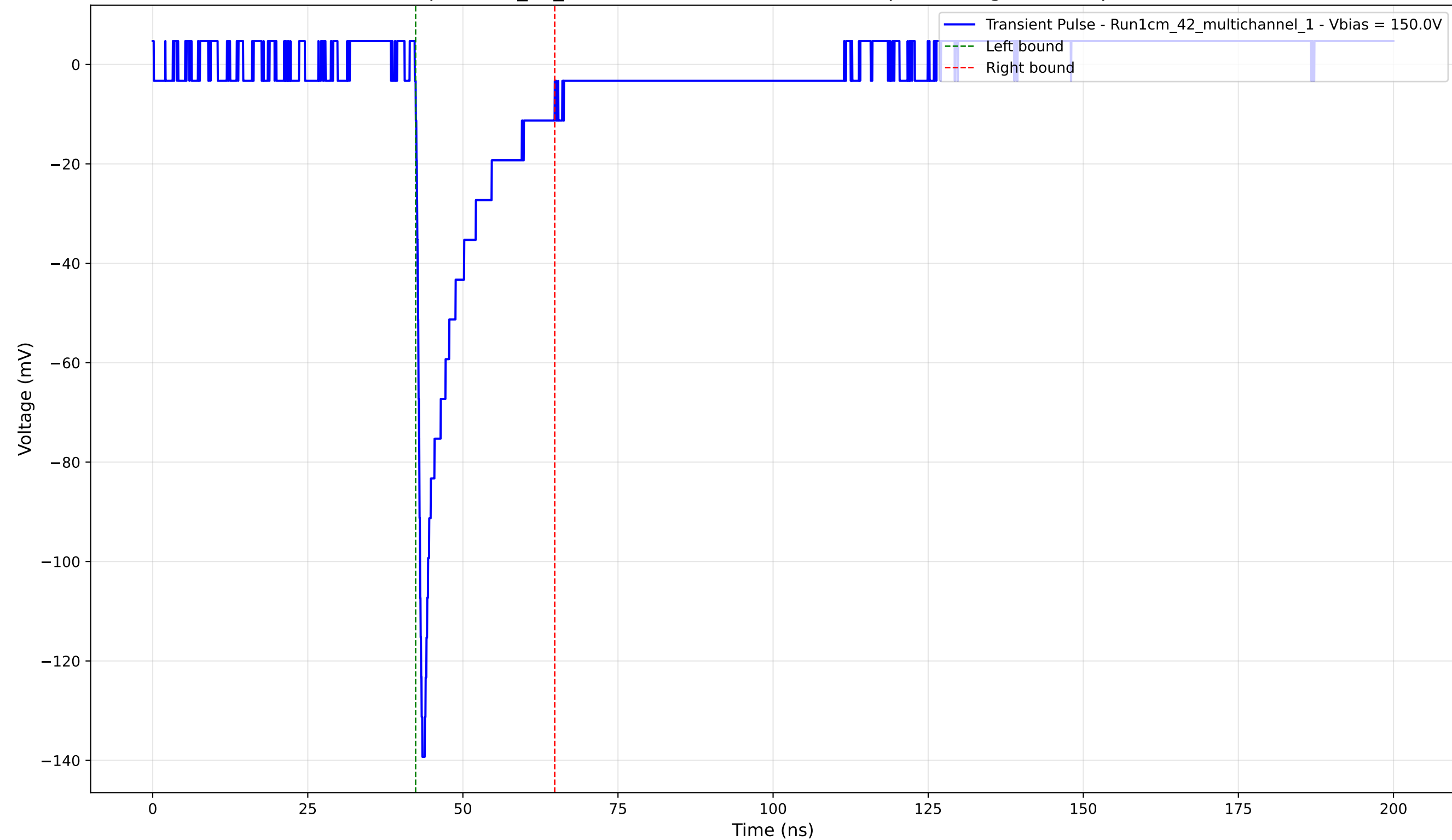
Transient Pulse - Sample: 1cm_42_multichannel - Position: 3070.0 \mu\text{m} - Charge: -17.06 pC - Rise Time: 0.85 ns
