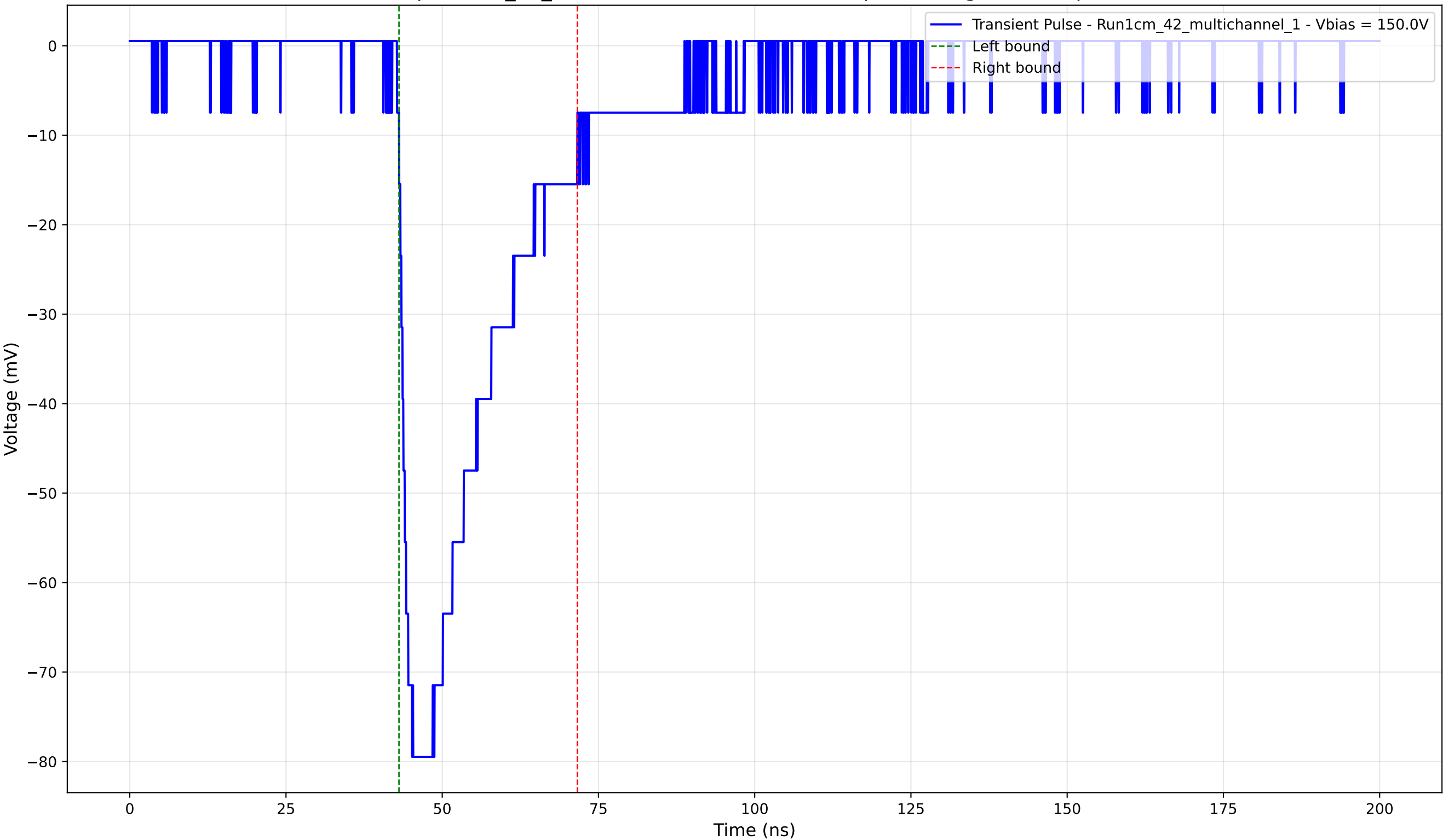
Transient Pulse - Sample: 1cm_42_multichannel - Position: 675.0 \mu\text{m} - Charge: -23.44 pC - Rise Time: 2.08 ns
