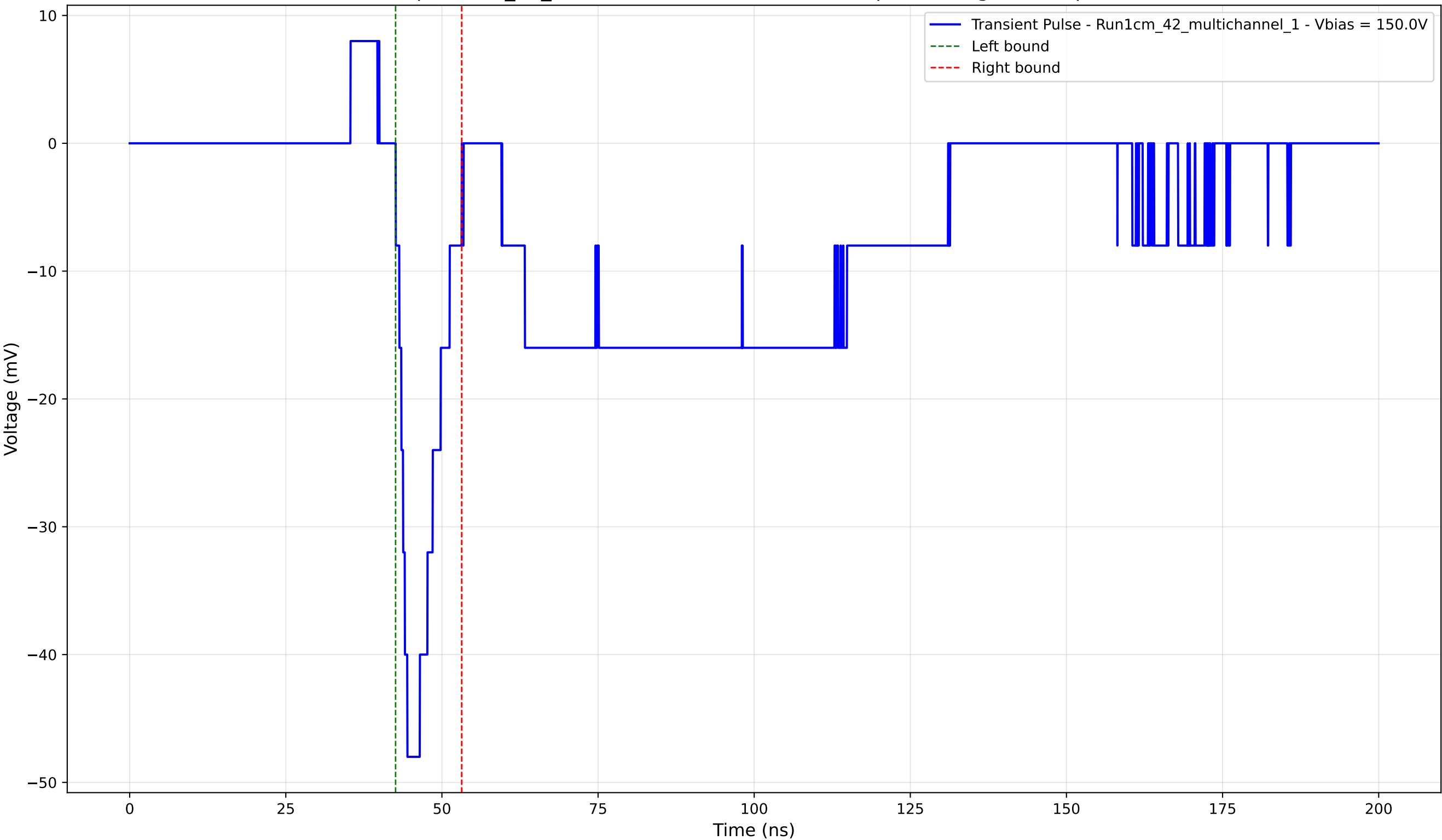
Transient Pulse - Sample: 1cm_42_multichannel - Position: 4155.0 \mu\text{m} - Charge: -5.64 pC - Rise Time: 1.87 ns
