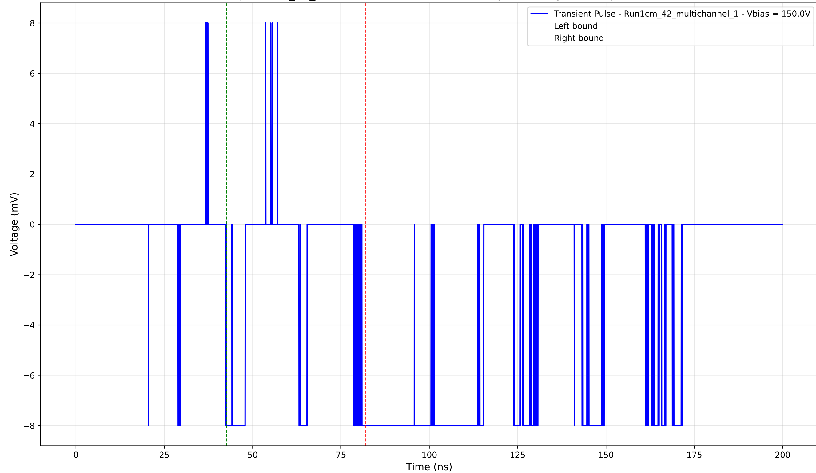
Transient Pulse - Sample: 1cm_42_multichannel - Position: 3915.0 \mu\text{m} - Charge: -1.53 pC - Rise Time: 0.02 ns
