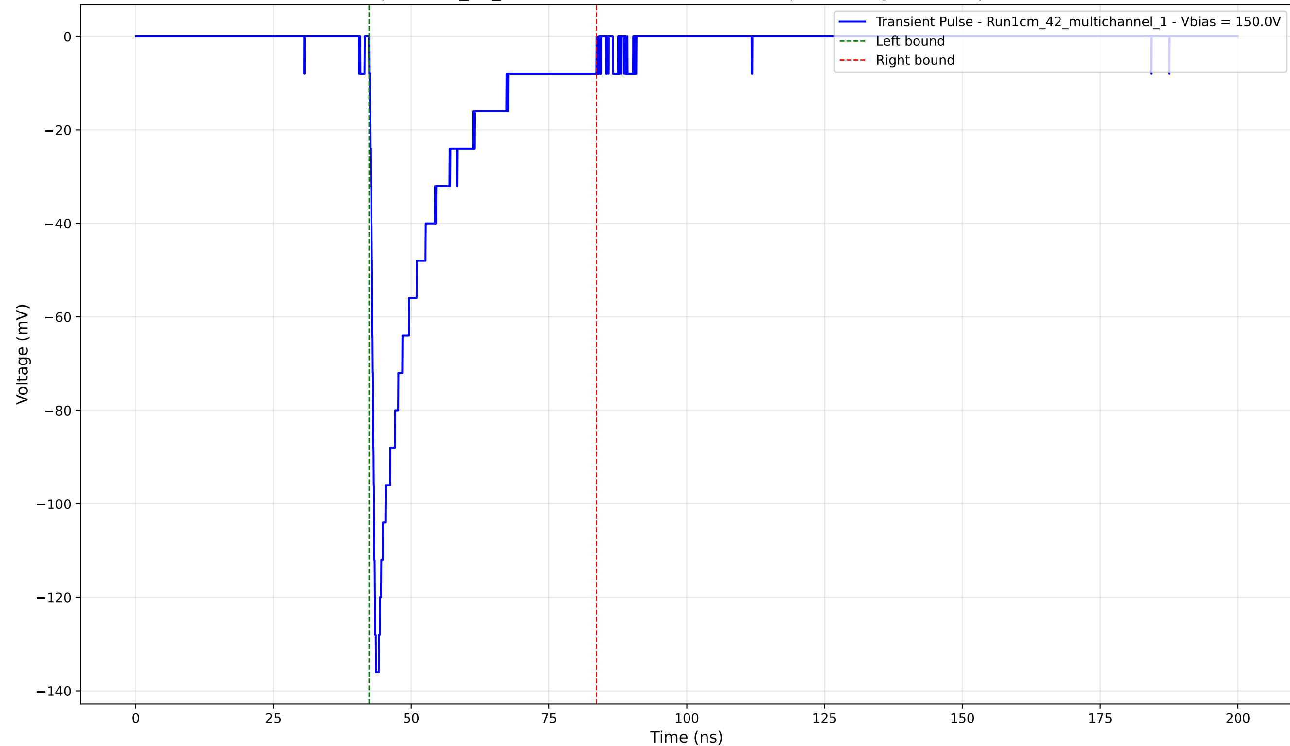
Transient Pulse - Sample: 1cm_42_multichannel - Position: 1570.0 \mu\text{m} - Charge: -25.42 pC - Rise Time: 0.97 ns
