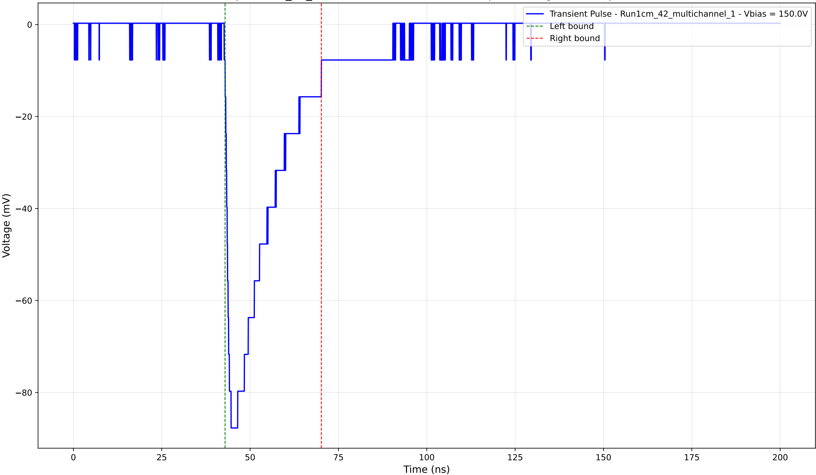
Transient Pulse - Sample: 1cm_42_multichannel - Position: 995.0 \mu\text{m} - Charge: -23.10 pC - Rise Time: 1.22 ns
