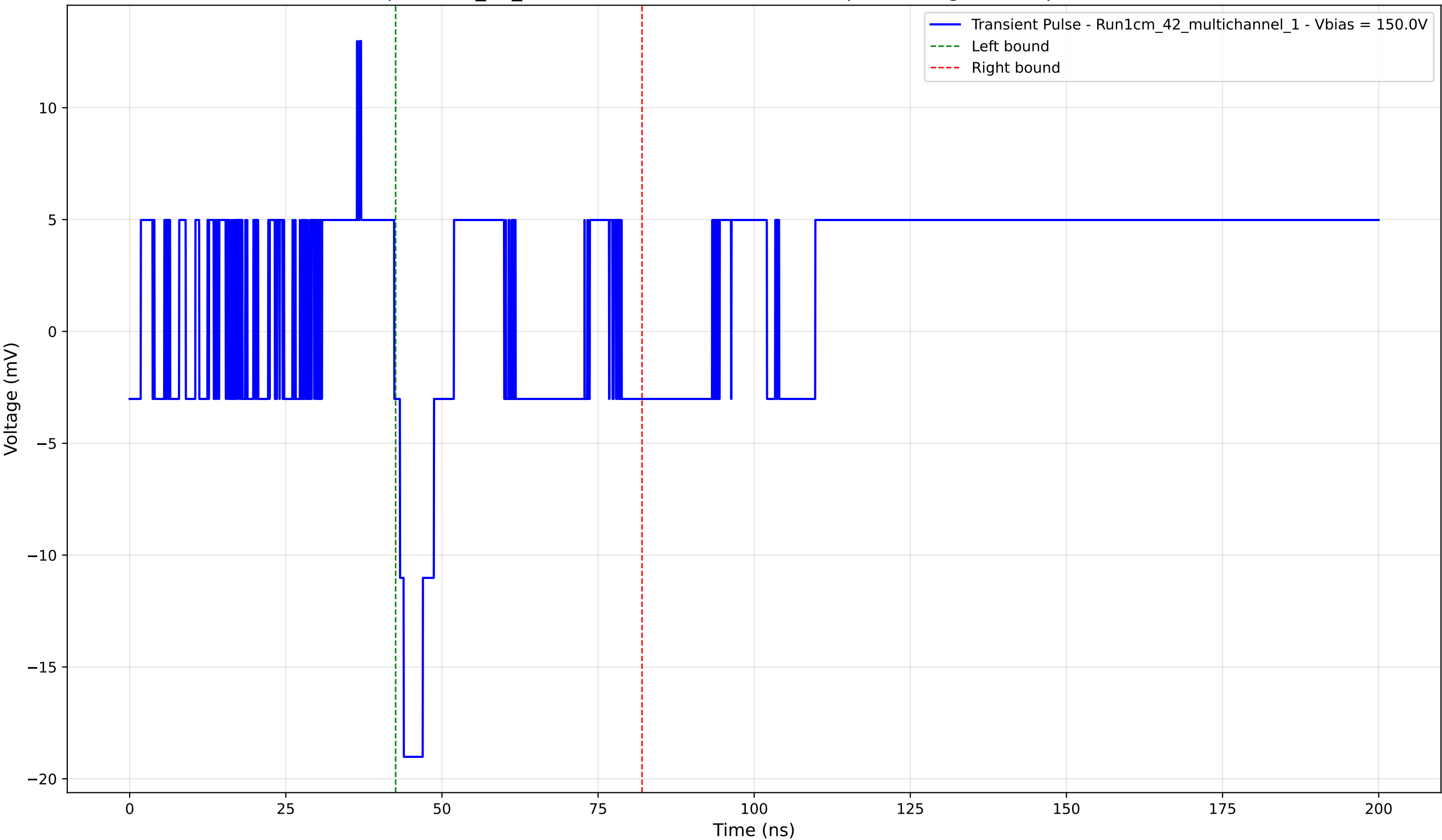
Transient Pulse - Sample: 1cm_42_multichannel - Position: 3860.0 \mu\text{m} - Charge: -1.66 pC - Rise Time: 0.00 ns (N/A)
