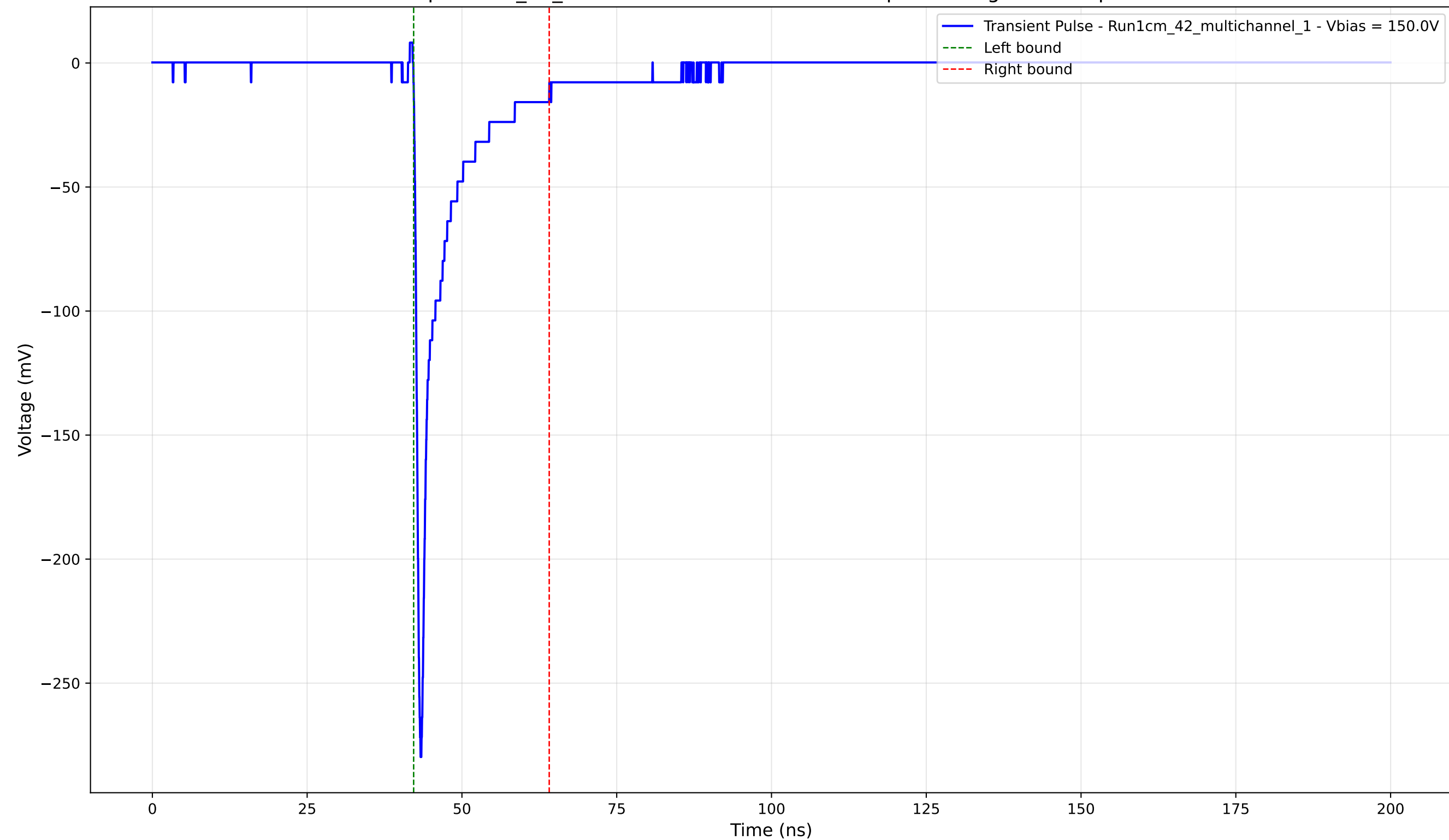
Transient Pulse - Sample: 1cm_42_multichannel - Position: 2040.0 \mu\text{m} - Charge: -23.72 pC - Rise Time: 0.81 ns
