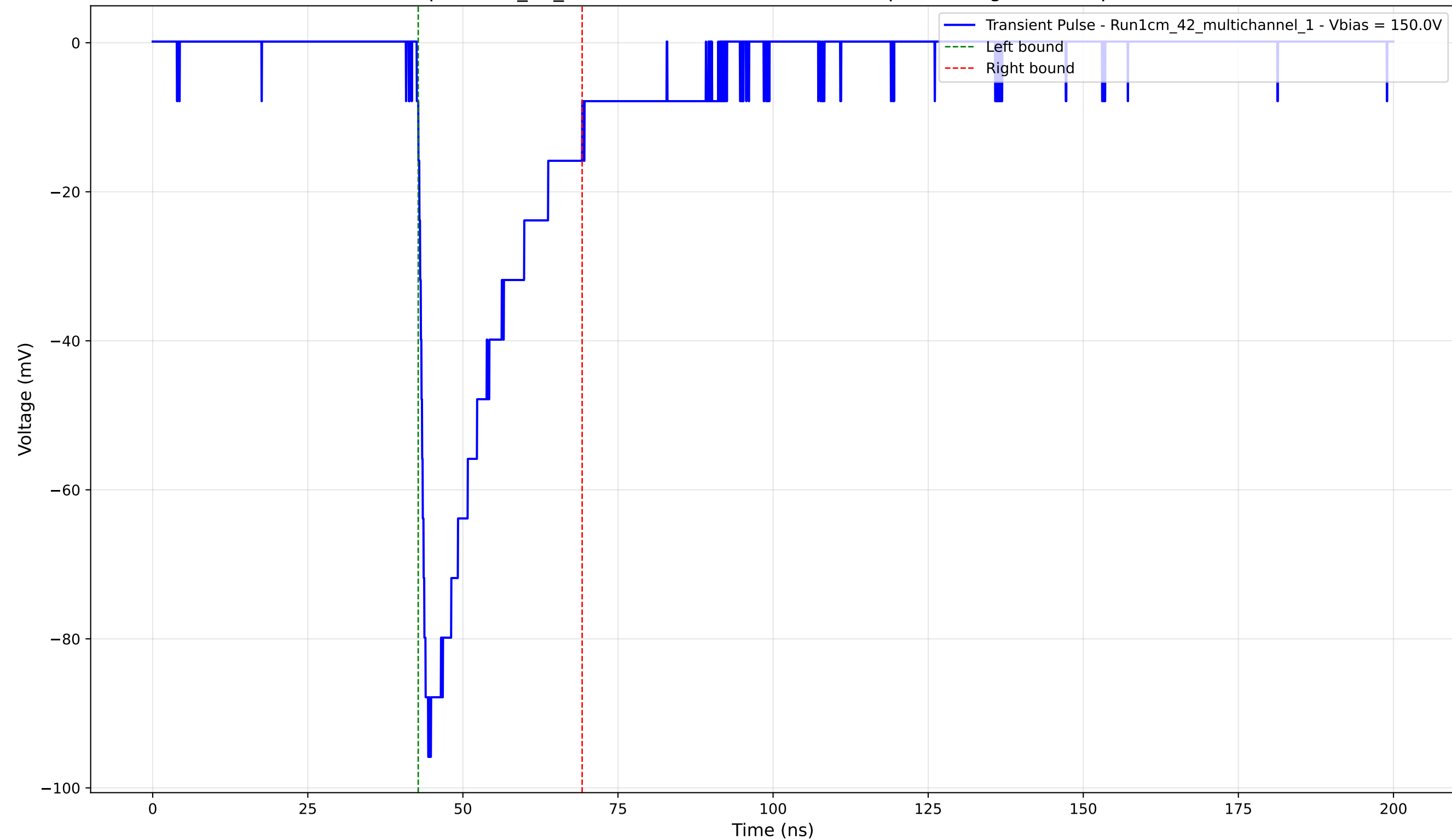
Transient Pulse - Sample: 1cm_42_multichannel - Position: 1155.0 \mu\text{m} - Charge: -22.85 pC - Rise Time: 1.18 ns
