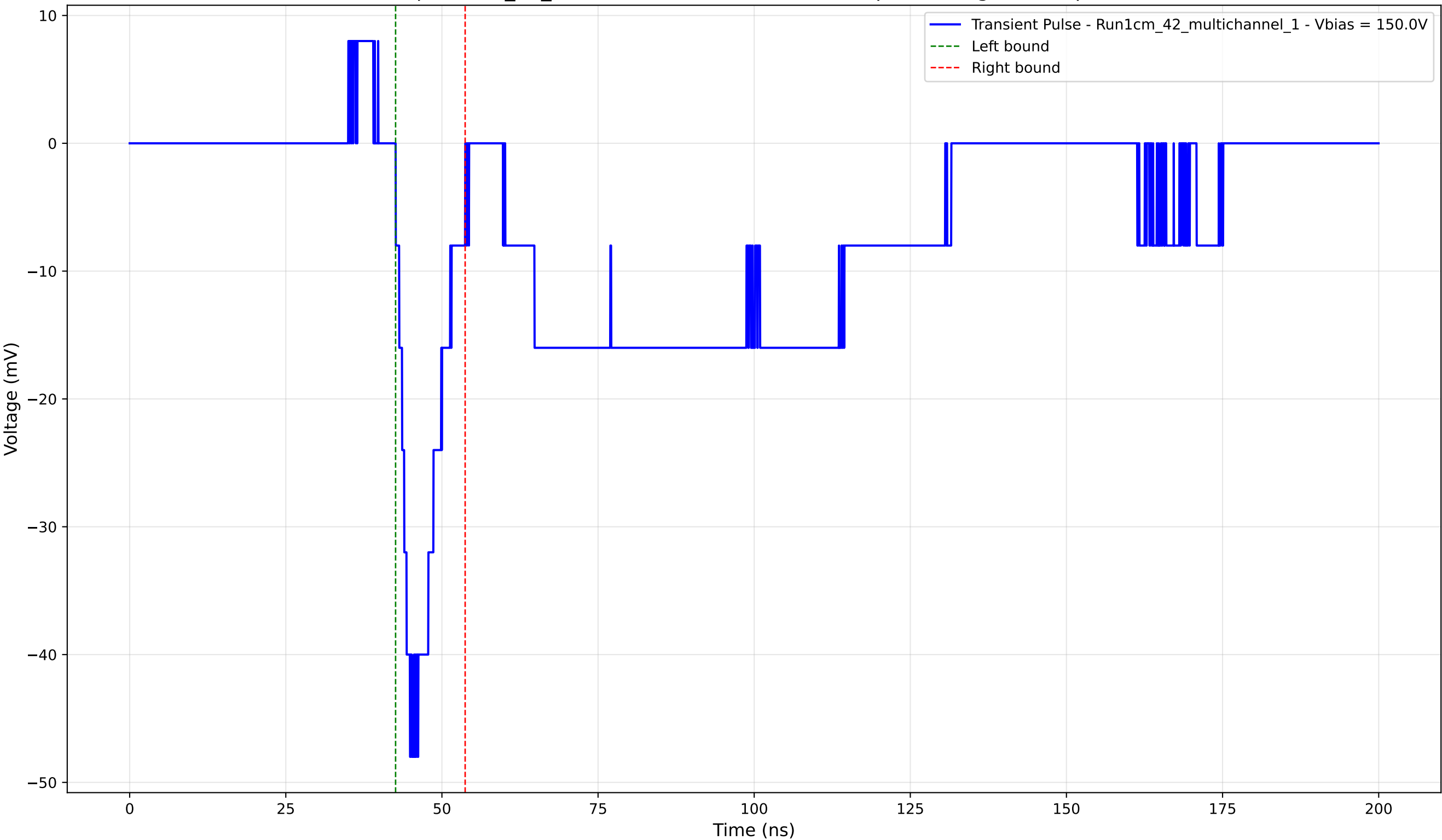
Transient Pulse - Sample: 1cm_42_multichannel - Position: 4495.0 \mu\text{m} - Charge: -5.54 pC - Rise Time: 2.29 ns
