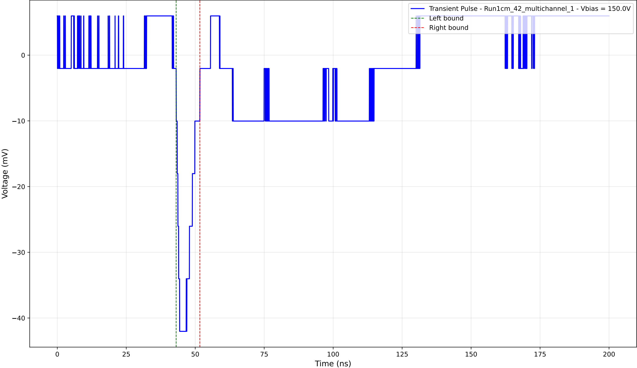
Transient Pulse - Sample: 1cm_42_multichannel - Position: 4135.0 \mu\text{m} - Charge: -4.61 pC - Rise Time: 1.25 ns
