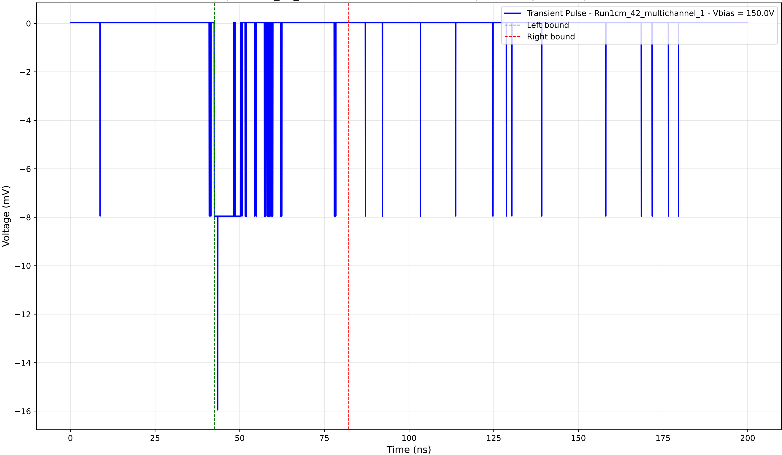
Transient Pulse - Sample: 1cm_42_multichannel - Position: 1890.0 \mu\text{m} - Charge: -1.51 pC - Rise Time: 1.04 ns
