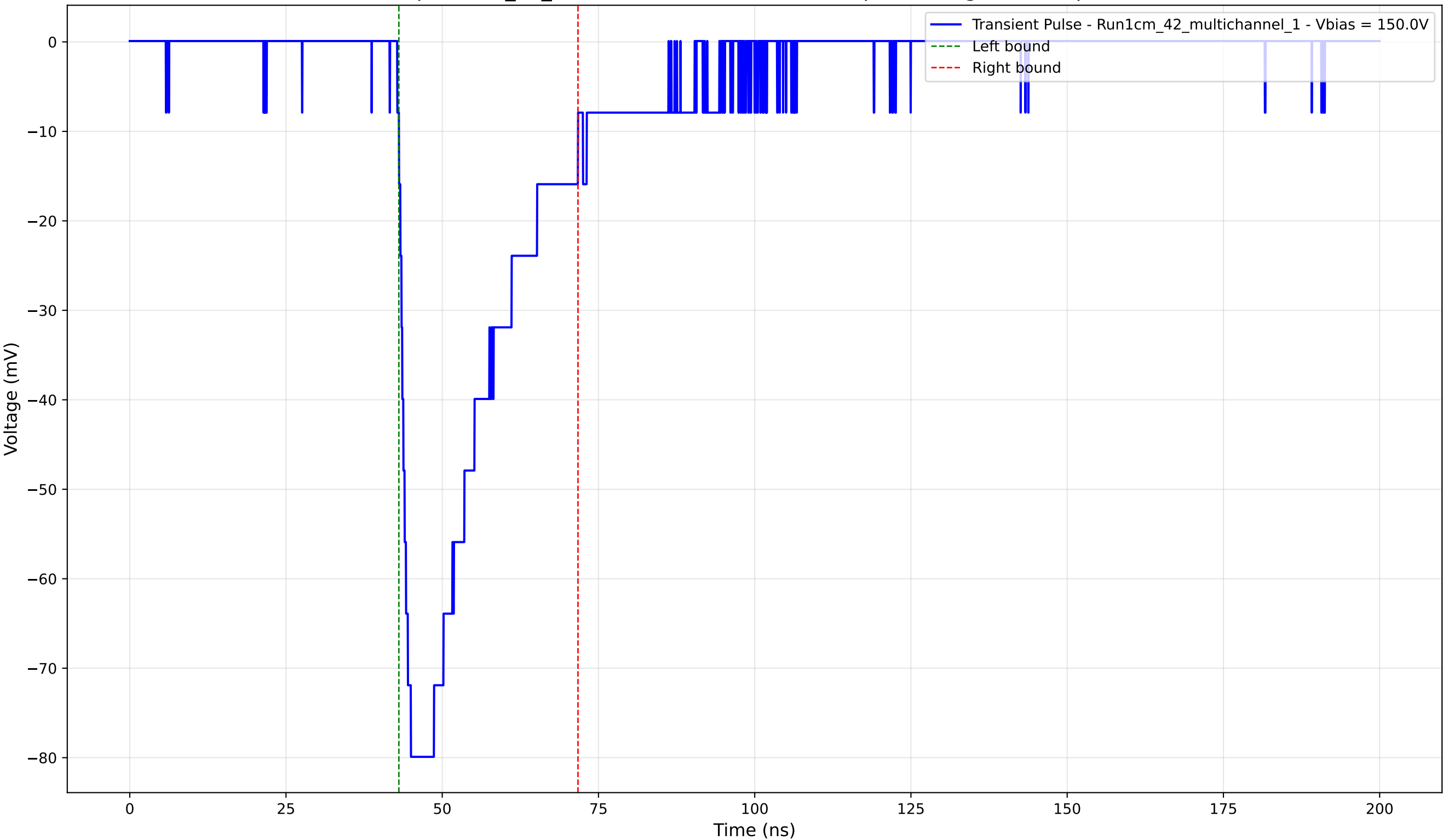
Transient Pulse - Sample: 1cm_42_multichannel - Position: 705.0 \mu\text{m} - Charge: -23.78 pC - Rise Time: 1.92 ns
