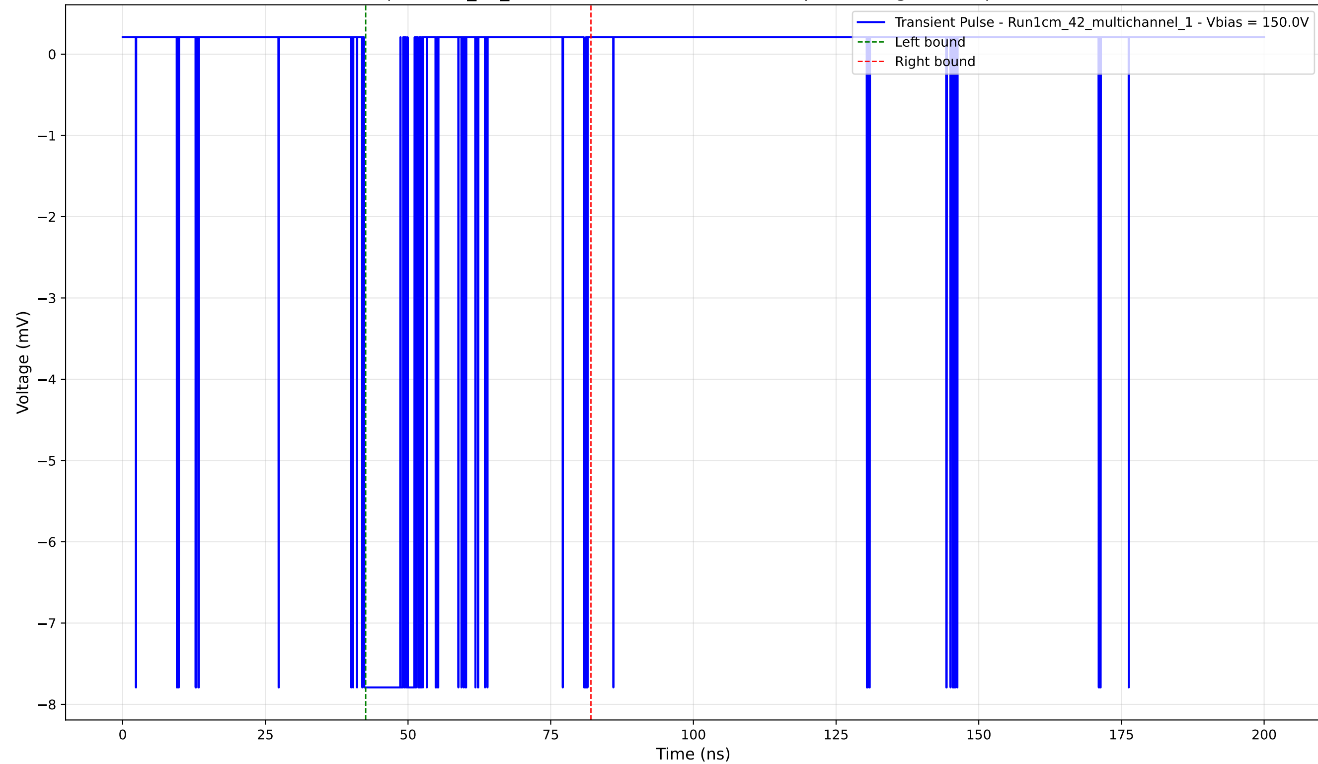
Transient Pulse - Sample: 1cm_42_multichannel - Position: 2905.0 \mu\text{m} - Charge: -1.41 pC - Rise Time: 0.02 ns
