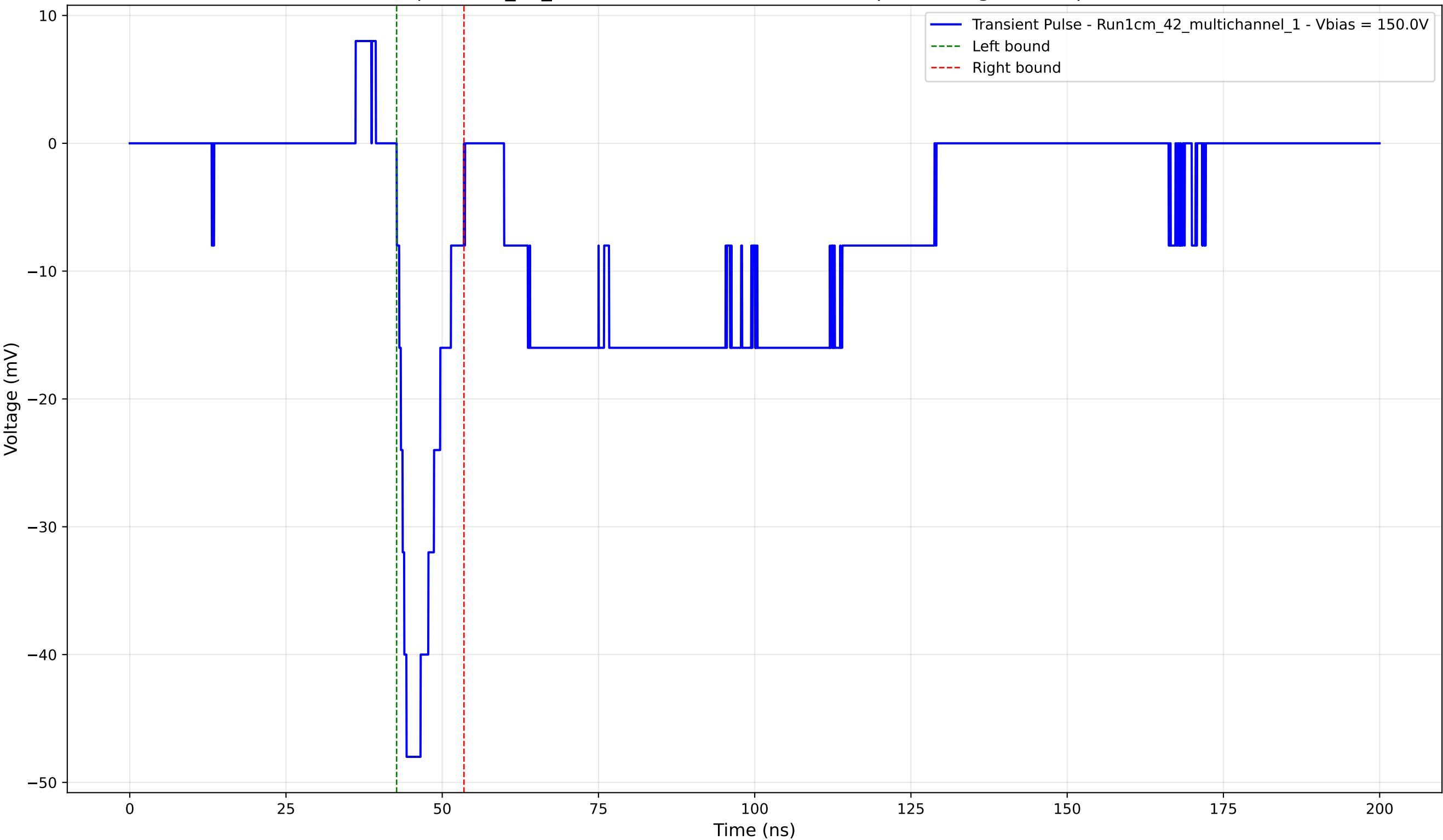
Transient Pulse - Sample: 1cm_42_multichannel - Position: 4070.0 \mu\text{m} - Charge: -5.84 pC - Rise Time: 1.57 ns
