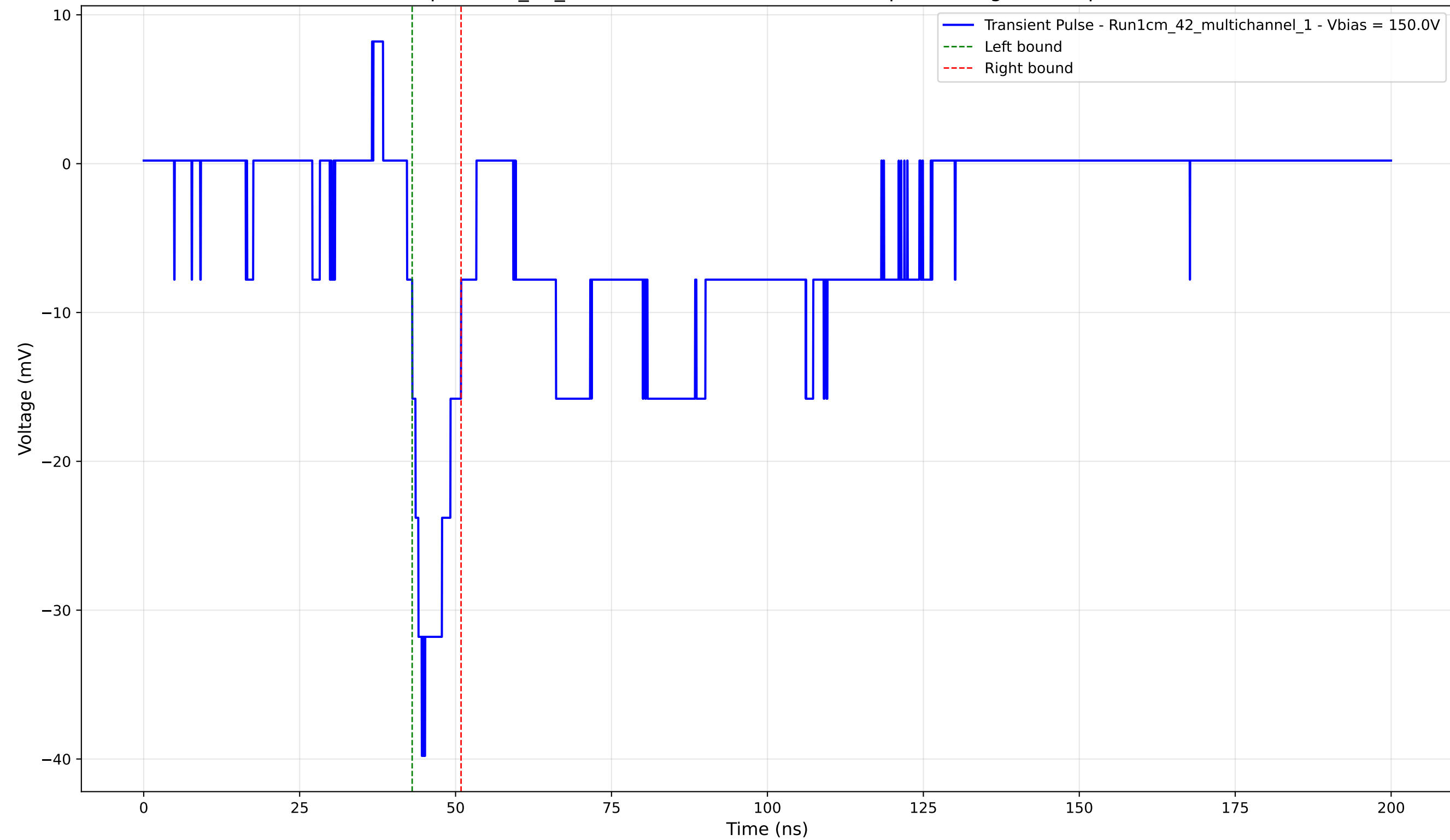
Transient Pulse - Sample: 1cm_42_multichannel - Position: 4830.0 \mu\text{m} - Charge: -4.02 pC - Rise Time: 2.37 ns
