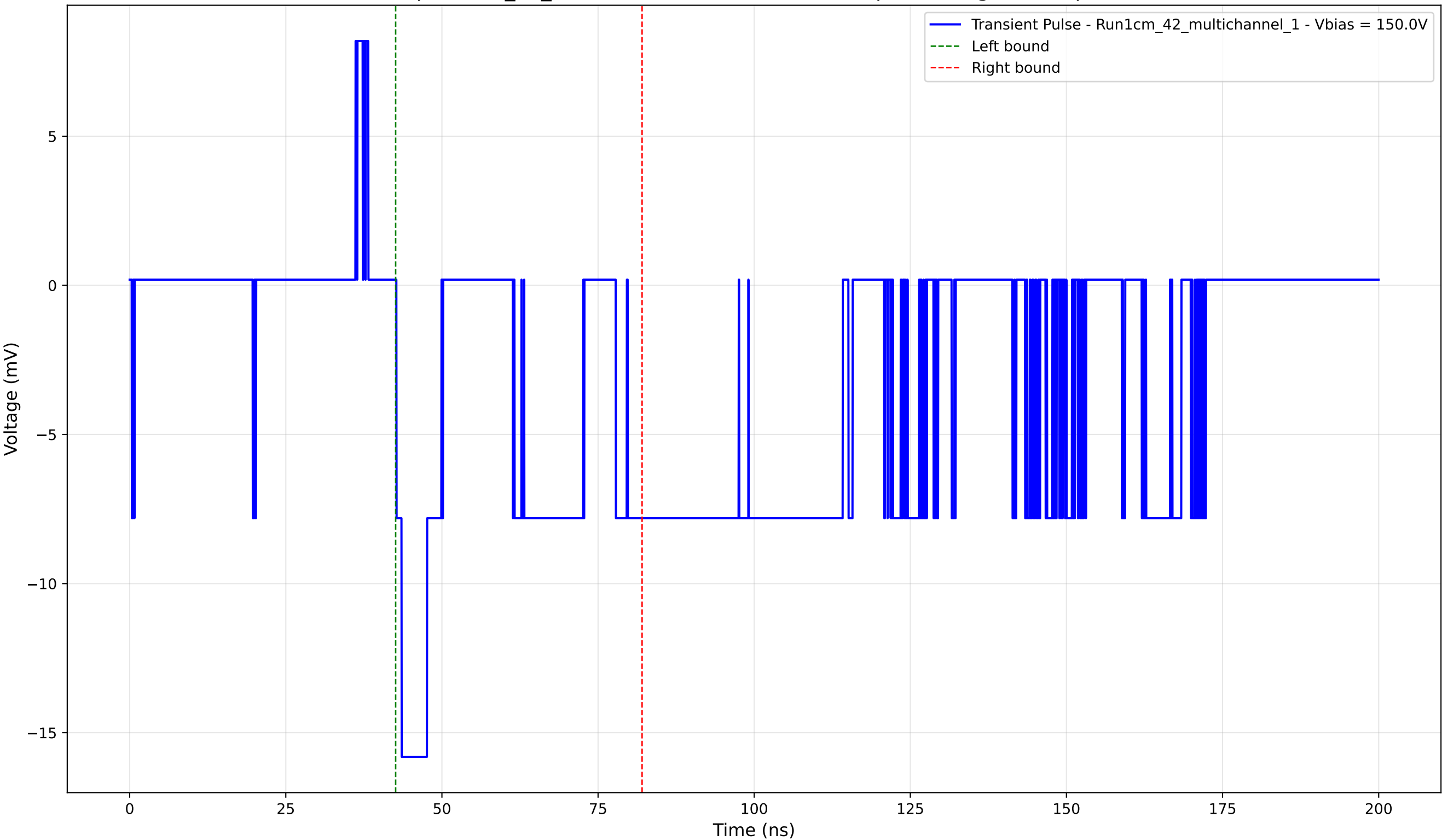
Transient Pulse - Sample: 1cm_42_multichannel - Position: 3865.0 \mu\text{m} - Charge: -4.10 pC - Rise Time: 0.84 ns
