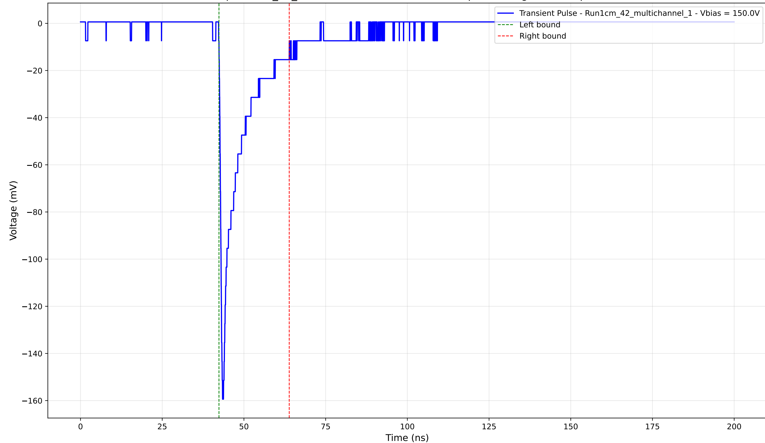
Transient Pulse - Sample: 1cm_42_multichannel - Position: 3030.0 \mu\text{m} - Charge: -19.50 pC - Rise Time: 0.90 ns
