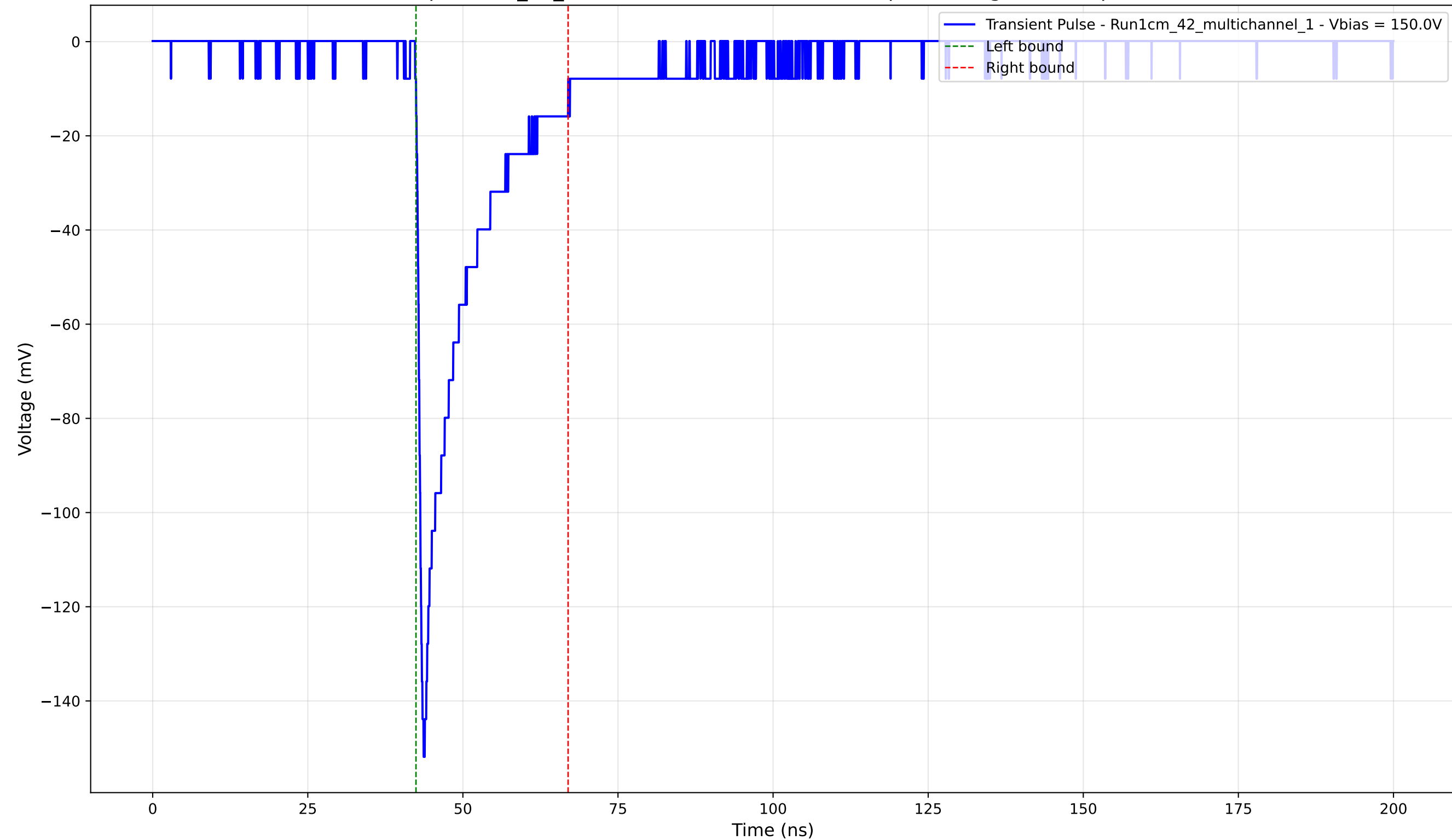
Transient Pulse - Sample: 1cm_42_multichannel - Position: 1630.0 \mu\text{m} - Charge: -22.96 pC - Rise Time: 1.02 ns
