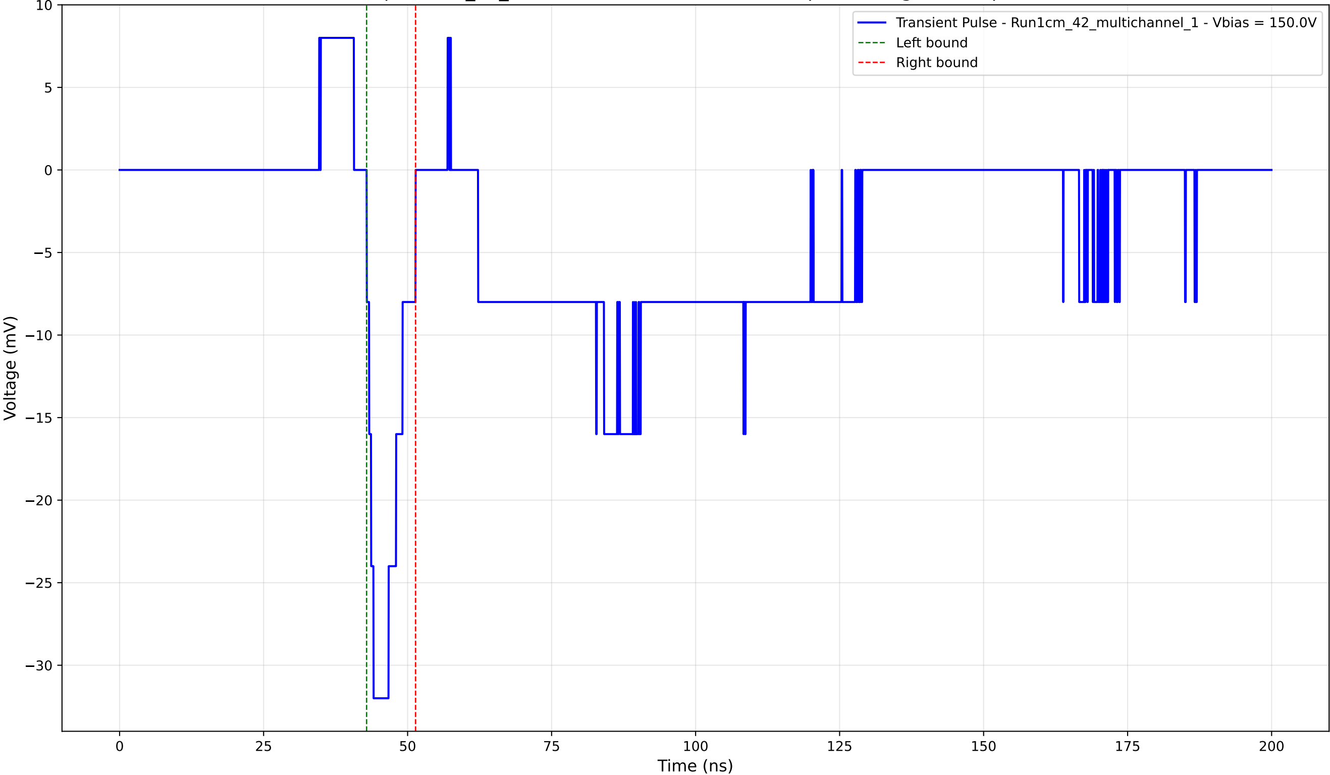
Transient Pulse - Sample: 1cm_42_multichannel - Position: 3960.0 \mu\text{m} - Charge: -3.40 pC - Rise Time: 1.19 ns
