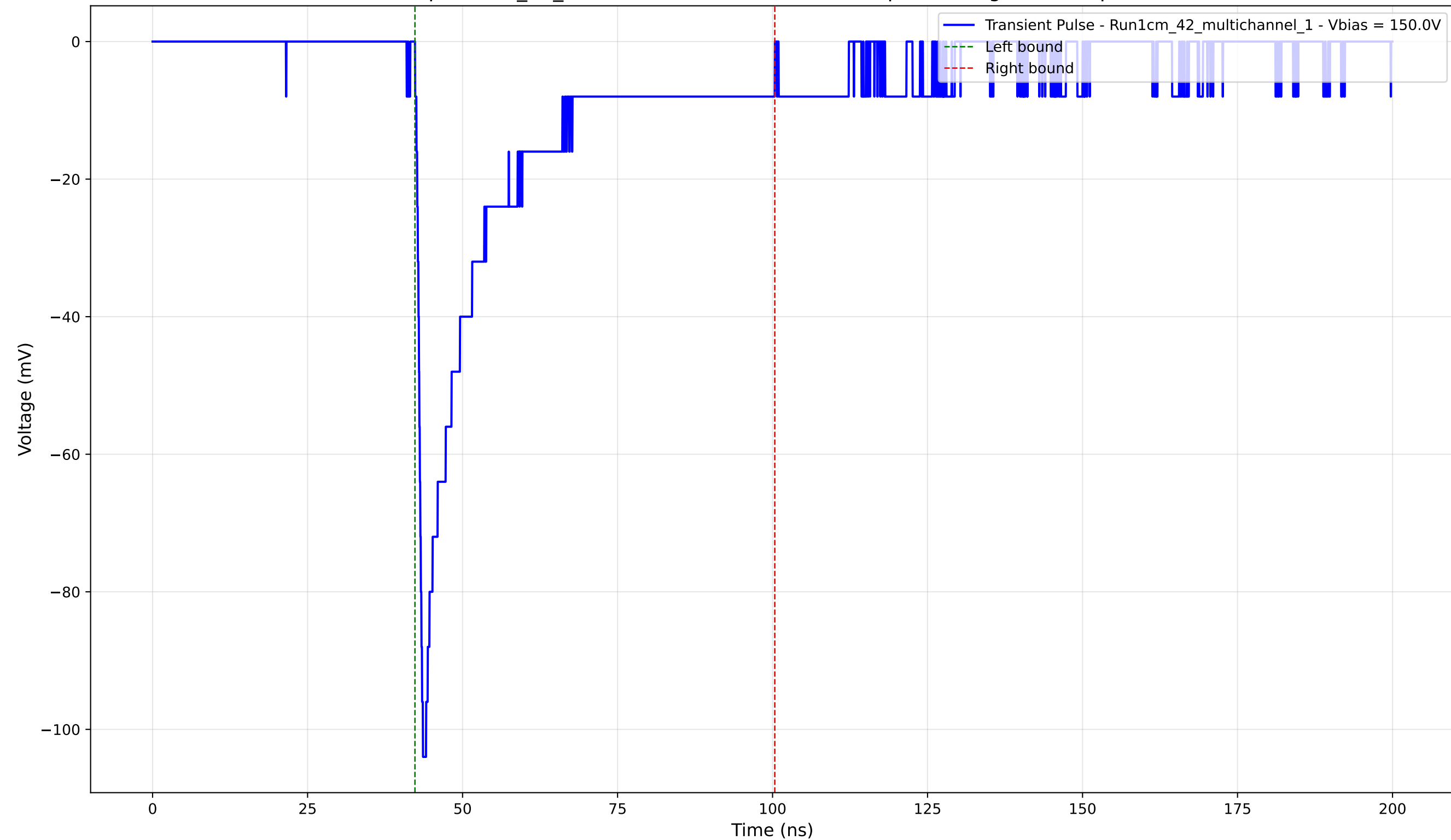
Transient Pulse - Sample: 1cm_42_multichannel - Position: 3290.0 \mu\text{m} - Charge: -22.64 pC - Rise Time: 0.91 ns
