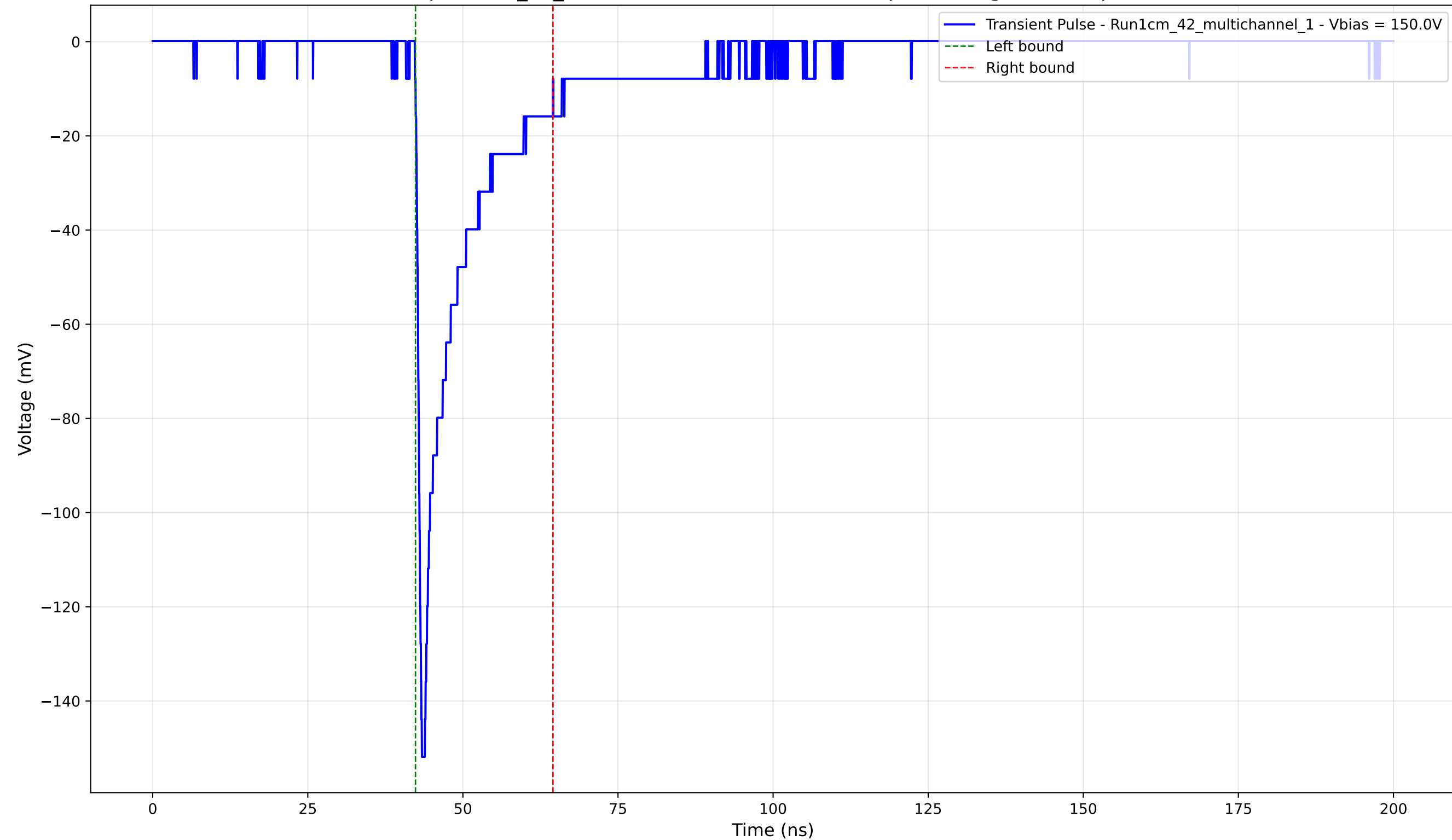
Transient Pulse - Sample: 1cm_42_multichannel - Position: 3045.0 \mu\text{m} - Charge: -19.78 pC - Rise Time: 0.92 ns
