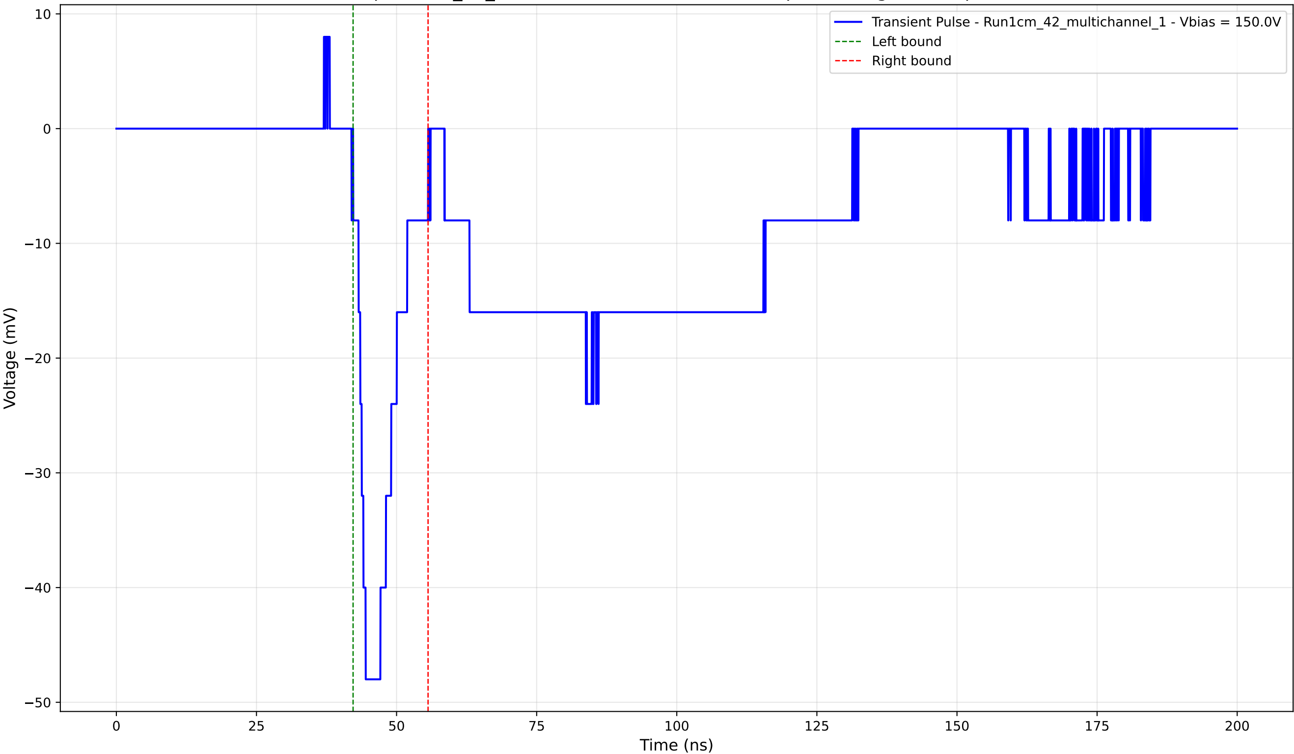
Transient Pulse - Sample: 1cm_42_multichannel - Position: 4270.0 \mu\text{m} - Charge: -6.48 pC - Rise Time: 2.23 ns
