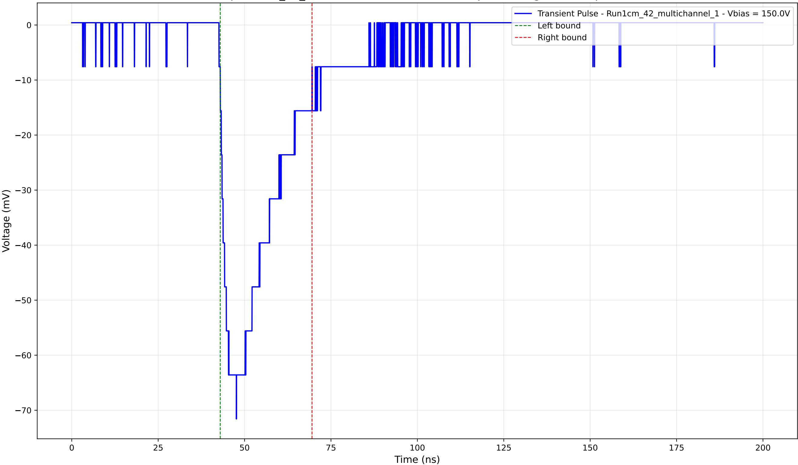
Transient Pulse - Sample: 1cm_42_multichannel - Position: 205.0 \mu\text{m} - Charge: -20.12 pC - Rise Time: 5.04 ns
