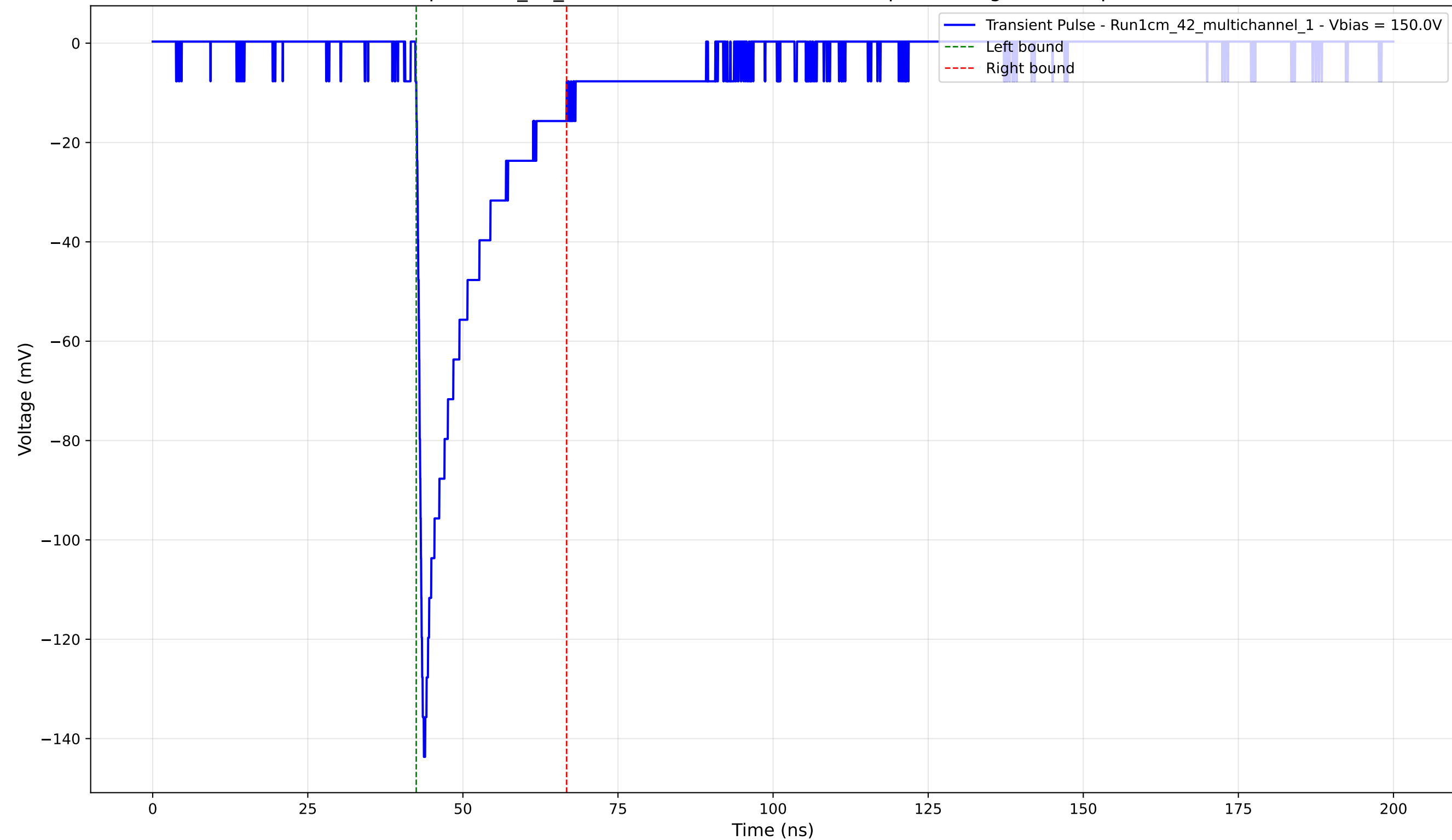
Transient Pulse - Sample: 1cm_42_multichannel - Position: 1590.0 \mu\text{m} - Charge: -22.53 pC - Rise Time: 1.02 ns
