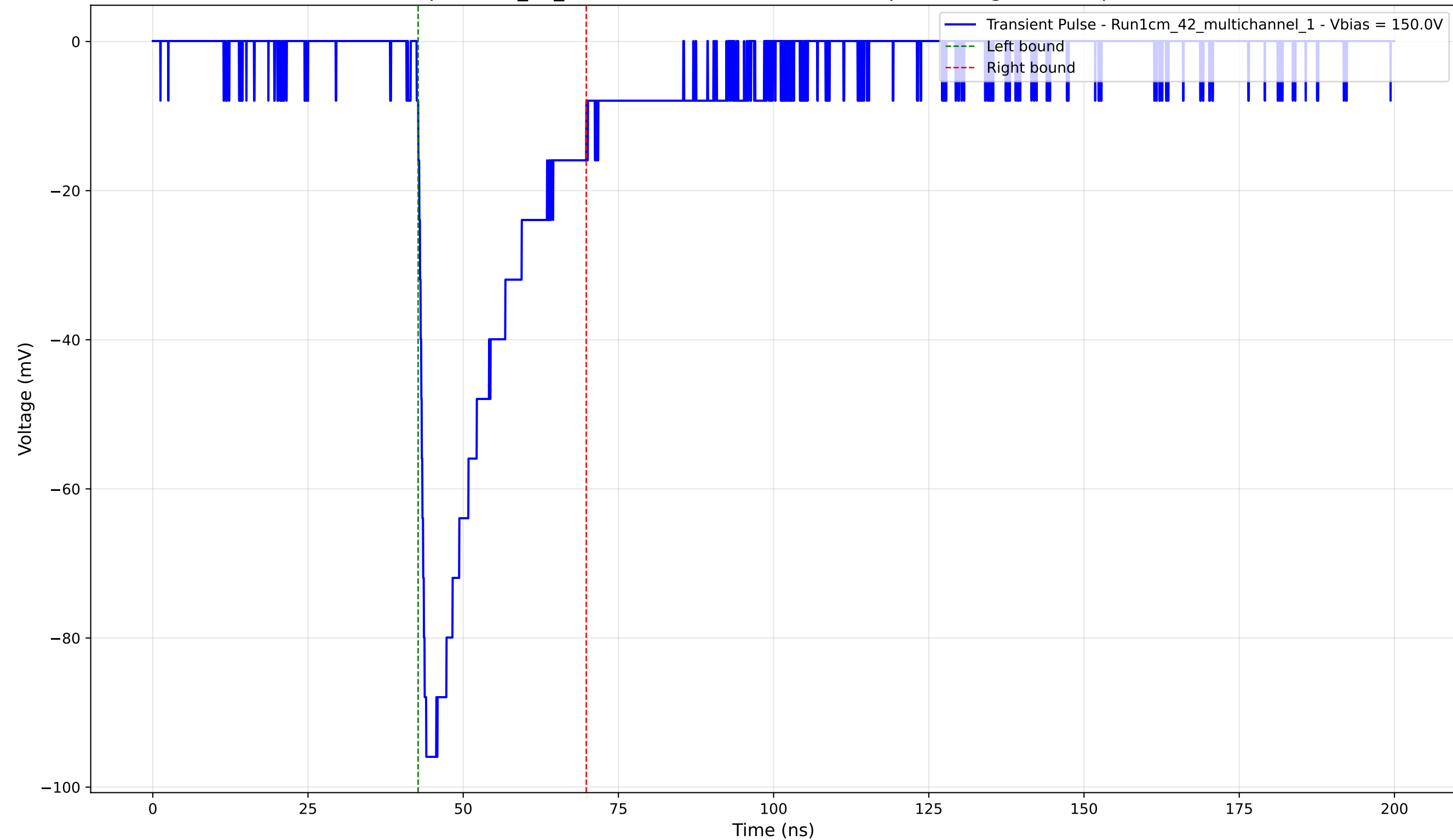
Transient Pulse - Sample: 1cm_42_multichannel - Position: 1205.0 \mu\text{m} - Charge: -23.70 pC - Rise Time: 1.04 ns
