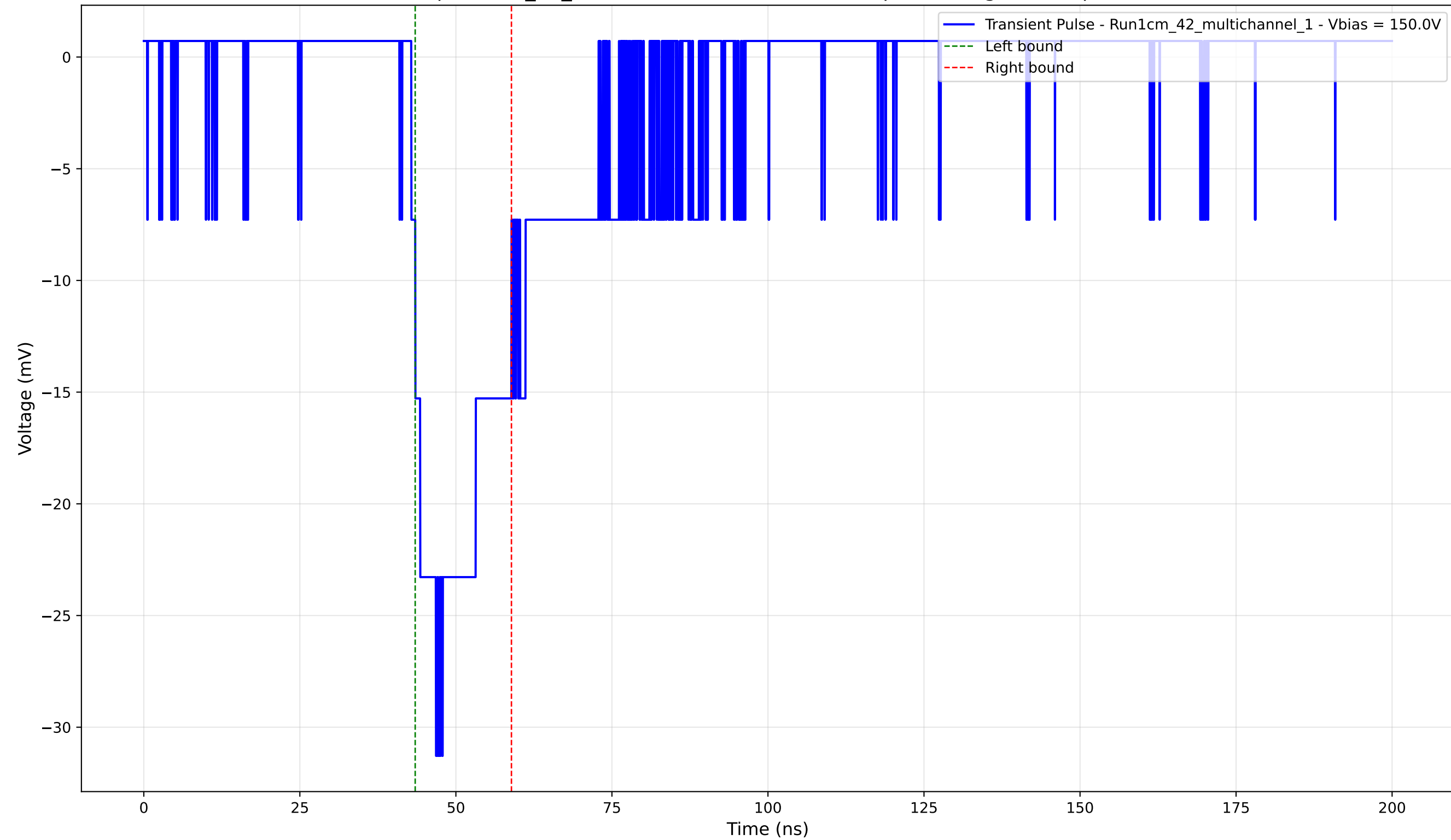
Transient Pulse - Sample: 1cm_42_multichannel - Position: 315.0 \mu\text{m} - Charge: -6.23 pC - Rise Time: 3.95 ns
