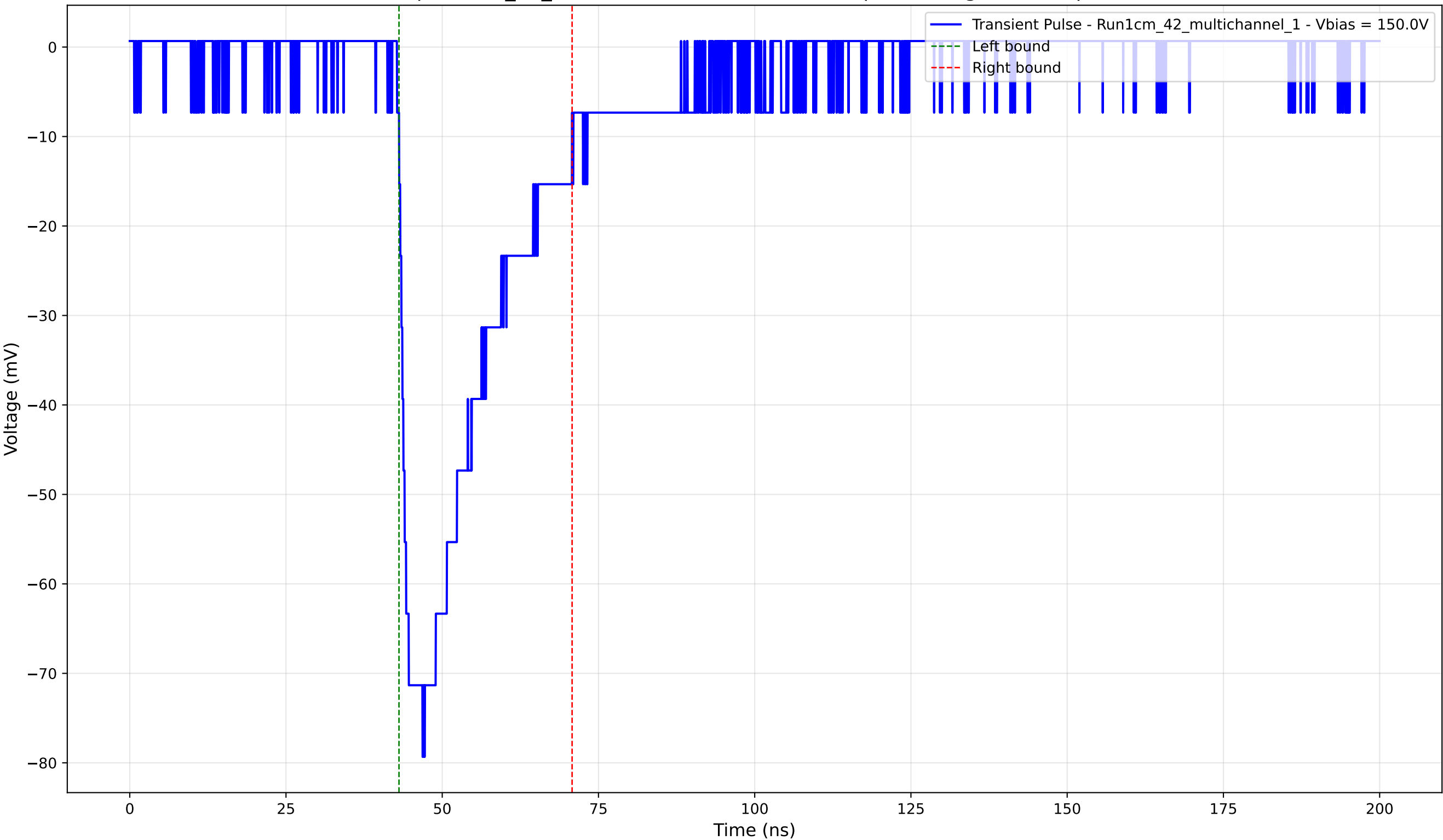
Transient Pulse - Sample: 1cm_42_multichannel - Position: 785.0 \mu\text{m} - Charge: -21.47 pC - Rise Time: 3.76 ns
