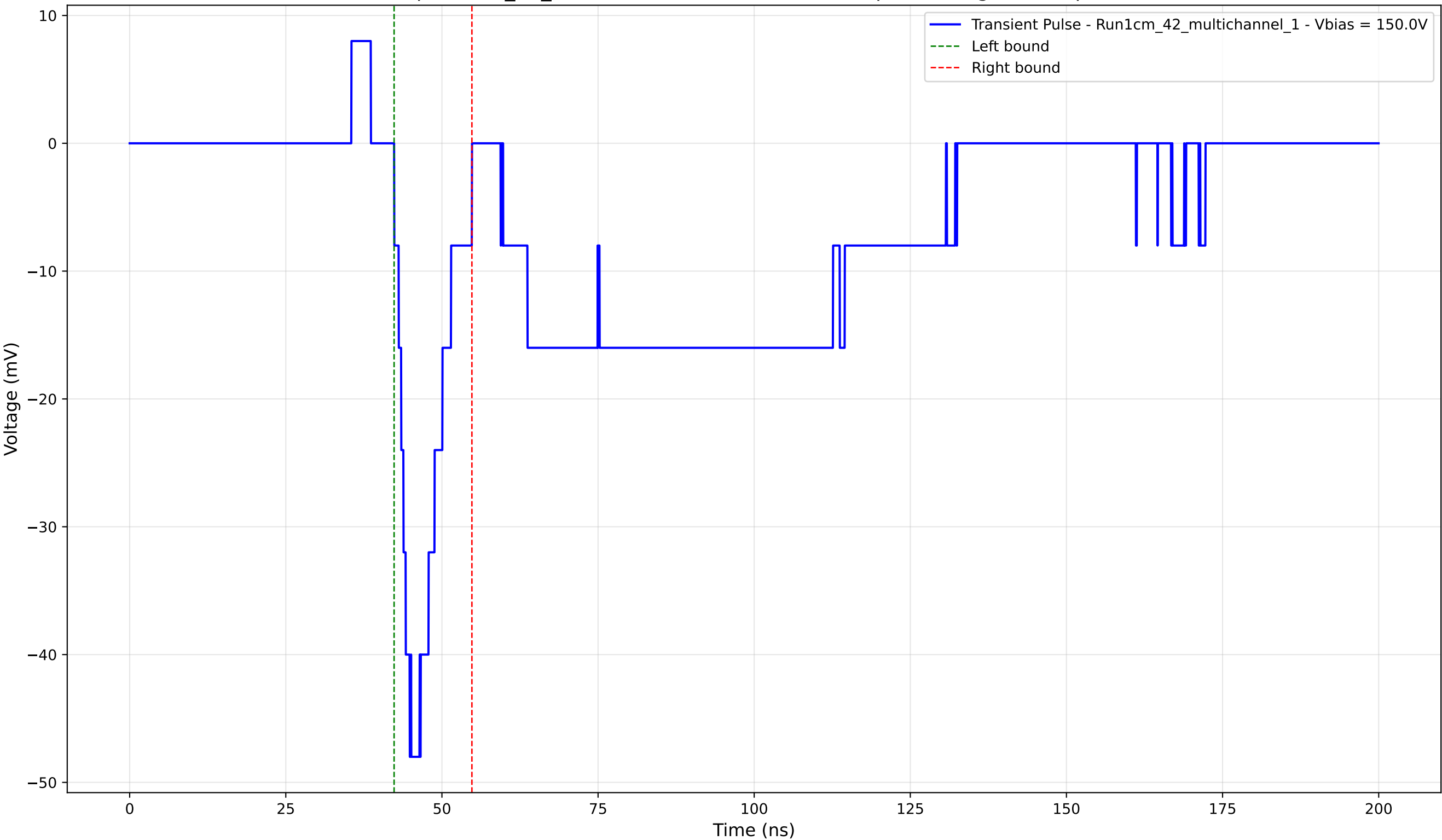
Transient Pulse - Sample: 1cm_42_multichannel - Position: 4640.0 \mu\text{m} - Charge: -6.03 pC - Rise Time: 2.49 ns
