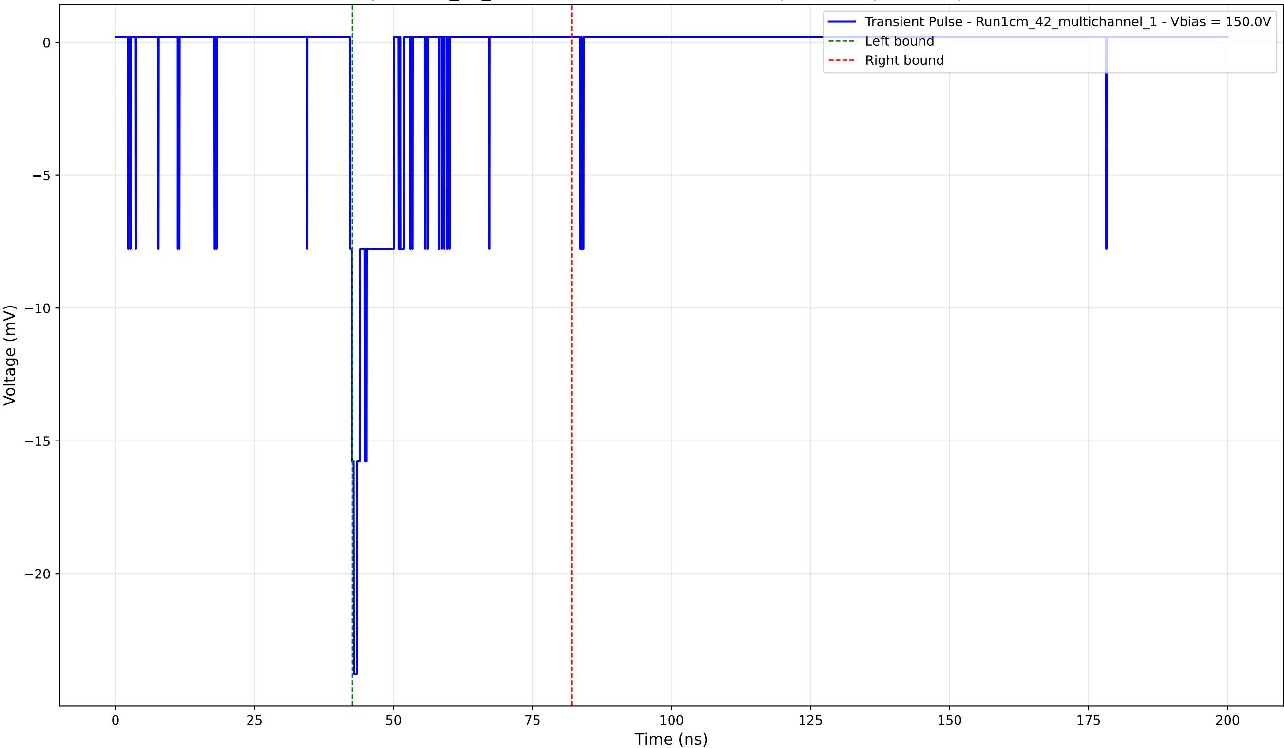
Transient Pulse - Sample: 1cm_42_multichannel - Position: 2370.0 \mu\text{m} - Charge: -1.63 pC - Rise Time: 0.63 ns
