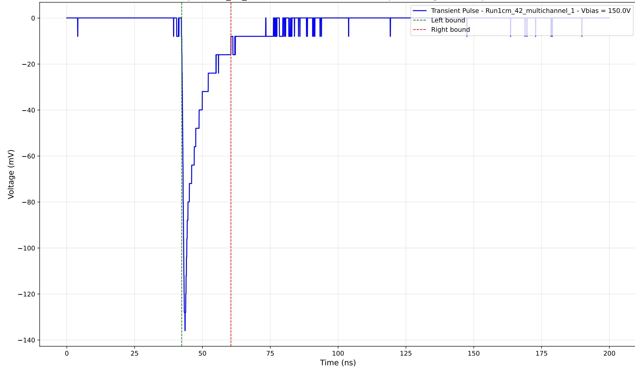
Transient Pulse - Sample: 1cm_42_multichannel - Position: 1820.0 \mu\text{m} - Charge: -14.83 pC - Rise Time: 0.93 ns
