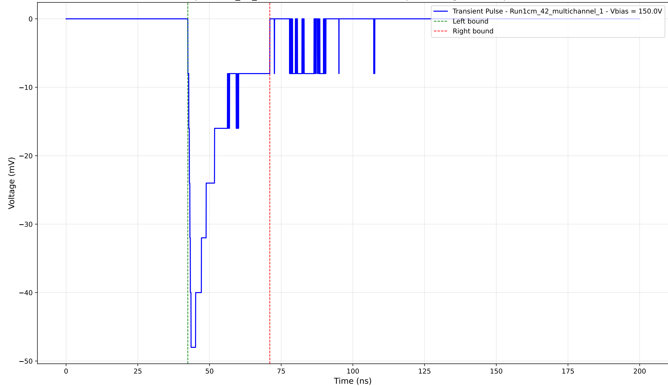
Transient Pulse - Sample: 1cm_42_multichannel - Position: 3455.0 \mu\text{m} - Charge: -10.04 pC - Rise Time: 1.11 ns
