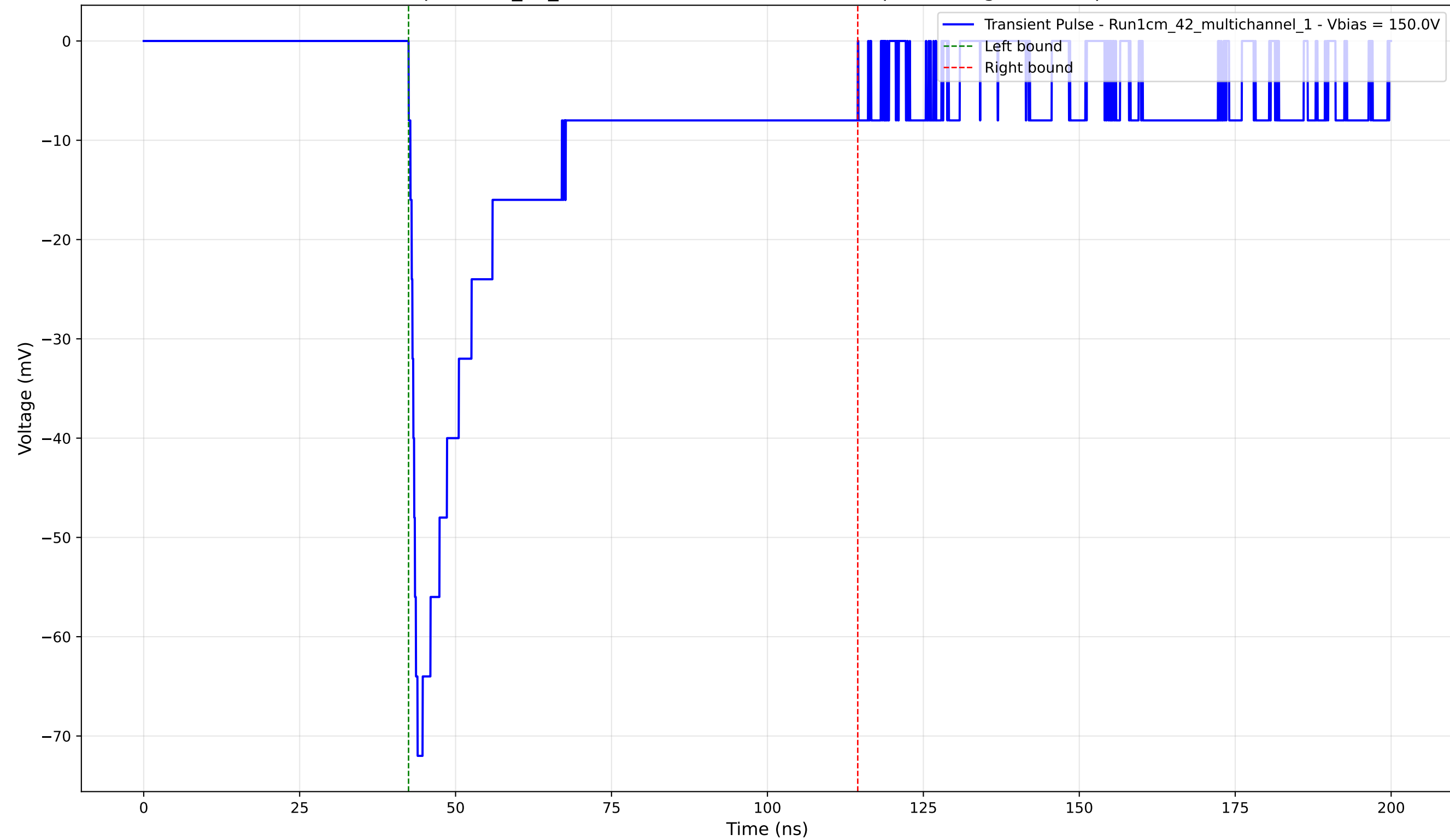
Transient Pulse - Sample: 1cm_42_multichannel - Position: 3595.0 \mu\text{m} - Charge: -22.18 pC - Rise Time: 1.42 ns
