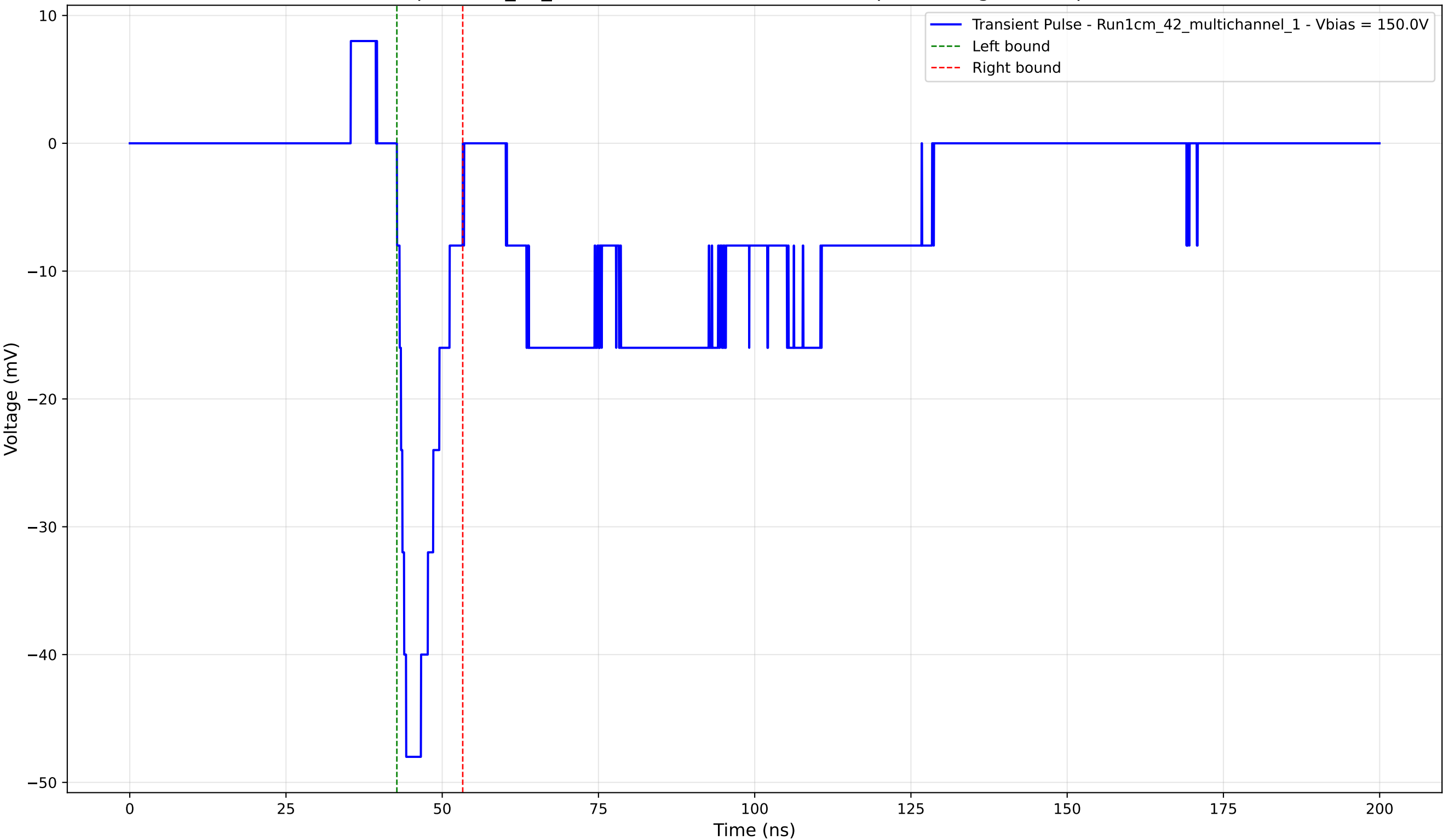
Transient Pulse - Sample: 1cm_42_multichannel - Position: 4025.0 \mu\text{m} - Charge: -5.72 pC - Rise Time: 1.47 ns
