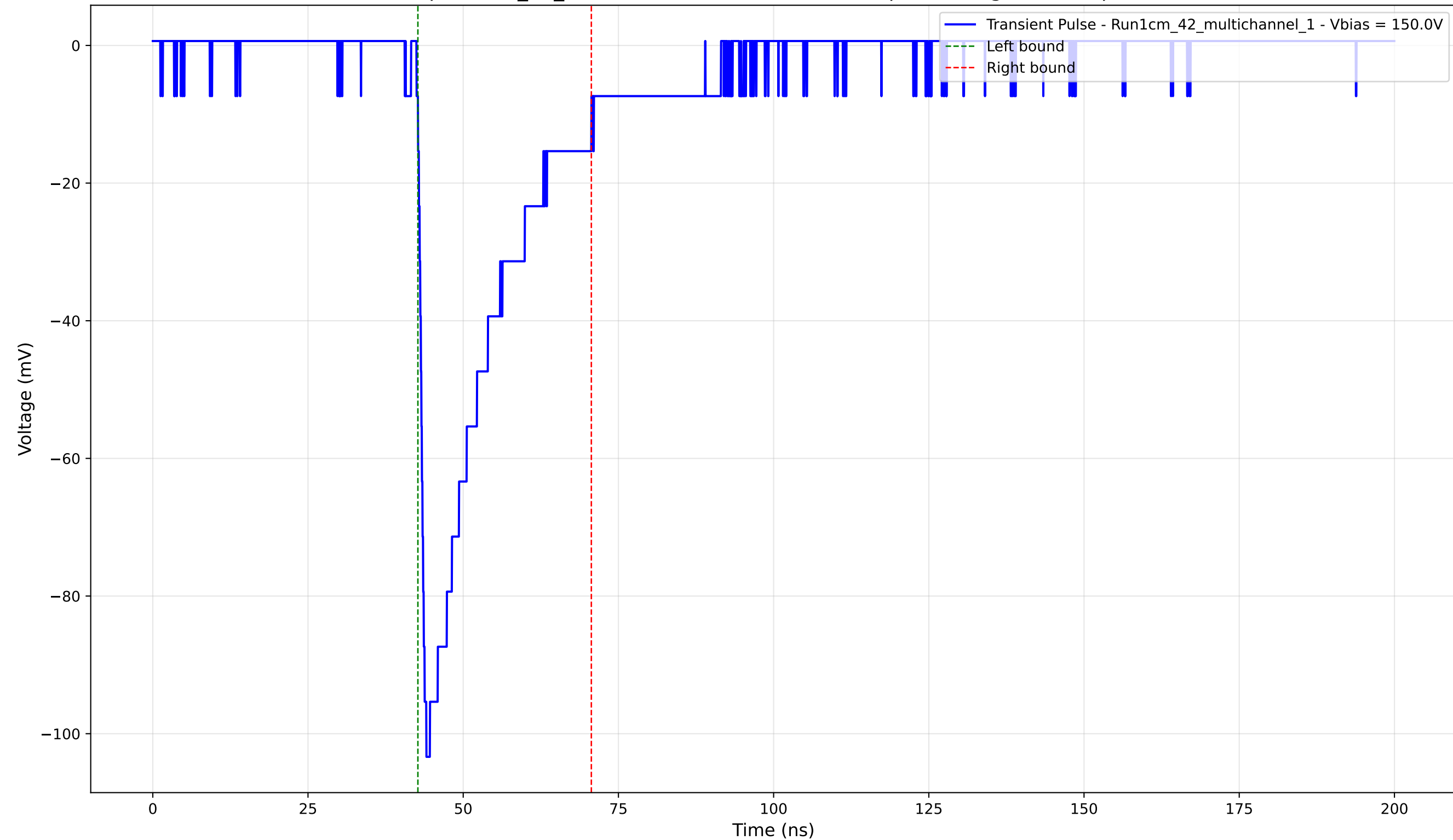
Transient Pulse - Sample: 1cm_42_multichannel - Position: 1260.0 \mu\text{m} - Charge: -23.66 pC - Rise Time: 1.07 ns
