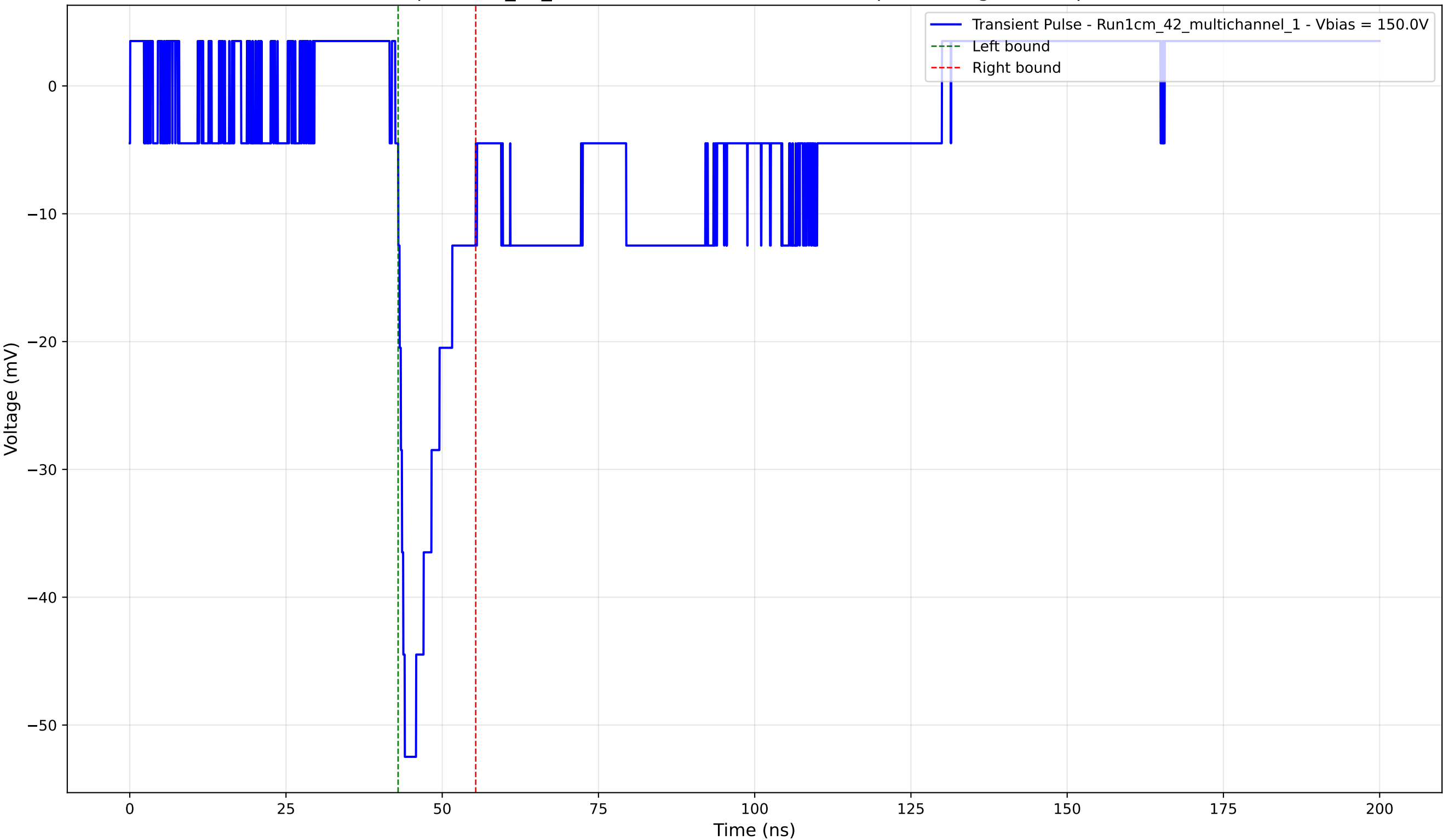
Transient Pulse - Sample: 1cm_42_multichannel - Position: 3820.0 \mu\text{m} - Charge: -7.00 pC - Rise Time: 1.06 ns
