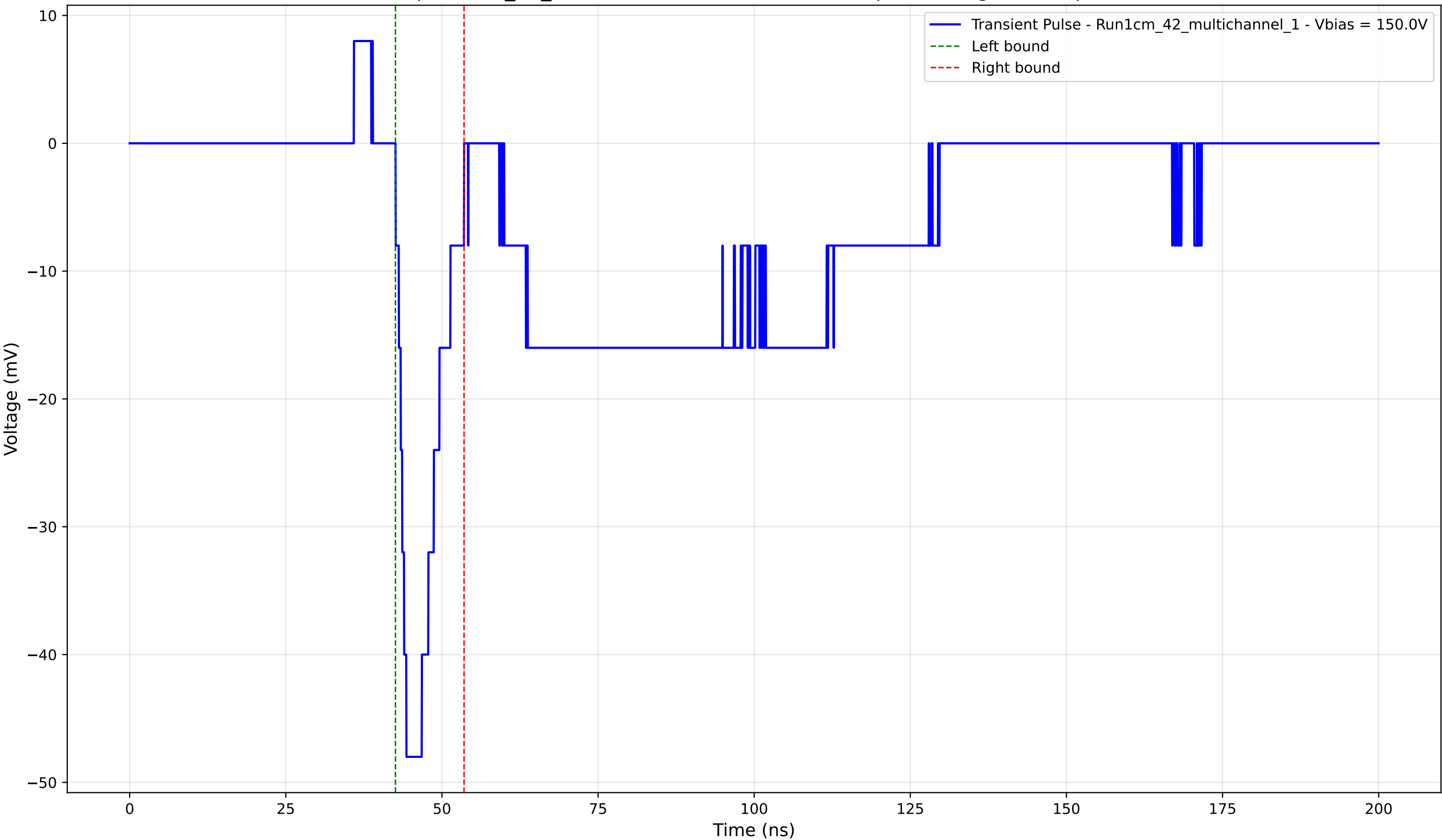
Transient Pulse - Sample: 1cm_42_multichannel - Position: 4075.0 \mu\text{m} - Charge: -5.89 pC - Rise Time: 1.73 ns
