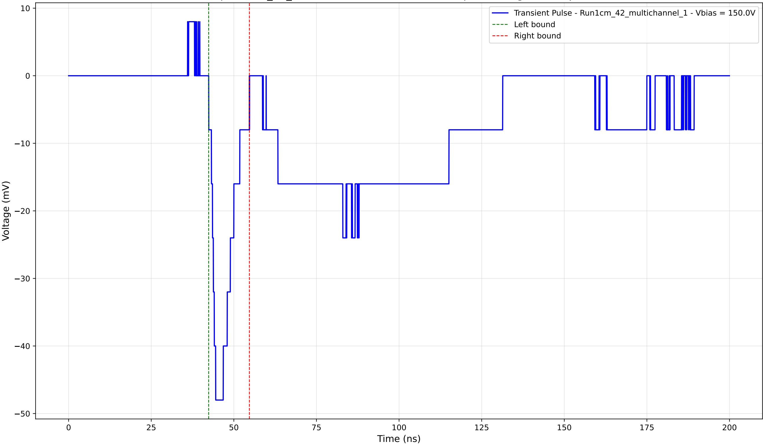
Transient Pulse - Sample: 1cm_42_multichannel - Position: 4255.0 \mu\text{m} - Charge: -6.19 pC - Rise Time: 2.11 ns
