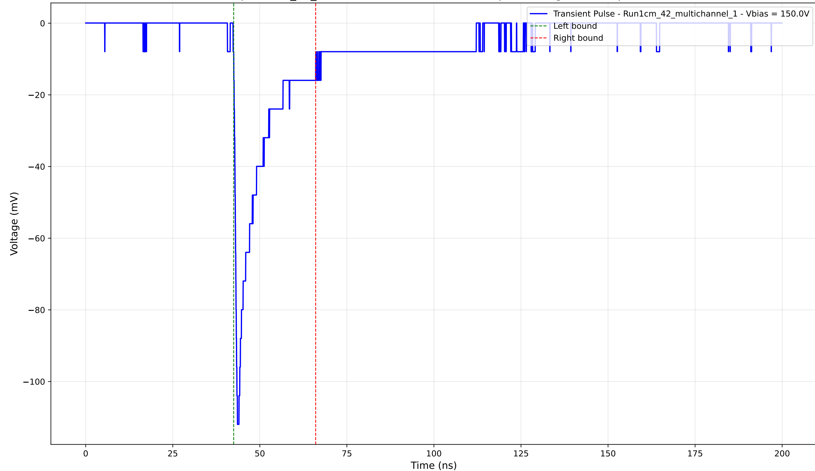
Transient Pulse - Sample: 1cm_42_multichannel - Position: 3230.0 \mu\text{m} - Charge: -16.52 pC - Rise Time: 0.91 ns
