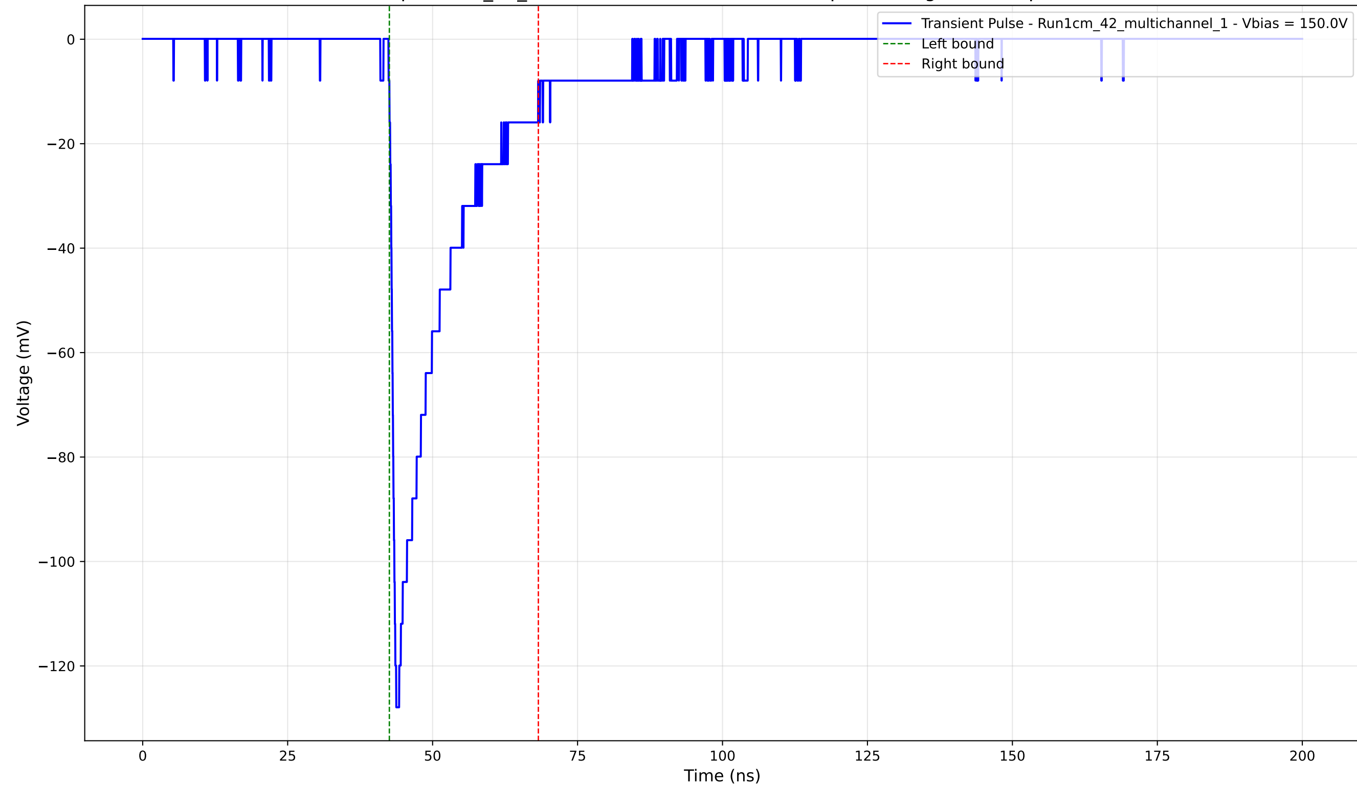
Transient Pulse - Sample: 1cm_42_multichannel - Position: 1490.0 \mu\text{m} - Charge: -23.41 pC - Rise Time: 1.01 ns
