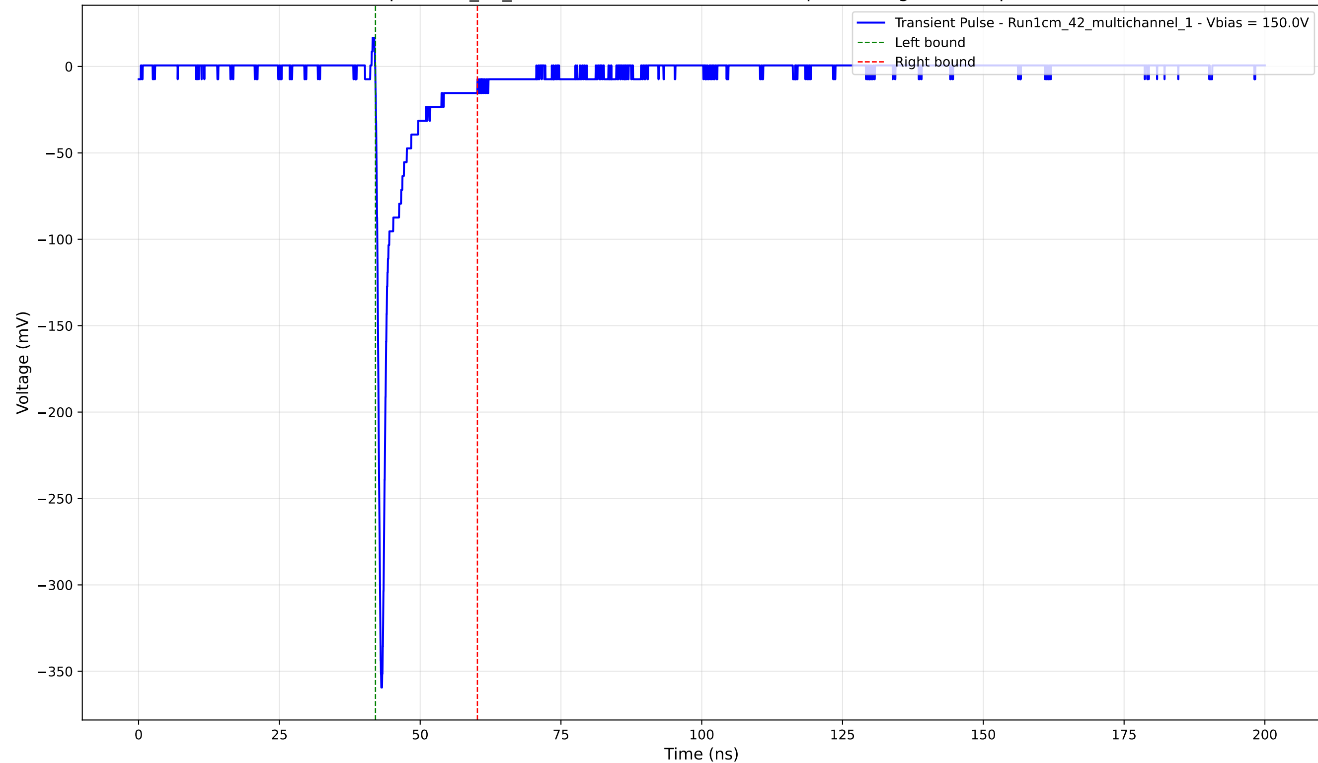
Transient Pulse - Sample: 1cm_42_multichannel - Position: 2315.0 \mu\text{m} - Charge: -20.94 pC - Rise Time: 0.73 ns
