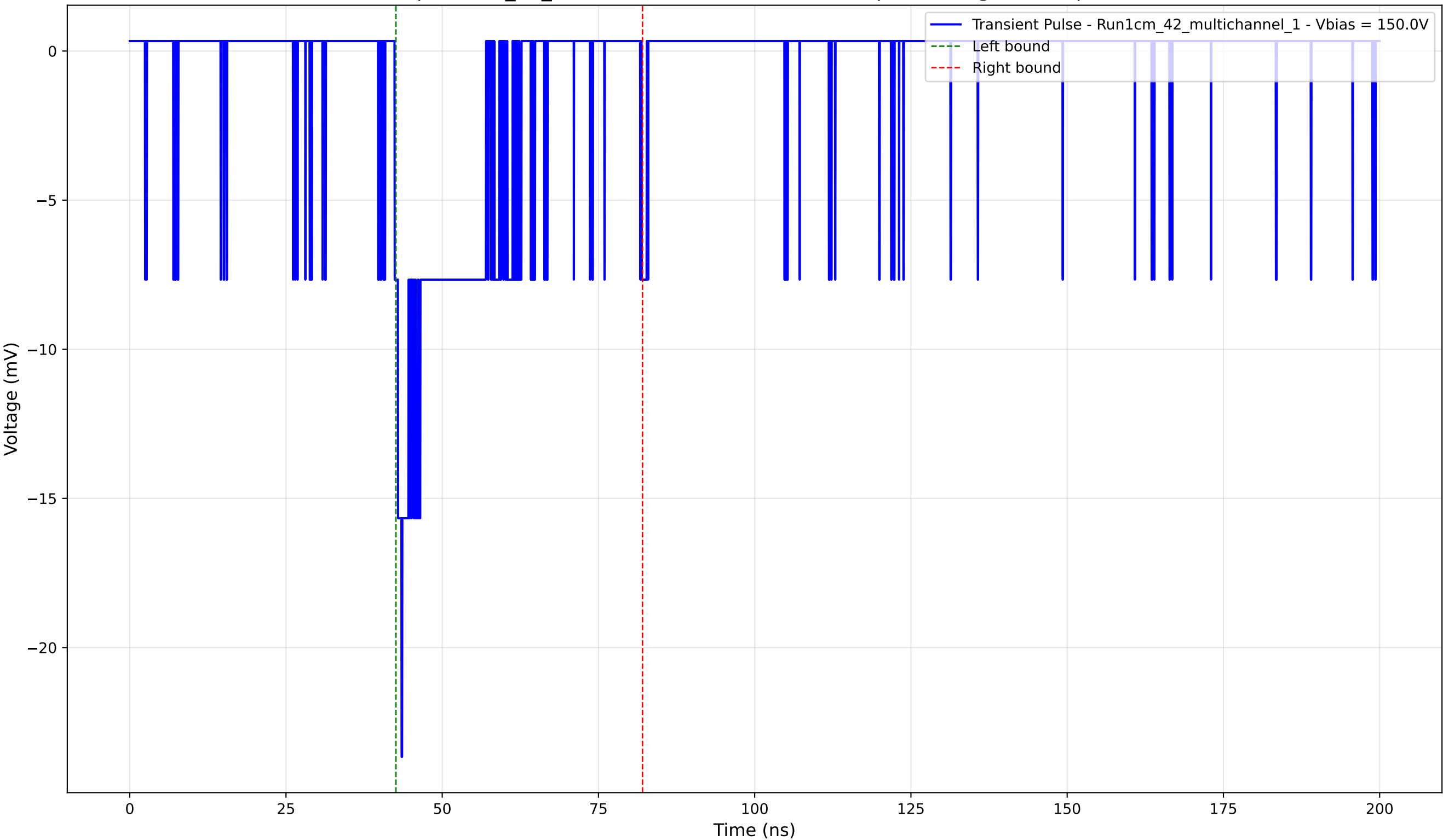
Transient Pulse - Sample: 1cm_42_multichannel - Position: 1855.0 \mu\text{m} - Charge: -3.20 pC - Rise Time: 1.11 ns
