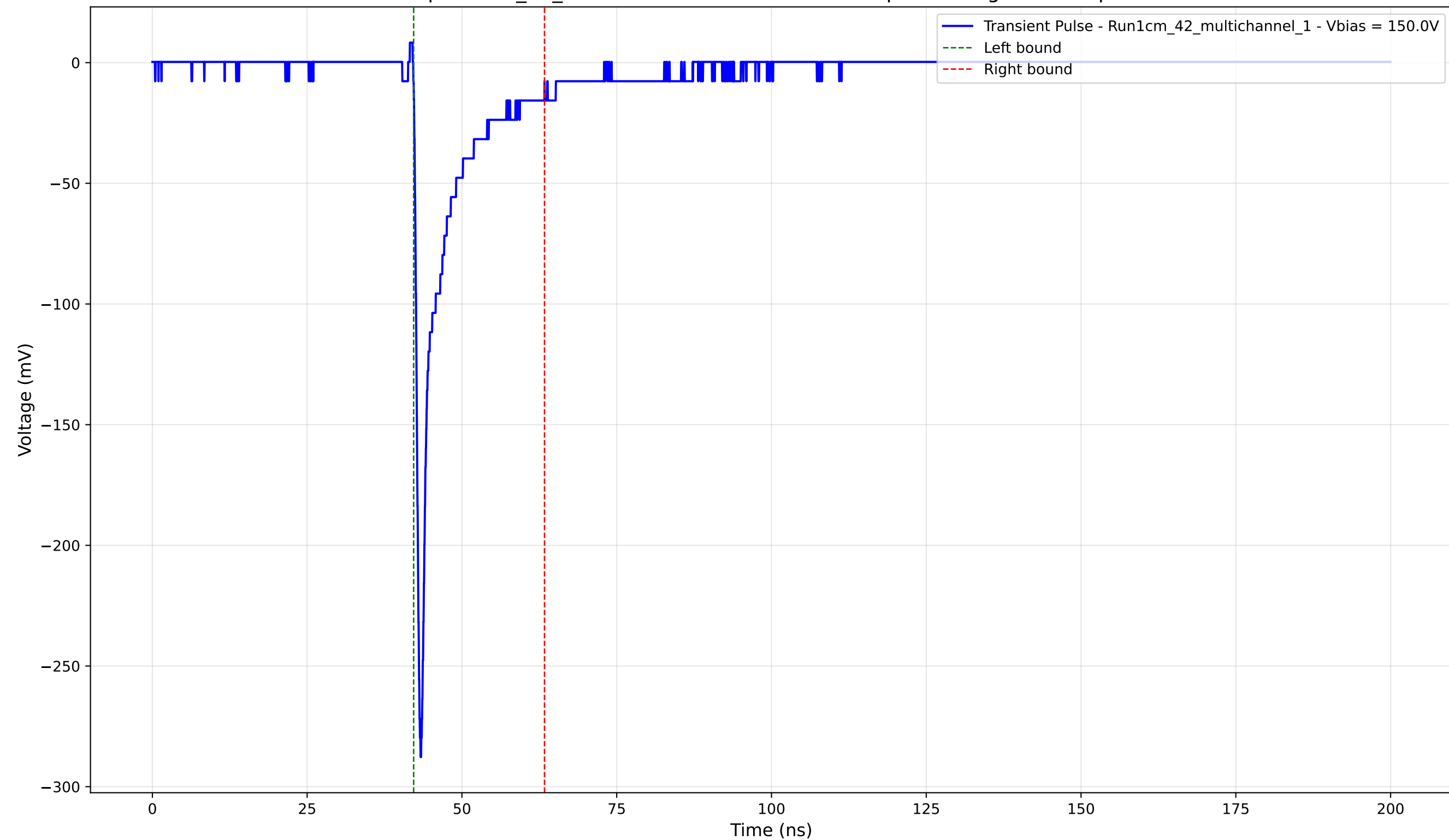
Transient Pulse - Sample: 1cm_42_multichannel - Position: 2060.0 \mu\text{m} - Charge: -23.47 pC - Rise Time: 0.81 ns
