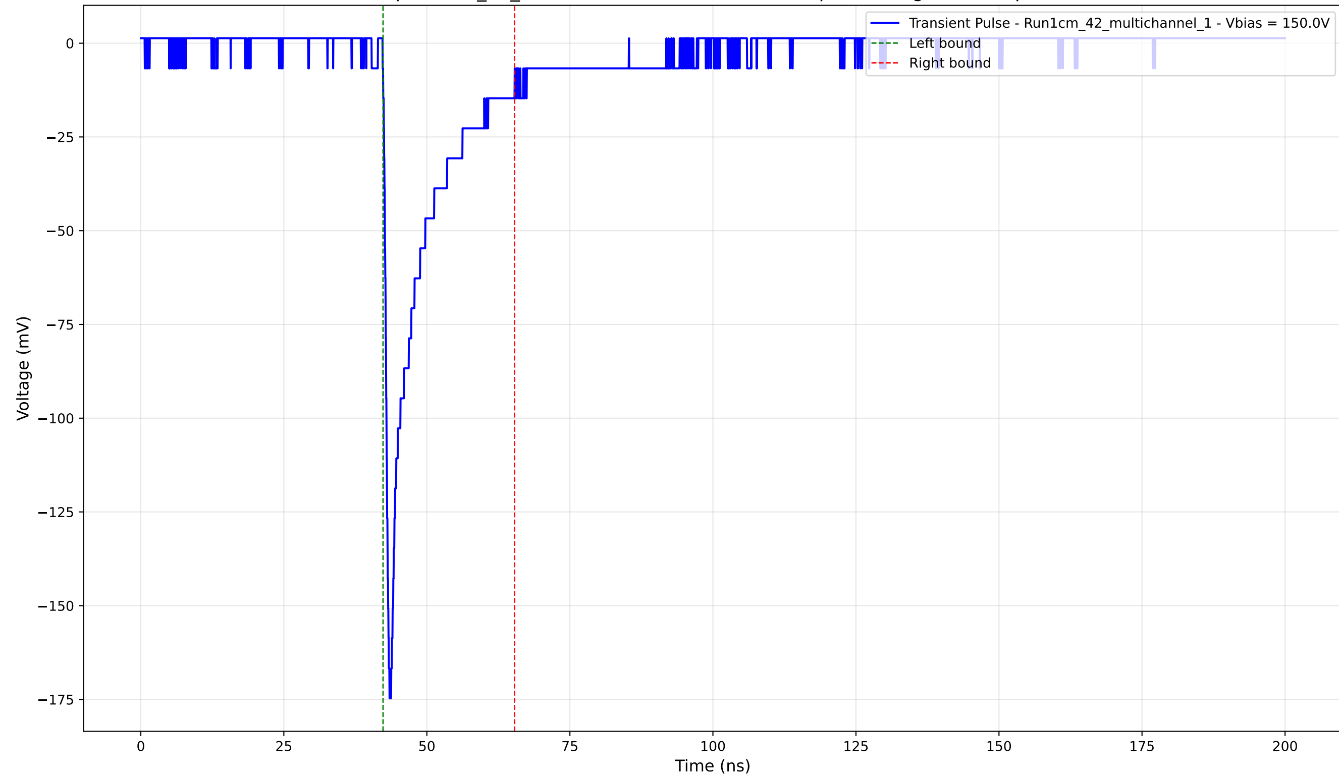
Transient Pulse - Sample: 1cm_42_multichannel - Position: 1775.0 \mu\text{m} - Charge: -21.68 pC - Rise Time: 0.83 ns
