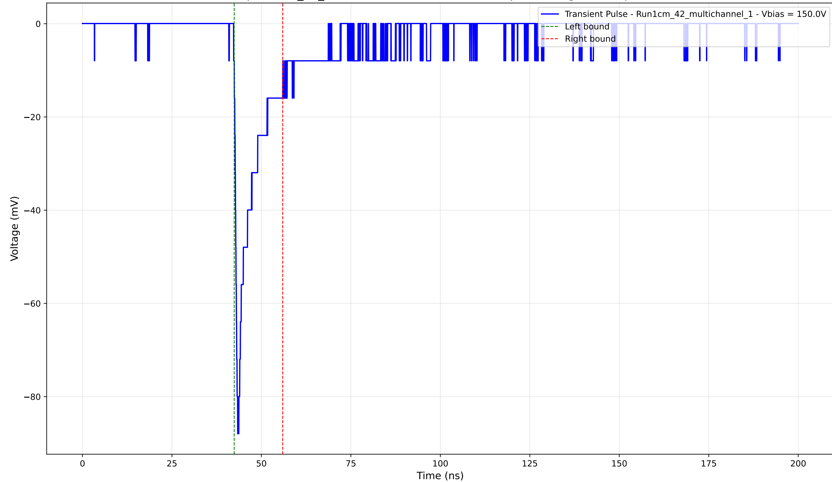
Transient Pulse - Sample: 1cm_42_multichannel - Position: 2945.0 \mu\text{m} - Charge: -8.93 pC - Rise Time: 0.80 ns
