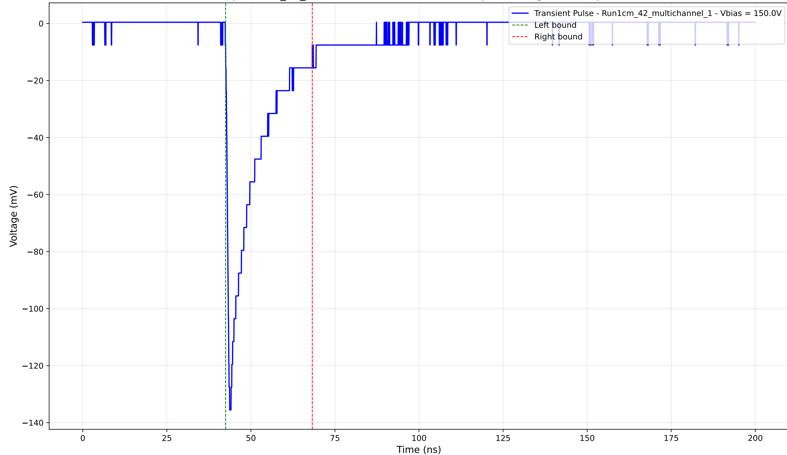
Transient Pulse - Sample: 1cm_42_multichannel - Position: 1540.0 \mu\text{m} - Charge: -23.28 pC - Rise Time: 1.00 ns
