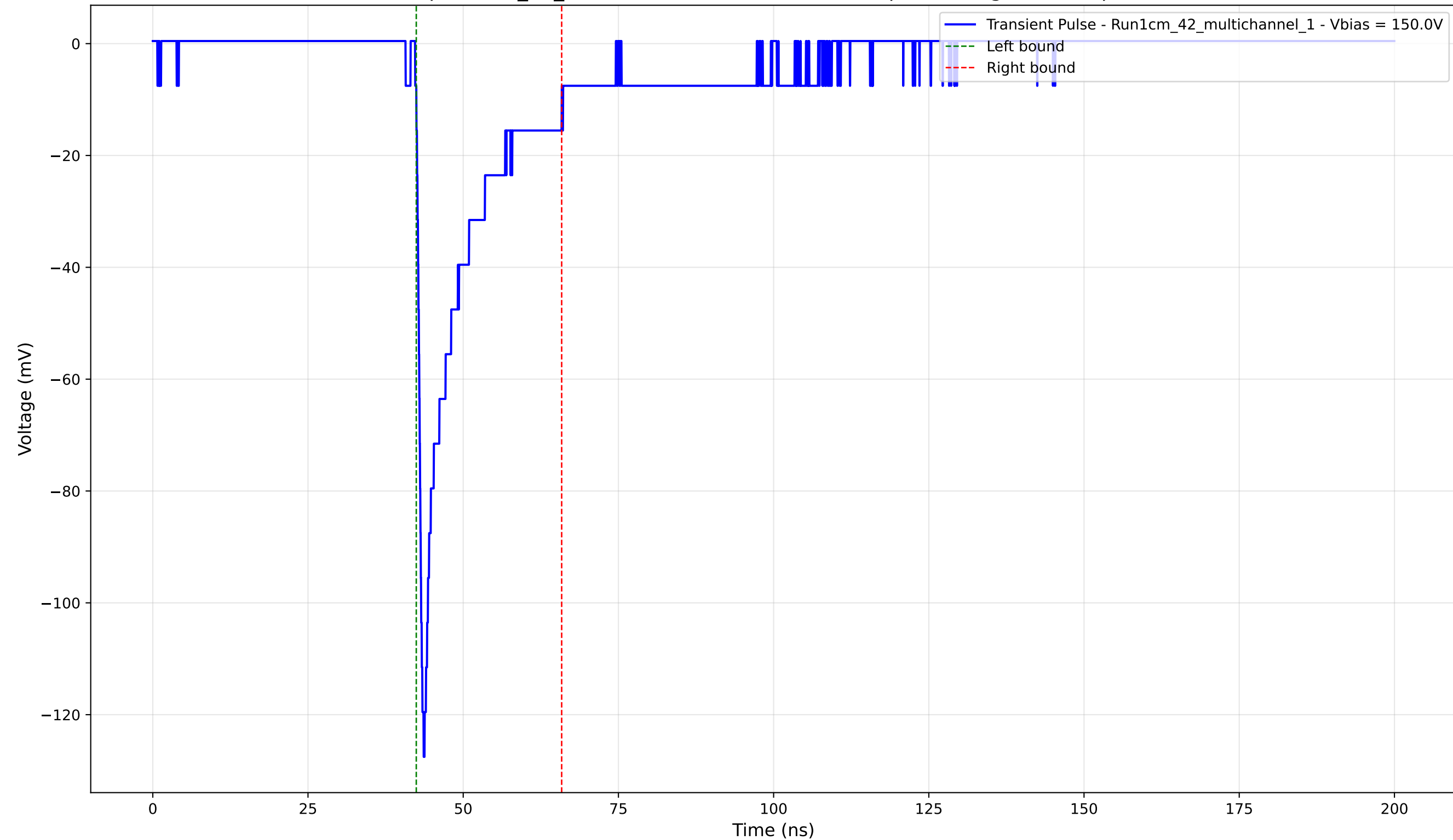
Transient Pulse - Sample: 1cm_42_multichannel - Position: 3150.0 \mu\text{m} - Charge: -16.94 pC - Rise Time: 0.97 ns
