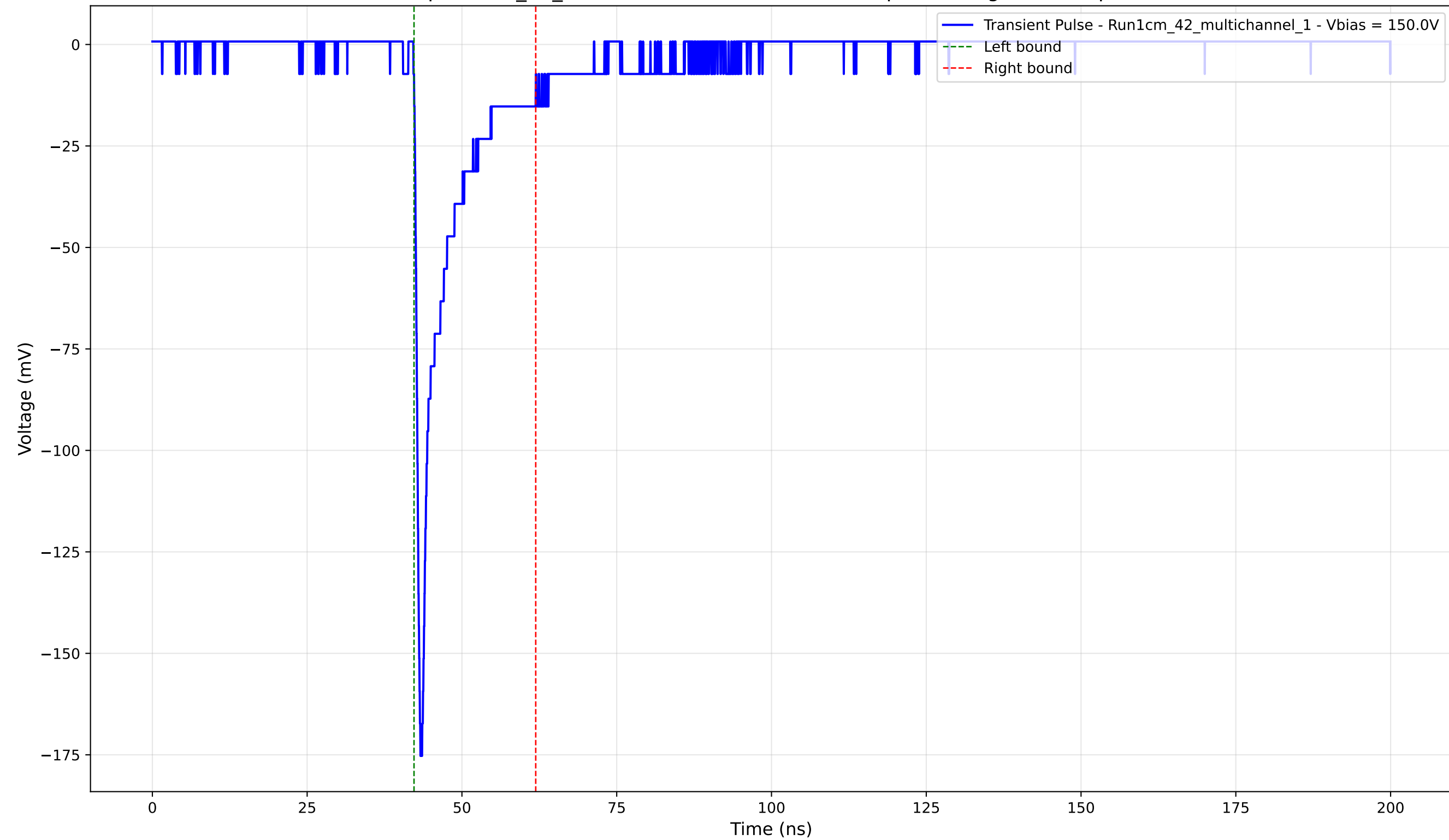
Transient Pulse - Sample: 1cm_42_multichannel - Position: 2825.0 \mu\text{m} - Charge: -16.59 pC - Rise Time: 0.79 ns
