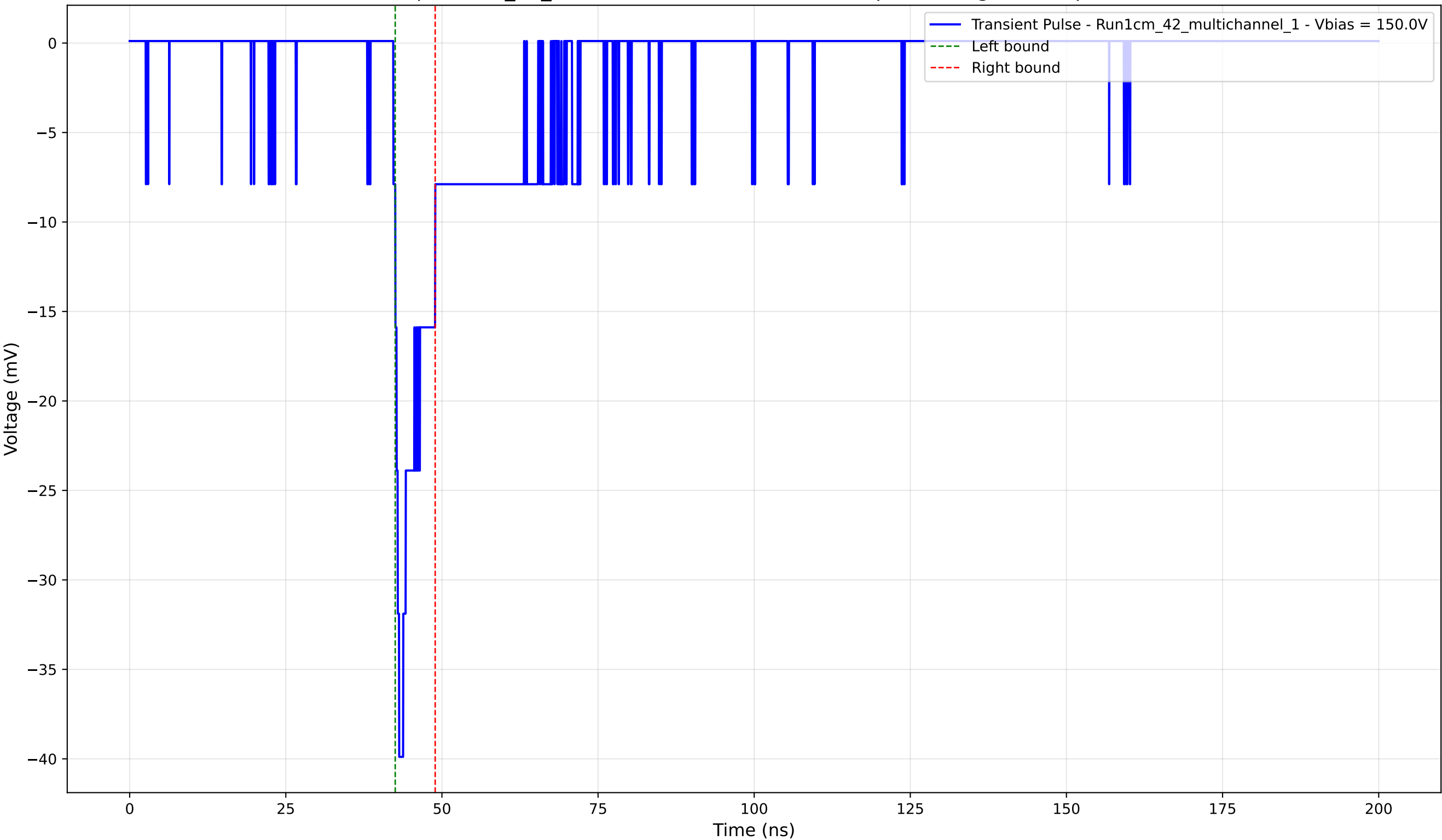
Transient Pulse - Sample: 1cm_42_multichannel - Position: 1915.0 \mu\text{m} - Charge: -2.88 pC - Rise Time: 0.93 ns
