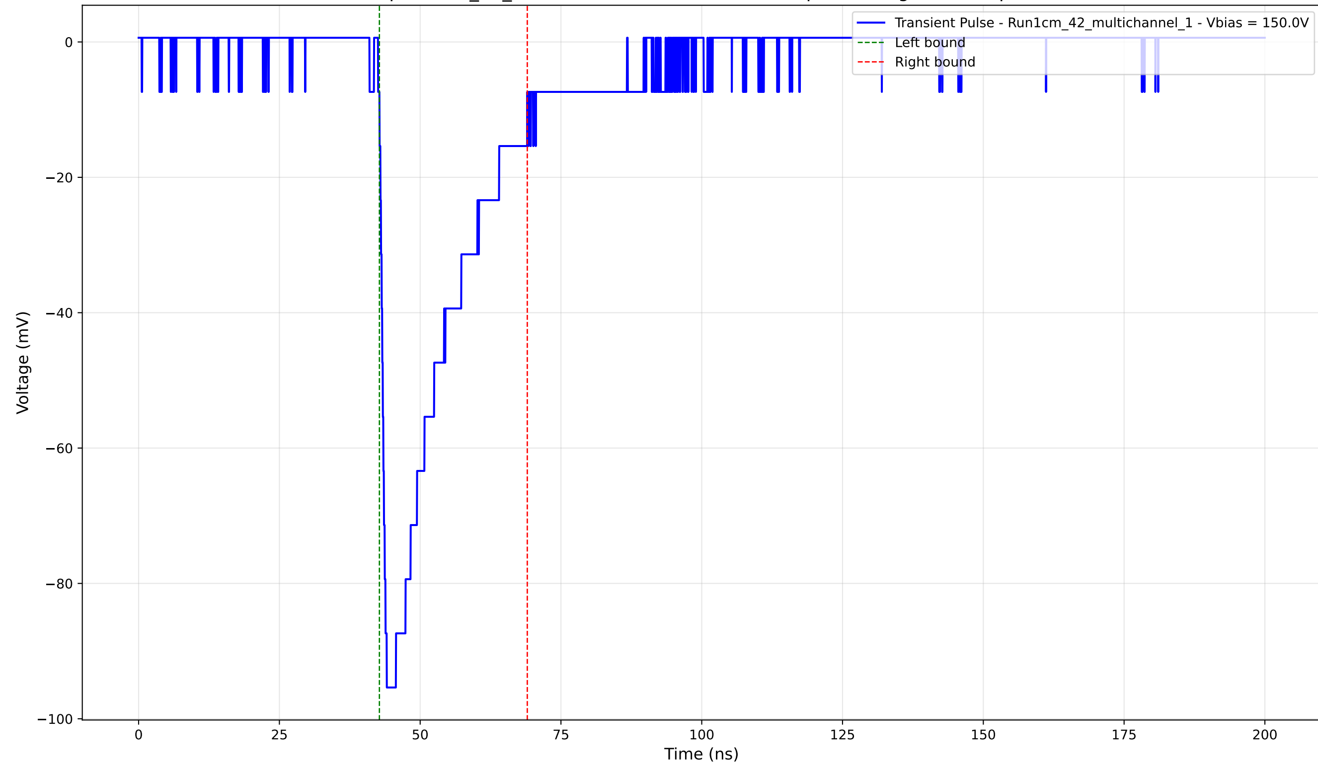
Transient Pulse - Sample: 1cm_42_multichannel - Position: 1185.0 \mu\text{m} - Charge: -23.38 pC - Rise Time: 1.07 ns
