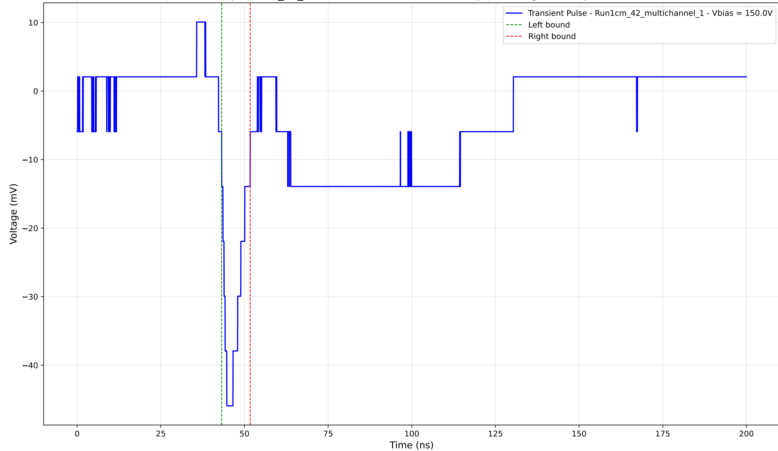
Transient Pulse - Sample: 1cm_42_multichannel - Position: 4520.0 \mu\text{m} - Charge: -5.12 pC - Rise Time: 2.47 ns
