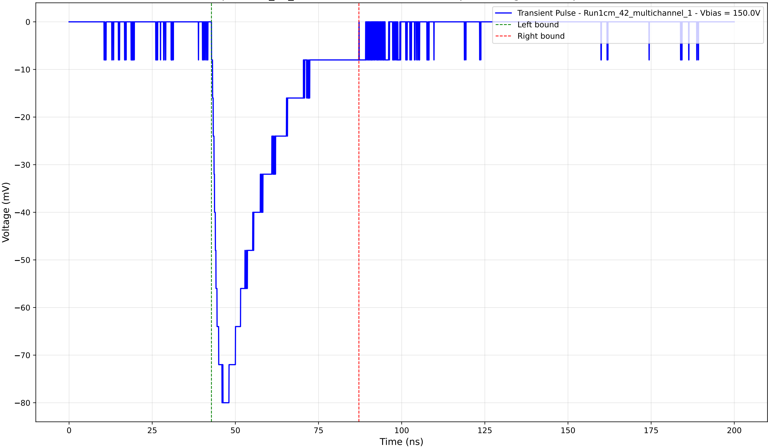
Transient Pulse - Sample: 1cm_42_multichannel - Position: 520.0 \mu\text{m} - Charge: -25.79 pC - Rise Time: 1.86 ns
