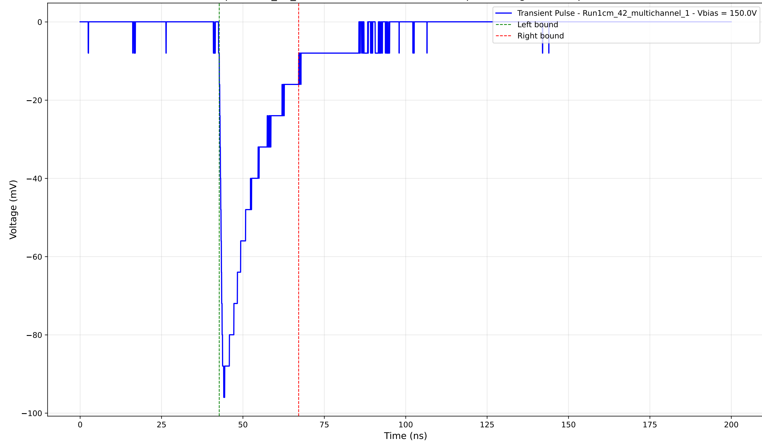
Transient Pulse - Sample: 1cm_42_multichannel - Position: 1290.0 \mu\text{m} - Charge: -20.59 pC - Rise Time: 1.02 ns
