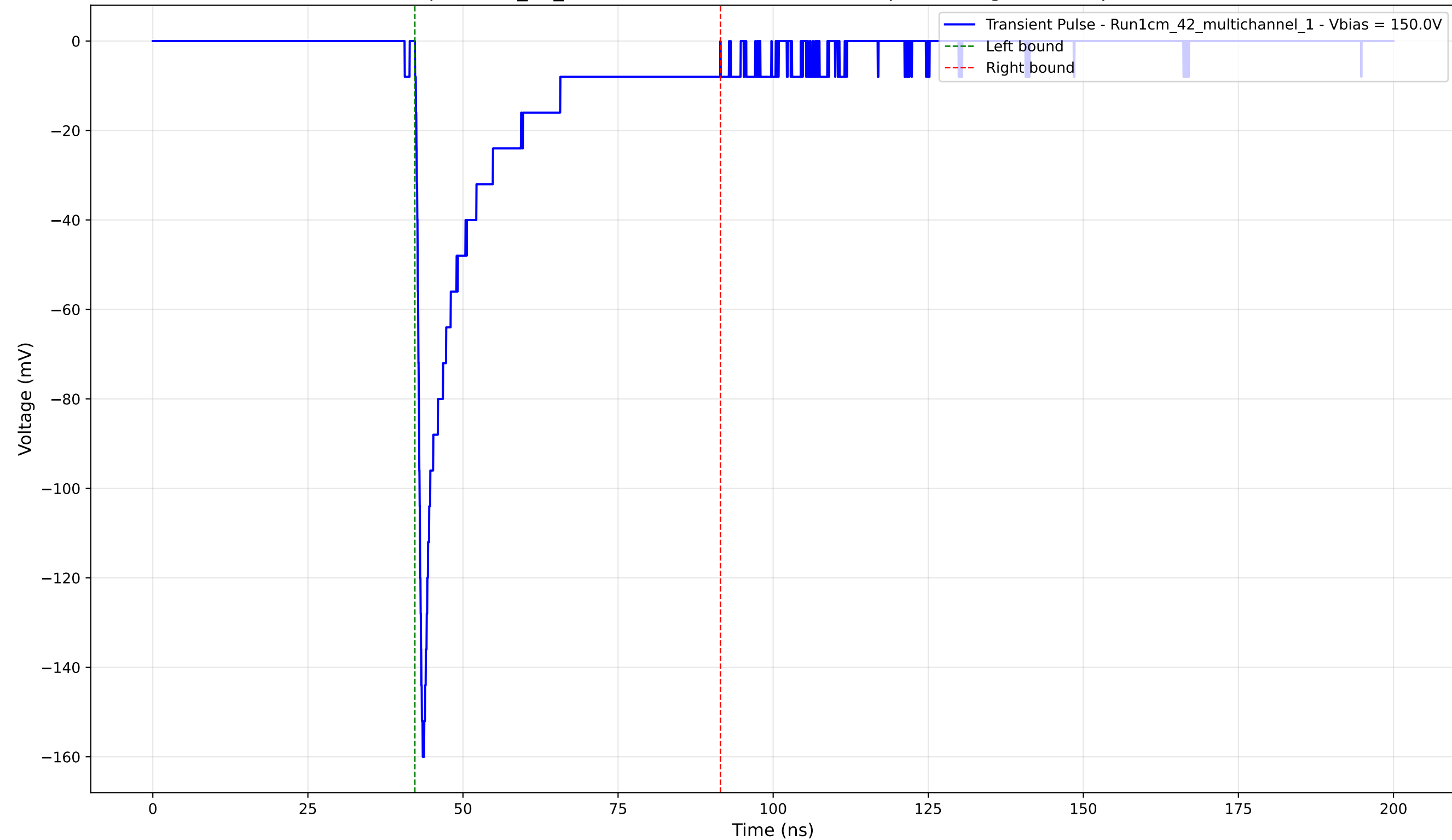
Transient Pulse - Sample: 1cm_42_multichannel - Position: 3035.0 \mu\text{m} - Charge: -24.36 pC - Rise Time: 0.82 ns
