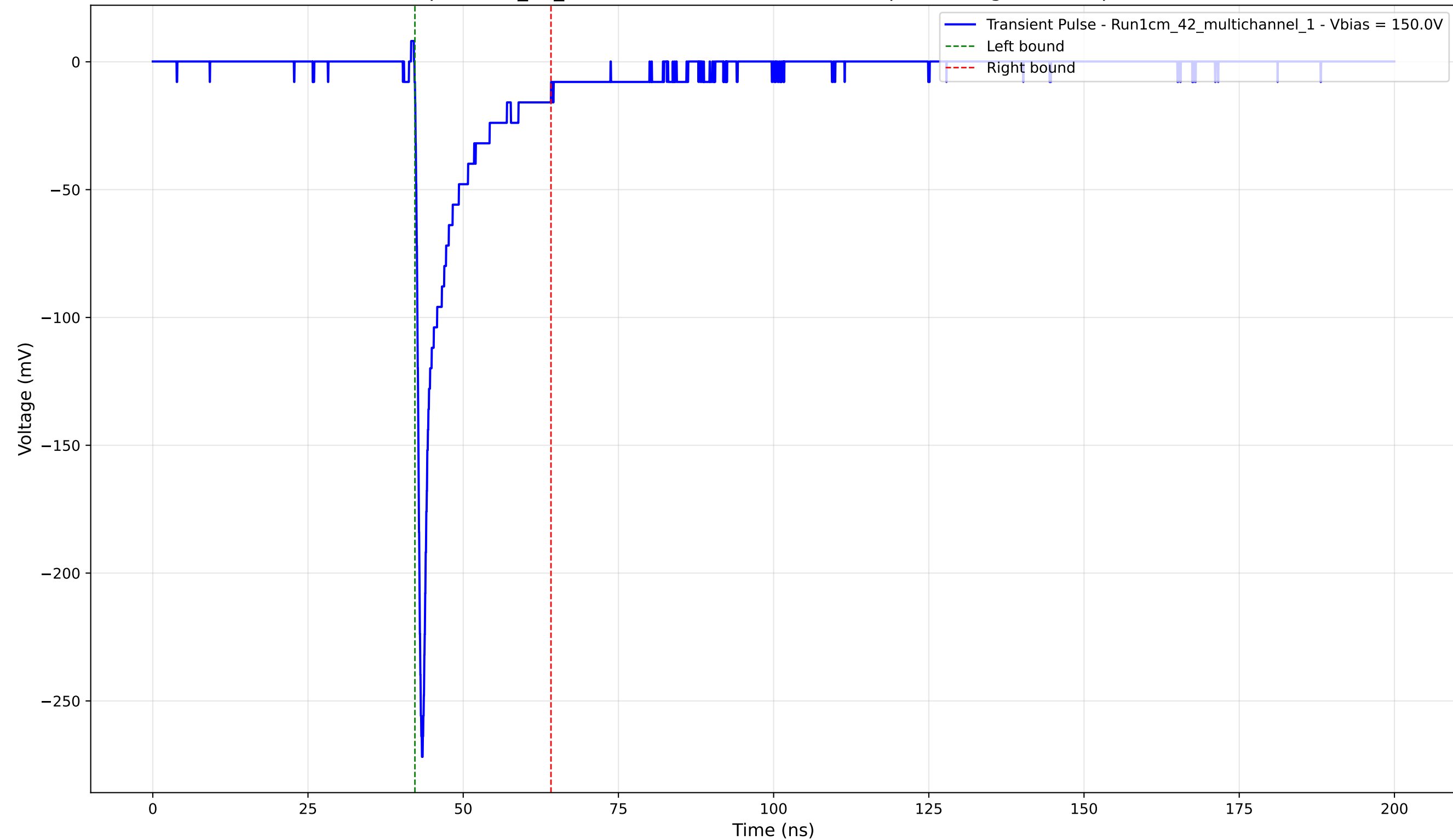
Transient Pulse - Sample: 1cm_42_multichannel - Position: 2020.0 \mu\text{m} - Charge: -23.61 pC - Rise Time: 0.81 ns
