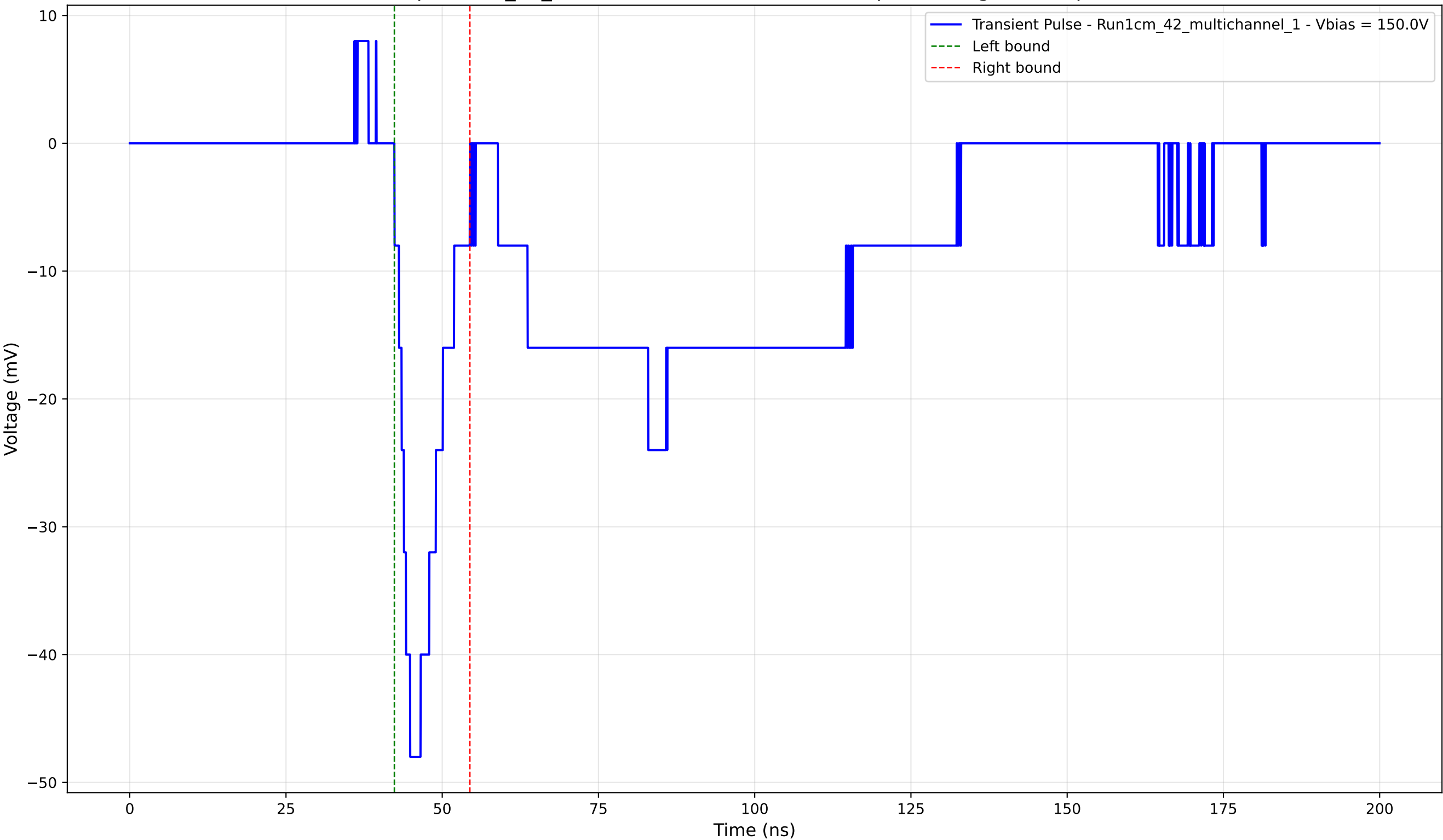
Transient Pulse - Sample: 1cm_42_multichannel - Position: 4630.0 \mu\text{m} - Charge: -6.08 pC - Rise Time: 2.51 ns
