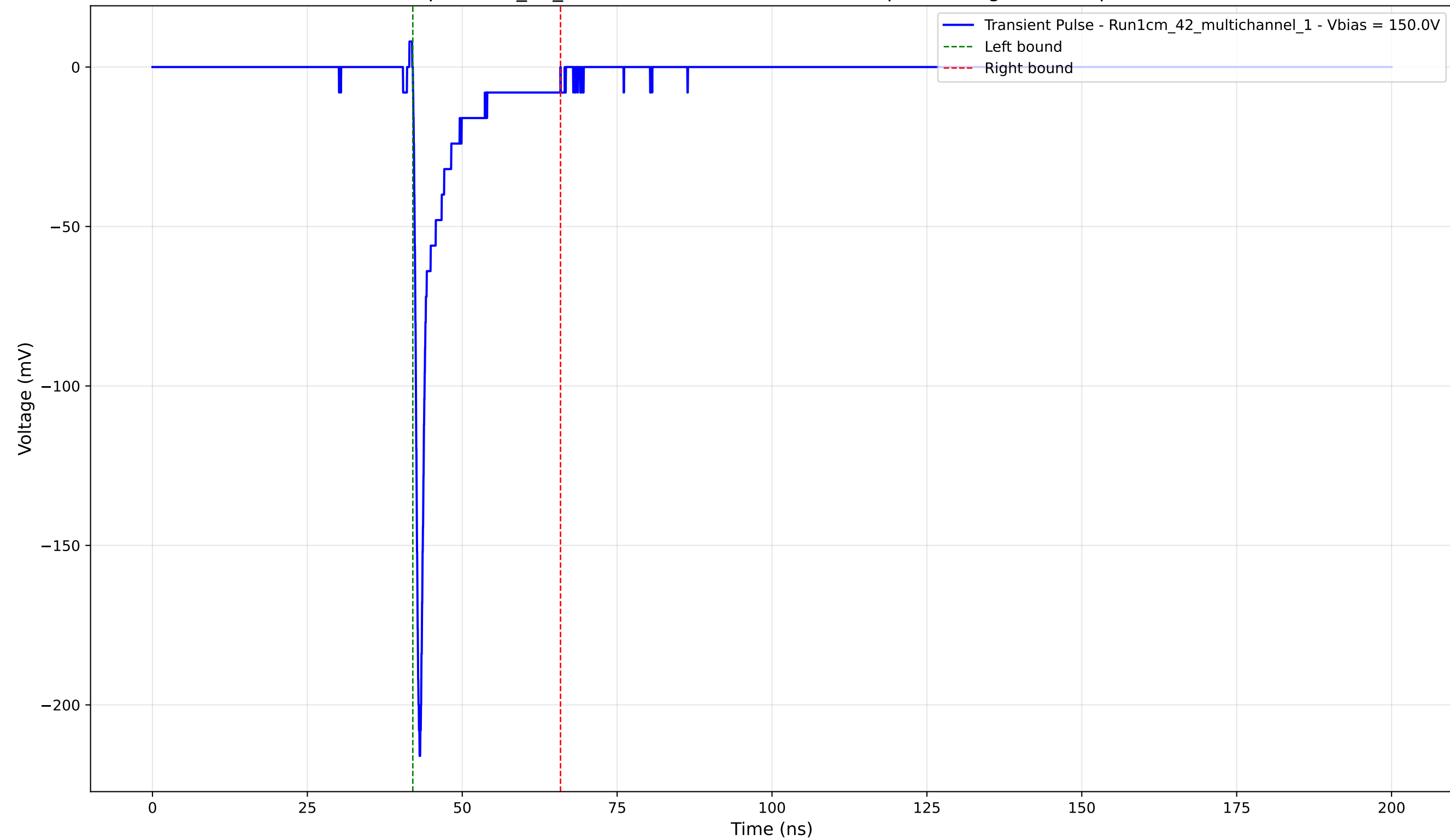
Transient Pulse - Sample: 1cm_42_multichannel - Position: 2335.0 \mu\text{m} - Charge: -13.34 pC - Rise Time: 0.77 ns
