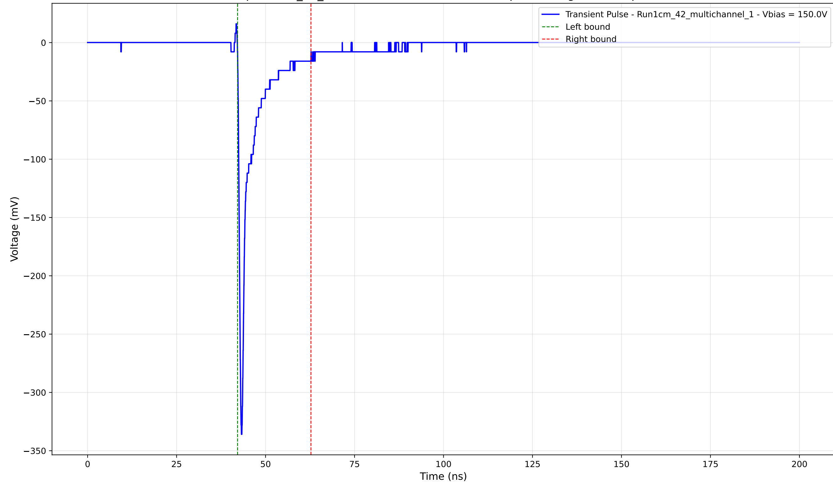
Transient Pulse - Sample: 1cm_42_multichannel - Position: 2155.0 \mu\text{m} - Charge: -24.27 pC - Rise Time: 0.75 ns
