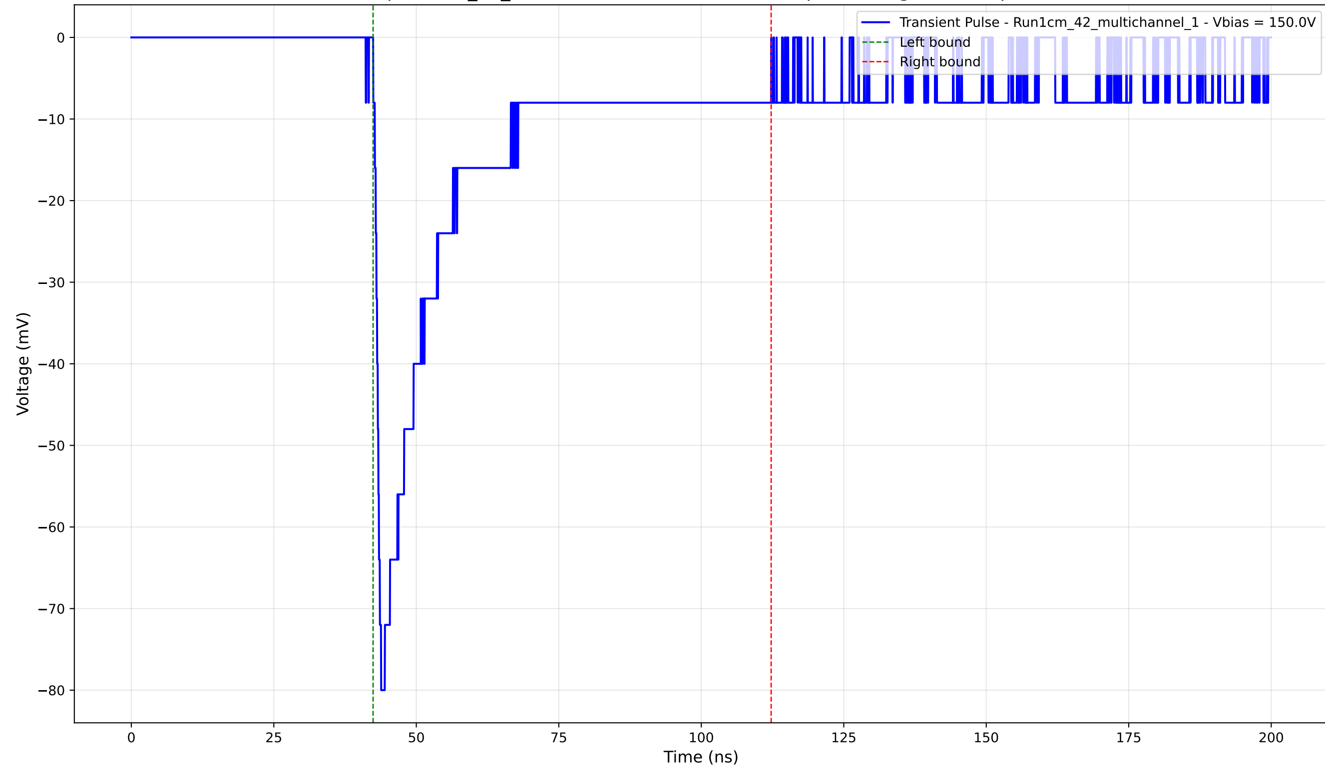
Transient Pulse - Sample: 1cm_42_multichannel - Position: 3515.0 \mu\text{m} - Charge: -22.90 pC - Rise Time: 0.90 ns
