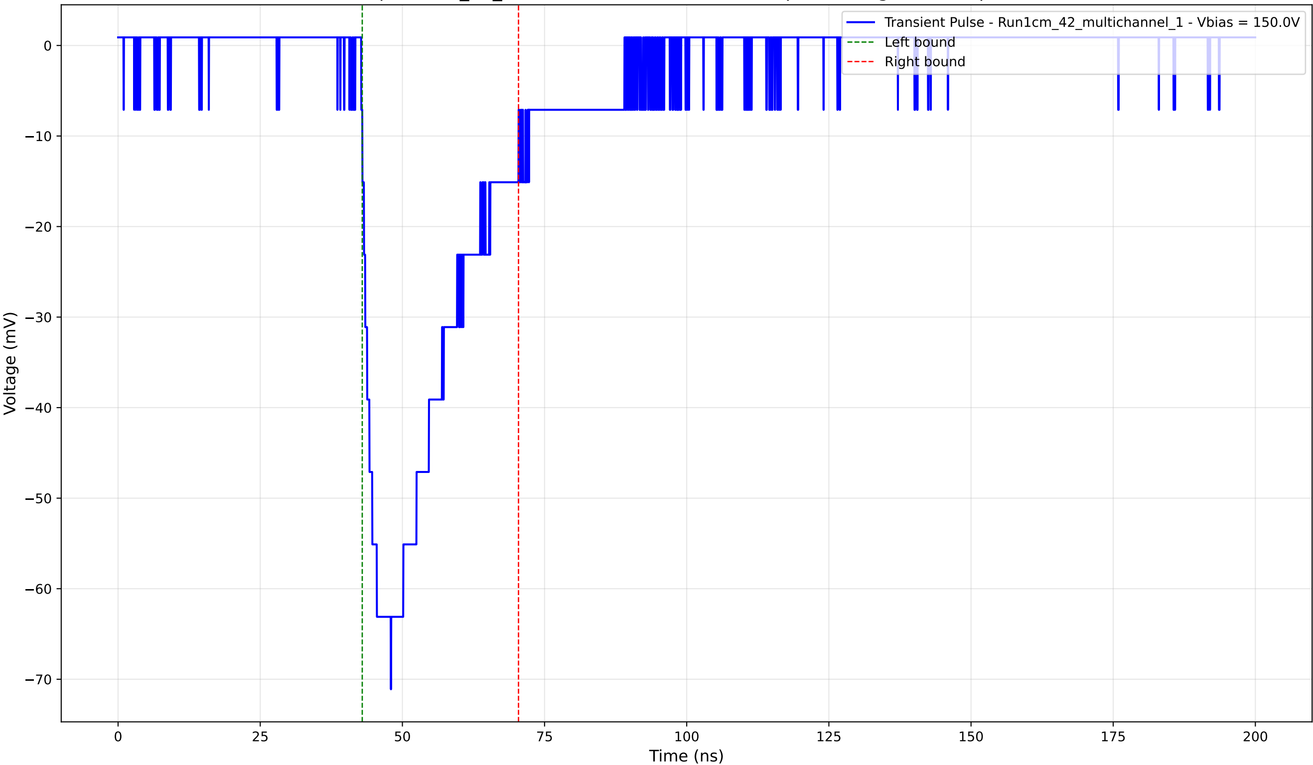
Transient Pulse - Sample: 1cm_42_multichannel - Position: 195.0 \mu\text{m} - Charge: -20.24 pC - Rise Time: 5.02 ns
