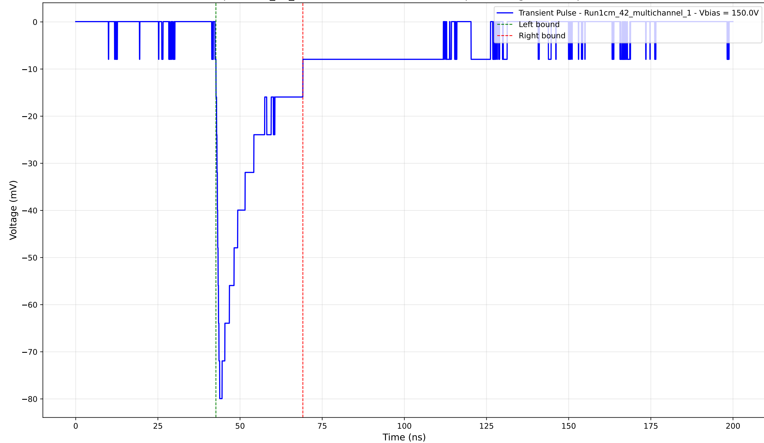
Transient Pulse - Sample: 1cm_42_multichannel - Position: 3520.0 \mu\text{m} - Charge: -16.88 pC - Rise Time: 1.14 ns
