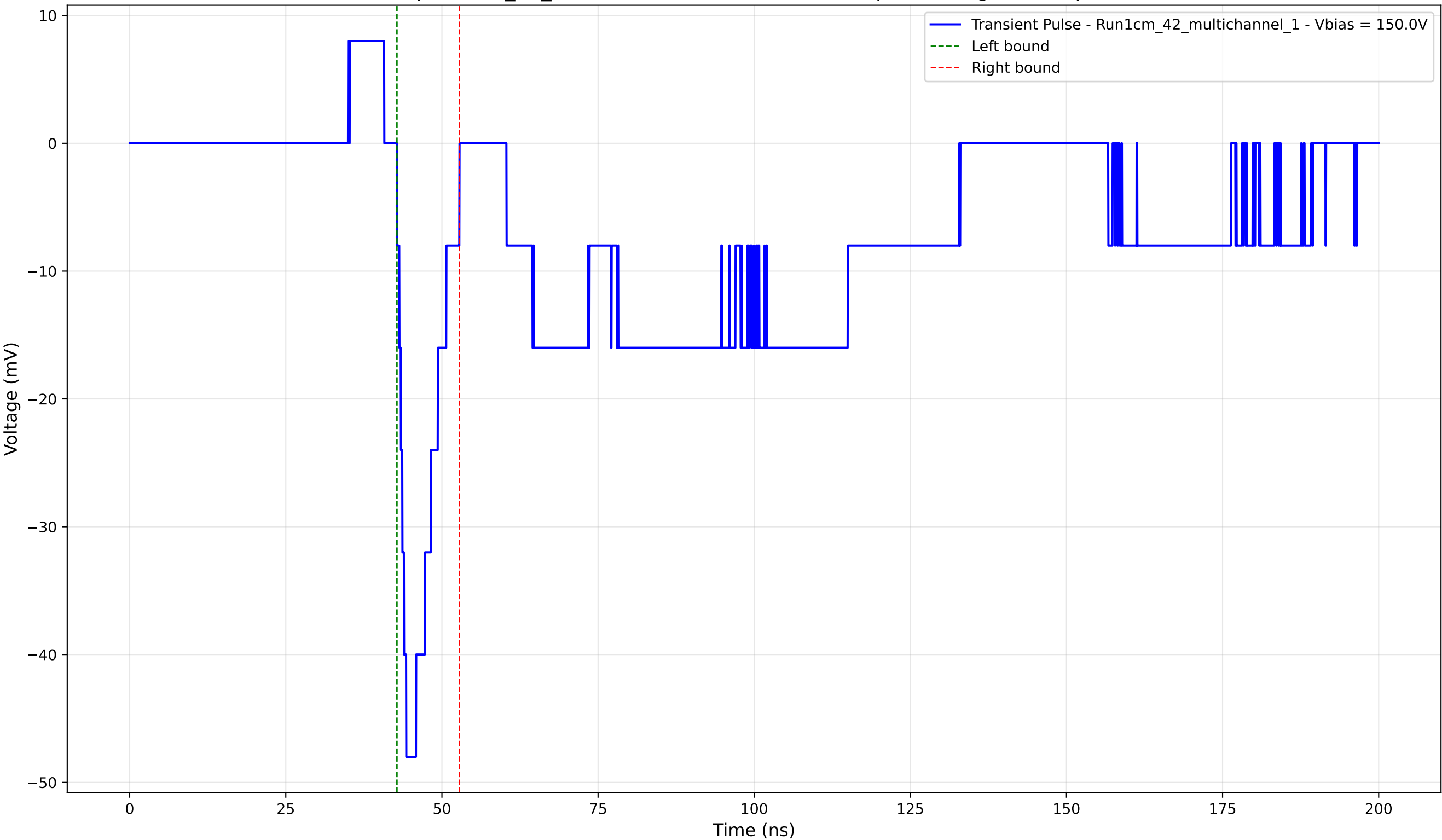
Transient Pulse - Sample: 1cm_42_multichannel - Position: 3980.0 \mu\text{m} - Charge: -5.27 pC - Rise Time: 1.47 ns
