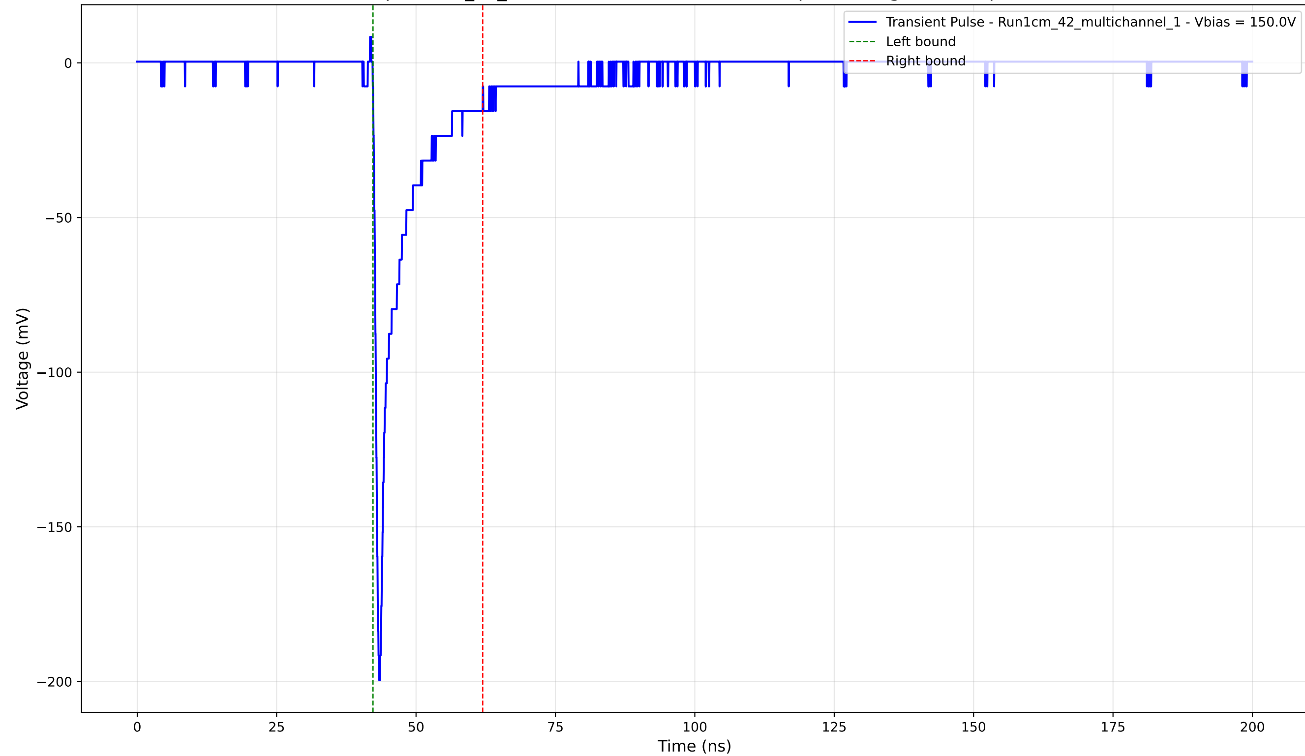
Transient Pulse - Sample: 1cm_42_multichannel - Position: 1950.0 \mu\text{m} - Charge: -18.64 pC - Rise Time: 0.83 ns
