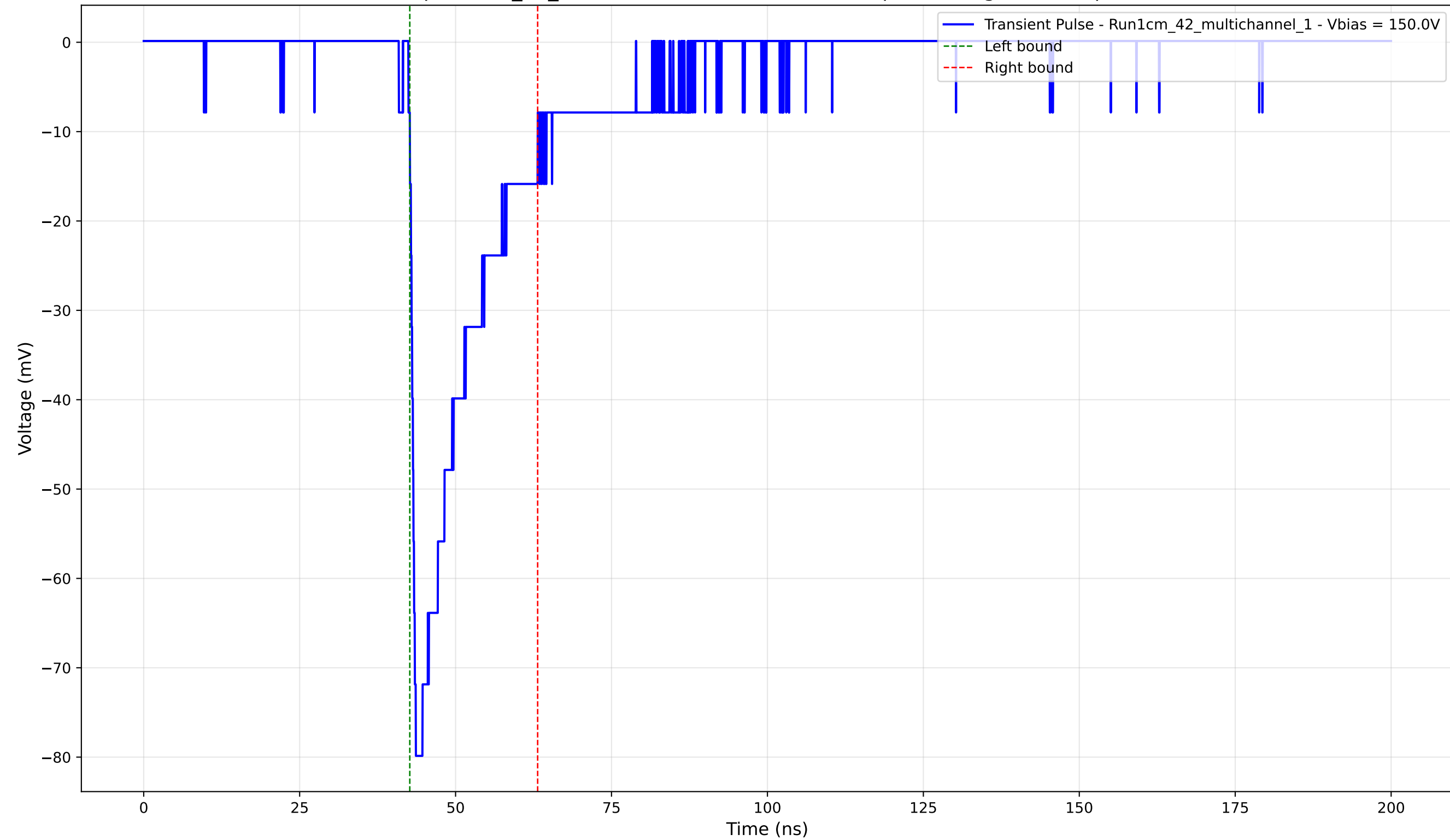
Transient Pulse - Sample: 1cm_42_multichannel - Position: 1435.0 \mu\text{m} - Charge: -15.06 pC - Rise Time: 0.96 ns
