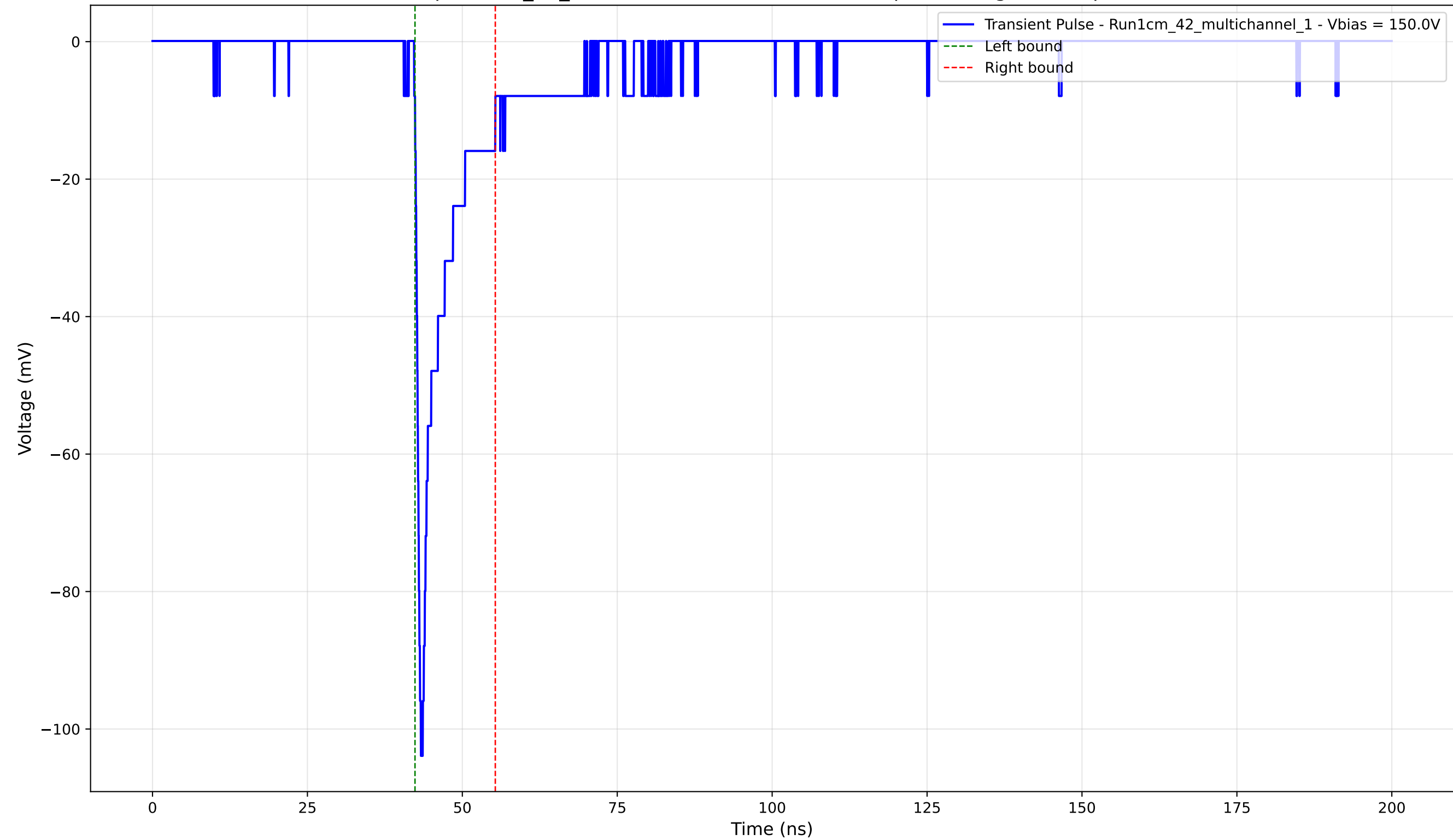
Transient Pulse - Sample: 1cm_42_multichannel - Position: 1930.0 \mu\text{m} - Charge: -8.88 pC - Rise Time: 0.79 ns
