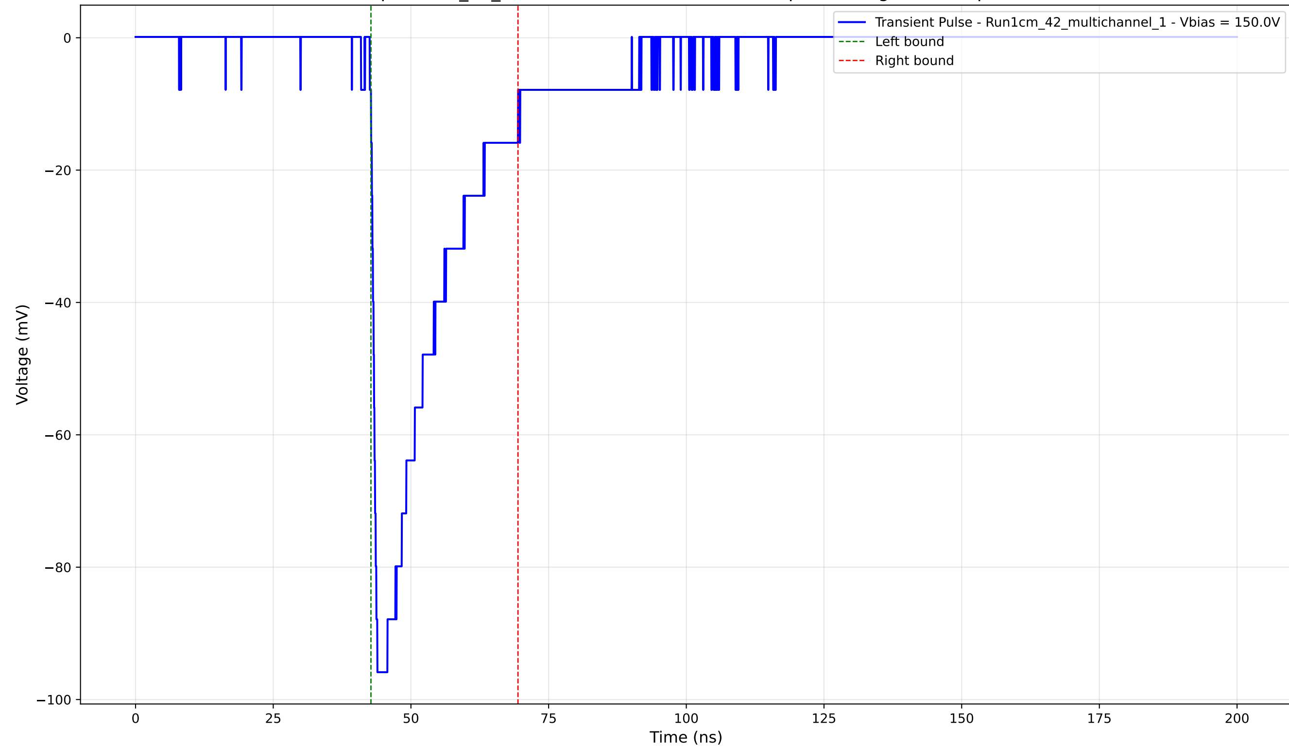
Transient Pulse - Sample: 1cm_42_multichannel - Position: 1230.0 \mu\text{m} - Charge: -23.42 pC - Rise Time: 0.98 ns
