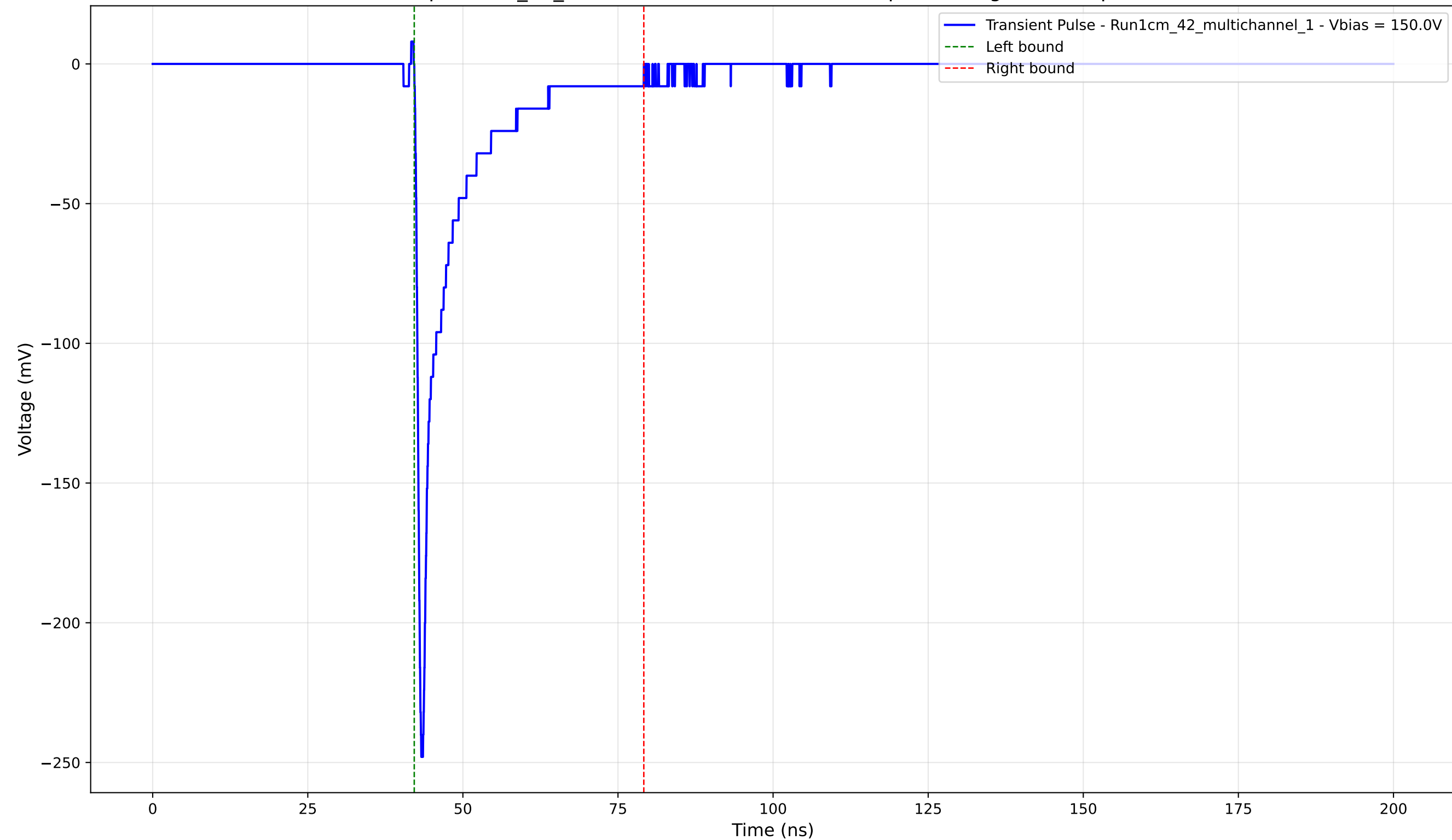
Transient Pulse - Sample: 1cm_42_multichannel - Position: 1985.0 \mu\text{m} - Charge: -25.65 pC - Rise Time: 0.78 ns
