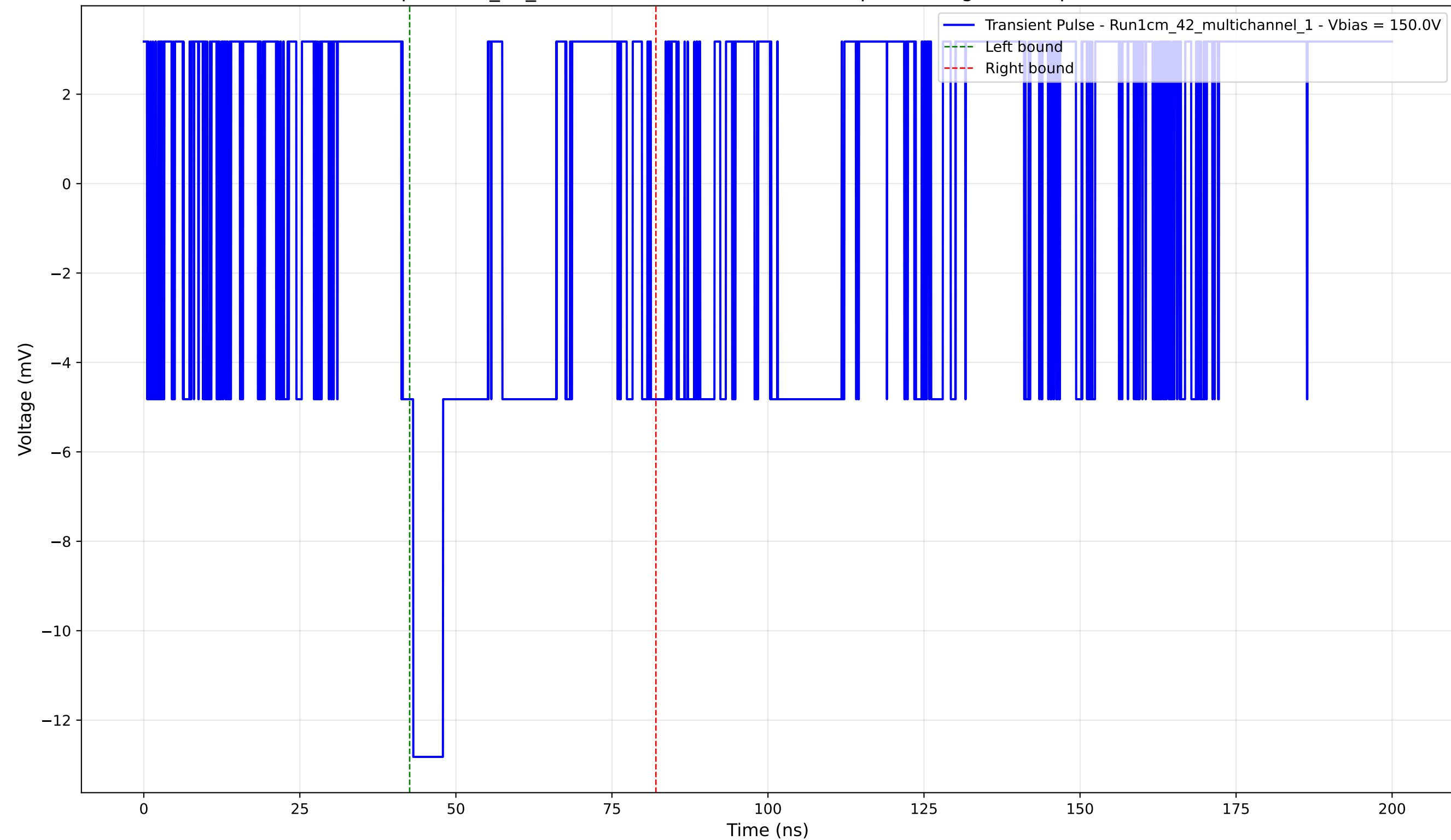
Transient Pulse - Sample: 1cm_42_multichannel - Position: 3435.0 \mu\text{m} - Charge: -2.28 pC - Rise Time: 0.00 ns (N/A)
