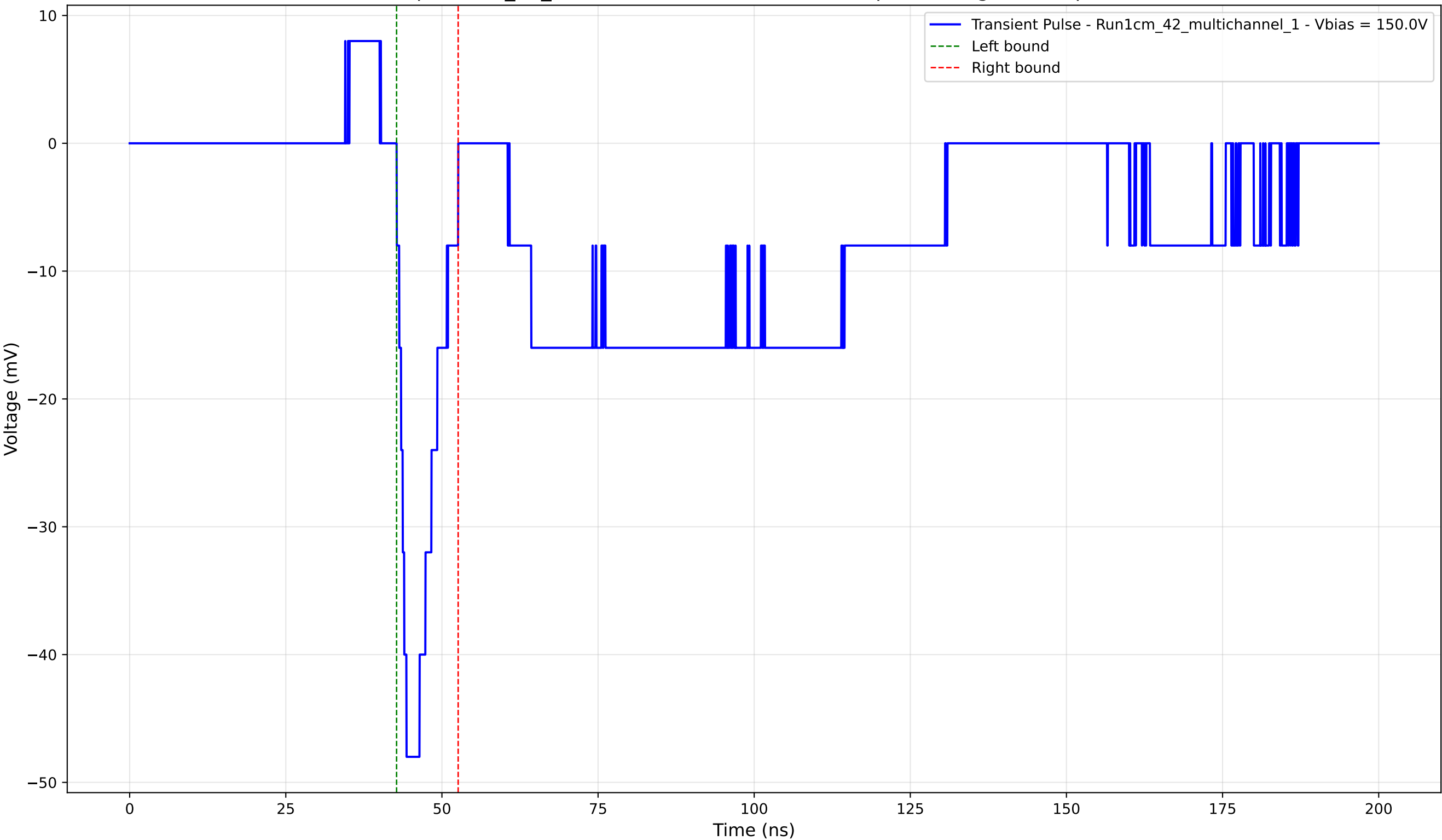
Transient Pulse - Sample: 1cm_42_multichannel - Position: 4065.0 \mu\text{m} - Charge: -5.34 pC - Rise Time: 1.57 ns
