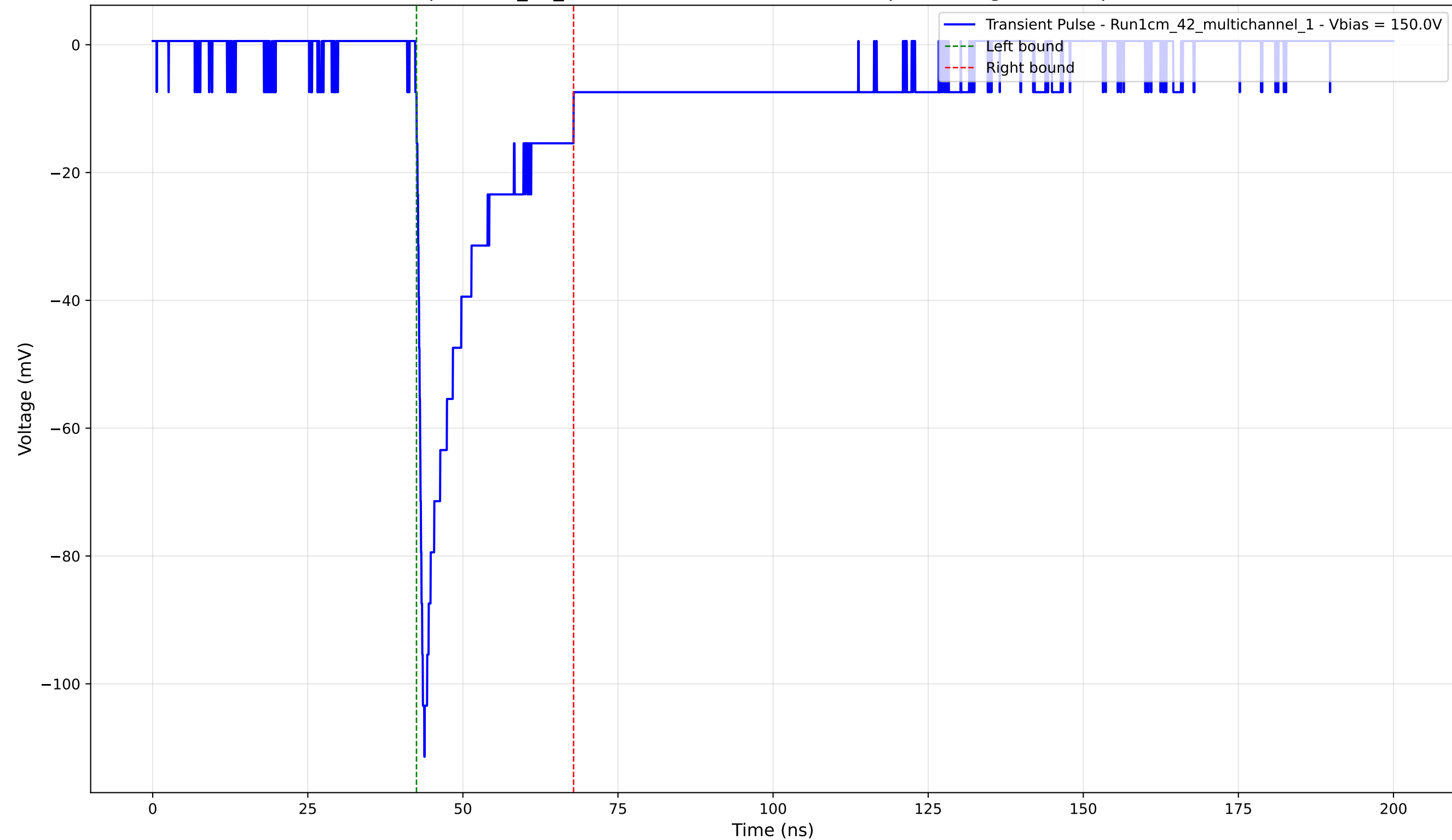
Transient Pulse - Sample: 1cm_42_multichannel - Position: 3280.0 \mu\text{m} - Charge: -17.76 pC - Rise Time: 1.01 ns
