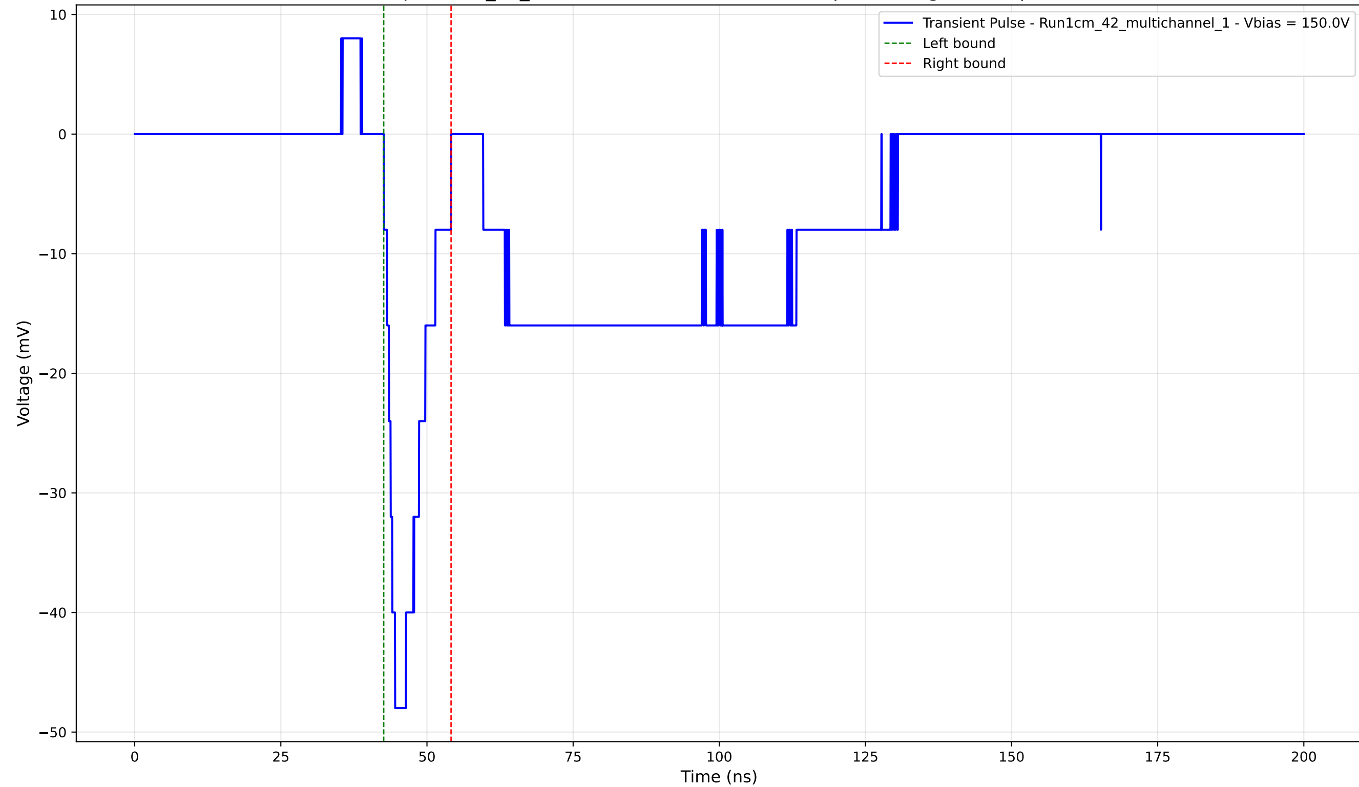
Transient Pulse - Sample: 1cm_42_multichannel - Position: 4160.0 \mu\text{m} - Charge: -5.81 pC - Rise Time: 1.93 ns
