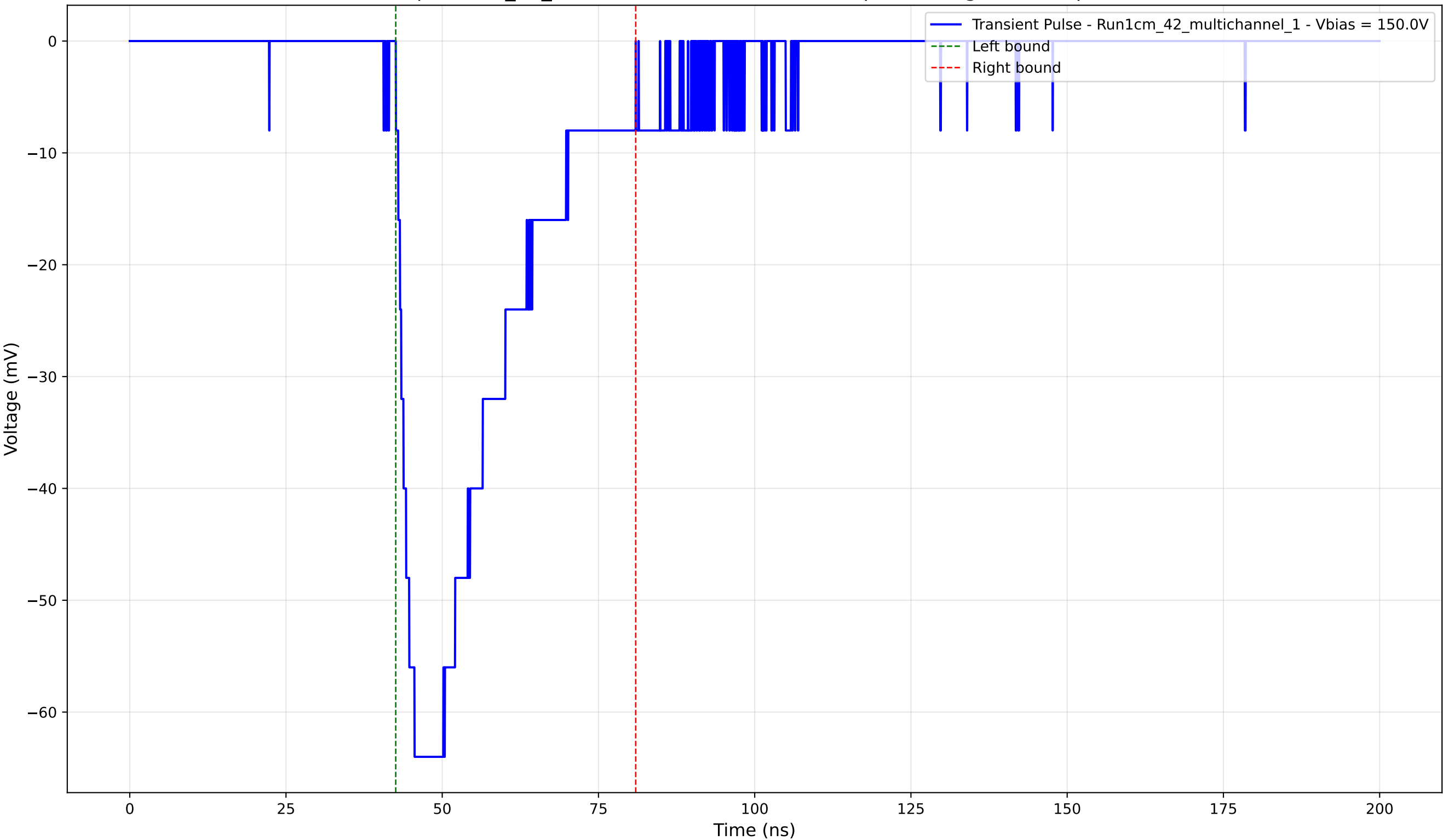
Transient Pulse - Sample: 1cm_42_multichannel - Position: 155.0 \mu\text{m} - Charge: -22.02 pC - Rise Time: 2.98 ns
