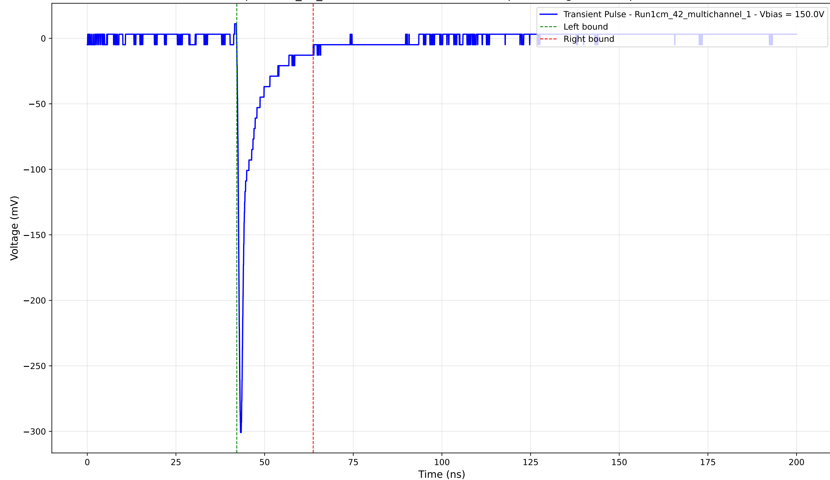
Transient Pulse - Sample: 1cm_42_multichannel - Position: 2655.0 \mu\text{m} - Charge: -22.19 pC - Rise Time: 0.76 ns
