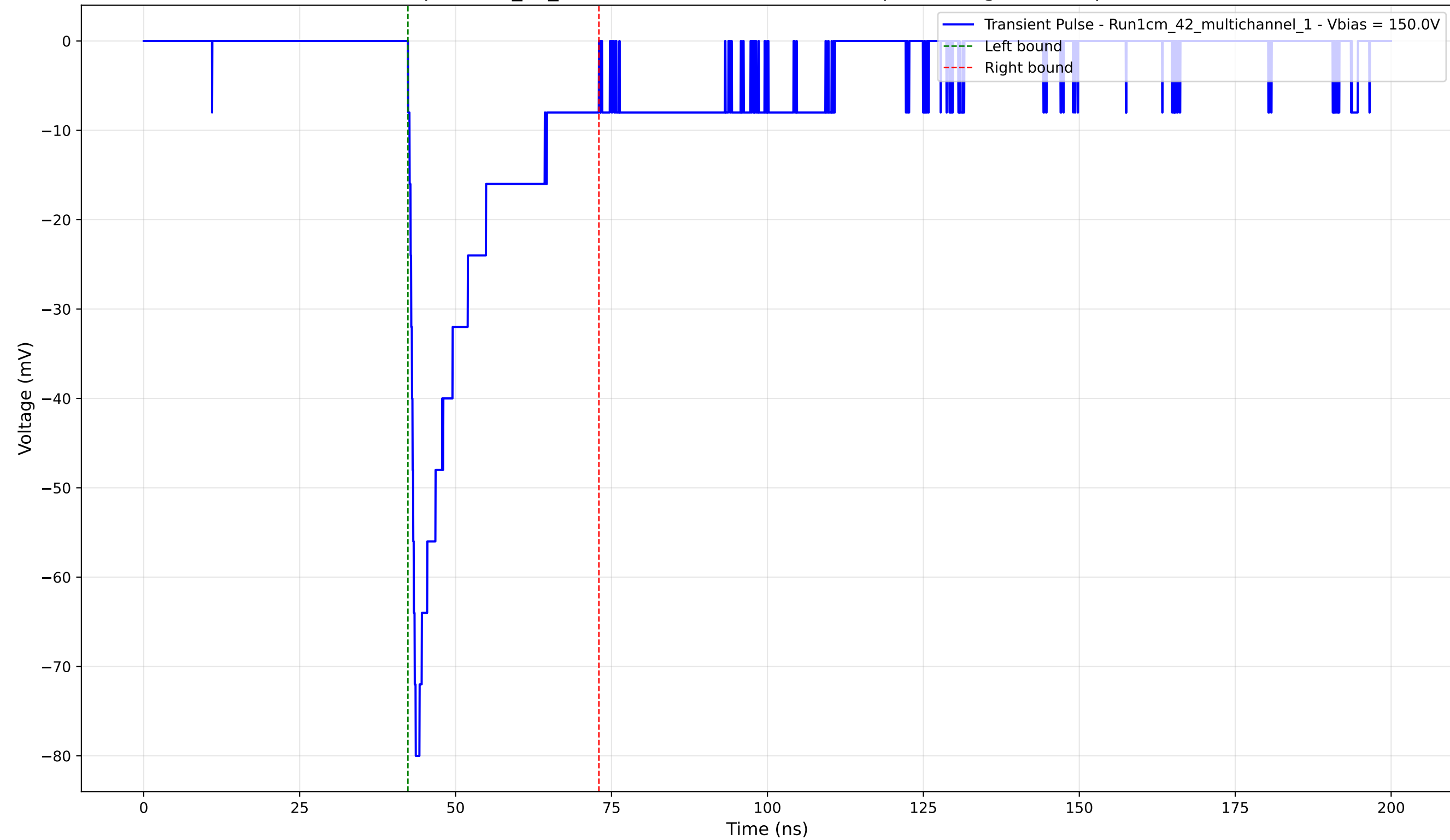
Transient Pulse - Sample: 1cm_42_multichannel - Position: 3330.0 \mu\text{m} - Charge: -14.82 pC - Rise Time: 0.84 ns
