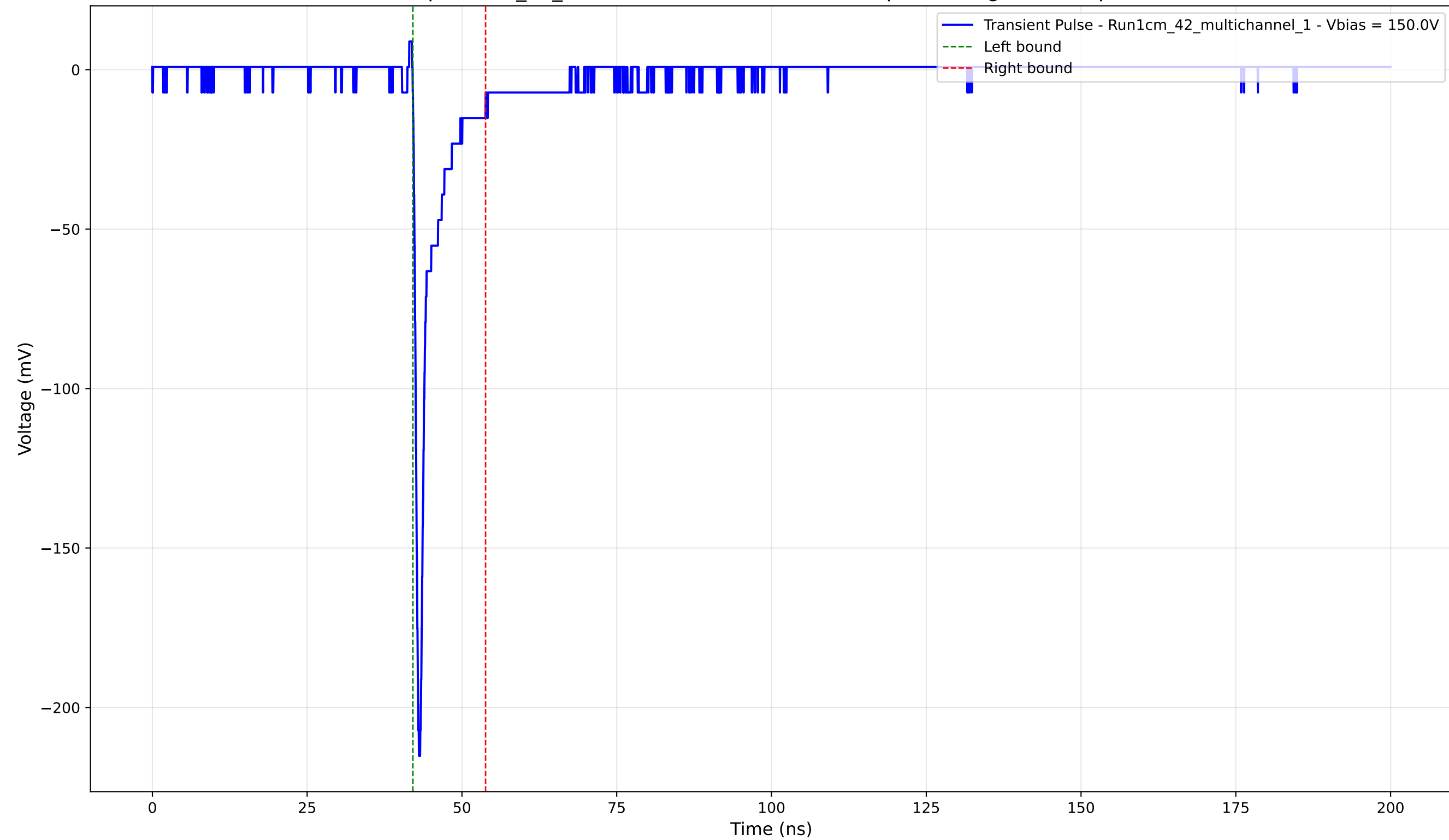
Transient Pulse - Sample: 1cm_42_multichannel - Position: 2440.0 \mu\text{m} - Charge: -11.46 pC - Rise Time: 0.76 ns
