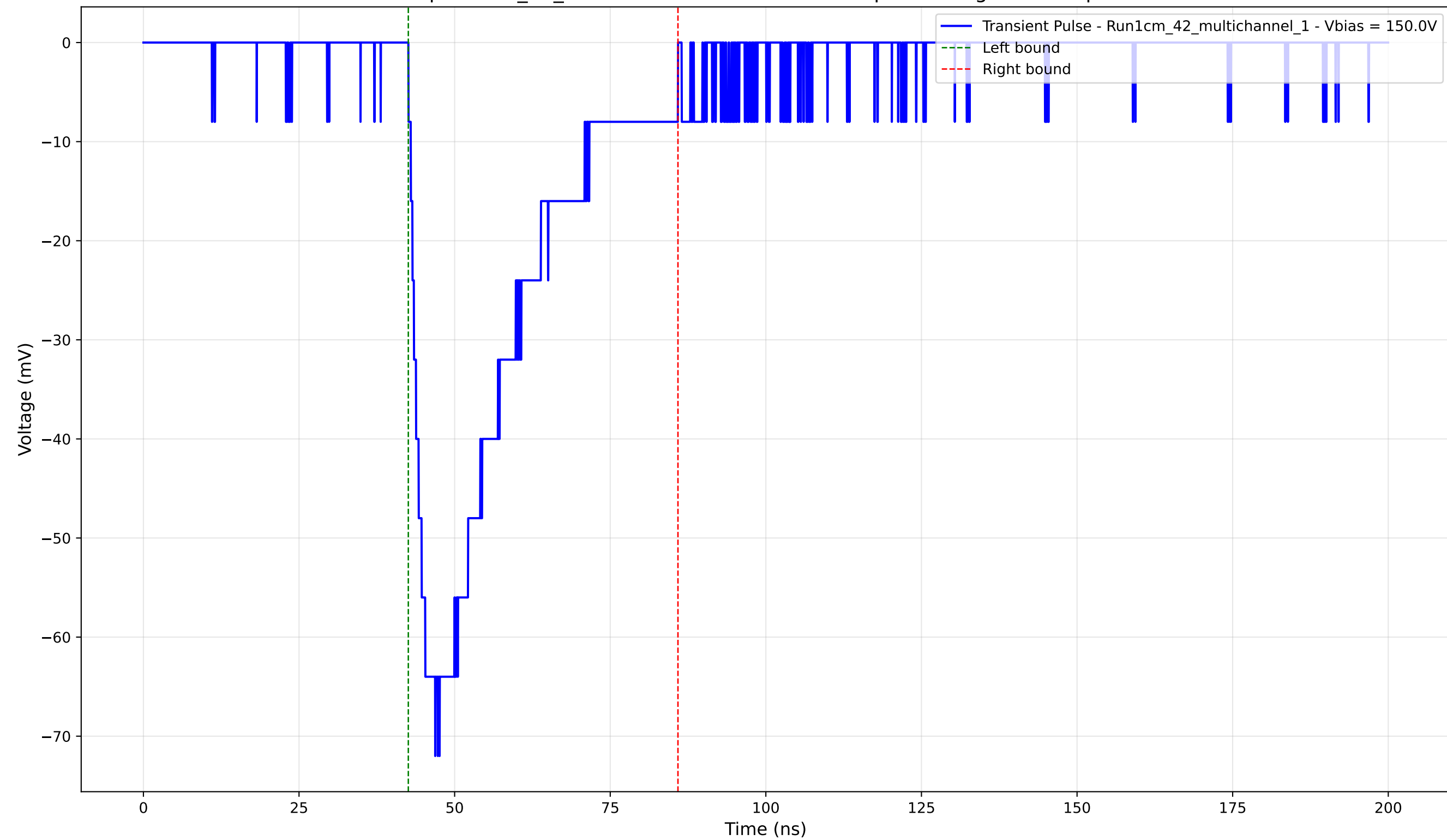
Transient Pulse - Sample: 1cm_42_multichannel - Position: 165.0 \mu\text{m} - Charge: -23.21 pC - Rise Time: 4.30 ns
