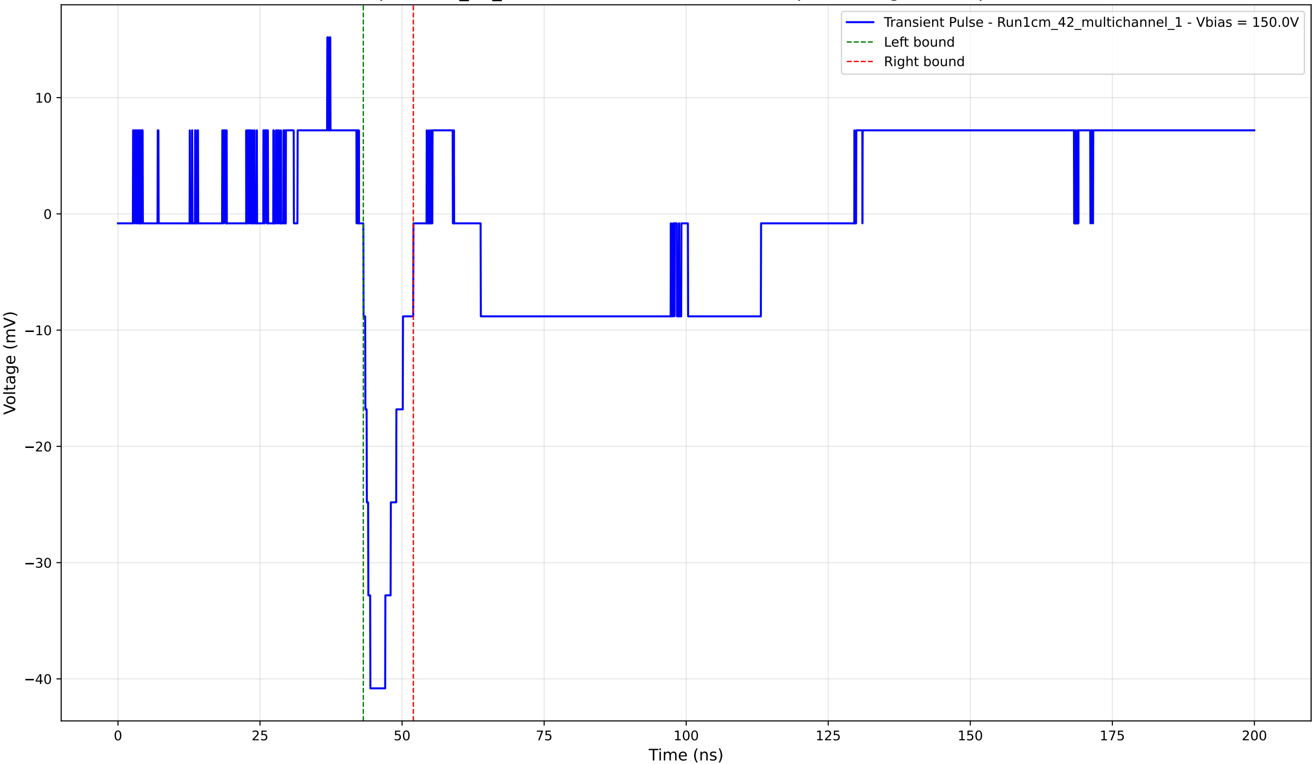
Transient Pulse - Sample: 1cm_42_multichannel - Position: 4240.0 \mu\text{m} - Charge: -4.50 pC - Rise Time: 1.21 ns
