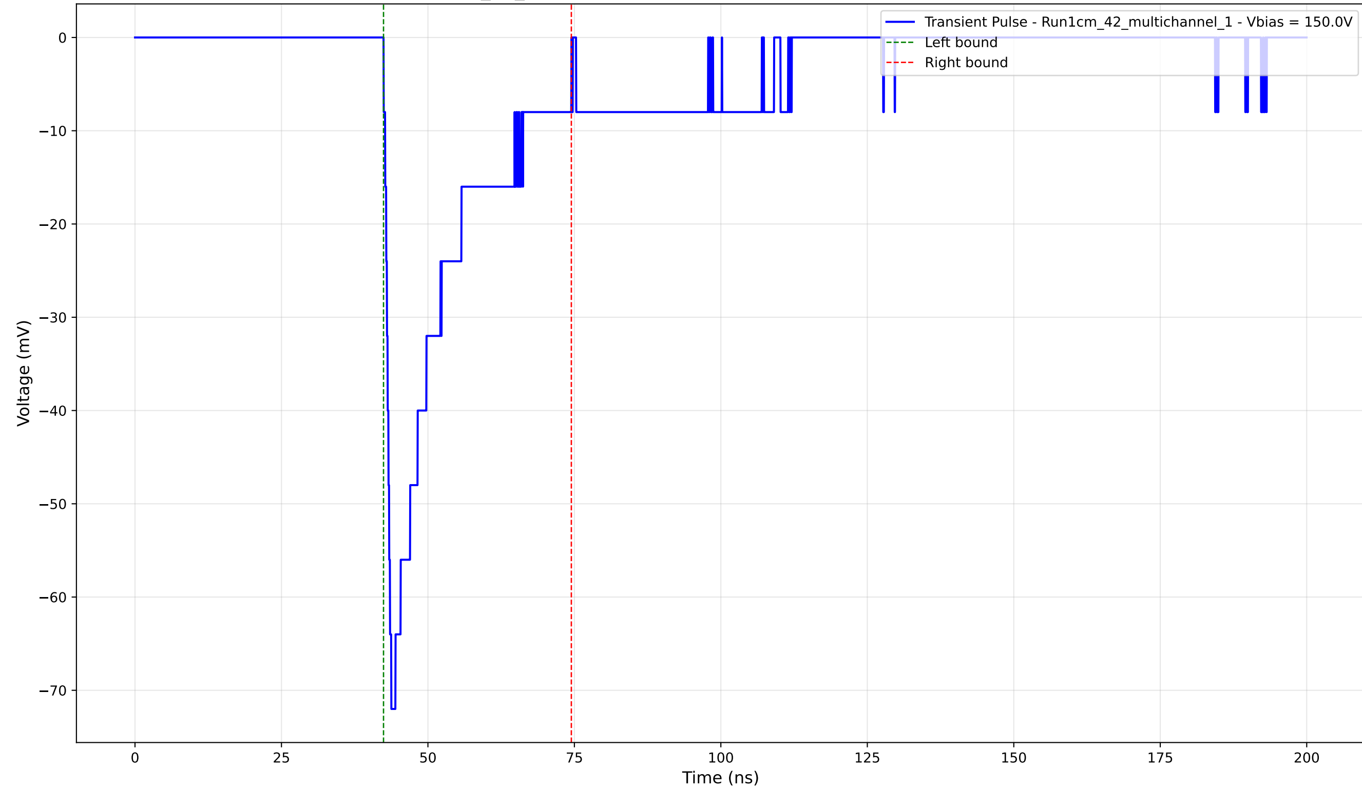
Transient Pulse - Sample: 1cm_42_multichannel - Position: 3470.0 \mu\text{m} - Charge: -15.16 pC - Rise Time: 1.30 ns
