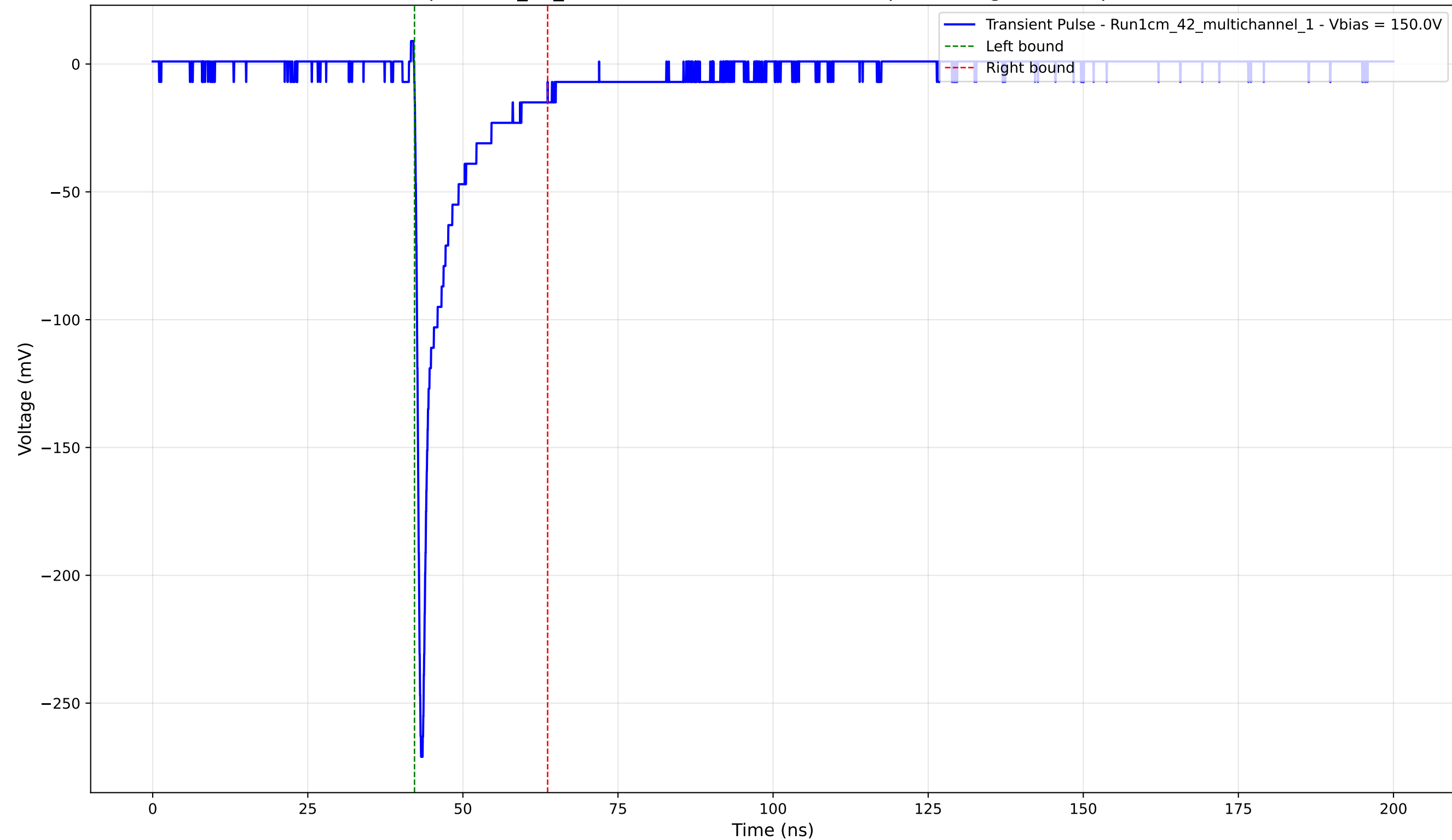
Transient Pulse - Sample: 1cm_42_multichannel - Position: 2035.0 \mu\text{m} - Charge: -23.47 pC - Rise Time: 0.79 ns
