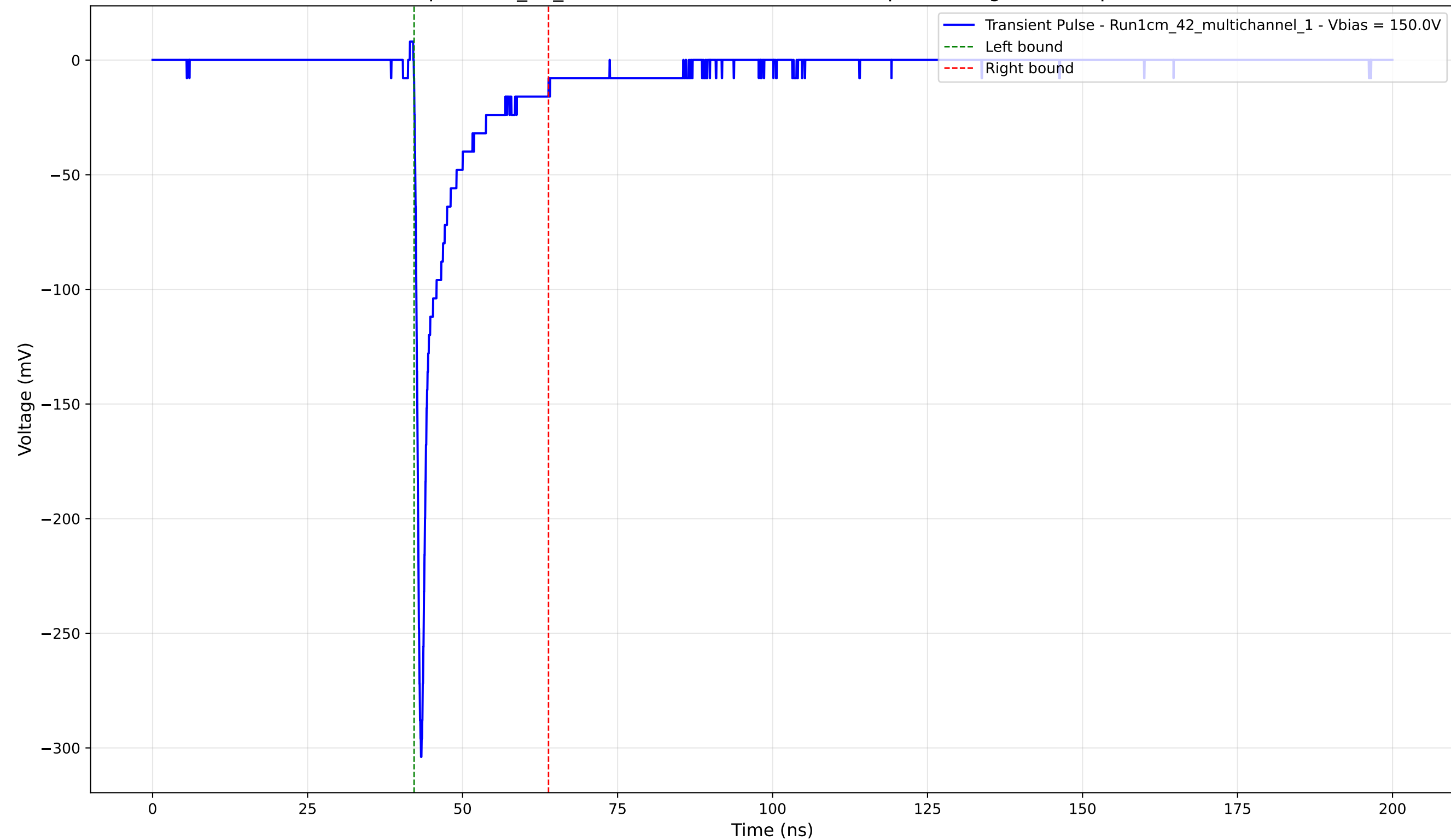
Transient Pulse - Sample: 1cm_42_multichannel - Position: 2090.0 \mu\text{m} - Charge: -23.89 pC - Rise Time: 0.82 ns
