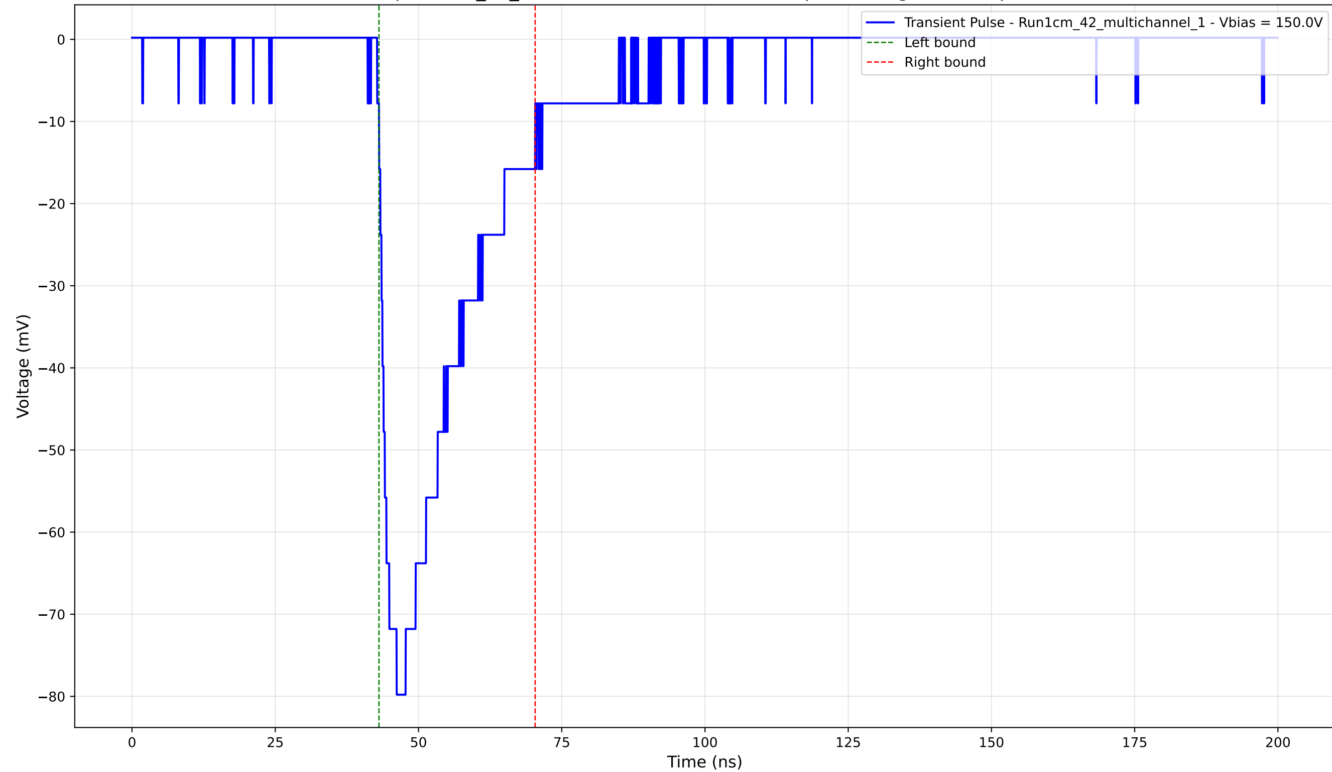
Transient Pulse - Sample: 1cm_42_multichannel - Position: 615.0 \mu\text{m} - Charge: -22.35 pC - Rise Time: 3.08 ns
