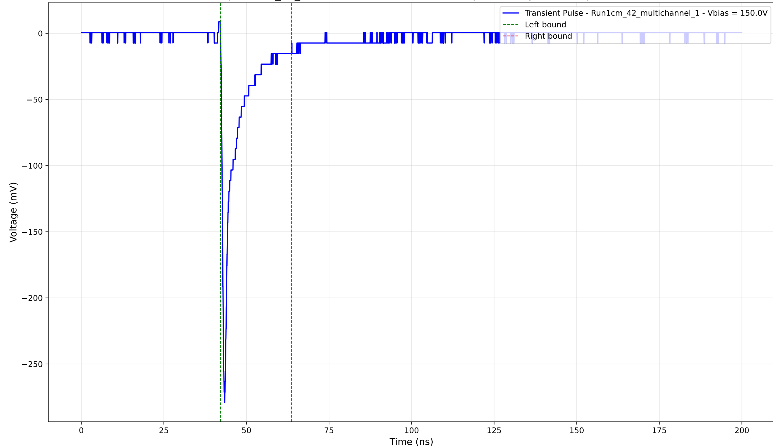
Transient Pulse - Sample: 1cm_42_multichannel - Position: 2030.0 \mu\text{m} - Charge: -23.64 pC - Rise Time: 0.79 ns
