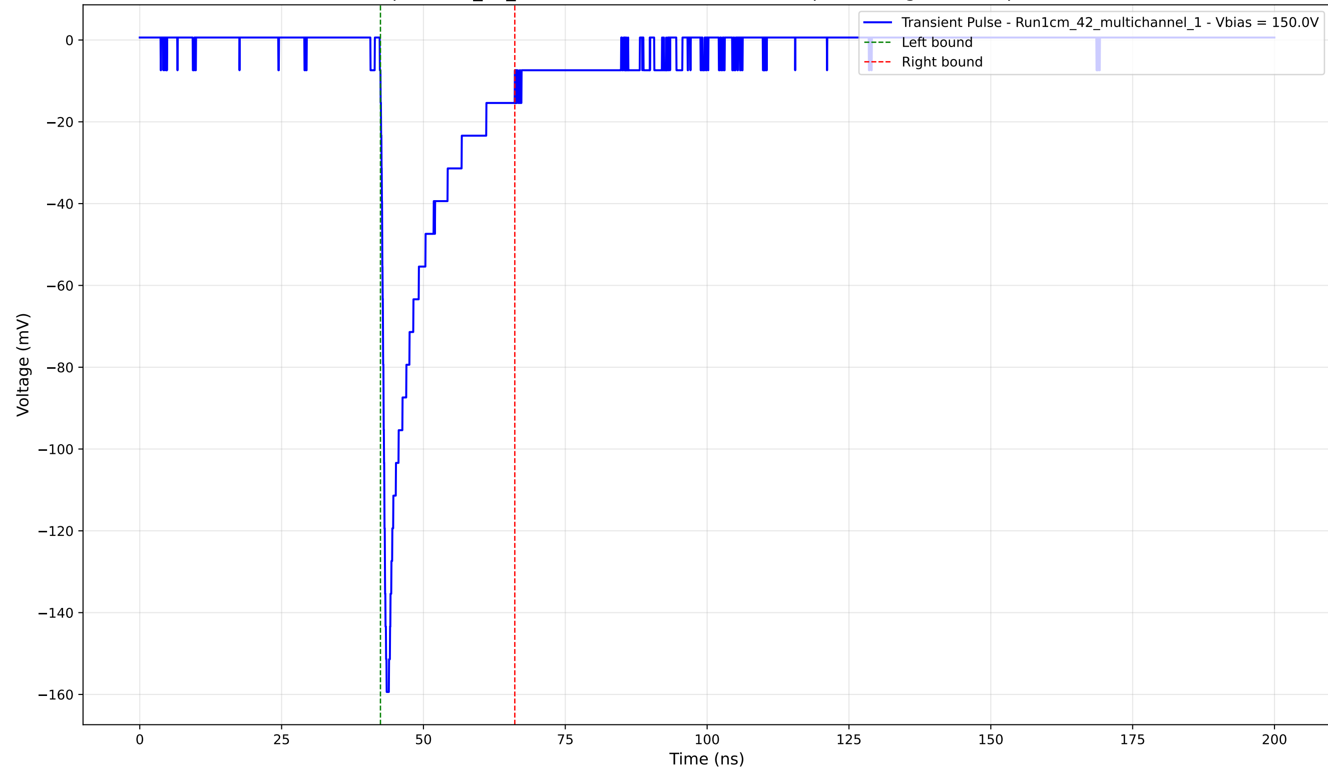
Transient Pulse - Sample: 1cm_42_multichannel - Position: 1690.0 \mu\text{m} - Charge: -22.54 pC - Rise Time: 0.90 ns
