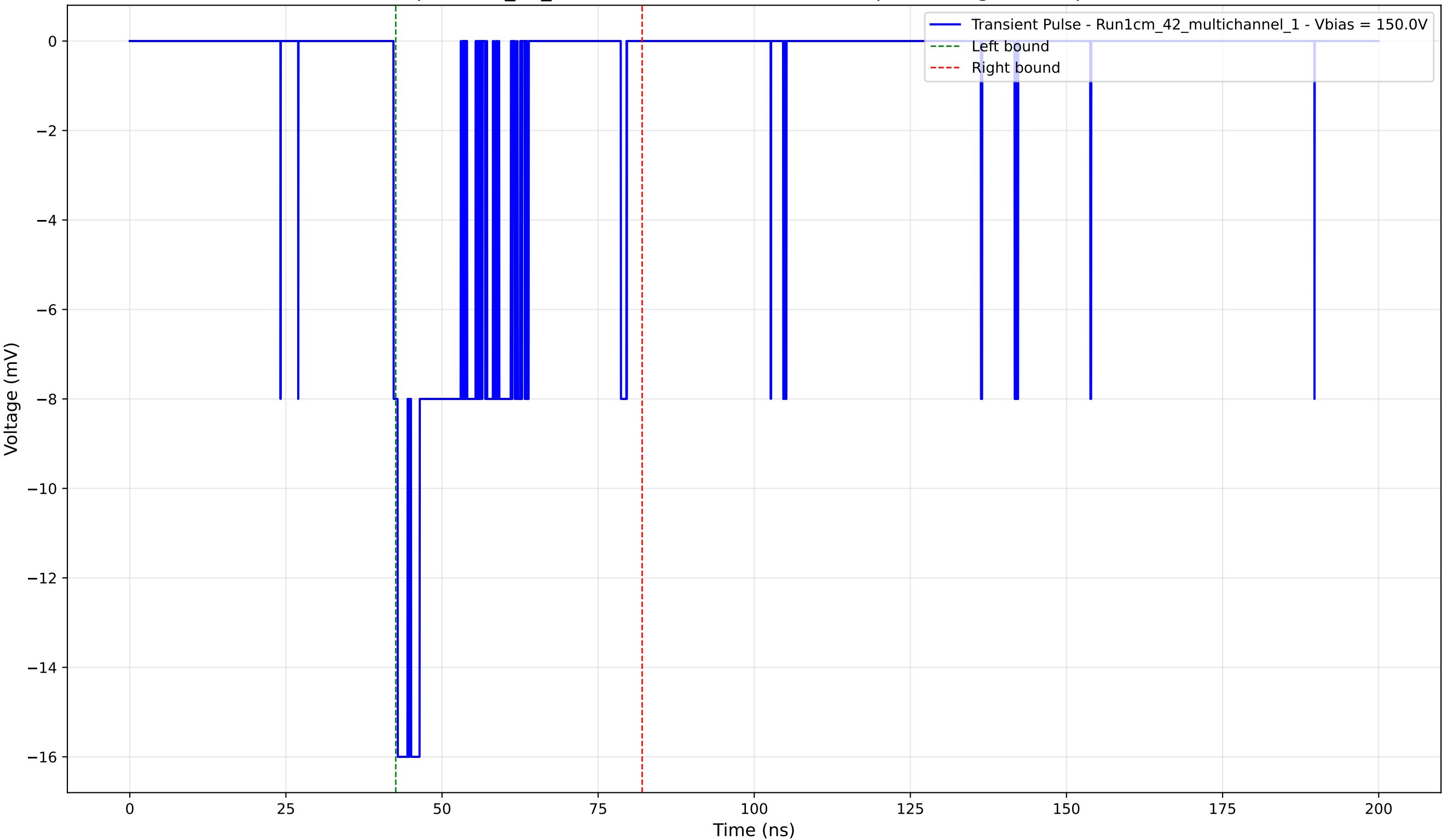
Transient Pulse - Sample: 1cm_42_multichannel - Position: 2920.0 \mu\text{m} - Charge: -3.56 pC - Rise Time: 0.68 ns
