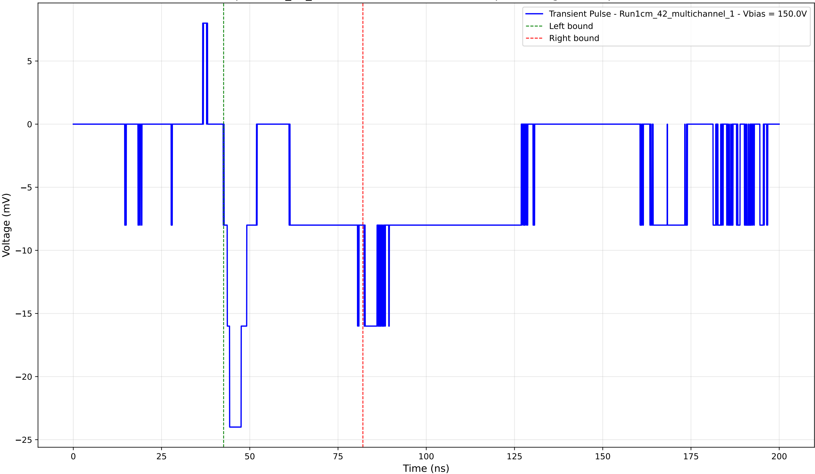
Transient Pulse - Sample: 1cm_42_multichannel - Position: 4455.0 \mu\text{m} - Charge: -6.23 pC - Rise Time: 1.57 ns
