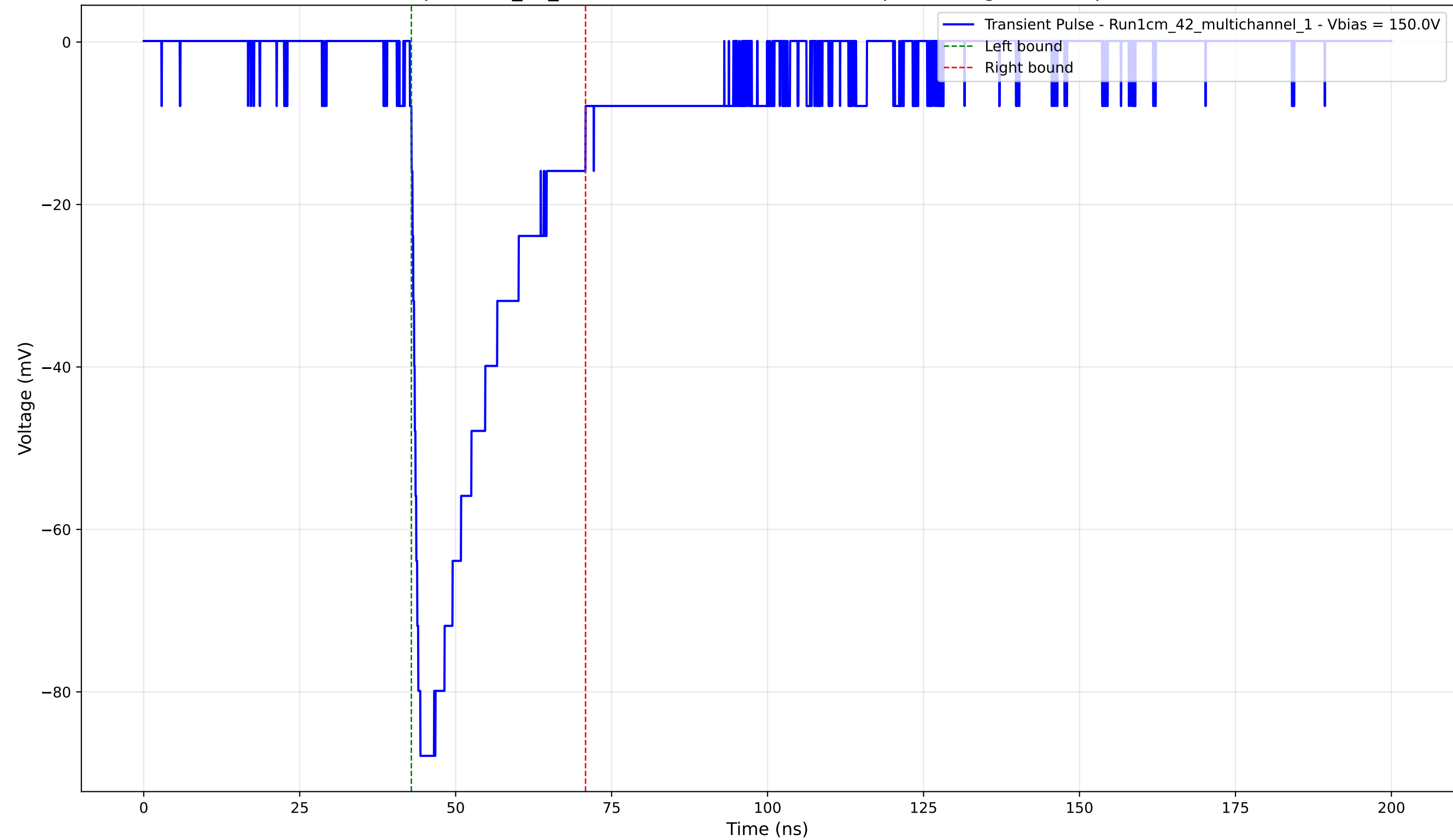
Transient Pulse - Sample: 1cm_42_multichannel - Position: 1045.0 \mu\text{m} - Charge: -23.45 pC - Rise Time: 1.10 ns
