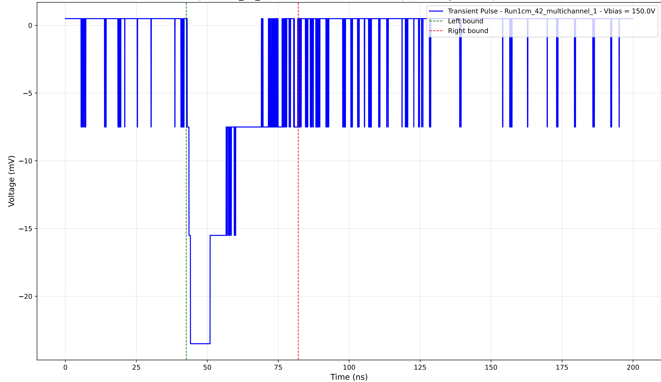
Transient Pulse - Sample: 1cm_42_multichannel - Position: 825.0 \mu\text{m} - Charge: -8.38 pC - Rise Time: 1.15 ns
