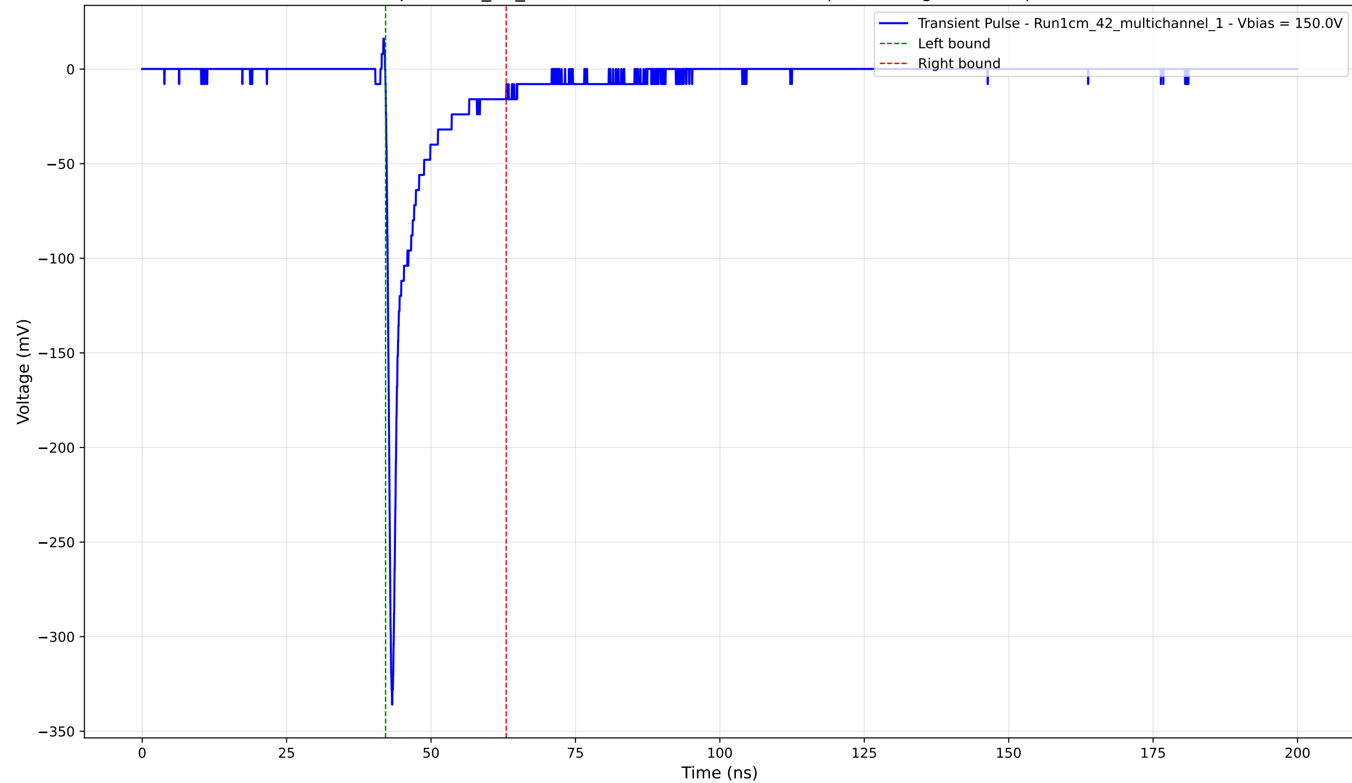
Transient Pulse - Sample: 1cm_42_multichannel - Position: 2150.0 \mu\text{m} - Charge: -24.15 pC - Rise Time: 0.77 ns
