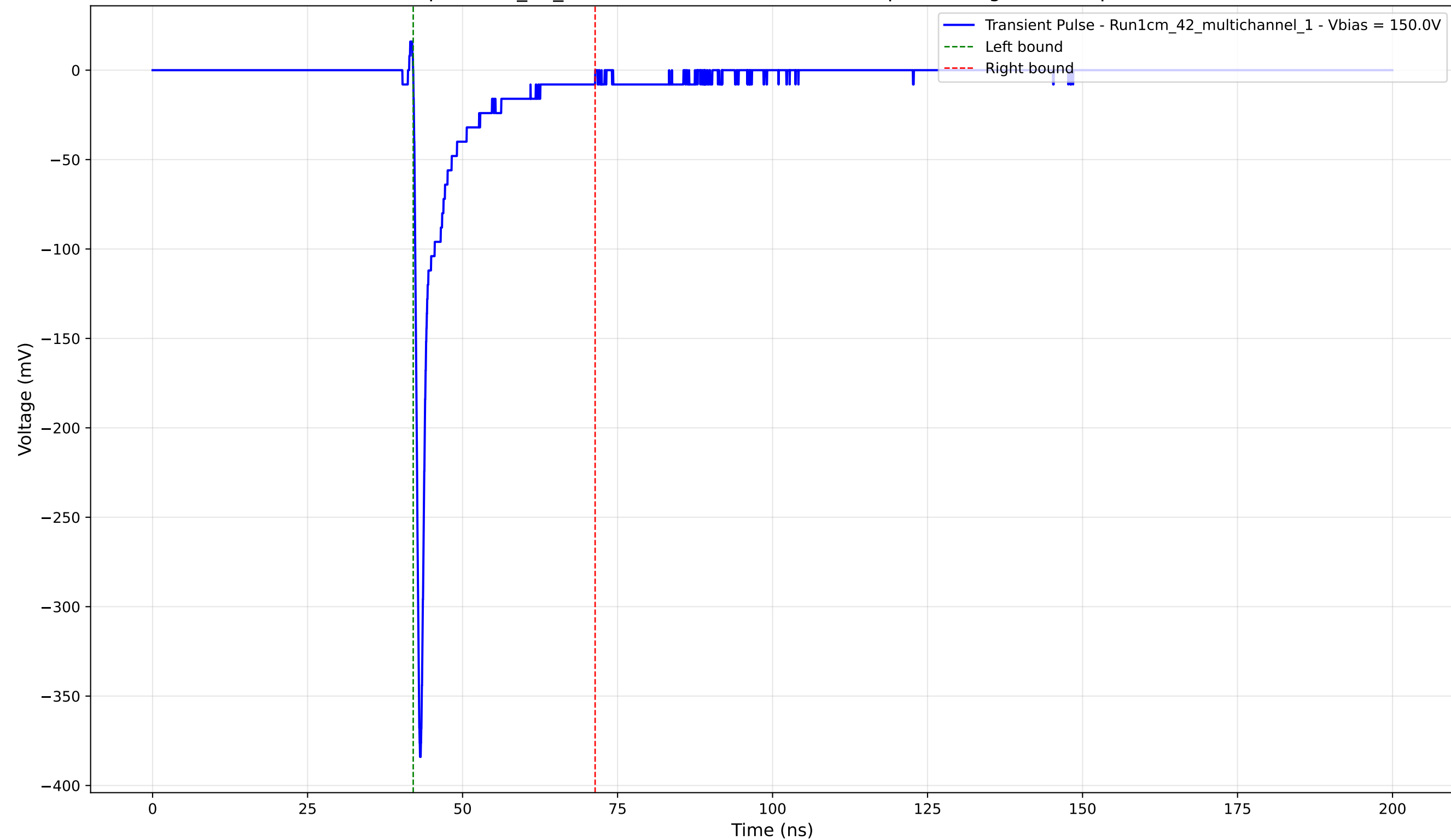
Transient Pulse - Sample: 1cm_42_multichannel - Position: 2520.0 \mu\text{m} - Charge: -25.60 pC - Rise Time: 0.76 ns
