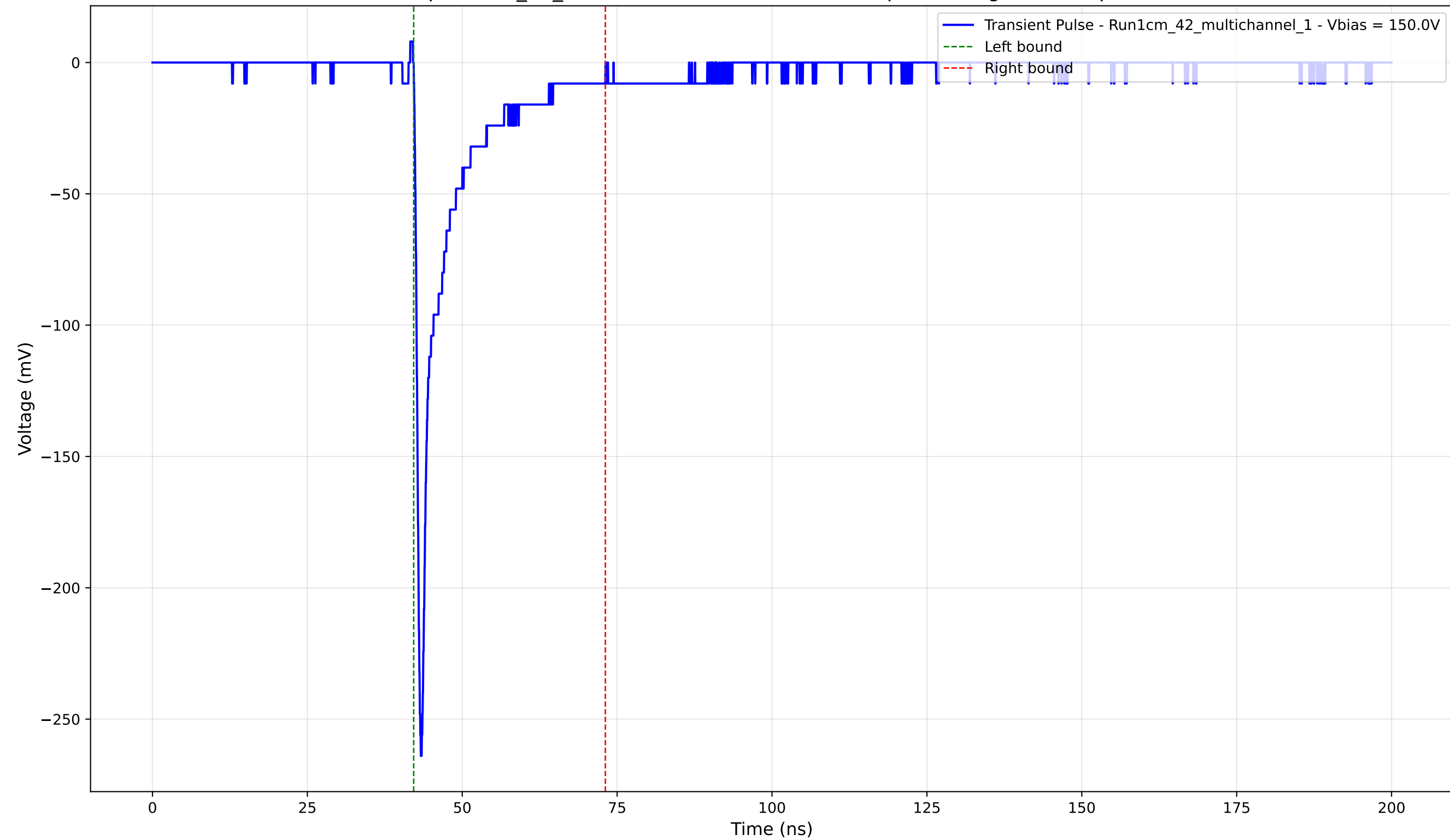
Transient Pulse - Sample: 1cm_42_multichannel - Position: 2745.0 \mu\text{m} - Charge: -24.11 pC - Rise Time: 0.79 ns
