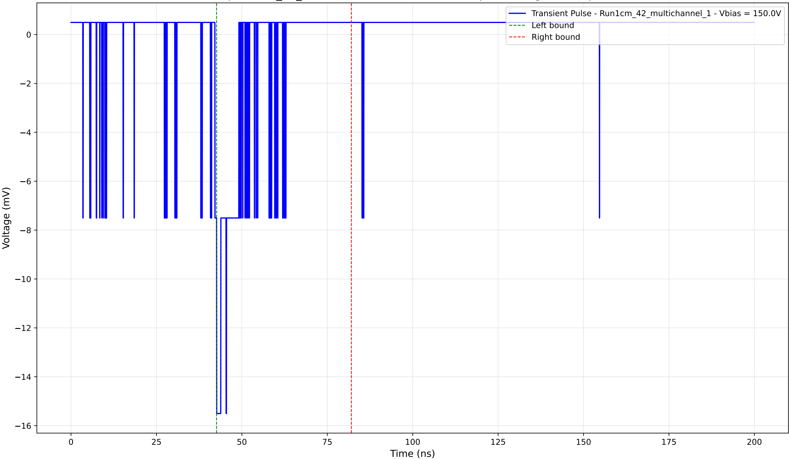
Transient Pulse - Sample: 1cm_42_multichannel - Position: 2400.0 \mu\text{m} - Charge: -1.25 pC - Rise Time: 0.52 ns
