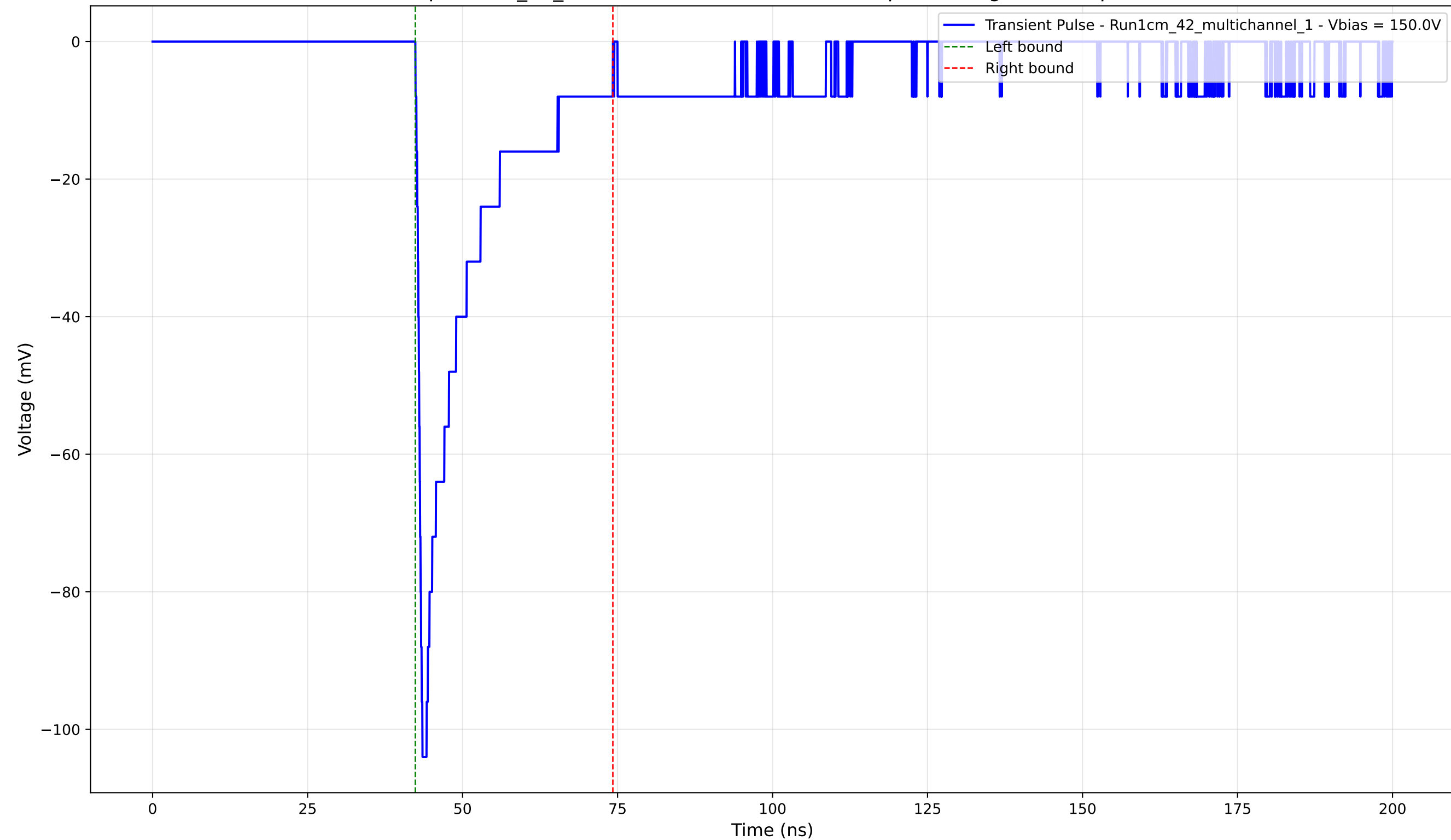
Transient Pulse - Sample: 1cm_42_multichannel - Position: 3255.0 \mu\text{m} - Charge: -17.31 pC - Rise Time: 0.85 ns
