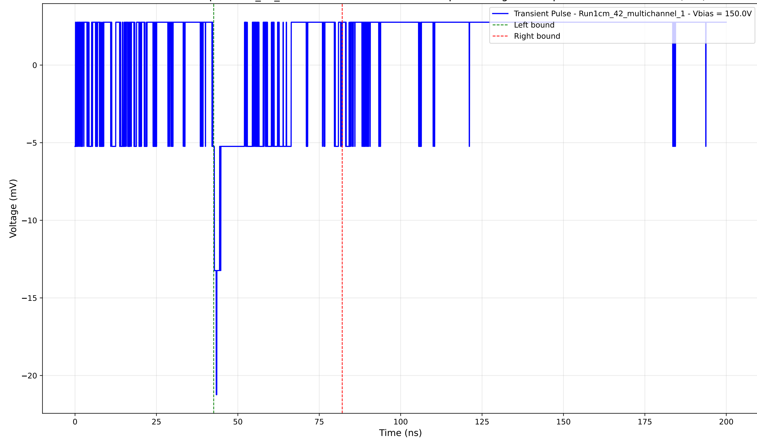
Transient Pulse - Sample: 1cm_42_multichannel - Position: 2870.0 \mu\text{m} - Charge: -1.66 pC - Rise Time: 0.00 ns (N/A)
