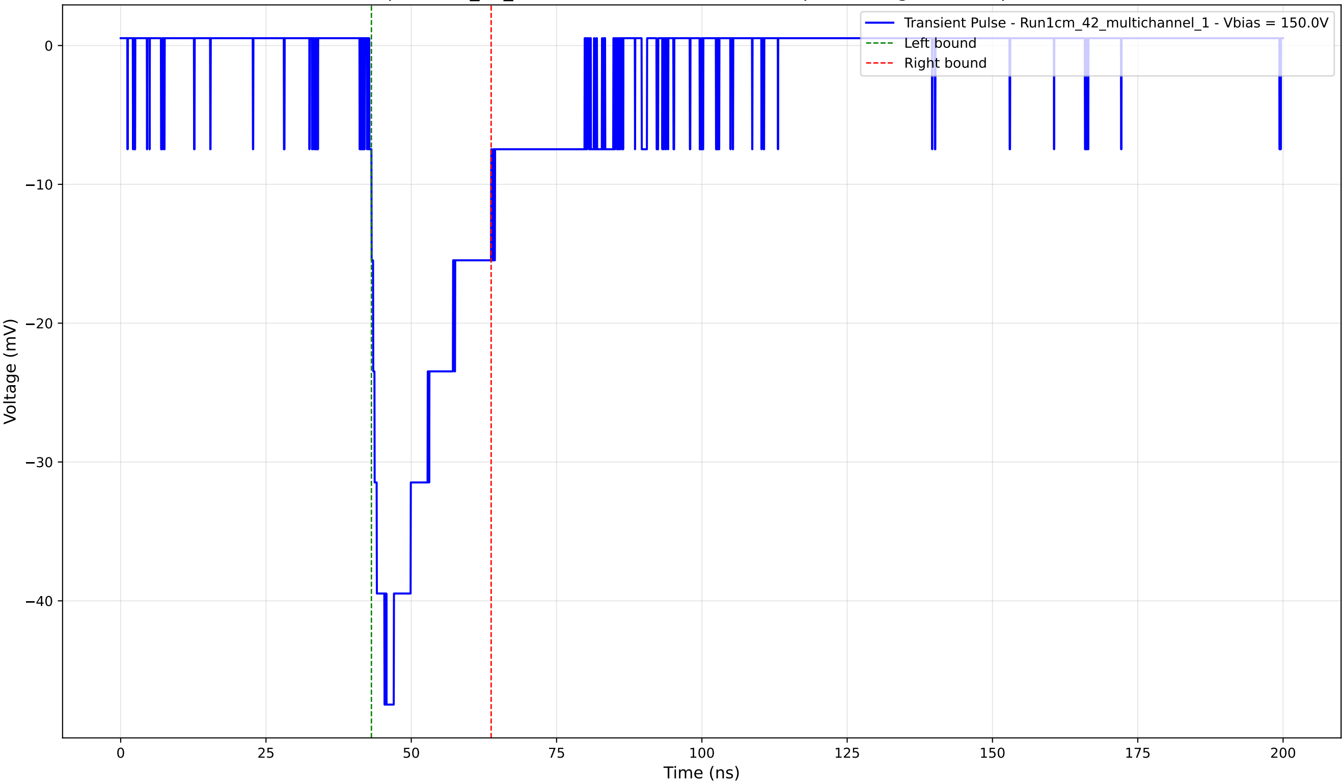
Transient Pulse - Sample: 1cm_42_multichannel - Position: 920.0 \mu\text{m} - Charge: -11.23 pC - Rise Time: 2.61 ns
