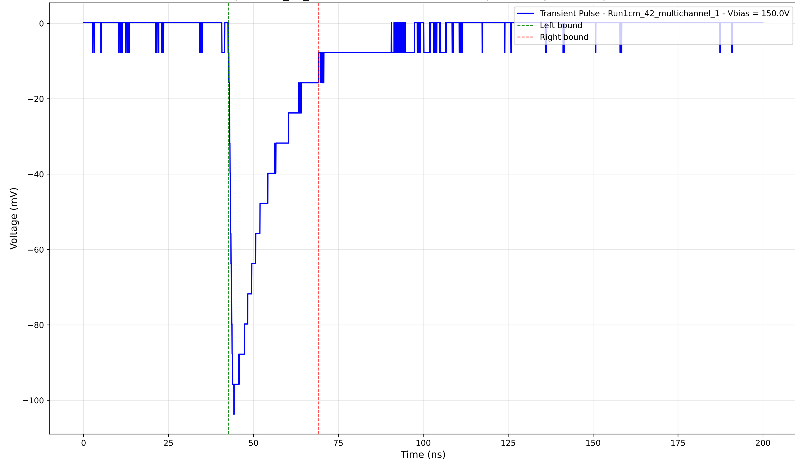
Transient Pulse - Sample: 1cm_42_multichannel - Position: 1235.0 \mu\text{m} - Charge: -23.53 pC - Rise Time: 1.11 ns
