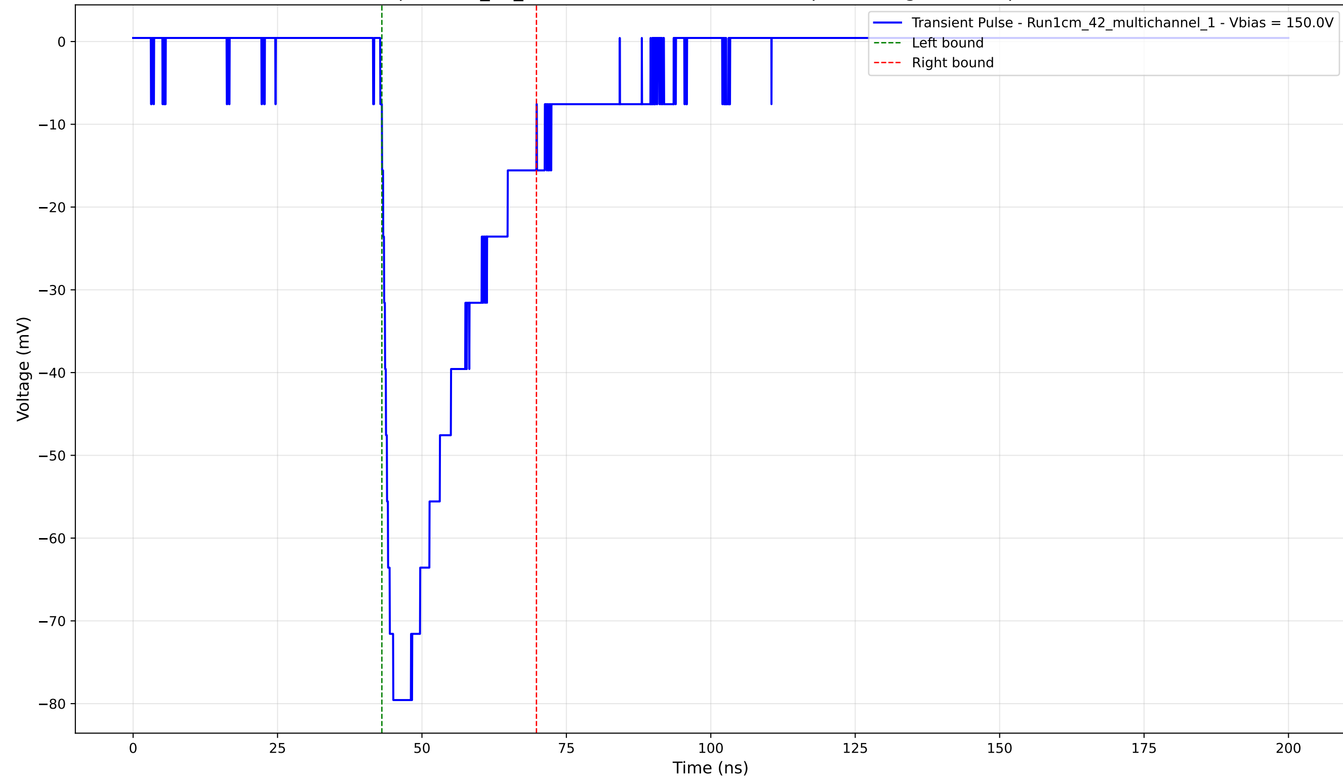
Transient Pulse - Sample: 1cm_42_multichannel - Position: 750.0 \mu\text{m} - Charge: -22.55 pC - Rise Time: 1.96 ns
