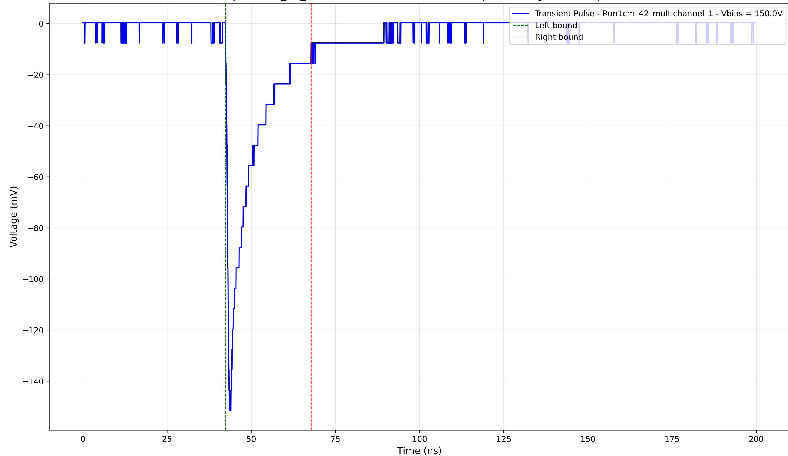
Transient Pulse - Sample: 1cm_42_multichannel - Position: 1655.0 \mu\text{m} - Charge: -23.12 pC - Rise Time: 0.96 ns
