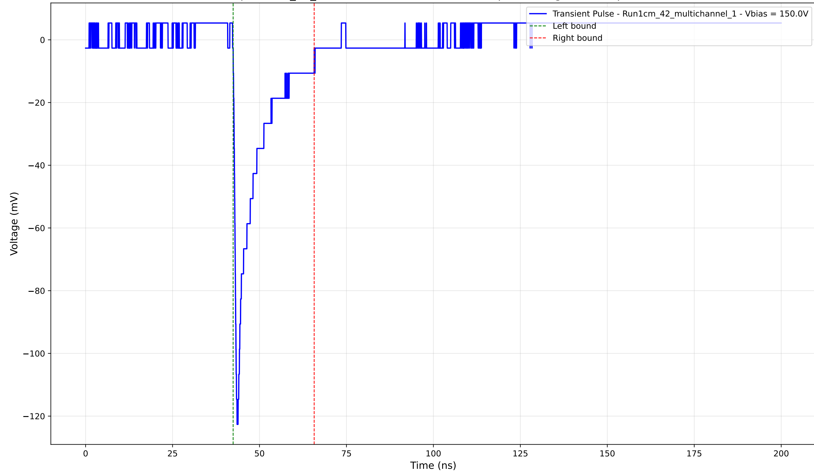
Transient Pulse - Sample: 1cm_42_multichannel - Position: 3140.0 \mu\text{m} - Charge: -15.10 pC - Rise Time: 0.86 ns
