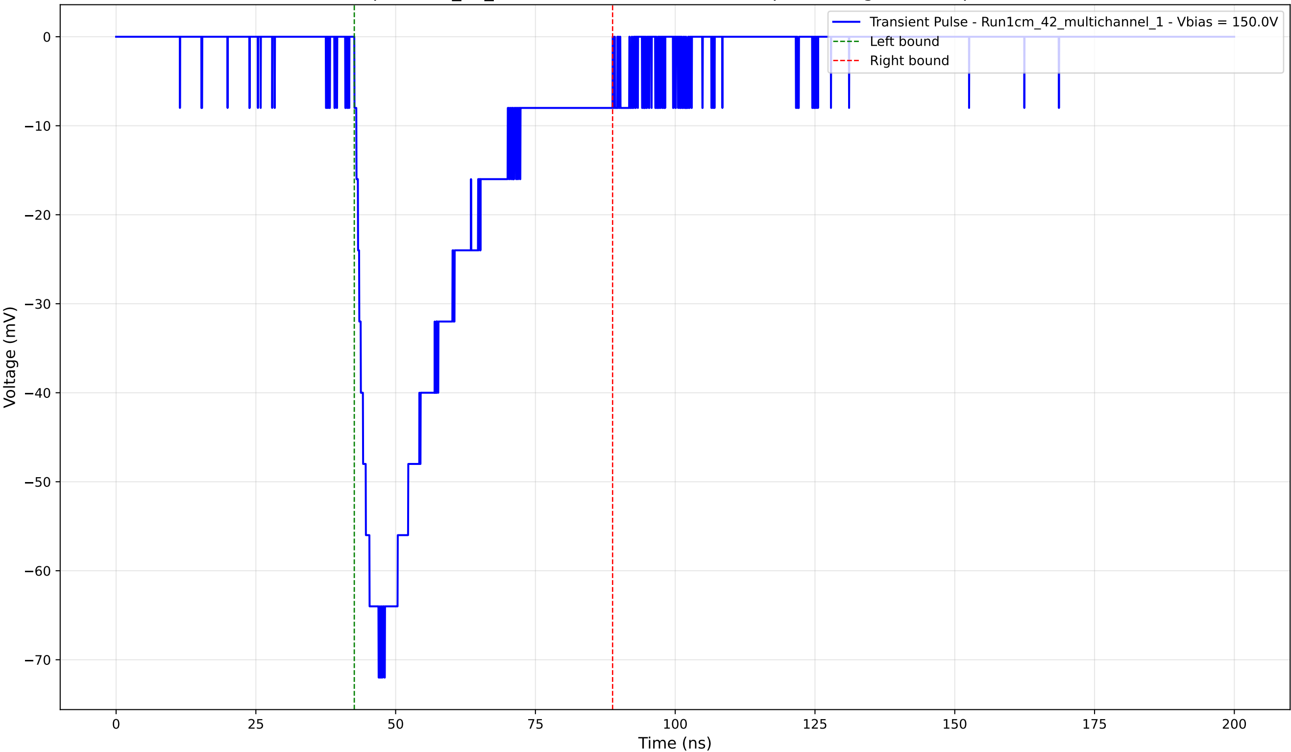
Transient Pulse - Sample: 1cm_42_multichannel - Position: 215.0 \mu\text{m} - Charge: -23.97 pC - Rise Time: 4.32 ns
