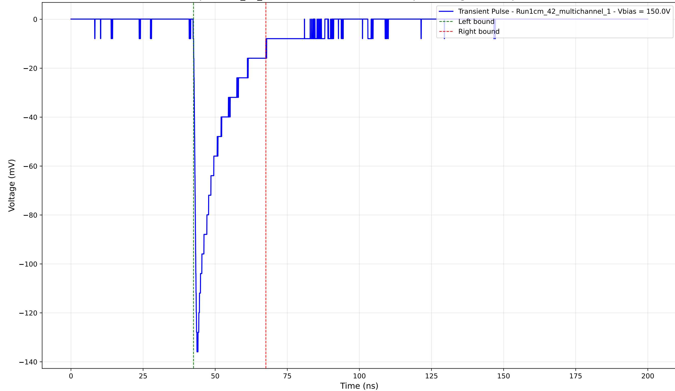
Transient Pulse - Sample: 1cm_42_multichannel - Position: 1550.0 \mu\text{m} - Charge: -22.83 pC - Rise Time: 1.01 ns
