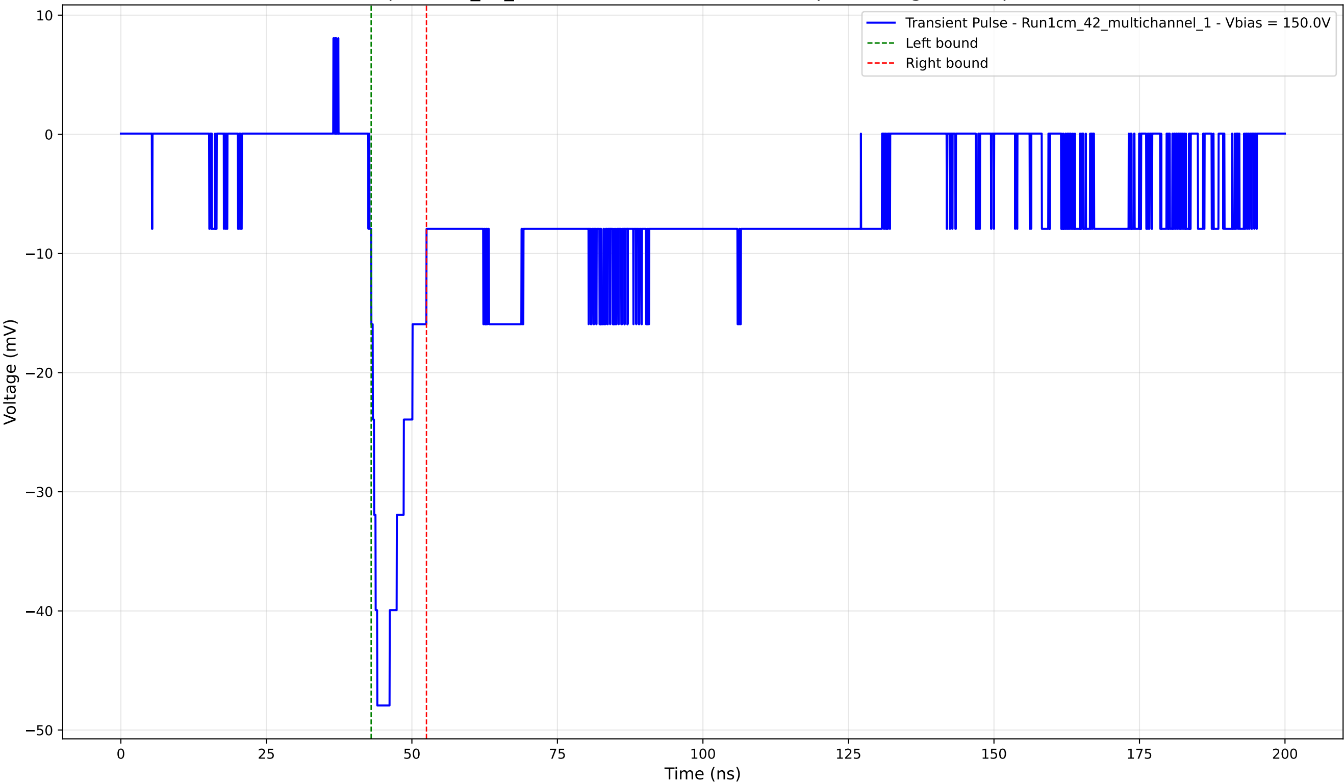
Transient Pulse - Sample: 1cm_42_multichannel - Position: 3835.0 \mu\text{m} - Charge: -5.86 pC - Rise Time: 1.35 ns
