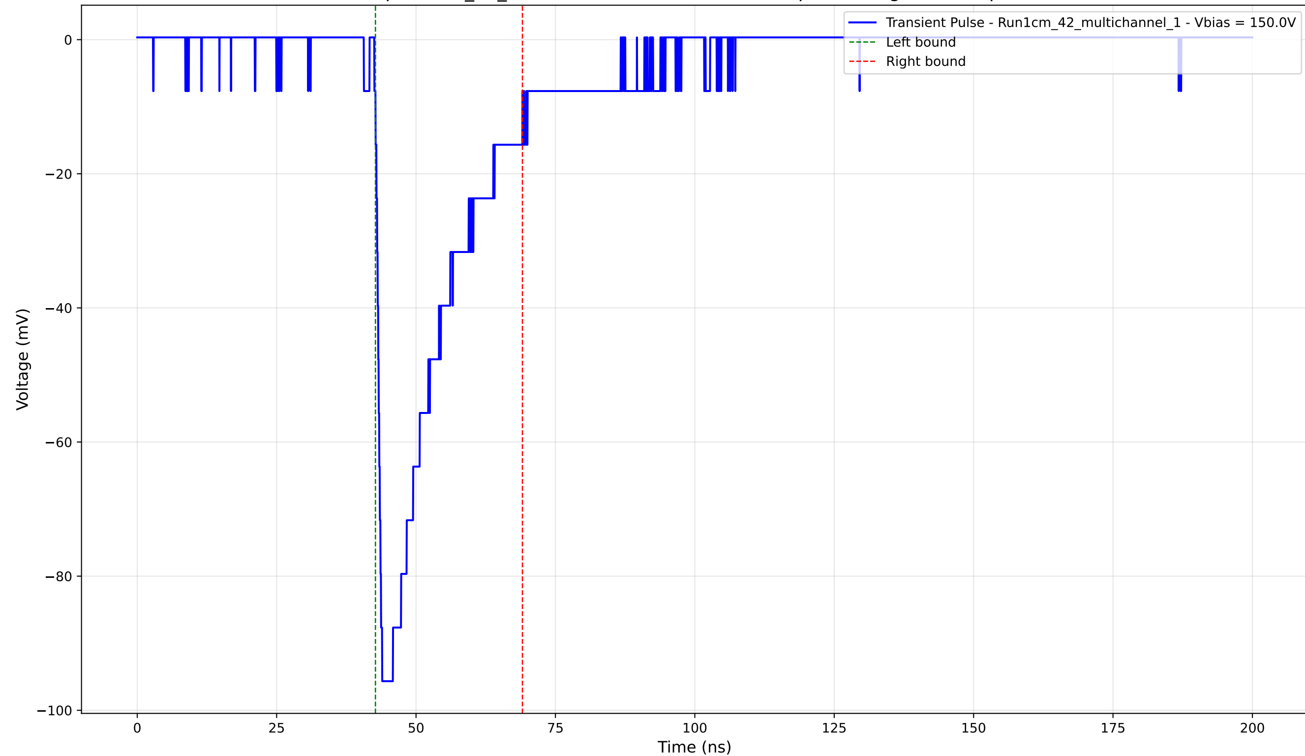
Transient Pulse - Sample: 1cm_42_multichannel - Position: 1225.0 \mu\text{m} - Charge: -23.42 pC - Rise Time: 1.00 ns
