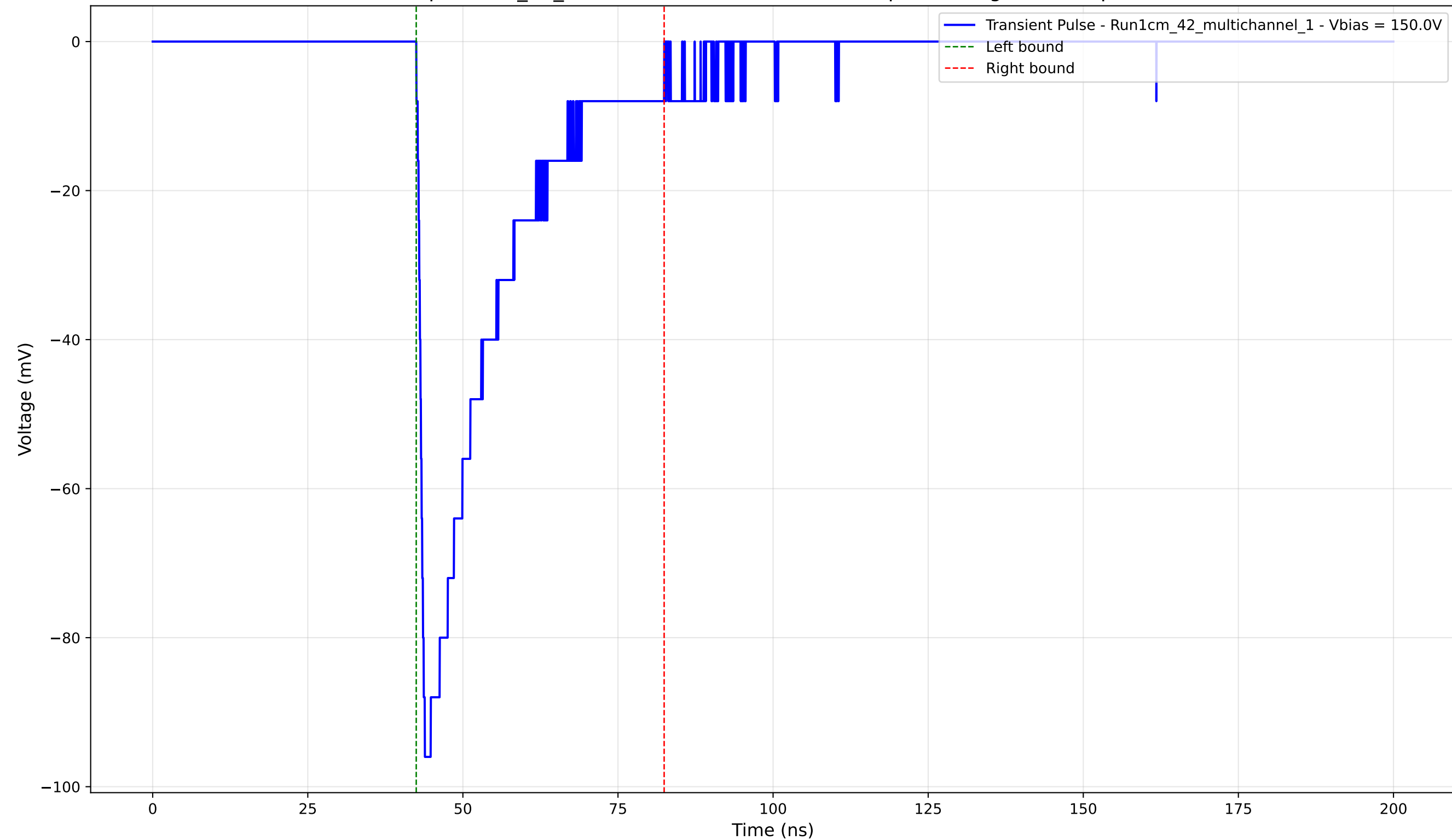
Transient Pulse - Sample: 1cm_42_multichannel - Position: 1285.0 \mu\text{m} - Charge: -24.06 pC - Rise Time: 0.98 ns
