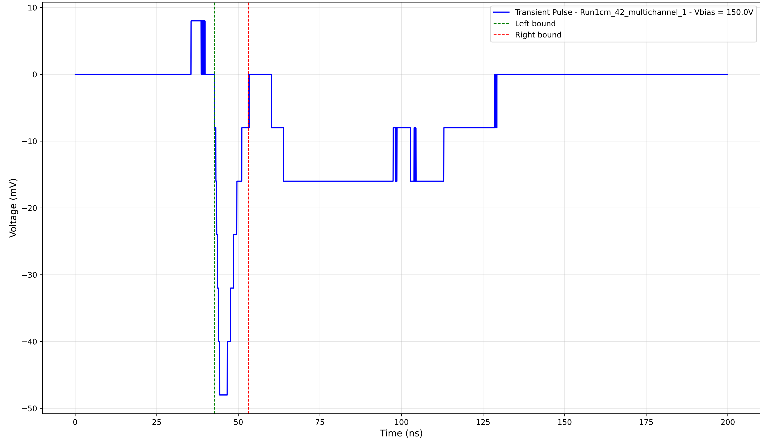
Transient Pulse - Sample: 1cm_42_multichannel - Position: 4030.0 \mu\text{m} - Charge: -5.67 pC - Rise Time: 1.53 ns
