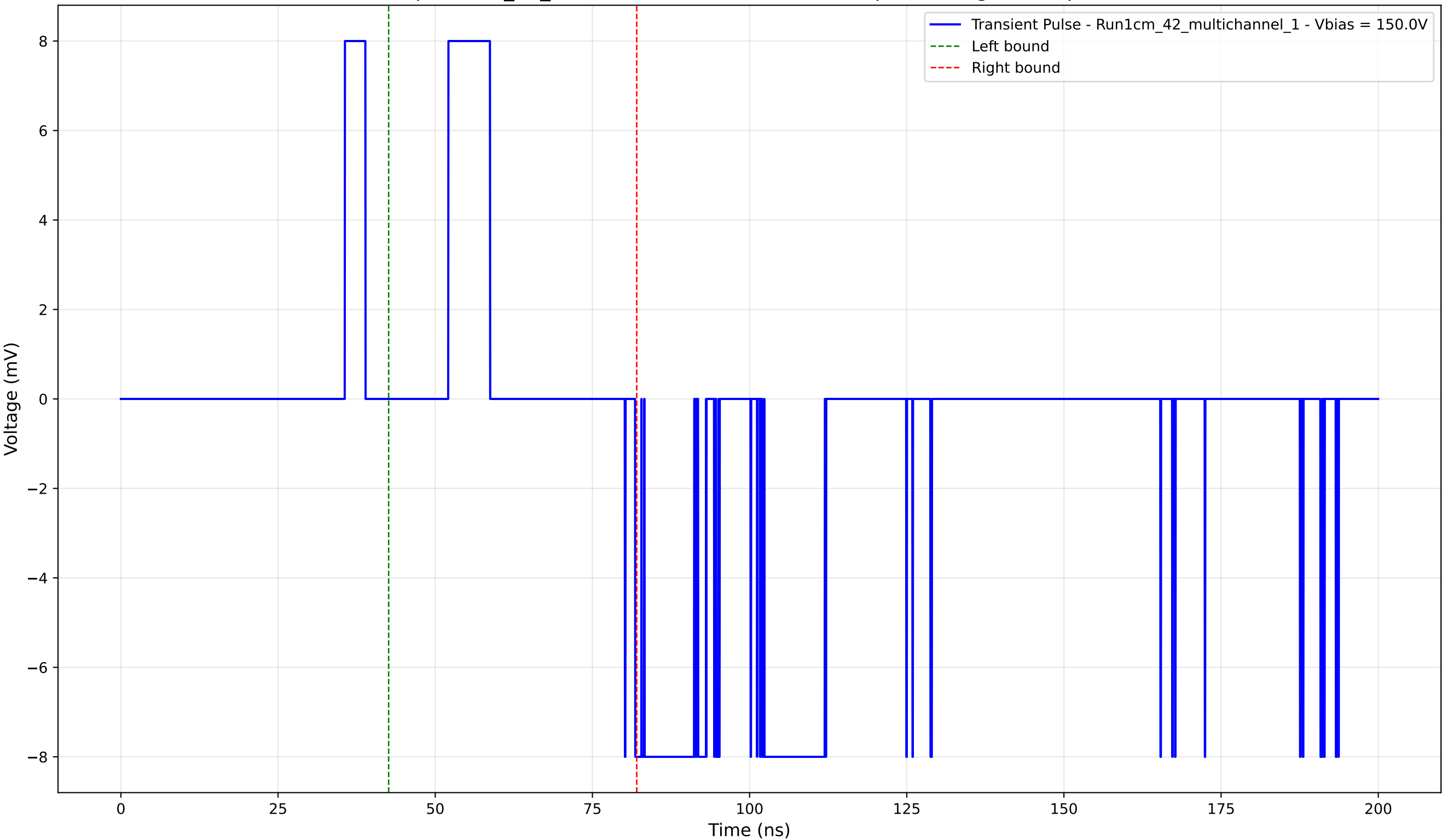
Transient Pulse - Sample: 1cm_42_multichannel - Position: 4400.0 \mu\text{m} - Charge: 1.01 pC - Rise Time: 0.02 ns
