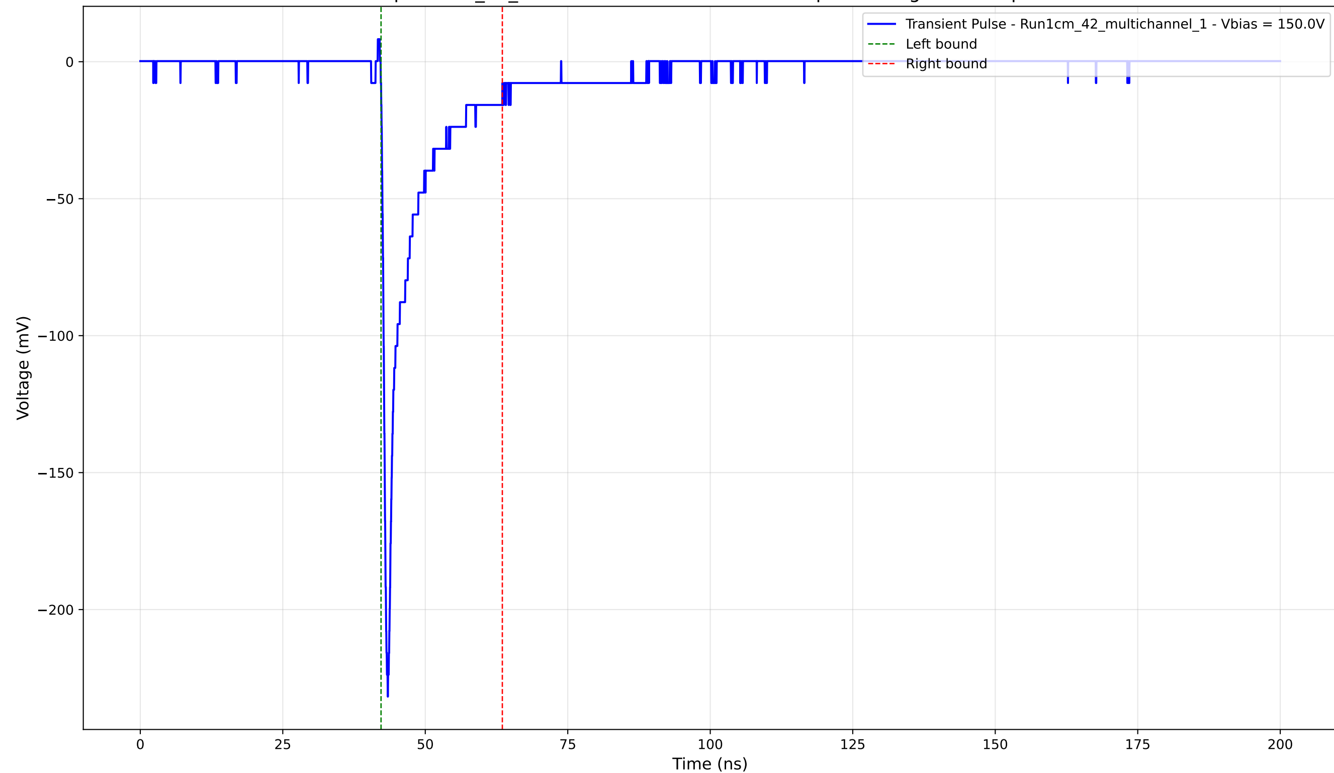
Transient Pulse - Sample: 1cm_42_multichannel - Position: 2795.0 \mu\text{m} - Charge: -21.02 pC - Rise Time: 0.86 ns
