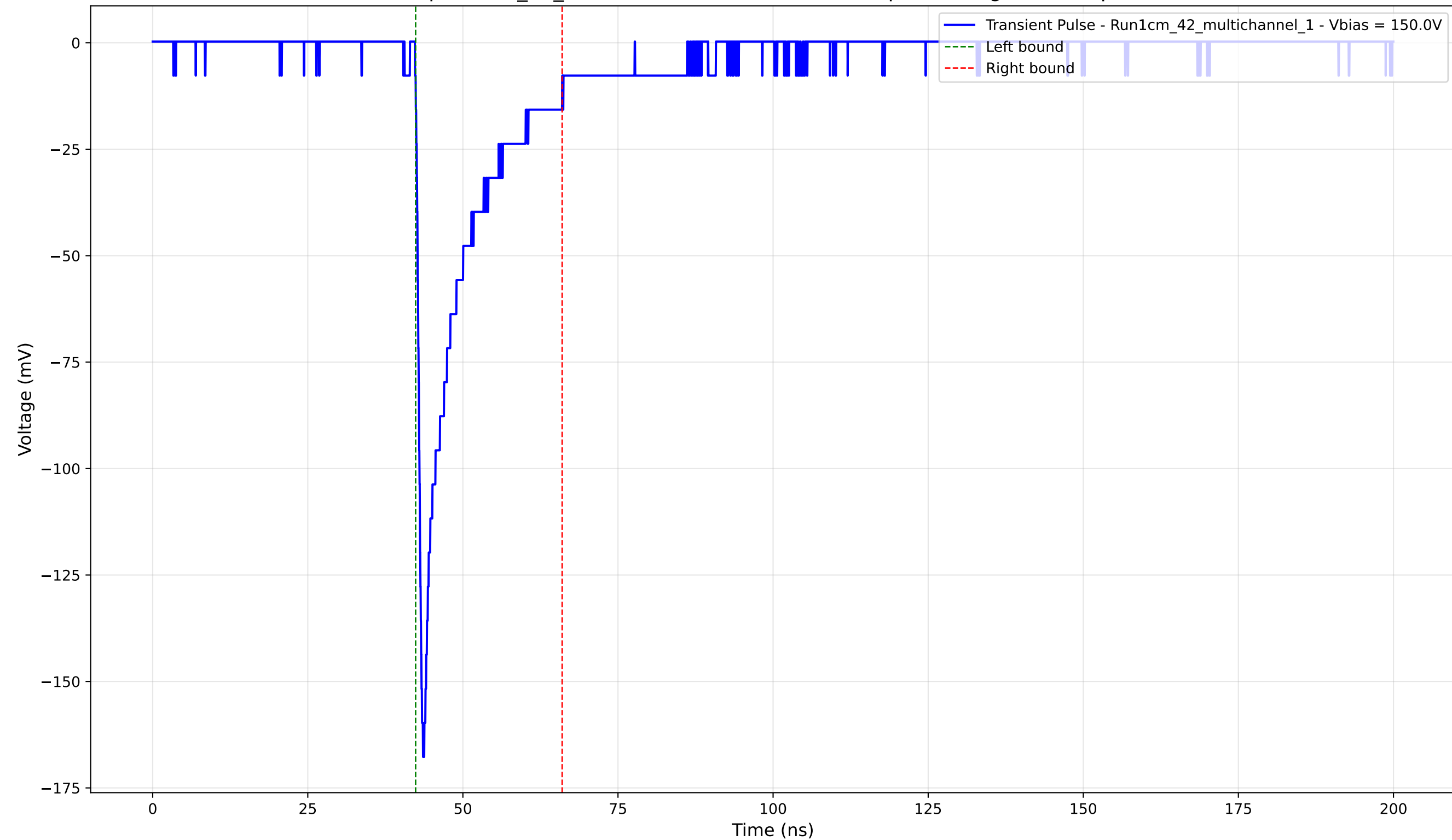
Transient Pulse - Sample: 1cm_42_multichannel - Position: 1715.0 \mu\text{m} - Charge: -22.36 pC - Rise Time: 0.86 ns
