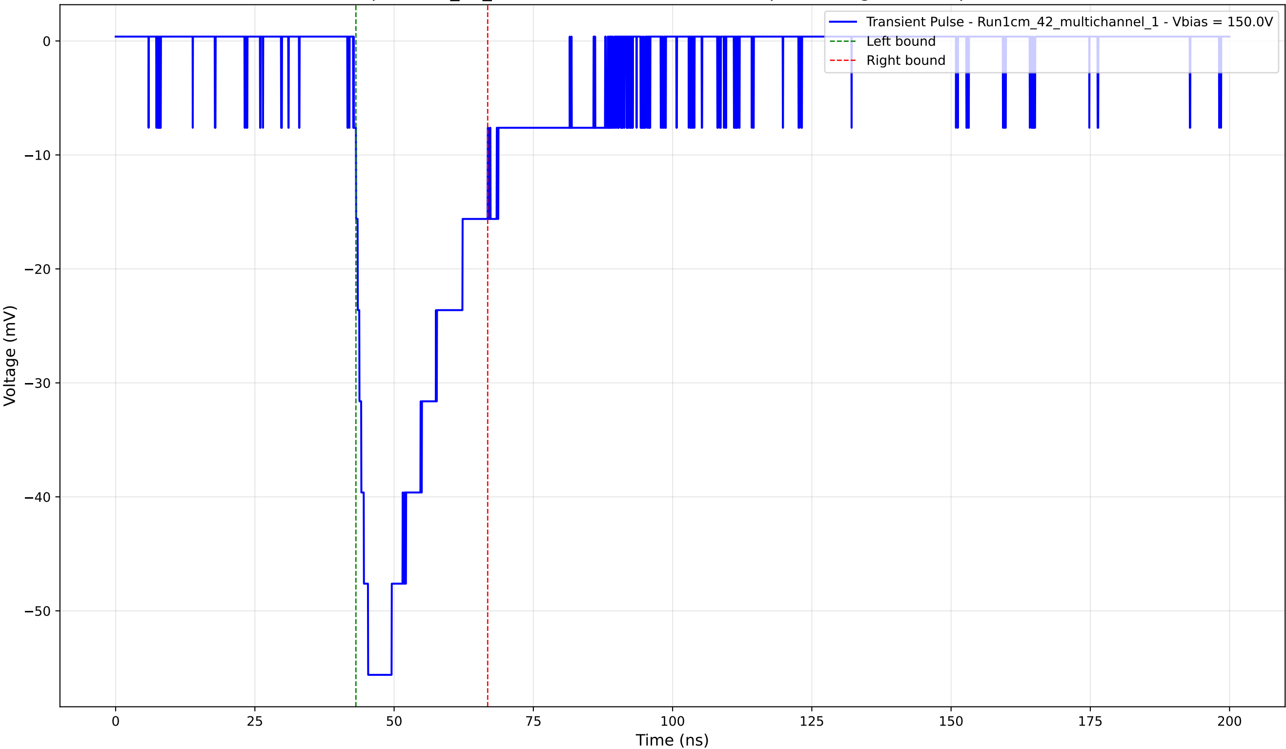
Transient Pulse - Sample: 1cm_42_multichannel - Position: 425.0 \mu\text{m} - Charge: -16.20 pC - Rise Time: 2.55 ns
