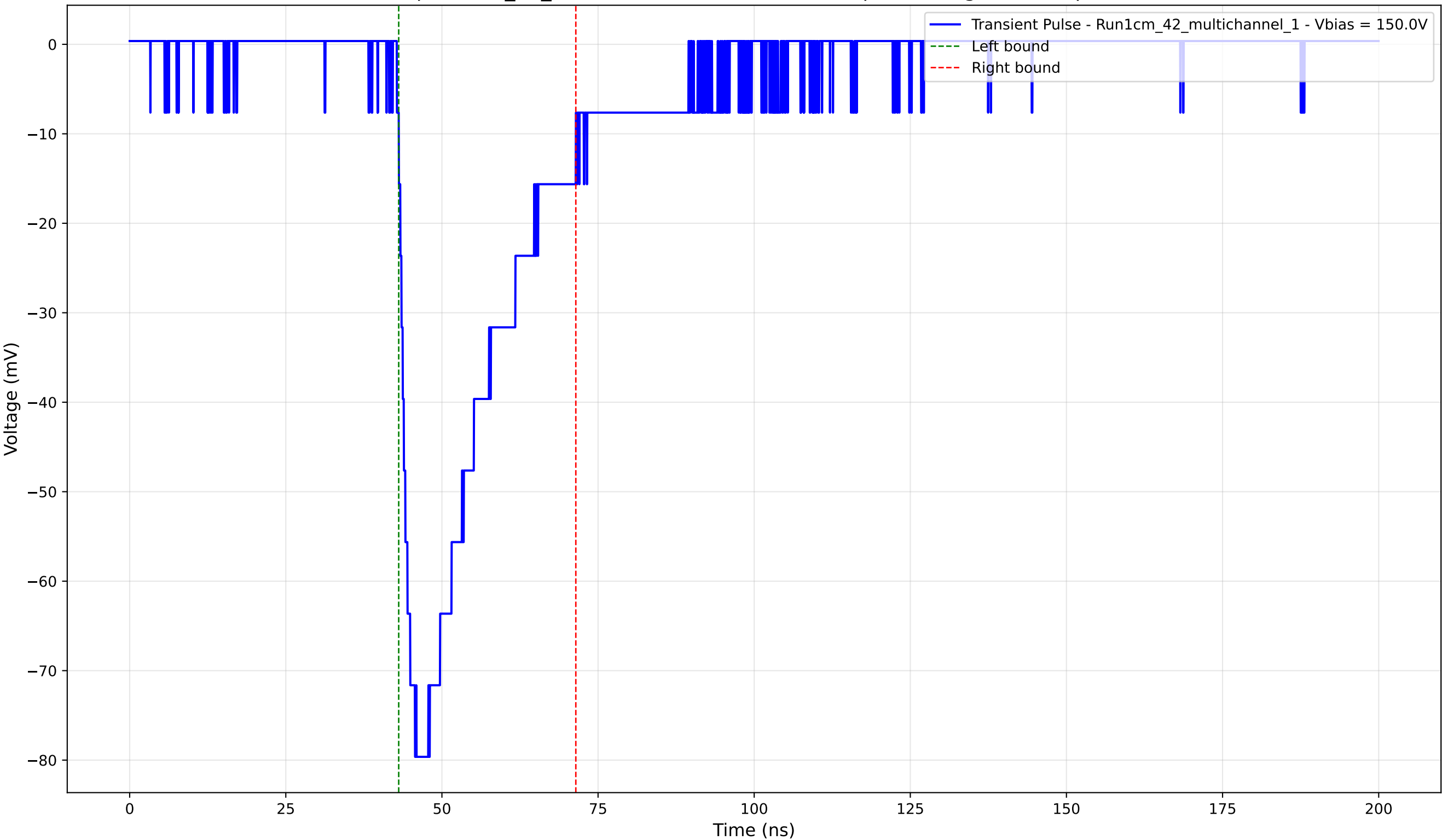
Transient Pulse - Sample: 1cm_42_multichannel - Position: 585.0 \mu\text{m} - Charge: -23.03 pC - Rise Time: 2.60 ns
