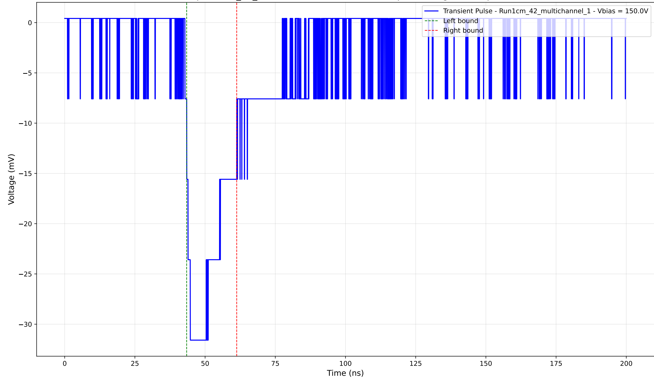
Transient Pulse - Sample: 1cm_42_multichannel - Position: 410.0 \mu\text{m} - Charge: -8.34 pC - Rise Time: 1.91 ns
