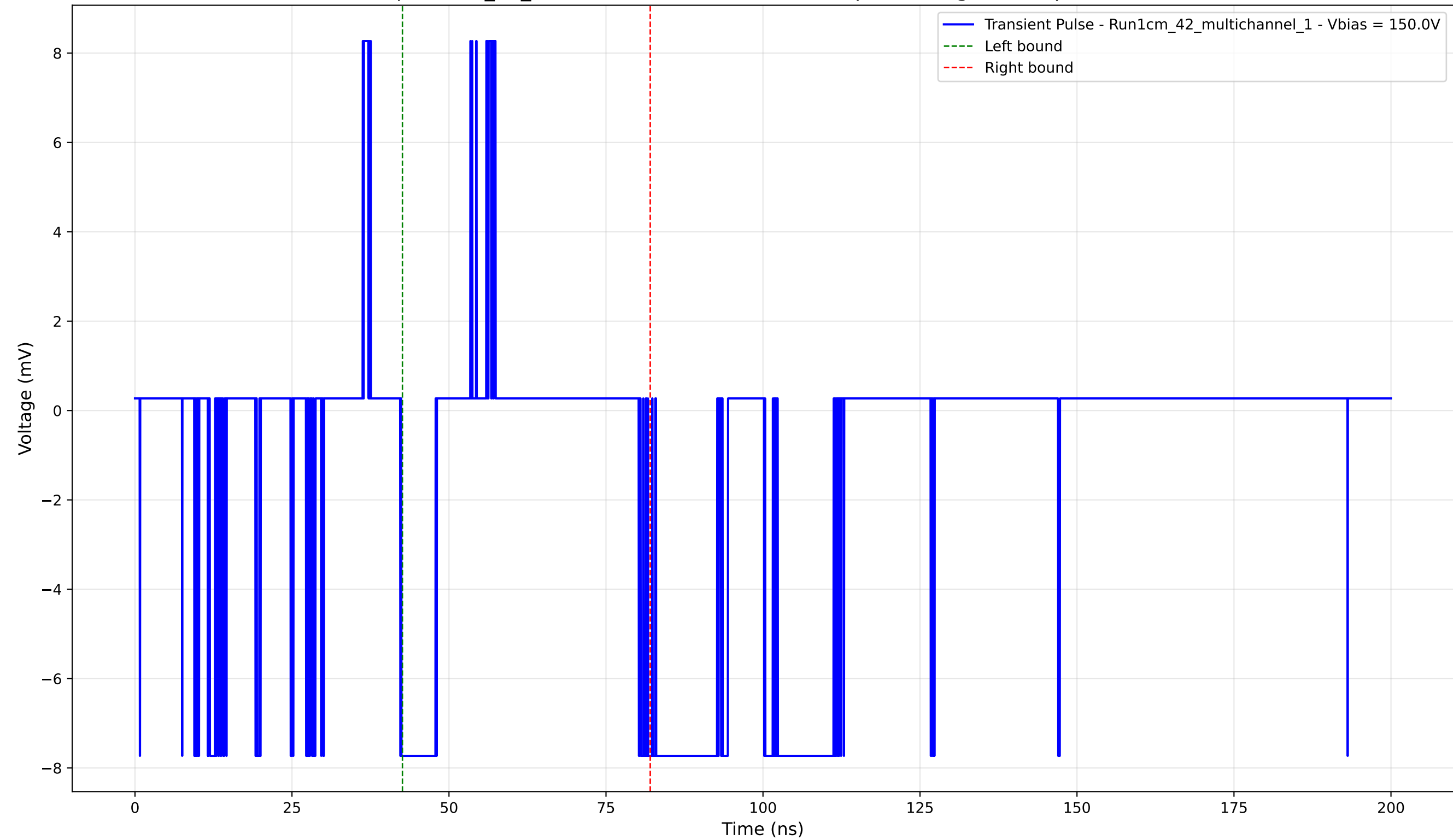
Transient Pulse - Sample: 1cm_42_multichannel - Position: 3910.0 \mu\text{m} - Charge: -0.67 pC - Rise Time: 0.00 ns (N/A)
