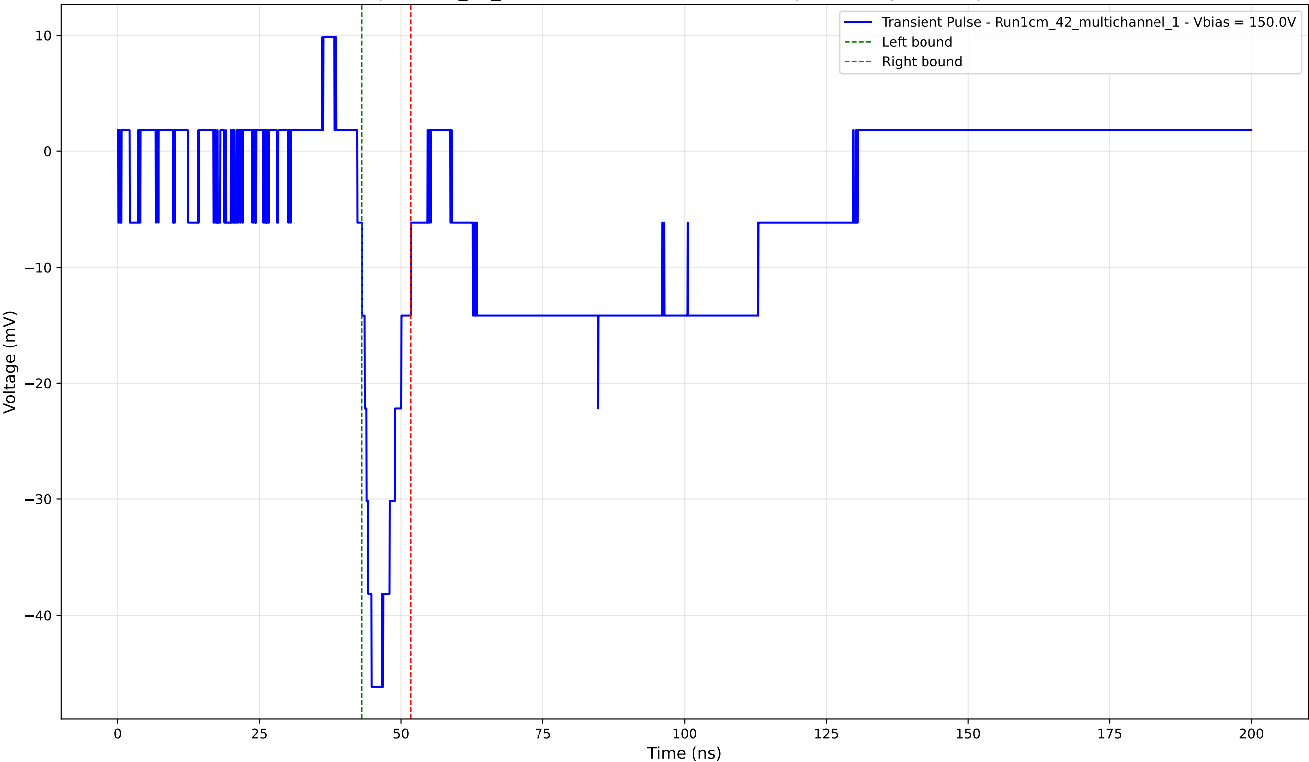
Transient Pulse - Sample: 1cm_42_multichannel - Position: 4645.0 \mu\text{m} - Charge: -5.25 pC - Rise Time: 2.49 ns
