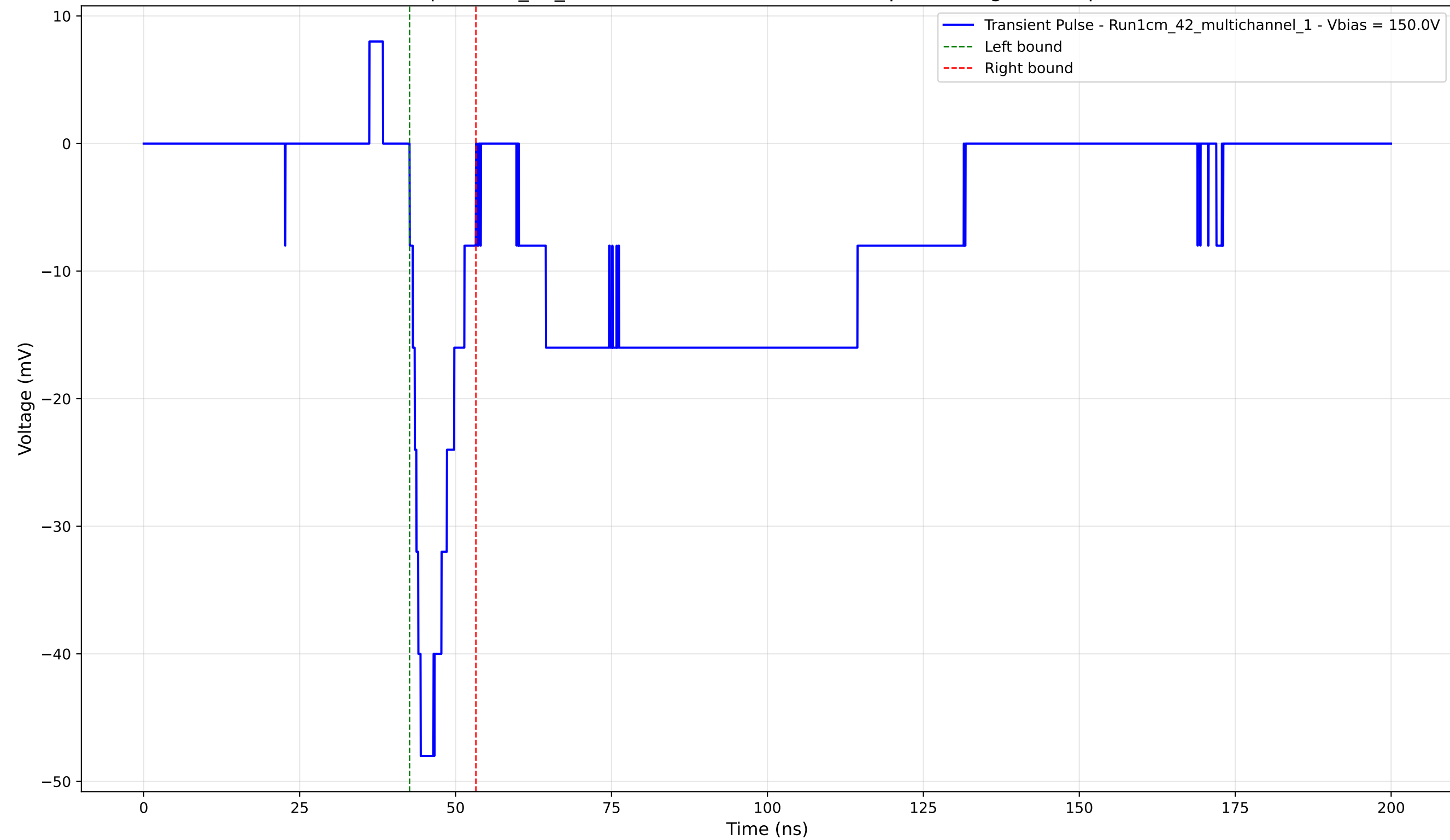
Transient Pulse - Sample: 1cm_42_multichannel - Position: 4130.0 \mu\text{m} - Charge: -5.75 pC - Rise Time: 1.77 ns
