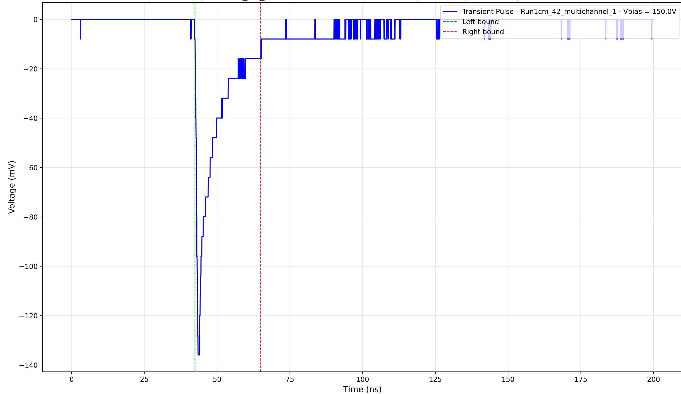
Transient Pulse - Sample: 1cm_42_multichannel - Position: 3090.0 \mu\text{m} - Charge: -18.26 pC - Rise Time: 0.93 ns
