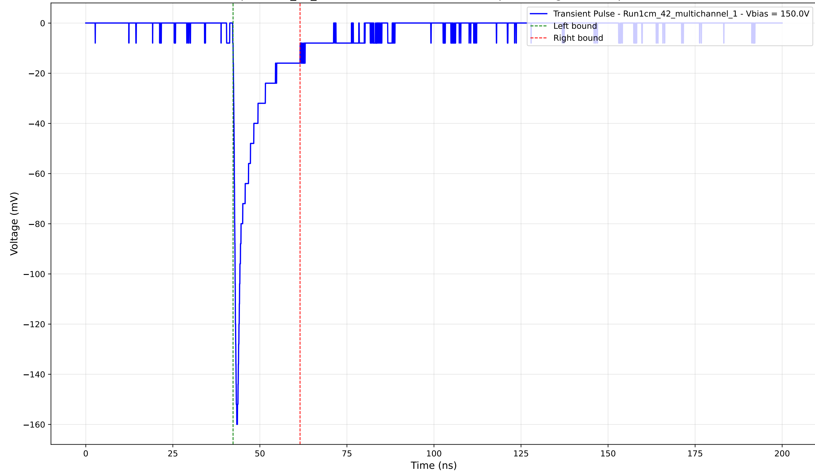
Transient Pulse - Sample: 1cm_42_multichannel - Position: 1940.0 \mu\text{m} - Charge: -15.46 pC - Rise Time: 0.84 ns
