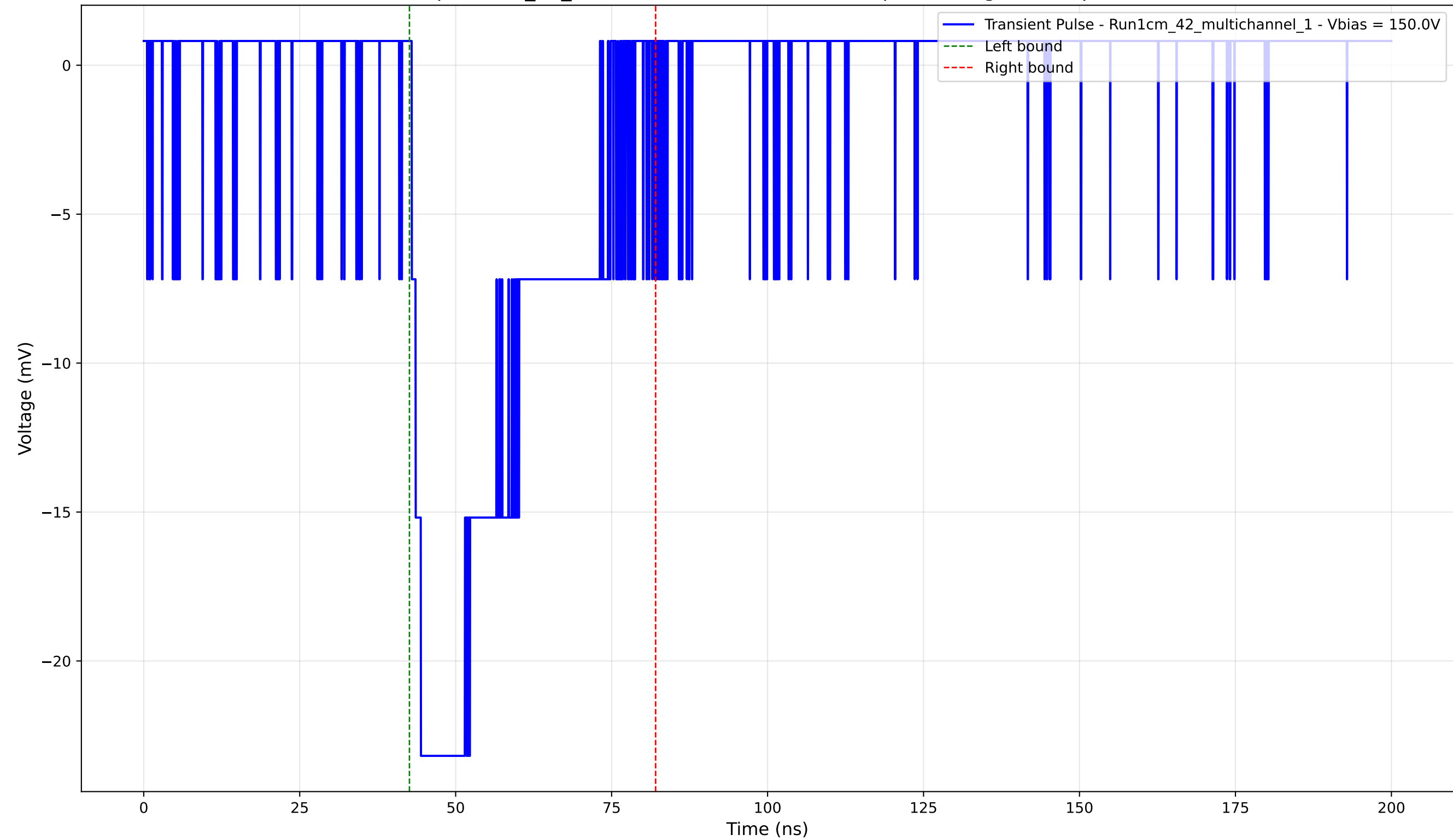
Transient Pulse - Sample: 1cm_42_multichannel - Position: 405.0 \mu\text{m} - Charge: -8.47 pC - Rise Time: 1.48 ns
