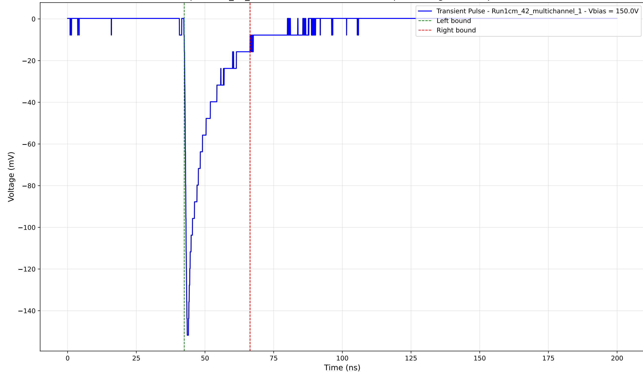
Transient Pulse - Sample: 1cm_42_multichannel - Position: 1660.0 \mu\text{m} - Charge: -22.51 pC - Rise Time: 0.94 ns
