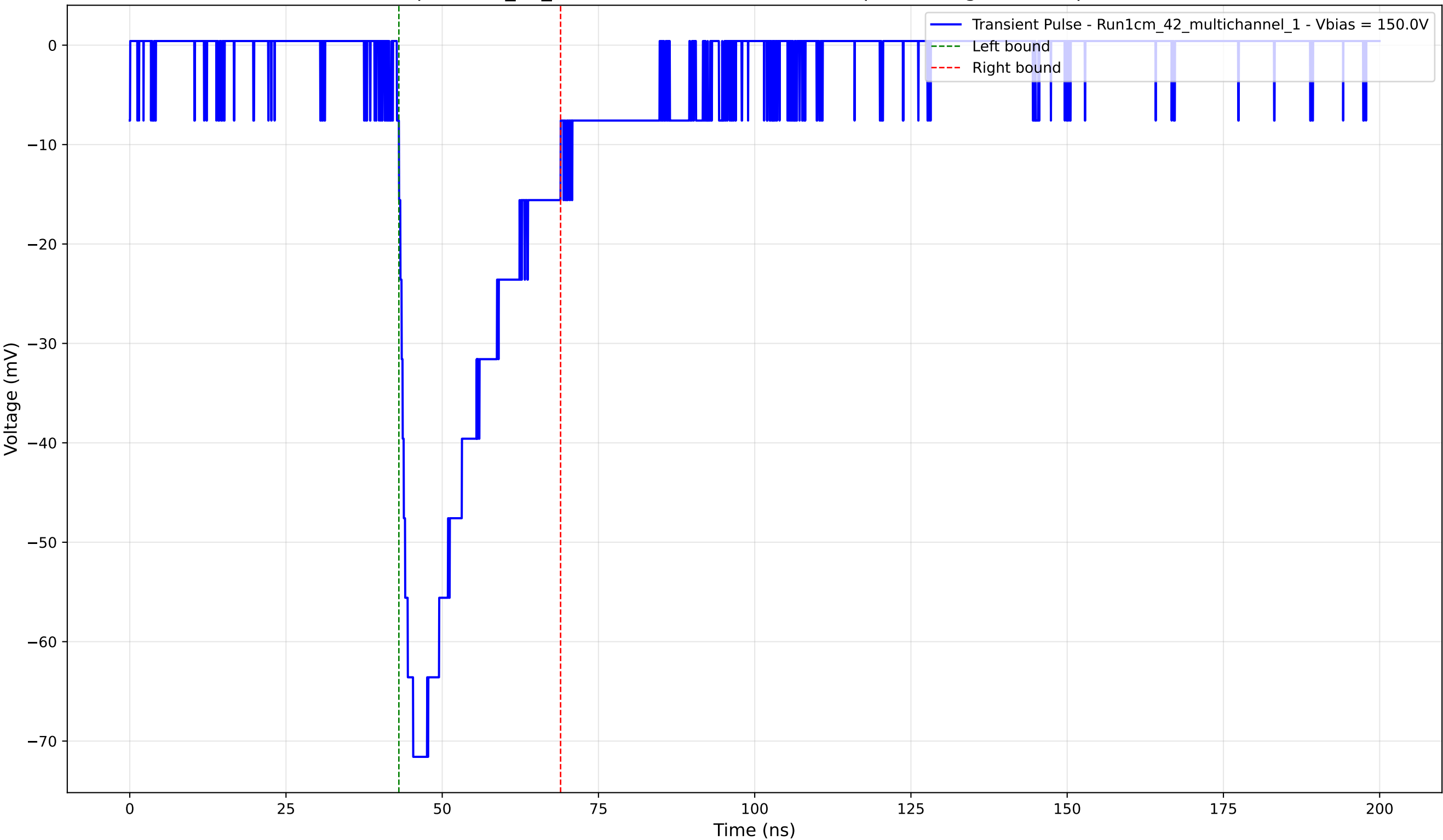
Transient Pulse - Sample: 1cm_42_multichannel - Position: 795.0 \mu\text{m} - Charge: -19.36 pC - Rise Time: 2.60 ns
