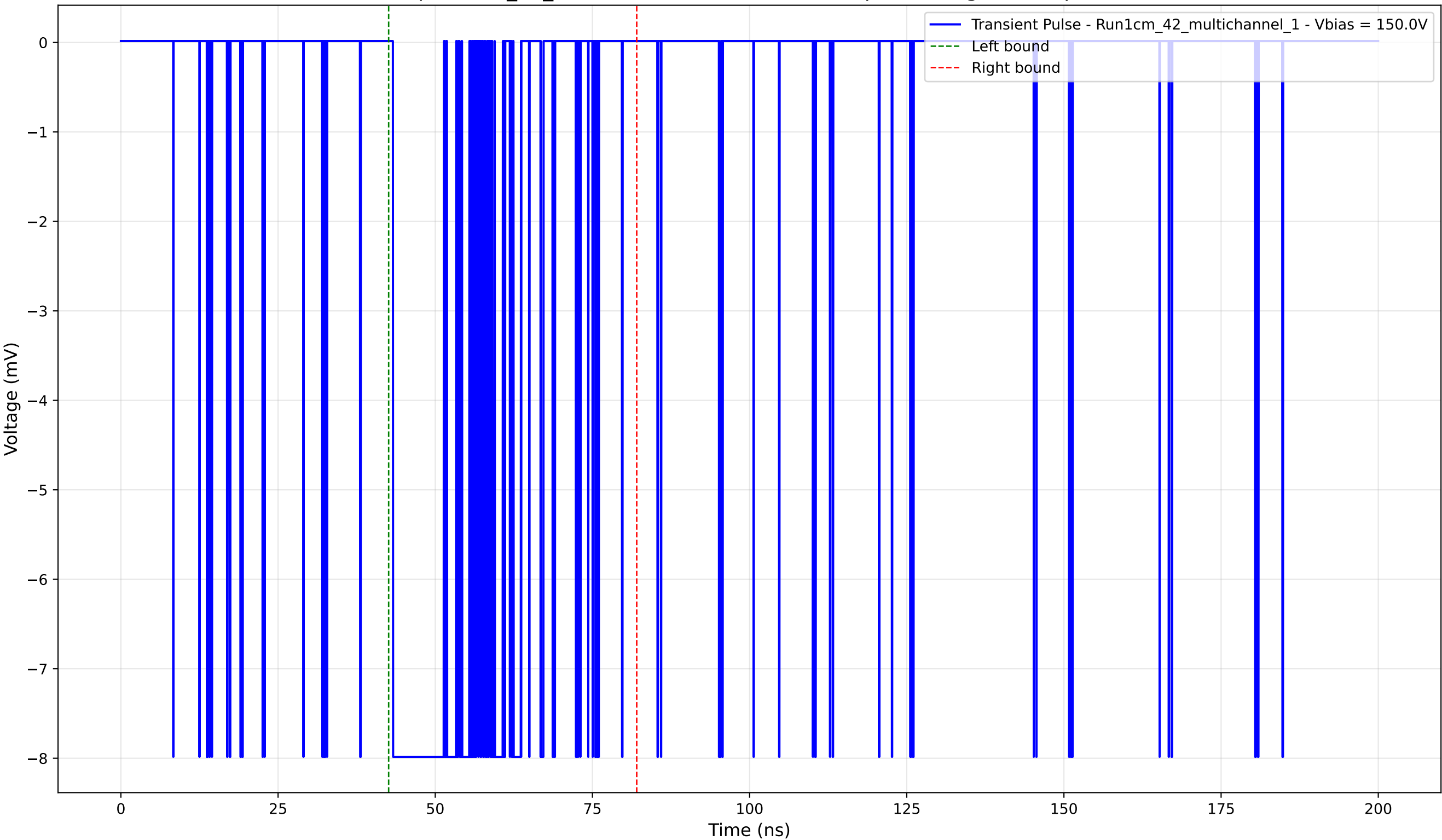
Transient Pulse - Sample: 1cm_42_multichannel - Position: 380.0 \mu\text{m} - Charge: -2.76 pC - Rise Time: 0.02 ns
