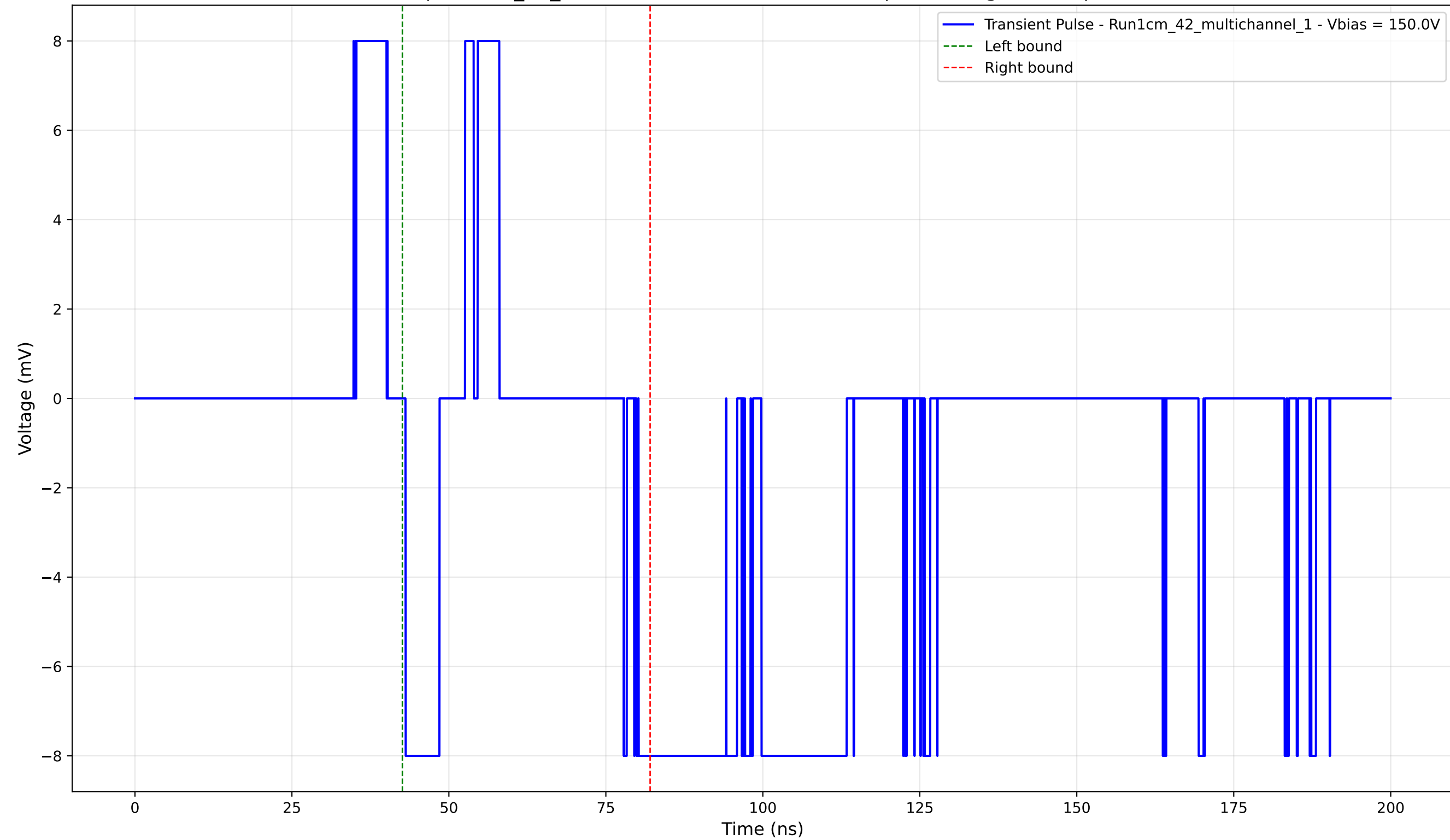
Transient Pulse - Sample: 1cm_42_multichannel - Position: 3940.0 \mu\text{m} - Charge: -0.51 pC - Rise Time: 0.02 ns
