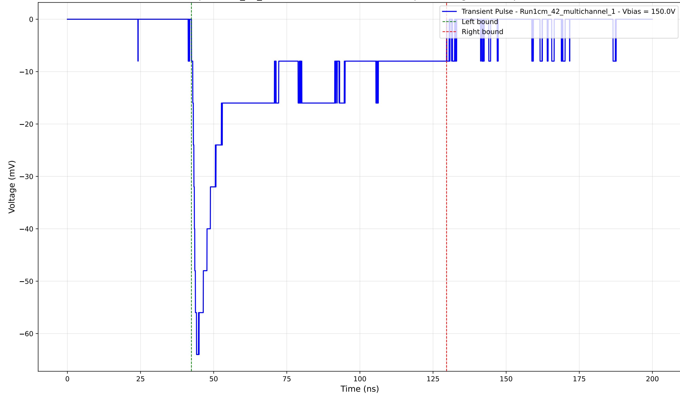
Transient Pulse - Sample: 1cm_42_multichannel - Position: 3730.0 \mu\text{m} - Charge: -25.83 pC - Rise Time: 1.72 ns
