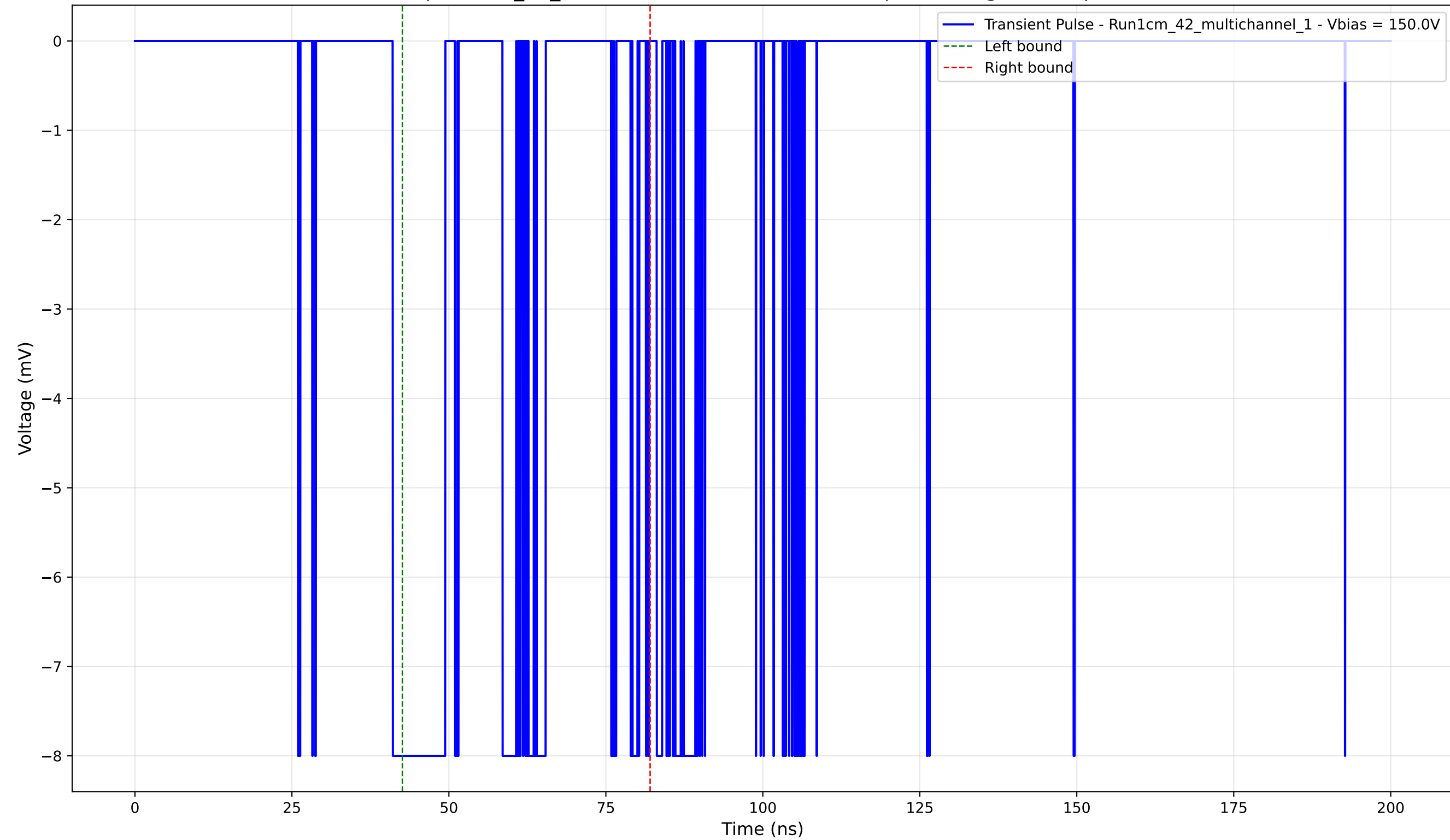
Transient Pulse - Sample: 1cm_42_multichannel - Position: 3380.0 \mu\text{m} - Charge: -2.44 pC - Rise Time: 0.02 ns
