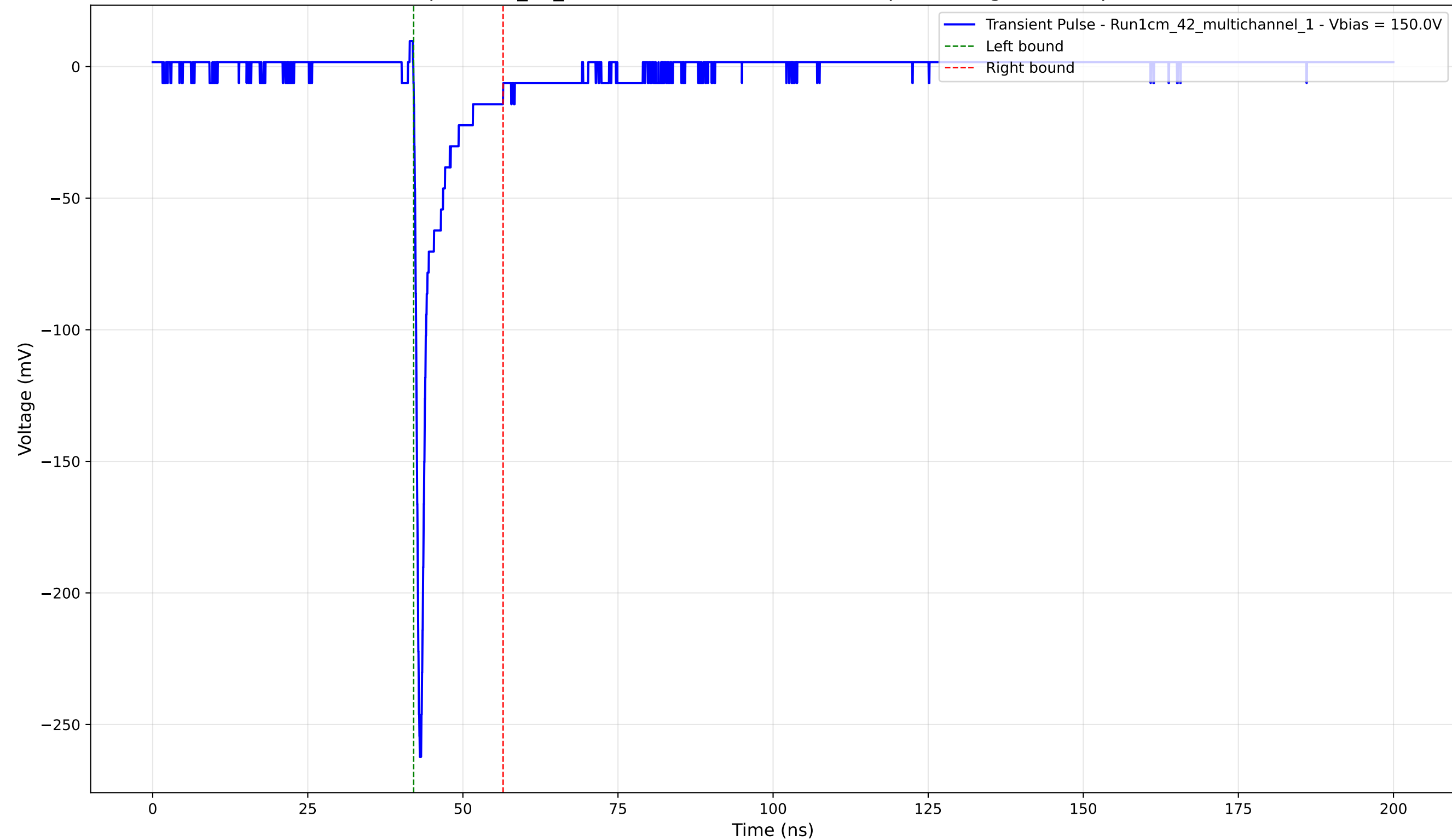
Transient Pulse - Sample: 1cm_42_multichannel - Position: 2330.0 \mu\text{m} - Charge: -14.50 pC - Rise Time: 0.72 ns
