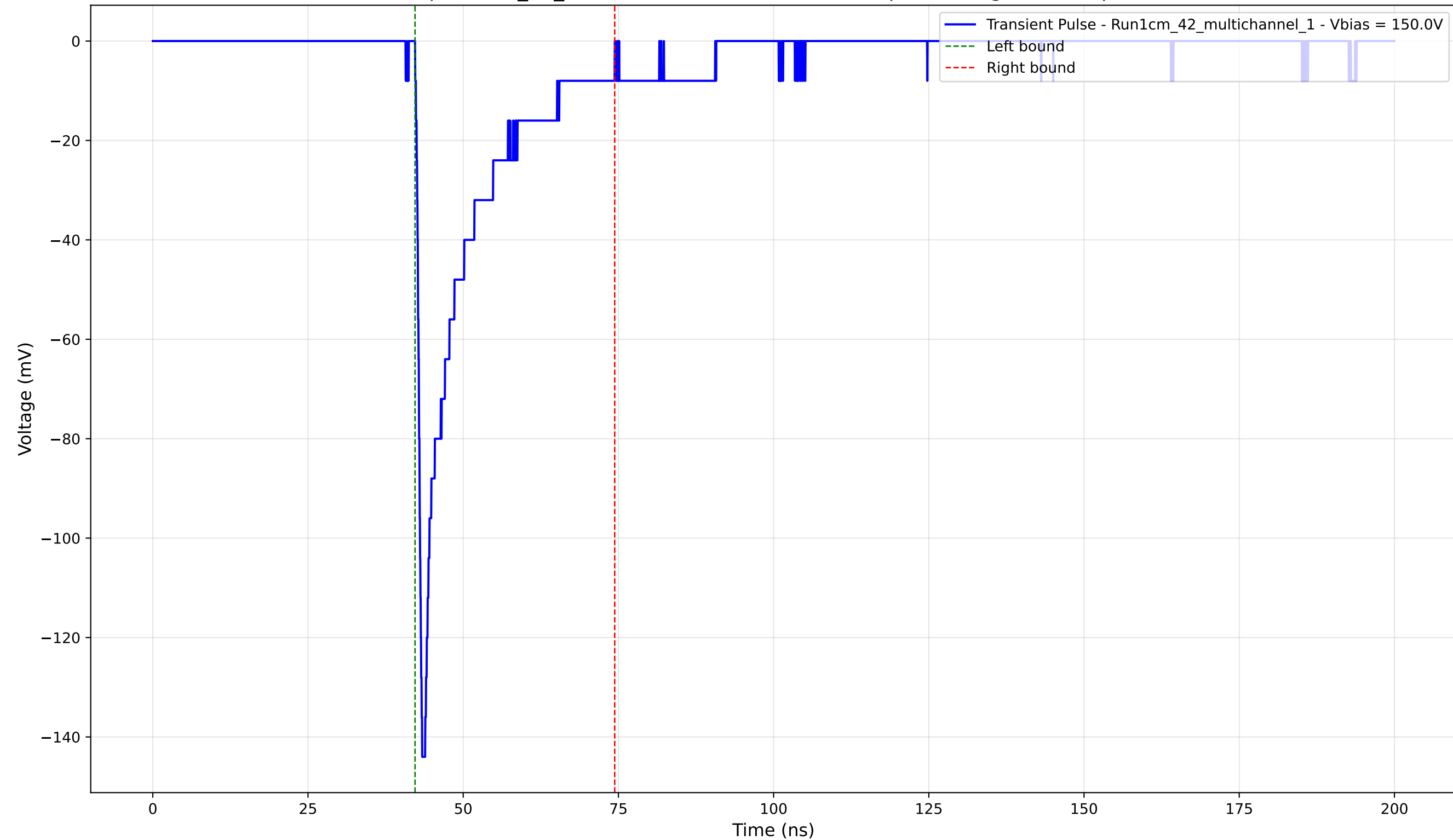
Transient Pulse - Sample: 1cm_42_multichannel - Position: 3060.0 \mu\text{m} - Charge: -20.59 pC - Rise Time: 0.92 ns
