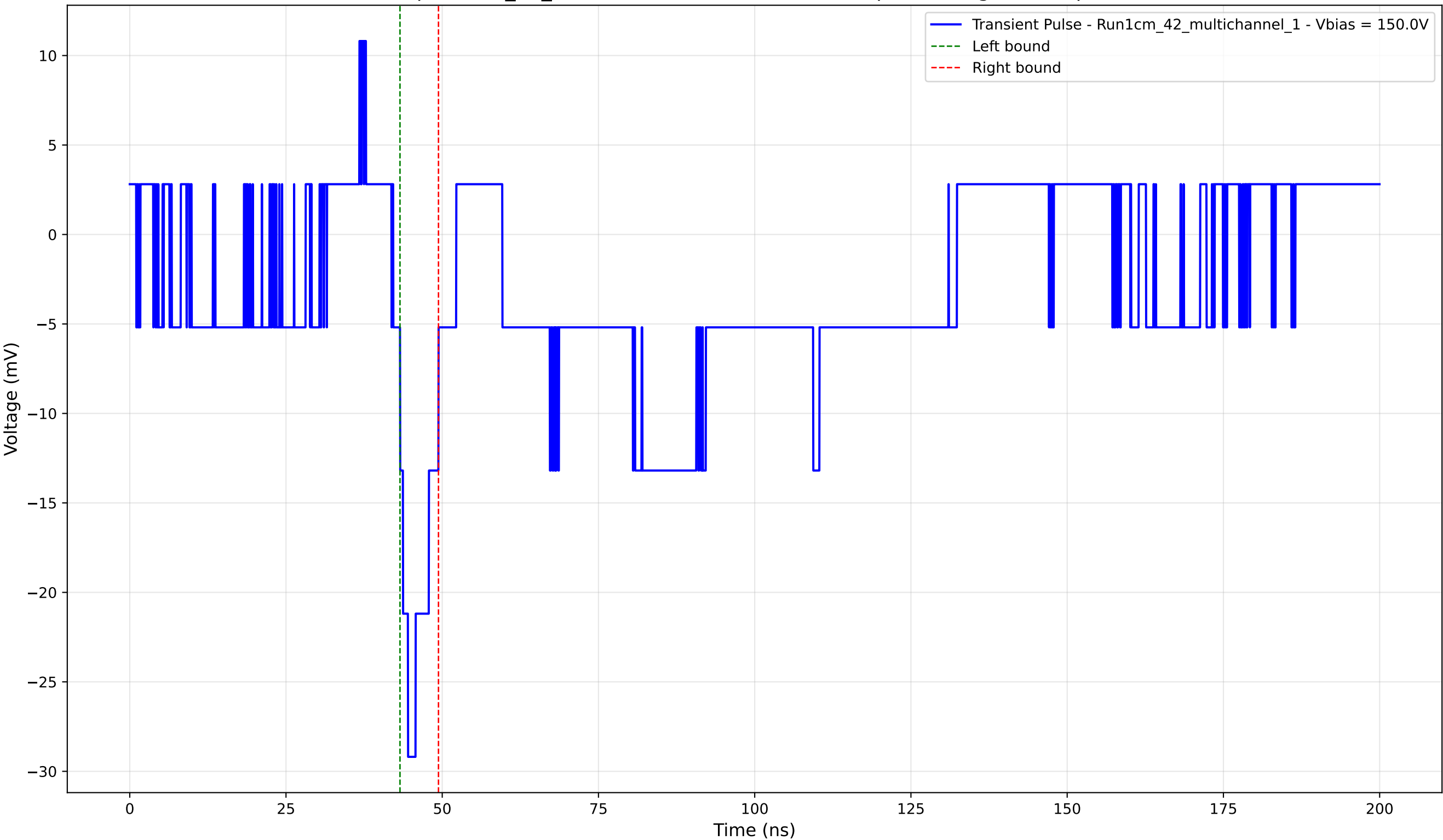
Transient Pulse - Sample: 1cm_42_multichannel - Position: 3955.0 \mu\text{m} - Charge: -2.48 pC - Rise Time: 2.38 ns
