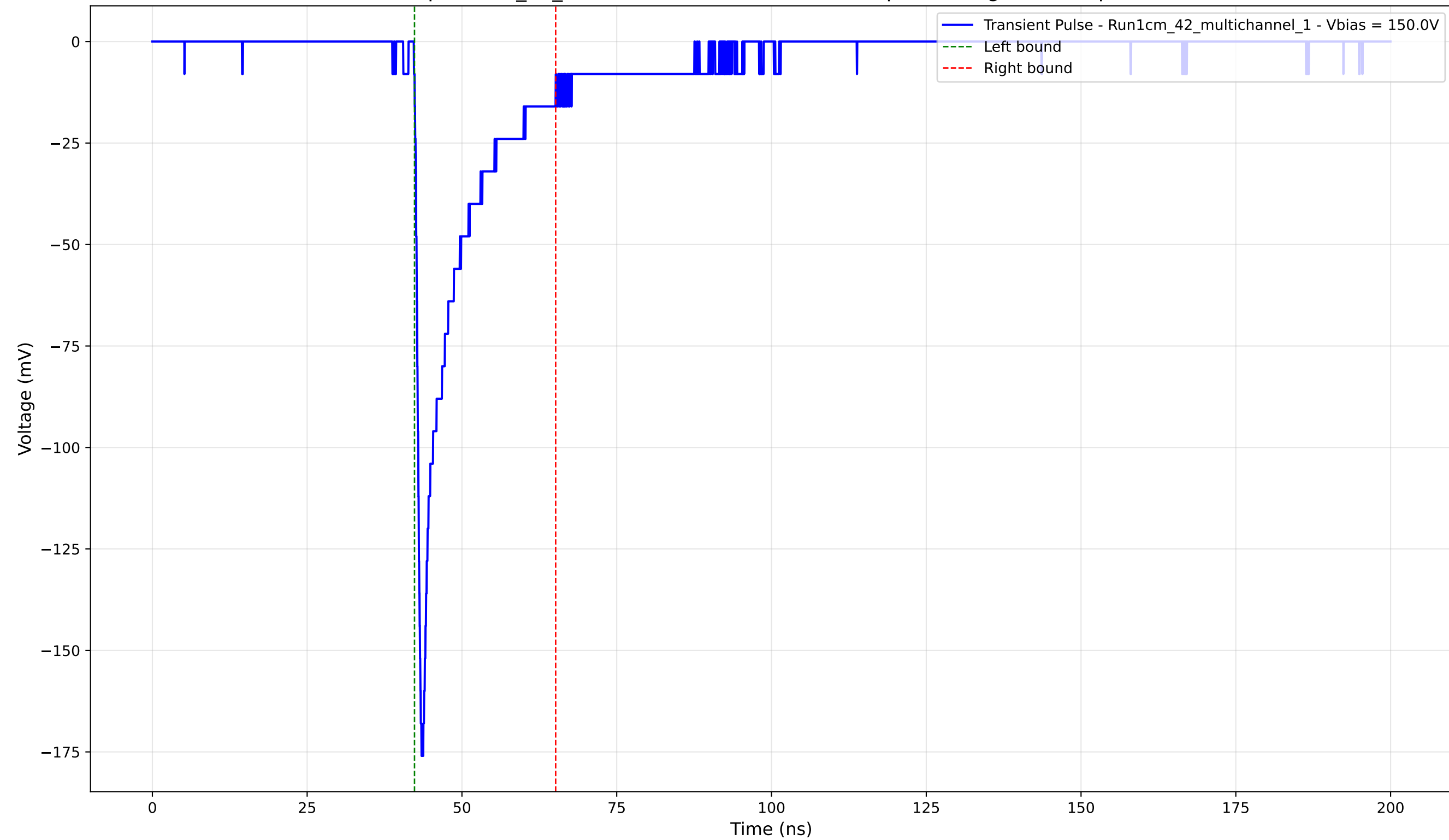
Transient Pulse - Sample: 1cm_42_multichannel - Position: 1780.0 \mu\text{m} - Charge: -21.86 pC - Rise Time: 0.86 ns
