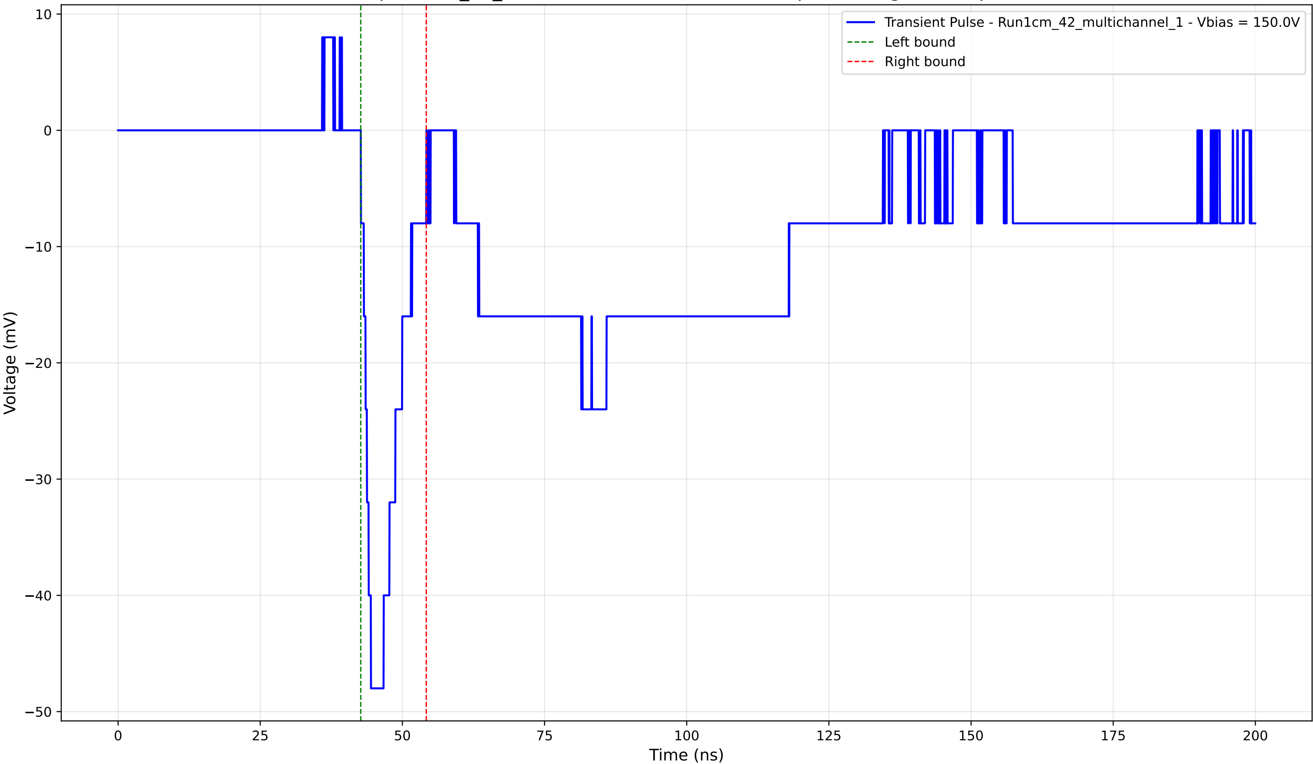
Transient Pulse - Sample: 1cm_42_multichannel - Position: 4175.0 \mu\text{m} - Charge: -5.96 pC - Rise Time: 1.77 ns
