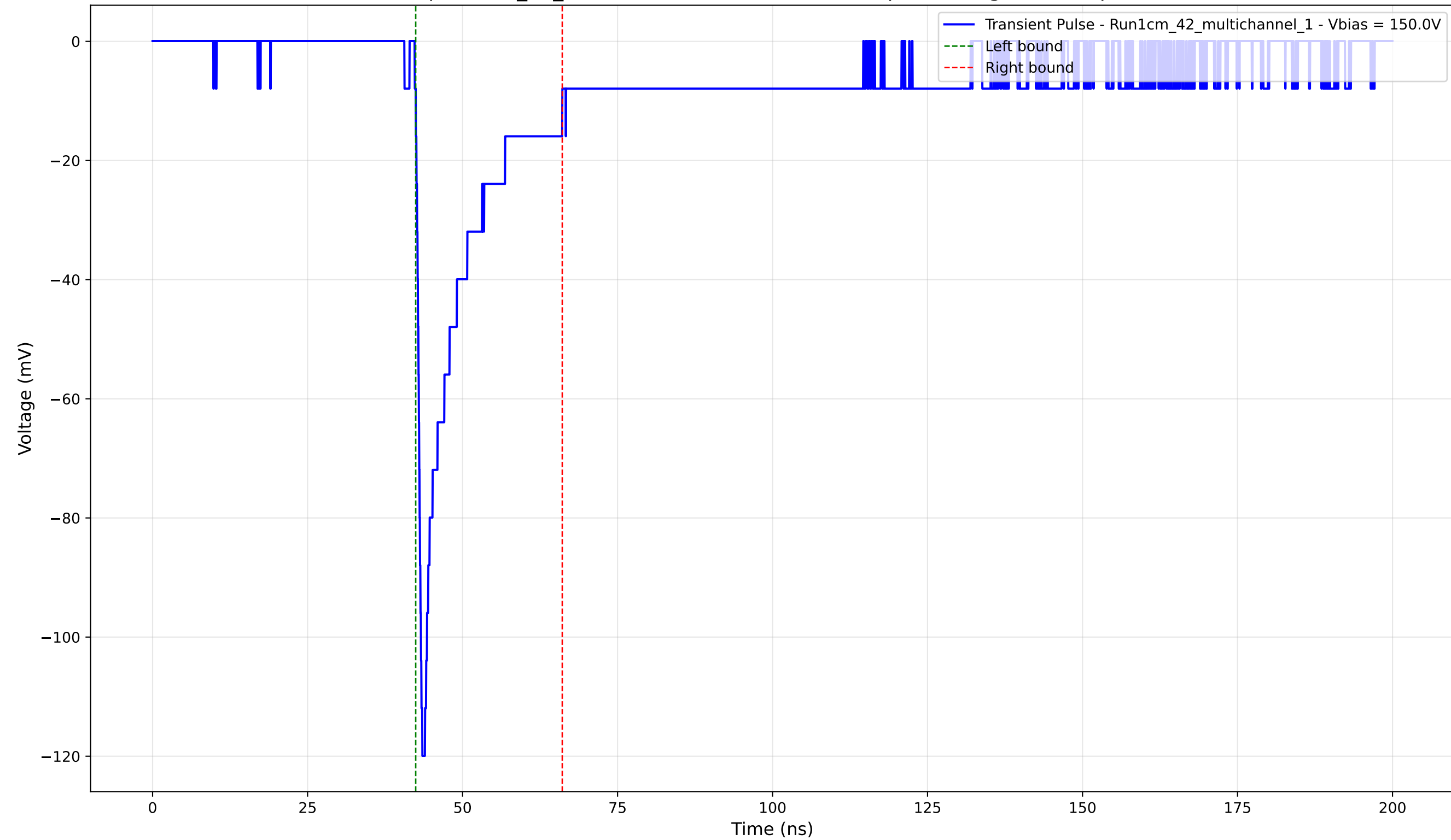
Transient Pulse - Sample: 1cm_42_multichannel - Position: 3165.0 \mu\text{m} - Charge: -16.87 pC - Rise Time: 0.91 ns
