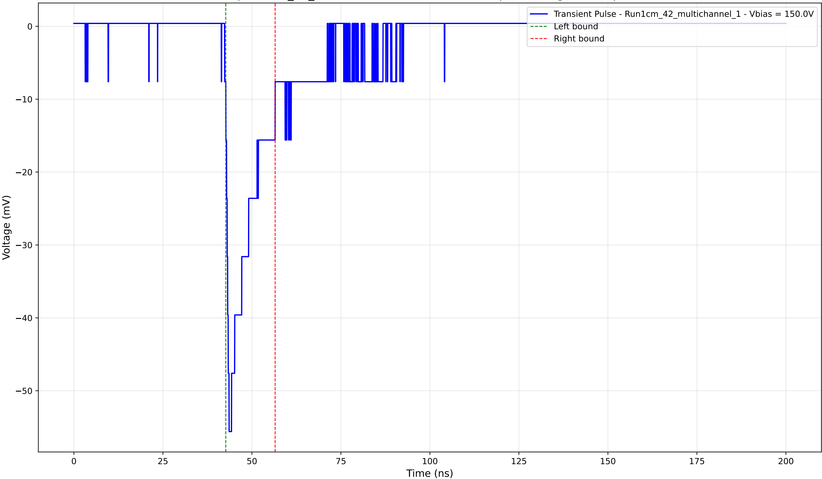
Transient Pulse - Sample: 1cm_42_multichannel - Position: 3345.0 \mu\text{m} - Charge: -7.75 pC - Rise Time: 1.25 ns
