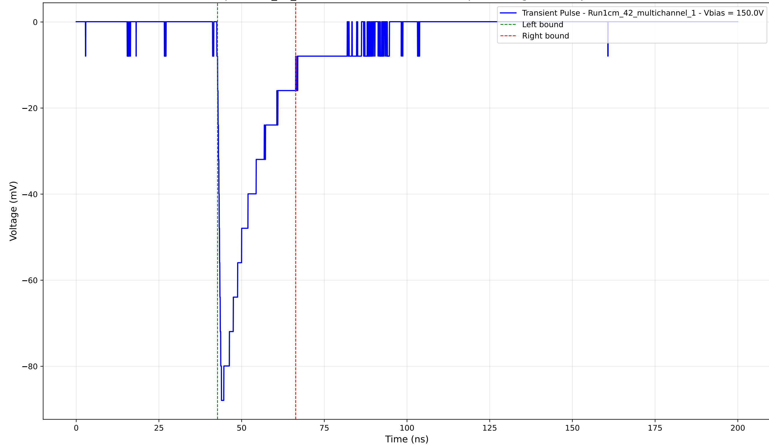
Transient Pulse - Sample: 1cm_42_multichannel - Position: 1300.0 \mu\text{m} - Charge: -18.96 pC - Rise Time: 0.96 ns
