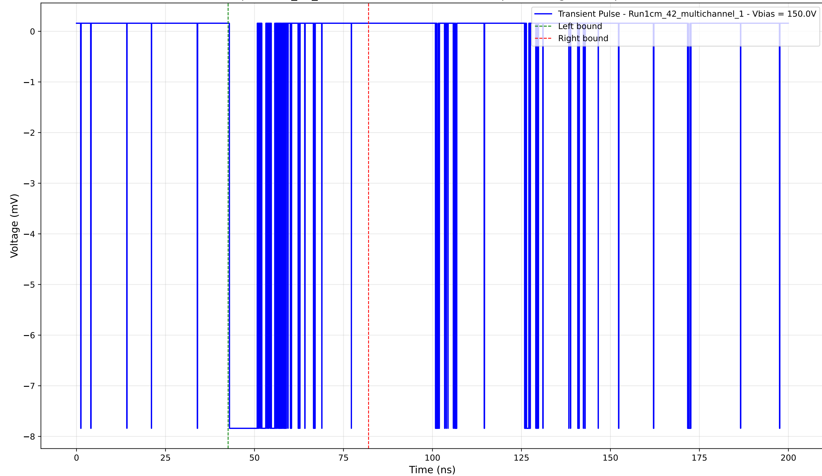
Transient Pulse - Sample: 1cm_42_multichannel - Position: 1365.0 \mu\text{m} - Charge: -1.98 pC - Rise Time: 0.02 ns
