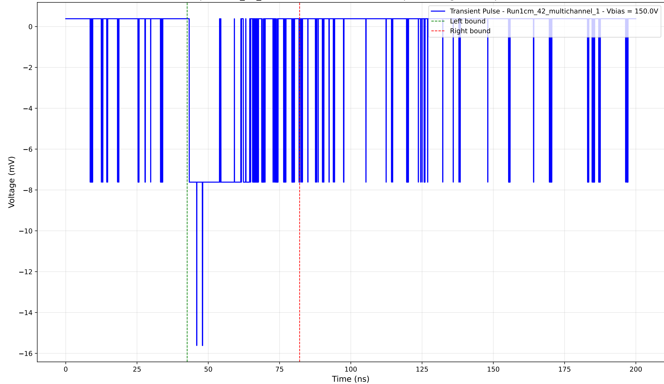
Transient Pulse - Sample: 1cm_42_multichannel - Position: 840.0 \mu\text{m} - Charge: -3.50 pC - Rise Time: 2.64 ns
