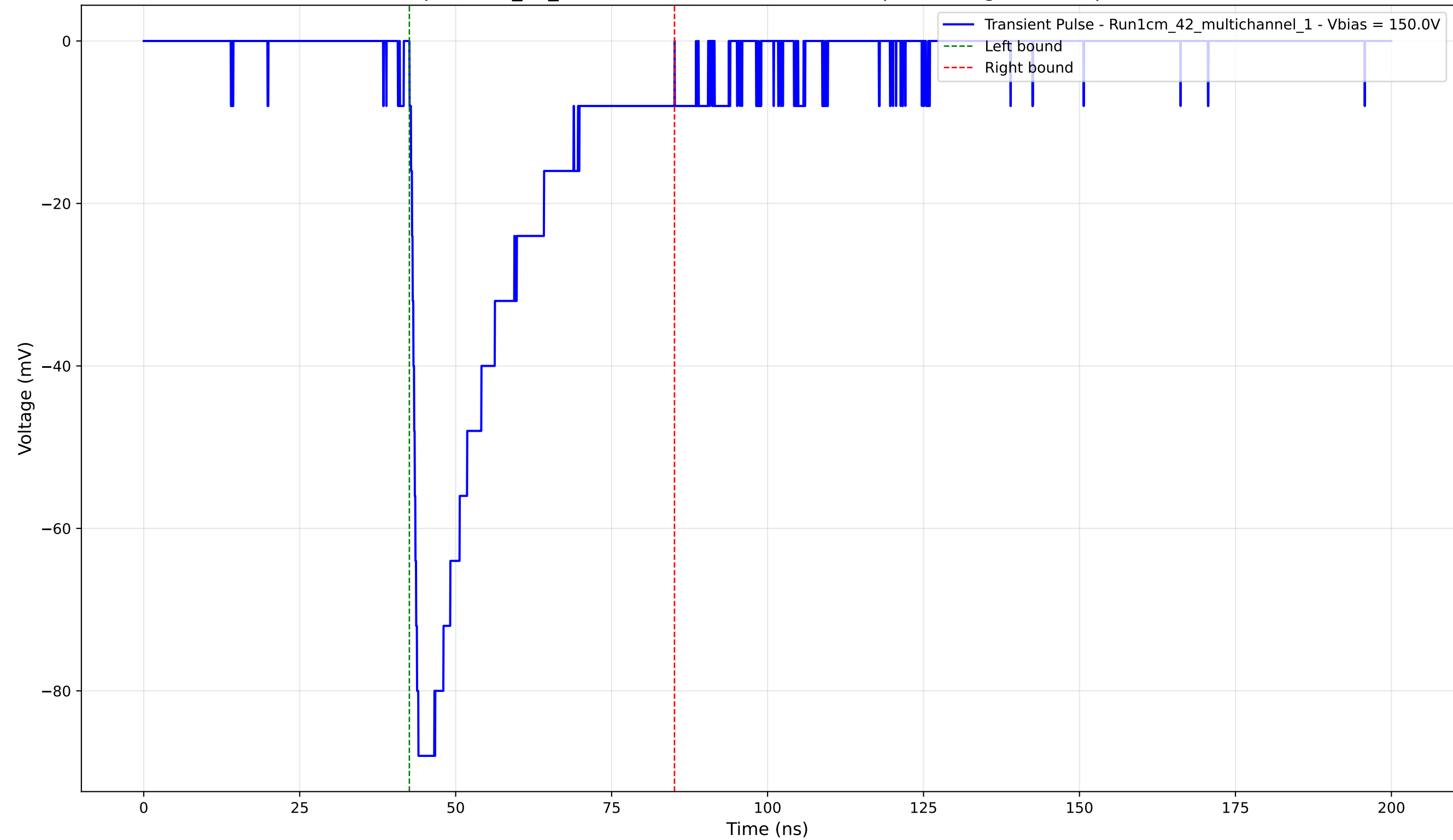
Transient Pulse - Sample: 1cm_42_multichannel - Position: 1140.0 \mu\text{m} - Charge: -25.40 pC - Rise Time: 0.98 ns
