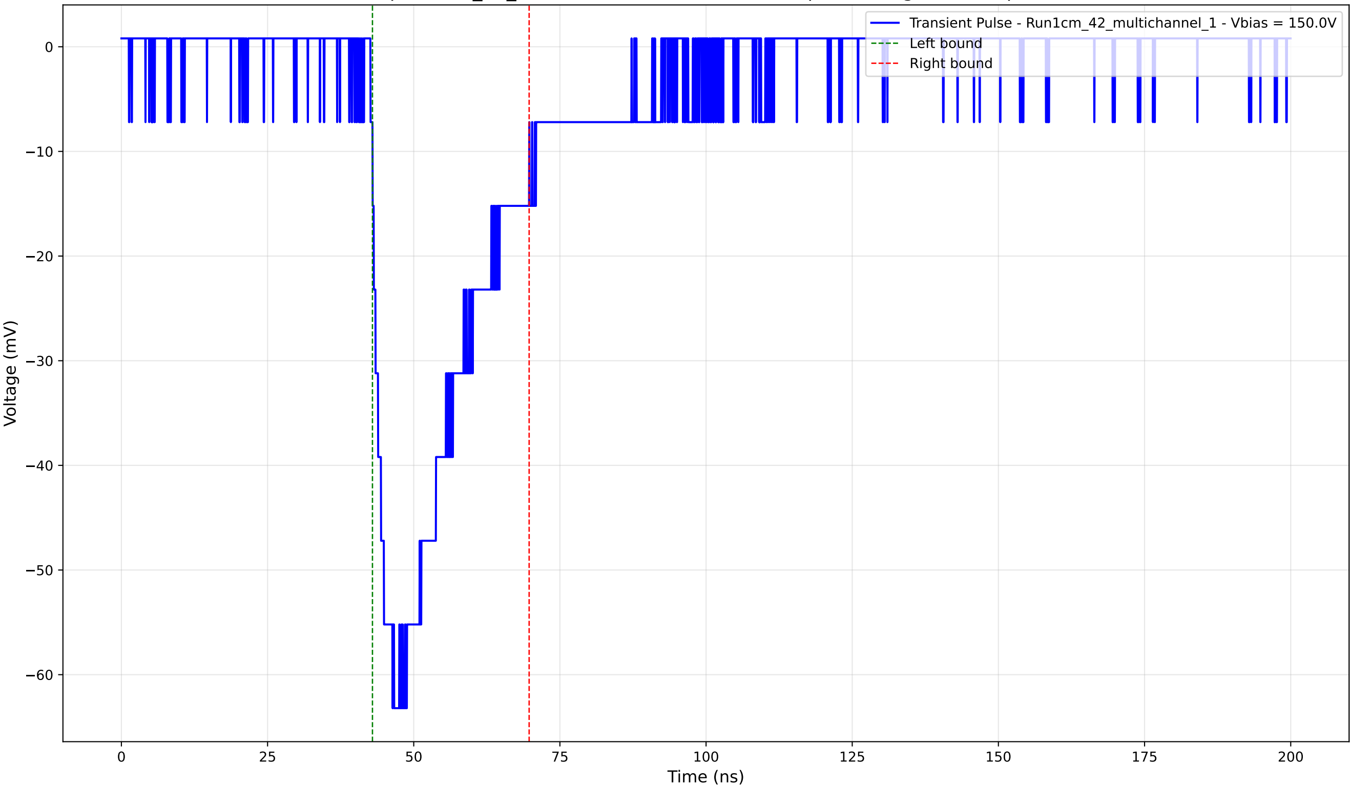
Transient Pulse - Sample: 1cm_42_multichannel - Position: 130.0 \mu\text{m} - Charge: -18.86 pC - Rise Time: 3.76 ns
