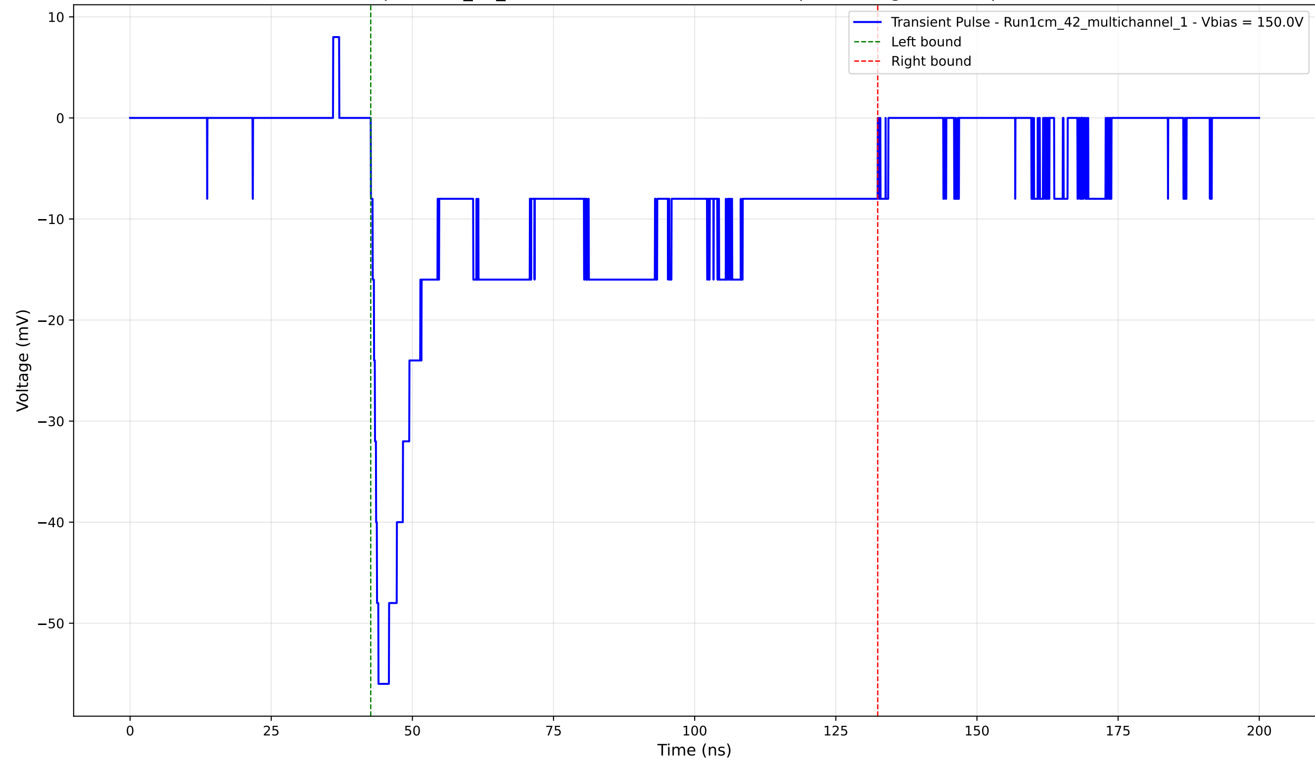
Transient Pulse - Sample: 1cm_42_multichannel - Position: 3805.0 \mu\text{m} - Charge: -24.50 pC - Rise Time: 1.35 ns
