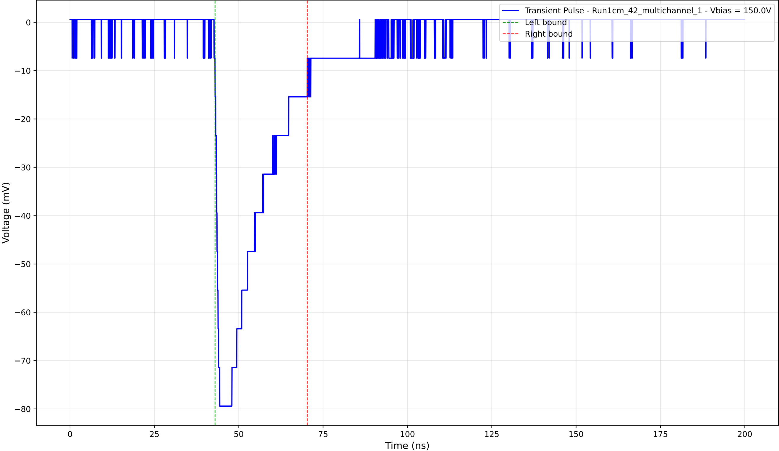
Transient Pulse - Sample: 1cm_42_multichannel - Position: 955.0 \mu\text{m} - Charge: -22.68 pC - Rise Time: 1.38 ns
