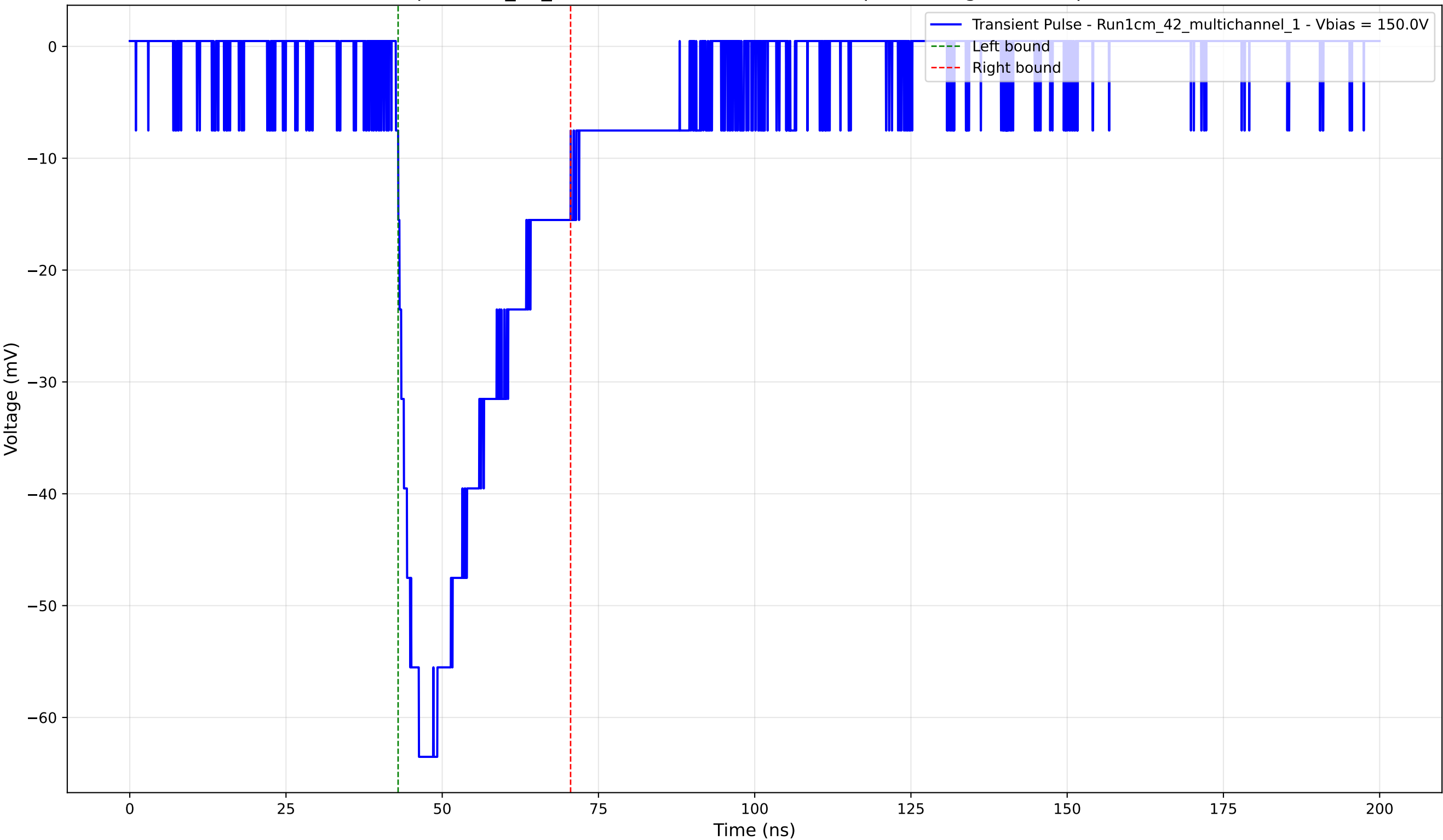
Transient Pulse - Sample: 1cm_42_multichannel - Position: 135.0 \mu\text{m} - Charge: -19.49 pC - Rise Time: 3.68 ns
