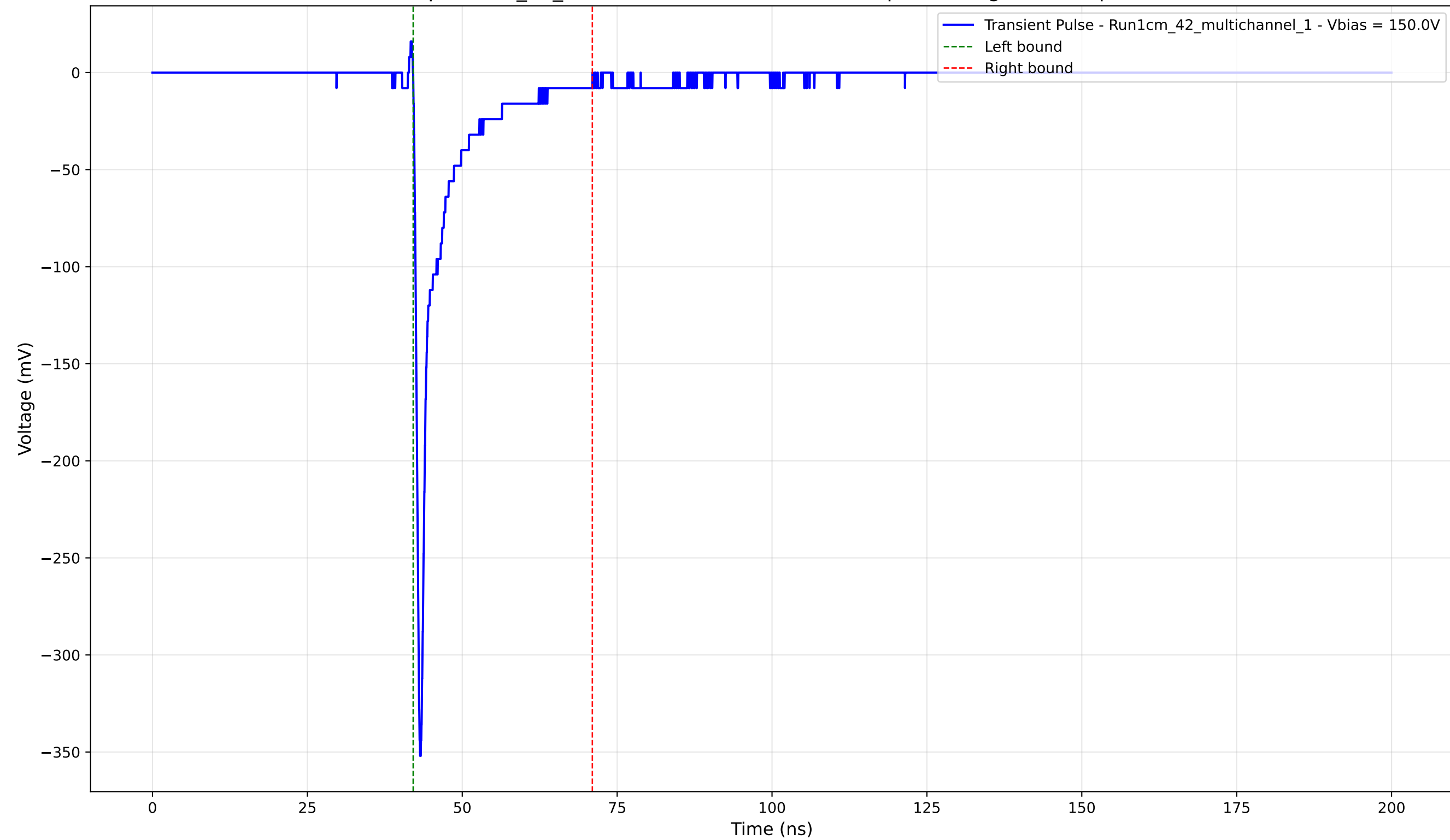
Transient Pulse - Sample: 1cm_42_multichannel - Position: 2190.0 \mu\text{m} - Charge: -25.59 pC - Rise Time: 0.75 ns
