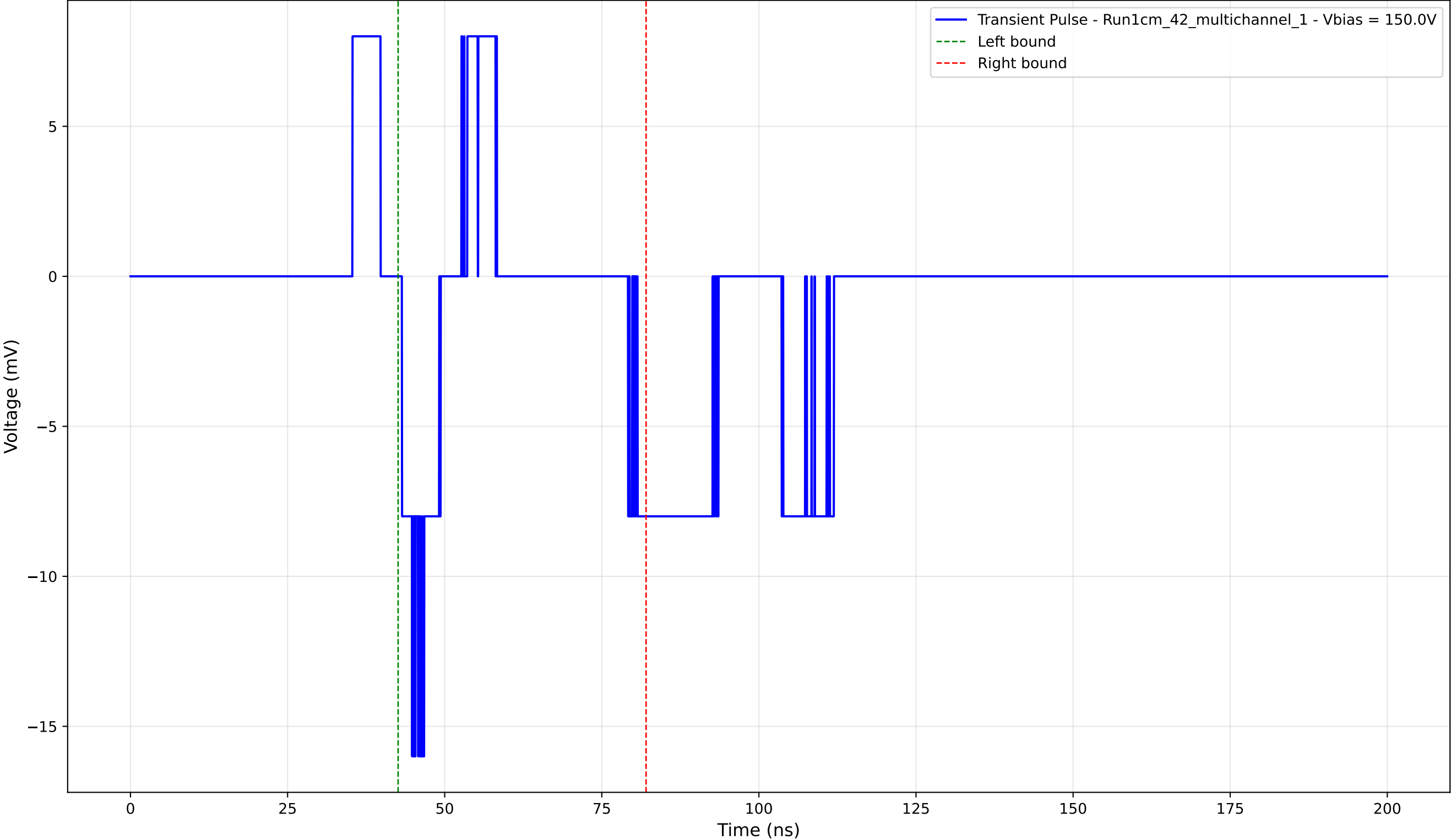
Transient Pulse - Sample: 1cm_42_multichannel - Position: 4445.0 \mu\text{m} - Charge: -0.71 pC - Rise Time: 1.62 ns
