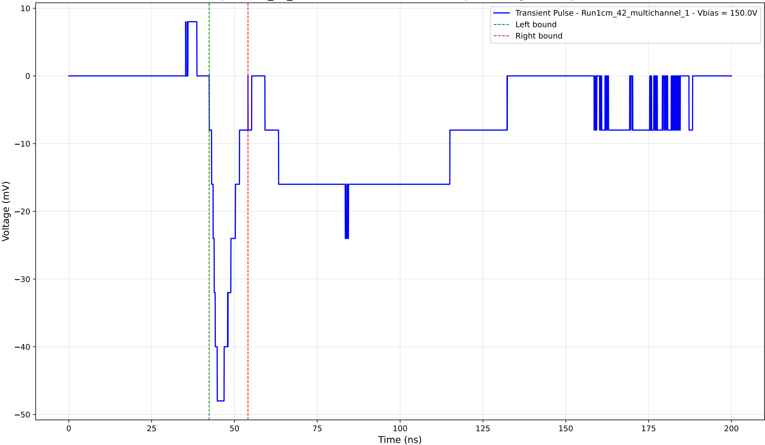
Transient Pulse - Sample: 1cm_42_multichannel - Position: 4525.0 \mu\text{m} - Charge: -6.04 pC - Rise Time: 2.43 ns
