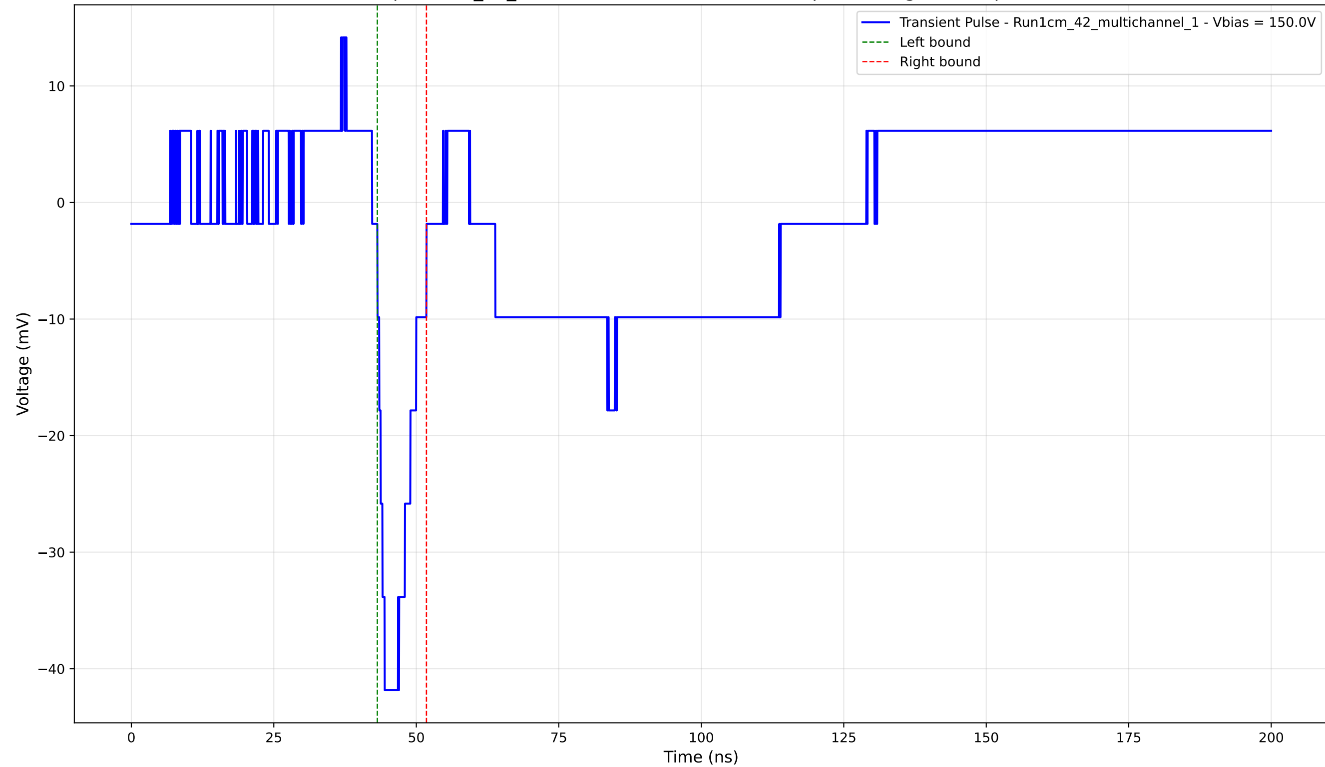
Transient Pulse - Sample: 1cm_42_multichannel - Position: 4225.0 \mu\text{m} - Charge: -4.59 pC - Rise Time: 1.27 ns
