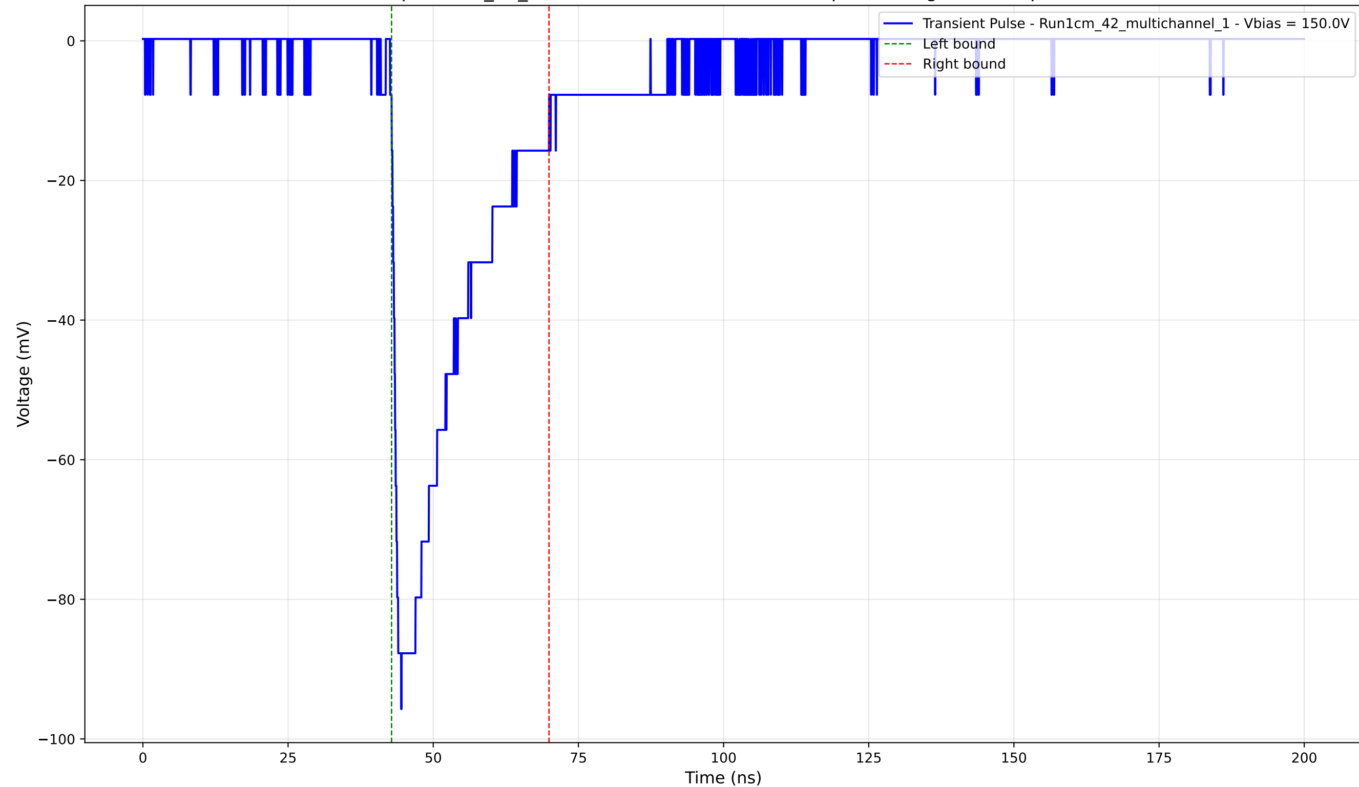
Transient Pulse - Sample: 1cm_42_multichannel - Position: 1150.0 \mu\text{m} - Charge: -23.02 pC - Rise Time: 1.14 ns
