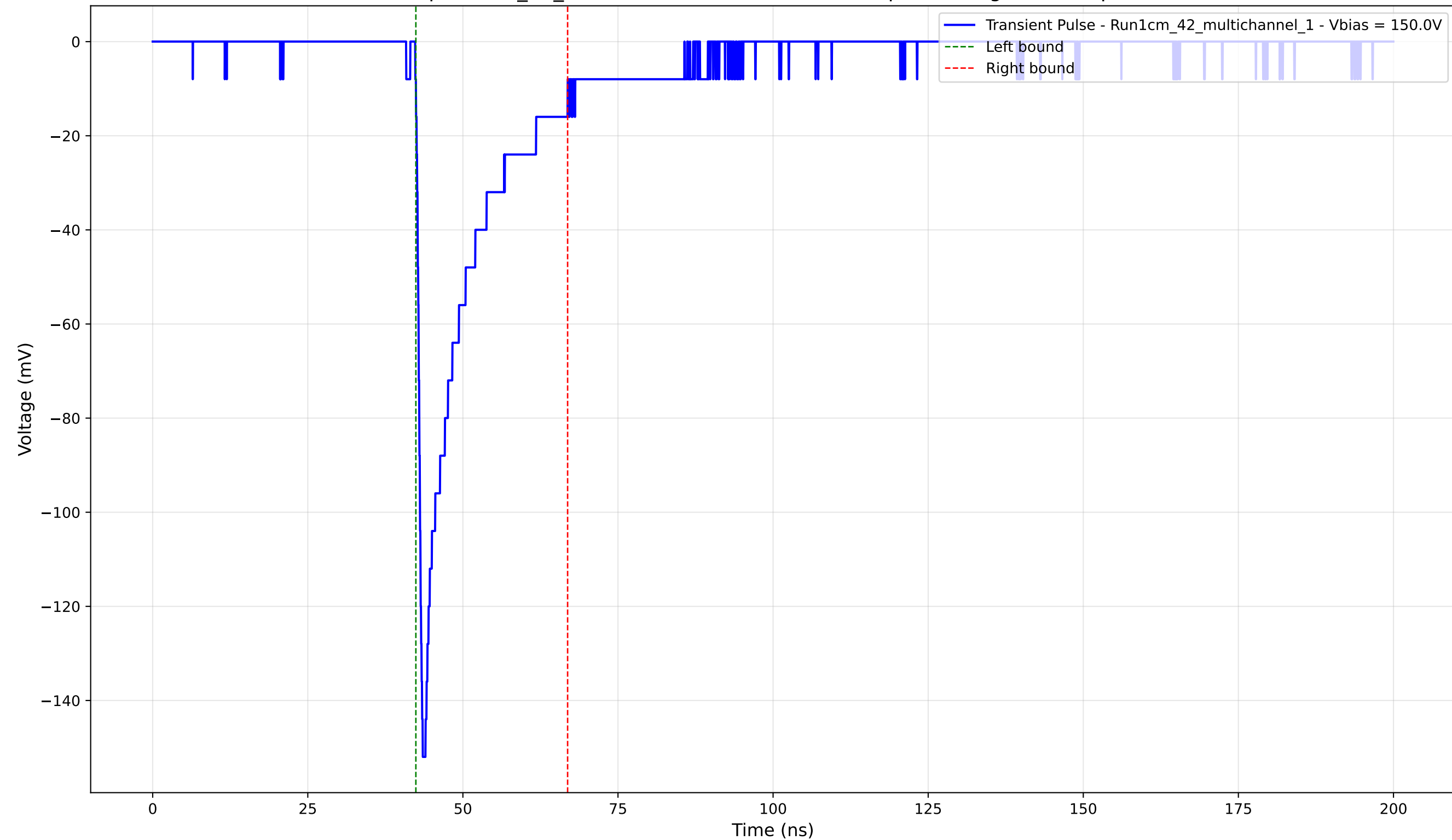
Transient Pulse - Sample: 1cm_42_multichannel - Position: 1650.0 \mu\text{m} - Charge: -22.91 pC - Rise Time: 0.98 ns
