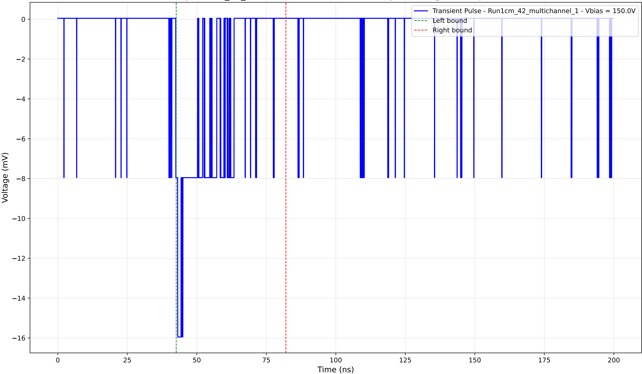
Transient Pulse - Sample: 1cm_42_multichannel - Position: 1860.0 \mu\text{m} - Charge: -2.93 pC - Rise Time: 0.70 ns
