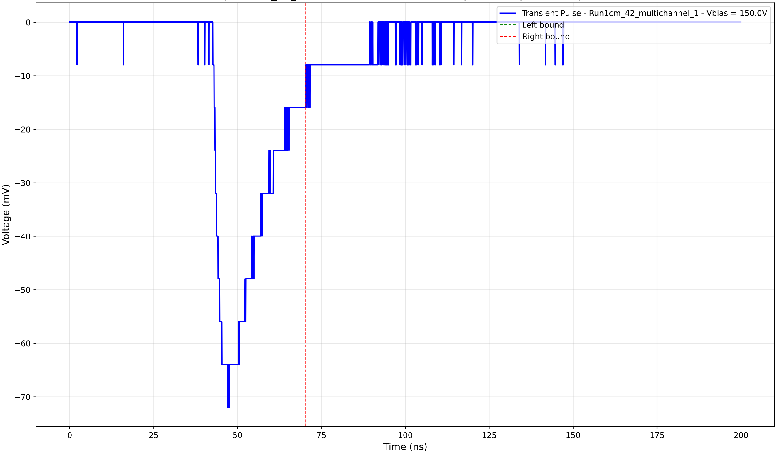
Transient Pulse - Sample: 1cm_42_multichannel - Position: 225.0 \mu\text{m} - Charge: -20.71 pC - Rise Time: 4.38 ns
