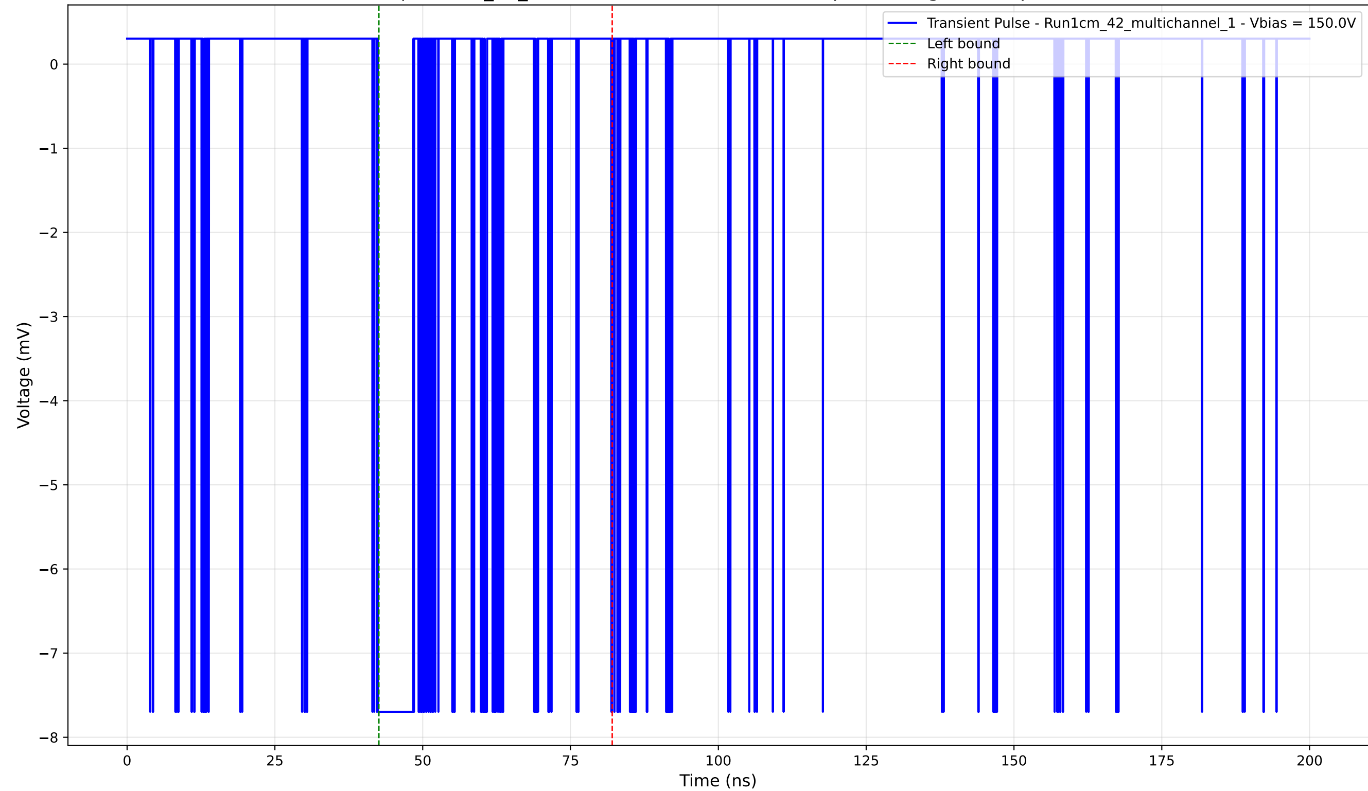
Transient Pulse - Sample: 1cm_42_multichannel - Position: 2890.0 \mu\text{m} - Charge: -1.39 pC - Rise Time: 0.02 ns
