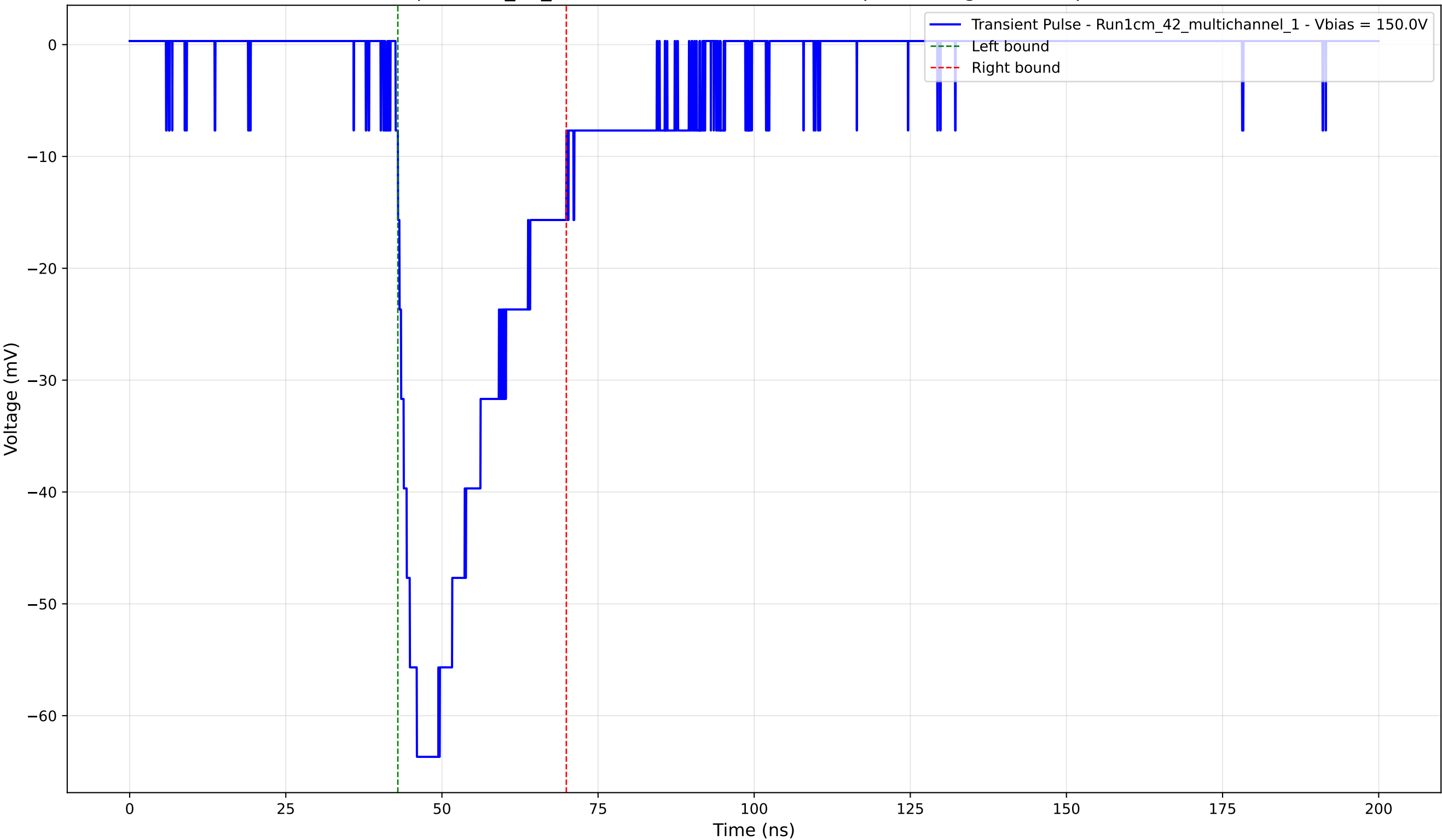
Transient Pulse - Sample: 1cm_42_multichannel - Position: 140.0 \mu\text{m} - Charge: -19.56 pC - Rise Time: 3.40 ns
