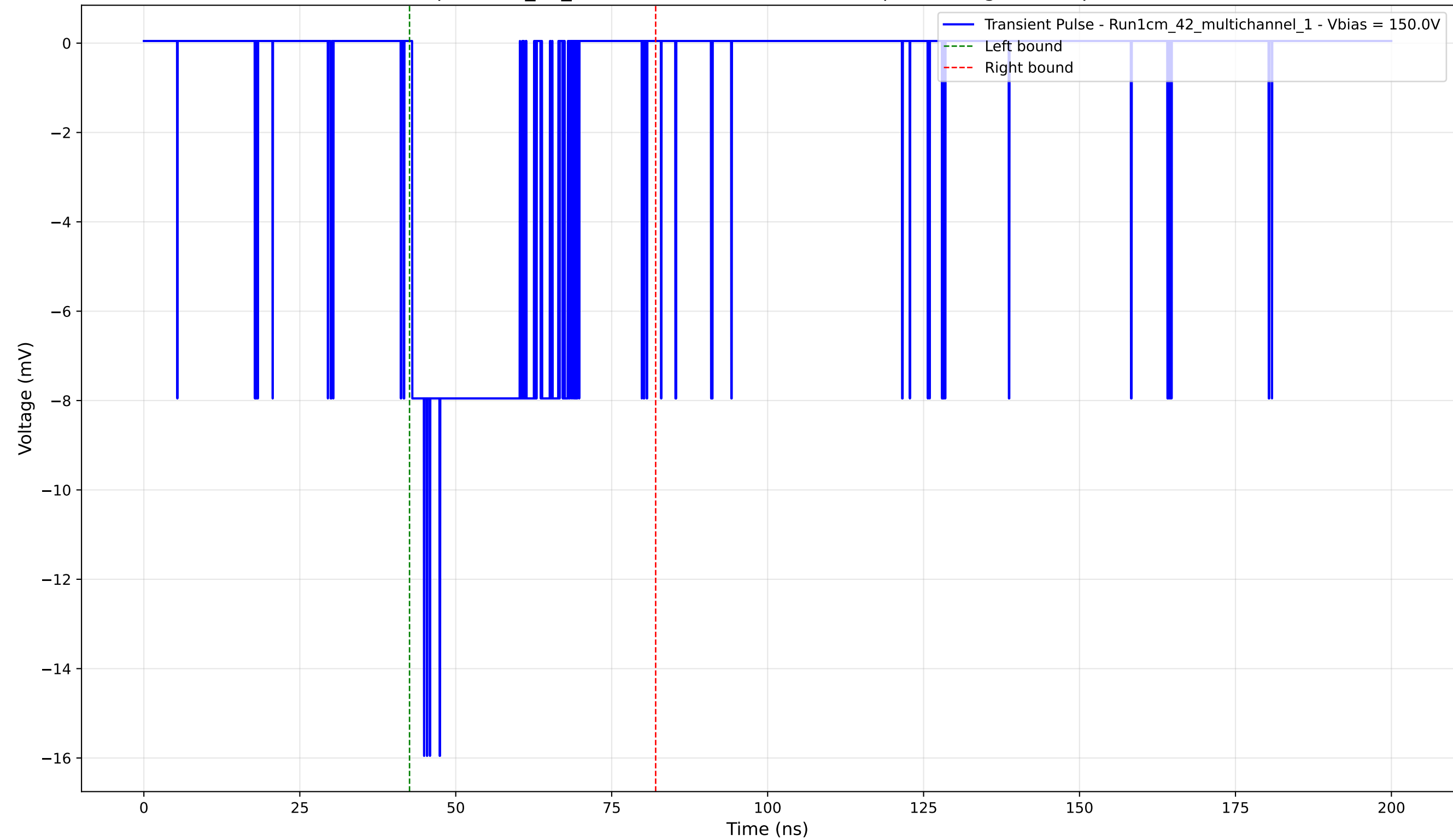
Transient Pulse - Sample: 1cm_42_multichannel - Position: 895.0 \mu\text{m} - Charge: -3.76 pC - Rise Time: 1.90 ns
