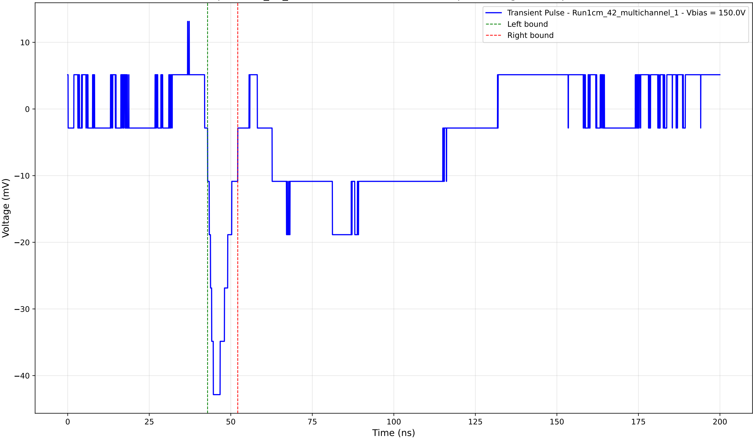
Transient Pulse - Sample: 1cm_42_multichannel - Position: 4620.0 \mu\text{m} - Charge: -4.92 pC - Rise Time: 1.76 ns
