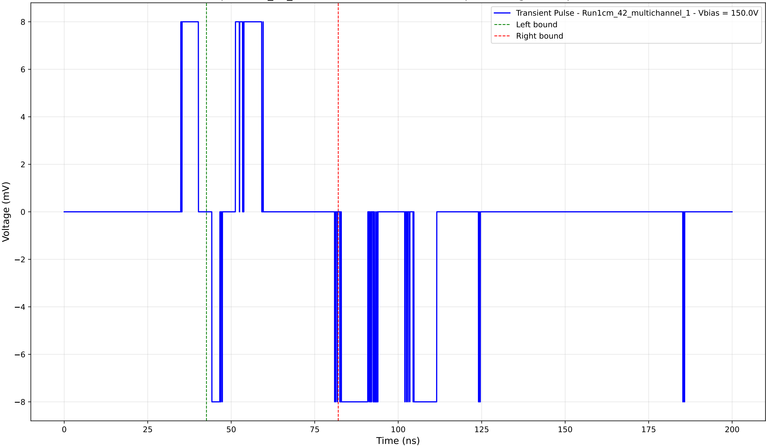
Transient Pulse - Sample: 1cm_42_multichannel - Position: 4380.0 \mu\text{m} - Charge: 0.76 pC - Rise Time: 0.02 ns
