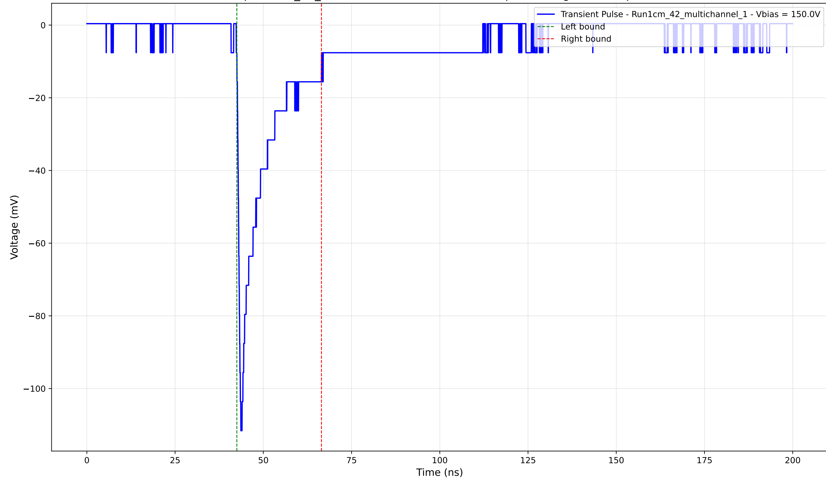
Transient Pulse - Sample: 1cm_42_multichannel - Position: 3245.0 \mu\text{m} - Charge: -16.59 pC - Rise Time: 0.97 ns
