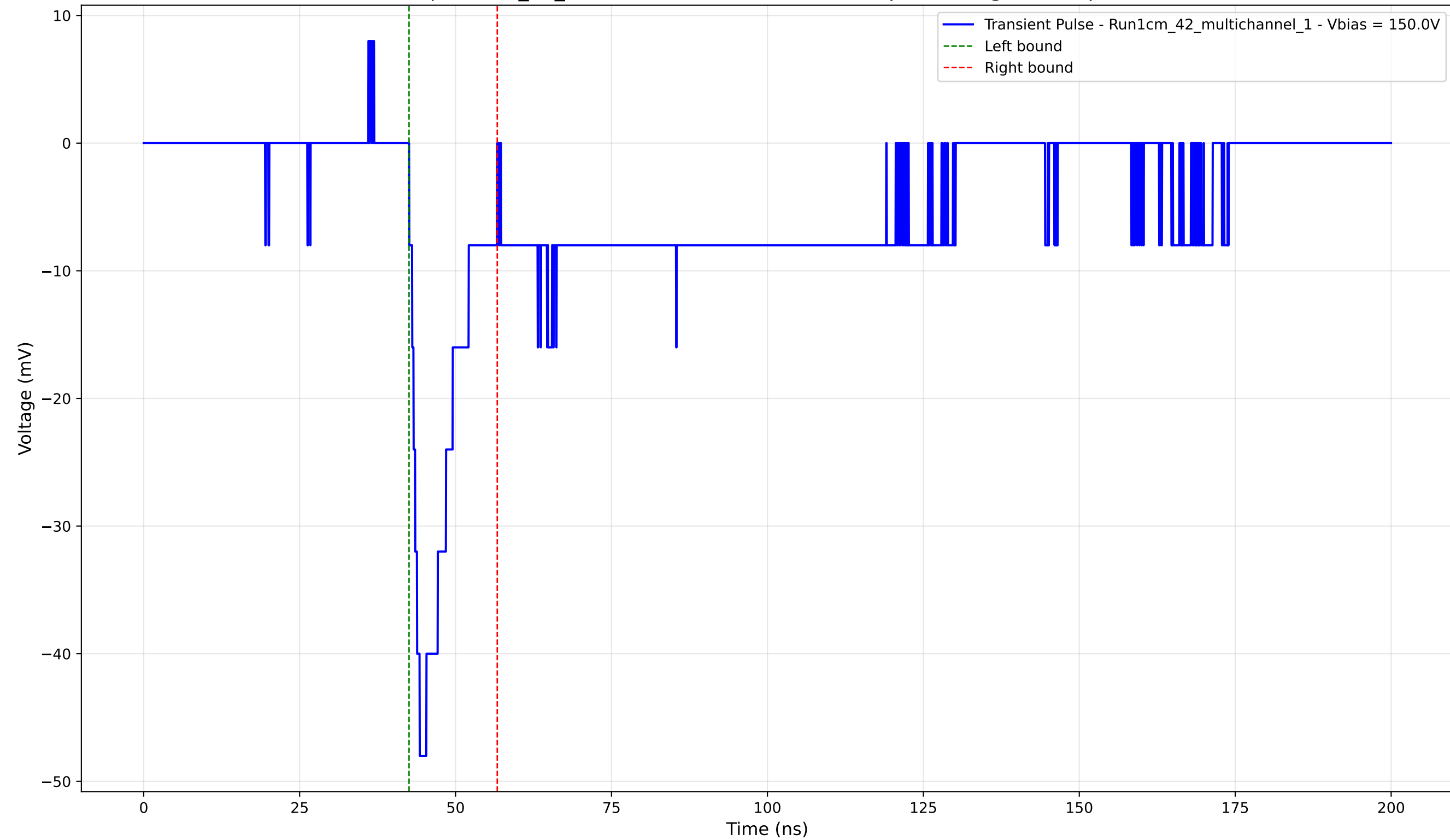
Transient Pulse - Sample: 1cm_42_multichannel - Position: 3840.0 \mu\text{m} - Charge: -6.21 pC - Rise Time: 1.69 ns
