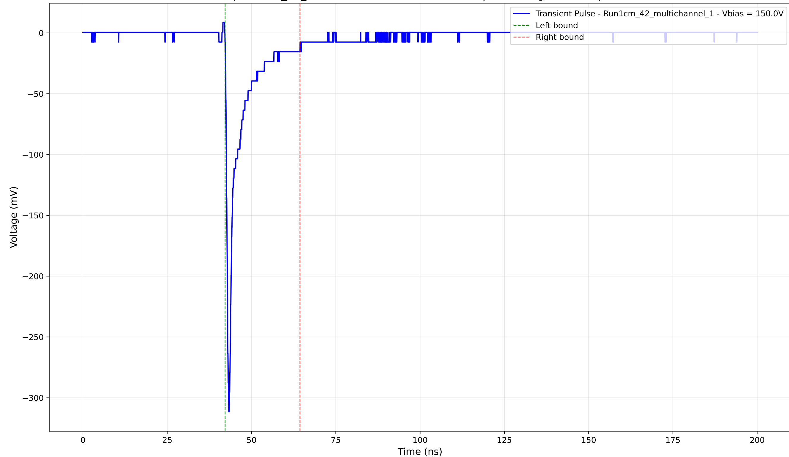
Transient Pulse - Sample: 1cm_42_multichannel - Position: 2105.0 \mu\text{m} - Charge: -24.02 pC - Rise Time: 0.80 ns
