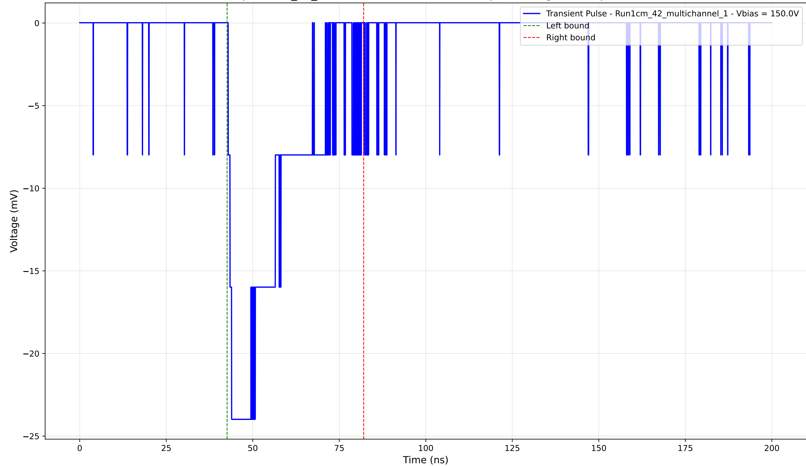
Transient Pulse - Sample: 1cm_42_multichannel - Position: 910.0 \mu\text{m} - Charge: -8.18 pC - Rise Time: 0.99 ns
