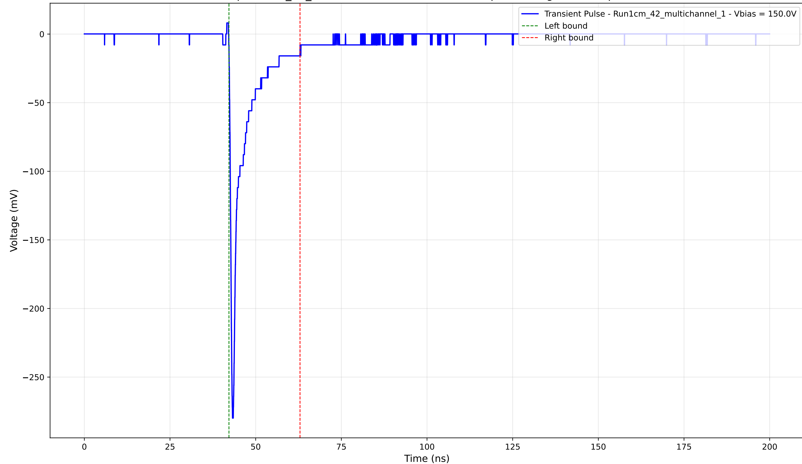
Transient Pulse - Sample: 1cm_42_multichannel - Position: 2705.0 \mu\text{m} - Charge: -22.54 pC - Rise Time: 0.77 ns
