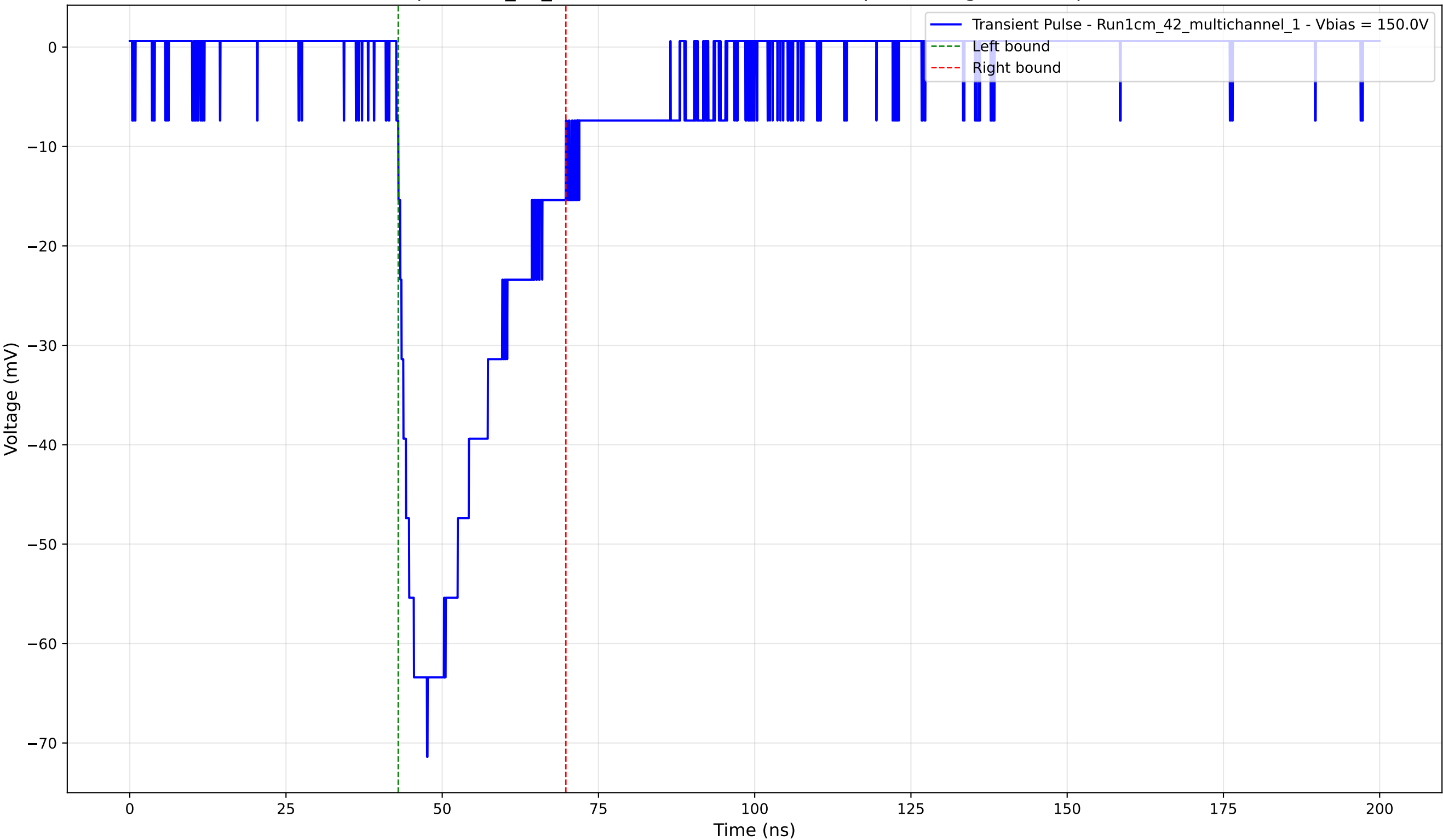
Transient Pulse - Sample: 1cm_42_multichannel - Position: 235.0 \mu\text{m} - Charge: -20.18 pC - Rise Time: 4.90 ns
