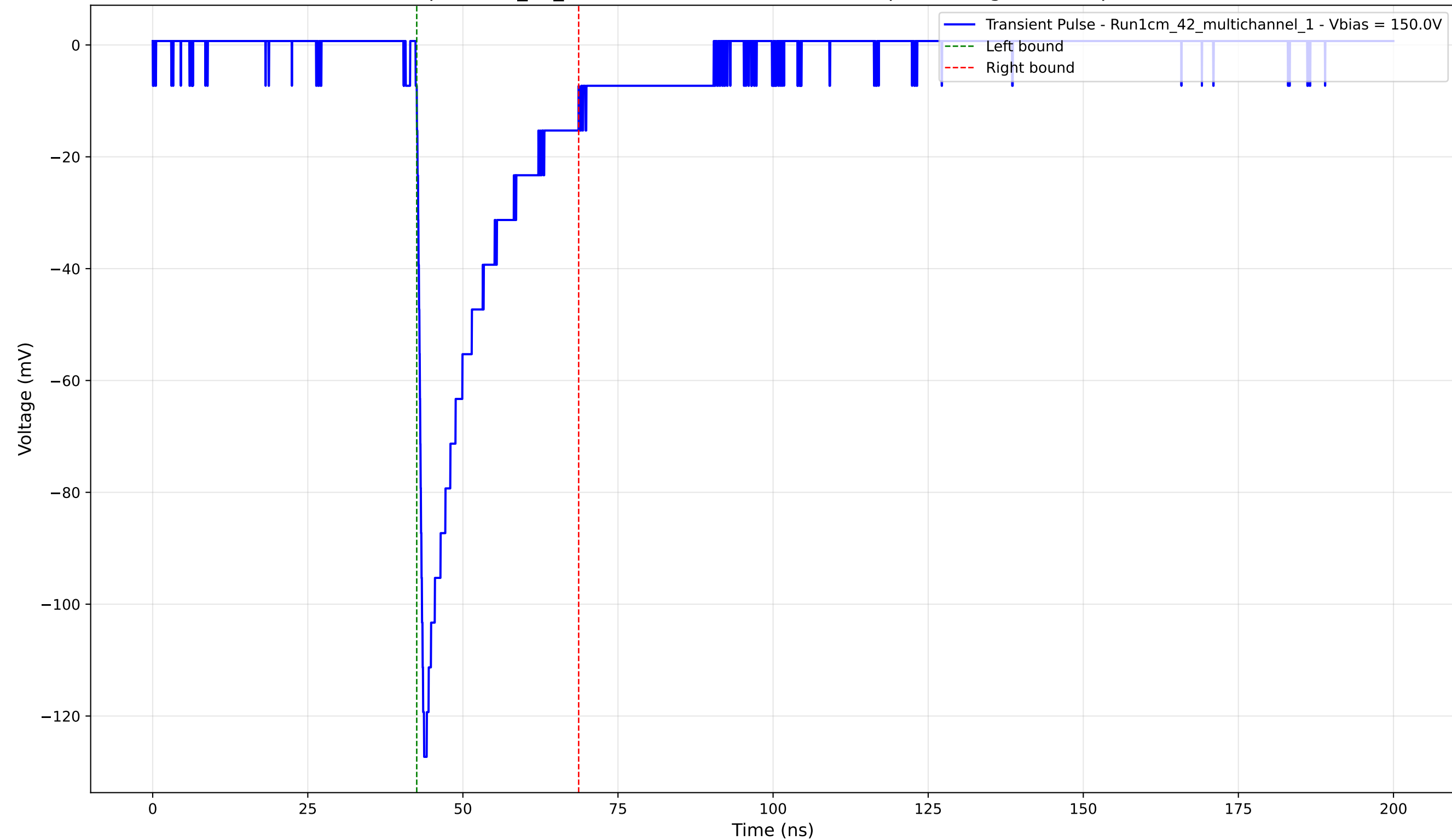
Transient Pulse - Sample: 1cm_42_multichannel - Position: 1480.0 \mu\text{m} - Charge: -23.38 pC - Rise Time: 1.01 ns
