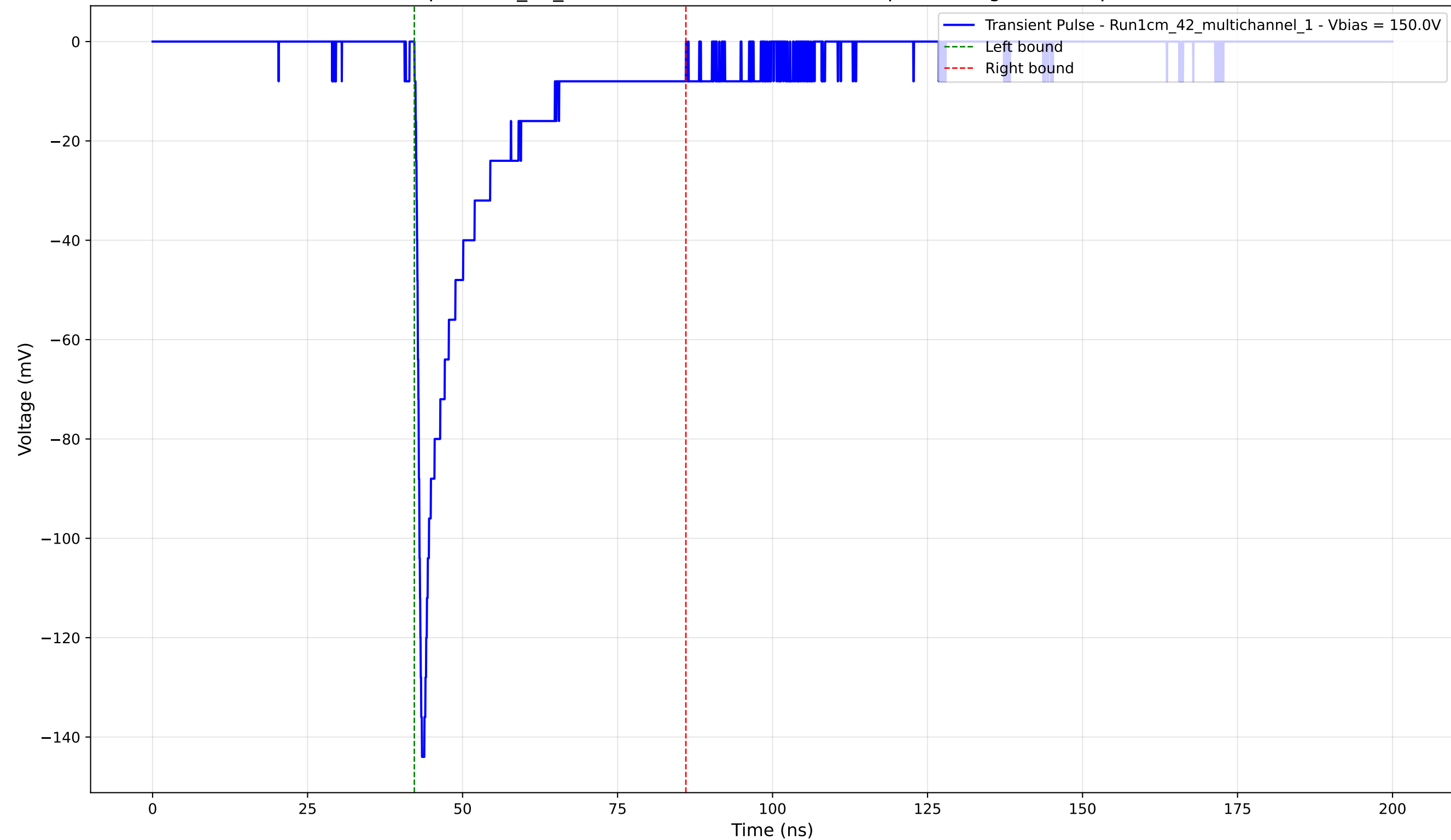
Transient Pulse - Sample: 1cm_42_multichannel - Position: 3065.0 \mu\text{m} - Charge: -22.49 pC - Rise Time: 0.90 ns
