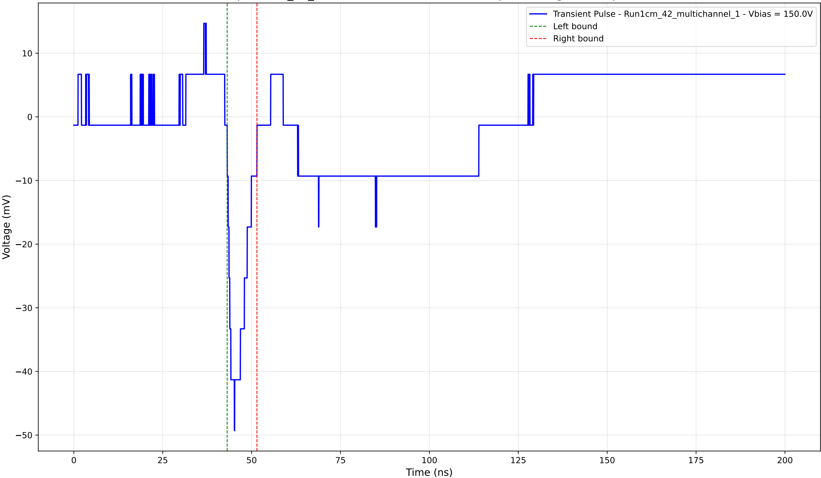
Transient Pulse - Sample: 1cm_42_multichannel - Position: 4040.0 \mu\text{m} - Charge: -4.52 pC - Rise Time: 2.01 ns
