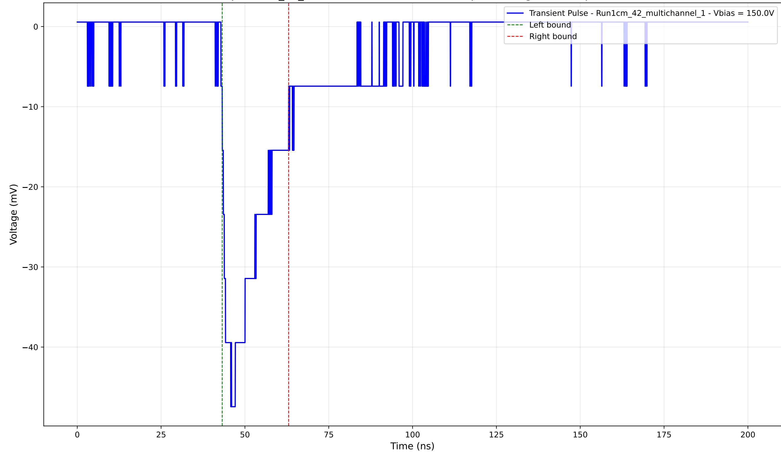
Transient Pulse - Sample: 1cm_42_multichannel - Position: 815.0 \mu\text{m} - Charge: -11.01 pC - Rise Time: 2.93 ns
