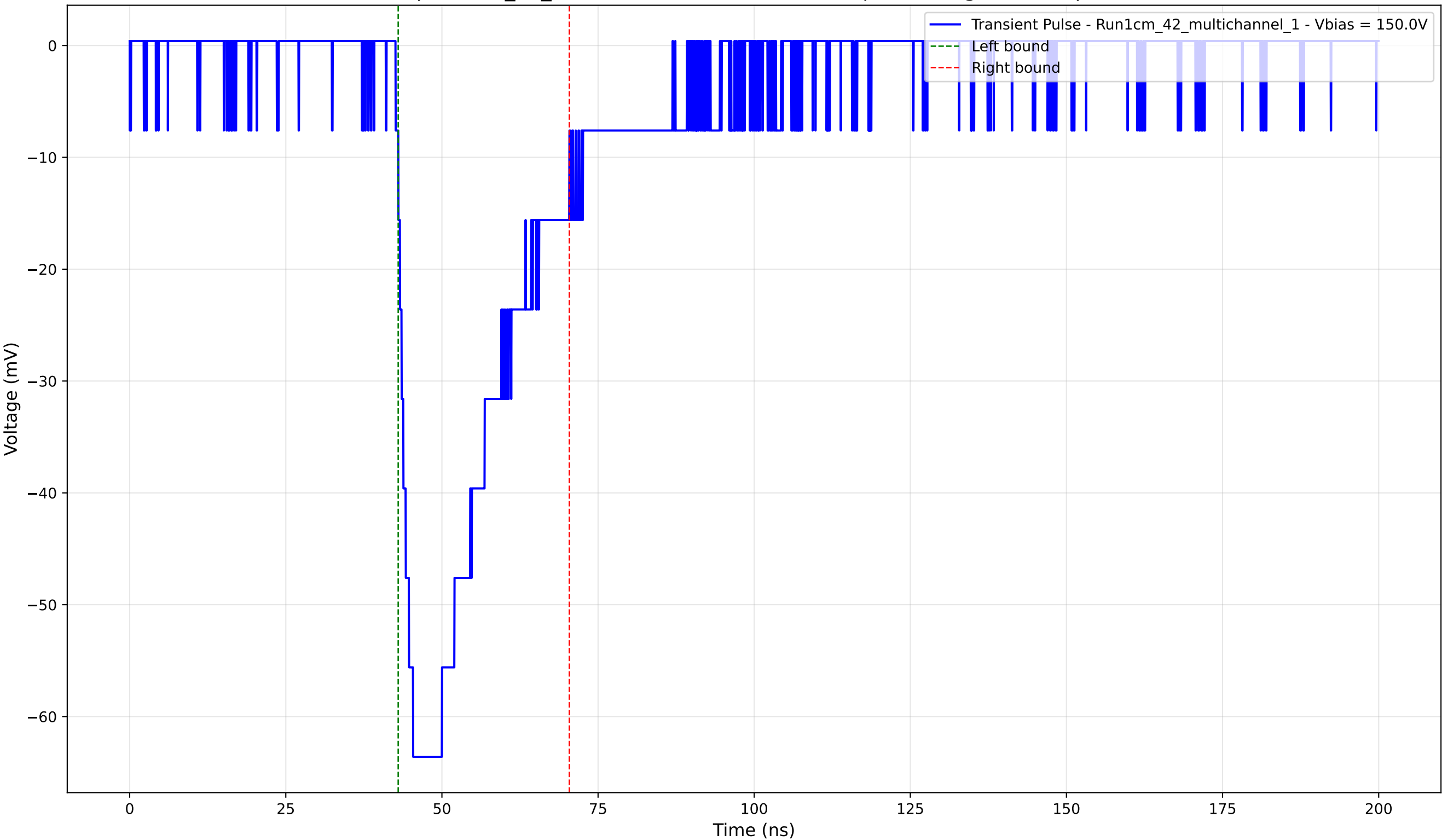
Transient Pulse - Sample: 1cm_42_multichannel - Position: 260.0 \mu\text{m} - Charge: -20.34 pC - Rise Time: 2.80 ns
