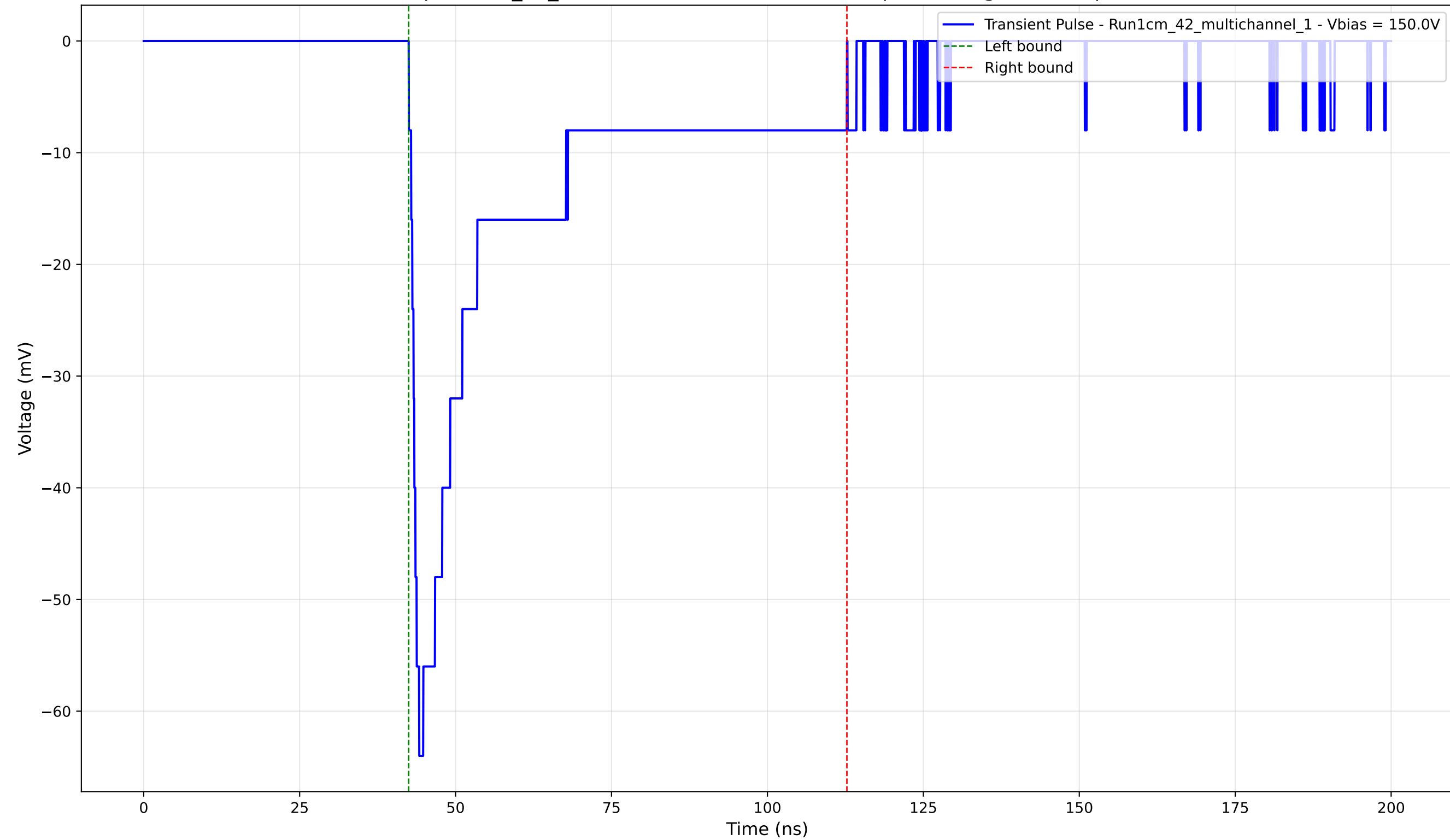
Transient Pulse - Sample: 1cm_42_multichannel - Position: 3700.0 \mu\text{m} - Charge: -20.33 pC - Rise Time: 1.66 ns
