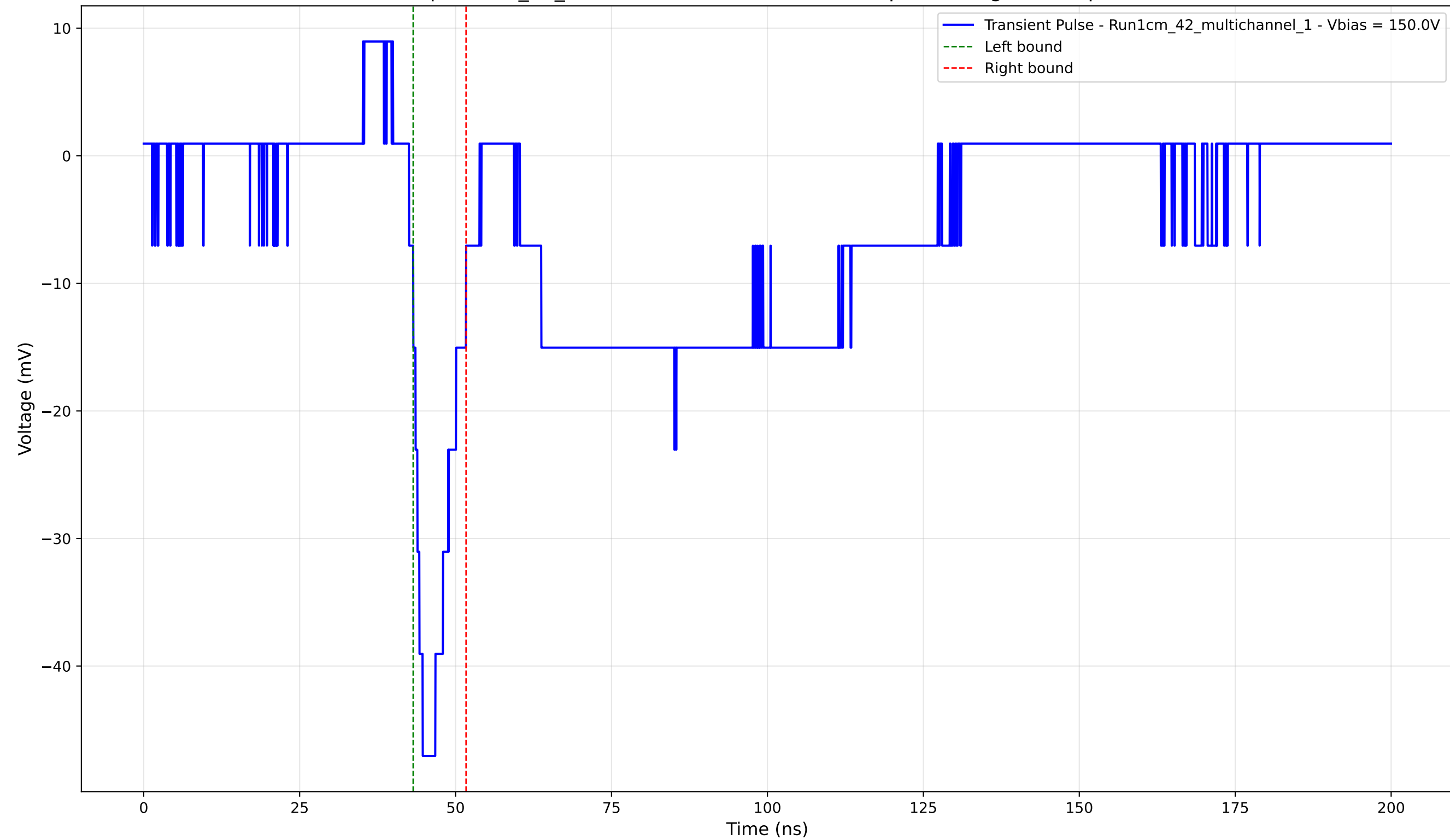
Transient Pulse - Sample: 1cm_42_multichannel - Position: 4555.0 \mu\text{m} - Charge: -5.32 pC - Rise Time: 2.19 ns
