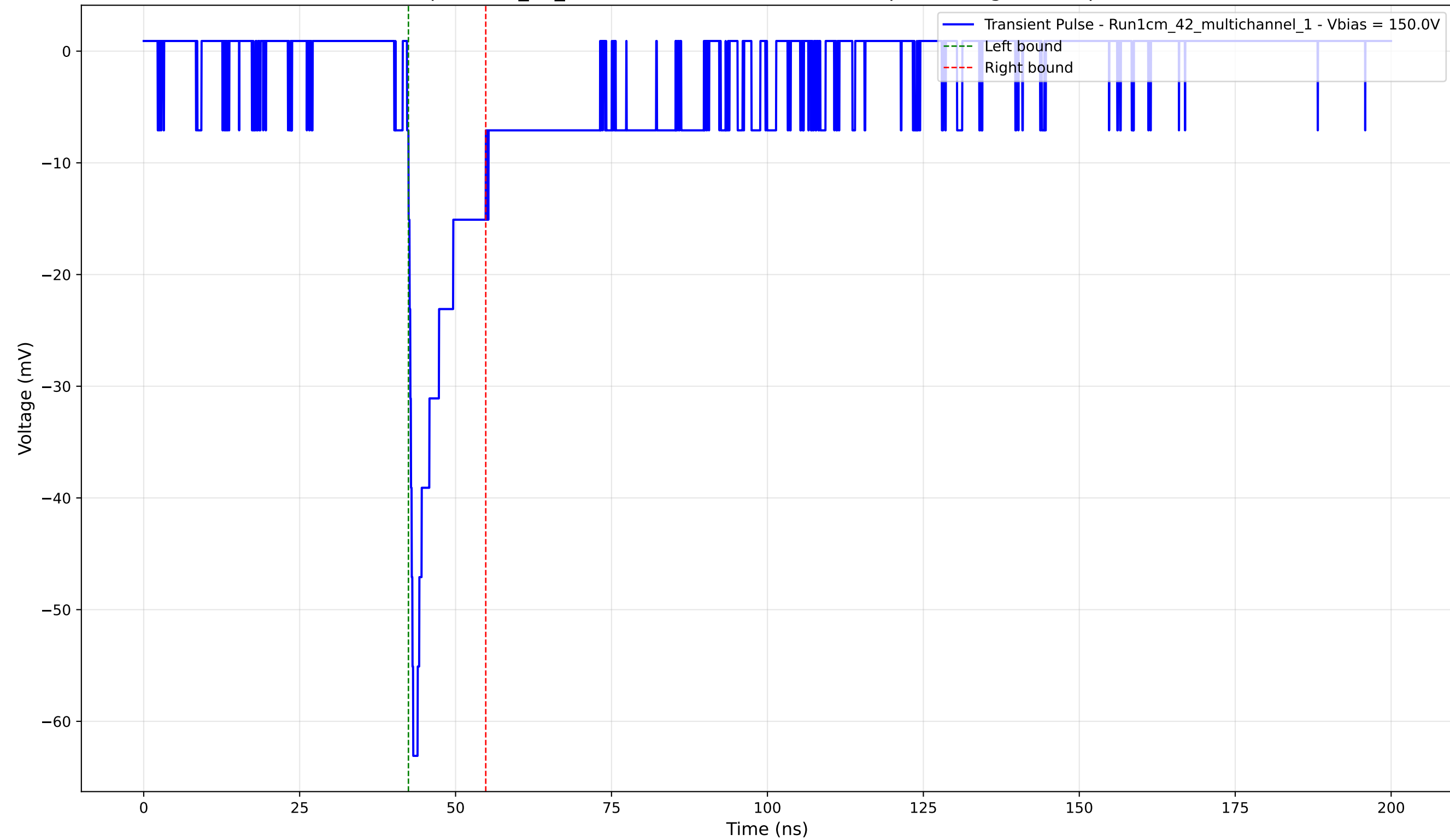
Transient Pulse - Sample: 1cm_42_multichannel - Position: 2940.0 \mu\text{m} - Charge: -6.62 pC - Rise Time: 0.98 ns
