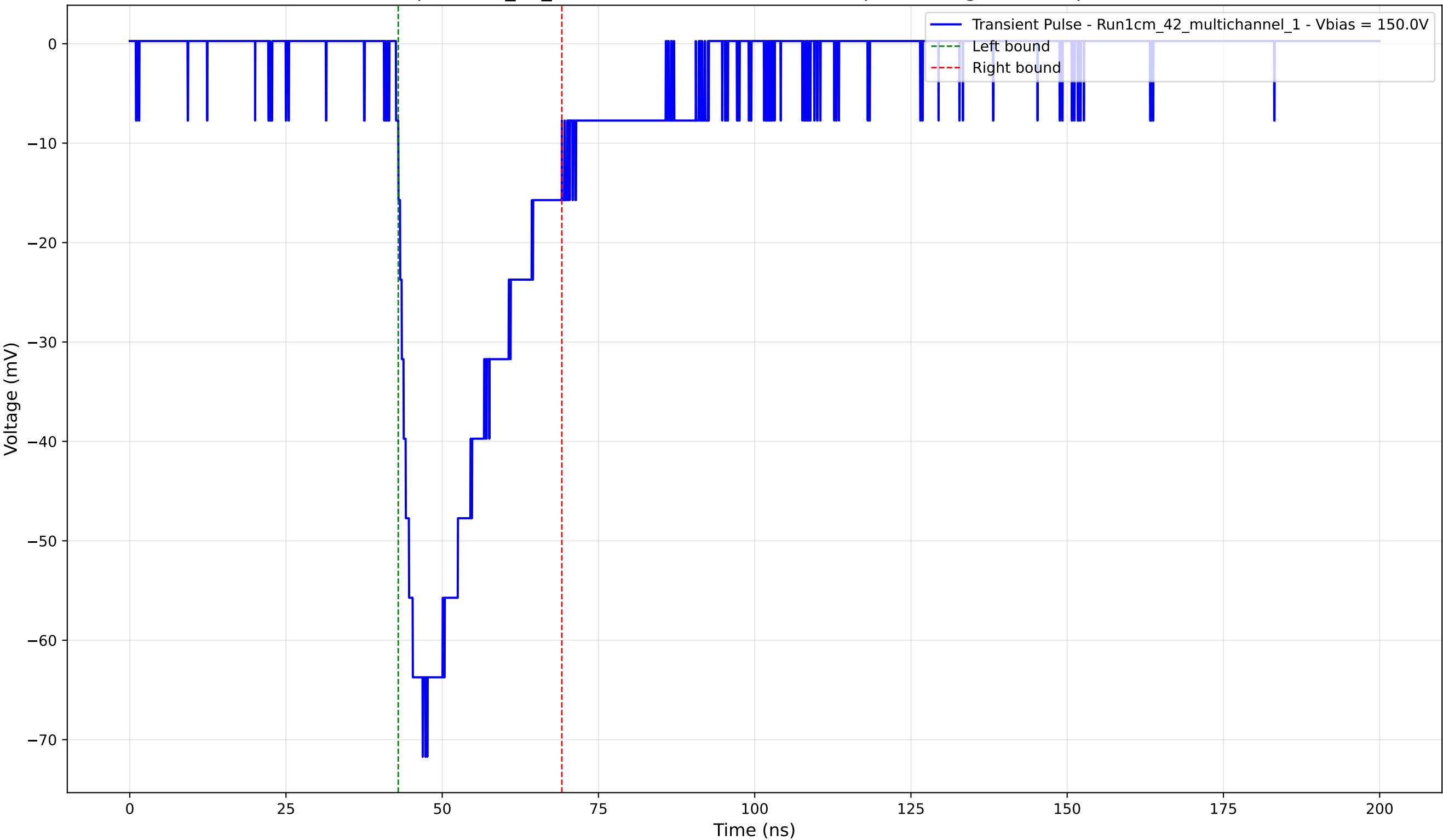
Transient Pulse - Sample: 1cm_42_multichannel - Position: 220.0 \mu\text{m} - Charge: -20.23 pC - Rise Time: 4.26 ns
