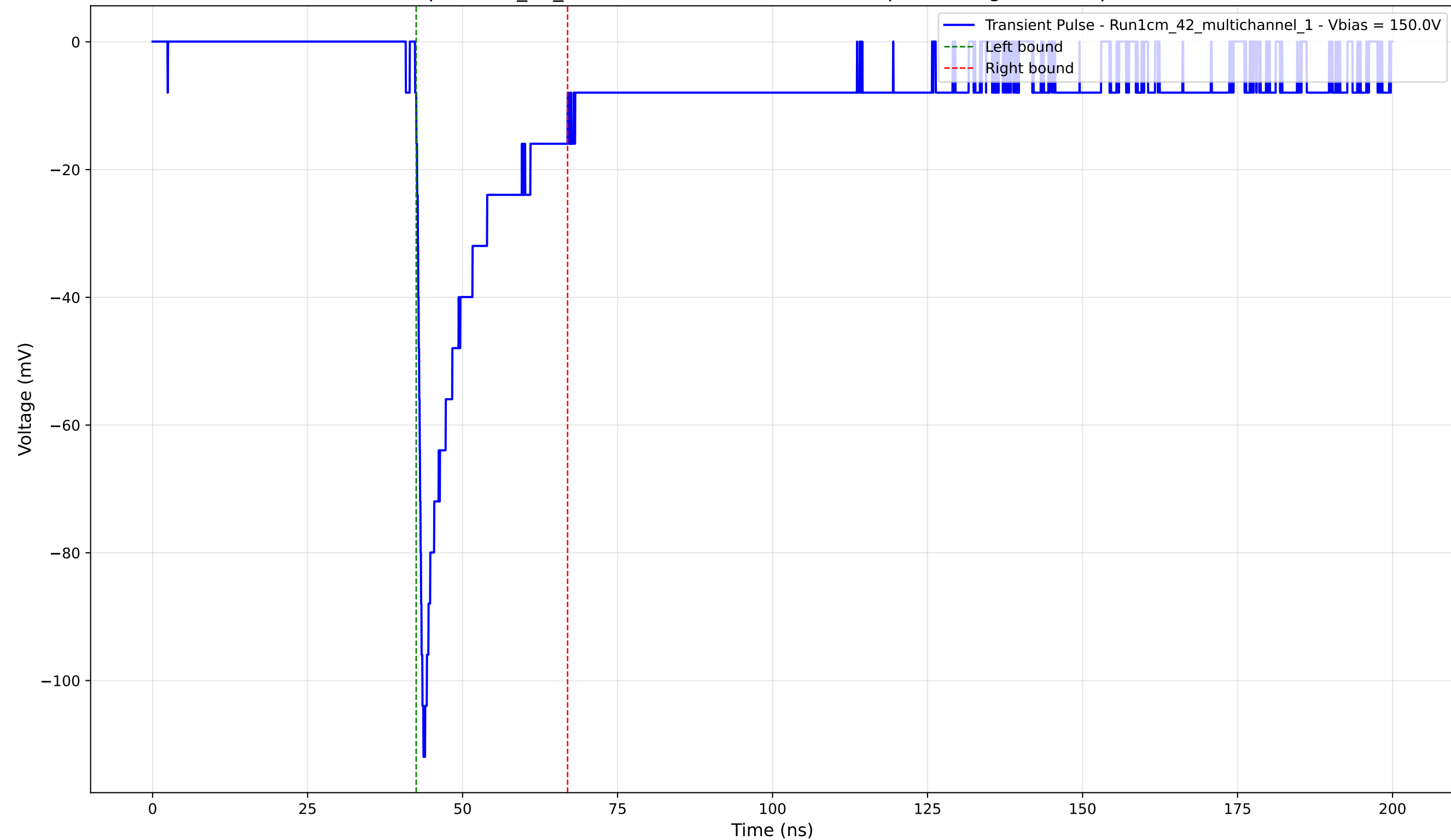
Transient Pulse - Sample: 1cm_42_multichannel - Position: 3265.0 \mu\text{m} - Charge: -17.90 pC - Rise Time: 0.99 ns
