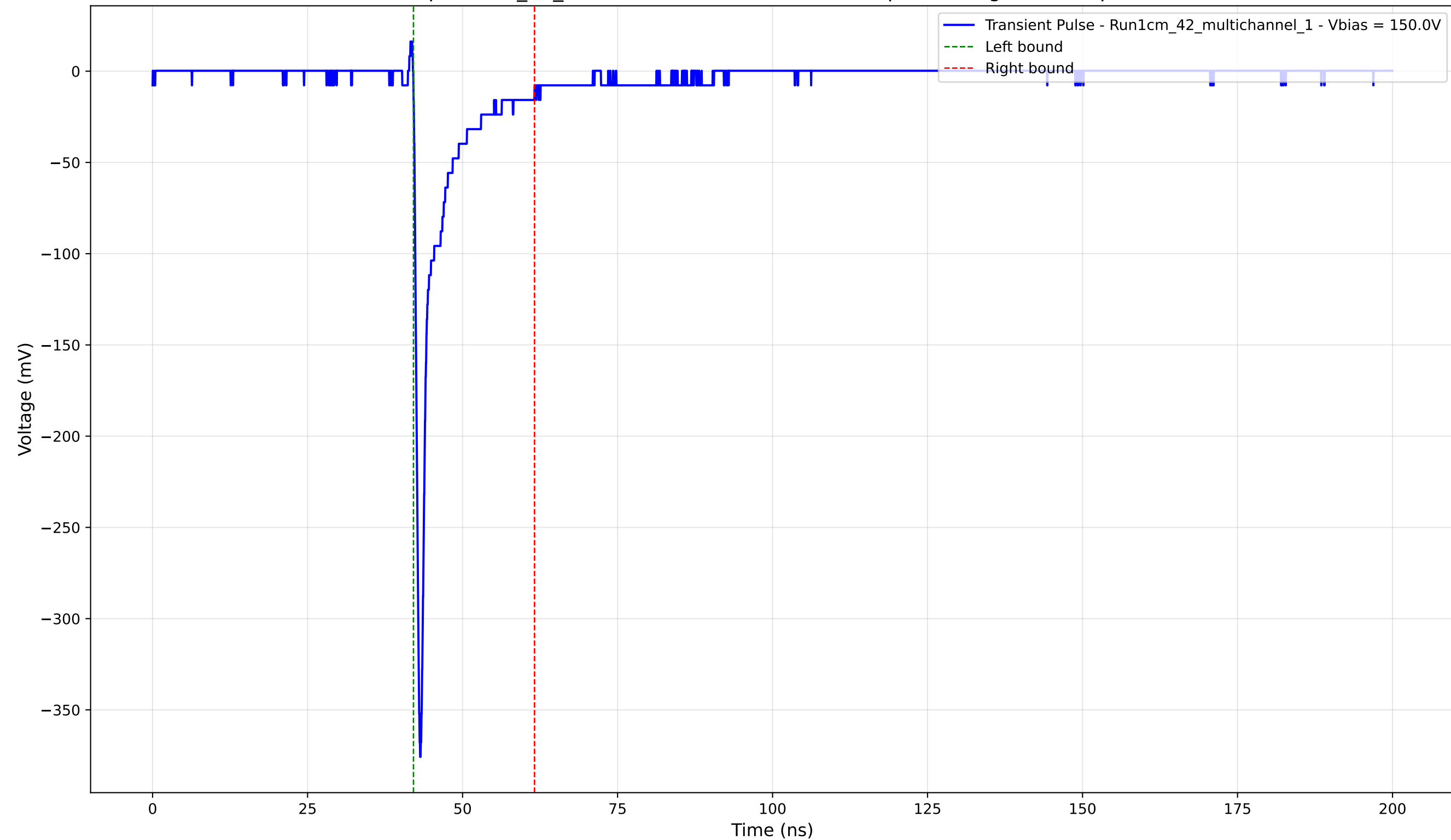
Transient Pulse - Sample: 1cm_42_multichannel - Position: 2535.0 \mu\text{m} - Charge: -23.88 pC - Rise Time: 0.77 ns
