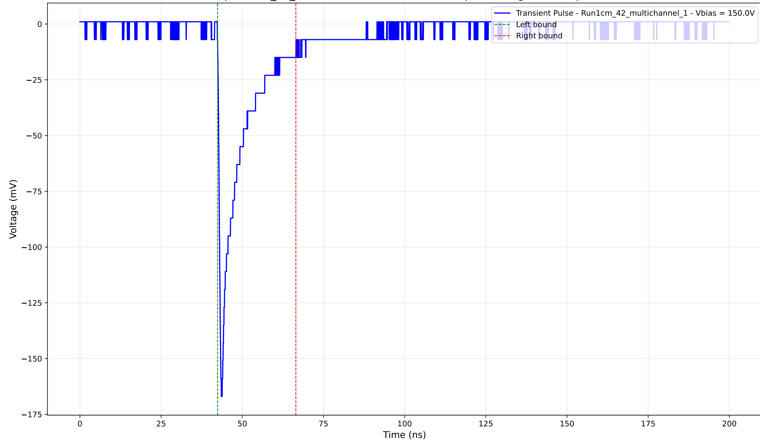
Transient Pulse - Sample: 1cm_42_multichannel - Position: 1710.0 \mu\text{m} - Charge: -22.61 pC - Rise Time: 0.84 ns
