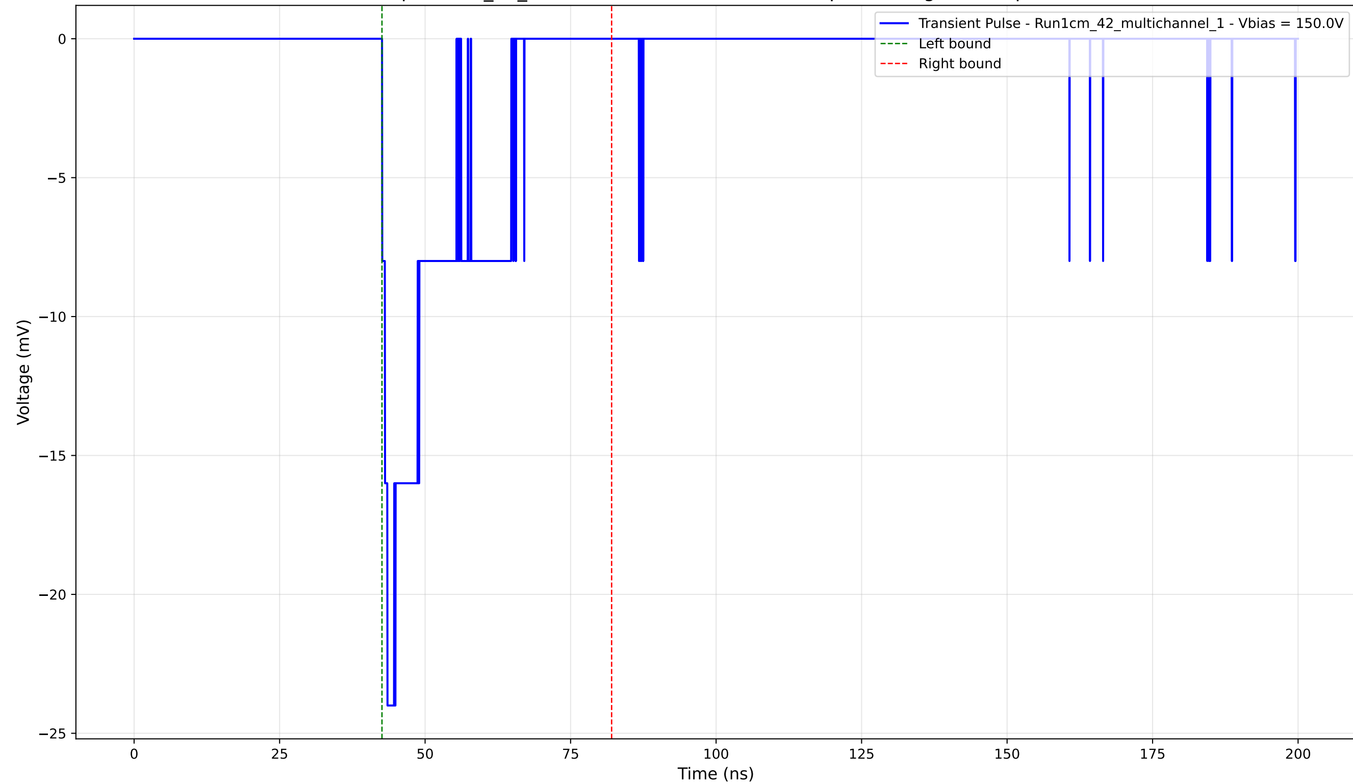
Transient Pulse - Sample: 1cm_42_multichannel - Position: 3440.0 \mu\text{m} - Charge: -4.60 pC - Rise Time: 0.91 ns
