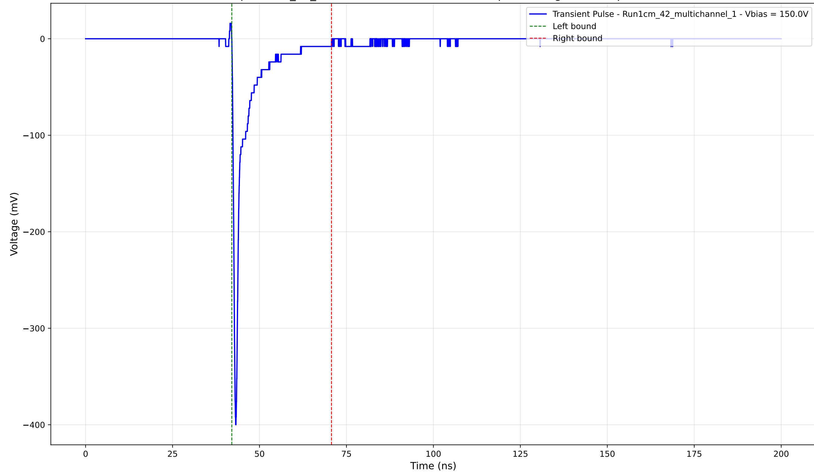
Transient Pulse - Sample: 1cm_42_multichannel - Position: 2265.0 \mu\text{m} - Charge: -26.04 pC - Rise Time: 0.72 ns
