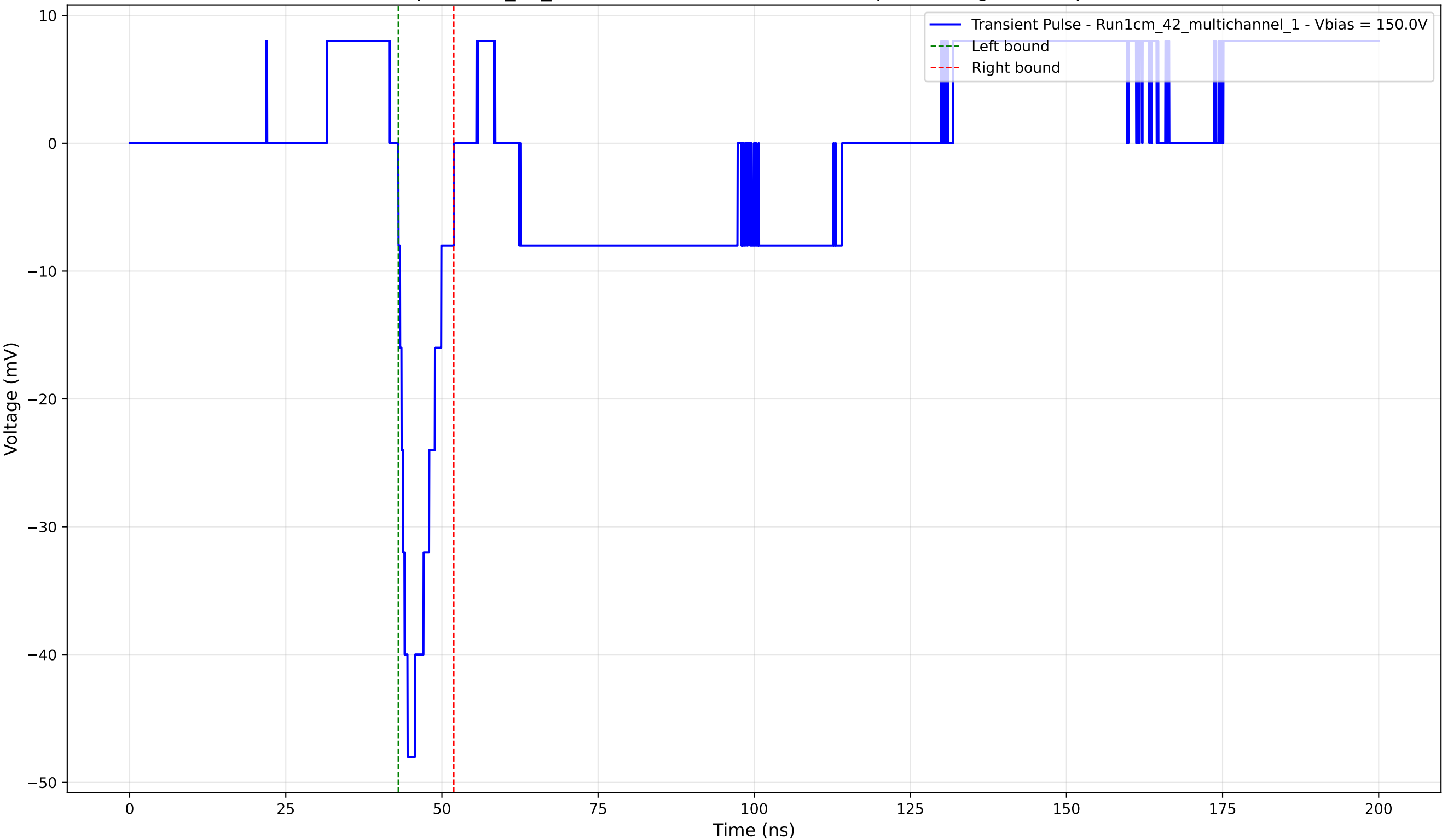
Transient Pulse - Sample: 1cm_42_multichannel - Position: 4020.0 \mu\text{m} - Charge: -4.68 pC - Rise Time: 1.47 ns
