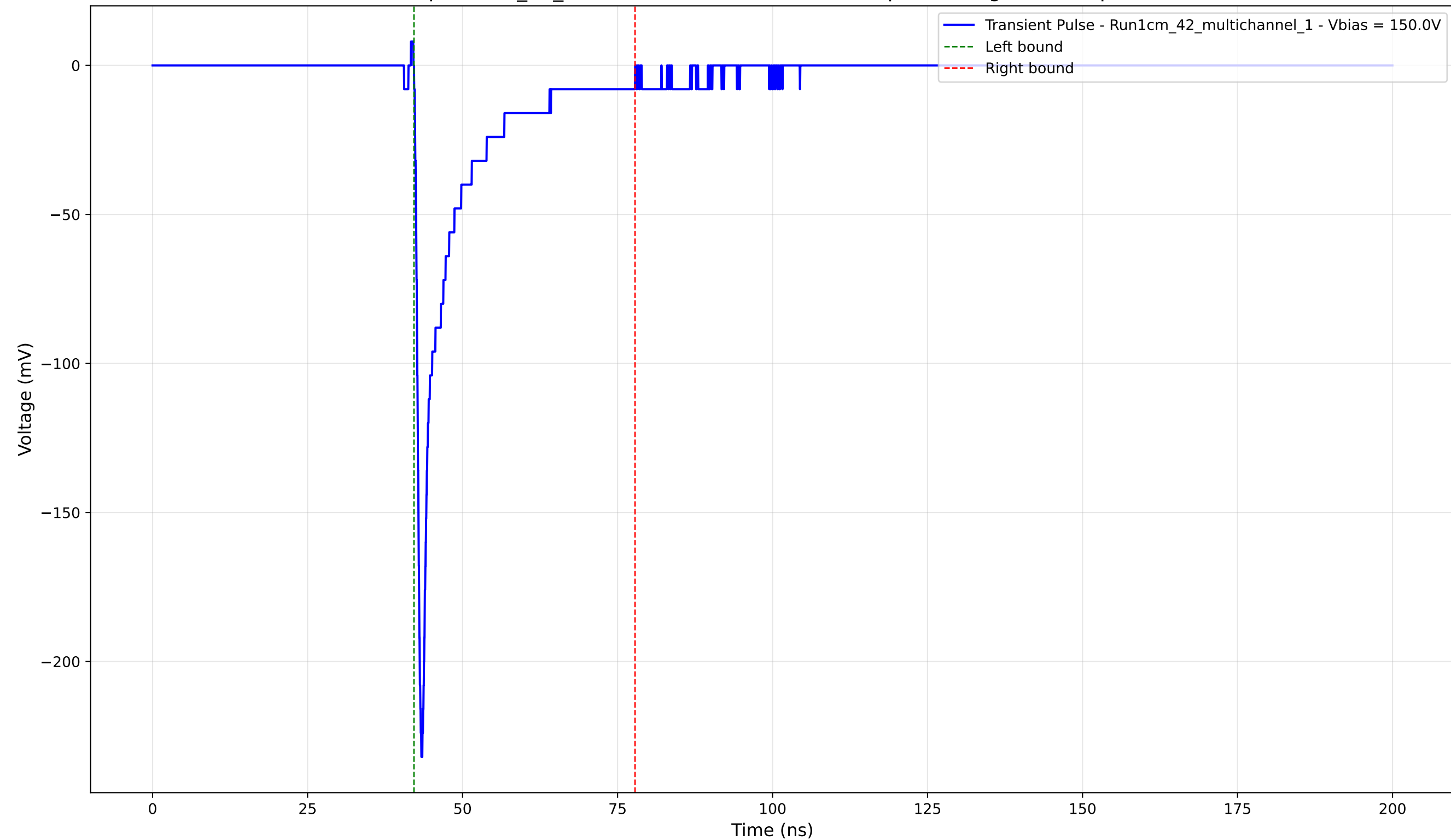
Transient Pulse - Sample: 1cm_42_multichannel - Position: 2790.0 \mu\text{m} - Charge: -23.40 pC - Rise Time: 0.84 ns
