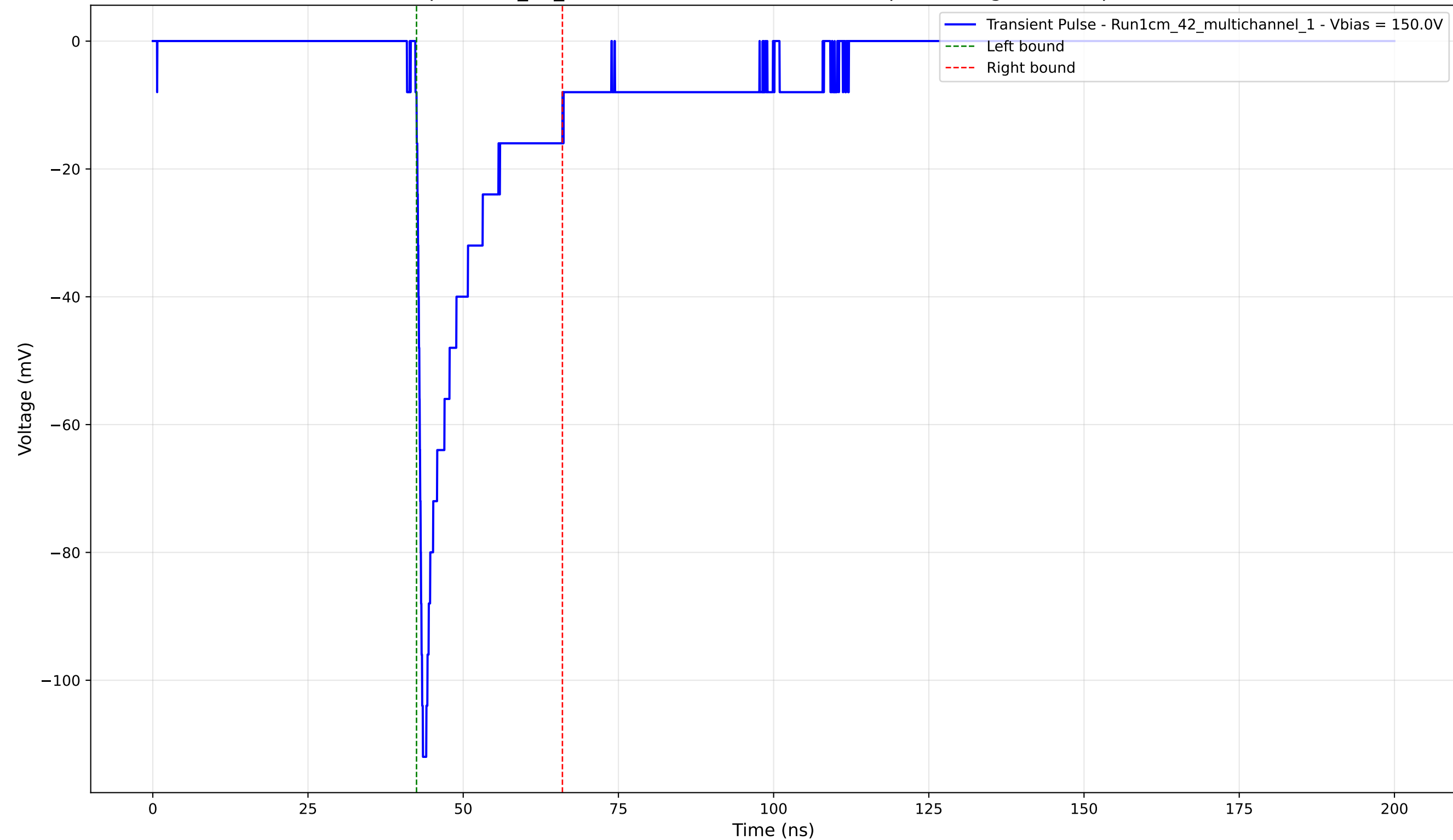
Transient Pulse - Sample: 1cm_42_multichannel - Position: 3215.0 \mu\text{m} - Charge: -16.36 pC - Rise Time: 0.89 ns
