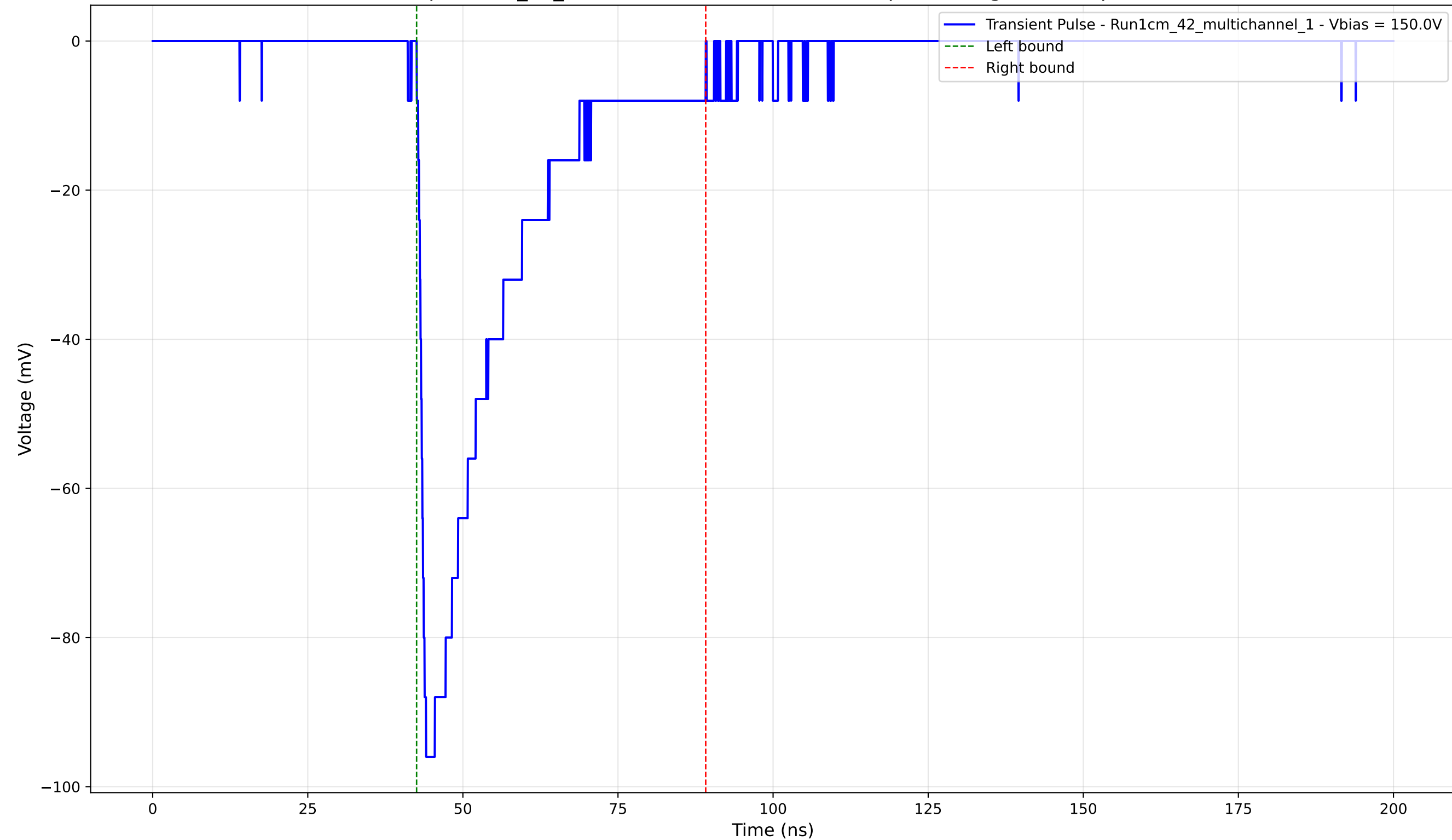
Transient Pulse - Sample: 1cm_42_multichannel - Position: 1195.0 \mu\text{m} - Charge: -26.50 pC - Rise Time: 1.04 ns
