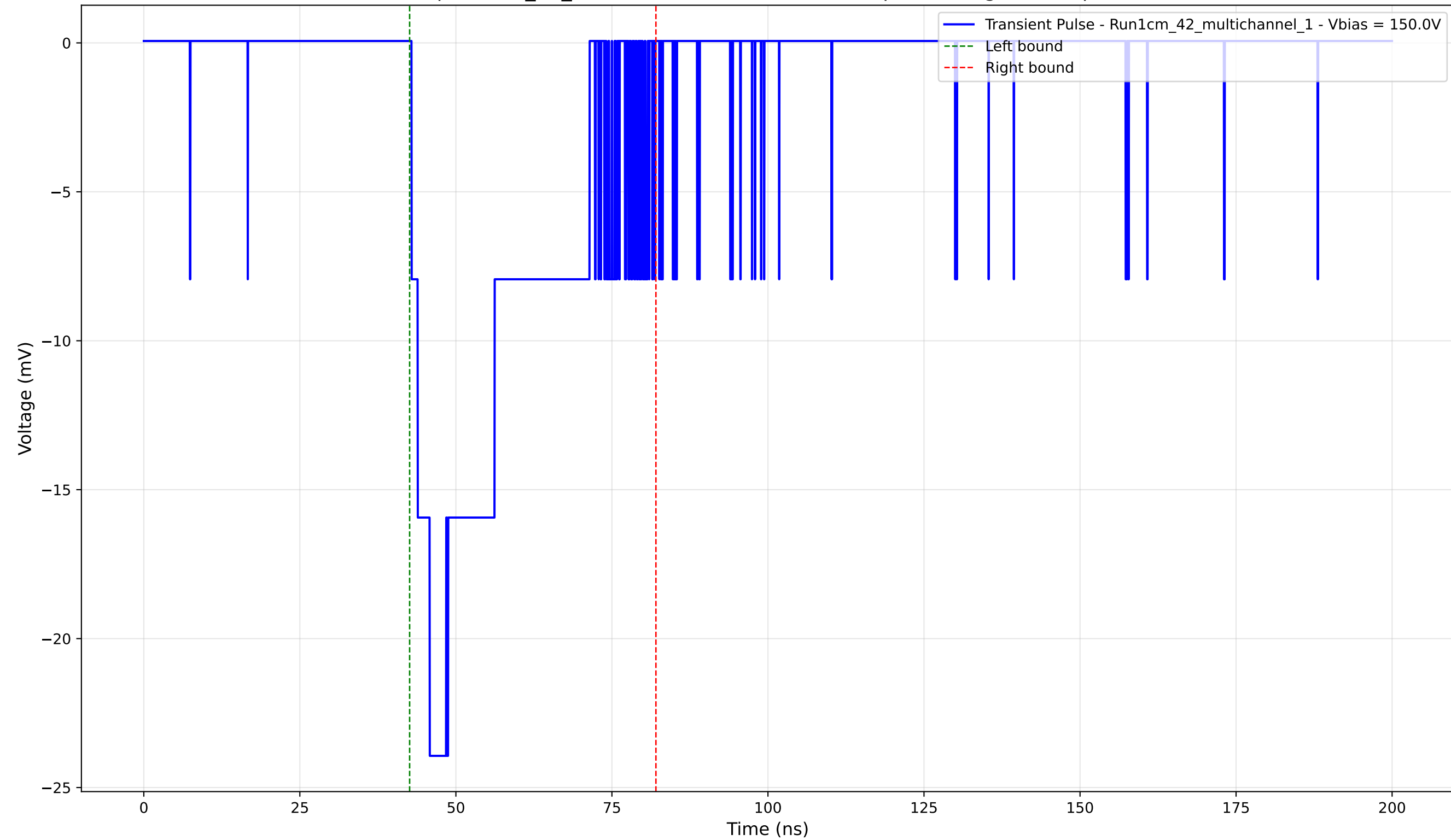
Transient Pulse - Sample: 1cm_42_multichannel - Position: 320.0 \mu\text{m} - Charge: -7.55 pC - Rise Time: 2.91 ns
