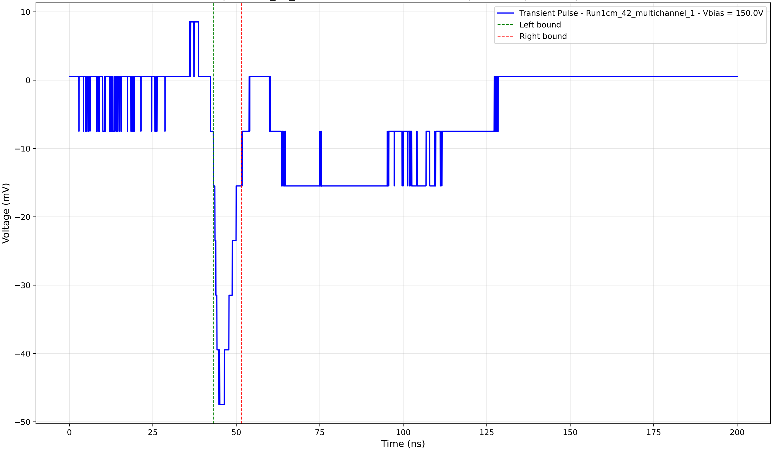
Transient Pulse - Sample: 1cm_42_multichannel - Position: 4600.0 \mu\text{m} - Charge: -5.26 pC - Rise Time: 2.51 ns
