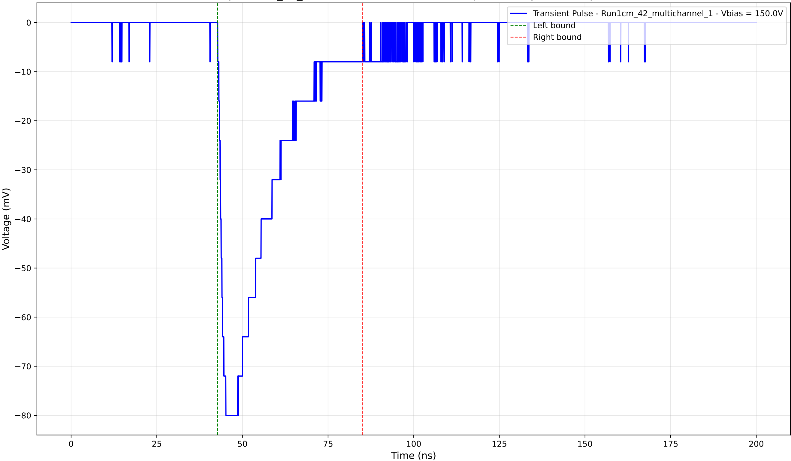
Transient Pulse - Sample: 1cm_42_multichannel - Position: 680.0 \mu\text{m} - Charge: -26.13 pC - Rise Time: 1.48 ns
