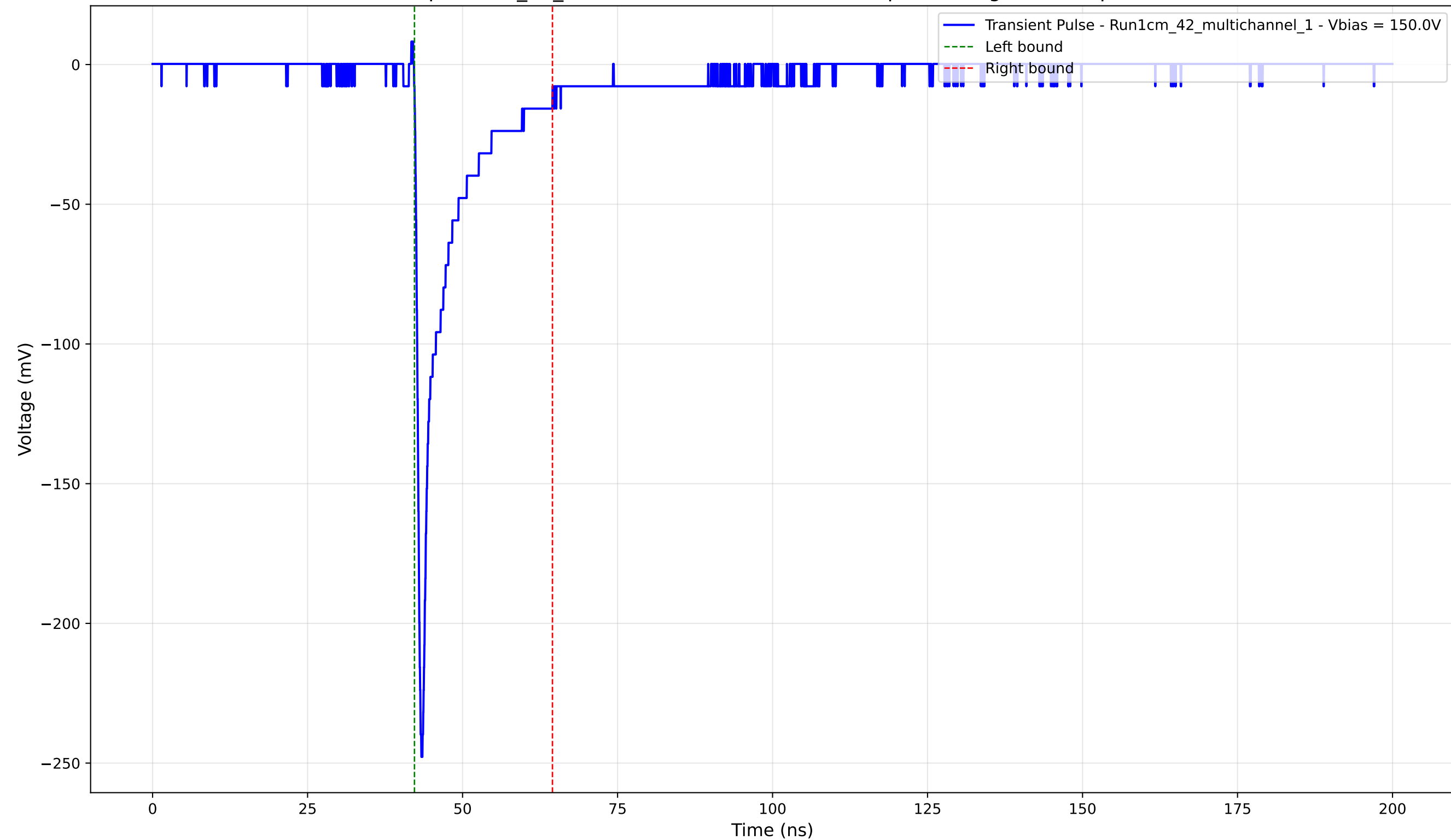
Transient Pulse - Sample: 1cm_42_multichannel - Position: 1980.0 \mu\text{m} - Charge: -23.42 pC - Rise Time: 0.78 ns
