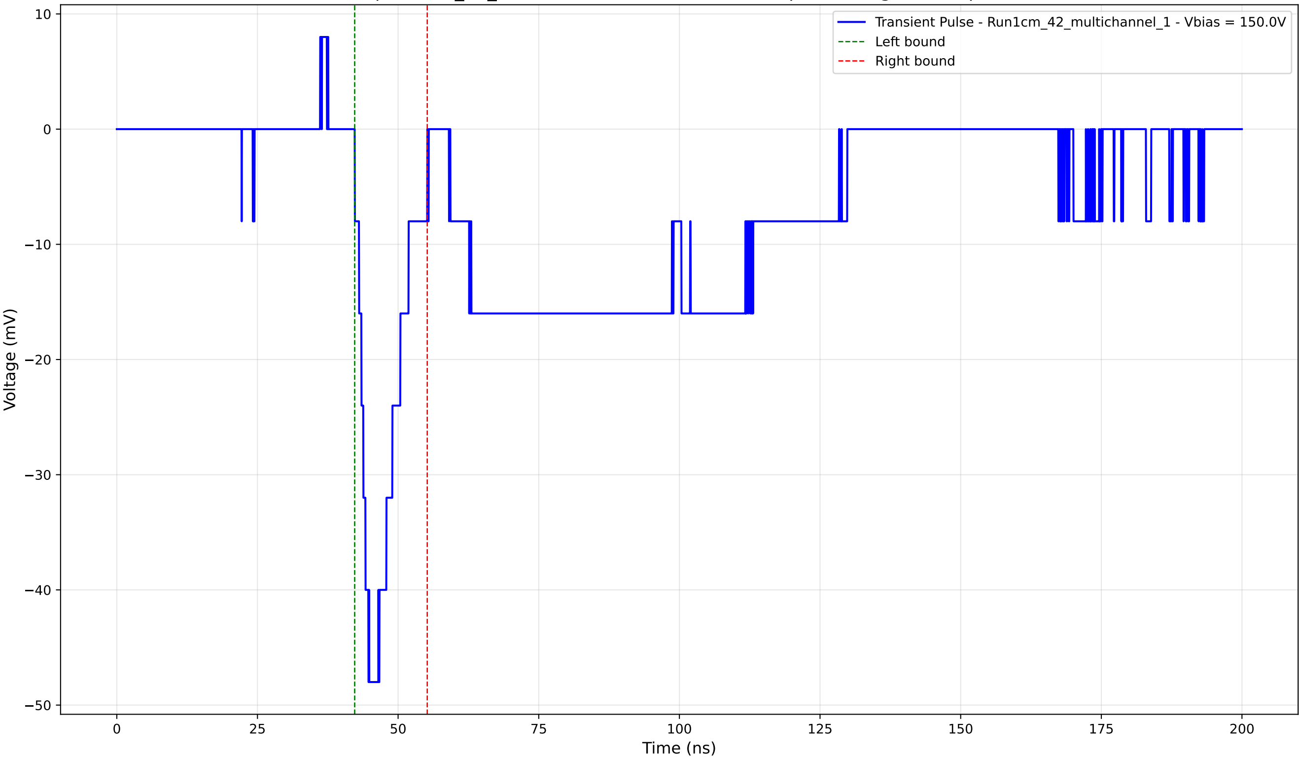
Transient Pulse - Sample: 1cm_42_multichannel - Position: 4635.0 \mu\text{m} - Charge: -6.30 pC - Rise Time: 2.43 ns
