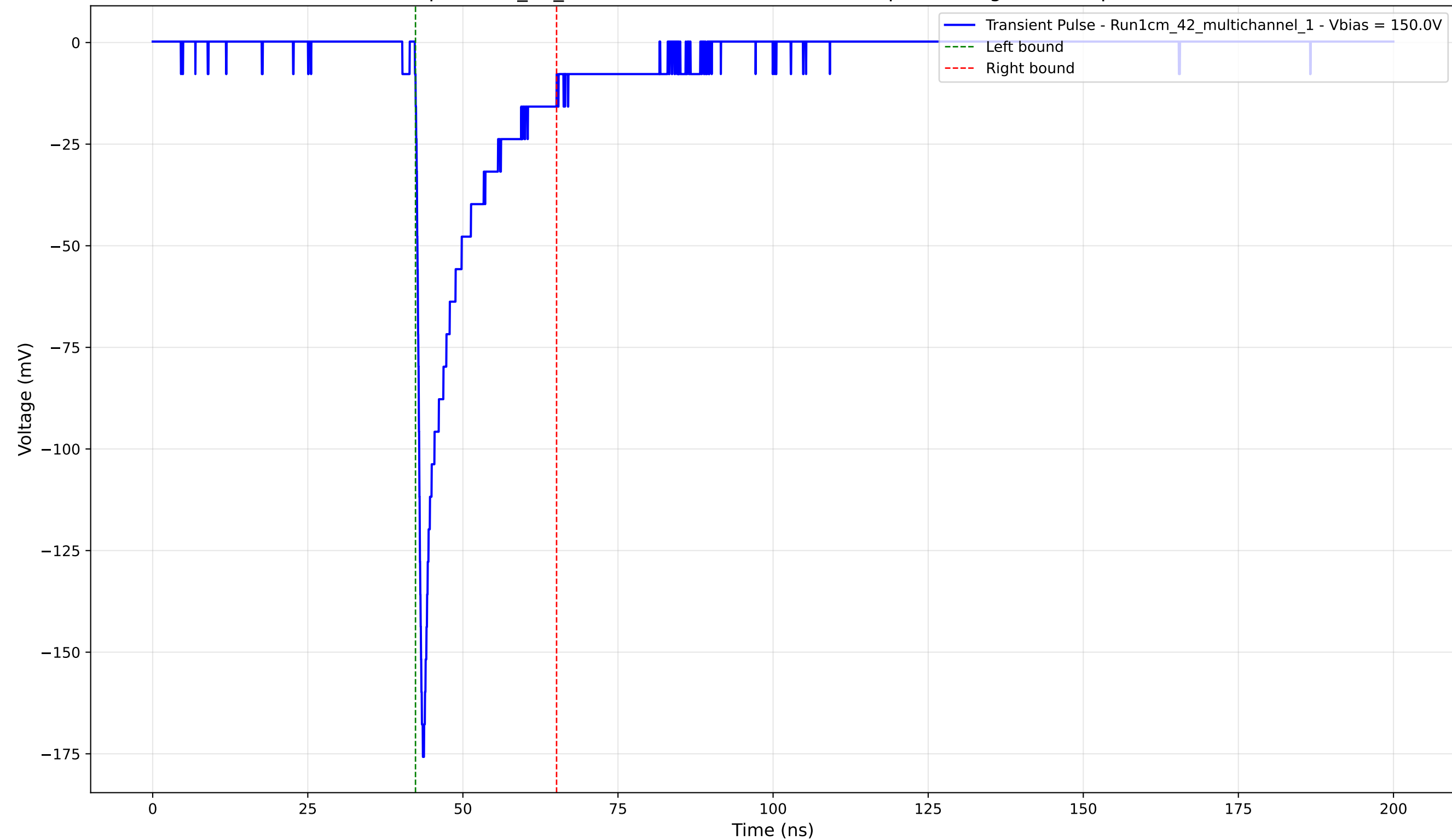
Transient Pulse - Sample: 1cm_42_multichannel - Position: 1760.0 \mu\text{m} - Charge: -21.89 pC - Rise Time: 0.86 ns
