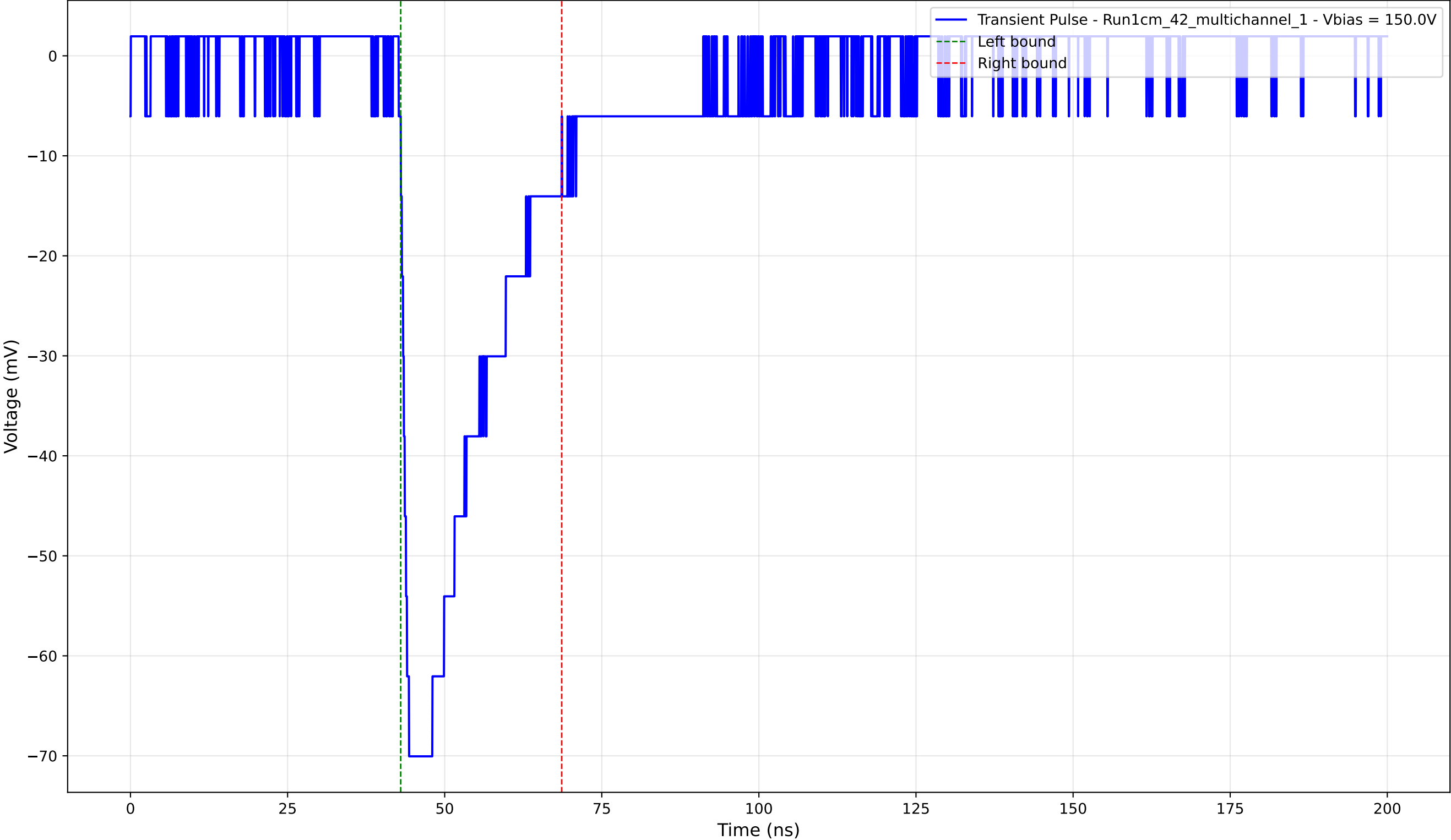
Transient Pulse - Sample: 1cm_42_multichannel - Position: 940.0 \mu\text{m} - Charge: -19.37 pC - Rise Time: 1.32 ns
