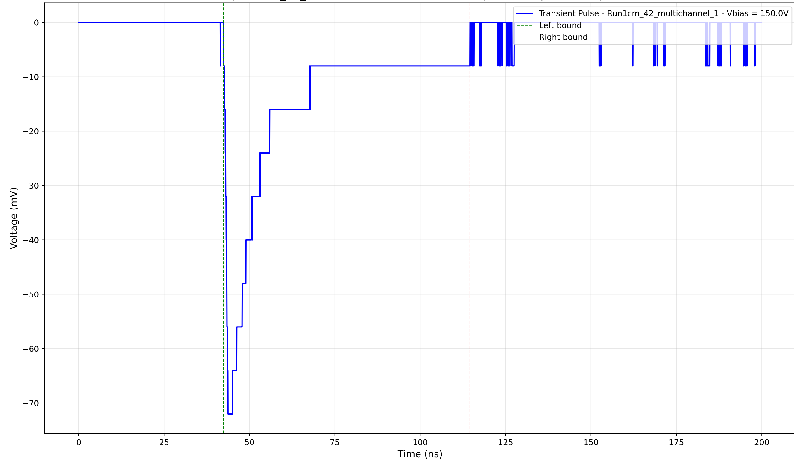
Transient Pulse - Sample: 1cm_42_multichannel - Position: 3545.0 \mu\text{m} - Charge: -22.70 pC - Rise Time: 1.28 ns
