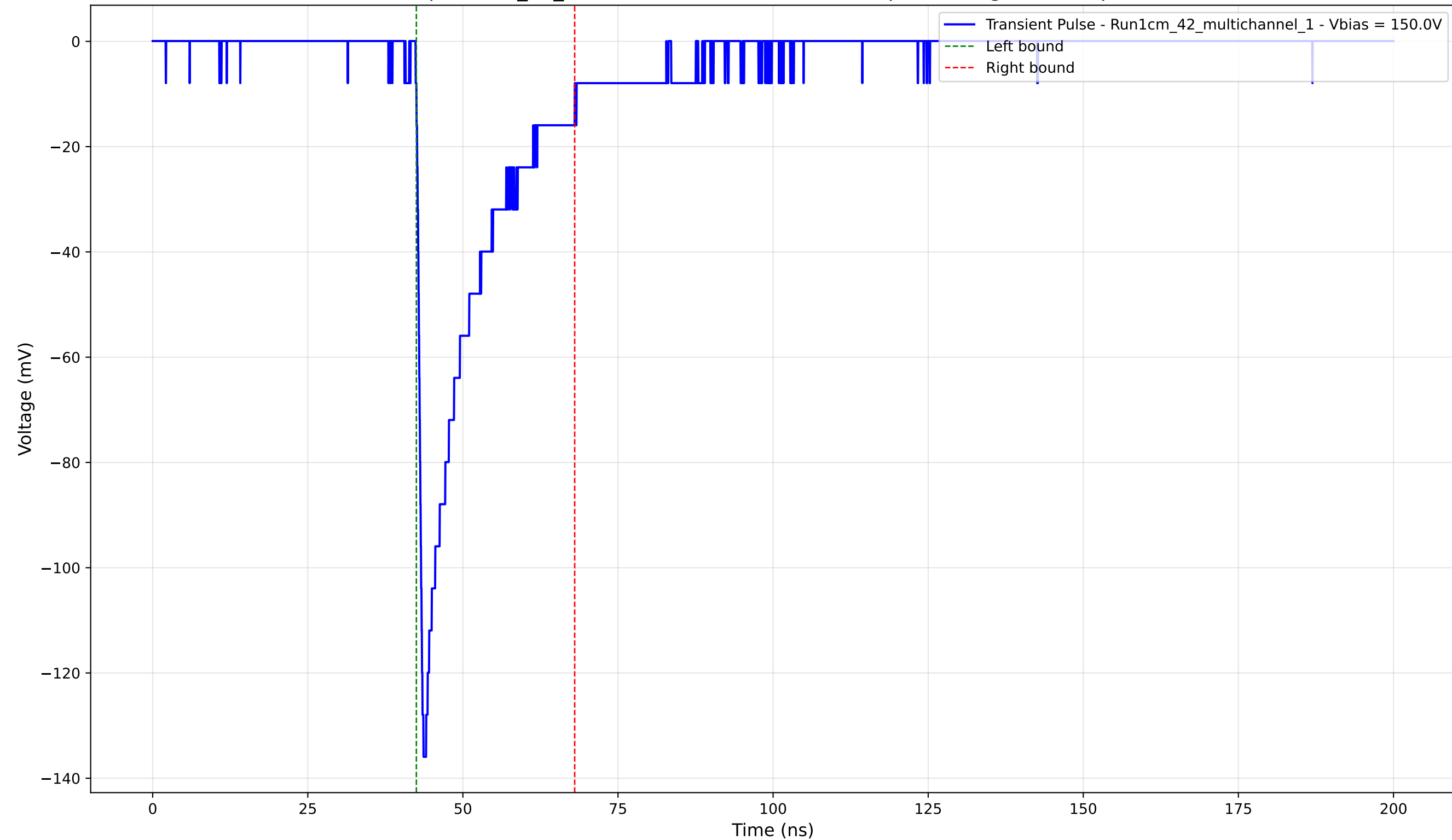
Transient Pulse - Sample: 1cm_42_multichannel - Position: 1555.0 \mu\text{m} - Charge: -23.29 pC - Rise Time: 0.97 ns
