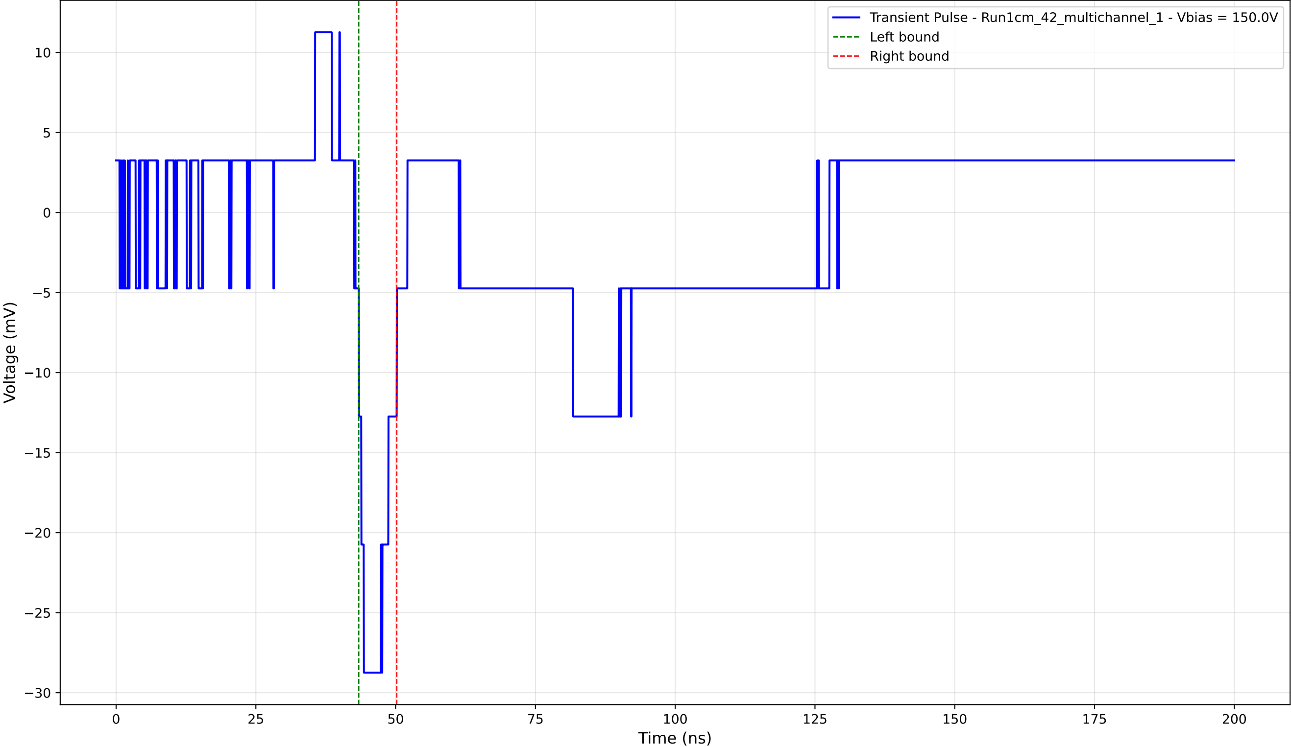
Transient Pulse - Sample: 1cm_42_multichannel - Position: 4345.0 \mu\text{m} - Charge: -3.01 pC - Rise Time: 0.00 ns (N/A)
