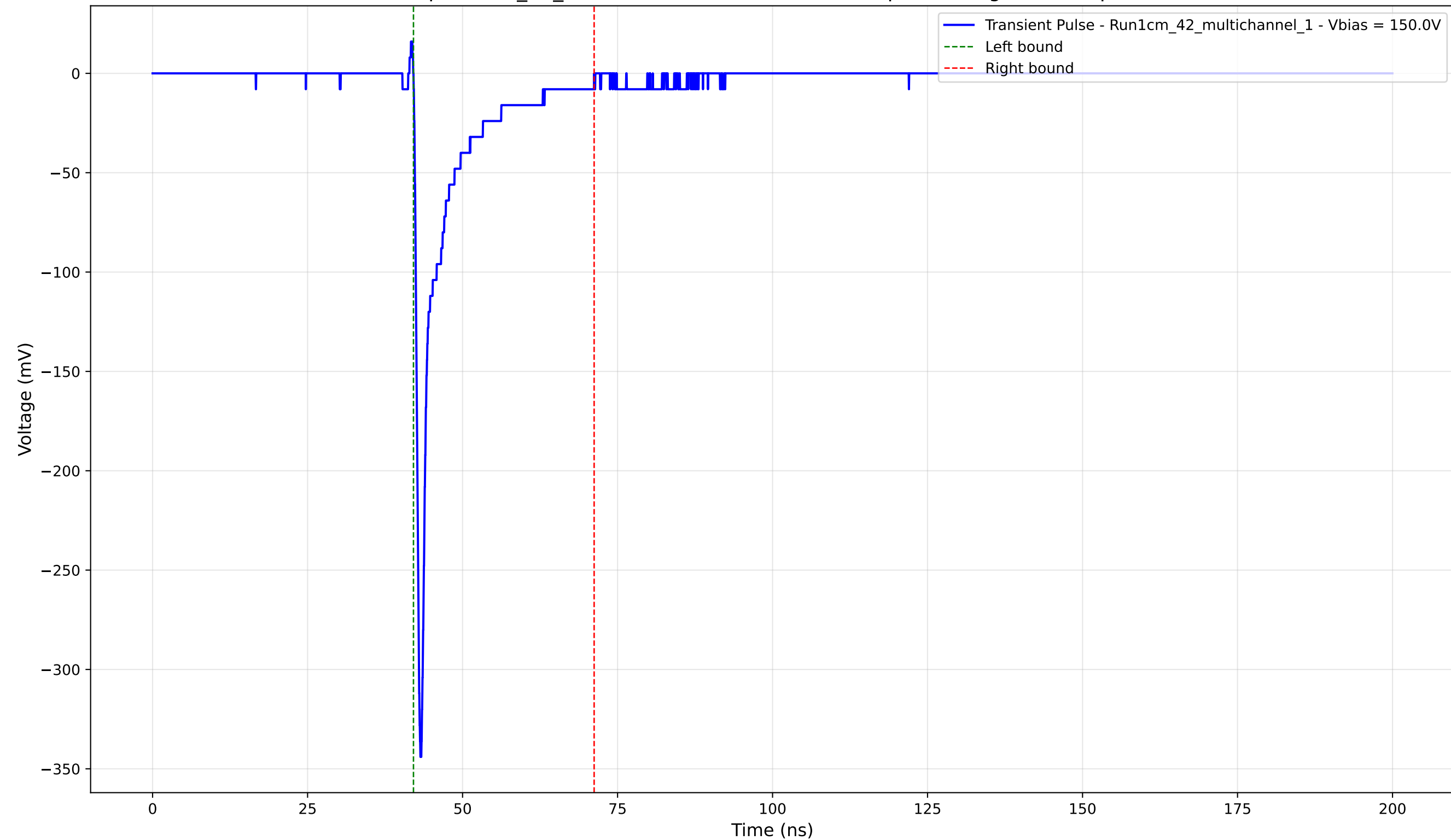
Transient Pulse - Sample: 1cm_42_multichannel - Position: 2180.0 \mu\text{m} - Charge: -25.45 pC - Rise Time: 0.75 ns
