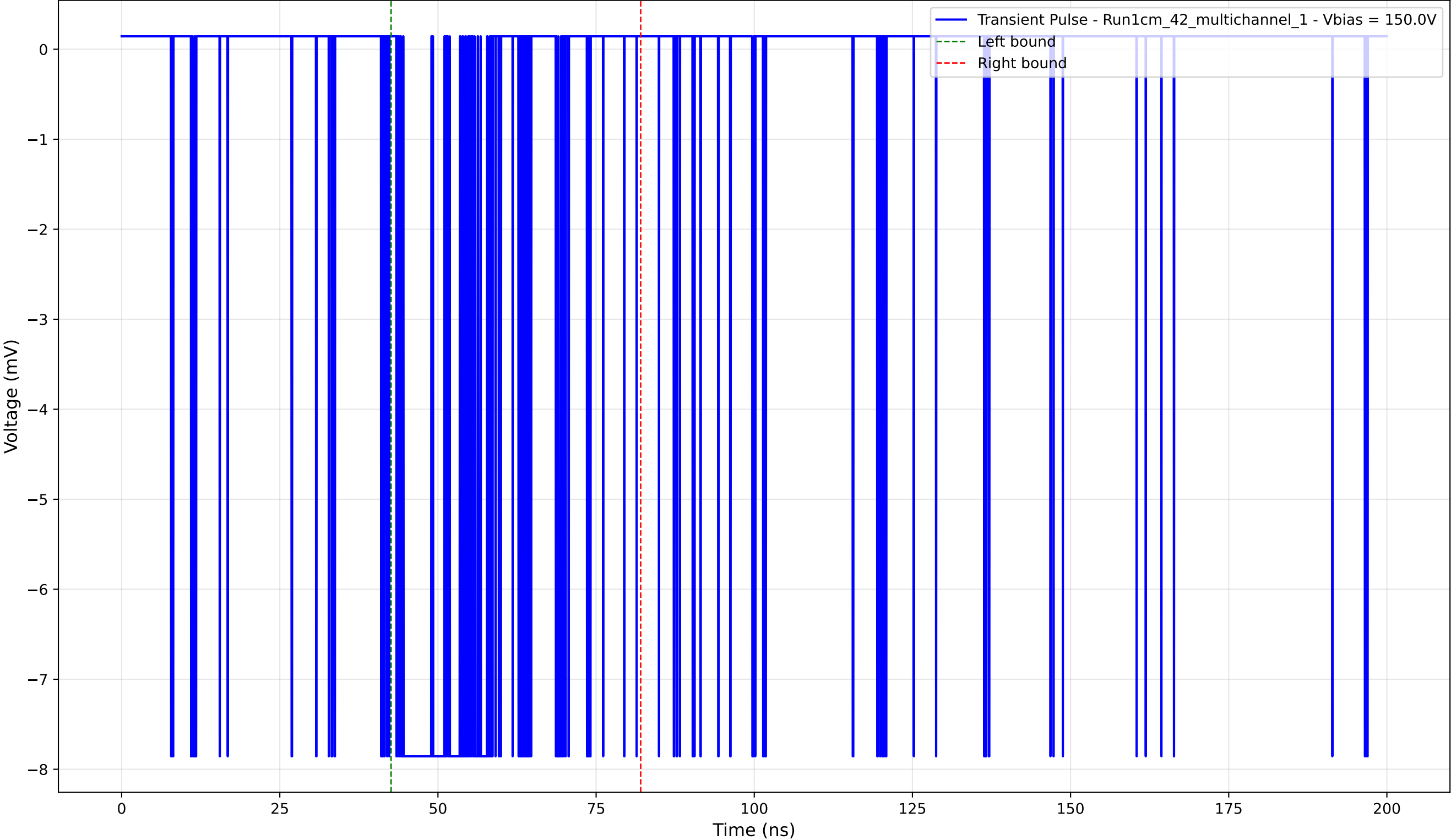
Transient Pulse - Sample: 1cm_42_multichannel - Position: 375.0 \mu\text{m} - Charge: -2.31 pC - Rise Time: 0.02 ns
