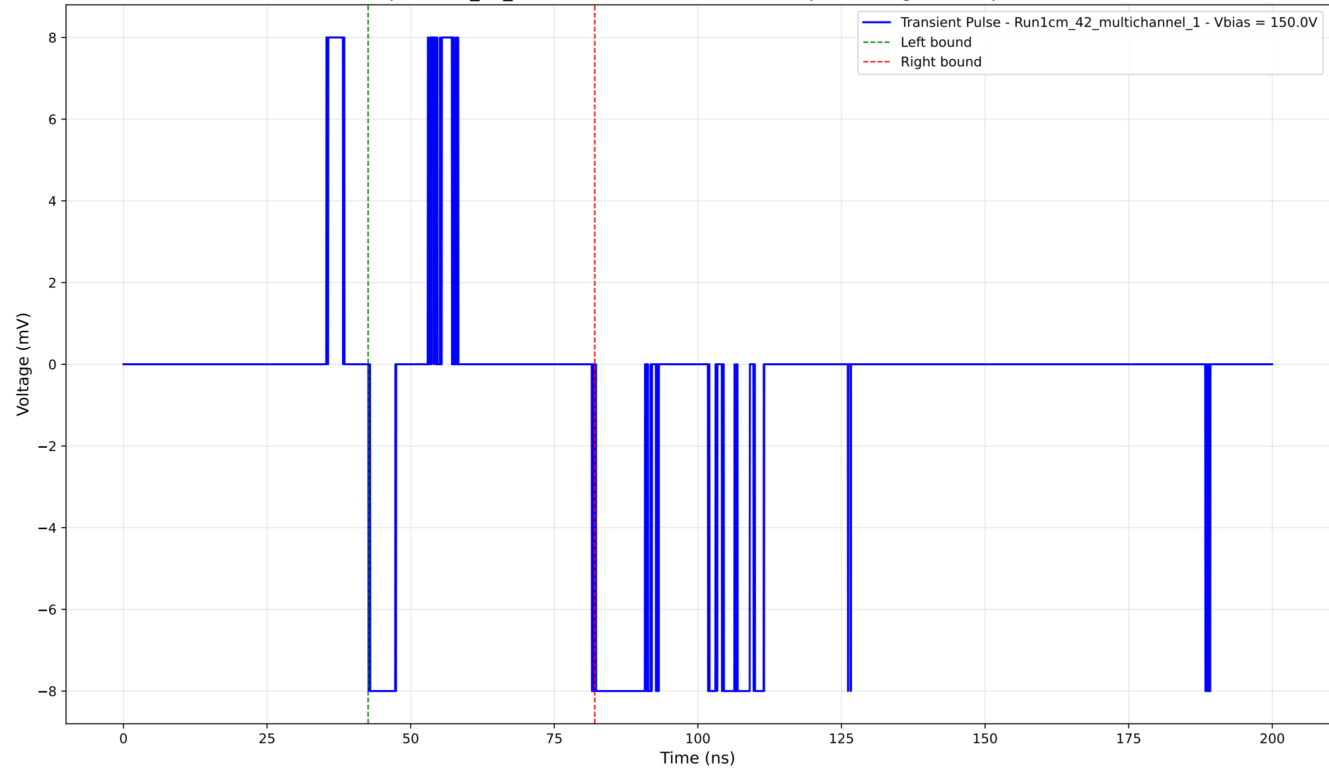
Transient Pulse - Sample: 1cm_42_multichannel - Position: 3900.0 \mu\text{m} - Charge: -0.25 pC - Rise Time: 0.02 ns
