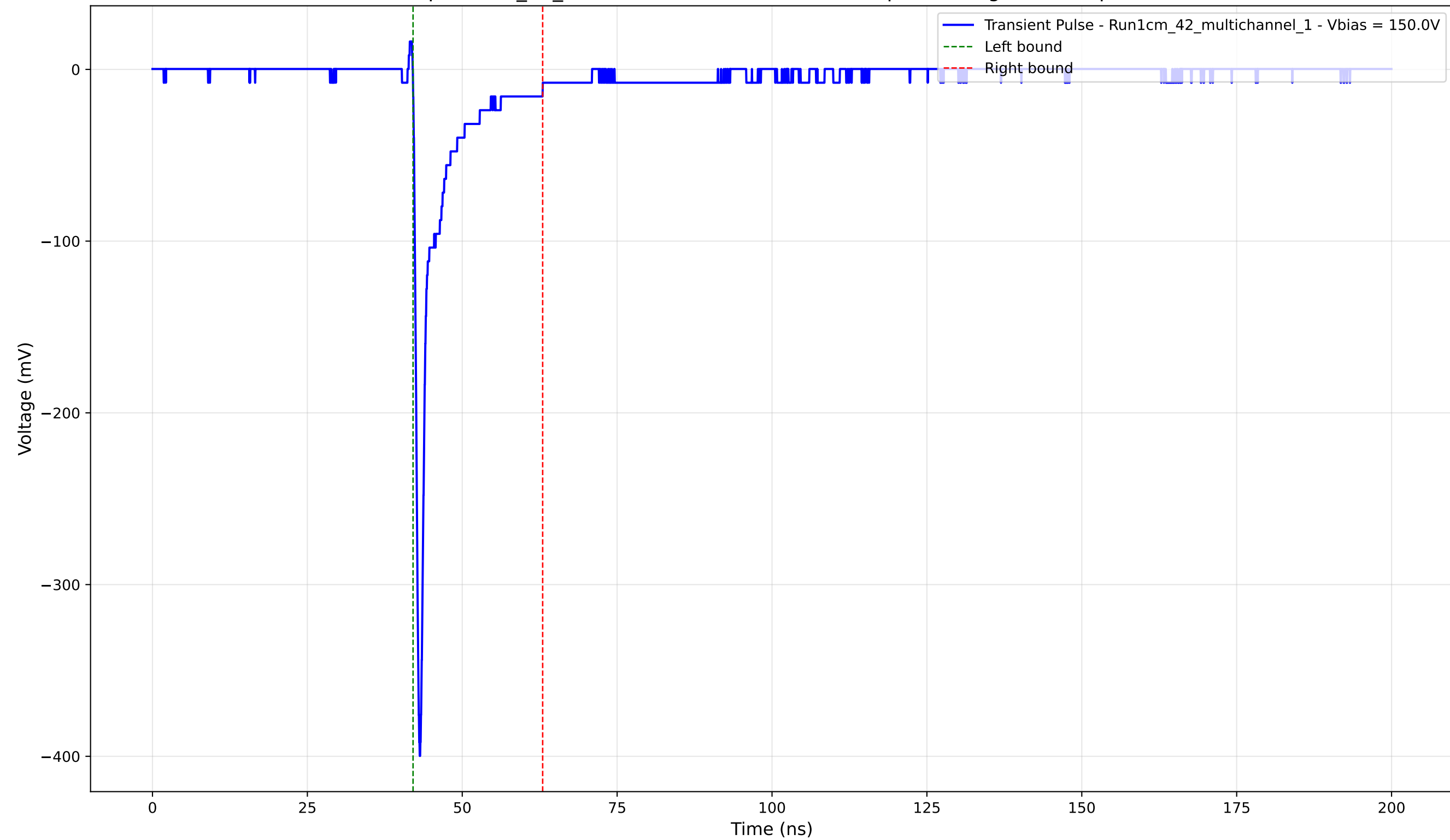
Transient Pulse - Sample: 1cm_42_multichannel - Position: 2485.0 \mu\text{m} - Charge: -24.41 pC - Rise Time: 0.74 ns
