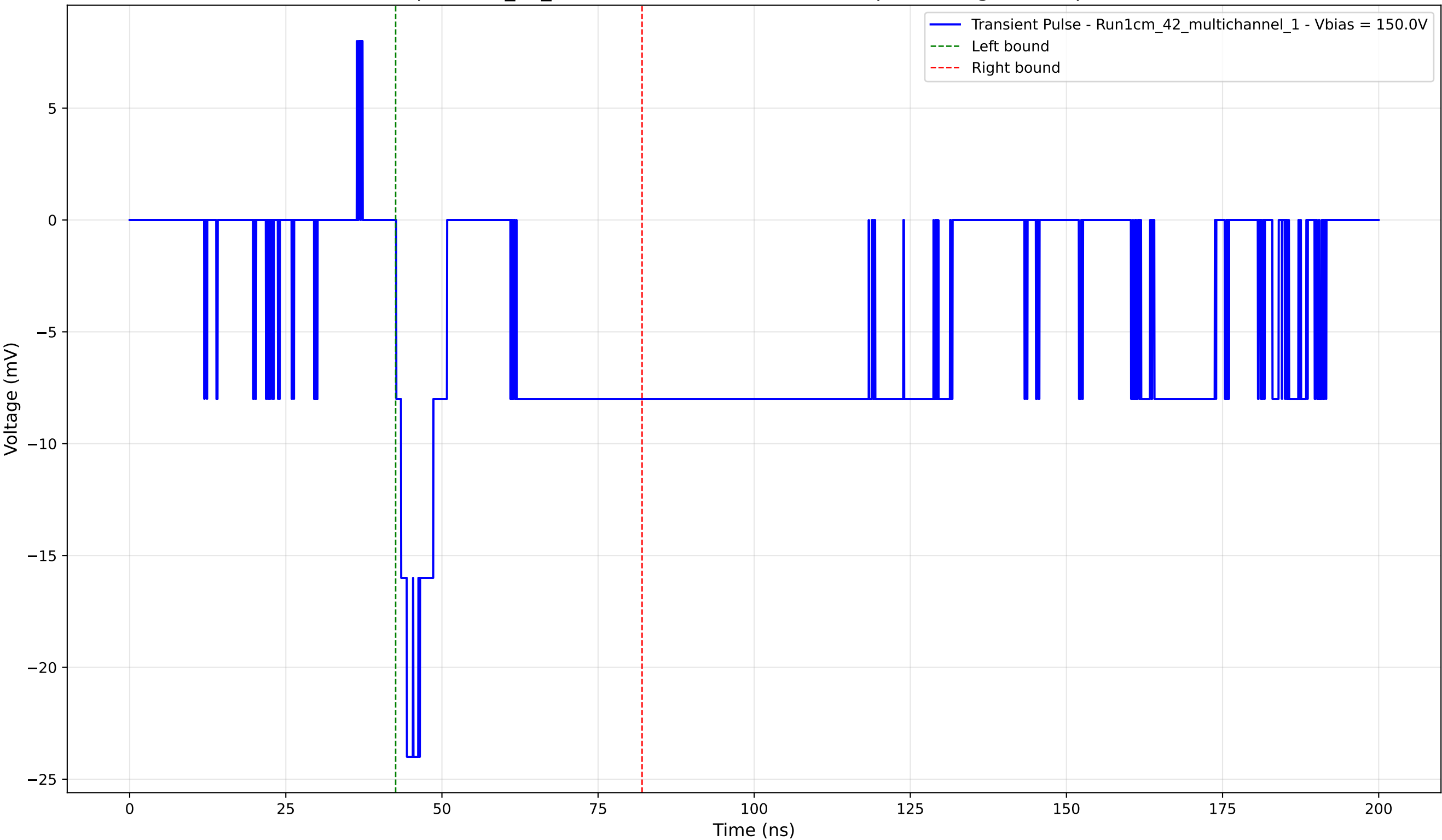
Transient Pulse - Sample: 1cm_42_multichannel - Position: 3950.0 \mu\text{m} - Charge: -5.73 pC - Rise Time: 1.71 ns
