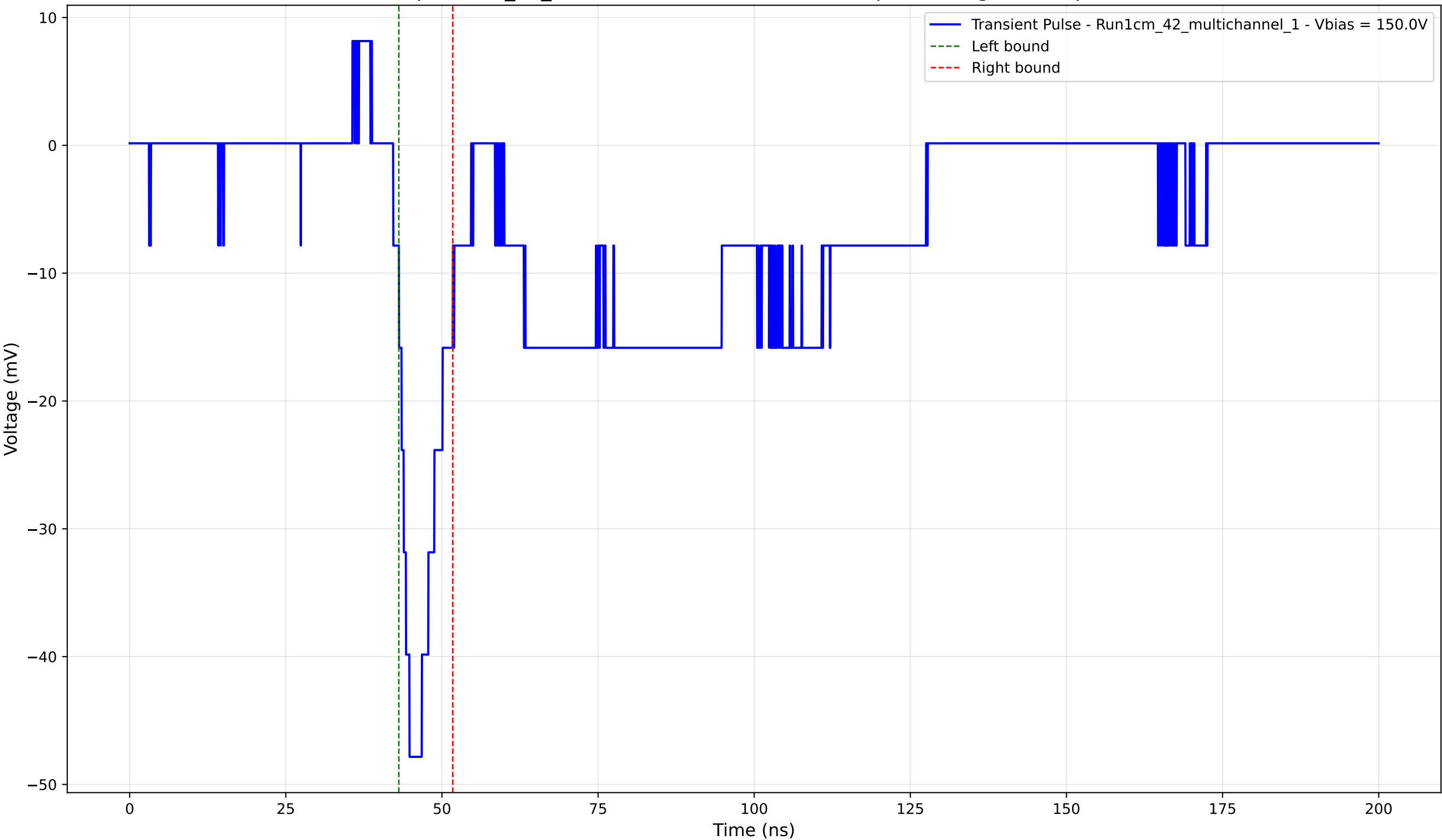
Transient Pulse - Sample: 1cm_42_multichannel - Position: 4500.0 \mu\text{m} - Charge: -5.46 pC - Rise Time: 2.61 ns
