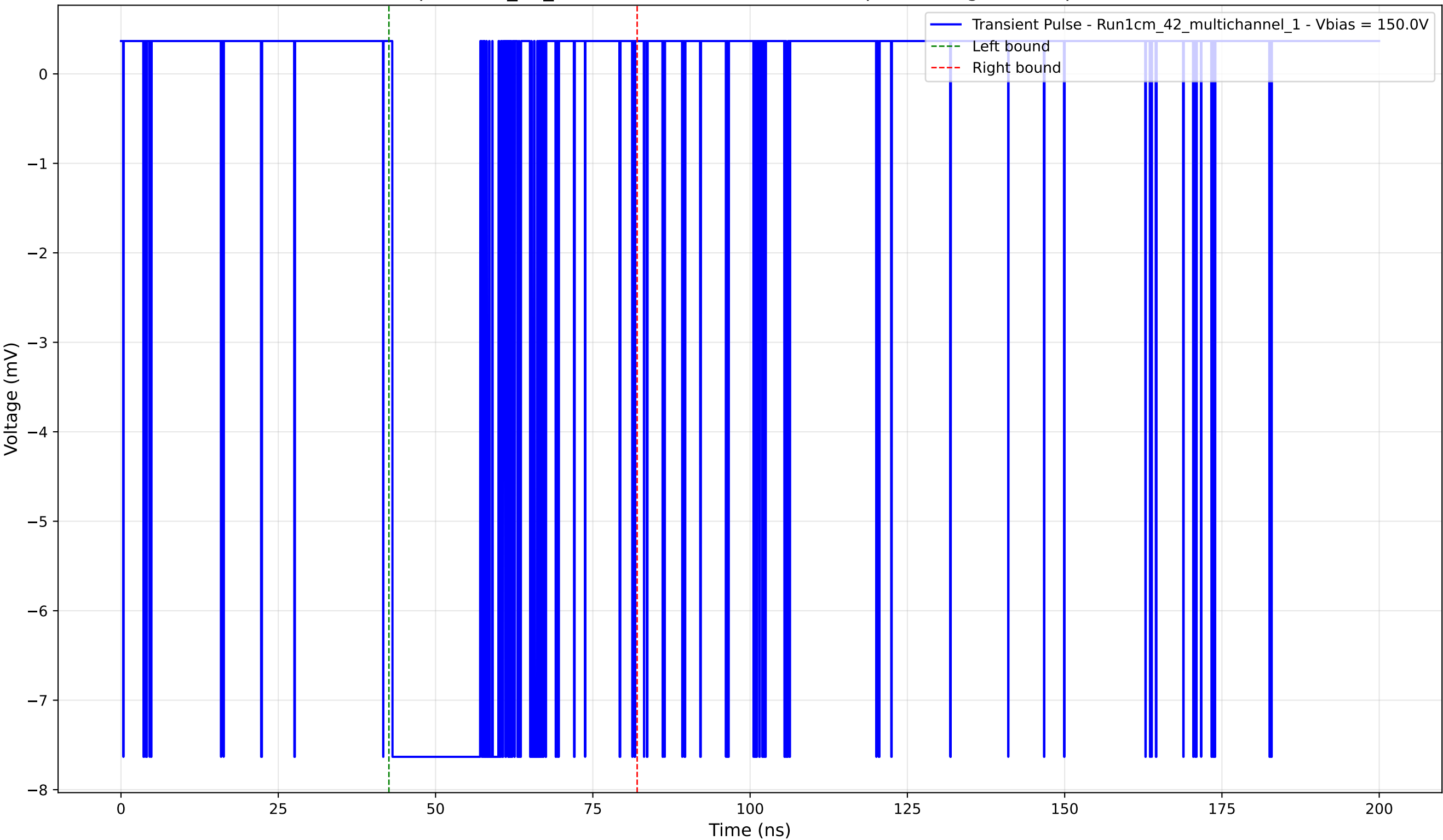
Transient Pulse - Sample: 1cm_42_multichannel - Position: 890.0 \mu\text{m} - Charge: -2.87 pC - Rise Time: 0.02 ns
