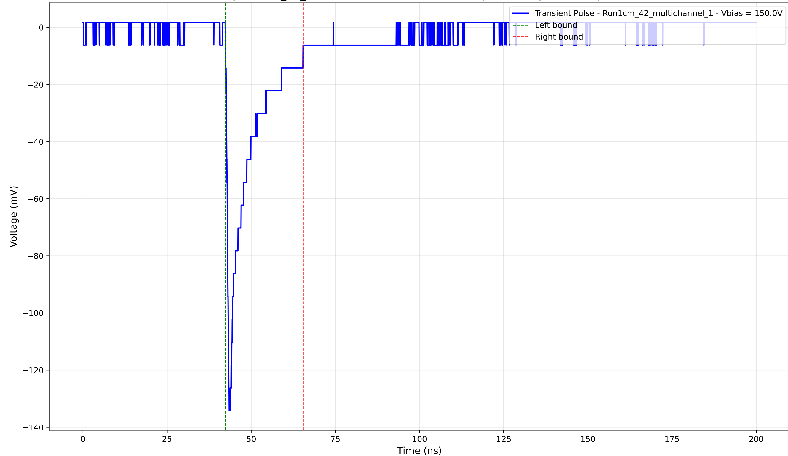
Transient Pulse - Sample: 1cm_42_multichannel - Position: 3085.0 \mu\text{m} - Charge: -17.94 pC - Rise Time: 0.90 ns
