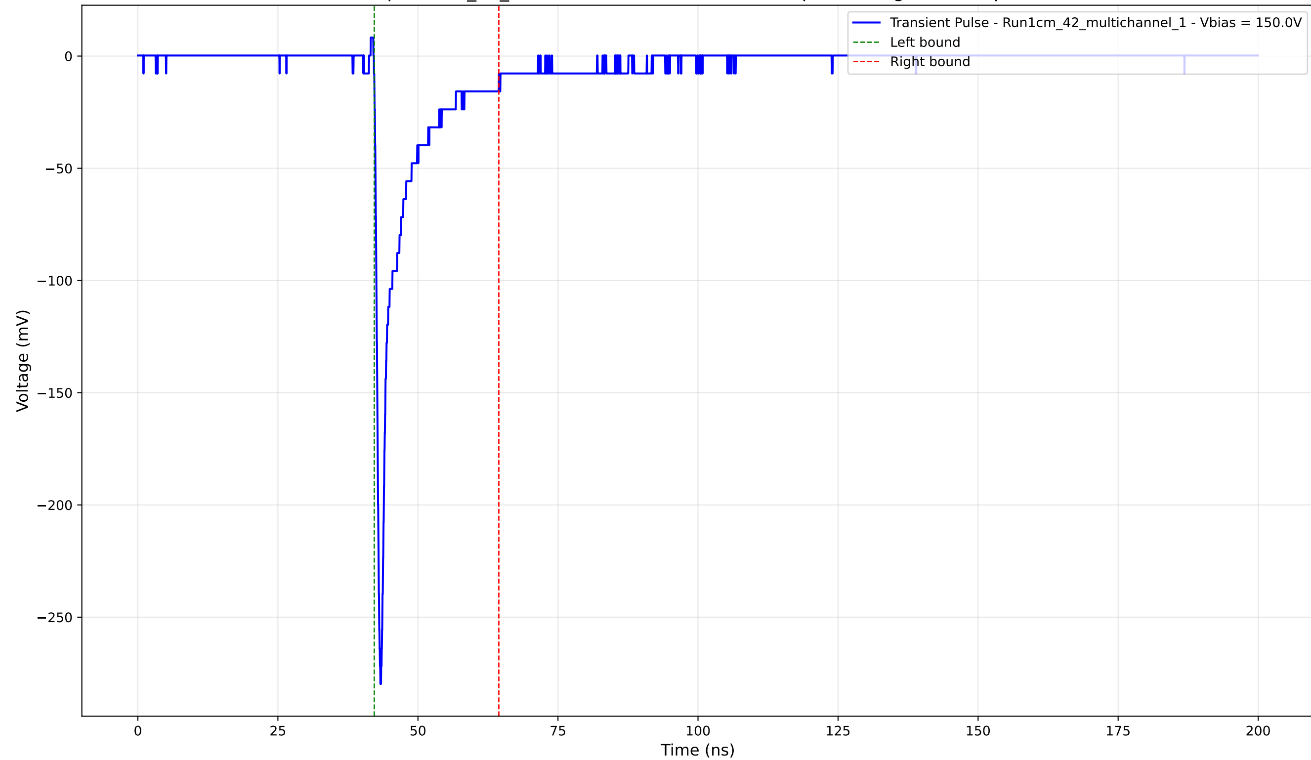
Transient Pulse - Sample: 1cm_42_multichannel - Position: 2710.0 \mu\text{m} - Charge: -23.02 pC - Rise Time: 0.79 ns
