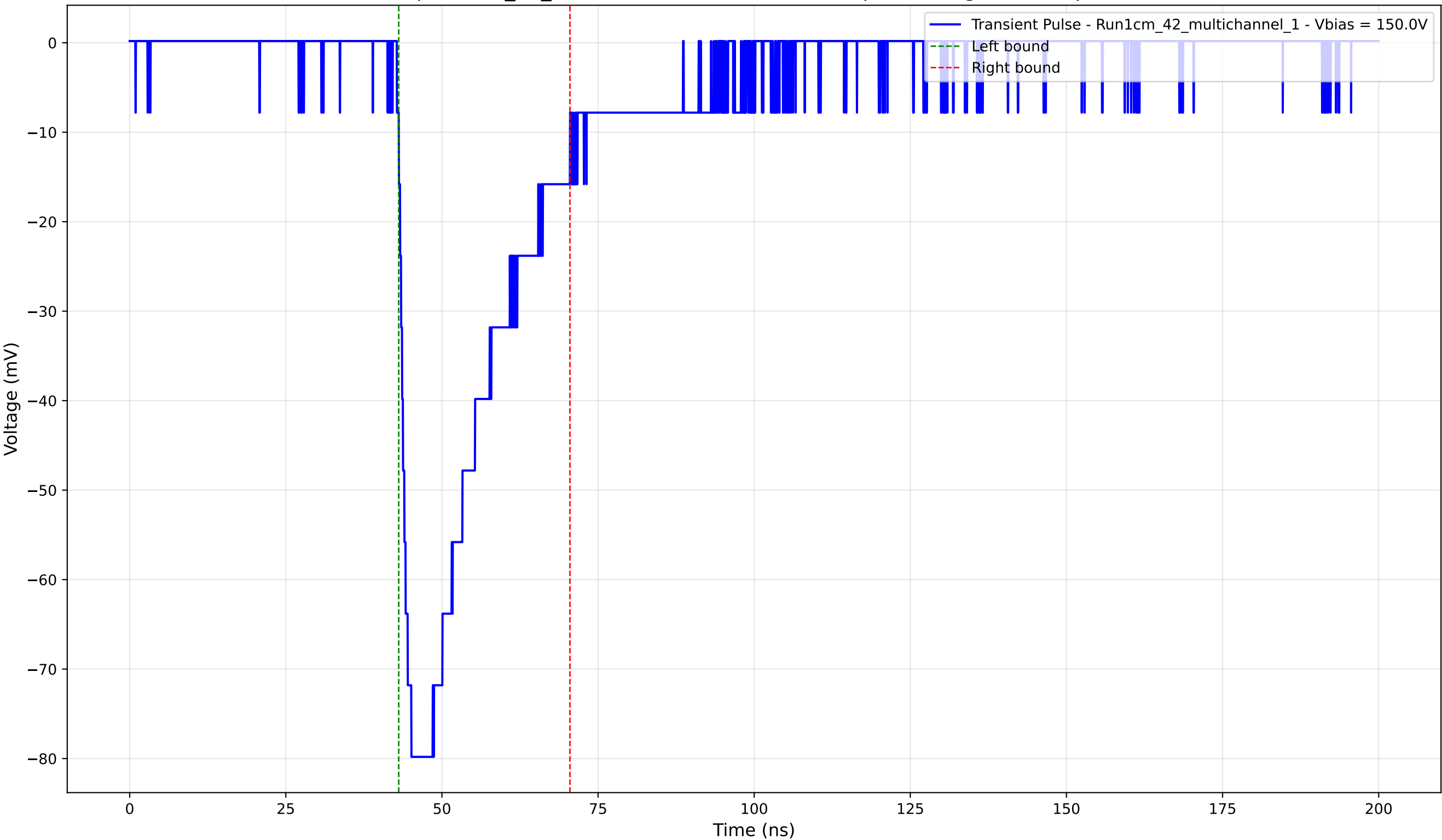
Transient Pulse - Sample: 1cm_42_multichannel - Position: 690.0 \mu\text{m} - Charge: -23.43 pC - Rise Time: 2.02 ns
