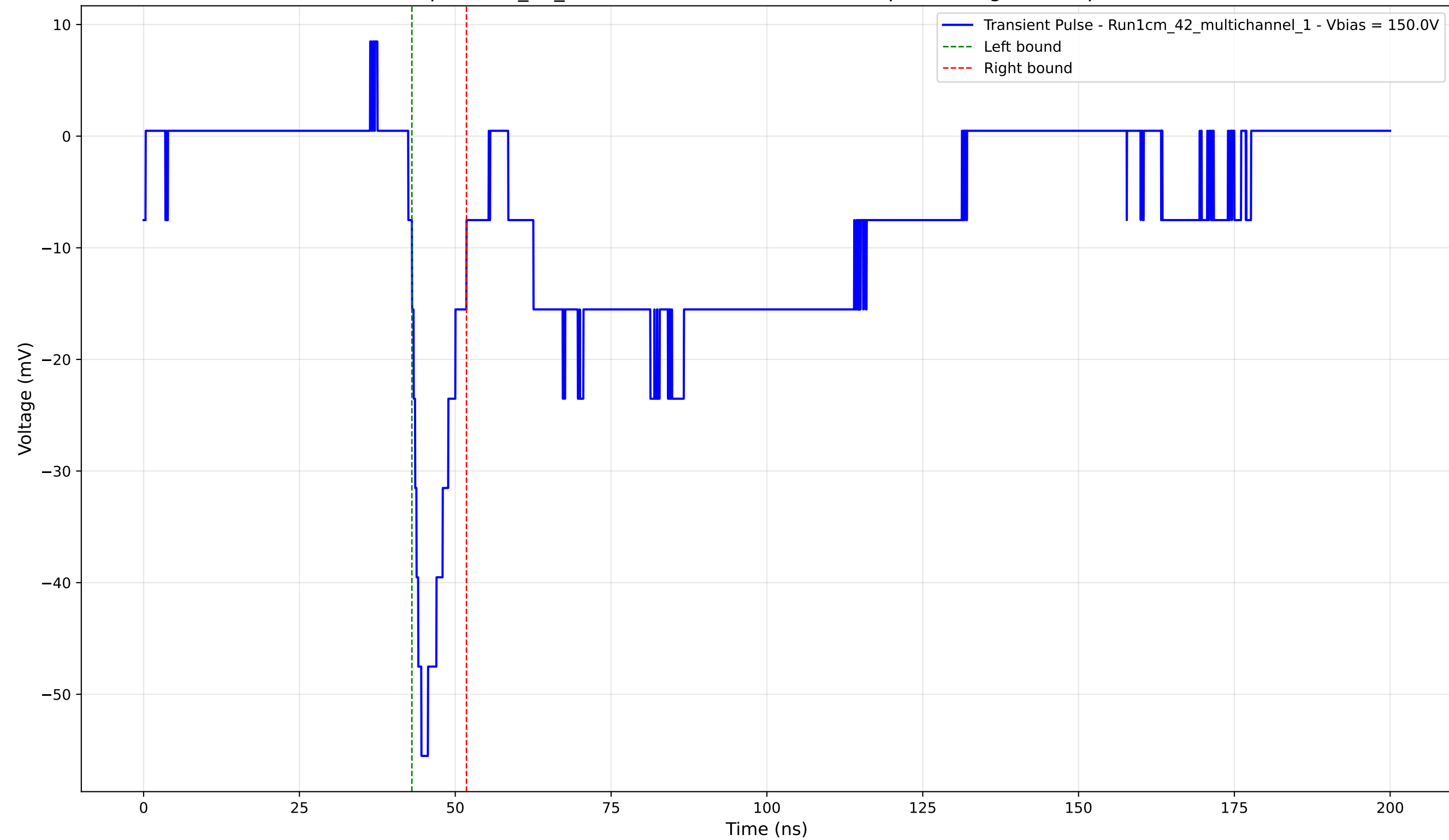
Transient Pulse - Sample: 1cm_42_multichannel - Position: 4010.0 \mu\text{m} - Charge: -5.95 pC - Rise Time: 2.11 ns
