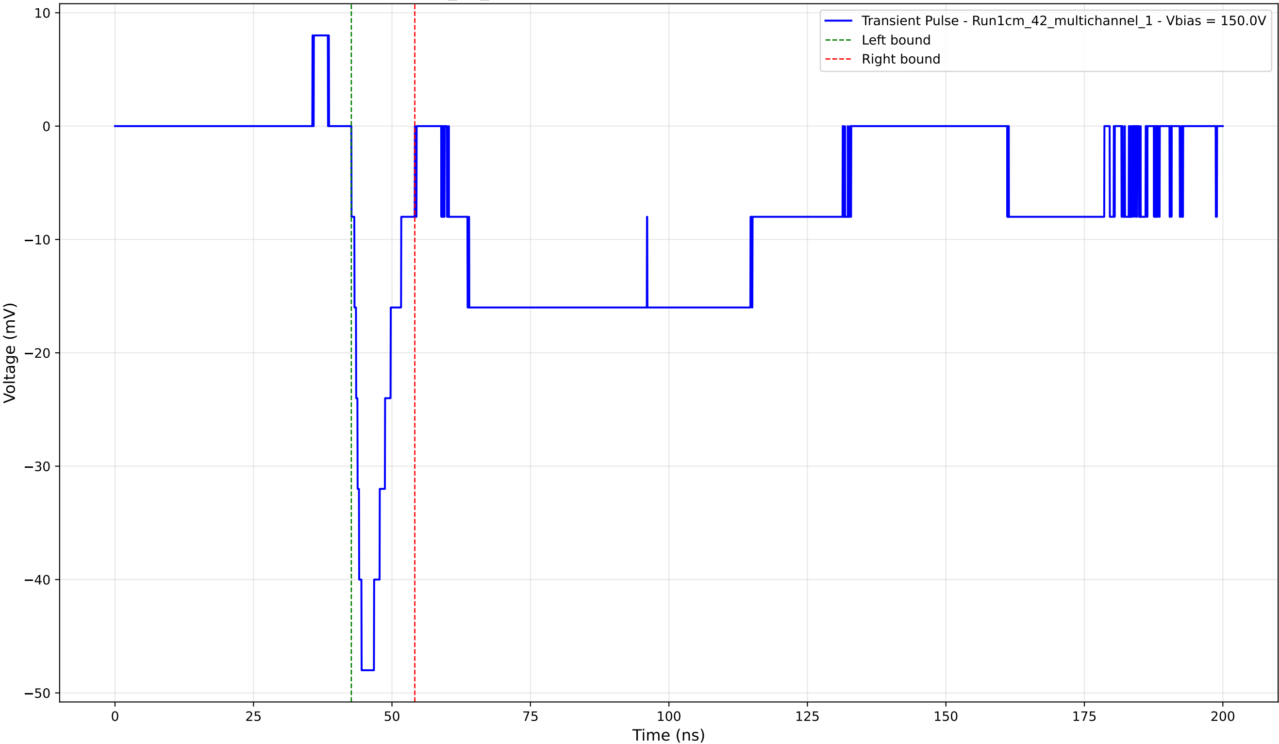
Transient Pulse - Sample: 1cm_42_multichannel - Position: 4215.0 \mu\text{m} - Charge: -5.93 pC - Rise Time: 1.83 ns
