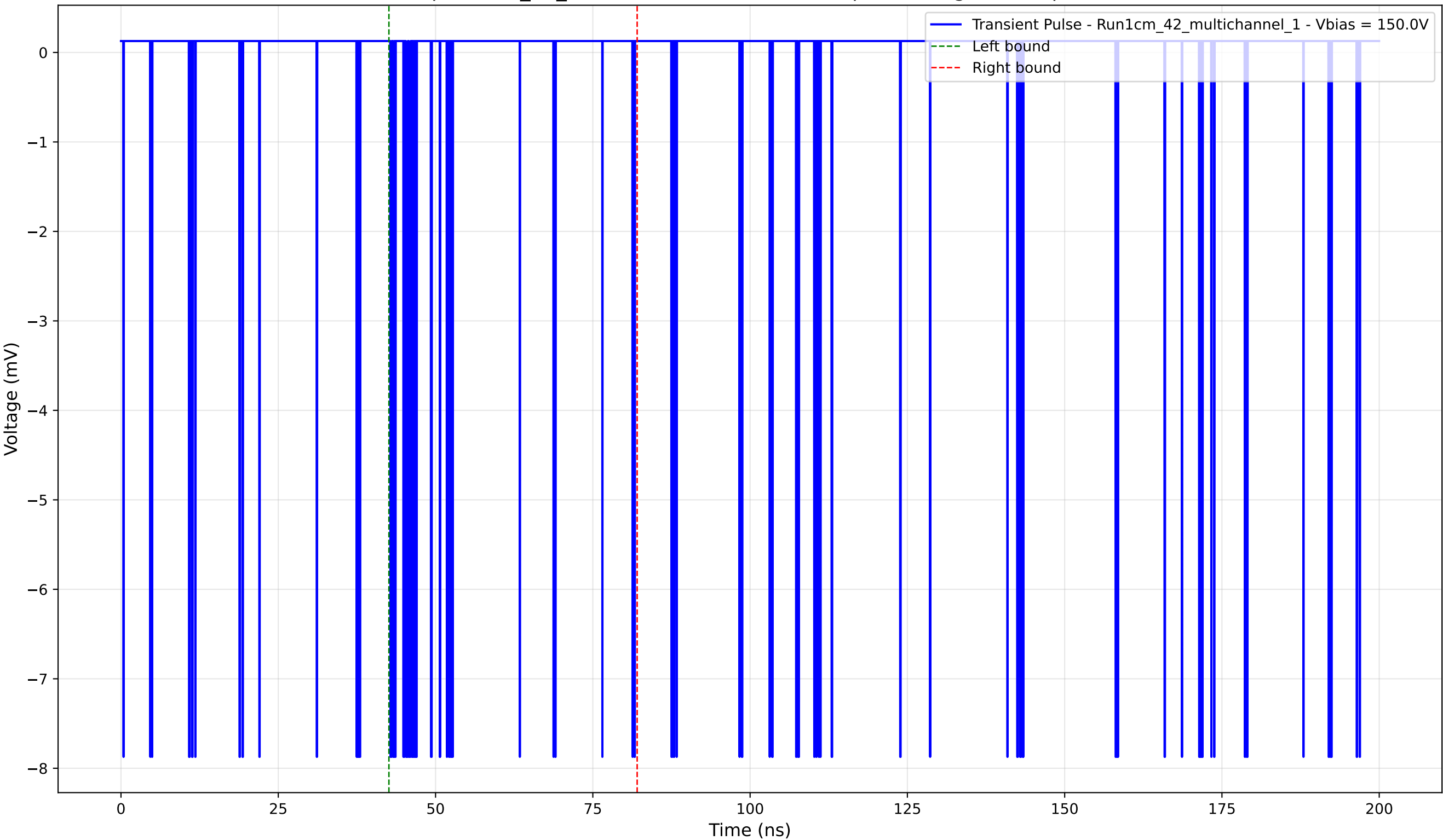
Transient Pulse - Sample: 1cm_42_multichannel - Position: 0.0 \mu\text{m} - Charge: -0.28 pC - Rise Time: 0.02 ns
