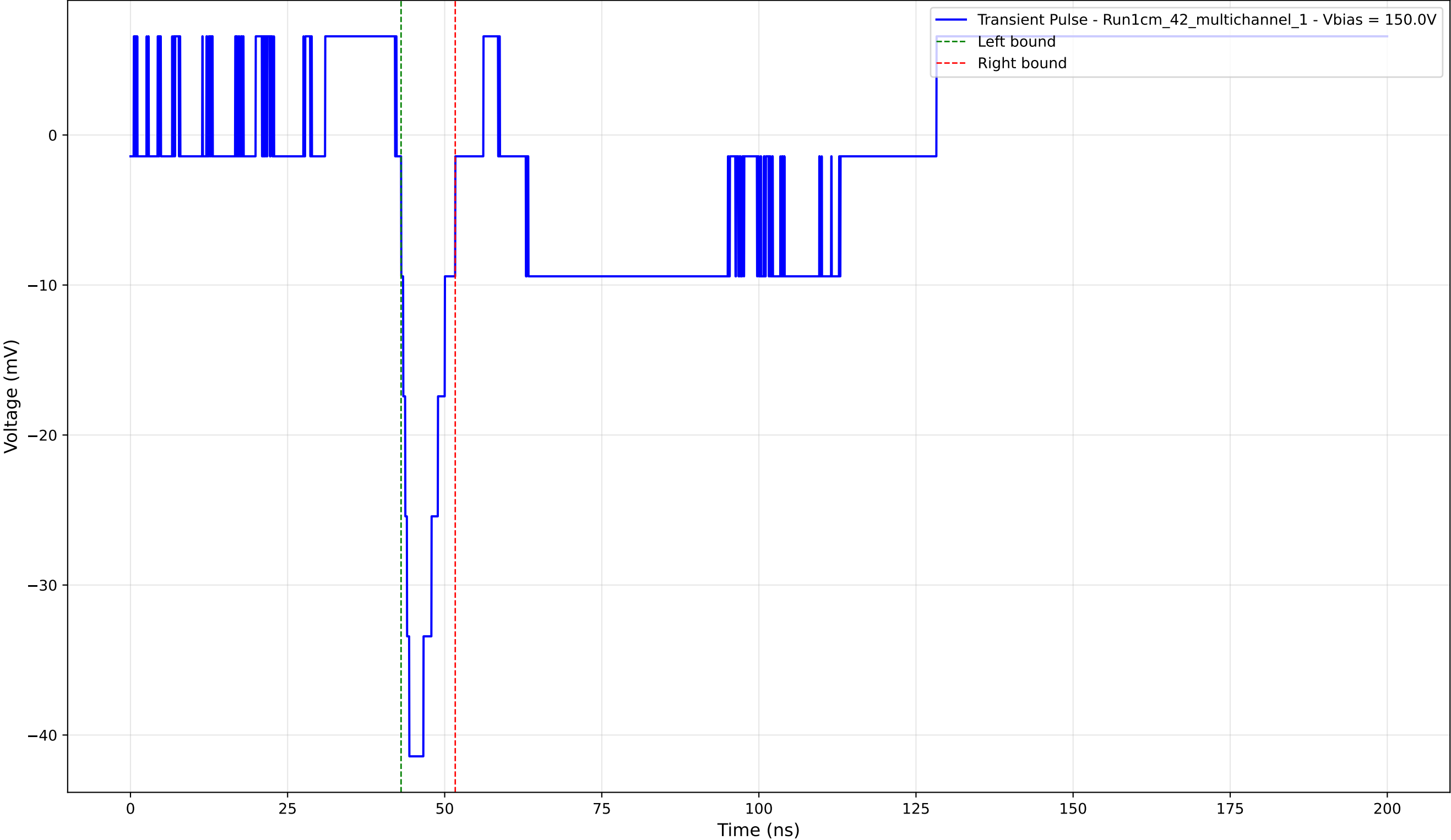
Transient Pulse - Sample: 1cm_42_multichannel - Position: 4165.0 \mu\text{m} - Charge: -4.50 pC - Rise Time: 1.29 ns
