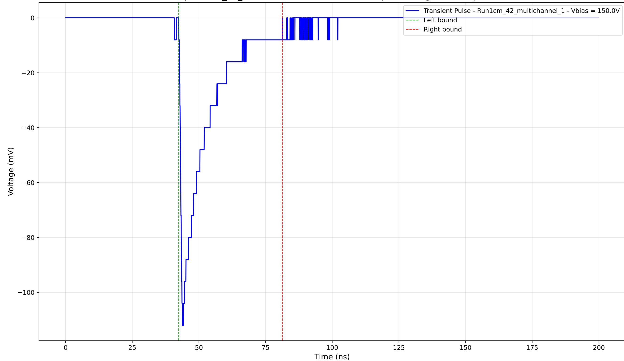
Transient Pulse - Sample: 1cm_42_multichannel - Position: 1450.0 \mu\text{m} - Charge: -22.76 pC - Rise Time: 0.99 ns
