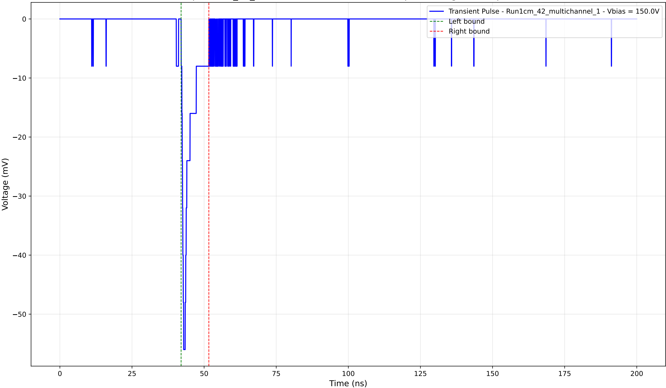
Transient Pulse - Sample: 1cm_42_multichannel - Position: 2355.0 \mu\text{m} - Charge: -3.42 pC - Rise Time: 0.87 ns
