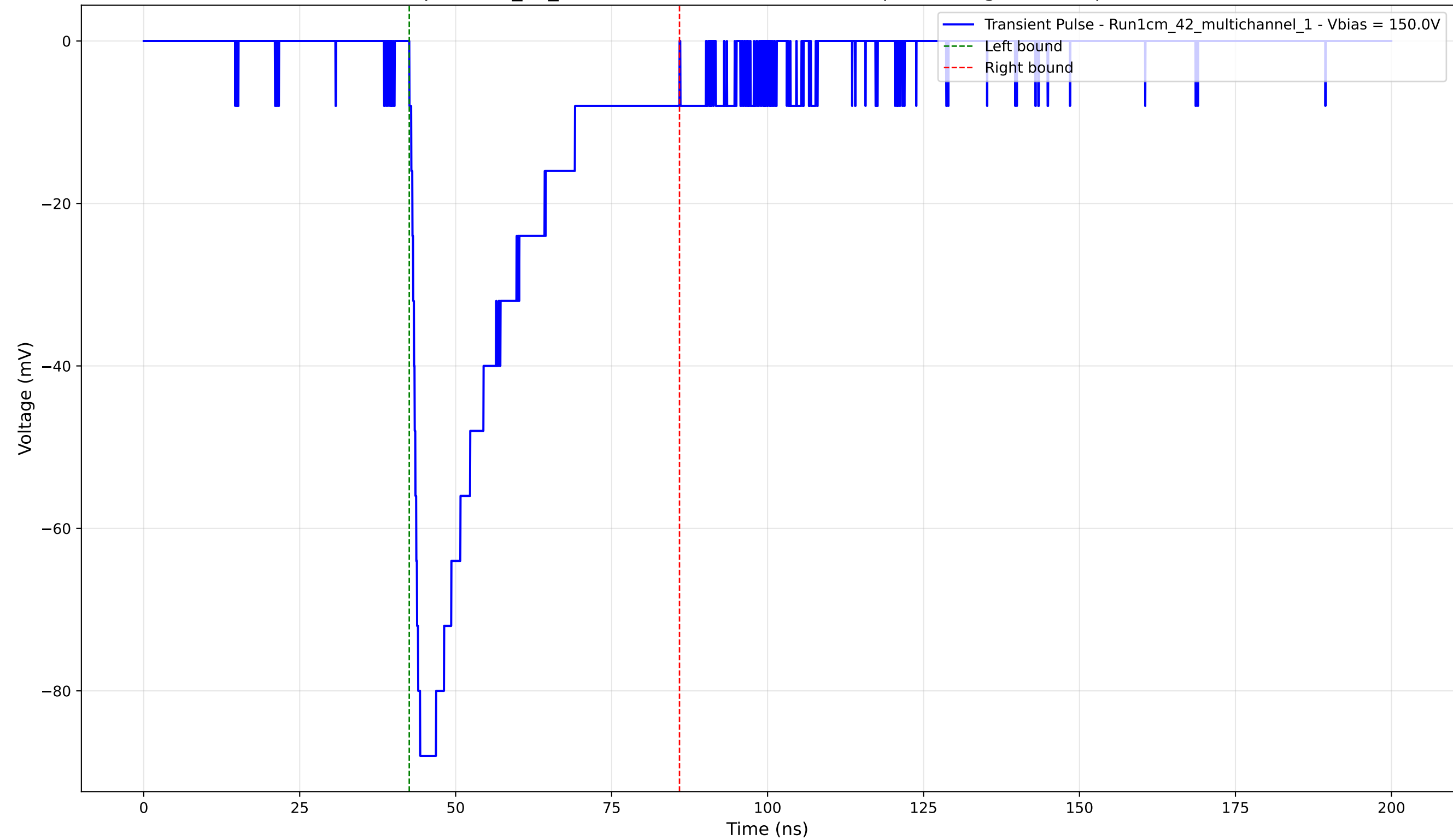
Transient Pulse - Sample: 1cm_42_multichannel - Position: 1075.0 \mu\text{m} - Charge: -25.64 pC - Rise Time: 1.12 ns
