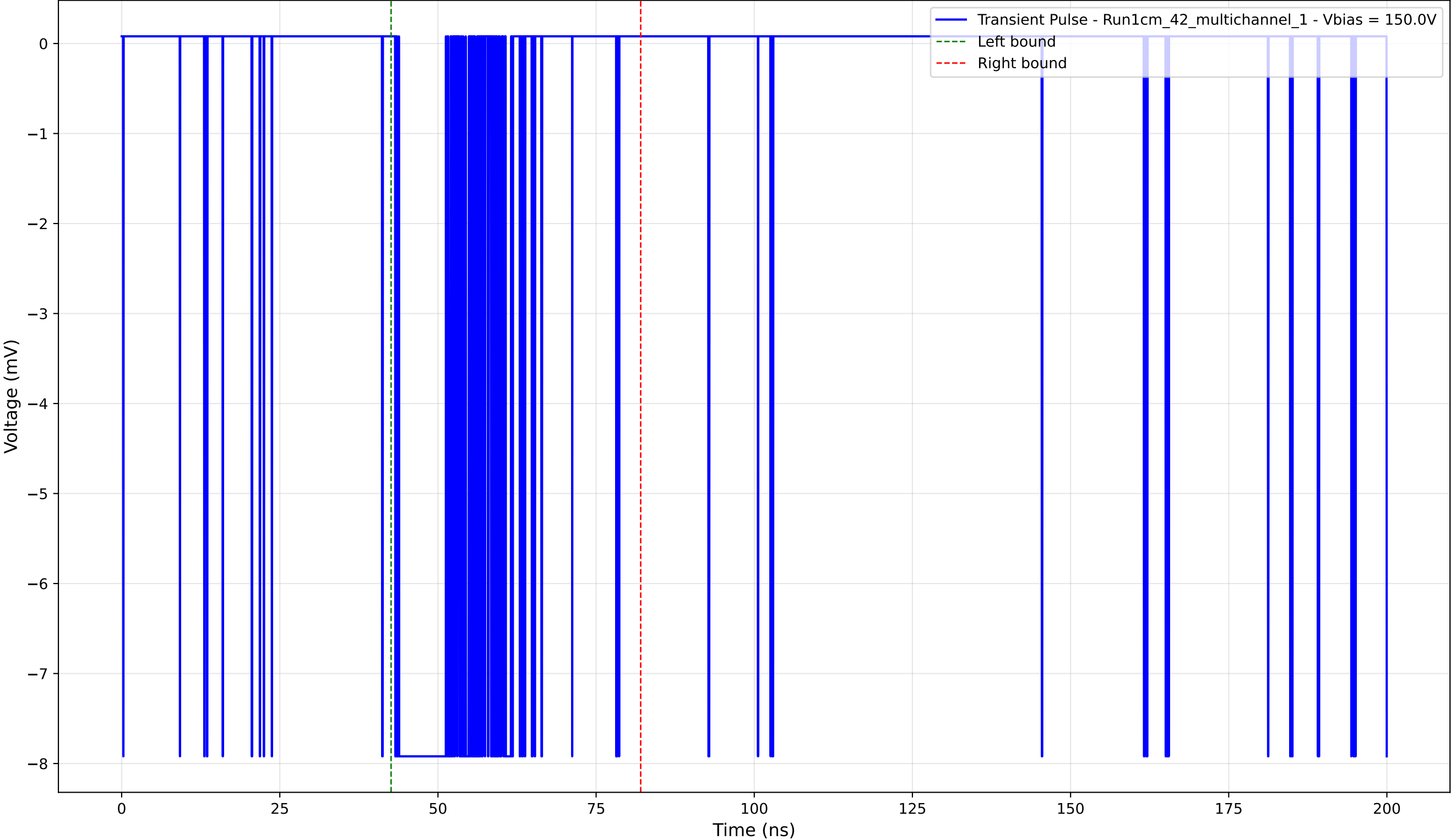
Transient Pulse - Sample: 1cm_42_multichannel - Position: 855.0 \mu\text{m} - Charge: -2.24 pC - Rise Time: 0.02 ns
