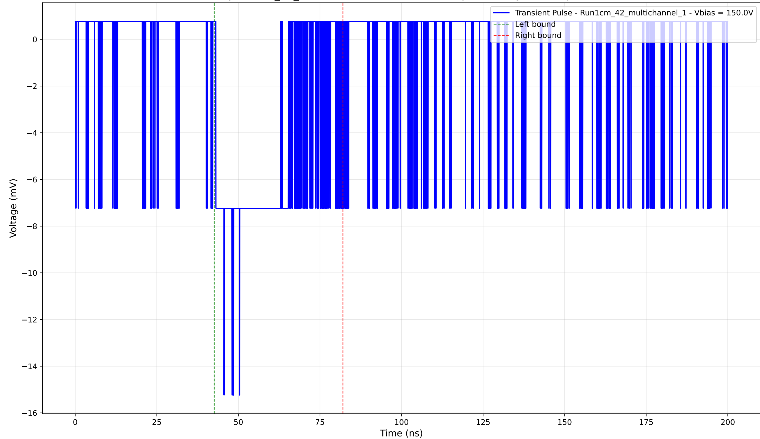
Transient Pulse - Sample: 1cm_42_multichannel - Position: 390.0 \mu\text{m} - Charge: -3.68 pC - Rise Time: 2.52 ns
