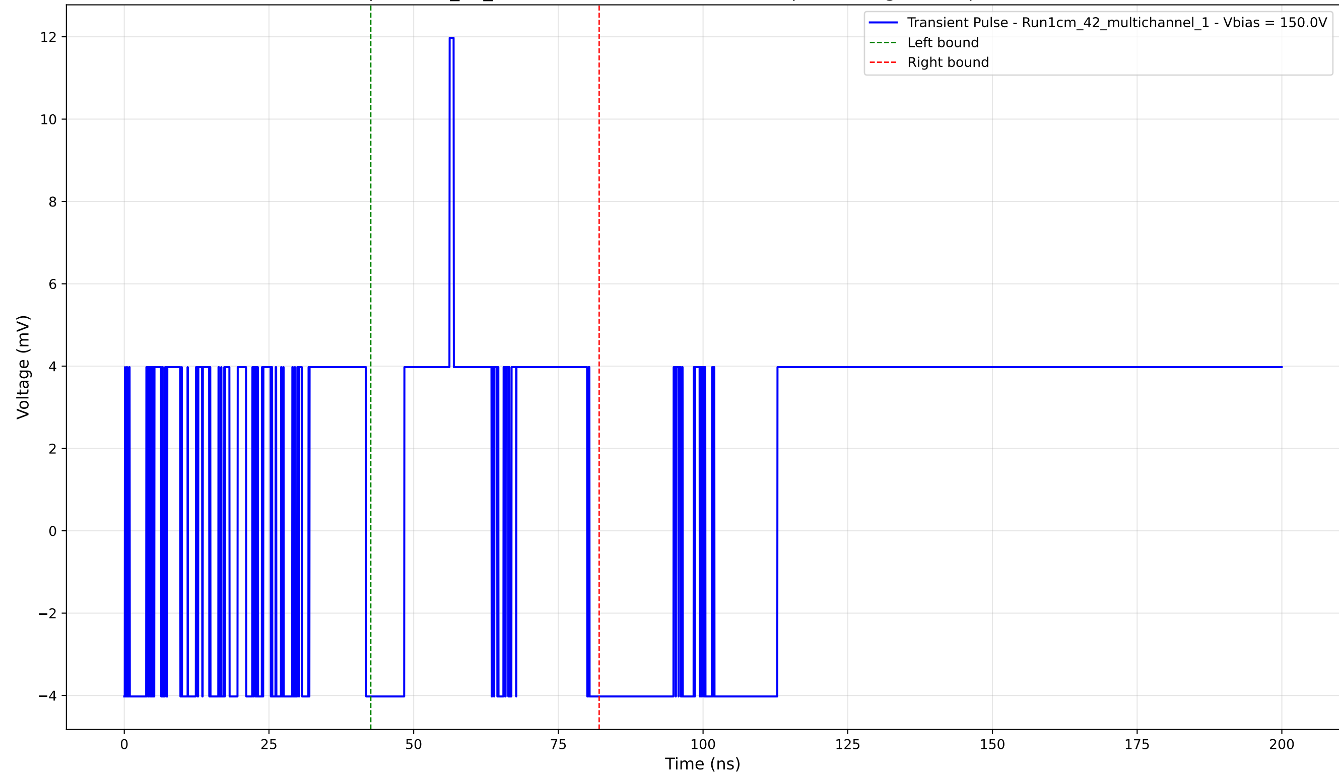
Transient Pulse - Sample: 1cm_42_multichannel - Position: 4405.0 \mu\text{m} - Charge: 1.74 pC - Rise Time: 0.00 ns (N/A)
