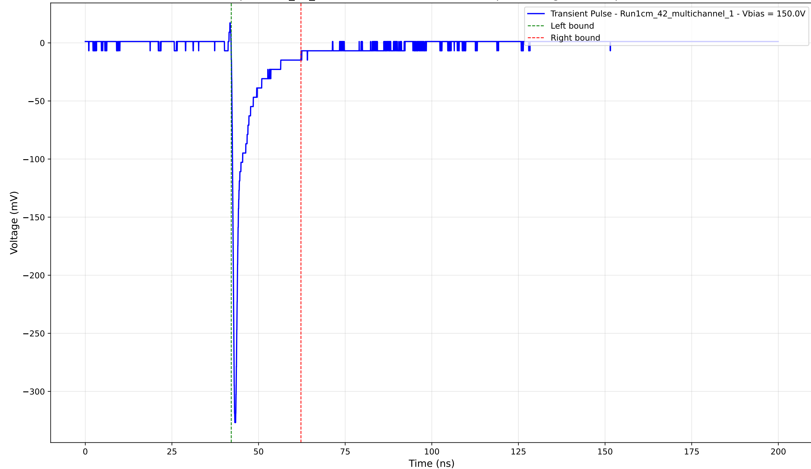
Transient Pulse - Sample: 1cm_42_multichannel - Position: 2600.0 \mu\text{m} - Charge: -22.75 pC - Rise Time: 0.72 ns
