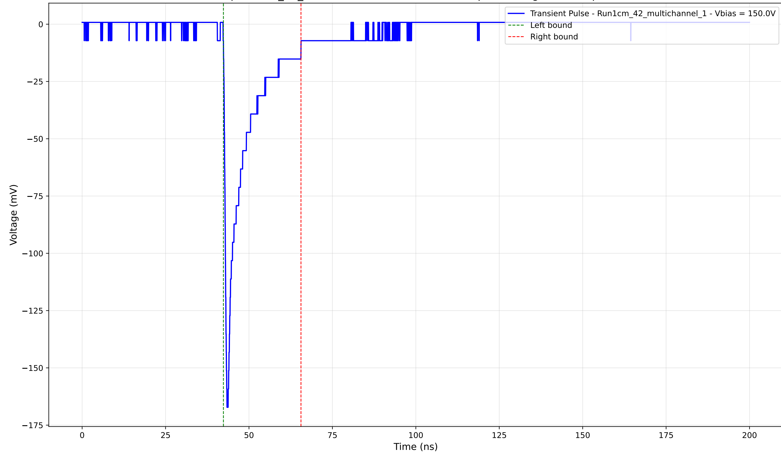
Transient Pulse - Sample: 1cm_42_multichannel - Position: 1800.0 \mu\text{m} - Charge: -20.45 pC - Rise Time: 0.82 ns
