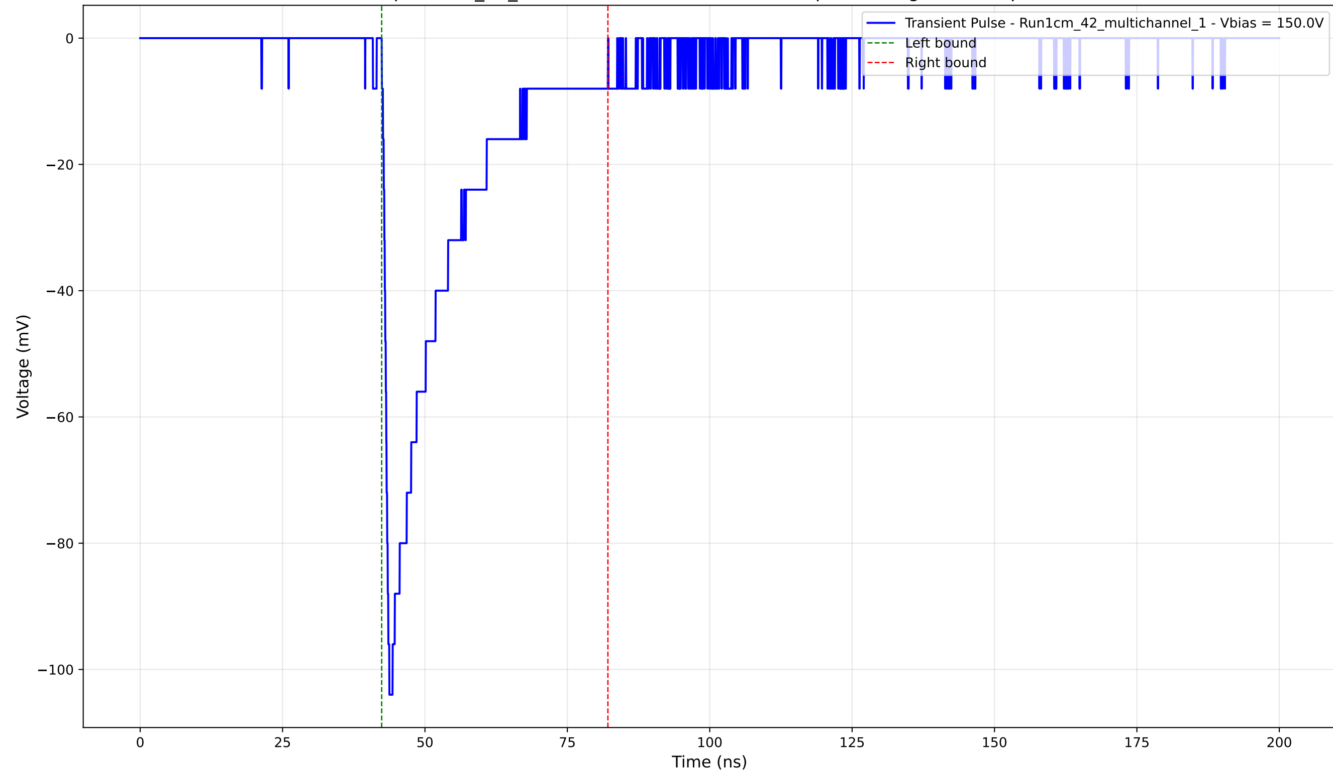
Transient Pulse - Sample: 1cm_42_multichannel - Position: 1445.0 \mu\text{m} - Charge: -22.48 pC - Rise Time: 0.95 ns
