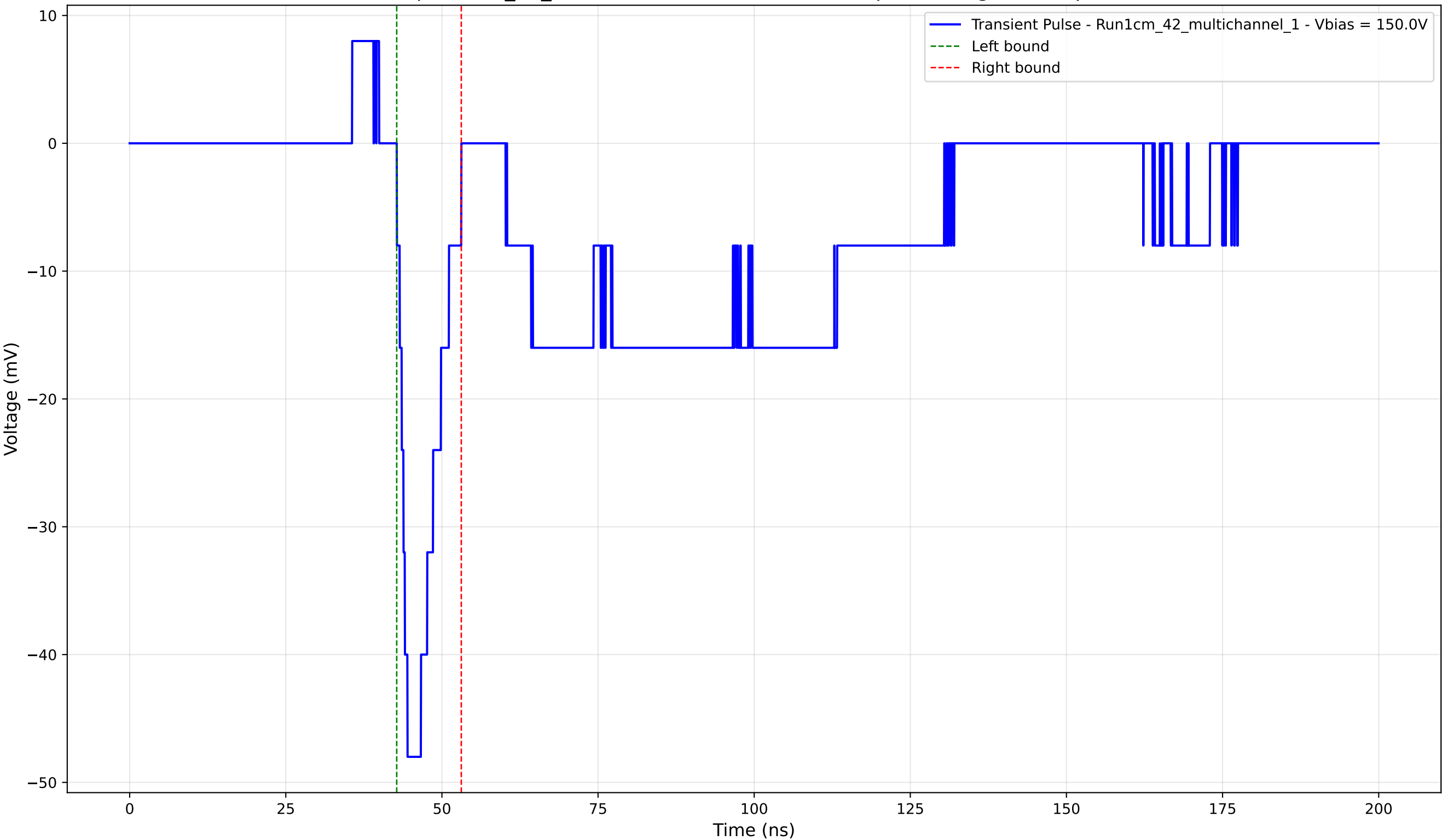
Transient Pulse - Sample: 1cm_42_multichannel - Position: 4210.0 \mu\text{m} - Charge: -5.59 pC - Rise Time: 1.71 ns
