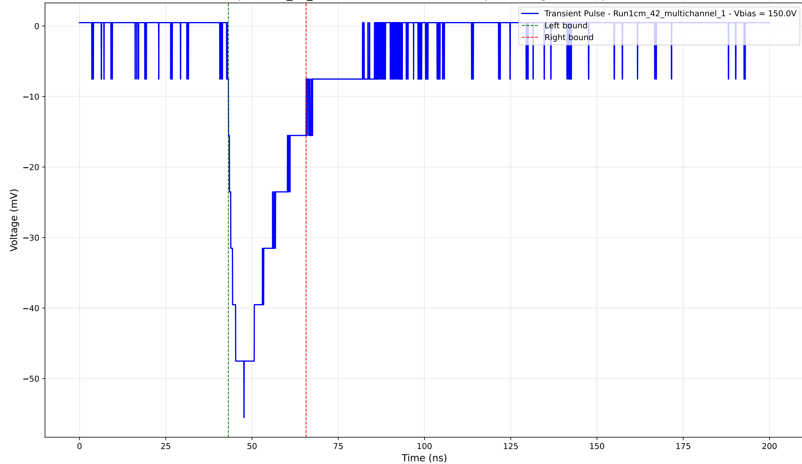
Transient Pulse - Sample: 1cm_42_multichannel - Position: 300.0 \mu\text{m} - Charge: -14.04 pC - Rise Time: 4.81 ns
