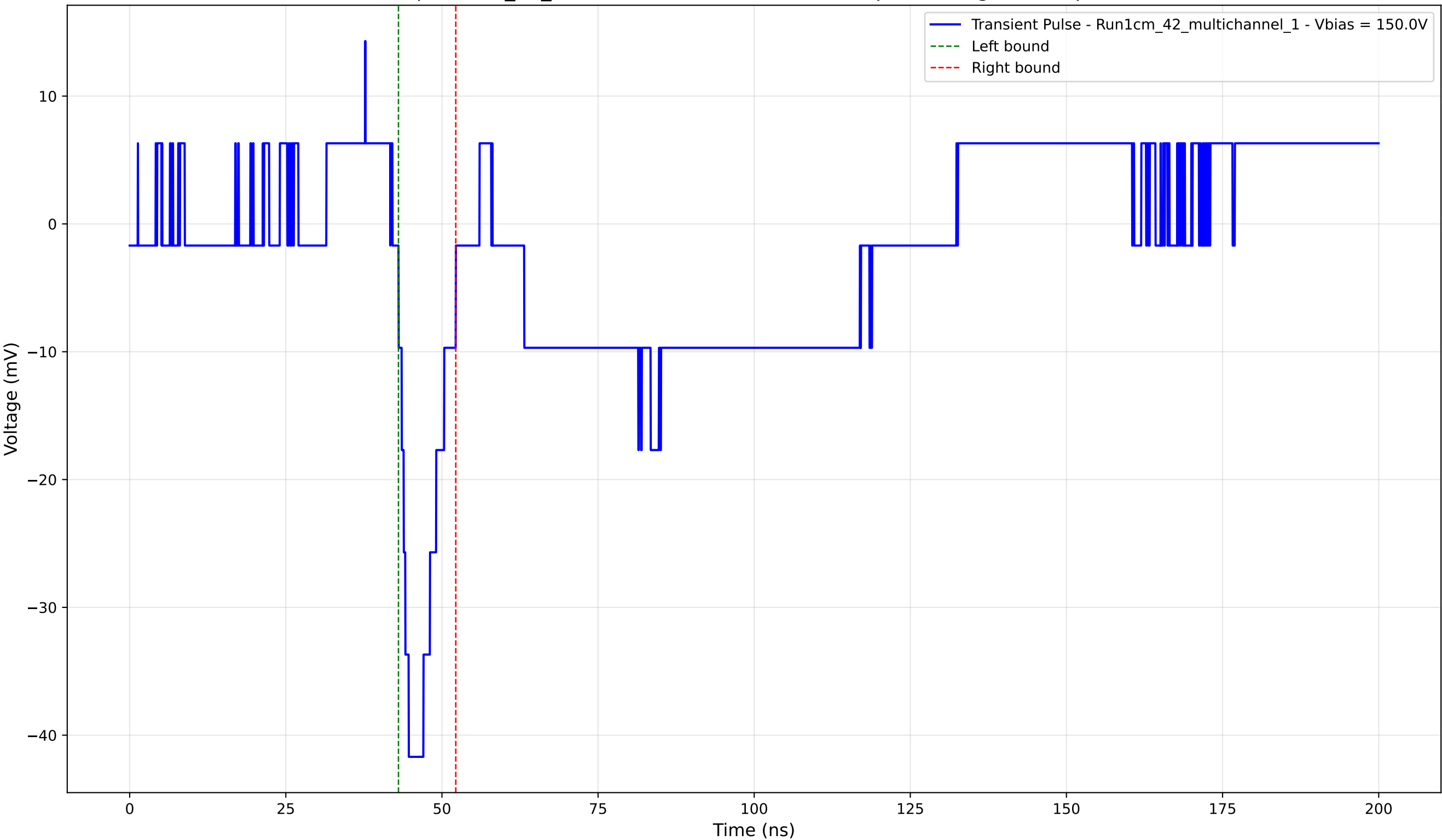
Transient Pulse - Sample: 1cm_42_multichannel - Position: 4535.0 \mu\text{m} - Charge: -4.70 pC - Rise Time: 1.63 ns
