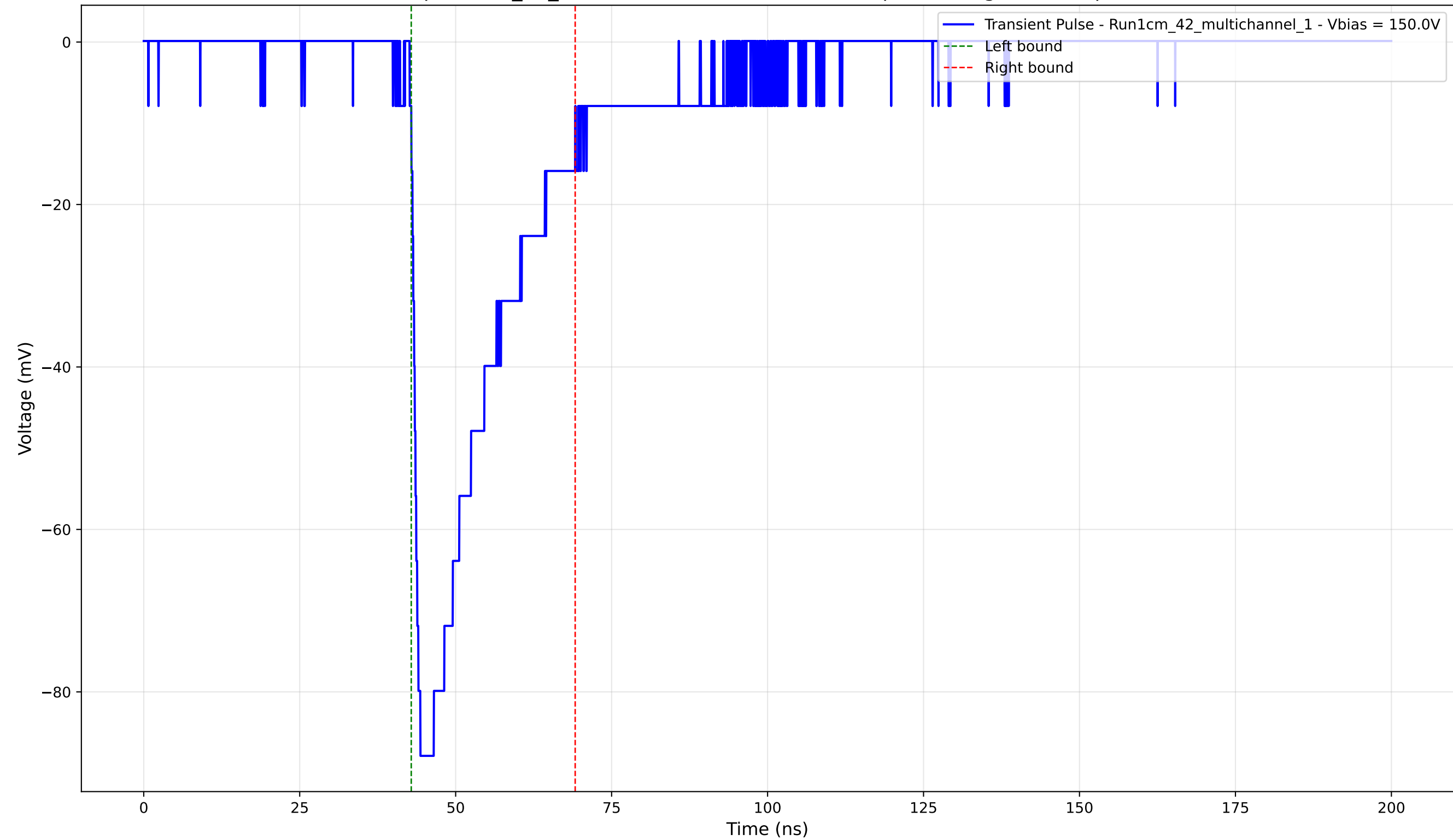
Transient Pulse - Sample: 1cm_42_multichannel - Position: 1055.0 \mu\text{m} - Charge: -22.93 pC - Rise Time: 1.14 ns
