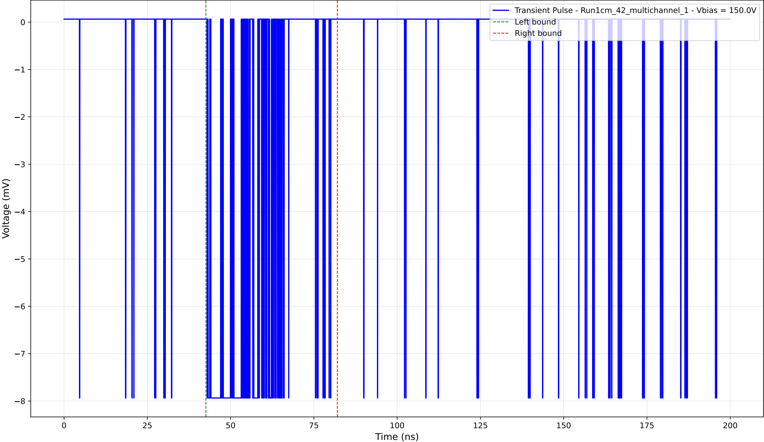
Transient Pulse - Sample: 1cm_42_multichannel - Position: 355.0 \mu\text{m} - Charge: -2.34 pC - Rise Time: 0.02 ns
