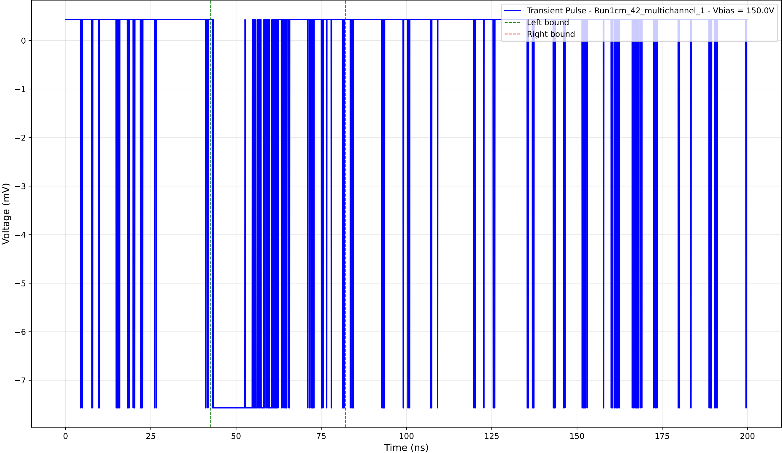
Transient Pulse - Sample: 1cm_42_multichannel - Position: 885.0 \mu\text{m} - Charge: -2.61 pC - Rise Time: 0.02 ns
