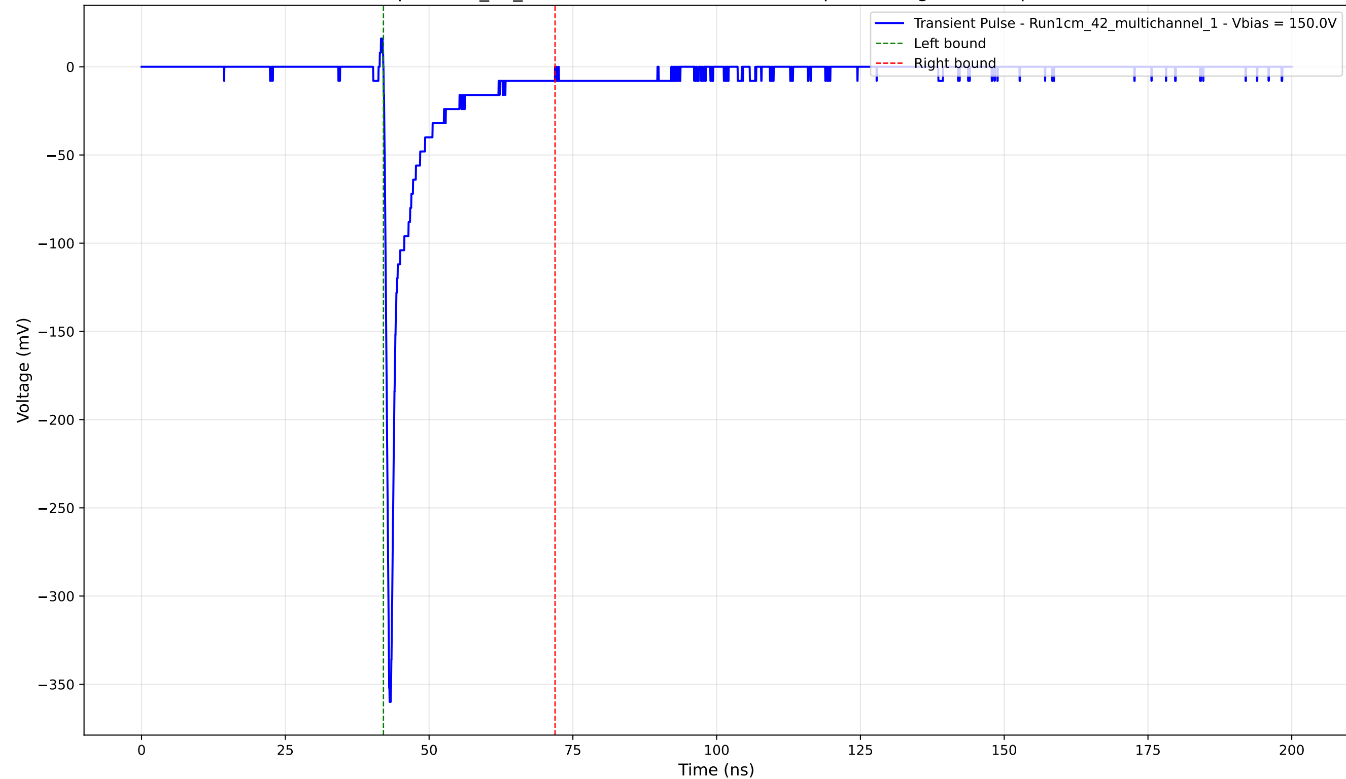
Transient Pulse - Sample: 1cm_42_multichannel - Position: 2555.0 \mu\text{m} - Charge: -25.28 pC - Rise Time: 0.74 ns
