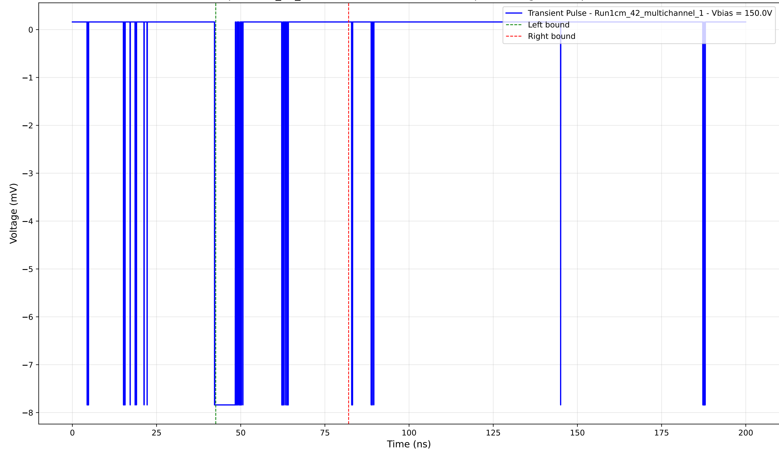
Transient Pulse - Sample: 1cm_42_multichannel - Position: 3415.0 \mu\text{m} - Charge: -1.10 pC - Rise Time: 0.02 ns
