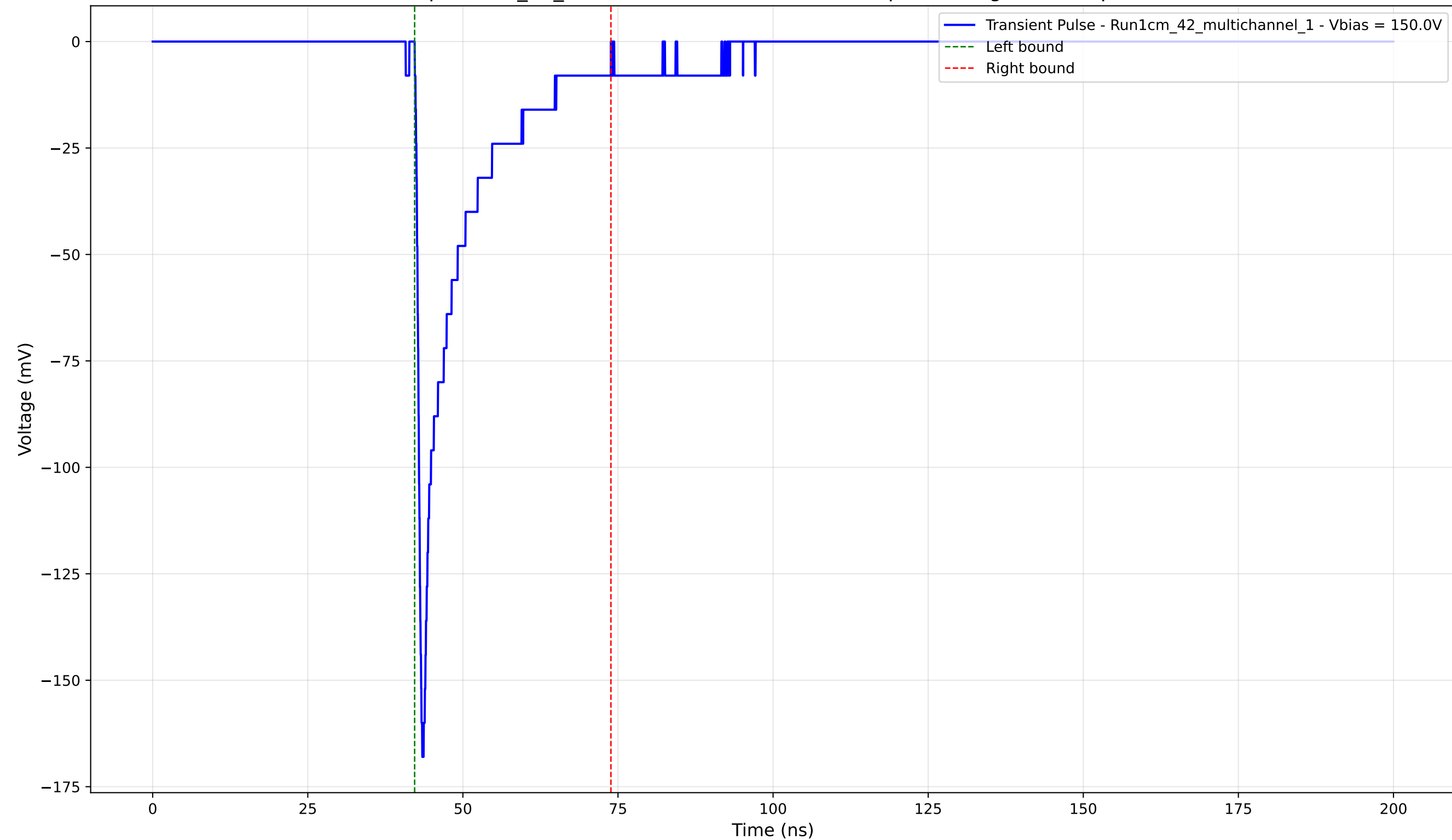
Transient Pulse - Sample: 1cm_42_multichannel - Position: 3005.0 \mu\text{m} - Charge: -21.88 pC - Rise Time: 0.84 ns
