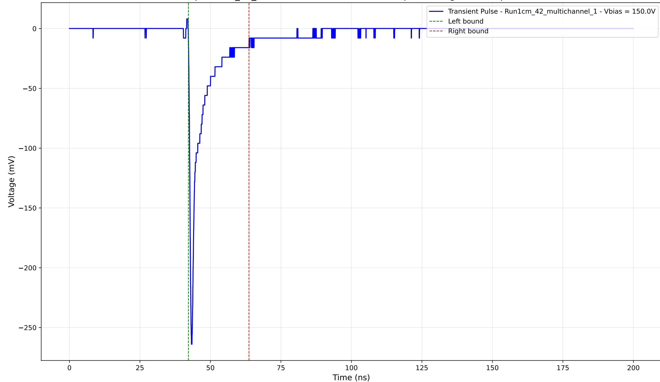
Transient Pulse - Sample: 1cm_42_multichannel - Position: 2740.0 \mu\text{m} - Charge: -22.63 pC - Rise Time: 0.79 ns
