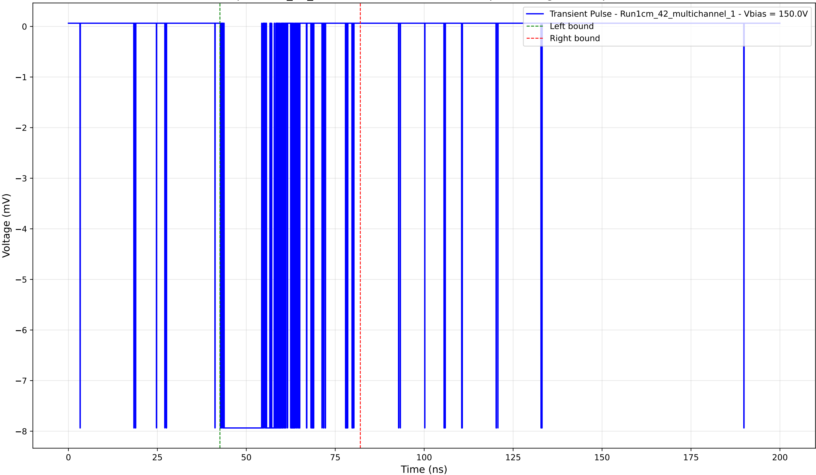
Transient Pulse - Sample: 1cm_42_multichannel - Position: 880.0 \mu\text{m} - Charge: -2.87 pC - Rise Time: 0.02 ns
