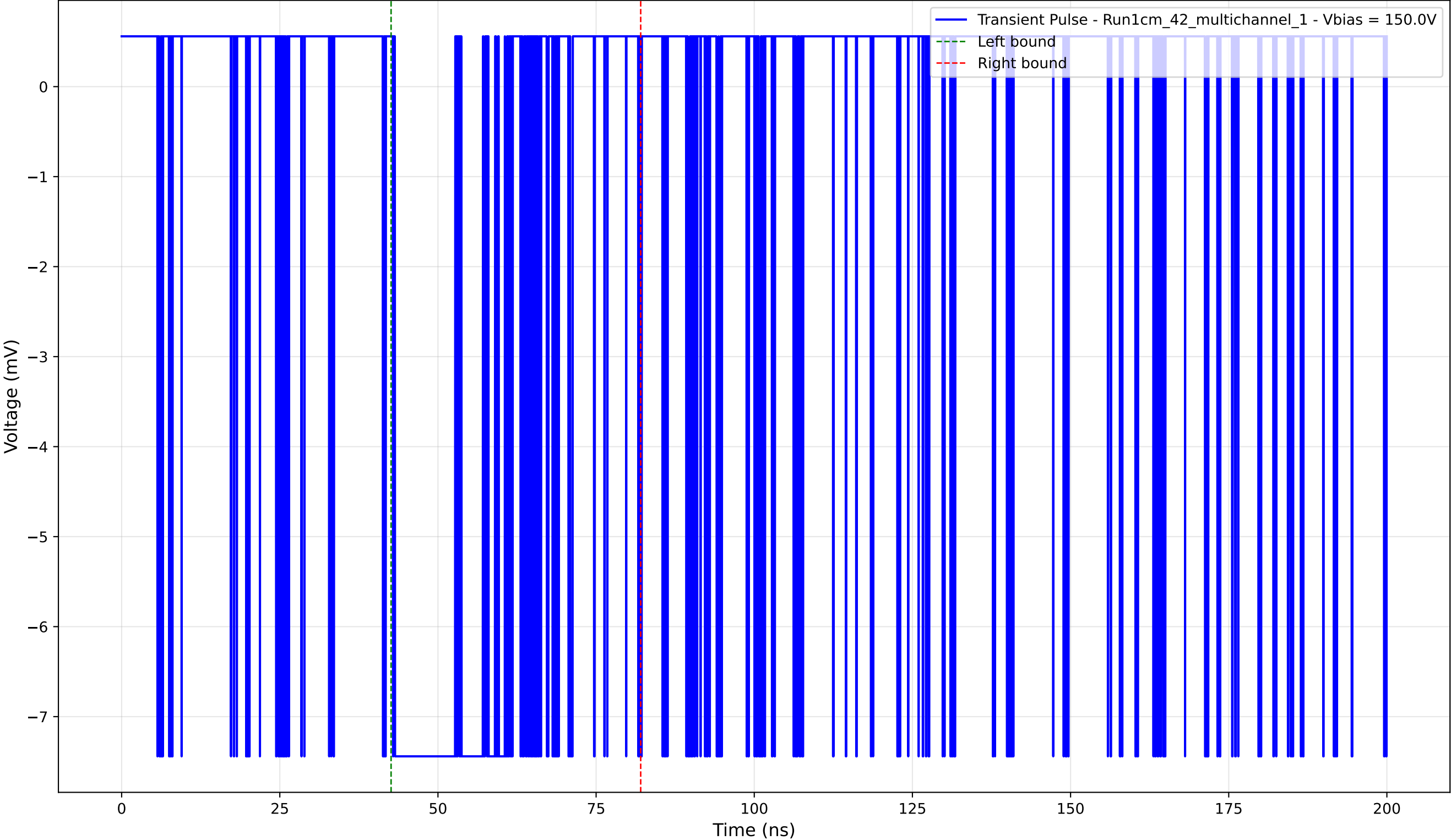
Transient Pulse - Sample: 1cm_42_multichannel - Position: 850.0 \mu\text{m} - Charge: -2.76 pC - Rise Time: 0.02 ns
