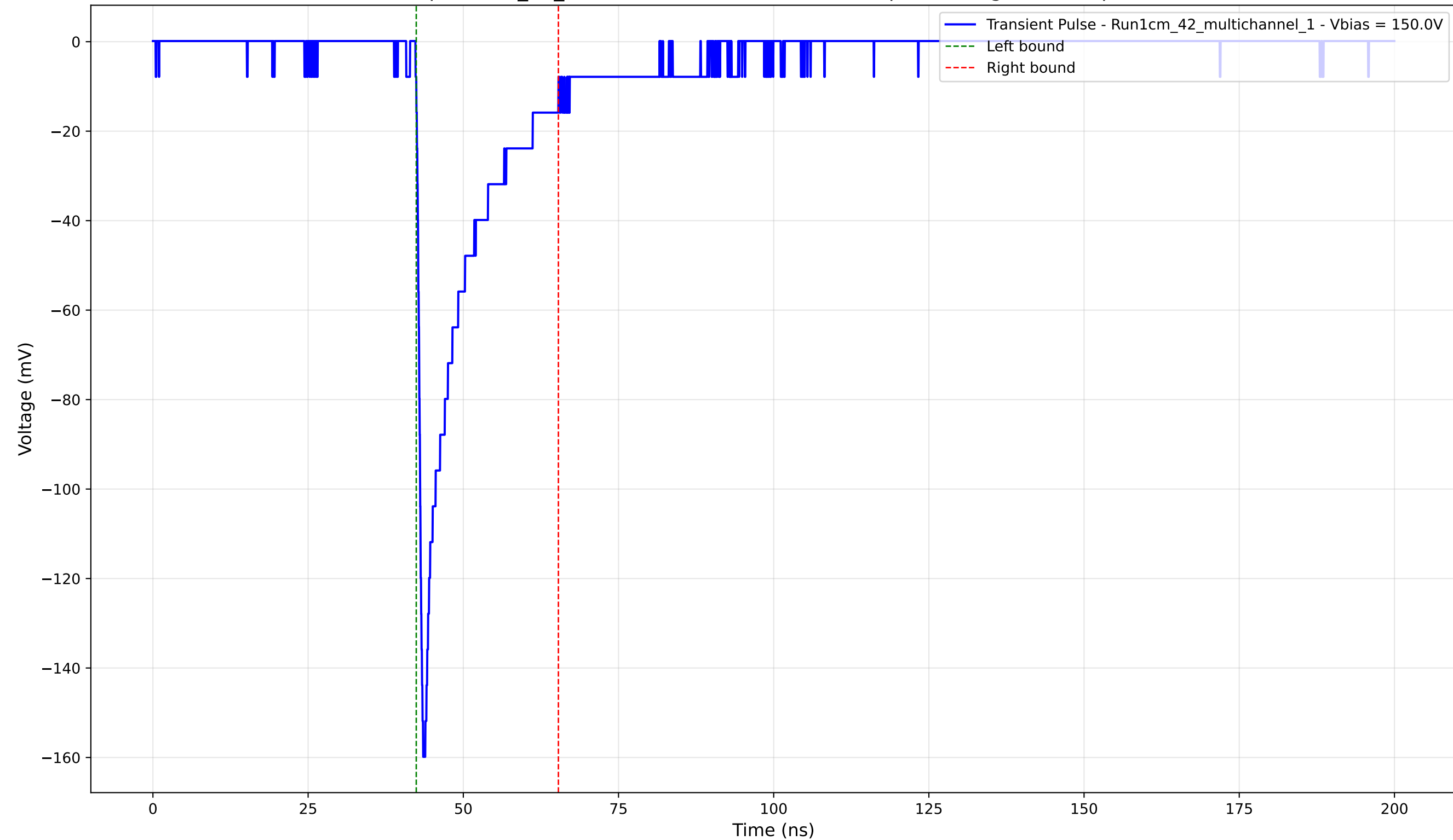
Transient Pulse - Sample: 1cm_42_multichannel - Position: 1685.0 \mu\text{m} - Charge: -22.39 pC - Rise Time: 0.92 ns
