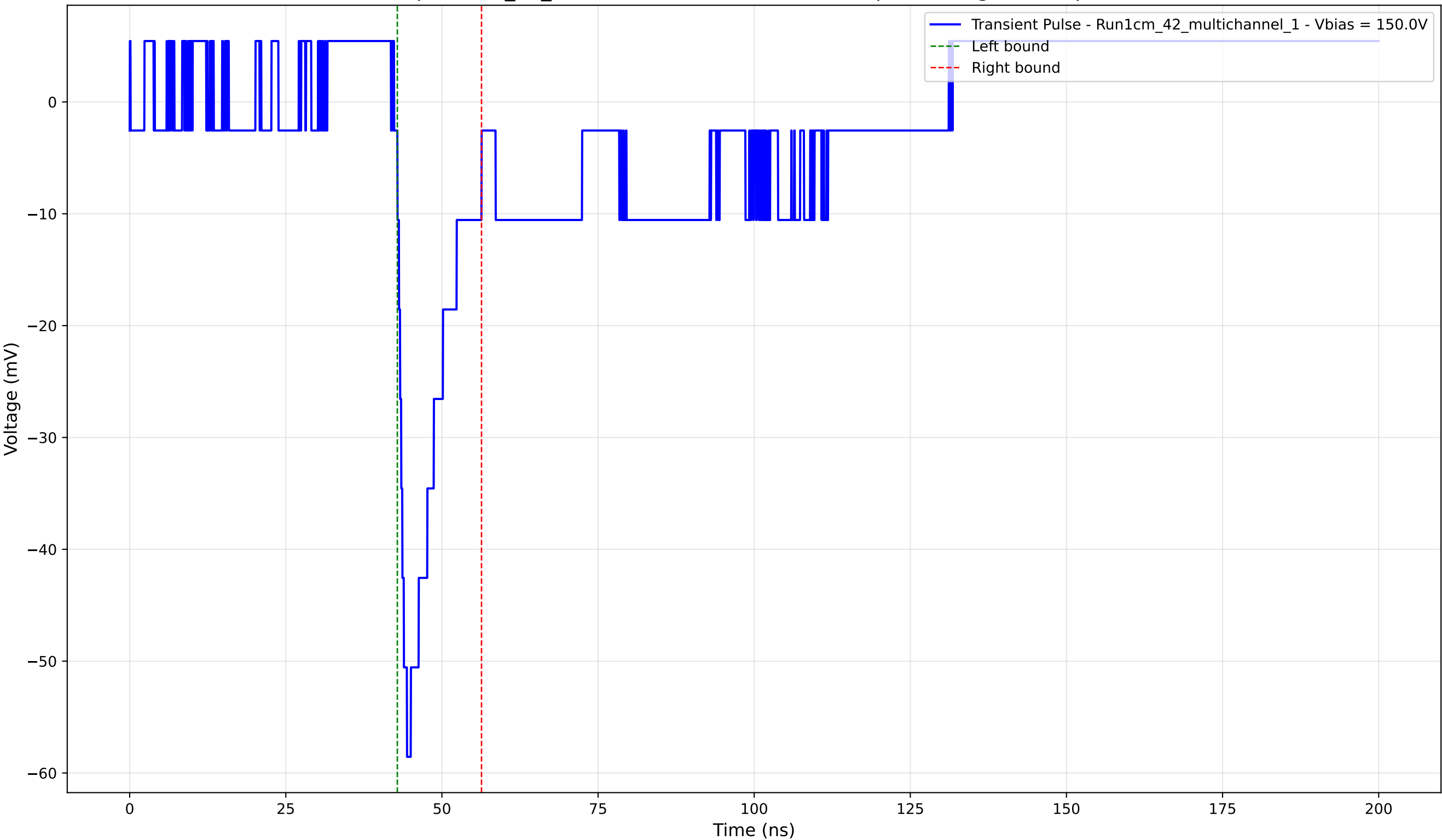
Transient Pulse - Sample: 1cm_42_multichannel - Position: 3790.0 \mu\text{m} - Charge: -7.37 pC - Rise Time: 1.53 ns
