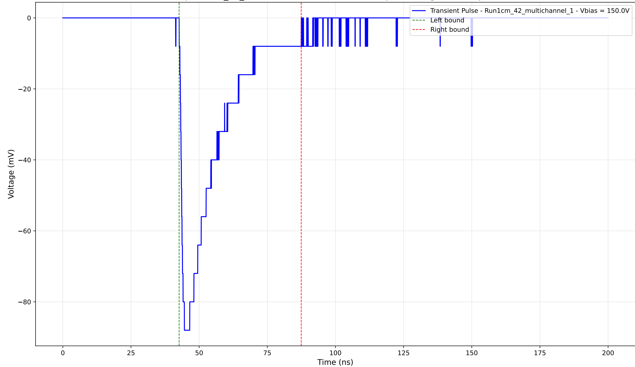
Transient Pulse - Sample: 1cm_42_multichannel - Position: 1025.0 \mu\text{m} - Charge: -25.95 pC - Rise Time: 1.18 ns
