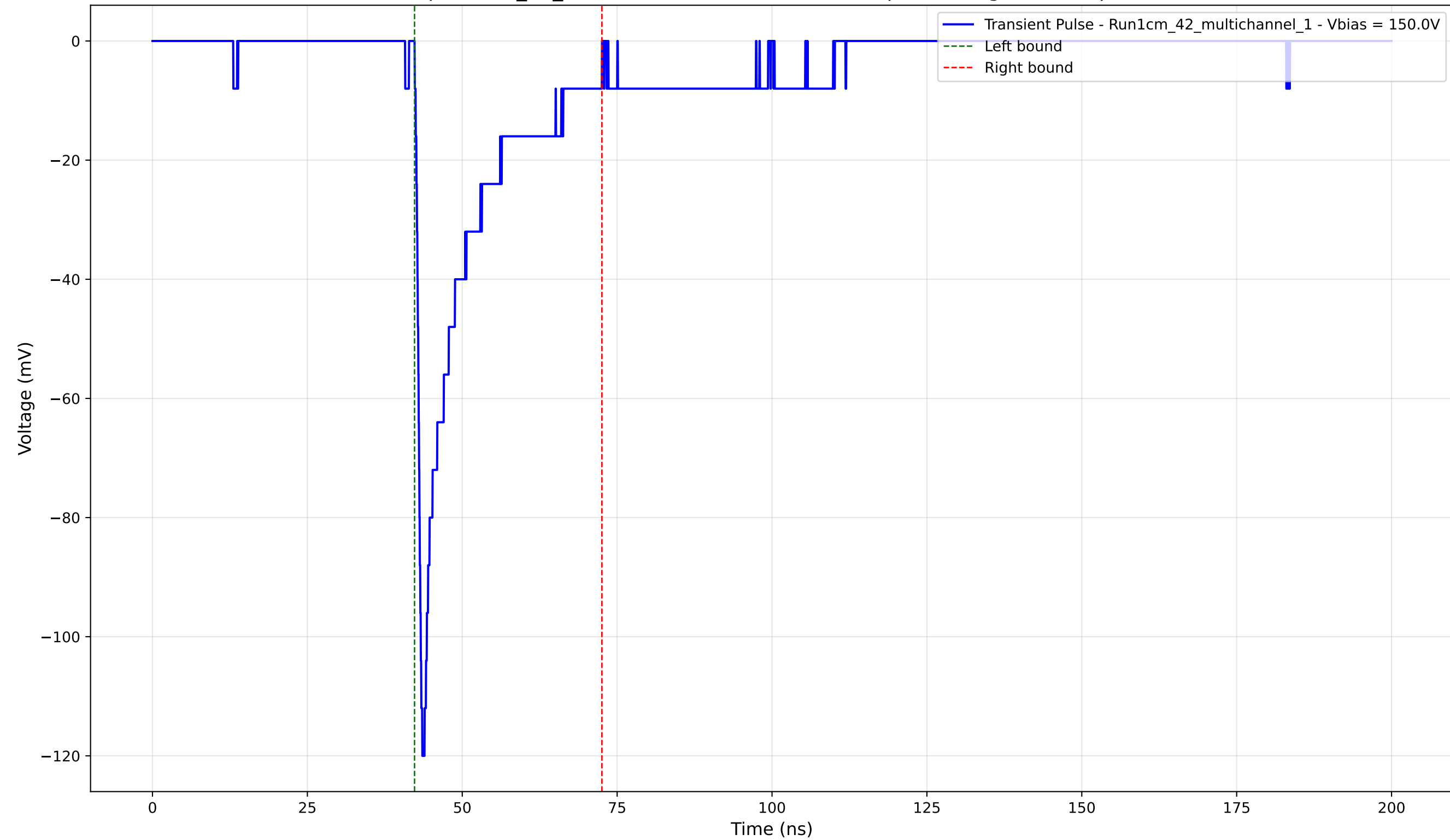
Transient Pulse - Sample: 1cm_42_multichannel - Position: 3170.0 \mu\text{m} - Charge: -17.73 pC - Rise Time: 0.91 ns
