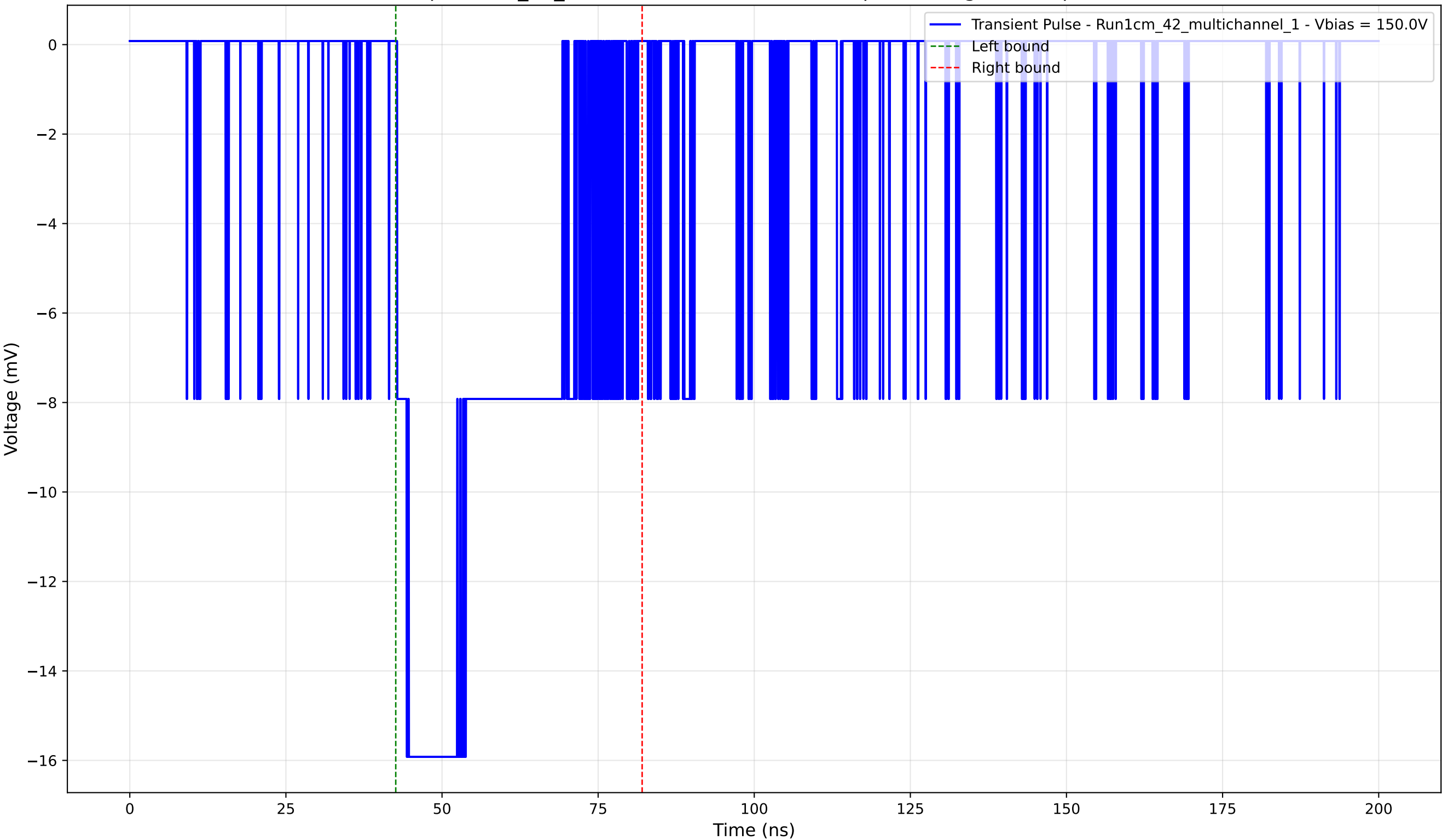
Transient Pulse - Sample: 1cm_42_multichannel - Position: 75.0 \mu\text{m} - Charge: -6.52 pC - Rise Time: 1.54 ns
