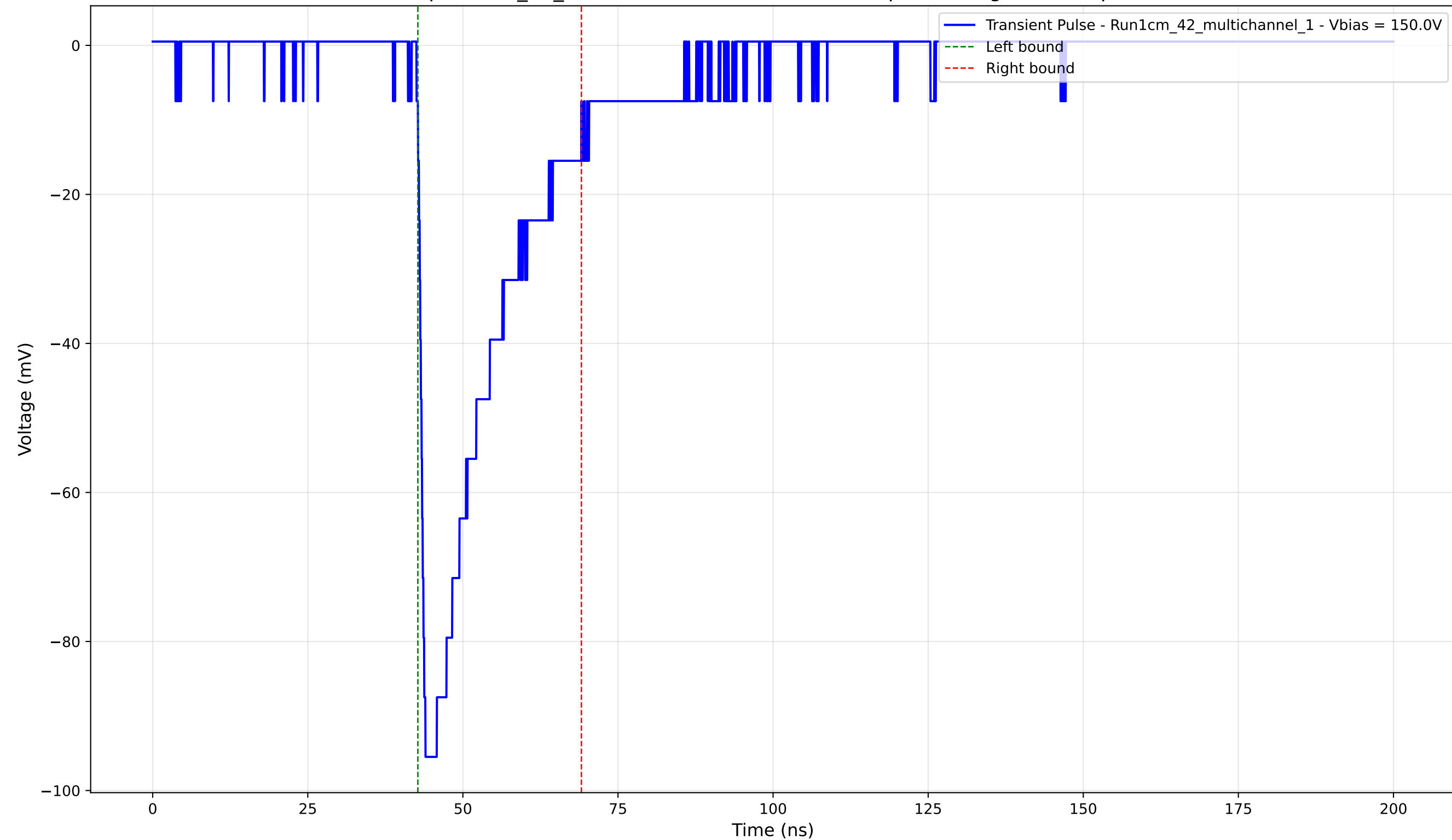
Transient Pulse - Sample: 1cm_42_multichannel - Position: 1210.0 \mu\text{m} - Charge: -23.20 pC - Rise Time: 1.01 ns
