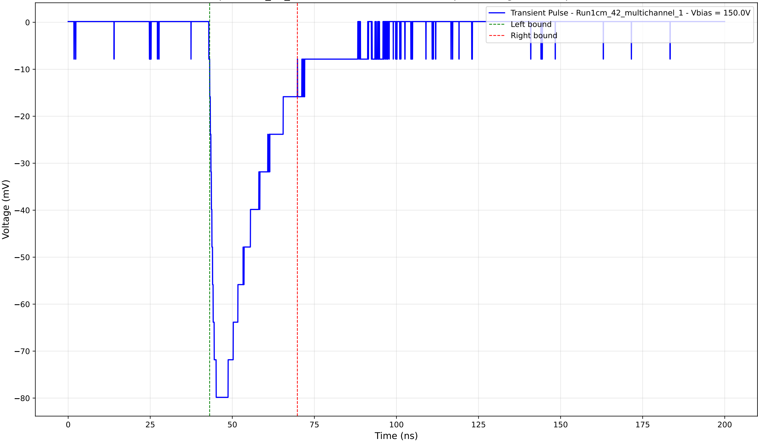
Transient Pulse - Sample: 1cm_42_multichannel - Position: 700.0 \mu\text{m} - Charge: -23.30 pC - Rise Time: 1.98 ns
