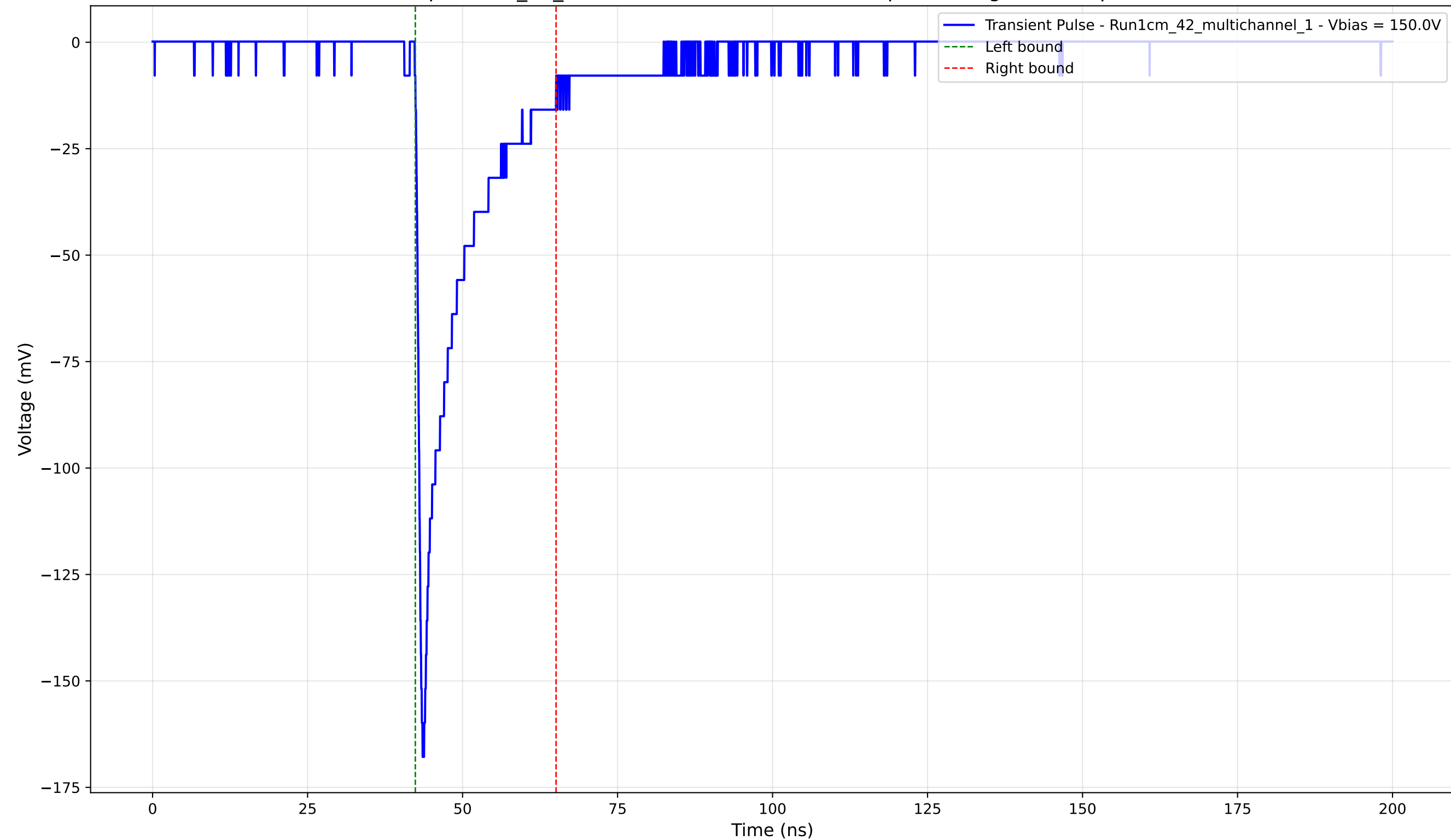
Transient Pulse - Sample: 1cm_42_multichannel - Position: 1700.0 \mu\text{m} - Charge: -22.55 pC - Rise Time: 0.84 ns
