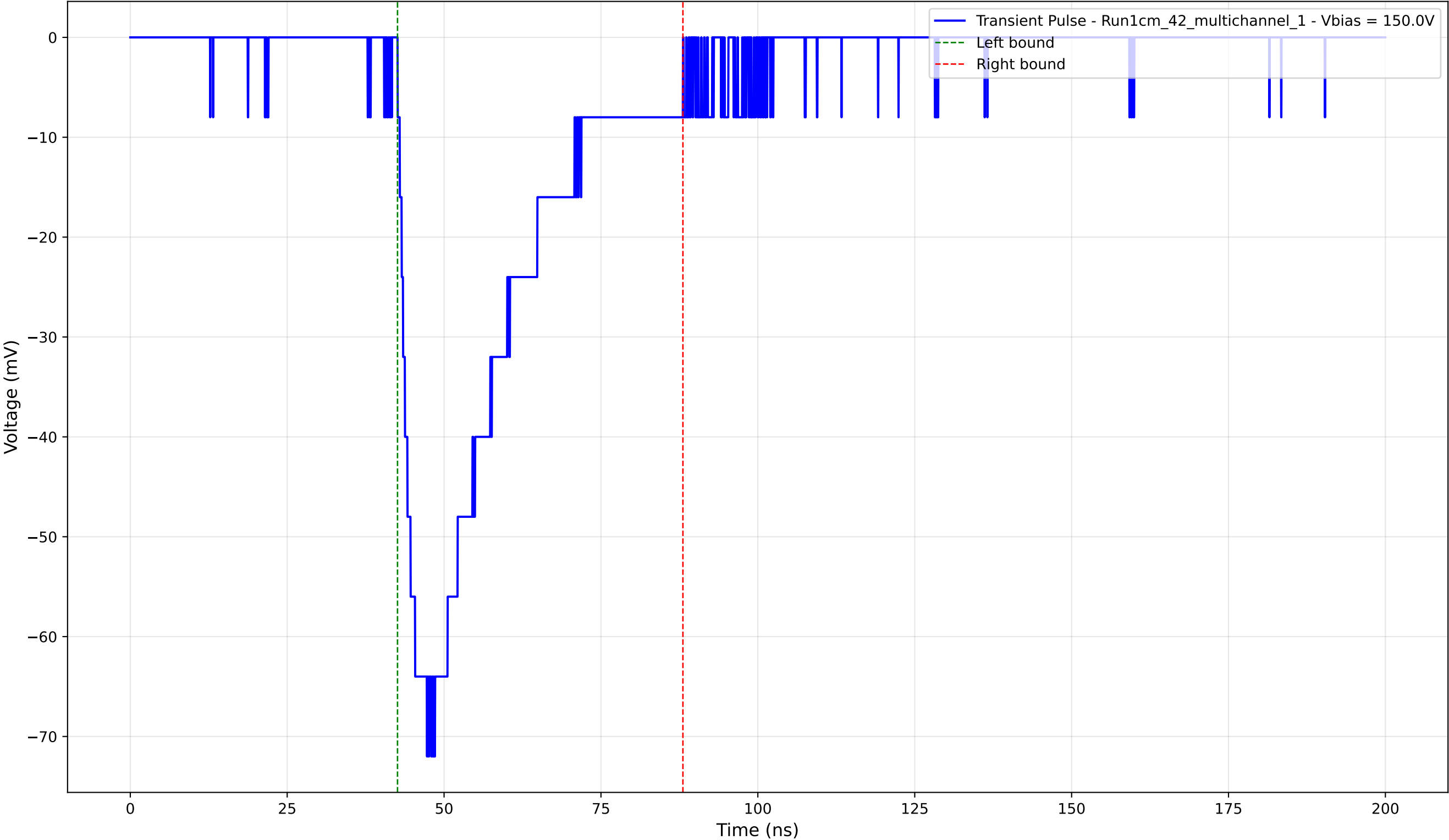
Transient Pulse - Sample: 1cm_42_multichannel - Position: 200.0 \mu\text{m} - Charge: -23.94 pC - Rise Time: 4.66 ns
