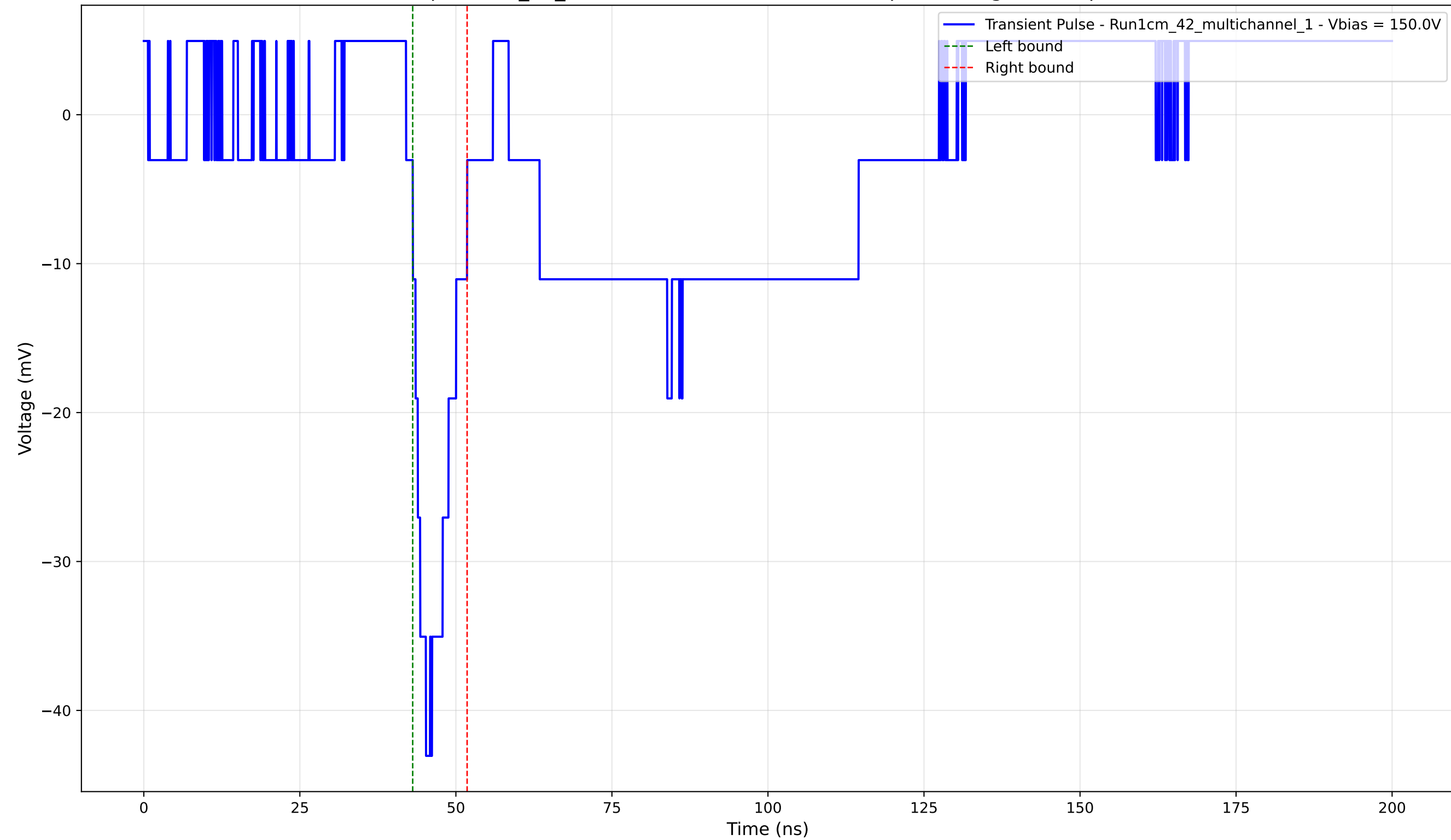
Transient Pulse - Sample: 1cm_42_multichannel - Position: 4480.0 \mu\text{m} - Charge: -4.46 pC - Rise Time: 2.12 ns
