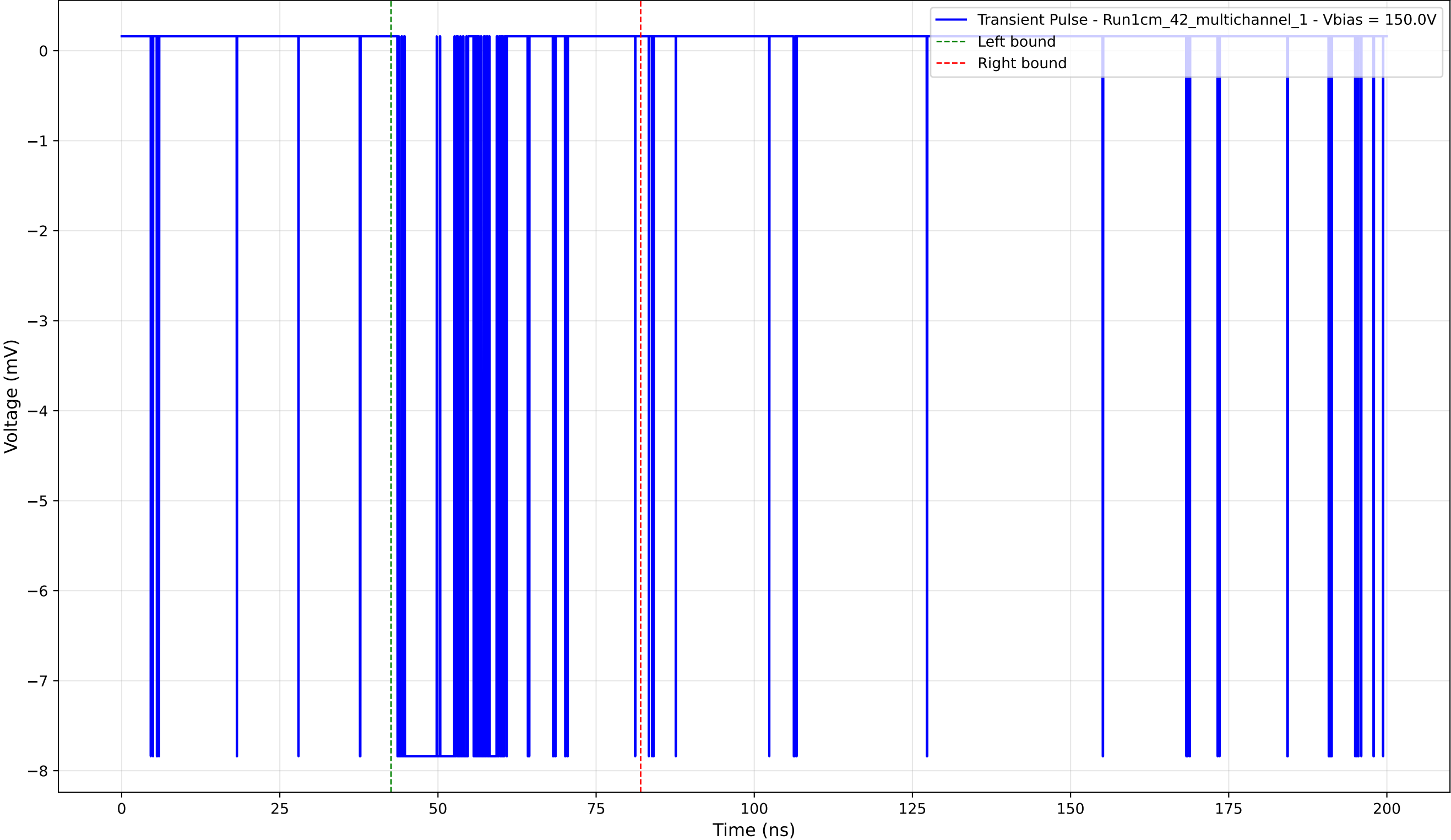
Transient Pulse - Sample: 1cm_42_multichannel - Position: 365.0 \mu\text{m} - Charge: -2.15 pC - Rise Time: 0.02 ns
