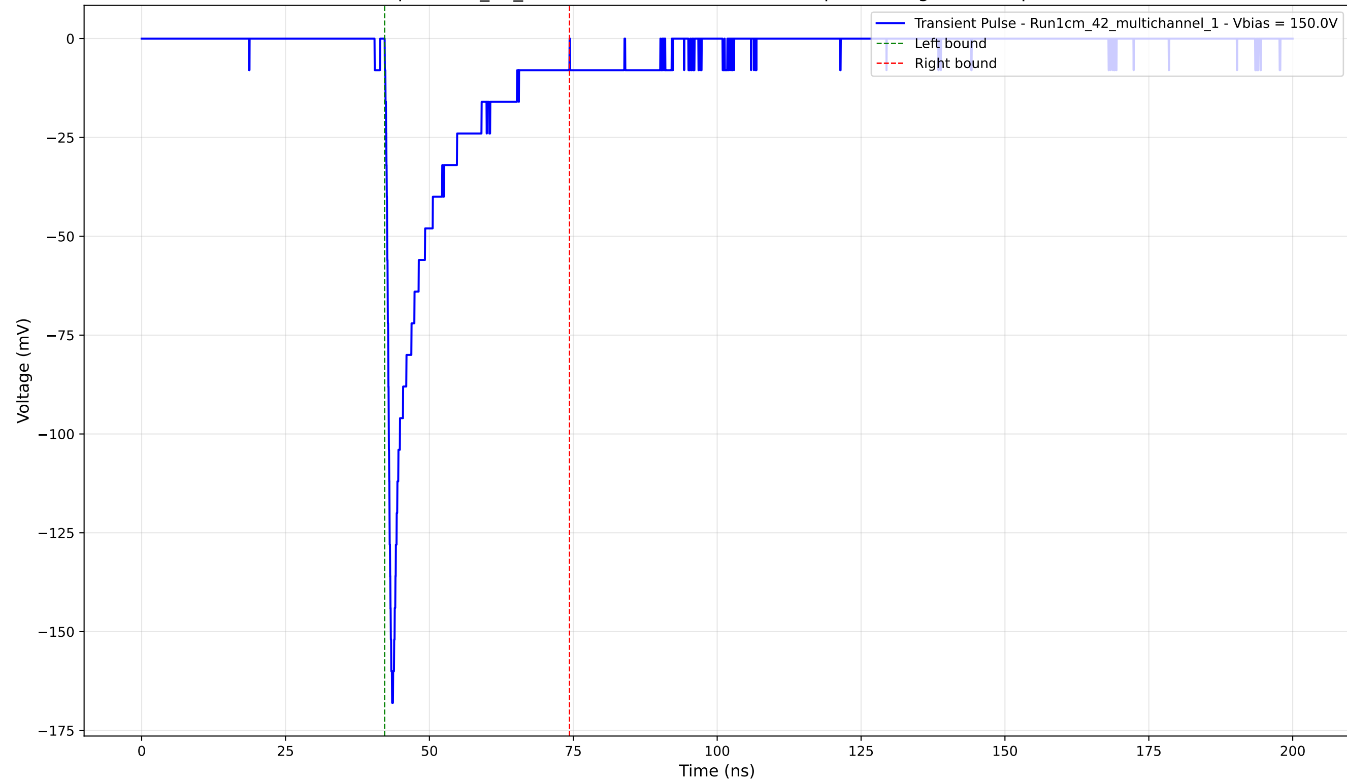
Transient Pulse - Sample: 1cm_42_multichannel - Position: 3015.0 \mu\text{m} - Charge: -21.98 pC - Rise Time: 0.84 ns
