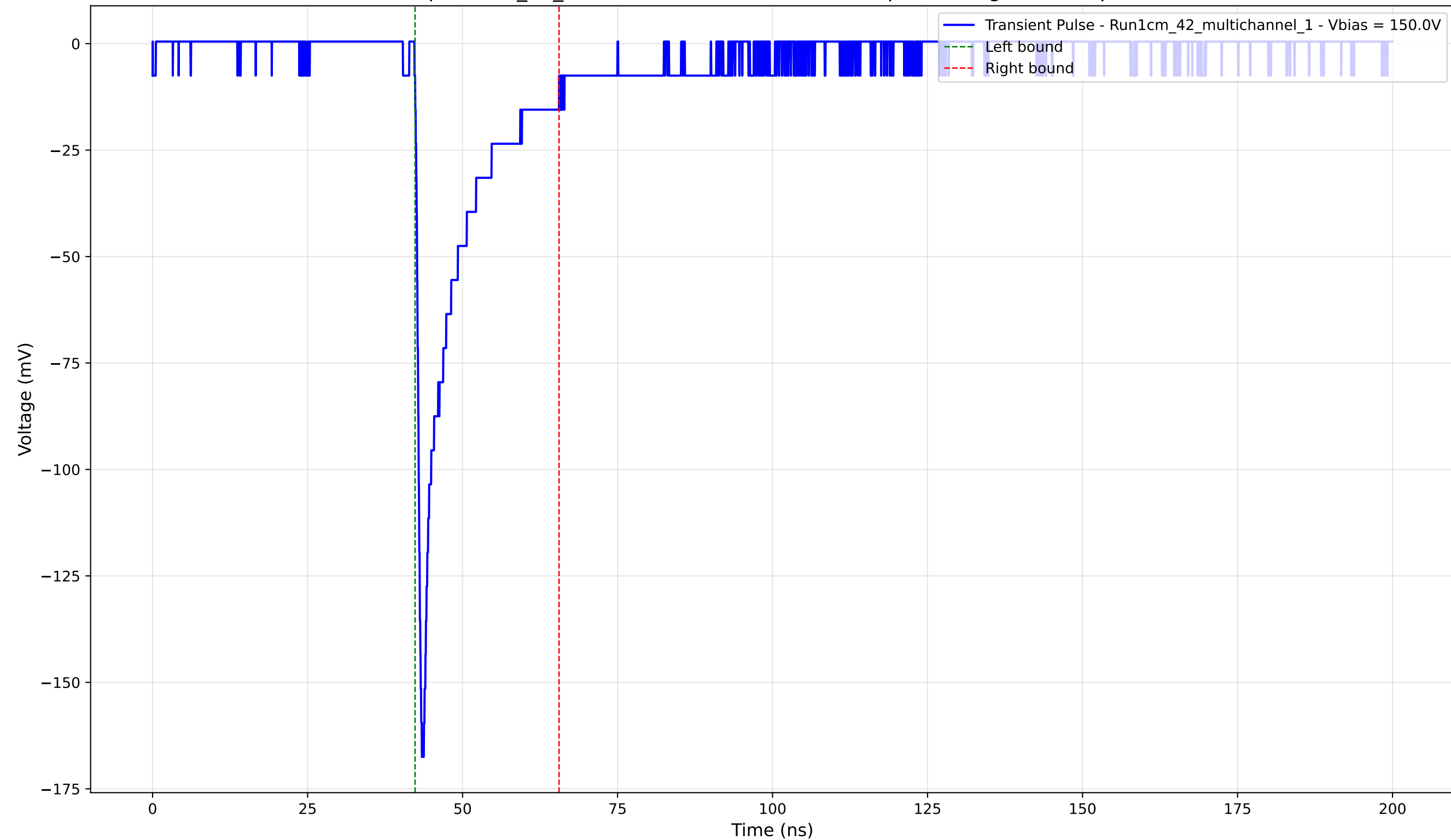
Transient Pulse - Sample: 1cm_42_multichannel - Position: 3000.0 \mu\text{m} - Charge: -20.50 pC - Rise Time: 0.82 ns
