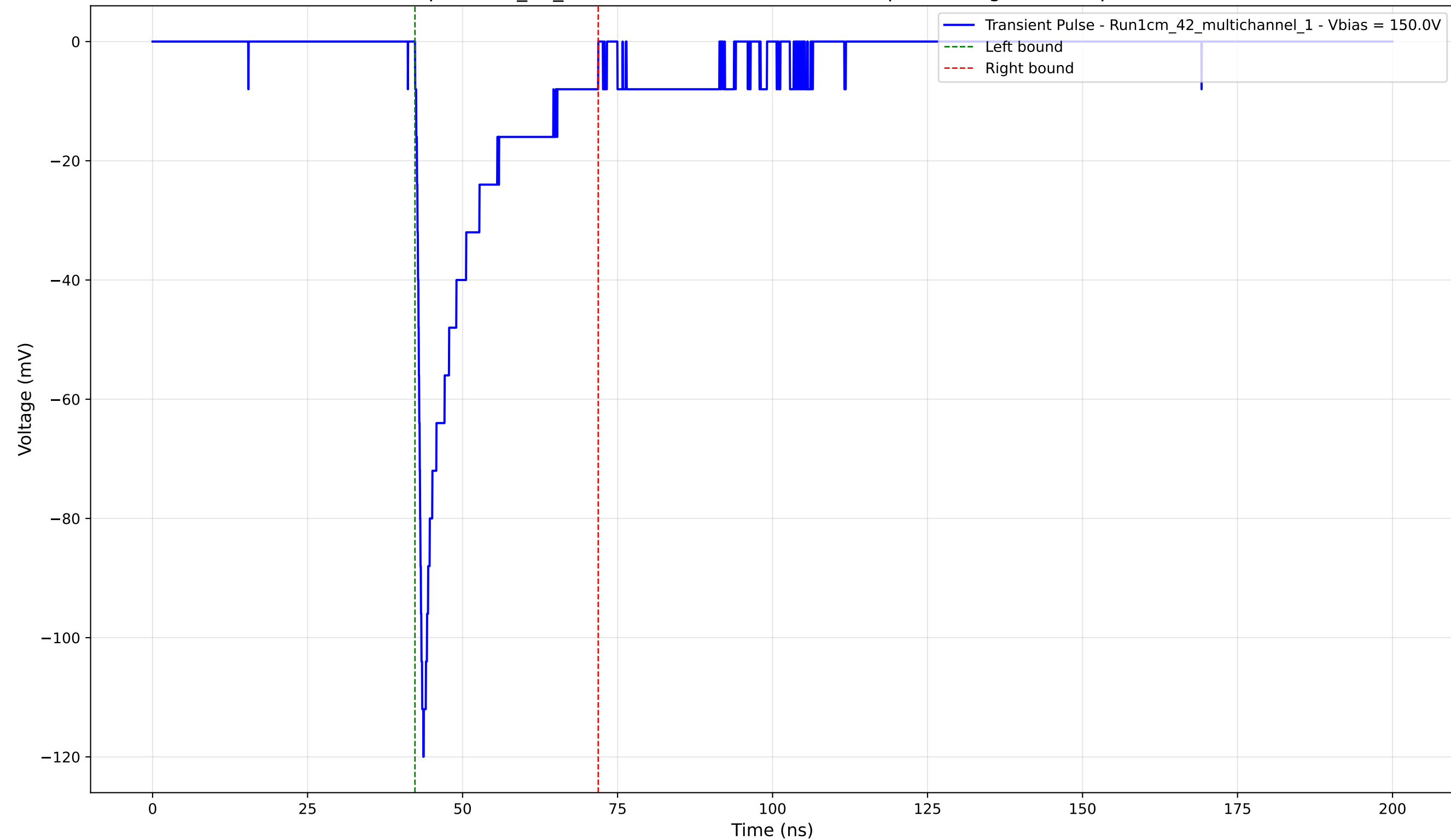
Transient Pulse - Sample: 1cm_42_multichannel - Position: 3205.0 \mu\text{m} - Charge: -17.09 pC - Rise Time: 0.97 ns
