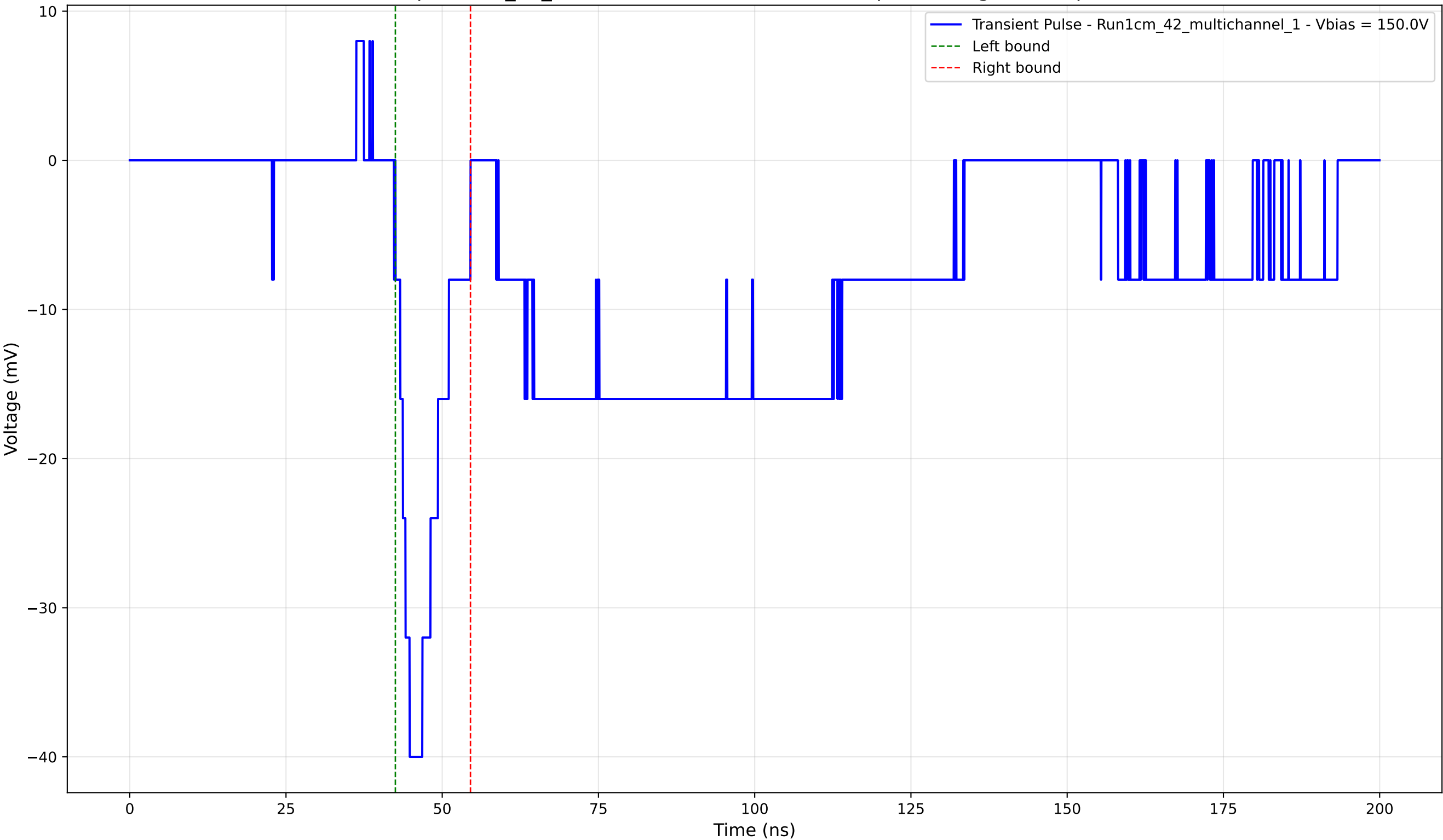
Transient Pulse - Sample: 1cm_42_multichannel - Position: 4470.0 \mu\text{m} - Charge: -5.03 pC - Rise Time: 2.27 ns
