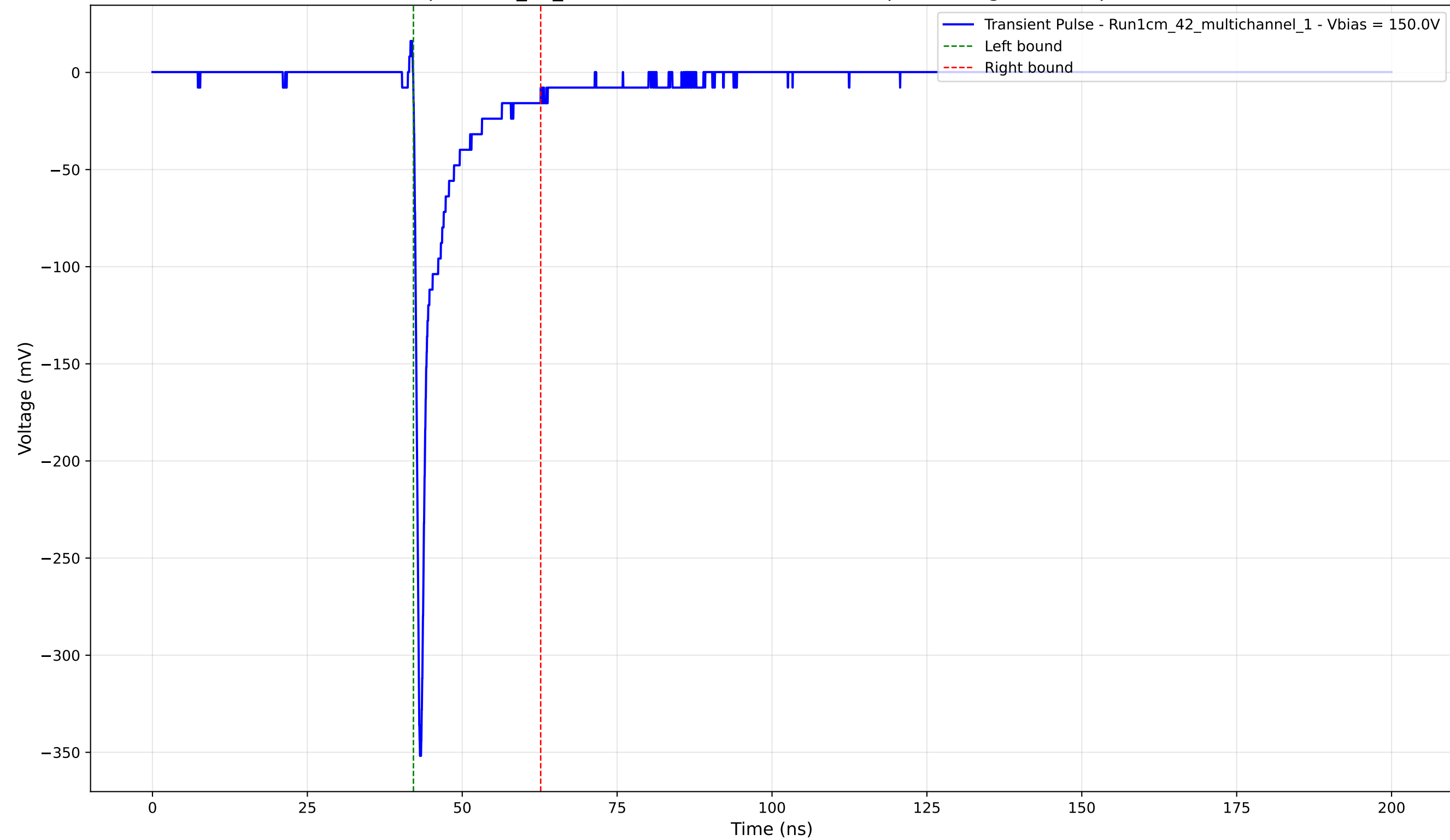
Transient Pulse - Sample: 1cm_42_multichannel - Position: 2195.0 \mu\text{m} - Charge: -24.27 pC - Rise Time: 0.74 ns
