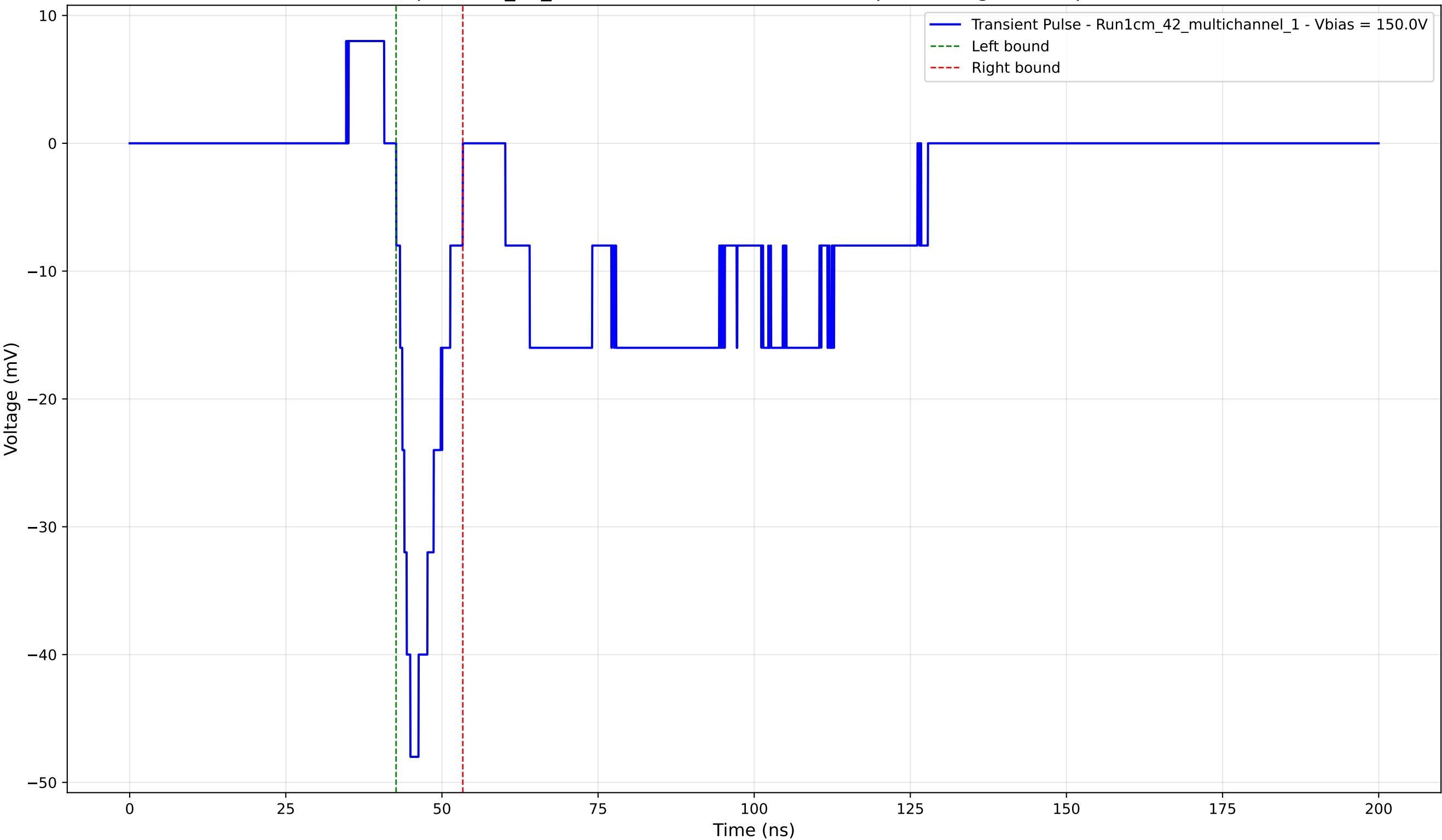
Transient Pulse - Sample: 1cm_42_multichannel - Position: 4575.0 \mu\text{m} - Charge: -5.48 pC - Rise Time: 2.27 ns
