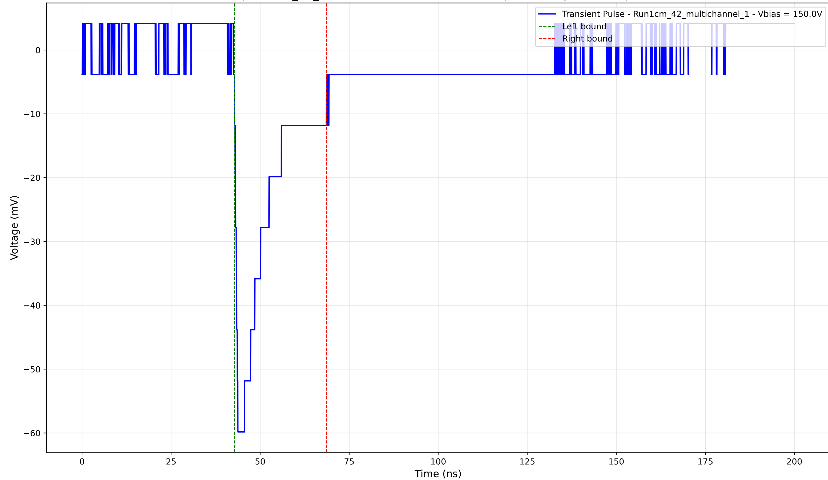
Transient Pulse - Sample: 1cm_42_multichannel - Position: 3625.0 \mu\text{m} - Charge: -12.51 pC - Rise Time: 0.97 ns
