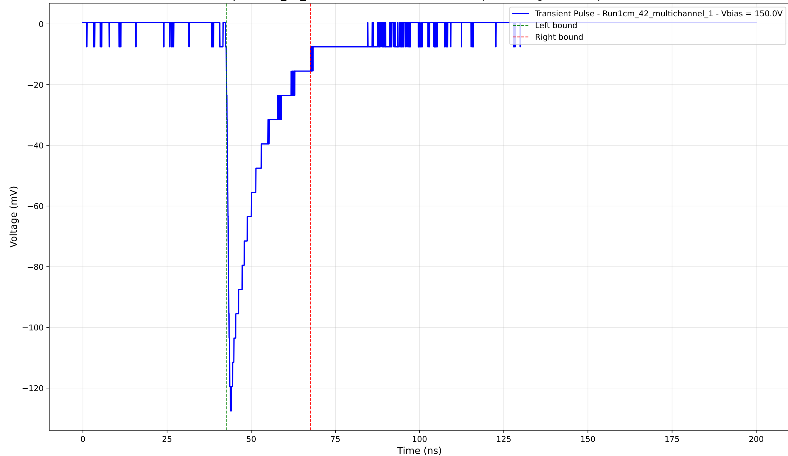
Transient Pulse - Sample: 1cm_42_multichannel - Position: 1475.0 \mu\text{m} - Charge: -22.95 pC - Rise Time: 1.05 ns
