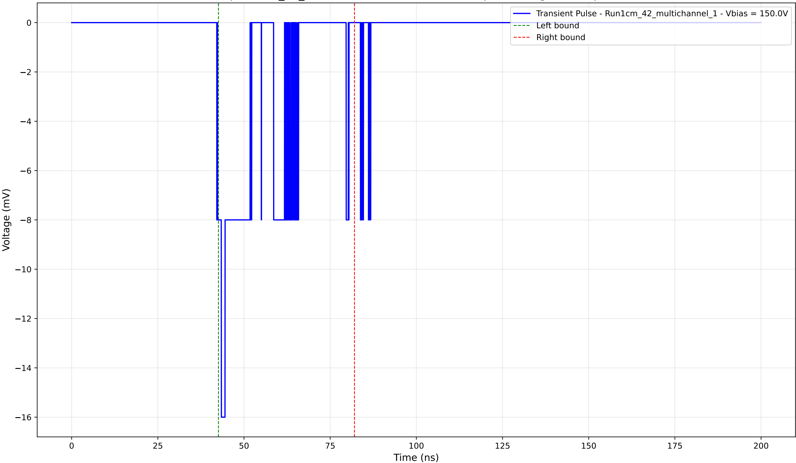
Transient Pulse - Sample: 1cm_42_multichannel - Position: 3370.0 \mu\text{m} - Charge: -2.72 pC - Rise Time: 1.12 ns
