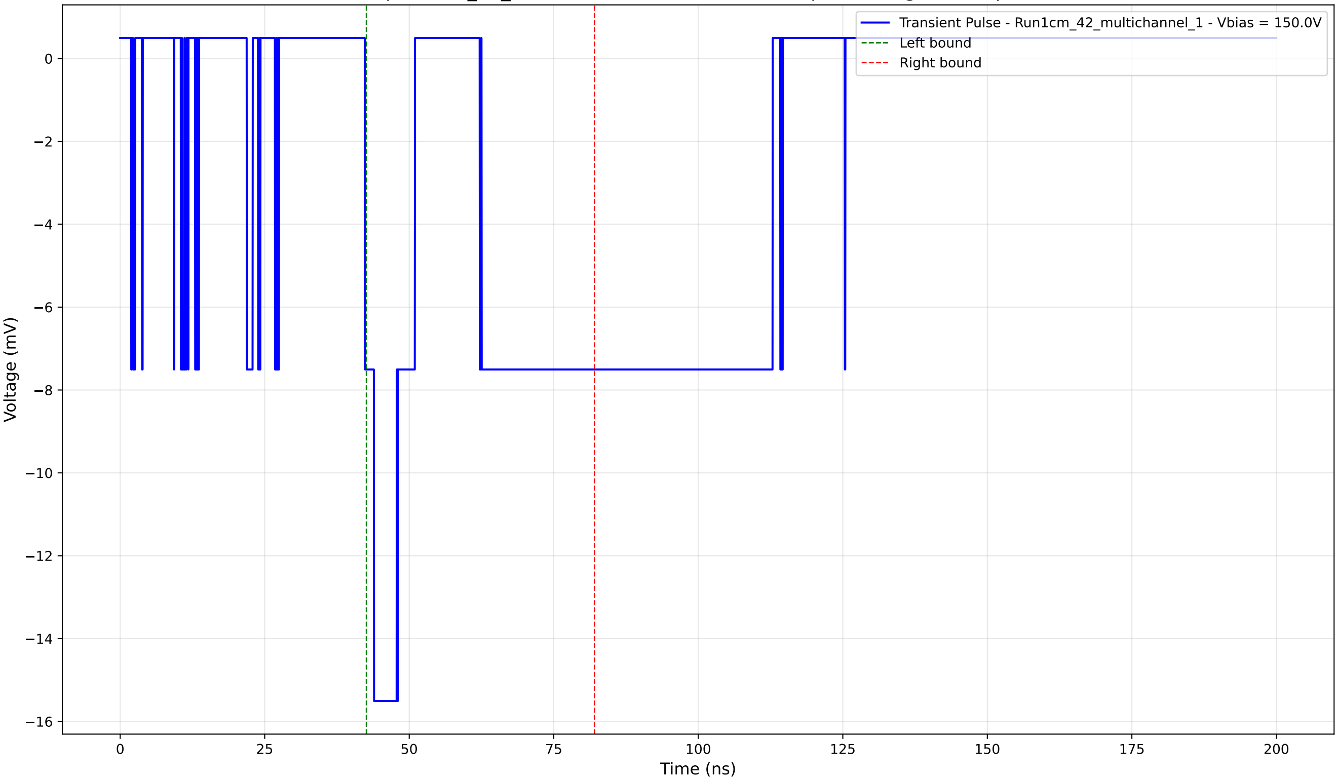
Transient Pulse - Sample: 1cm_42_multichannel - Position: 4365.0 \mu\text{m} - Charge: -4.76 pC - Rise Time: 1.58 ns
