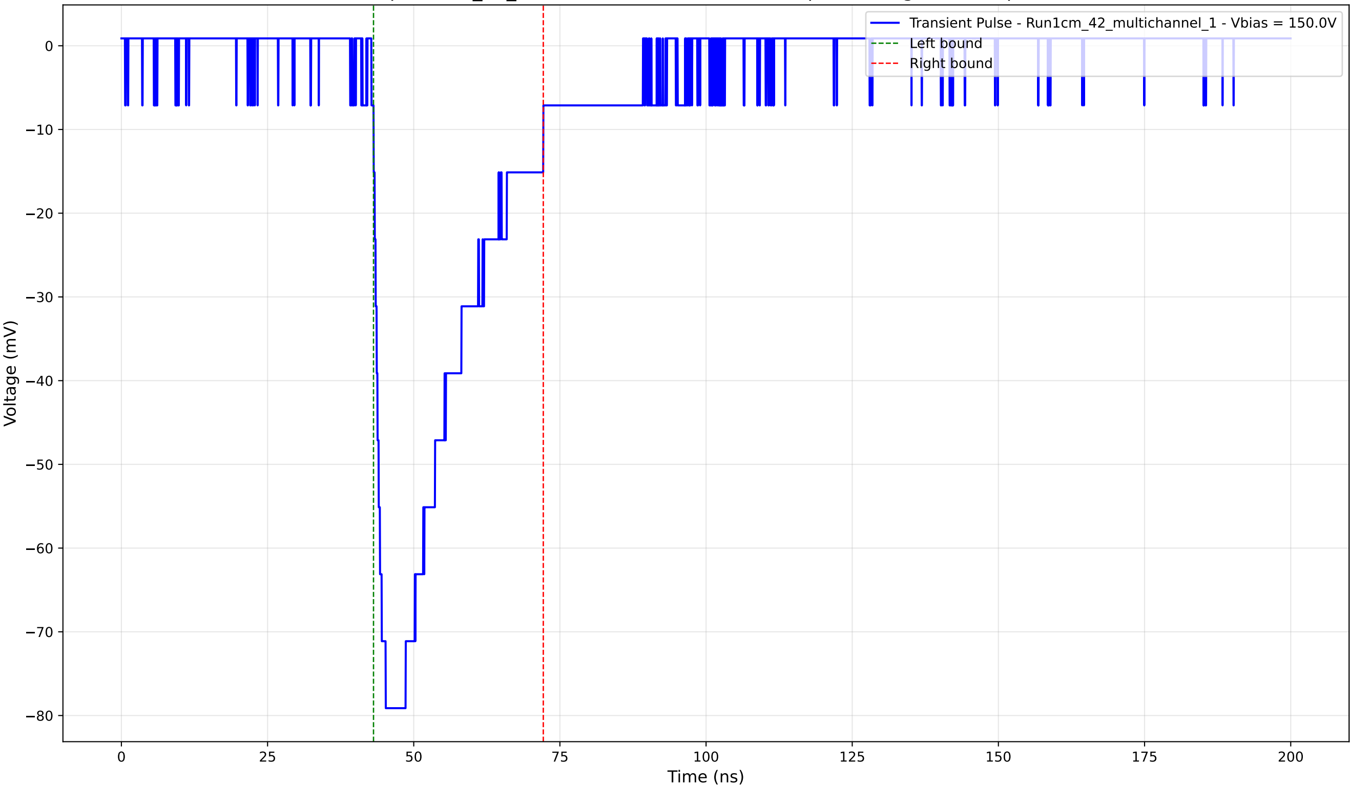
Transient Pulse - Sample: 1cm_42_multichannel - Position: 665.0 \mu\text{m} - Charge: -23.67 pC - Rise Time: 2.08 ns
