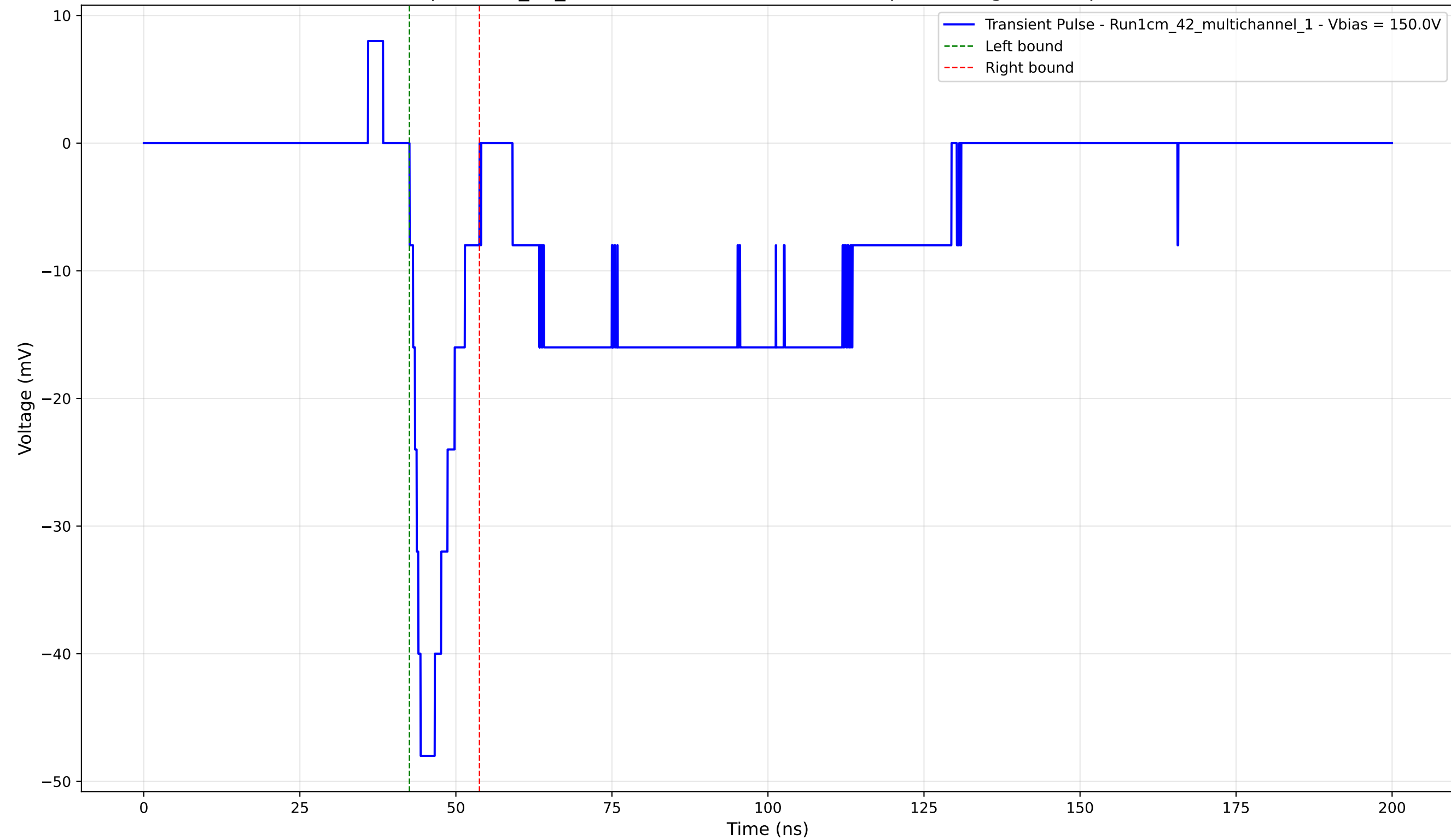
Transient Pulse - Sample: 1cm_42_multichannel - Position: 4115.0 \mu\text{m} - Charge: -5.88 pC - Rise Time: 1.77 ns
