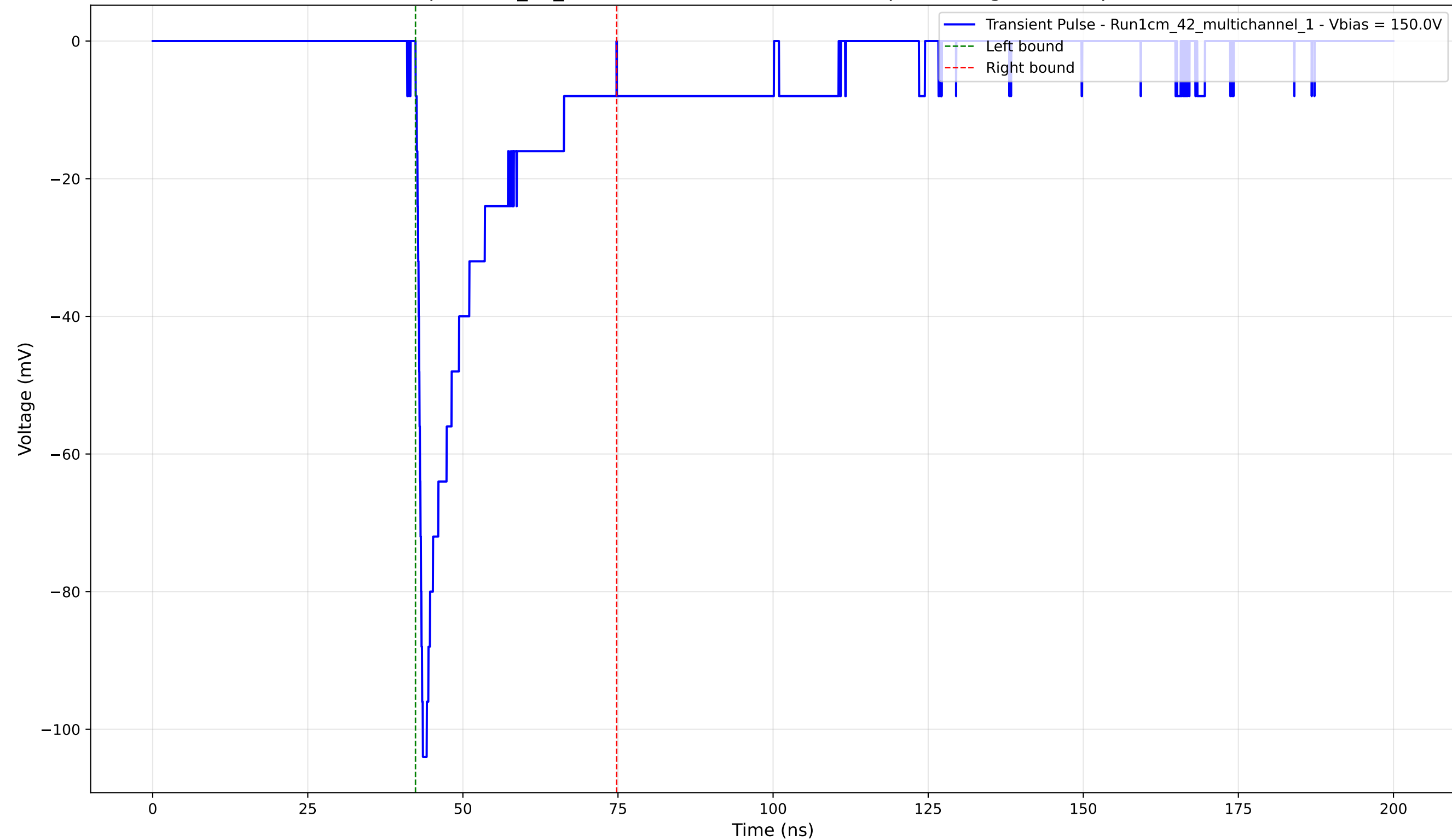
Transient Pulse - Sample: 1cm_42_multichannel - Position: 3270.0 \mu\text{m} - Charge: -18.25 pC - Rise Time: 0.87 ns
