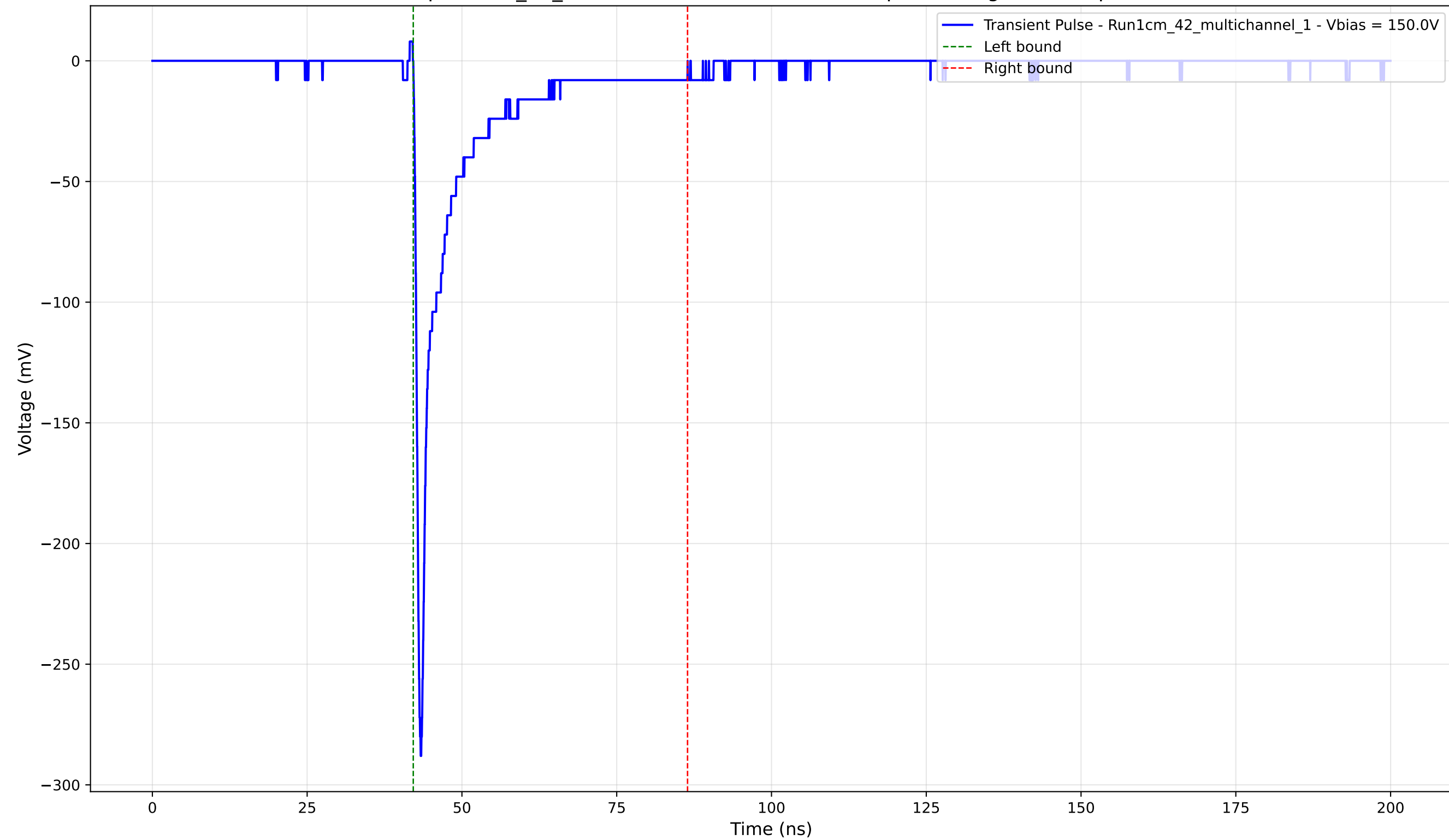
Transient Pulse - Sample: 1cm_42_multichannel - Position: 2055.0 \mu\text{m} - Charge: -27.57 pC - Rise Time: 0.81 ns
