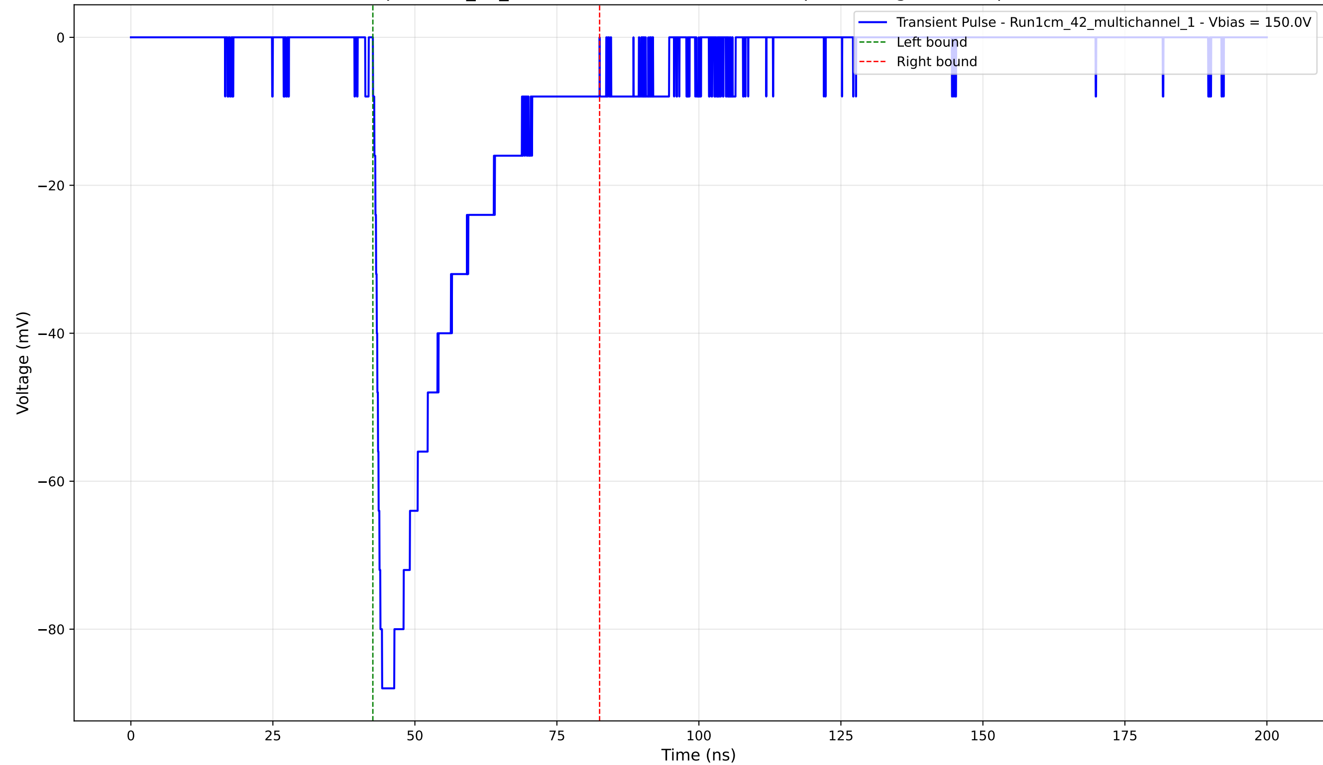
Transient Pulse - Sample: 1cm_42_multichannel - Position: 1100.0 \mu\text{m} - Charge: -24.77 pC - Rise Time: 1.08 ns
