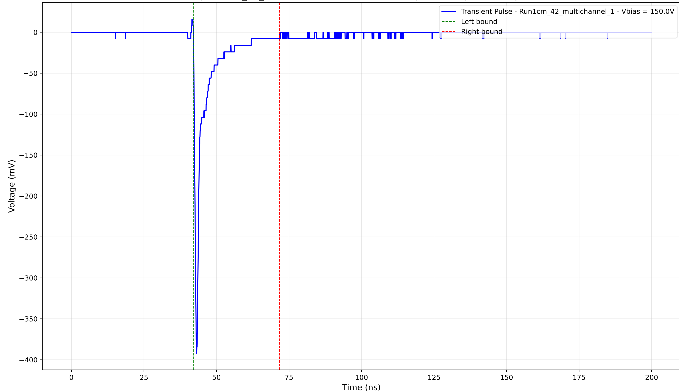
Transient Pulse - Sample: 1cm_42_multichannel - Position: 2500.0 \mu\text{m} - Charge: -25.79 pC - Rise Time: 0.74 ns
