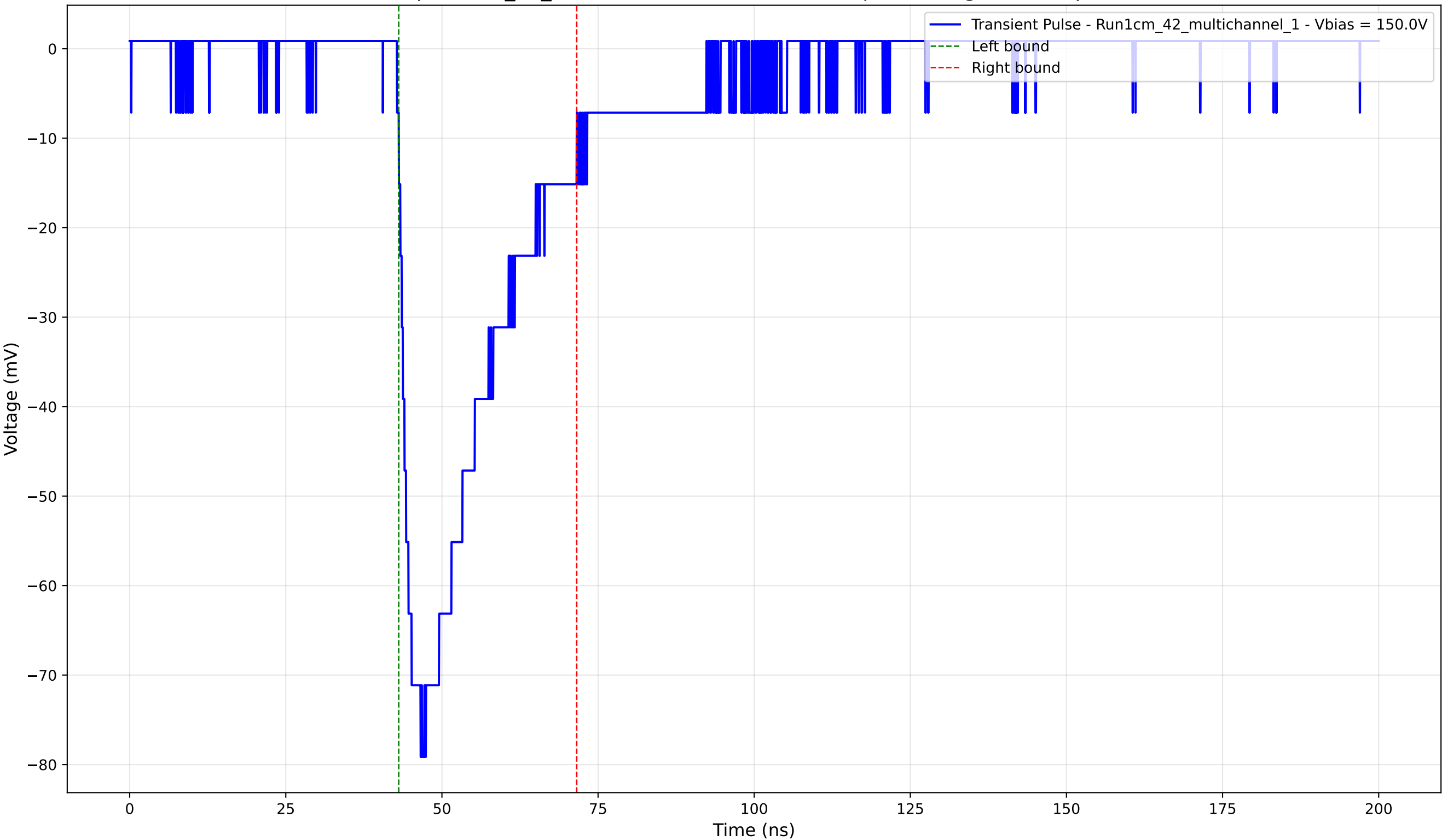
Transient Pulse - Sample: 1cm_42_multichannel - Position: 460.0 \mu\text{m} - Charge: -22.42 pC - Rise Time: 3.50 ns
