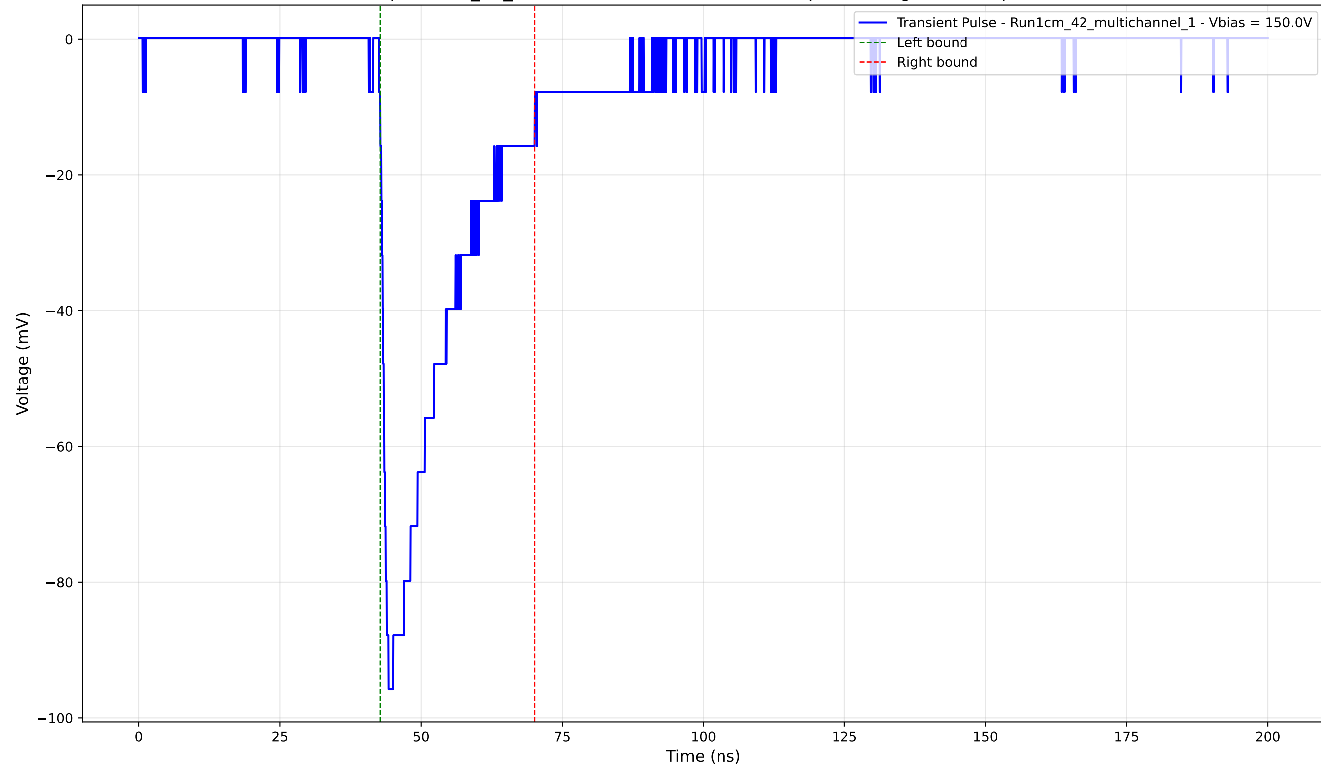
Transient Pulse - Sample: 1cm_42_multichannel - Position: 1165.0 \mu\text{m} - Charge: -23.36 pC - Rise Time: 1.14 ns
