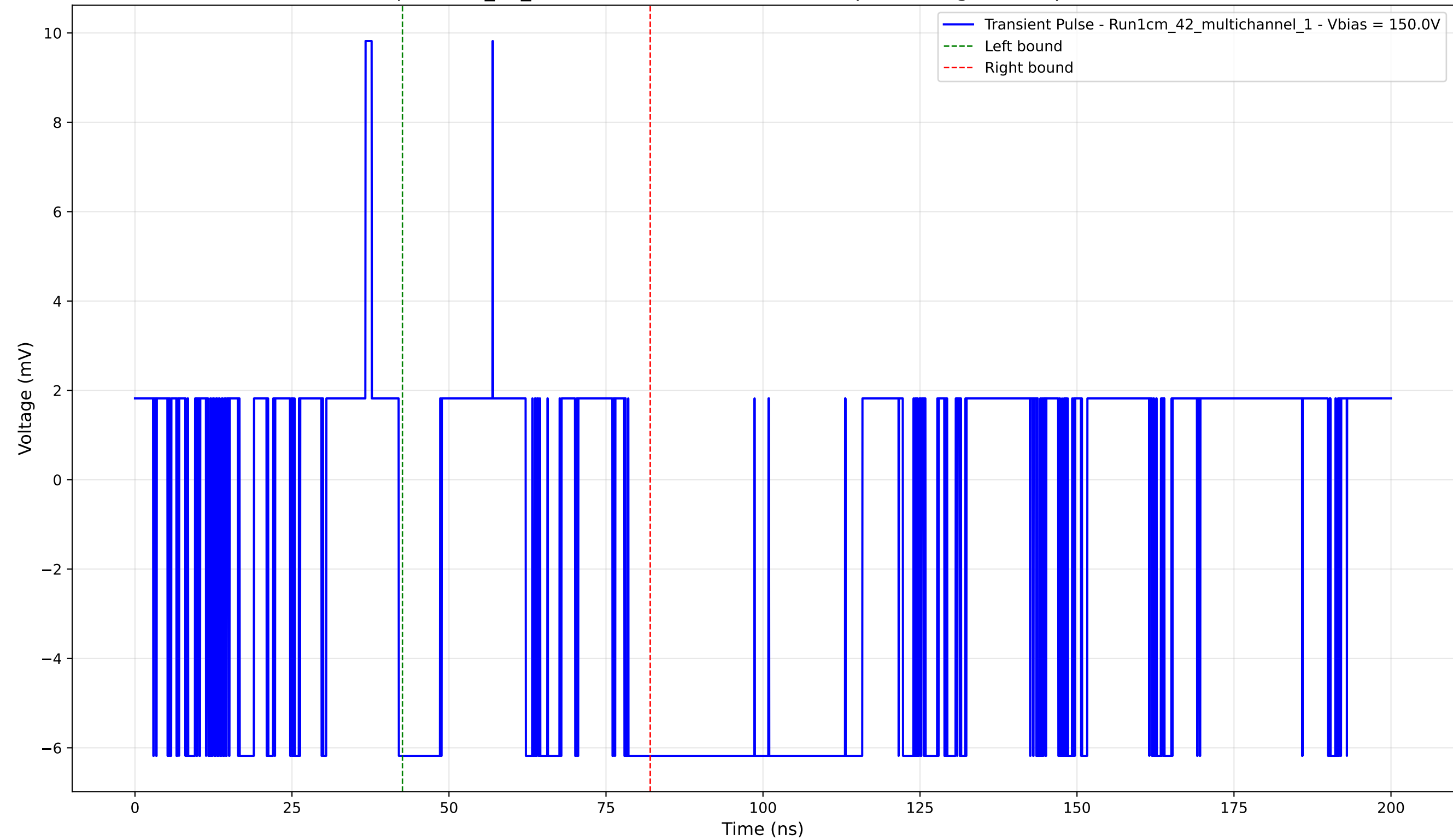
Transient Pulse - Sample: 1cm_42_multichannel - Position: 4425.0 \mu\text{m} - Charge: -1.07 pC - Rise Time: 0.00 ns (N/A)
