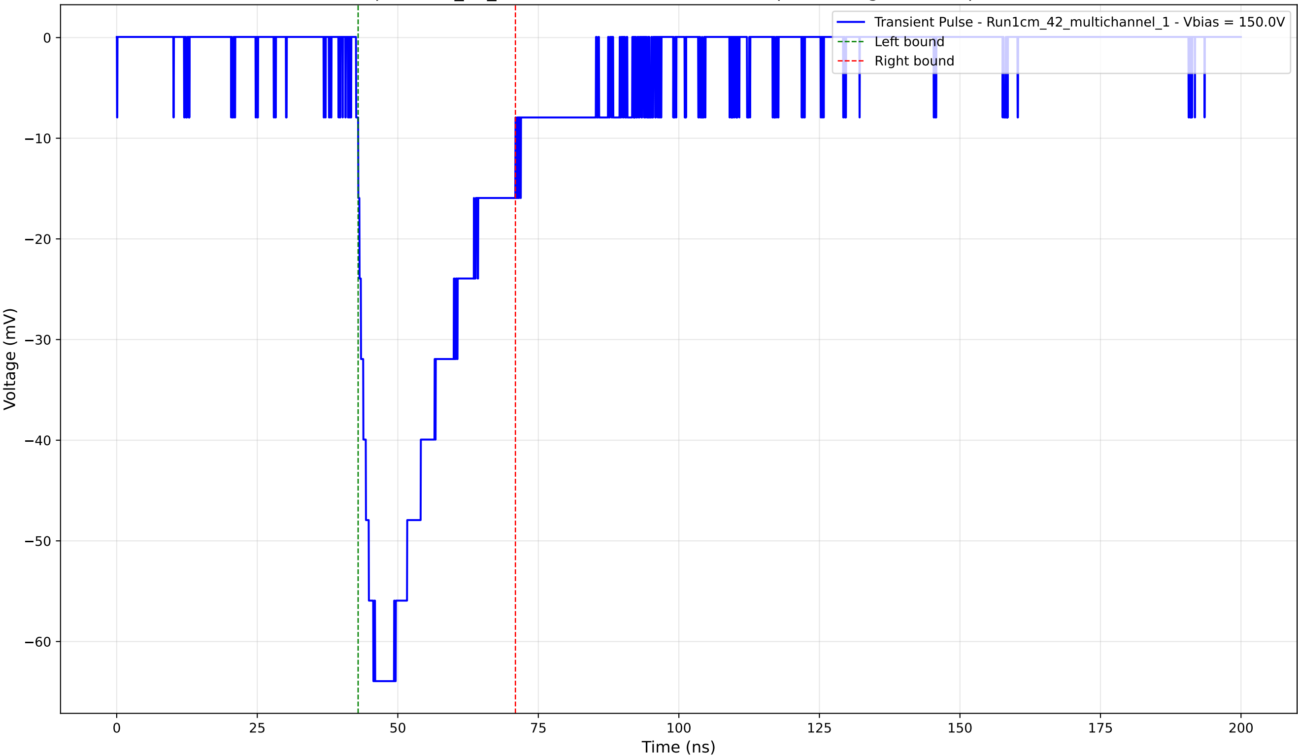
Transient Pulse - Sample: 1cm_42_multichannel - Position: 145.0 \mu\text{m} - Charge: -20.23 pC - Rise Time: 3.06 ns
