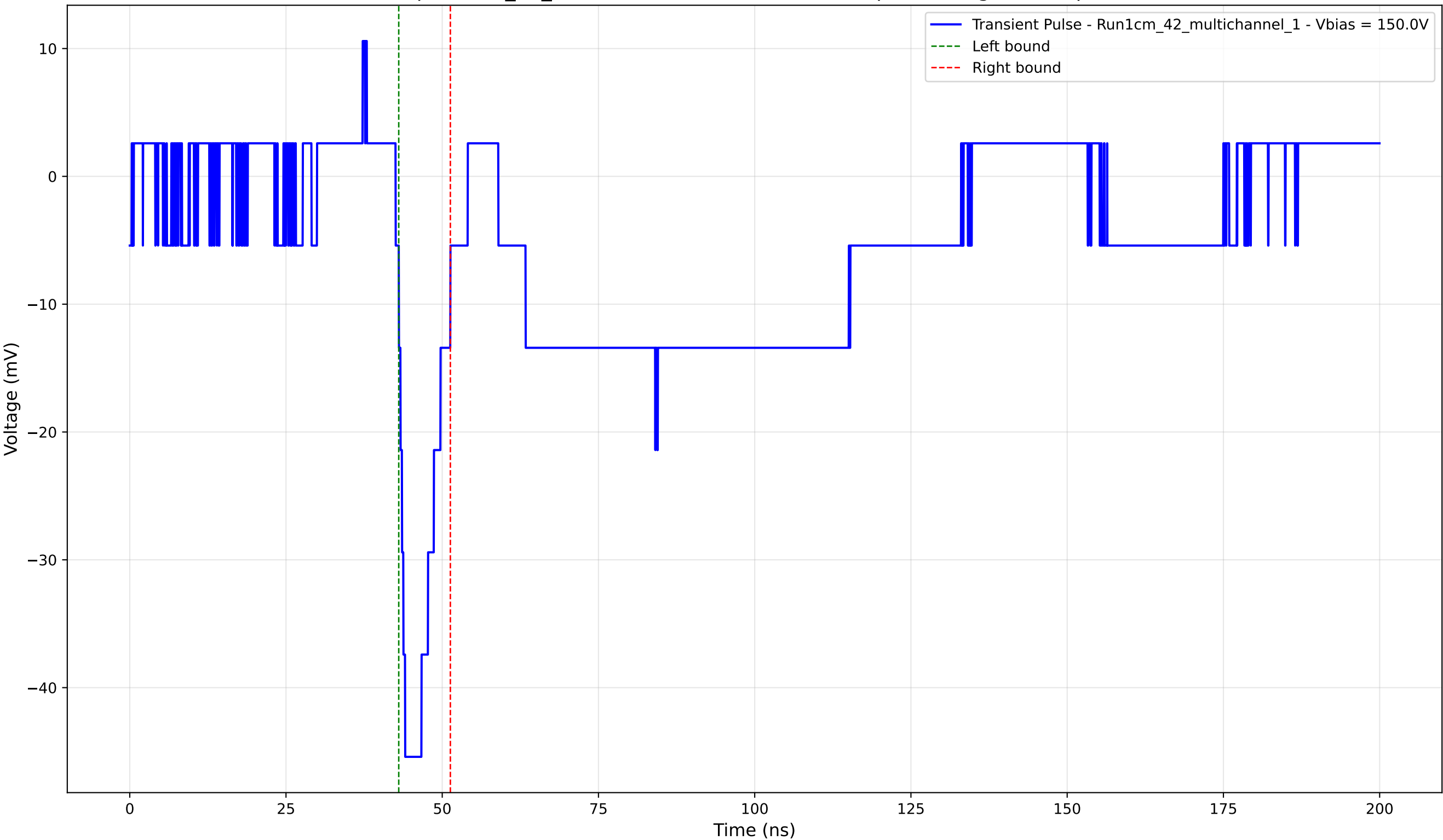
Transient Pulse - Sample: 1cm_42_multichannel - Position: 3985.0 \mu\text{m} - Charge: -5.10 pC - Rise Time: 1.53 ns
