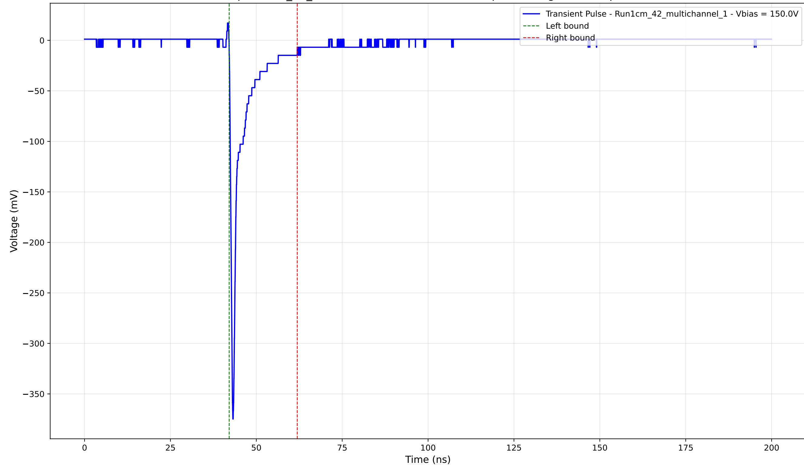
Transient Pulse - Sample: 1cm_42_multichannel - Position: 2220.0 \mu\text{m} - Charge: -24.08 pC - Rise Time: 0.75 ns
