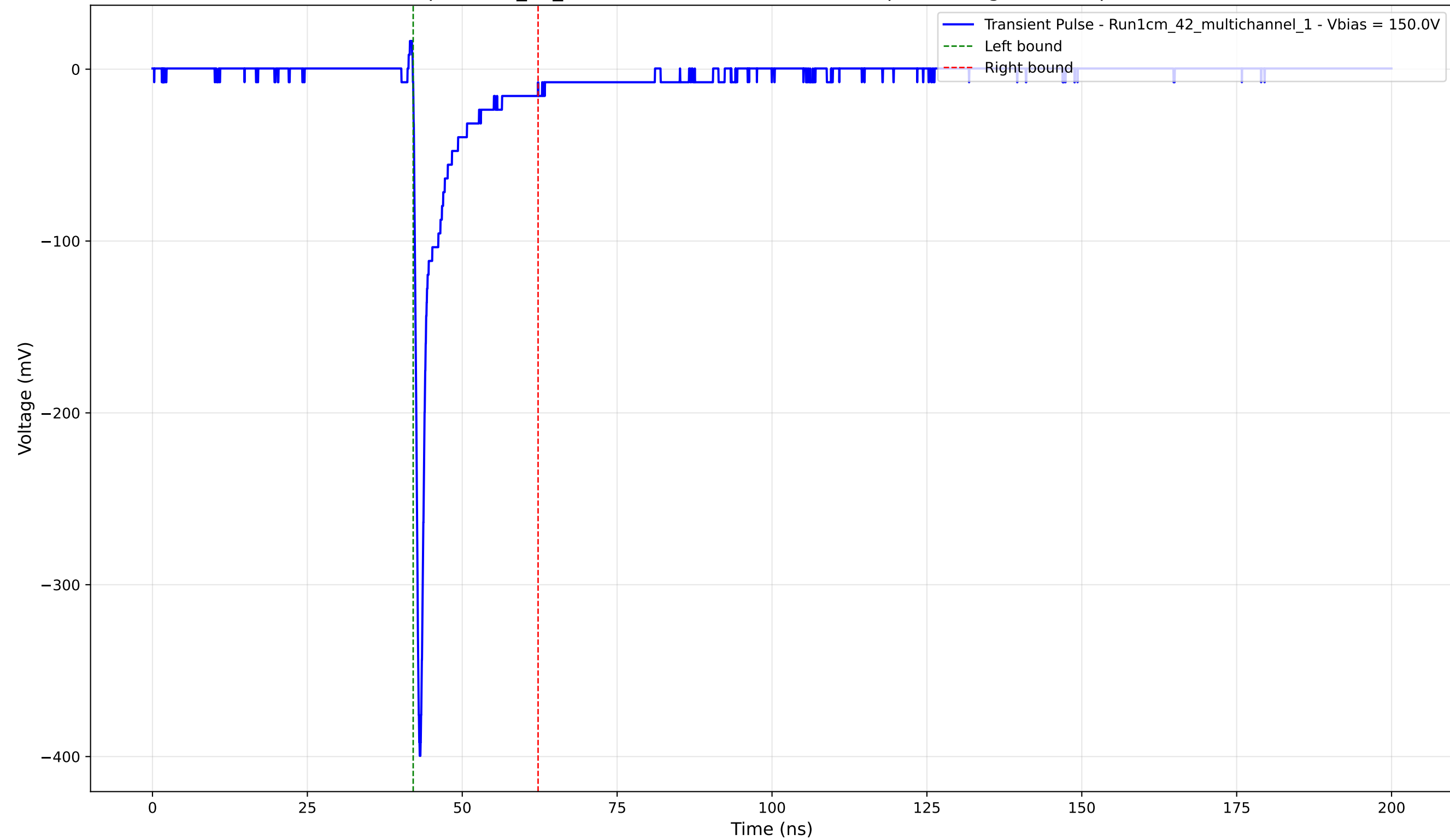
Transient Pulse - Sample: 1cm_42_multichannel - Position: 2270.0 \mu\text{m} - Charge: -24.70 pC - Rise Time: 0.74 ns
