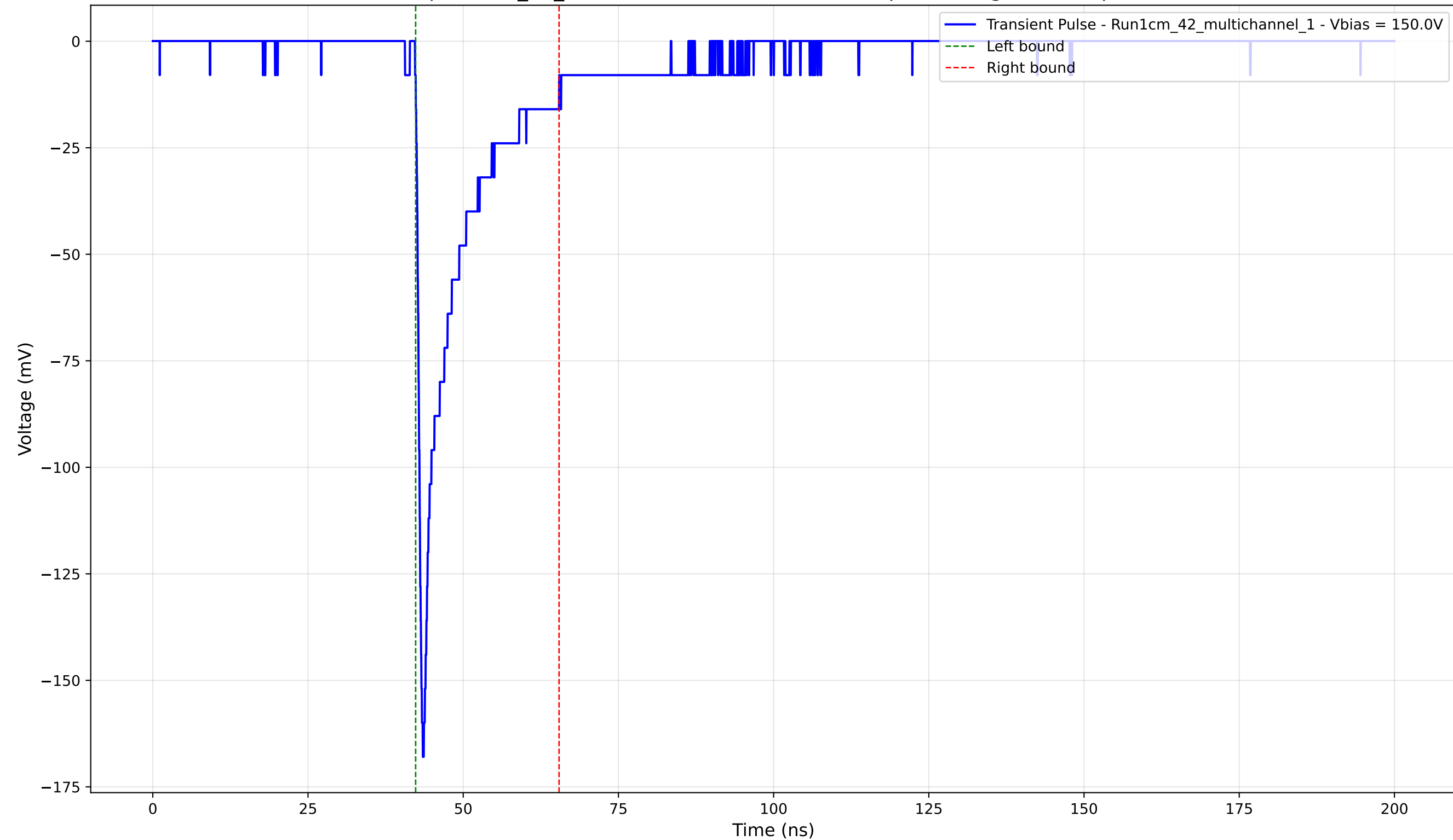
Transient Pulse - Sample: 1cm_42_multichannel - Position: 3010.0 \mu\text{m} - Charge: -20.60 pC - Rise Time: 0.84 ns
