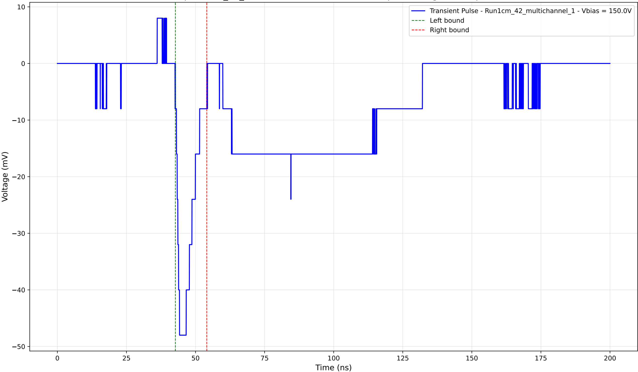
Transient Pulse - Sample: 1cm_42_multichannel - Position: 4035.0 \mu\text{m} - Charge: -6.04 pC - Rise Time: 1.49 ns
