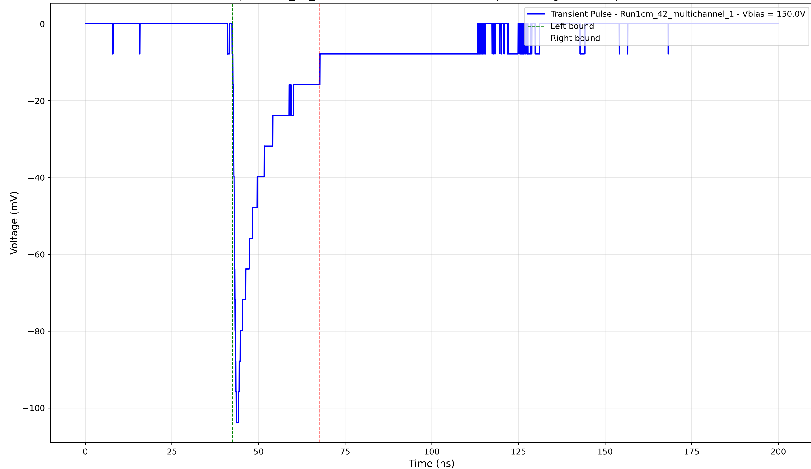
Transient Pulse - Sample: 1cm_42_multichannel - Position: 3285.0 \mu\text{m} - Charge: -17.71 pC - Rise Time: 0.89 ns
