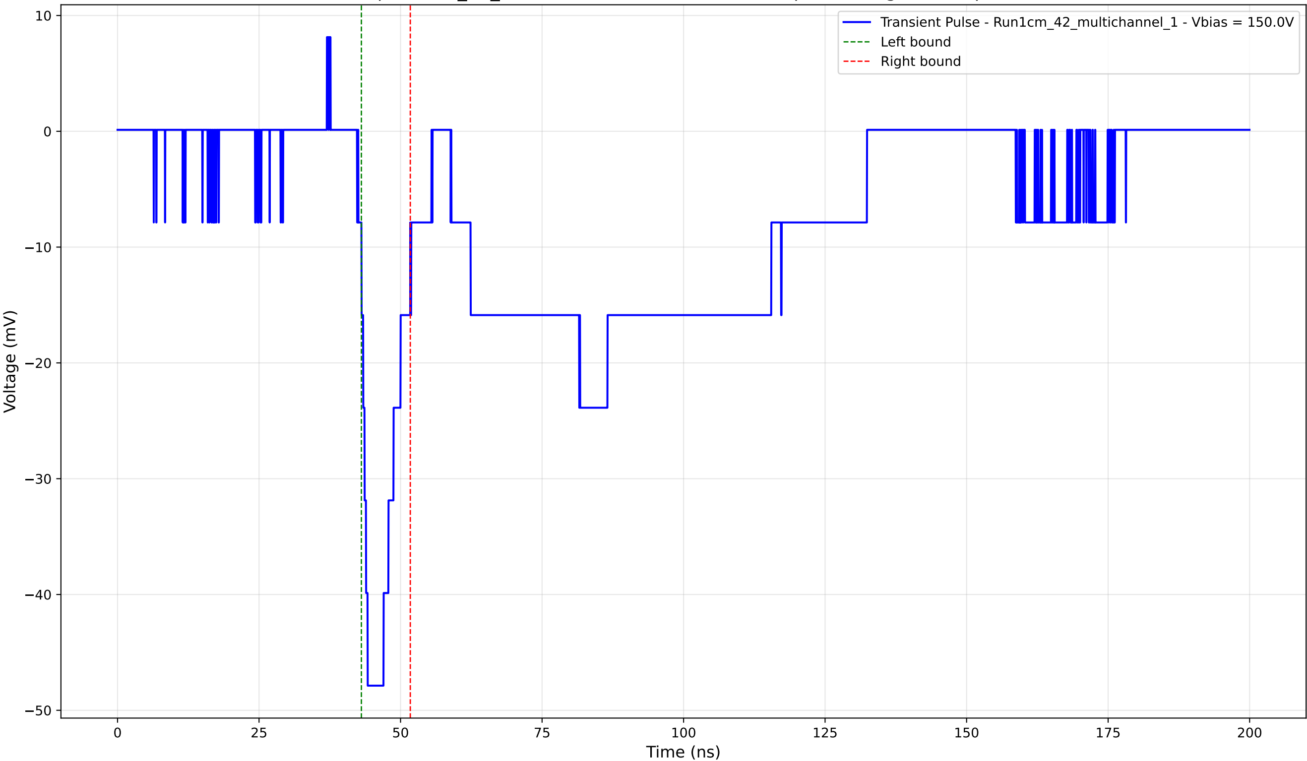
Transient Pulse - Sample: 1cm_42_multichannel - Position: 4080.0 \mu\text{m} - Charge: -5.70 pC - Rise Time: 1.65 ns
