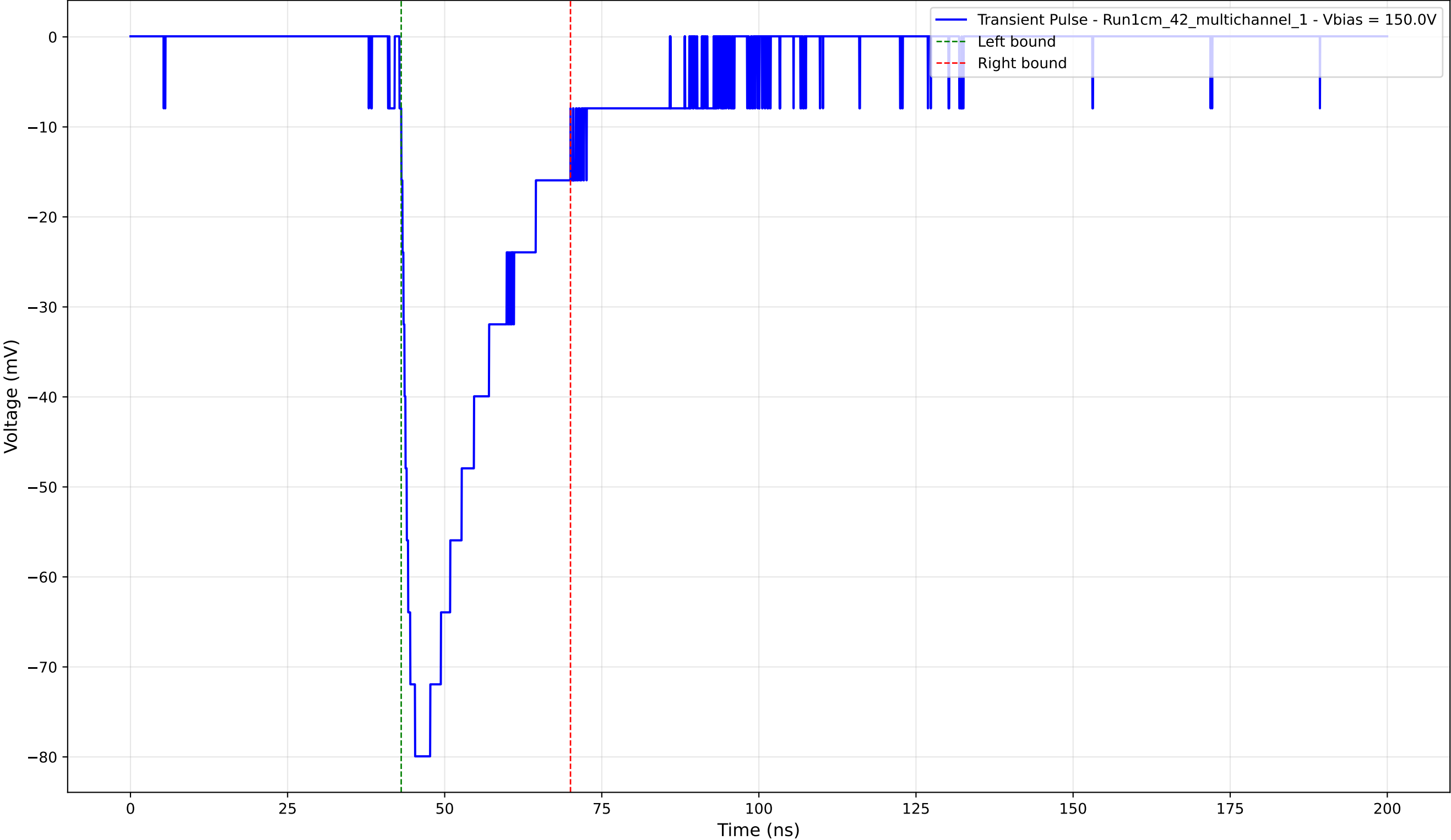
Transient Pulse - Sample: 1cm_42_multichannel - Position: 770.0 \mu\text{m} - Charge: -22.24 pC - Rise Time: 2.20 ns
