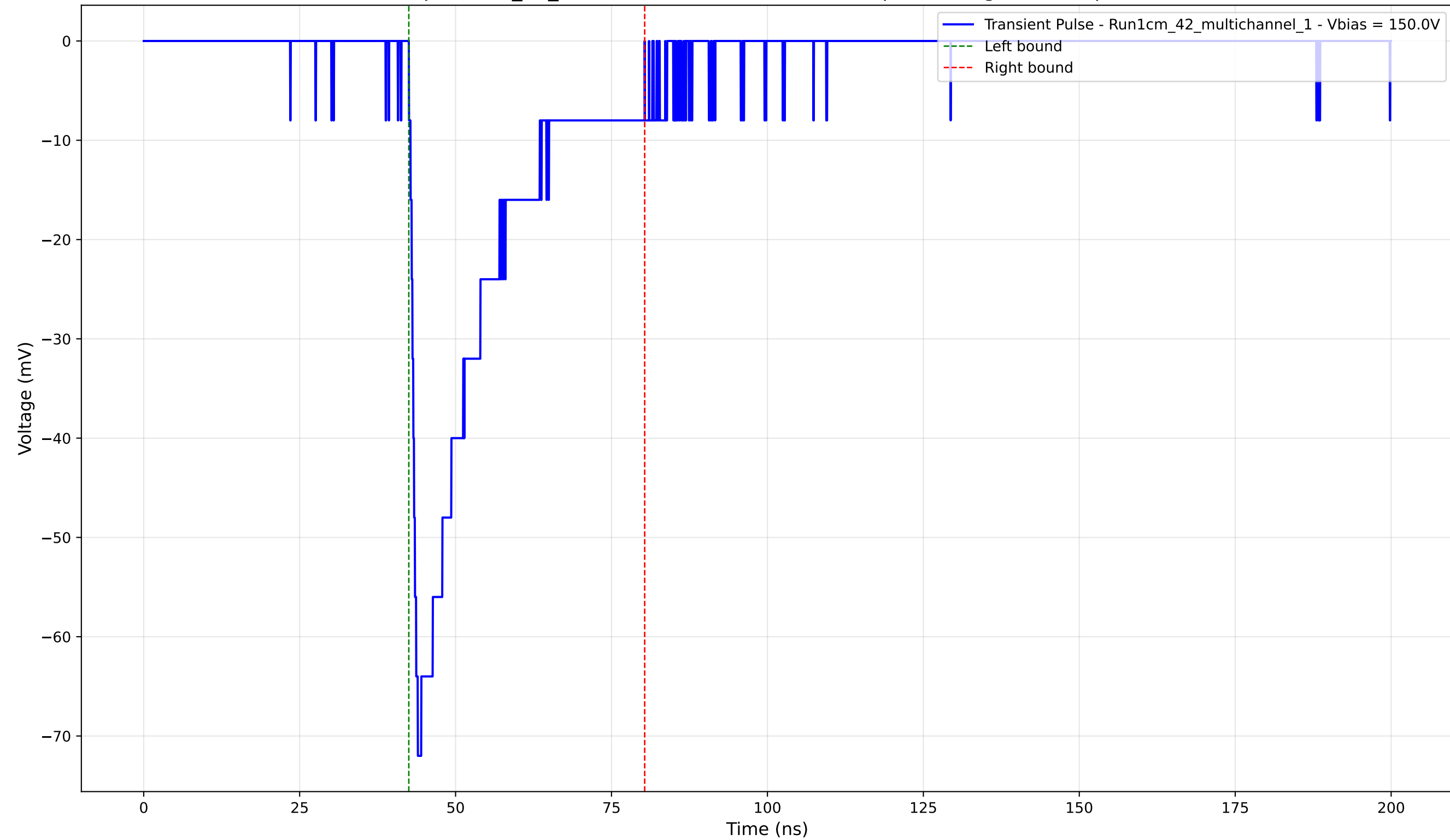
Transient Pulse - Sample: 1cm_42_multichannel - Position: 1315.0 \mu\text{m} - Charge: -16.92 pC - Rise Time: 1.42 ns
