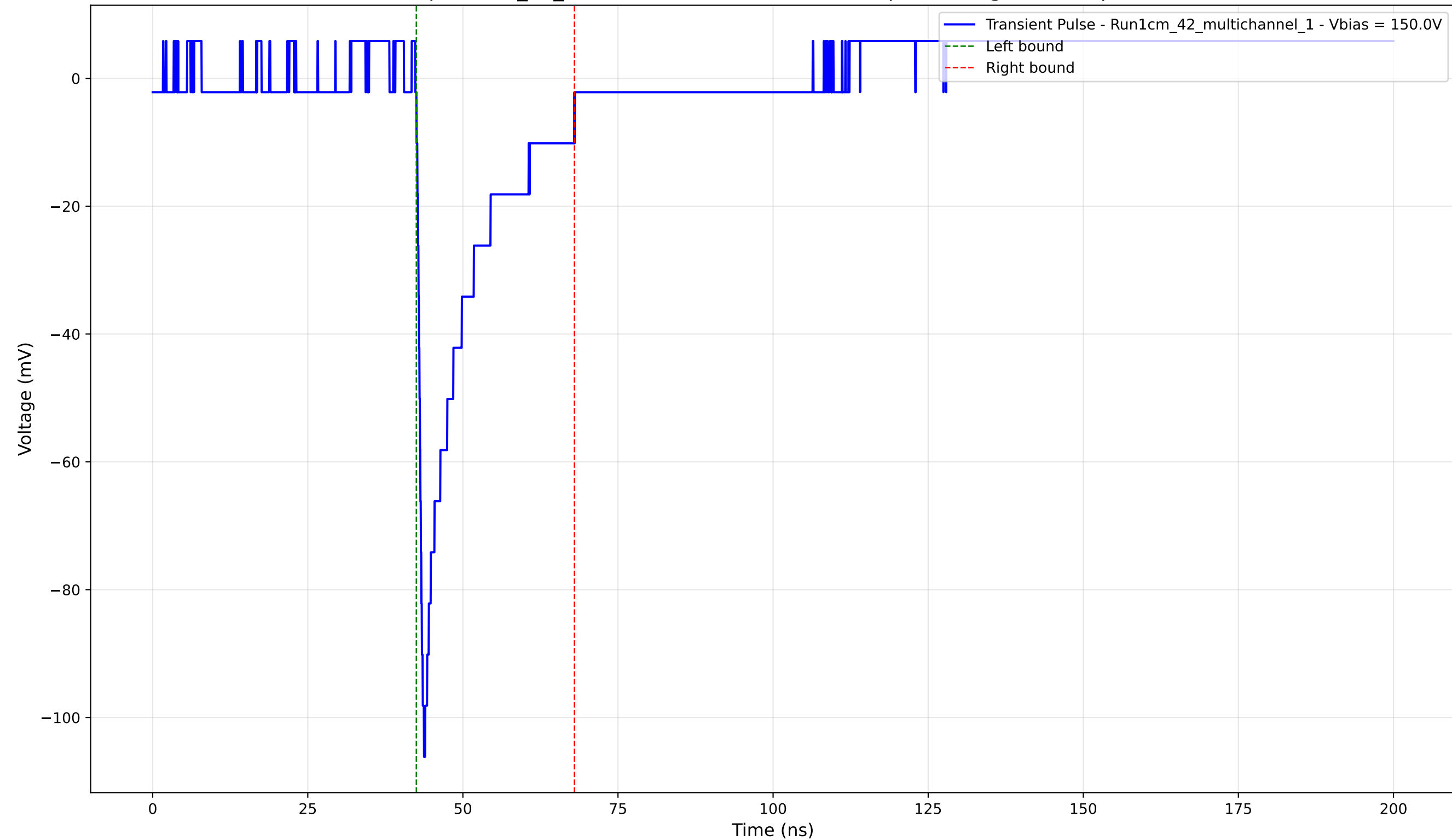
Transient Pulse - Sample: 1cm_42_multichannel - Position: 3275.0 \mu\text{m} - Charge: -15.47 pC - Rise Time: 0.88 ns
