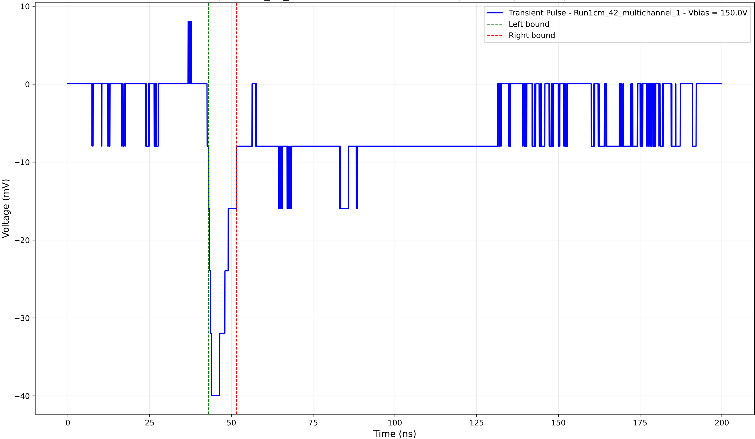
Transient Pulse - Sample: 1cm_42_multichannel - Position: 3845.0 \mu\text{m} - Charge: -4.72 pC - Rise Time: 1.35 ns
