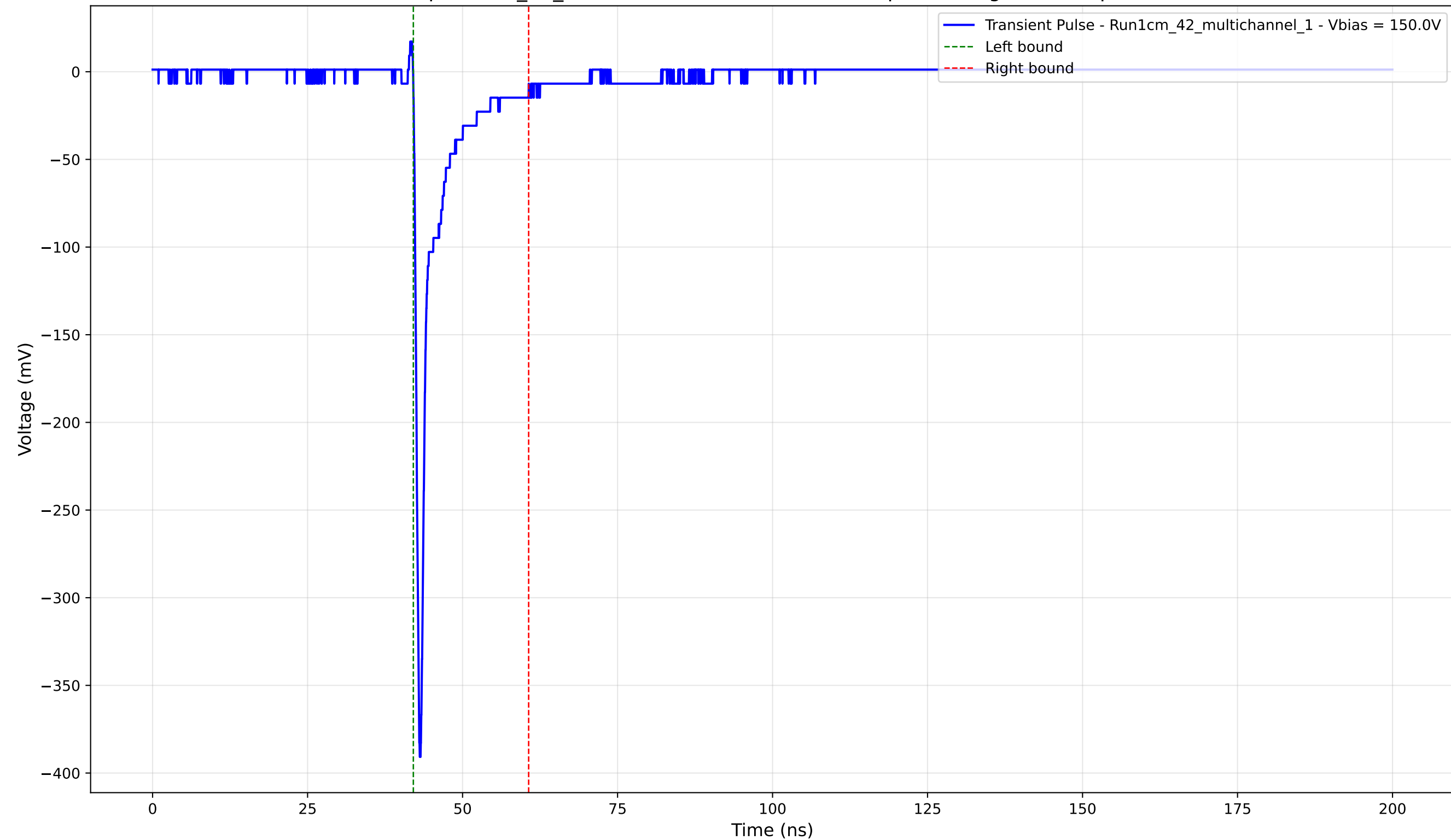
Transient Pulse - Sample: 1cm_42_multichannel - Position: 2305.0 \mu\text{m} - Charge: -22.64 pC - Rise Time: 0.74 ns
