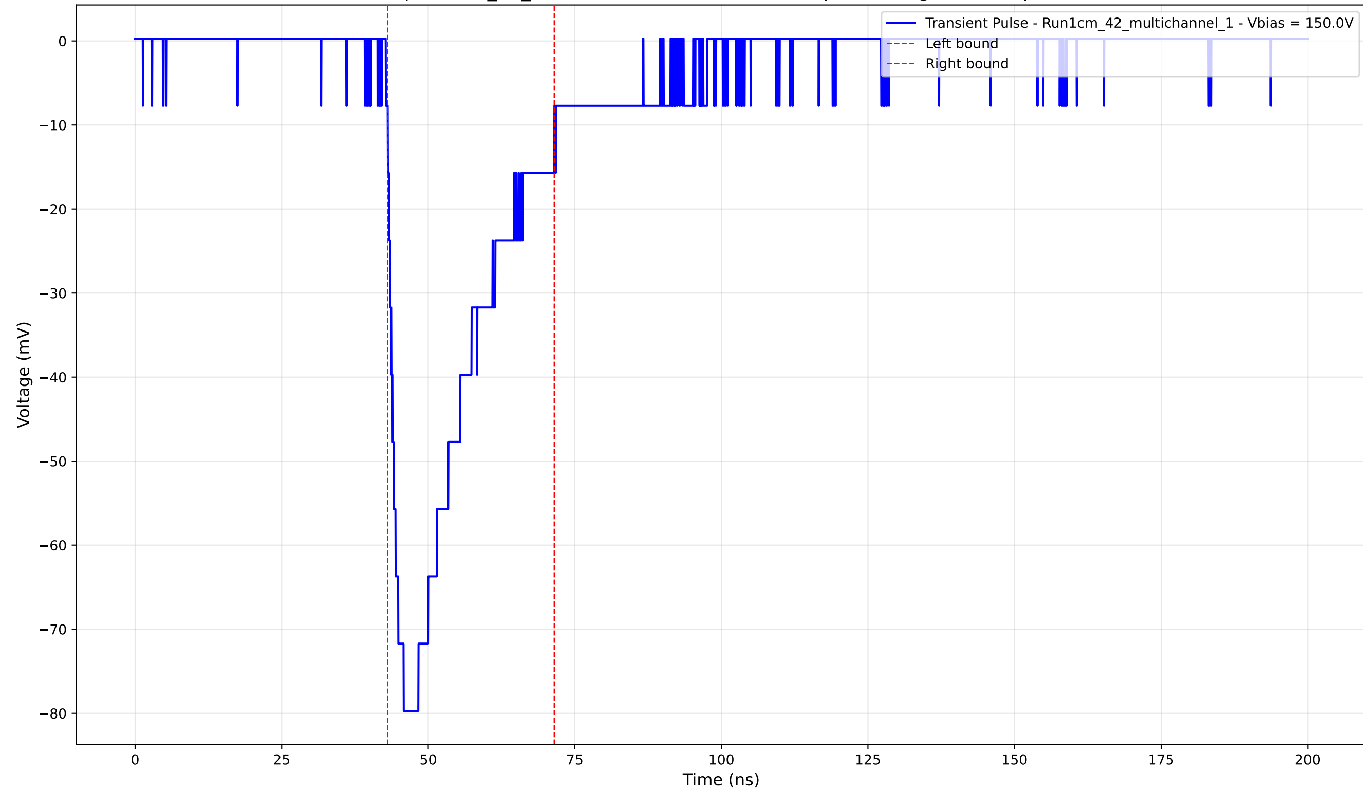
Transient Pulse - Sample: 1cm_42_multichannel - Position: 570.0 \mu\text{m} - Charge: -23.23 pC - Rise Time: 2.72 ns
