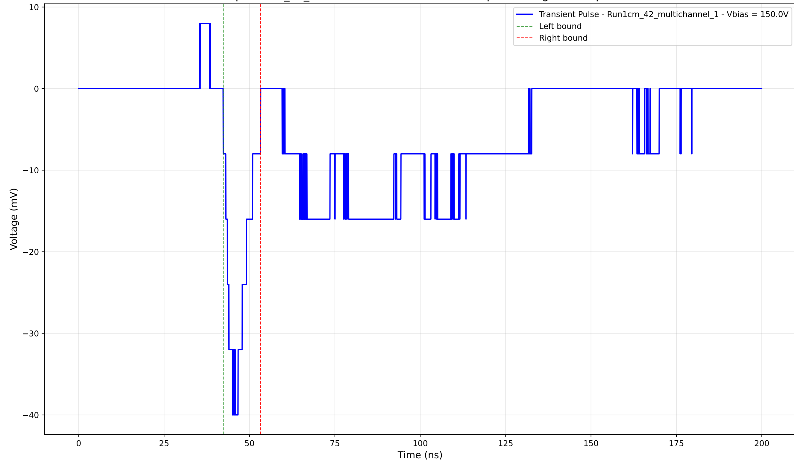
Transient Pulse - Sample: 1cm_42_multichannel - Position: 4820.0 \mu\text{m} - Charge: -4.74 pC - Rise Time: 2.69 ns
