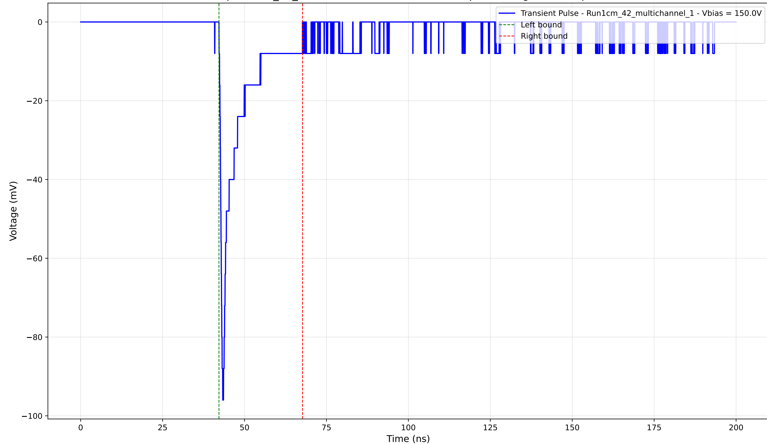
Transient Pulse - Sample: 1cm_42_multichannel - Position: 2845.0 \mu\text{m} - Charge: -10.11 pC - Rise Time: 0.80 ns
