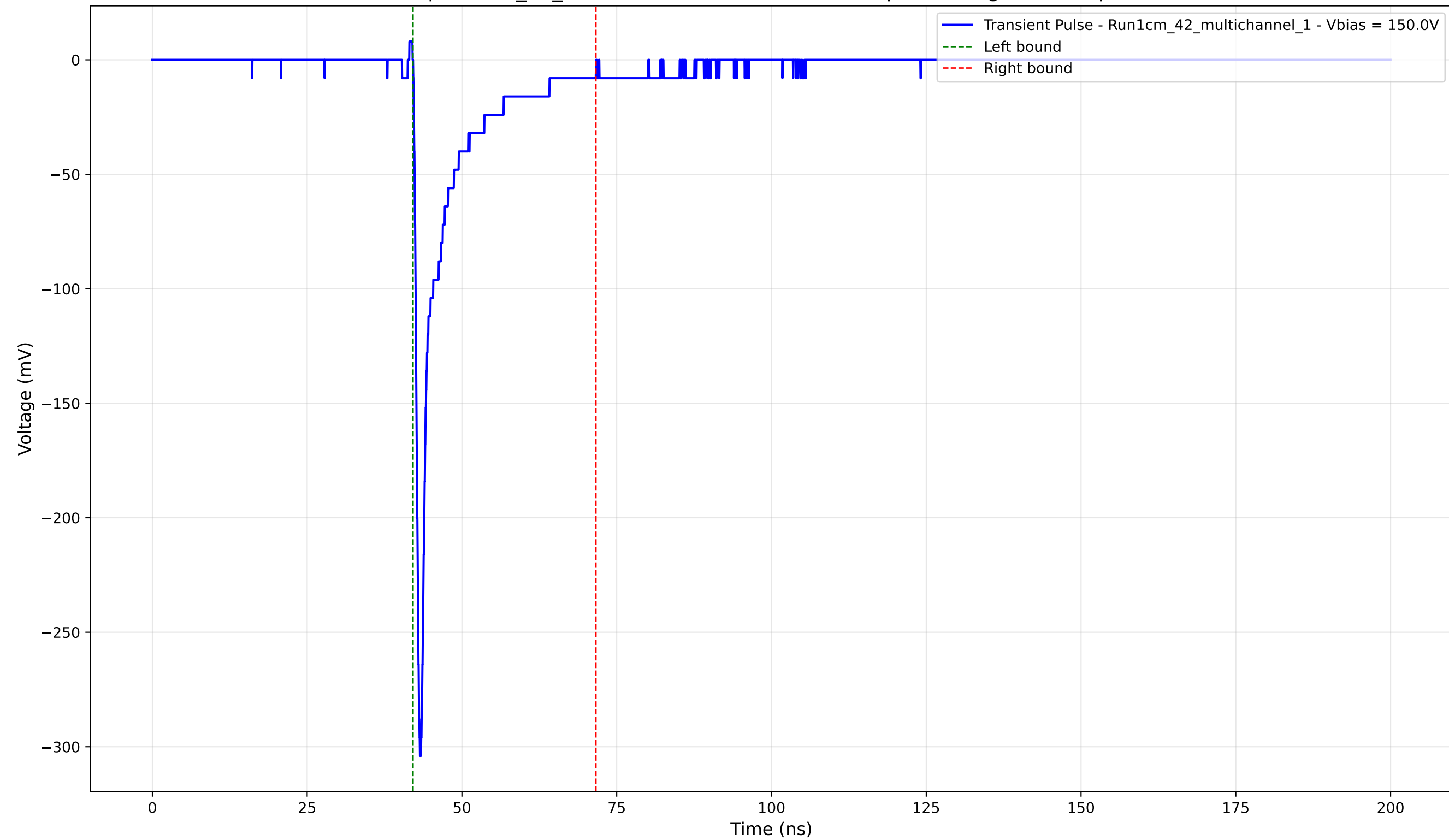
Transient Pulse - Sample: 1cm_42_multichannel - Position: 2650.0 \mu\text{m} - Charge: -24.49 pC - Rise Time: 0.78 ns
