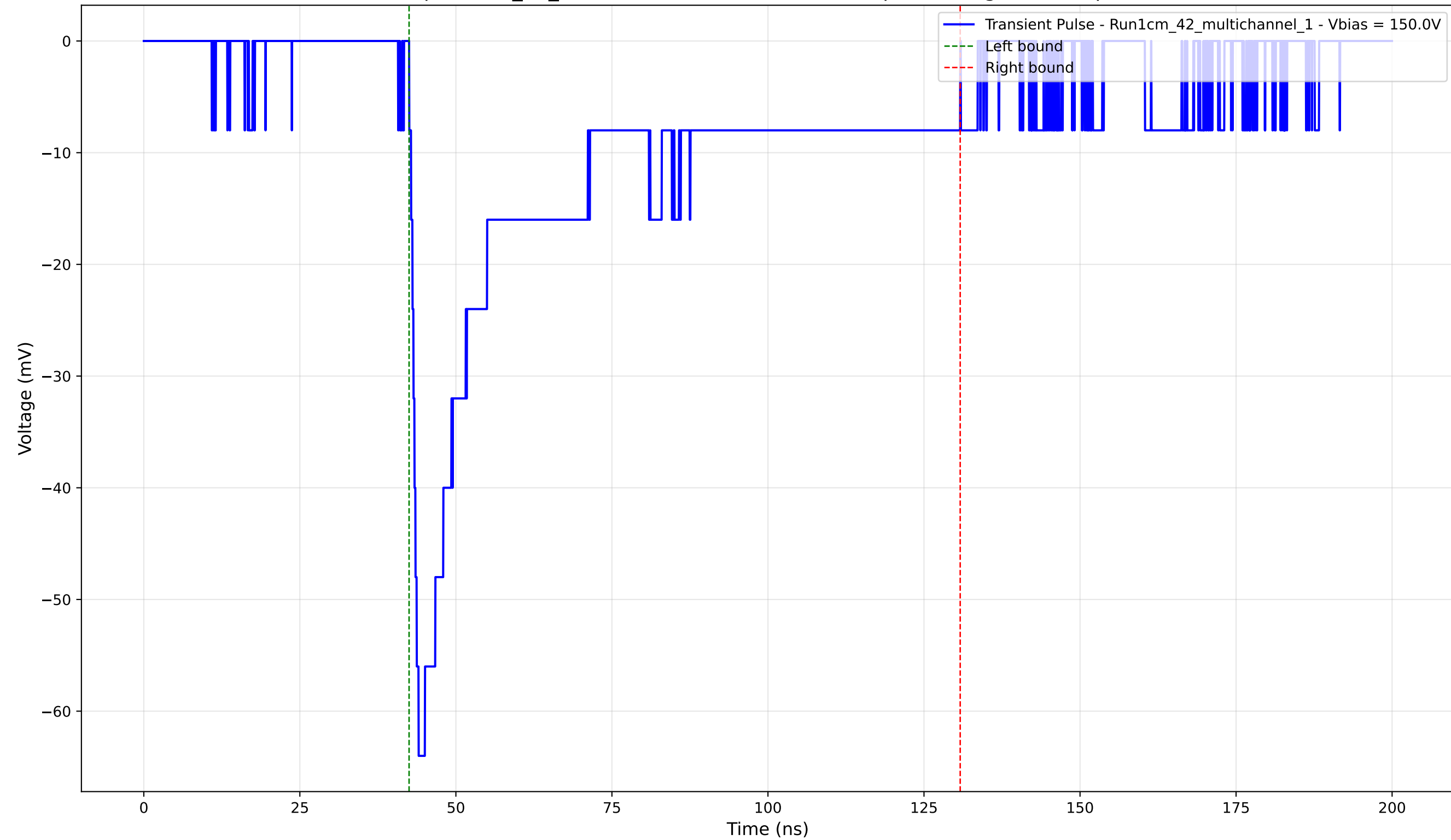
Transient Pulse - Sample: 1cm_42_multichannel - Position: 3670.0 \mu\text{m} - Charge: -24.77 pC - Rise Time: 1.50 ns
