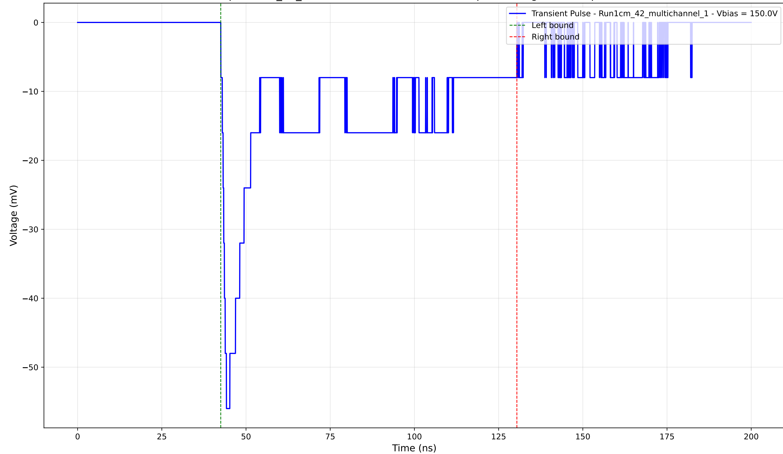
Transient Pulse - Sample: 1cm_42_multichannel - Position: 3825.0 \mu\text{m} - Charge: -25.06 pC - Rise Time: 1.67 ns
