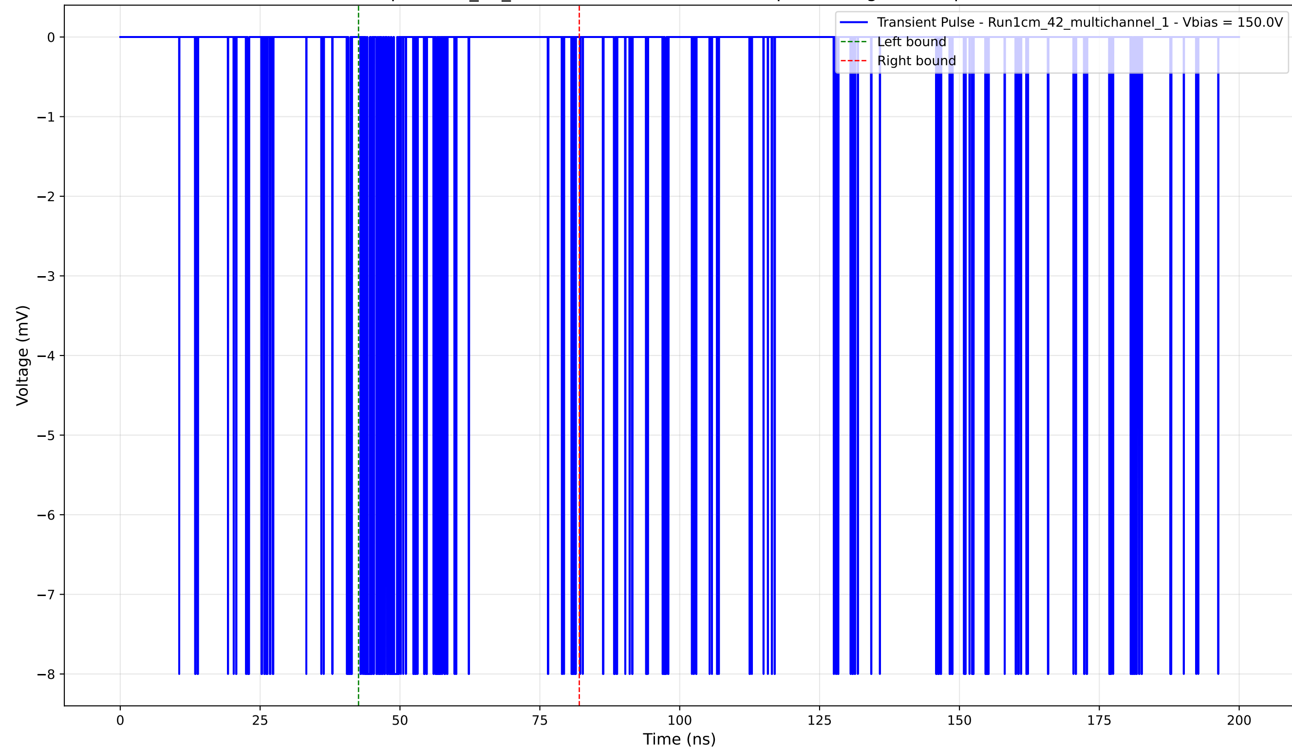
Transient Pulse - Sample: 1cm_42_multichannel - Position: 10.0 \mu\text{m} - Charge: -1.00 pC - Rise Time: 0.02 ns
