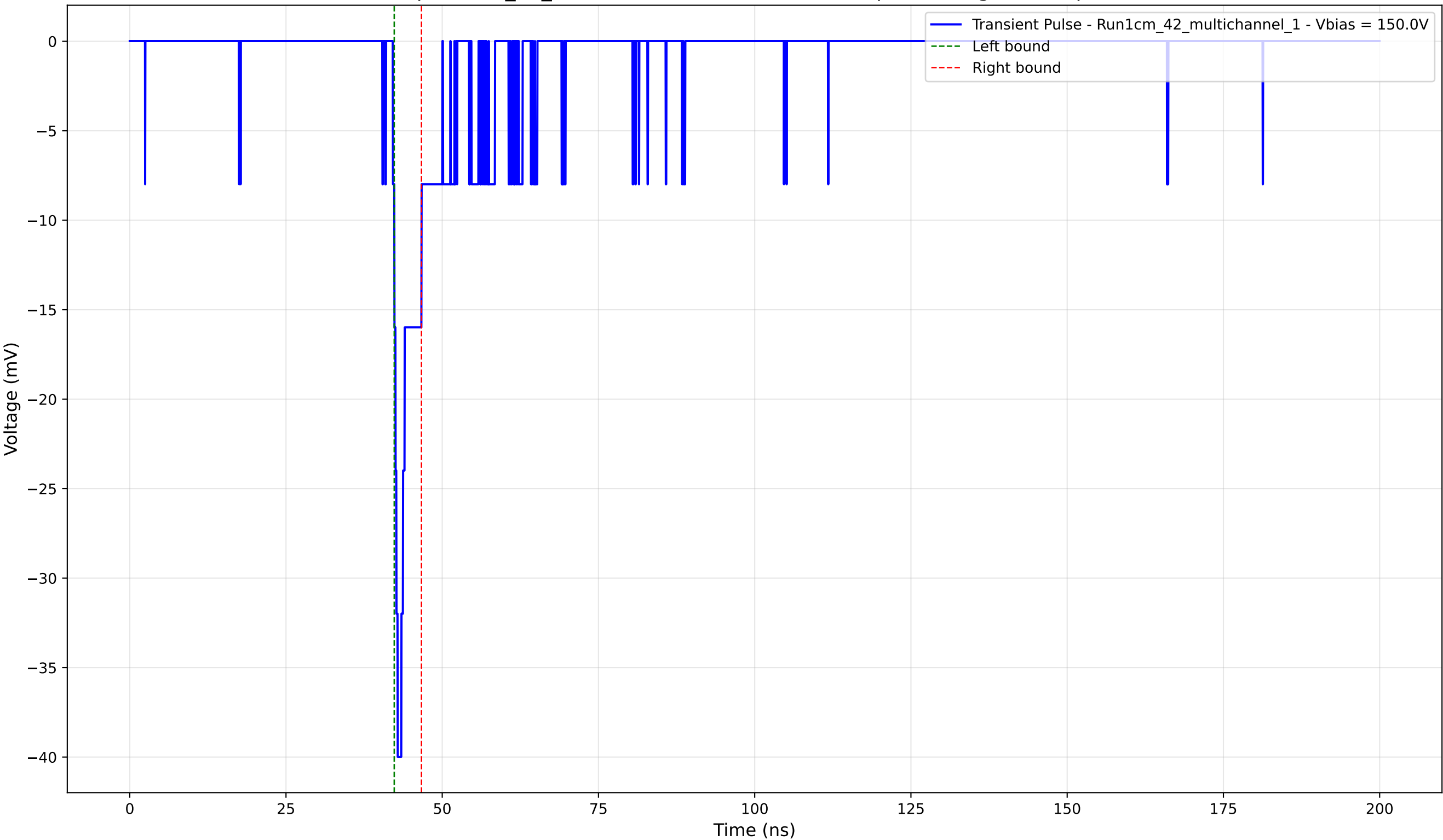
Transient Pulse - Sample: 1cm_42_multichannel - Position: 2415.0 \mu\text{m} - Charge: -1.89 pC - Rise Time: 0.77 ns
