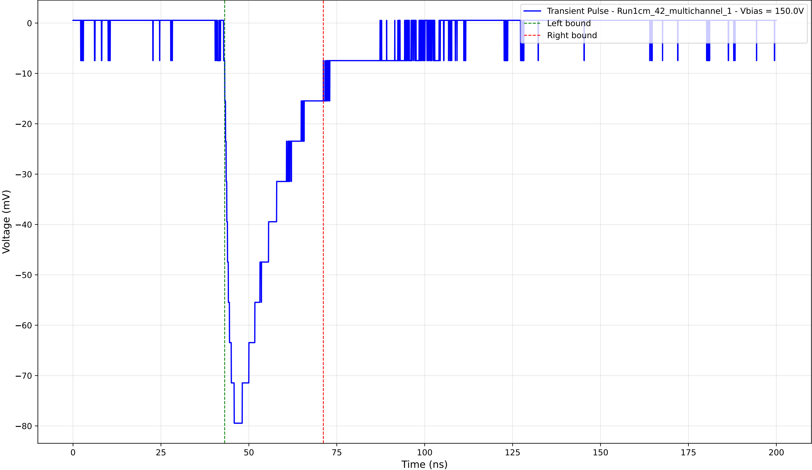
Transient Pulse - Sample: 1cm_42_multichannel - Position: 555.0 \mu\text{m} - Charge: -22.94 pC - Rise Time: 2.70 ns
