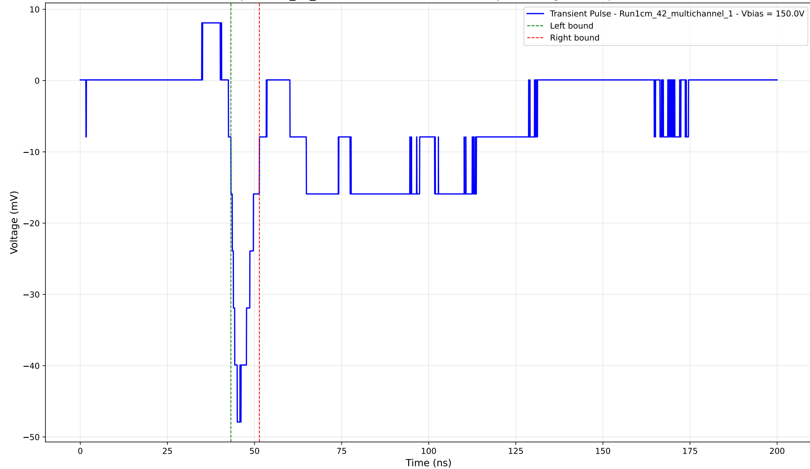
Transient Pulse - Sample: 1cm_42_multichannel - Position: 4595.0 \mu\text{m} - Charge: -5.03 pC - Rise Time: 2.53 ns
