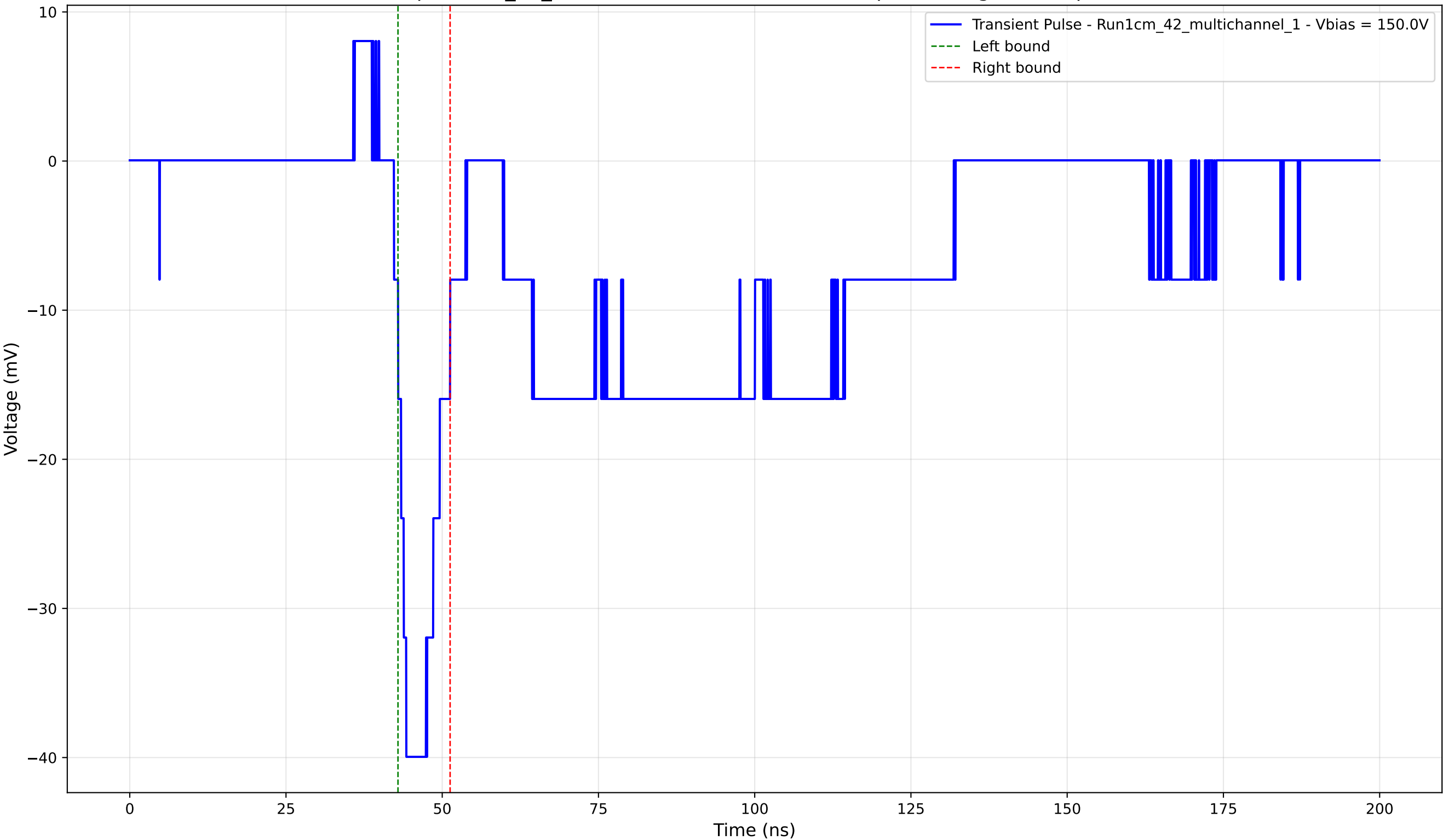
Transient Pulse - Sample: 1cm_42_multichannel - Position: 4745.0 \mu\text{m} - Charge: -4.91 pC - Rise Time: 1.97 ns
