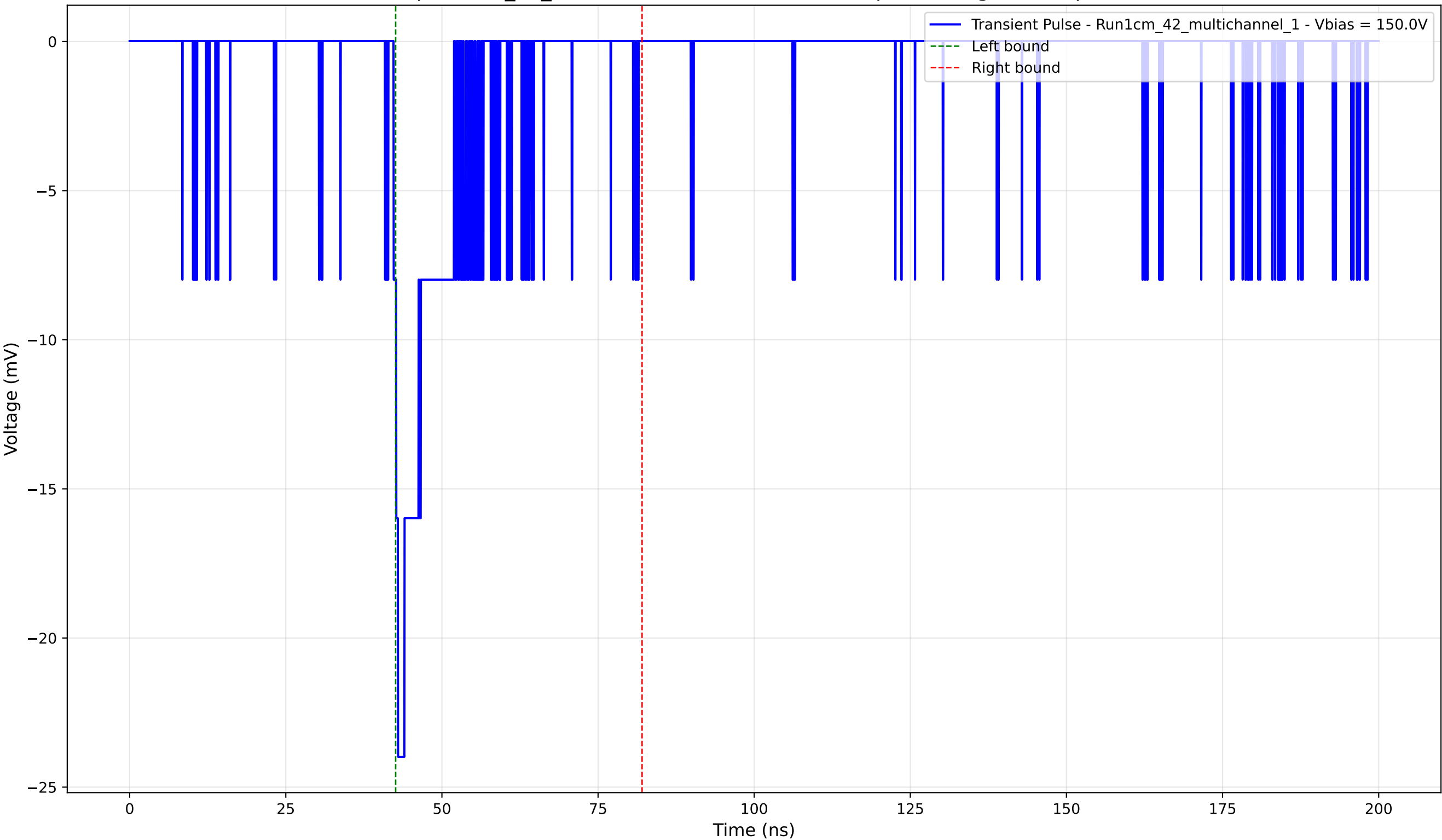
Transient Pulse - Sample: 1cm_42_multichannel - Position: 2865.0 \mu\text{m} - Charge: -3.14 pC - Rise Time: 0.71 ns
