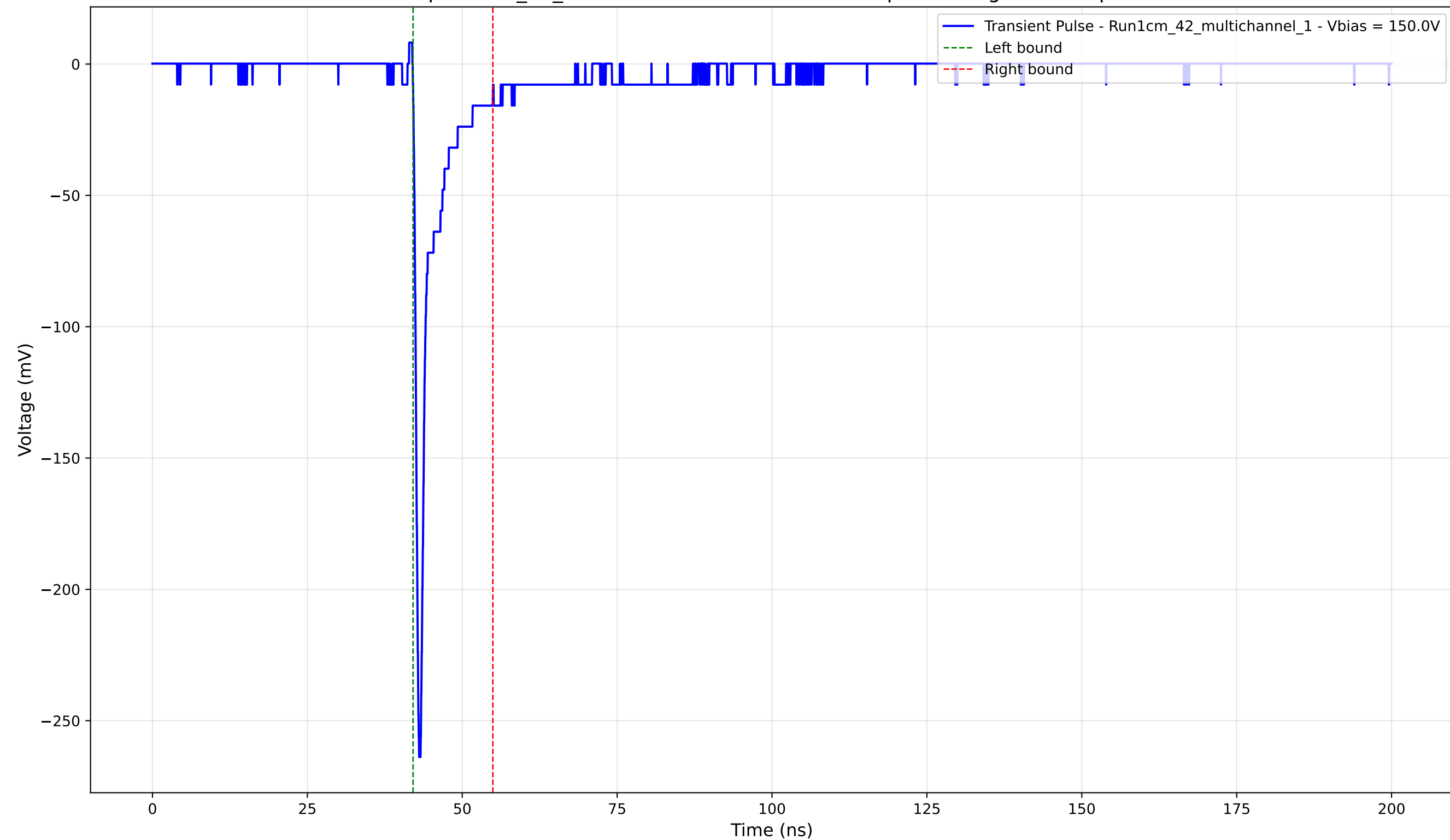
Transient Pulse - Sample: 1cm_42_multichannel - Position: 2445.0 \mu\text{m} - Charge: -14.43 pC - Rise Time: 0.71 ns
