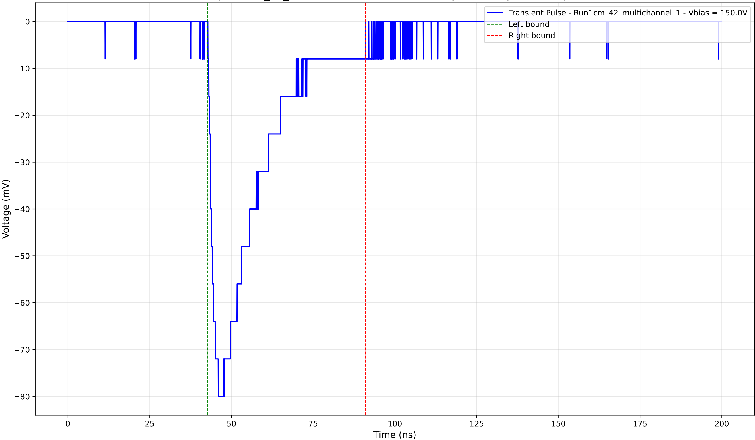
Transient Pulse - Sample: 1cm_42_multichannel - Position: 495.0 \mu\text{m} - Charge: -26.33 pC - Rise Time: 1.96 ns
