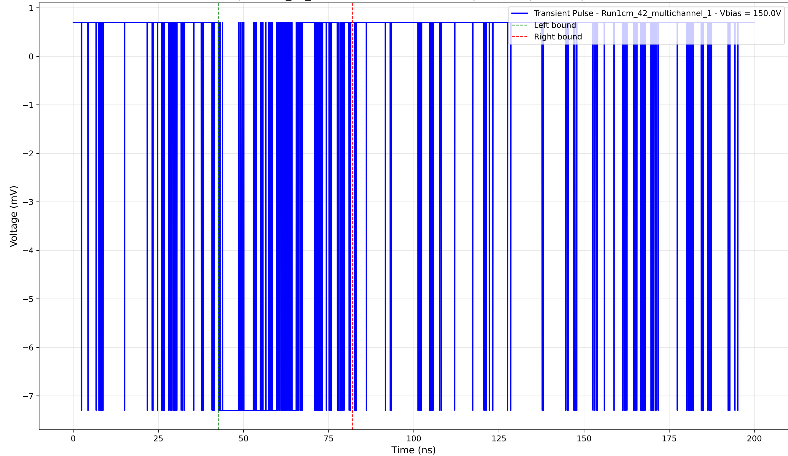
Transient Pulse - Sample: 1cm_42_multichannel - Position: 55.0 \mu\text{m} - Charge: -2.88 pC - Rise Time: 0.02 ns
