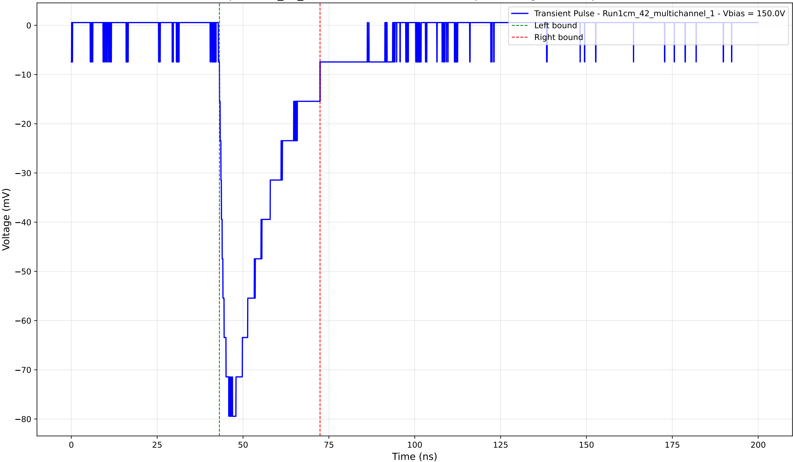
Transient Pulse - Sample: 1cm_42_multichannel - Position: 565.0 \mu\text{m} - Charge: -23.14 pC - Rise Time: 2.74 ns
