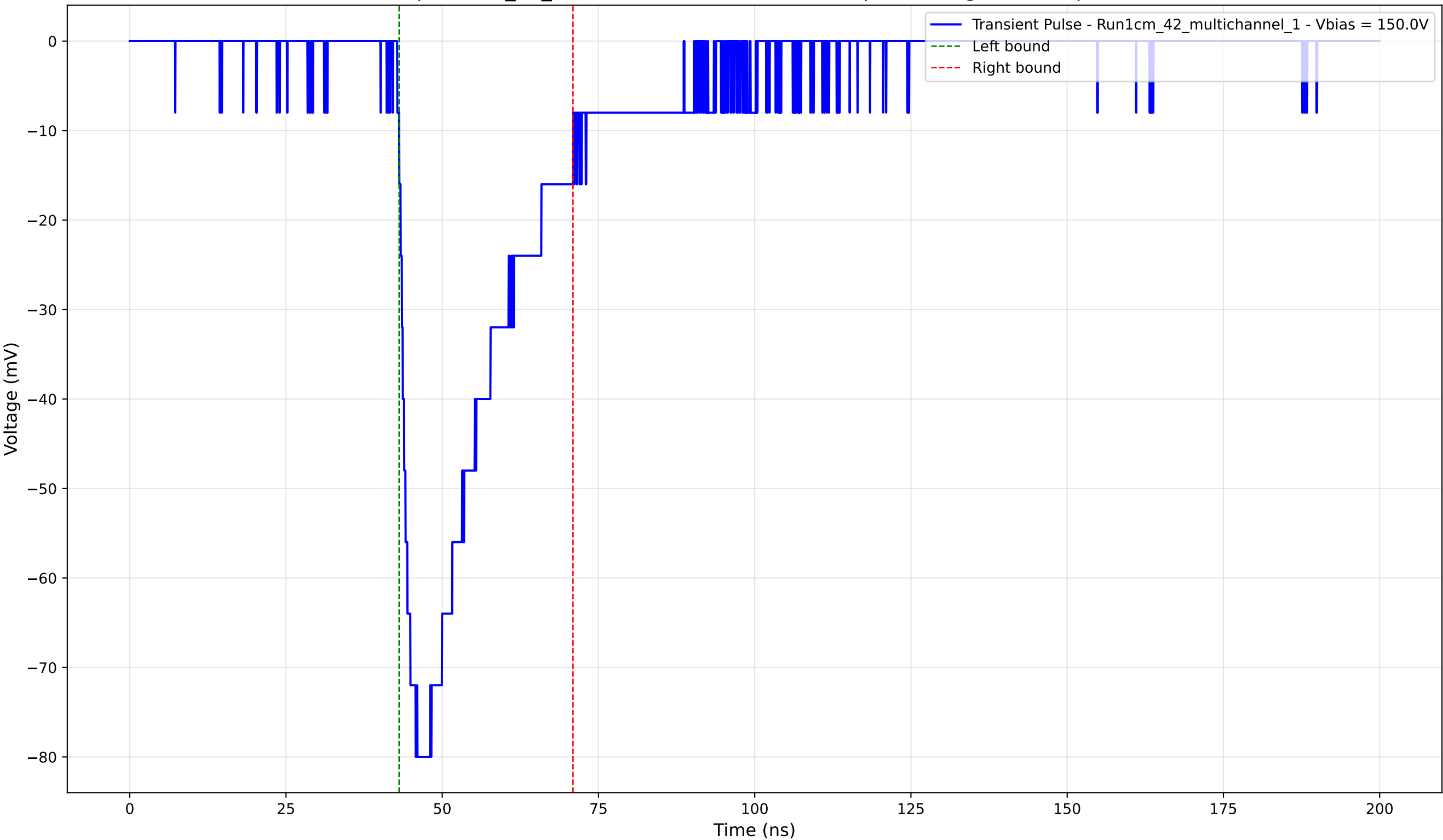
Transient Pulse - Sample: 1cm_42_multichannel - Position: 575.0 \mu\text{m} - Charge: -23.19 pC - Rise Time: 2.64 ns
