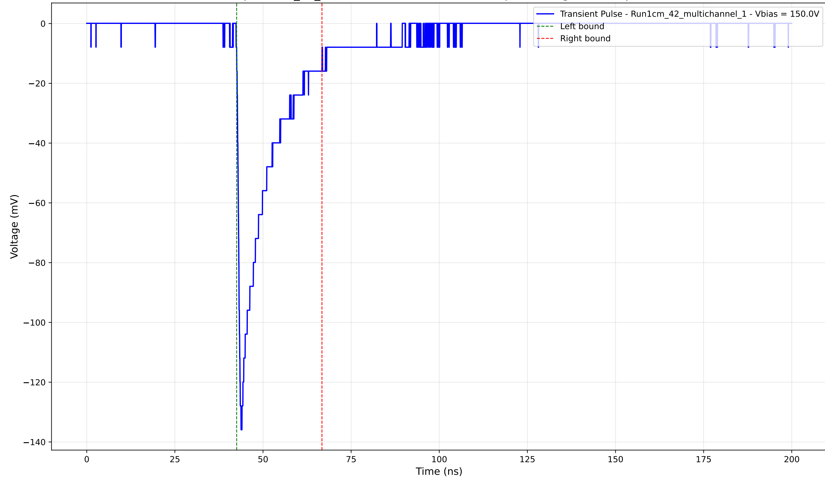
Transient Pulse - Sample: 1cm_42_multichannel - Position: 1535.0 \mu\text{m} - Charge: -22.83 pC - Rise Time: 1.01 ns
