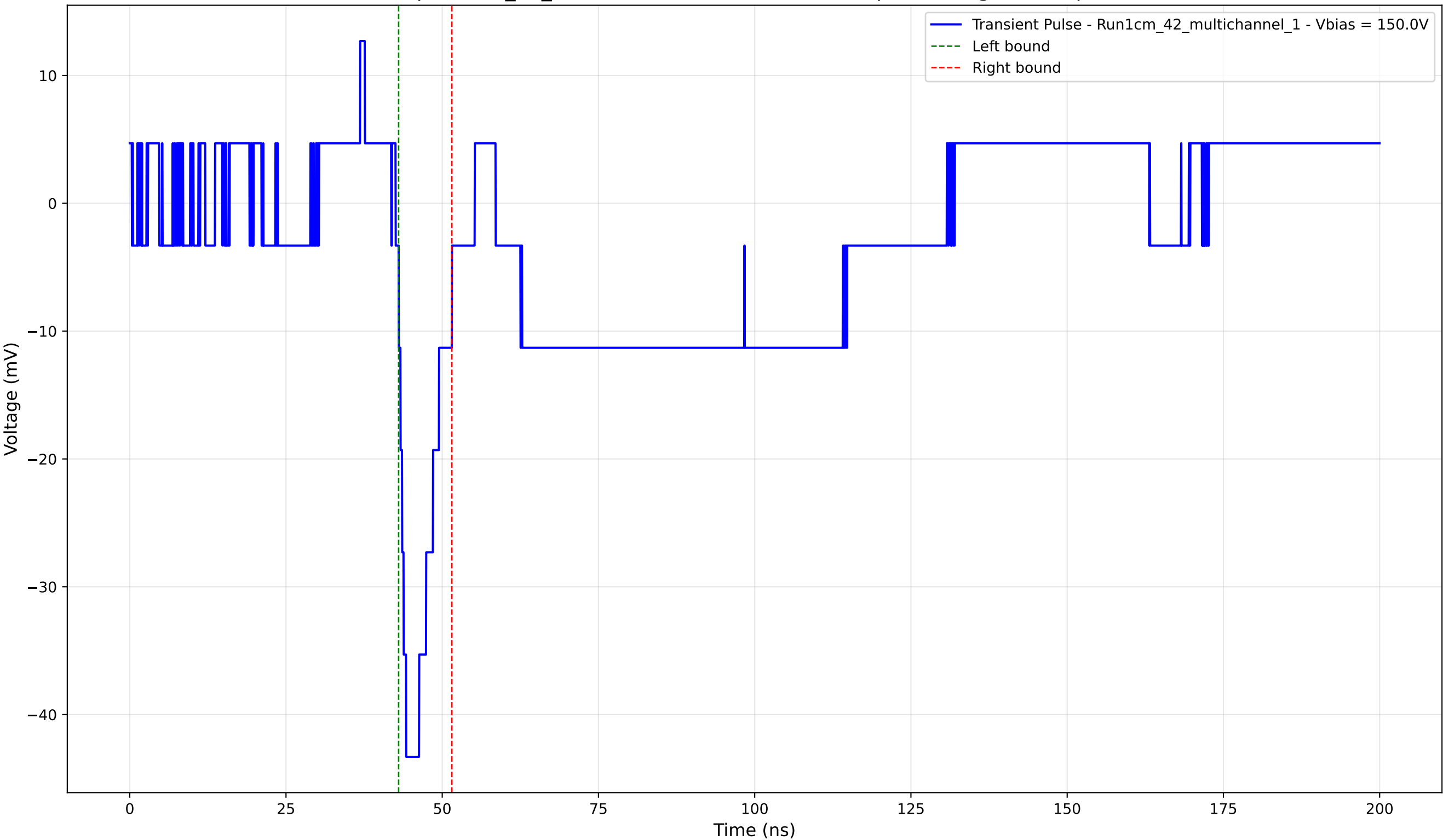
Transient Pulse - Sample: 1cm_42_multichannel - Position: 3975.0 \mu\text{m} - Charge: -4.61 pC - Rise Time: 1.20 ns
