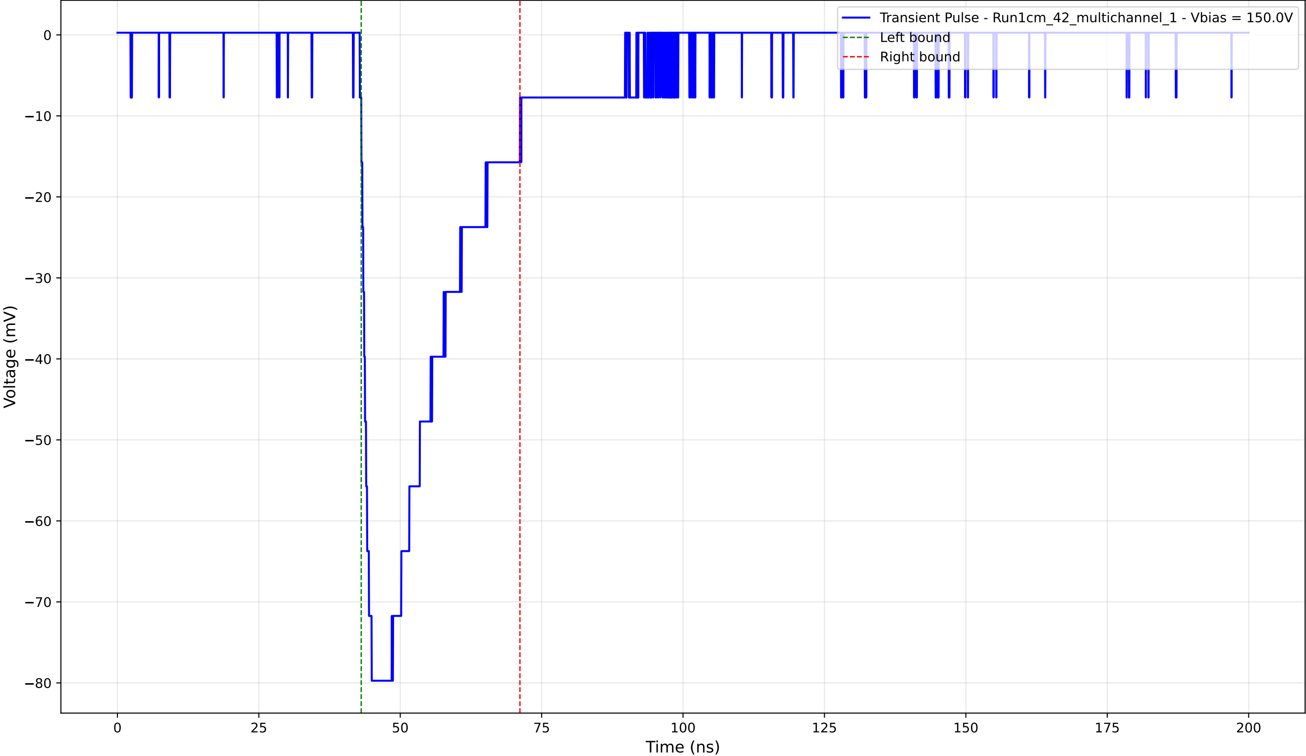
Transient Pulse - Sample: 1cm_42_multichannel - Position: 720.0 \mu\text{m} - Charge: -23.49 pC - Rise Time: 1.84 ns
