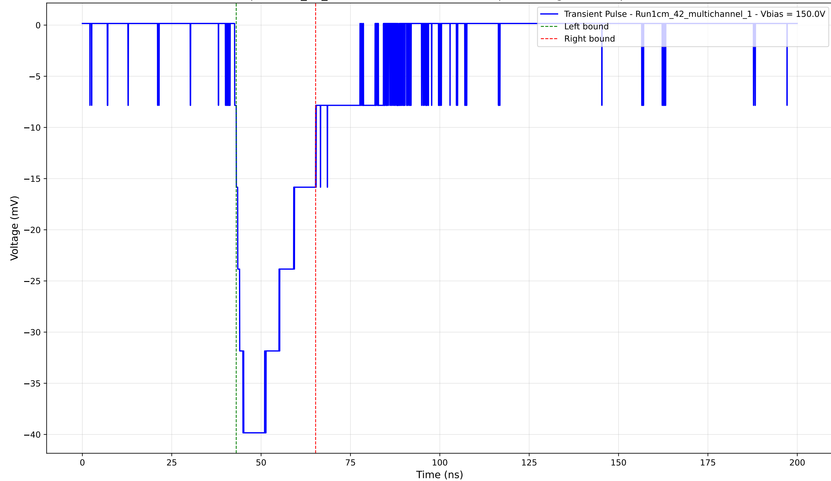
Transient Pulse - Sample: 1cm_42_multichannel - Position: 95.0 \mu\text{m} - Charge: -12.33 pC - Rise Time: 2.33 ns
