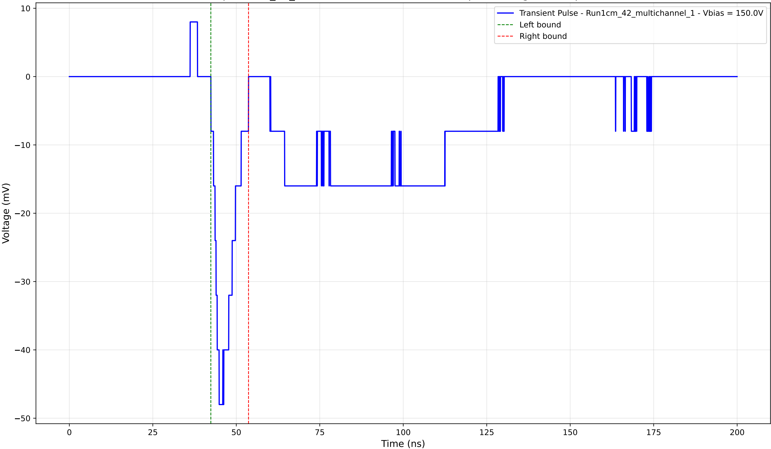
Transient Pulse - Sample: 1cm_42_multichannel - Position: 4515.0 \mu\text{m} - Charge: -5.64 pC - Rise Time: 2.47 ns
