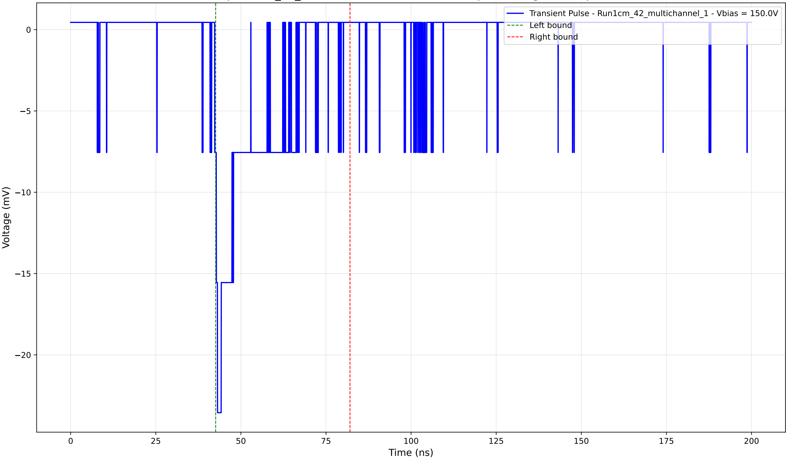
Transient Pulse - Sample: 1cm_42_multichannel - Position: 2925.0 \mu\text{m} - Charge: -4.35 pC - Rise Time: 0.83 ns
