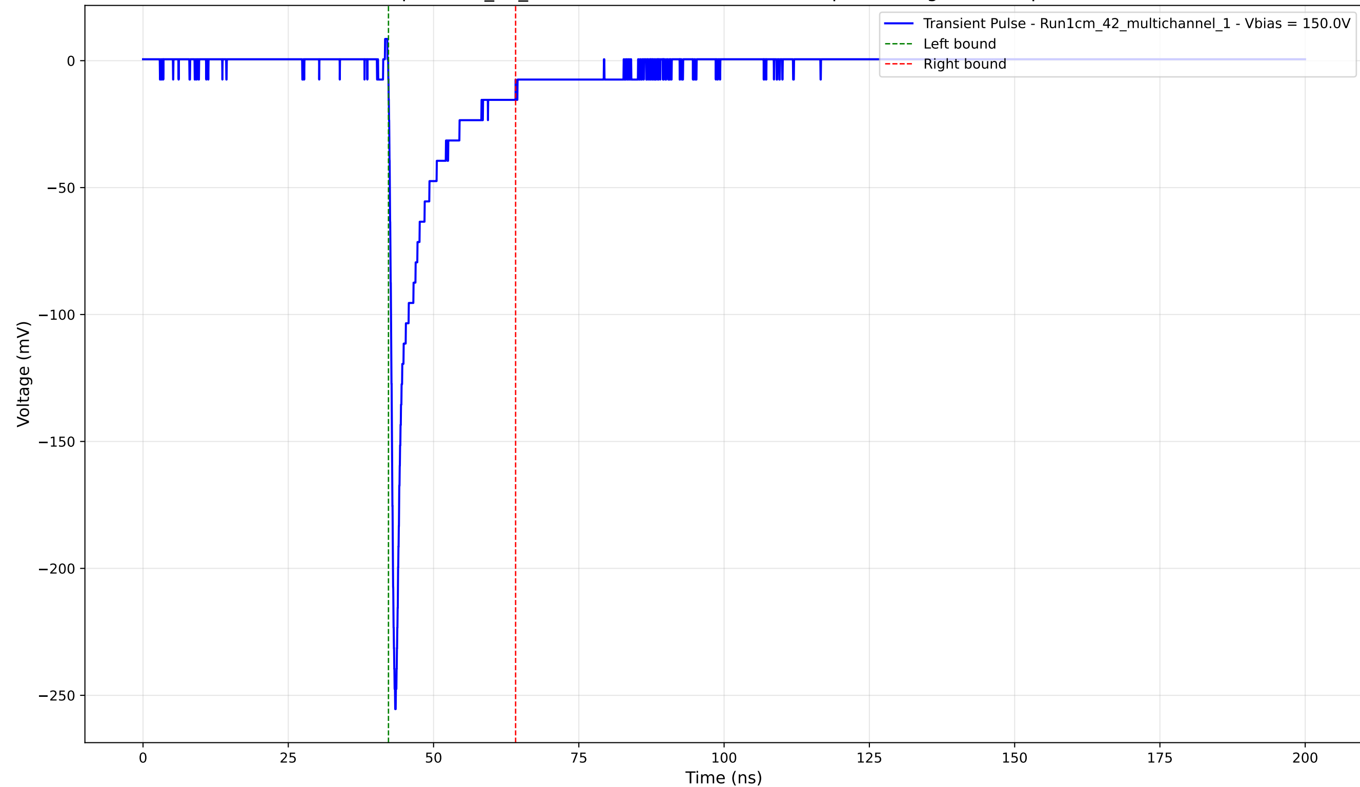
Transient Pulse - Sample: 1cm_42_multichannel - Position: 1990.0 \mu\text{m} - Charge: -22.99 pC - Rise Time: 0.79 ns
