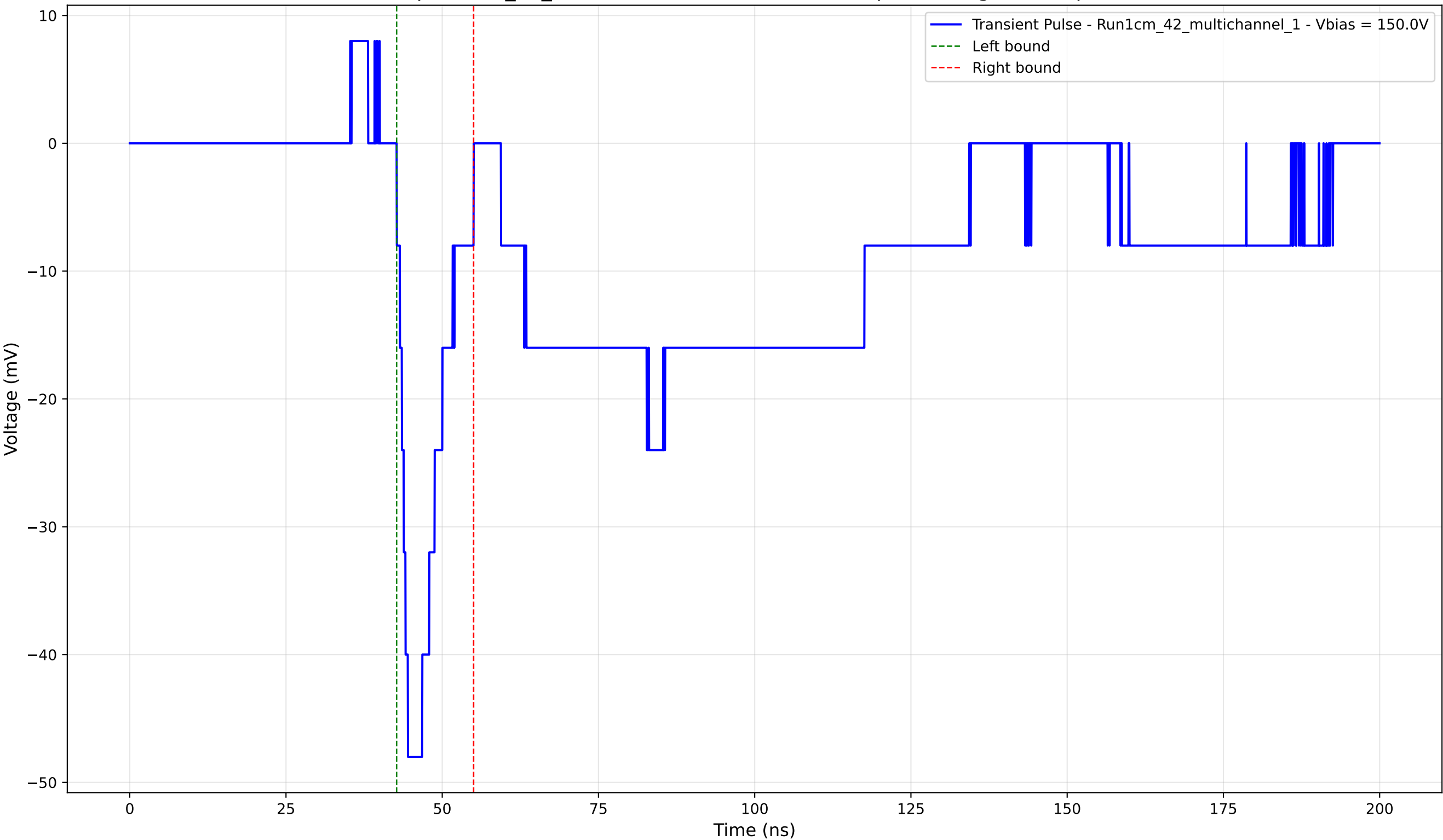
Transient Pulse - Sample: 1cm_42_multichannel - Position: 4285.0 \mu\text{m} - Charge: -6.13 pC - Rise Time: 1.79 ns
