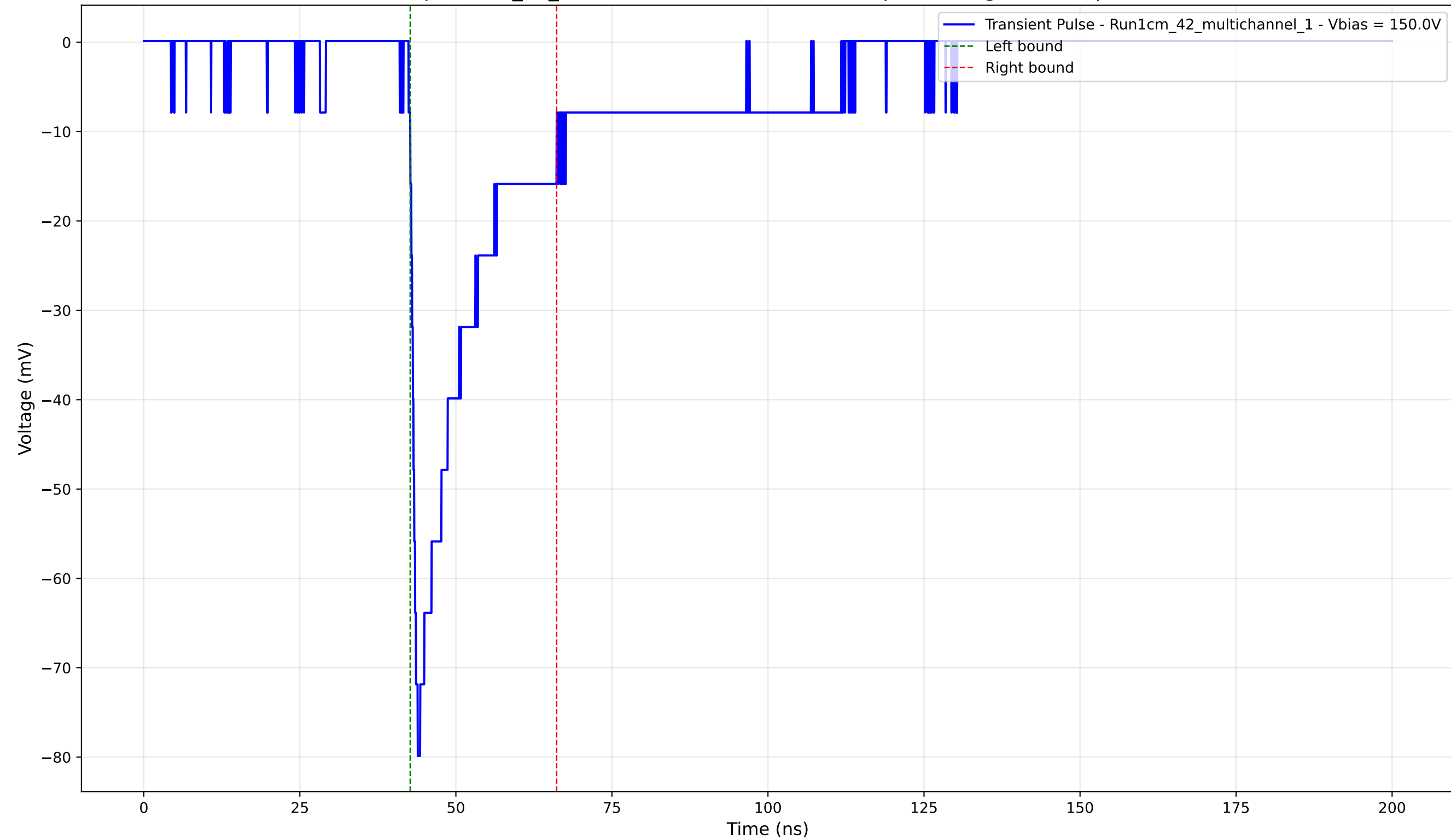
Transient Pulse - Sample: 1cm_42_multichannel - Position: 3480.0 \mu\text{m} - Charge: -14.79 pC - Rise Time: 1.20 ns
