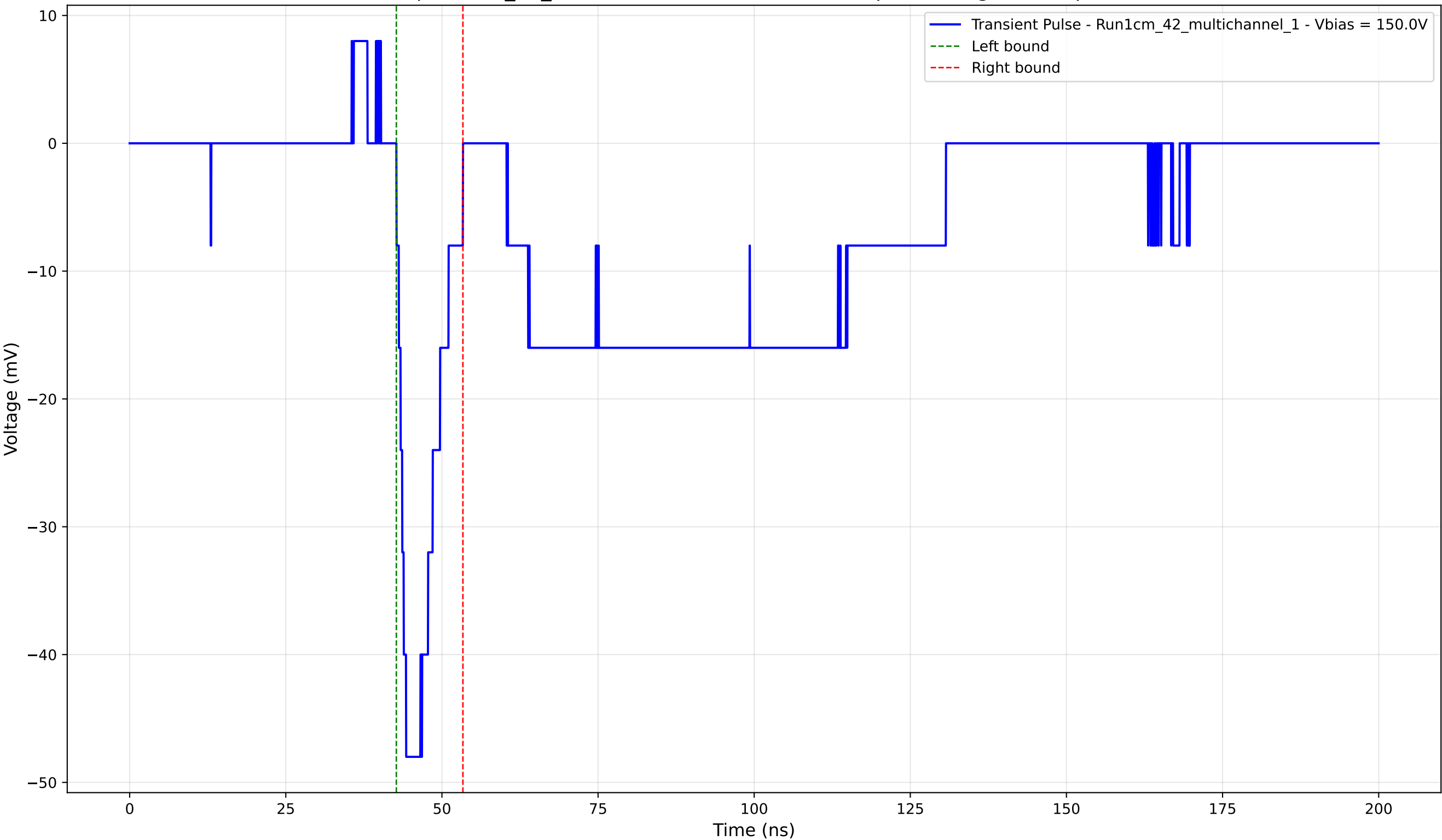
Transient Pulse - Sample: 1cm_42_multichannel - Position: 4045.0 \mu\text{m} - Charge: -5.77 pC - Rise Time: 1.55 ns
