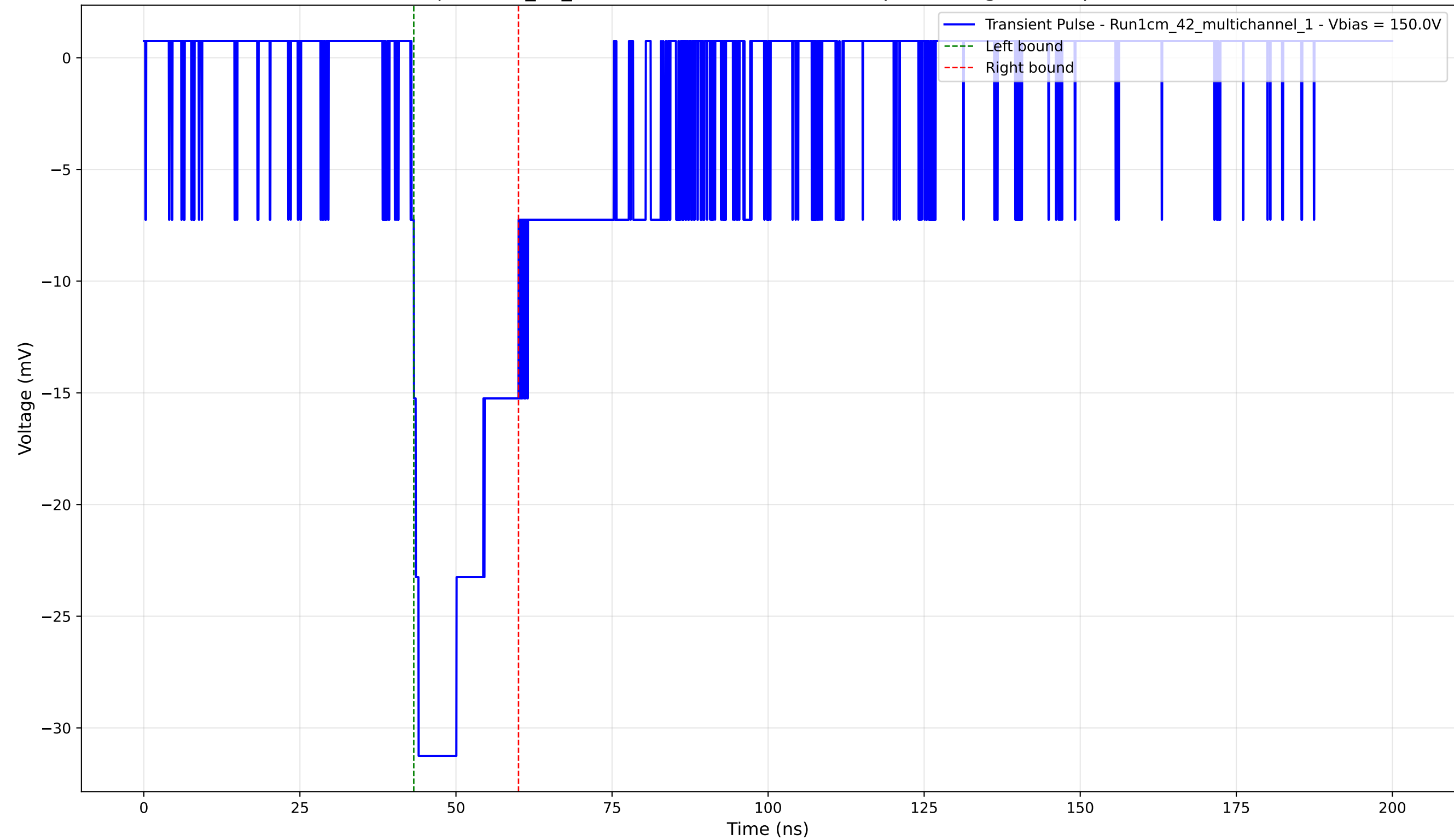
Transient Pulse - Sample: 1cm_42_multichannel - Position: 915.0 \mu\text{m} - Charge: -7.84 pC - Rise Time: 1.13 ns
