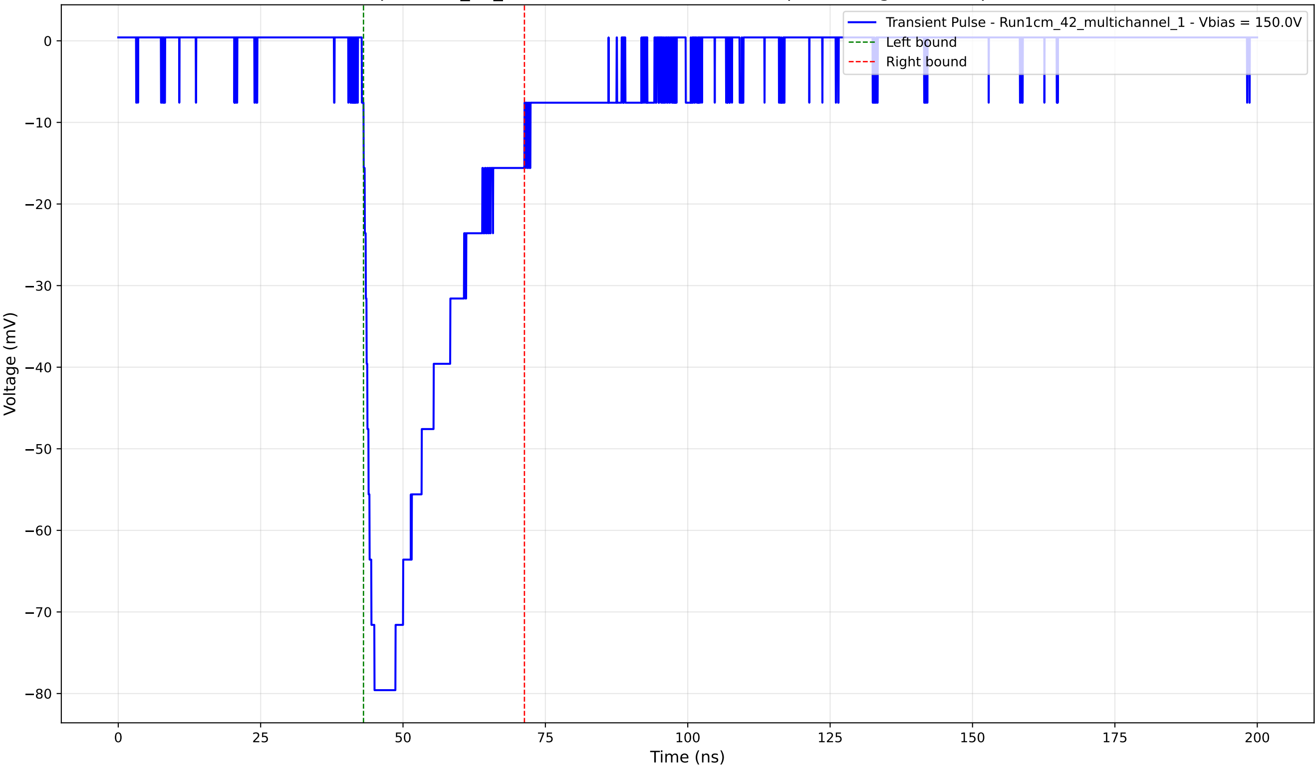
Transient Pulse - Sample: 1cm_42_multichannel - Position: 740.0 \mu\text{m} - Charge: -23.40 pC - Rise Time: 1.92 ns
