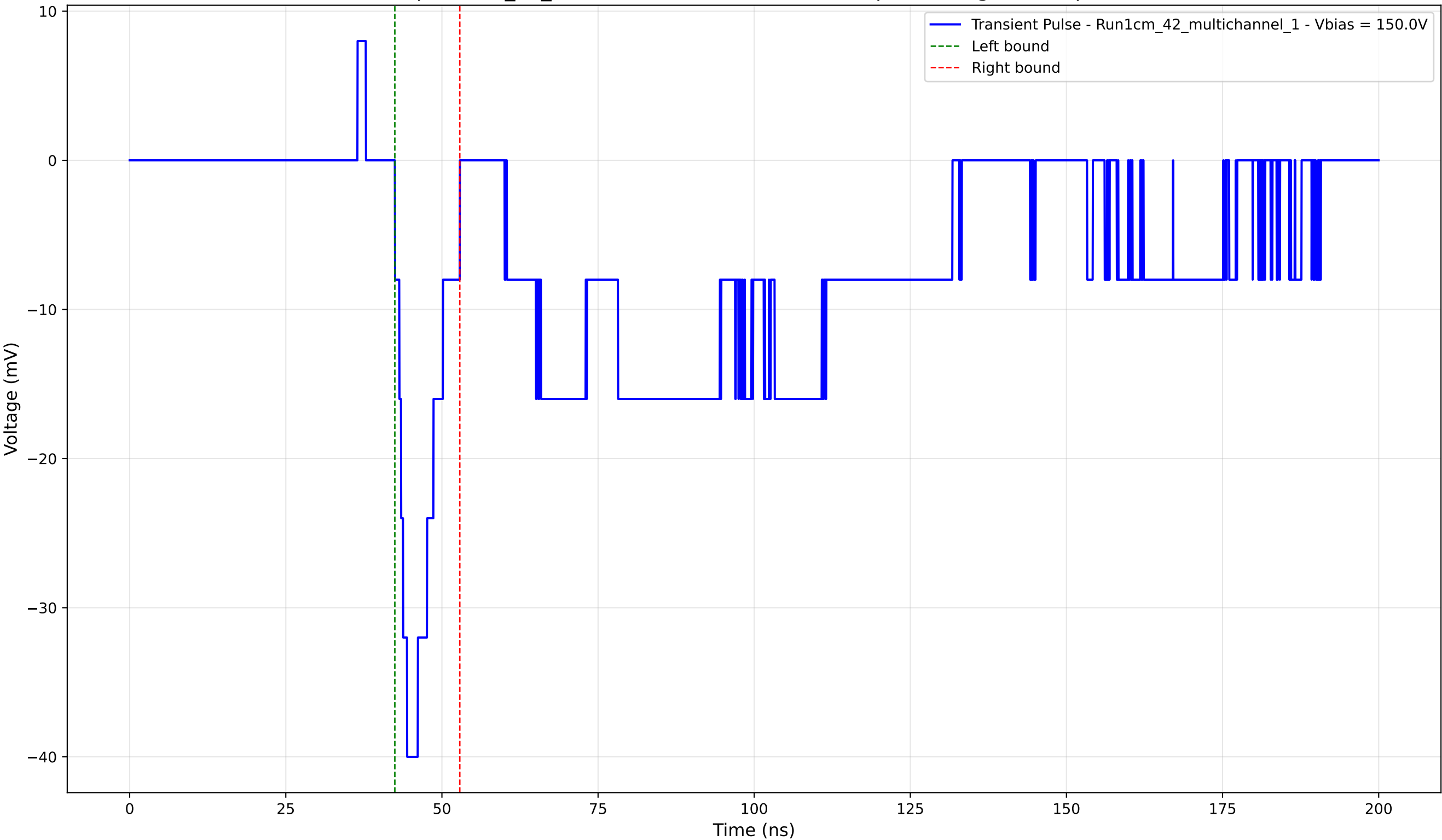
Transient Pulse - Sample: 1cm_42_multichannel - Position: 3965.0 \mu\text{m} - Charge: -4.50 pC - Rise Time: 1.95 ns
