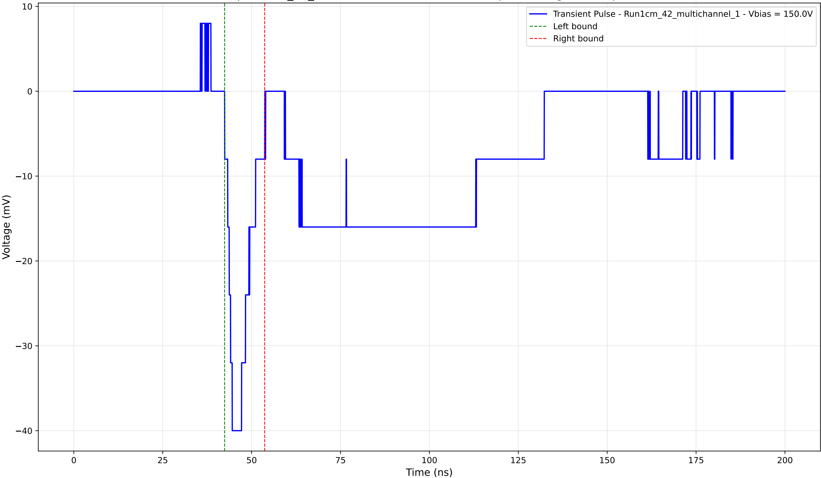
Transient Pulse - Sample: 1cm_42_multichannel - Position: 4335.0 \mu\text{m} - Charge: -5.05 pC - Rise Time: 2.13 ns
