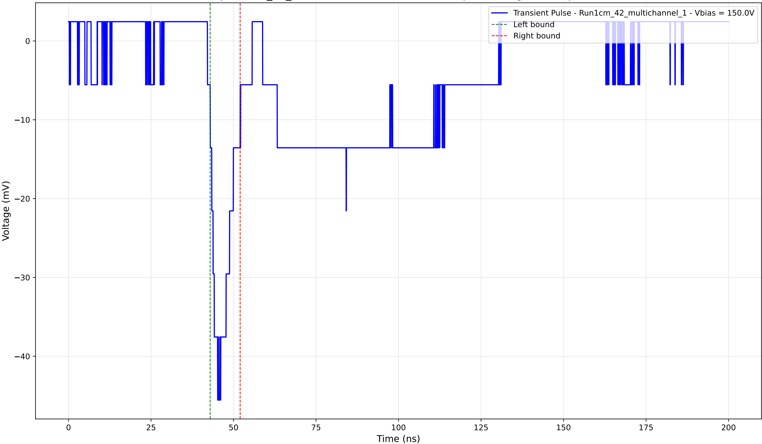
Transient Pulse - Sample: 1cm_42_multichannel - Position: 4720.0 \mu\text{m} - Charge: -4.98 pC - Rise Time: 3.09 ns
