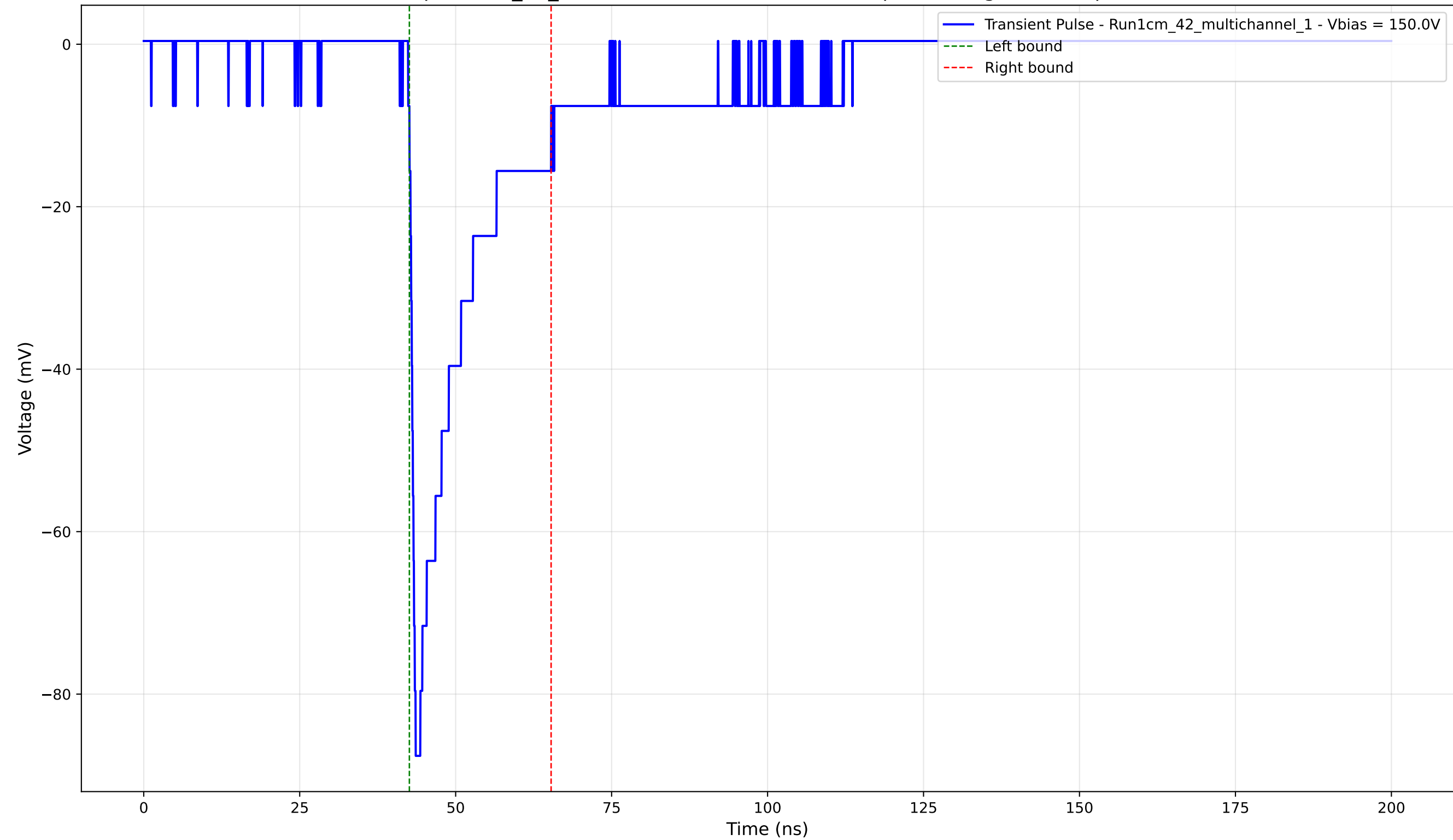
Transient Pulse - Sample: 1cm_42_multichannel - Position: 3320.0 \mu\text{m} - Charge: -15.03 pC - Rise Time: 0.86 ns
