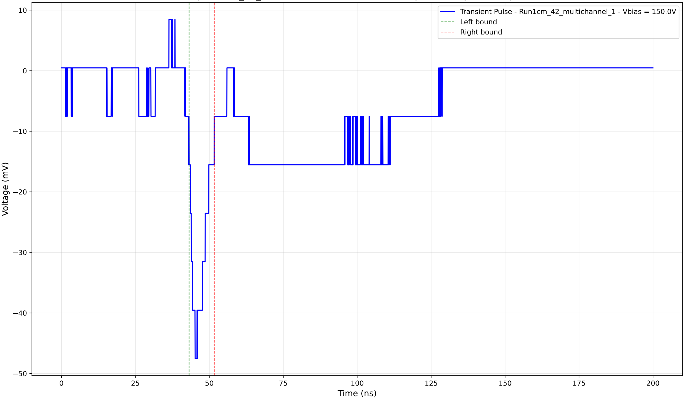
Transient Pulse - Sample: 1cm_42_multichannel - Position: 4485.0 \mu\text{m} - Charge: -5.06 pC - Rise Time: 3.21 ns
