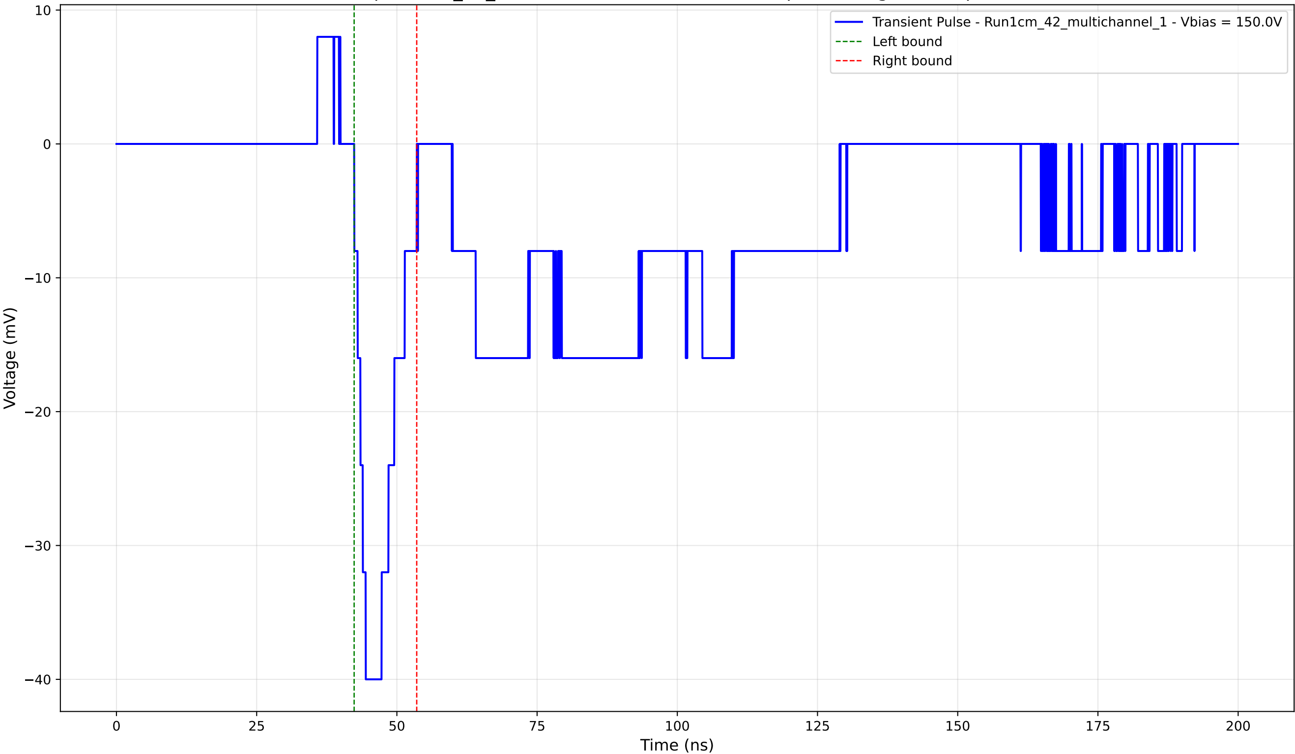
Transient Pulse - Sample: 1cm_42_multichannel - Position: 4790.0 \mu\text{m} - Charge: -5.28 pC - Rise Time: 2.05 ns
