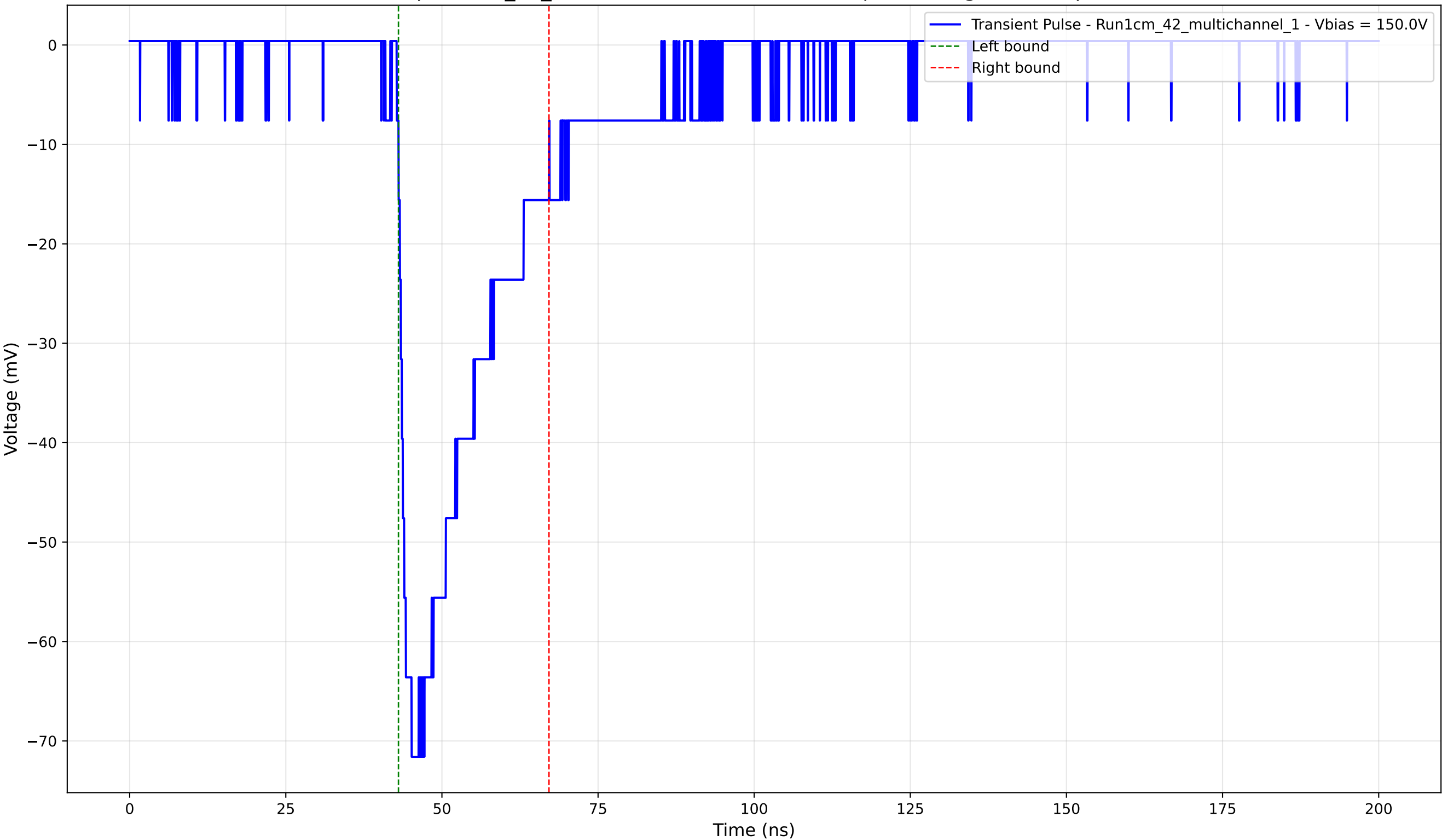
Transient Pulse - Sample: 1cm_42_multichannel - Position: 935.0 \mu\text{m} - Charge: -18.28 pC - Rise Time: 2.38 ns
