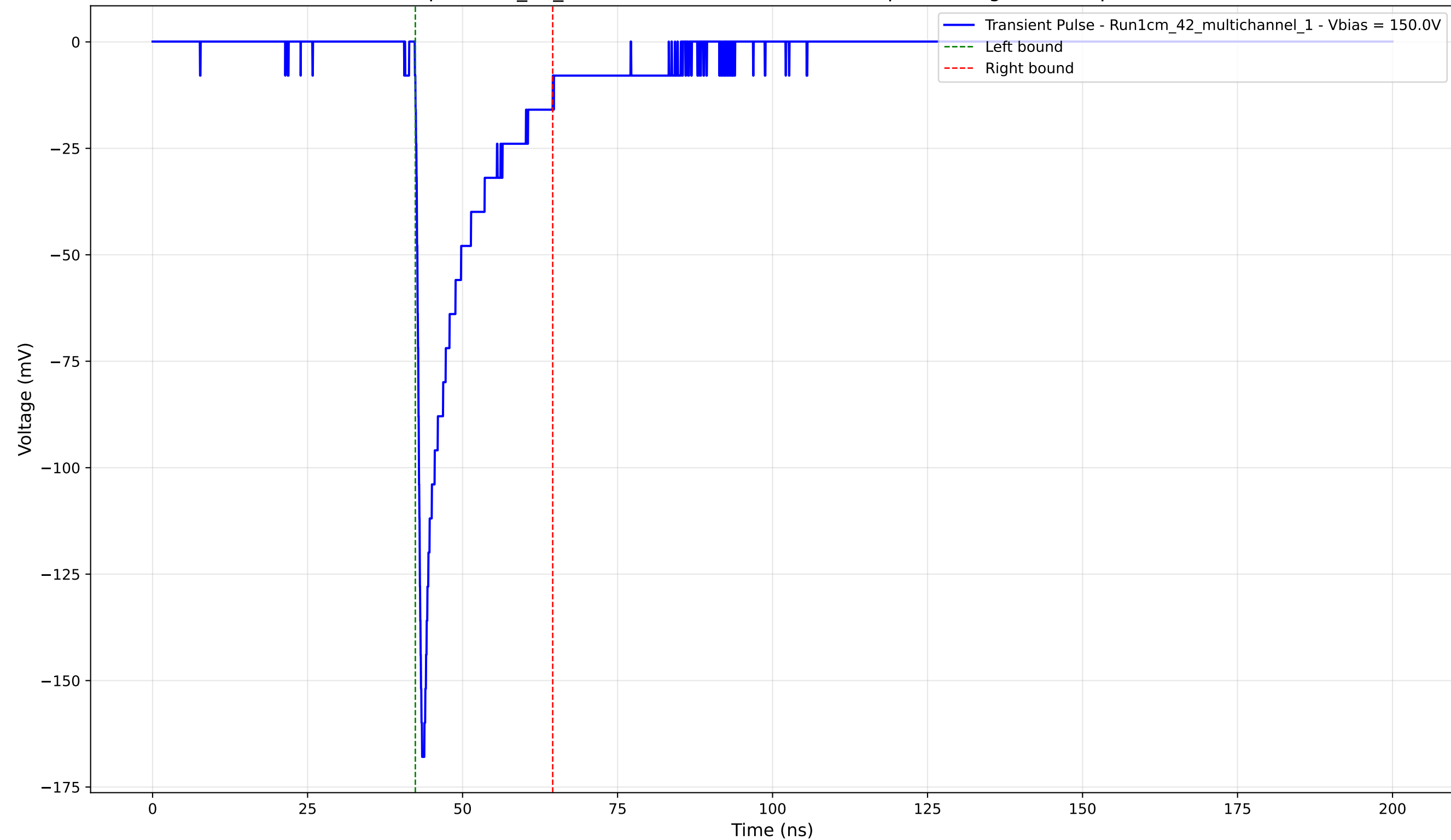
Transient Pulse - Sample: 1cm_42_multichannel - Position: 1740.0 \mu\text{m} - Charge: -21.82 pC - Rise Time: 0.82 ns
