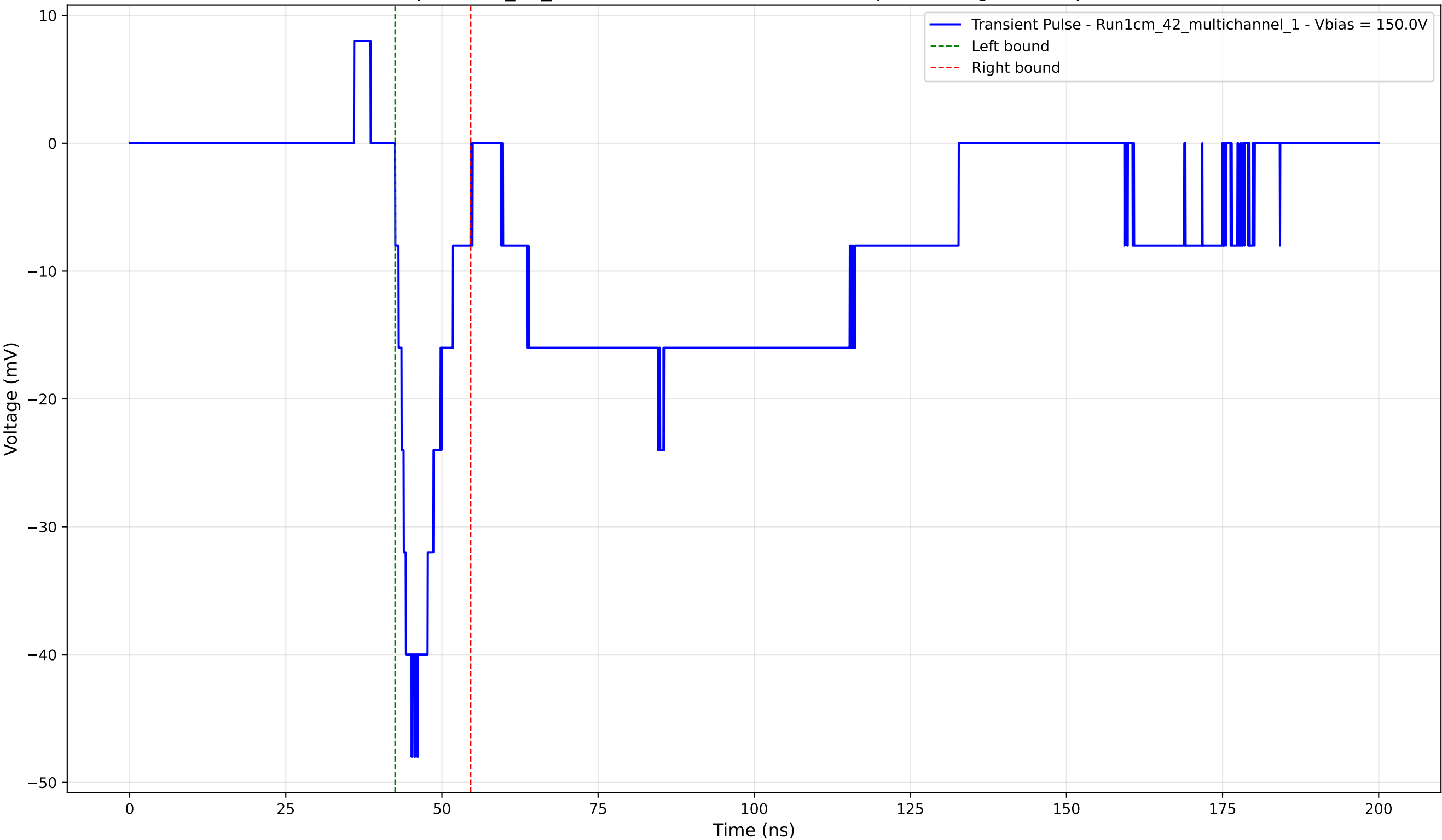
Transient Pulse - Sample: 1cm_42_multichannel - Position: 4665.0 \mu\text{m} - Charge: -5.70 pC - Rise Time: 2.63 ns
