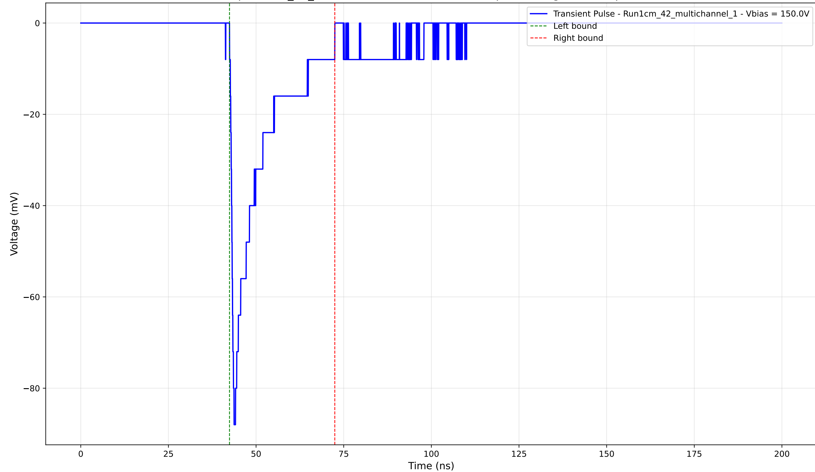
Transient Pulse - Sample: 1cm_42_multichannel - Position: 3325.0 \mu\text{m} - Charge: -15.11 pC - Rise Time: 0.90 ns
