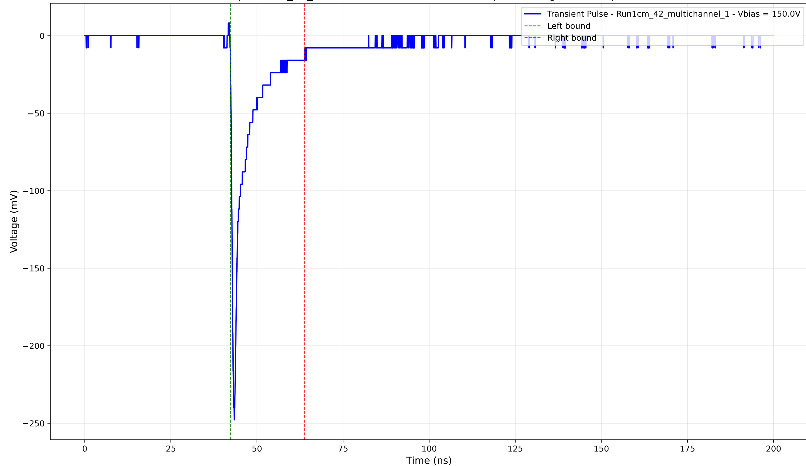
Transient Pulse - Sample: 1cm_42_multichannel - Position: 2770.0 \mu\text{m} - Charge: -21.83 pC - Rise Time: 0.78 ns
