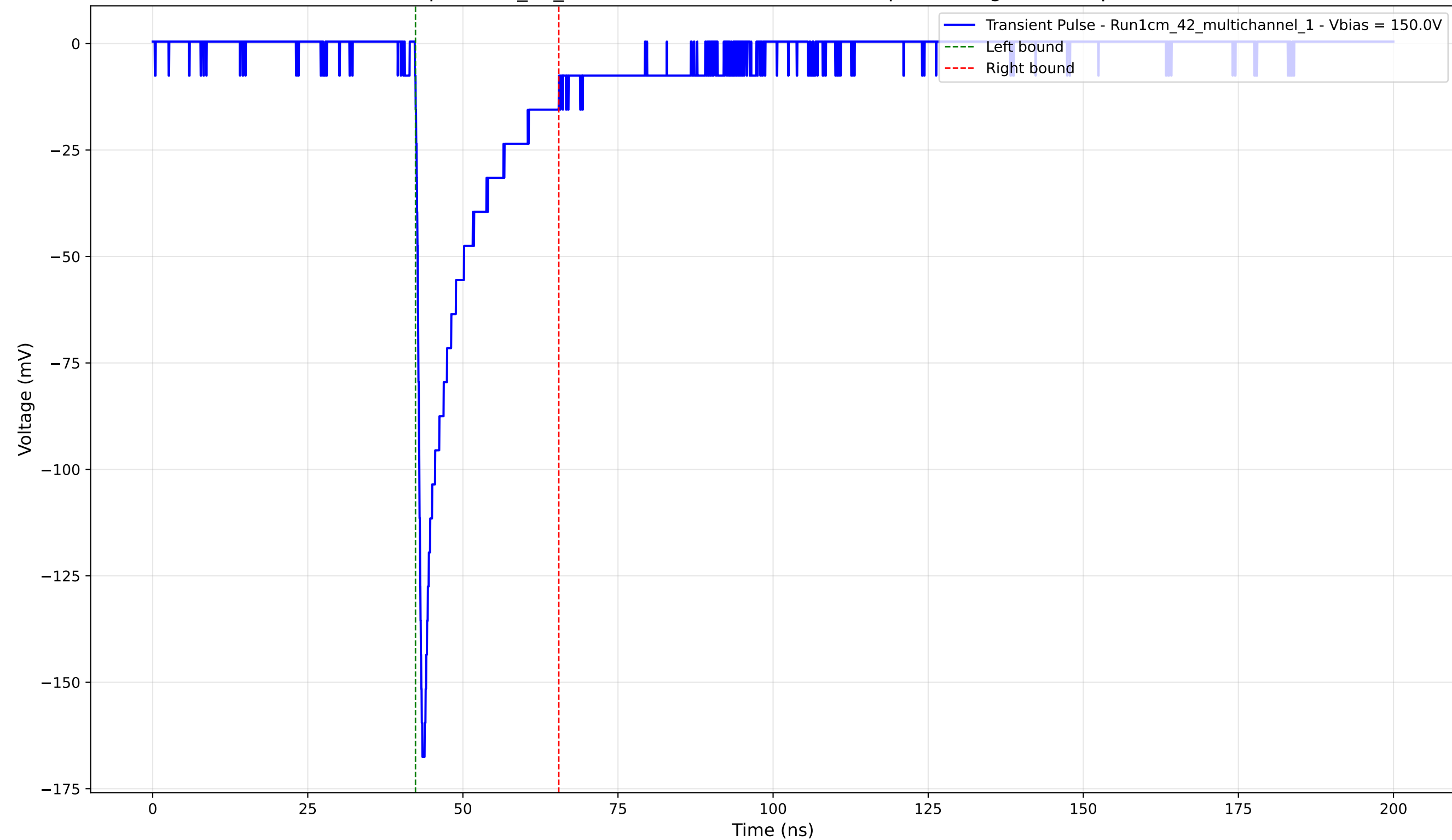
Transient Pulse - Sample: 1cm_42_multichannel - Position: 1730.0 \mu\text{m} - Charge: -22.35 pC - Rise Time: 0.84 ns
