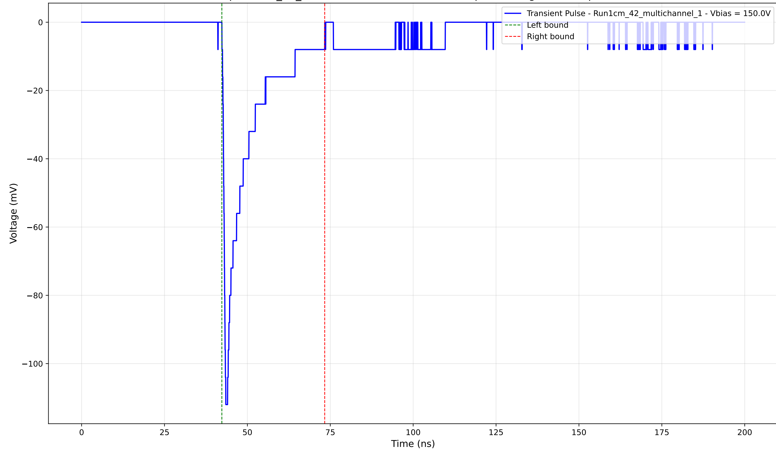
Transient Pulse - Sample: 1cm_42_multichannel - Position: 3195.0 \mu\text{m} - Charge: -16.96 pC - Rise Time: 0.87 ns
