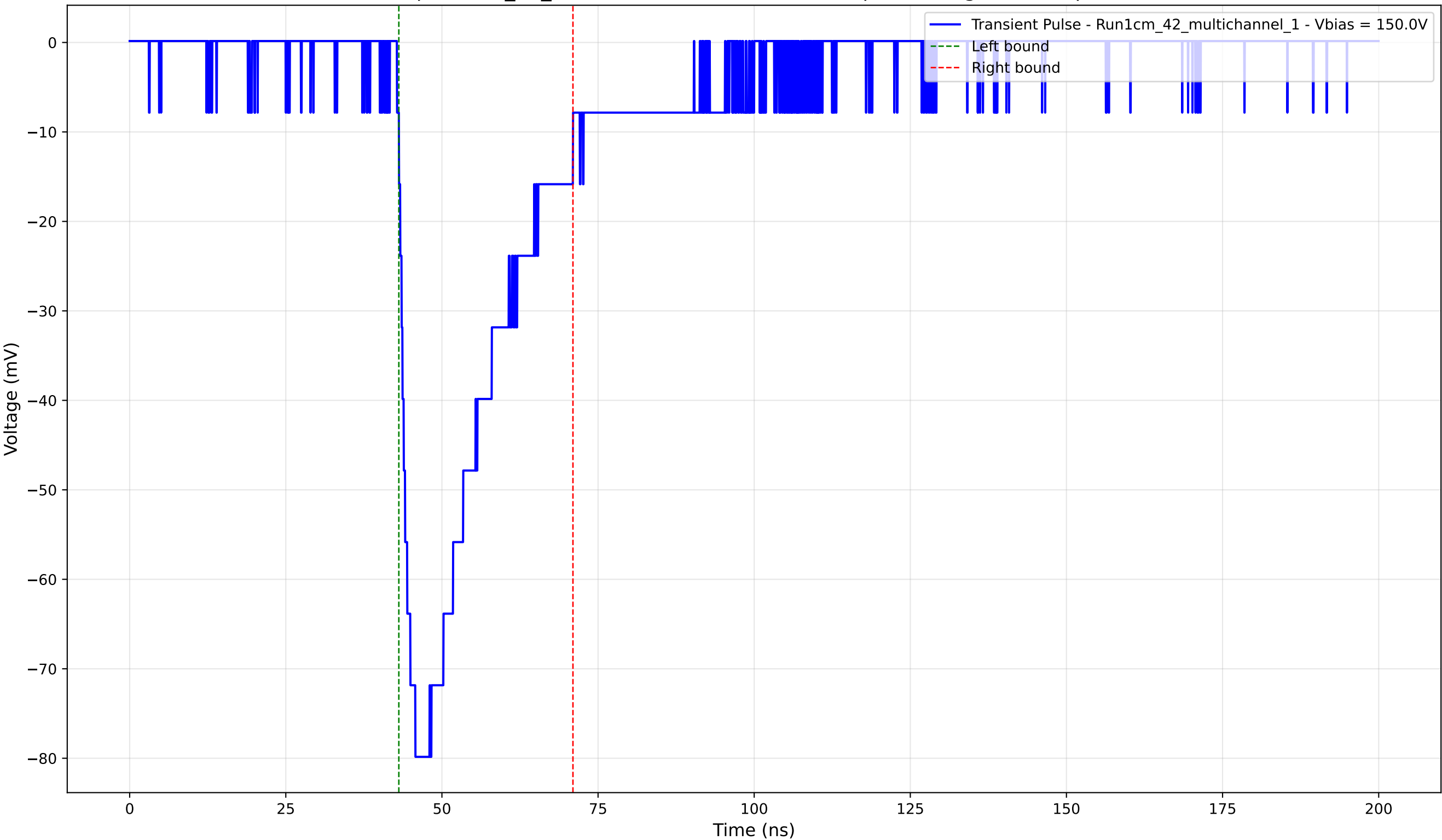
Transient Pulse - Sample: 1cm_42_multichannel - Position: 550.0 \mu\text{m} - Charge: -23.26 pC - Rise Time: 2.64 ns
