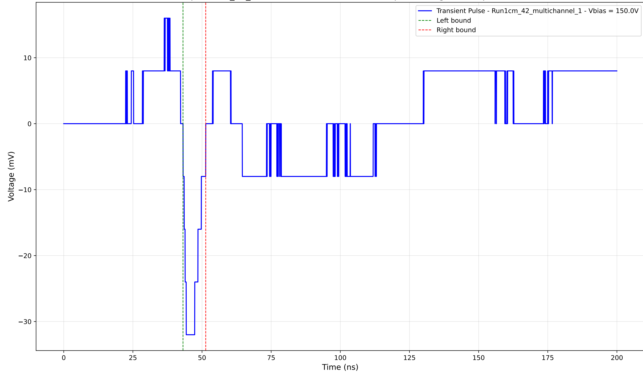
Transient Pulse - Sample: 1cm_42_multichannel - Position: 4725.0 \mu\text{m} - Charge: -3.54 pC - Rise Time: 1.15 ns
