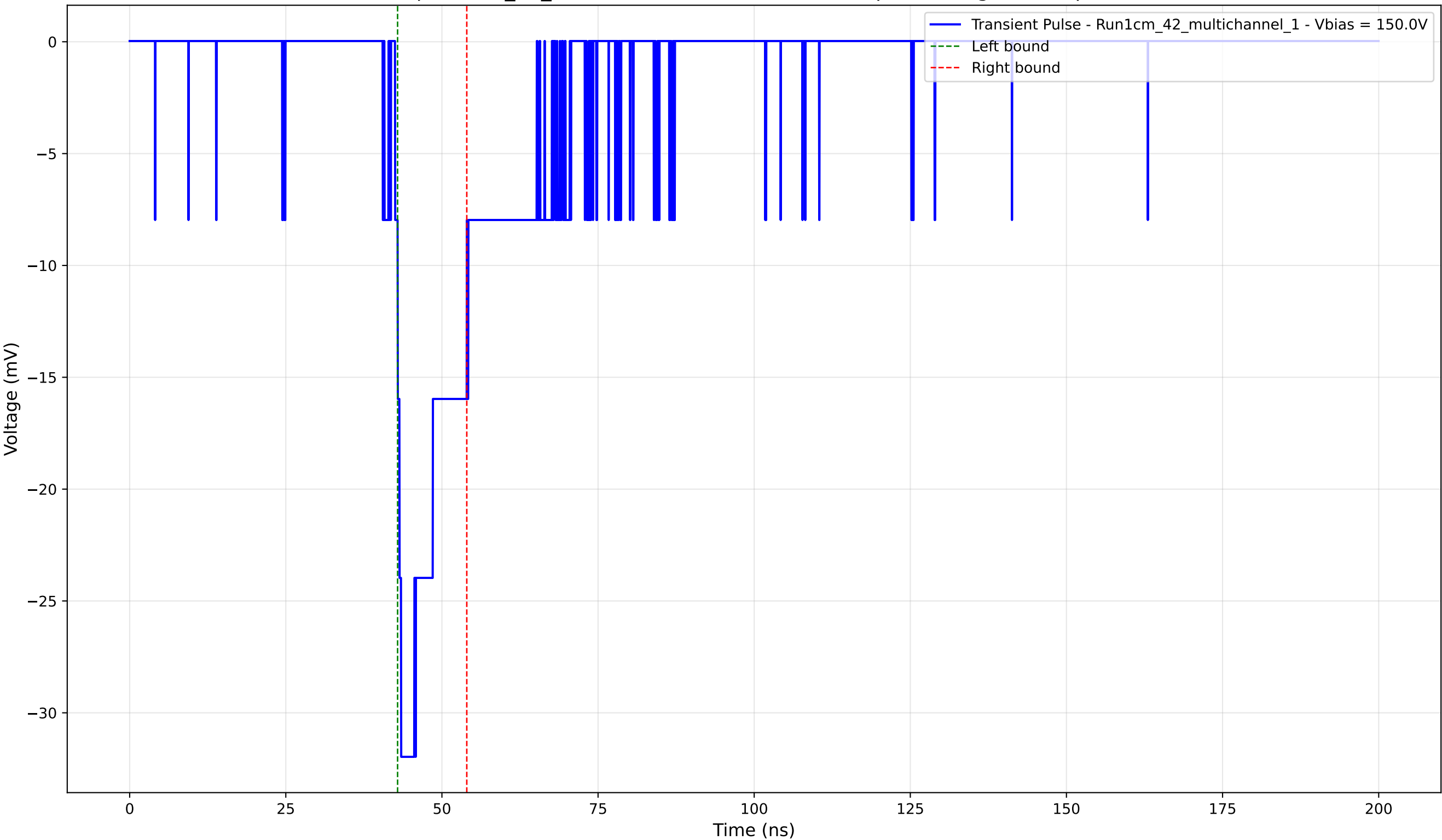
Transient Pulse - Sample: 1cm_42_multichannel - Position: 1415.0 \mu\text{m} - Charge: -4.74 pC - Rise Time: 0.97 ns
