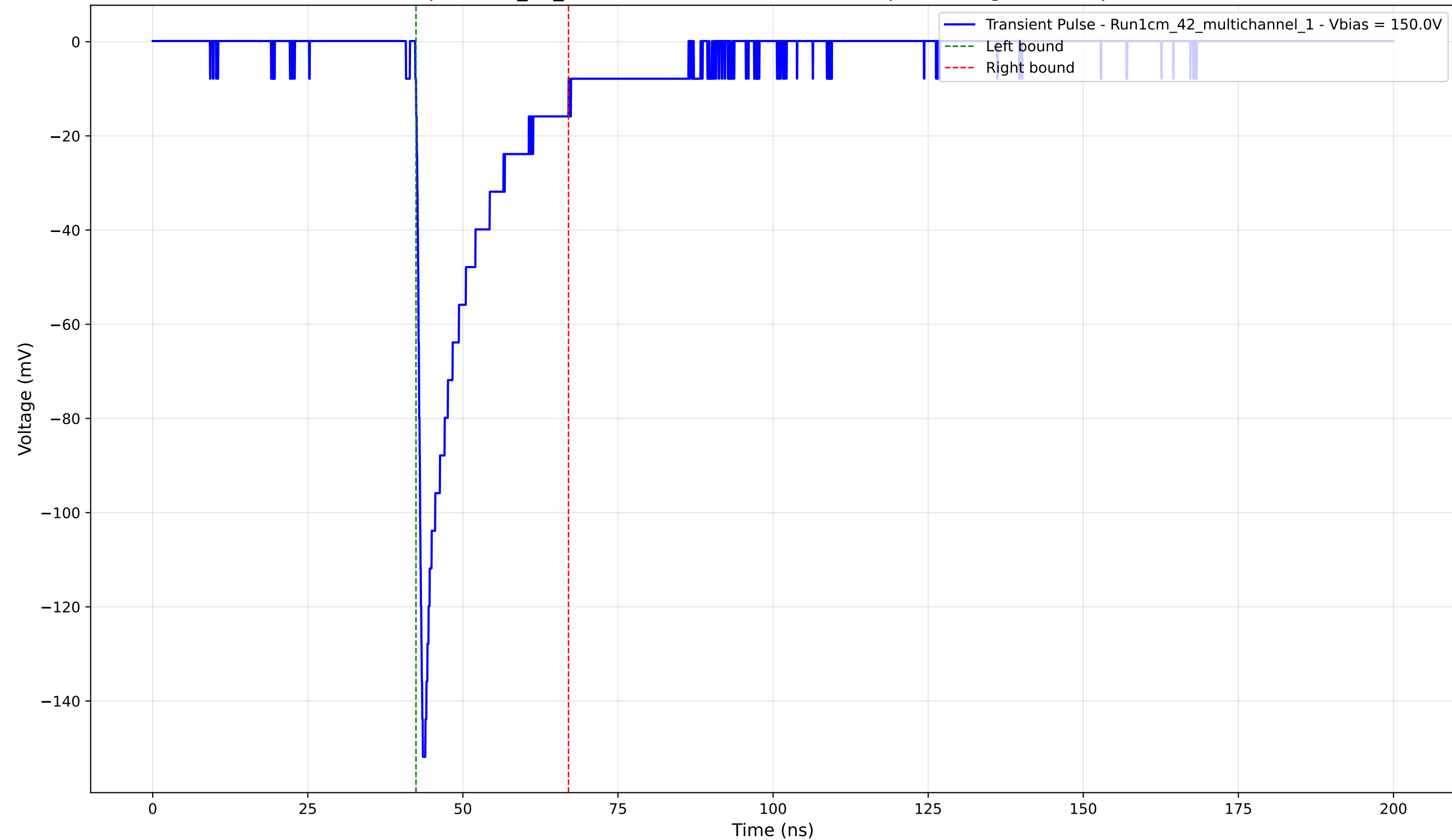
Transient Pulse - Sample: 1cm_42_multichannel - Position: 1640.0 \mu\text{m} - Charge: -22.75 pC - Rise Time: 0.98 ns
