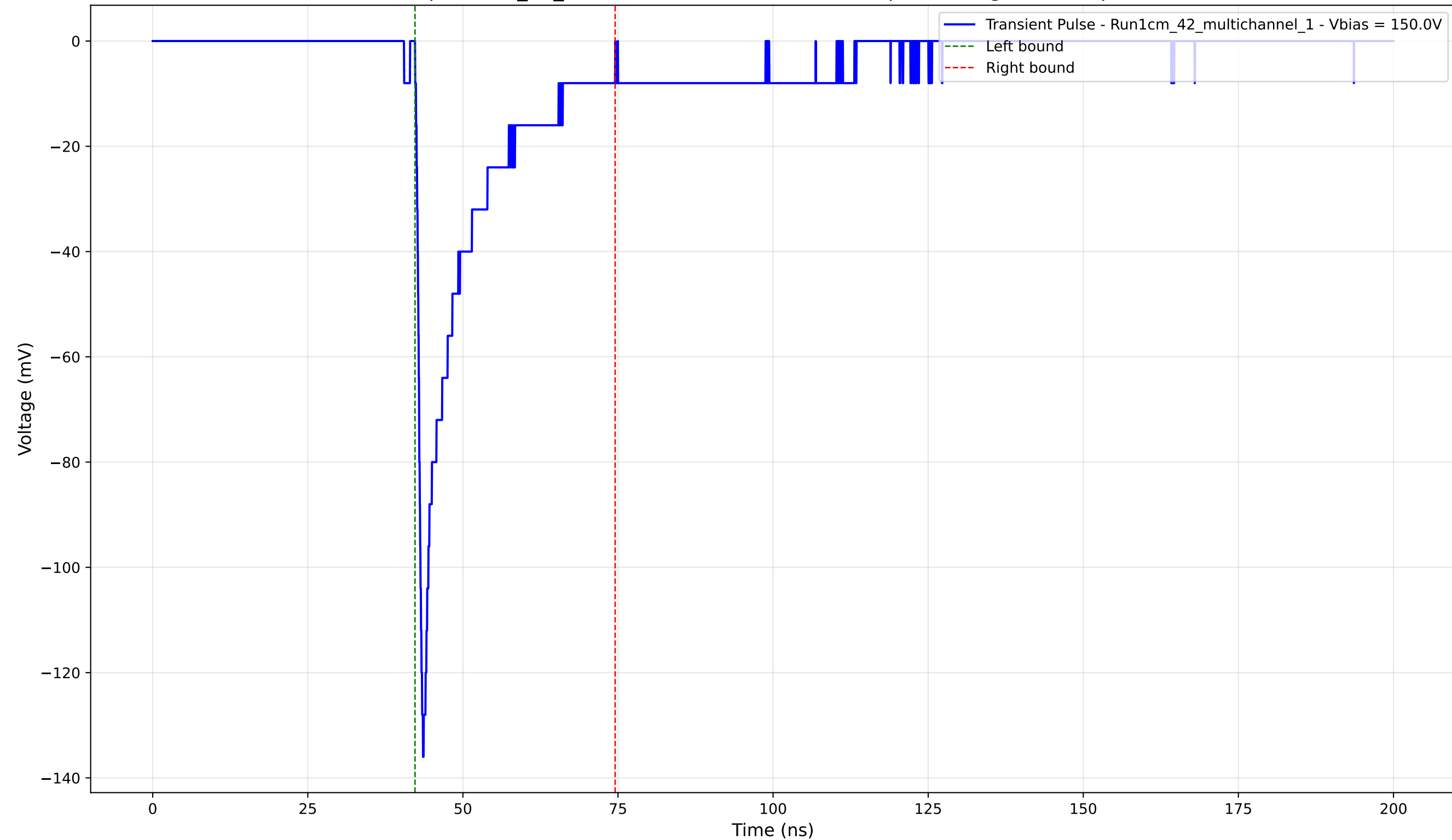
Transient Pulse - Sample: 1cm_42_multichannel - Position: 3110.0 \mu\text{m} - Charge: -19.46 pC - Rise Time: 0.99 ns
