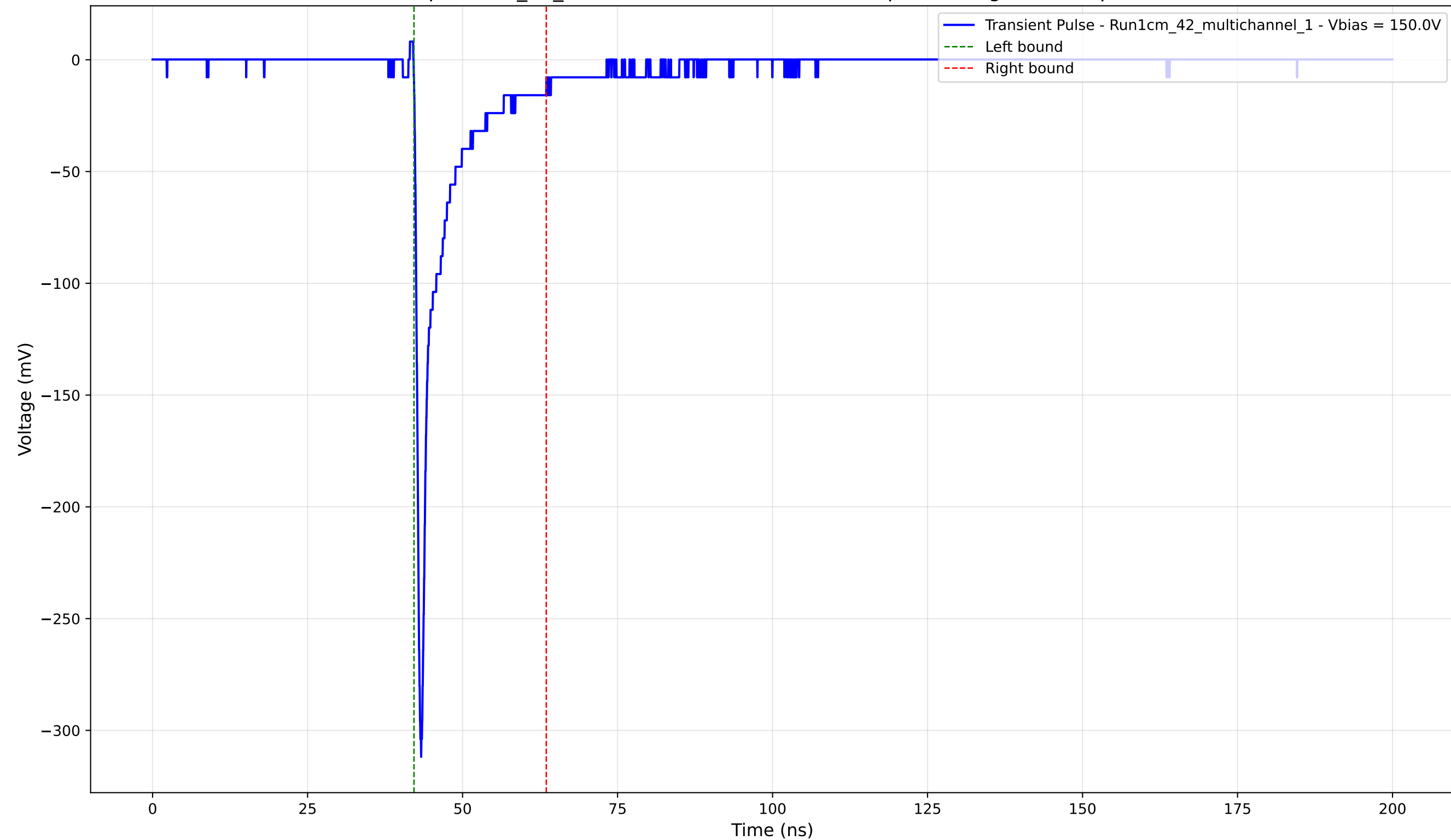
Transient Pulse - Sample: 1cm_42_multichannel - Position: 2110.0 \mu\text{m} - Charge: -23.70 pC - Rise Time: 0.82 ns
