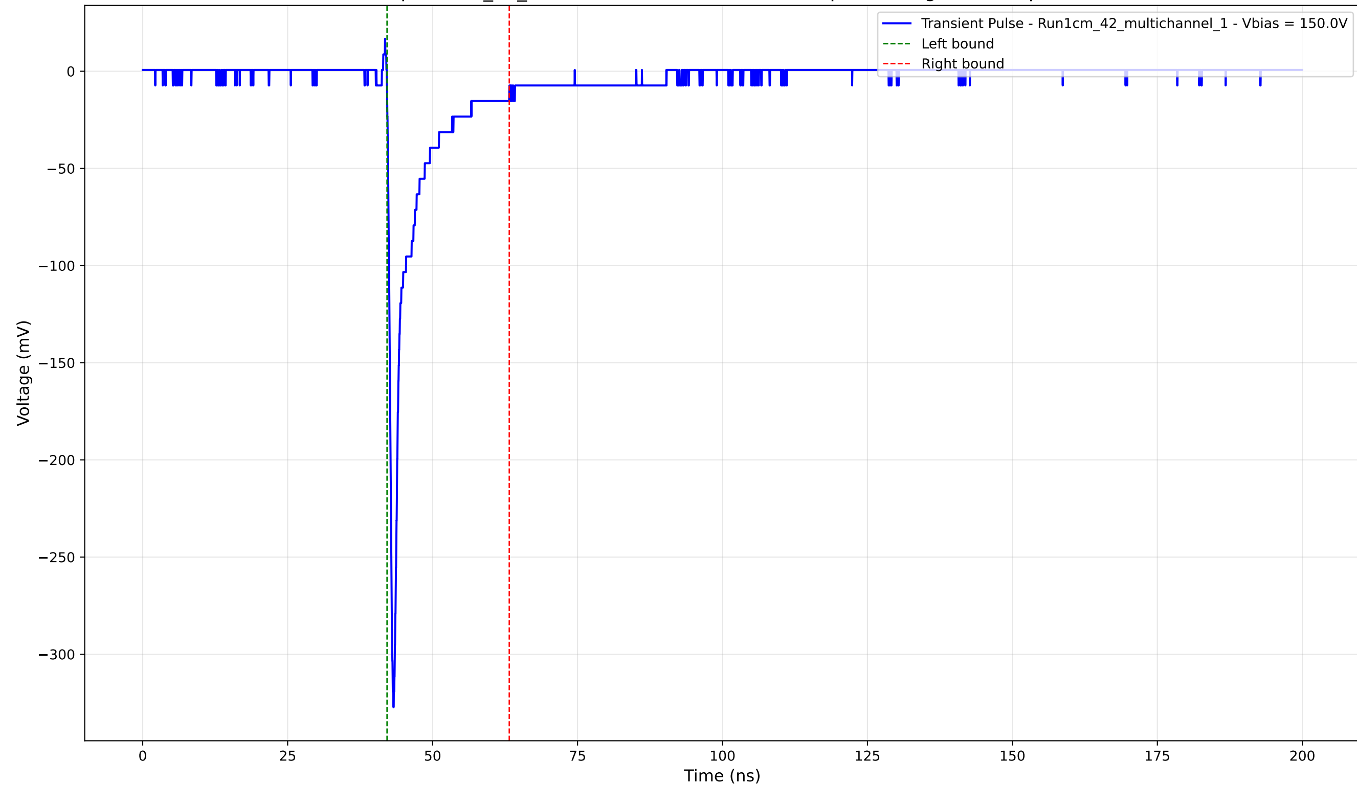
Transient Pulse - Sample: 1cm_42_multichannel - Position: 2615.0 \mu\text{m} - Charge: -23.21 pC - Rise Time: 0.76 ns
