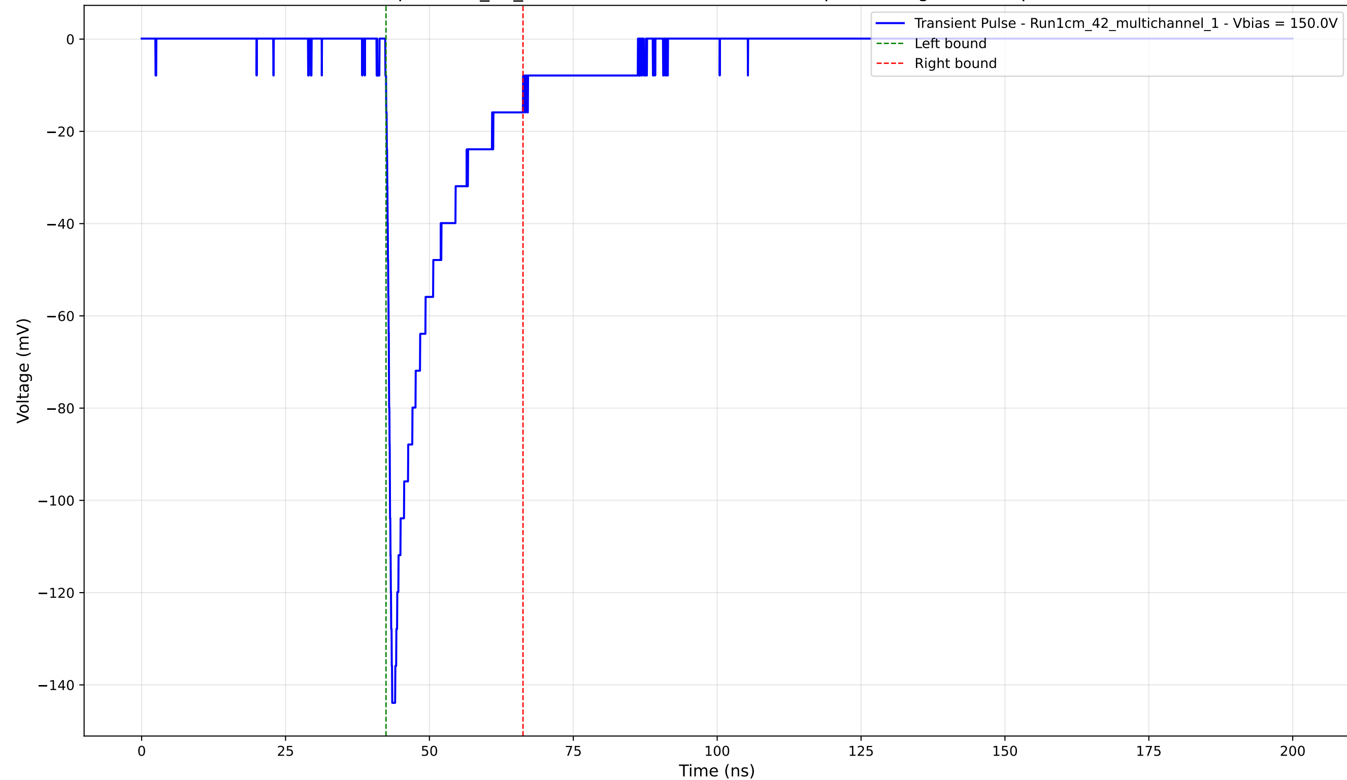
Transient Pulse - Sample: 1cm_42_multichannel - Position: 1615.0 \mu\text{m} - Charge: -22.42 pC - Rise Time: 0.96 ns
