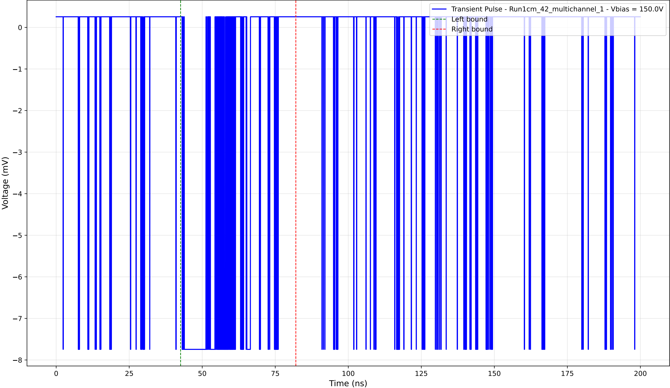
Transient Pulse - Sample: 1cm_42_multichannel - Position: 875.0 \mu\text{m} - Charge: -2.50 pC - Rise Time: 0.02 ns
