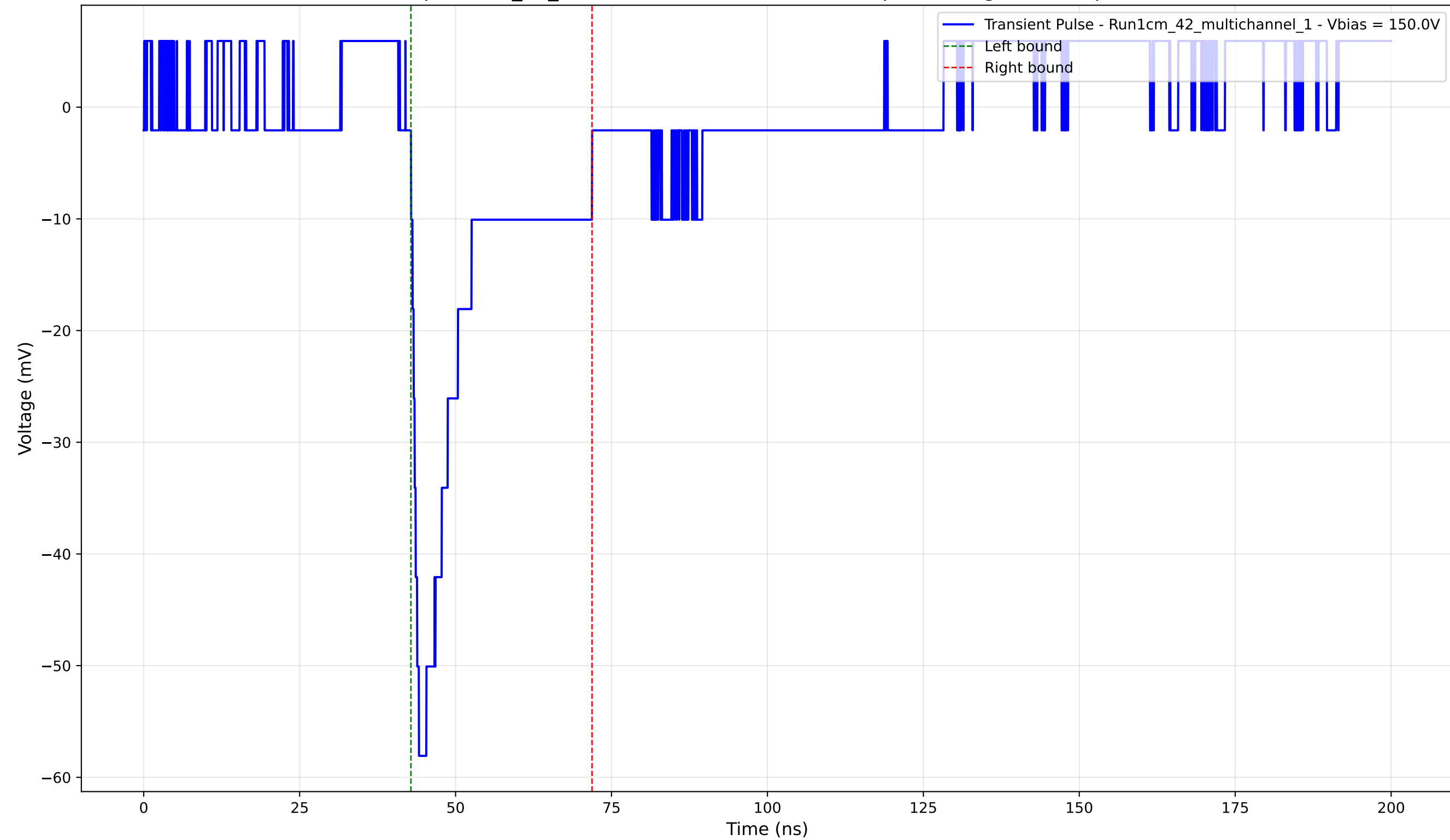
Transient Pulse - Sample: 1cm_42_multichannel - Position: 3780.0 \mu\text{m} - Charge: -10.67 pC - Rise Time: 1.27 ns
