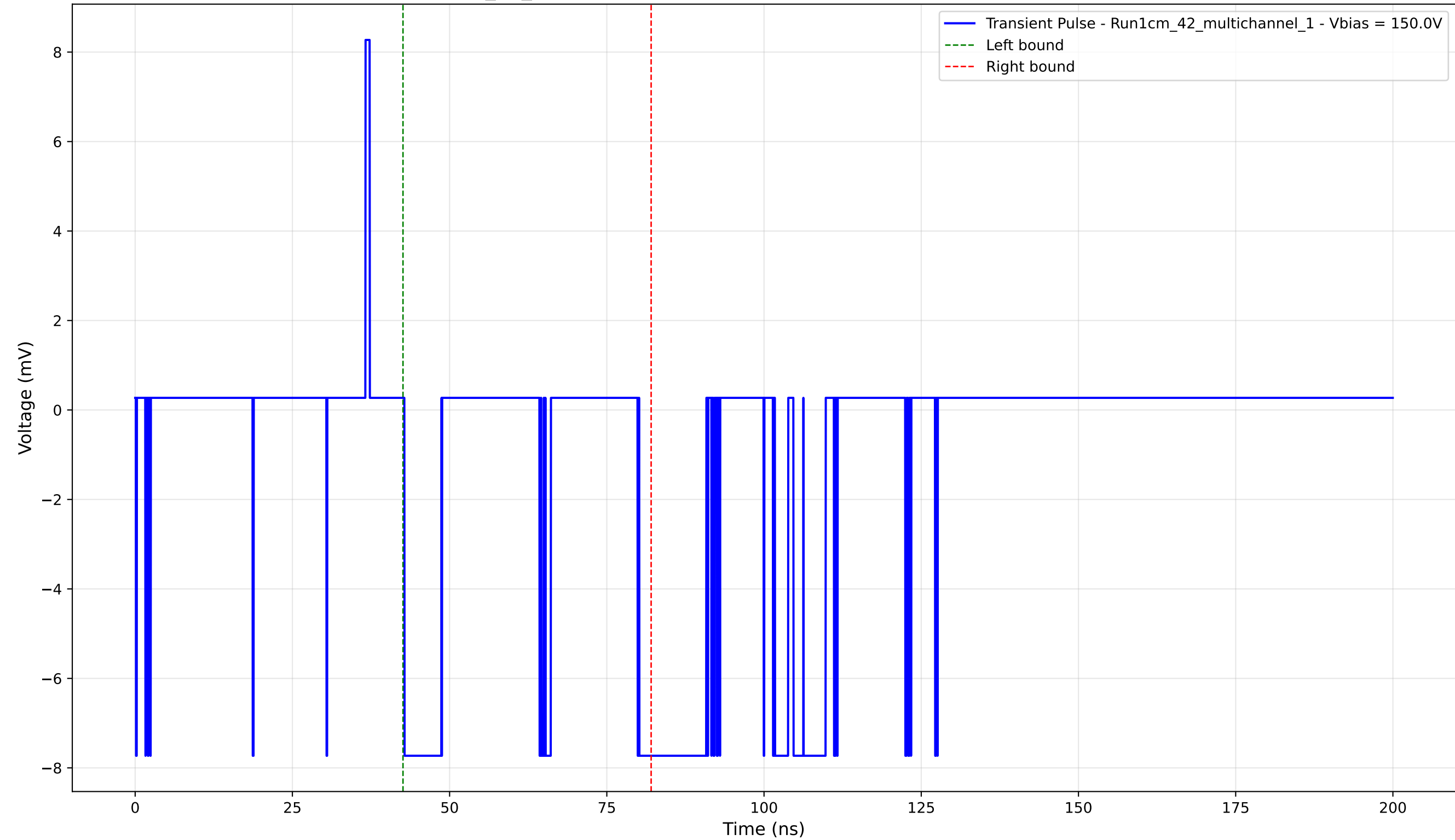
Transient Pulse - Sample: 1cm_42_multichannel - Position: 3875.0 \mu\text{m} - Charge: -1.32 pC - Rise Time: 0.00 ns (N/A)
