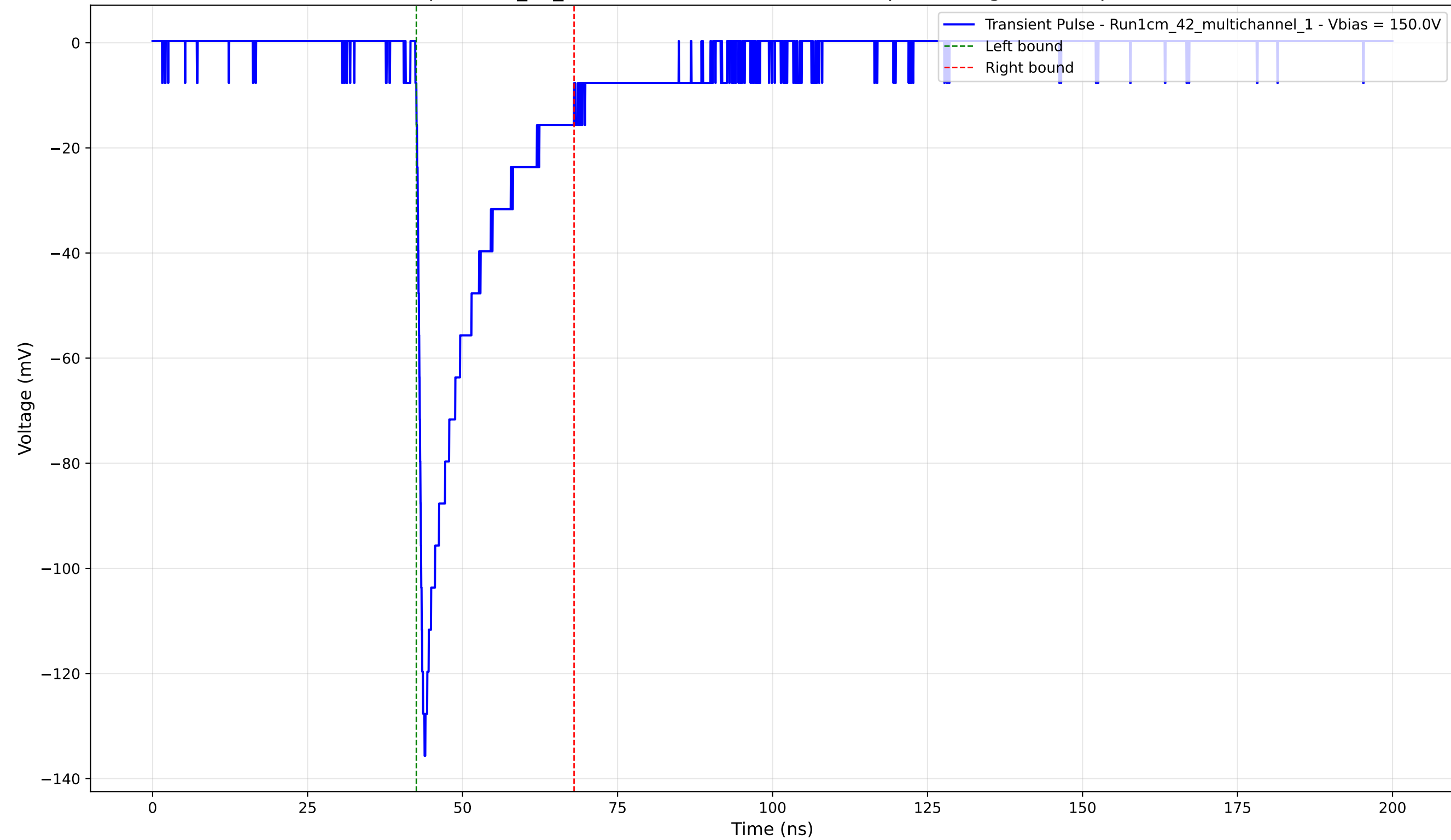
Transient Pulse - Sample: 1cm_42_multichannel - Position: 1520.0 \mu\text{m} - Charge: -23.10 pC - Rise Time: 1.07 ns
