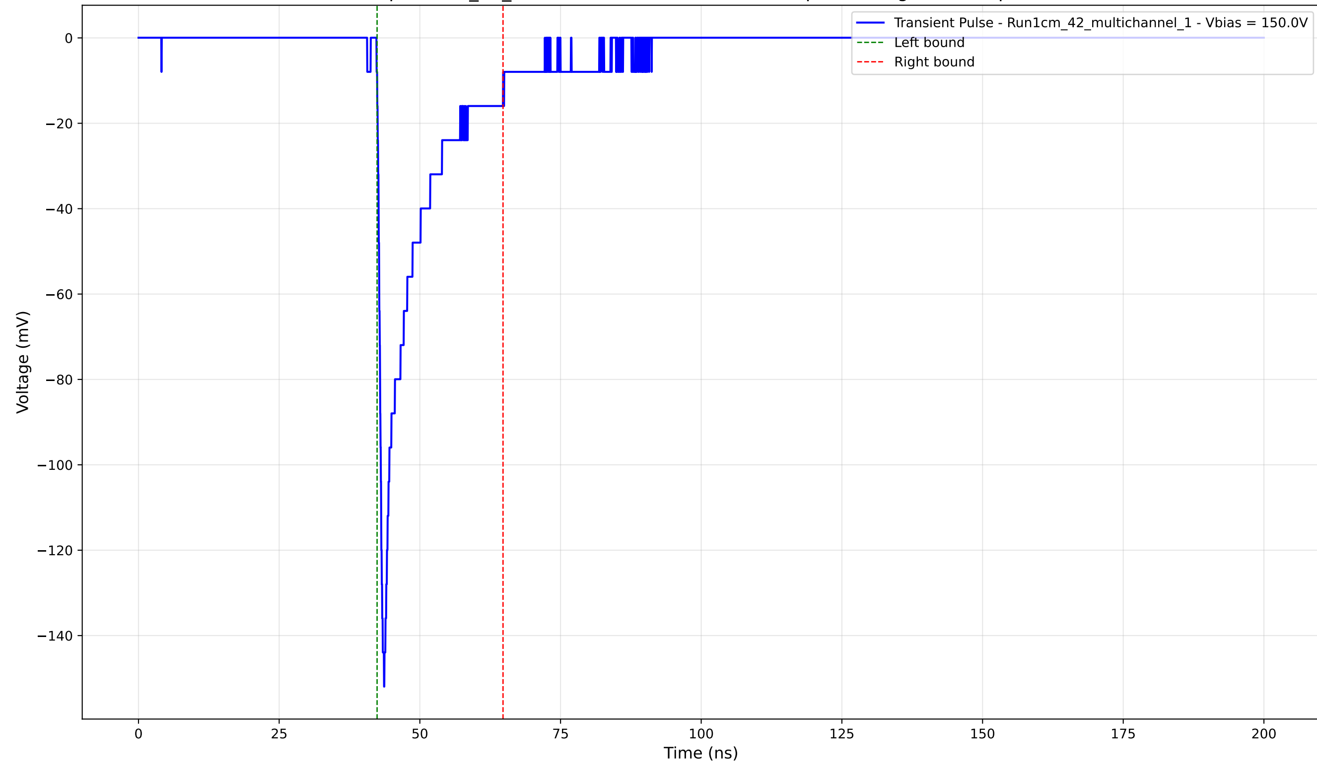
Transient Pulse - Sample: 1cm_42_multichannel - Position: 3055.0 \mu\text{m} - Charge: -18.82 pC - Rise Time: 0.98 ns
