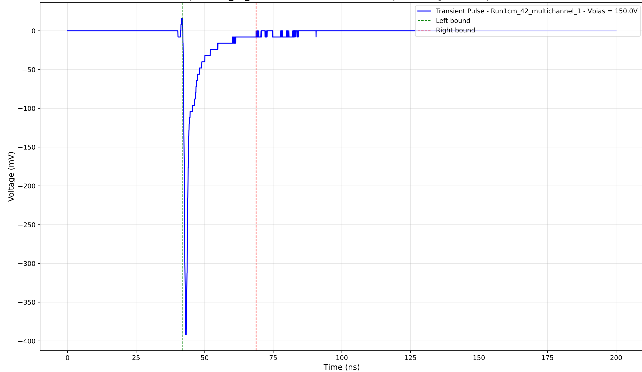
Transient Pulse - Sample: 1cm_42_multichannel - Position: 2495.0 \mu\text{m} - Charge: -24.57 pC - Rise Time: 0.72 ns
