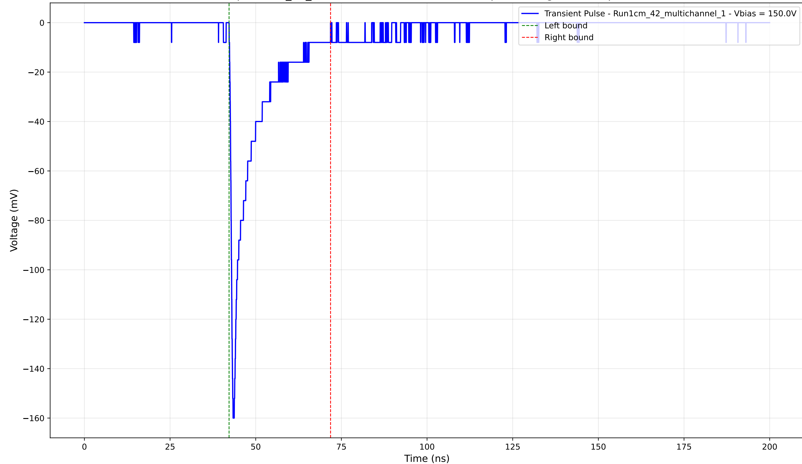
Transient Pulse - Sample: 1cm_42_multichannel - Position: 2970.0 \mu\text{m} - Charge: -20.50 pC - Rise Time: 0.78 ns
