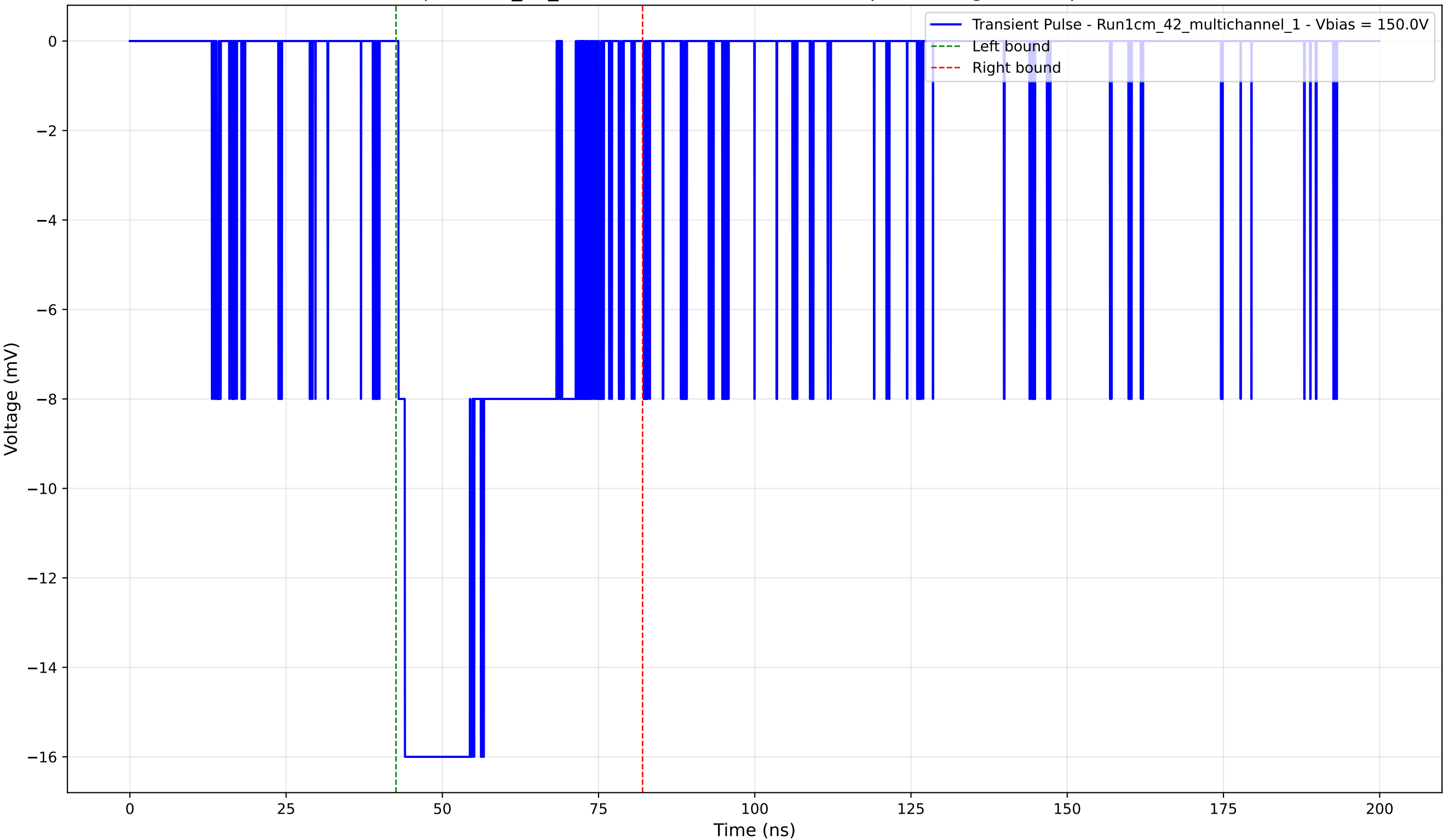
Transient Pulse - Sample: 1cm_42_multichannel - Position: 400.0 \mu\text{m} - Charge: -6.78 pC - Rise Time: 1.04 ns
