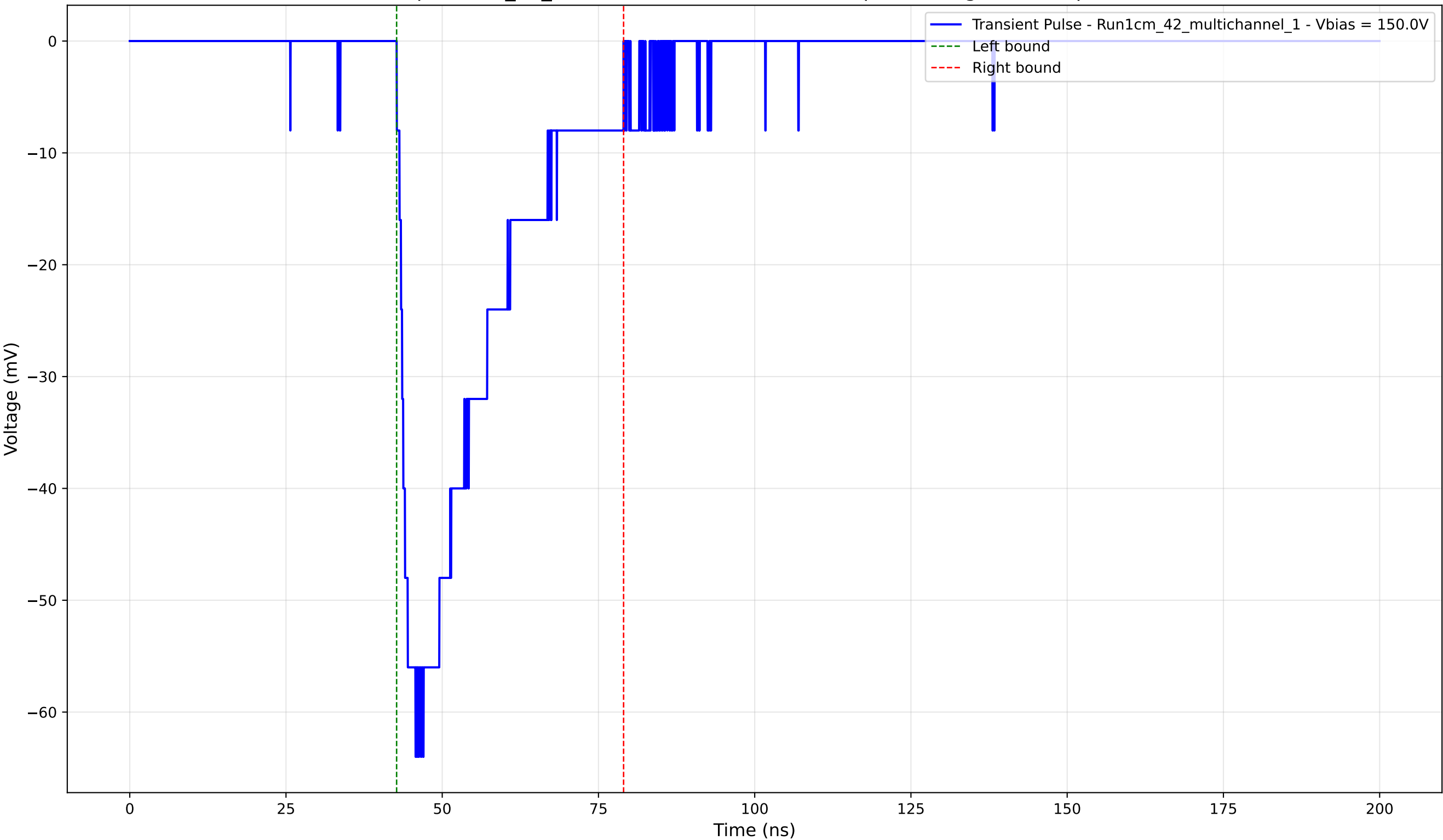
Transient Pulse - Sample: 1cm_42_multichannel - Position: 805.0 \mu\text{m} - Charge: -18.28 pC - Rise Time: 3.00 ns
