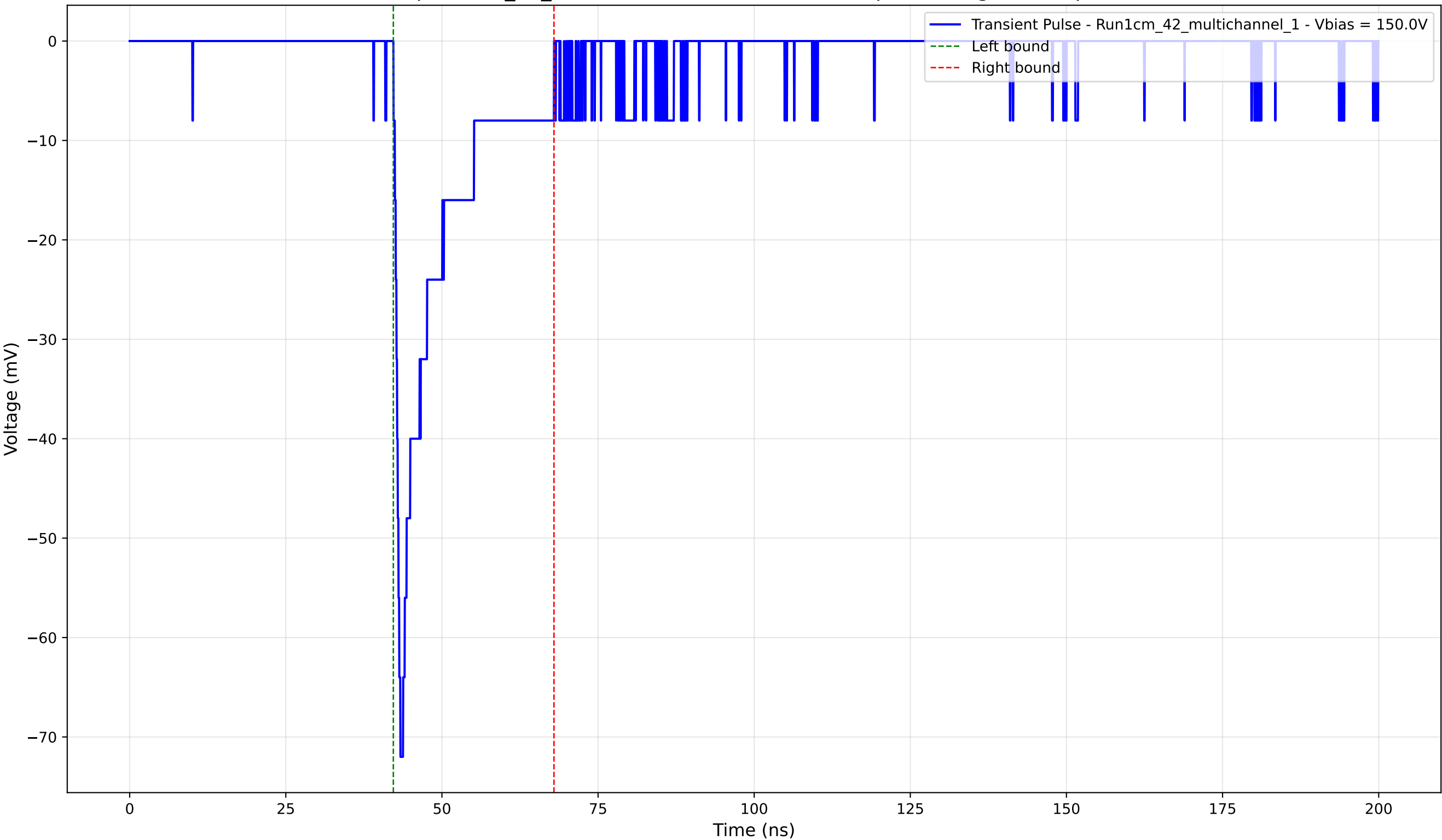
Transient Pulse - Sample: 1cm_42_multichannel - Position: 1835.0 \mu\text{m} - Charge: -9.46 pC - Rise Time: 1.10 ns
