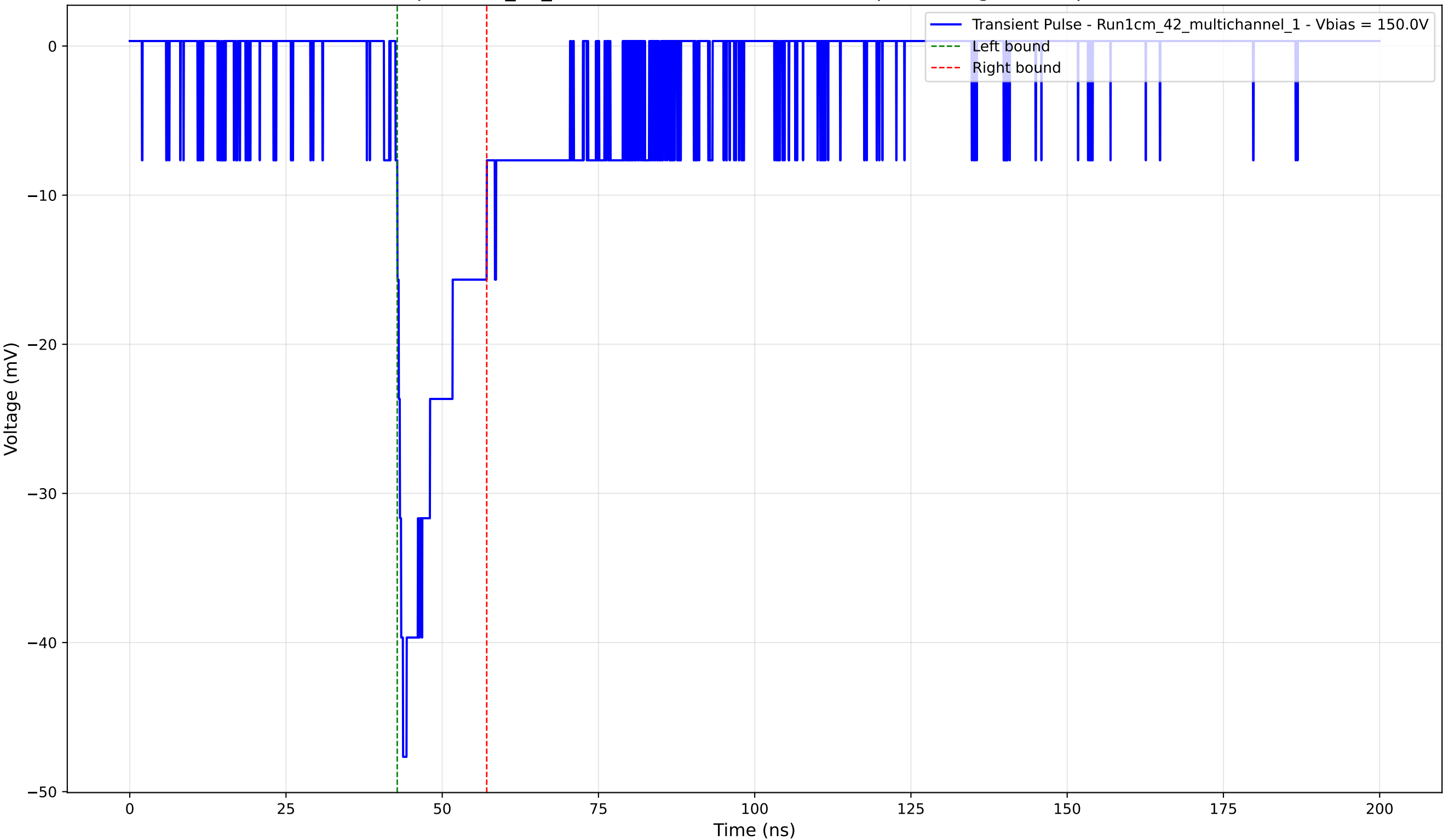
Transient Pulse - Sample: 1cm_42_multichannel - Position: 1420.0 \mu\text{m} - Charge: -7.20 pC - Rise Time: 1.21 ns
