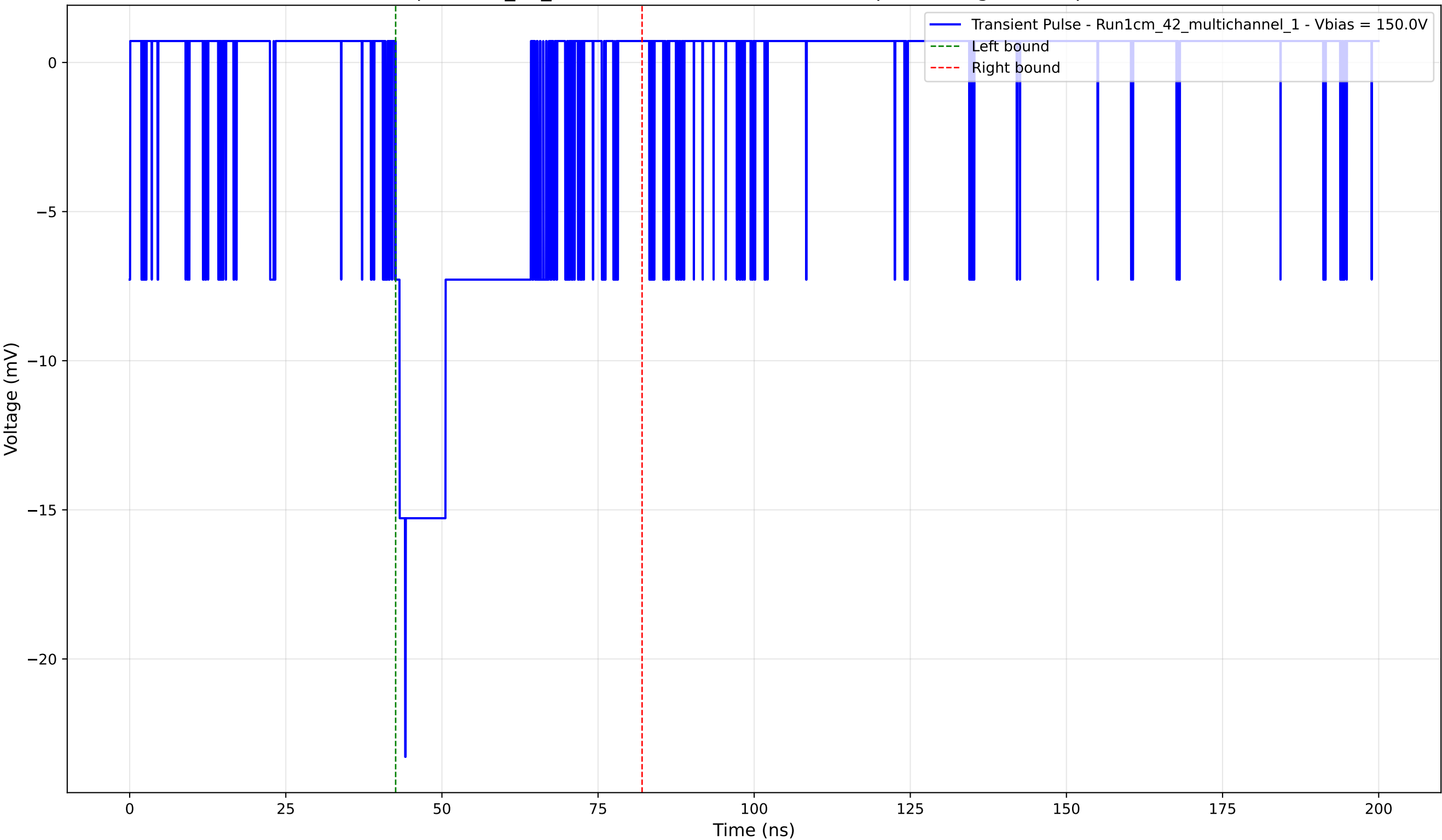
Transient Pulse - Sample: 1cm_42_multichannel - Position: 1340.0 \mu\text{m} - Charge: -4.89 pC - Rise Time: 1.54 ns
