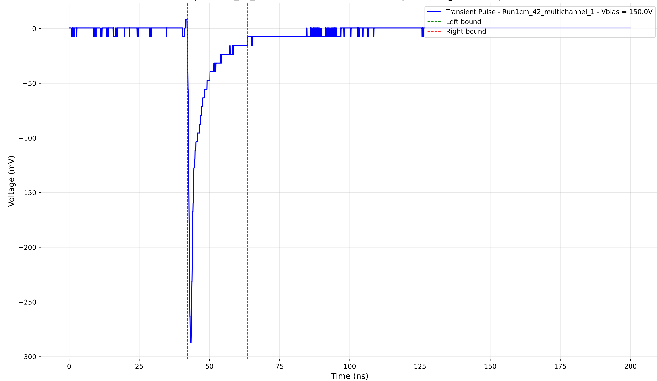
Transient Pulse - Sample: 1cm_42_multichannel - Position: 2070.0 \mu\text{m} - Charge: -23.55 pC - Rise Time: 0.79 ns
