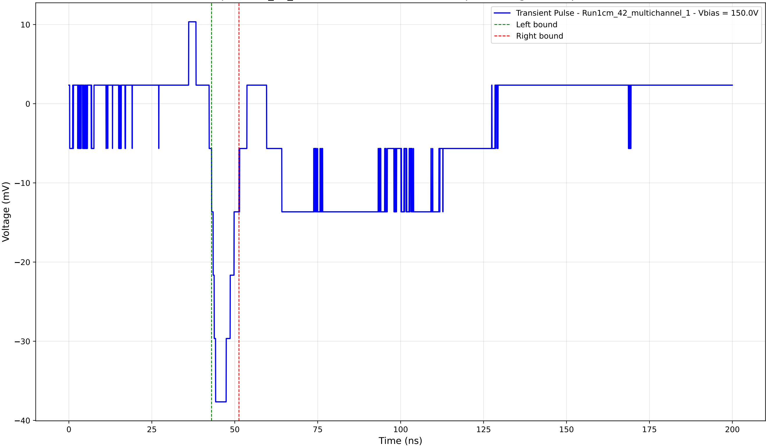
Transient Pulse - Sample: 1cm_42_multichannel - Position: 4780.0 \mu\text{m} - Charge: -4.54 pC - Rise Time: 1.95 ns
