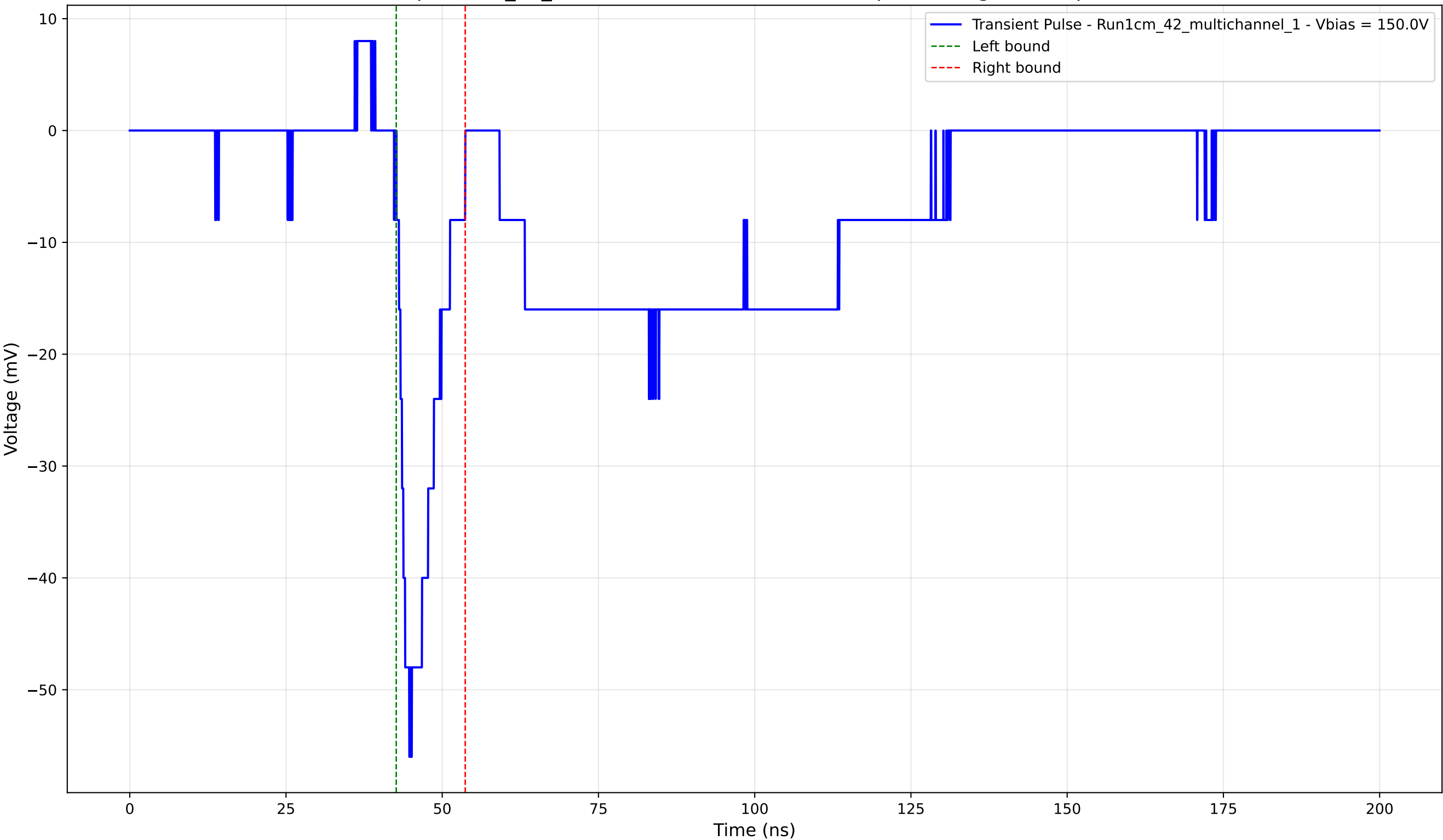
Transient Pulse - Sample: 1cm_42_multichannel - Position: 3995.0 \mu\text{m} - Charge: -6.02 pC - Rise Time: 2.07 ns
