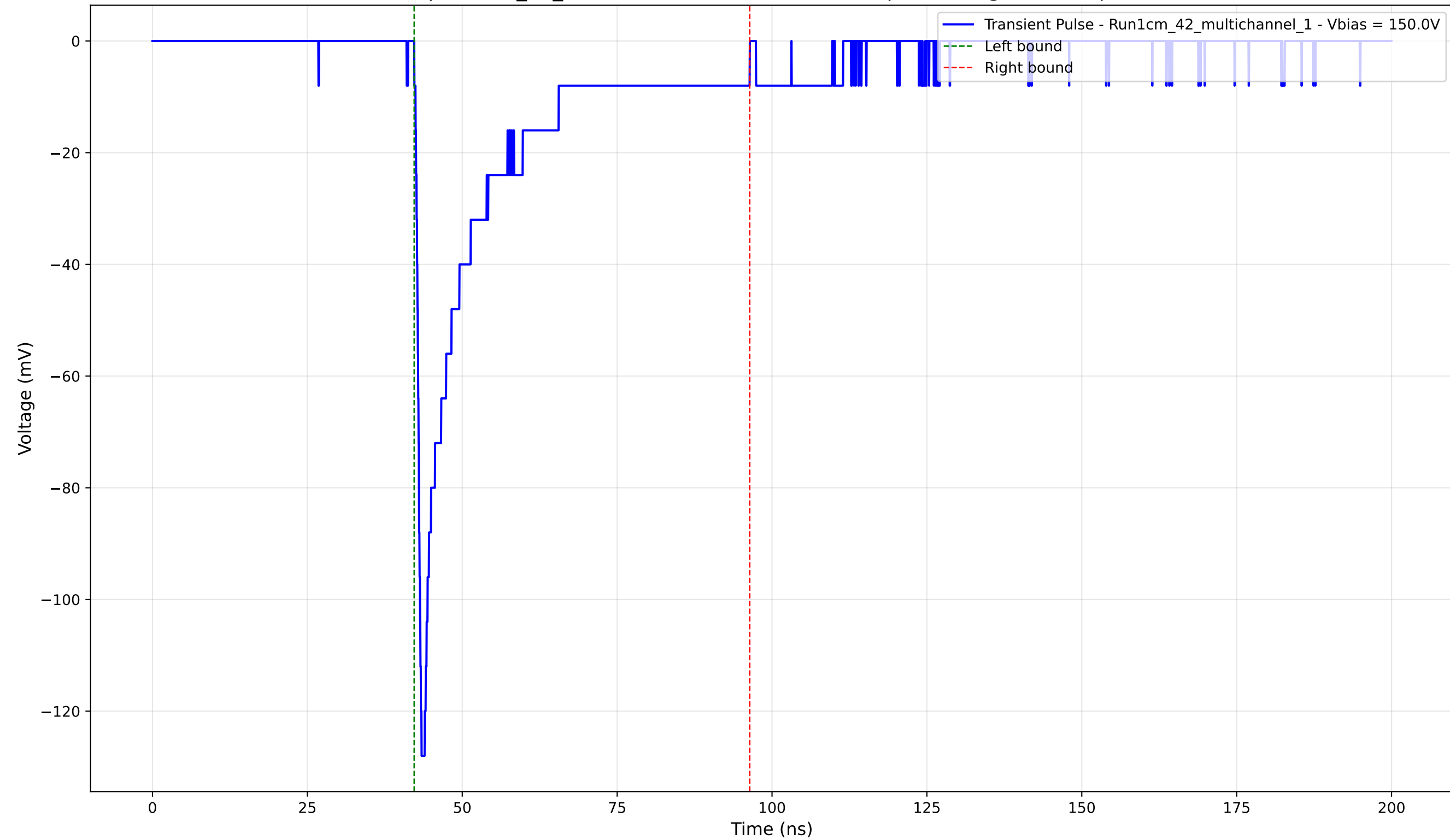
Transient Pulse - Sample: 1cm_42_multichannel - Position: 3115.0 \mu\text{m} - Charge: -23.04 pC - Rise Time: 0.87 ns
