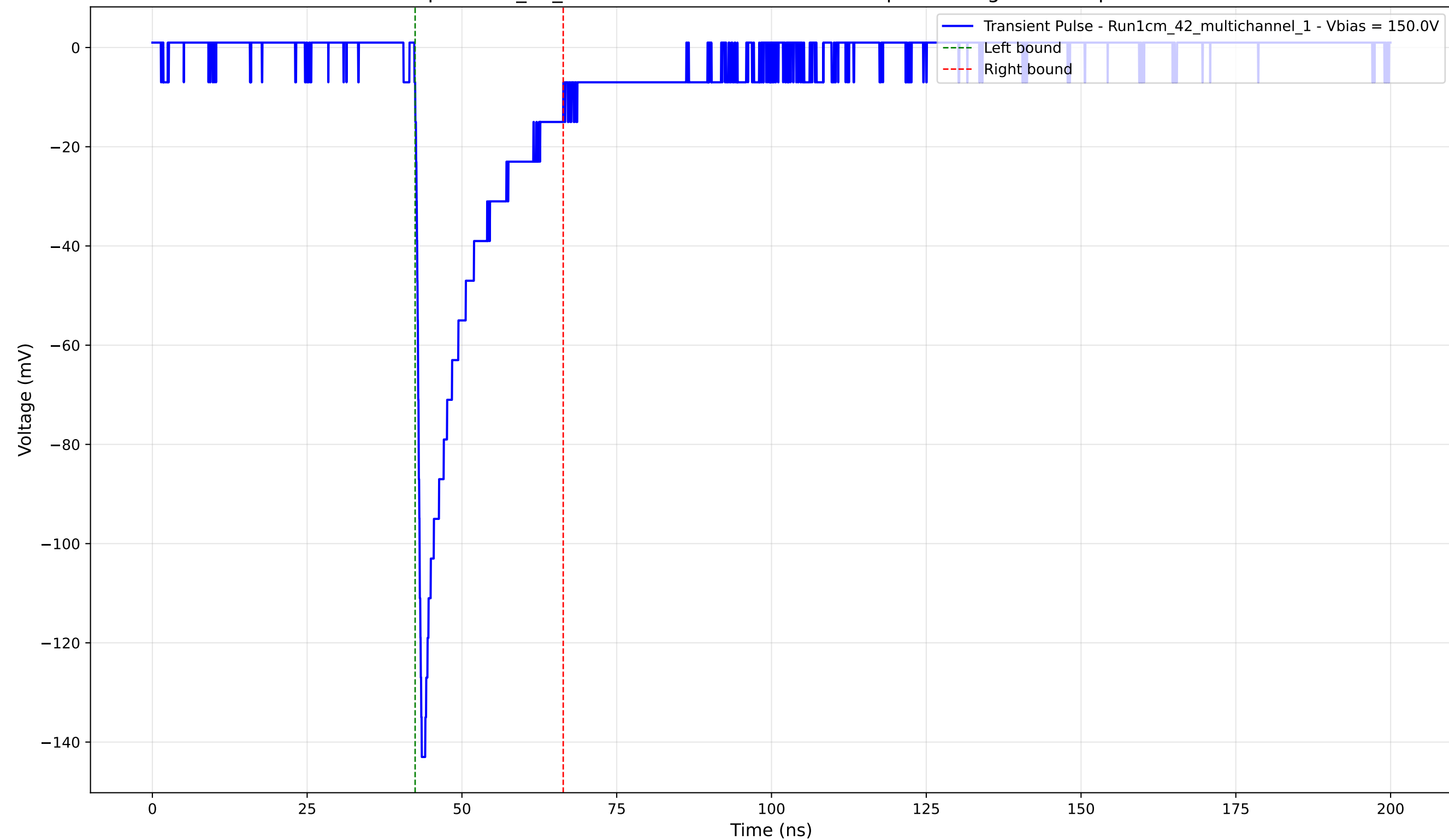
Transient Pulse - Sample: 1cm_42_multichannel - Position: 1625.0 \mu\text{m} - Charge: -22.31 pC - Rise Time: 0.96 ns
