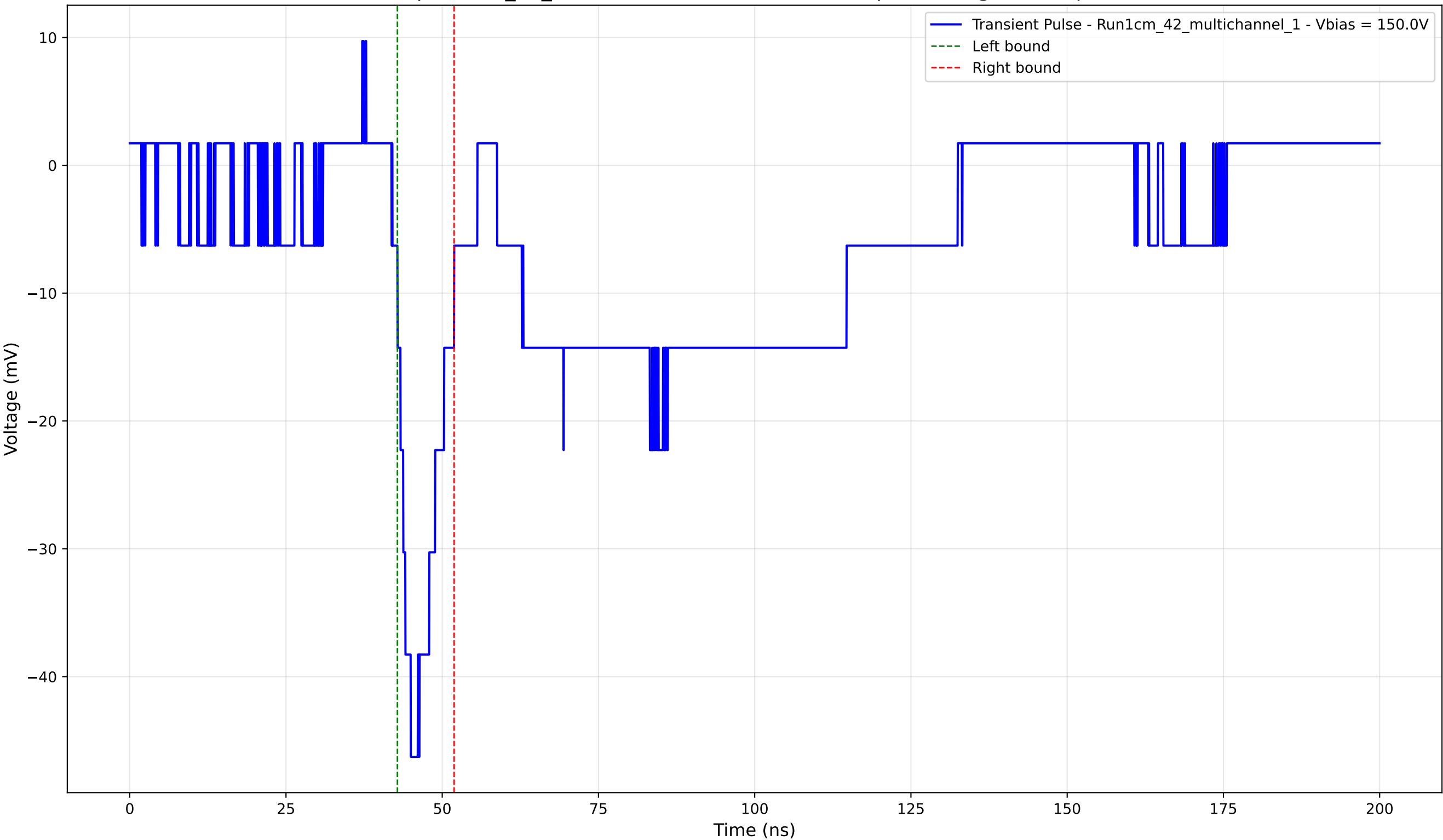
Transient Pulse - Sample: 1cm_42_multichannel - Position: 4760.0 \mu\text{m} - Charge: -5.33 pC - Rise Time: 2.95 ns
