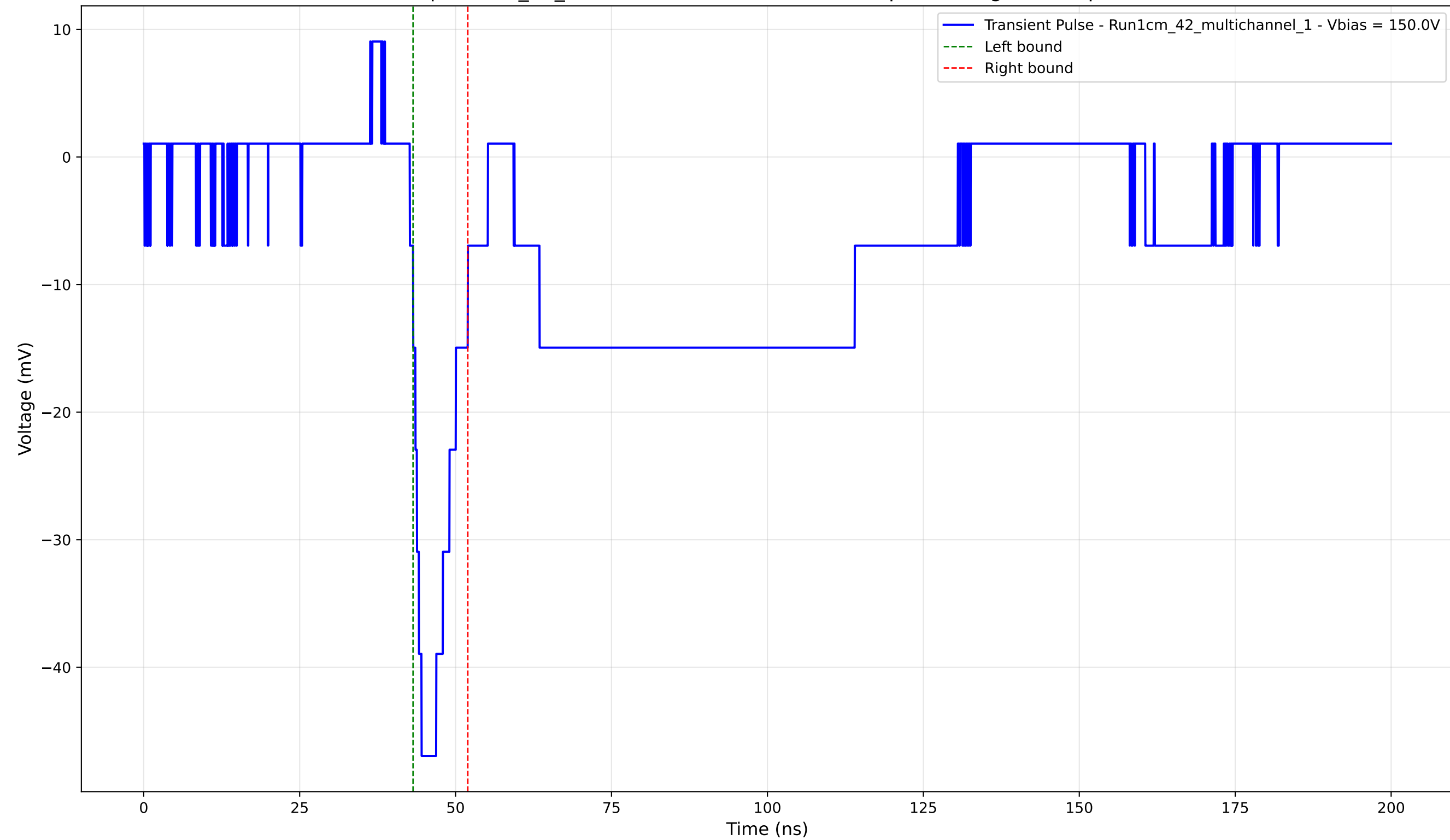
Transient Pulse - Sample: 1cm_42_multichannel - Position: 4245.0 \mu\text{m} - Charge: -5.49 pC - Rise Time: 1.89 ns
