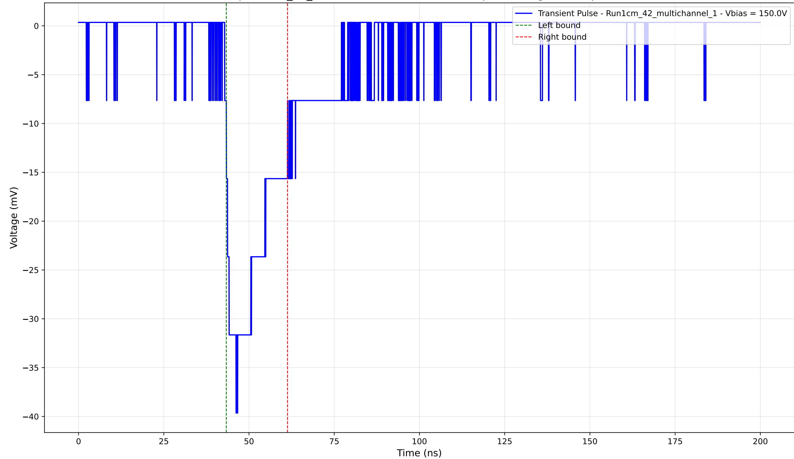
Transient Pulse - Sample: 1cm_42_multichannel - Position: 820.0 \mu\text{m} - Charge: -8.47 pC - Rise Time: 3.35 ns
