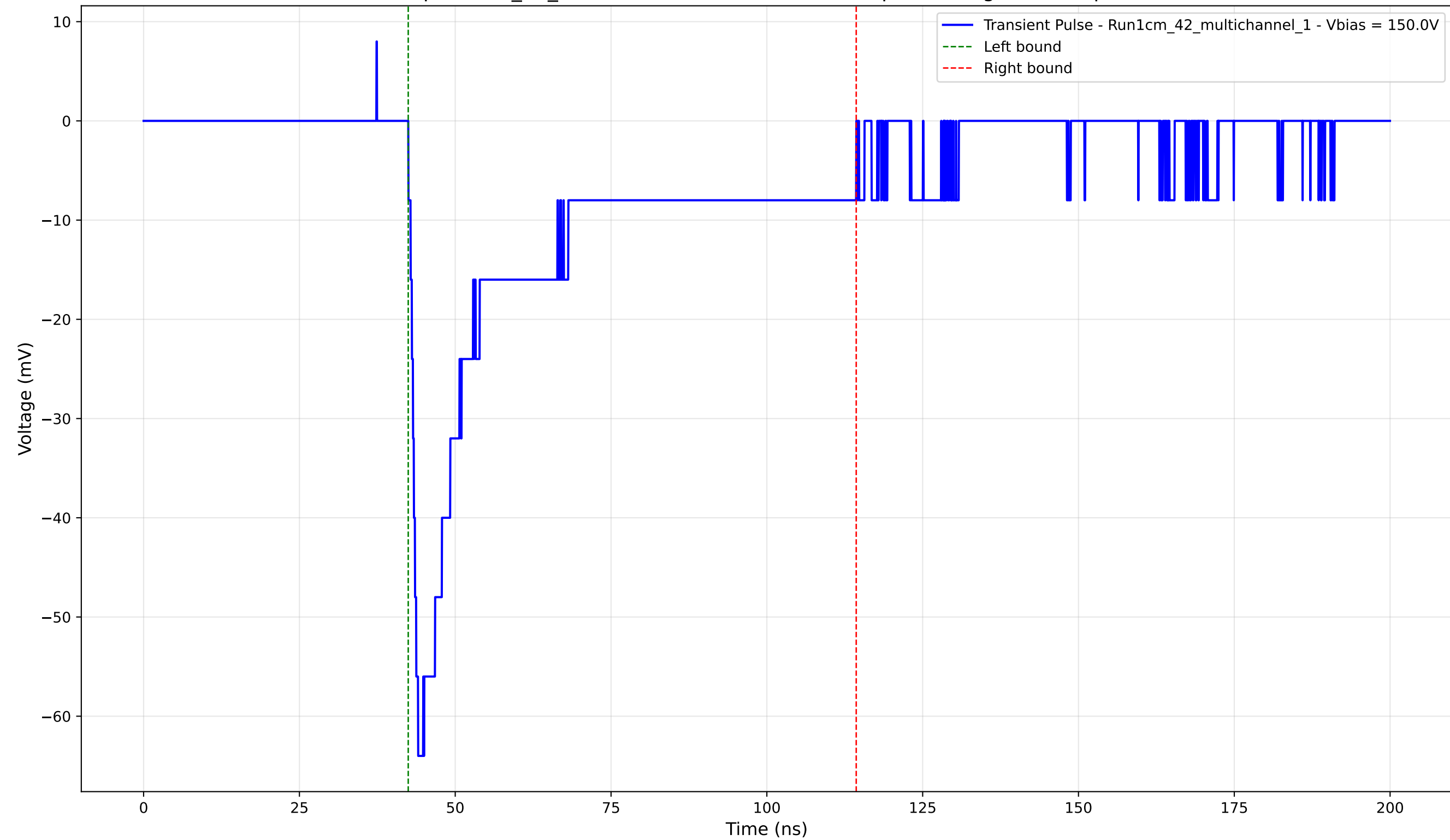
Transient Pulse - Sample: 1cm_42_multichannel - Position: 3705.0 \mu\text{m} - Charge: -20.63 pC - Rise Time: 1.56 ns
