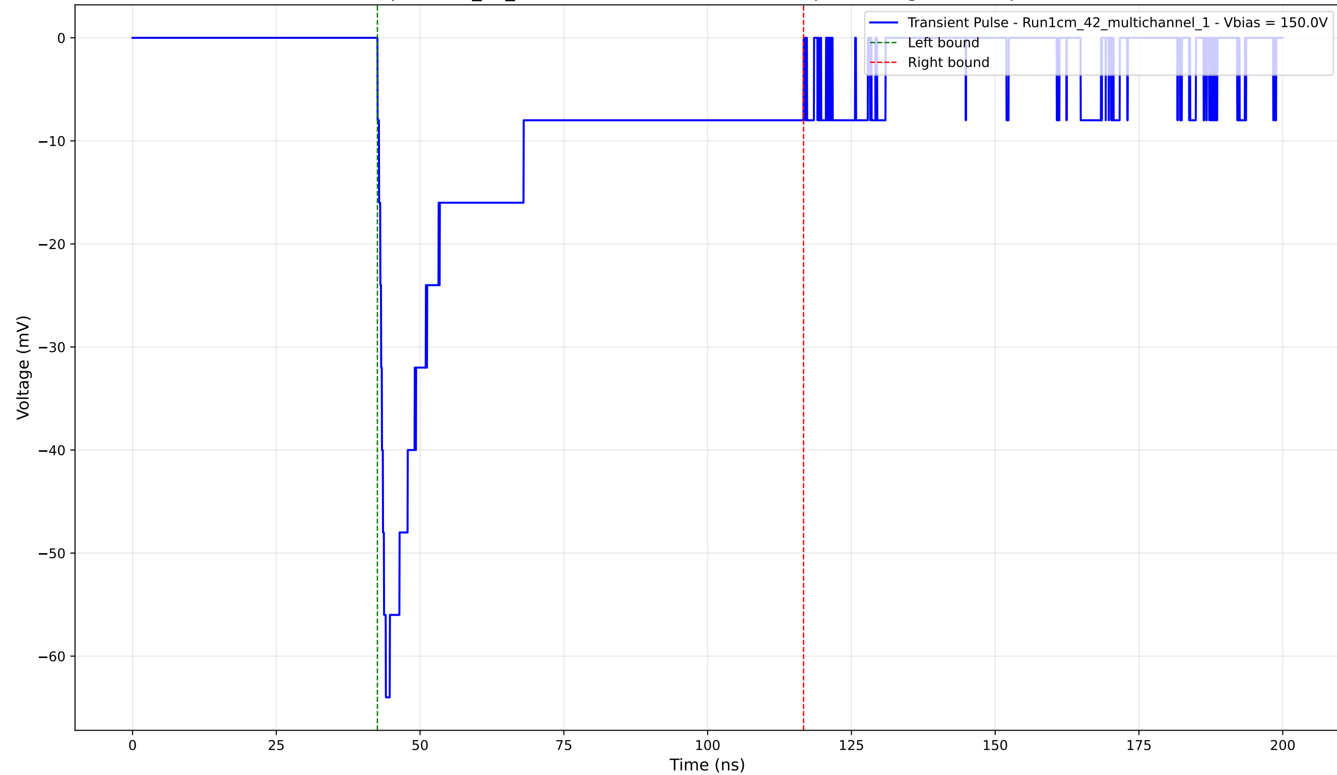
Transient Pulse - Sample: 1cm_42_multichannel - Position: 3680.0 \mu\text{m} - Charge: -20.93 pC - Rise Time: 1.44 ns
