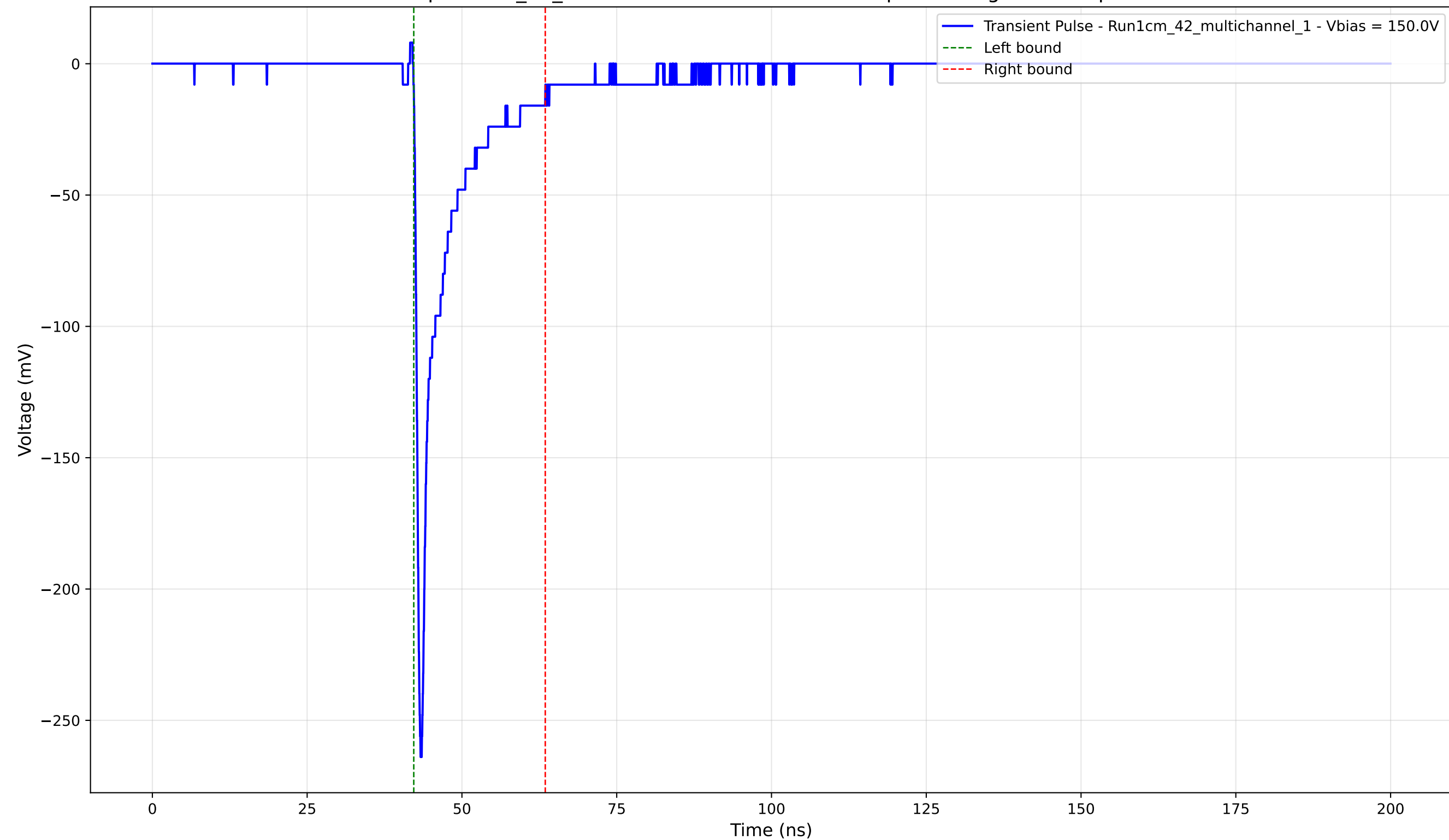
Transient Pulse - Sample: 1cm_42_multichannel - Position: 2010.0 \mu\text{m} - Charge: -23.44 pC - Rise Time: 0.79 ns
