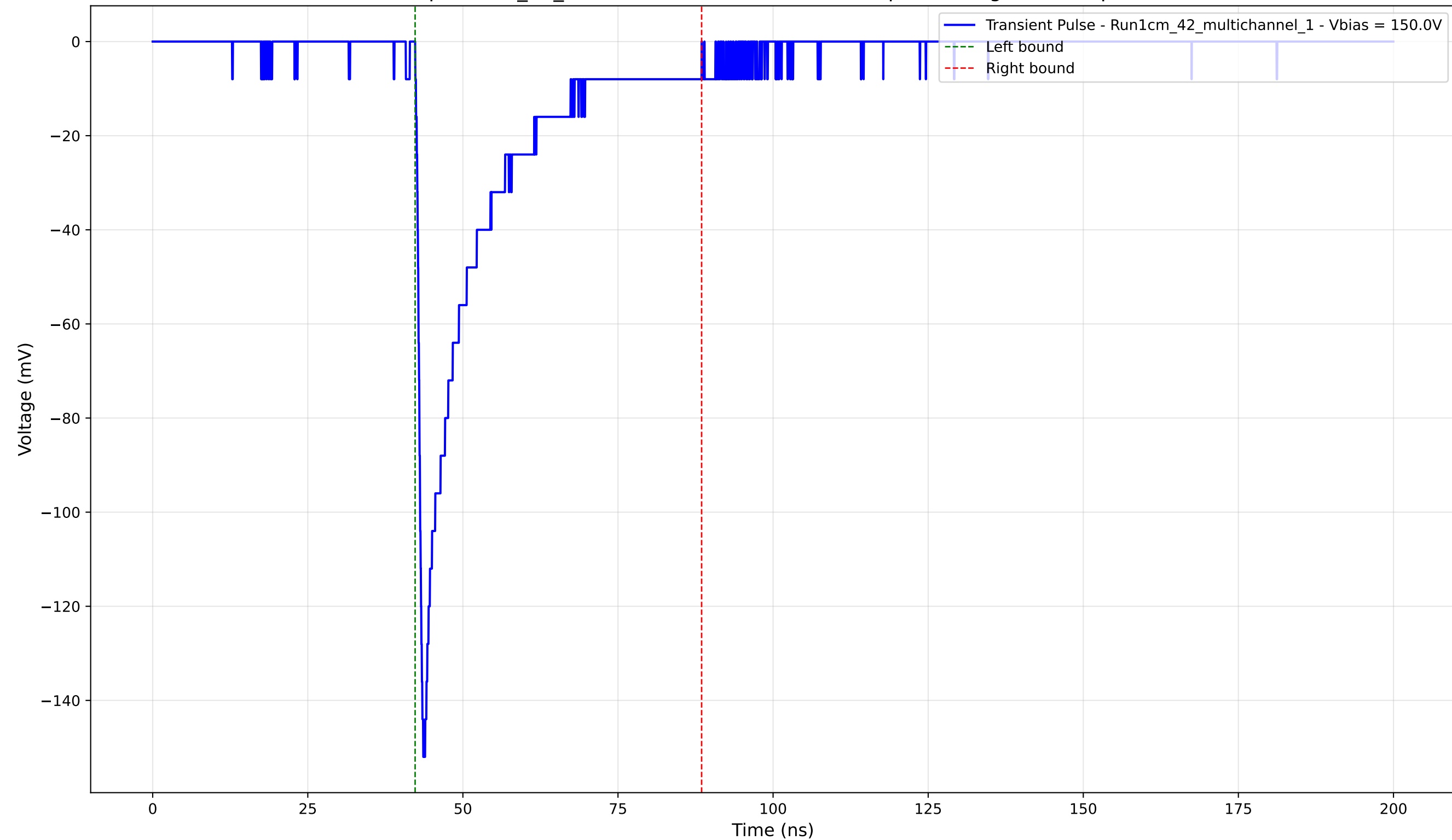
Transient Pulse - Sample: 1cm_42_multichannel - Position: 1635.0 \mu\text{m} - Charge: -26.74 pC - Rise Time: 1.02 ns
