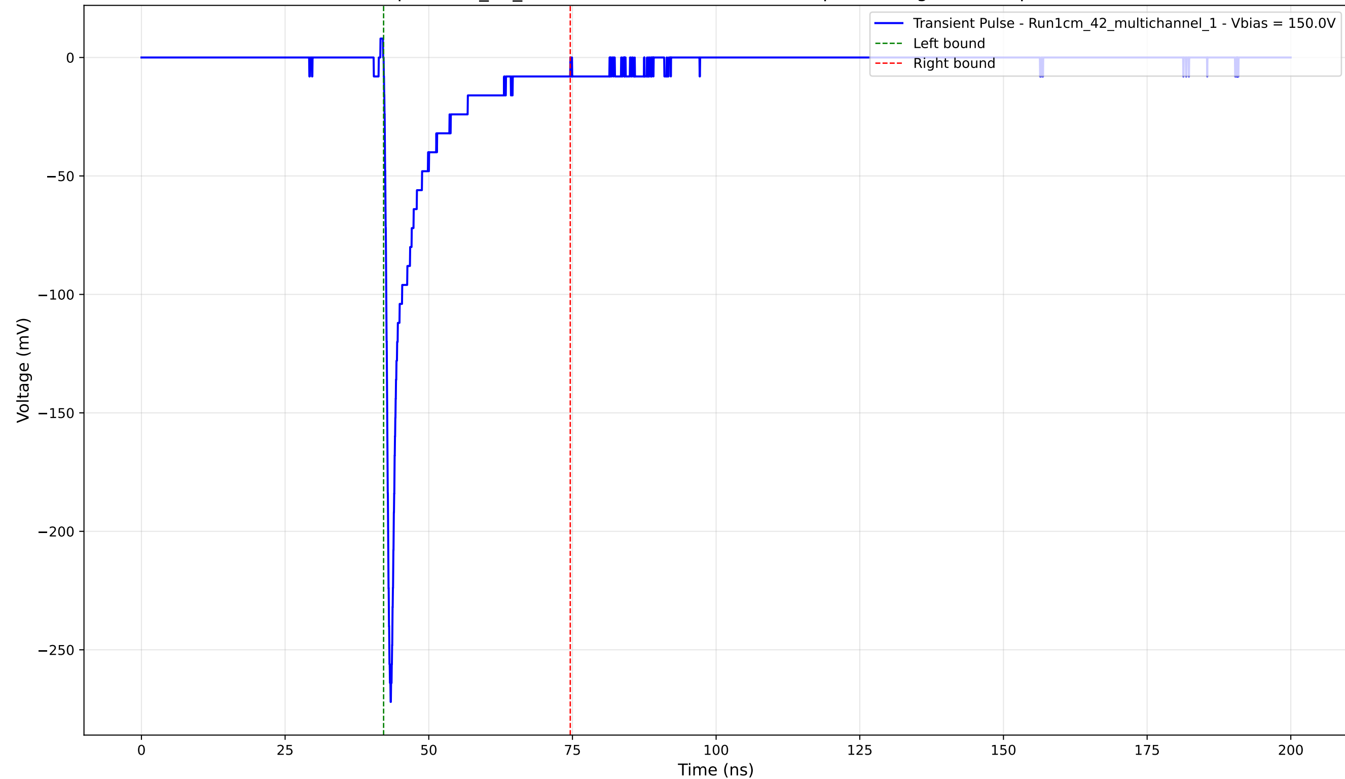
Transient Pulse - Sample: 1cm_42_multichannel - Position: 2725.0 \mu\text{m} - Charge: -24.15 pC - Rise Time: 0.79 ns
