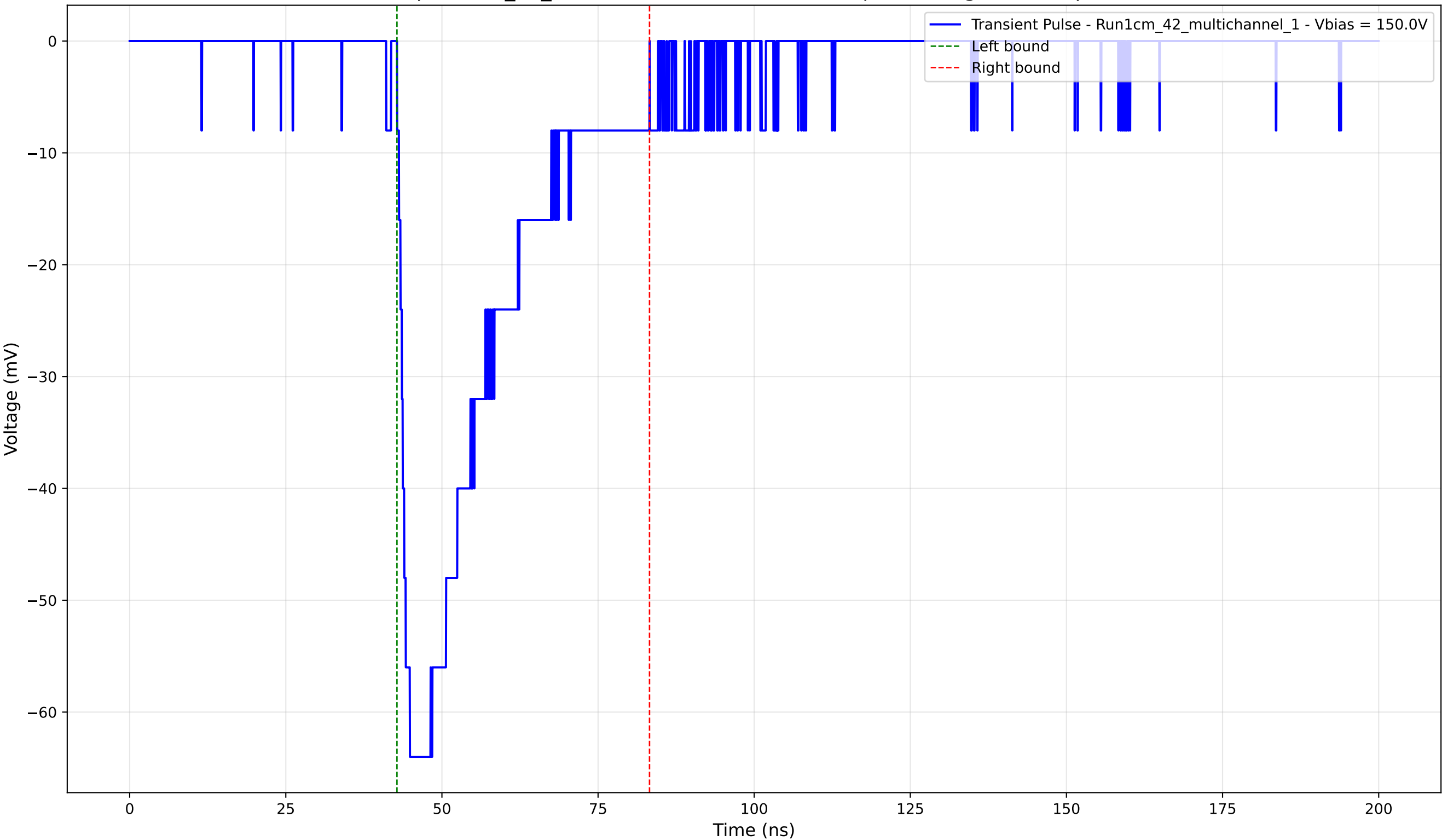
Transient Pulse - Sample: 1cm_42_multichannel - Position: 800.0 \mu\text{m} - Charge: -20.46 pC - Rise Time: 2.04 ns
