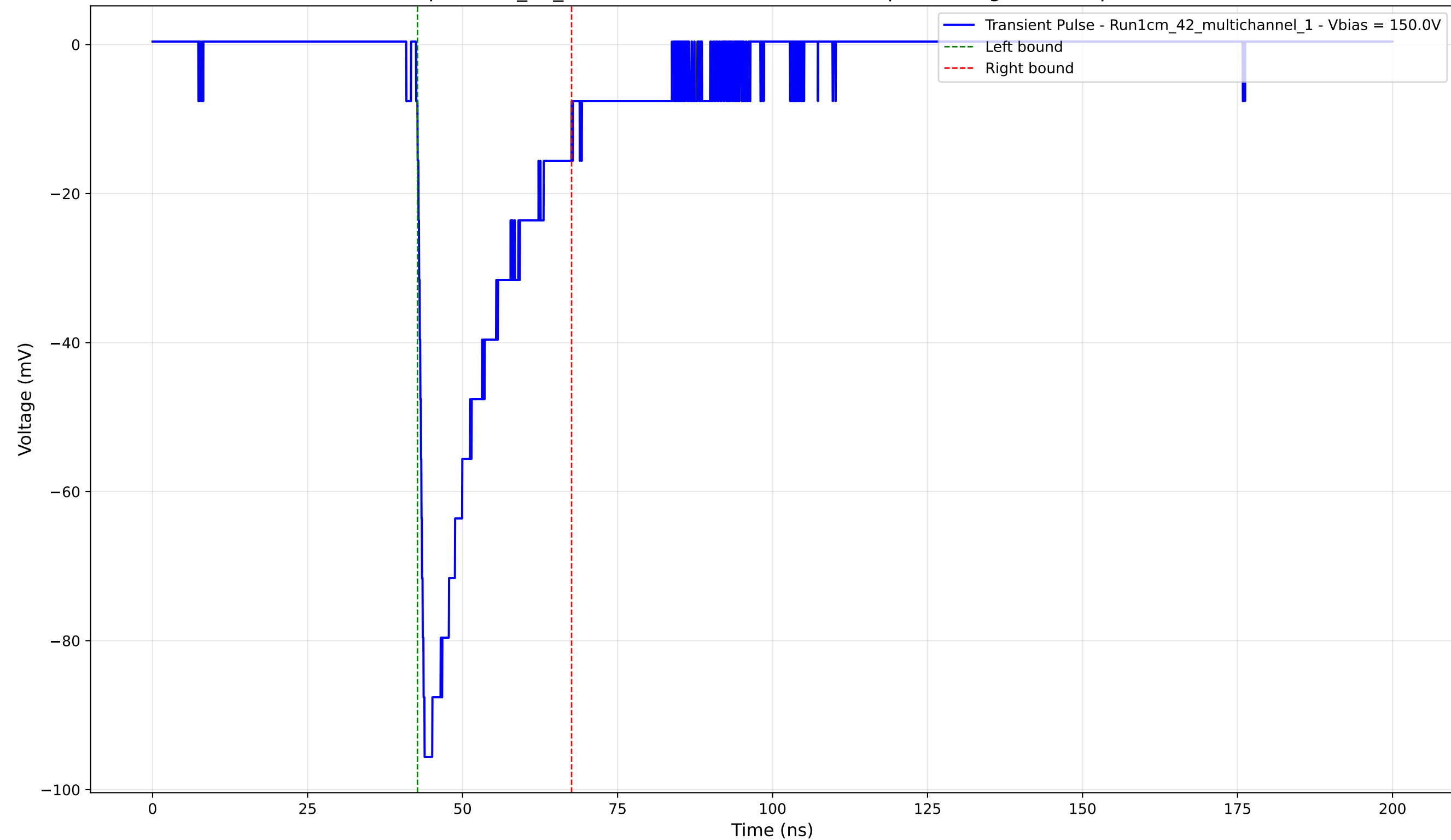
Transient Pulse - Sample: 1cm_42_multichannel - Position: 1280.0 \mu\text{m} - Charge: -21.70 pC - Rise Time: 0.98 ns
