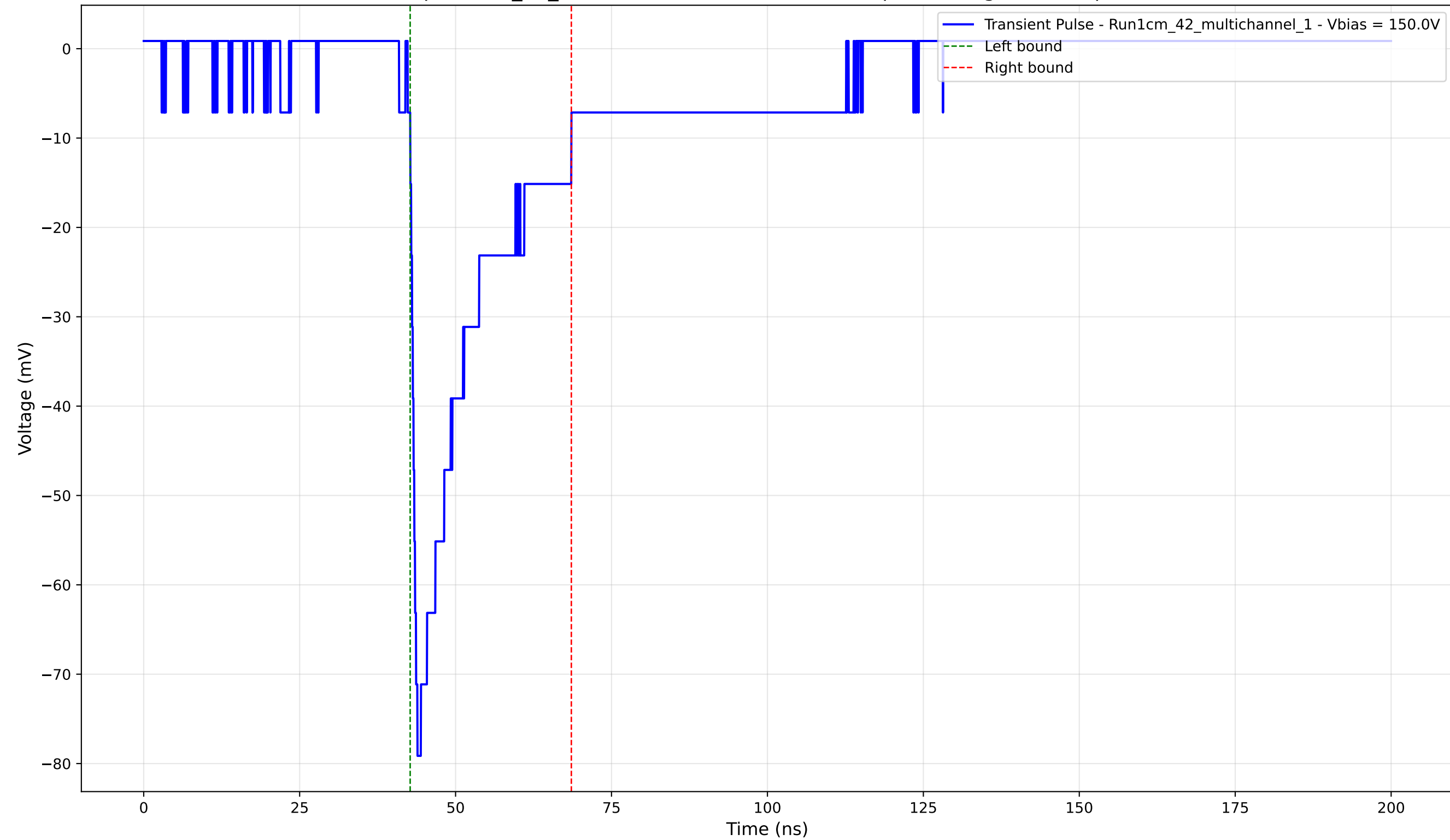
Transient Pulse - Sample: 1cm_42_multichannel - Position: 3535.0 \mu\text{m} - Charge: -16.34 pC - Rise Time: 1.16 ns
