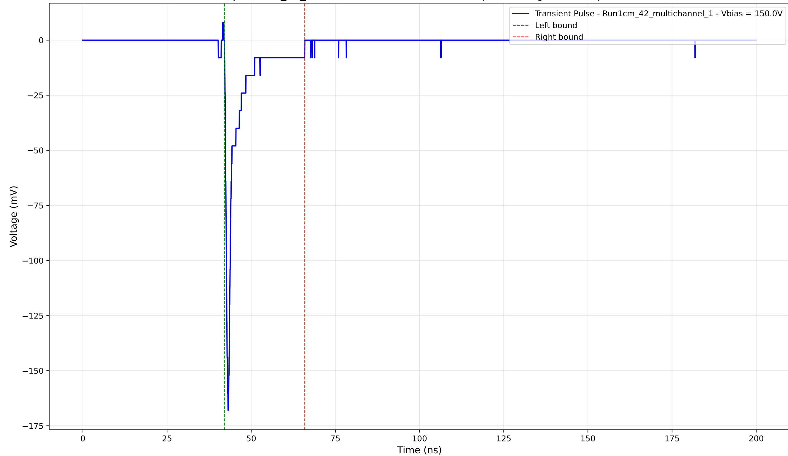
Transient Pulse - Sample: 1cm_42_multichannel - Position: 2340.0 \mu\text{m} - Charge: -10.63 pC - Rise Time: 0.72 ns
