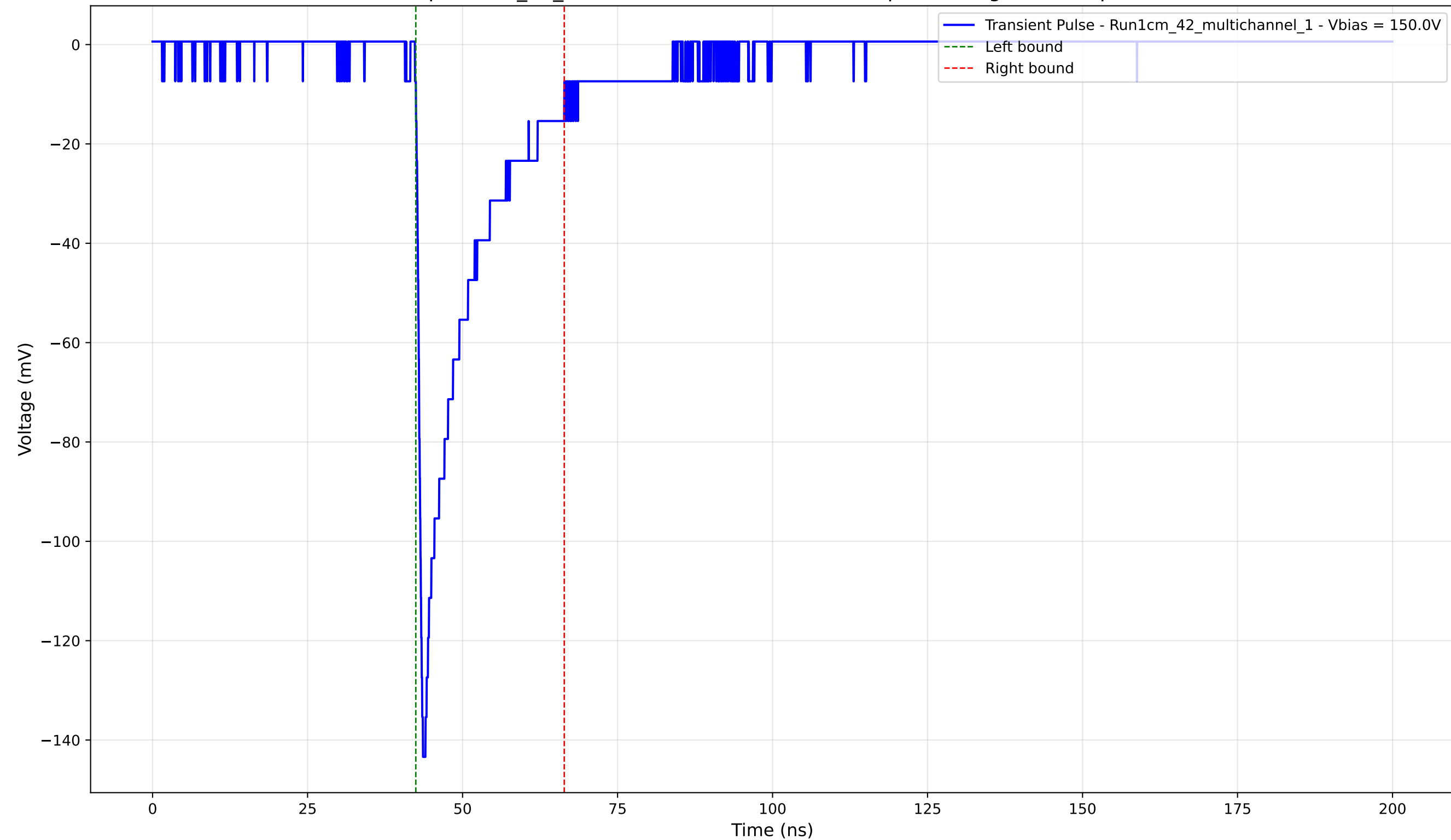
Transient Pulse - Sample: 1cm_42_multichannel - Position: 1600.0 \mu\text{m} - Charge: -22.46 pC - Rise Time: 1.00 ns
