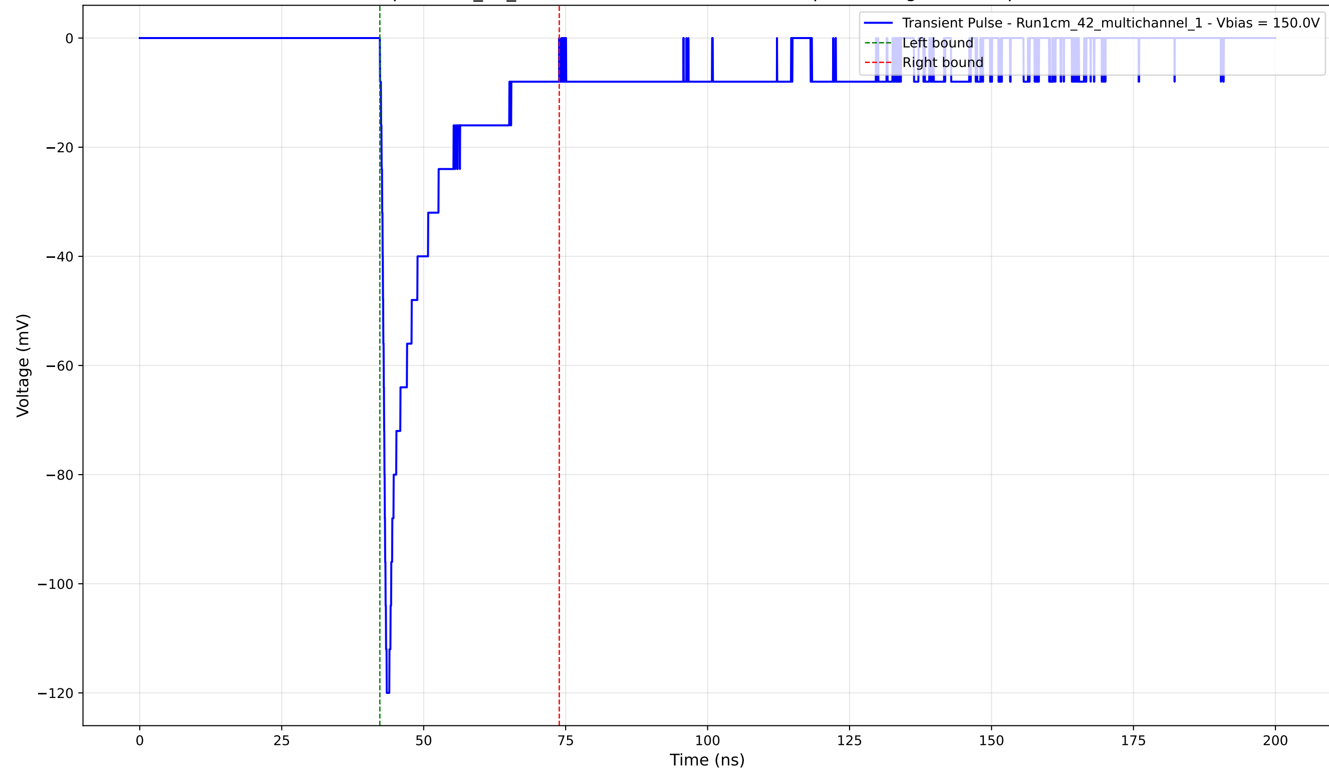
Transient Pulse - Sample: 1cm_42_multichannel - Position: 3160.0 \mu\text{m} - Charge: -17.67 pC - Rise Time: 0.89 ns
