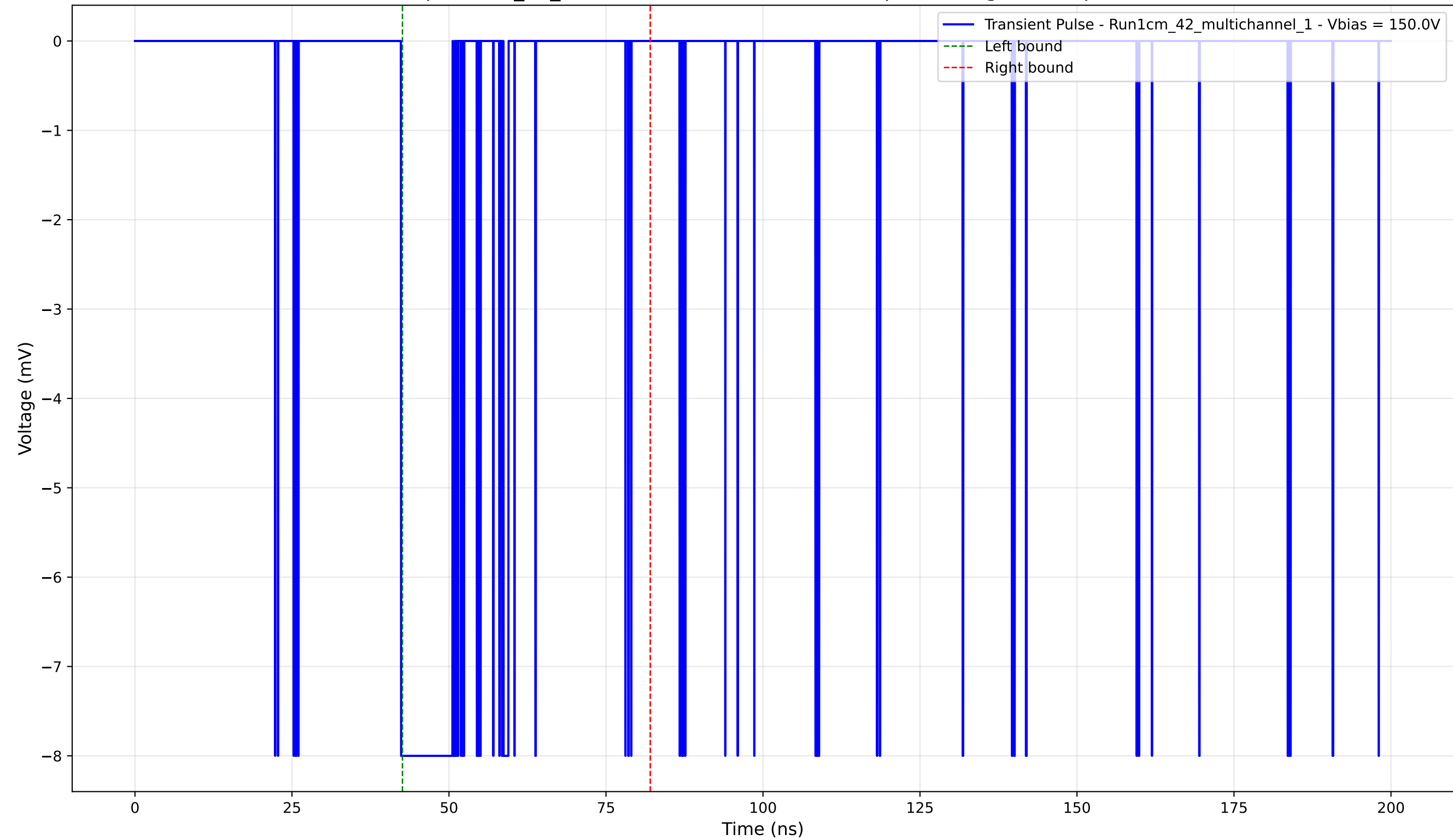
Transient Pulse - Sample: 1cm_42_multichannel - Position: 1870.0 \mu\text{m} - Charge: -1.66 pC - Rise Time: 0.02 ns
