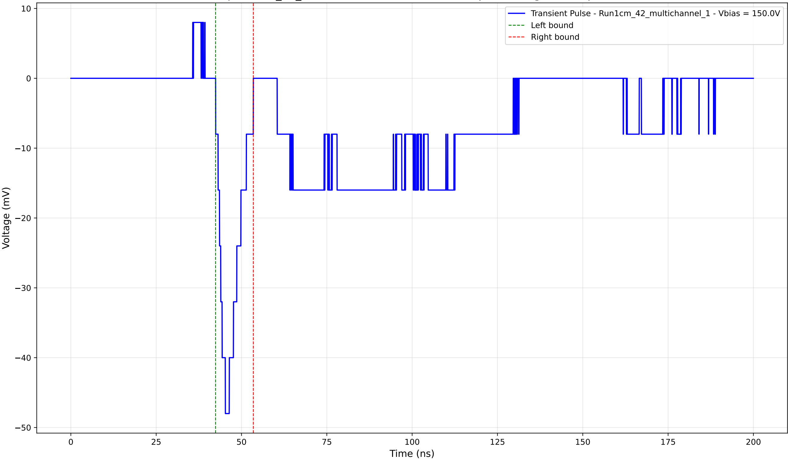
Transient Pulse - Sample: 1cm_42_multichannel - Position: 4675.0 \mu\text{m} - Charge: -5.56 pC - Rise Time: 2.85 ns
