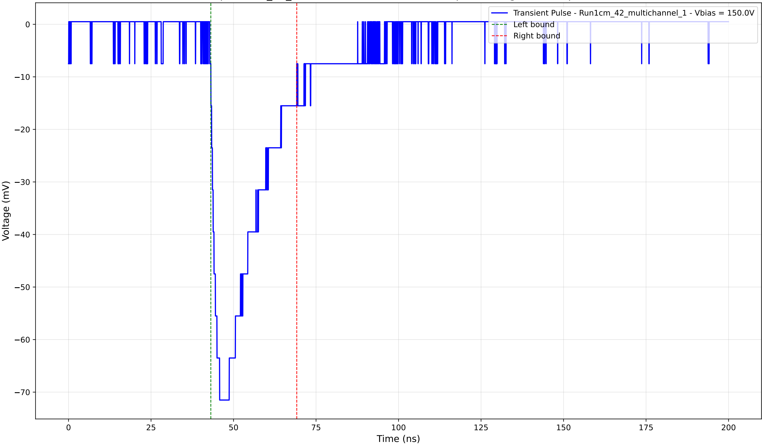
Transient Pulse - Sample: 1cm_42_multichannel - Position: 440.0 \mu\text{m} - Charge: -20.57 pC - Rise Time: 3.00 ns
