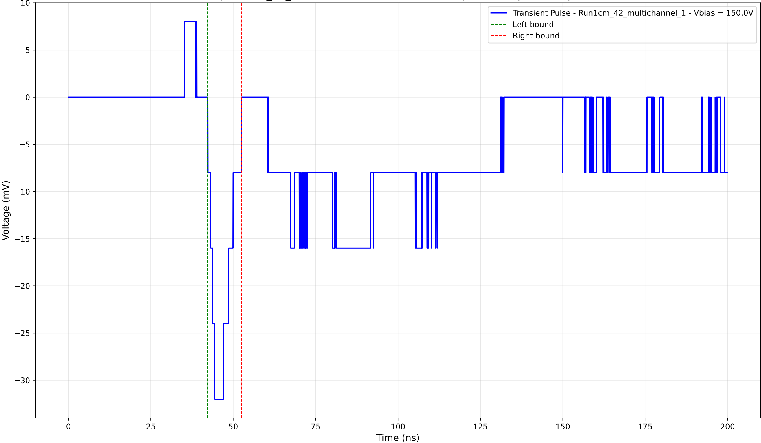
Transient Pulse - Sample: 1cm_42_multichannel - Position: 4840.0 \mu\text{m} - Charge: -3.94 pC - Rise Time: 2.09 ns
