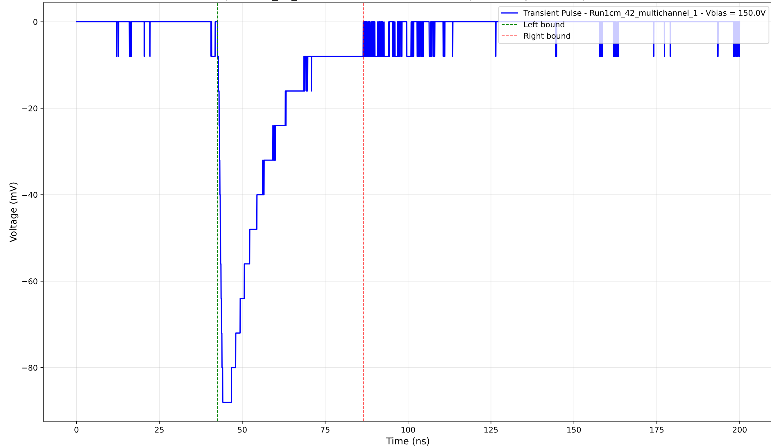
Transient Pulse - Sample: 1cm_42_multichannel - Position: 1115.0 \mu\text{m} - Charge: -25.47 pC - Rise Time: 1.06 ns
