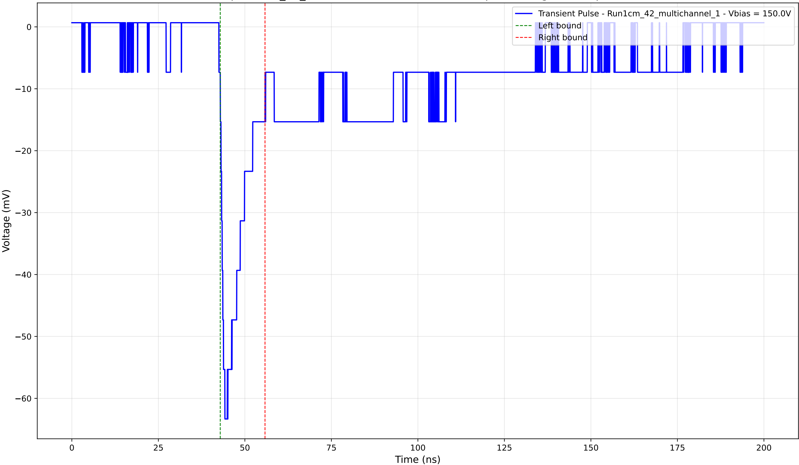
Transient Pulse - Sample: 1cm_42_multichannel - Position: 3765.0 \mu\text{m} - Charge: -8.49 pC - Rise Time: 1.72 ns
