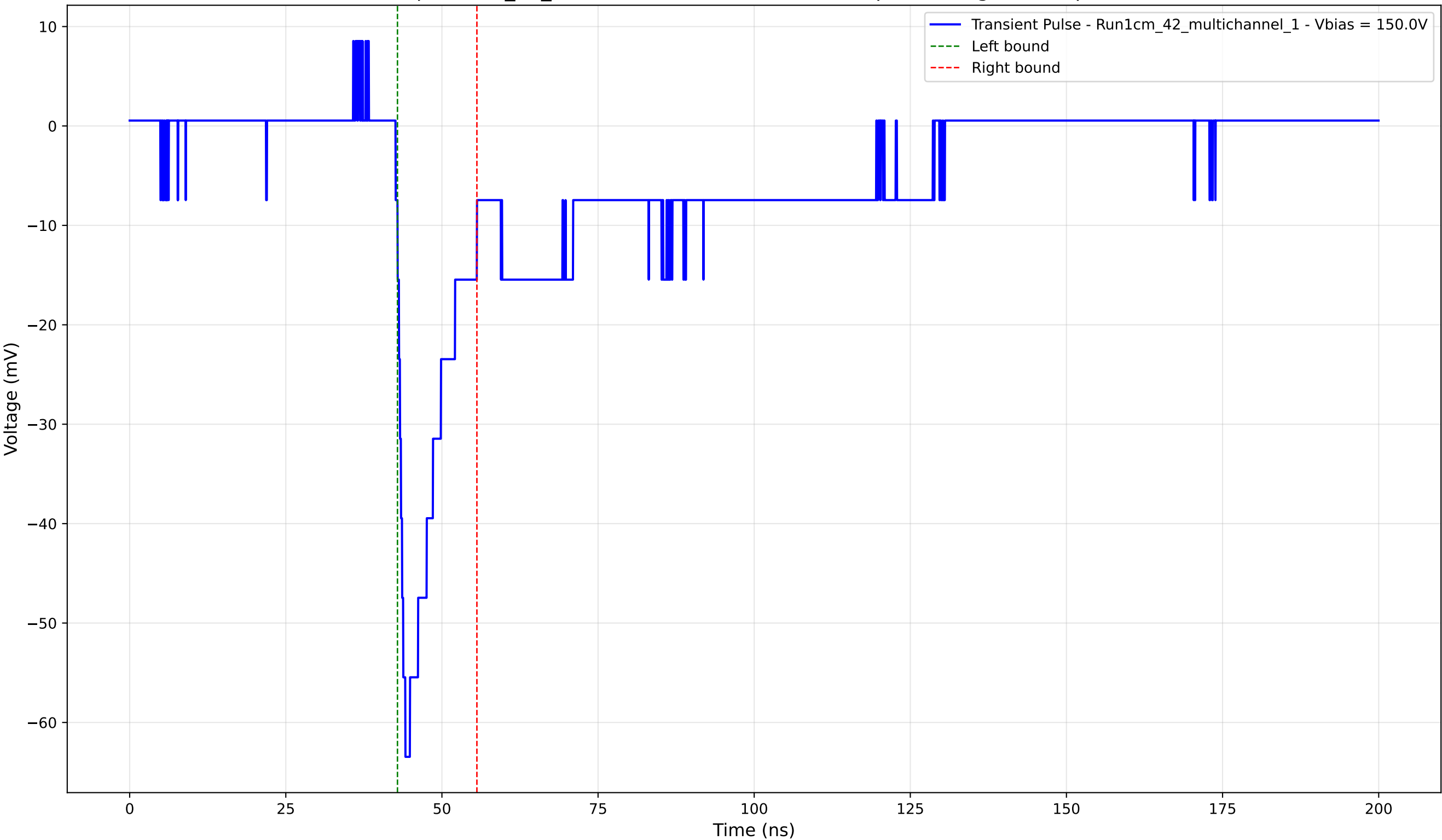
Transient Pulse - Sample: 1cm_42_multichannel - Position: 3745.0 \mu\text{m} - Charge: -8.36 pC - Rise Time: 1.56 ns
