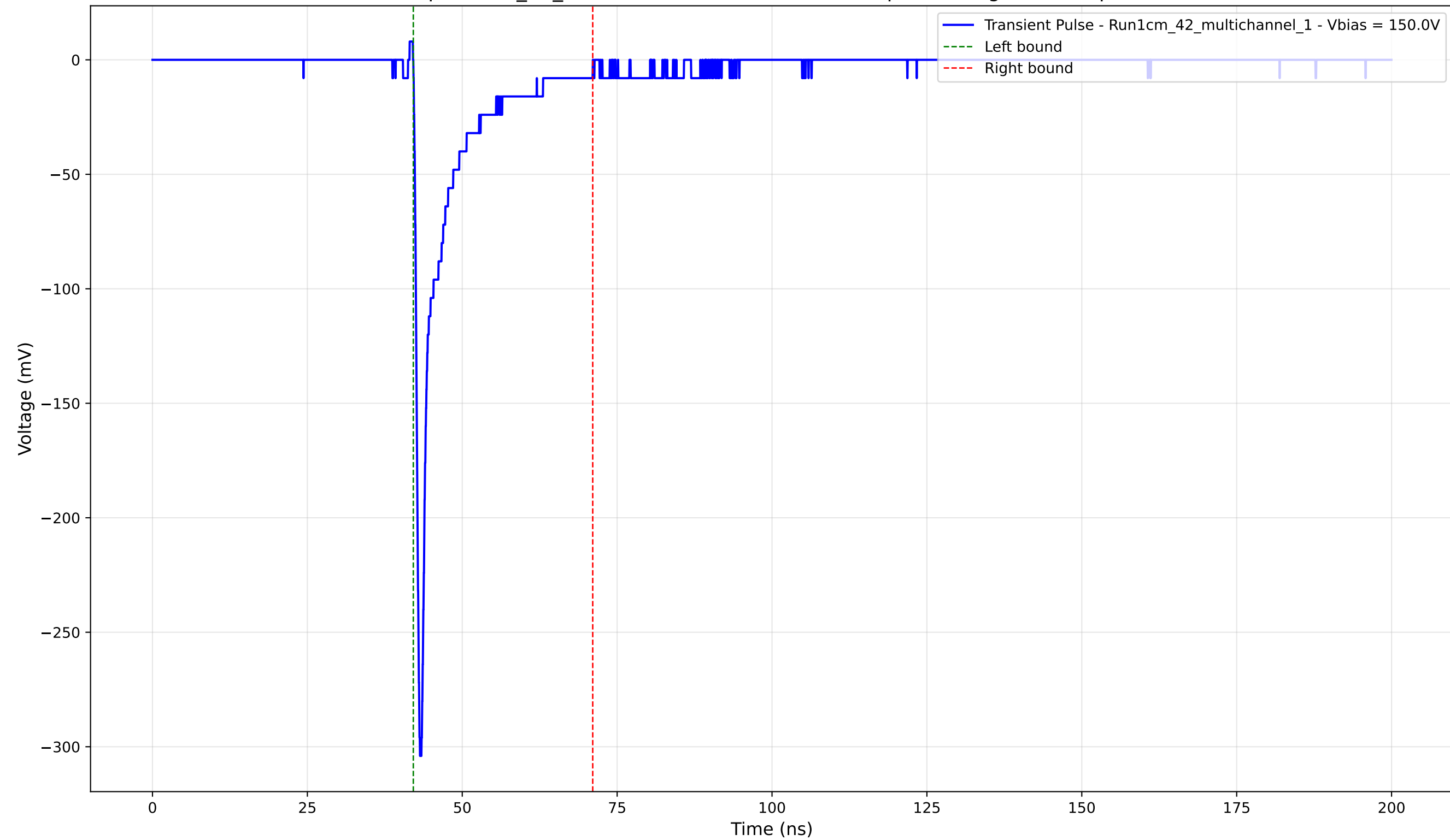
Transient Pulse - Sample: 1cm_42_multichannel - Position: 2640.0 \mu\text{m} - Charge: -23.91 pC - Rise Time: 0.77 ns
