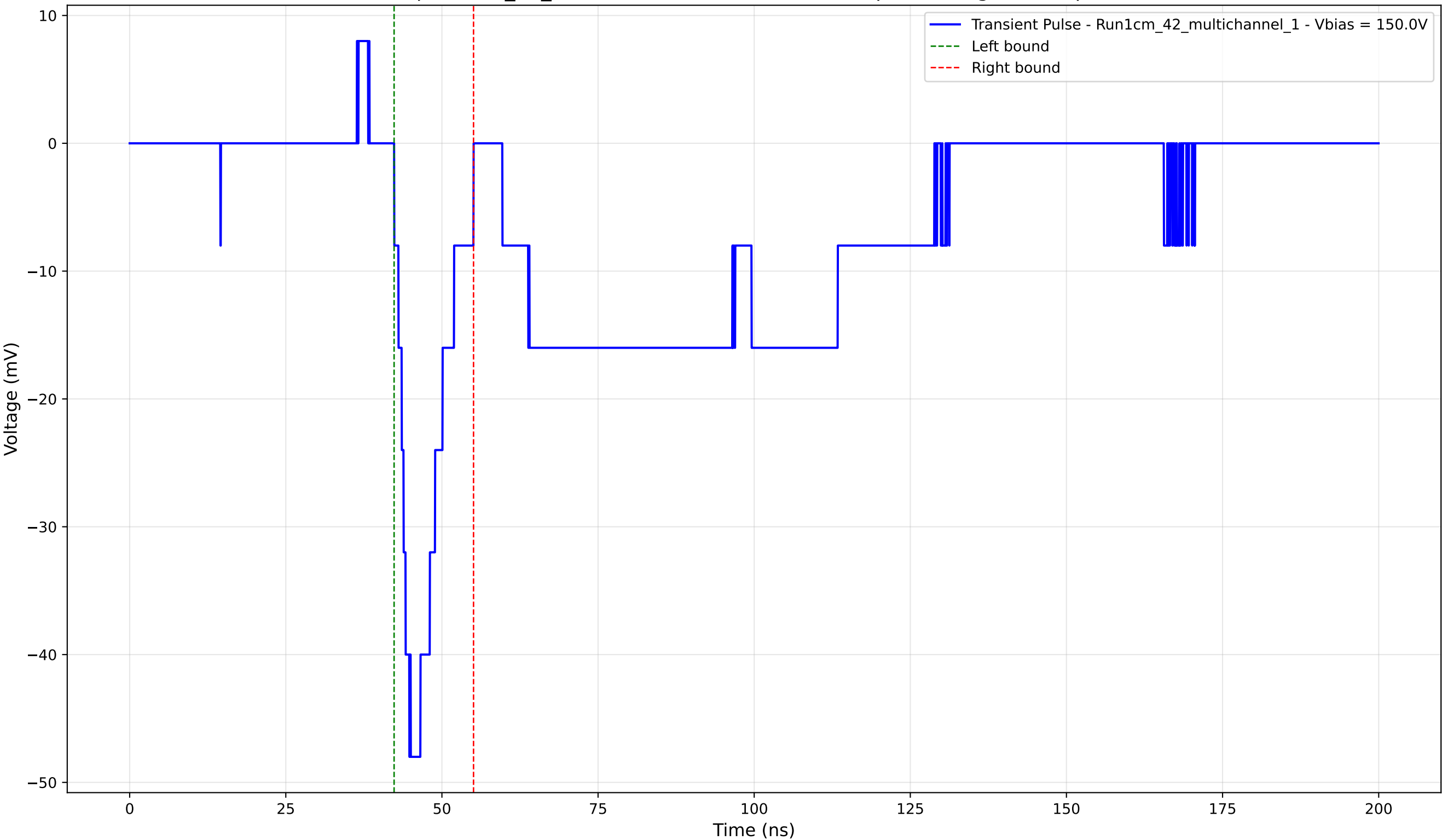
Transient Pulse - Sample: 1cm_42_multichannel - Position: 4660.0 \mu\text{m} - Charge: -6.20 pC - Rise Time: 2.43 ns
