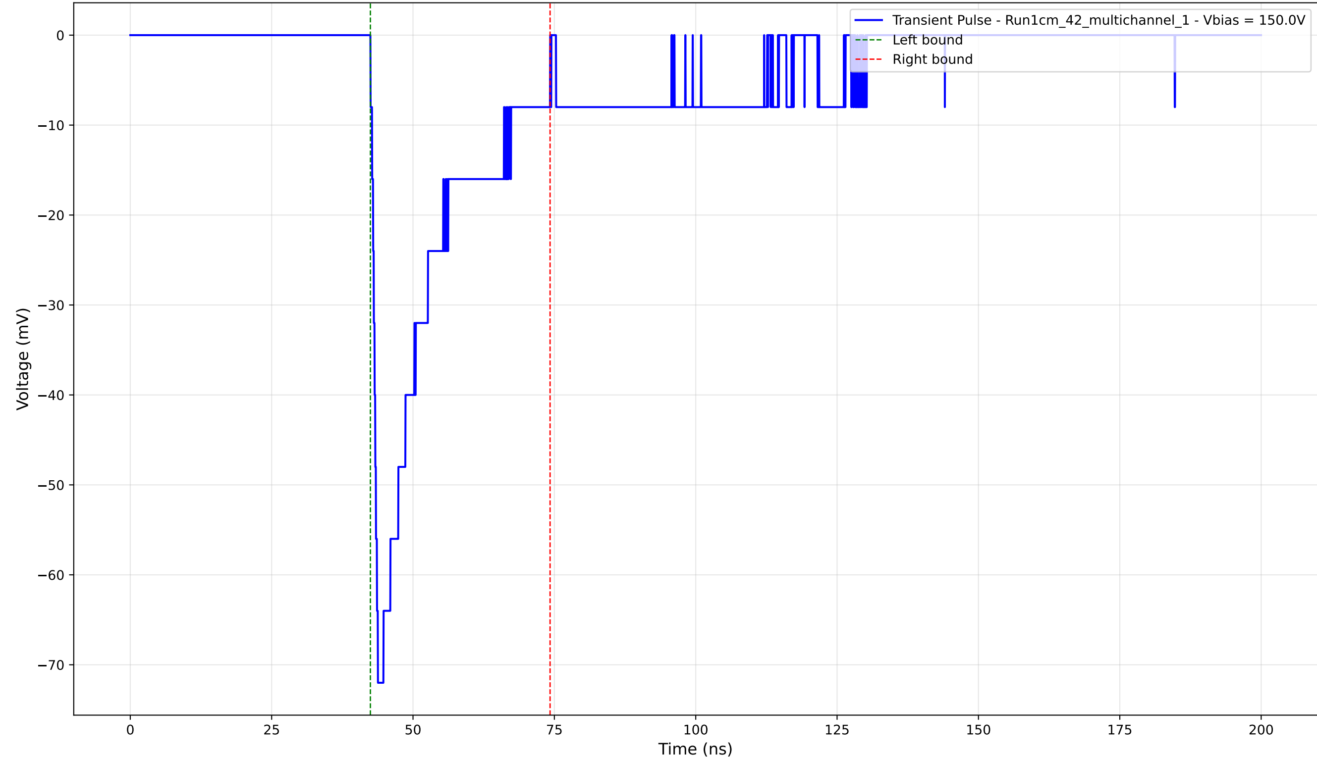
Transient Pulse - Sample: 1cm_42_multichannel - Position: 3555.0 \mu\text{m} - Charge: -15.73 pC - Rise Time: 1.30 ns
