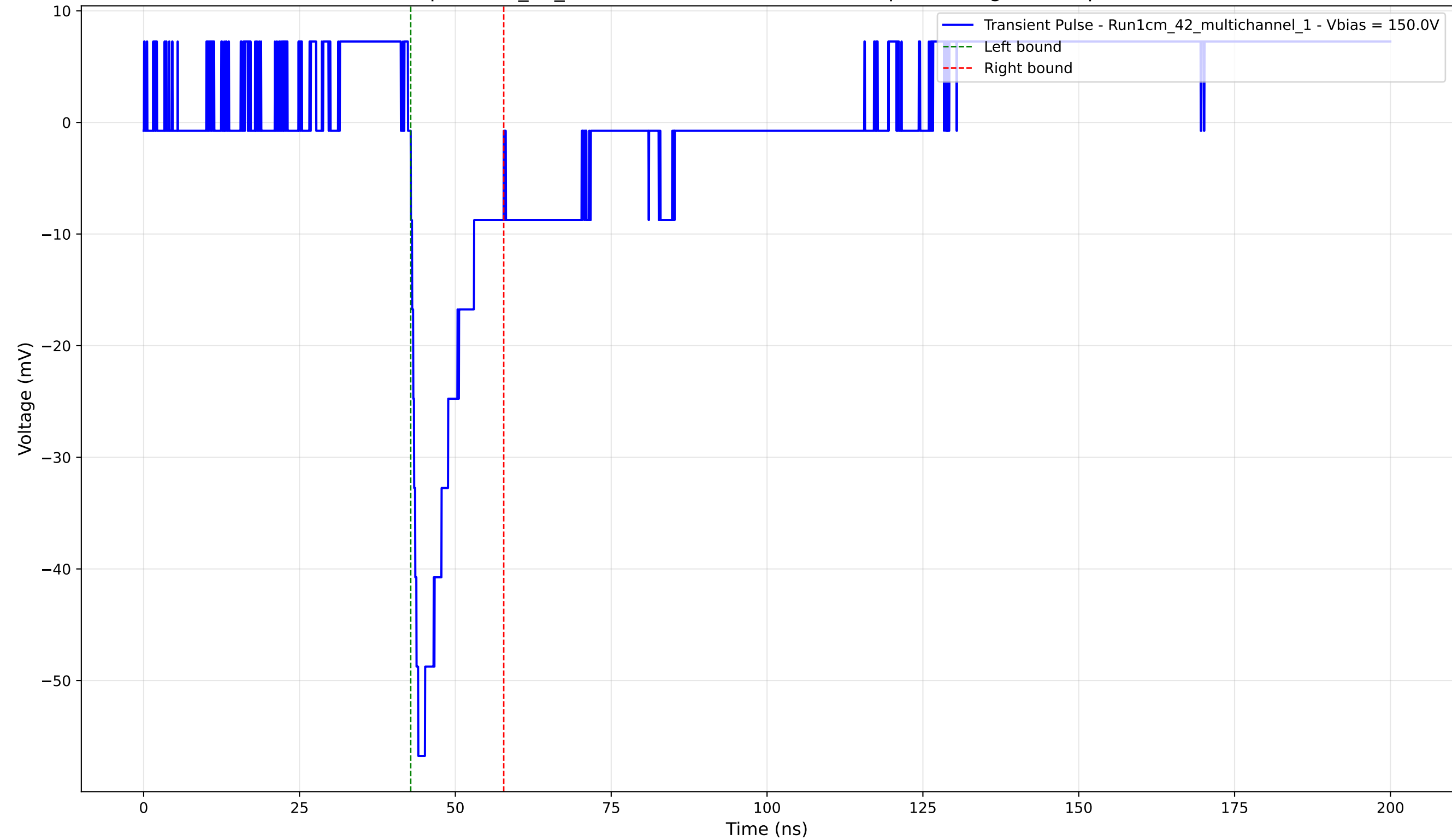
Transient Pulse - Sample: 1cm_42_multichannel - Position: 3725.0 \mu\text{m} - Charge: -7.54 pC - Rise Time: 1.19 ns
