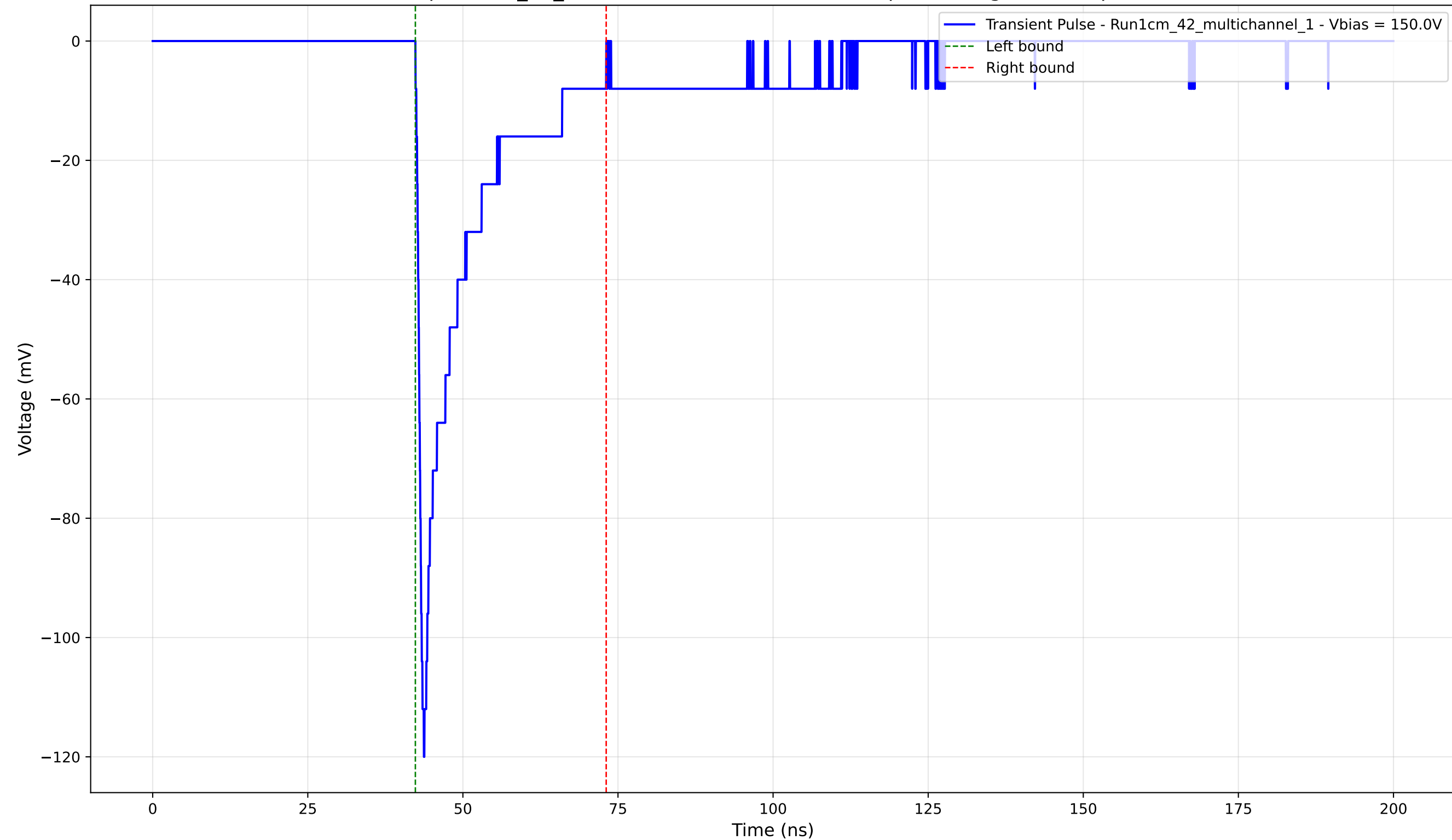
Transient Pulse - Sample: 1cm_42_multichannel - Position: 3200.0 \mu\text{m} - Charge: -17.57 pC - Rise Time: 0.99 ns
