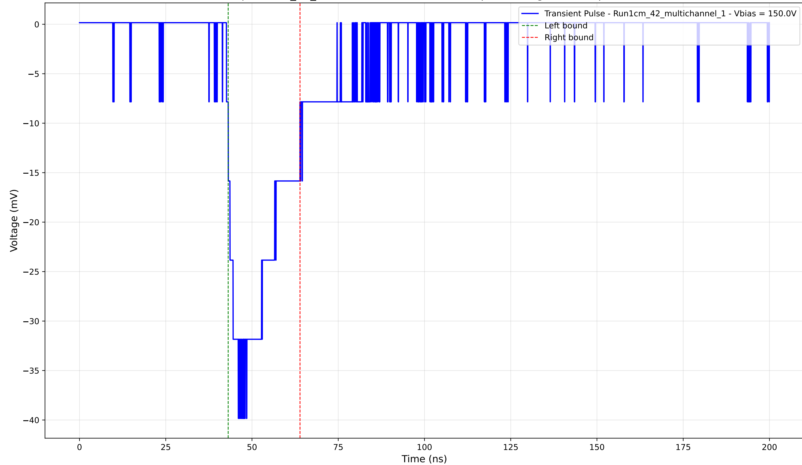
Transient Pulse - Sample: 1cm_42_multichannel - Position: 90.0 \mu\text{m} - Charge: -10.19 pC - Rise Time: 3.43 ns
