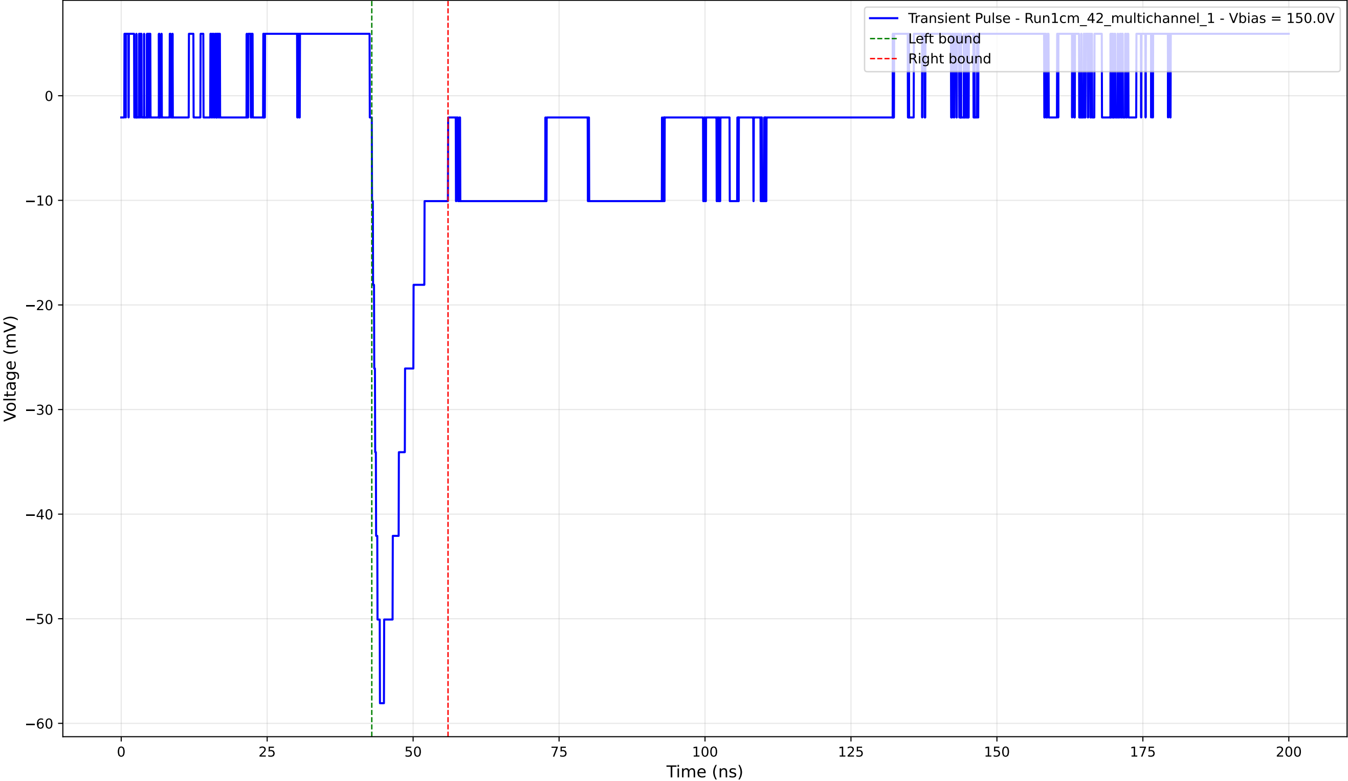
Transient Pulse - Sample: 1cm_42_multichannel - Position: 3785.0 \mu\text{m} - Charge: -7.10 pC - Rise Time: 1.37 ns
