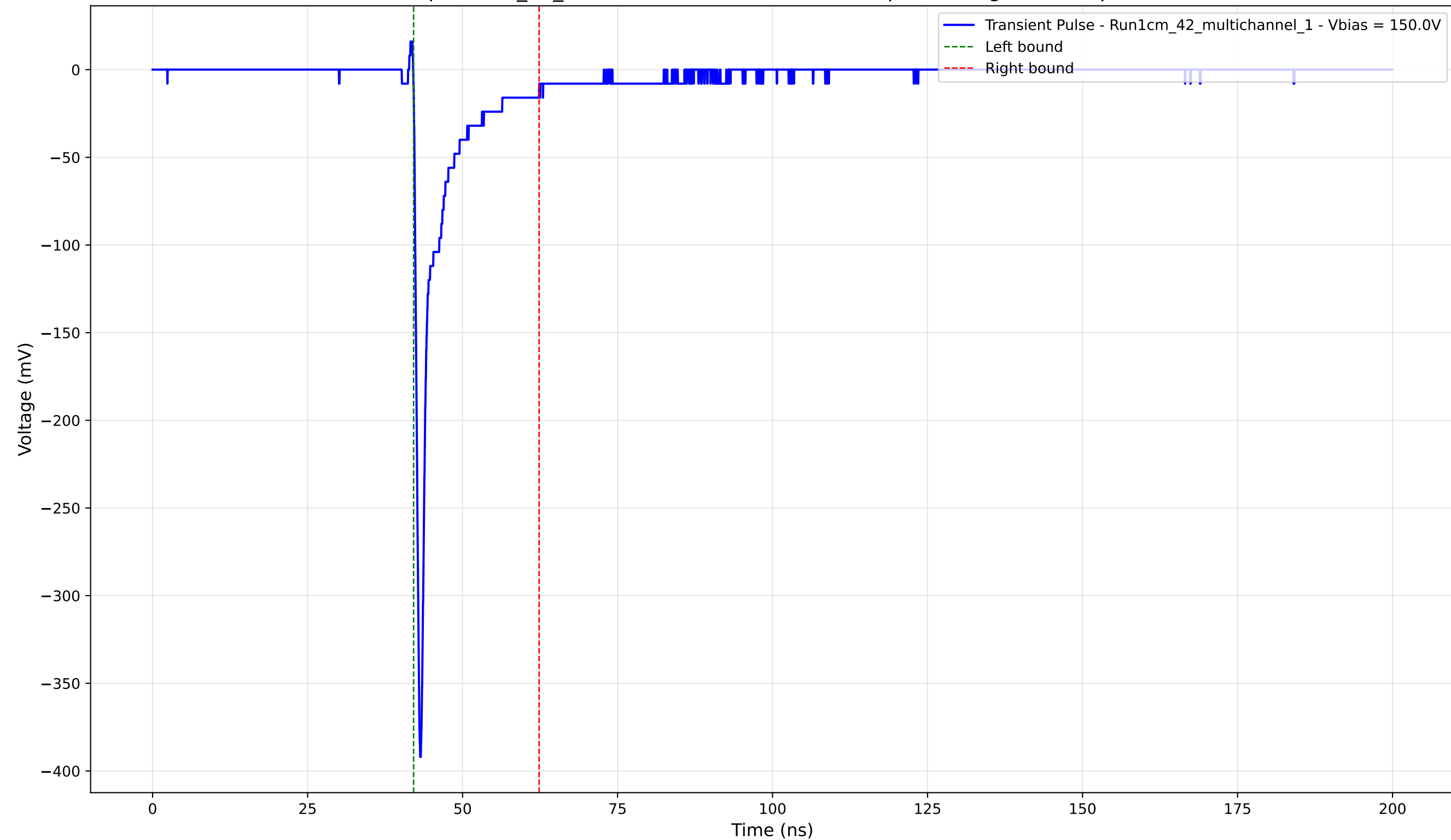
Transient Pulse - Sample: 1cm_42_multichannel - Position: 2245.0 \mu\text{m} - Charge: -25.07 pC - Rise Time: 0.74 ns
