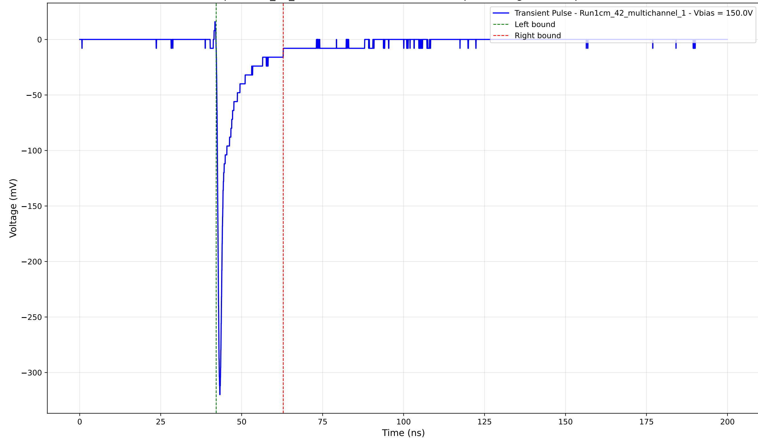
Transient Pulse - Sample: 1cm_42_multichannel - Position: 2630.0 \mu\text{m} - Charge: -23.09 pC - Rise Time: 0.78 ns
