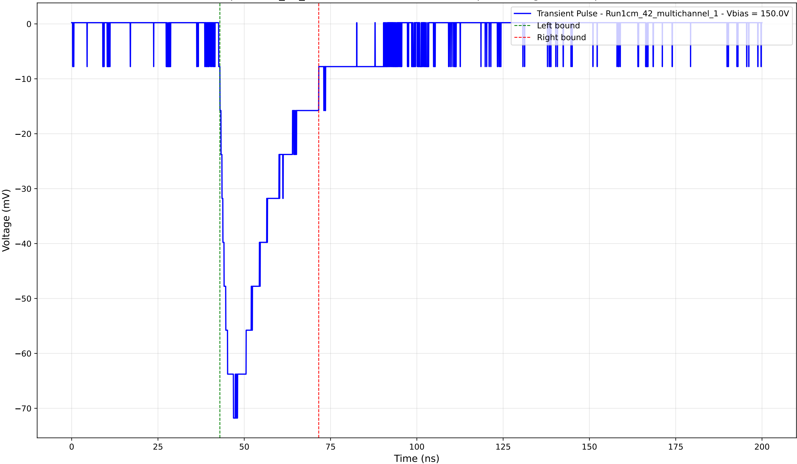
Transient Pulse - Sample: 1cm_42_multichannel - Position: 230.0 \mu\text{m} - Charge: -21.03 pC - Rise Time: 4.28 ns
