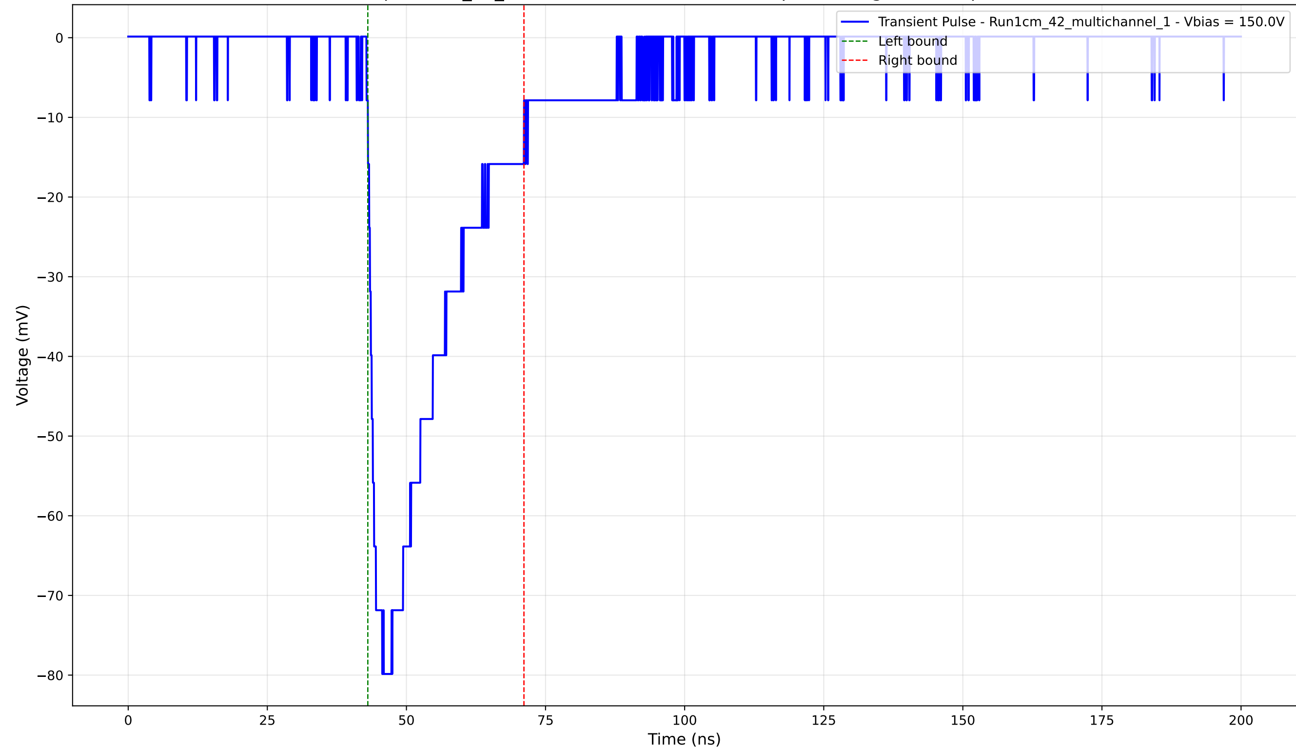
Transient Pulse - Sample: 1cm_42_multichannel - Position: 780.0 \mu\text{m} - Charge: -22.33 pC - Rise Time: 2.58 ns
