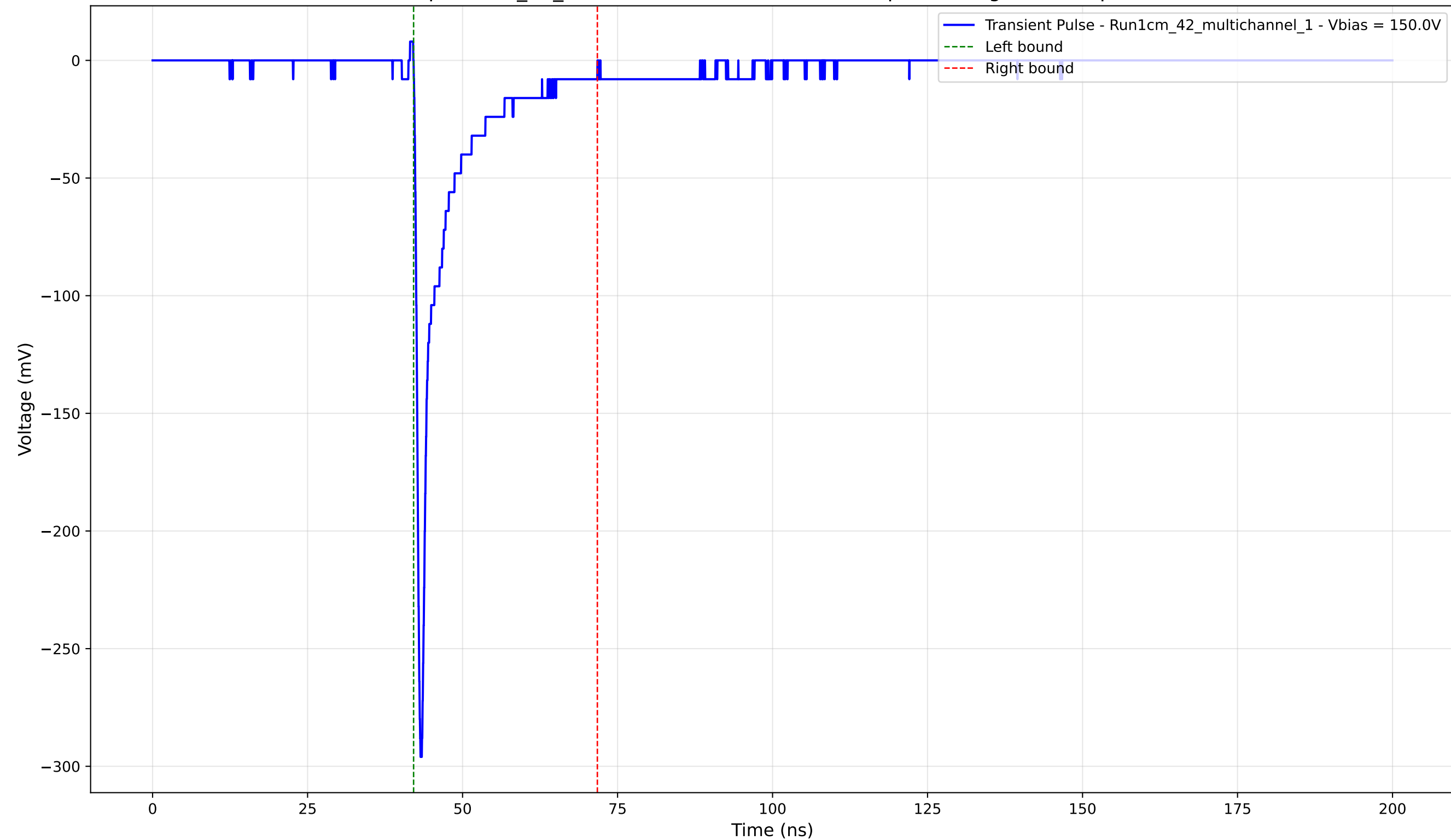
Transient Pulse - Sample: 1cm_42_multichannel - Position: 2665.0 \mu\text{m} - Charge: -24.55 pC - Rise Time: 0.77 ns
