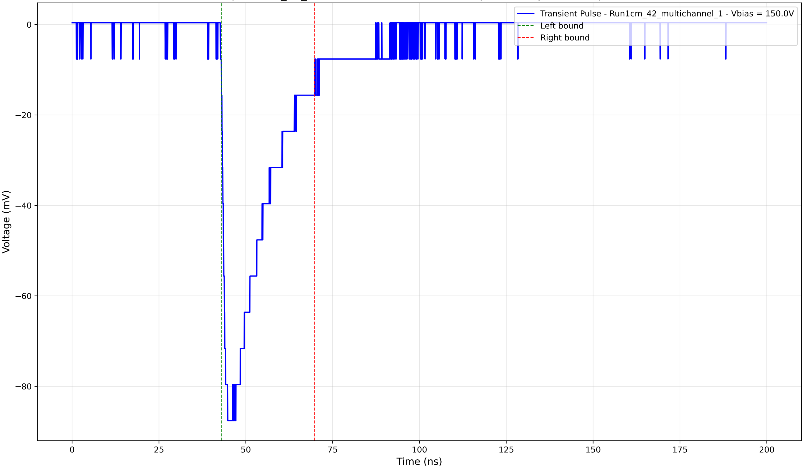
Transient Pulse - Sample: 1cm_42_multichannel - Position: 970.0 \mu\text{m} - Charge: -23.08 pC - Rise Time: 1.26 ns
