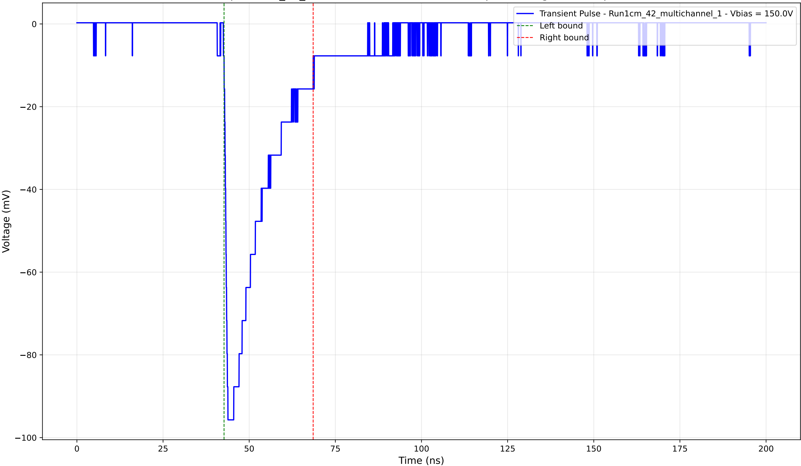
Transient Pulse - Sample: 1cm_42_multichannel - Position: 1275.0 \mu\text{m} - Charge: -22.58 pC - Rise Time: 0.96 ns
