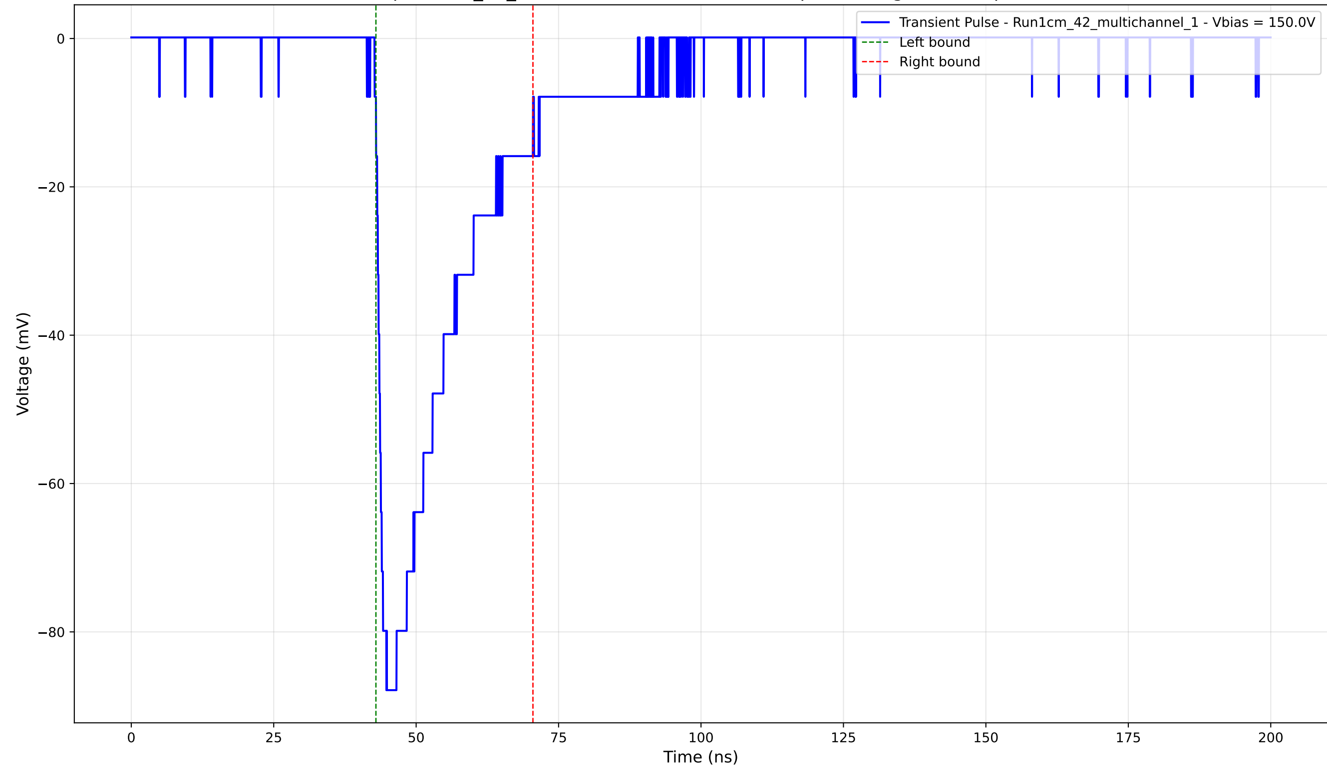
Transient Pulse - Sample: 1cm_42_multichannel - Position: 985.0 \mu\text{m} - Charge: -23.41 pC - Rise Time: 1.24 ns
