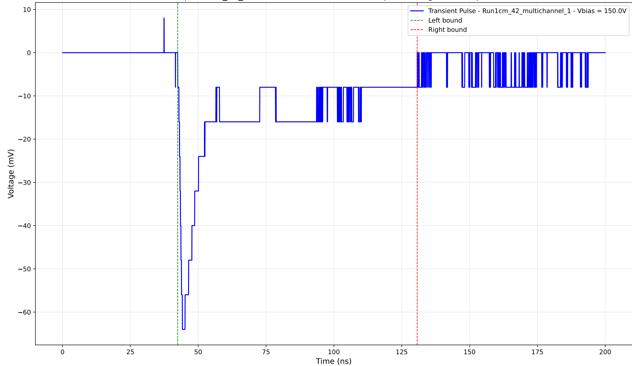
Transient Pulse - Sample: 1cm_42_multichannel - Position: 3770.0 \mu\text{m} - Charge: -26.57 pC - Rise Time: 1.70 ns
