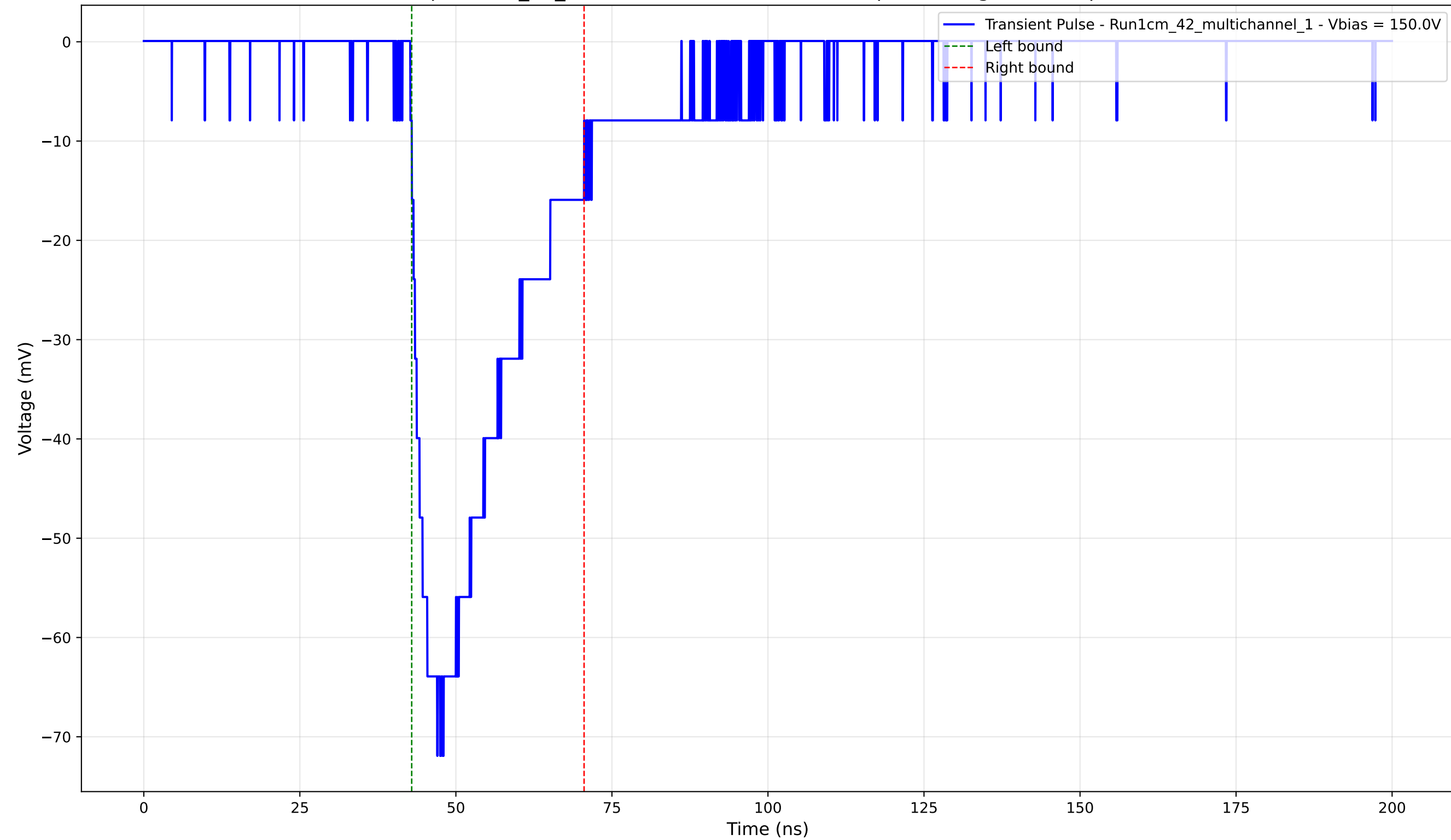
Transient Pulse - Sample: 1cm_42_multichannel - Position: 180.0 \mu\text{m} - Charge: -20.89 pC - Rise Time: 4.30 ns
