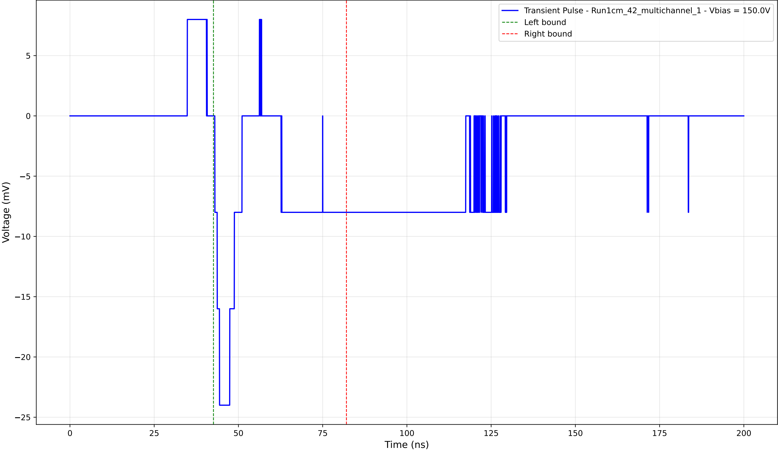
Transient Pulse - Sample: 1cm_42_multichannel - Position: 4355.0 \mu\text{m} - Charge: -5.62 pC - Rise Time: 1.39 ns
