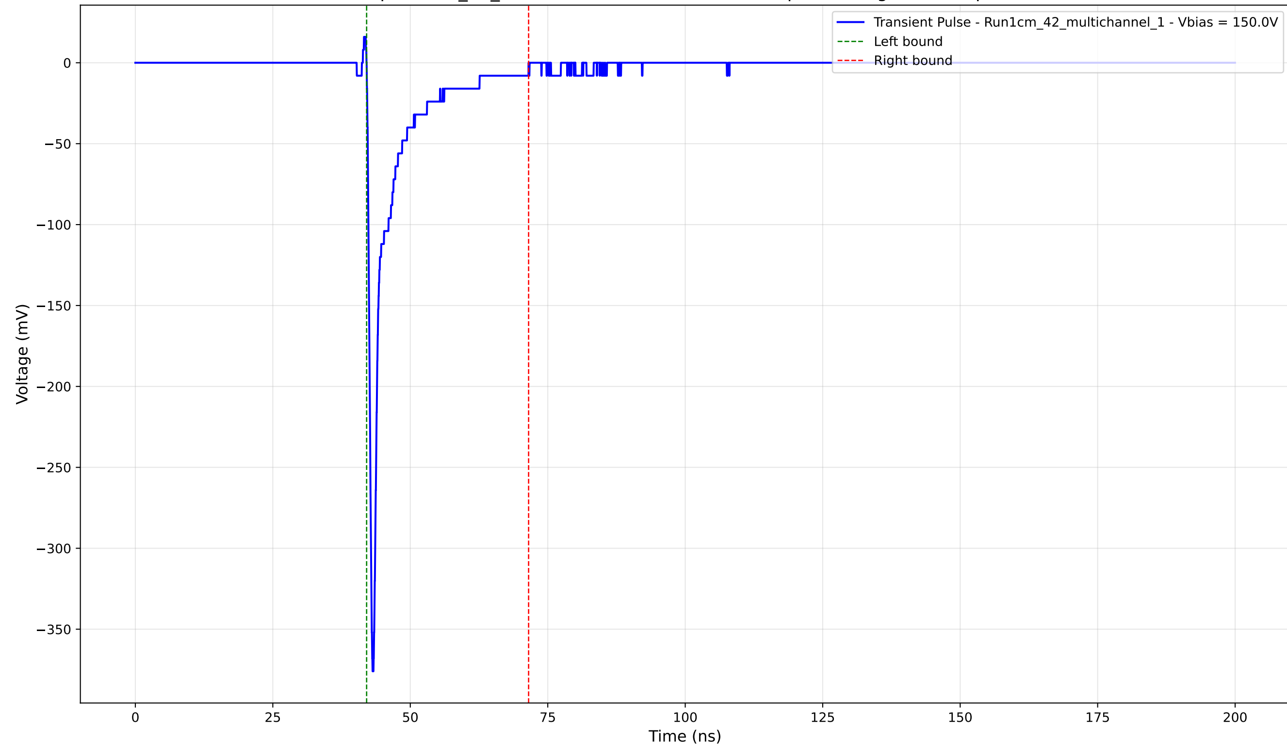
Transient Pulse - Sample: 1cm_42_multichannel - Position: 2230.0 \mu\text{m} - Charge: -26.03 pC - Rise Time: 0.75 ns
