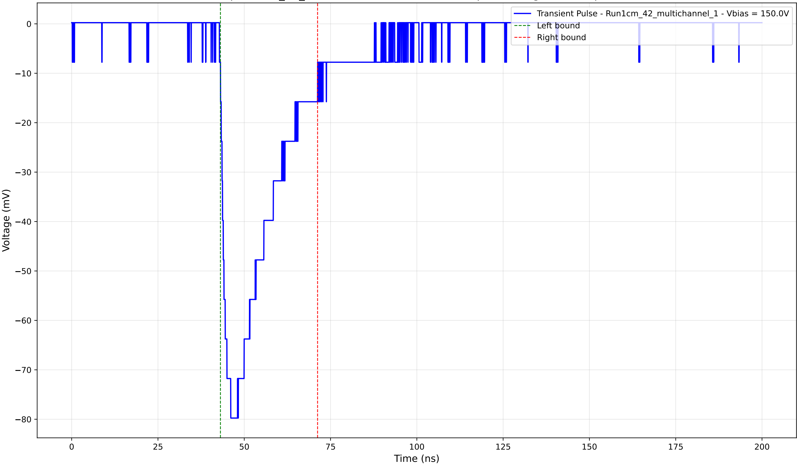
Transient Pulse - Sample: 1cm_42_multichannel - Position: 525.0 \mu\text{m} - Charge: -23.15 pC - Rise Time: 2.98 ns
