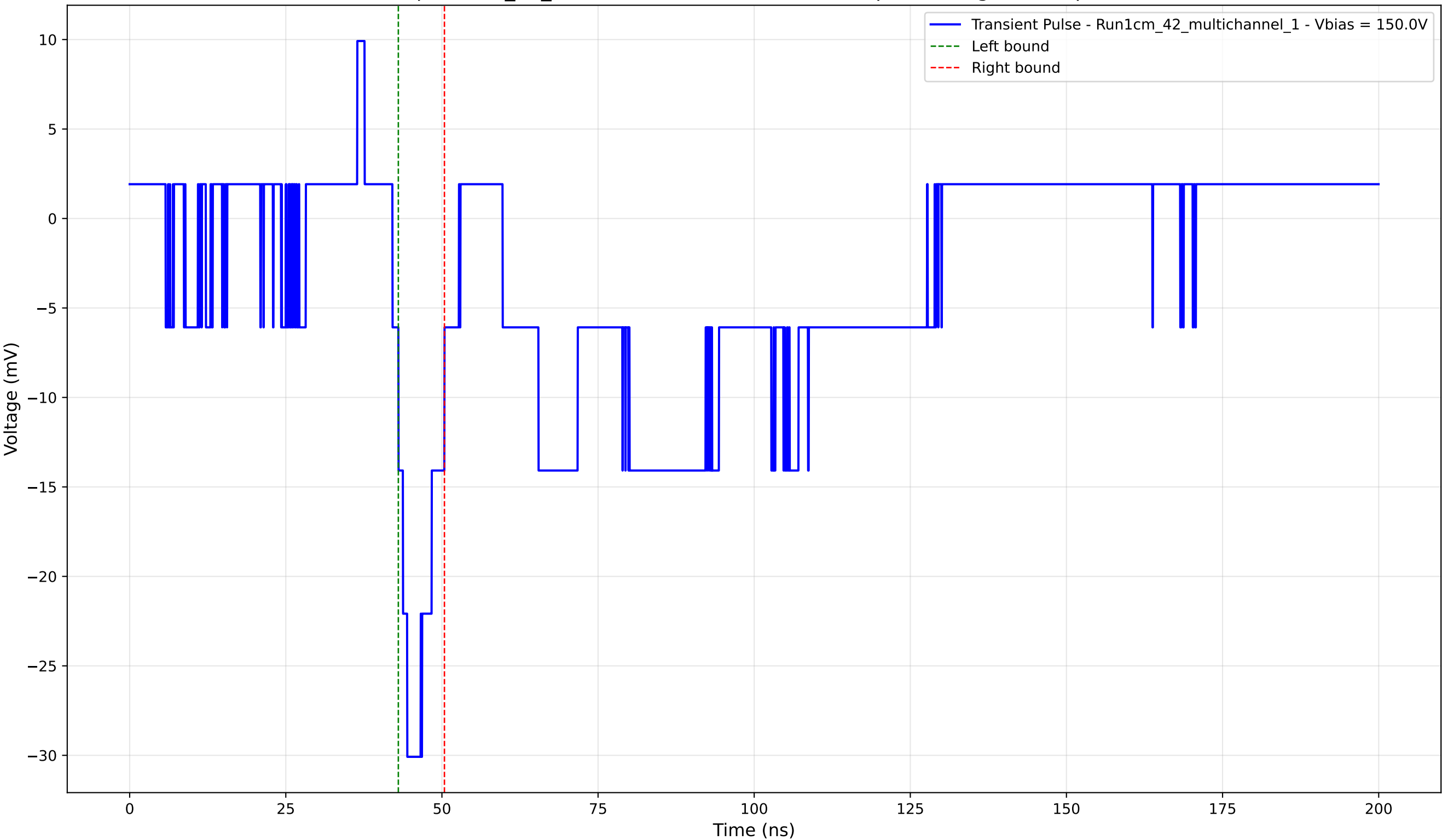
Transient Pulse - Sample: 1cm_42_multichannel - Position: 4845.0 \mu\text{m} - Charge: -3.18 pC - Rise Time: 2.37 ns
