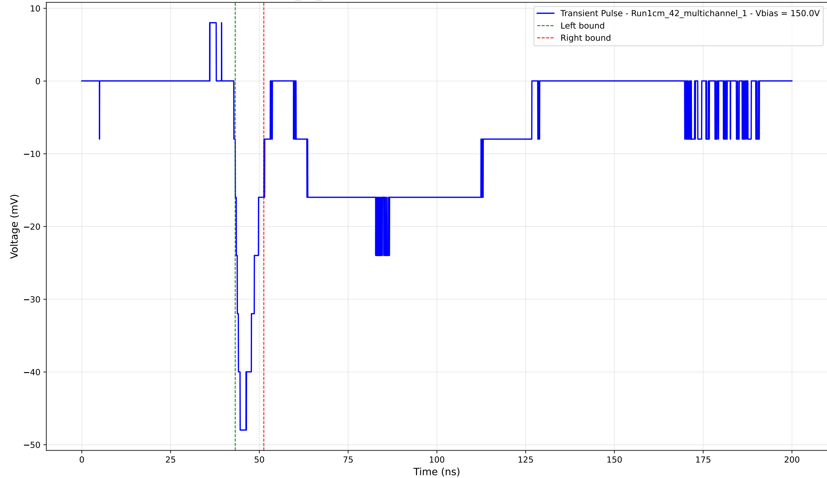
Transient Pulse - Sample: 1cm_42_multichannel - Position: 4145.0 \mu\text{m} - Charge: -5.21 pC - Rise Time: 1.77 ns
