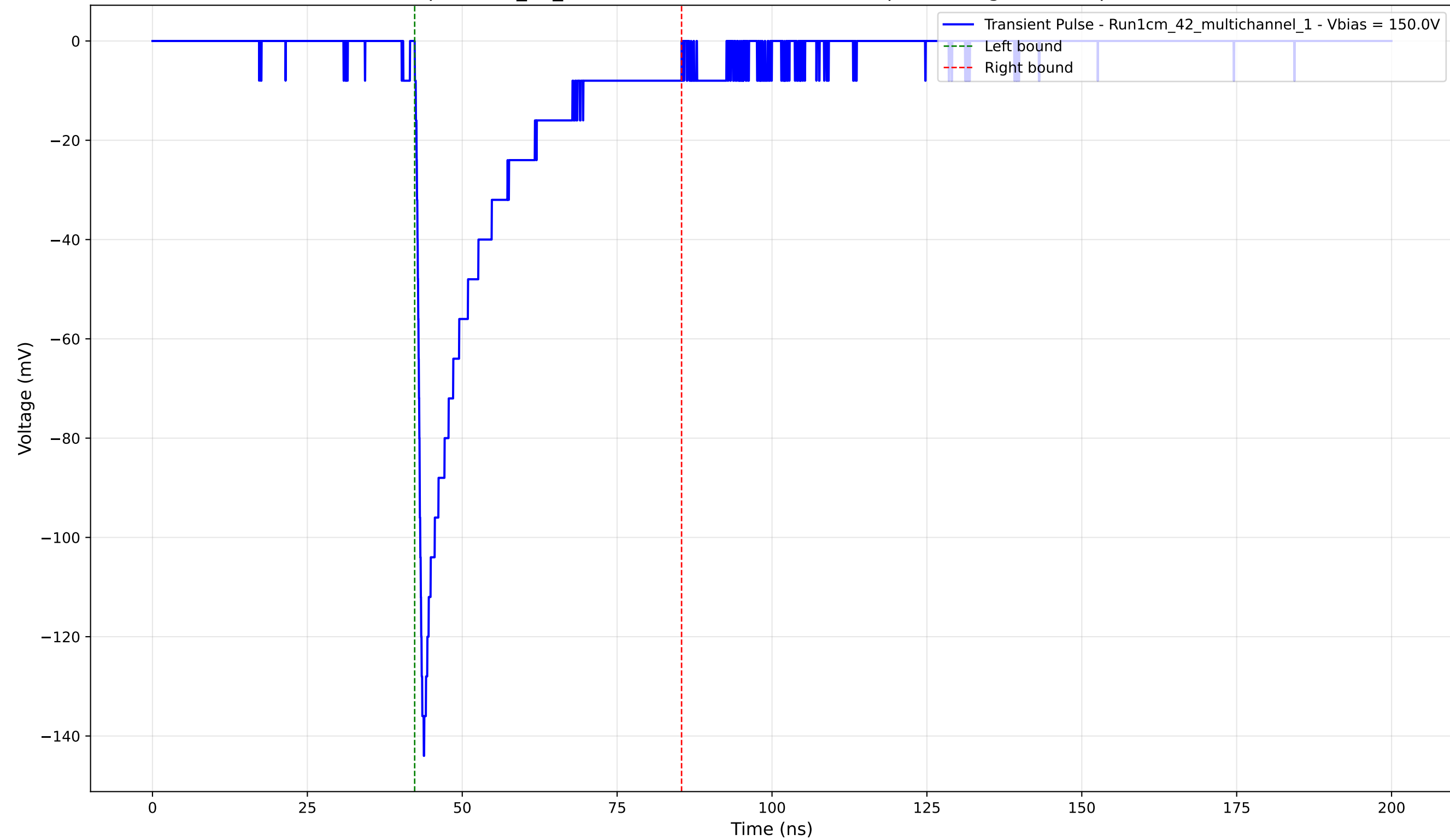
Transient Pulse - Sample: 1cm_42_multichannel - Position: 1575.0 \mu\text{m} - Charge: -26.14 pC - Rise Time: 1.04 ns
