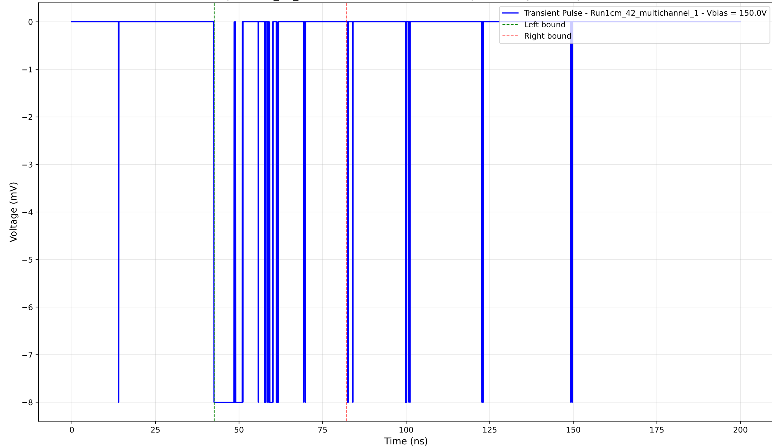
Transient Pulse - Sample: 1cm_42_multichannel - Position: 2885.0 \mu\text{m} - Charge: -1.65 pC - Rise Time: 0.02 ns
