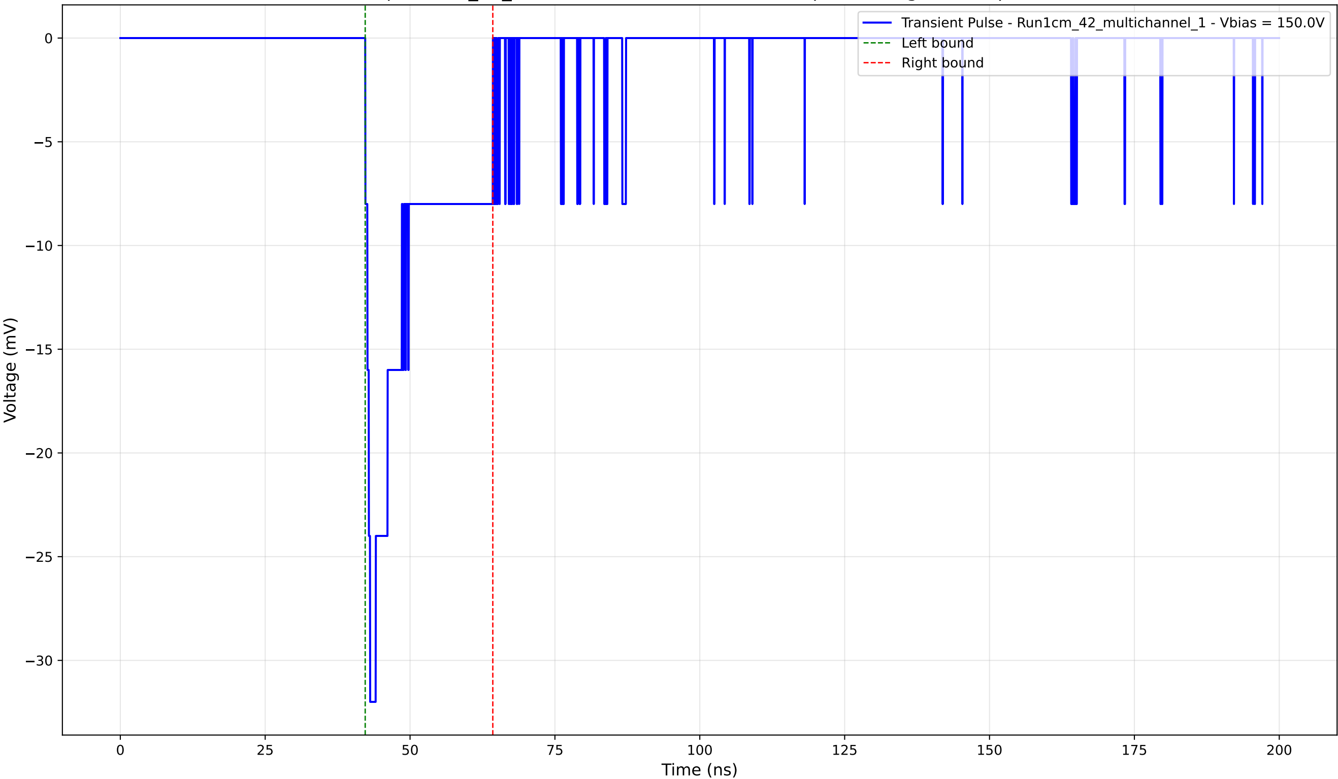
Transient Pulse - Sample: 1cm_42_multichannel - Position: 2930.0 \mu\text{m} - Charge: -5.21 pC - Rise Time: 0.83 ns
