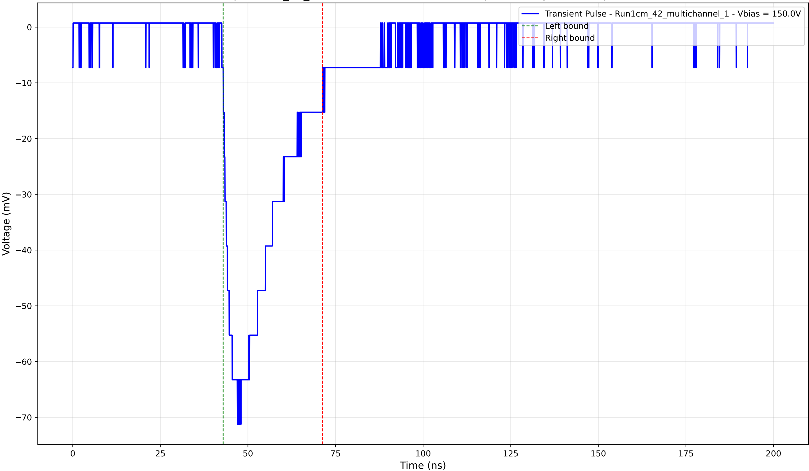
Transient Pulse - Sample: 1cm_42_multichannel - Position: 160.0 \mu\text{m} - Charge: -20.77 pC - Rise Time: 4.40 ns
