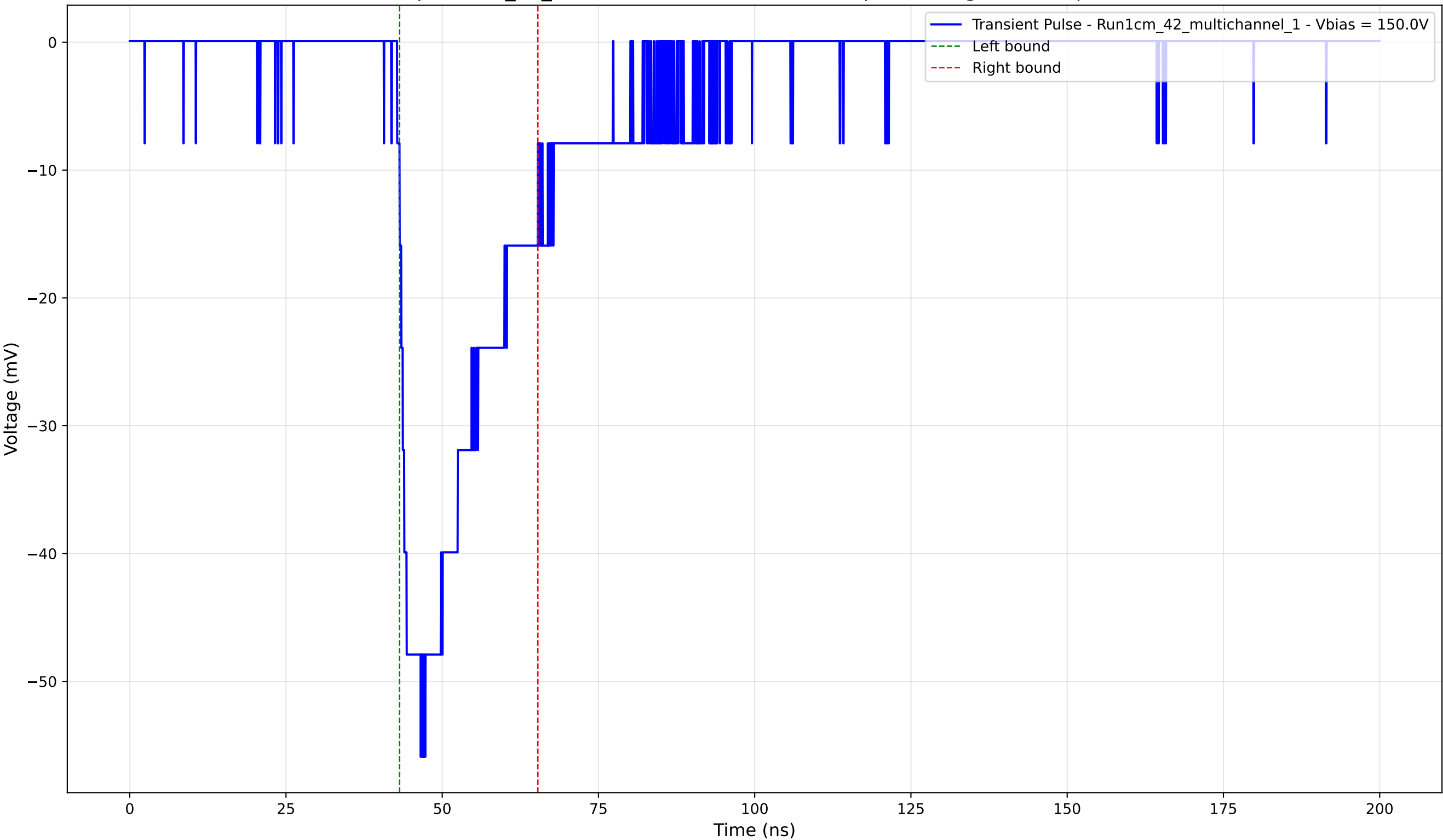
Transient Pulse - Sample: 1cm_42_multichannel - Position: 810.0 \mu\text{m} - Charge: -13.91 pC - Rise Time: 3.79 ns
