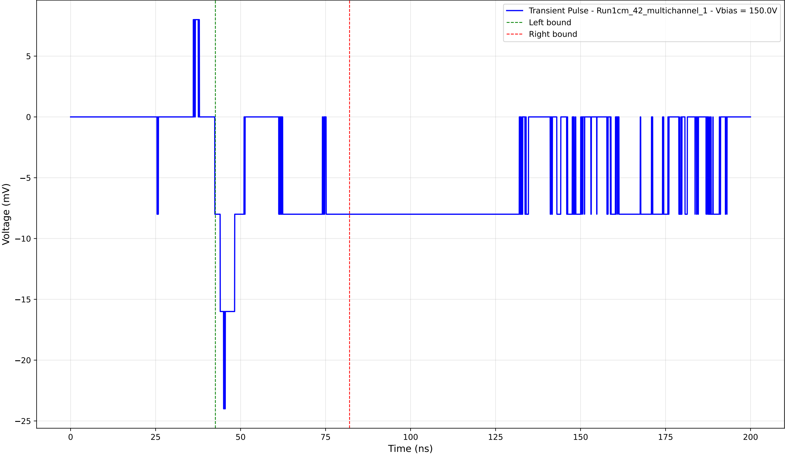
Transient Pulse - Sample: 1cm_42_multichannel - Position: 4450.0 \mu\text{m} - Charge: -5.18 pC - Rise Time: 2.59 ns
