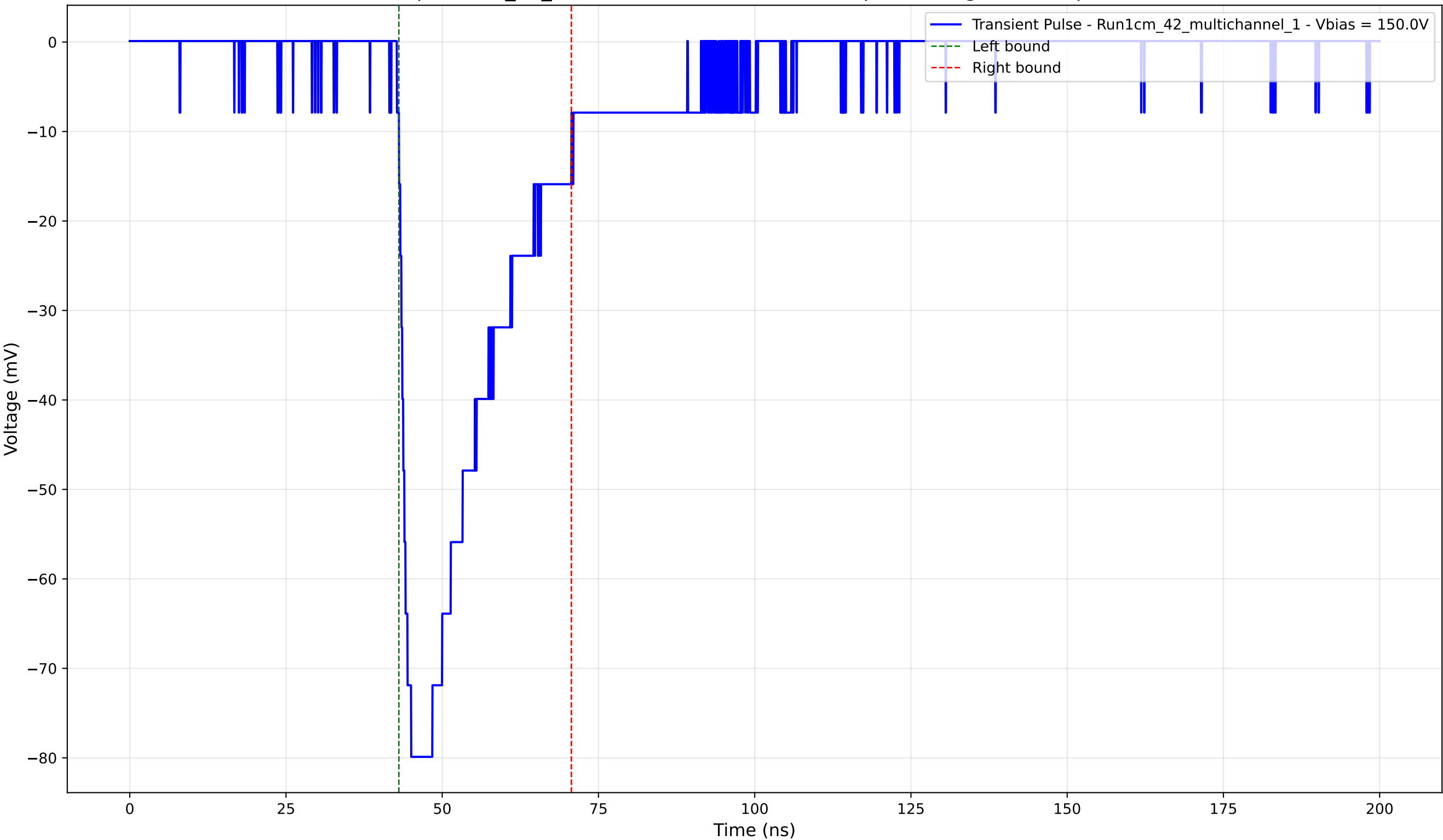
Transient Pulse - Sample: 1cm_42_multichannel - Position: 745.0 \mu\text{m} - Charge: -23.30 pC - Rise Time: 1.96 ns
