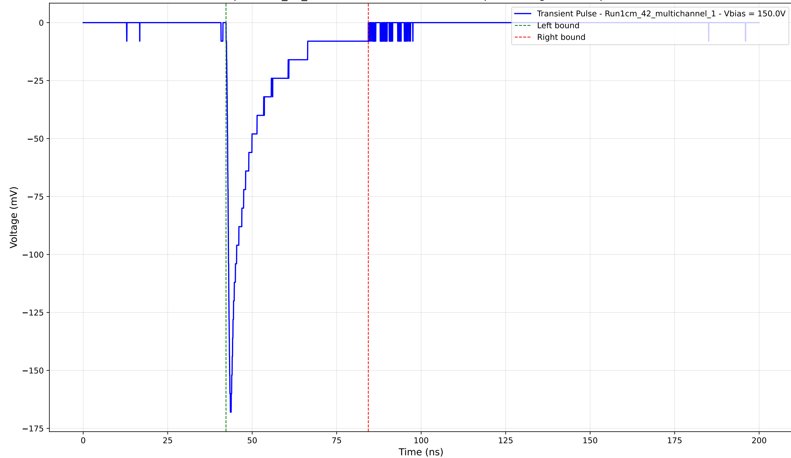
Transient Pulse - Sample: 1cm_42_multichannel - Position: 1725.0 \mu\text{m} - Charge: -25.34 pC - Rise Time: 0.84 ns
