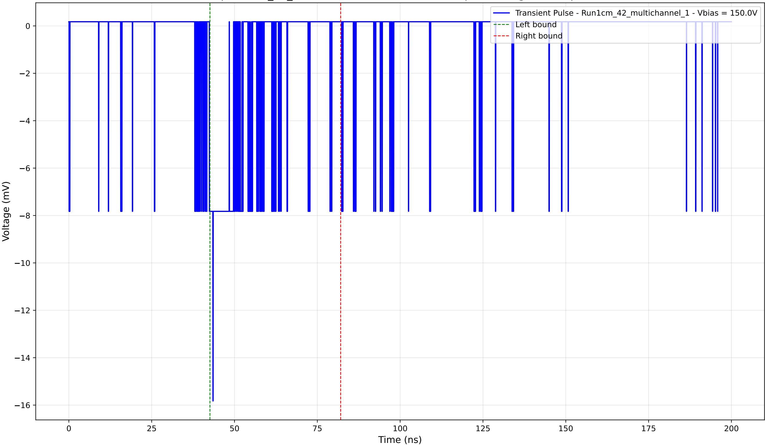
Transient Pulse - Sample: 1cm_42_multichannel - Position: 1875.0 \mu\text{m} - Charge: -1.71 pC - Rise Time: 1.10 ns
