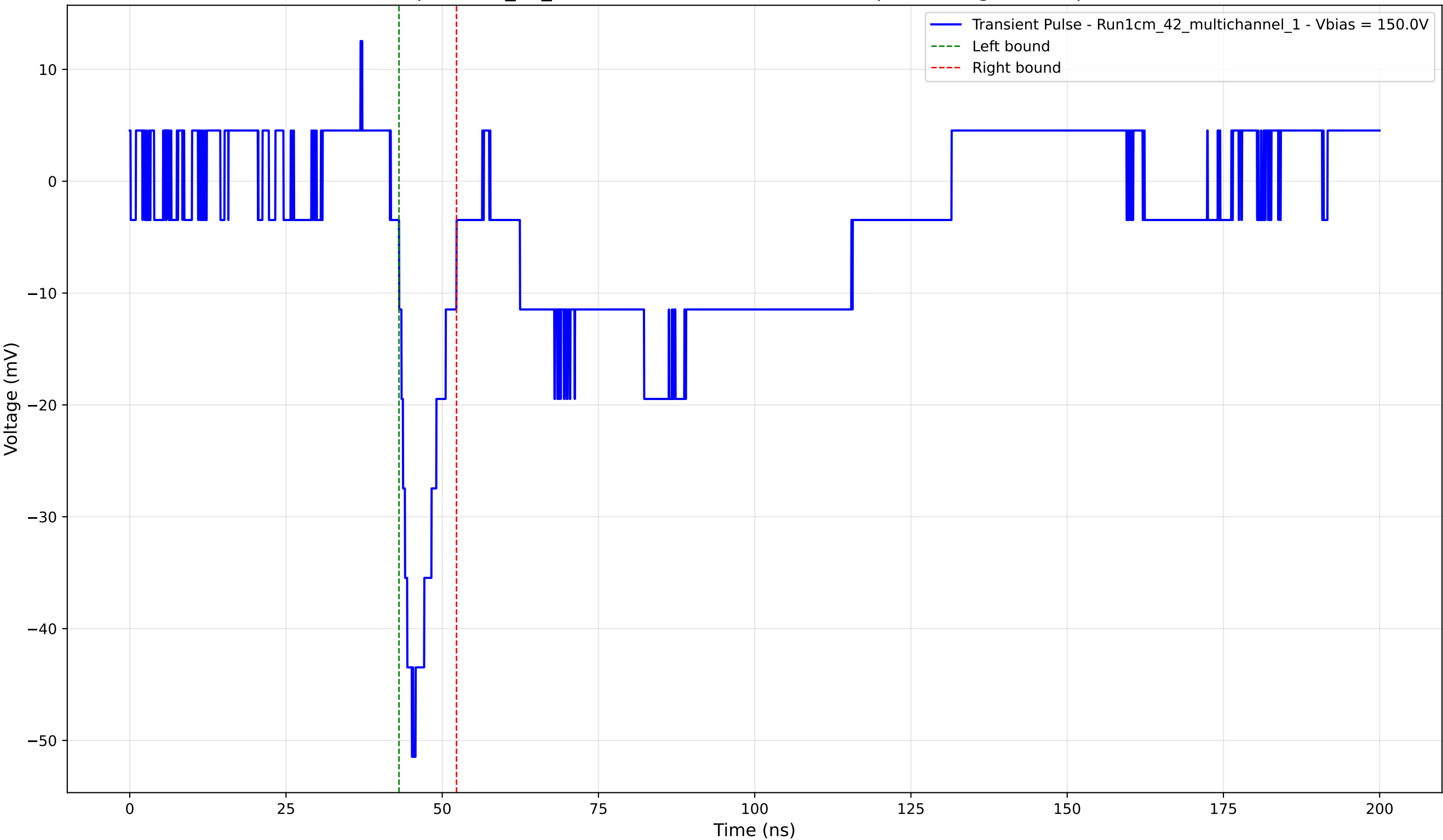
Transient Pulse - Sample: 1cm_42_multichannel - Position: 4280.0 \mu\text{m} - Charge: -5.28 pC - Rise Time: 2.06 ns
