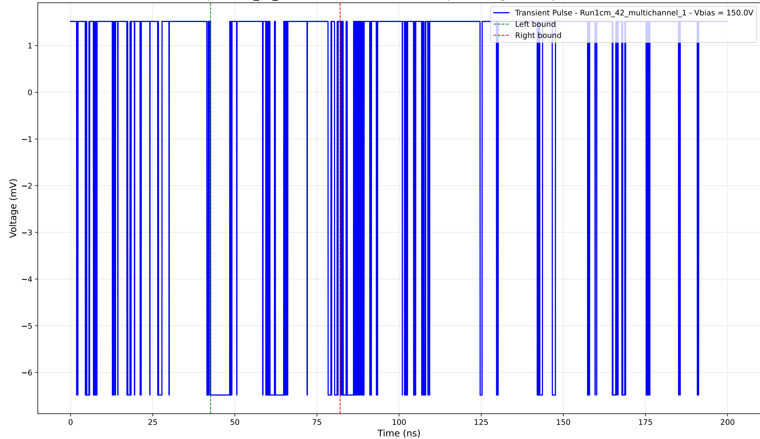
Transient Pulse - Sample: 1cm_42_multichannel - Position: 3405.0 \mu\text{m} - Charge: -0.96 pC - Rise Time: 0.00 ns (N/A)
