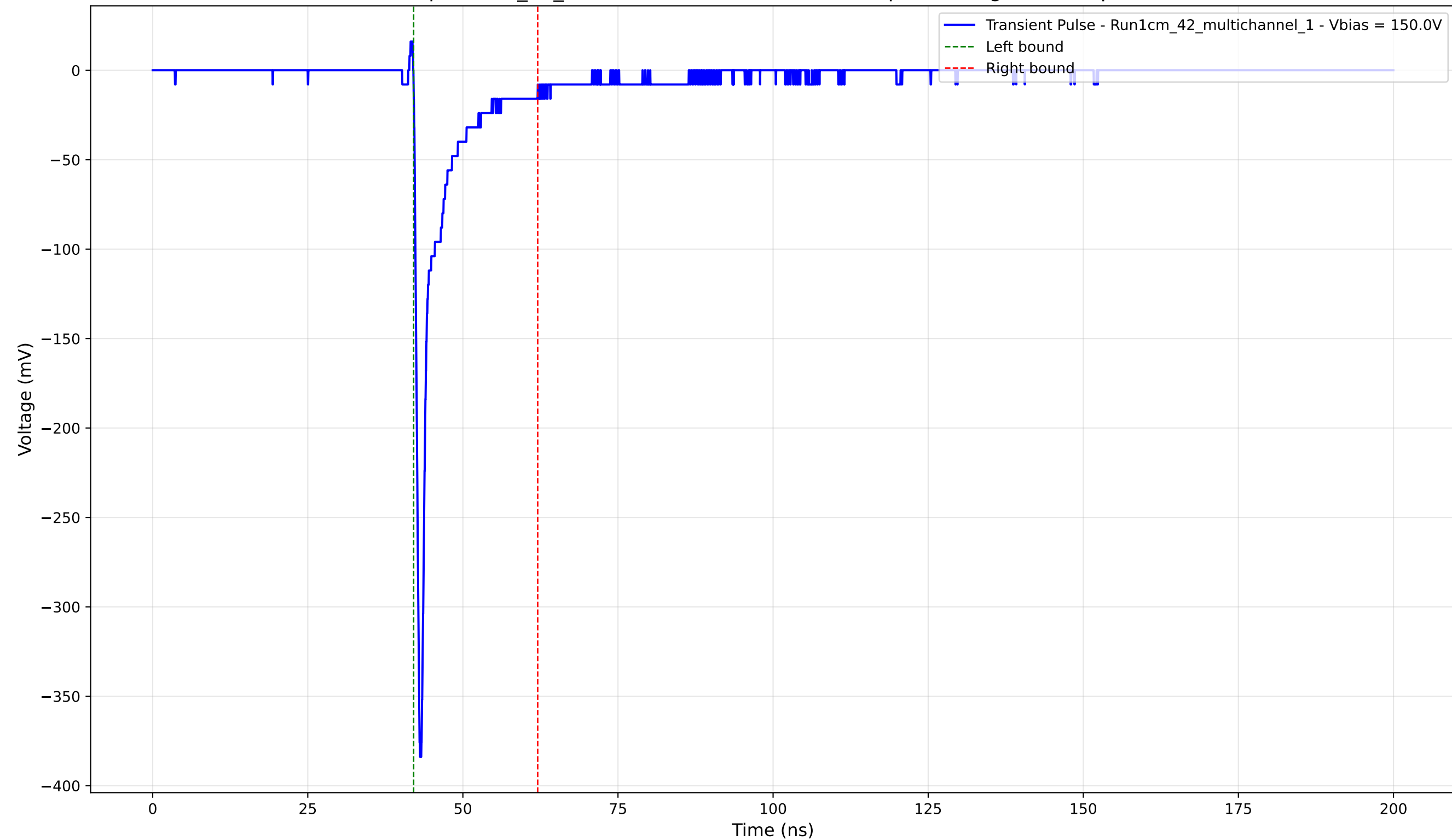
Transient Pulse - Sample: 1cm_42_multichannel - Position: 2510.0 \mu\text{m} - Charge: -24.09 pC - Rise Time: 0.73 ns
