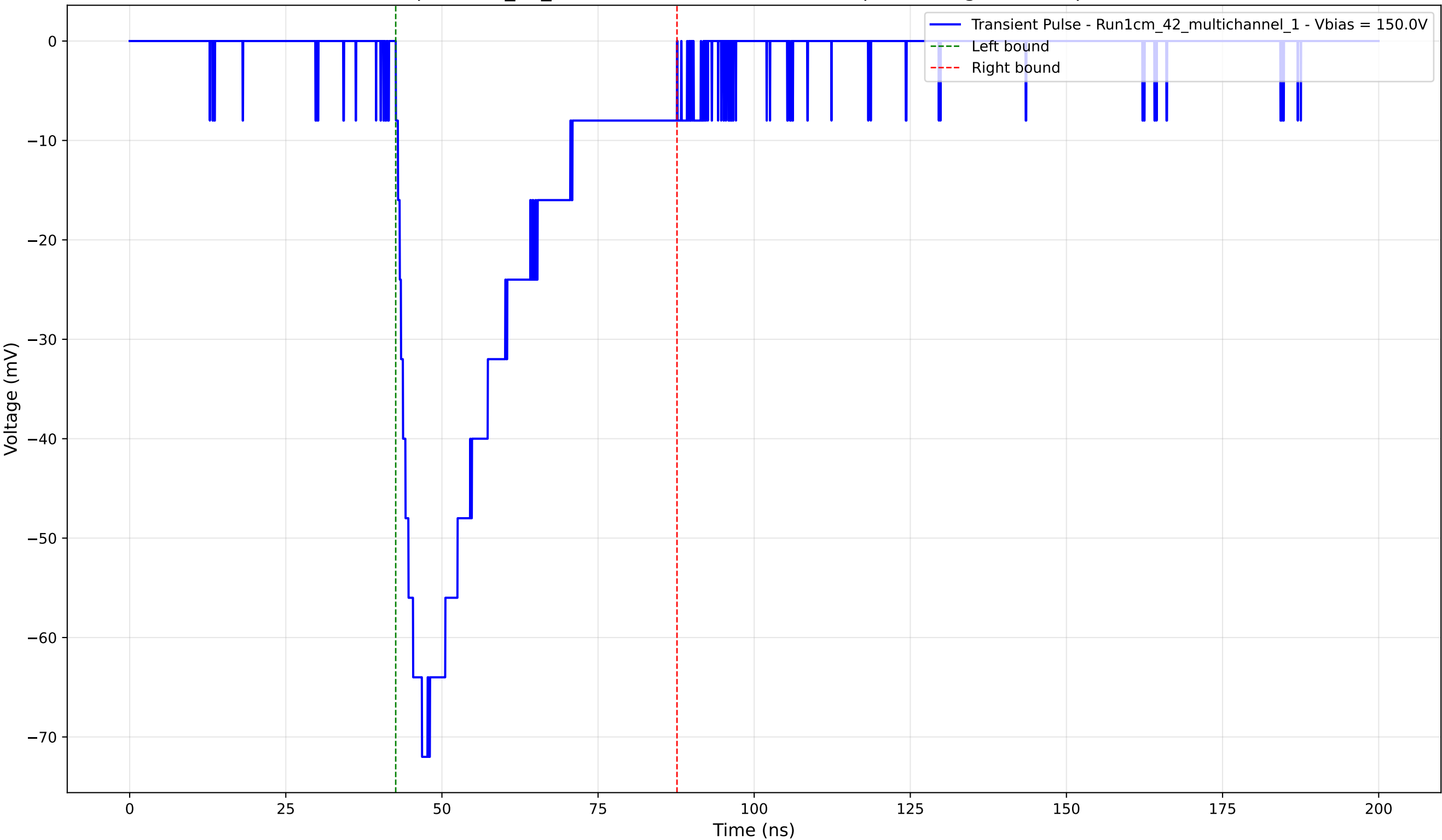
Transient Pulse - Sample: 1cm_42_multichannel - Position: 185.0 \mu\text{m} - Charge: -23.96 pC - Rise Time: 4.18 ns
