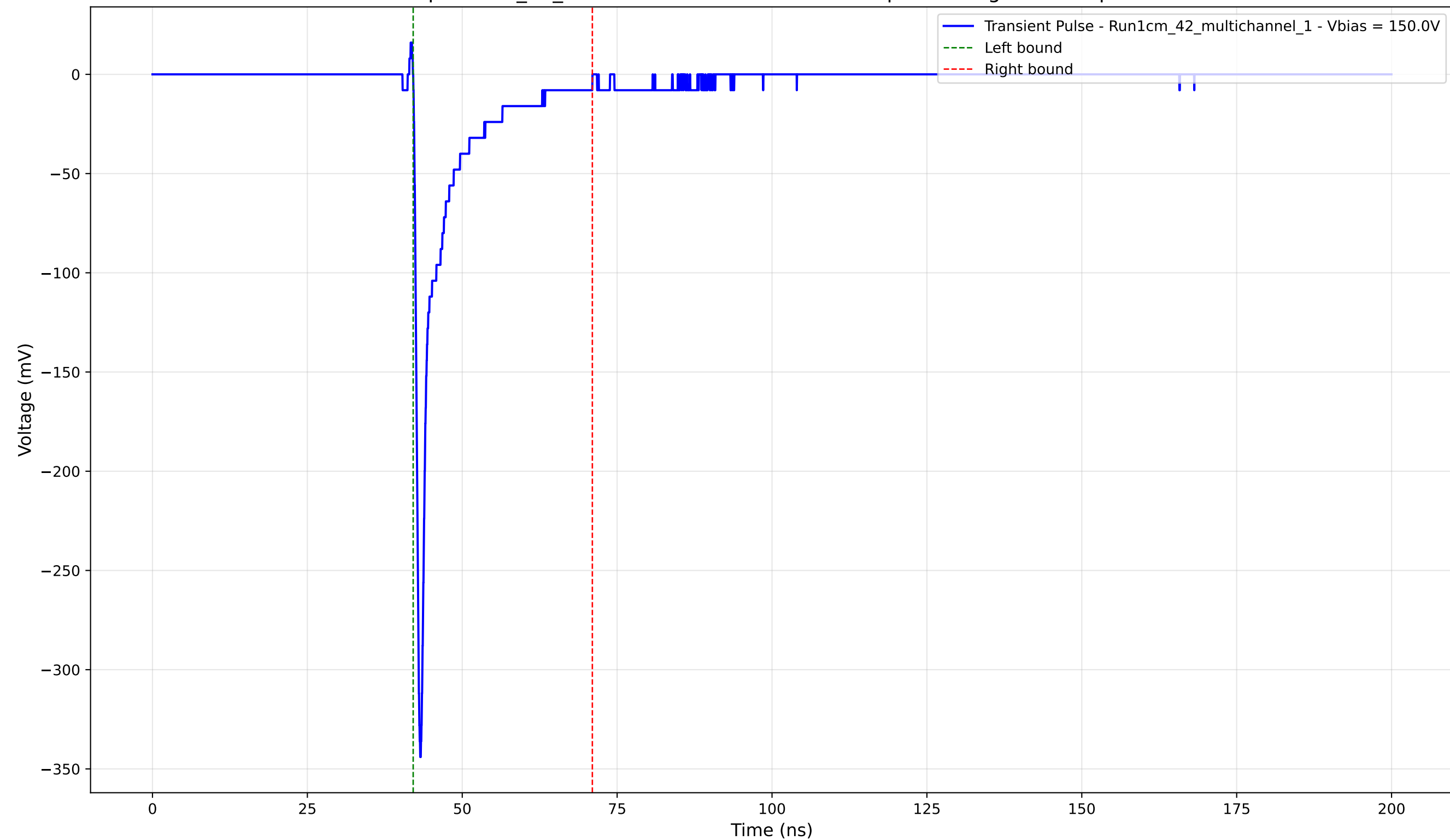
Transient Pulse - Sample: 1cm_42_multichannel - Position: 2175.0 \mu\text{m} - Charge: -25.45 pC - Rise Time: 0.75 ns
