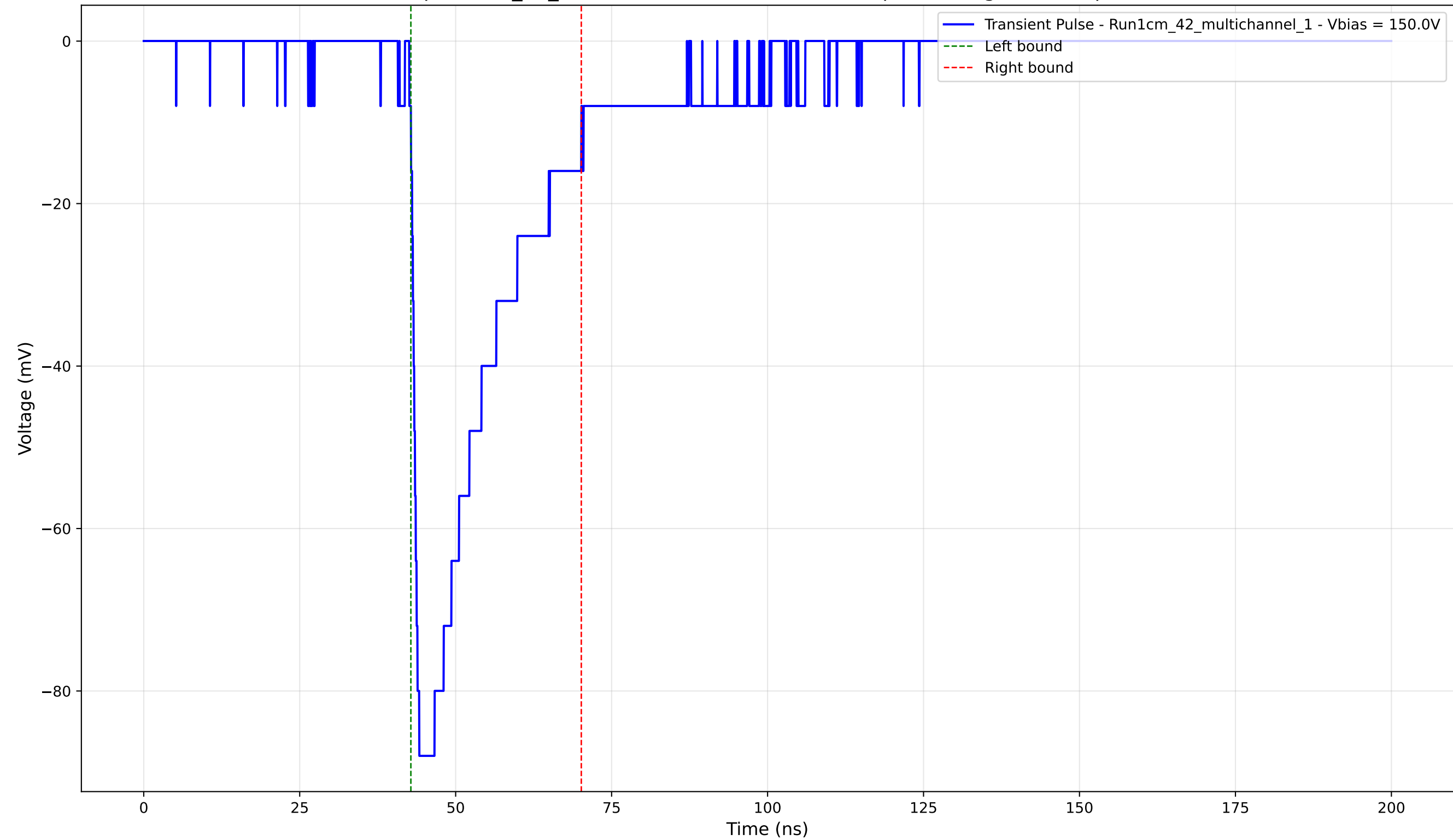
Transient Pulse - Sample: 1cm_42_multichannel - Position: 1105.0 \mu\text{m} - Charge: -23.25 pC - Rise Time: 1.06 ns
