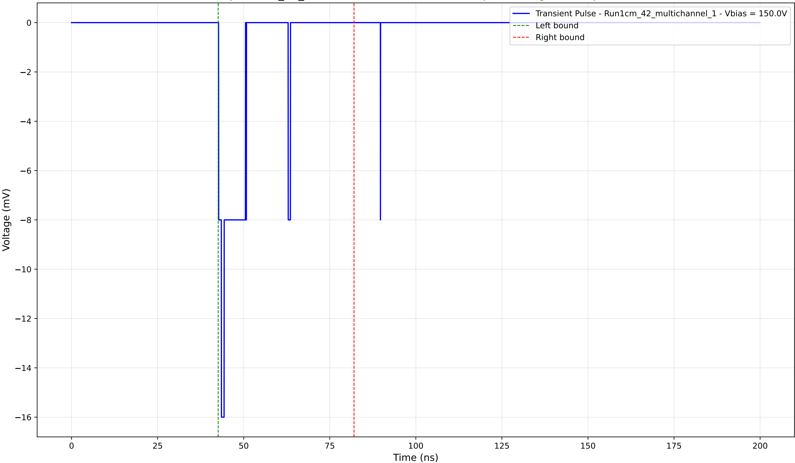
Transient Pulse - Sample: 1cm_42_multichannel - Position: 3430.0 \mu\text{m} - Charge: -1.50 pC - Rise Time: 0.82 ns
