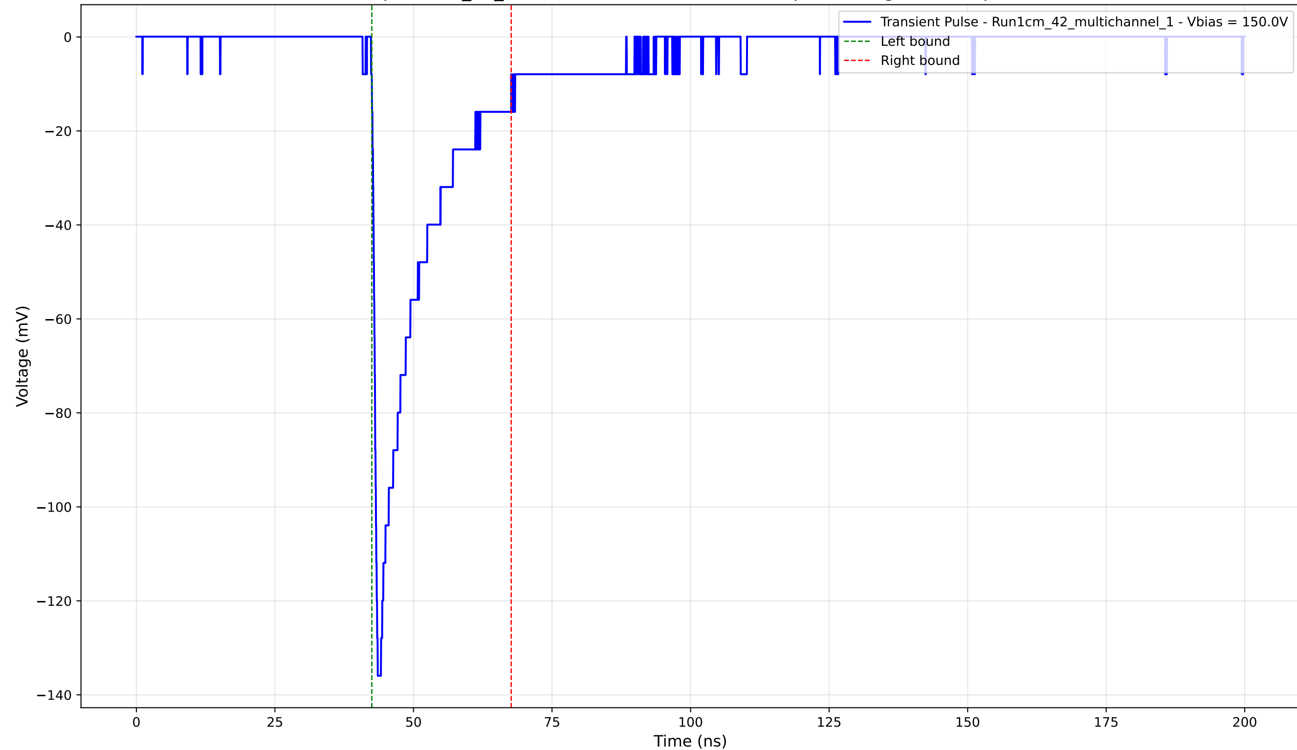
Transient Pulse - Sample: 1cm_42_multichannel - Position: 1580.0 \mu\text{m} - Charge: -23.04 pC - Rise Time: 0.95 ns
