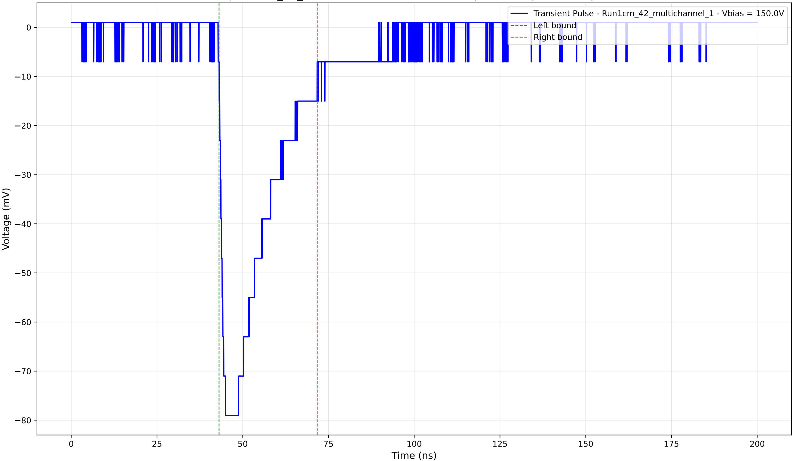
Transient Pulse - Sample: 1cm_42_multichannel - Position: 695.0 \mu\text{m} - Charge: -23.50 pC - Rise Time: 1.90 ns
