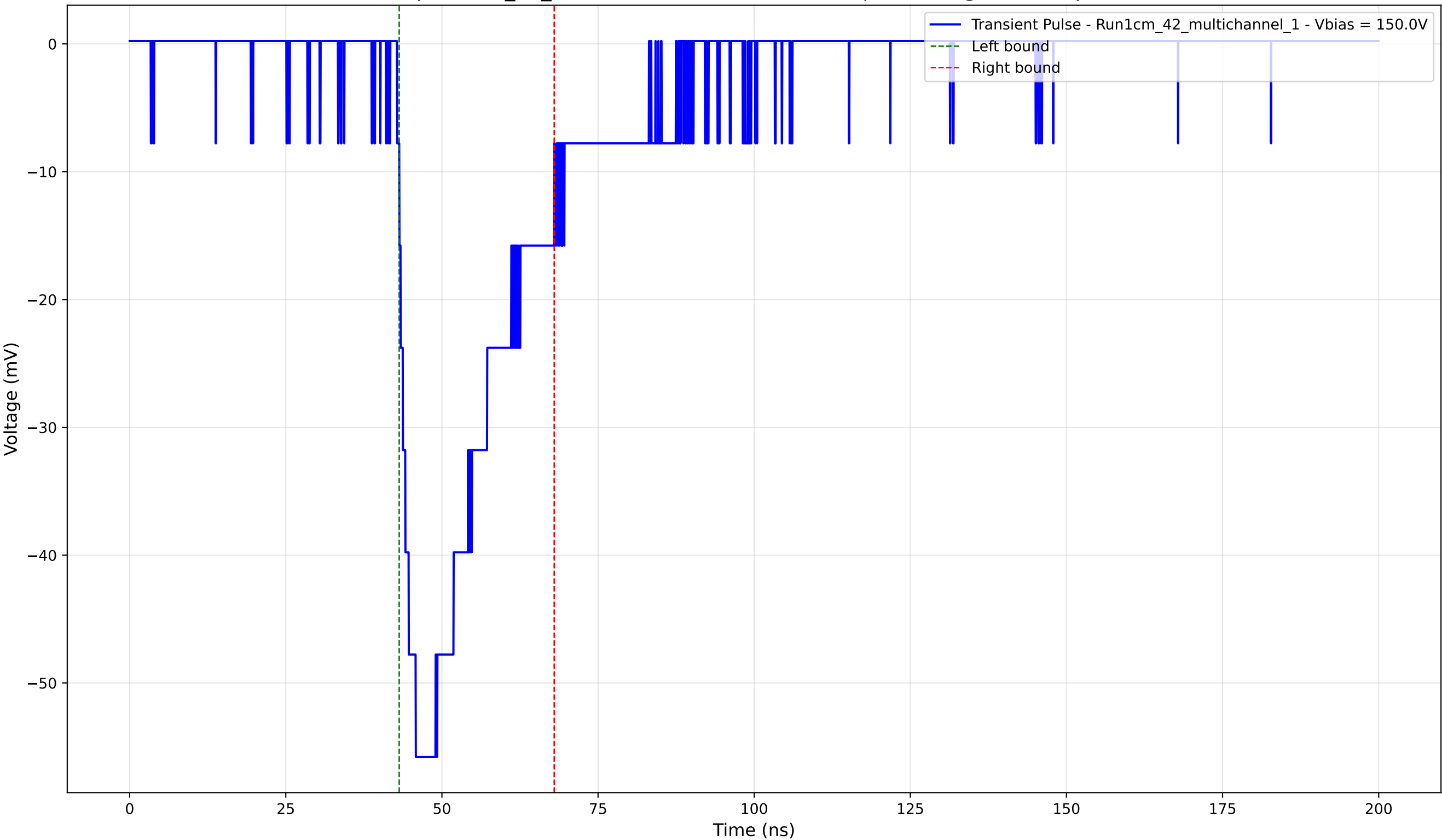
Transient Pulse - Sample: 1cm_42_multichannel - Position: 295.0 \mu\text{m} - Charge: -16.28 pC - Rise Time: 2.99 ns
