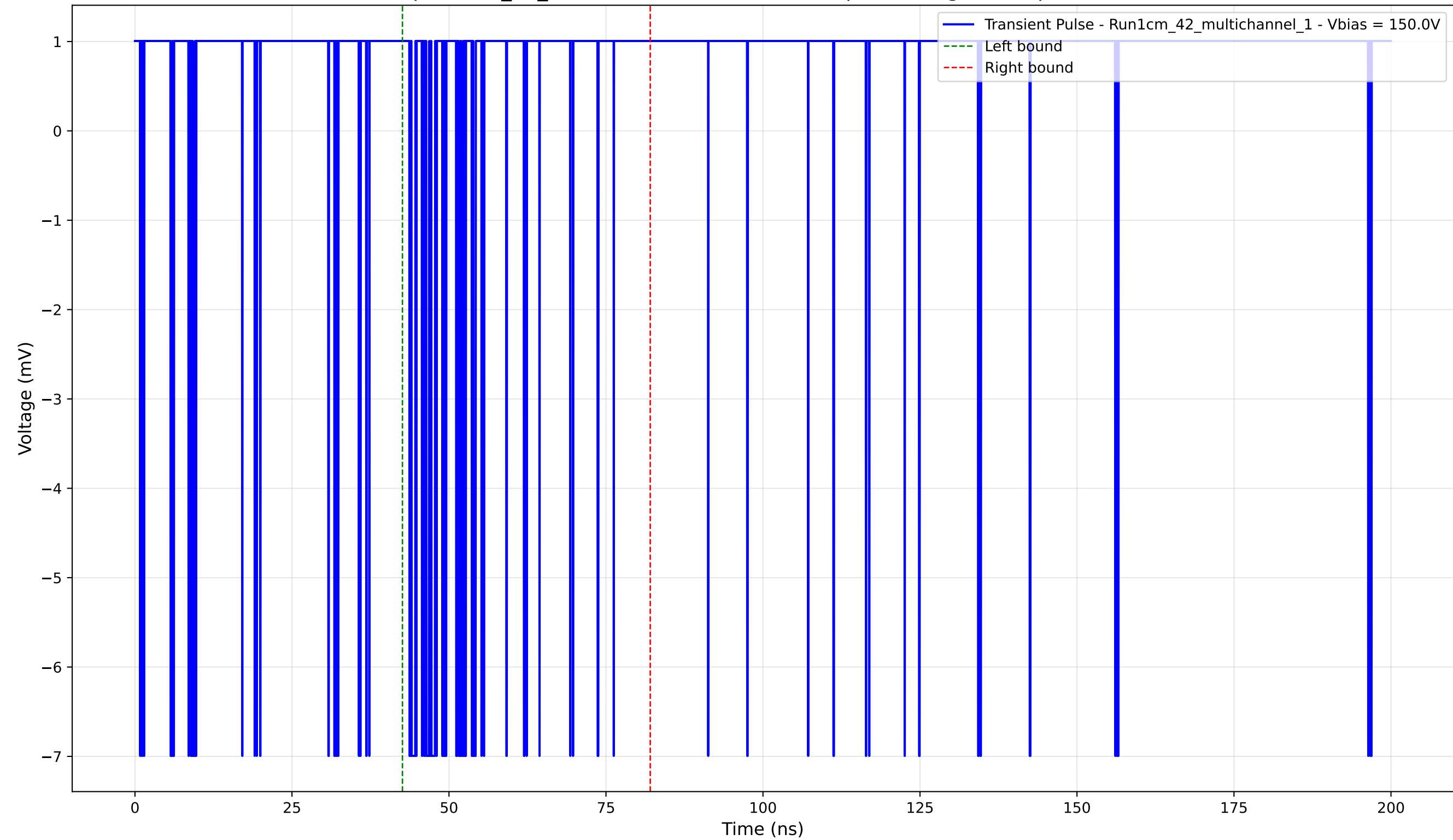
Transient Pulse - Sample: 1cm_42_multichannel - Position: 25.0 \mu\text{m} - Charge: 0.05 pC - Rise Time: 0.00 ns (N/A)
