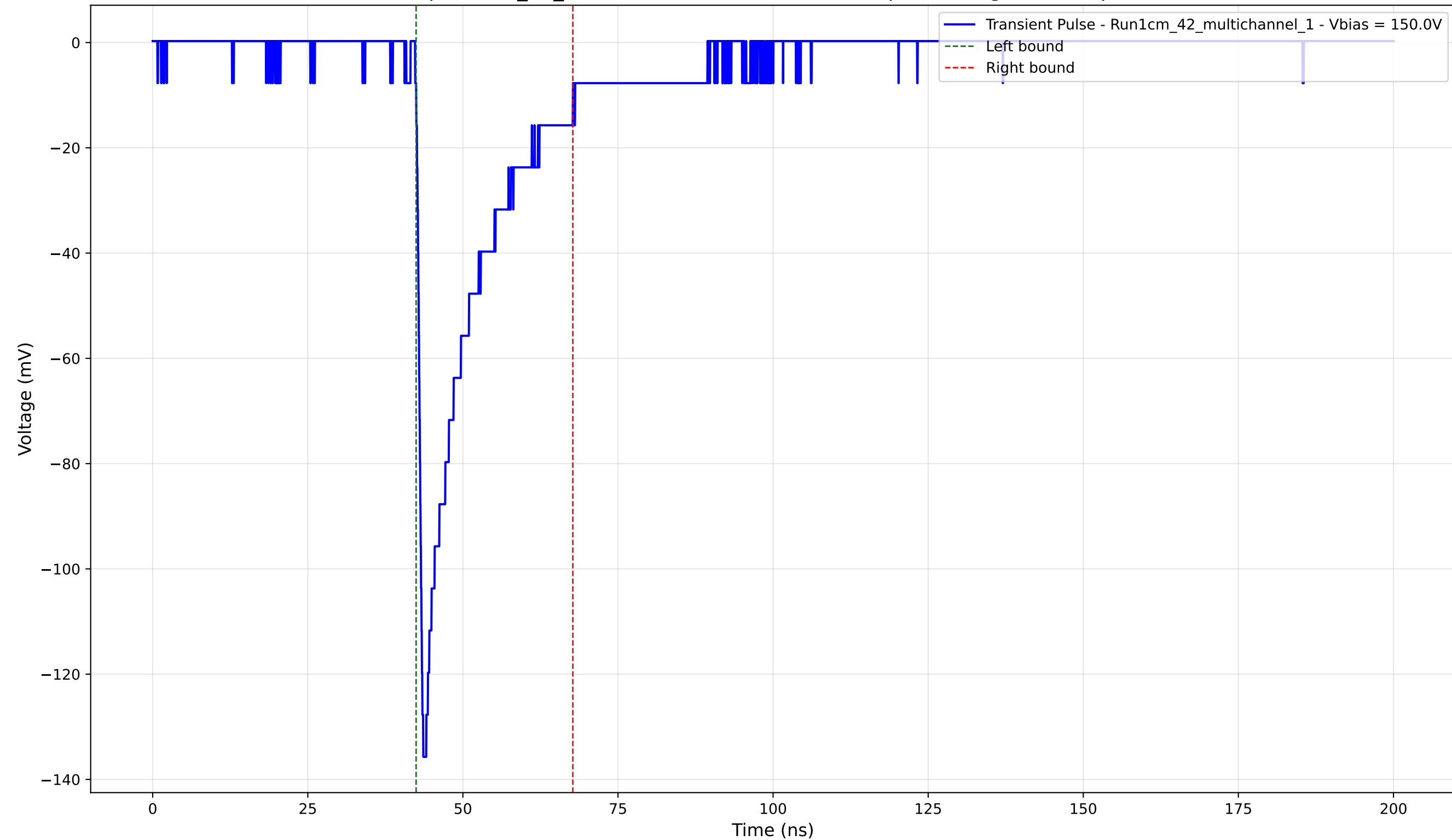
Transient Pulse - Sample: 1cm_42_multichannel - Position: 1565.0 \mu\text{m} - Charge: -23.18 pC - Rise Time: 0.99 ns
