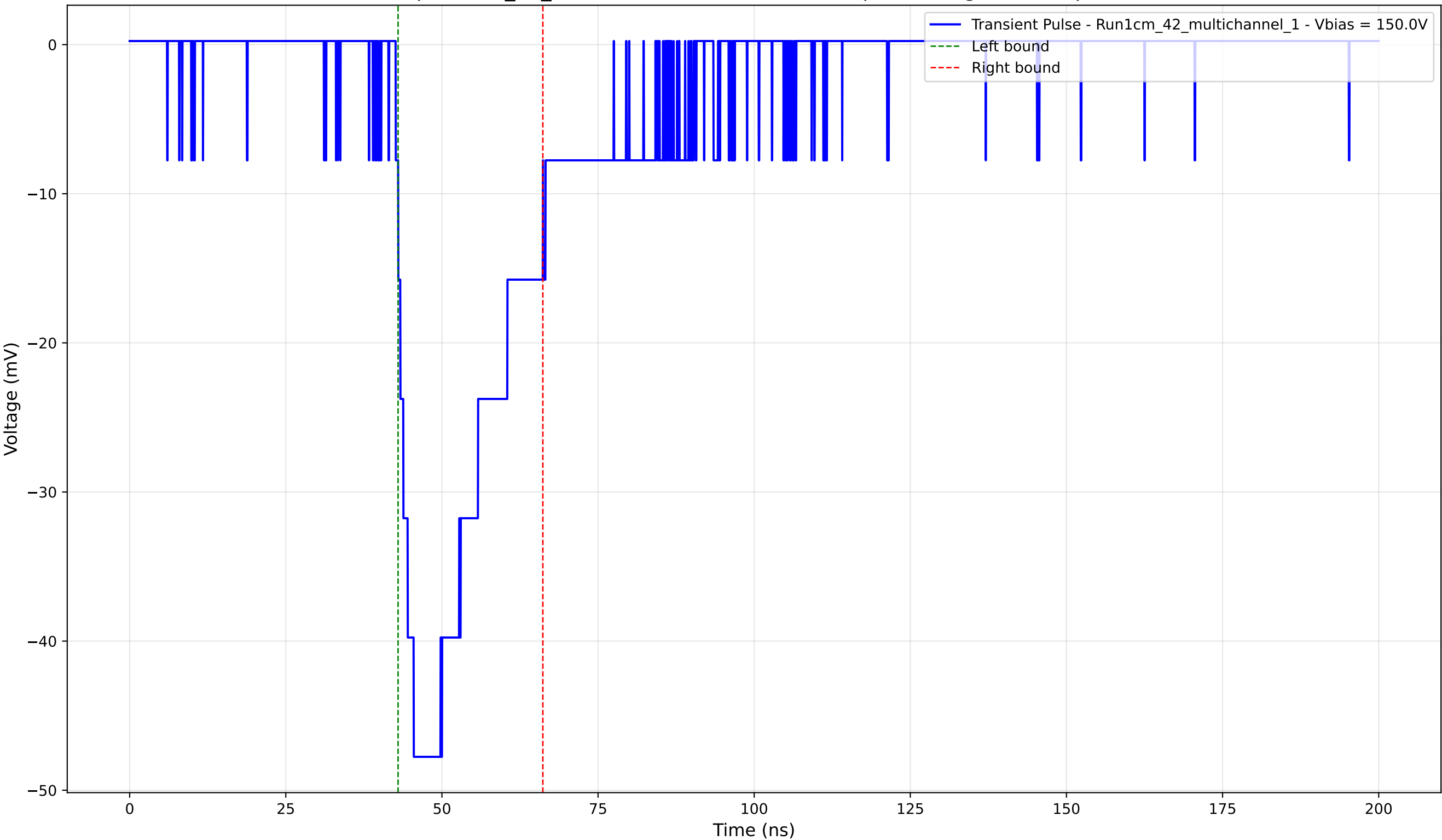
Transient Pulse - Sample: 1cm_42_multichannel - Position: 100.0 \mu\text{m} - Charge: -14.00 pC - Rise Time: 2.89 ns
