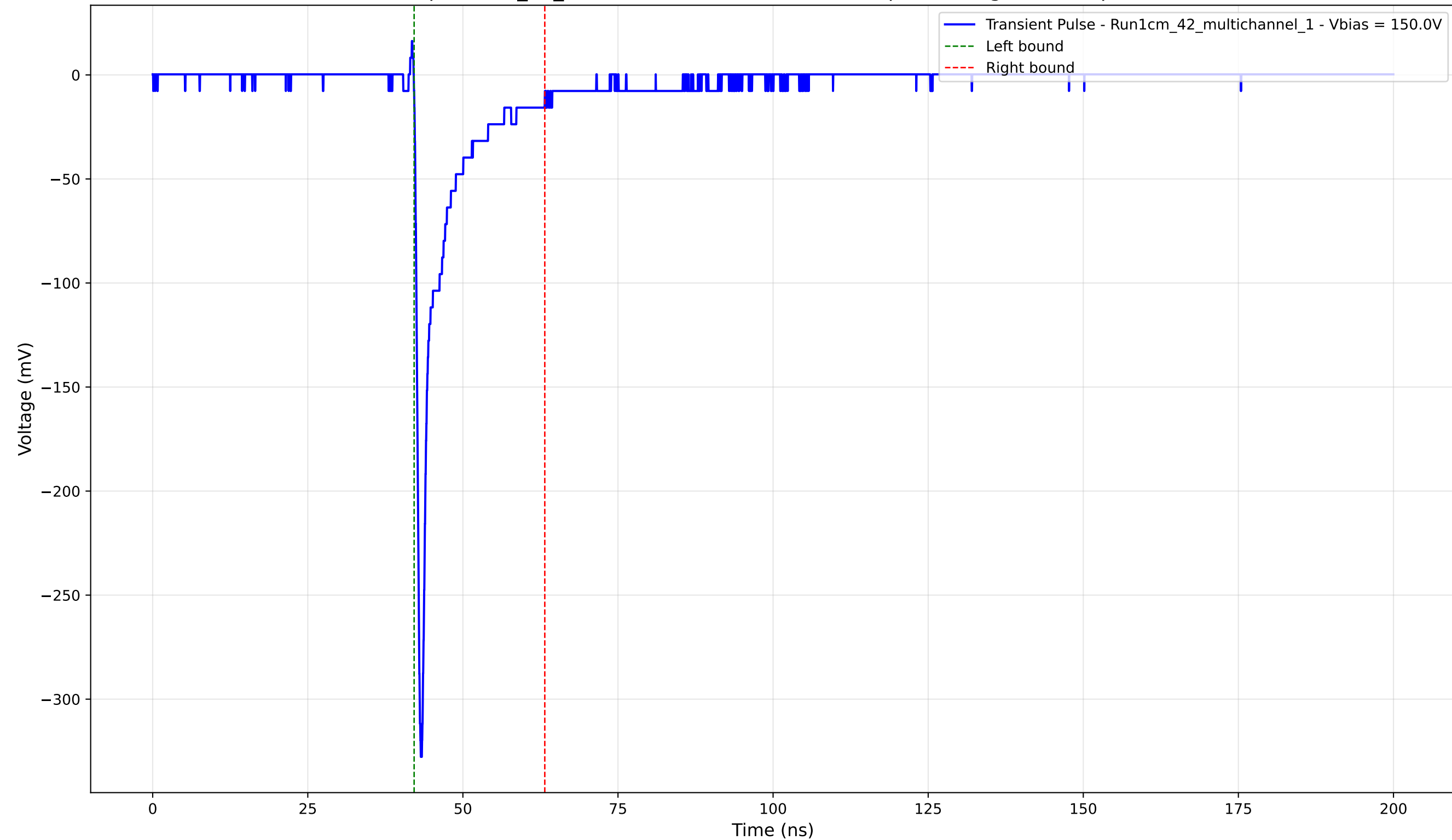
Transient Pulse - Sample: 1cm_42_multichannel - Position: 2140.0 \mu\text{m} - Charge: -24.36 pC - Rise Time: 0.74 ns
