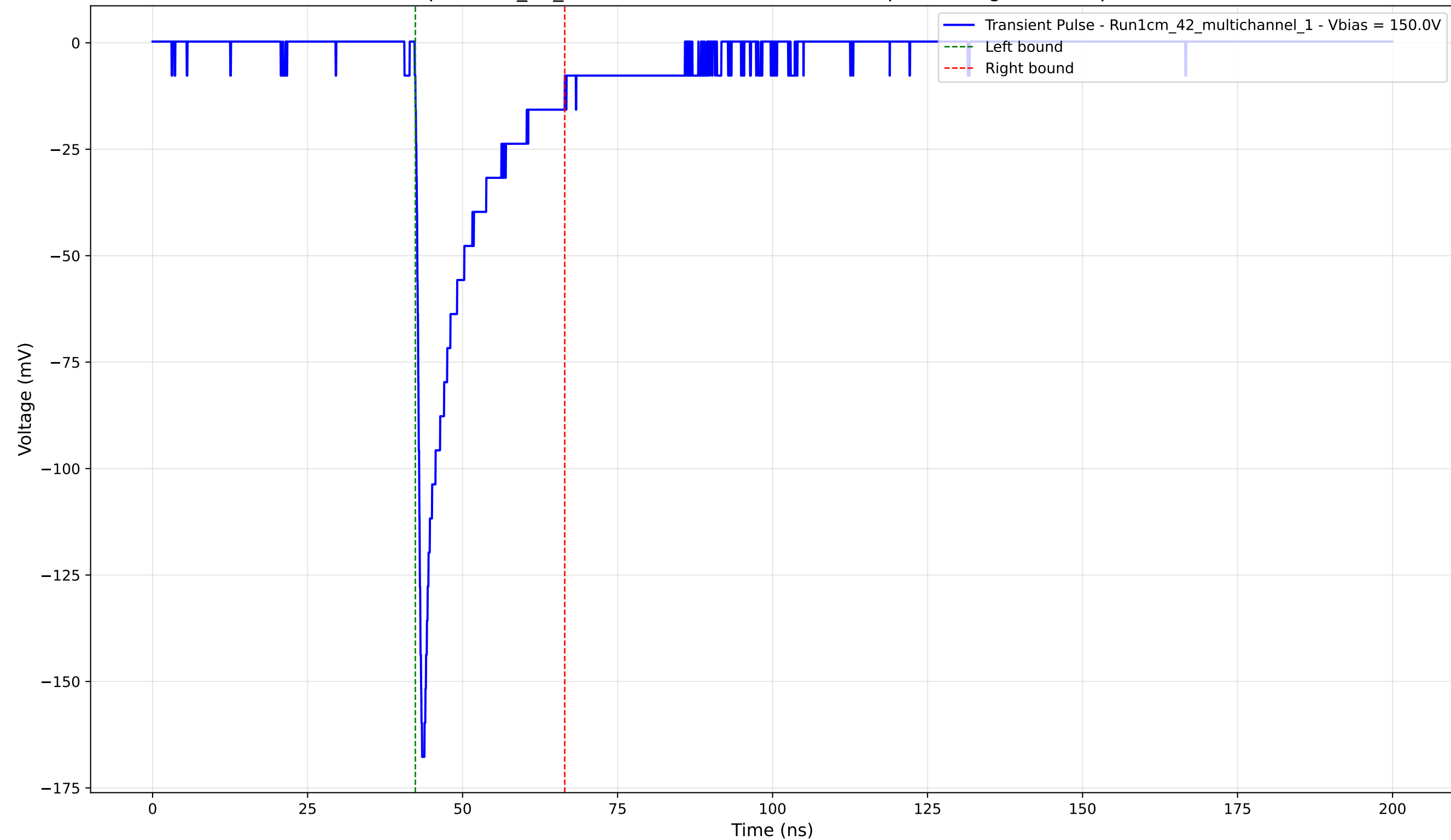
Transient Pulse - Sample: 1cm_42_multichannel - Position: 1720.0 \mu\text{m} - Charge: -22.84 pC - Rise Time: 0.84 ns
