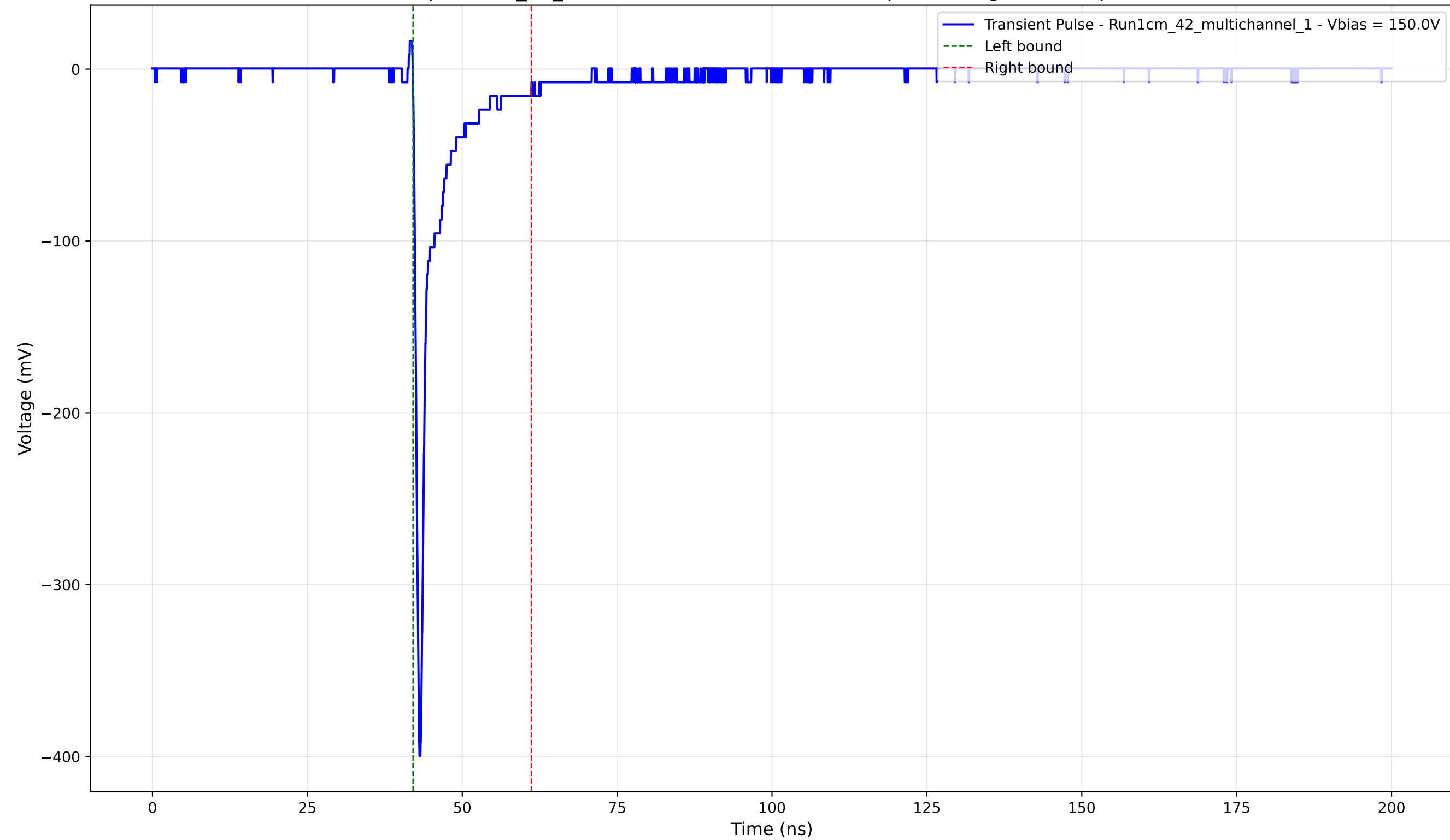
Transient Pulse - Sample: 1cm_42_multichannel - Position: 2300.0 \mu\text{m} - Charge: -23.79 pC - Rise Time: 0.72 ns
