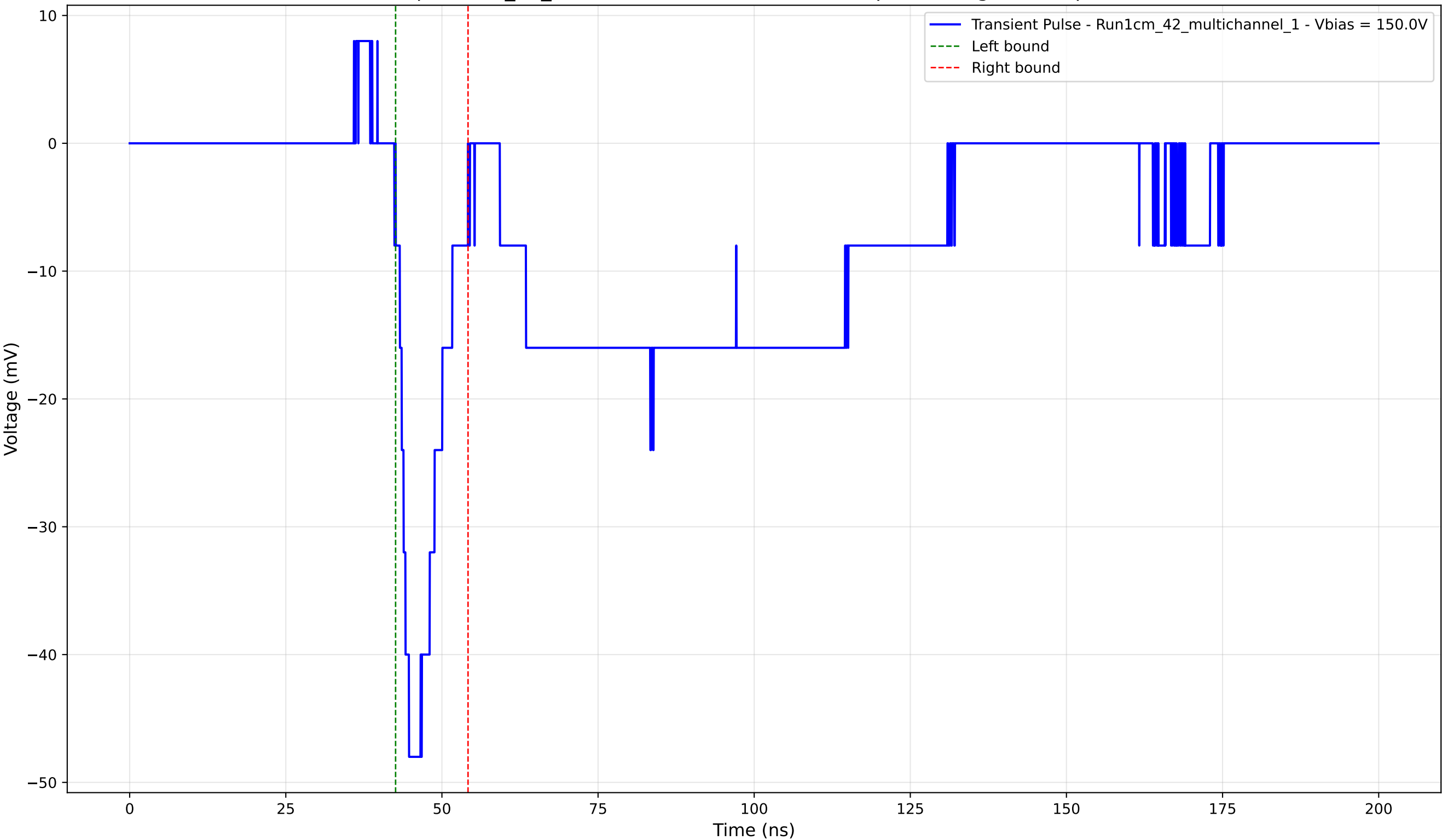
Transient Pulse - Sample: 1cm_42_multichannel - Position: 4290.0 \mu\text{m} - Charge: -5.97 pC - Rise Time: 2.13 ns
