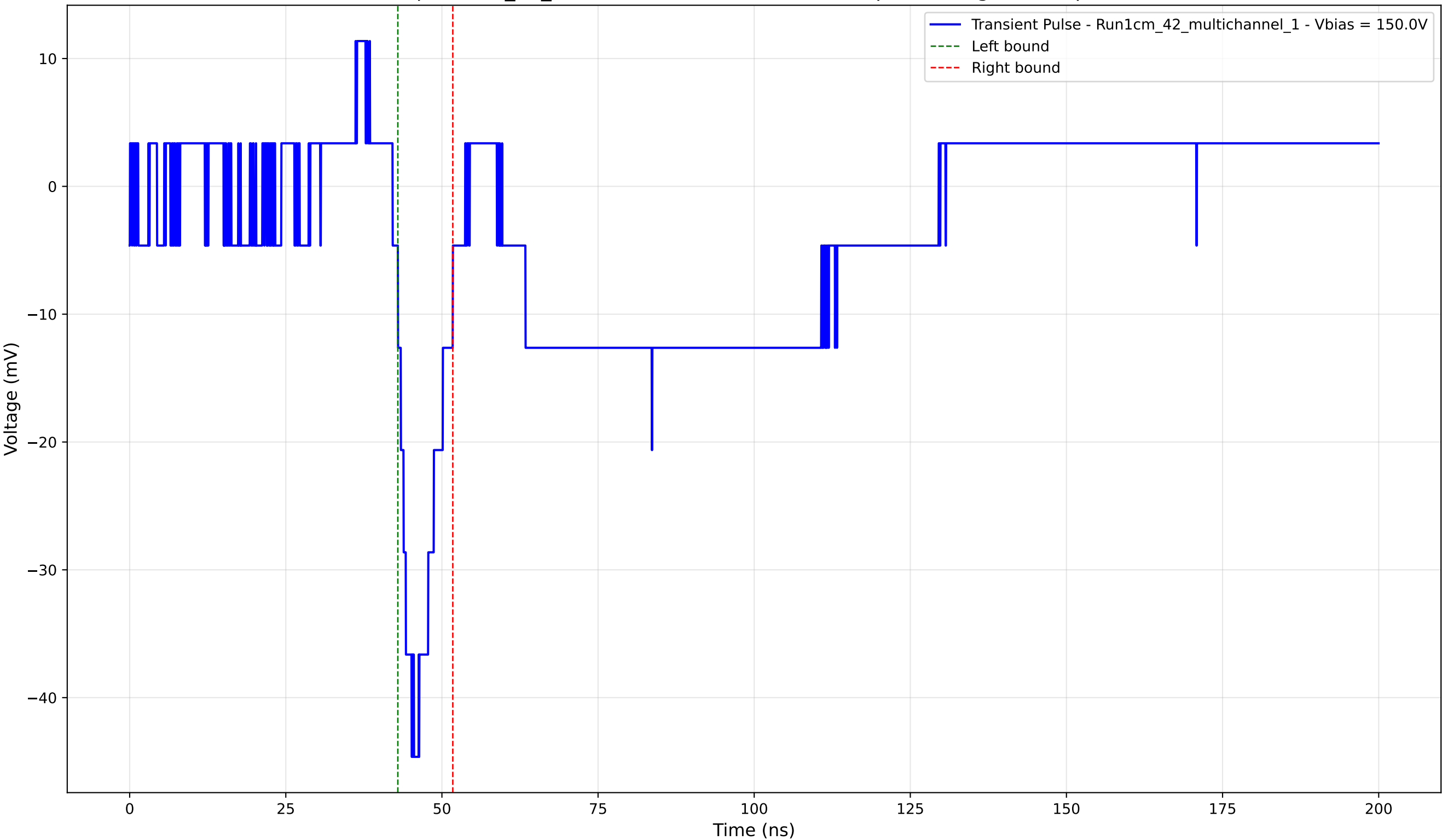
Transient Pulse - Sample: 1cm_42_multichannel - Position: 4730.0 \mu\text{m} - Charge: -4.81 pC - Rise Time: 3.04 ns
