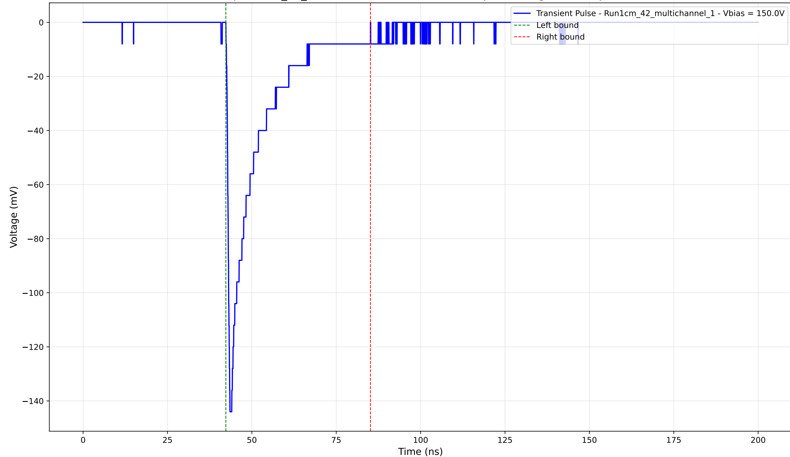
Transient Pulse - Sample: 1cm_42_multichannel - Position: 1620.0 \mu\text{m} - Charge: -25.56 pC - Rise Time: 0.96 ns
