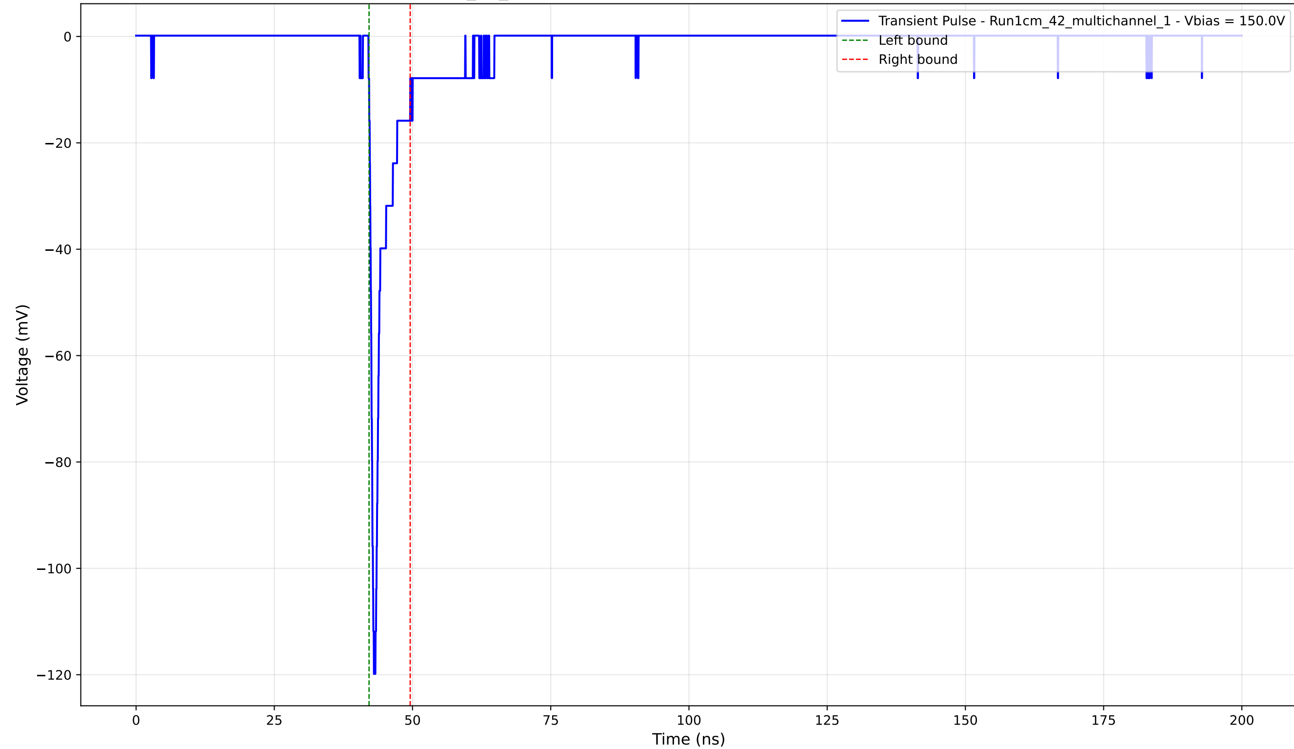
Transient Pulse - Sample: 1cm_42_multichannel - Position: 2345.0 \mu\text{m} - Charge: -5.88 pC - Rise Time: 0.75 ns
