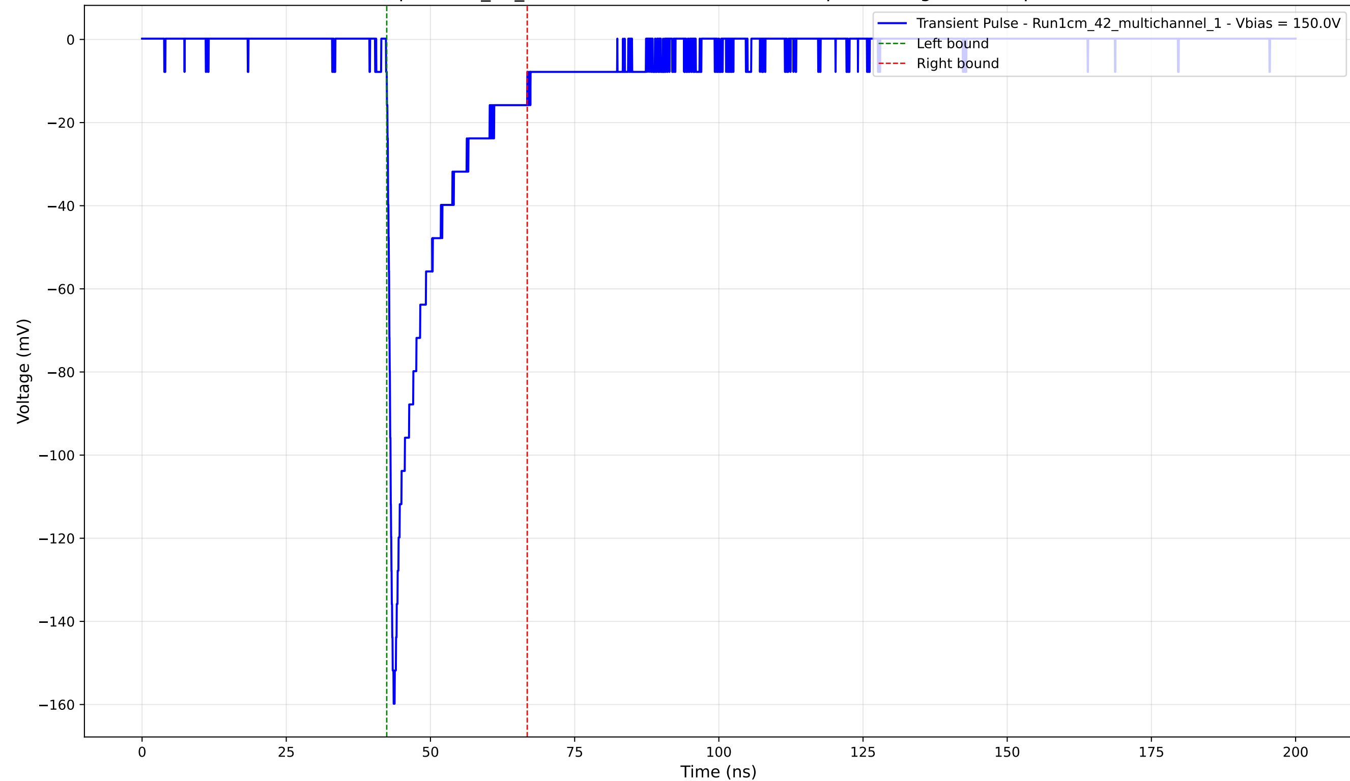
Transient Pulse - Sample: 1cm_42_multichannel - Position: 1675.0 \mu\text{m} - Charge: -22.62 pC - Rise Time: 0.92 ns
