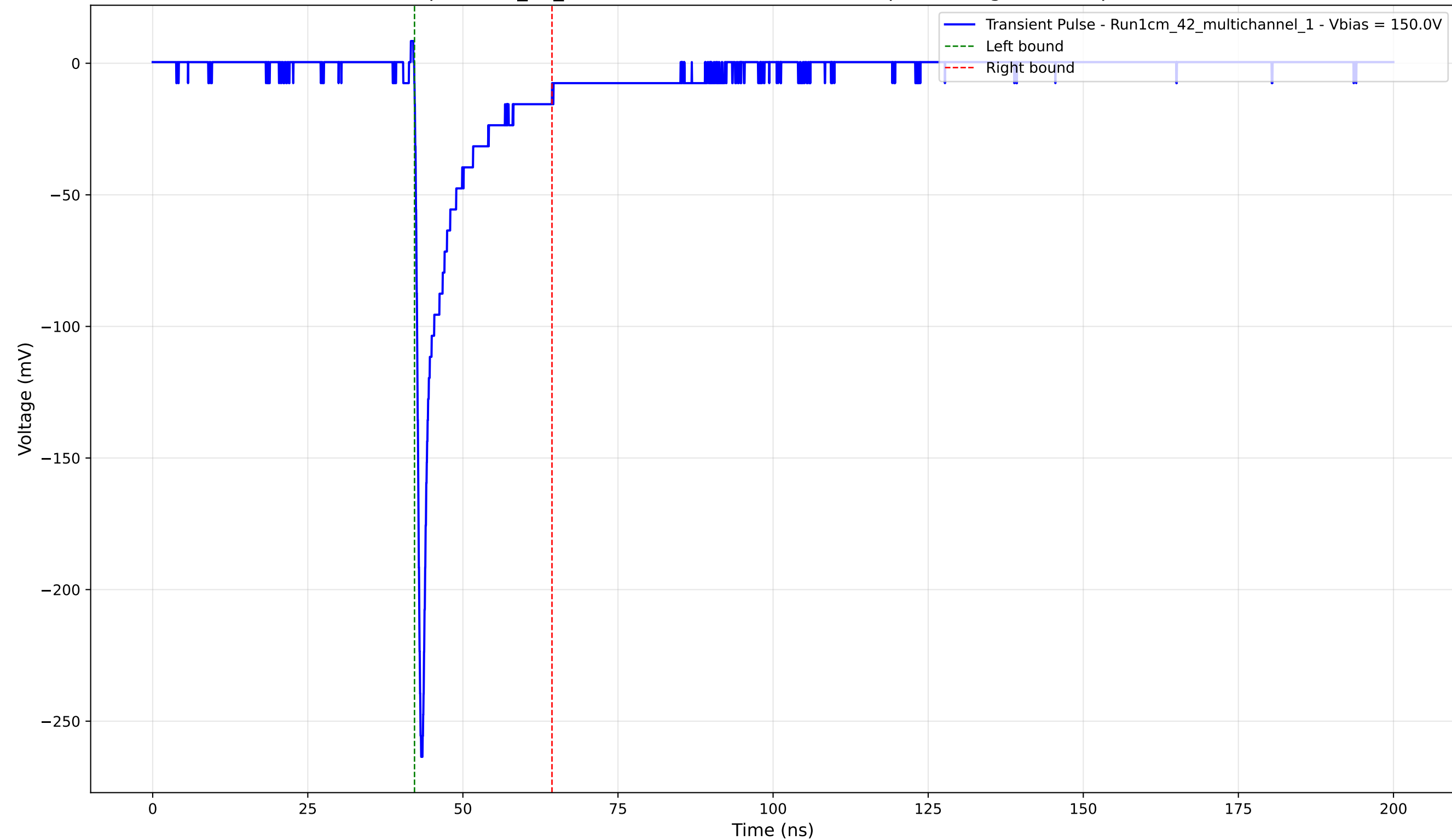
Transient Pulse - Sample: 1cm_42_multichannel - Position: 2735.0 \mu\text{m} - Charge: -22.66 pC - Rise Time: 0.79 ns
