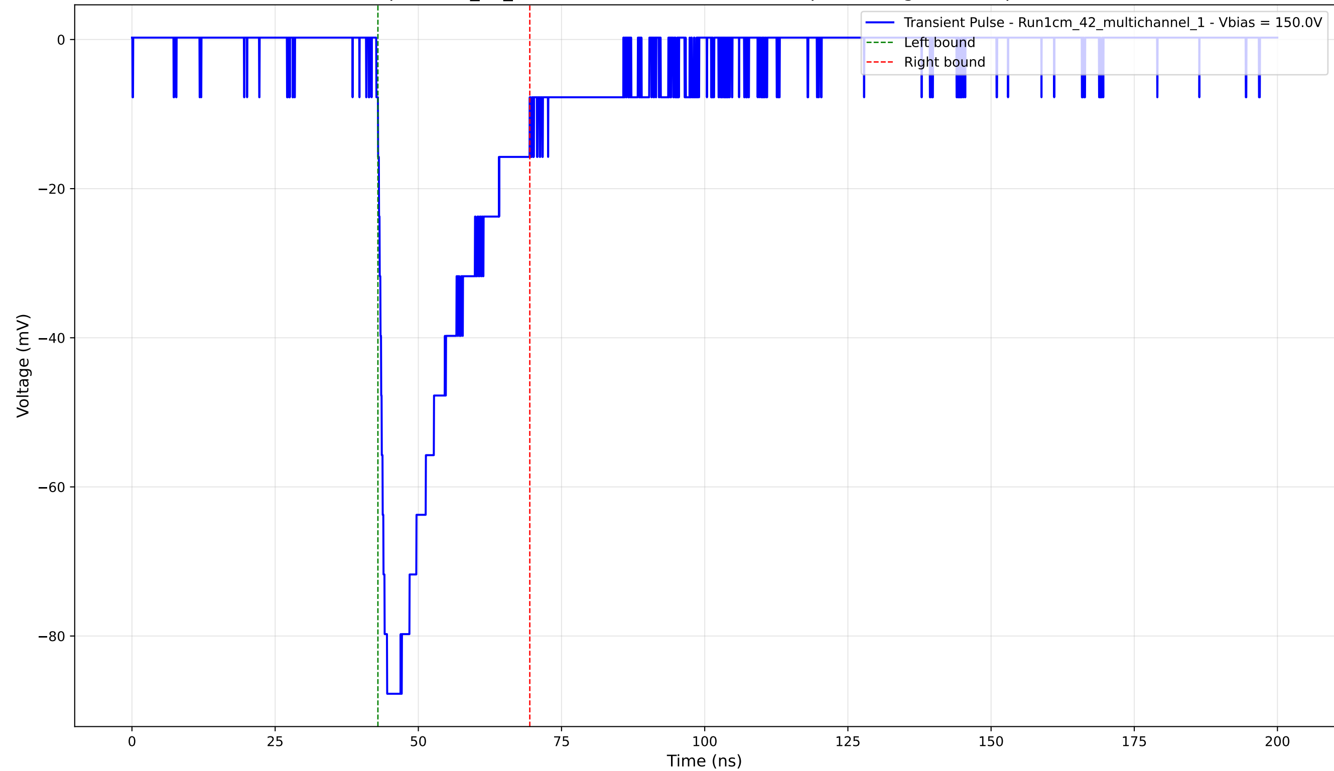
Transient Pulse - Sample: 1cm_42_multichannel - Position: 1005.0 \mu\text{m} - Charge: -23.17 pC - Rise Time: 1.16 ns
