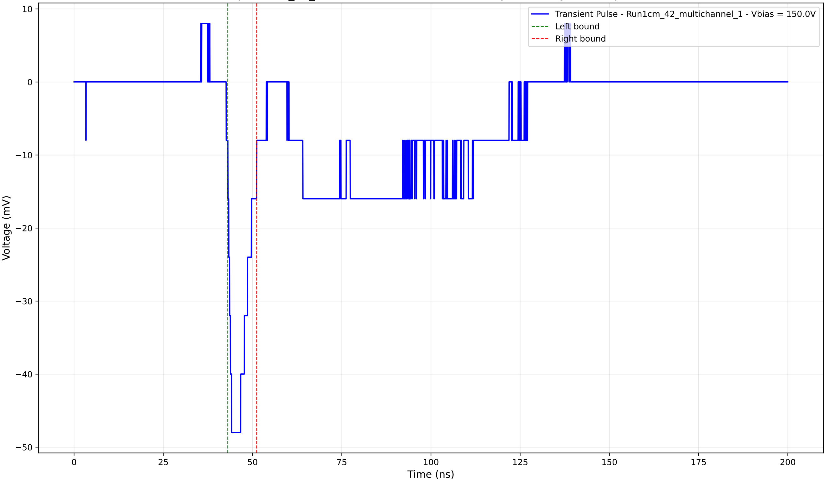
Transient Pulse - Sample: 1cm_42_multichannel - Position: 4015.0 \mu\text{m} - Charge: -5.44 pC - Rise Time: 1.53 ns
