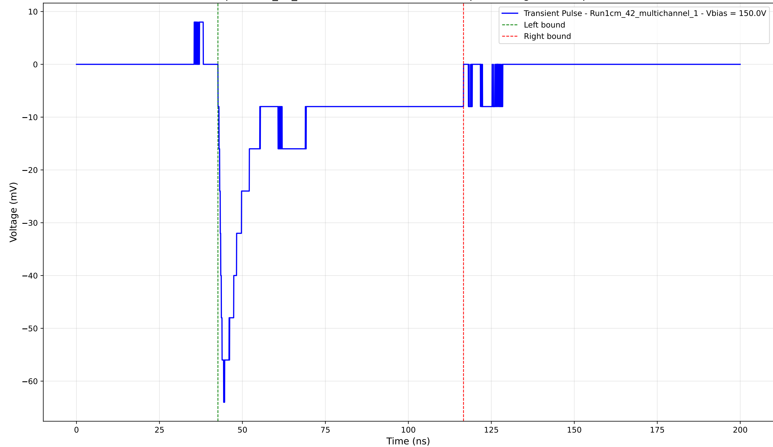
Transient Pulse - Sample: 1cm_42_multichannel - Position: 3750.0 \mu\text{m} - Charge: -19.26 pC - Rise Time: 1.70 ns
