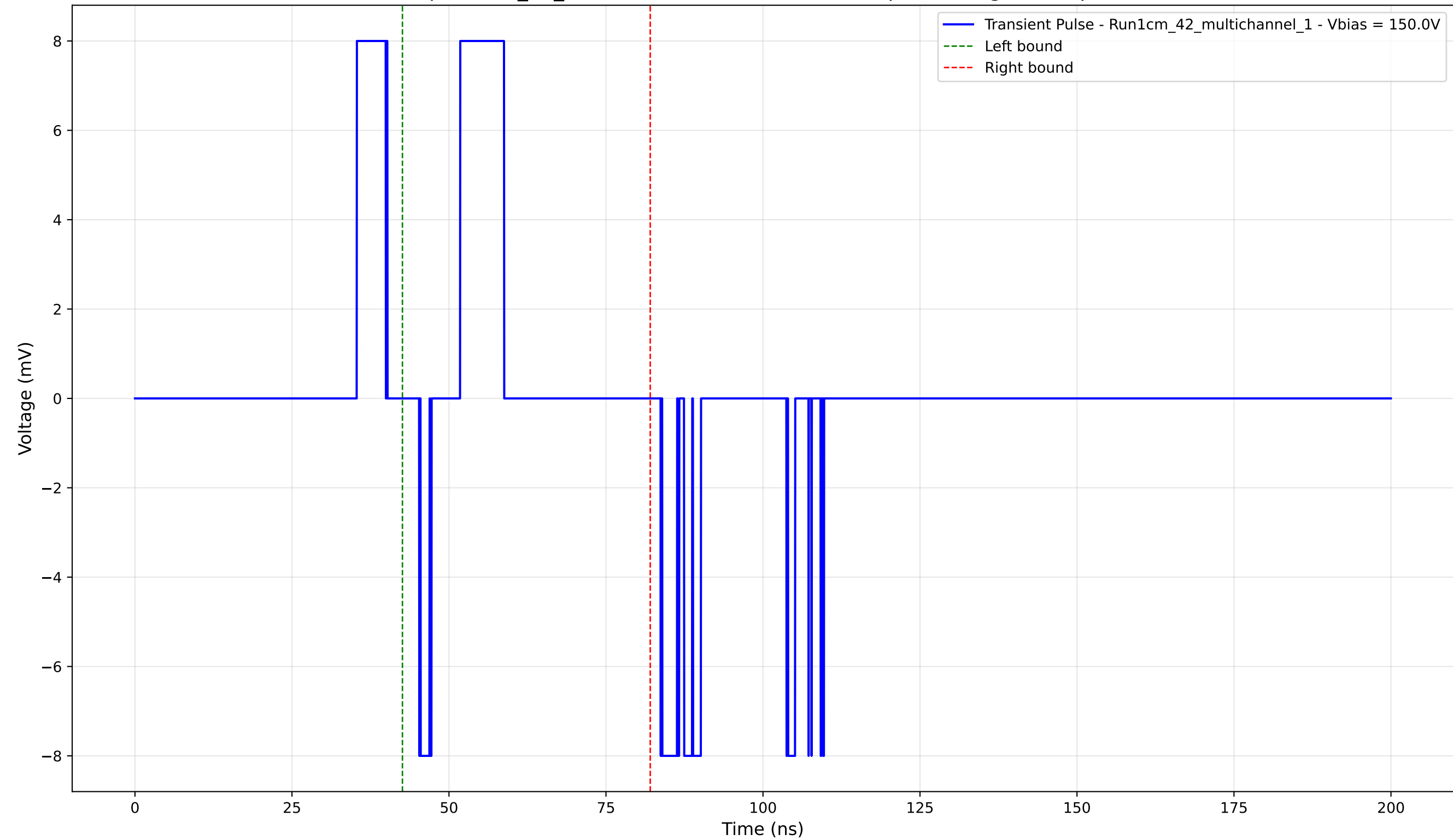
Transient Pulse - Sample: 1cm_42_multichannel - Position: 4430.0 \mu\text{m} - Charge: 0.84 pC - Rise Time: 0.02 ns
