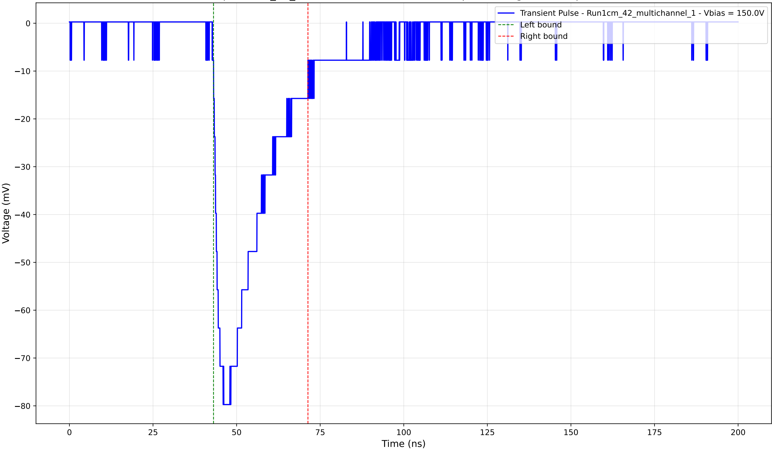
Transient Pulse - Sample: 1cm_42_multichannel - Position: 505.0 \mu\text{m} - Charge: -23.31 pC - Rise Time: 2.86 ns
