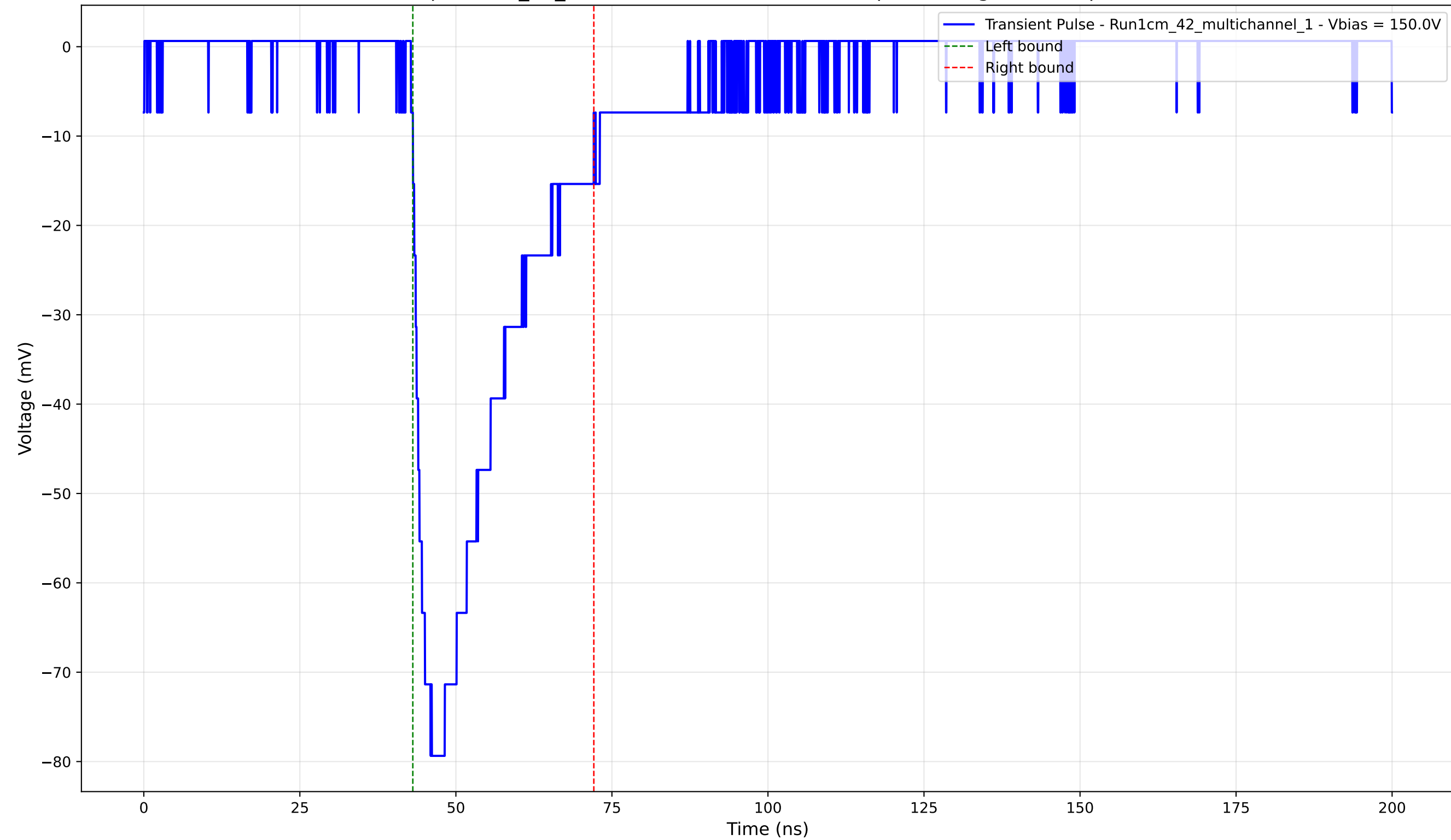
Transient Pulse - Sample: 1cm_42_multichannel - Position: 510.0 \mu\text{m} - Charge: -23.09 pC - Rise Time: 2.84 ns
