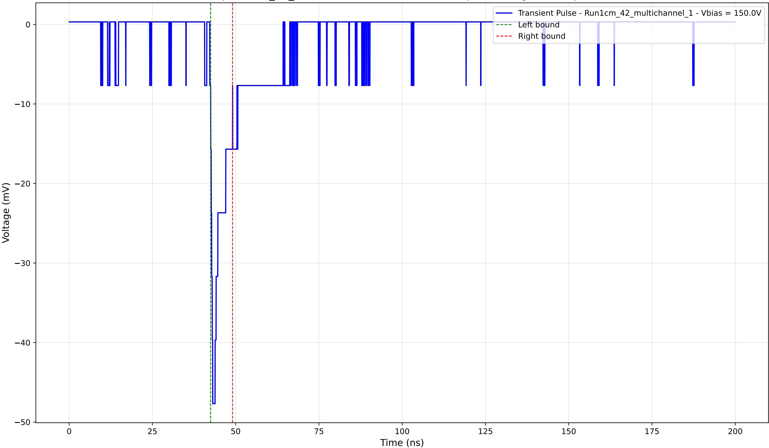
Transient Pulse - Sample: 1cm_42_multichannel - Position: 2855.0 \mu\text{m} - Charge: -3.36 pC - Rise Time: 0.89 ns
