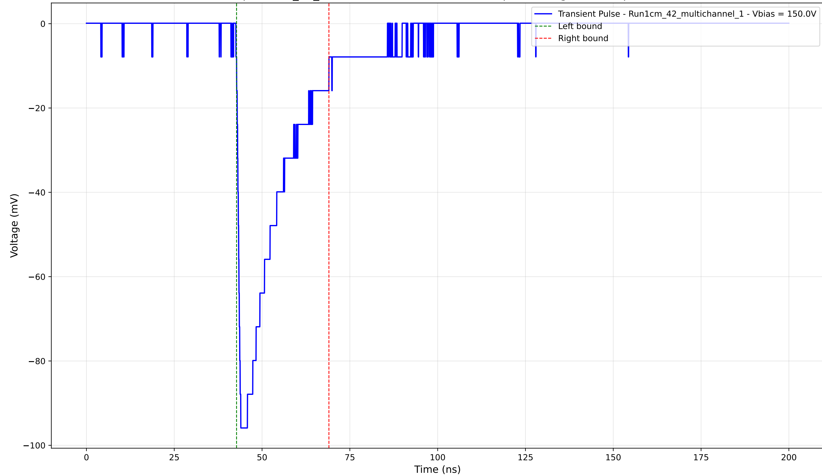
Transient Pulse - Sample: 1cm_42_multichannel - Position: 1215.0 \mu\text{m} - Charge: -23.42 pC - Rise Time: 1.02 ns
