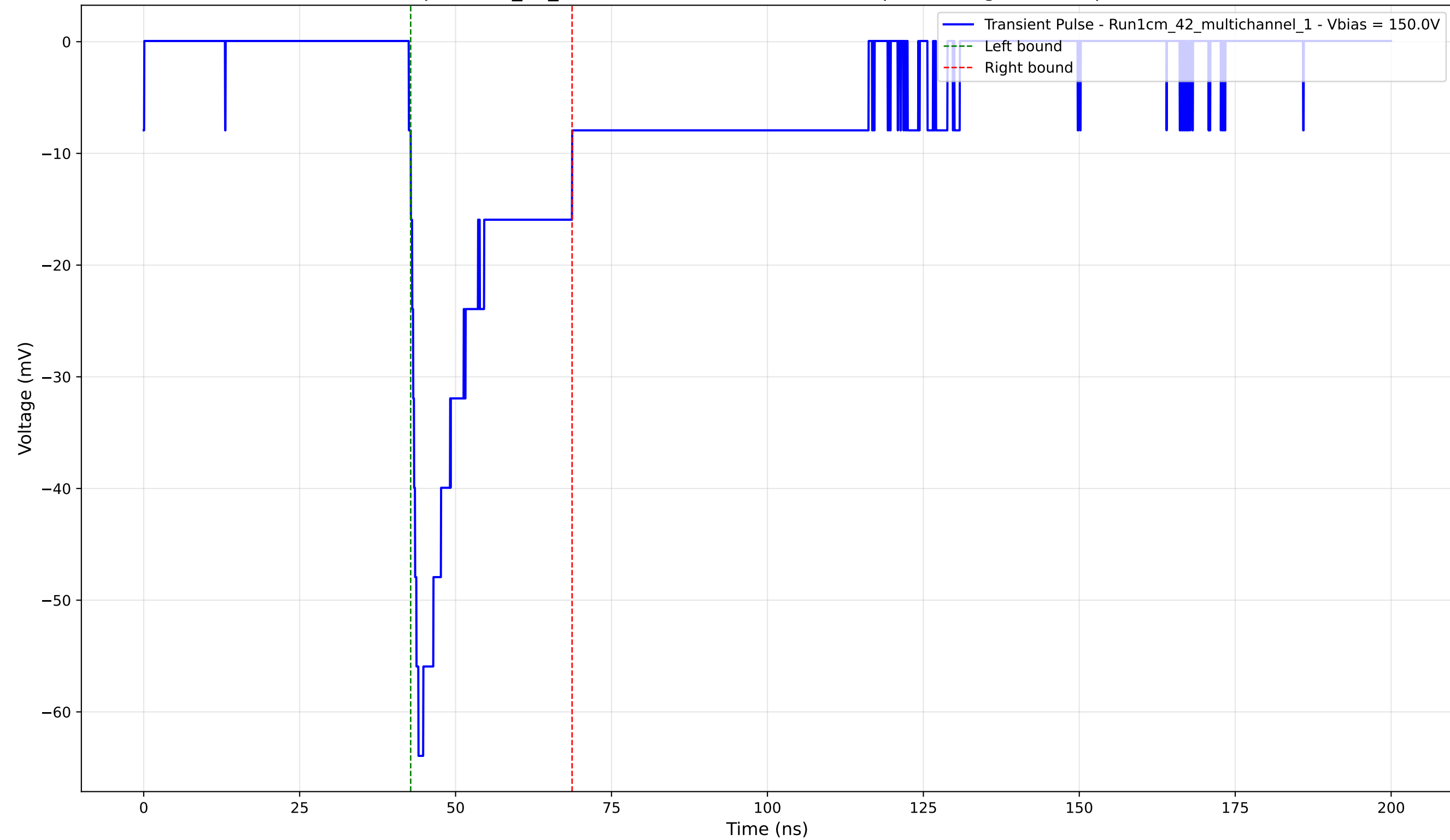
Transient Pulse - Sample: 1cm_42_multichannel - Position: 3675.0 \mu\text{m} - Charge: -13.54 pC - Rise Time: 1.54 ns
