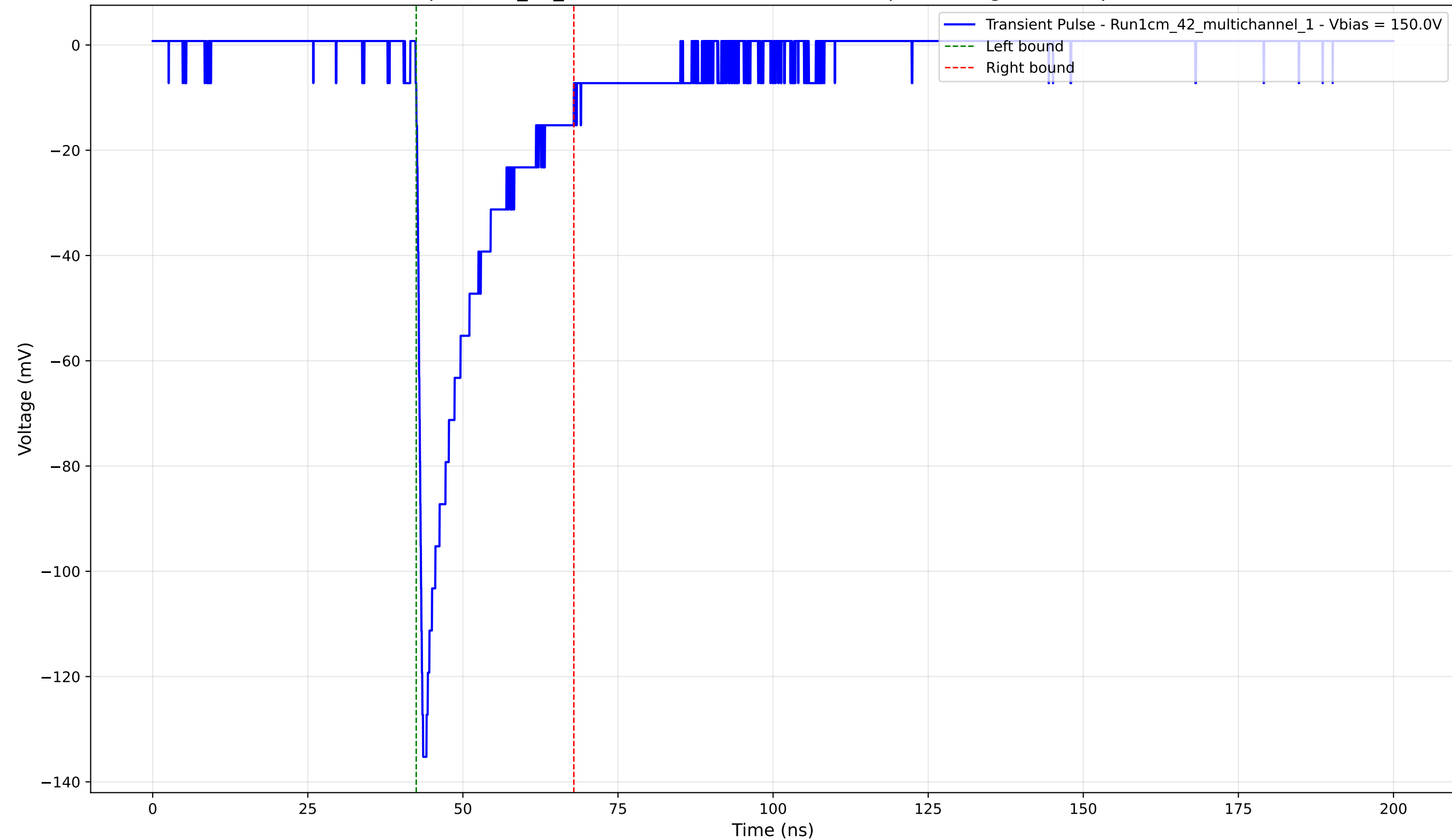
Transient Pulse - Sample: 1cm_42_multichannel - Position: 1560.0 \mu\text{m} - Charge: -22.98 pC - Rise Time: 0.96 ns
