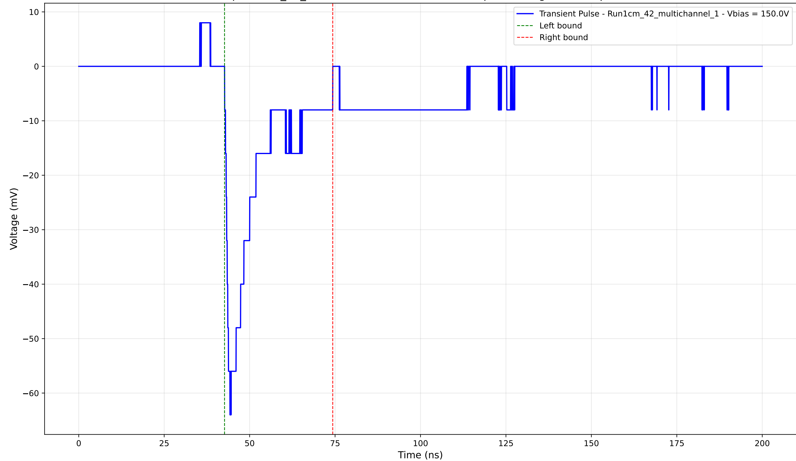
Transient Pulse - Sample: 1cm_42_multichannel - Position: 3715.0 \mu\text{m} - Charge: -12.04 pC - Rise Time: 1.56 ns
