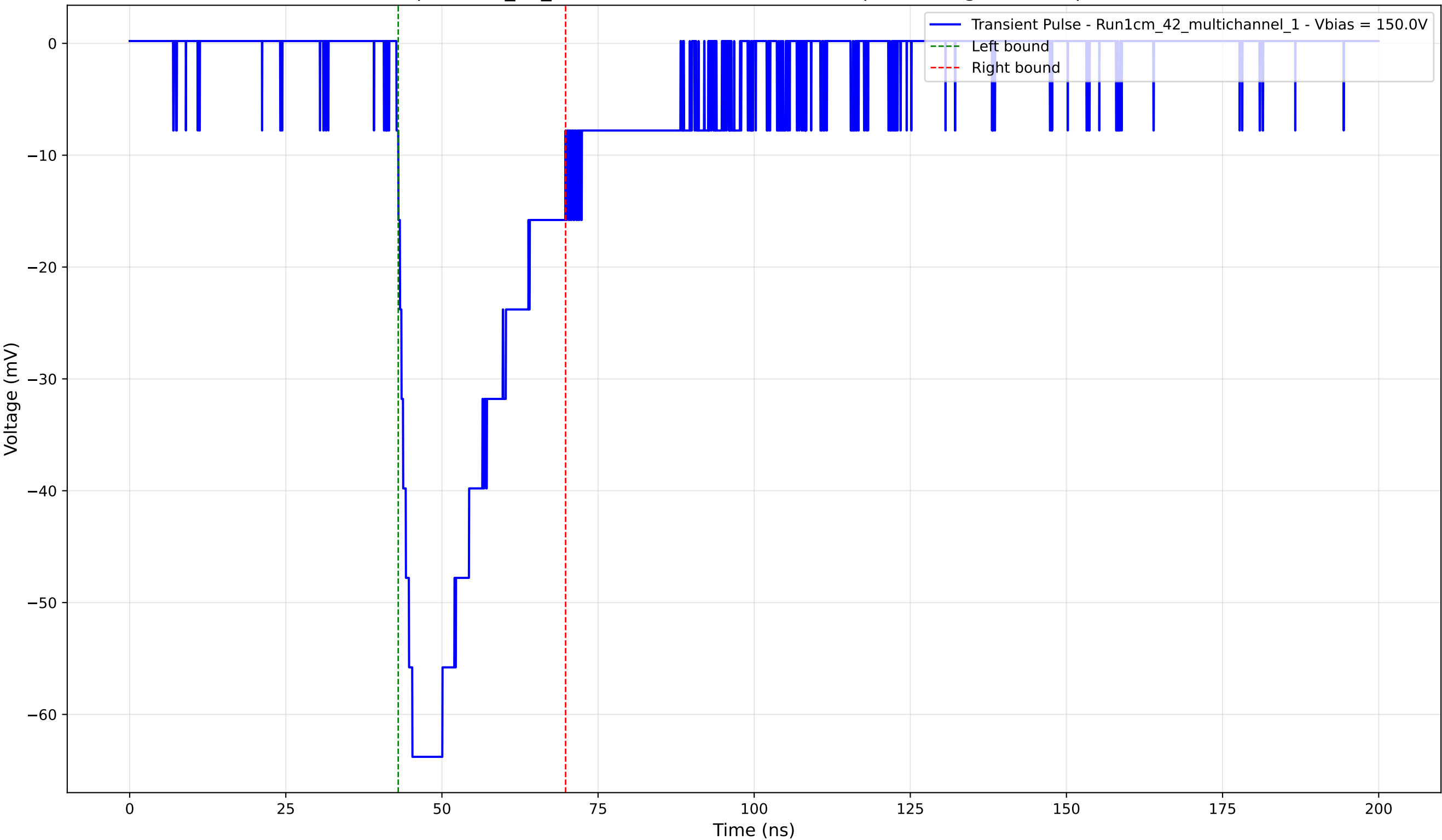
Transient Pulse - Sample: 1cm_42_multichannel - Position: 240.0 \mu\text{m} - Charge: -20.11 pC - Rise Time: 2.54 ns
