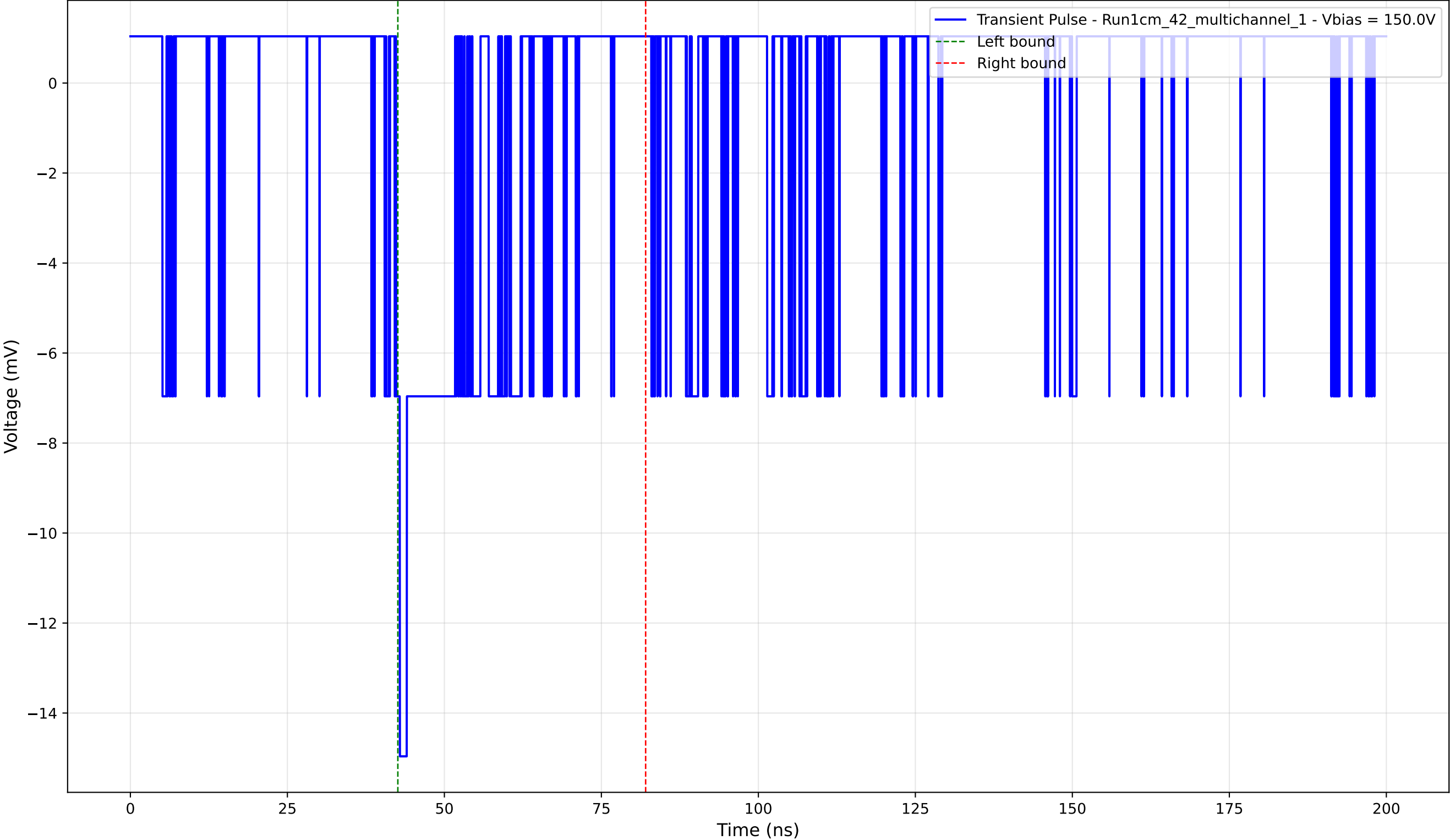
Transient Pulse - Sample: 1cm_42_multichannel - Position: 2875.0 \mu\text{m} - Charge: -2.14 pC - Rise Time: 0.60 ns
