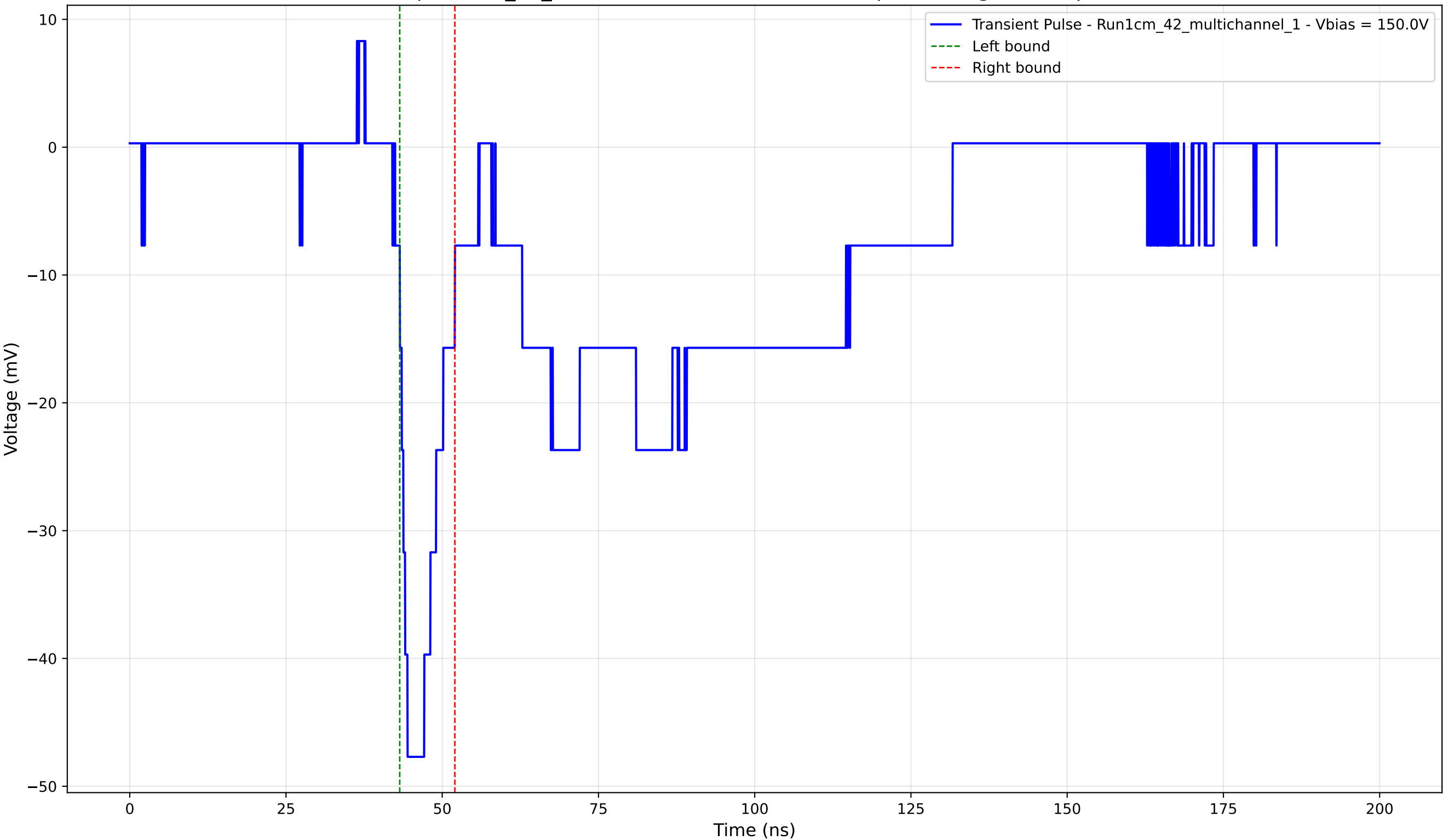
Transient Pulse - Sample: 1cm_42_multichannel - Position: 4250.0 \mu\text{m} - Charge: -5.74 pC - Rise Time: 1.99 ns
