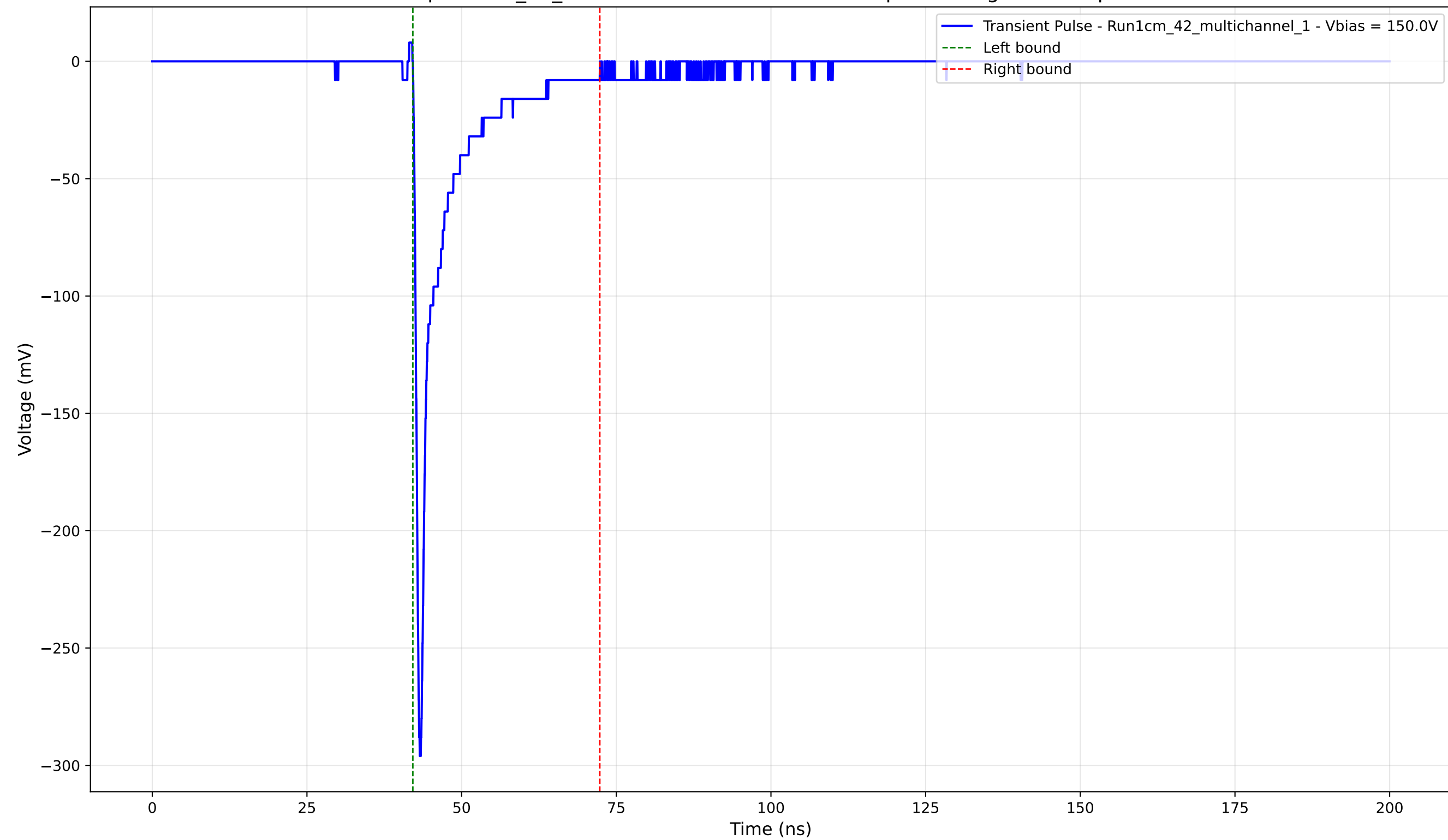
Transient Pulse - Sample: 1cm_42_multichannel - Position: 2670.0 \mu\text{m} - Charge: -24.33 pC - Rise Time: 0.79 ns
