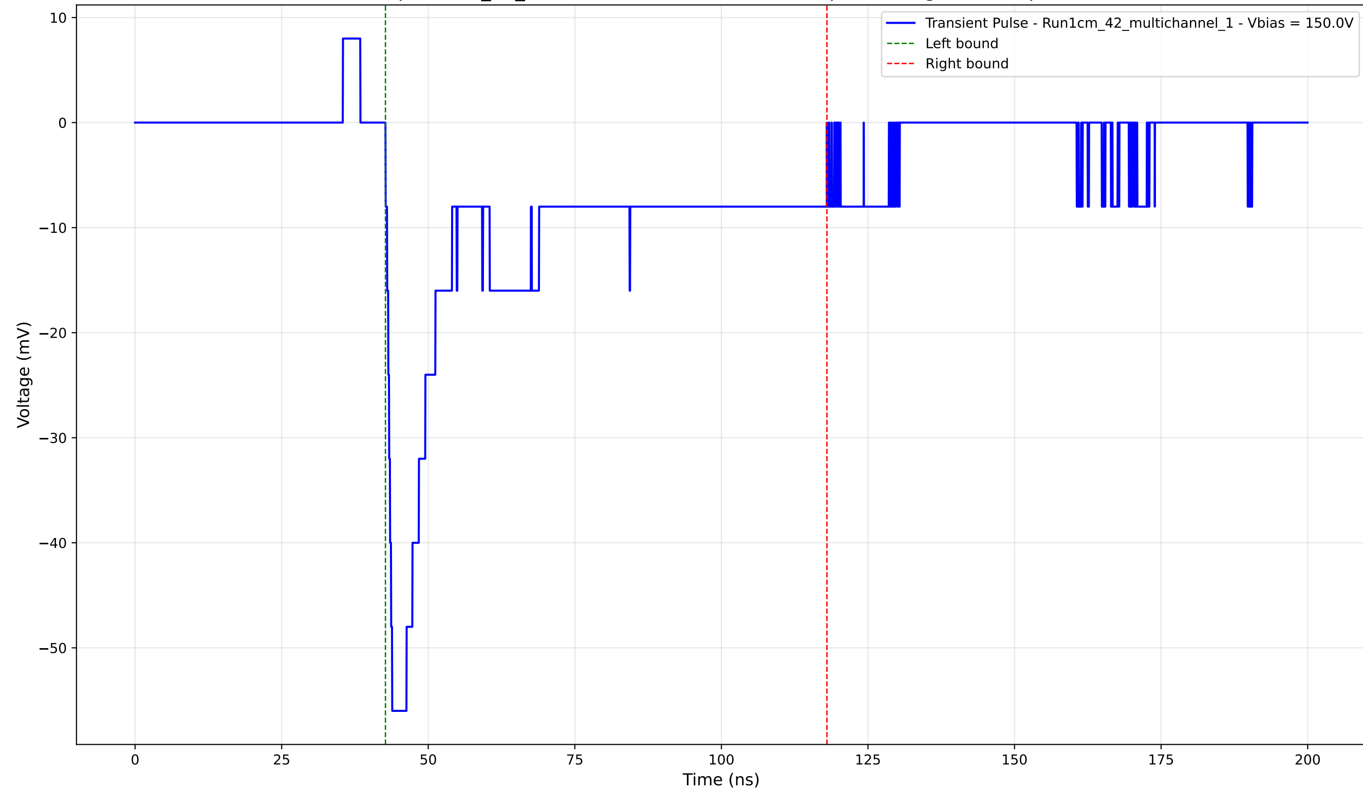
Transient Pulse - Sample: 1cm_42_multichannel - Position: 3760.0 \mu\text{m} - Charge: -19.24 pC - Rise Time: 1.13 ns
