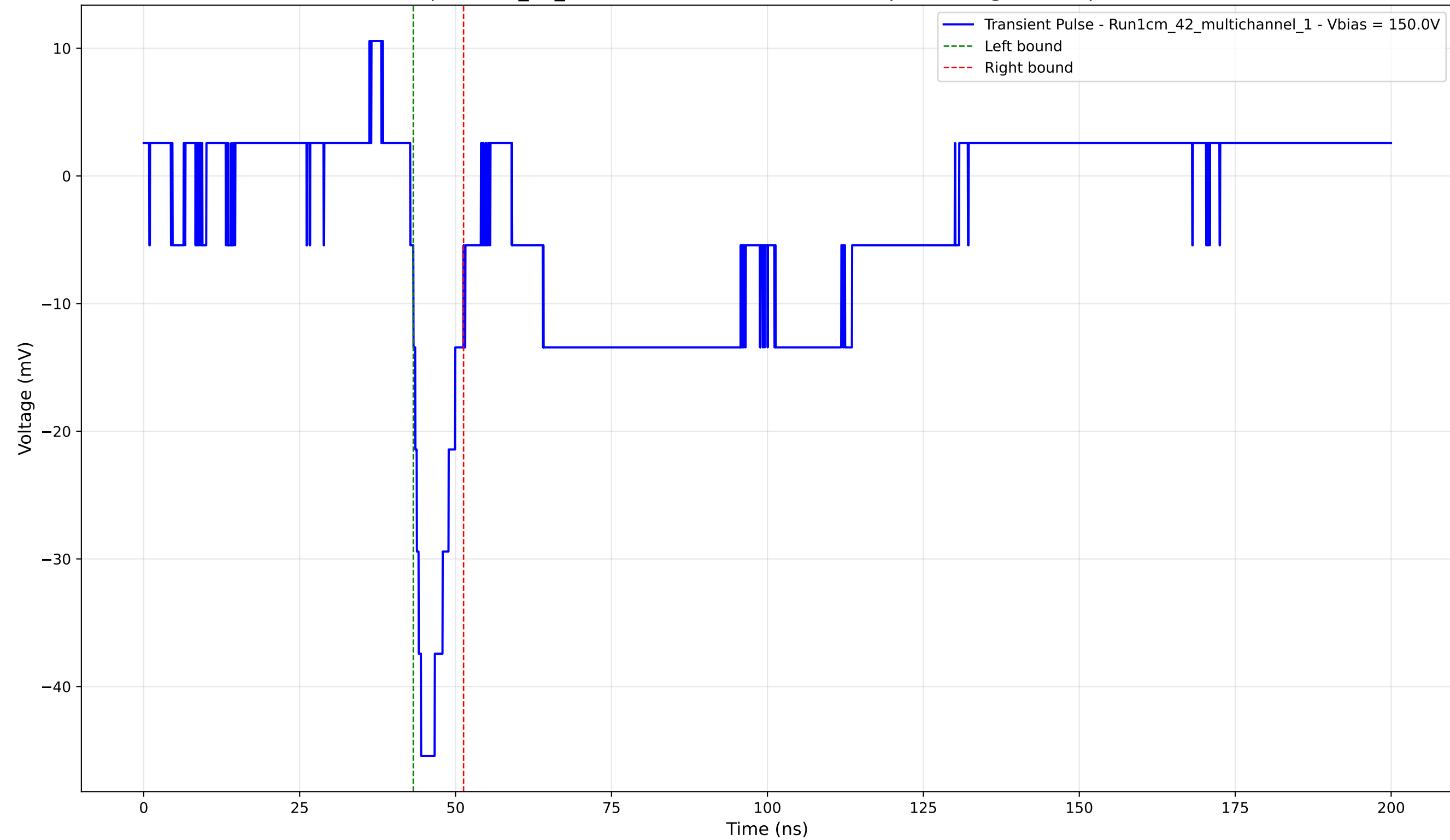
Transient Pulse - Sample: 1cm_42_multichannel - Position: 4205.0 \mu\text{m} - Charge: -4.97 pC - Rise Time: 1.73 ns
