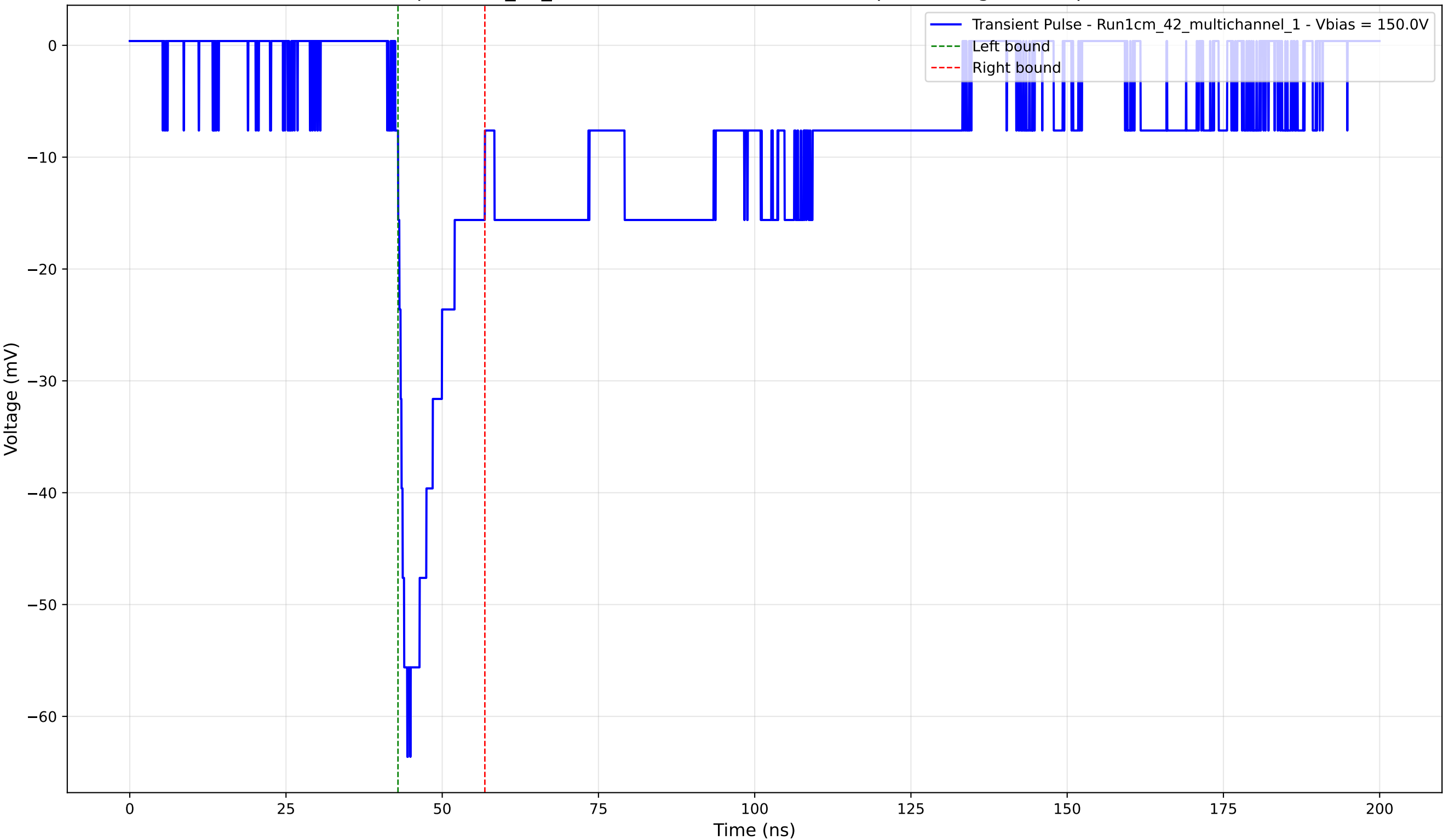
Transient Pulse - Sample: 1cm_42_multichannel - Position: 3800.0 \mu\text{m} - Charge: -8.65 pC - Rise Time: 1.92 ns
