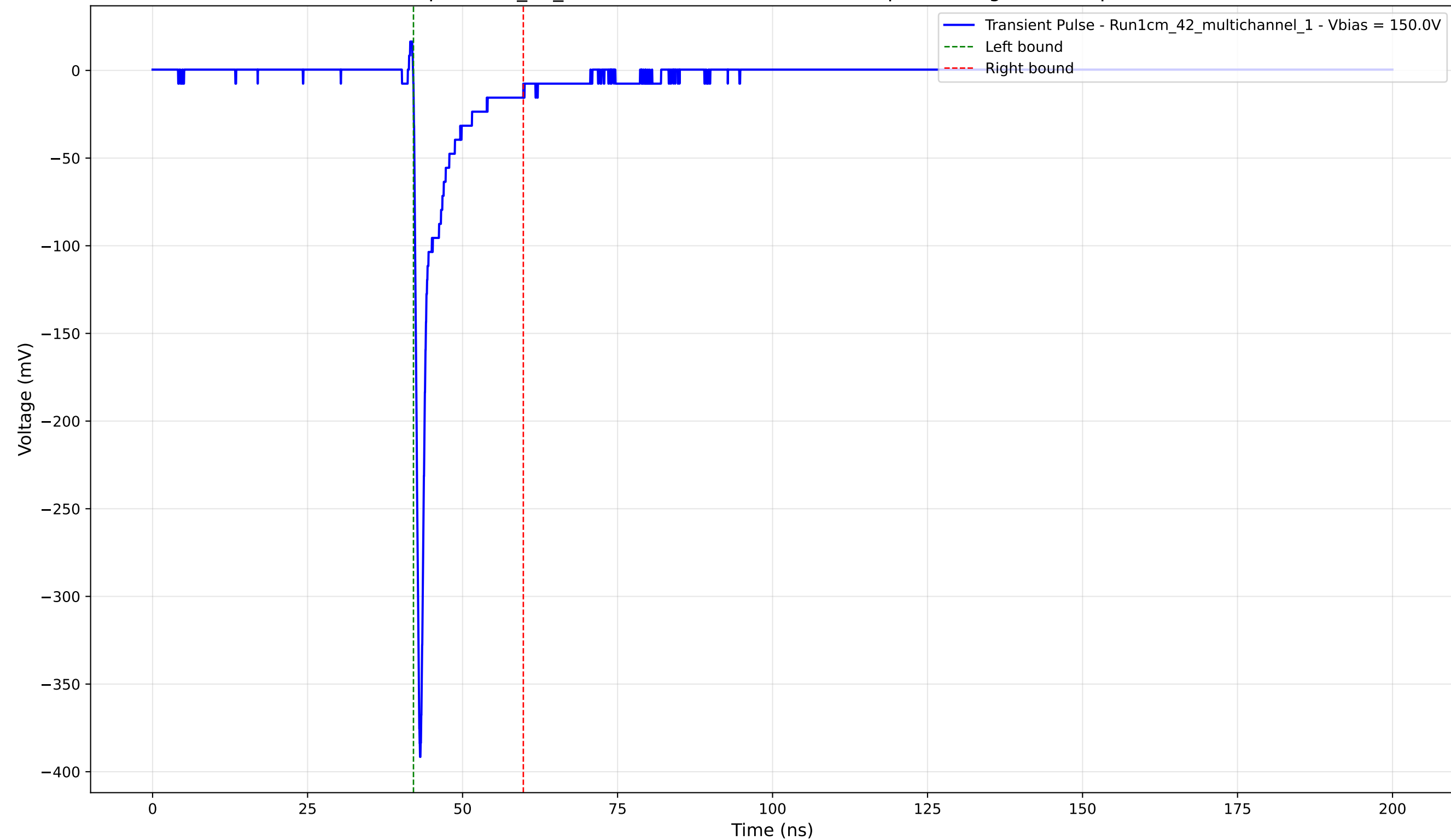
Transient Pulse - Sample: 1cm_42_multichannel - Position: 2470.0 \mu\text{m} - Charge: -22.15 pC - Rise Time: 0.74 ns
