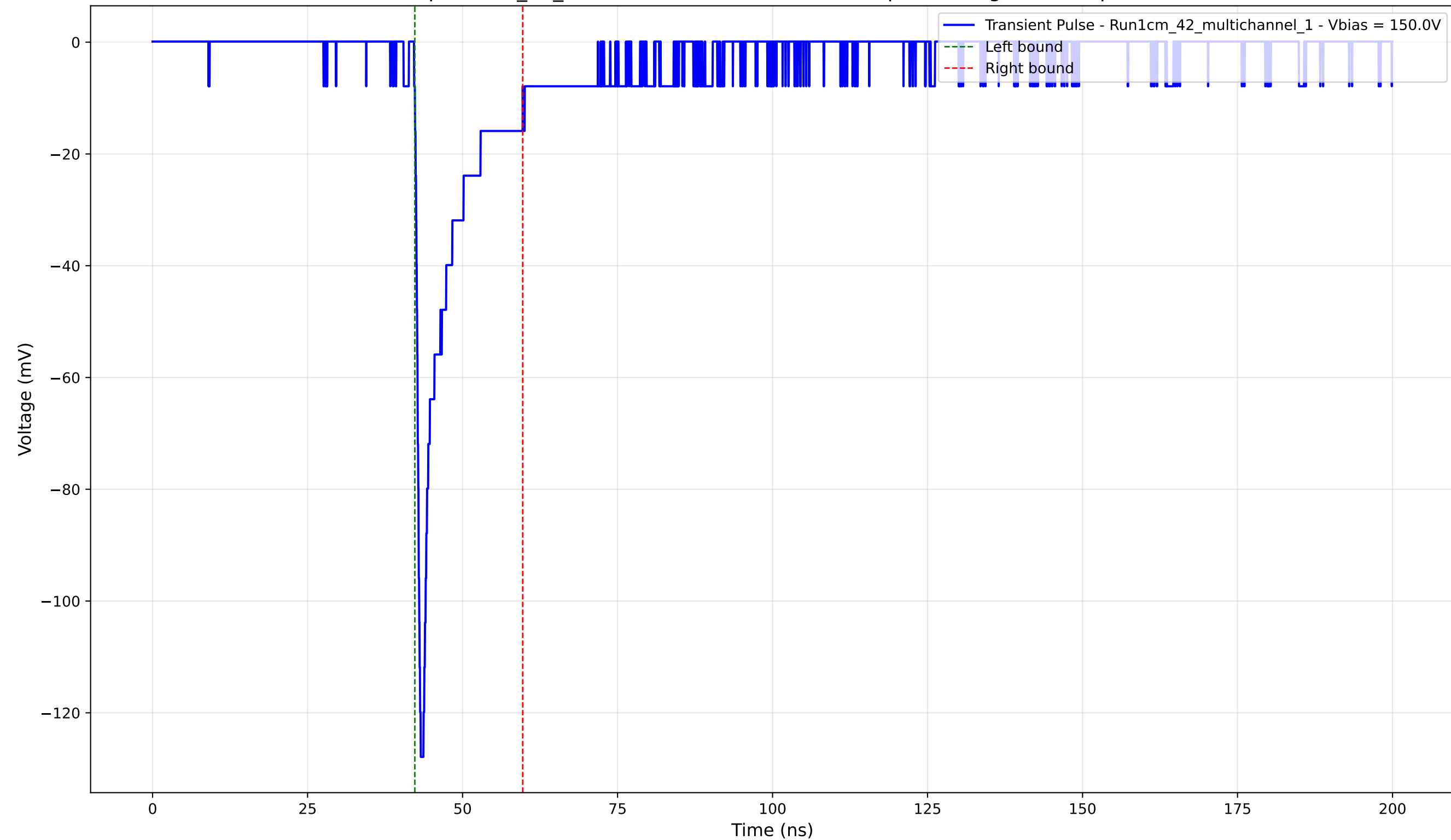
Transient Pulse - Sample: 1cm_42_multichannel - Position: 1935.0 \mu\text{m} - Charge: -12.63 pC - Rise Time: 0.83 ns
