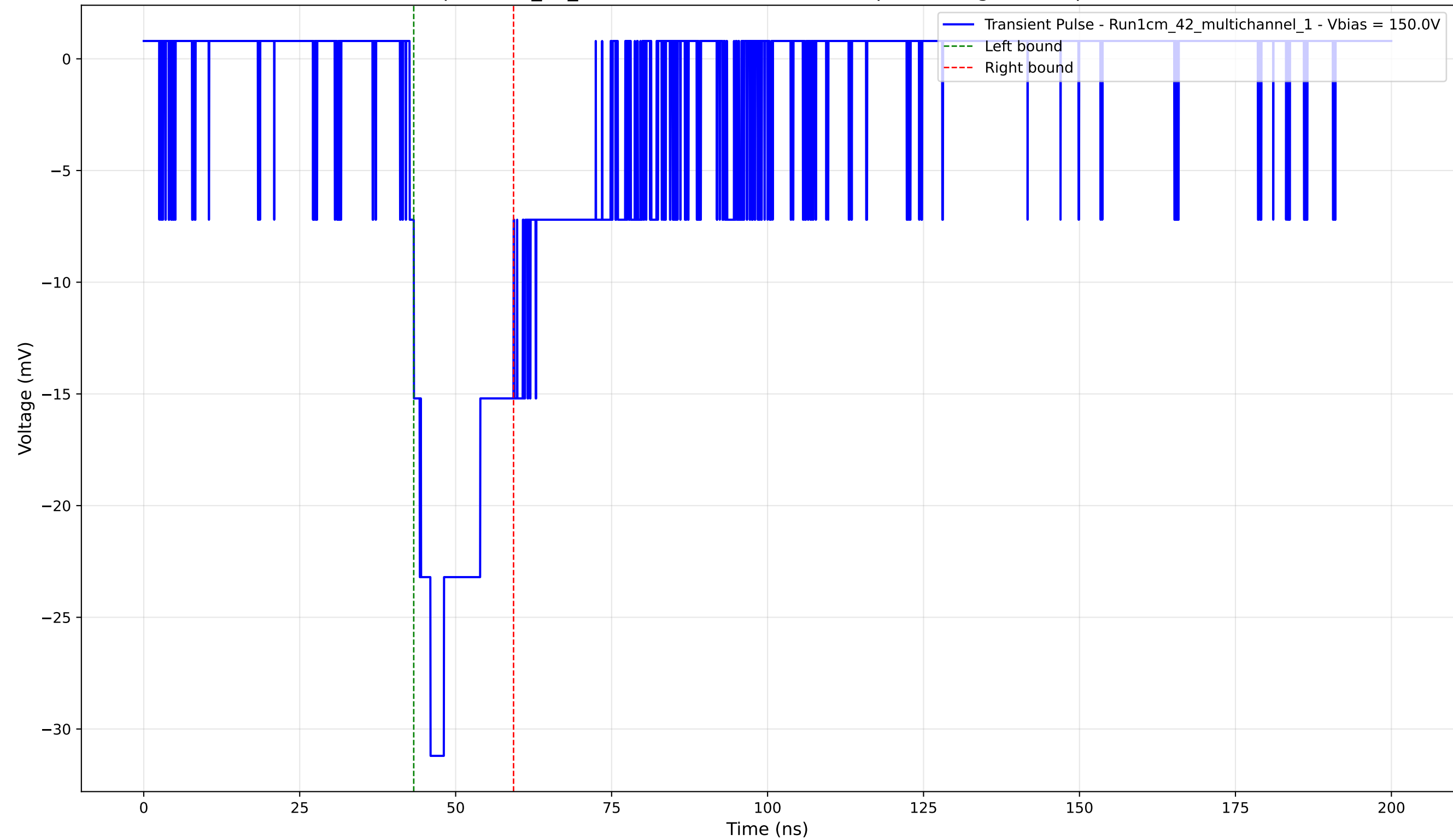
Transient Pulse - Sample: 1cm_42_multichannel - Position: 85.0 \mu\text{m} - Charge: -6.75 pC - Rise Time: 3.35 ns
