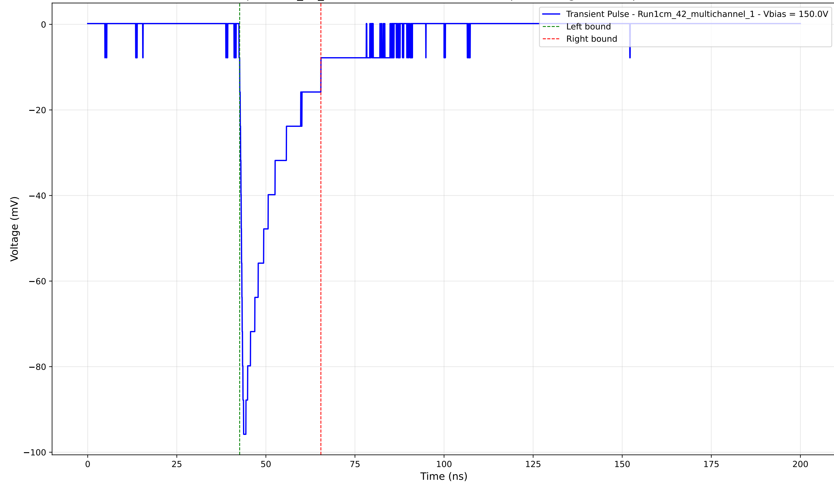
Transient Pulse - Sample: 1cm_42_multichannel - Position: 1440.0 \mu\text{m} - Charge: -17.72 pC - Rise Time: 0.92 ns
