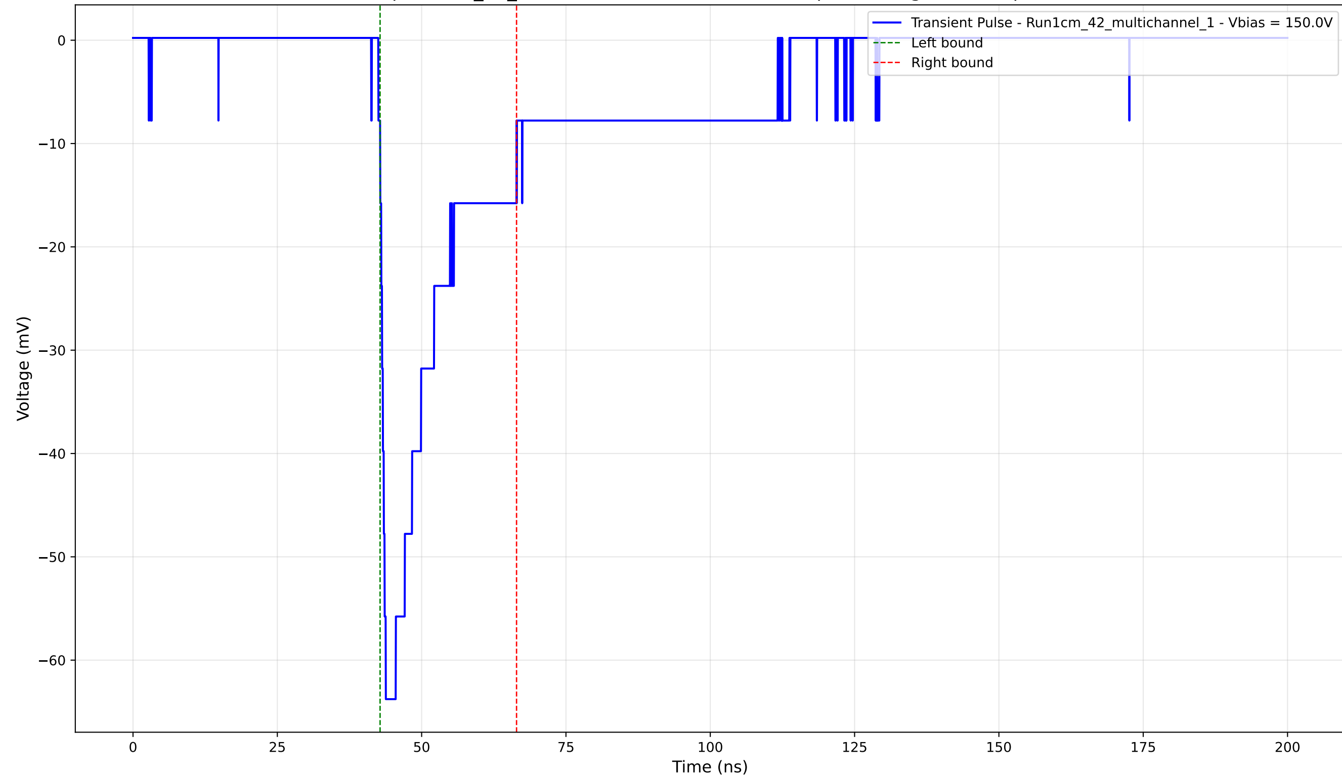
Transient Pulse - Sample: 1cm_42_multichannel - Position: 3630.0 \mu\text{m} - Charge: -13.57 pC - Rise Time: 1.28 ns
