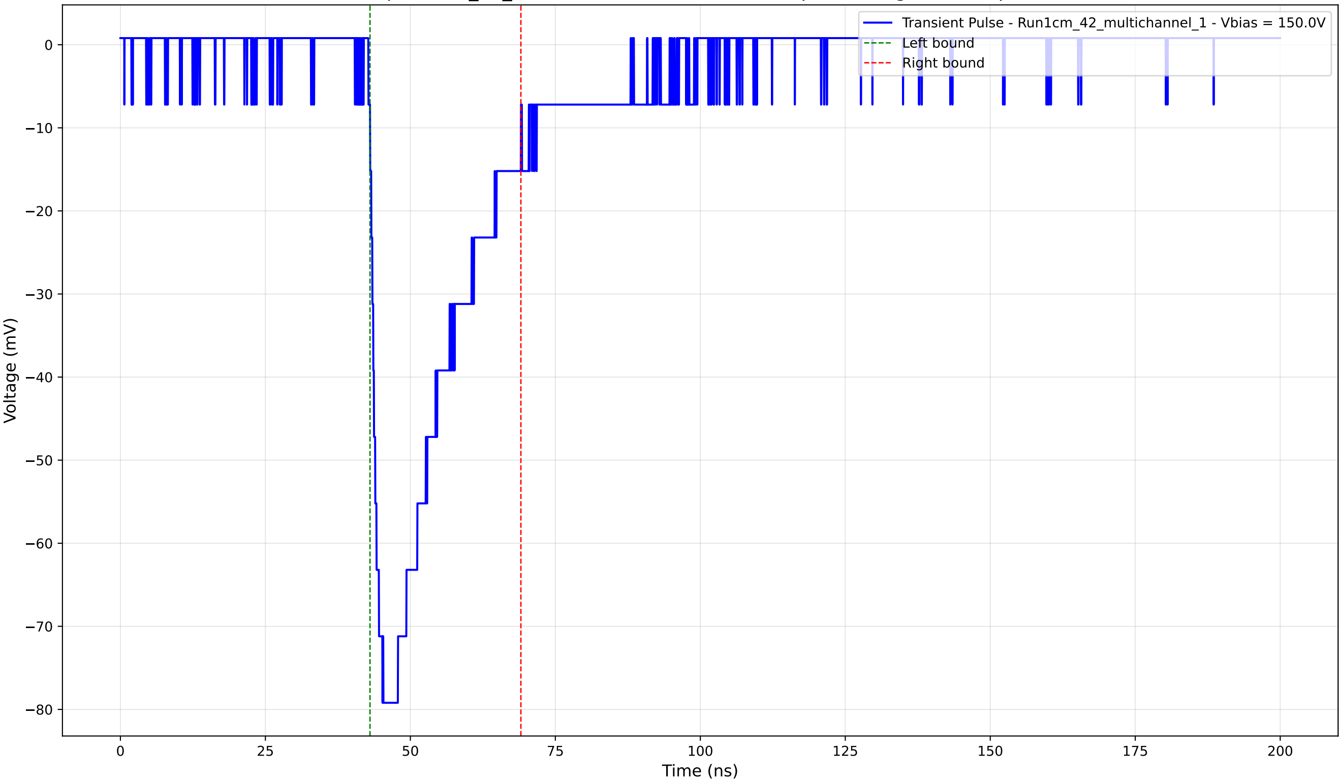
Transient Pulse - Sample: 1cm_42_multichannel - Position: 775.0 \mu\text{m} - Charge: -21.77 pC - Rise Time: 2.14 ns
