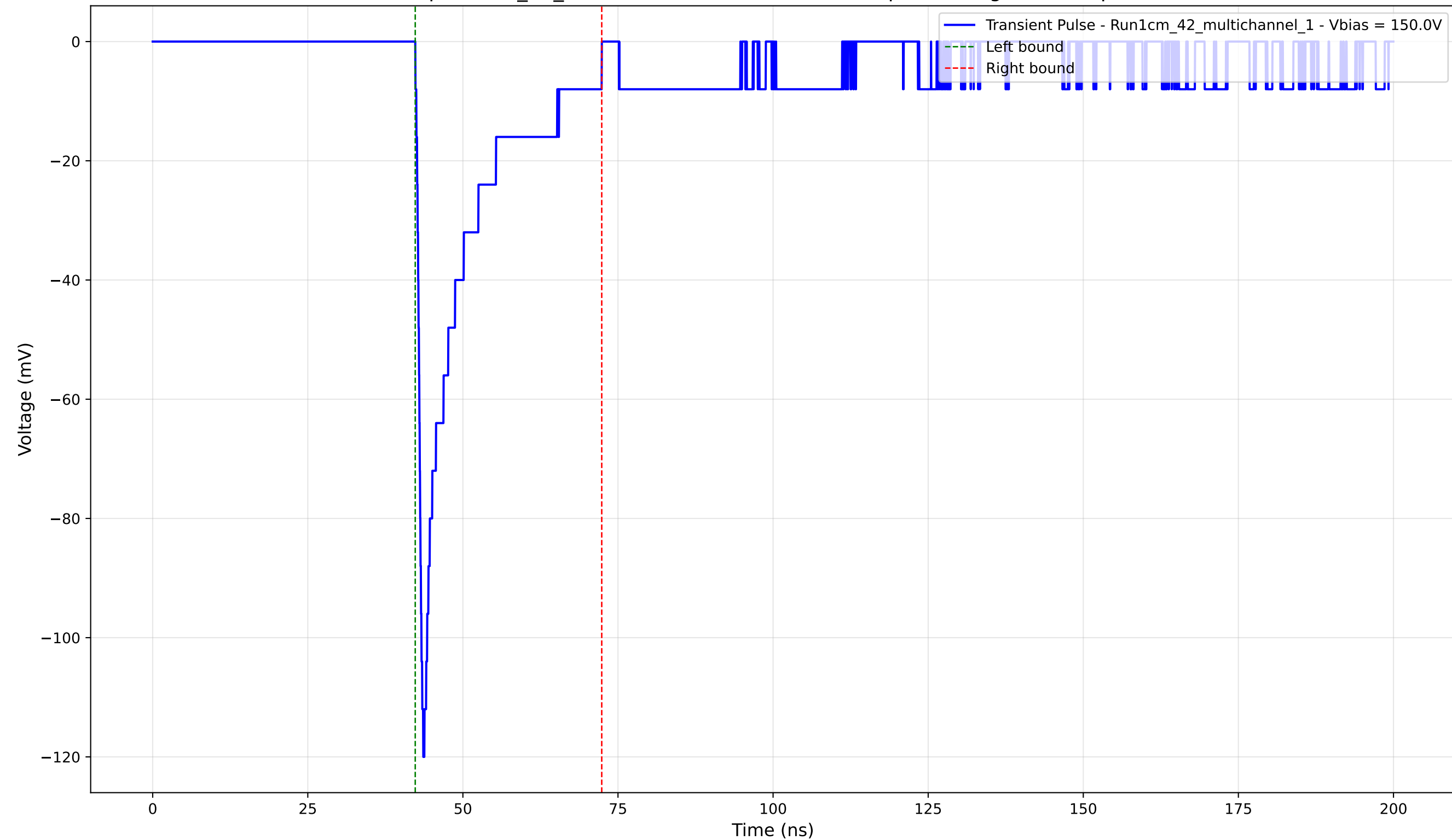
Transient Pulse - Sample: 1cm_42_multichannel - Position: 3185.0 \mu\text{m} - Charge: -17.00 pC - Rise Time: 0.95 ns
