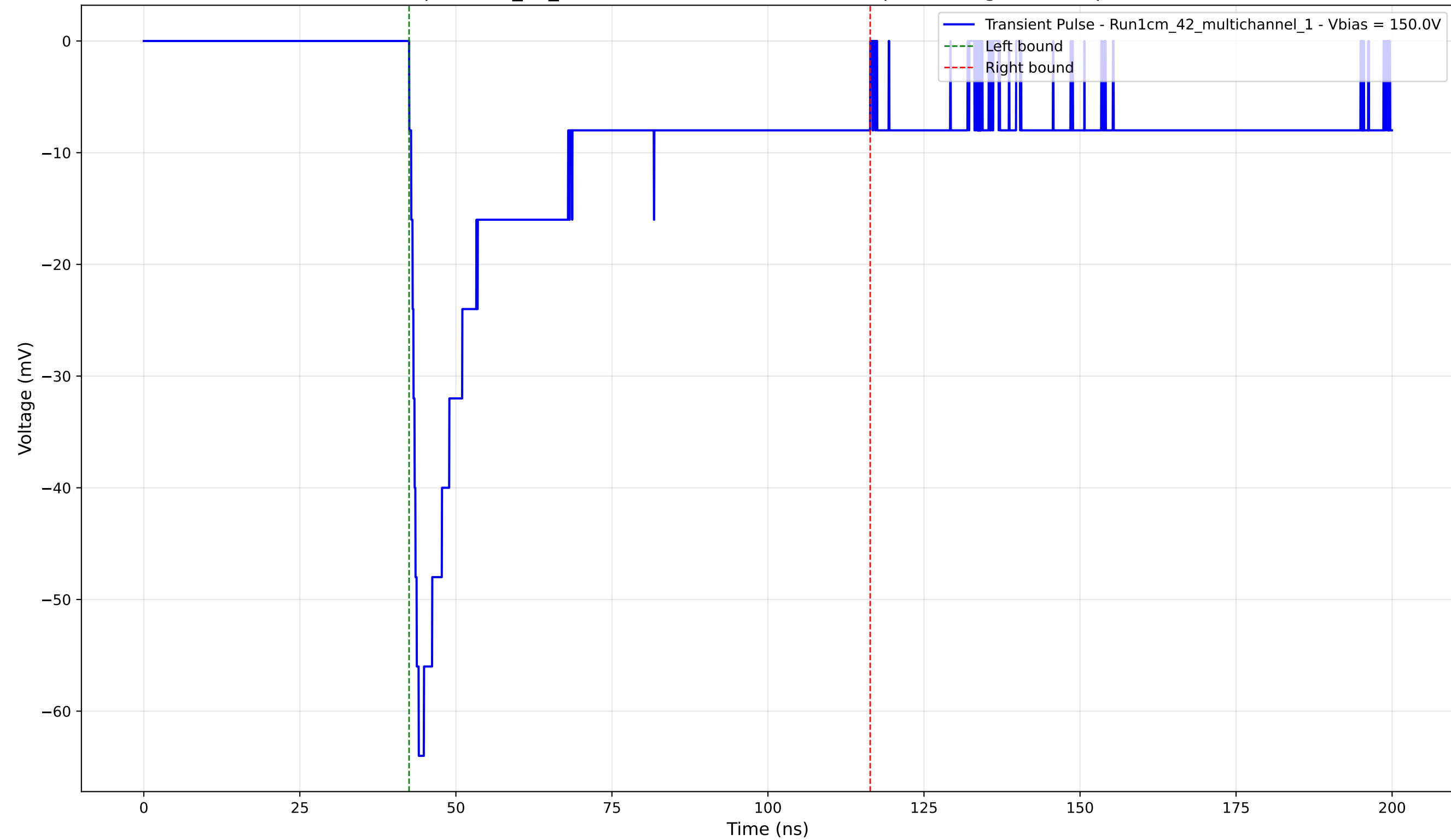
Transient Pulse - Sample: 1cm_42_multichannel - Position: 3685.0 \mu\text{m} - Charge: -20.88 pC - Rise Time: 1.52 ns
