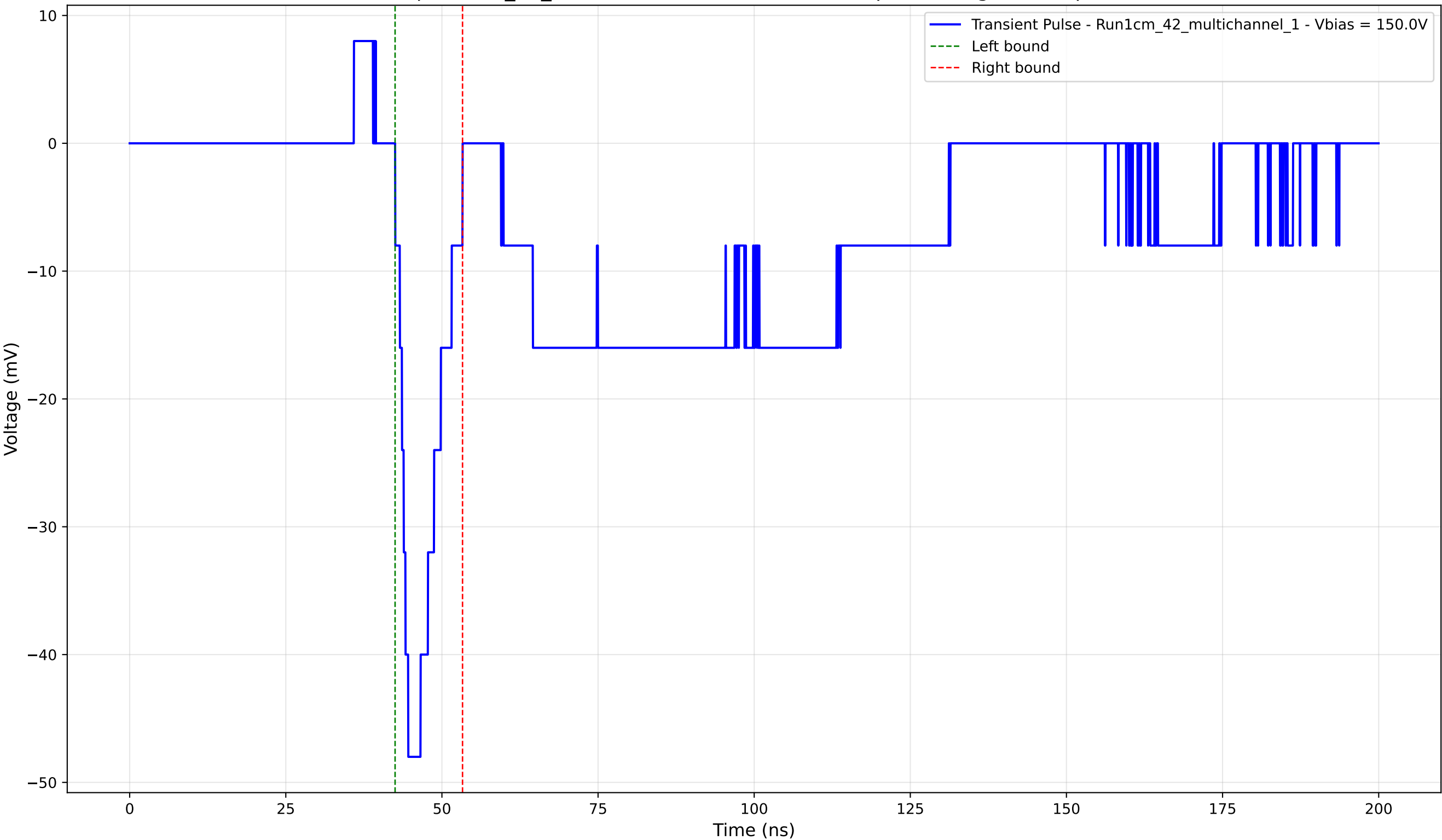
Transient Pulse - Sample: 1cm_42_multichannel - Position: 4295.0 \mu\text{m} - Charge: -5.72 pC - Rise Time: 2.09 ns
