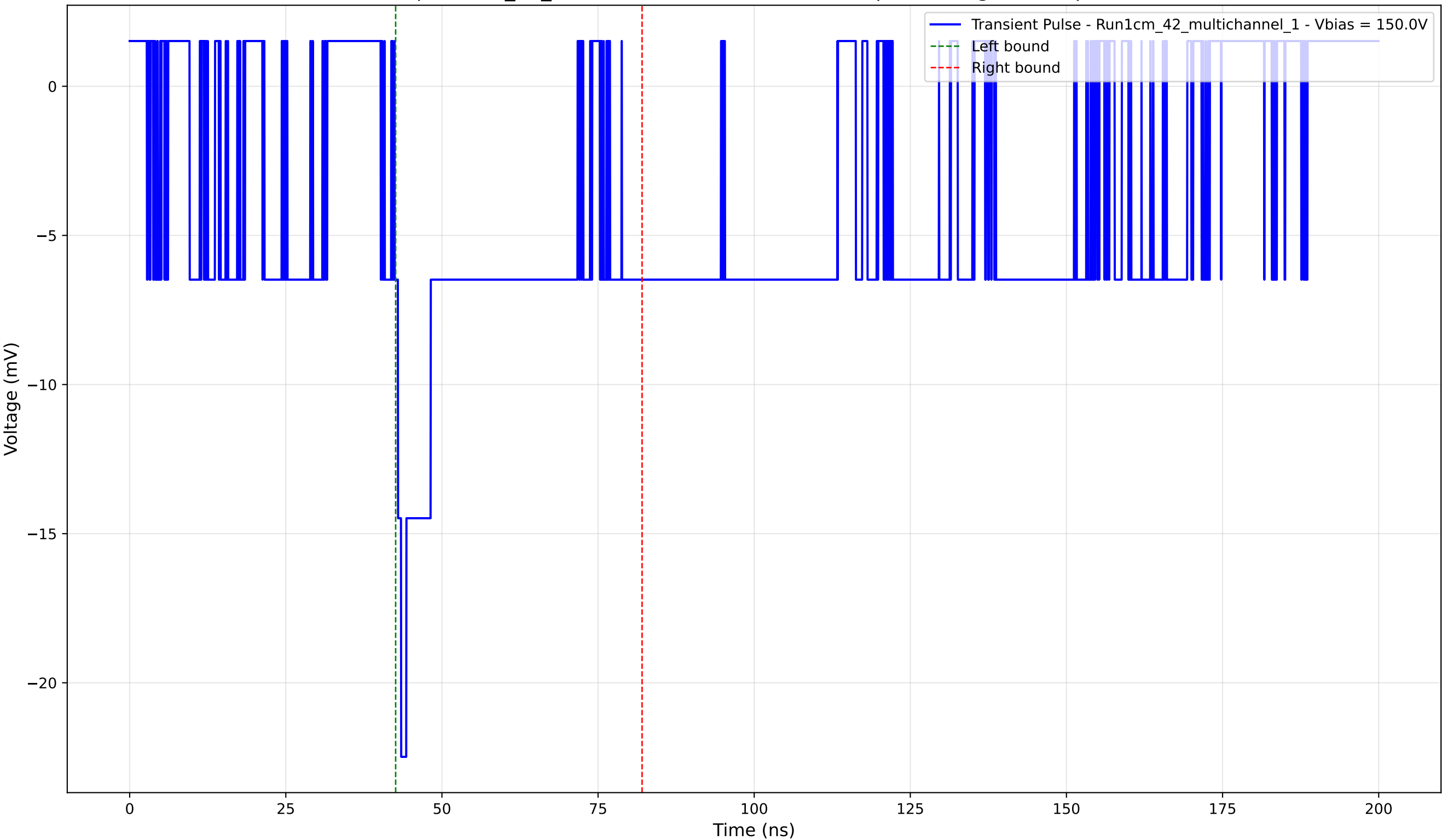
Transient Pulse - Sample: 1cm_42_multichannel - Position: 3365.0 \mu\text{m} - Charge: -5.63 pC - Rise Time: 1.06 ns
