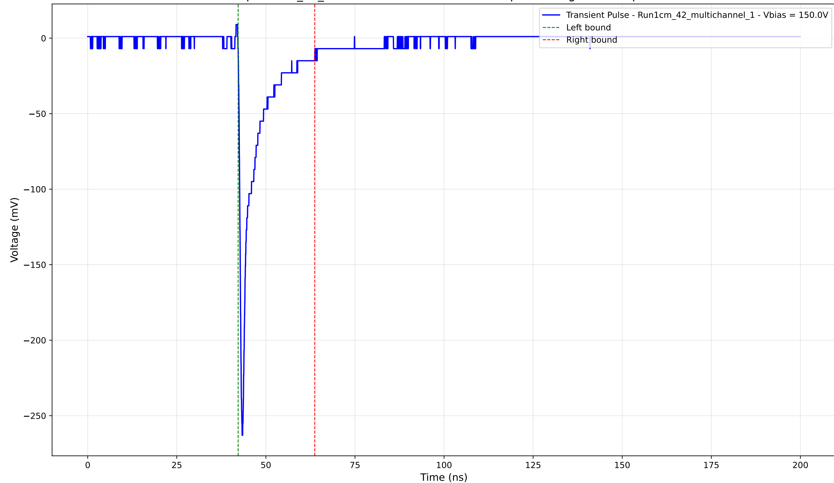
Transient Pulse - Sample: 1cm_42_multichannel - Position: 2005.0 \mu\text{m} - Charge: -23.10 pC - Rise Time: 0.79 ns
