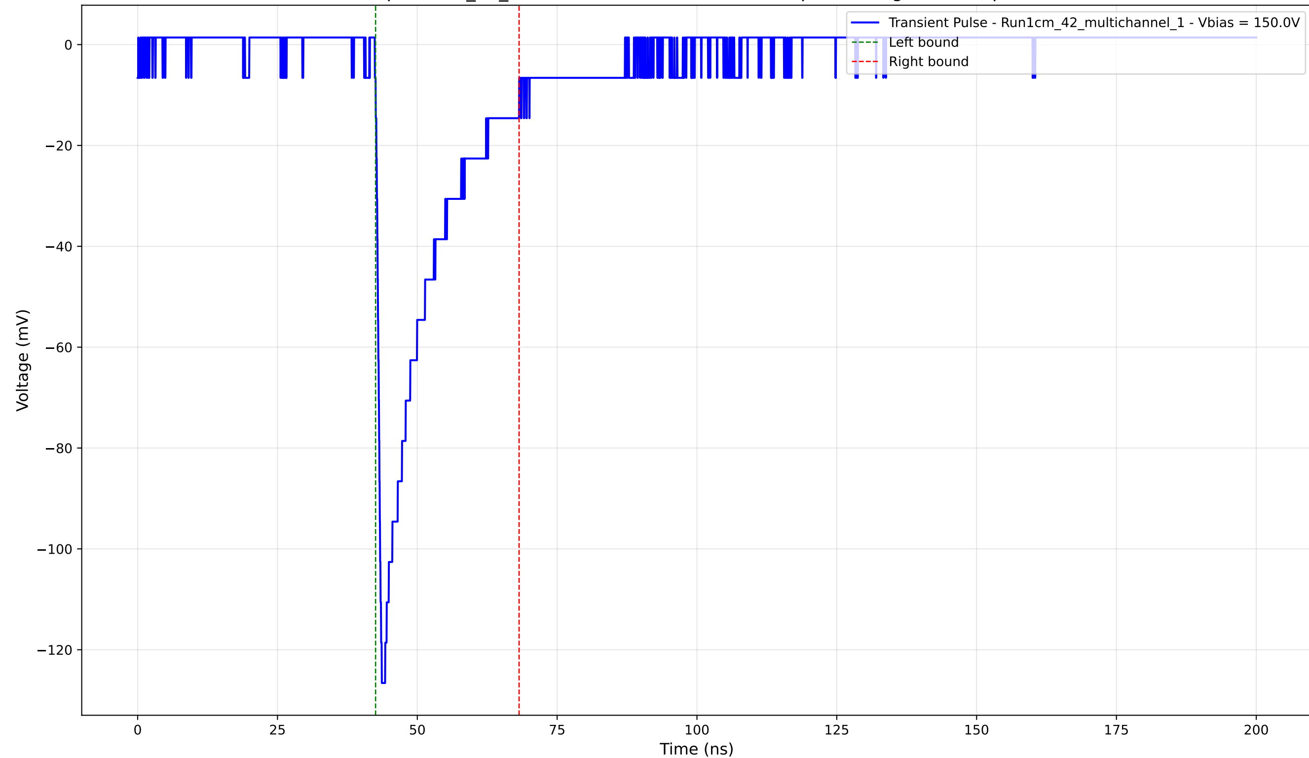
Transient Pulse - Sample: 1cm_42_multichannel - Position: 1505.0 \mu\text{m} - Charge: -22.87 pC - Rise Time: 0.96 ns
