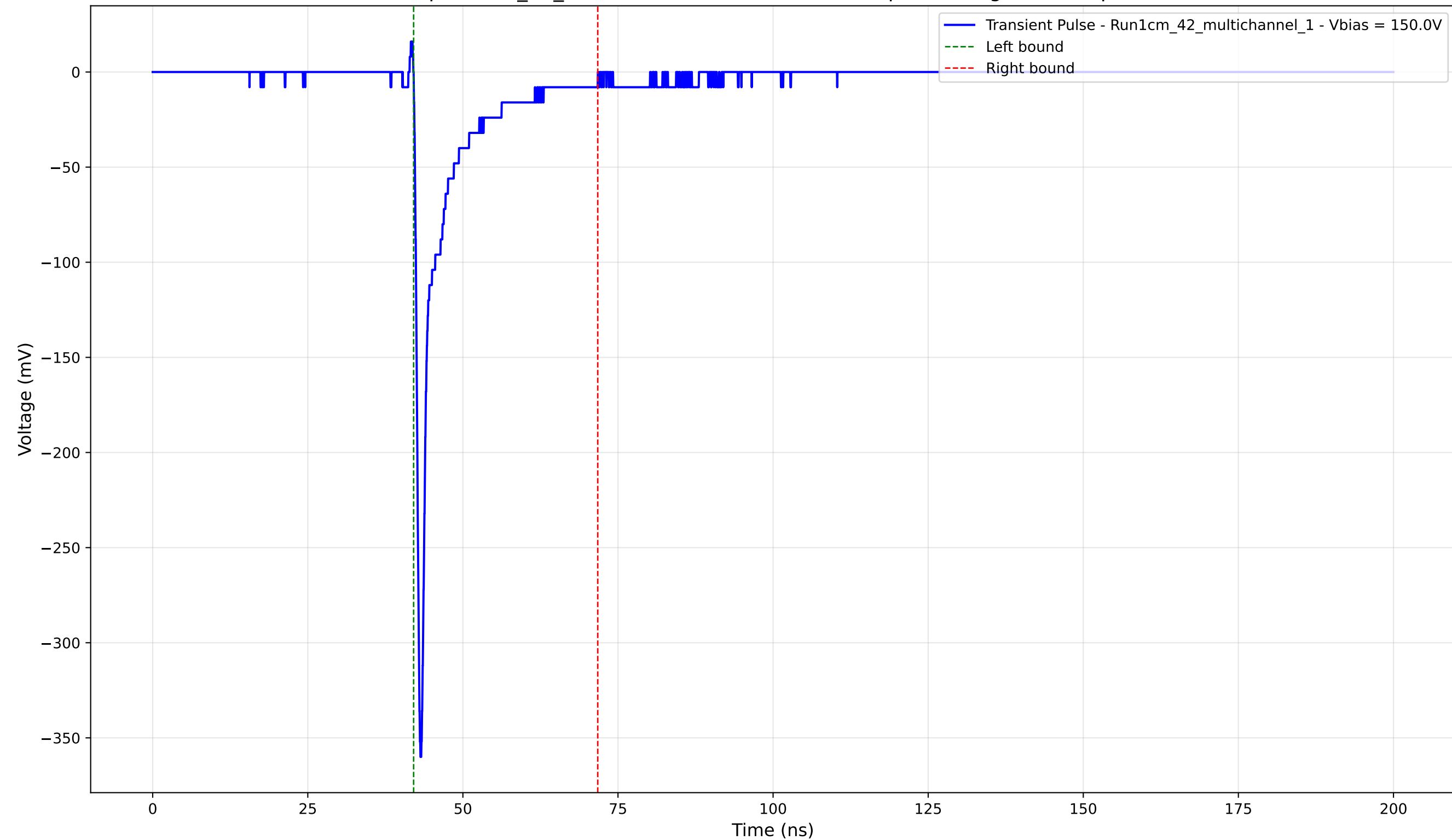
Transient Pulse - Sample: 1cm_42_multichannel - Position: 2560.0 \mu\text{m} - Charge: -25.44 pC - Rise Time: 0.74 ns
