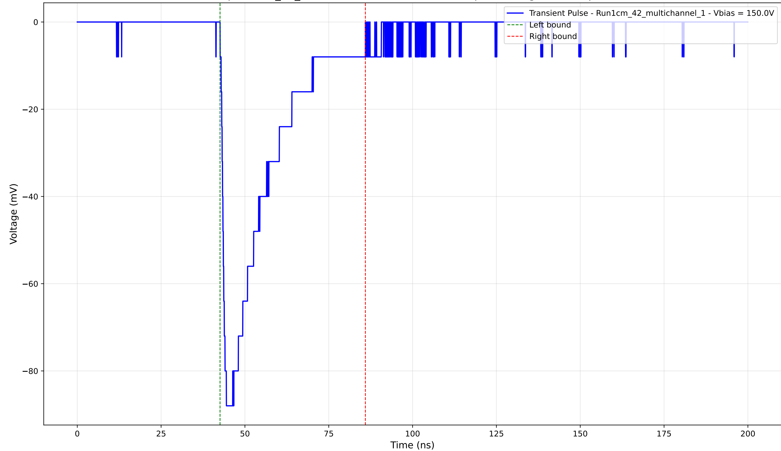
Transient Pulse - Sample: 1cm_42_multichannel - Position: 1060.0 \mu\text{m} - Charge: -25.67 pC - Rise Time: 1.18 ns
