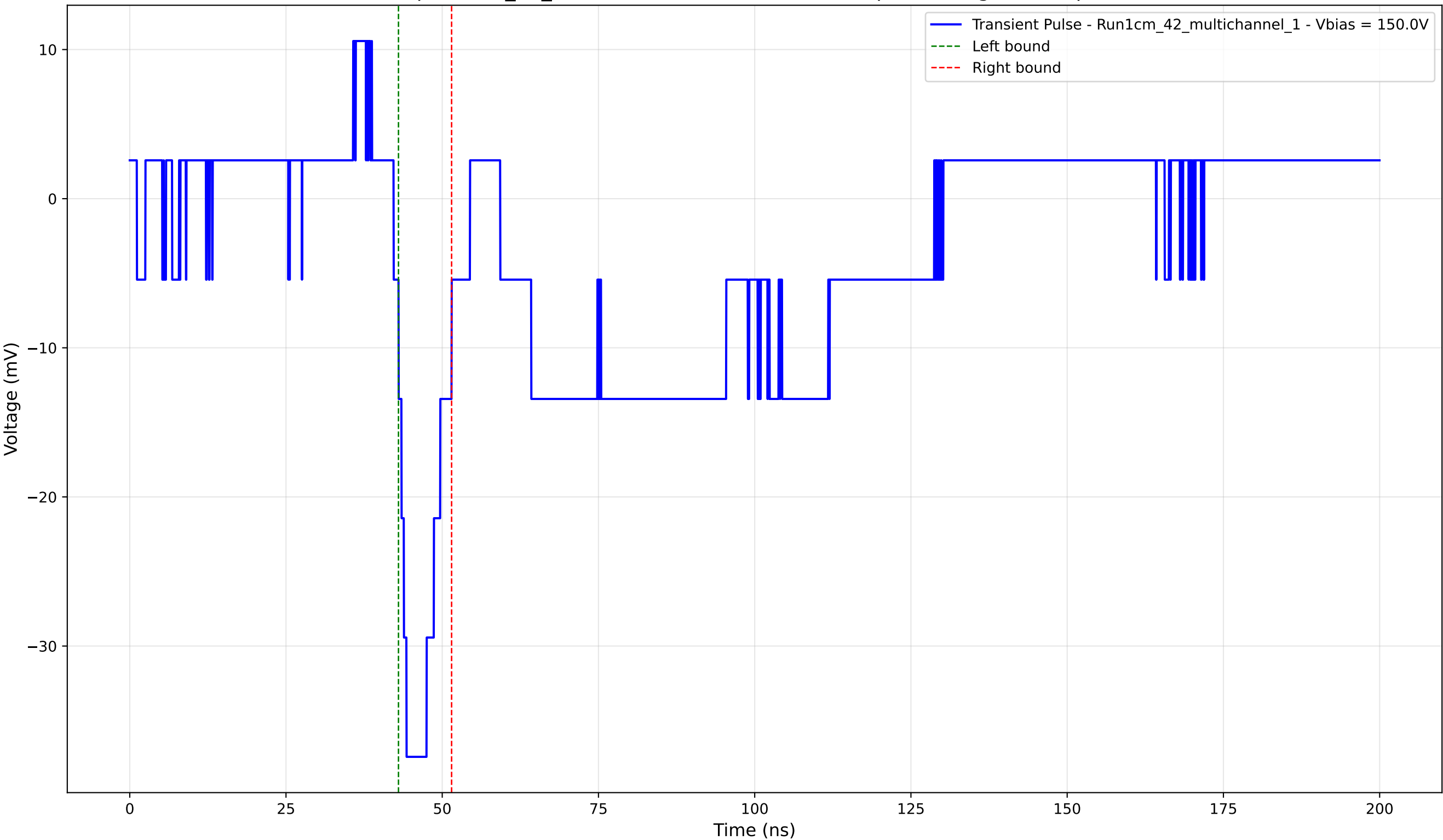
Transient Pulse - Sample: 1cm_42_multichannel - Position: 4755.0 \mu\text{m} - Charge: -4.55 pC - Rise Time: 2.07 ns
