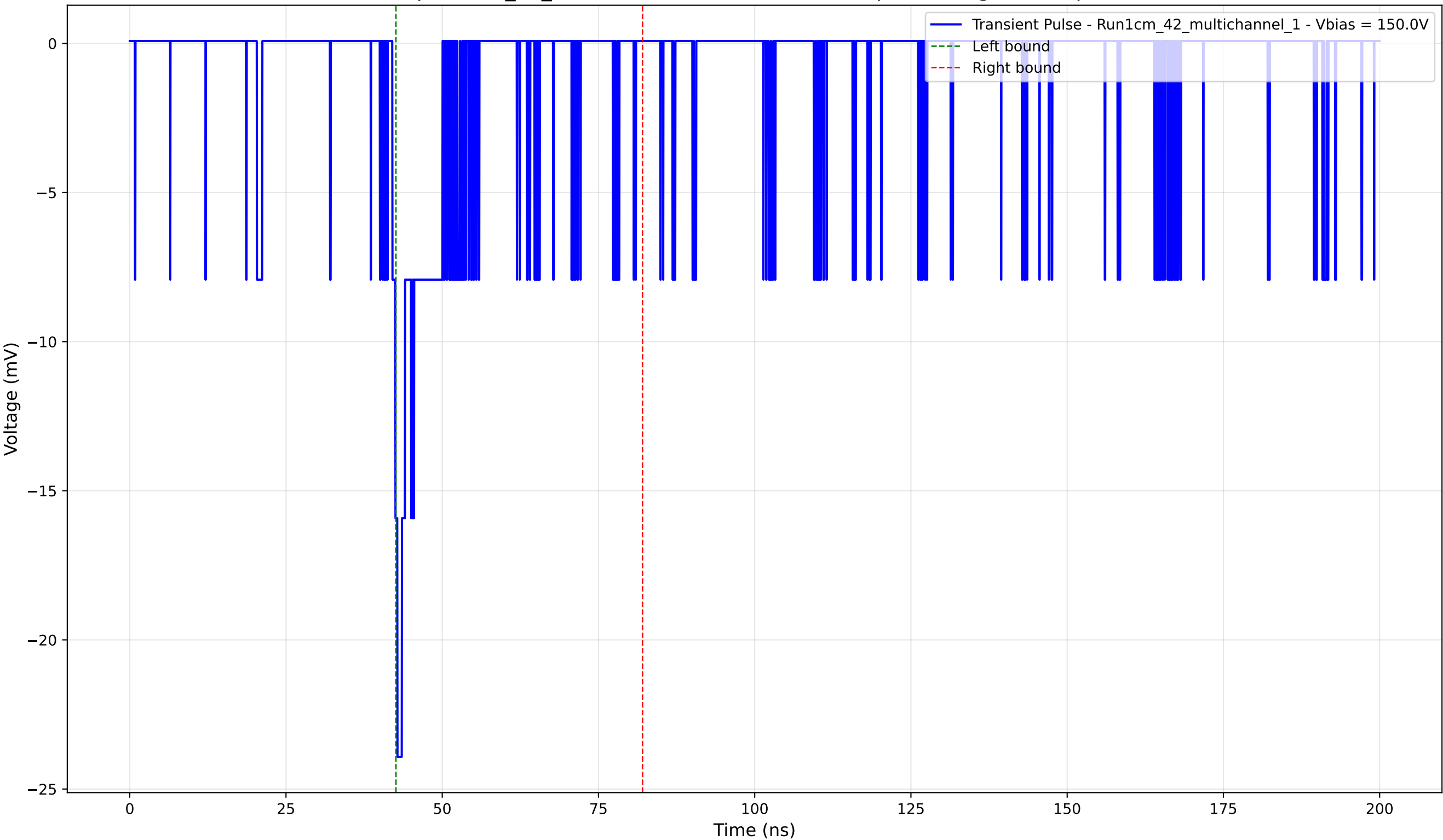
Transient Pulse - Sample: 1cm_42_multichannel - Position: 2405.0 \mu\text{m} - Charge: -2.26 pC - Rise Time: 0.81 ns
