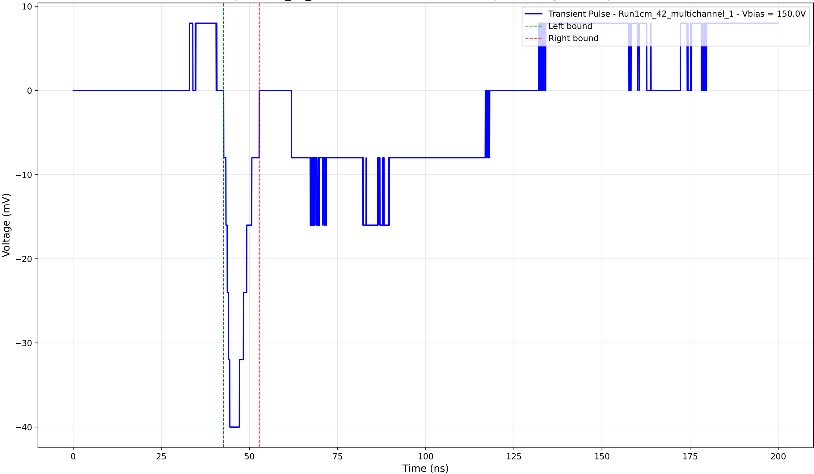
Transient Pulse - Sample: 1cm_42_multichannel - Position: 4670.0 \mu\text{m} - Charge: -4.79 pC - Rise Time: 1.73 ns
