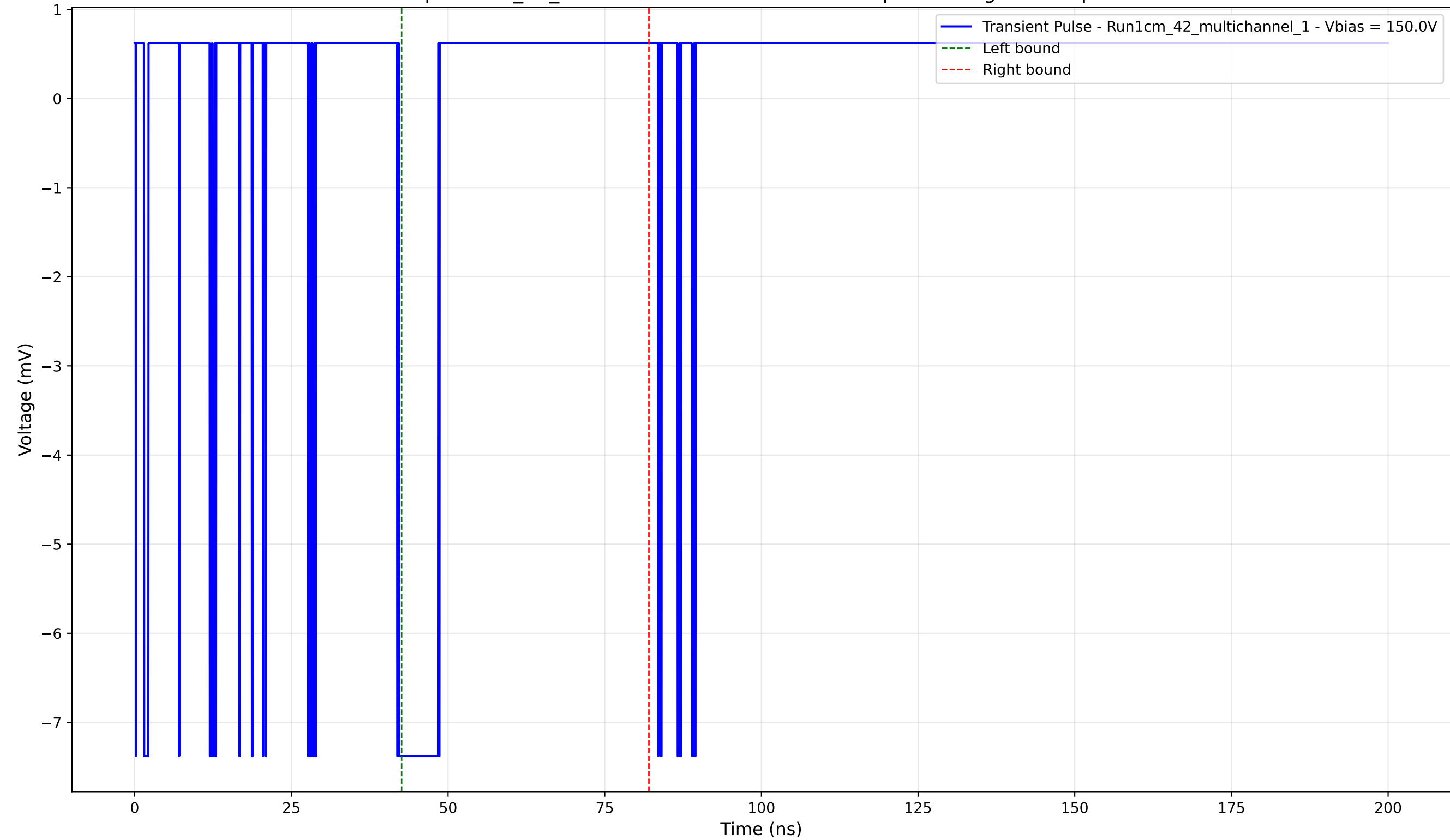
Transient Pulse - Sample: 1cm_42_multichannel - Position: 3400.0 \mu\text{m} - Charge: -0.45 pC - Rise Time: 0.02 ns
