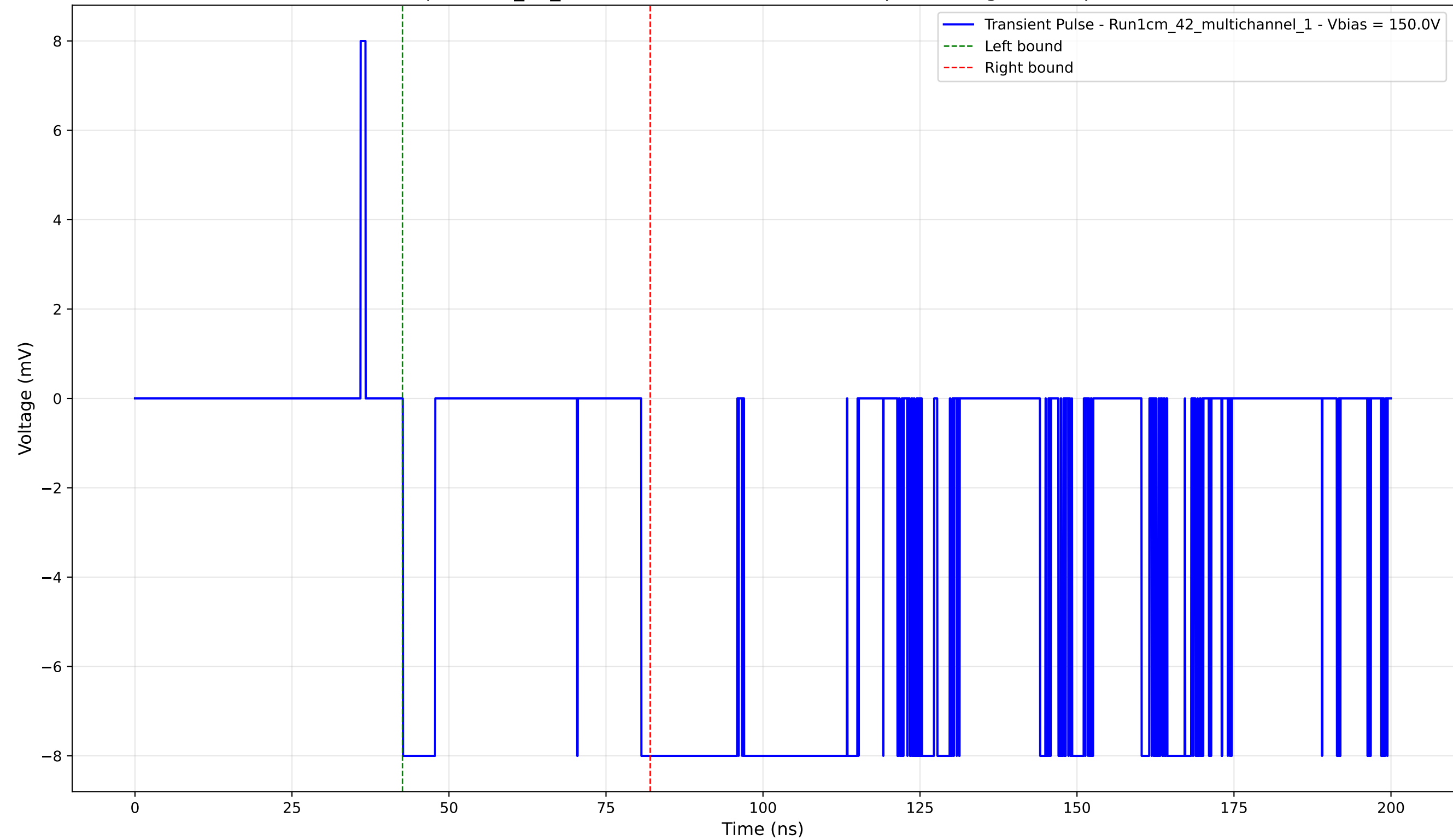
Transient Pulse - Sample: 1cm_42_multichannel - Position: 4395.0 \mu\text{m} - Charge: -1.07 pC - Rise Time: 0.02 ns
