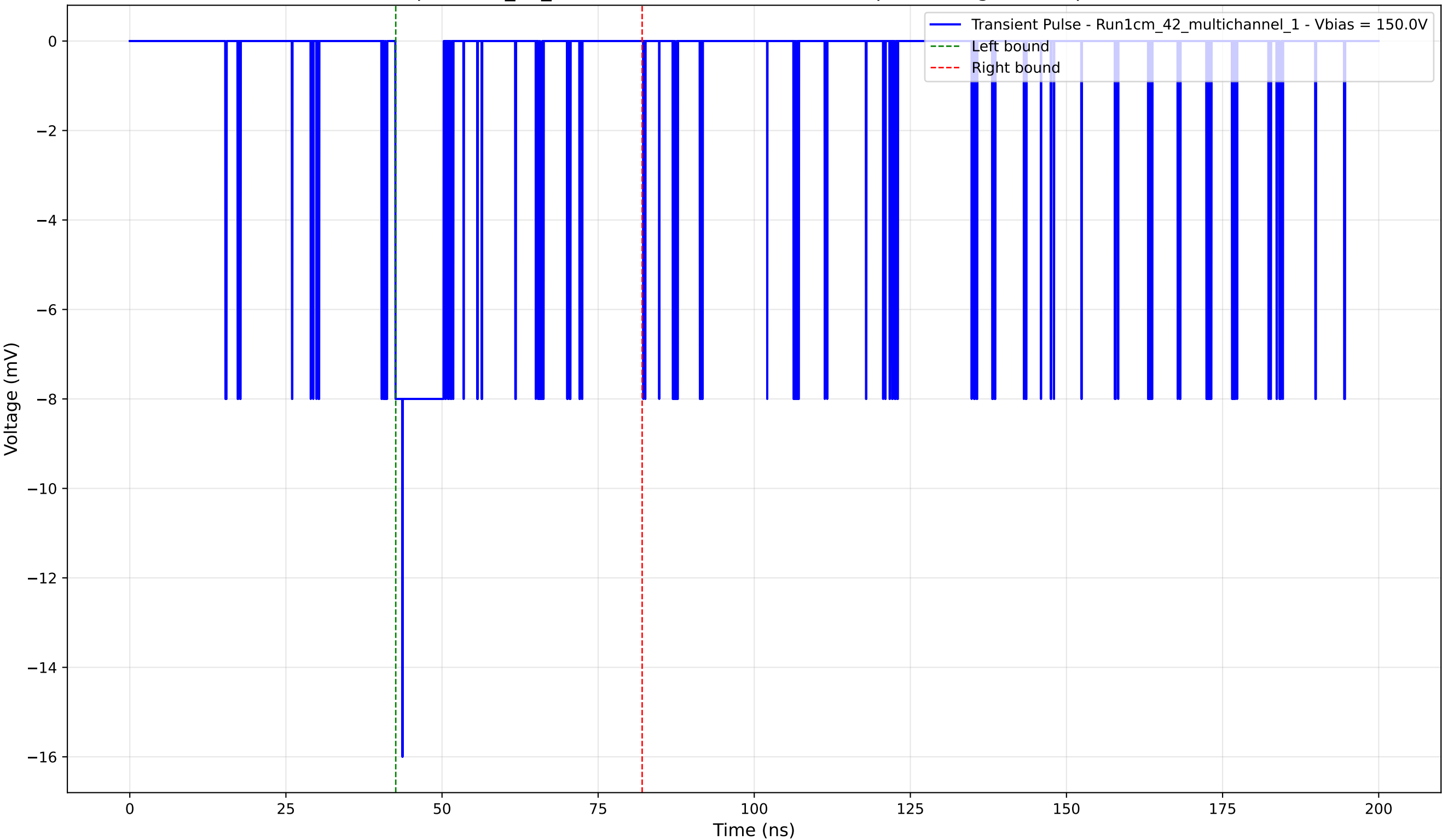
Transient Pulse - Sample: 1cm_42_multichannel - Position: 1885.0 \mu\text{m} - Charge: -1.53 pC - Rise Time: 1.12 ns
