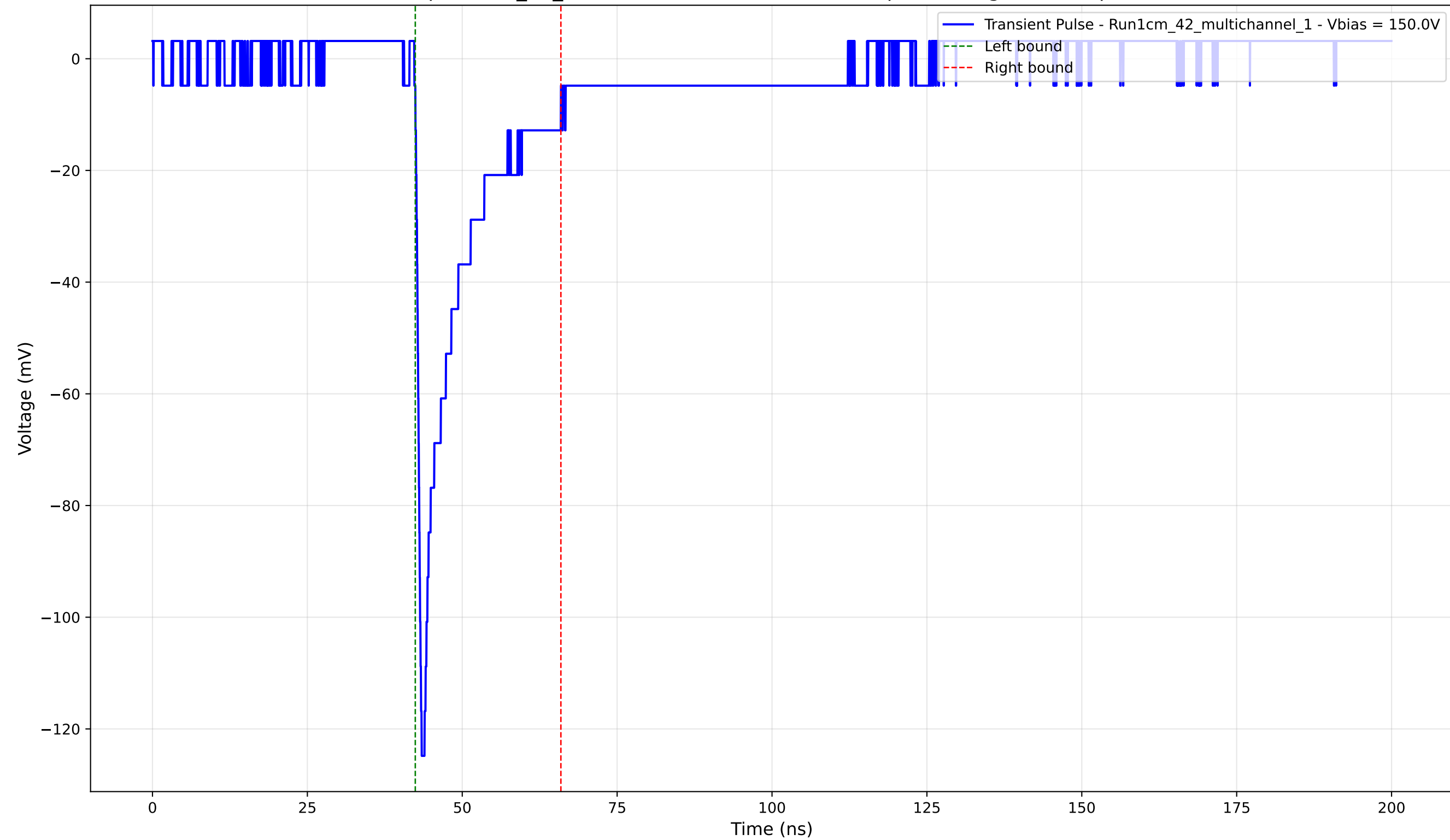
Transient Pulse - Sample: 1cm_42_multichannel - Position: 3130.0 \mu\text{m} - Charge: -16.42 pC - Rise Time: 0.90 ns
