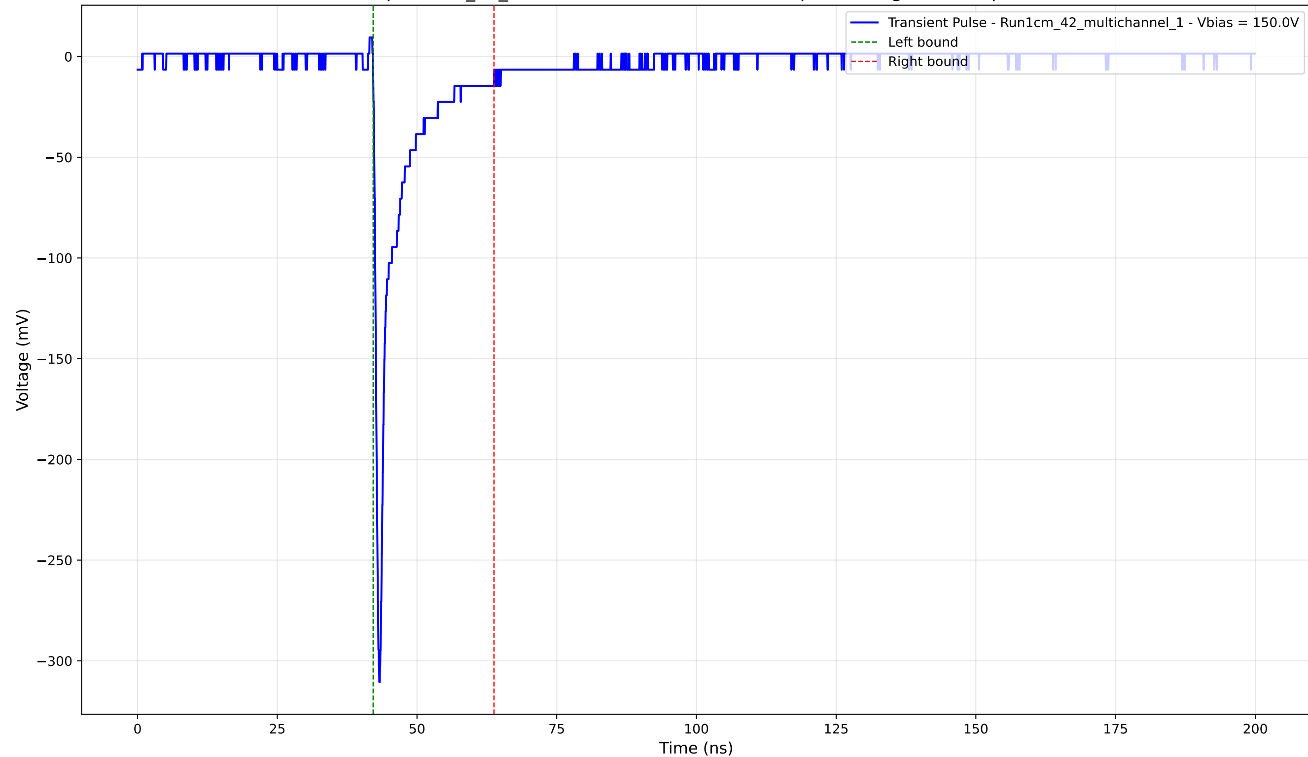
Transient Pulse - Sample: 1cm_42_multichannel - Position: 2645.0 \mu\text{m} - Charge: -22.88 pC - Rise Time: 0.78 ns
