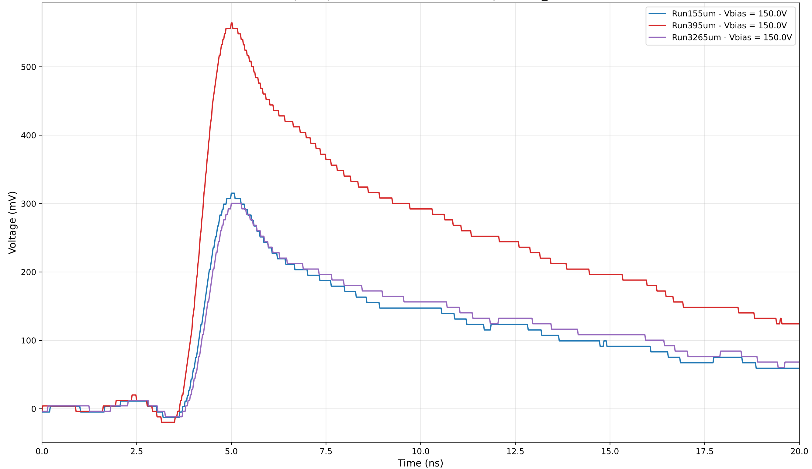
Superimposed Transient Pulses - Sample: 1cm_42
