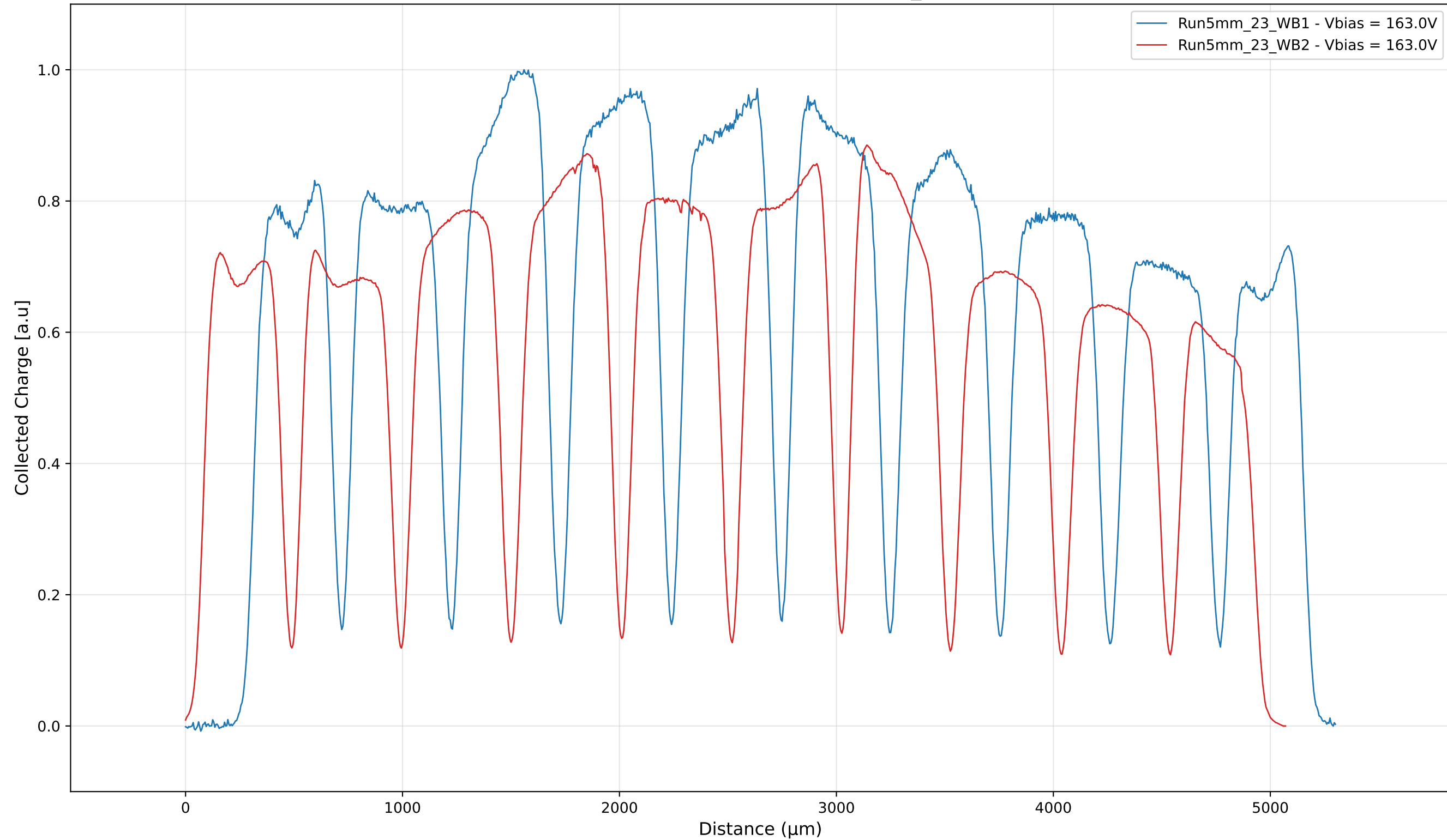
Collected Charge - Sample: 5mm_23
