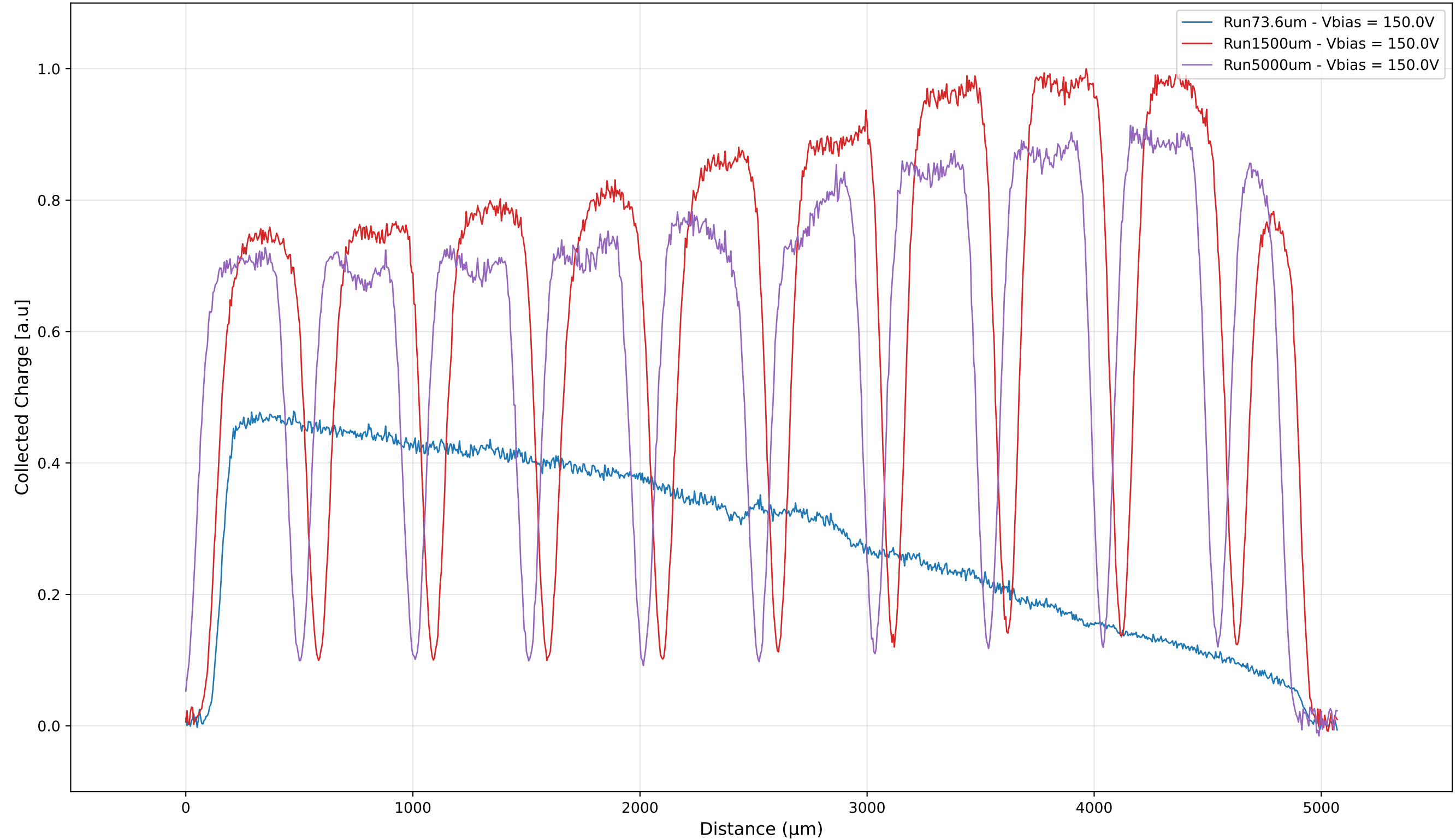
Collected Charge - Sample: 1cm_42
