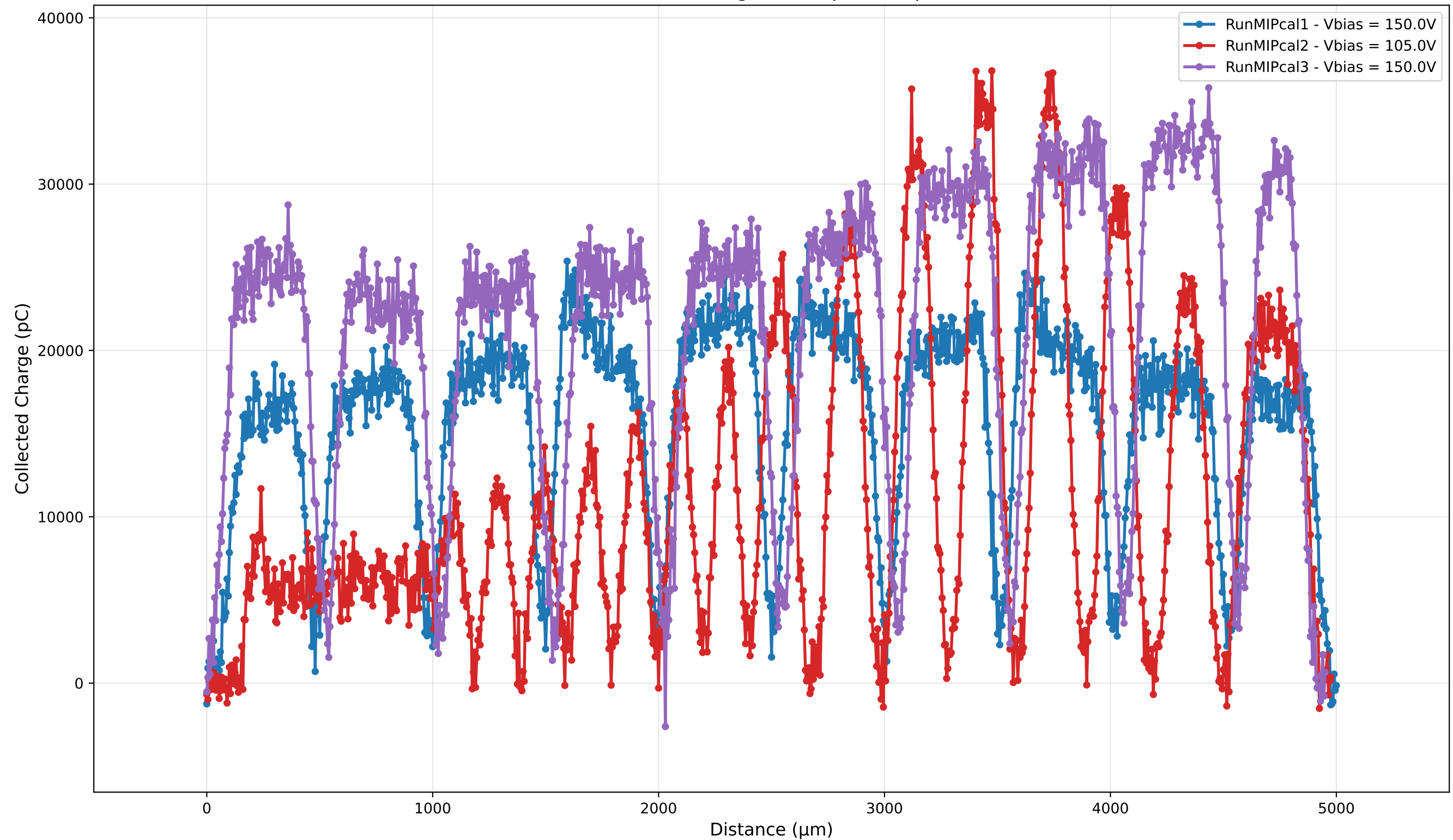
Collected Charge - Multiple Samples
