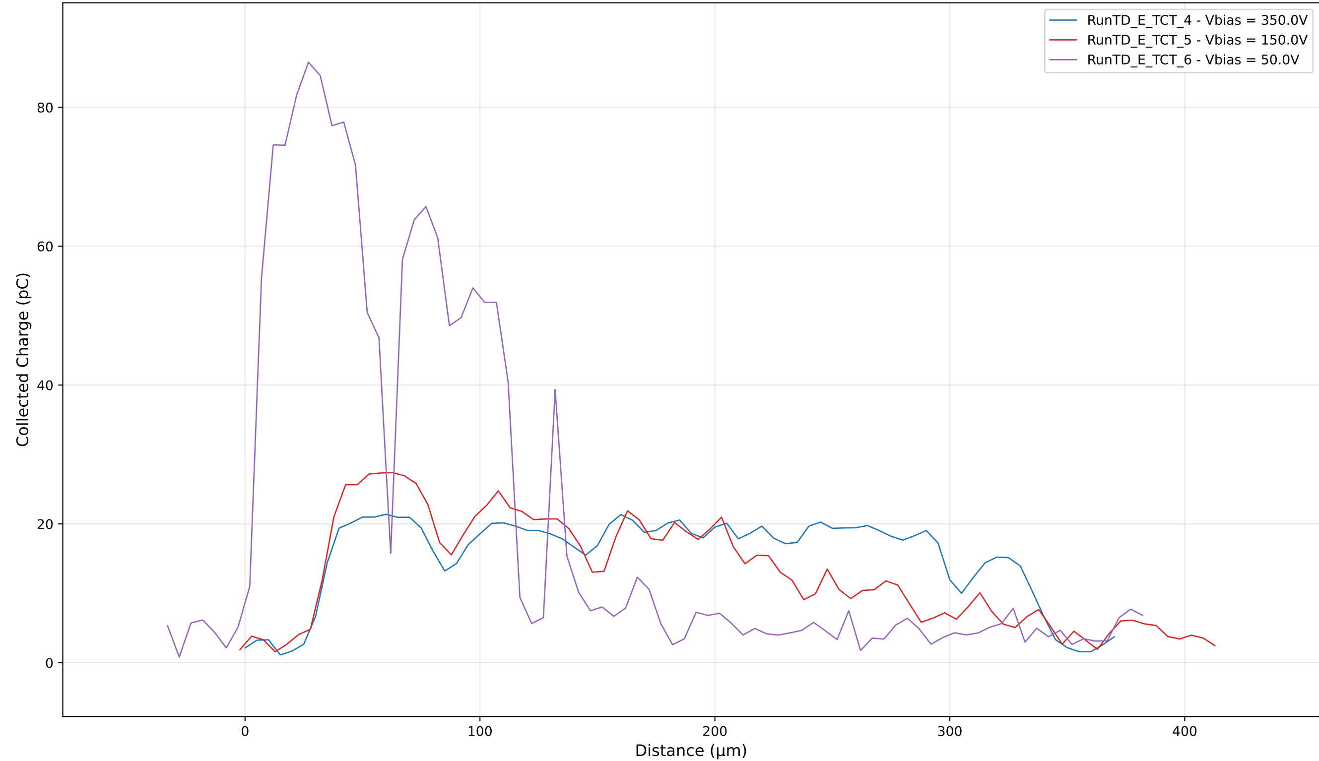
Collected Charge - Sample: TD
