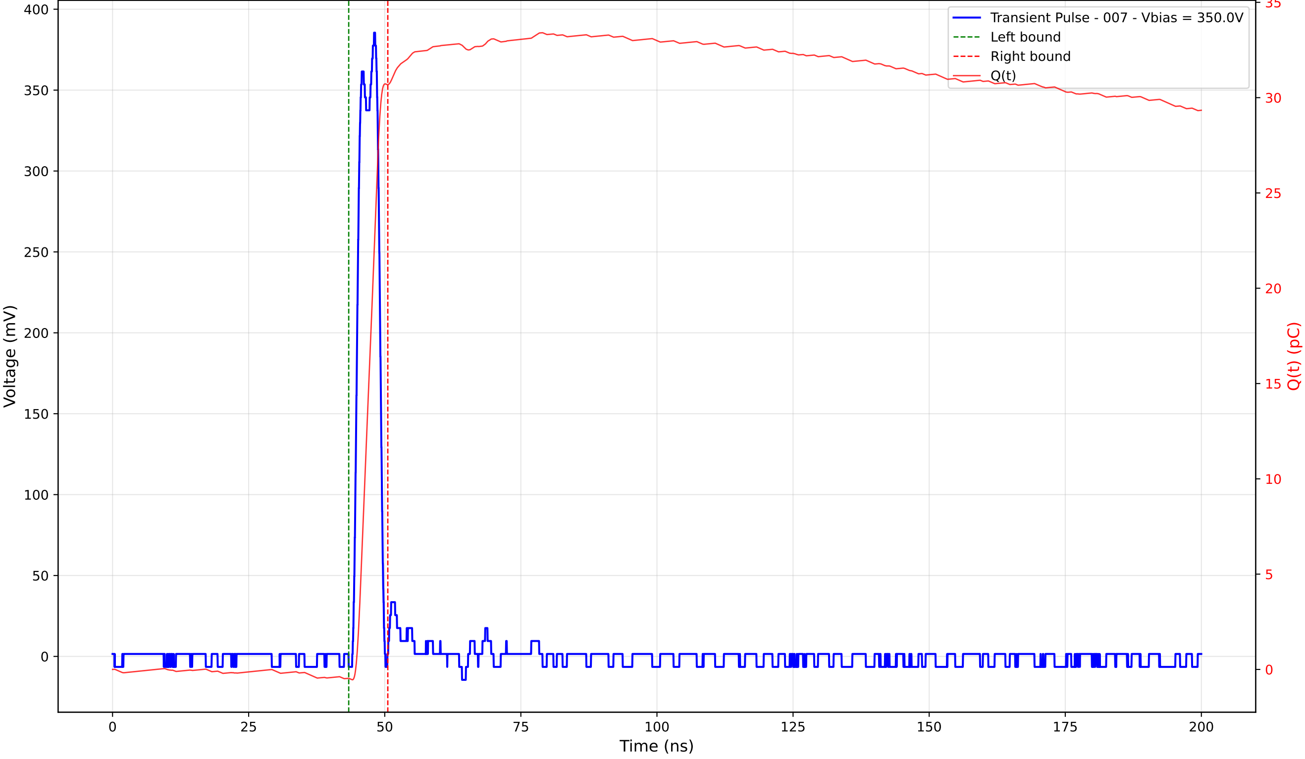
Transient Pulse - Sample: 4003 - Position: 370.0 \mu\text{m} - Charge: 31.14 pC - Rise Time: 1.29 ns
