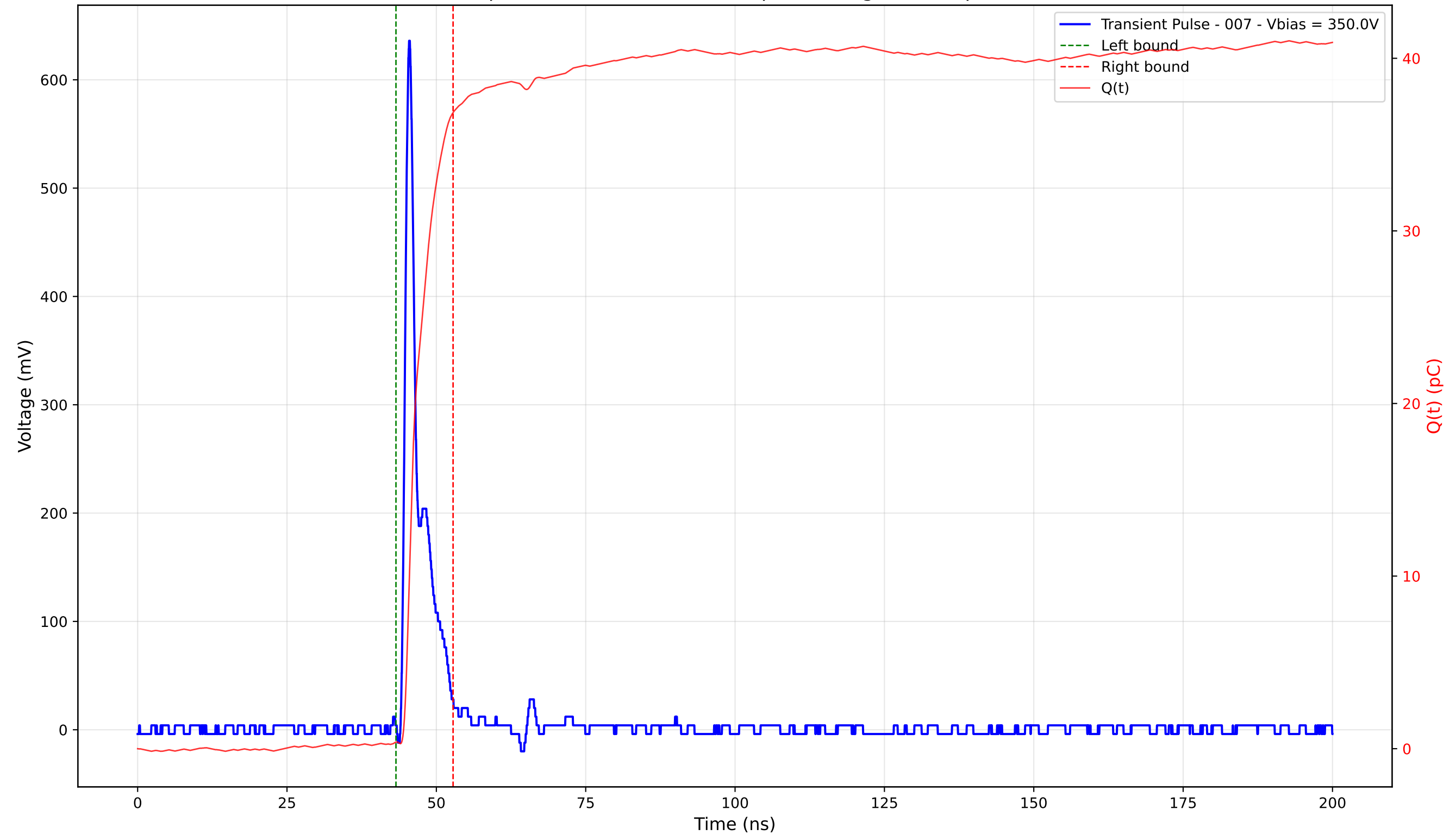
Transient Pulse - Sample: 4003 - Position: 140.0 \mu\text{m} - Charge: 36.48 pC - Rise Time: 0.91 ns
