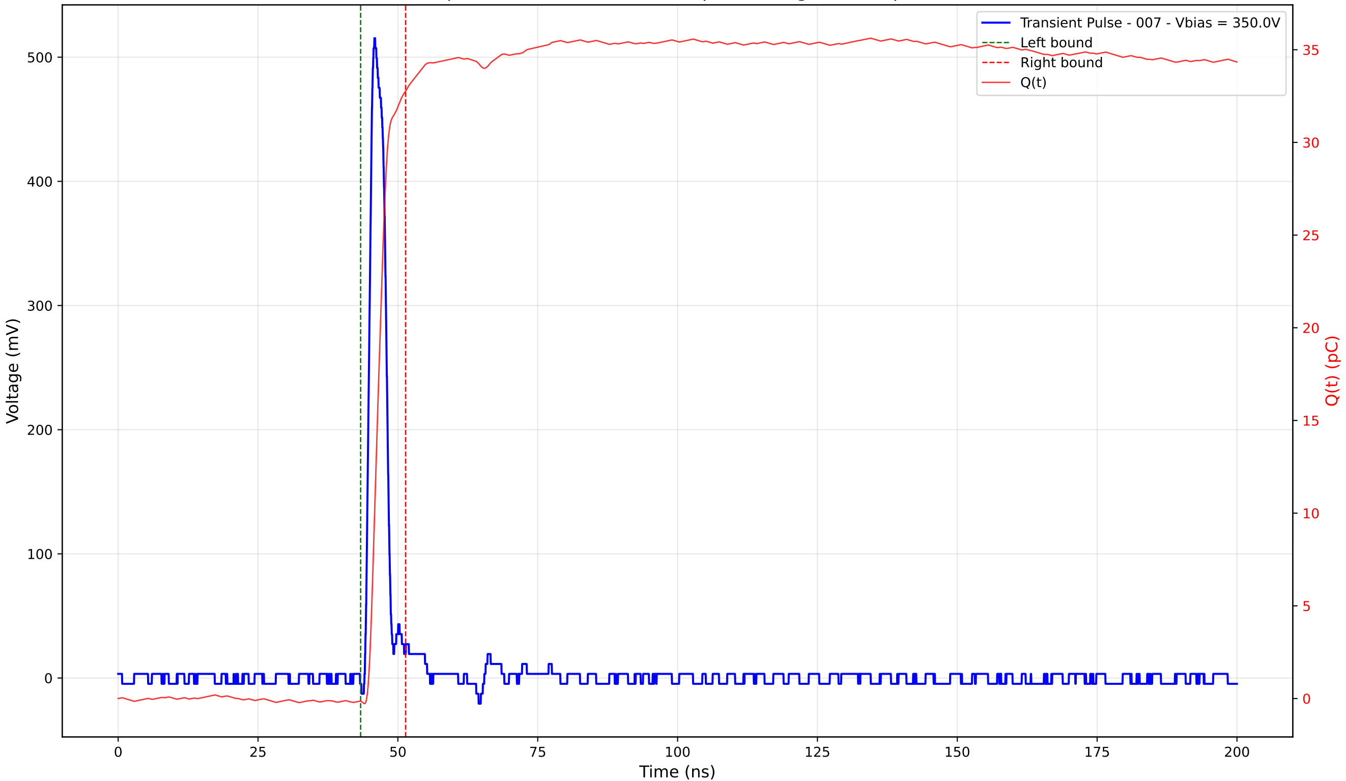
Transient Pulse - Sample: 4003 - Position: 300.0 \mu\text{m} - Charge: 32.91 pC - Rise Time: 1.10 ns
