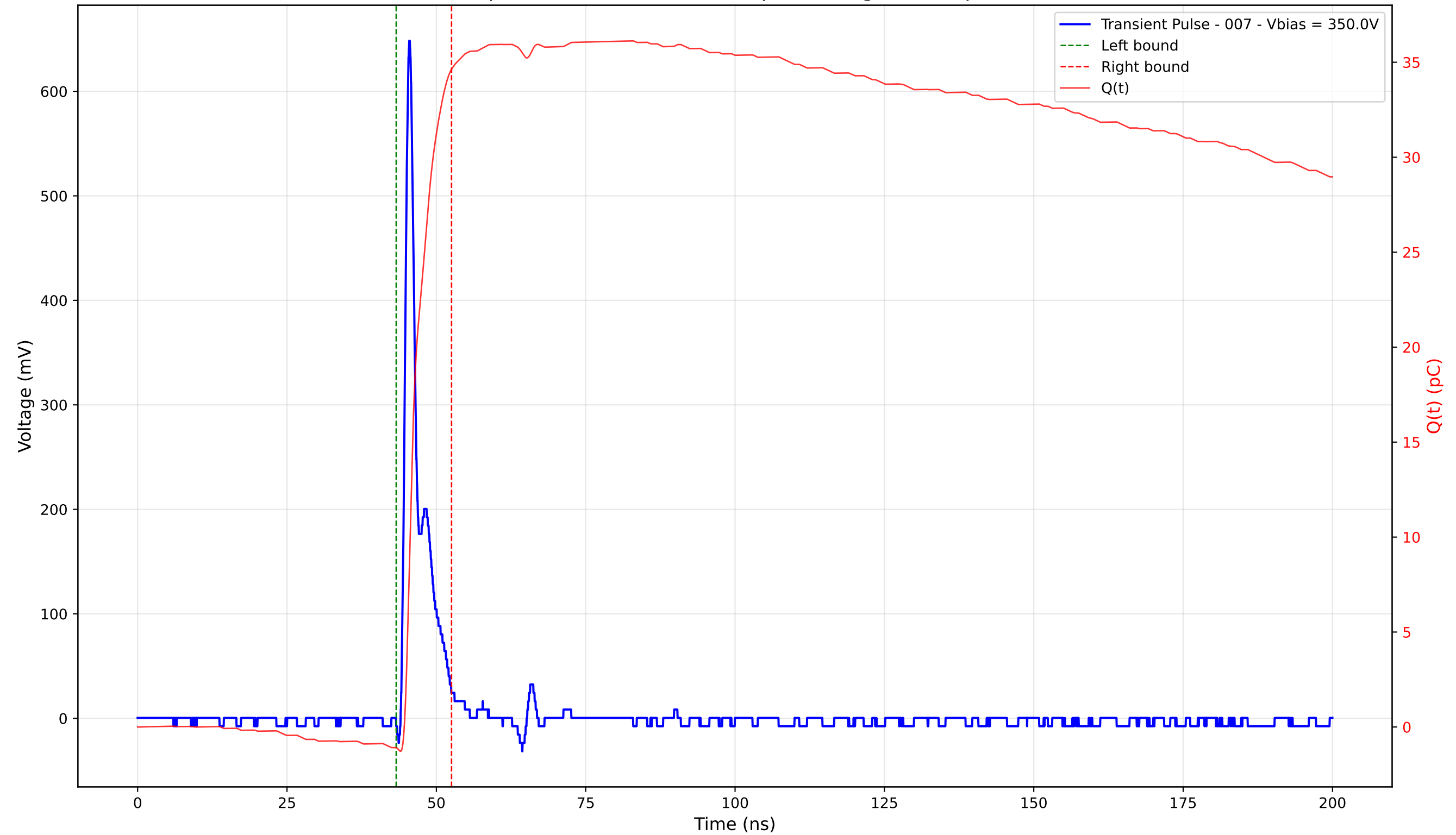
Transient Pulse - Sample: 4003 - Position: 150.0 \mu\text{m} - Charge: 35.71 pC - Rise Time: 0.92 ns
