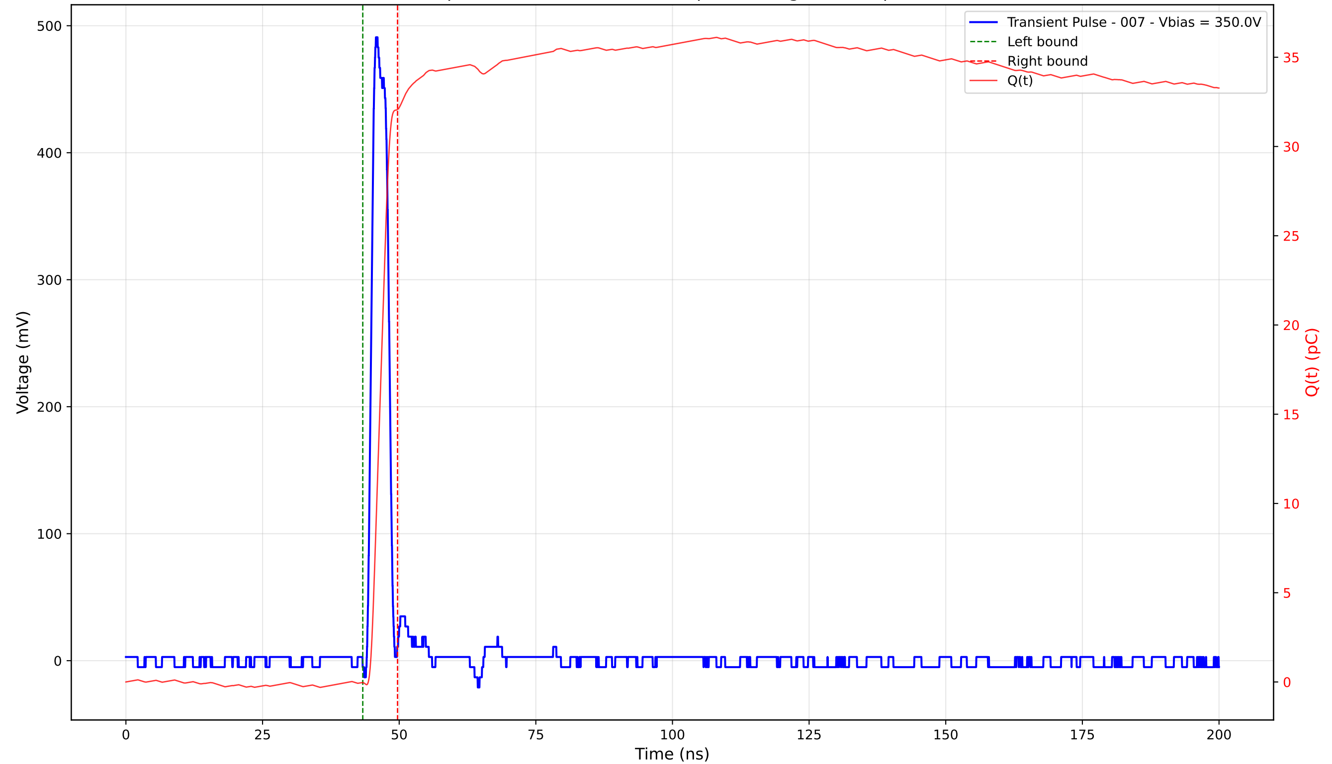
Transient Pulse - Sample: 4003 - Position: 315.0 \mu\text{m} - Charge: 32.10 pC - Rise Time: 1.06 ns
