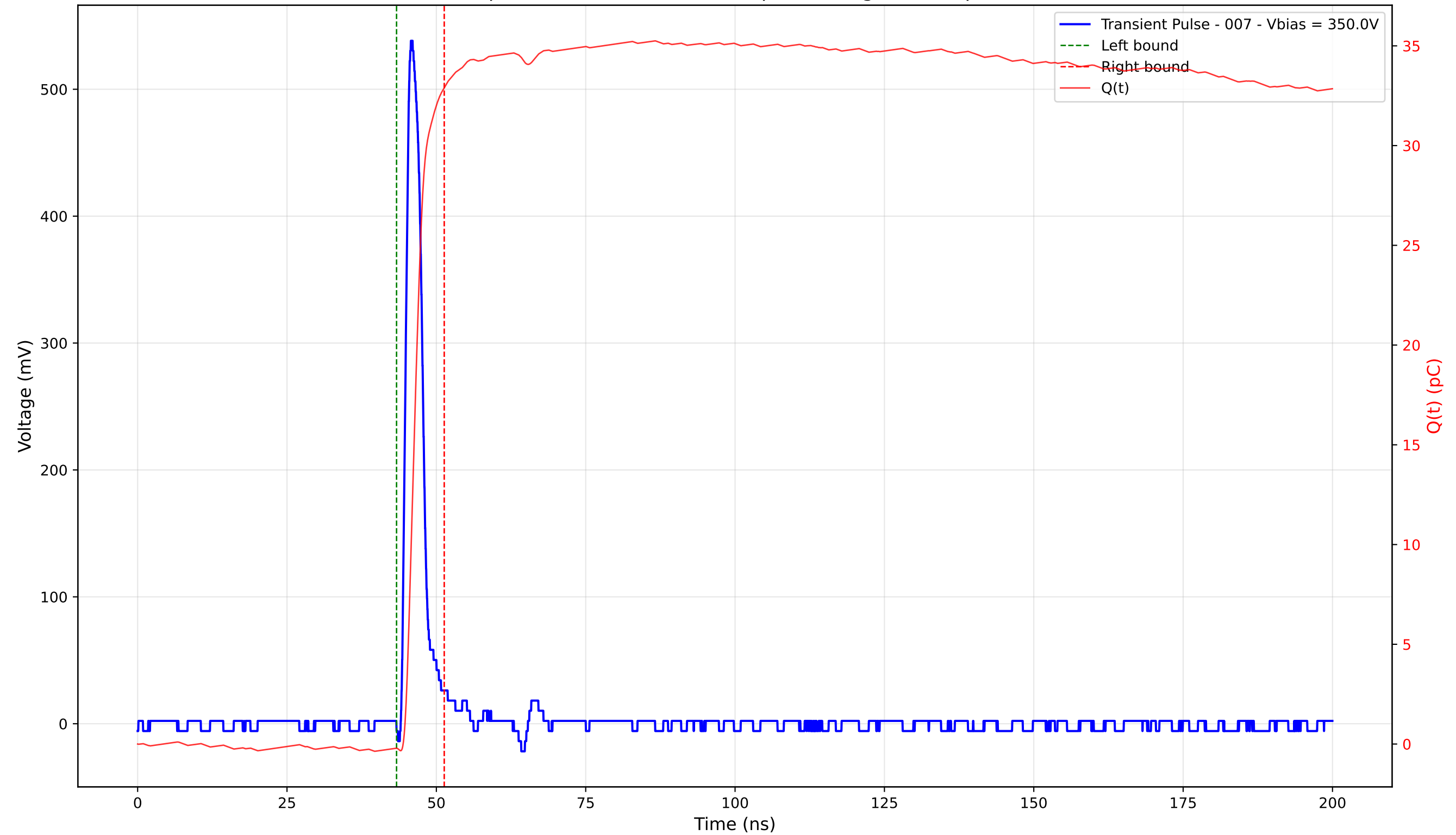
Transient Pulse - Sample: 4003 - Position: 280.0 \mu\text{m} - Charge: 33.11 pC - Rise Time: 1.07 ns
