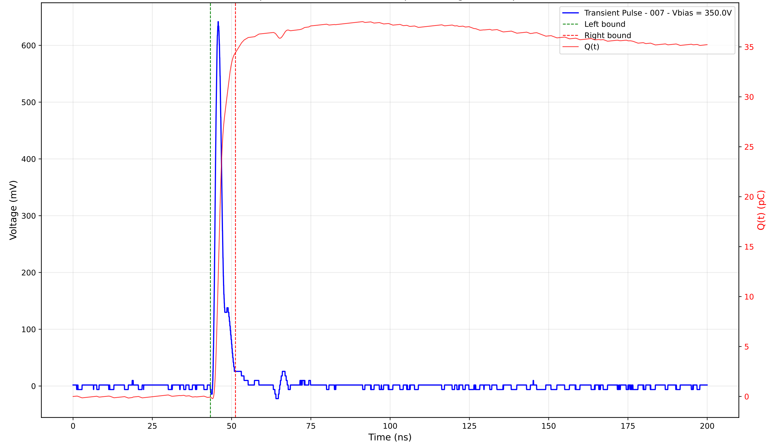
Transient Pulse - Sample: 4003 - Position: 225.0 \mu\text{m} - Charge: 34.50 pC - Rise Time: 1.08 ns
