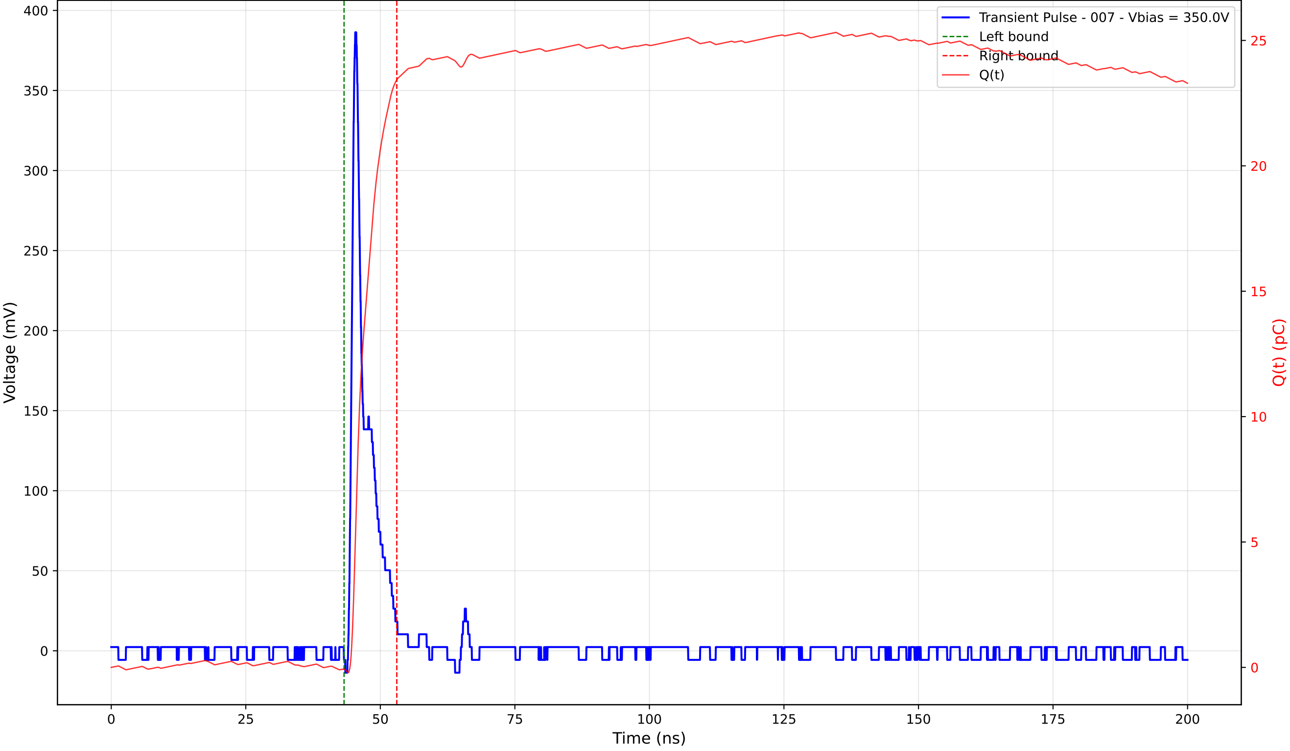
Transient Pulse - Sample: 4003 - Position: 100.0 \mu\text{m} - Charge: 23.50 pC - Rise Time: 0.89 ns
