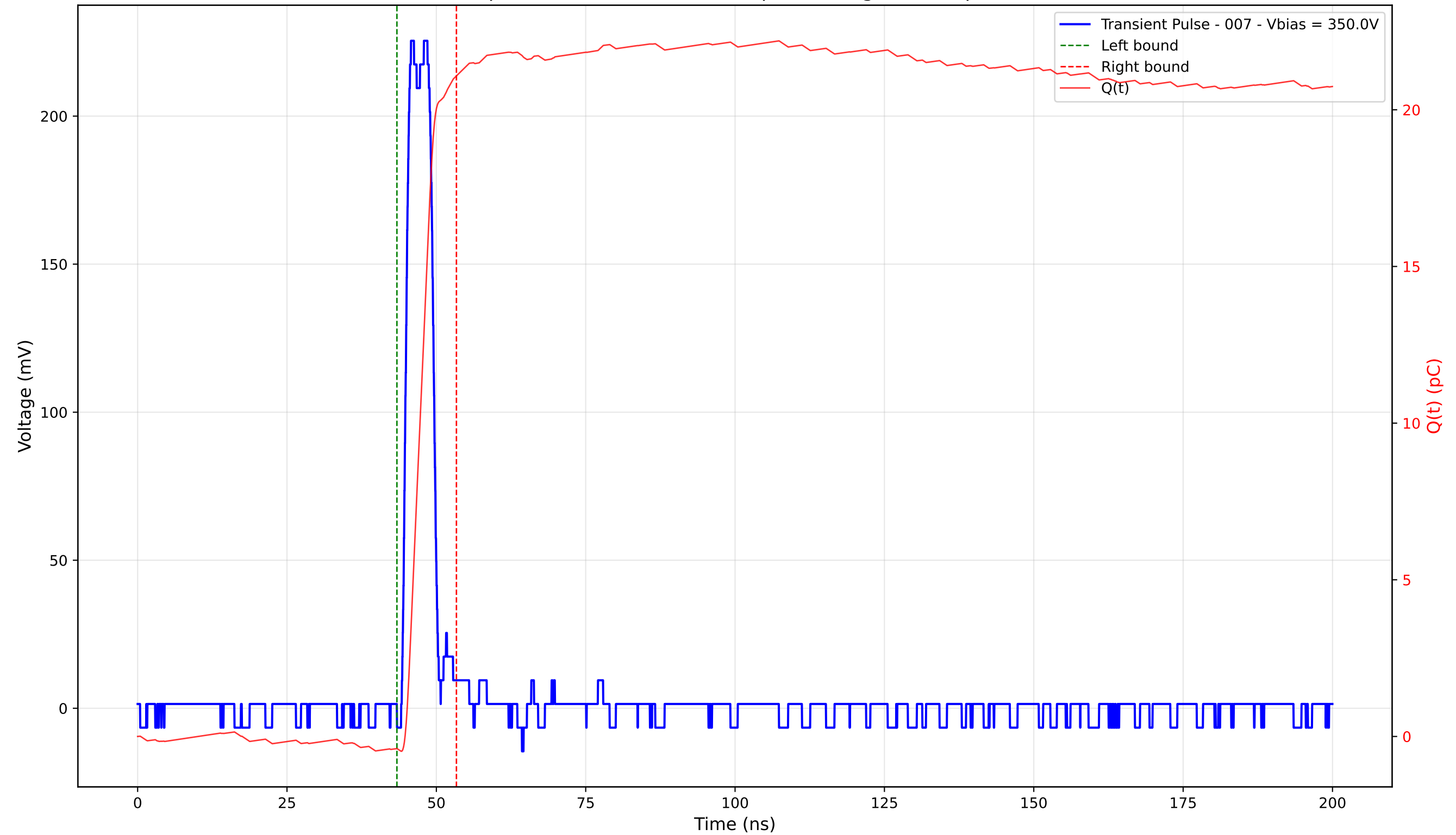
Transient Pulse - Sample: 4003 - Position: 390.0 \mu\text{m} - Charge: 21.47 pC - Rise Time: 1.13 ns
