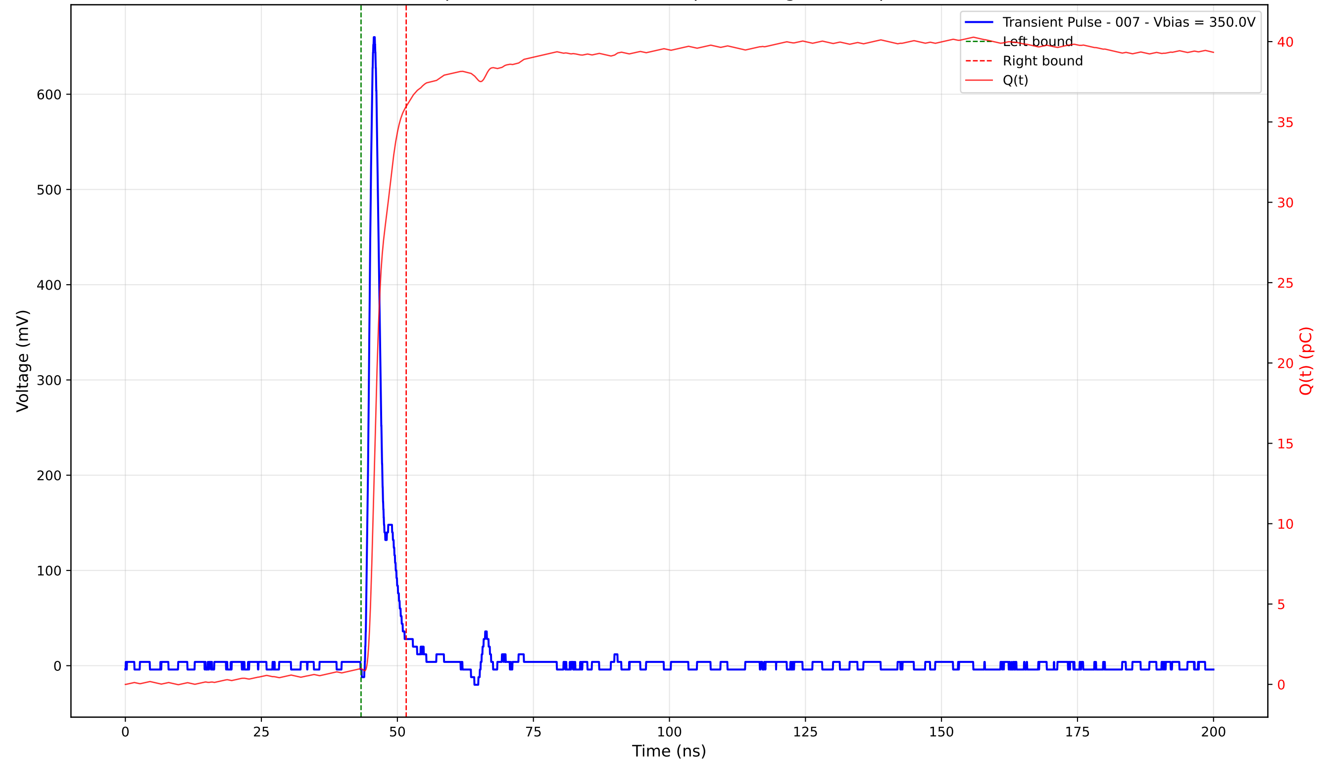
Transient Pulse - Sample: 4003 - Position: 210.0 \mu\text{m} - Charge: 34.99 pC - Rise Time: 1.04 ns
