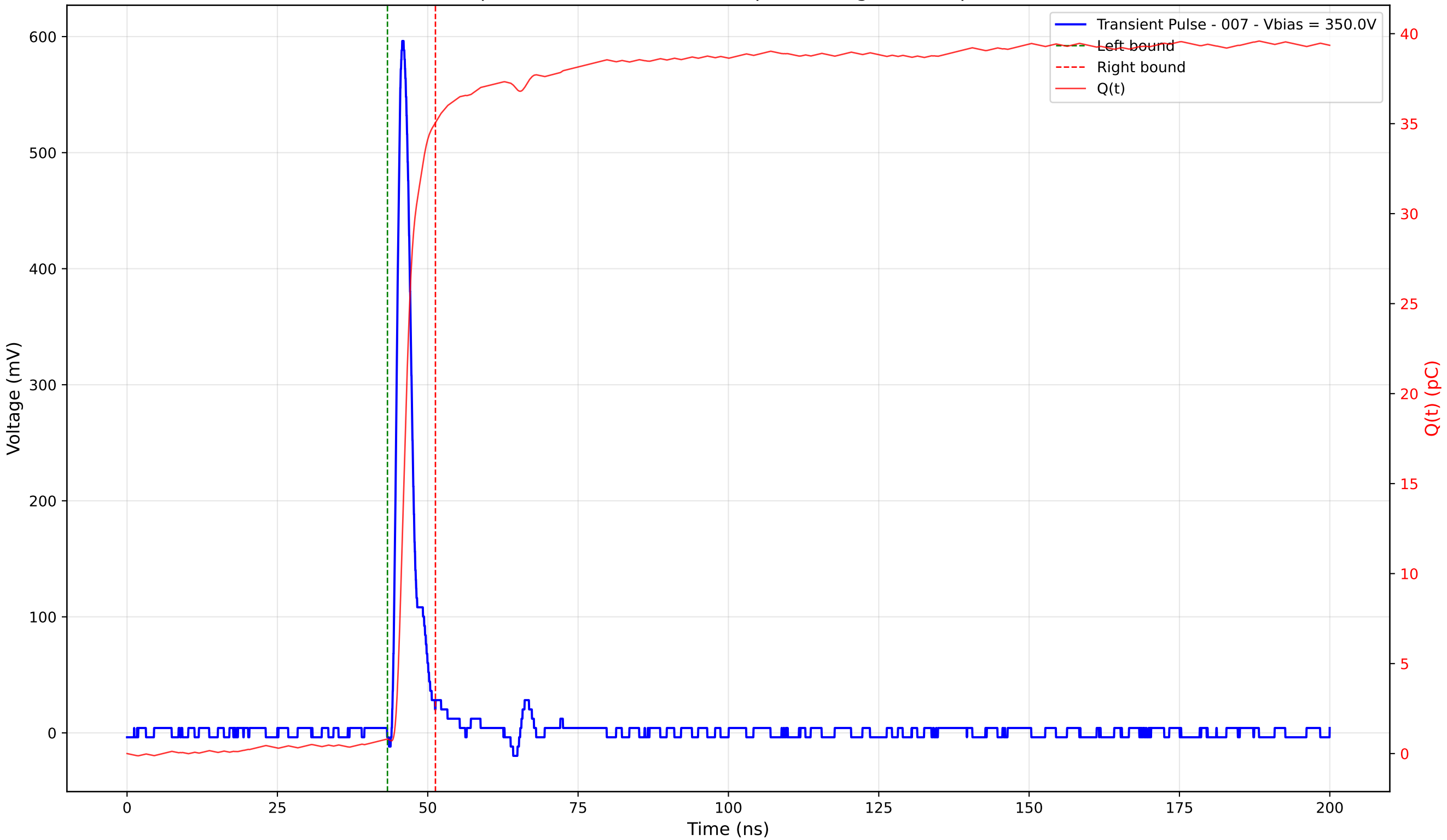
Transient Pulse - Sample: 4003 - Position: 250.0 \mu\text{m} - Charge: 34.24 pC - Rise Time: 1.10 ns
