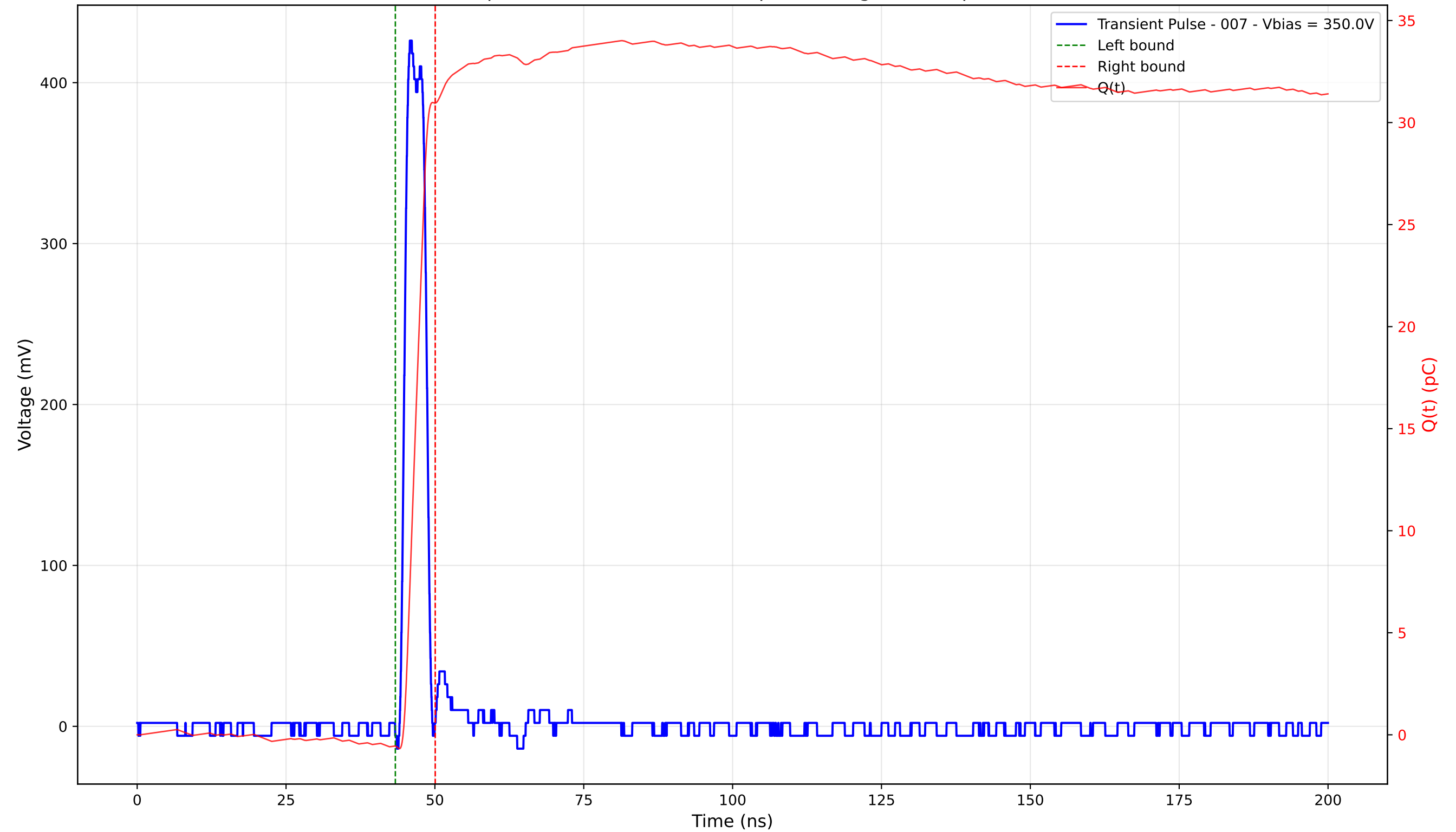
Transient Pulse - Sample: 4003 - Position: 345.0 \mu\text{m} - Charge: 31.50 pC - Rise Time: 1.08 ns
