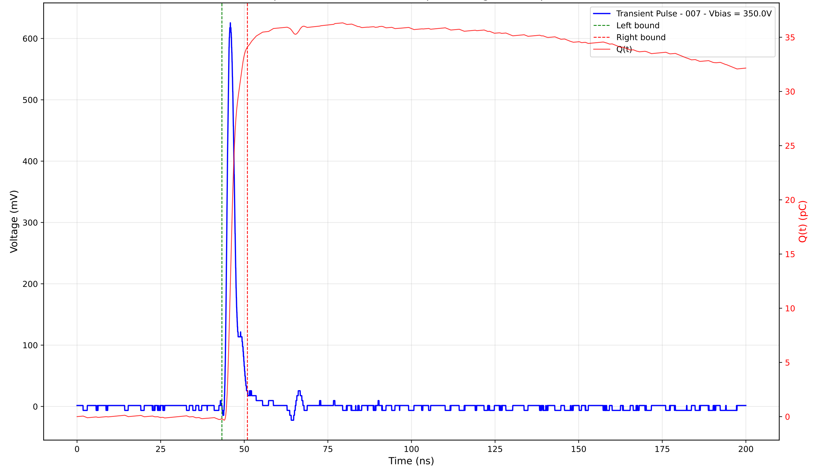
Transient Pulse - Sample: 4003 - Position: 240.0 \mu\text{m} - Charge: 34.30 pC - Rise Time: 1.11 ns
