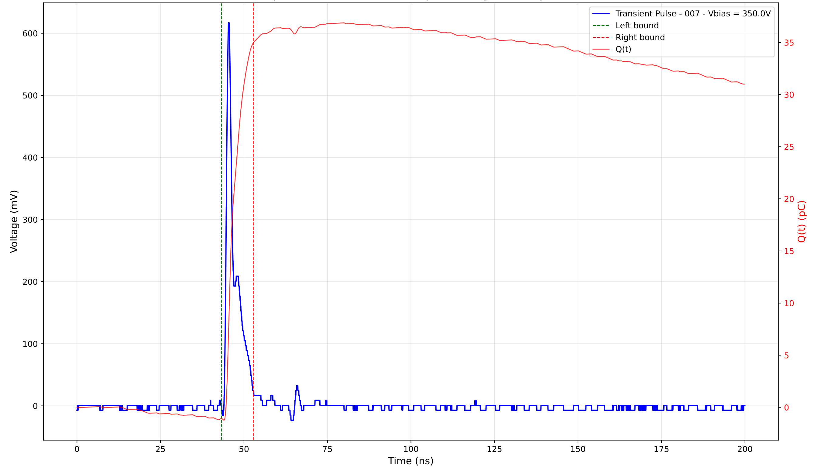
Transient Pulse - Sample: 4003 - Position: 130.0 \mu\text{m} - Charge: 36.03 pC - Rise Time: 0.89 ns
