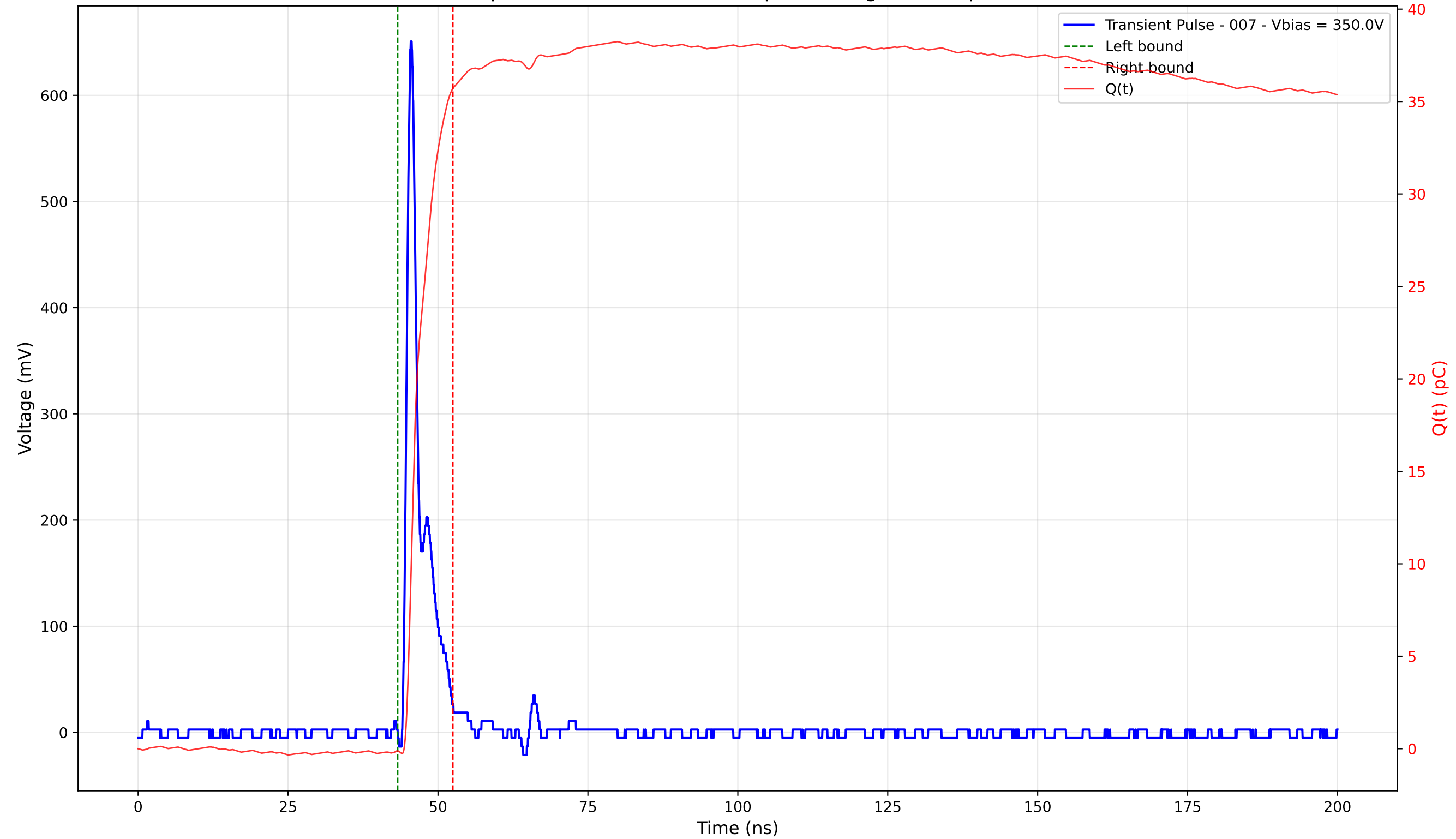
Transient Pulse - Sample: 4003 - Position: 155.0 \mu\text{m} - Charge: 35.82 pC - Rise Time: 0.94 ns
