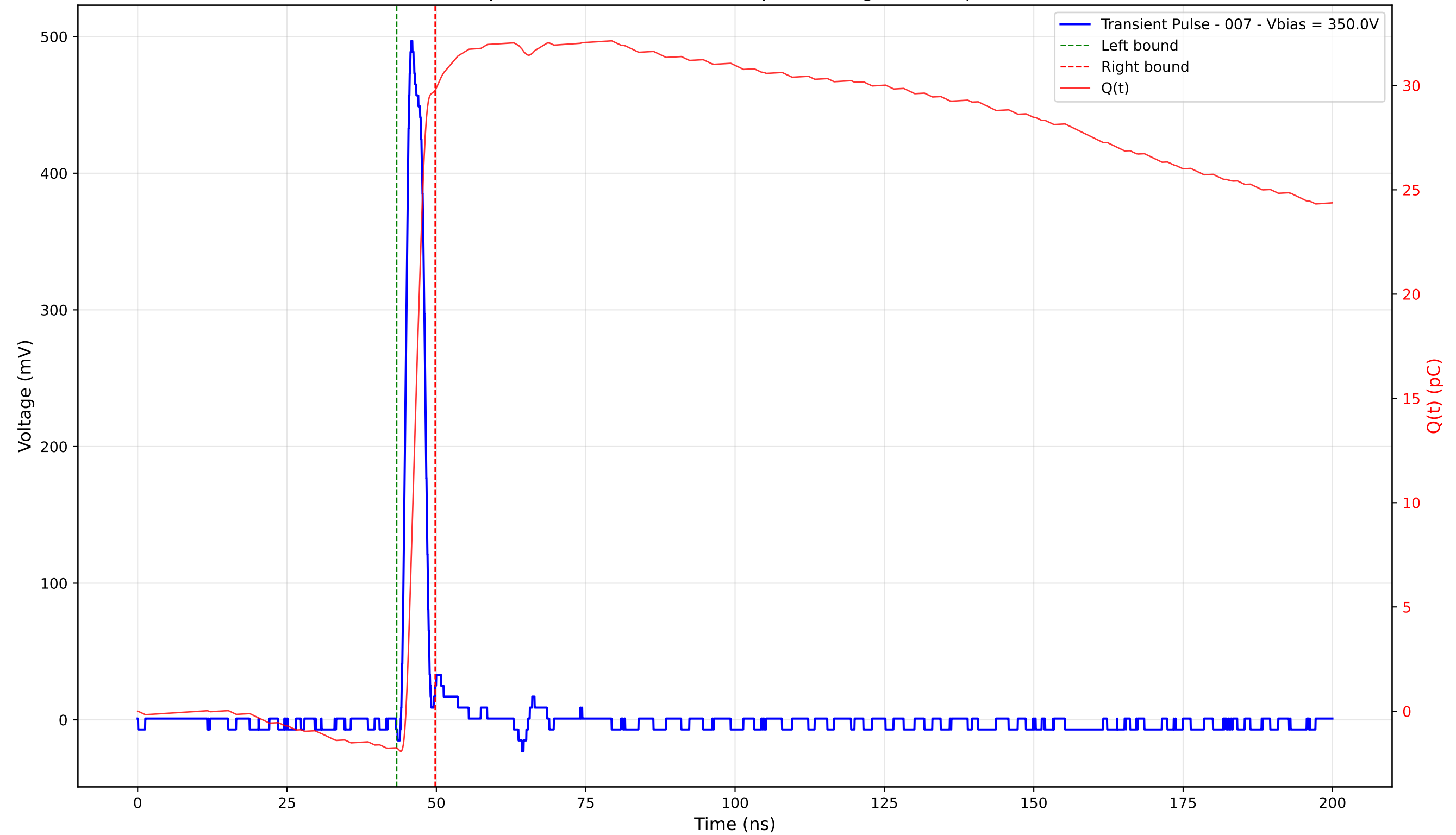
Transient Pulse - Sample: 4003 - Position: 310.0 \mu\text{m} - Charge: 31.54 pC - Rise Time: 1.08 ns
