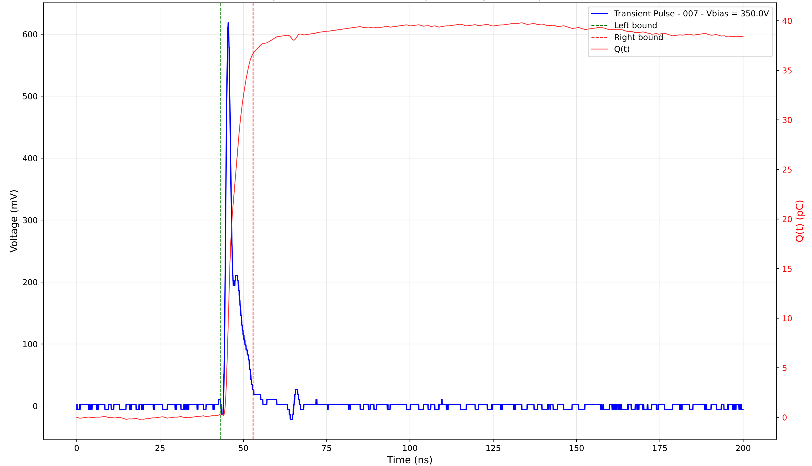
Transient Pulse - Sample: 4003 - Position: 125.0 \mu\text{m} - Charge: 36.35 pC - Rise Time: 0.90 ns
