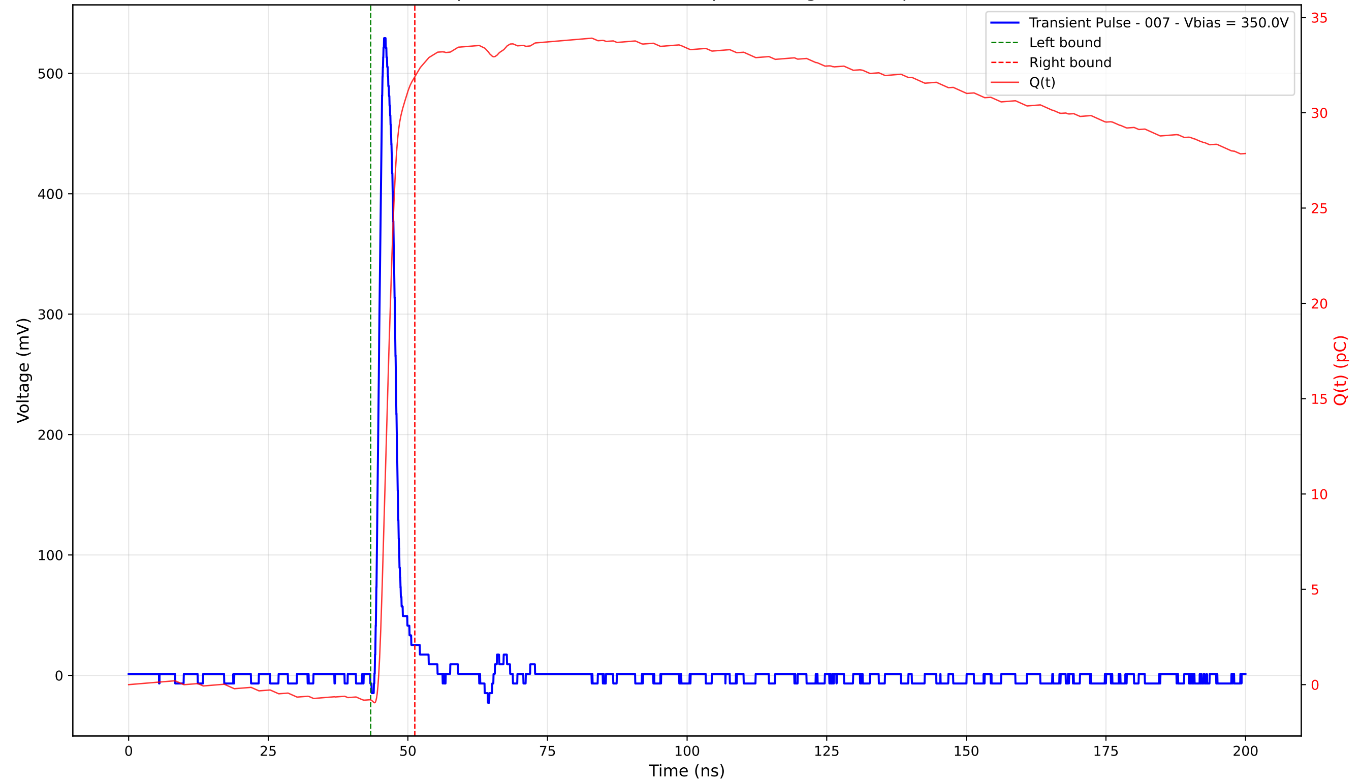
Transient Pulse - Sample: 4003 - Position: 285.0 \mu\text{m} - Charge: 32.69 pC - Rise Time: 1.09 ns
