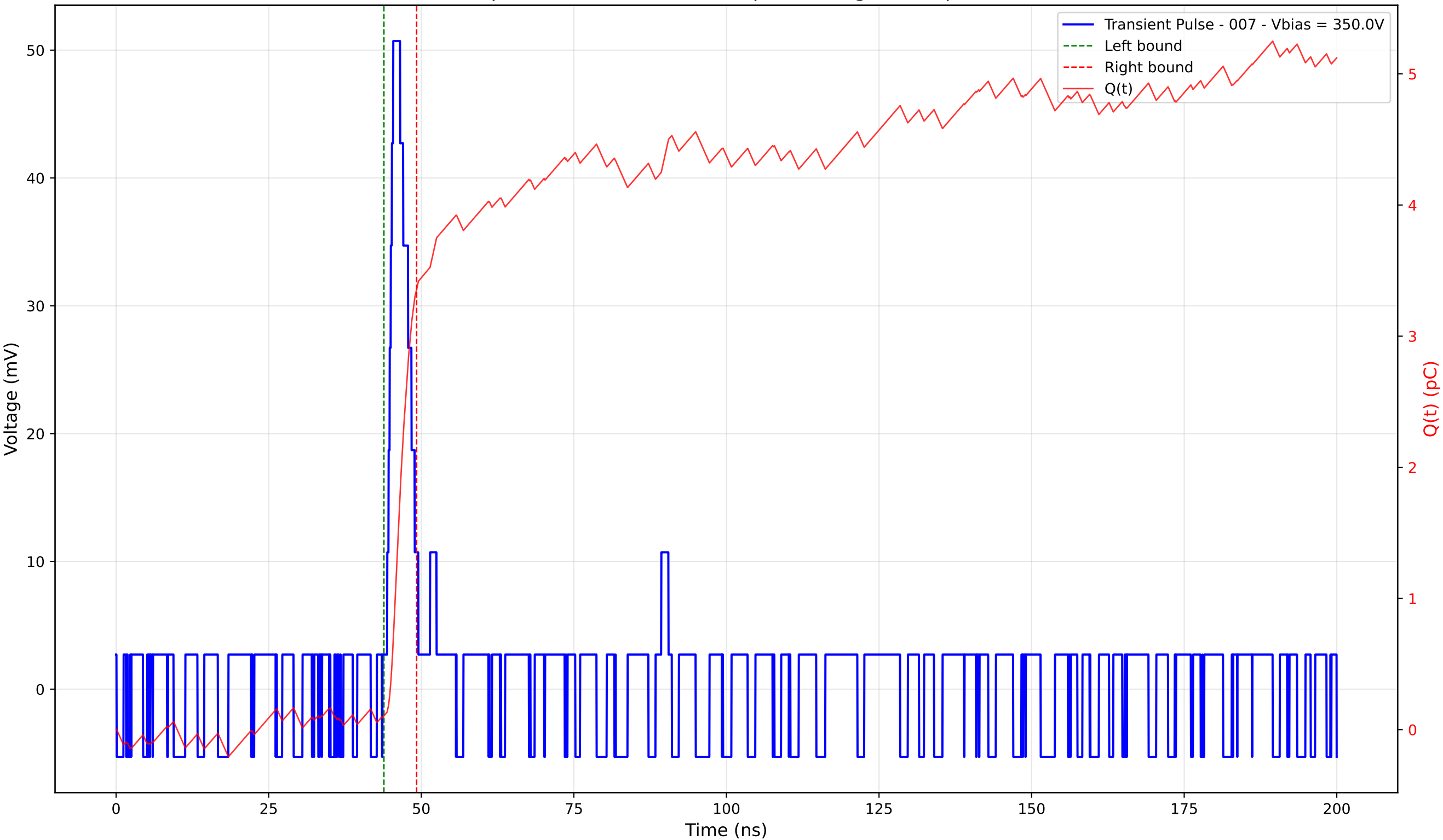
Transient Pulse - Sample: 4003 - Position: 55.0 \mu\text{m} - Charge: 3.26 pC - Rise Time: 0.99 ns
