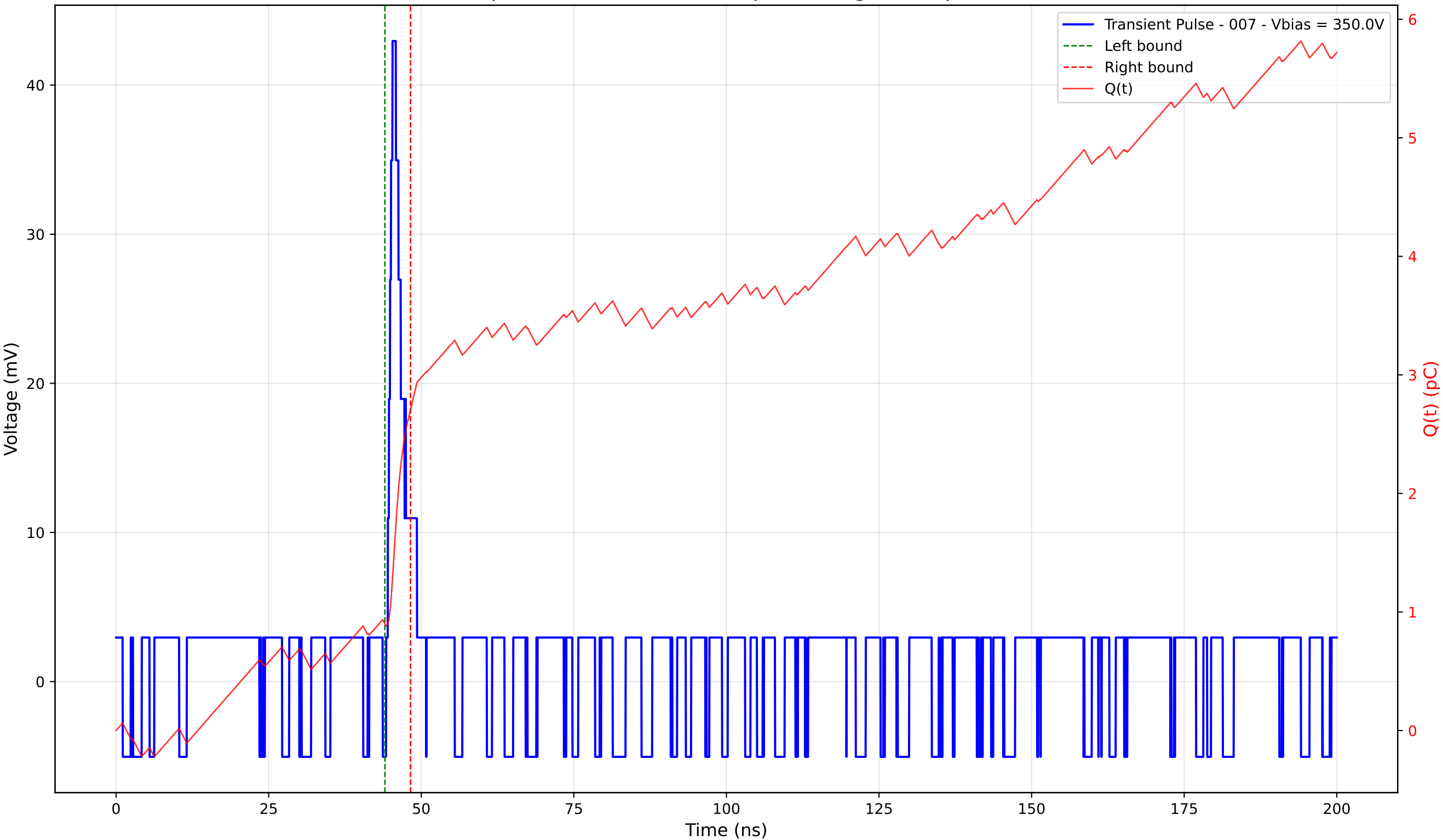
Transient Pulse - Sample: 4003 - Position: 35.0 \mu\text{m} - Charge: 1.81 pC - Rise Time: 0.78 ns
