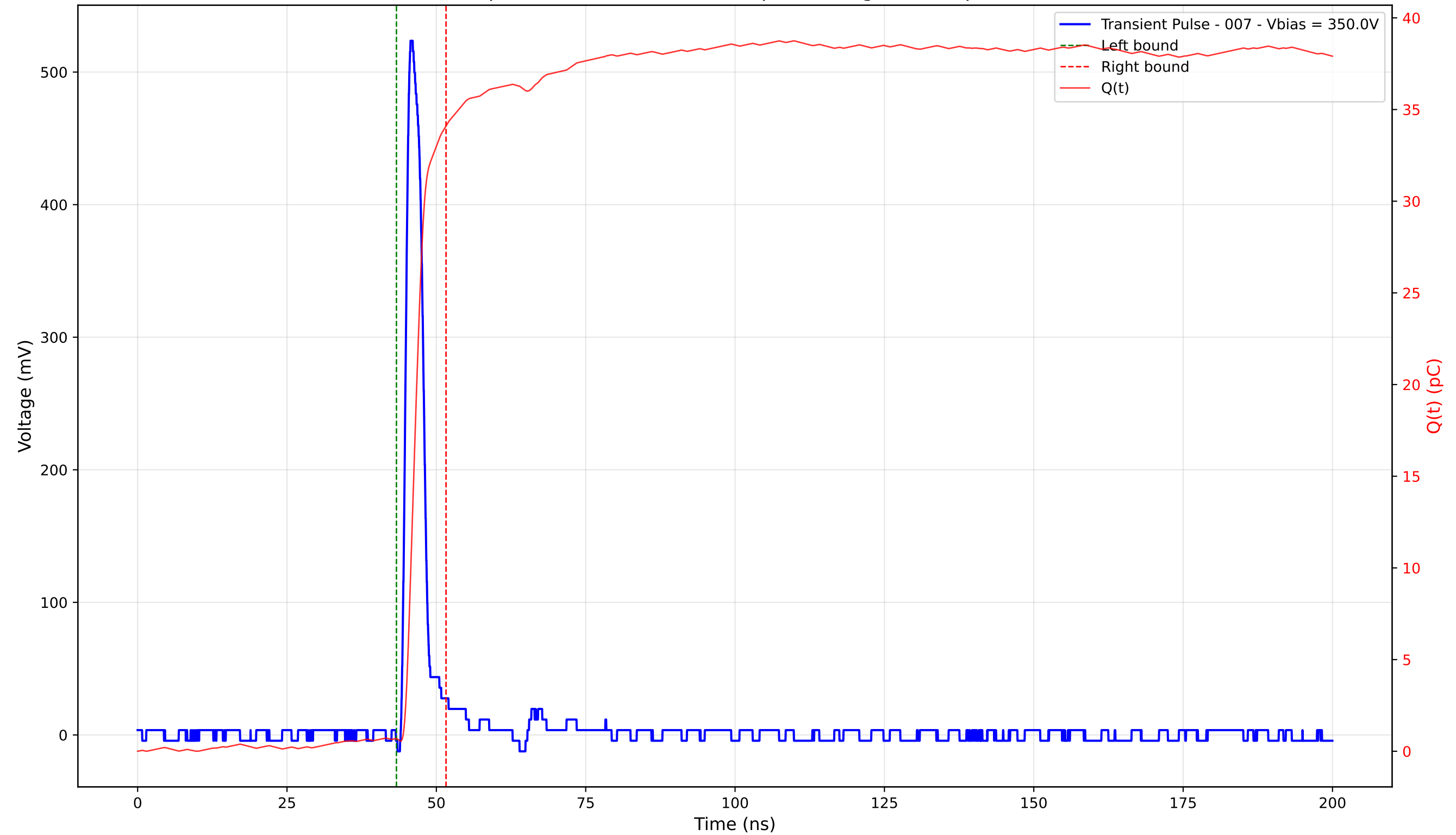
Transient Pulse - Sample: 4003 - Position: 290.0 \mu\text{m} - Charge: 33.42 pC - Rise Time: 1.06 ns
