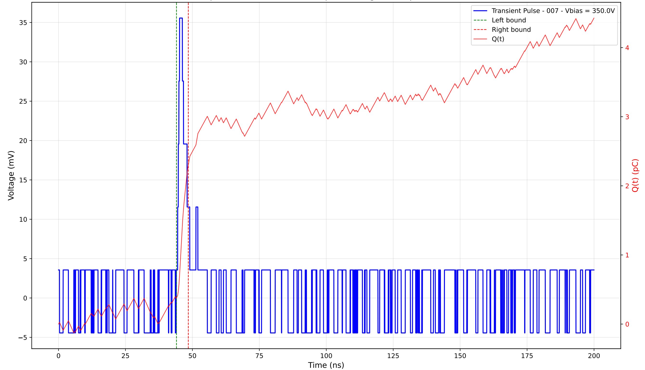
Transient Pulse - Sample: 4003 - Position: 30.0 \mu\text{m} - Charge: 1.92 pC - Rise Time: 0.00 ns (N/A)
