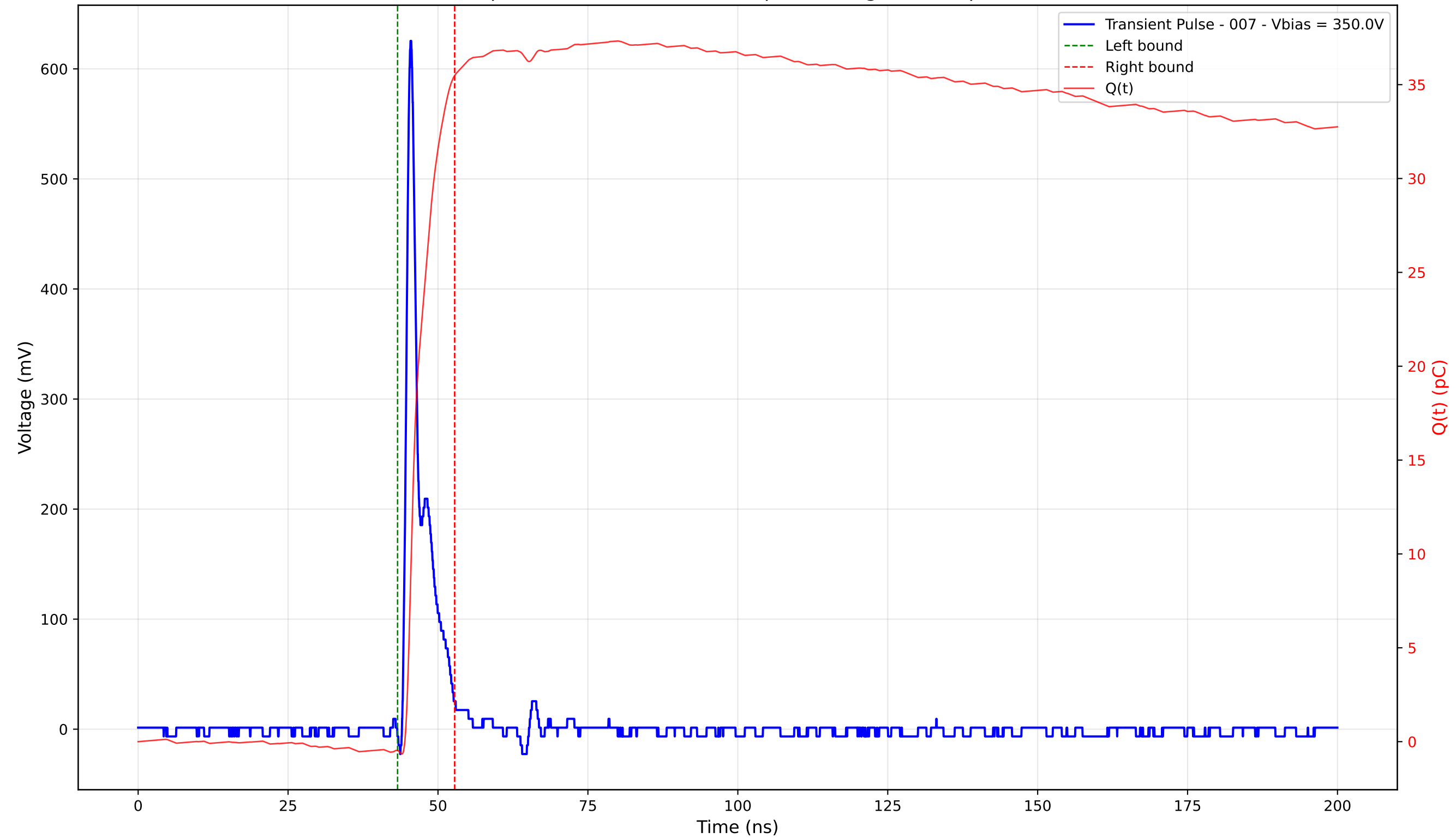
Transient Pulse - Sample: 4003 - Position: 135.0 \mu\text{m} - Charge: 35.95 pC - Rise Time: 0.91 ns
