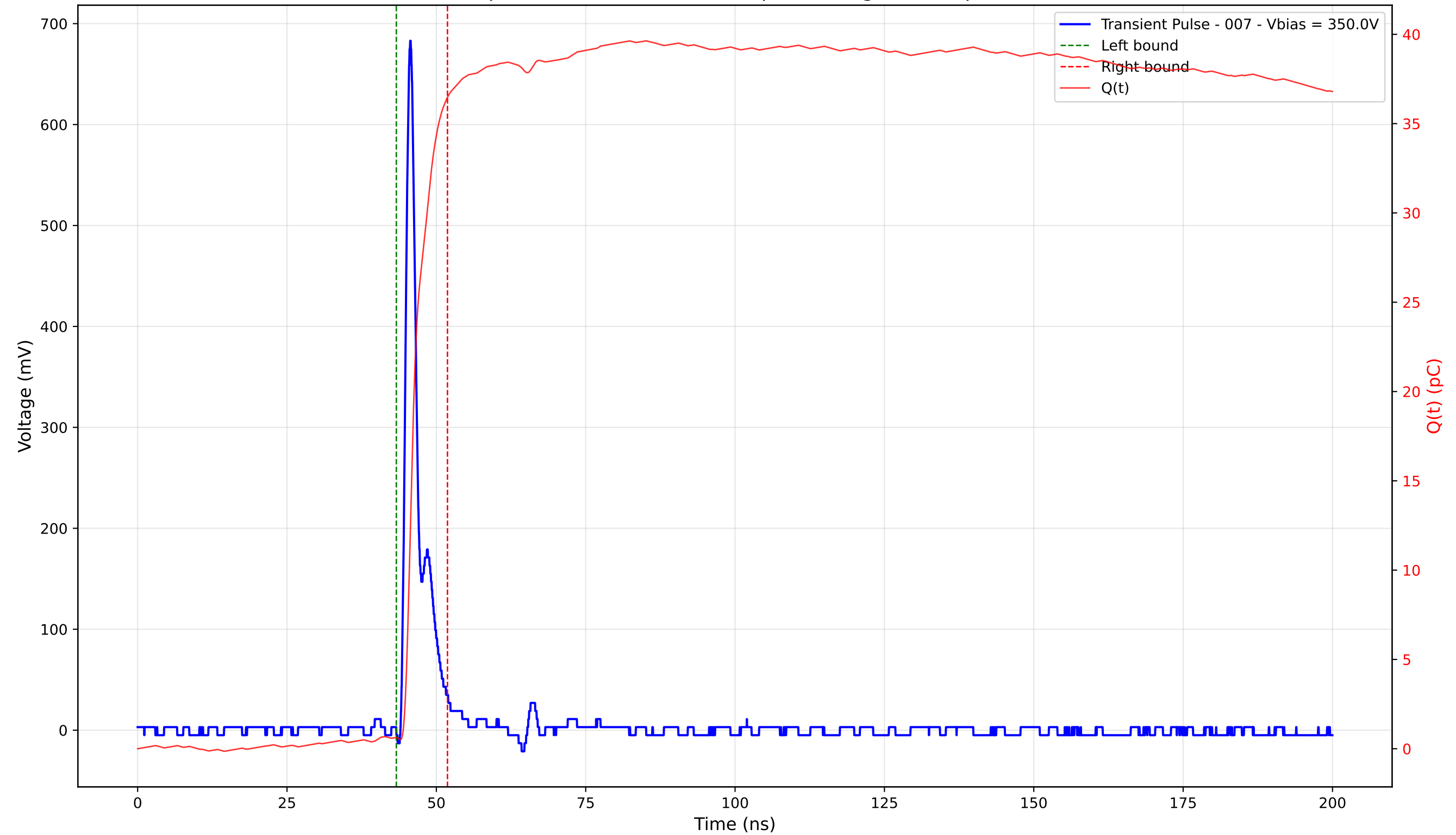
Transient Pulse - Sample: 4003 - Position: 190.0 \mu\text{m} - Charge: 35.85 pC - Rise Time: 1.01 ns
