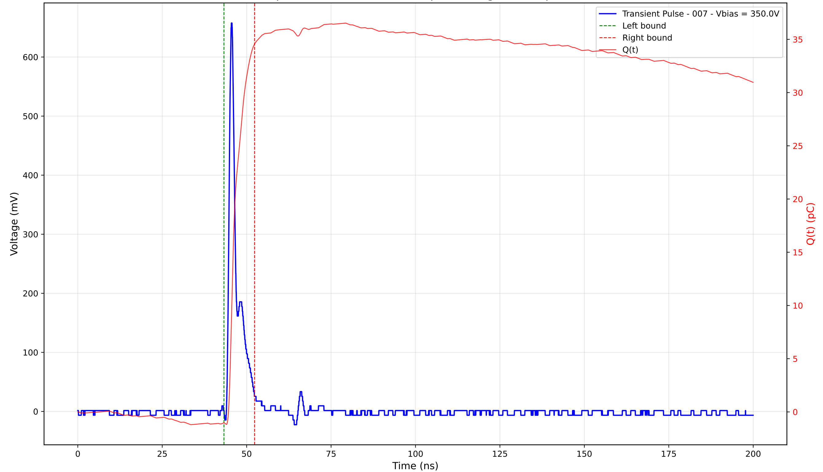
Transient Pulse - Sample: 4003 - Position: 165.0 \mu\text{m} - Charge: 35.60 pC - Rise Time: 0.96 ns
