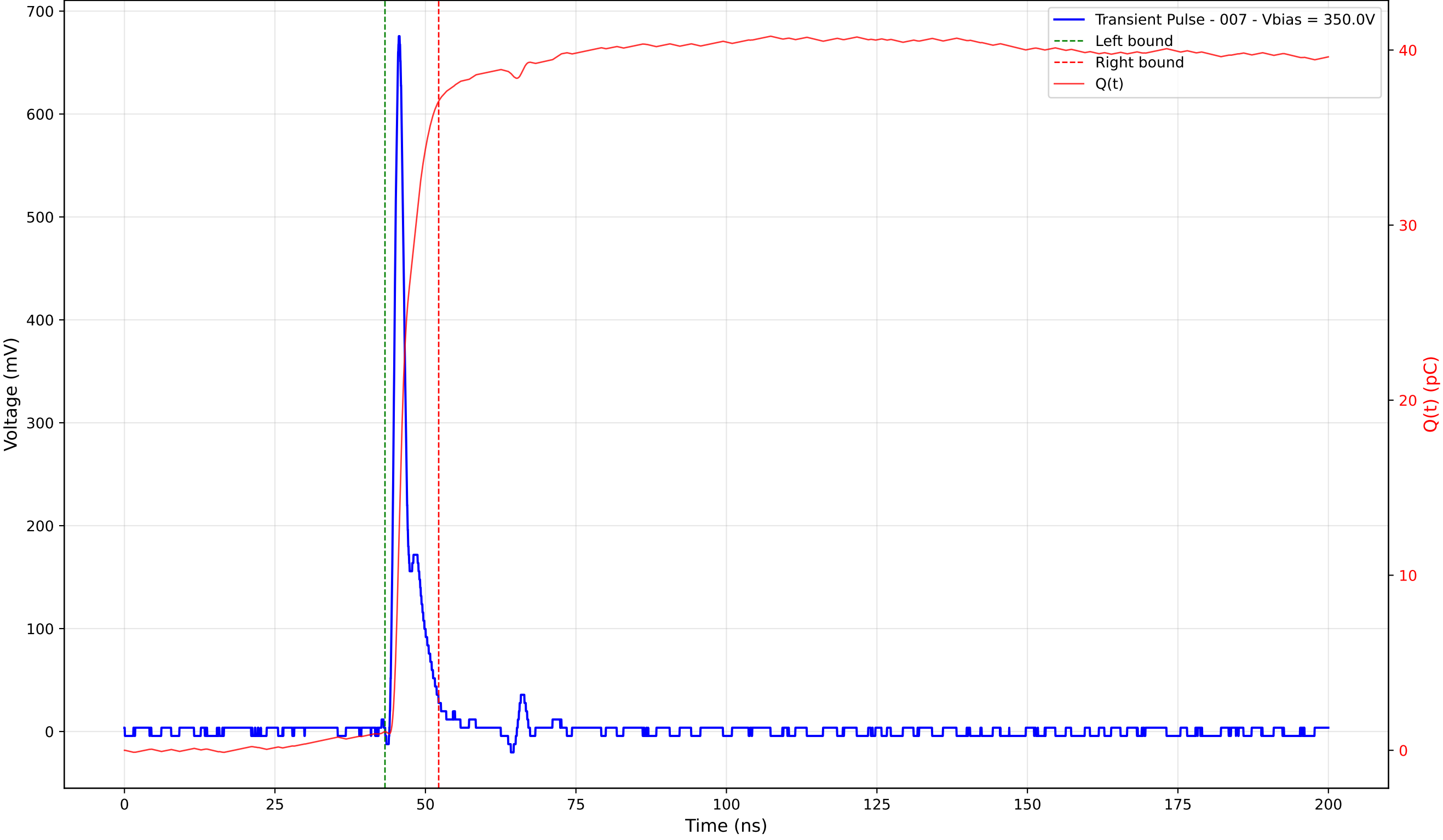
Transient Pulse - Sample: 4003 - Position: 185.0 \mu\text{m} - Charge: 36.02 pC - Rise Time: 1.01 ns
