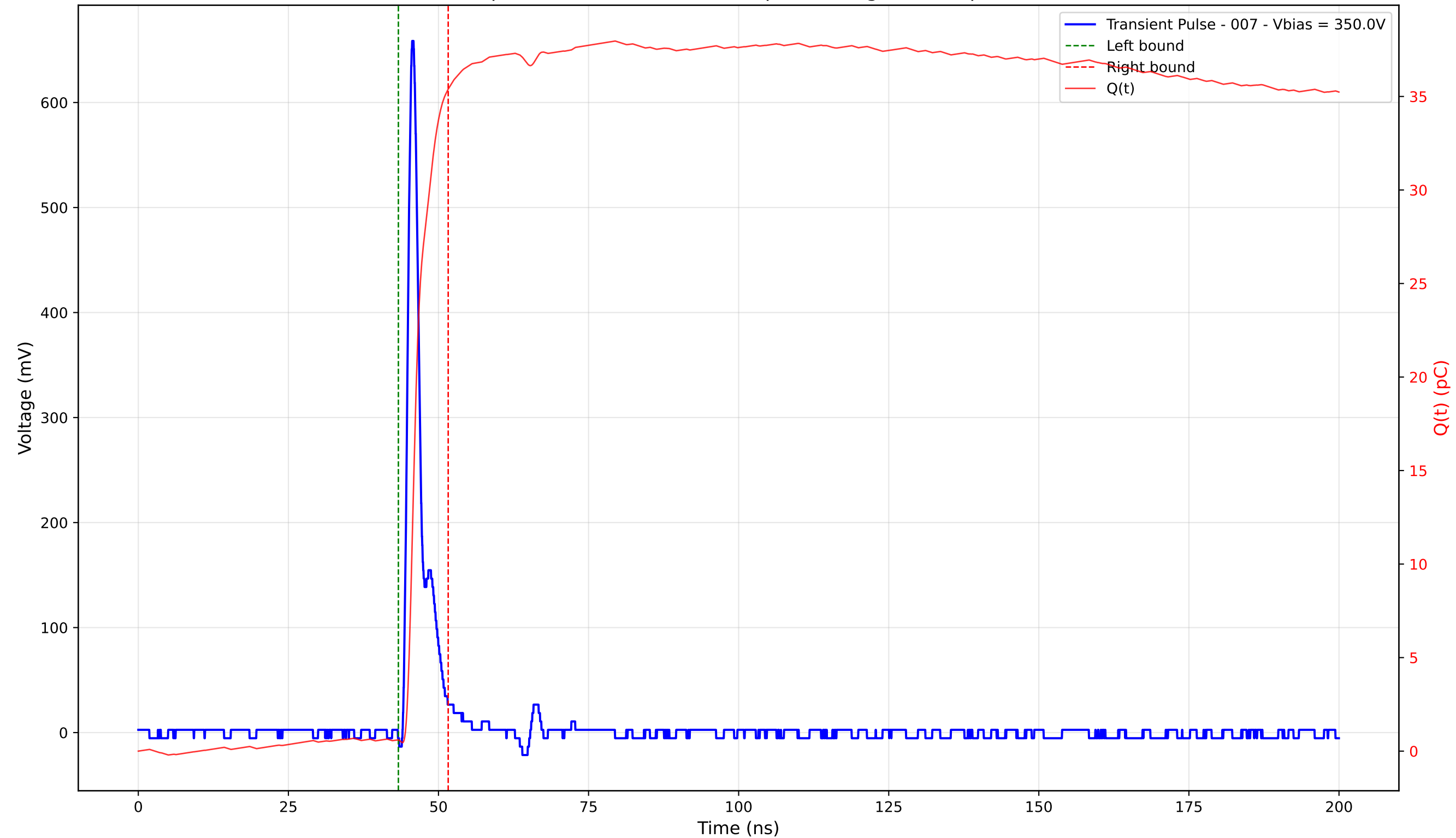
Transient Pulse - Sample: 4003 - Position: 205.0 \mu\text{m} - Charge: 34.80 pC - Rise Time: 1.06 ns
