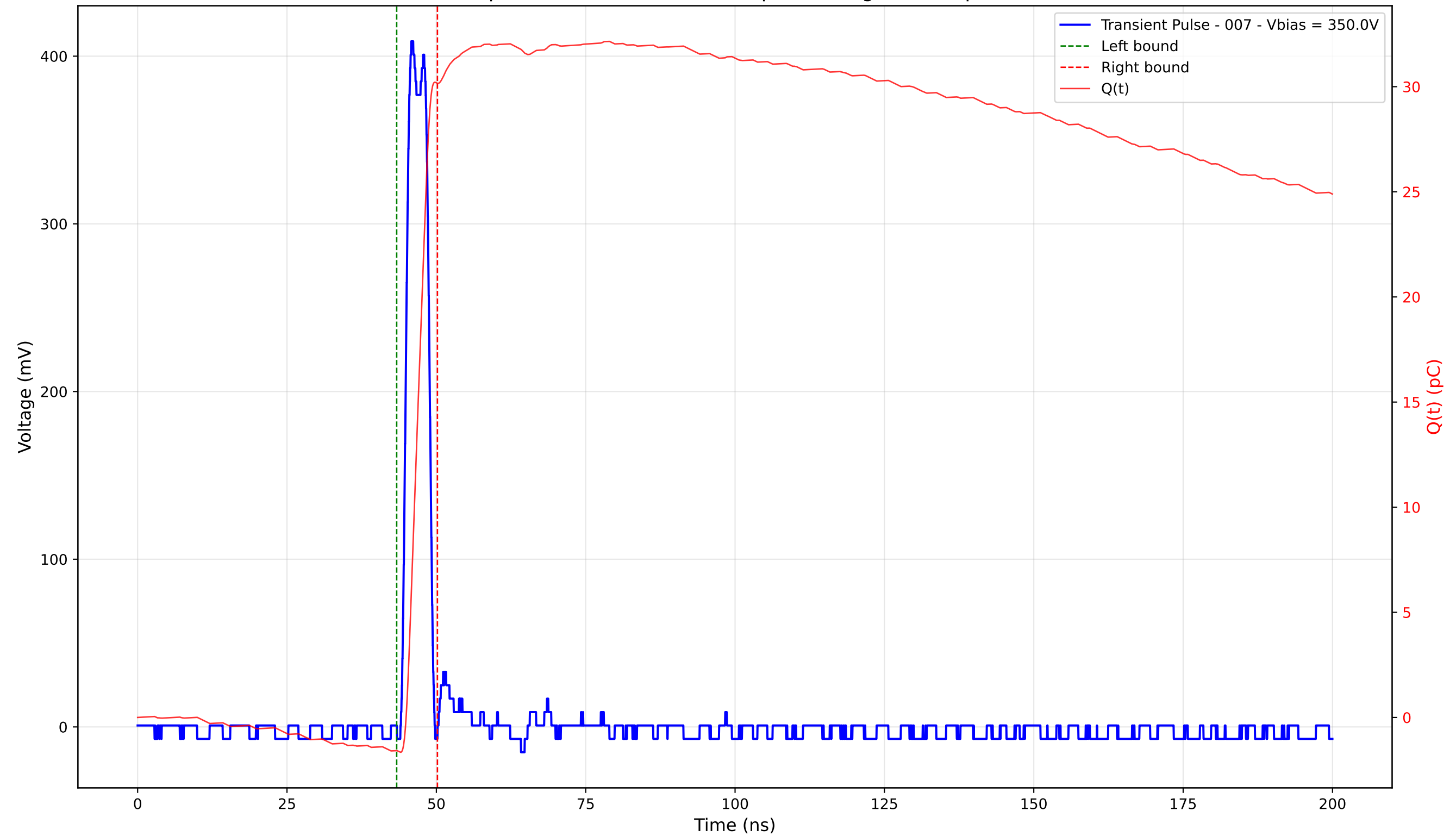
Transient Pulse - Sample: 4003 - Position: 355.0 \mu\text{m} - Charge: 31.73 pC - Rise Time: 1.10 ns
