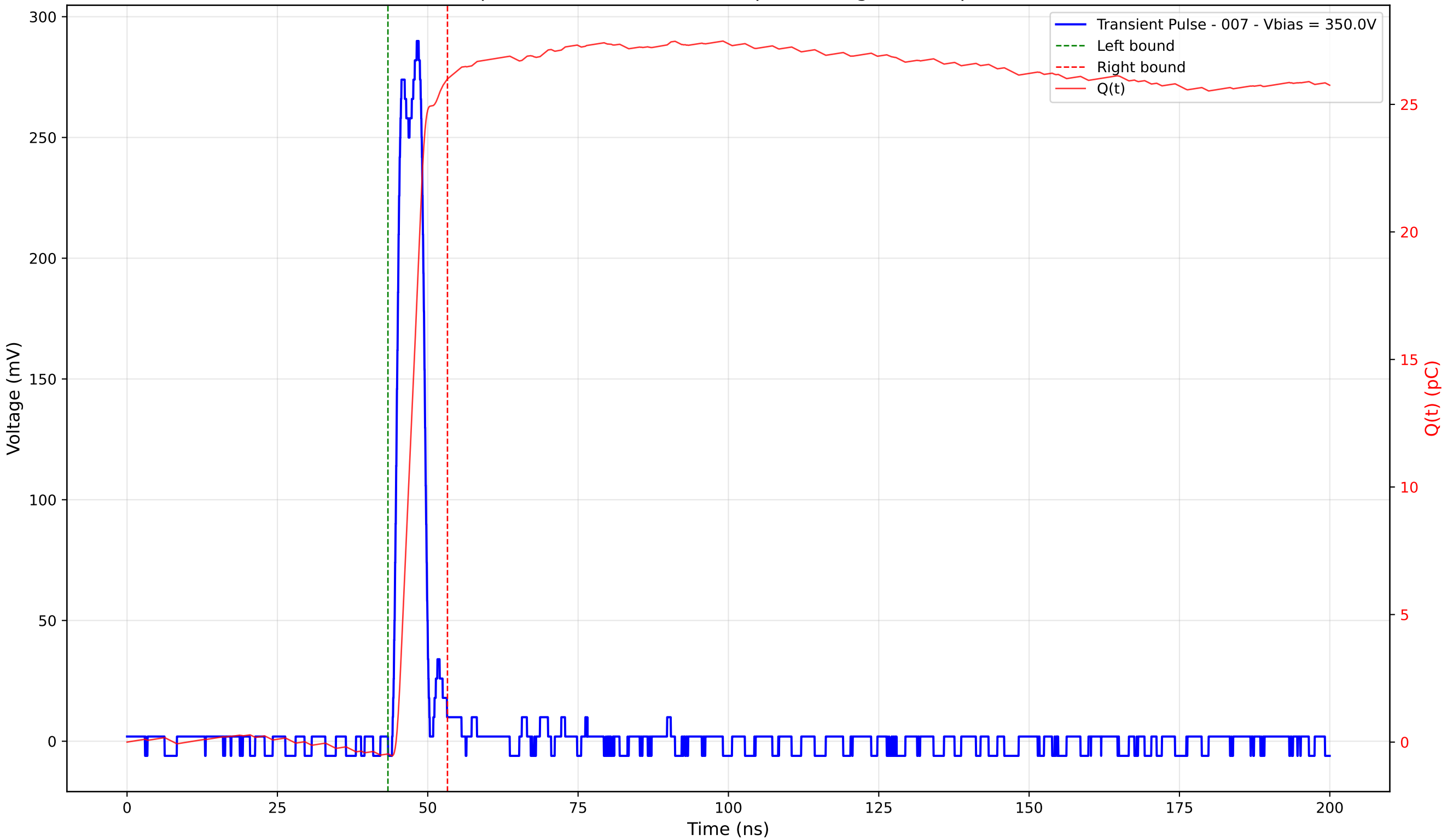
Transient Pulse - Sample: 4003 - Position: 385.0 \mu\text{m} - Charge: 26.46 pC - Rise Time: 1.17 ns
