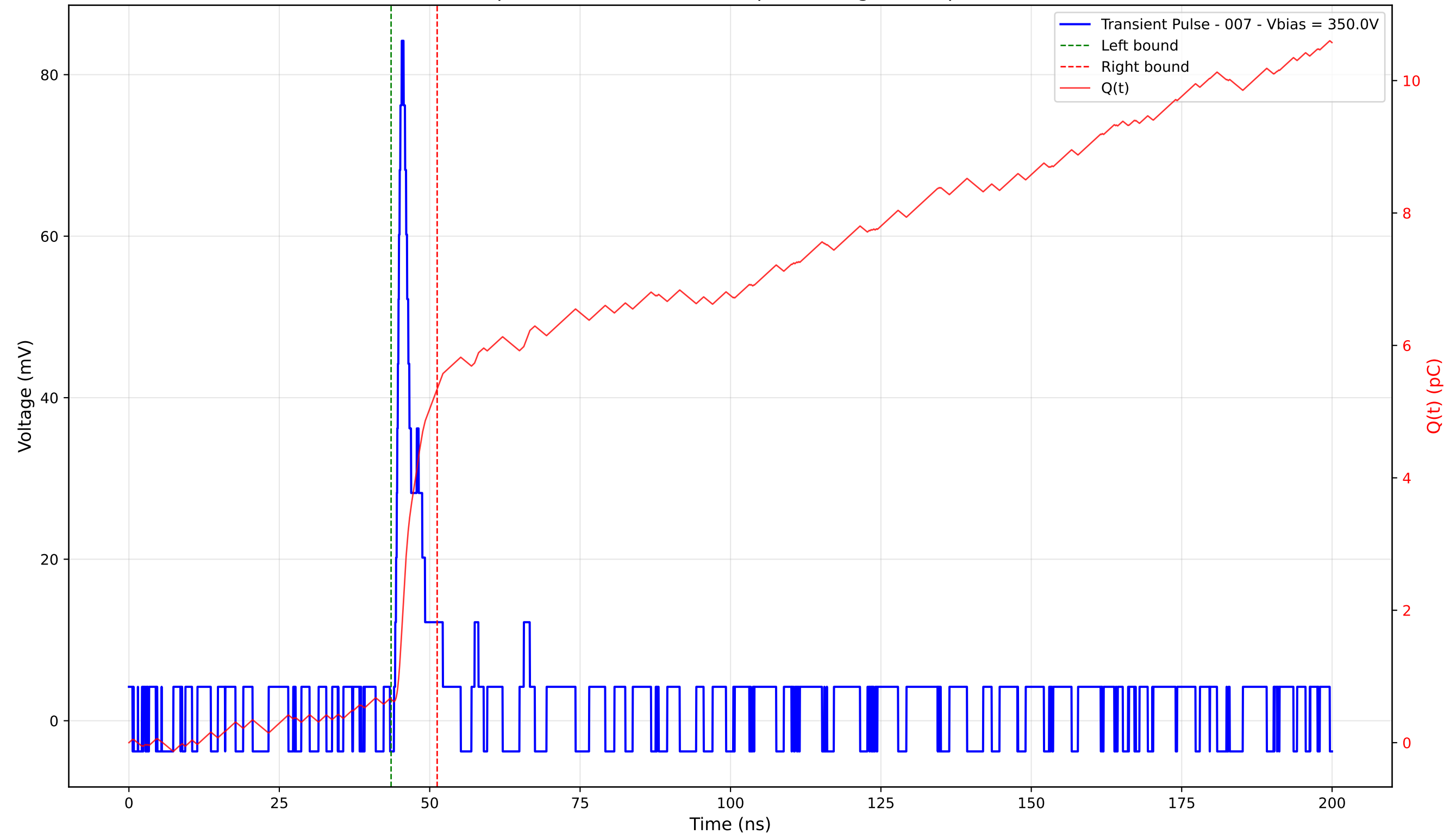
Transient Pulse - Sample: 4003 - Position: 80.0 \mu\text{m} - Charge: 4.69 pC - Rise Time: 0.87 ns
