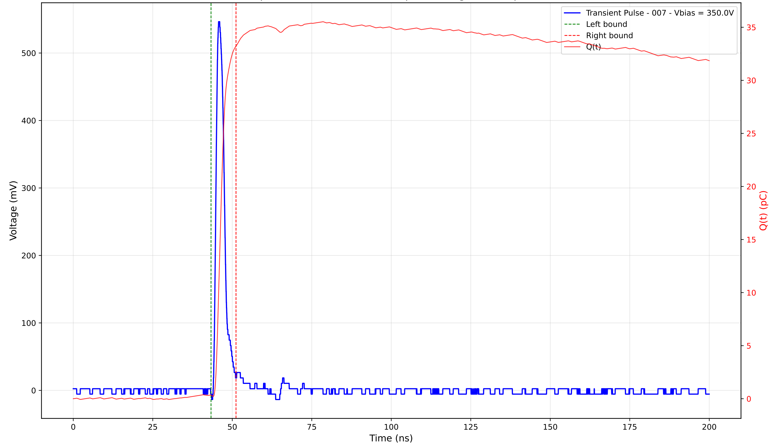
Transient Pulse - Sample: 4003 - Position: 270.0 \mu\text{m} - Charge: 32.89 pC - Rise Time: 1.07 ns
