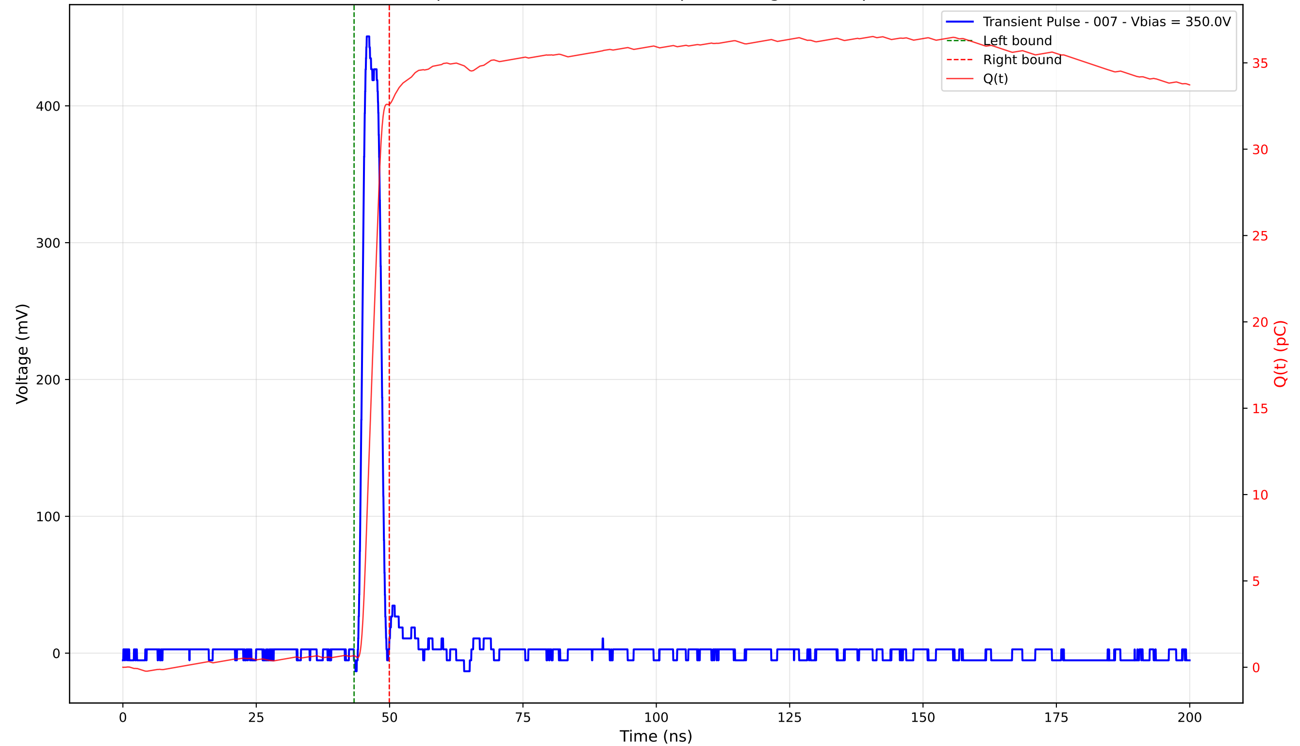
Transient Pulse - Sample: 4003 - Position: 335.0 \mu\text{m} - Charge: 31.92 pC - Rise Time: 1.09 ns
