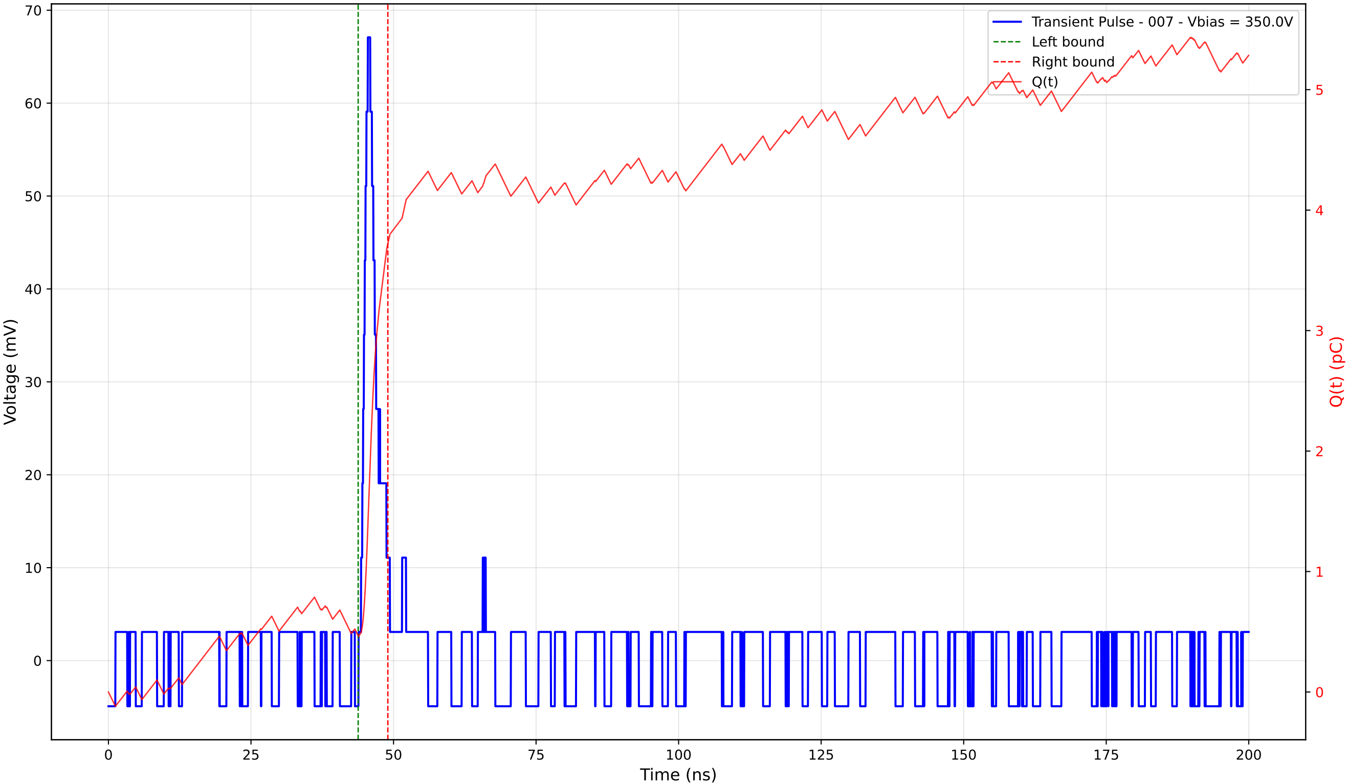
Transient Pulse - Sample: 4003 - Position: 45.0 \mu\text{m} - Charge: 3.25 pC - Rise Time: 1.19 ns
