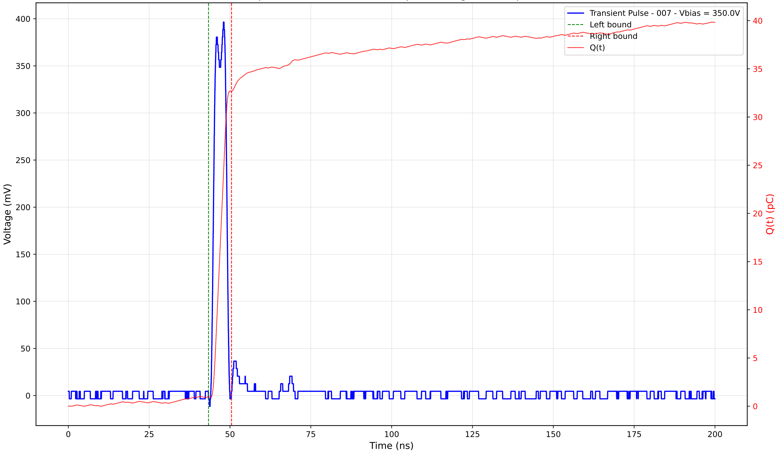
Transient Pulse - Sample: 4003 - Position: 365.0 \mu\text{m} - Charge: 31.69 pC - Rise Time: 1.25 ns
