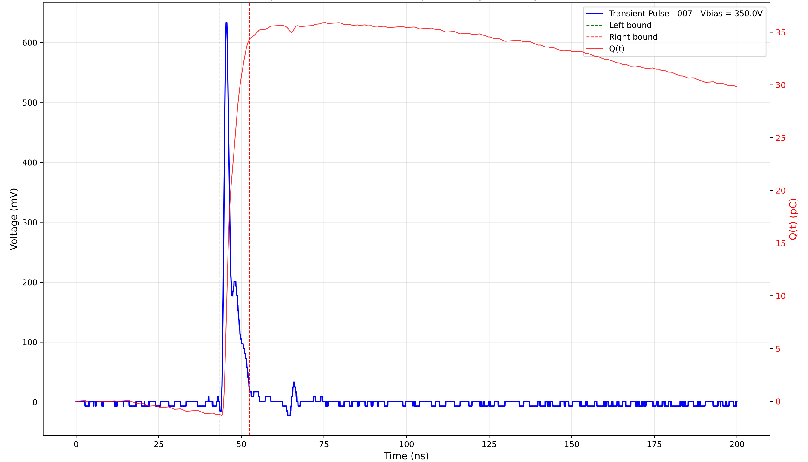
Transient Pulse - Sample: 4003 - Position: 145.0 \mu\text{m} - Charge: 35.52 pC - Rise Time: 0.91 ns
