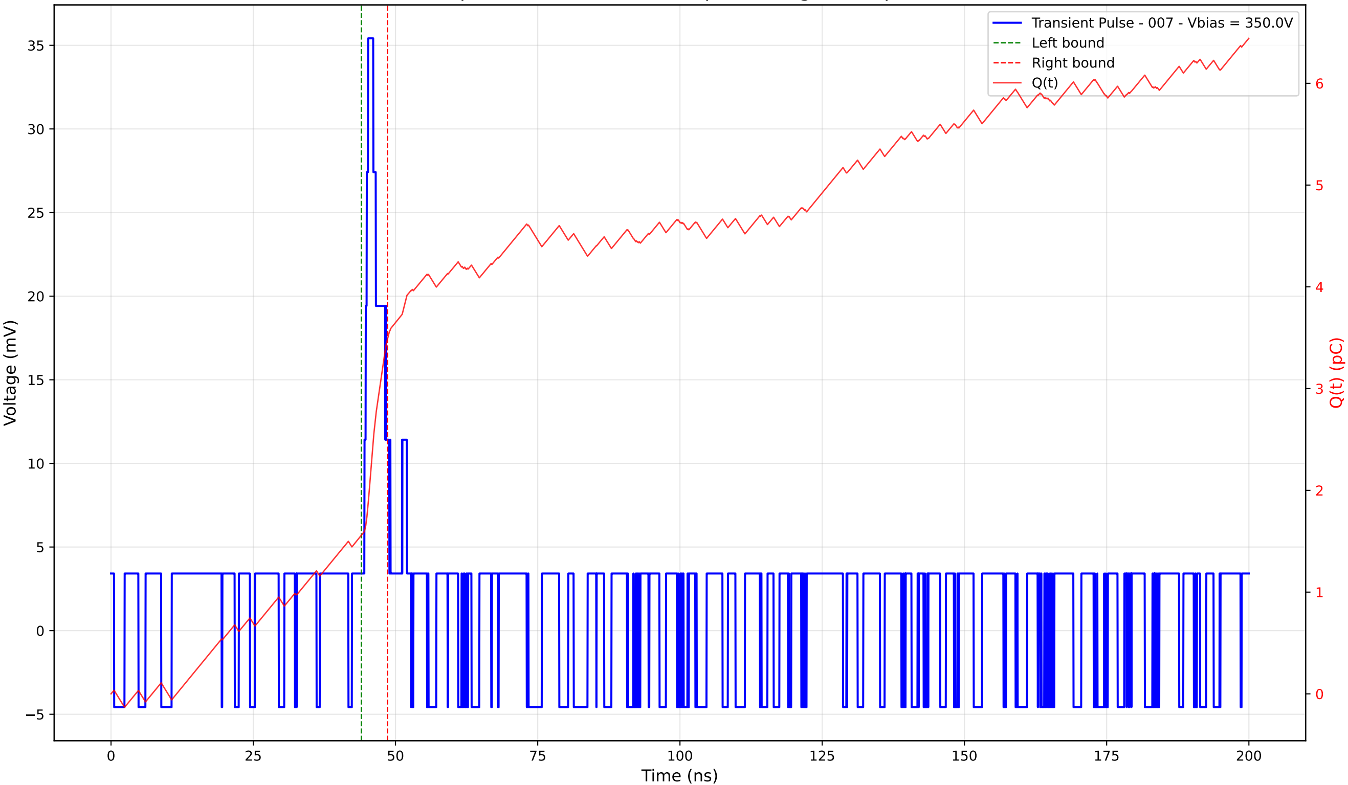
Transient Pulse - Sample: 4003 - Position: 20.0 \mu\text{m} - Charge: 1.93 pC - Rise Time: 0.66 ns
