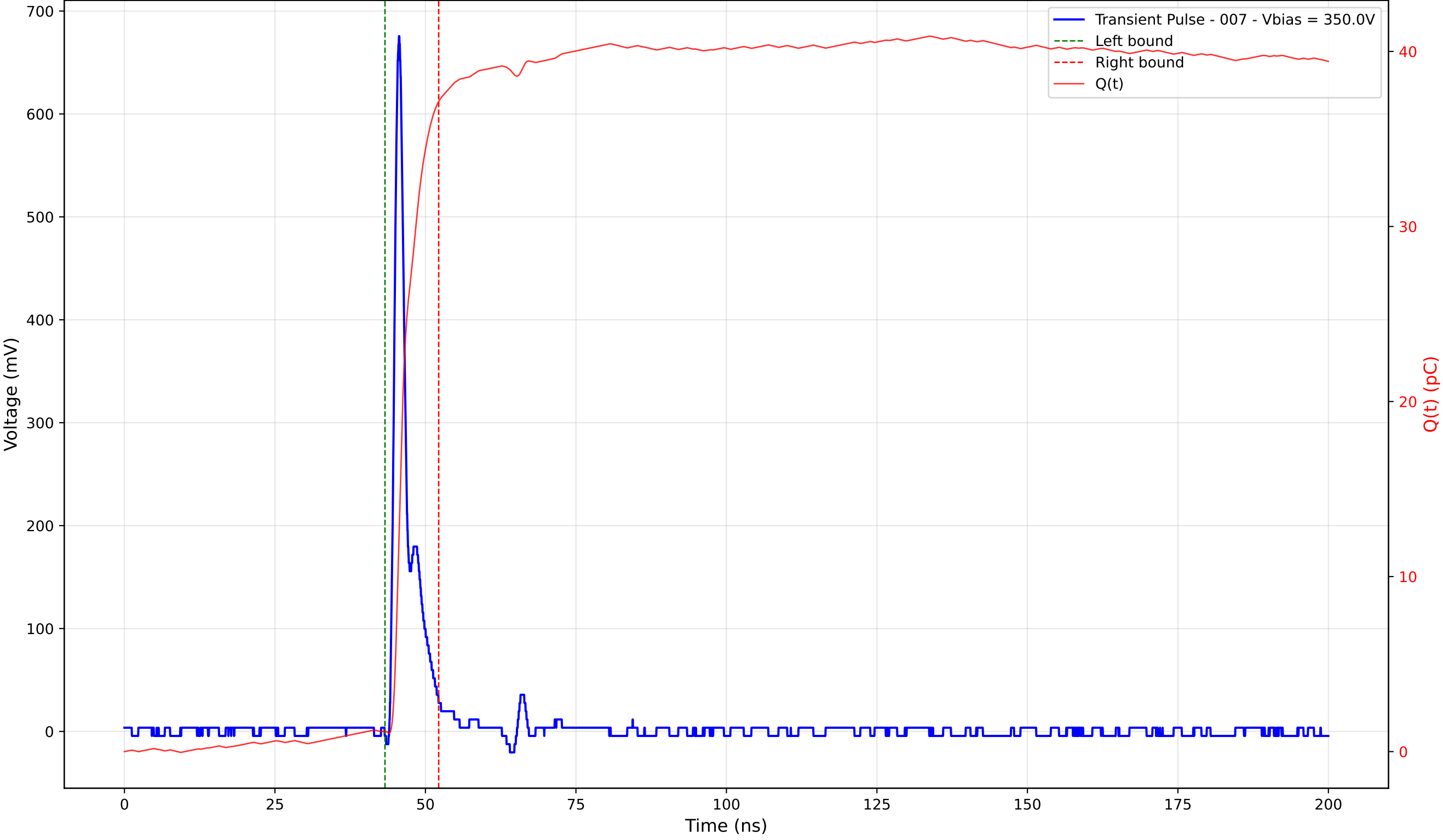
Transient Pulse - Sample: 4003 - Position: 180.0 \mu\text{m} - Charge: 35.97 pC - Rise Time: 1.01 ns
