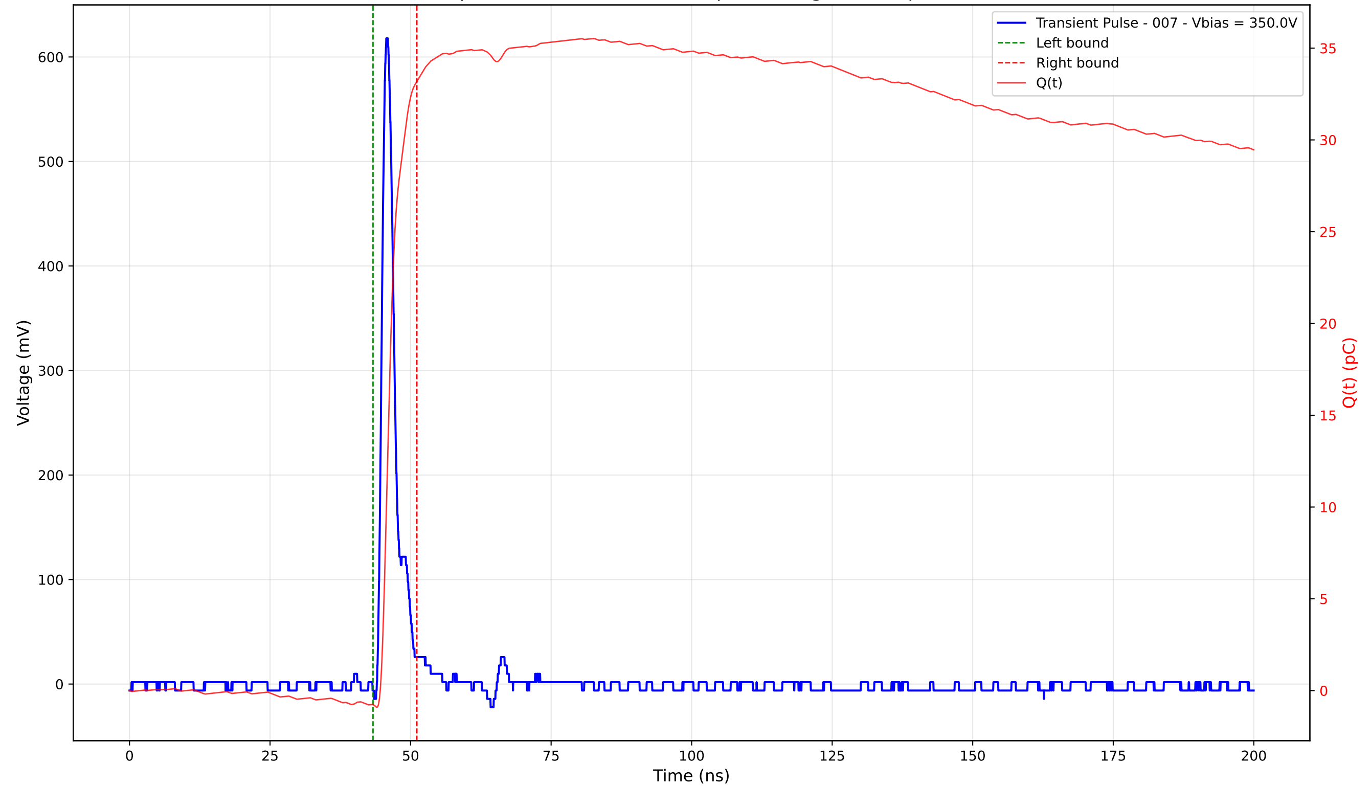
Transient Pulse - Sample: 4003 - Position: 235.0 \mu\text{m} - Charge: 33.95 pC - Rise Time: 1.08 ns
