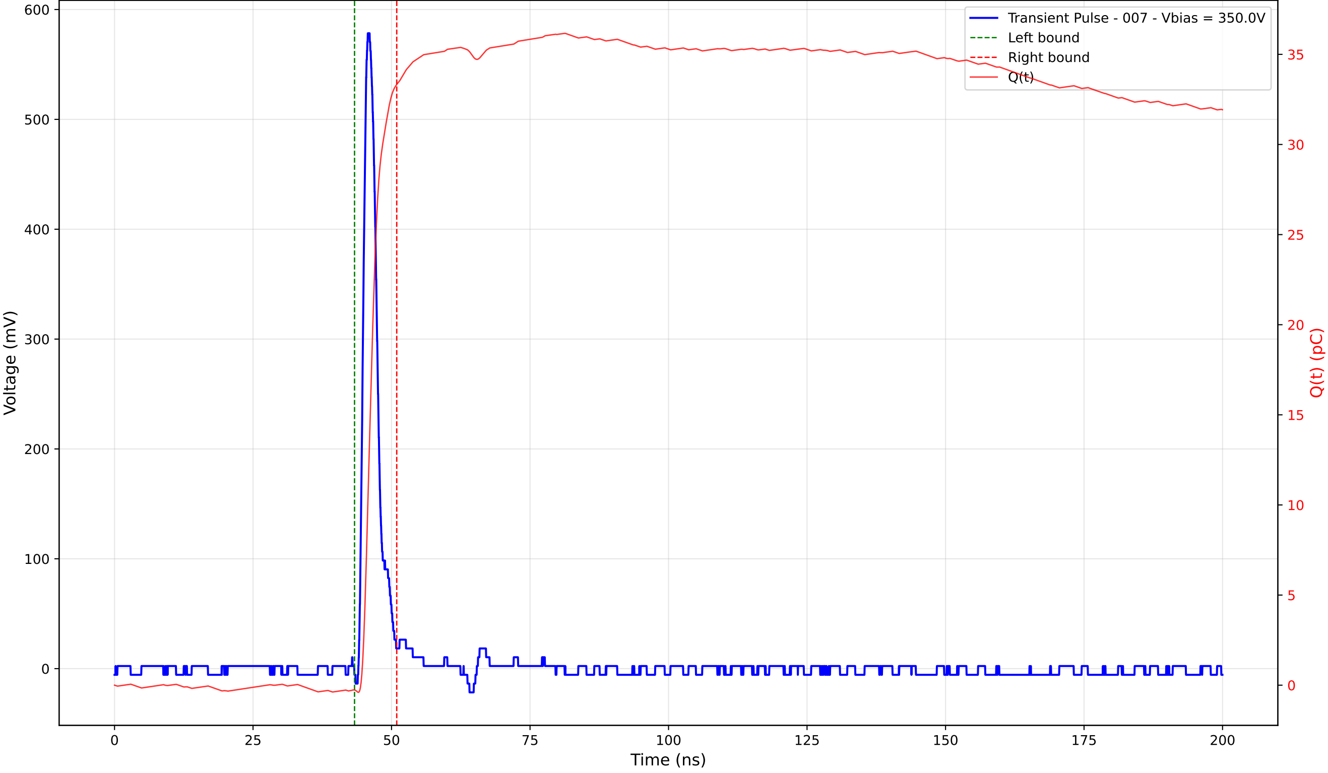
Transient Pulse - Sample: 4003 - Position: 260.0 \mu\text{m} - Charge: 33.59 pC - Rise Time: 1.08 ns
