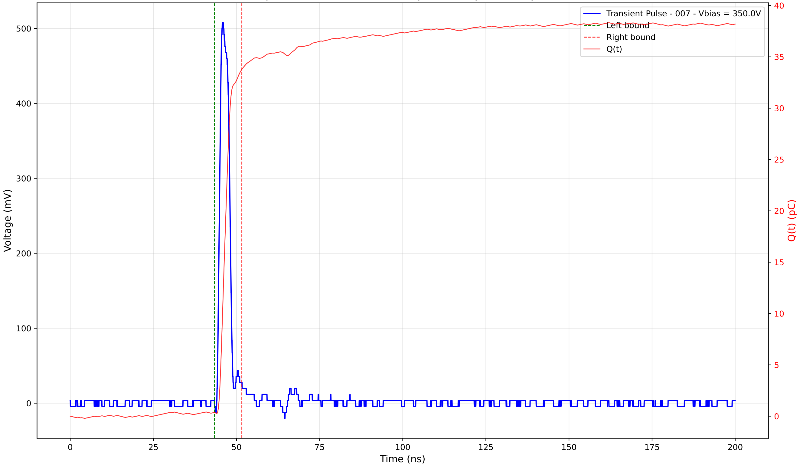
Transient Pulse - Sample: 4003 - Position: 305.0 \mu\text{m} - Charge: 33.43 pC - Rise Time: 1.08 ns
