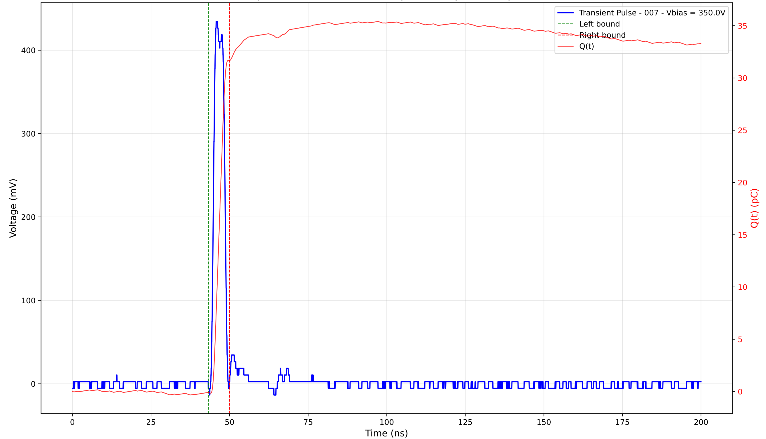
Transient Pulse - Sample: 4003 - Position: 340.0 \mu\text{m} - Charge: 31.76 pC - Rise Time: 1.12 ns
