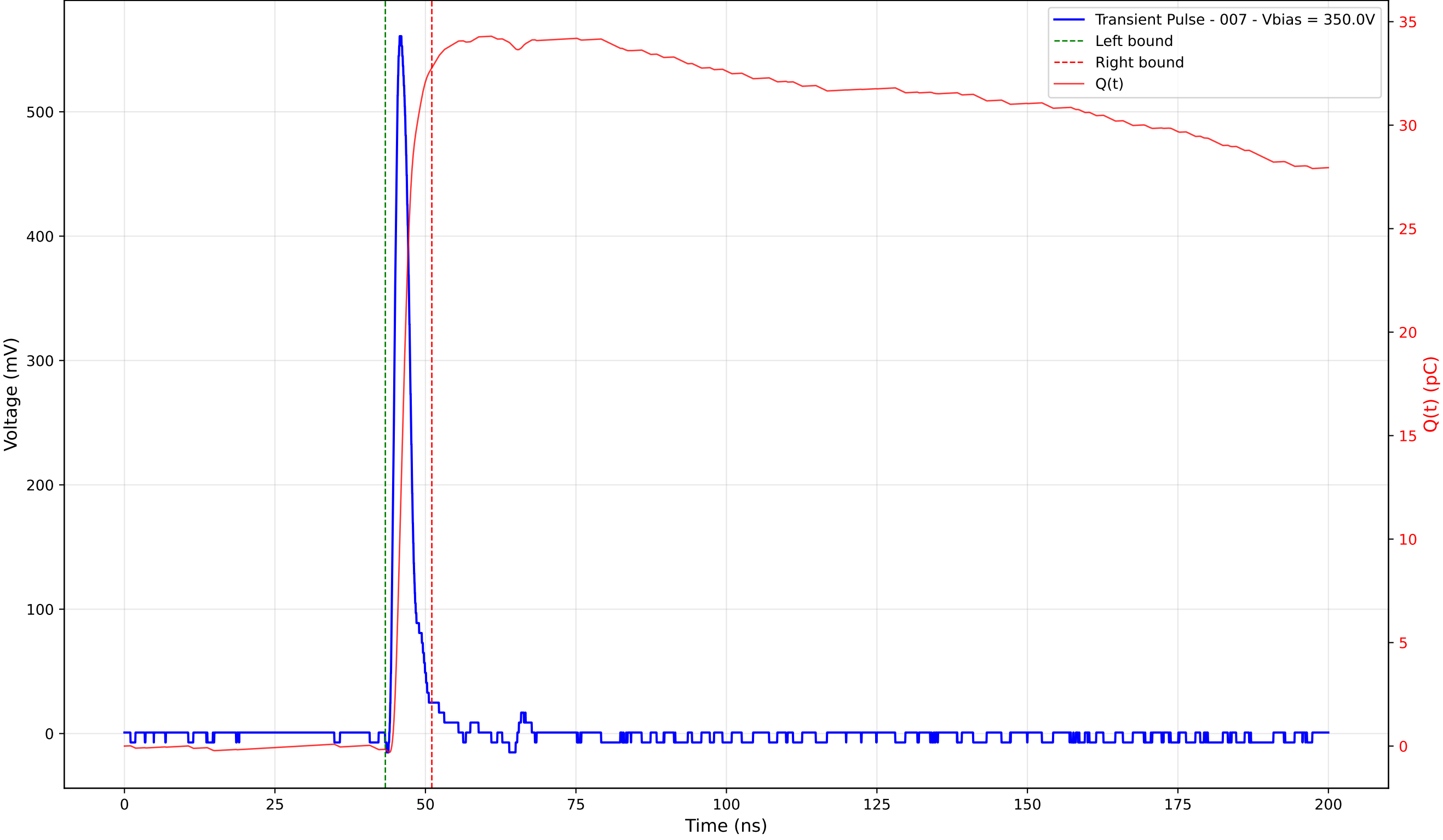
Transient Pulse - Sample: 4003 - Position: 265.0 \mu\text{m} - Charge: 32.93 pC - Rise Time: 1.06 ns
