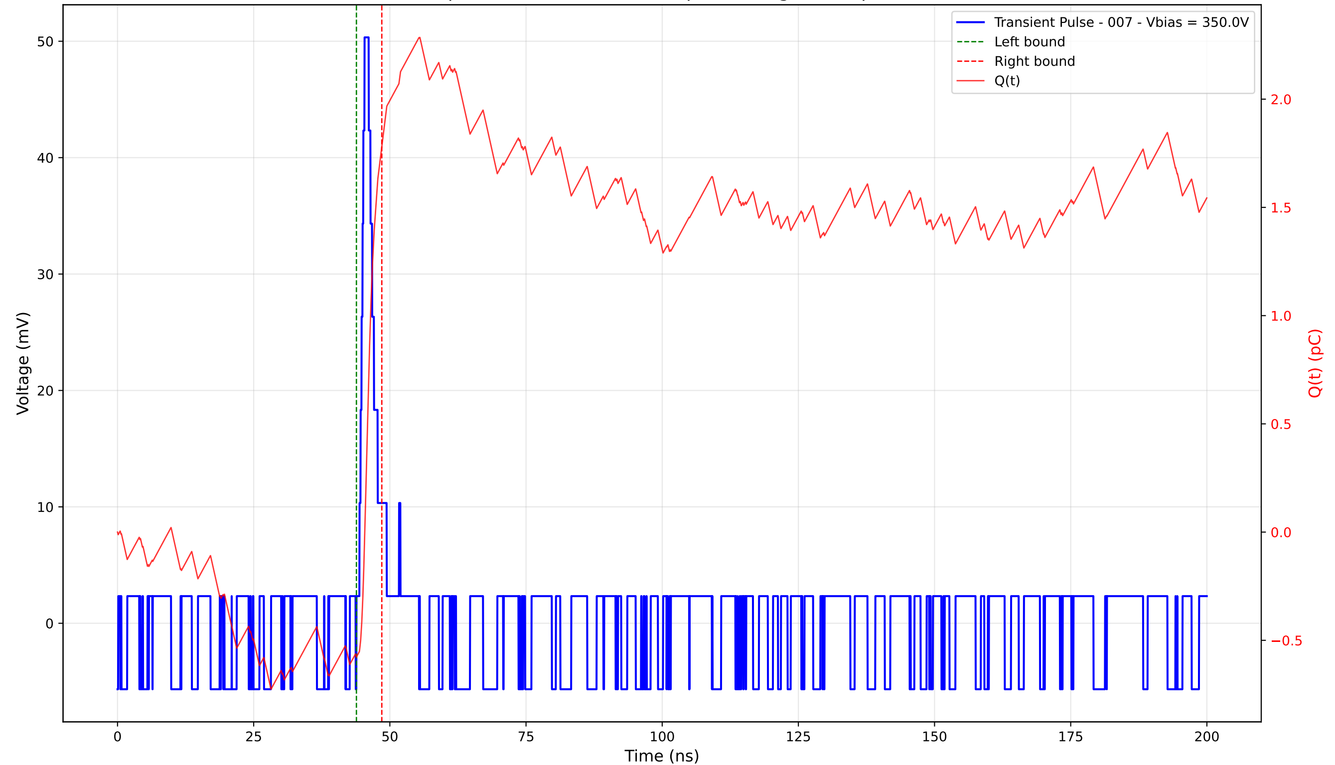
Transient Pulse - Sample: 4003 - Position: 40.0 \mu\text{m} - Charge: 2.36 pC - Rise Time: 0.93 ns
