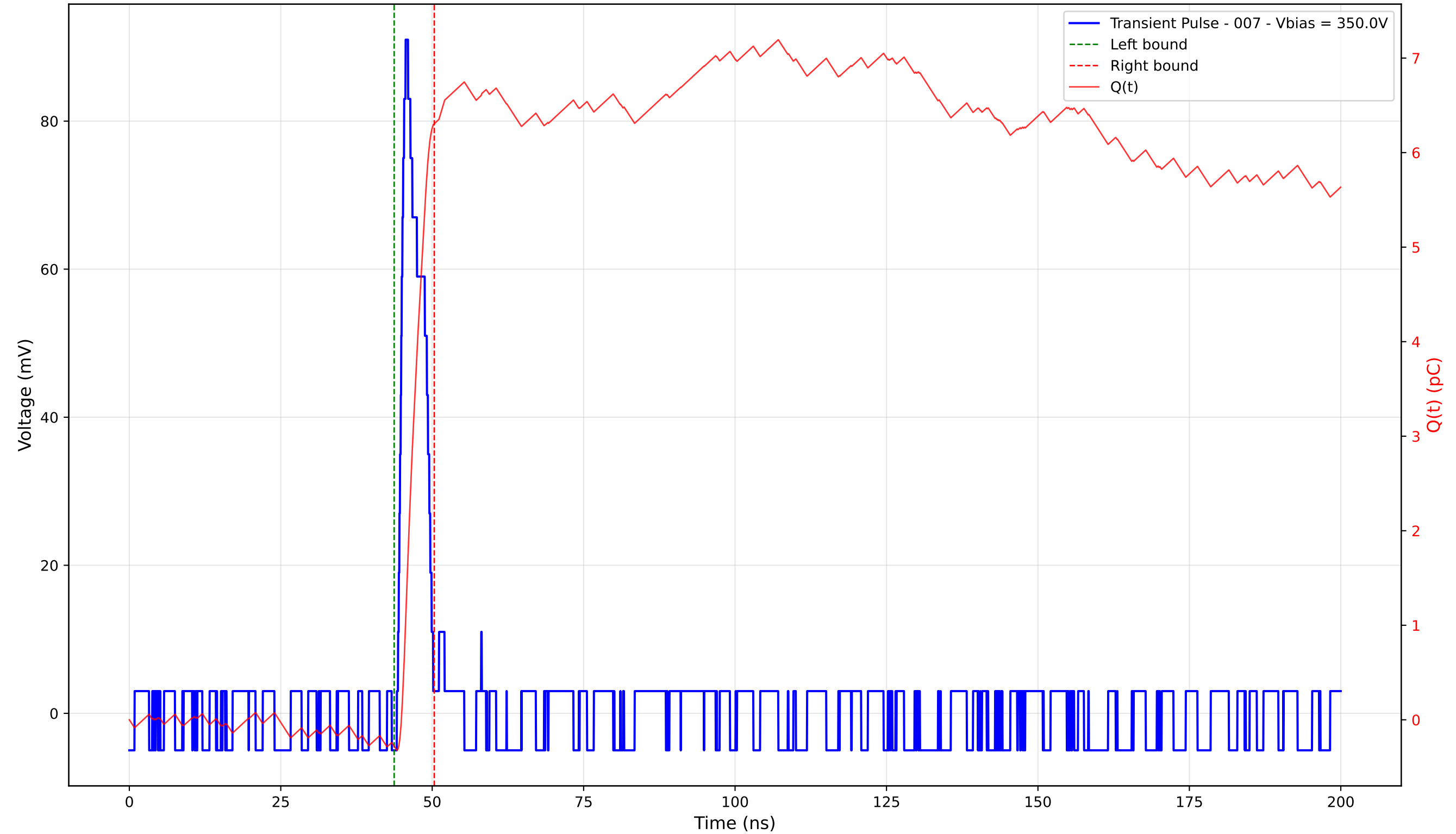
Transient Pulse - Sample: 4003 - Position: 405.0 \mu\text{m} - Charge: 6.58 pC - Rise Time: 1.00 ns
