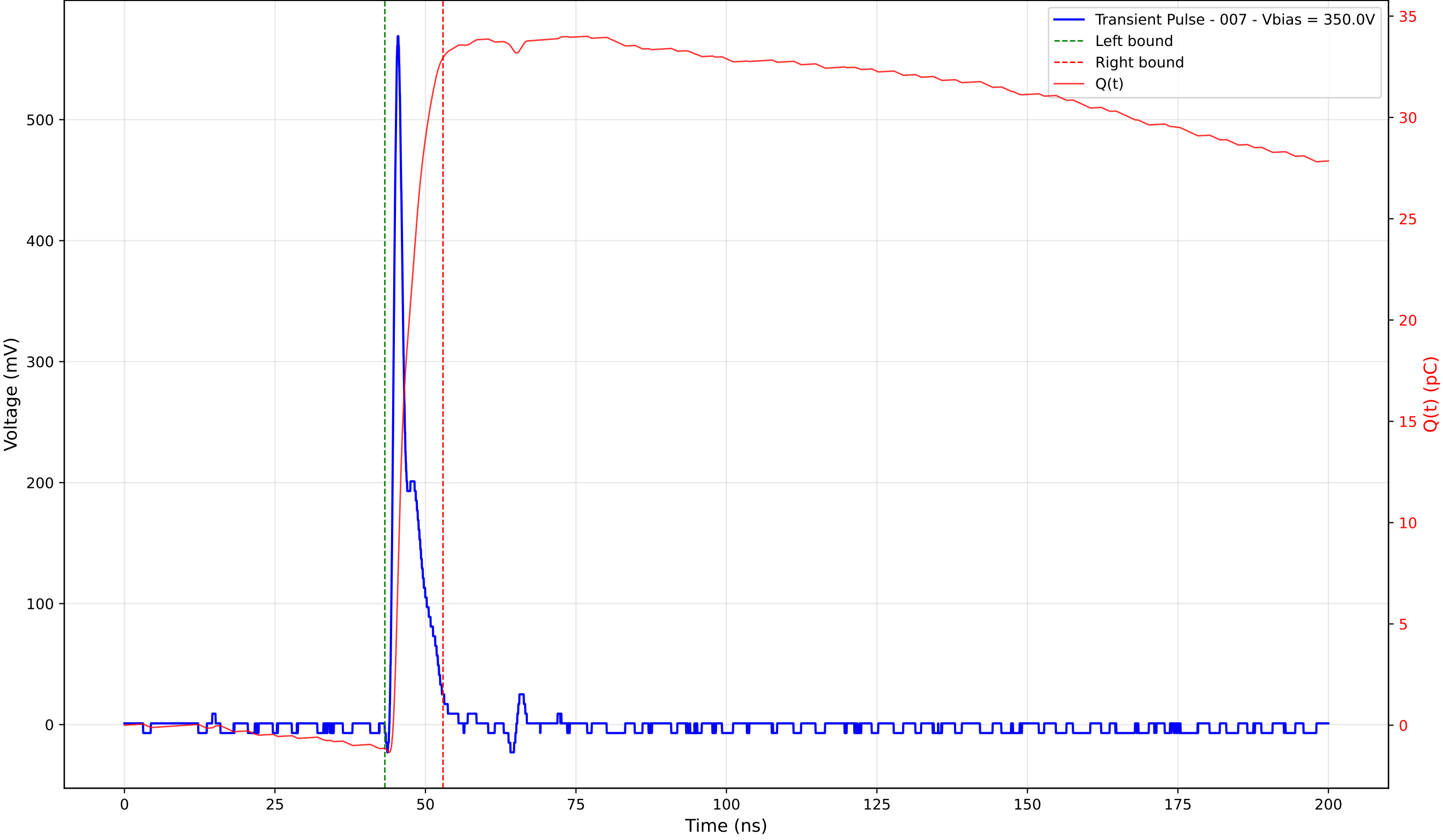
Transient Pulse - Sample: 4003 - Position: 115.0 \mu\text{m} - Charge: 34.09 pC - Rise Time: 0.88 ns
