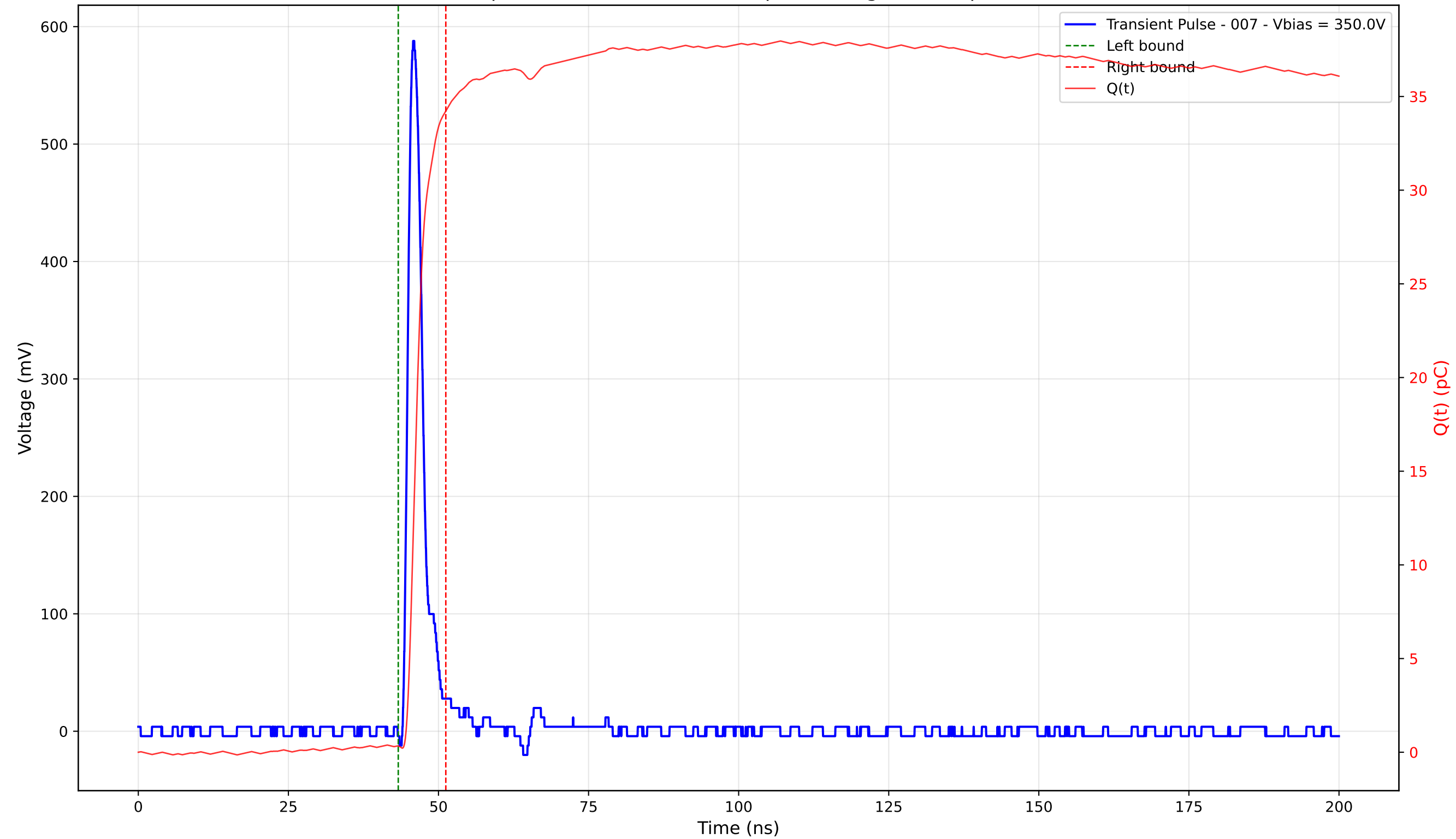
Transient Pulse - Sample: 4003 - Position: 255.0 \mu\text{m} - Charge: 33.89 pC - Rise Time: 1.10 ns
