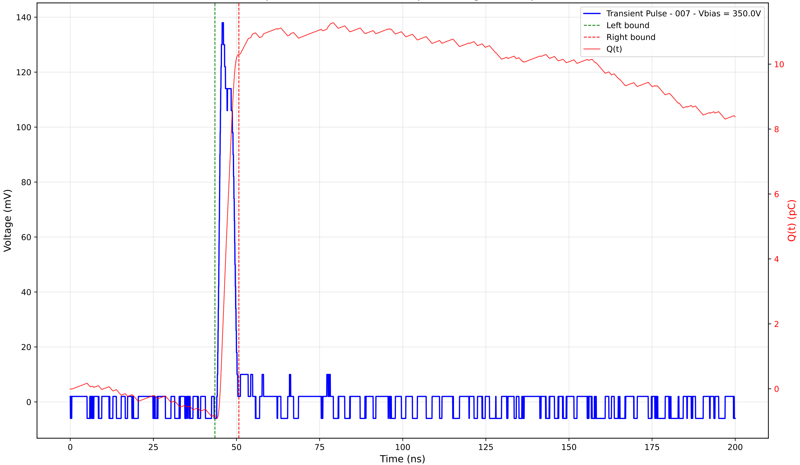
Transient Pulse - Sample: 4003 - Position: 400.0 \mu\text{m} - Charge: 11.15 pC - Rise Time: 1.11 ns
