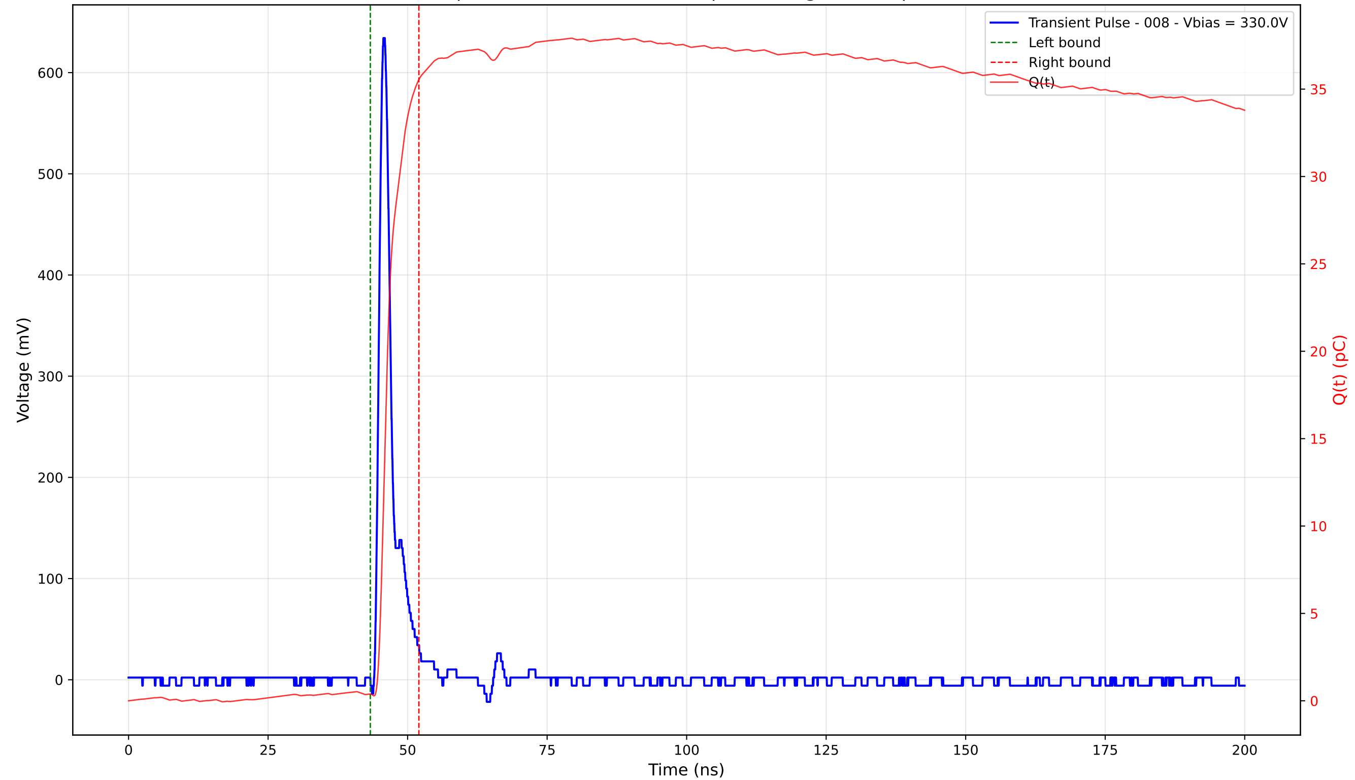
Transient Pulse - Sample: 4003 - Position: 220.0 \mu\text{m} - Charge: 35.16 pC - Rise Time: 1.07 ns
