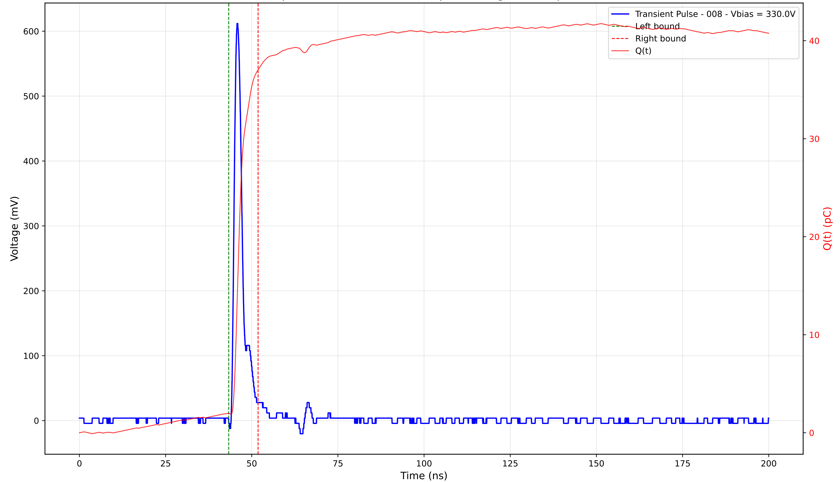
Transient Pulse - Sample: 4003 - Position: 240.0 \mu\text{m} - Charge: 35.04 pC - Rise Time: 1.08 ns
