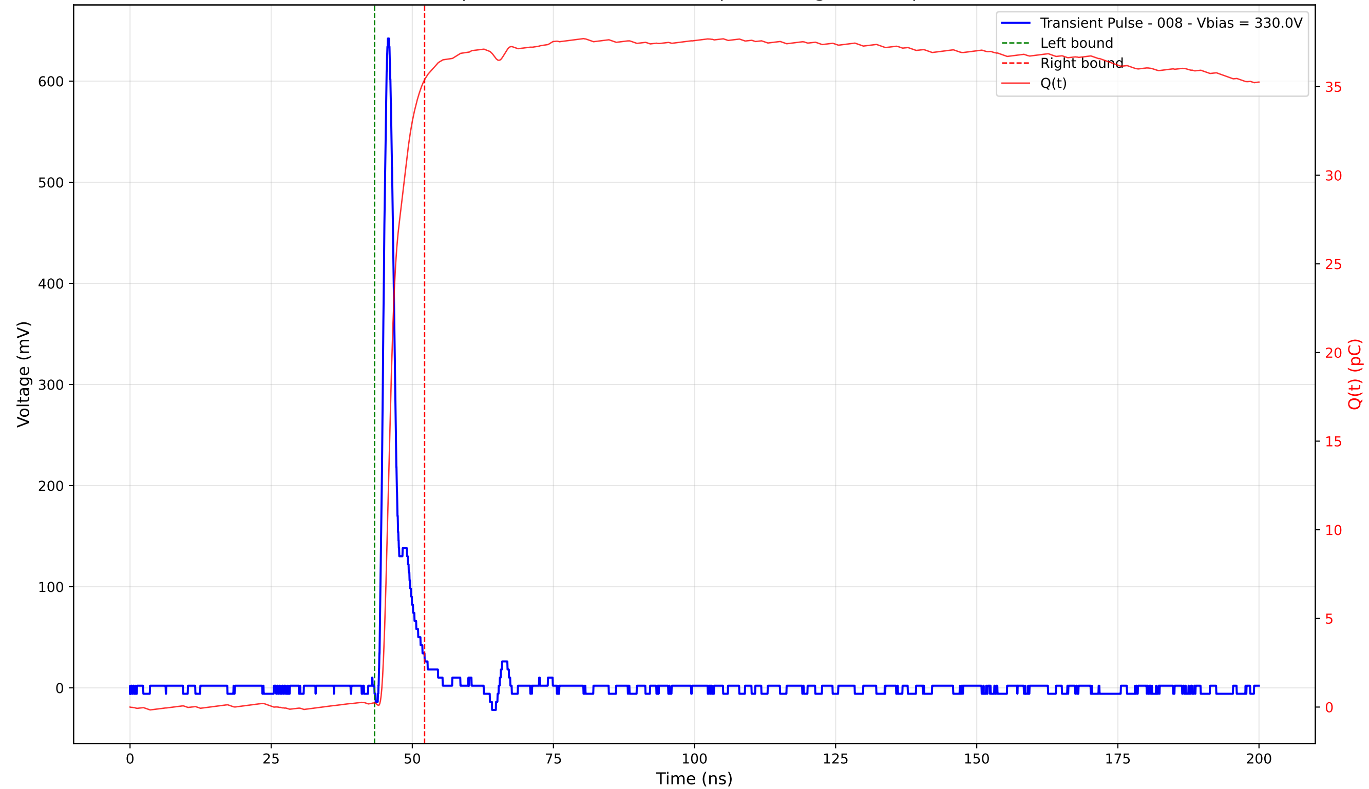
Transient Pulse - Sample: 4003 - Position: 215.0 \mu\text{m} - Charge: 35.16 pC - Rise Time: 1.04 ns
