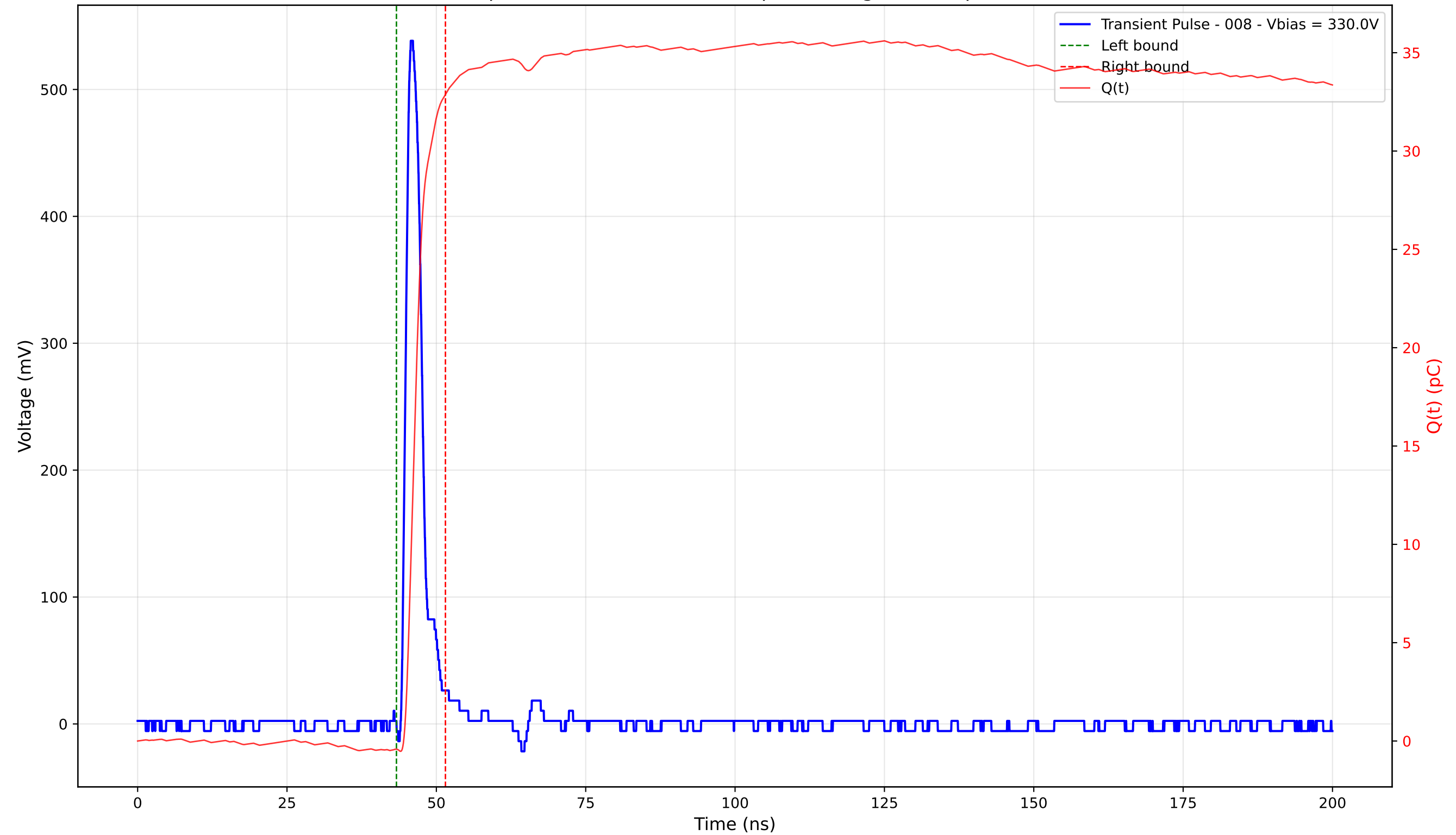
Transient Pulse - Sample: 4003 - Position: 270.0 \mu\text{m} - Charge: 33.29 pC - Rise Time: 1.09 ns
