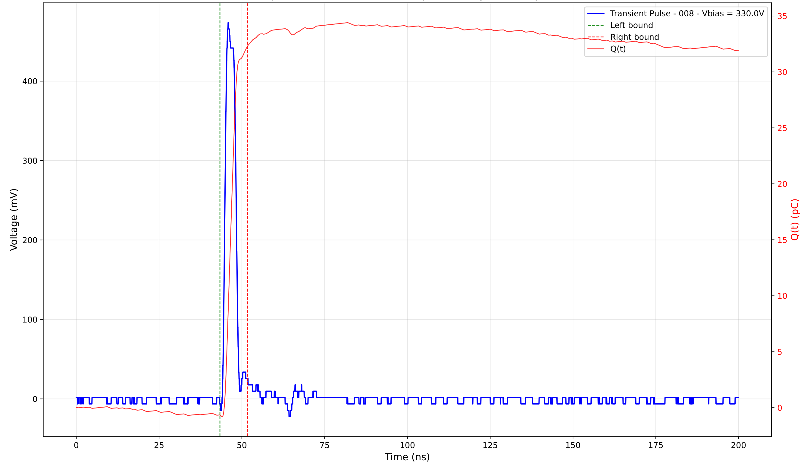
Transient Pulse - Sample: 4003 - Position: 315.0 \mu\text{m} - Charge: 33.00 pC - Rise Time: 1.13 ns
