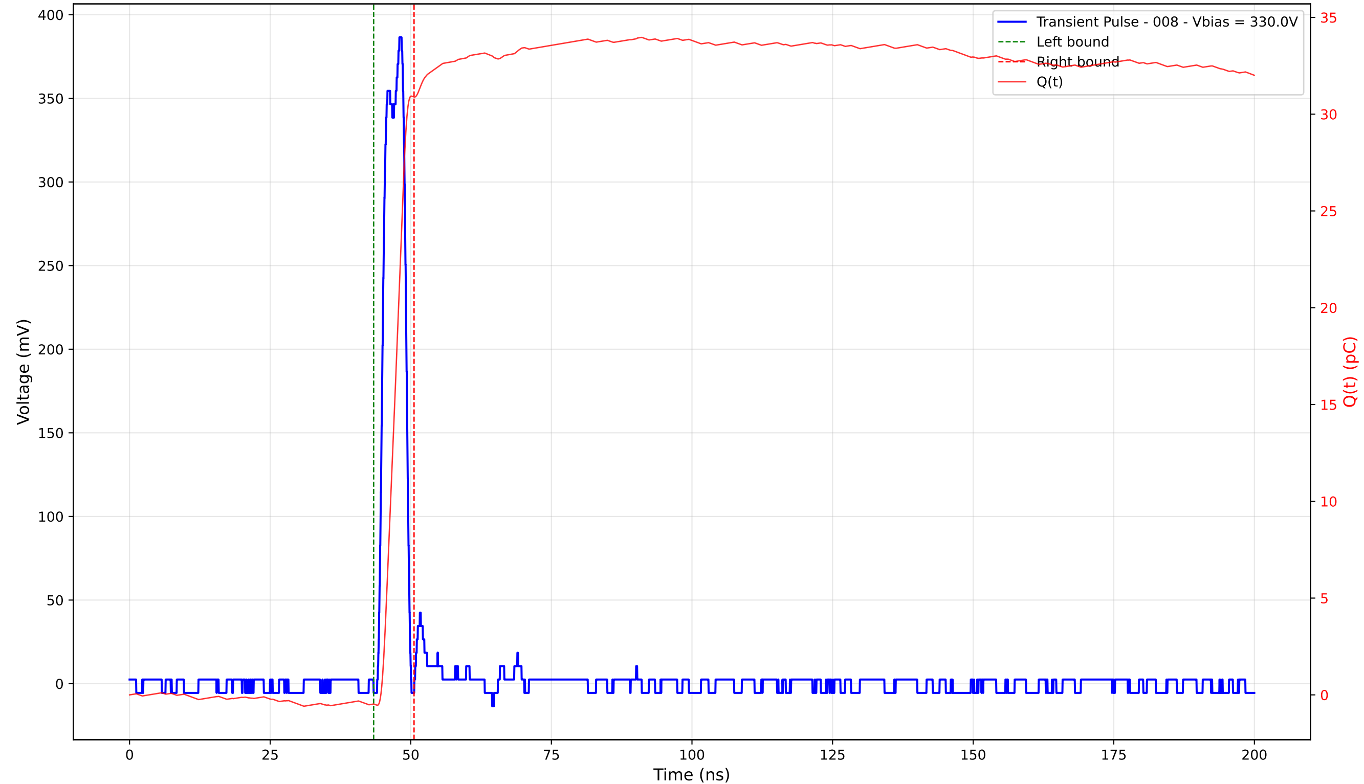
Transient Pulse - Sample: 4003 - Position: 365.0 \mu\text{m} - Charge: 31.36 pC - Rise Time: 1.47 ns
