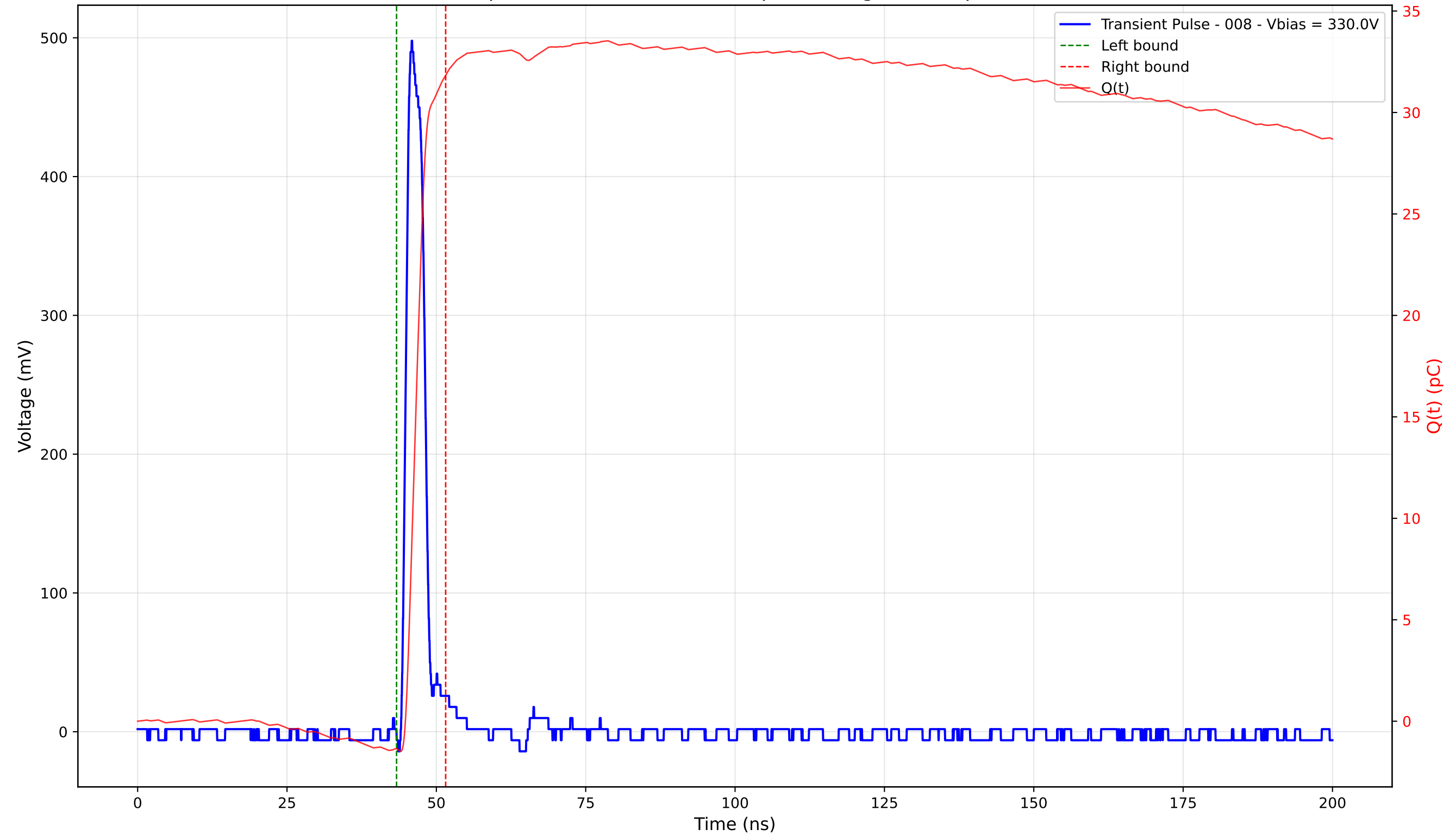
Transient Pulse - Sample: 4003 - Position: 305.0 \mu\text{m} - Charge: 33.19 pC - Rise Time: 1.08 ns
