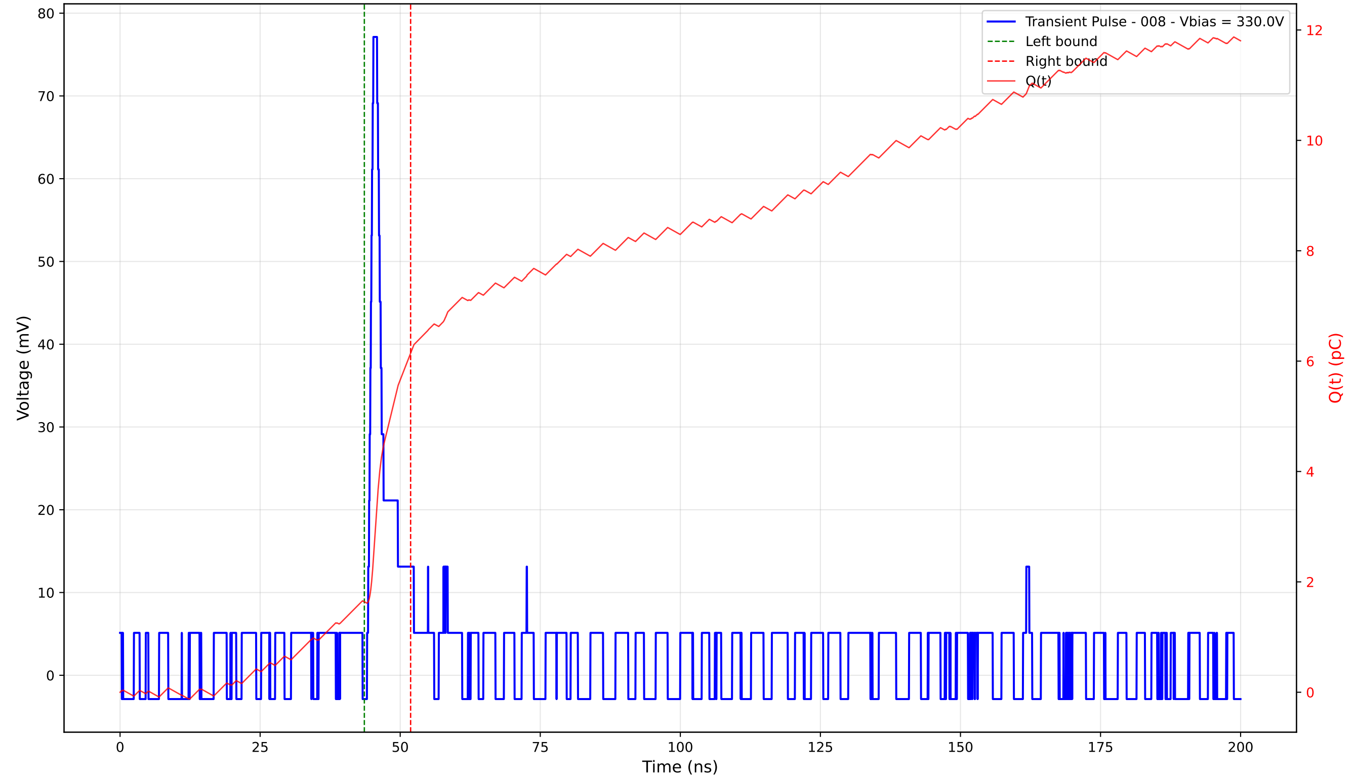
Transient Pulse - Sample: 4003 - Position: 80.0 \mu\text{m} - Charge: 4.51 pC - Rise Time: 0.93 ns
