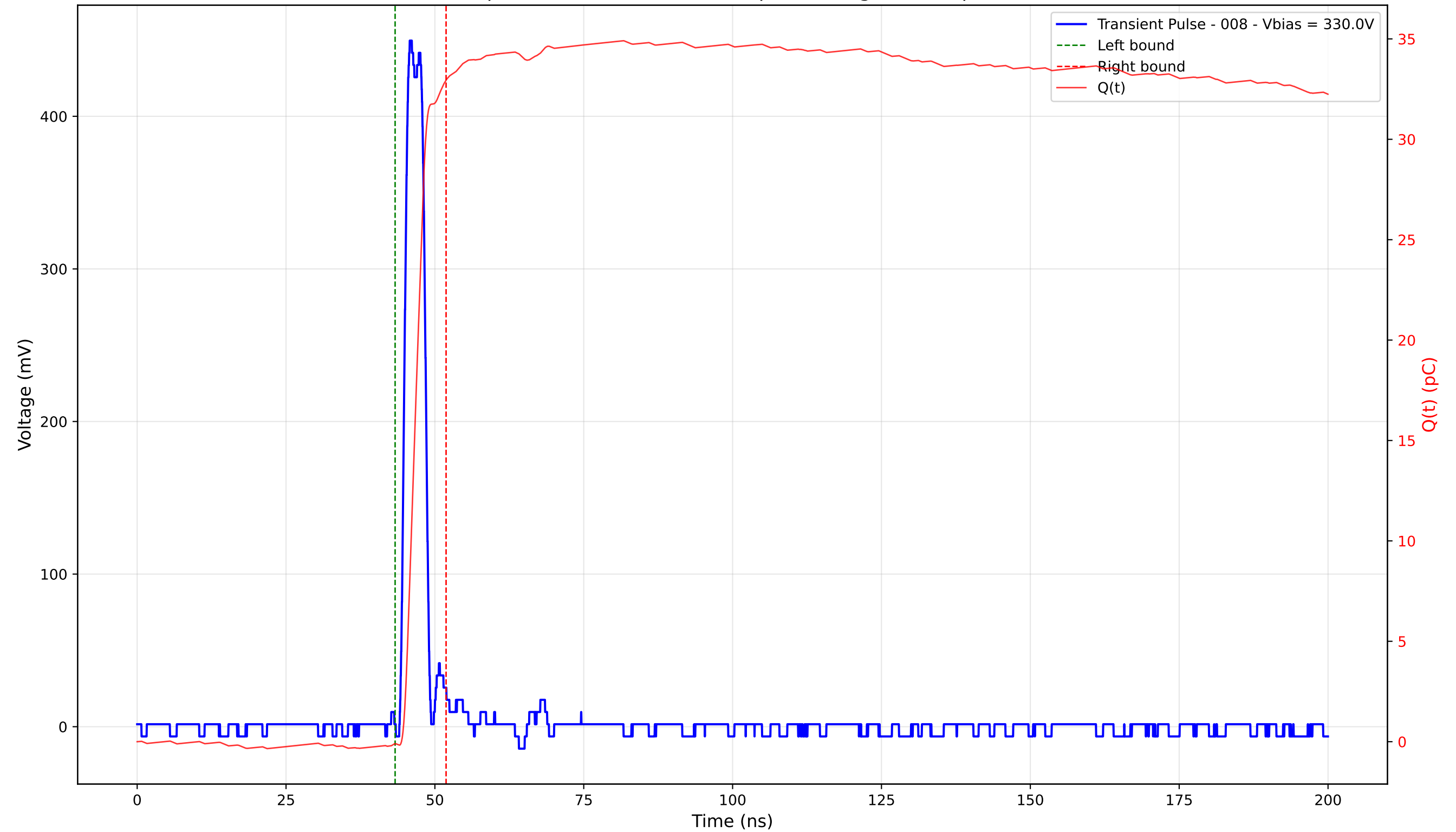
Transient Pulse - Sample: 4003 - Position: 325.0 \mu\text{m} - Charge: 33.06 pC - Rise Time: 1.11 ns
