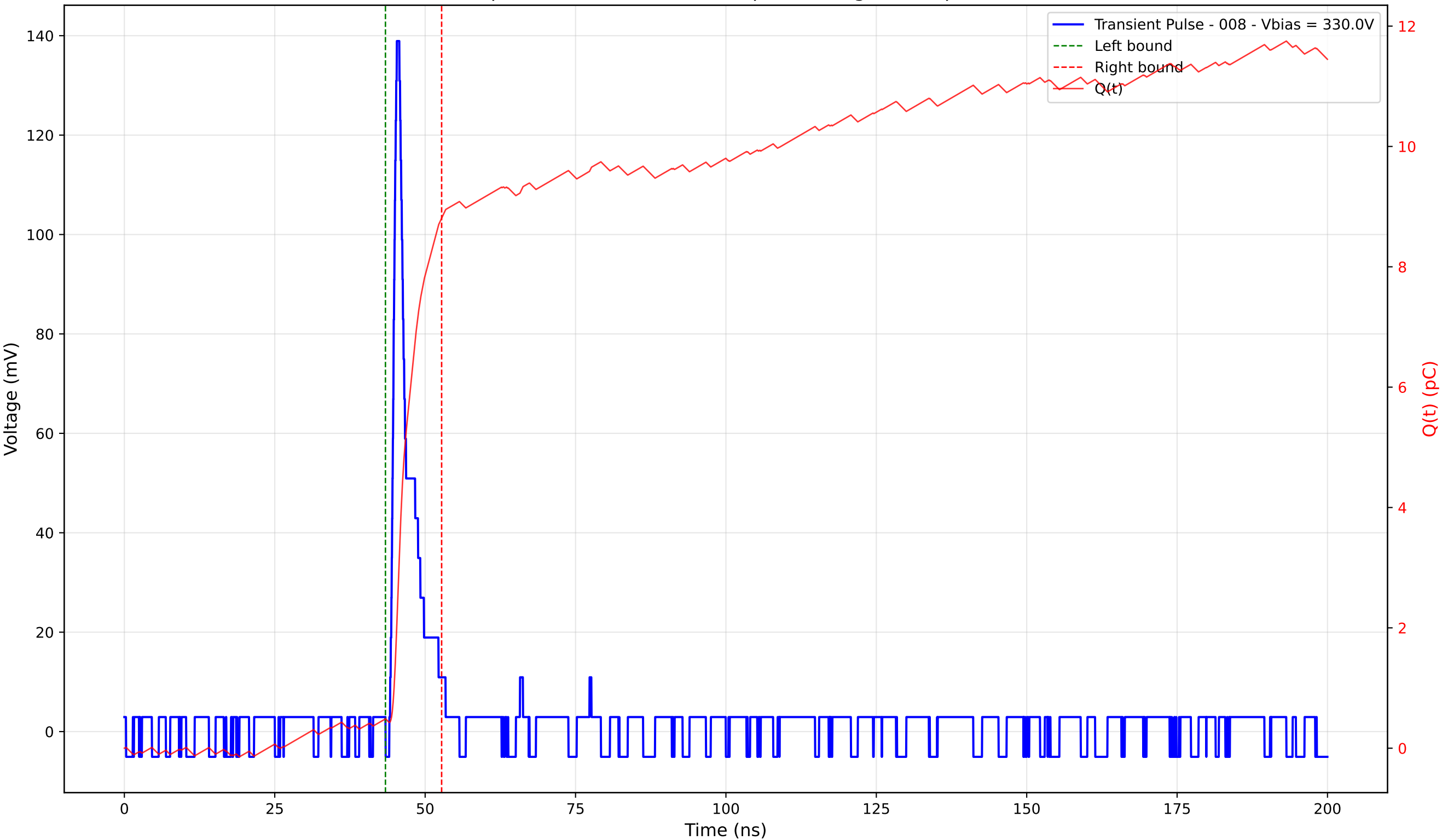
Transient Pulse - Sample: 4003 - Position: 85.0 \mu\text{m} - Charge: 8.32 pC - Rise Time: 0.91 ns
