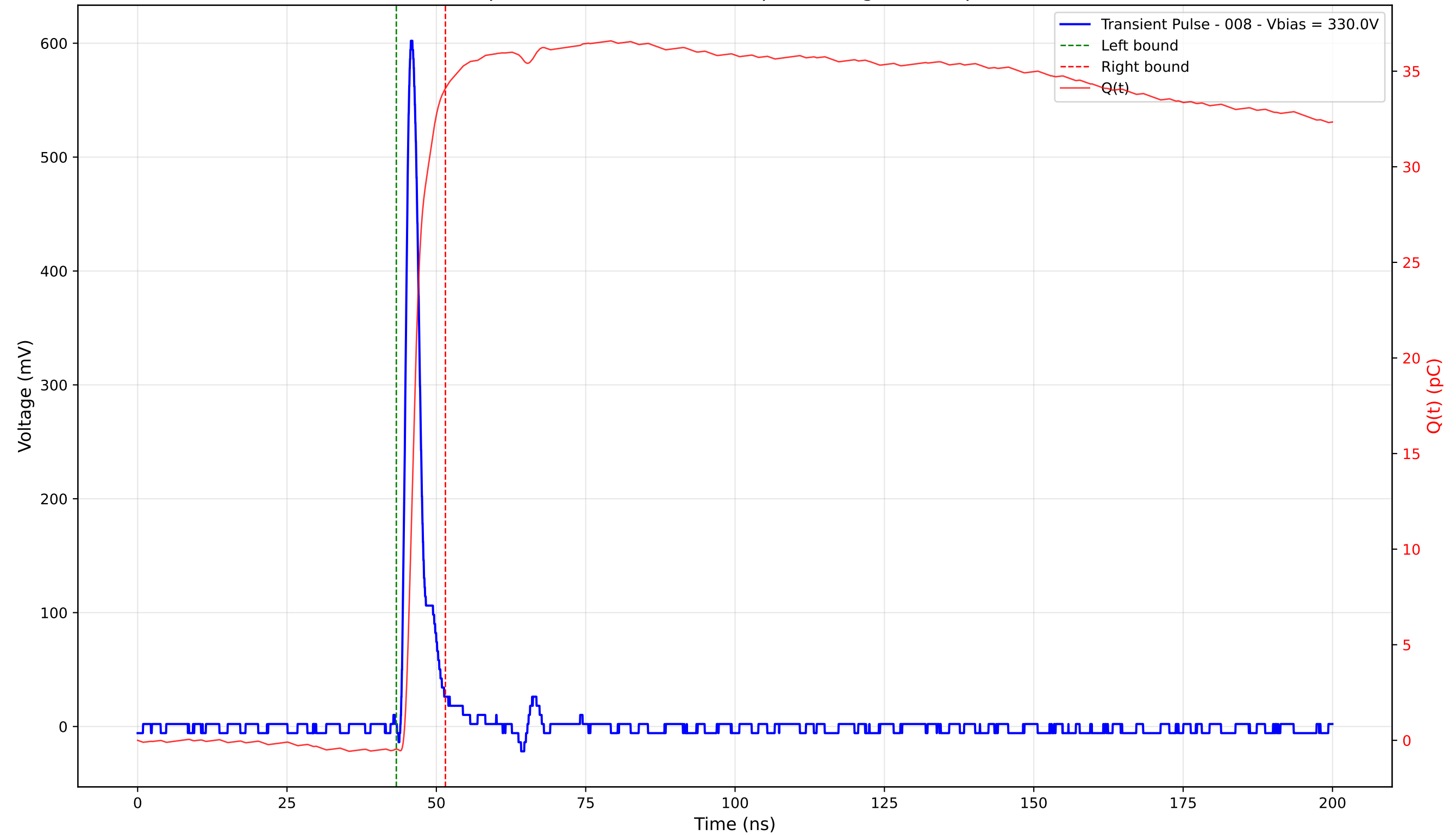
Transient Pulse - Sample: 4003 - Position: 245.0 \mu\text{m} - Charge: 34.56 pC - Rise Time: 1.10 ns
