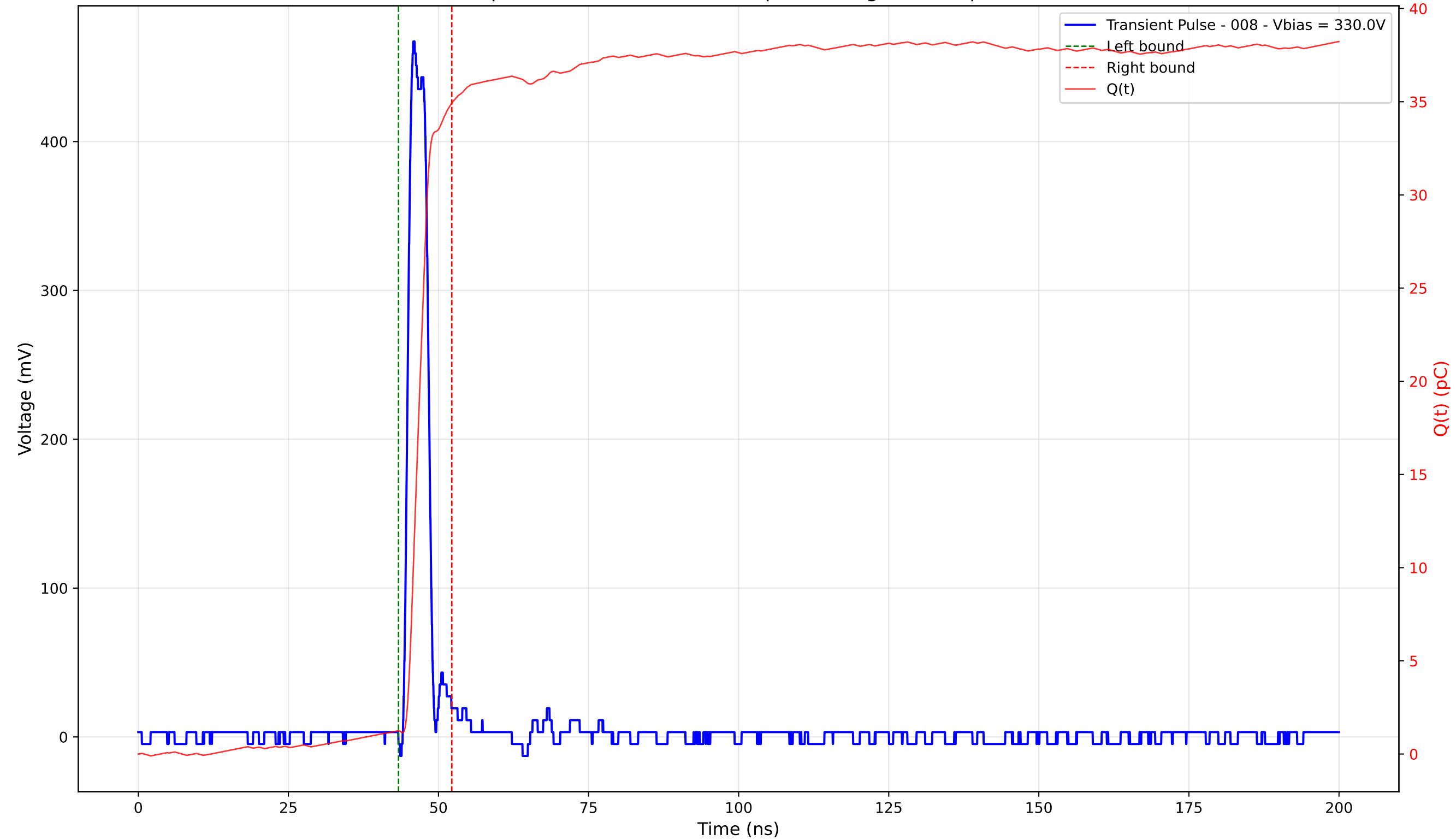
Transient Pulse - Sample: 4003 - Position: 320.0 \mu\text{m} - Charge: 33.68 pC - Rise Time: 1.13 ns
