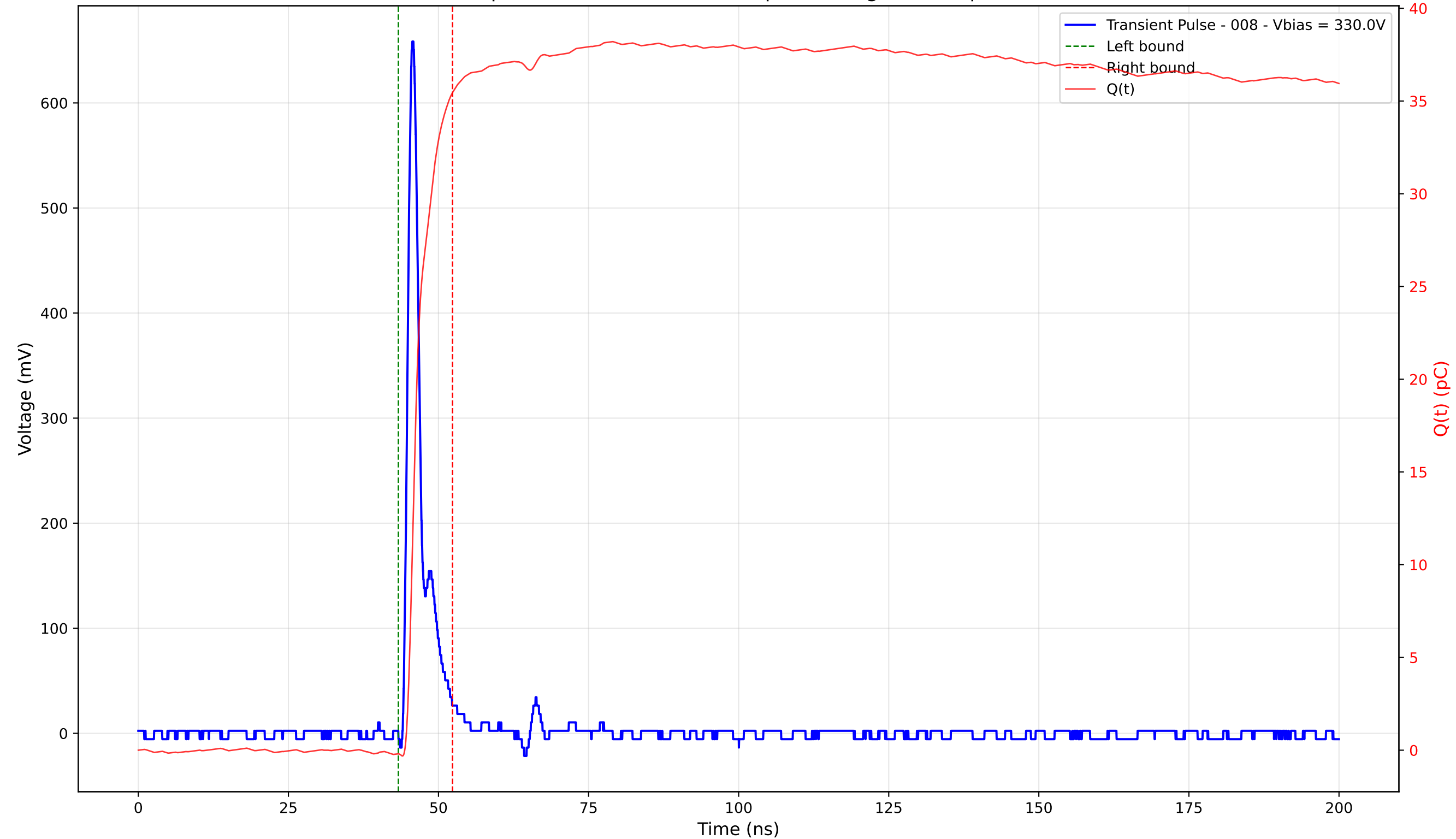
Transient Pulse - Sample: 4003 - Position: 205.0 \mu\text{m} - Charge: 35.64 pC - Rise Time: 1.06 ns
