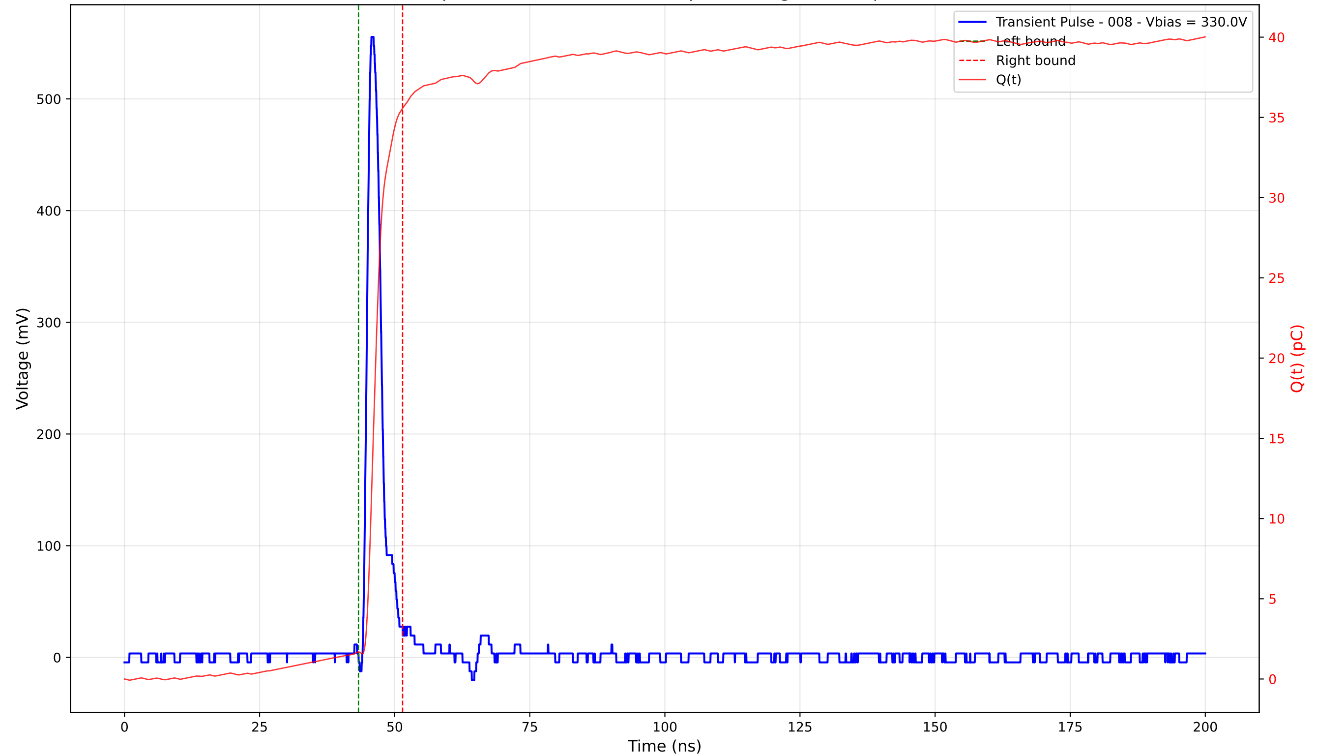
Transient Pulse - Sample: 4003 - Position: 265.0 \mu\text{m} - Charge: 33.89 pC - Rise Time: 1.09 ns
