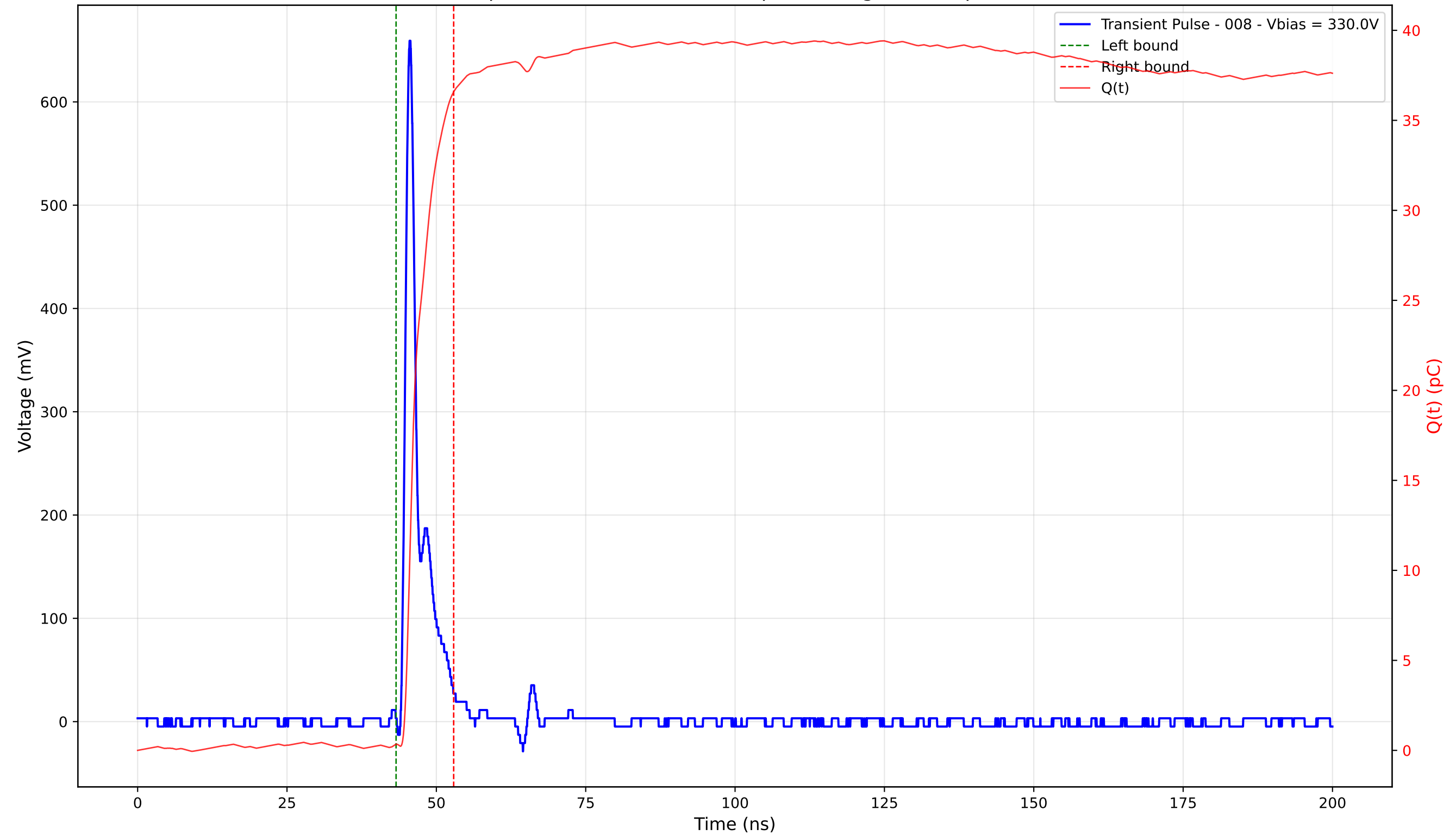
Transient Pulse - Sample: 4003 - Position: 170.0 \mu\text{m} - Charge: 36.25 pC - Rise Time: 0.98 ns
