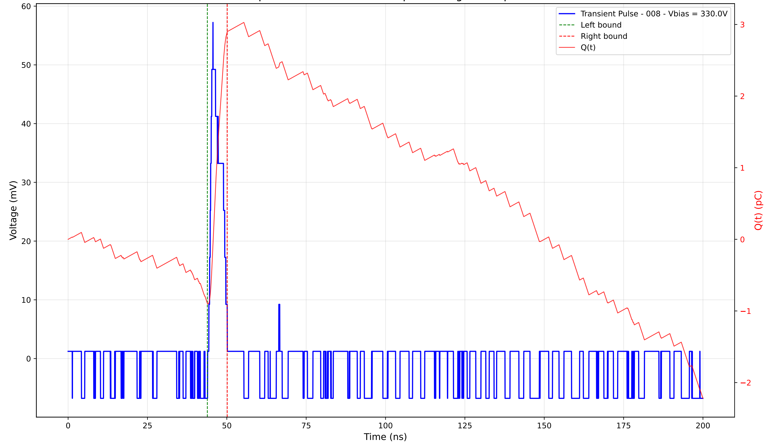
Transient Pulse - Sample: 4003 - Position: 410.0 \mu\text{m} - Charge: 3.79 pC - Rise Time: 1.29 ns
