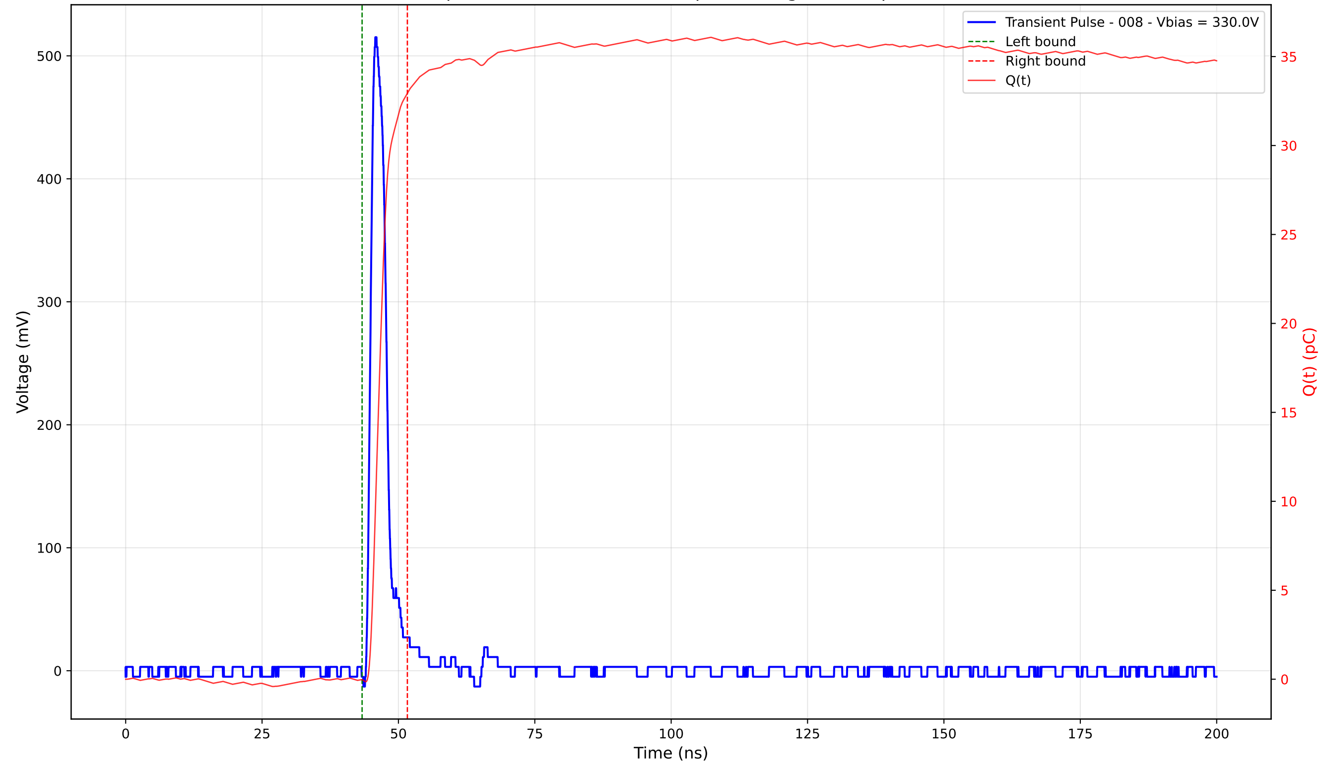
Transient Pulse - Sample: 4003 - Position: 285.0 \mu\text{m} - Charge: 32.97 pC - Rise Time: 1.09 ns
