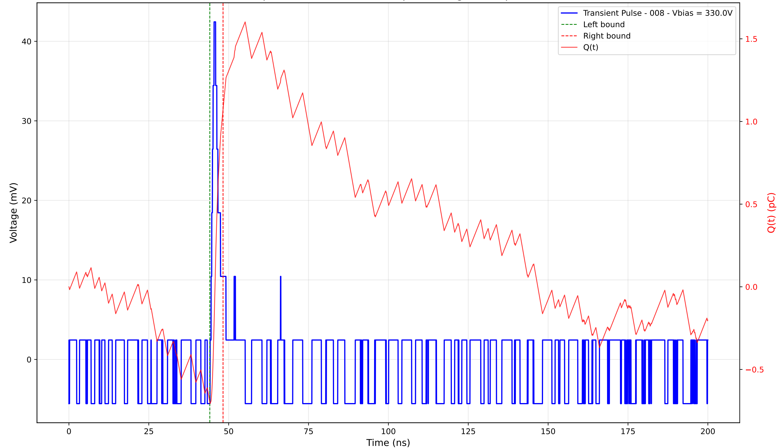
Transient Pulse - Sample: 4003 - Position: 25.0 \mu\text{m} - Charge: 1.77 pC - Rise Time: 0.94 ns
