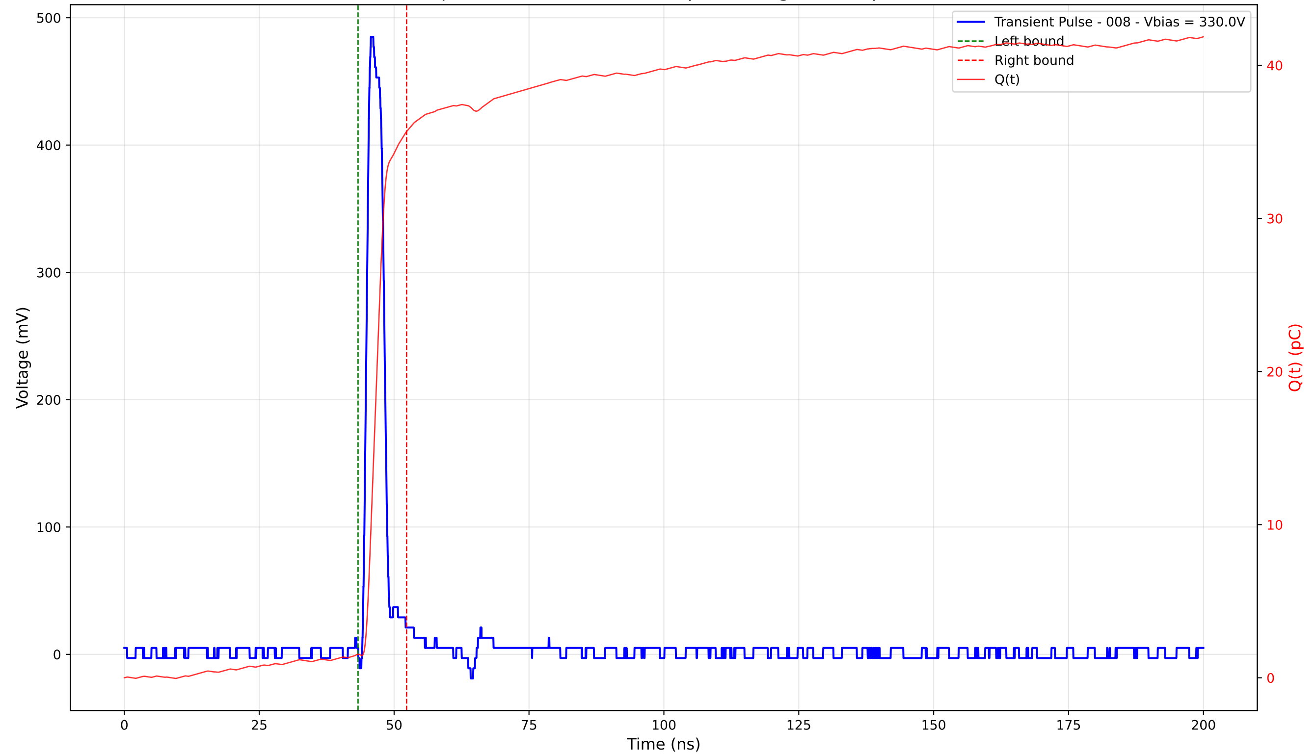
Transient Pulse - Sample: 4003 - Position: 310.0 \mu\text{m} - Charge: 34.13 pC - Rise Time: 1.07 ns
