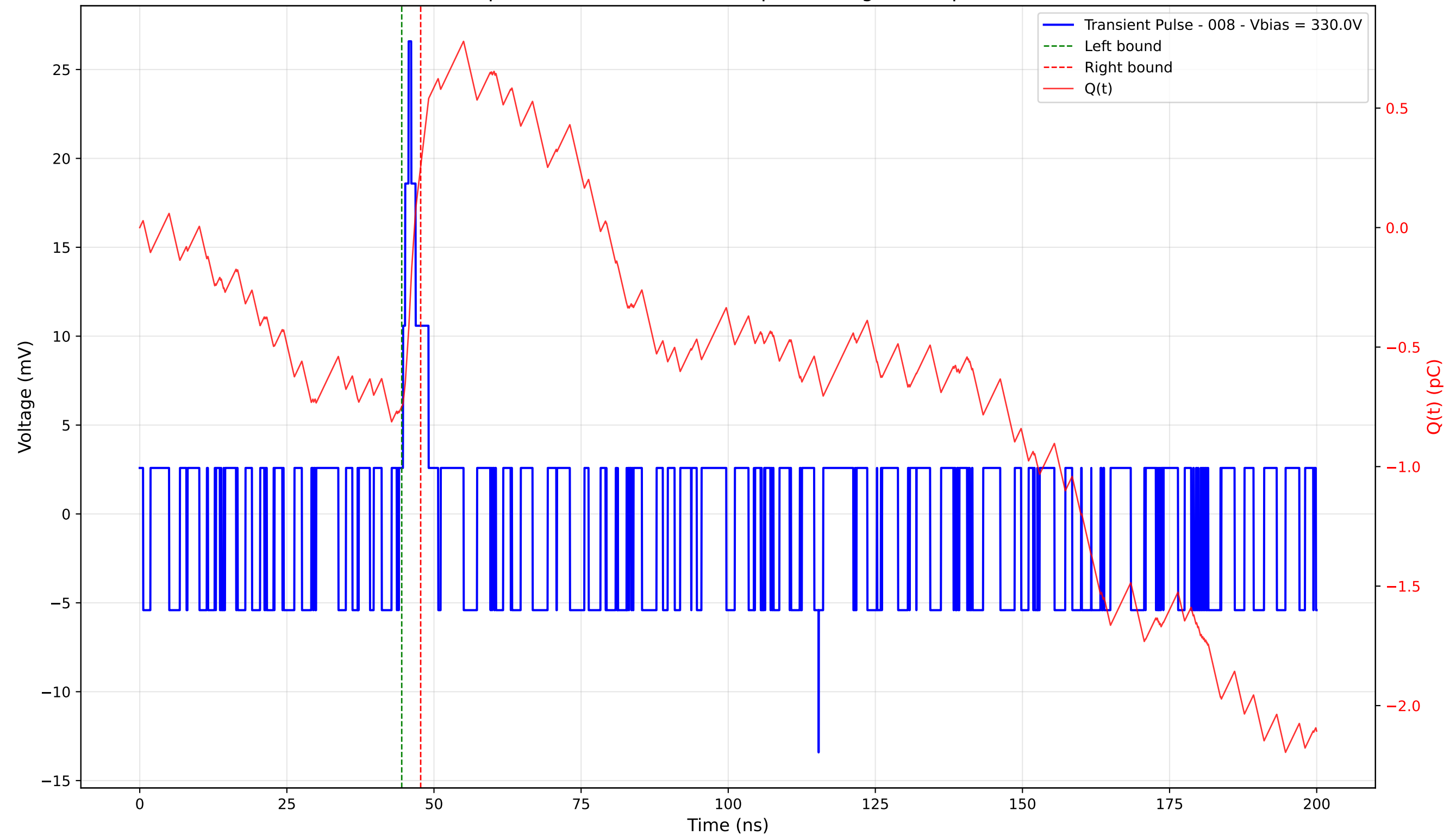
Transient Pulse - Sample: 4003 - Position: 420.0 \mu\text{m} - Charge: 1.01 pC - Rise Time: 0.96 ns
