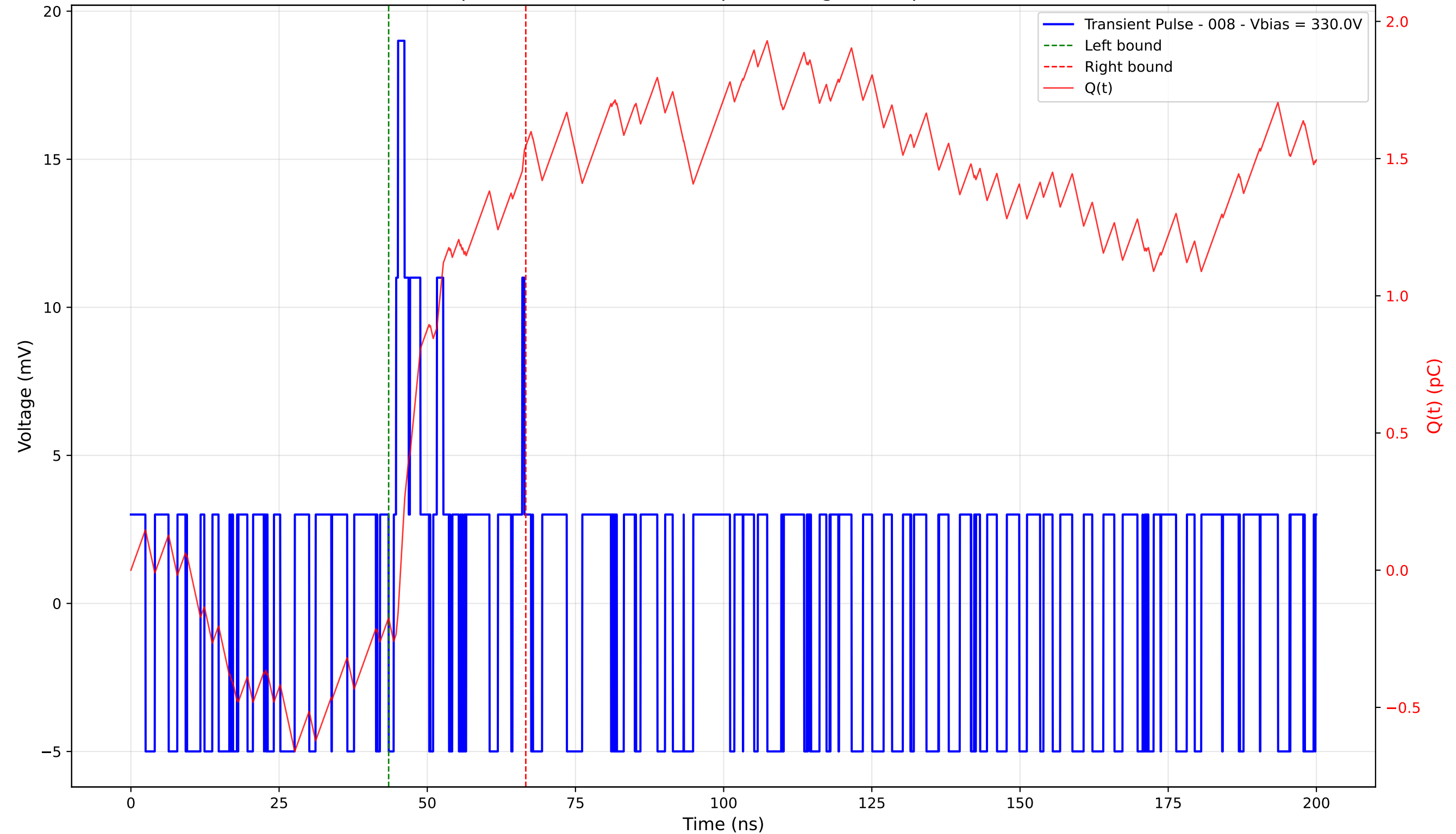
Transient Pulse - Sample: 4003 - Position: 65.0 \mu\text{m} - Charge: 1.72 pC - Rise Time: 0.00 ns (N/A)
