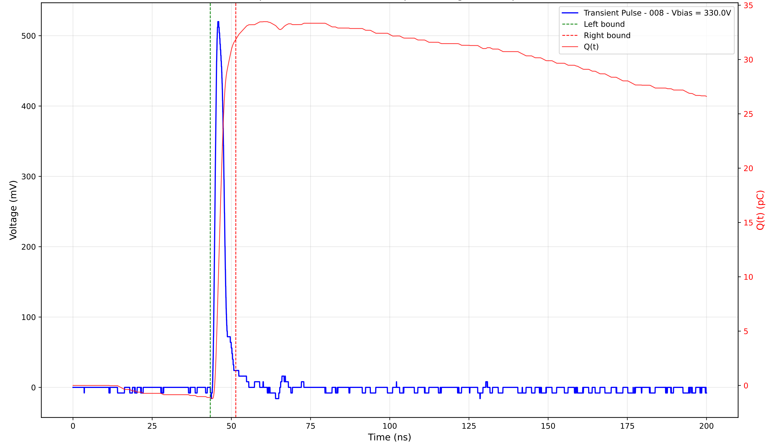
Transient Pulse - Sample: 4003 - Position: 280.0 \mu\text{m} - Charge: 32.96 pC - Rise Time: 1.09 ns
