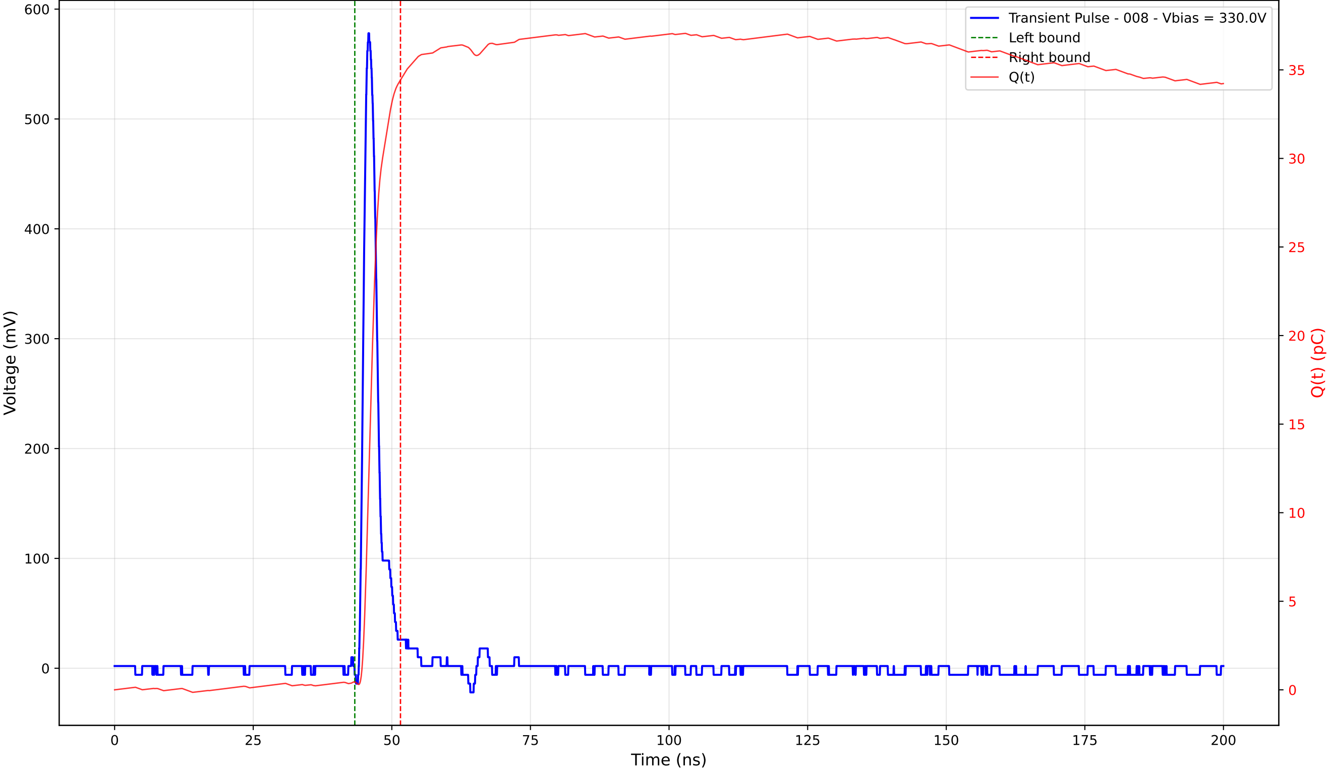
Transient Pulse - Sample: 4003 - Position: 255.0 \mu\text{m} - Charge: 33.99 pC - Rise Time: 1.08 ns
