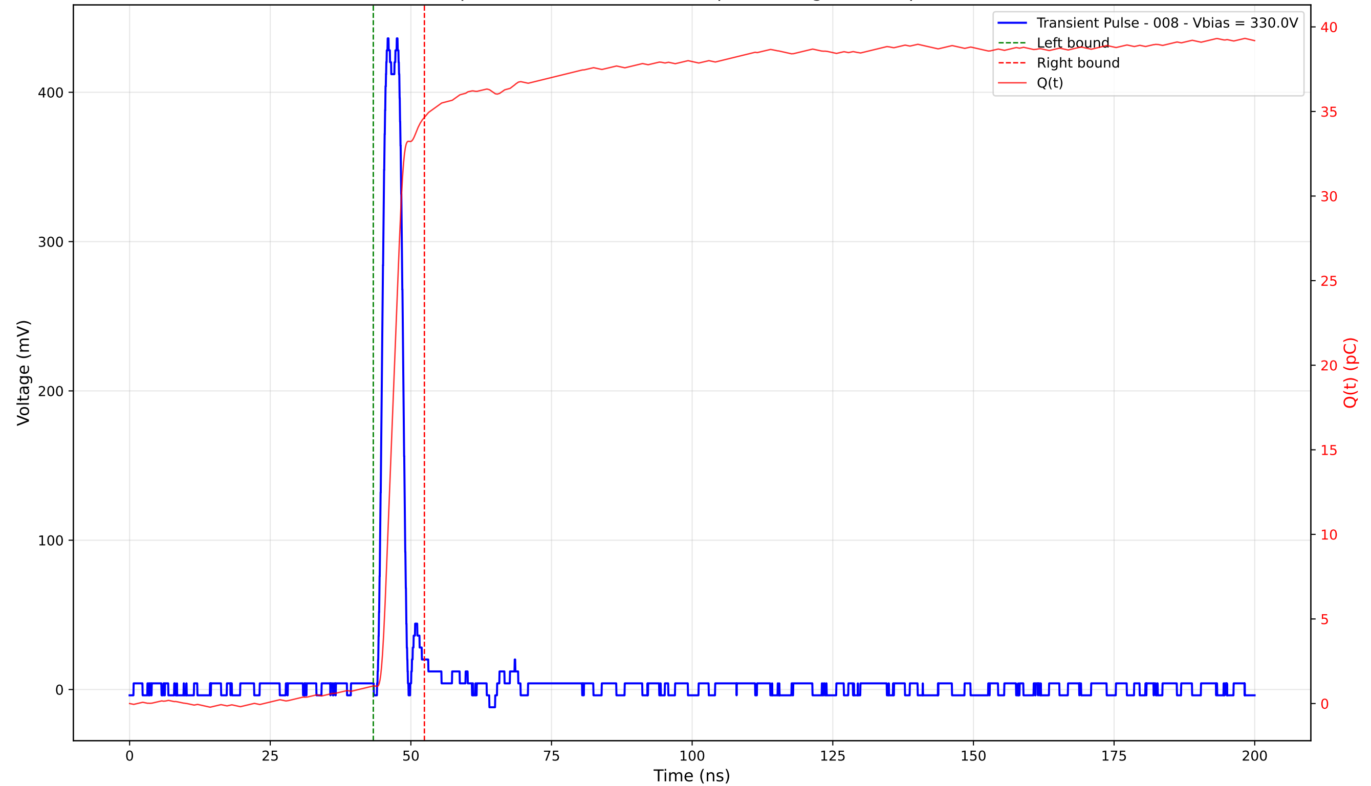
Transient Pulse - Sample: 4003 - Position: 335.0 \mu\text{m} - Charge: 33.61 pC - Rise Time: 1.16 ns
