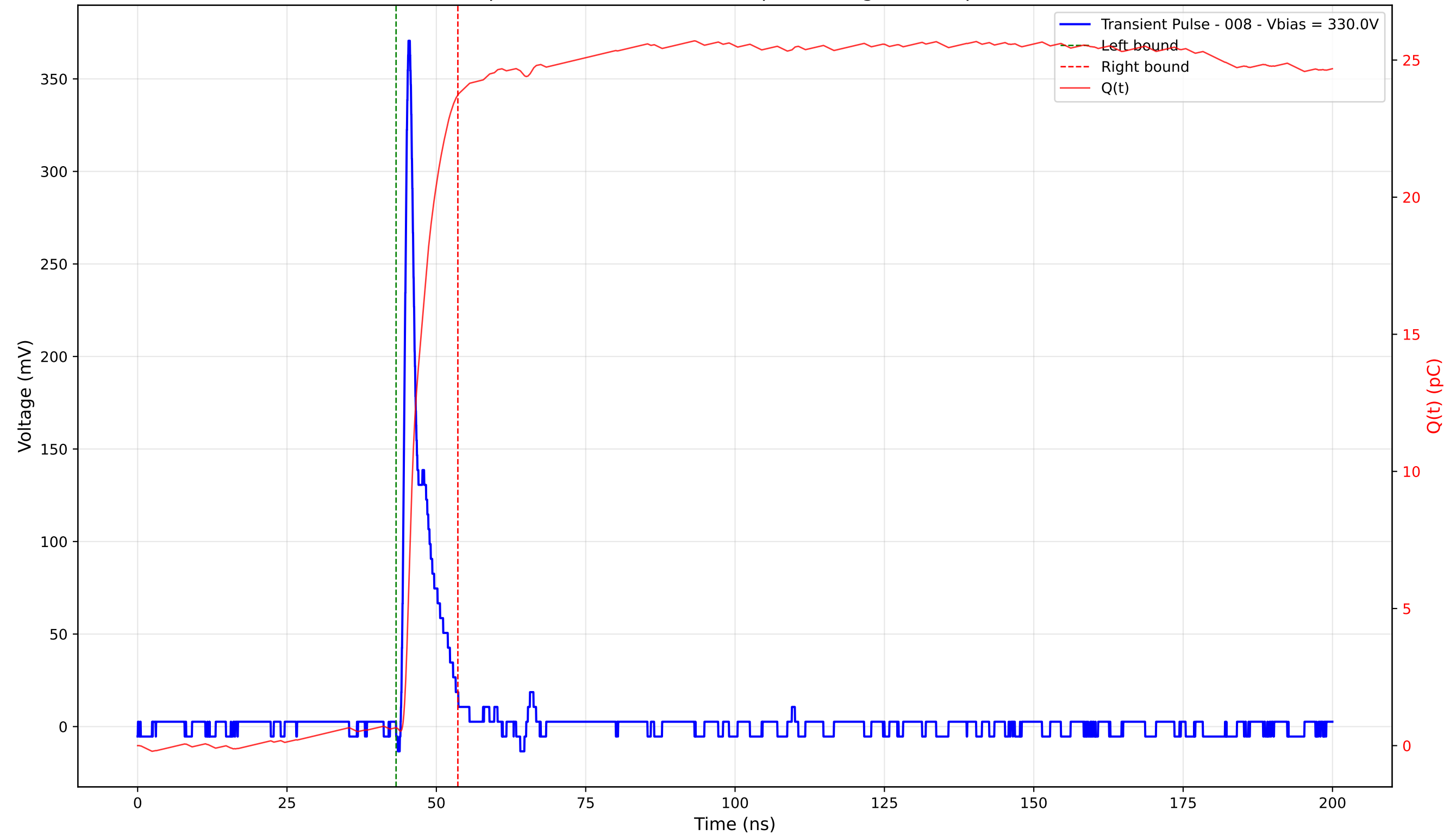
Transient Pulse - Sample: 4003 - Position: 100.0 \mu\text{m} - Charge: 23.07 pC - Rise Time: 0.91 ns
