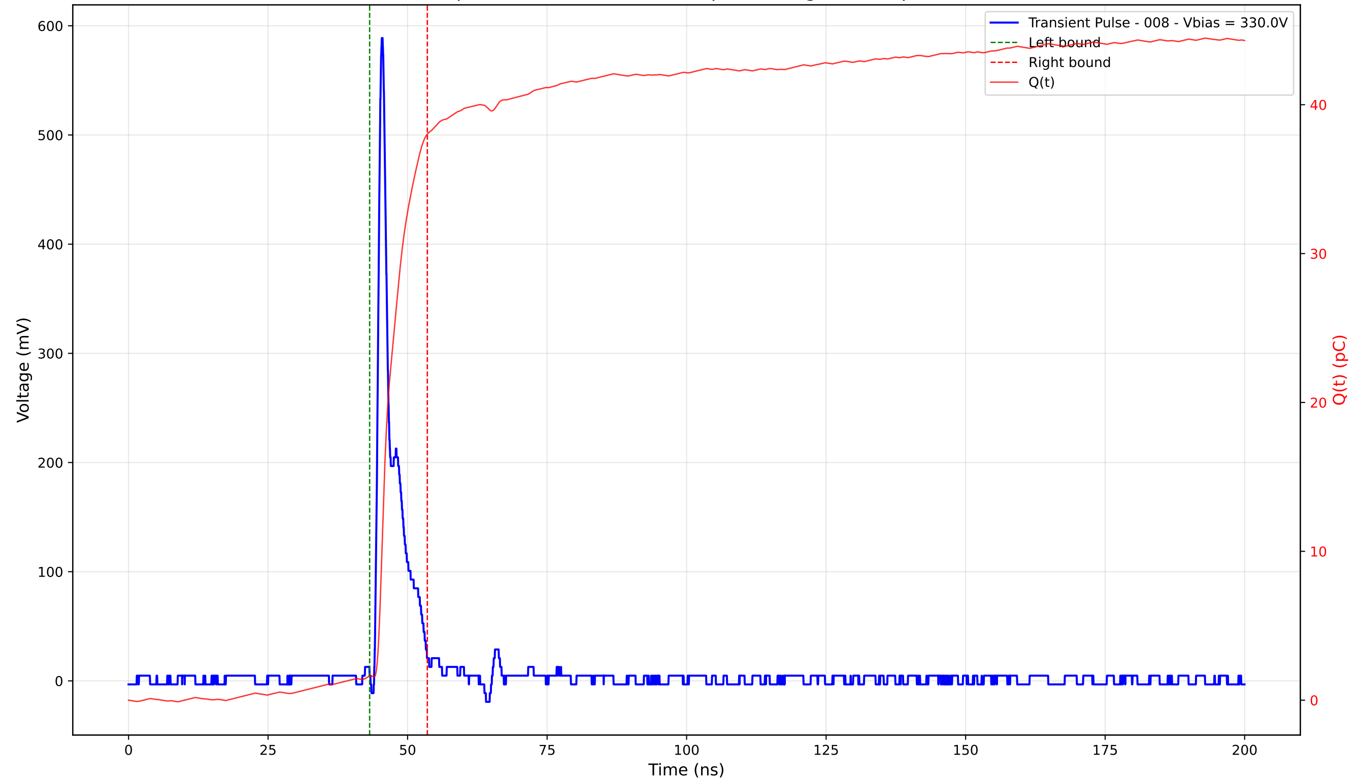
Transient Pulse - Sample: 4003 - Position: 120.0 \mu\text{m} - Charge: 36.38 pC - Rise Time: 0.88 ns
