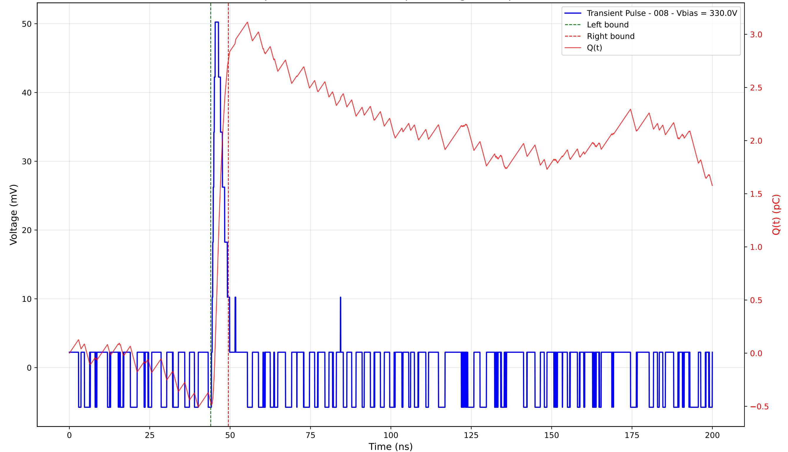
Transient Pulse - Sample: 4003 - Position: 55.0 \mu\text{m} - Charge: 3.22 pC - Rise Time: 0.93 ns
