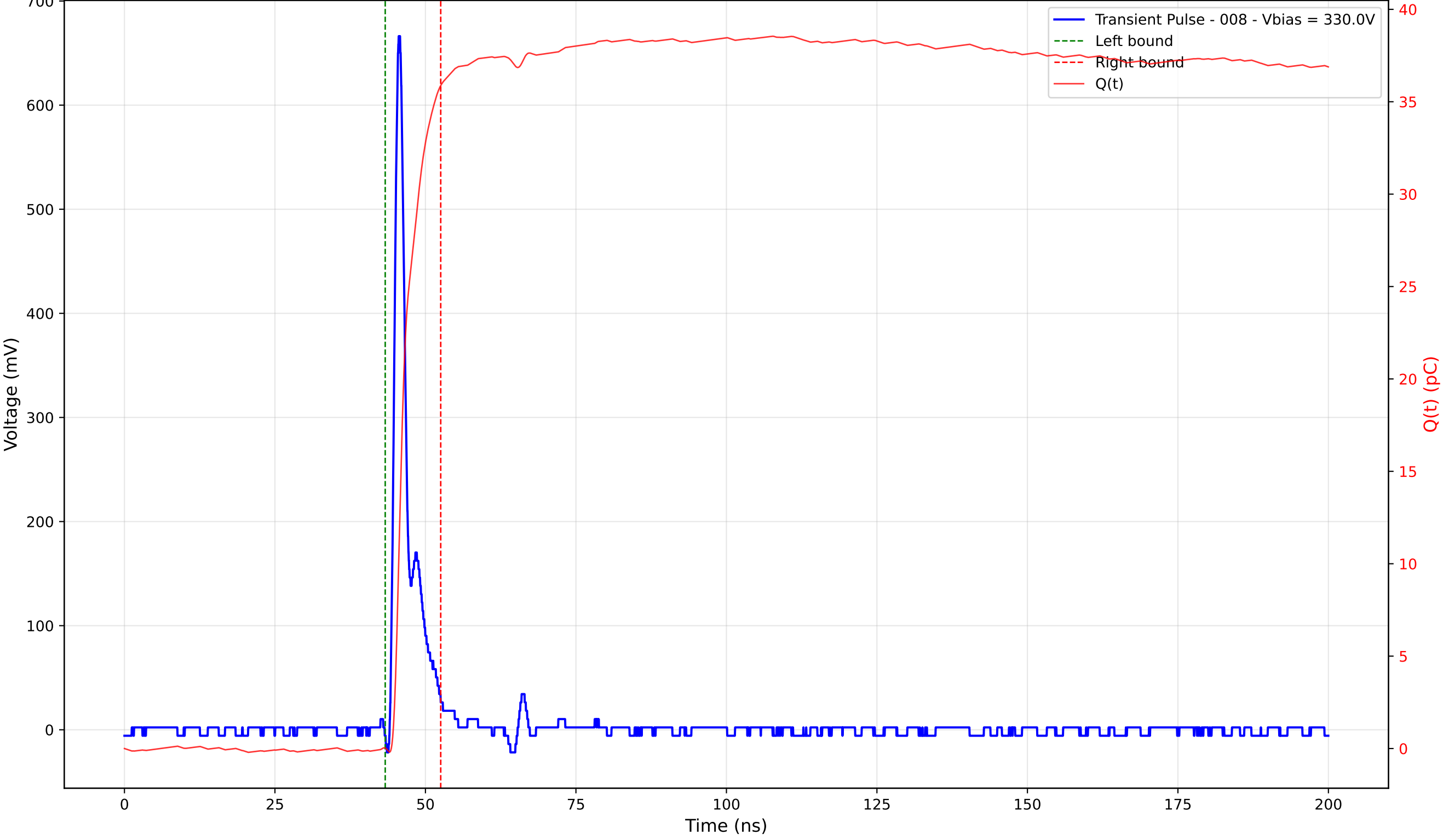
Transient Pulse - Sample: 4003 - Position: 190.0 \mu\text{m} - Charge: 35.85 pC - Rise Time: 0.98 ns
