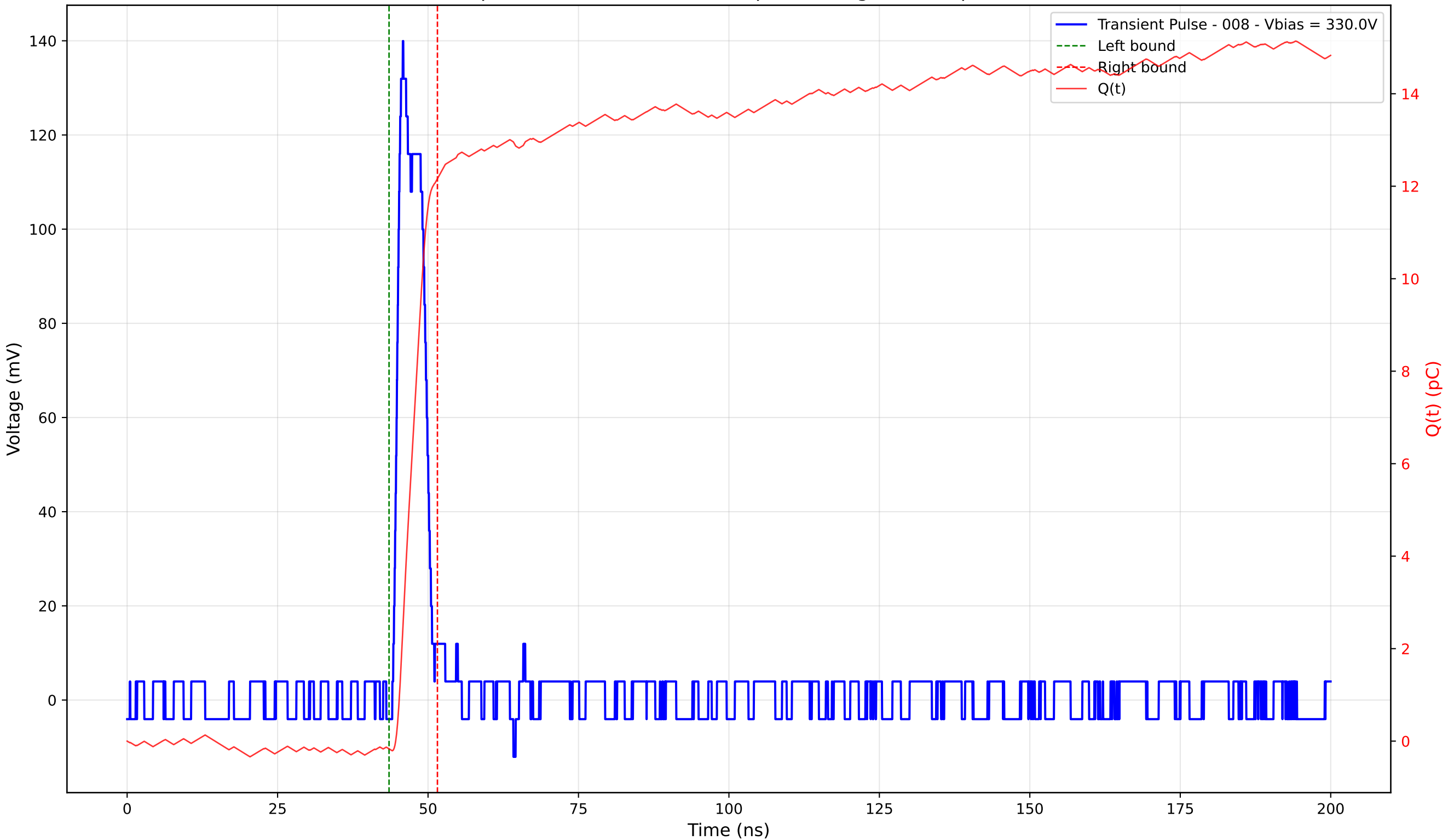
Transient Pulse - Sample: 4003 - Position: 400.0 \mu\text{m} - Charge: 12.33 pC - Rise Time: 1.17 ns
