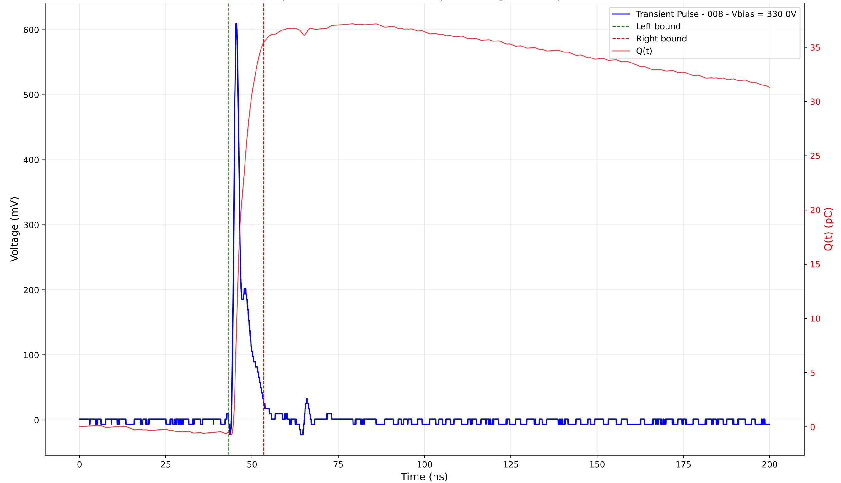
Transient Pulse - Sample: 4003 - Position: 130.0 \mu\text{m} - Charge: 35.96 pC - Rise Time: 0.90 ns
