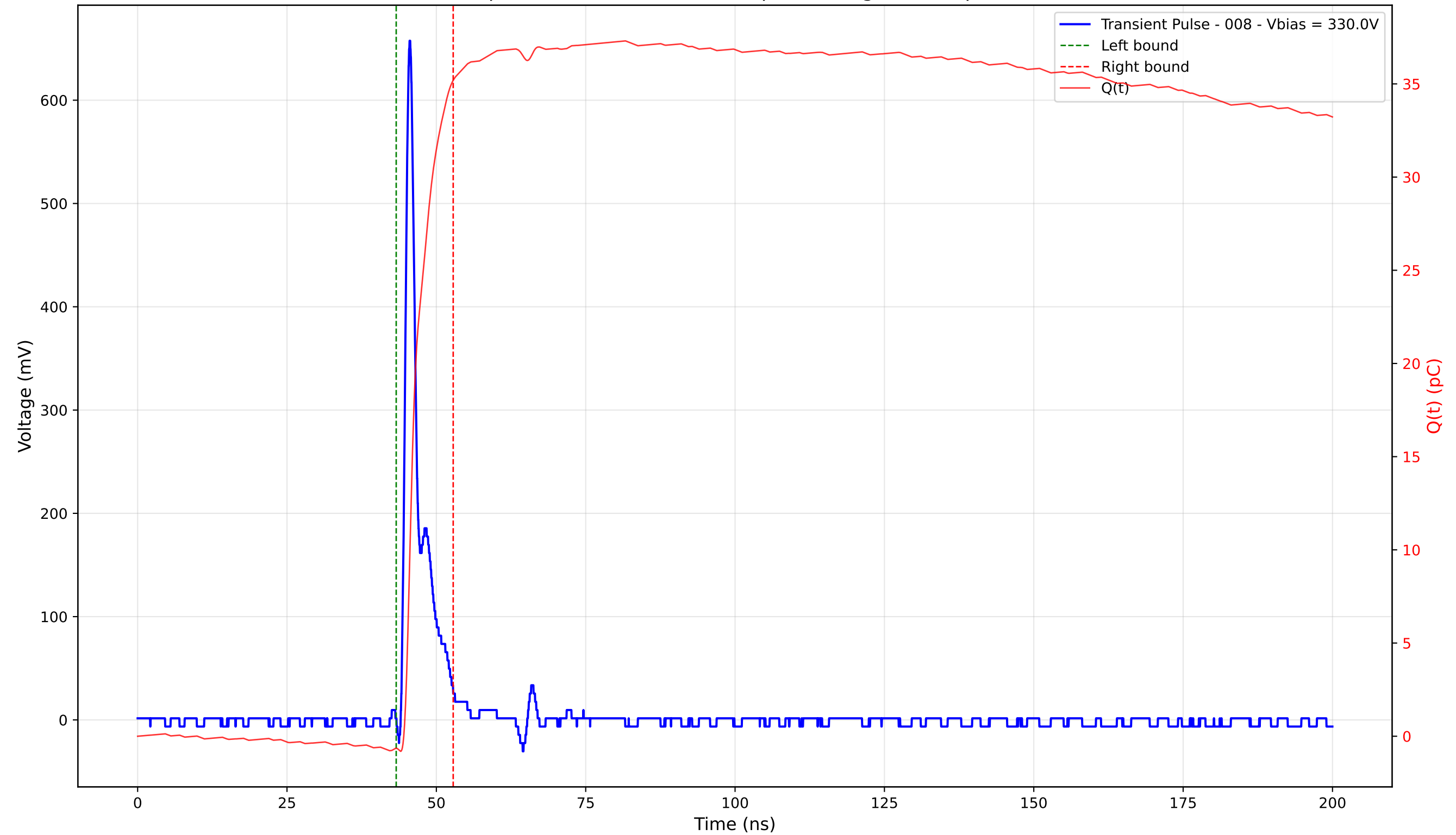
Transient Pulse - Sample: 4003 - Position: 165.0 \mu\text{m} - Charge: 35.84 pC - Rise Time: 0.96 ns
