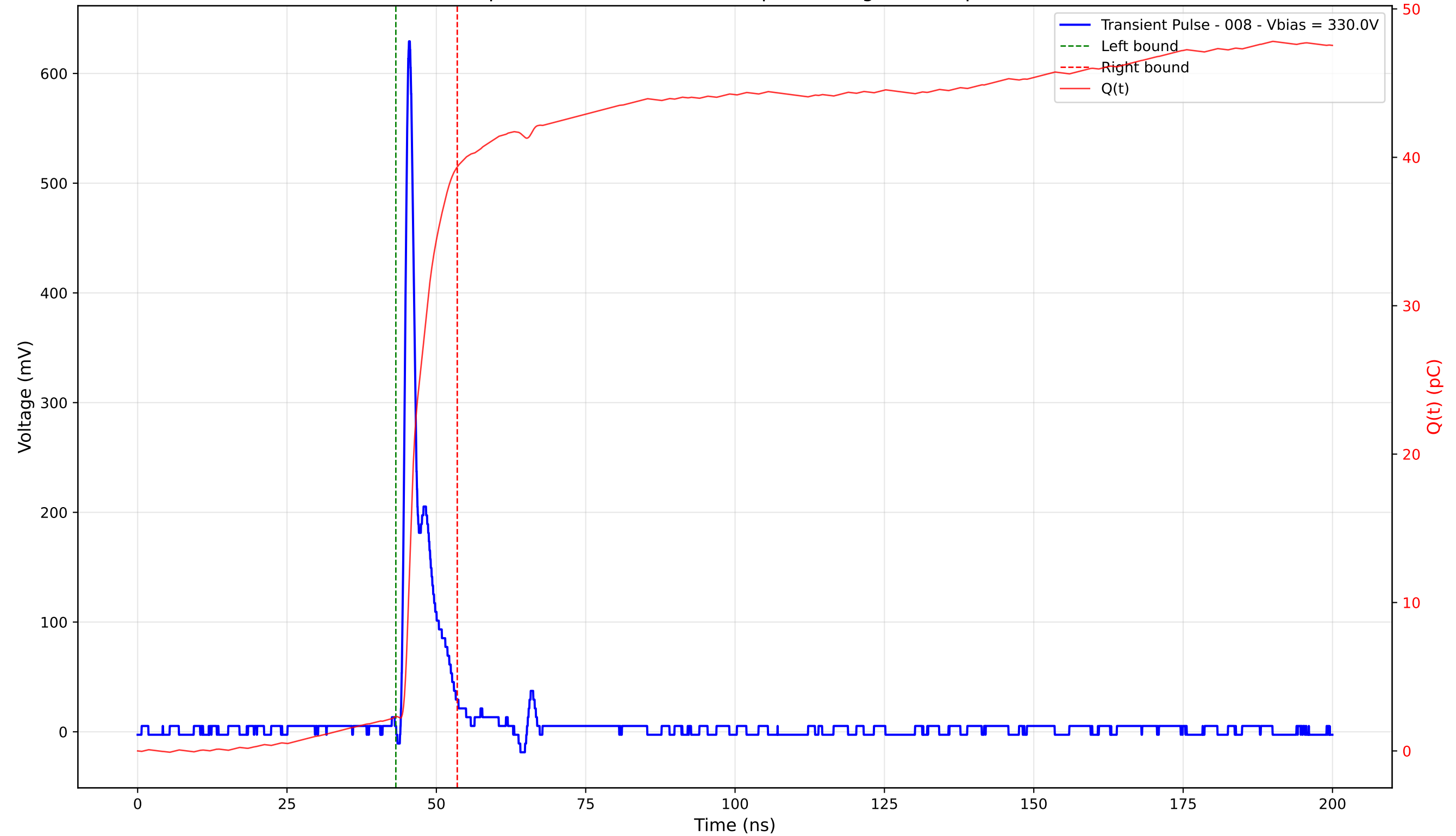
Transient Pulse - Sample: 4003 - Position: 140.0 \mu\text{m} - Charge: 37.04 pC - Rise Time: 0.92 ns
