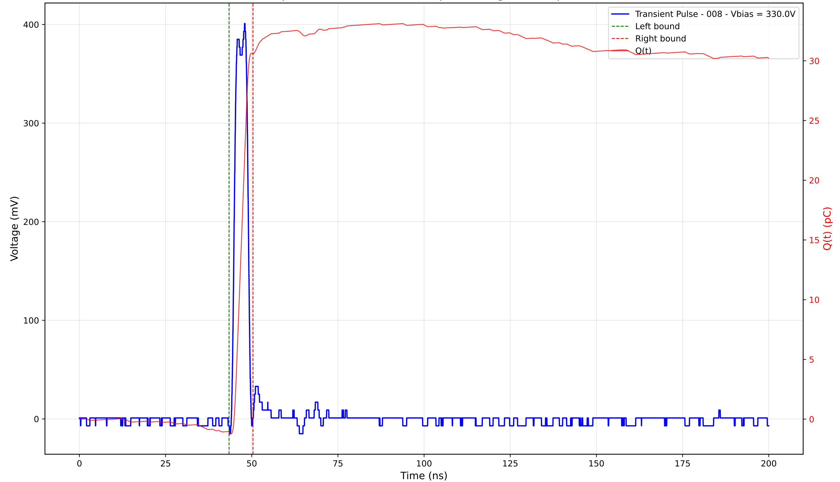
Transient Pulse - Sample: 4003 - Position: 355.0 \mu\text{m} - Charge: 31.67 pC - Rise Time: 1.20 ns
