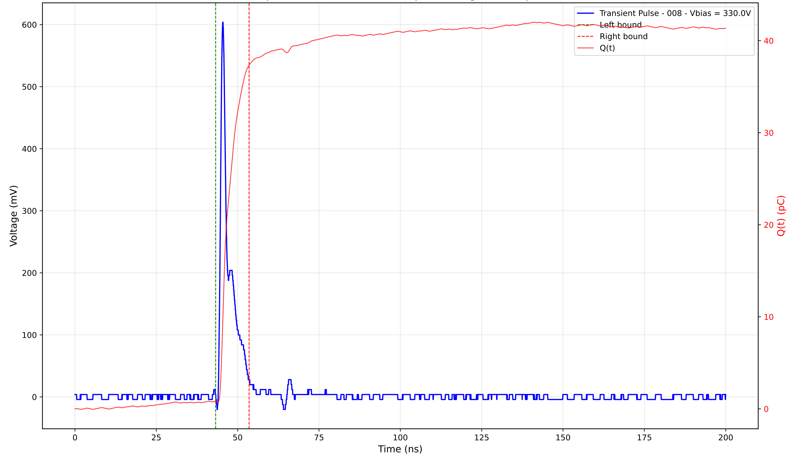
Transient Pulse - Sample: 4003 - Position: 125.0 \mu\text{m} - Charge: 36.46 pC - Rise Time: 0.90 ns
