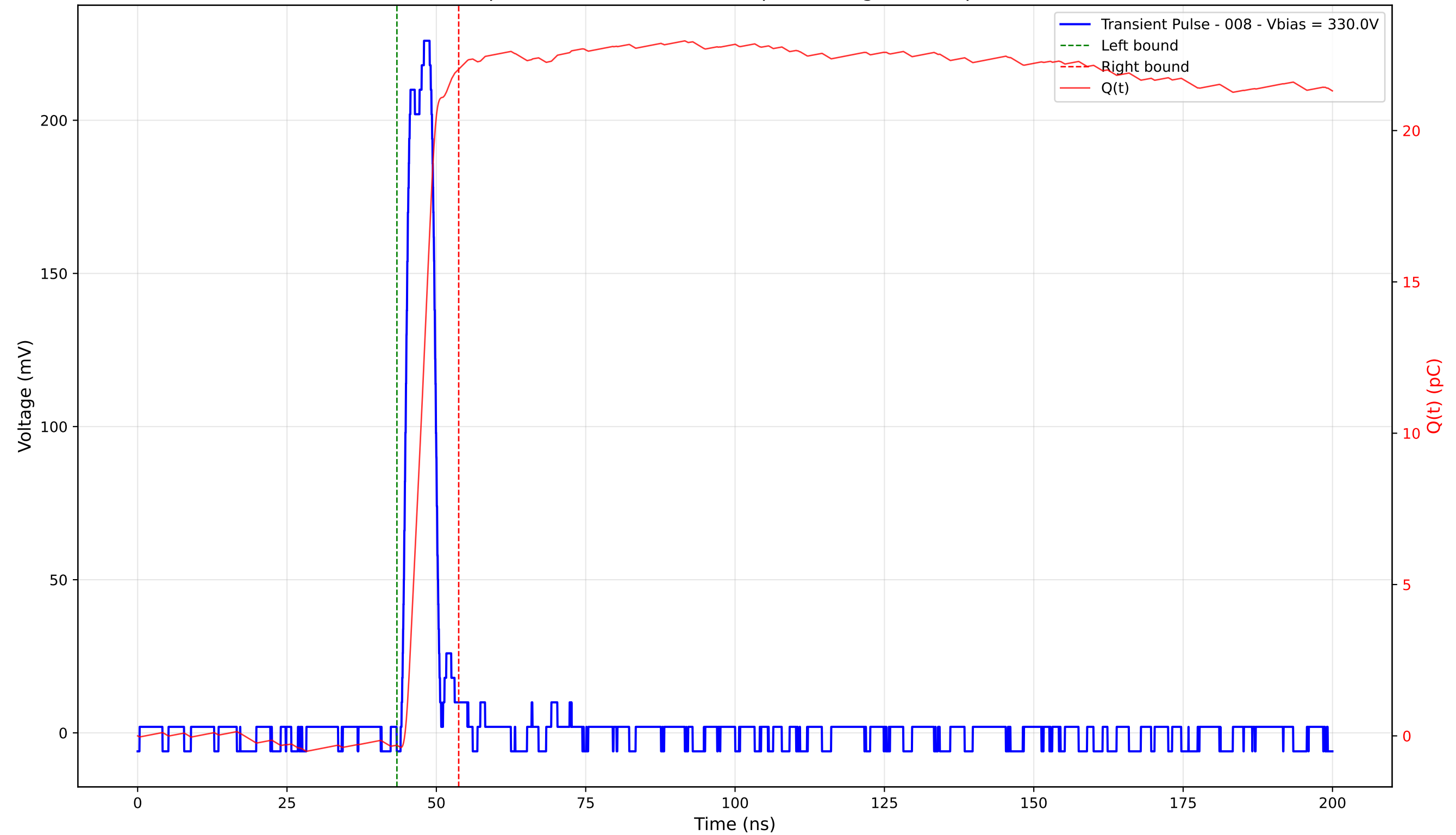
Transient Pulse - Sample: 4003 - Position: 390.0 \mu\text{m} - Charge: 22.34 pC - Rise Time: 1.31 ns
