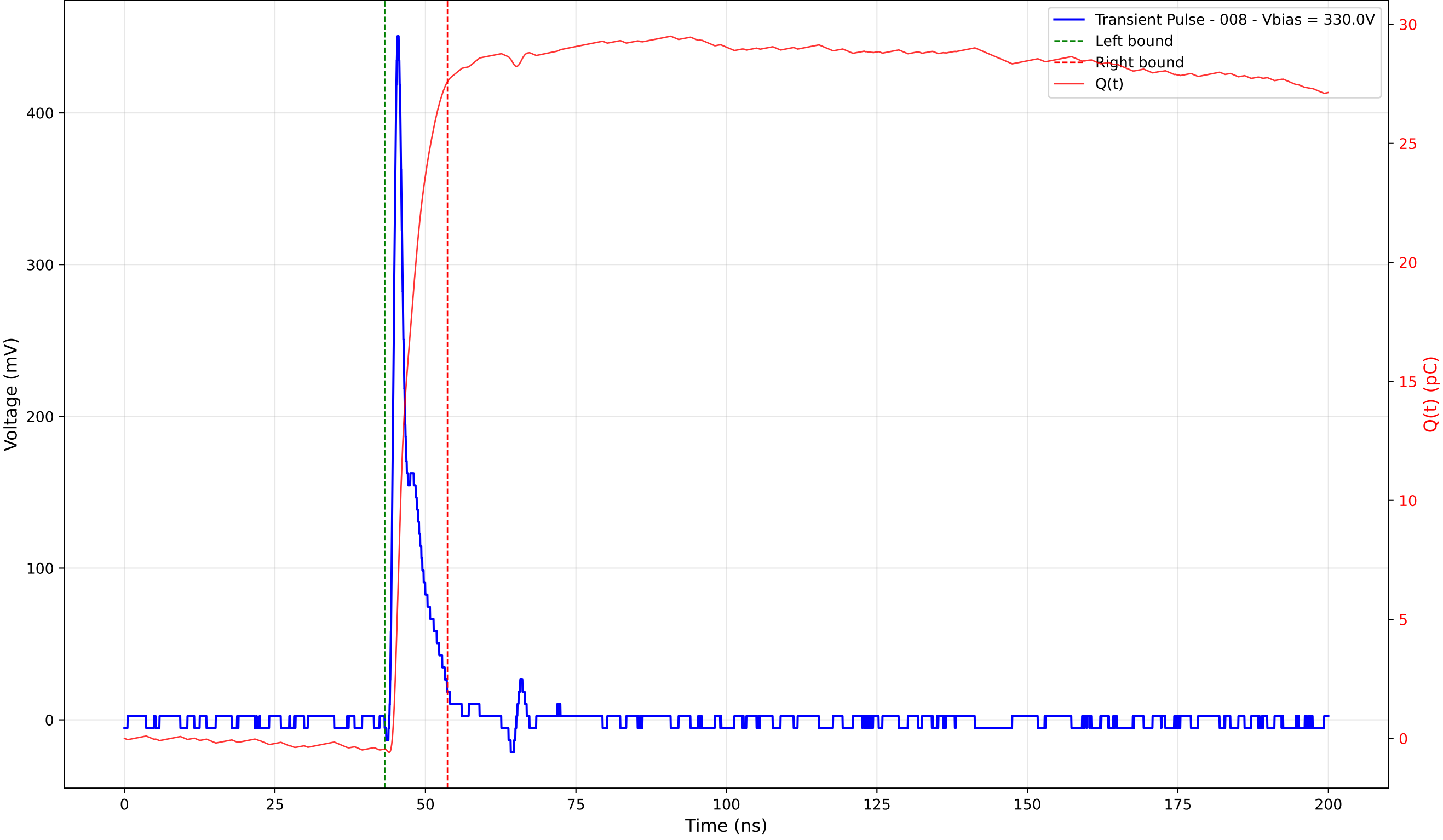
Transient Pulse - Sample: 4003 - Position: 105.0 \mu\text{m} - Charge: 28.04 pC - Rise Time: 0.90 ns
