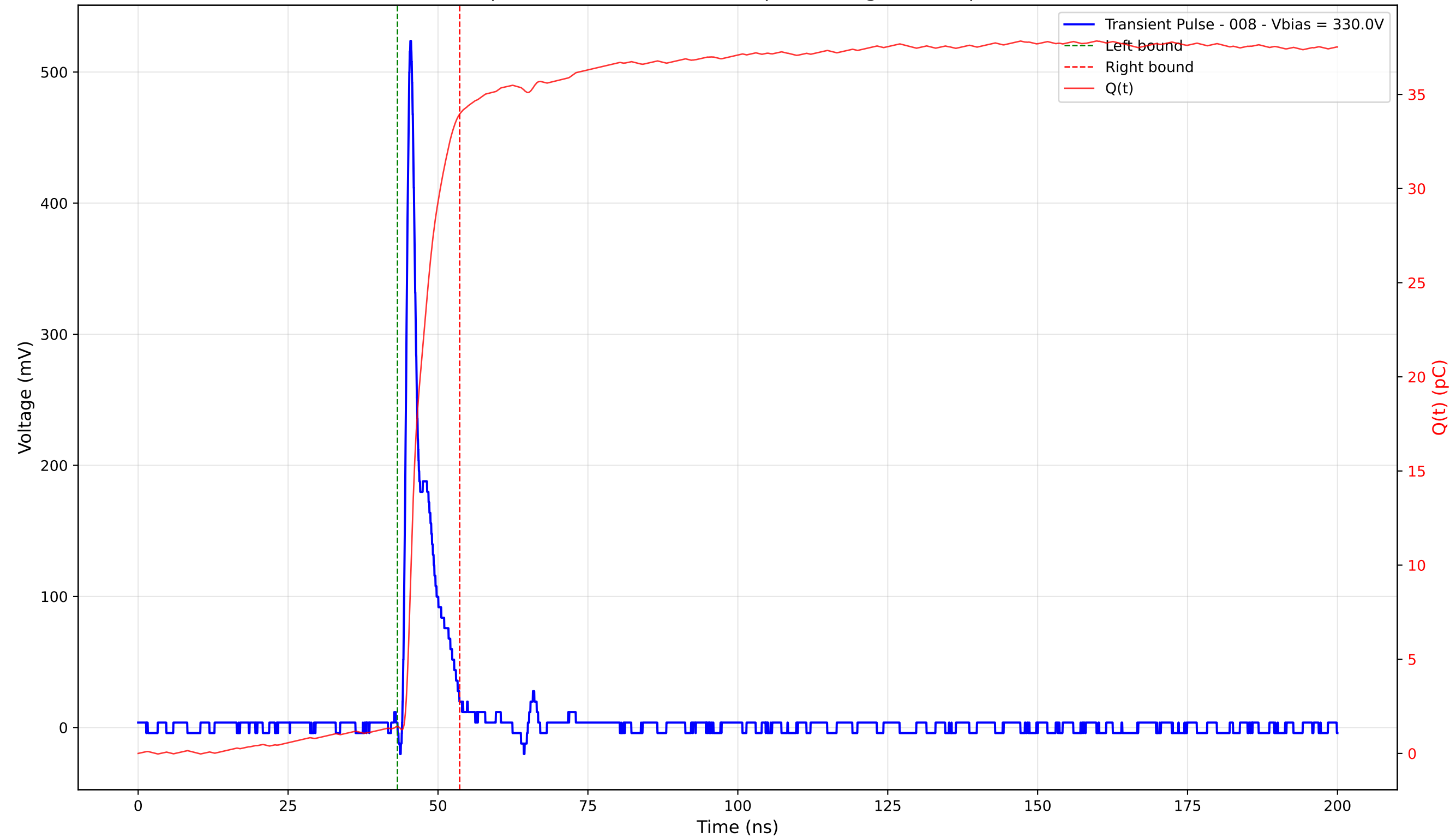
Transient Pulse - Sample: 4003 - Position: 110.0 \mu\text{m} - Charge: 32.53 pC - Rise Time: 0.89 ns
