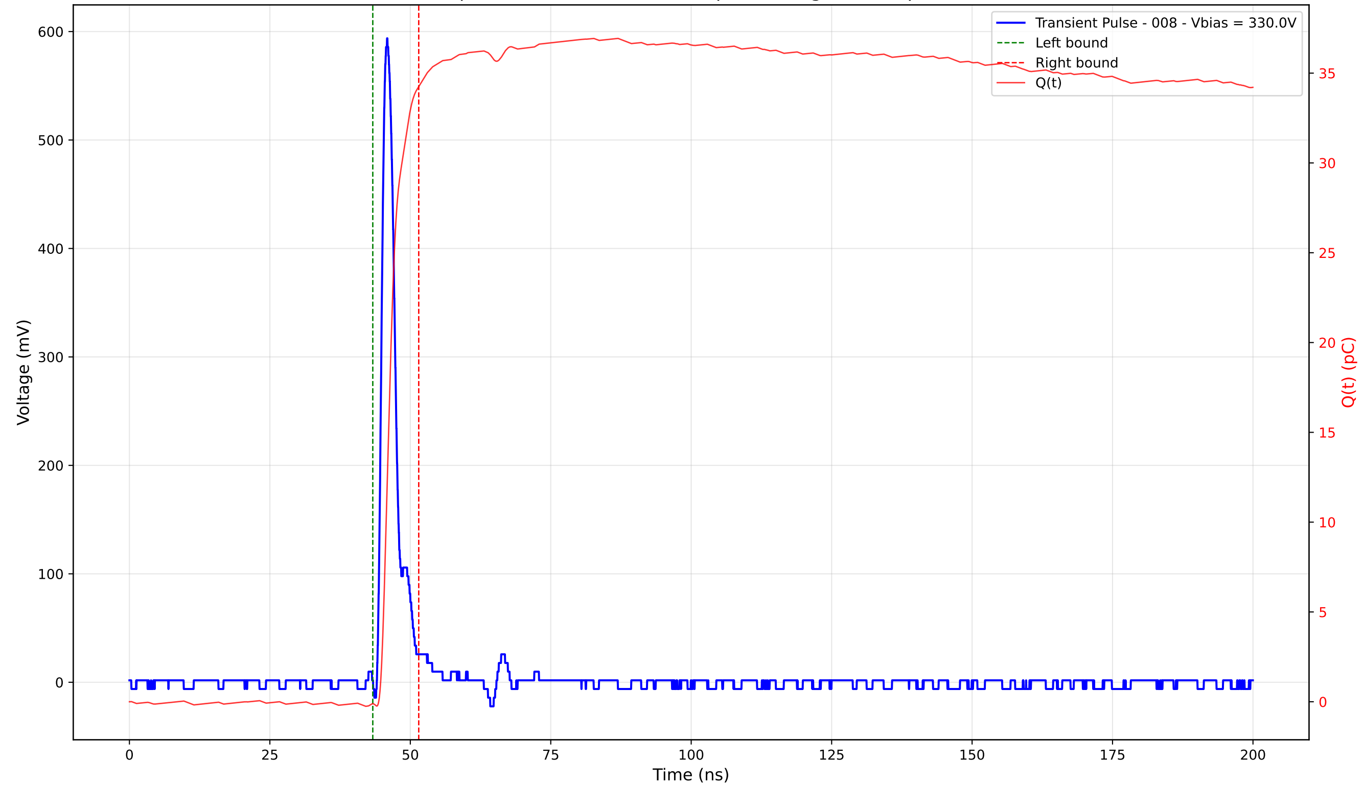
Transient Pulse - Sample: 4003 - Position: 250.0 \mu\text{m} - Charge: 34.36 pC - Rise Time: 1.09 ns
