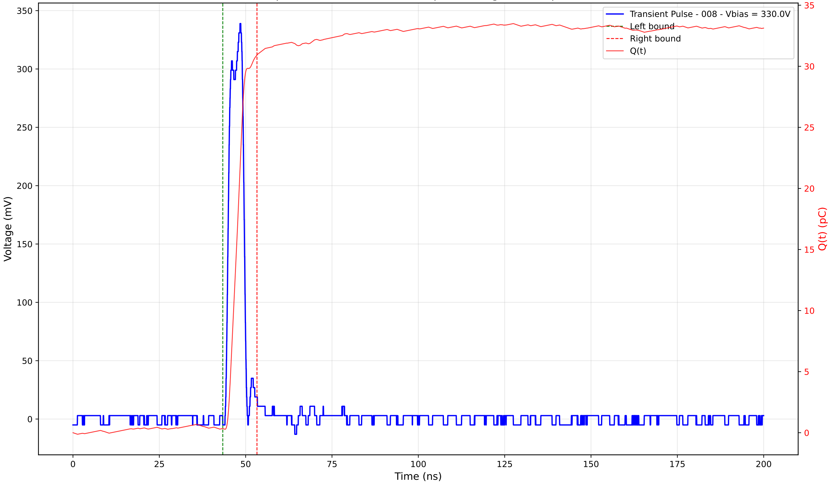
Transient Pulse - Sample: 4003 - Position: 380.0 \mu\text{m} - Charge: 30.59 pC - Rise Time: 1.56 ns
