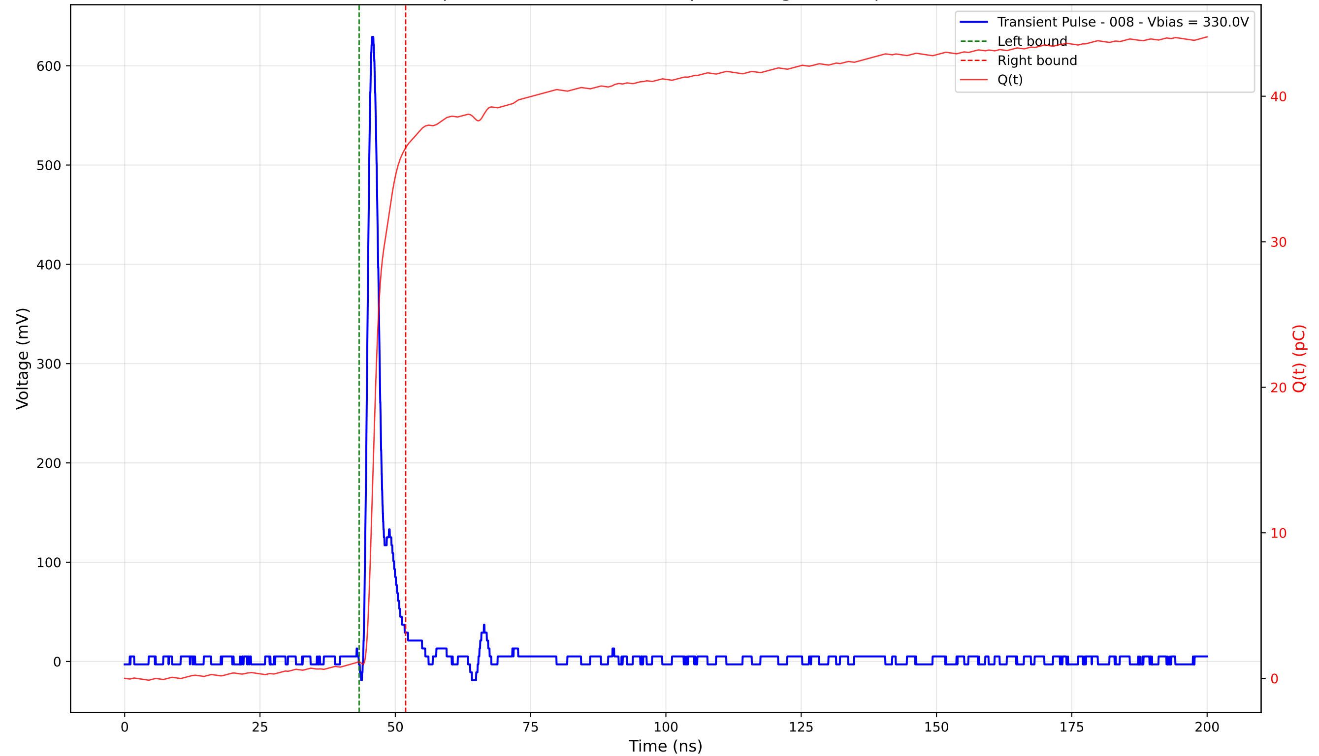
Transient Pulse - Sample: 4003 - Position: 230.0 \mu\text{m} - Charge: 35.33 pC - Rise Time: 1.08 ns
