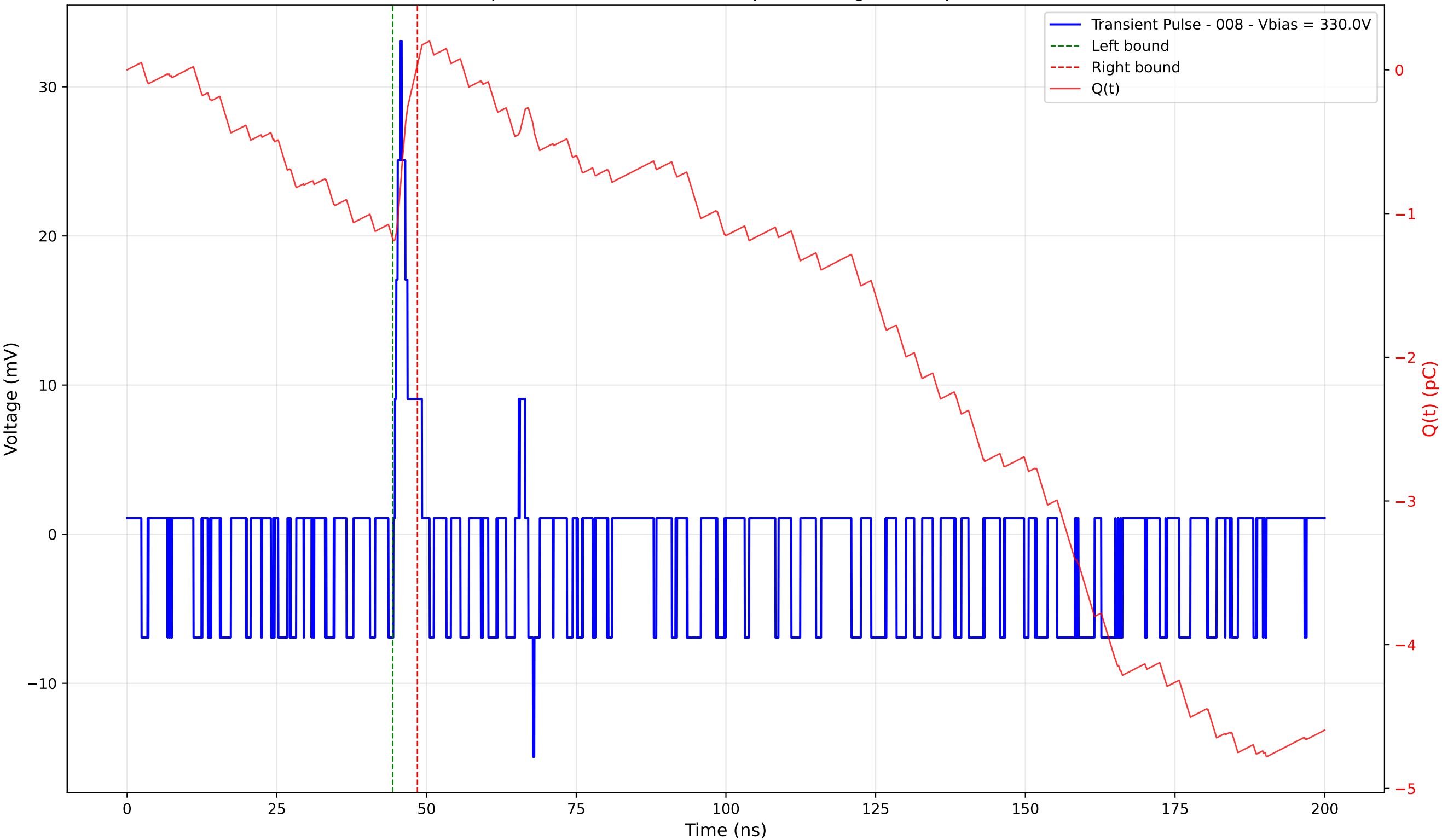
Transient Pulse - Sample: 4003 - Position: 15.0 \mu\text{m} - Charge: 1.21 pC - Rise Time: 0.95 ns
