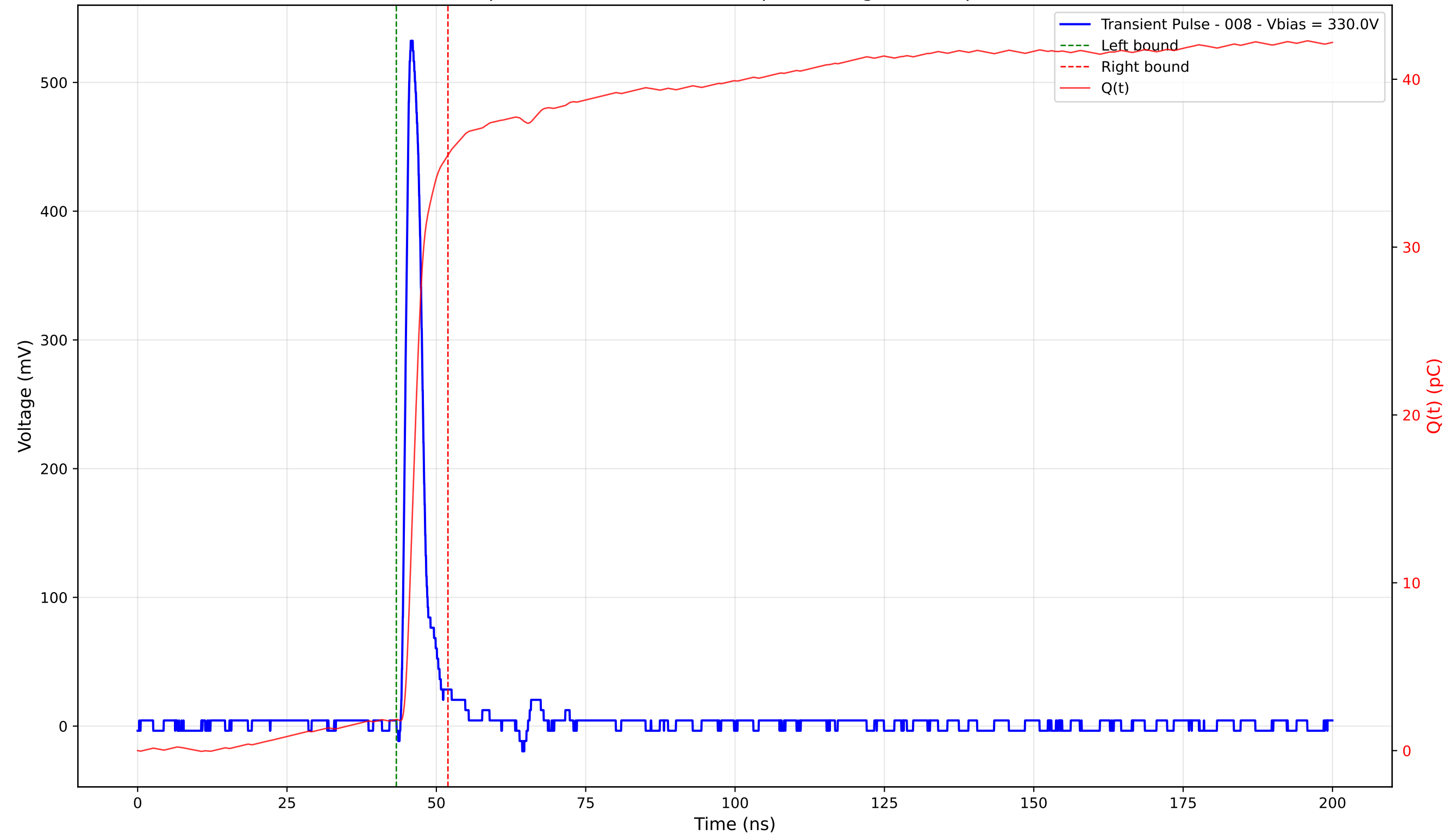
Transient Pulse - Sample: 4003 - Position: 275.0 \mu\text{m} - Charge: 33.61 pC - Rise Time: 1.10 ns
