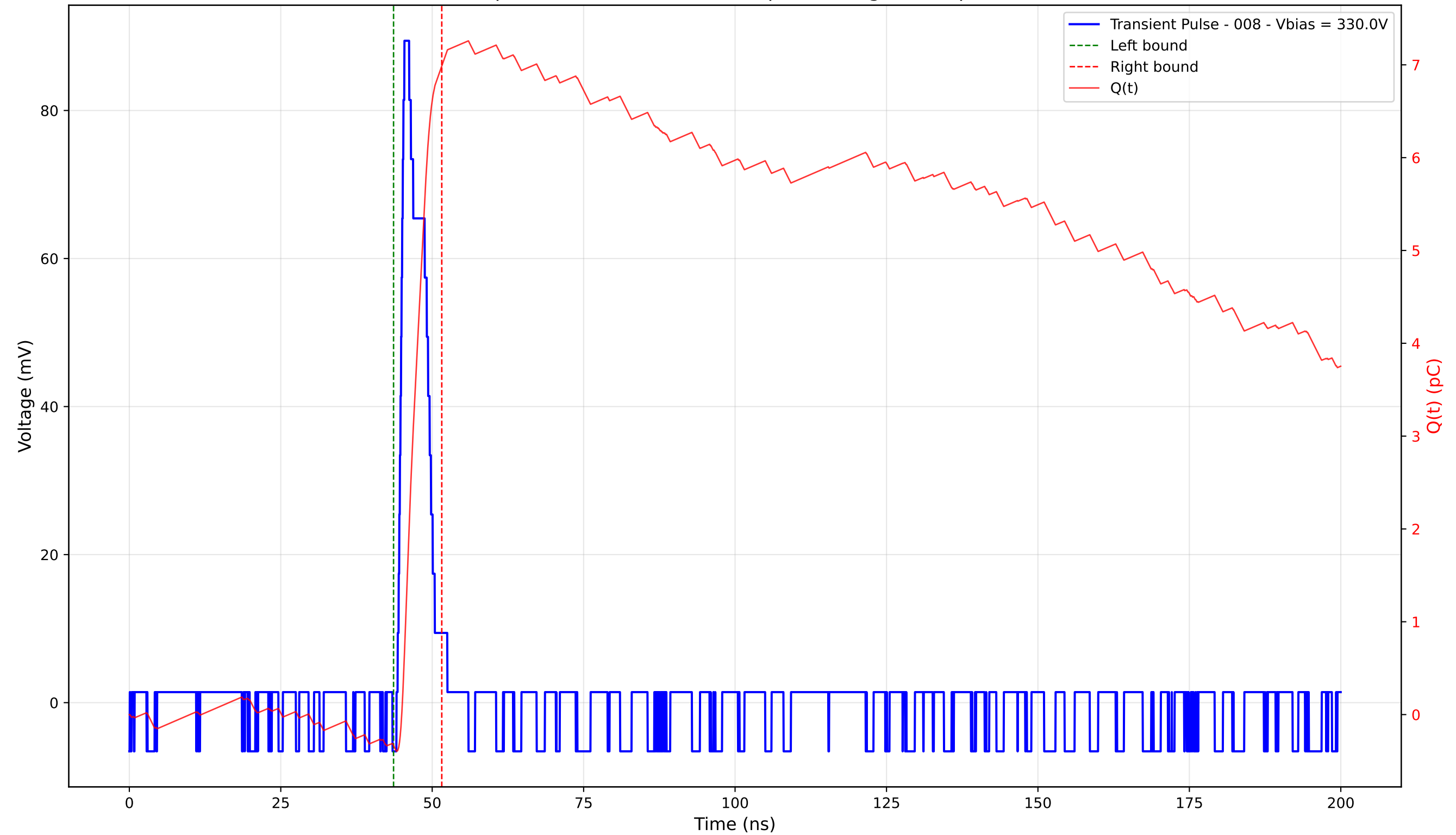
Transient Pulse - Sample: 4003 - Position: 405.0 \mu\text{m} - Charge: 7.32 pC - Rise Time: 0.94 ns
