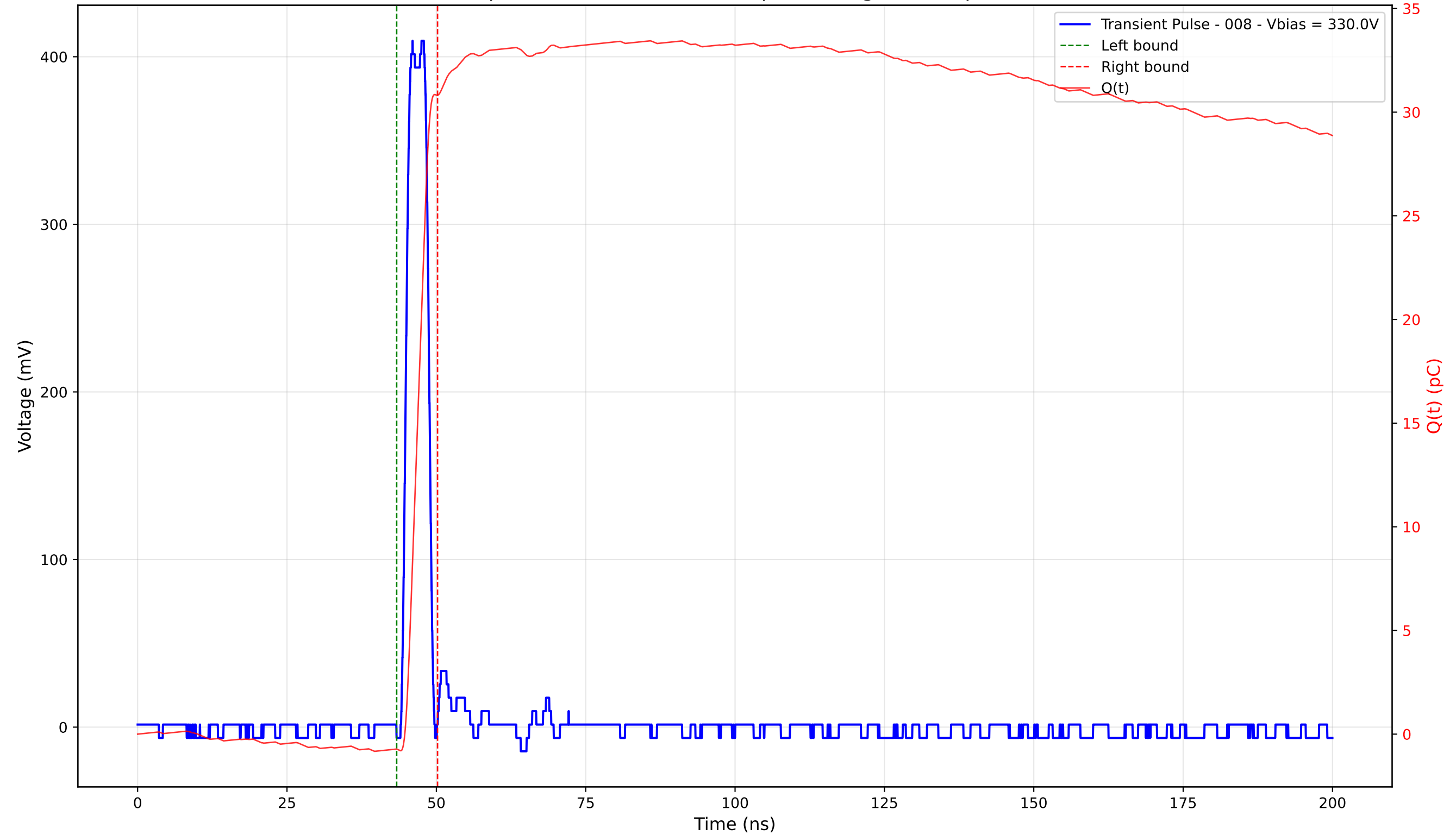
Transient Pulse - Sample: 4003 - Position: 345.0 \mu\text{m} - Charge: 31.54 pC - Rise Time: 1.16 ns
