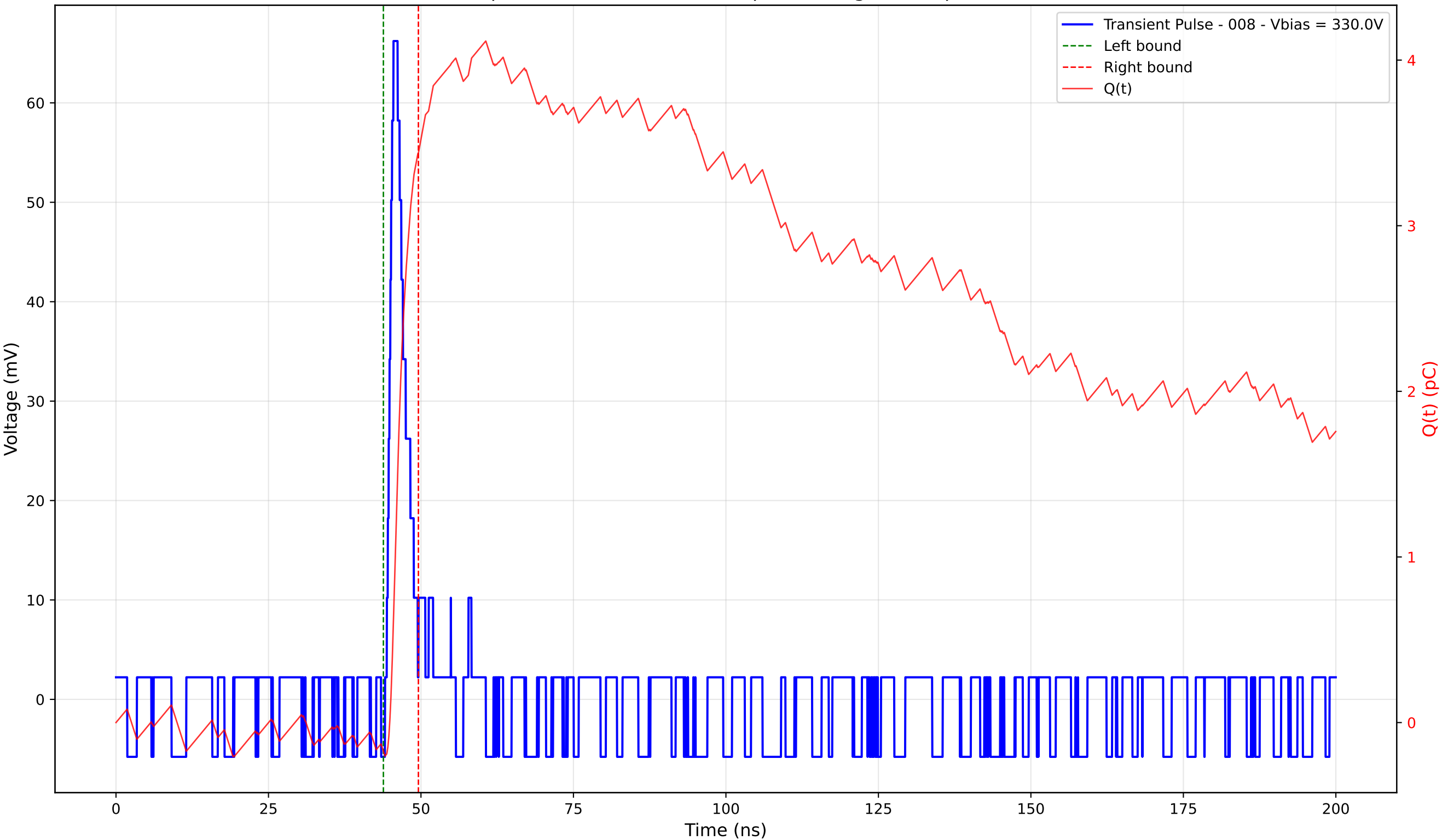
Transient Pulse - Sample: 4003 - Position: 50.0 \mu\text{m} - Charge: 3.61 pC - Rise Time: 1.09 ns
