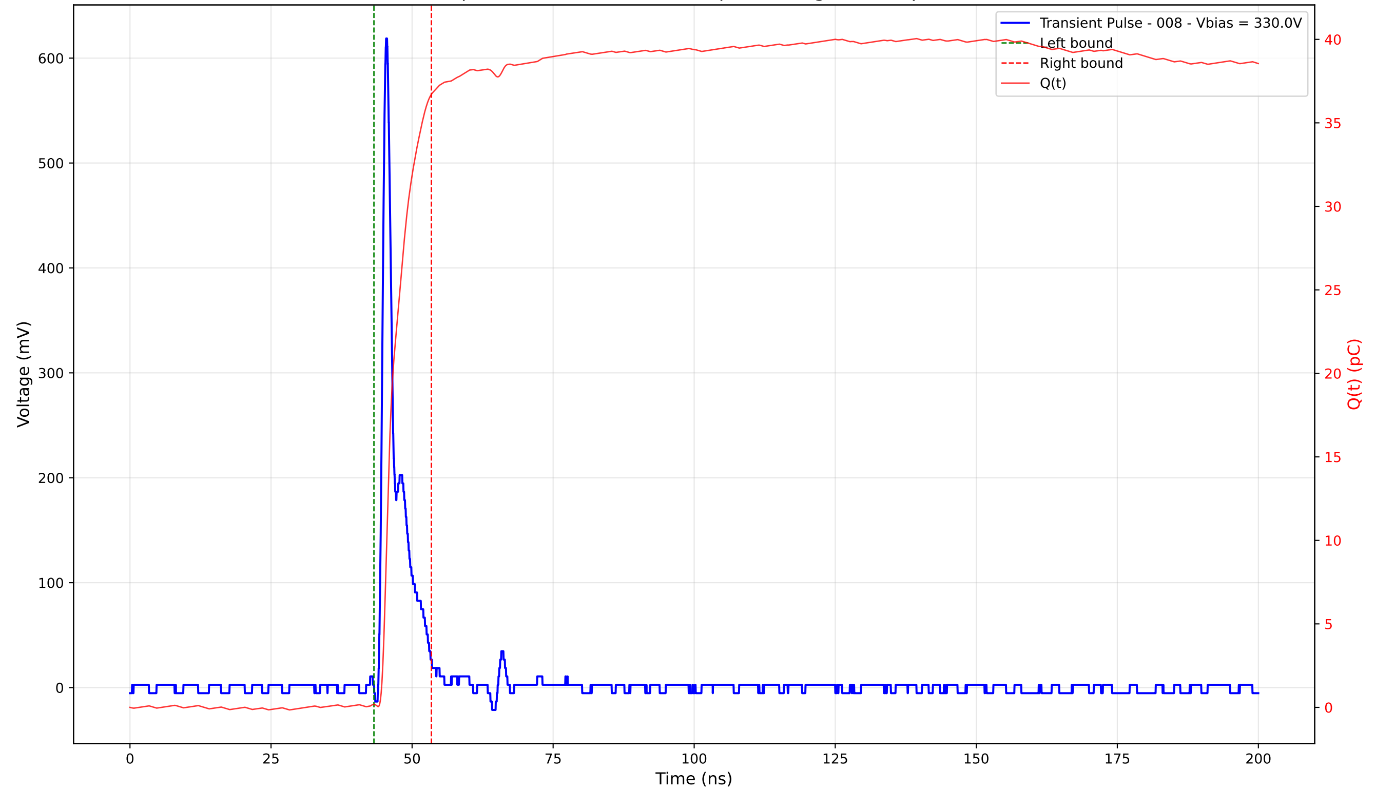
Transient Pulse - Sample: 4003 - Position: 135.0 \mu\text{m} - Charge: 36.52 pC - Rise Time: 0.90 ns
