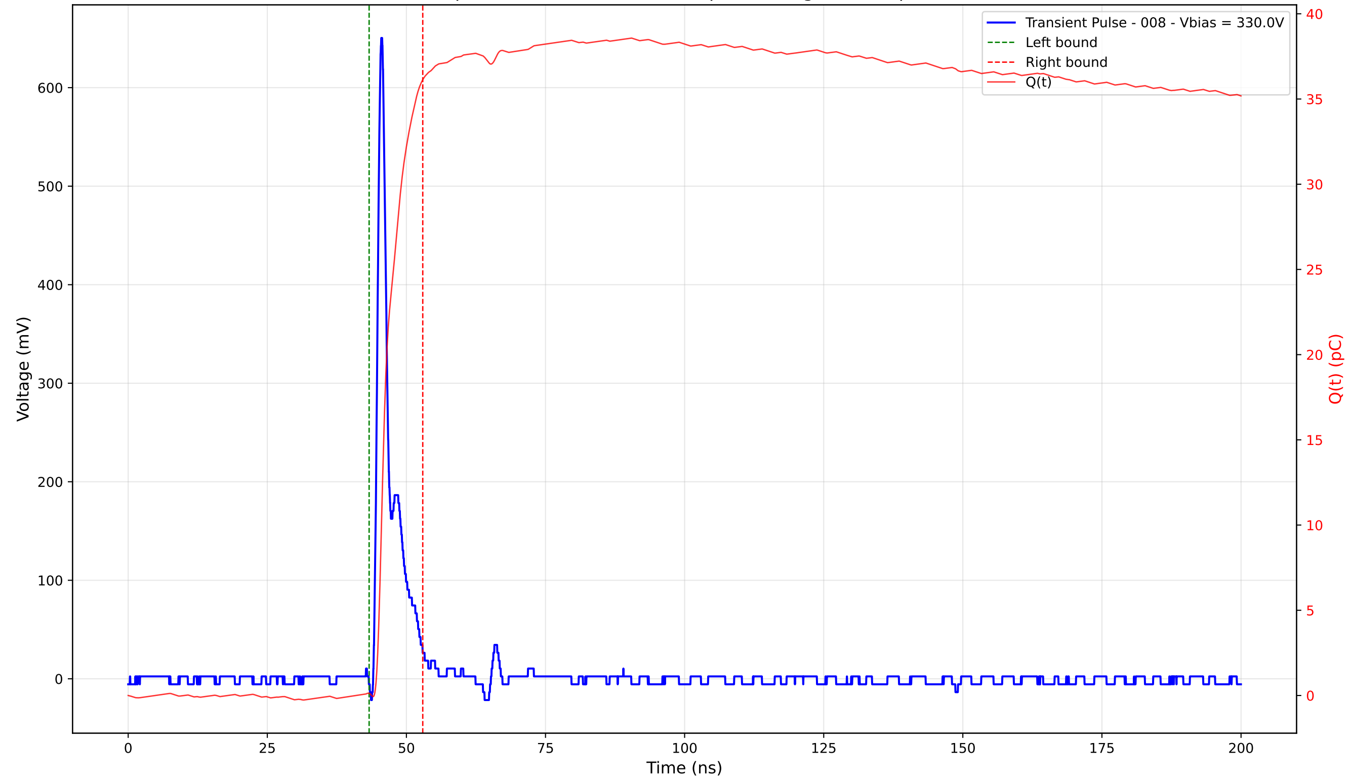
Transient Pulse - Sample: 4003 - Position: 160.0 \mu\text{m} - Charge: 36.01 pC - Rise Time: 0.94 ns
