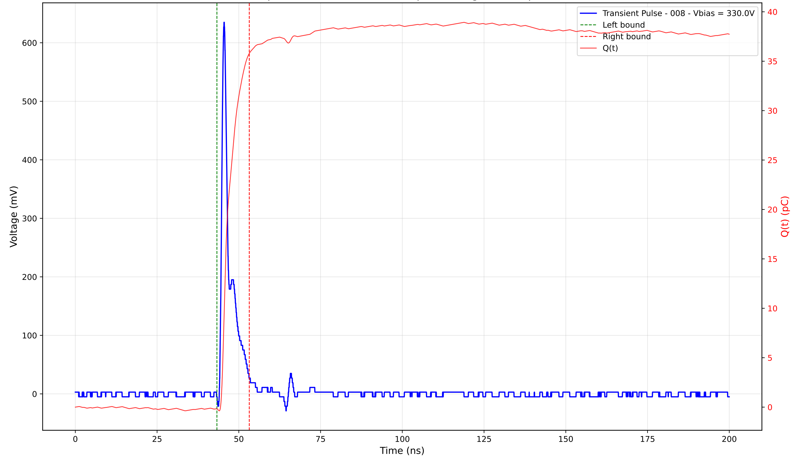
Transient Pulse - Sample: 4003 - Position: 145.0 \mu\text{m} - Charge: 35.96 pC - Rise Time: 0.93 ns
