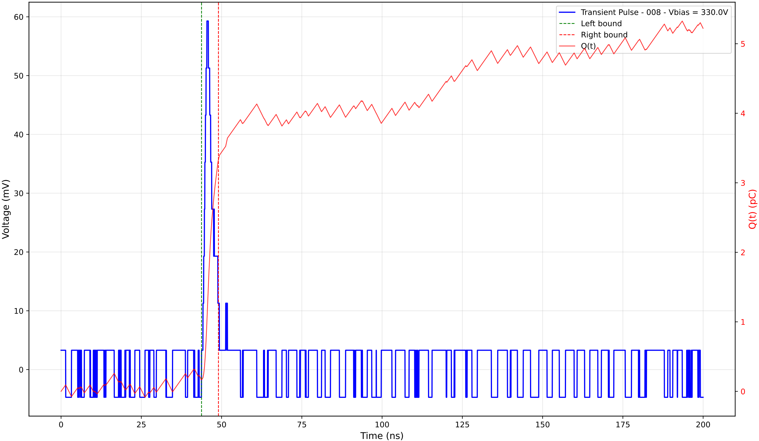
Transient Pulse - Sample: 4003 - Position: 45.0 \mu\text{m} - Charge: 3.17 pC - Rise Time: 1.23 ns
