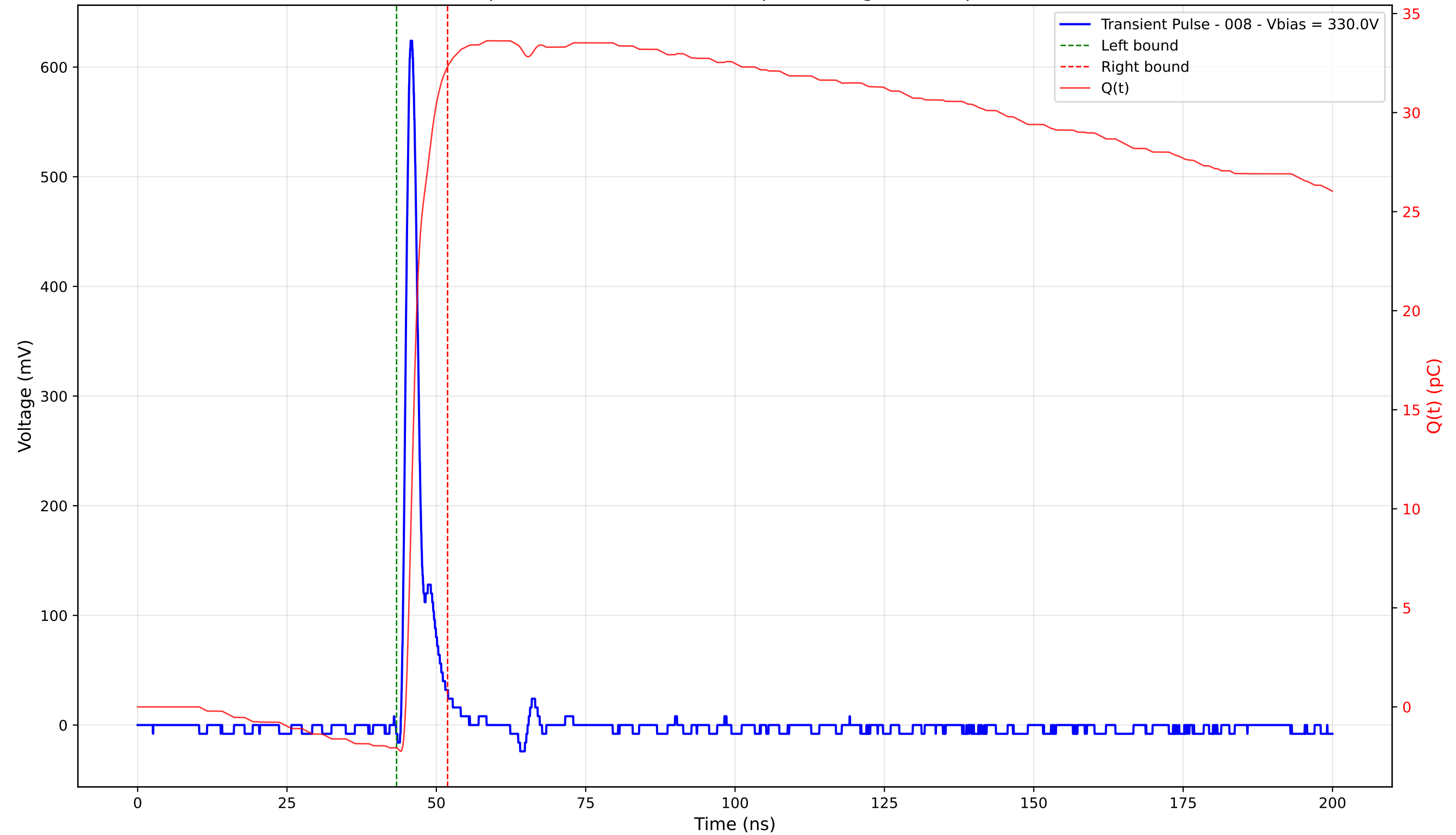
Transient Pulse - Sample: 4003 - Position: 225.0 \mu\text{m} - Charge: 34.39 pC - Rise Time: 1.07 ns
