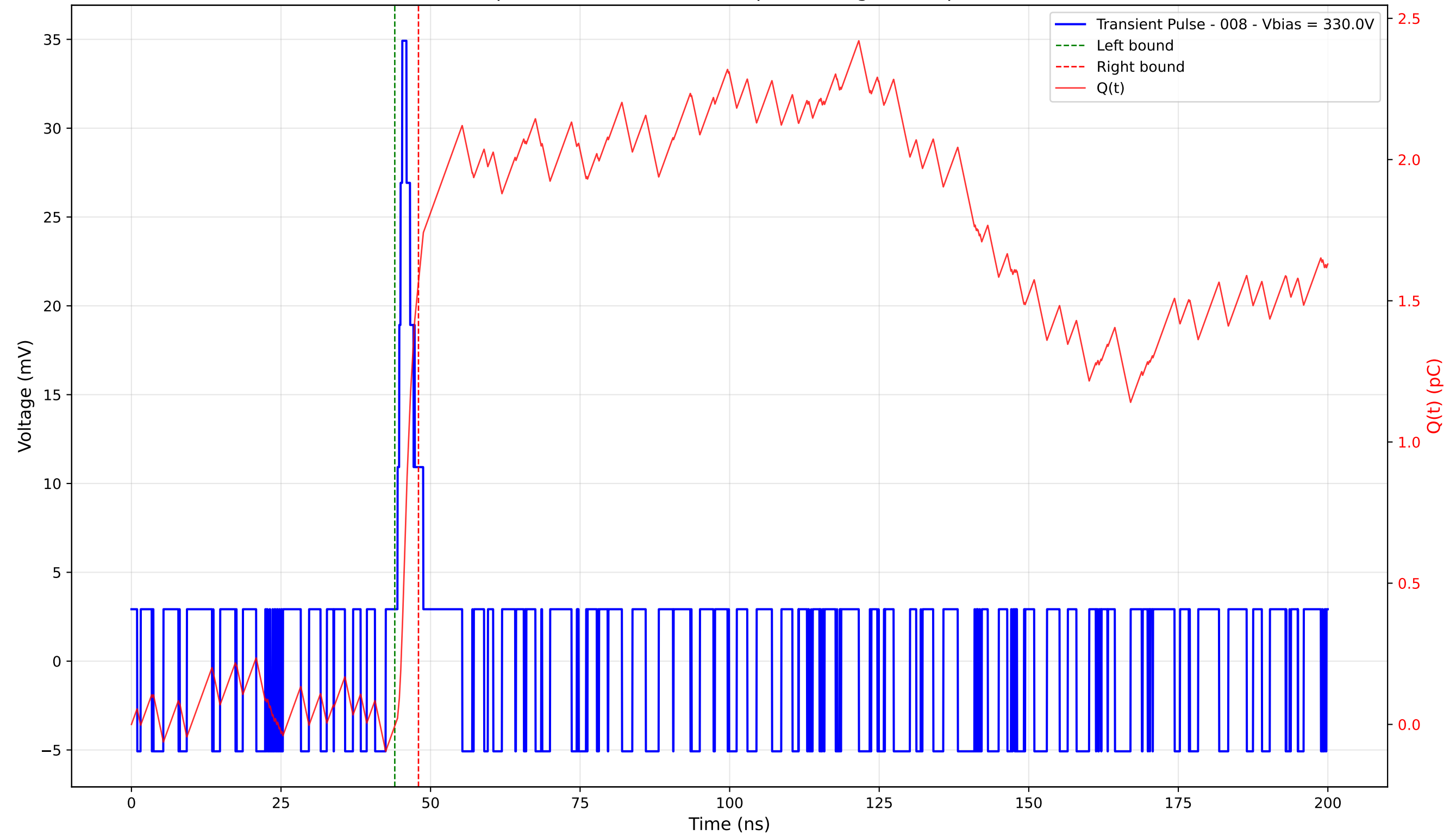
Transient Pulse - Sample: 4003 - Position: 35.0 \mu\text{m} - Charge: 1.57 pC - Rise Time: 0.80 ns
