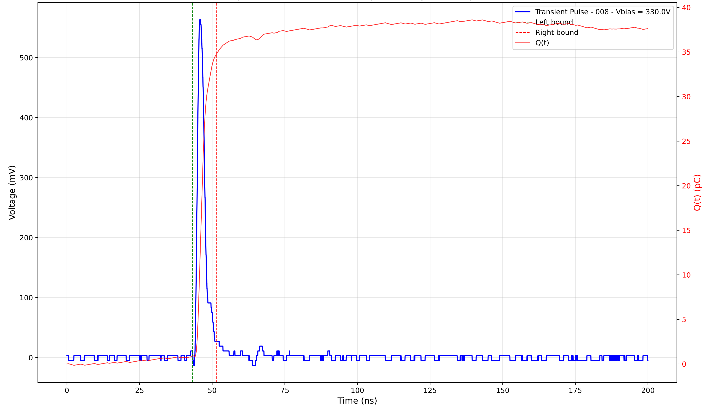
Transient Pulse - Sample: 4003 - Position: 260.0 \mu\text{m} - Charge: 33.90 pC - Rise Time: 1.07 ns
