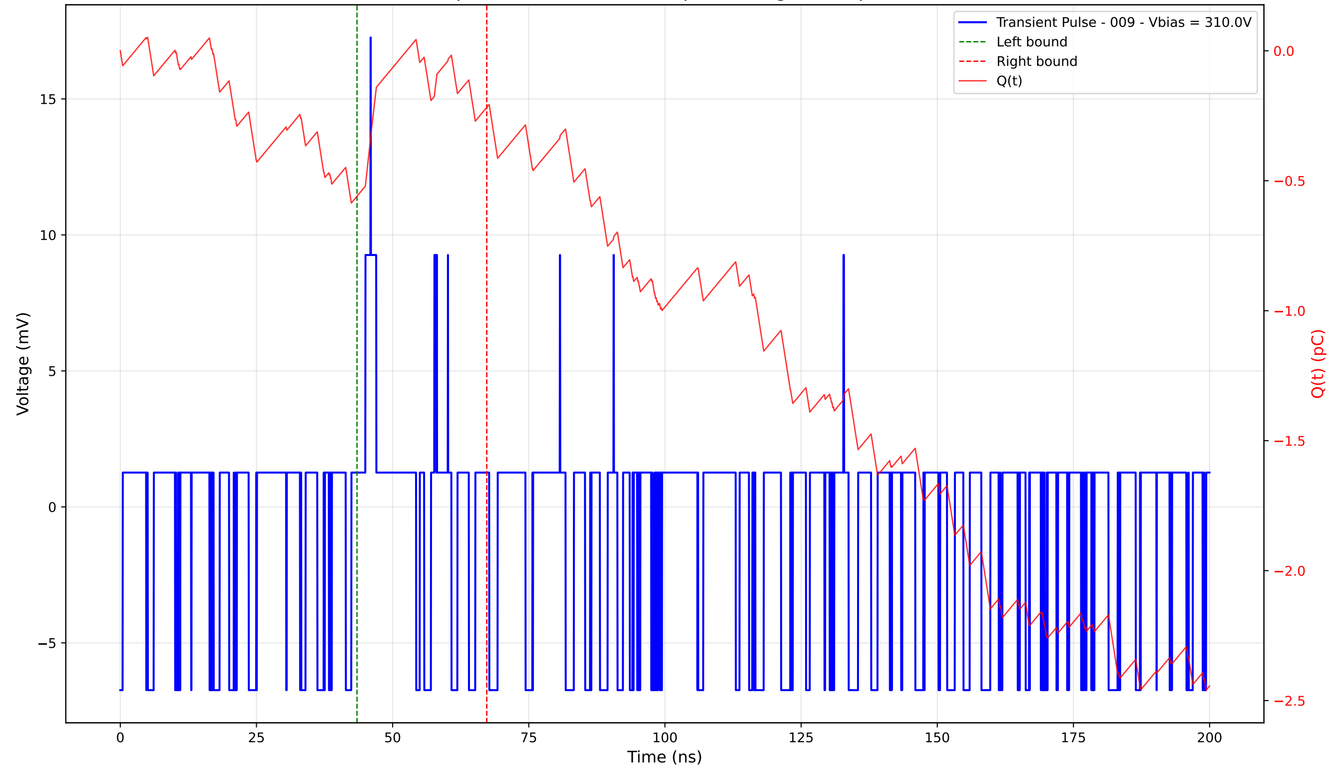
Transient Pulse - Sample: 4003 - Position: 0.0 \mu\text{m} - Charge: 0.34 pC - Rise Time: 0.96 ns
