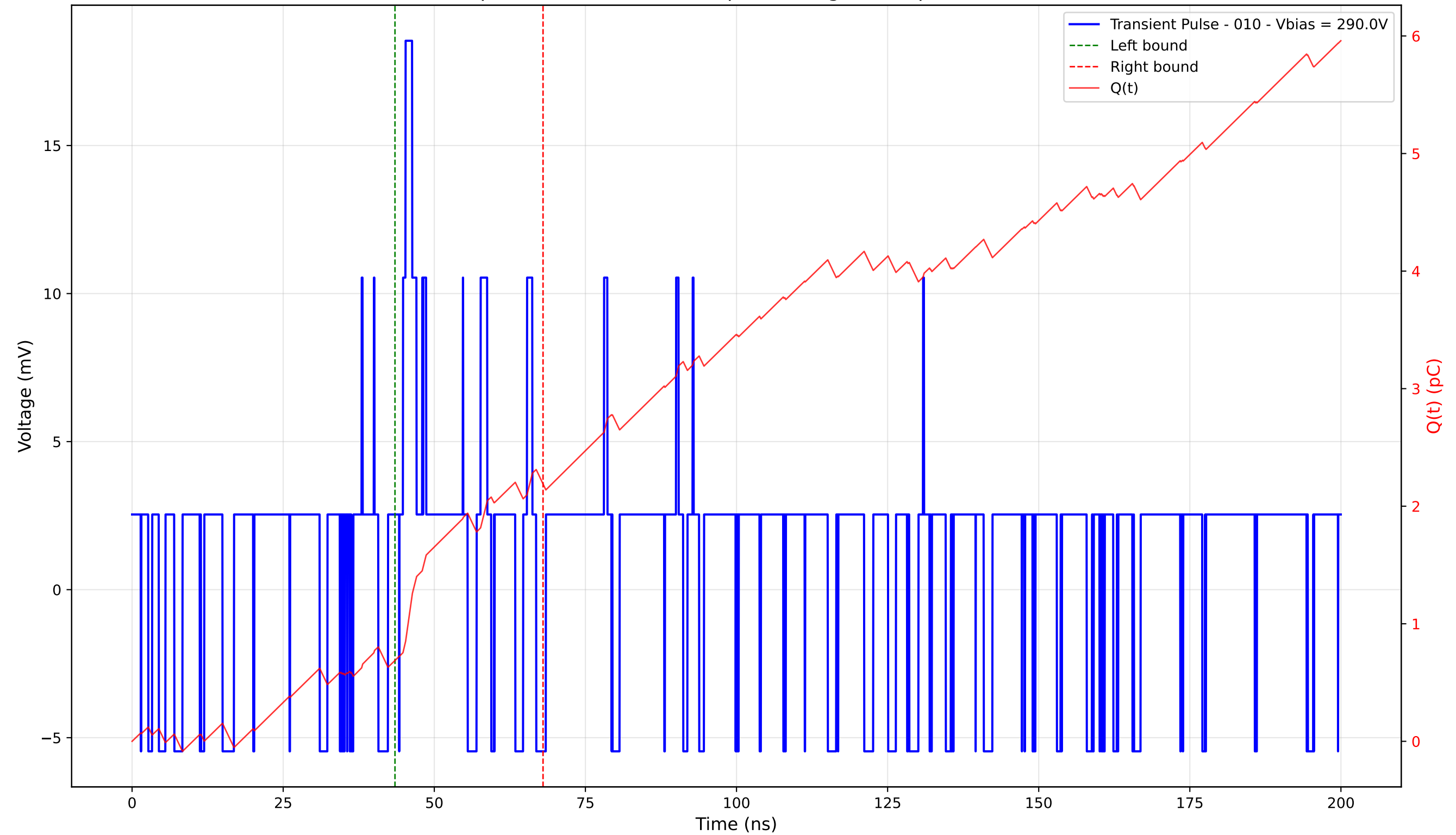
Transient Pulse - Sample: 4003 - Position: 5.0 \mu\text{m} - Charge: 1.50 pC - Rise Time: 0.00 ns (N/A)
