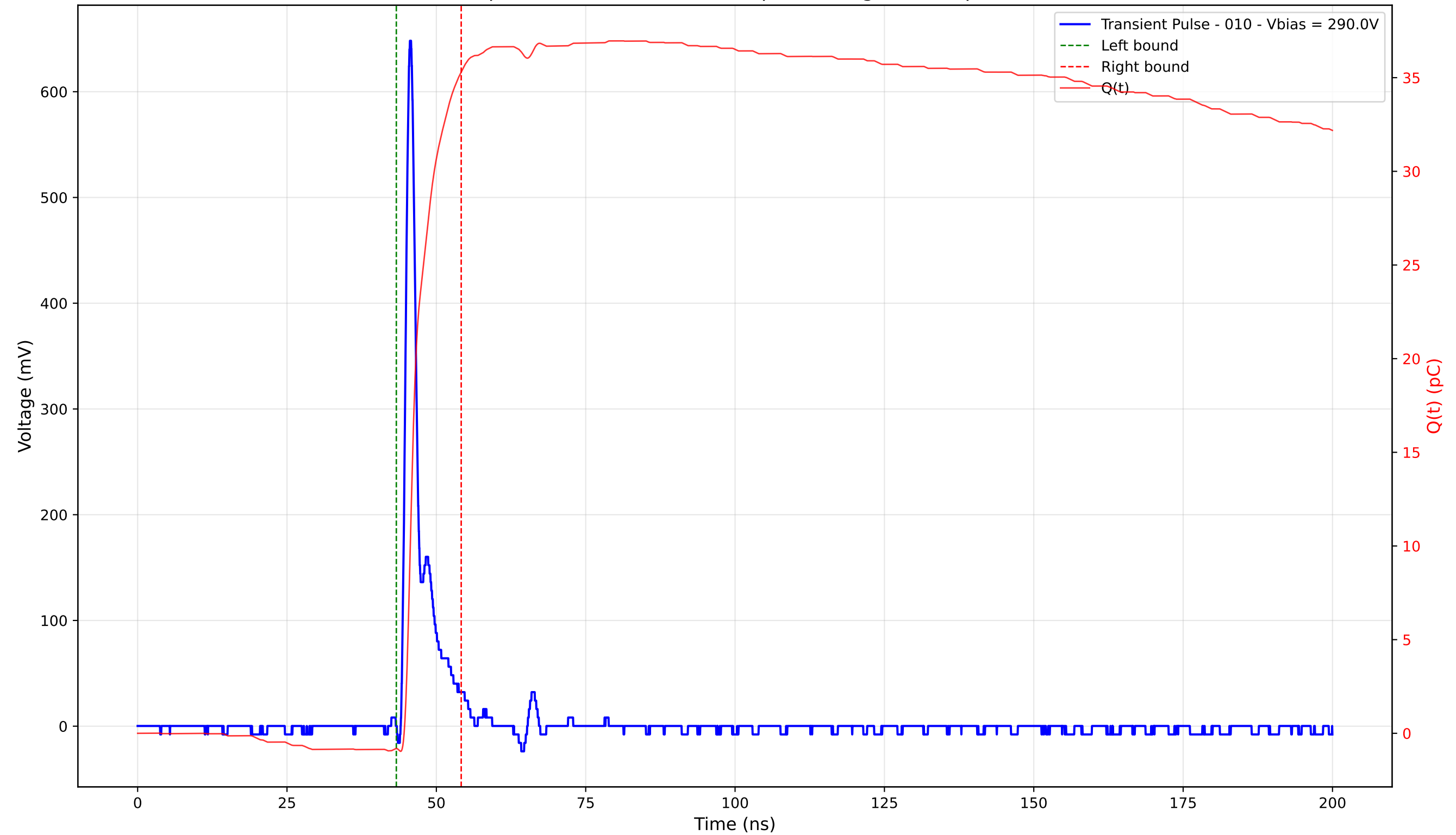
Transient Pulse - Sample: 4003 - Position: 185.0 \mu\text{m} - Charge: 36.11 pC - Rise Time: 1.00 ns
