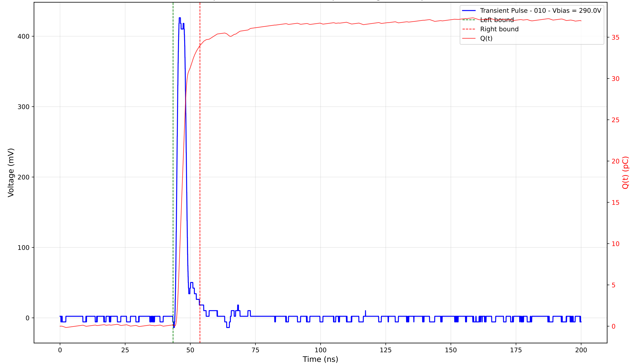
Transient Pulse - Sample: 4003 - Position: 315.0 \mu\text{m} - Charge: 33.84 pC - Rise Time: 1.10 ns
