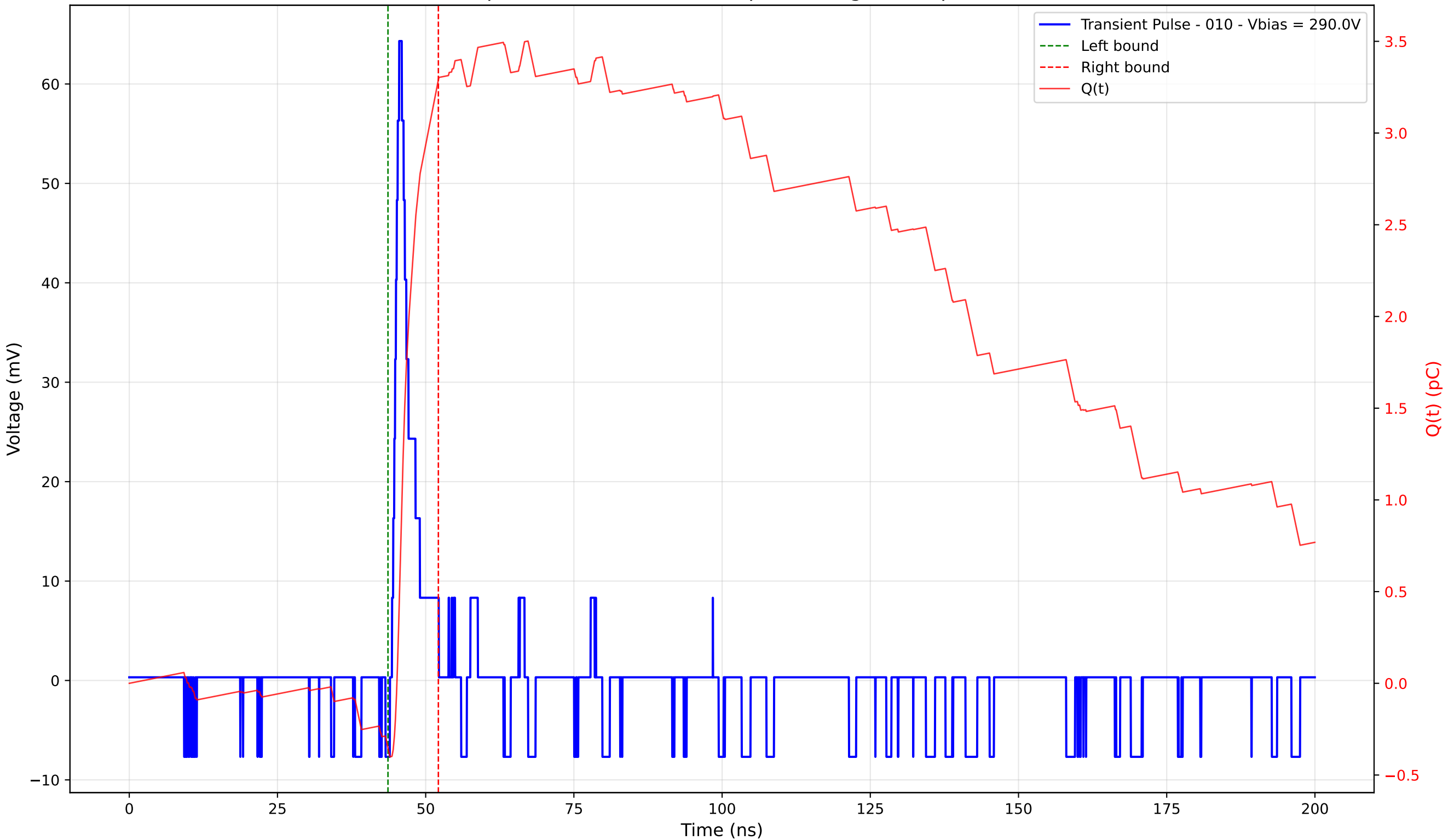
Transient Pulse - Sample: 4003 - Position: 50.0 \mu\text{m} - Charge: 3.64 pC - Rise Time: 1.20 ns
