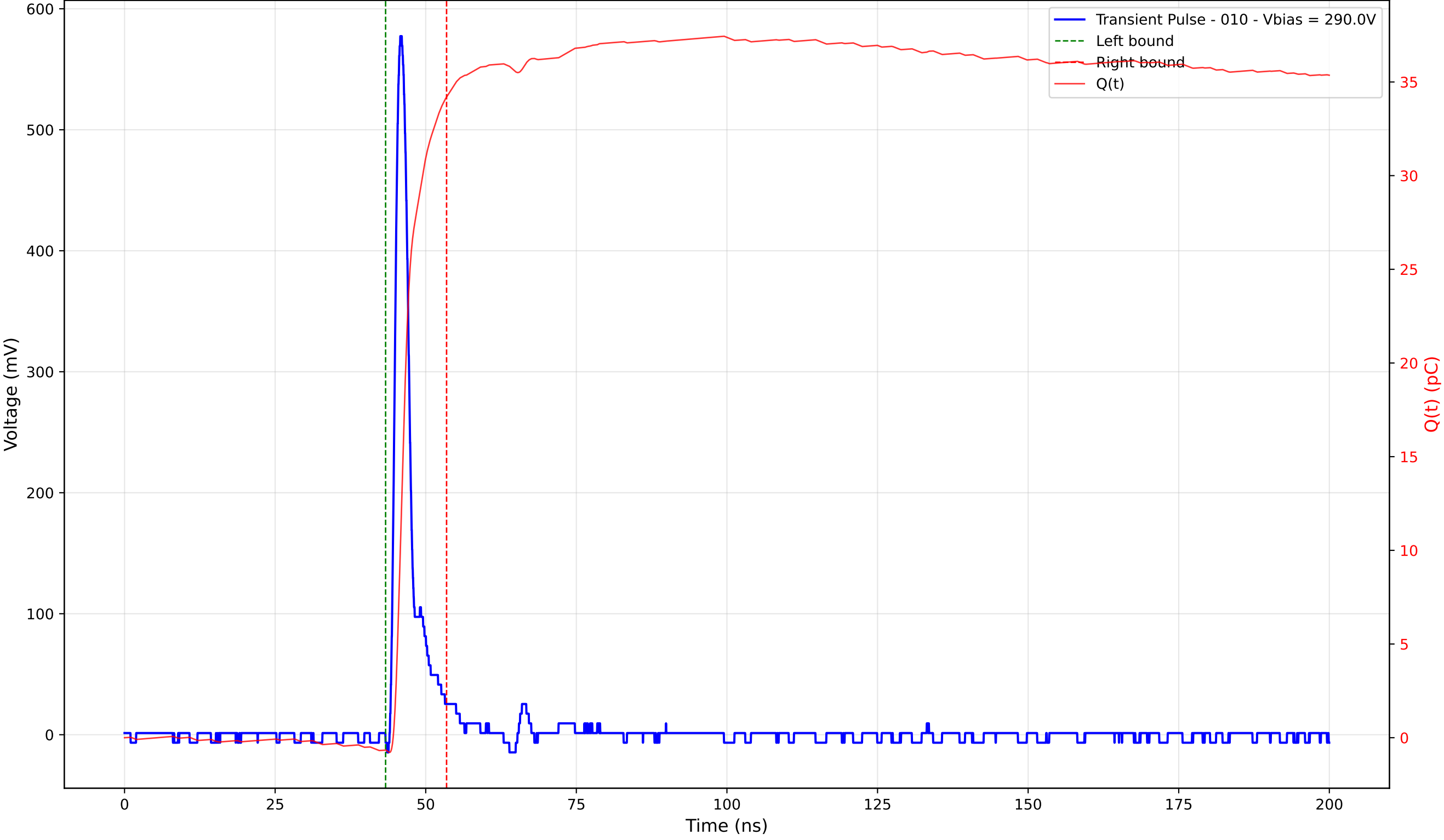
Transient Pulse - Sample: 4003 - Position: 240.0 \mu\text{m} - Charge: 34.85 pC - Rise Time: 1.10 ns
