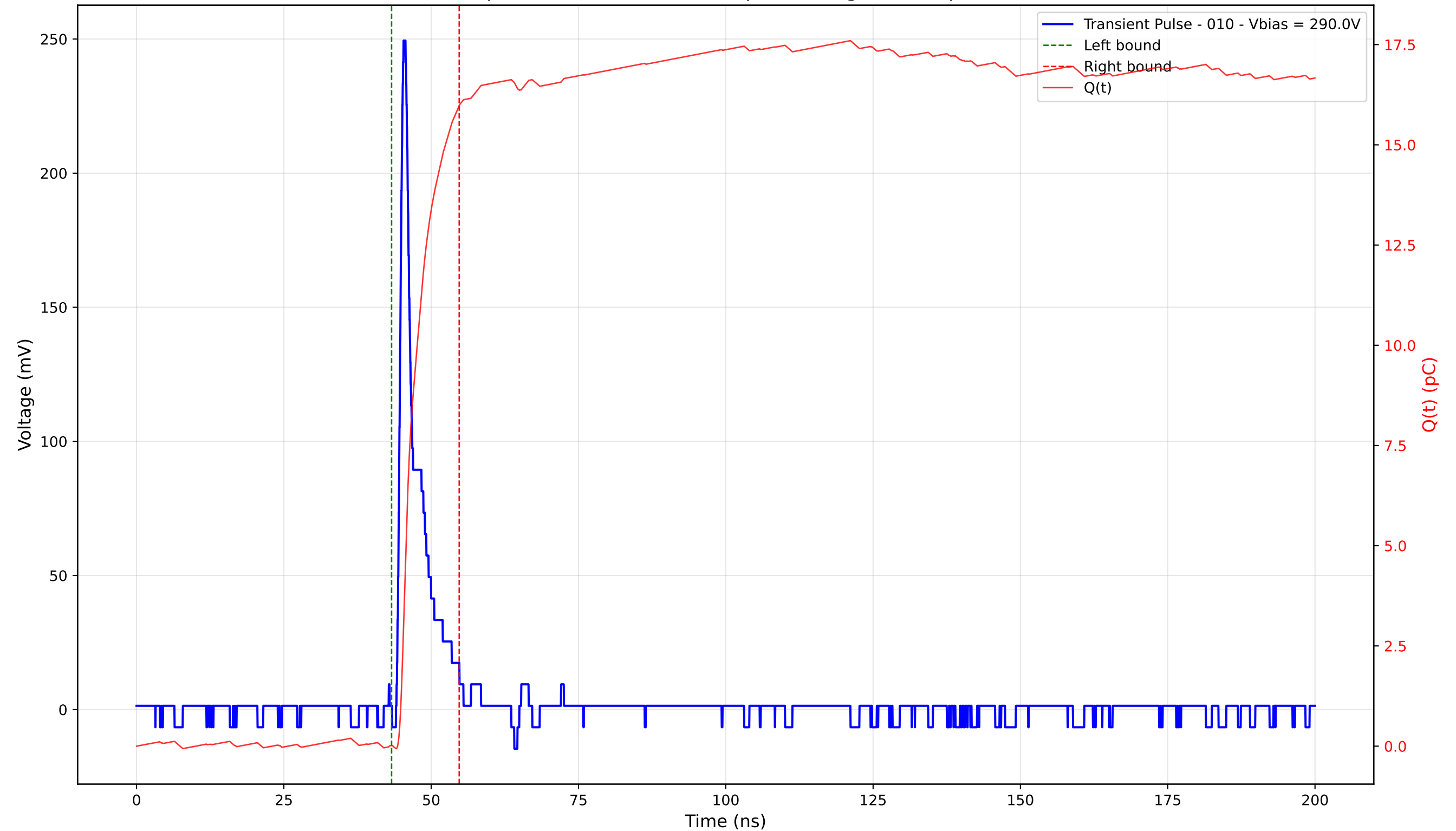
Transient Pulse - Sample: 4003 - Position: 95.0 \mu\text{m} - Charge: 15.97 pC - Rise Time: 0.86 ns
