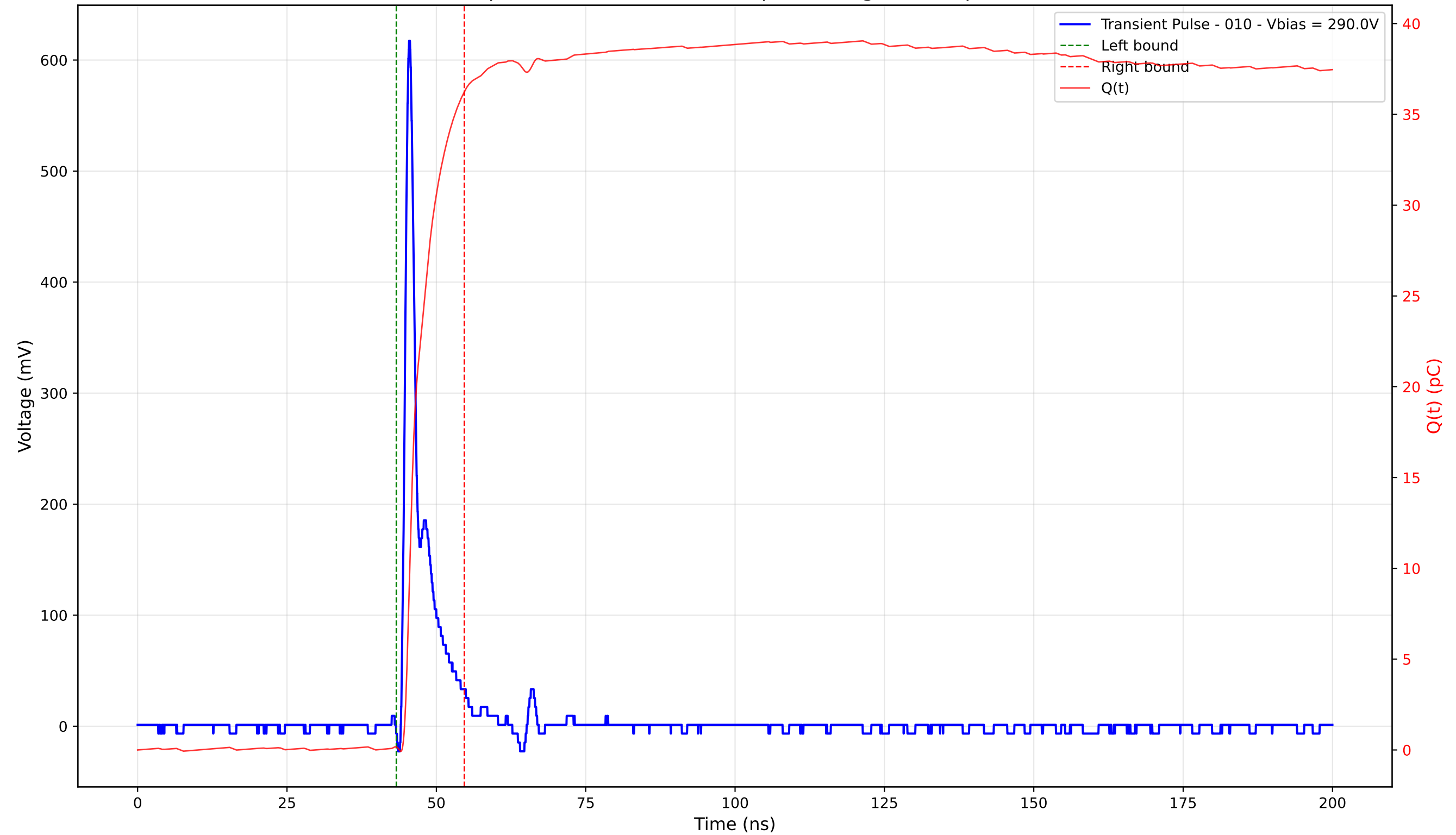
Transient Pulse - Sample: 4003 - Position: 145.0 \mu\text{m} - Charge: 36.07 pC - Rise Time: 0.91 ns
