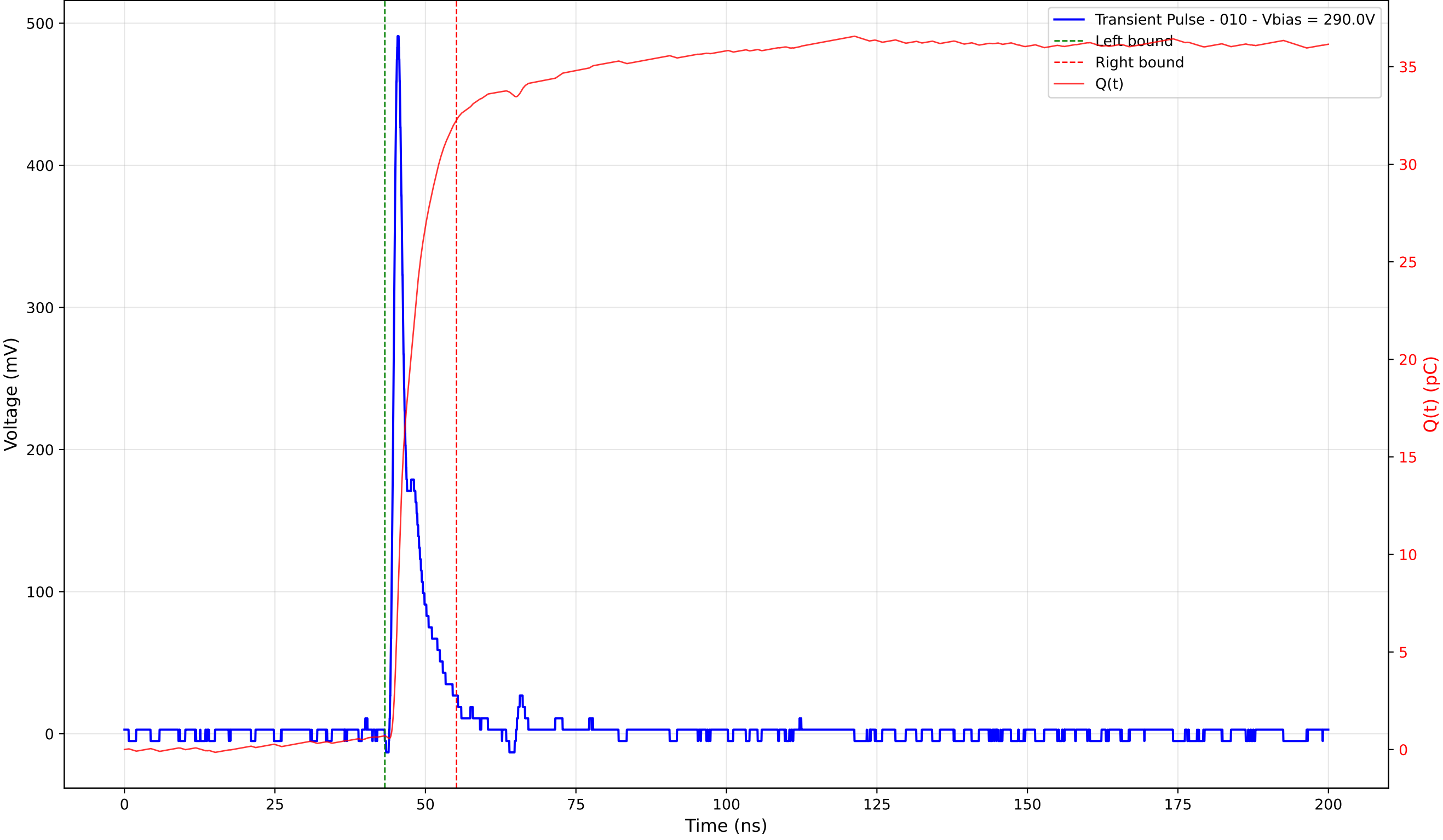
Transient Pulse - Sample: 4003 - Position: 110.0 \mu\text{m} - Charge: 31.57 pC - Rise Time: 0.90 ns
