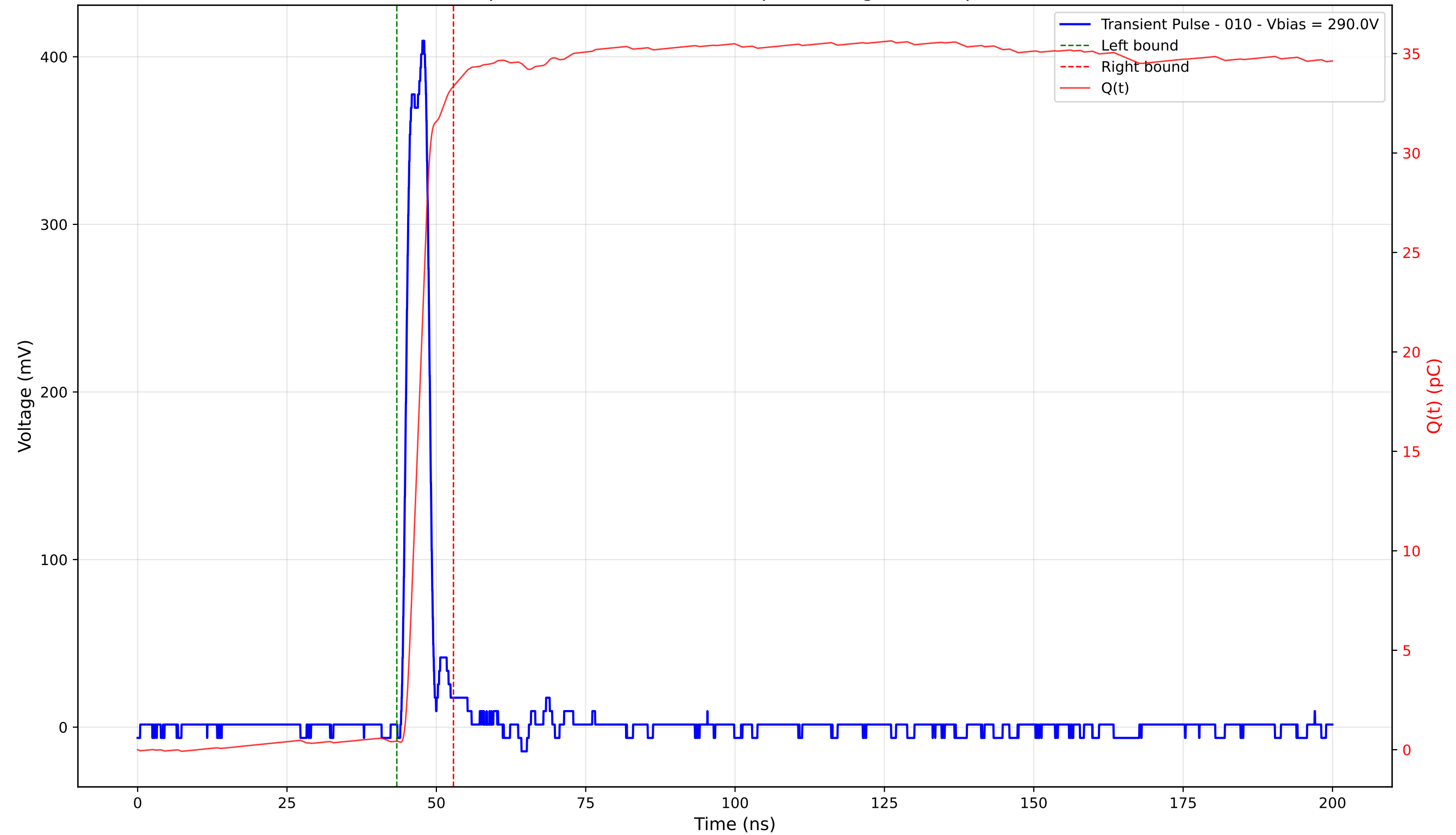
Transient Pulse - Sample: 4003 - Position: 335.0 \mu\text{m} - Charge: 32.92 pC - Rise Time: 1.40 ns
