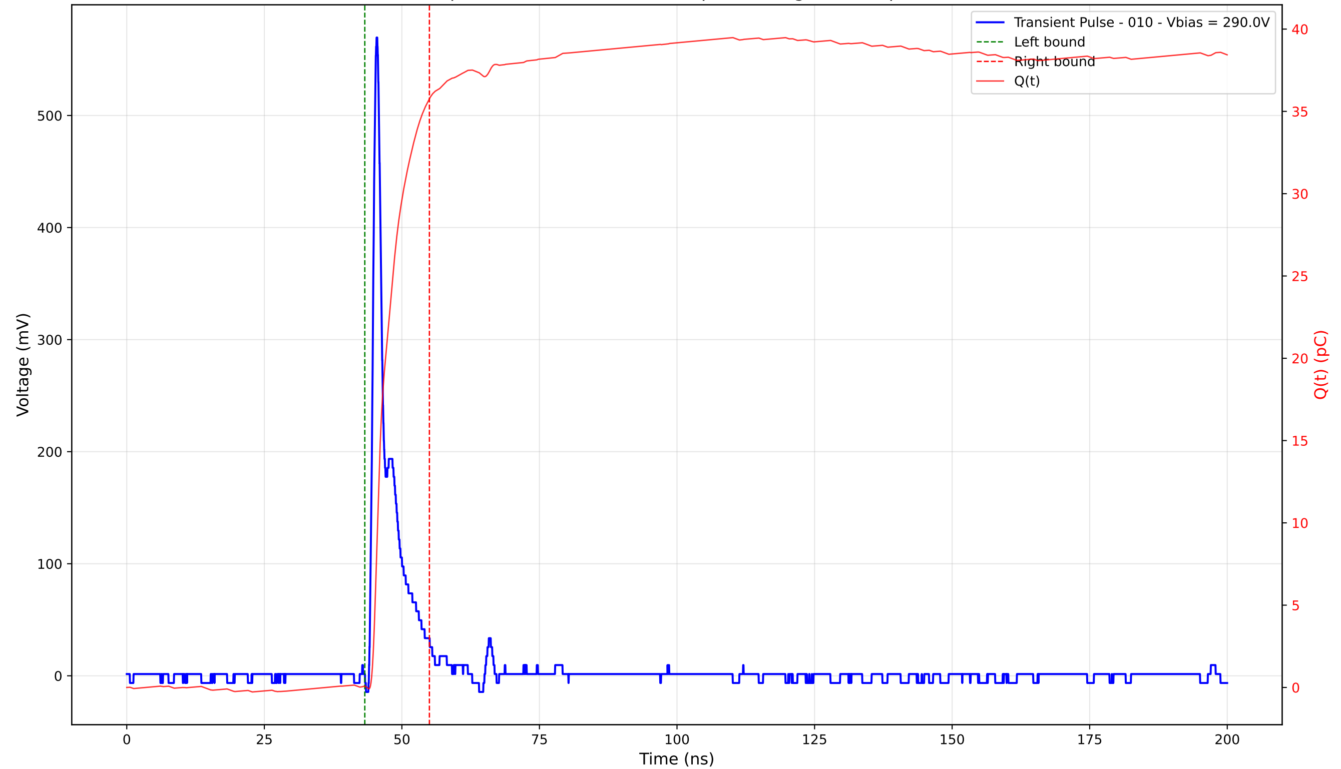
Transient Pulse - Sample: 4003 - Position: 120.0 \mu\text{m} - Charge: 35.70 pC - Rise Time: 0.90 ns
