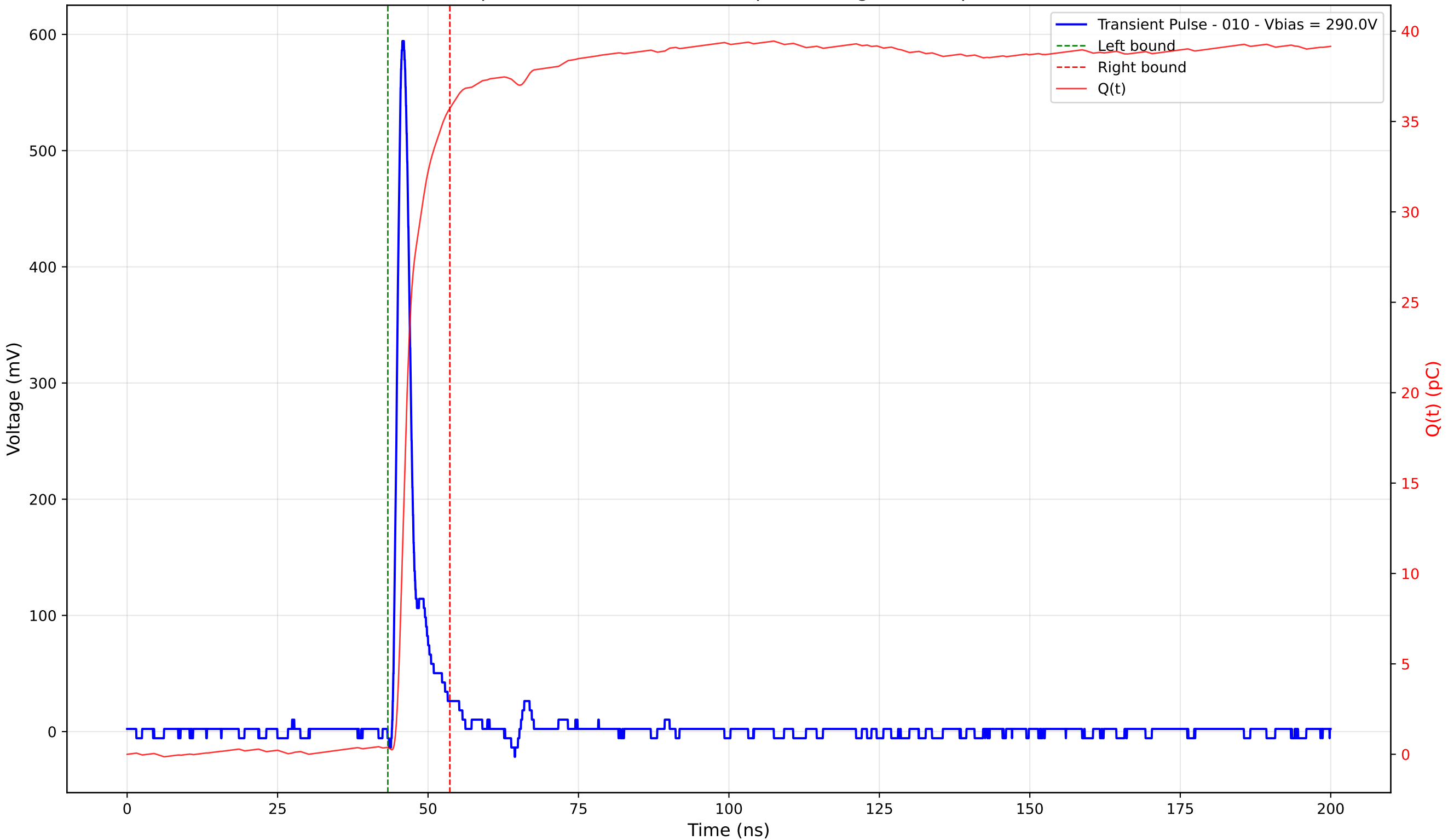
Transient Pulse - Sample: 4003 - Position: 230.0 \mu\text{m} - Charge: 35.35 pC - Rise Time: 1.10 ns
