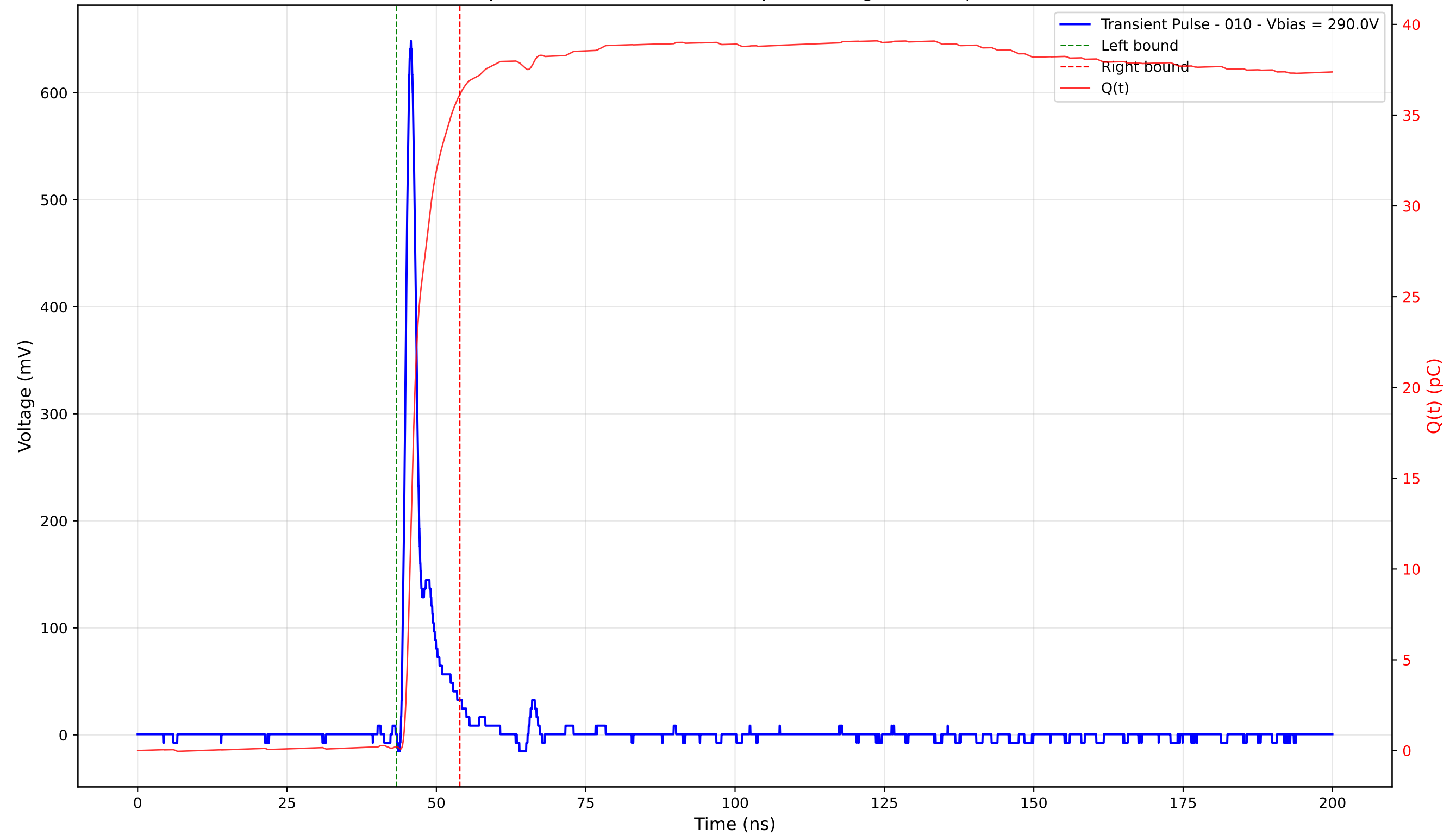
Transient Pulse - Sample: 4003 - Position: 200.0 \mu\text{m} - Charge: 35.91 pC - Rise Time: 1.04 ns
