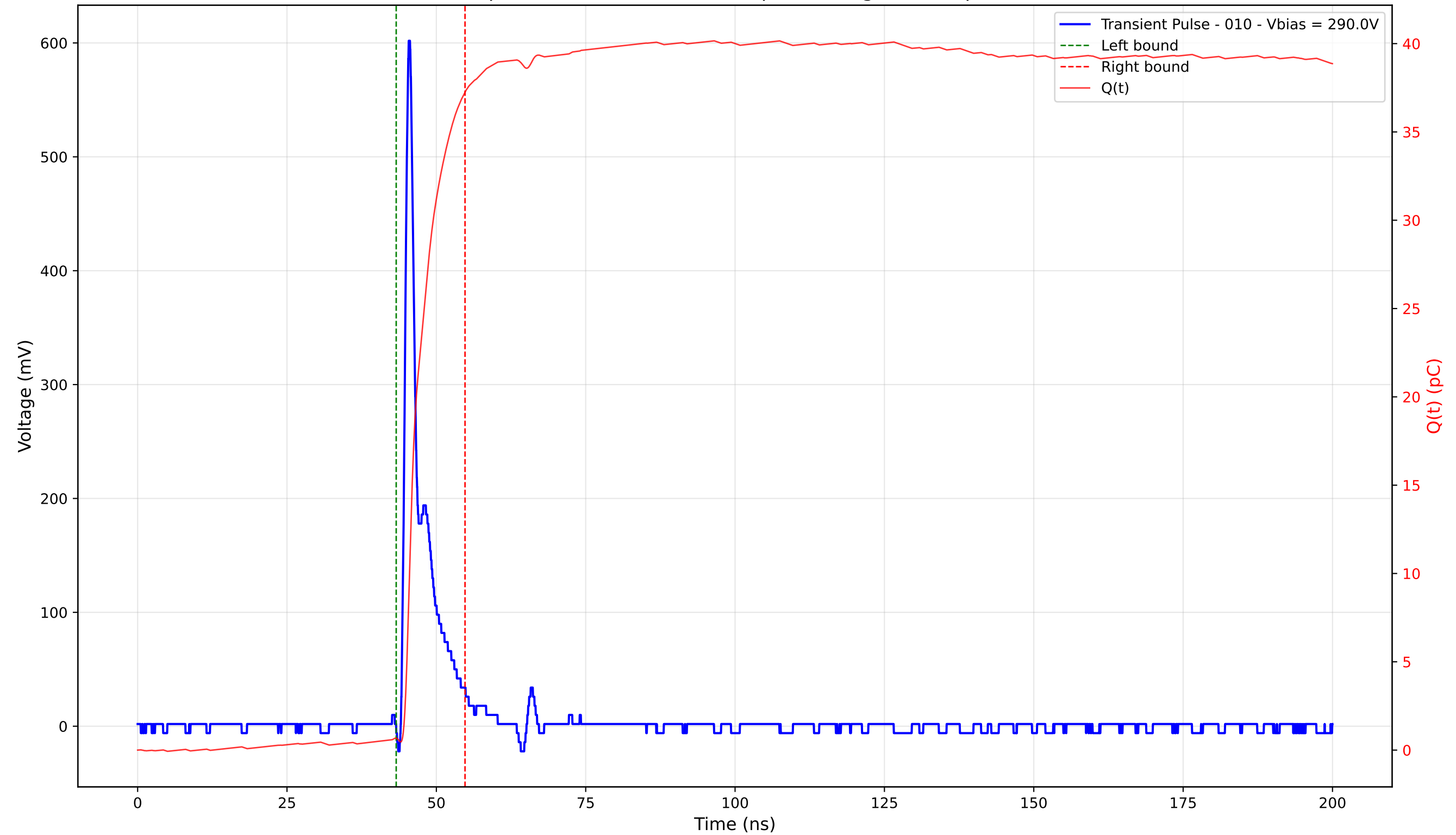
Transient Pulse - Sample: 4003 - Position: 135.0 \mu\text{m} - Charge: 36.58 pC - Rise Time: 0.88 ns
