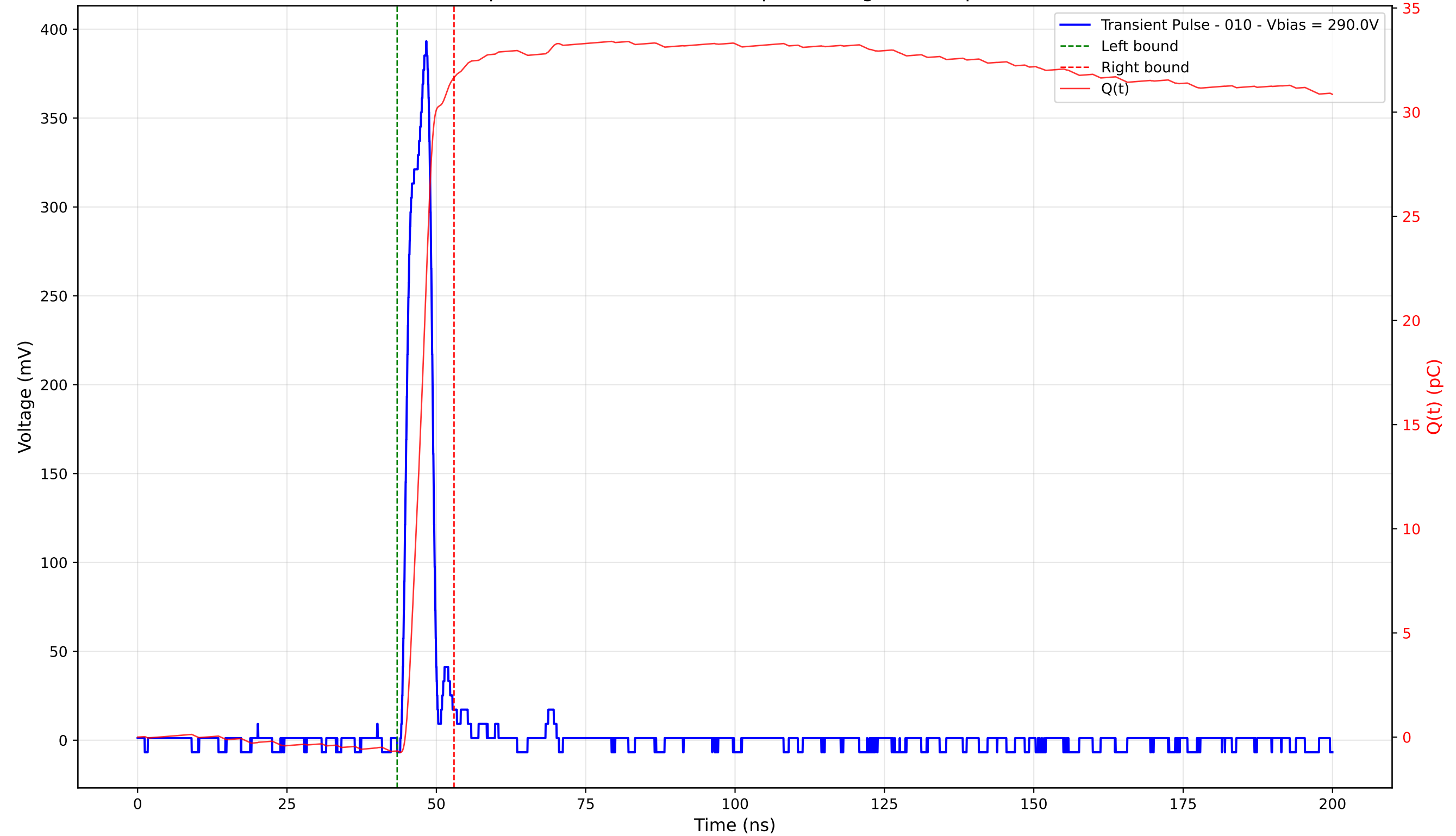
Transient Pulse - Sample: 4003 - Position: 355.0 \mu\text{m} - Charge: 32.32 pC - Rise Time: 3.18 ns
