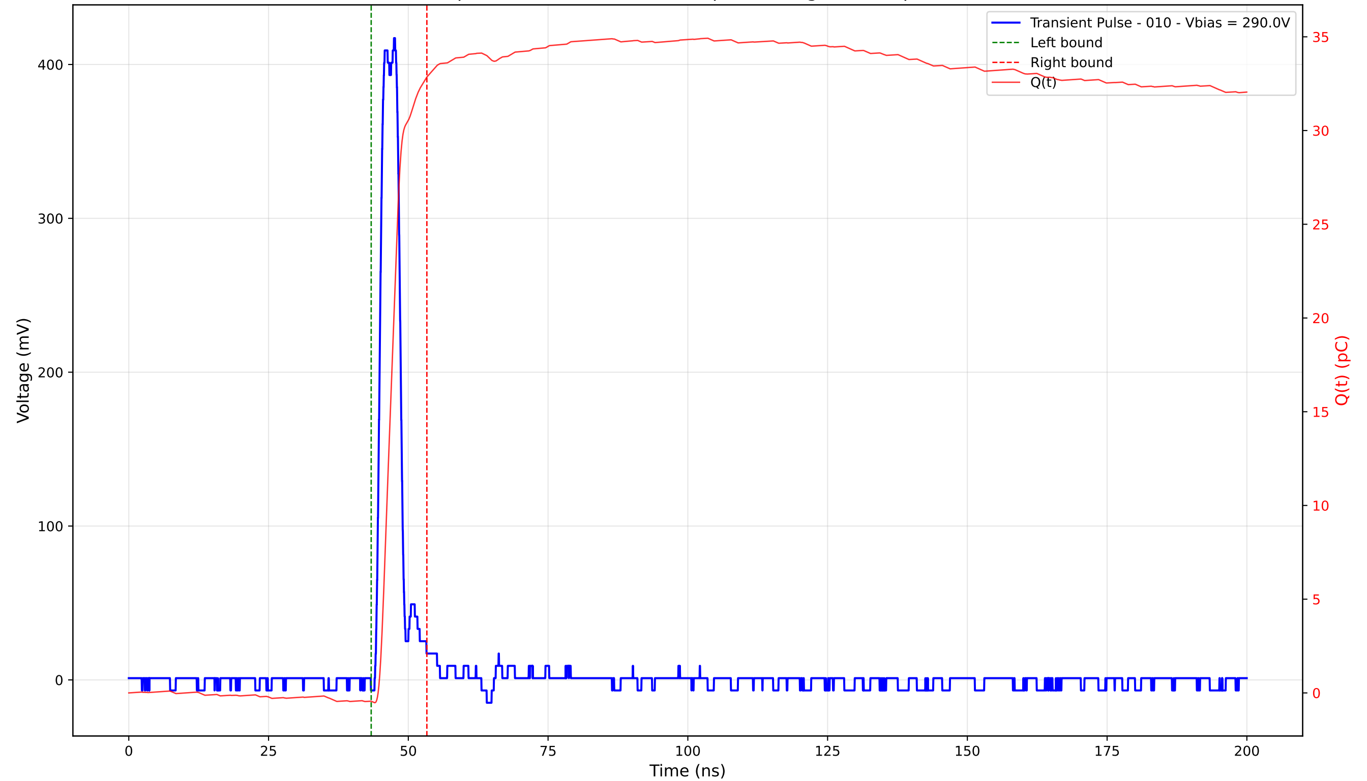
Transient Pulse - Sample: 4003 - Position: 320.0 \mu\text{m} - Charge: 33.30 pC - Rise Time: 1.16 ns
