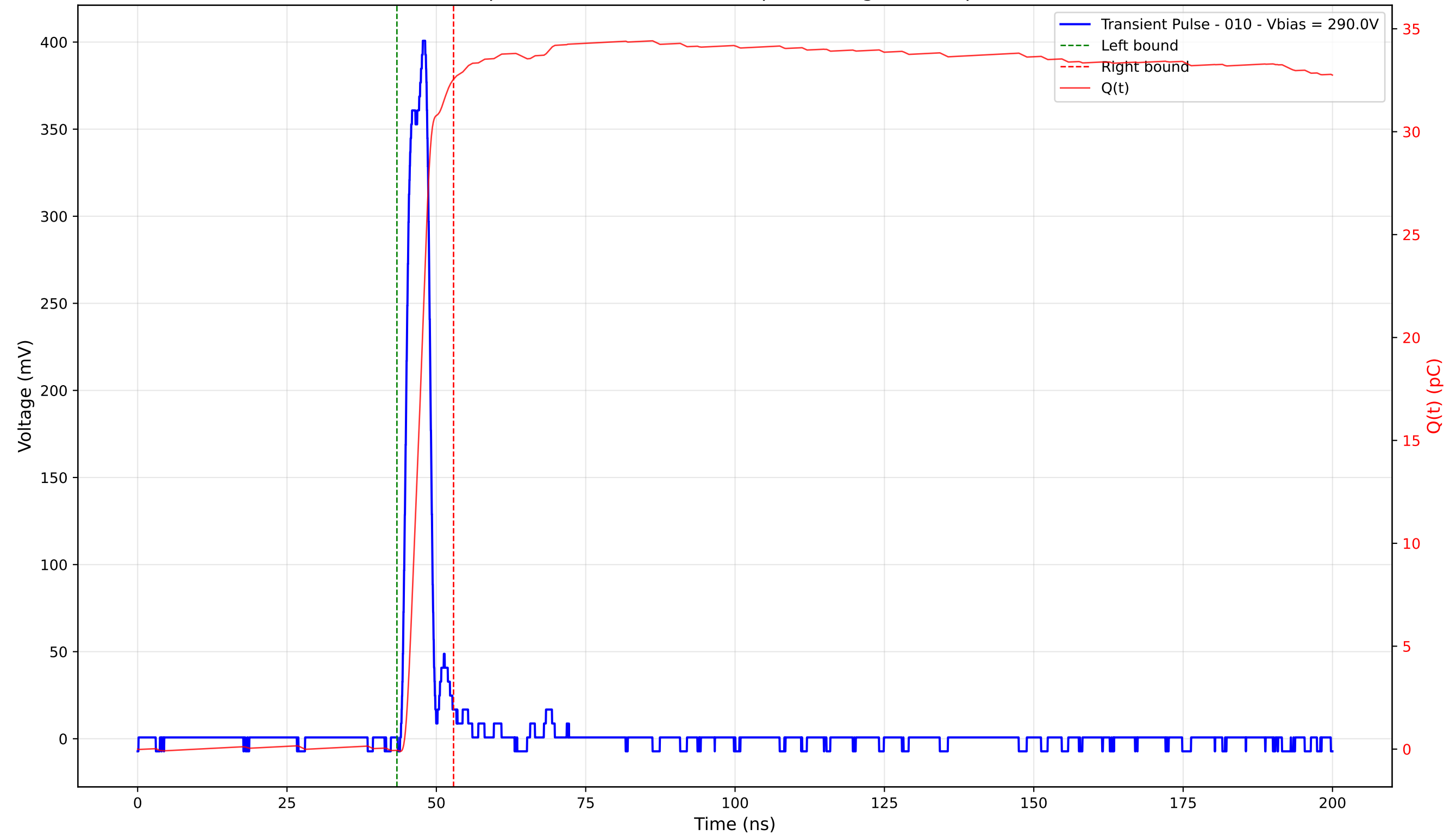
Transient Pulse - Sample: 4003 - Position: 340.0 \mu\text{m} - Charge: 32.61 pC - Rise Time: 1.56 ns
