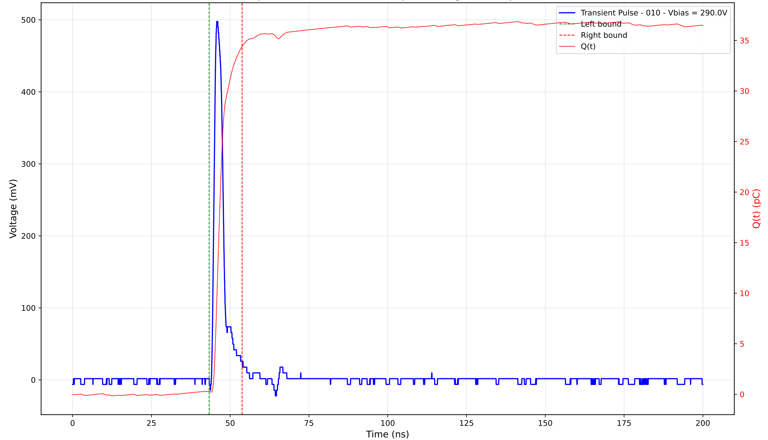
Transient Pulse - Sample: 4003 - Position: 275.0 \mu\text{m} - Charge: 34.11 pC - Rise Time: 1.08 ns
