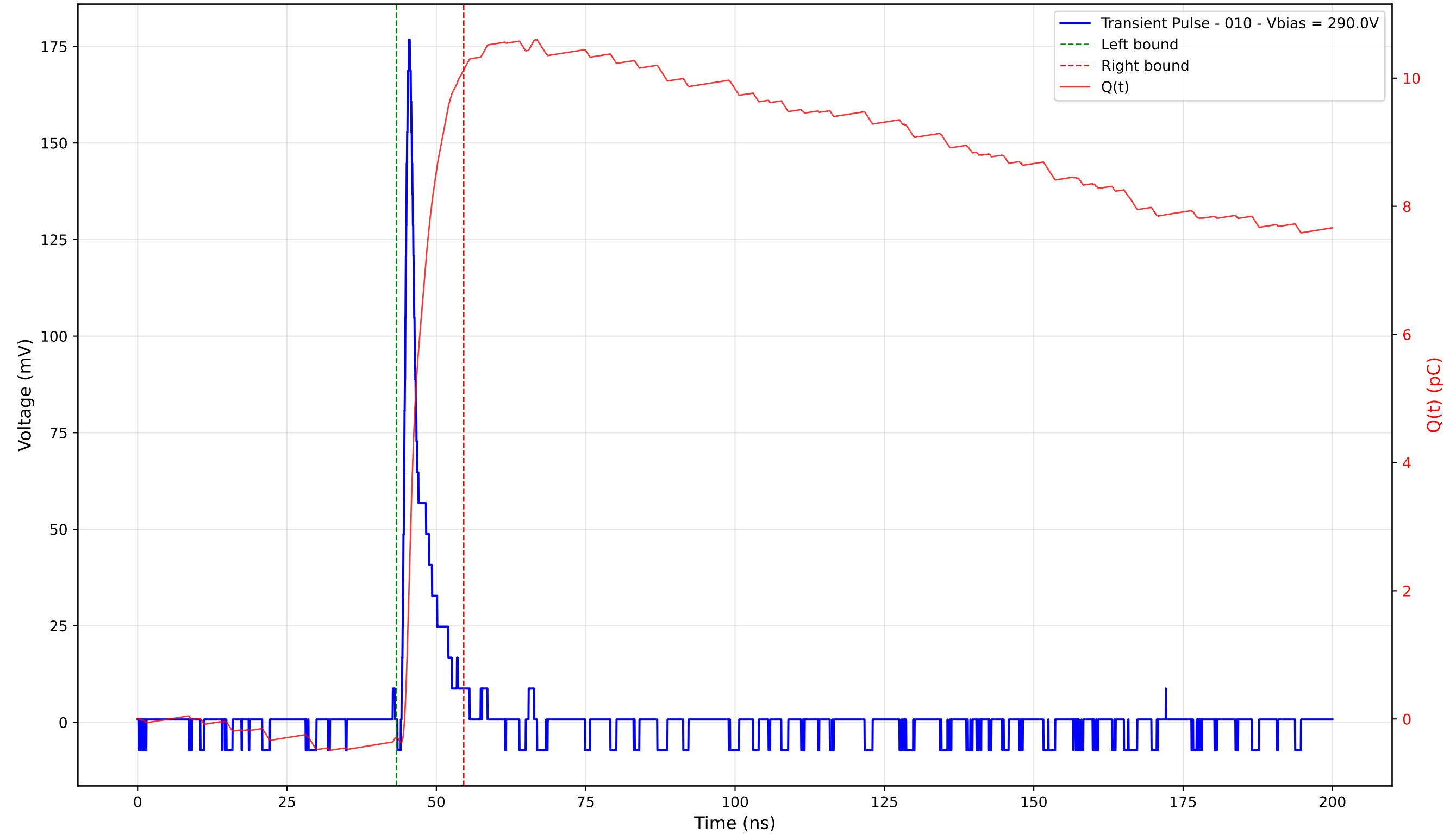
Transient Pulse - Sample: 4003 - Position: 90.0 \mu\text{m} - Charge: 10.42 pC - Rise Time: 0.86 ns
