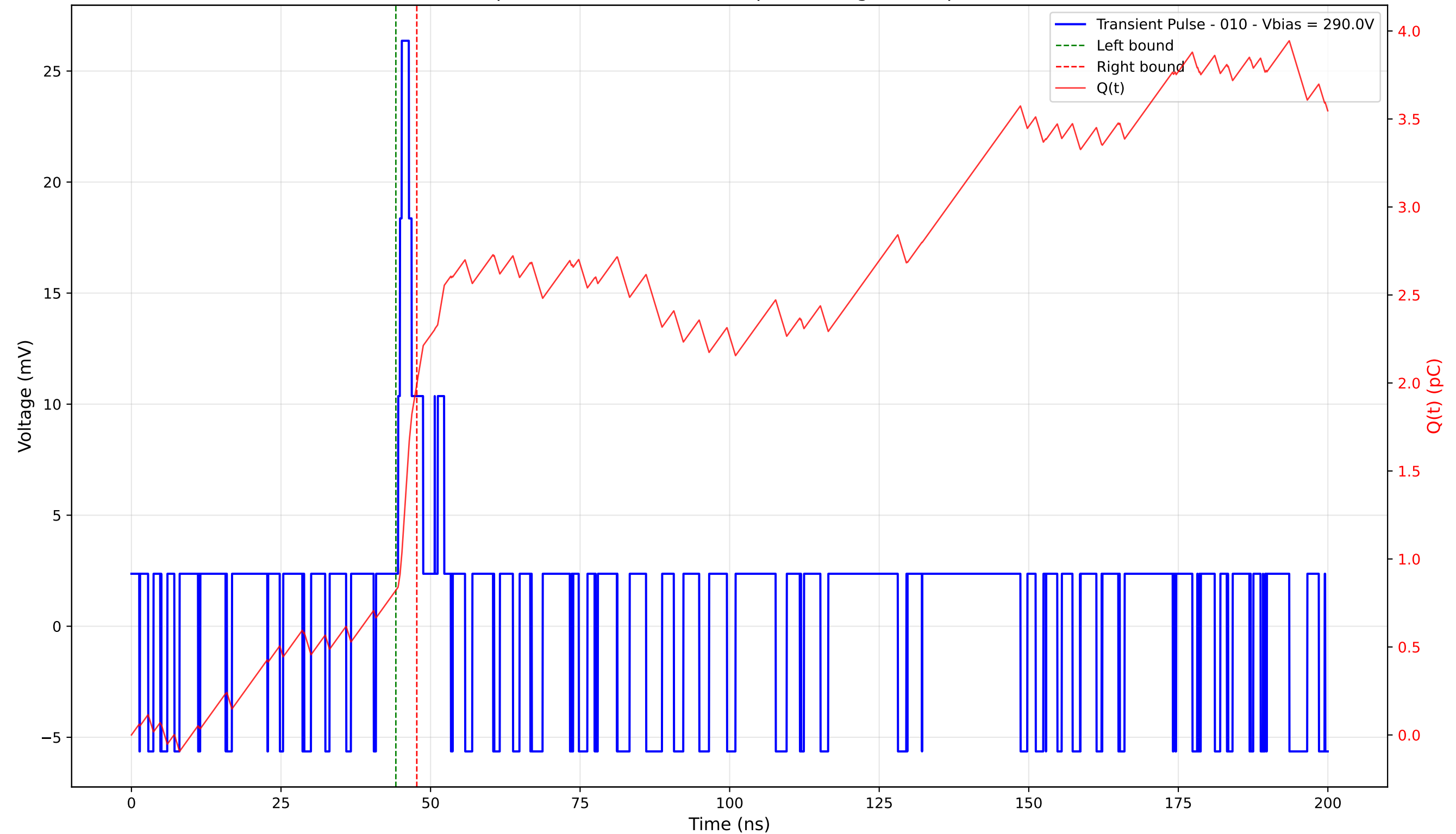
Transient Pulse - Sample: 4003 - Position: 15.0 \mu\text{m} - Charge: 1.17 pC - Rise Time: 0.62 ns
