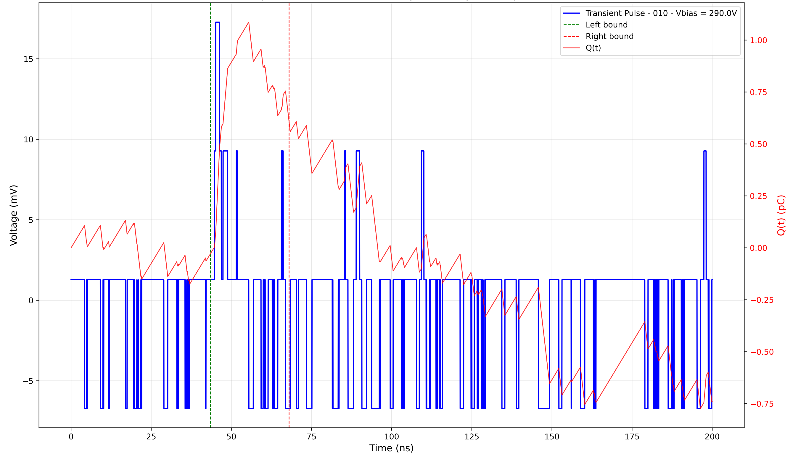
Transient Pulse - Sample: 4003 - Position: 425.0 \mu\text{m} - Charge: 0.64 pC - Rise Time: 0.38 ns
