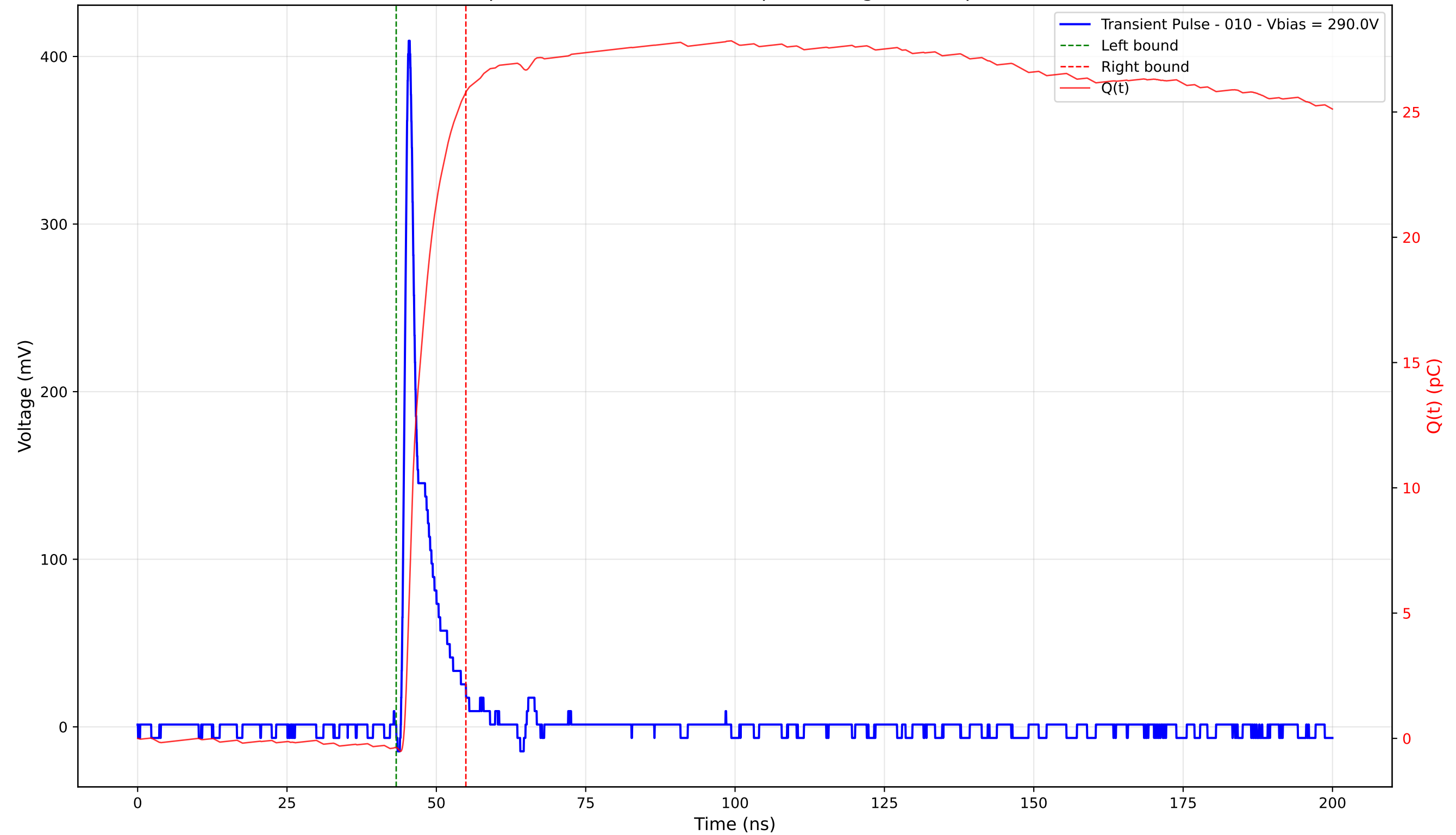
Transient Pulse - Sample: 4003 - Position: 105.0 \mu\text{m} - Charge: 26.16 pC - Rise Time: 0.90 ns
