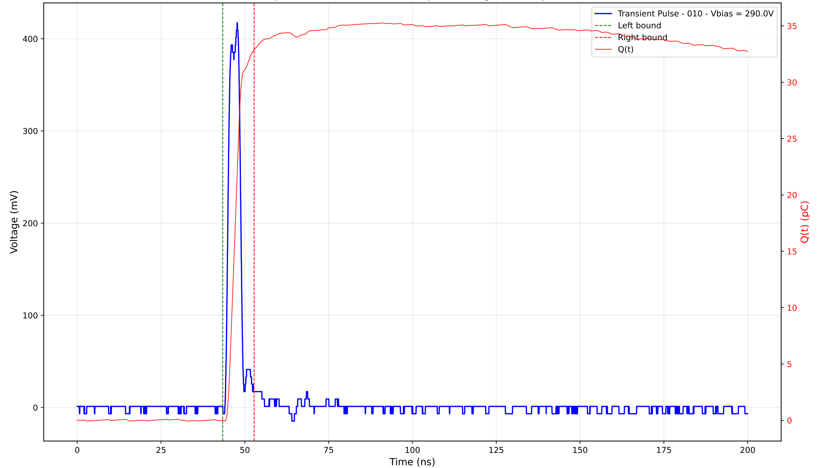
Transient Pulse - Sample: 4003 - Position: 330.0 \mu\text{m} - Charge: 32.87 pC - Rise Time: 1.32 ns
