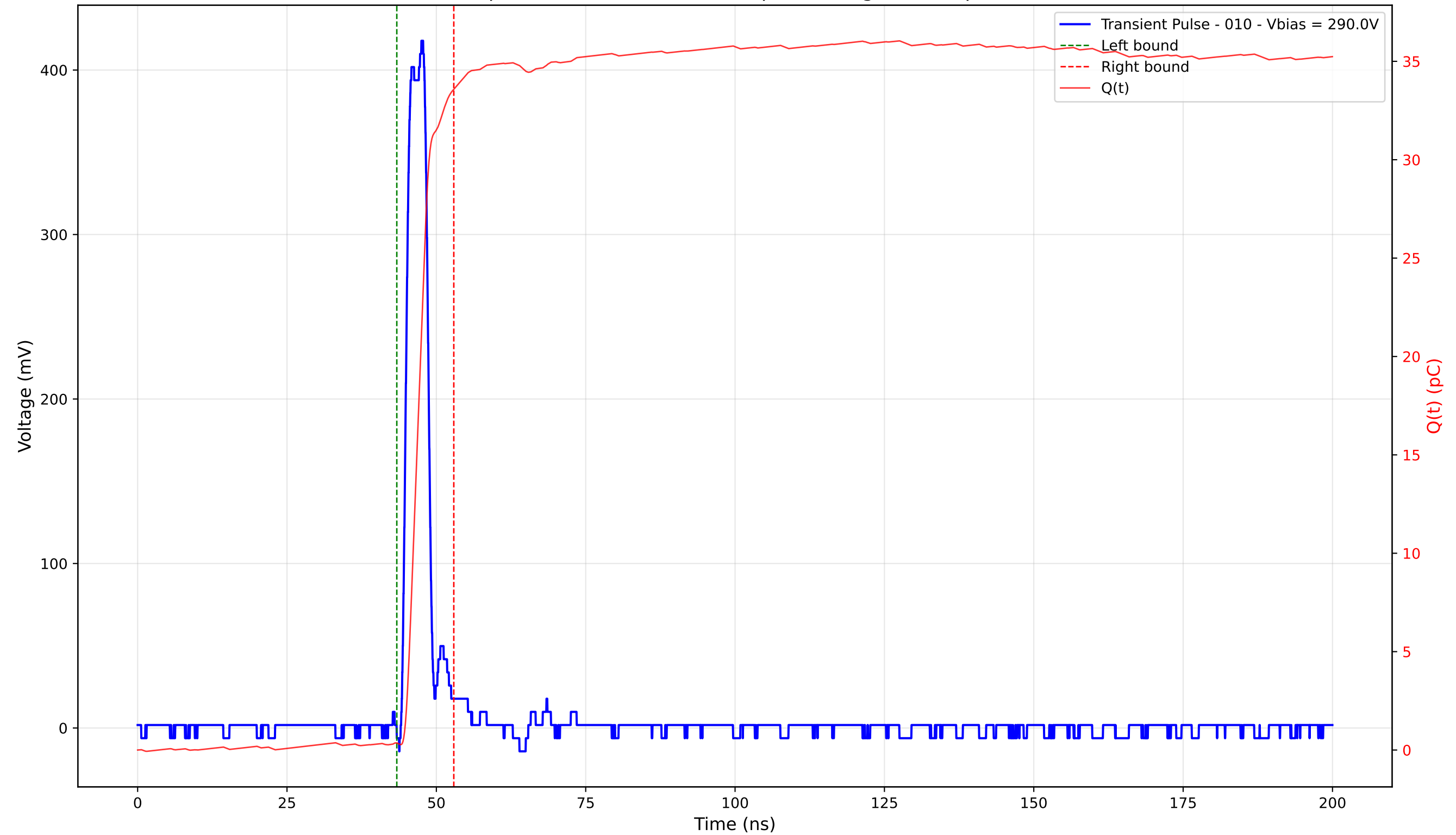
Transient Pulse - Sample: 4003 - Position: 325.0 \mu\text{m} - Charge: 33.22 pC - Rise Time: 1.22 ns
