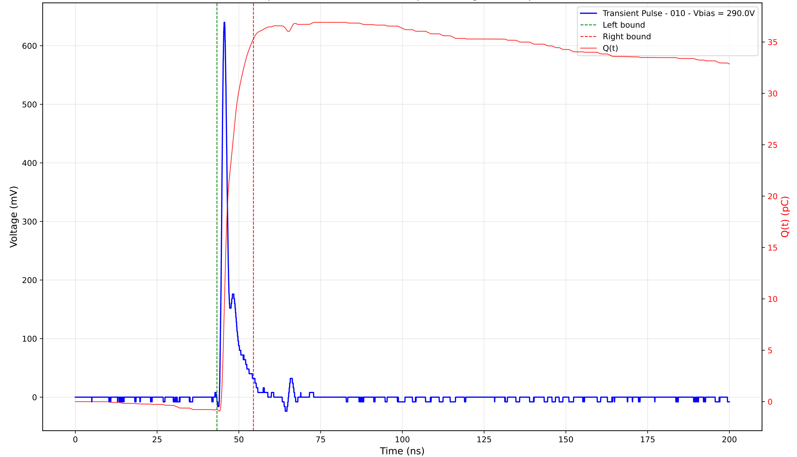
Transient Pulse - Sample: 4003 - Position: 165.0 \mu\text{m} - Charge: 36.06 pC - Rise Time: 0.94 ns
