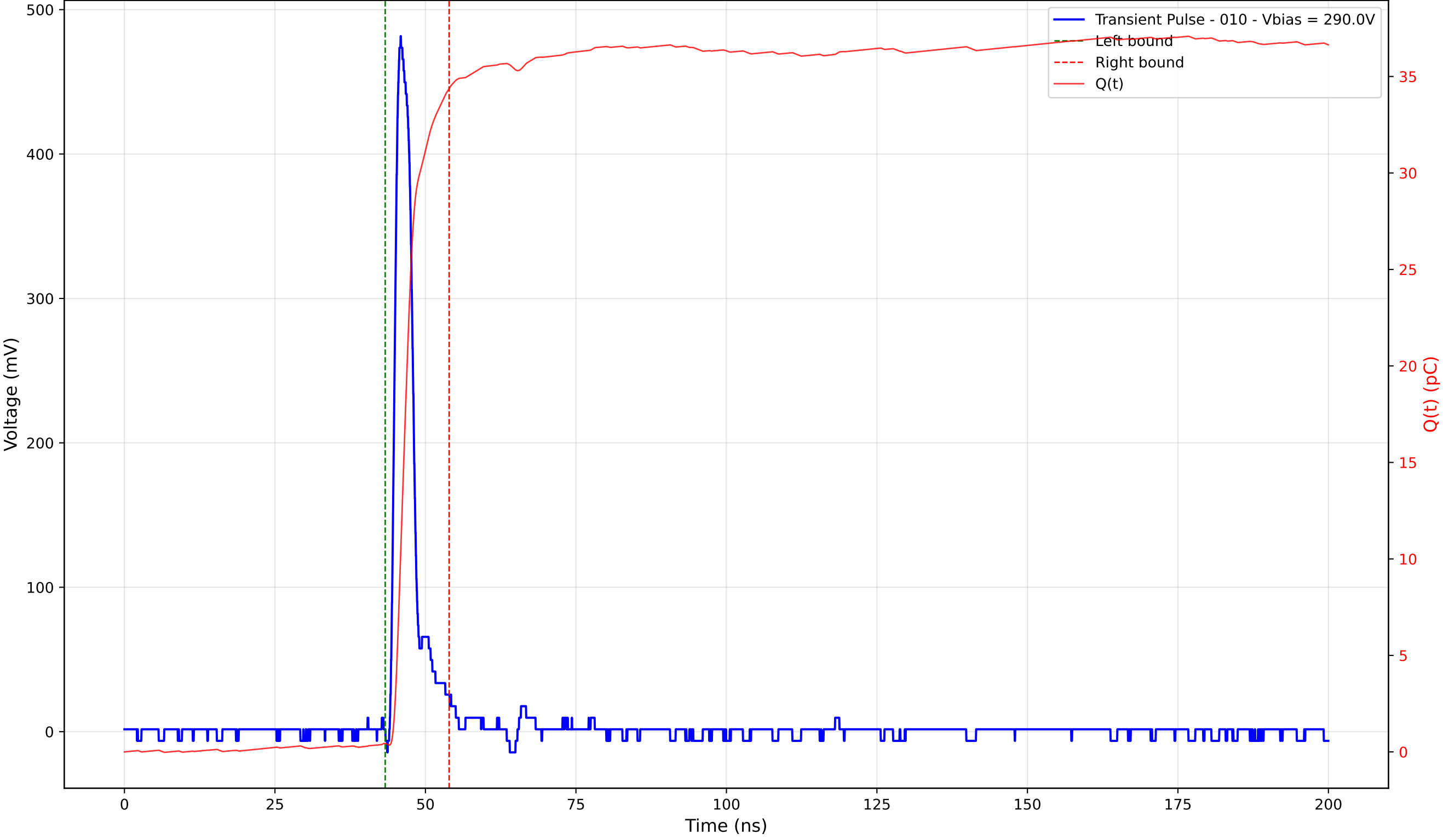
Transient Pulse - Sample: 4003 - Position: 285.0 \mu\text{m} - Charge: 33.94 pC - Rise Time: 1.10 ns
