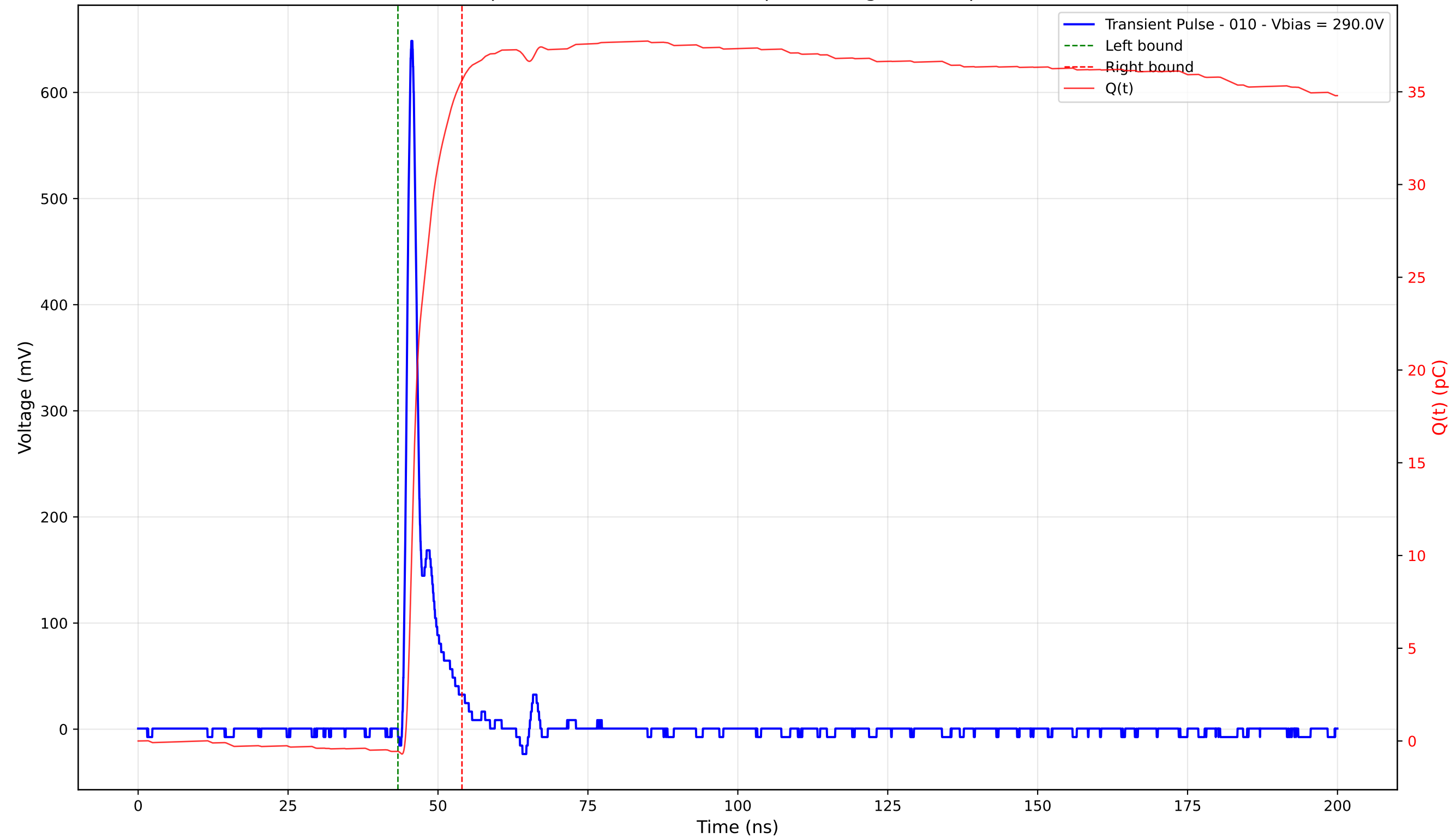
Transient Pulse - Sample: 4003 - Position: 180.0 \mu\text{m} - Charge: 36.17 pC - Rise Time: 1.00 ns
