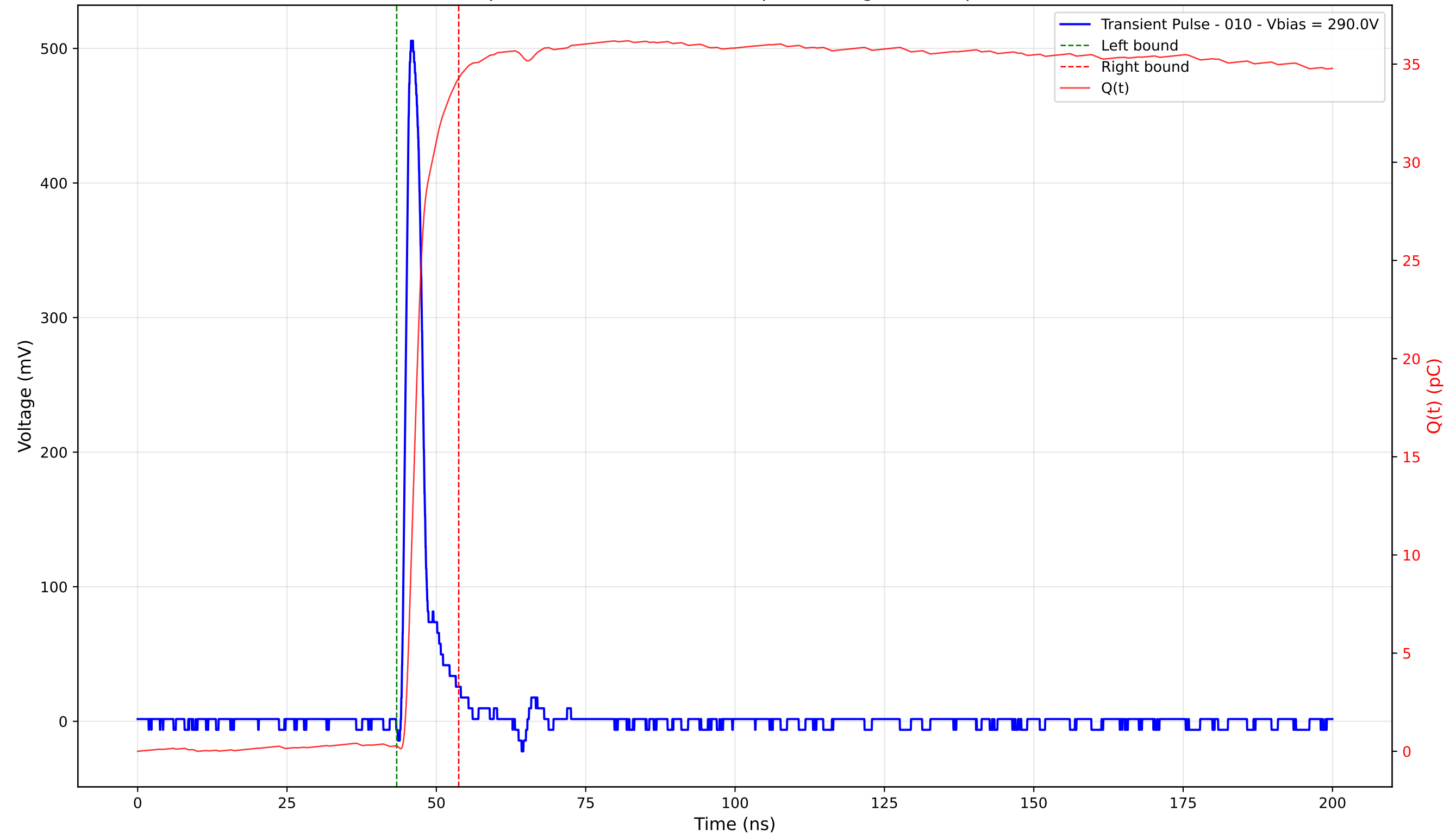
Transient Pulse - Sample: 4003 - Position: 270.0 \mu\text{m} - Charge: 34.02 pC - Rise Time: 1.07 ns
