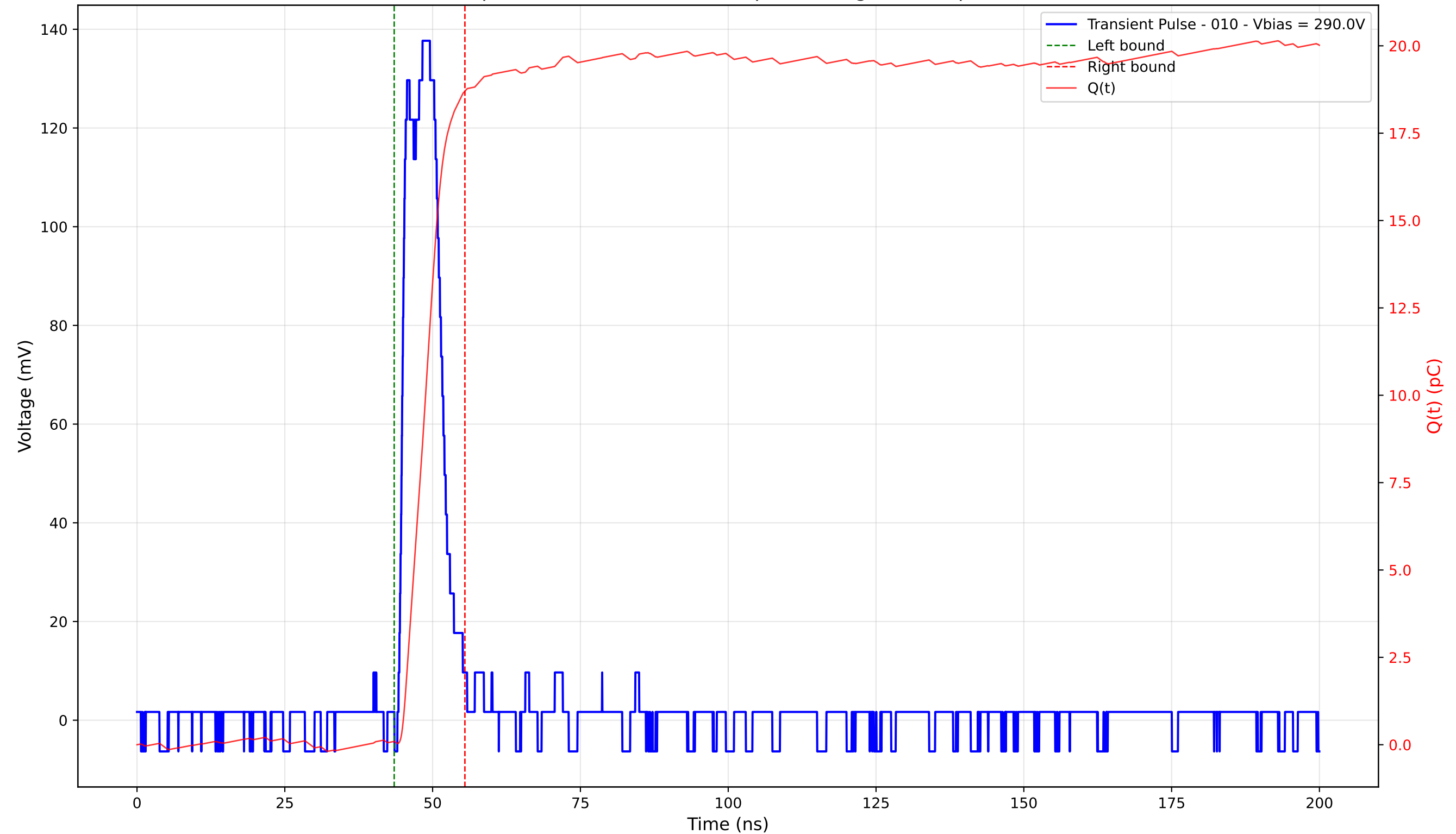
Transient Pulse - Sample: 4003 - Position: 395.0 \mu\text{m} - Charge: 18.61 pC - Rise Time: 1.29 ns
