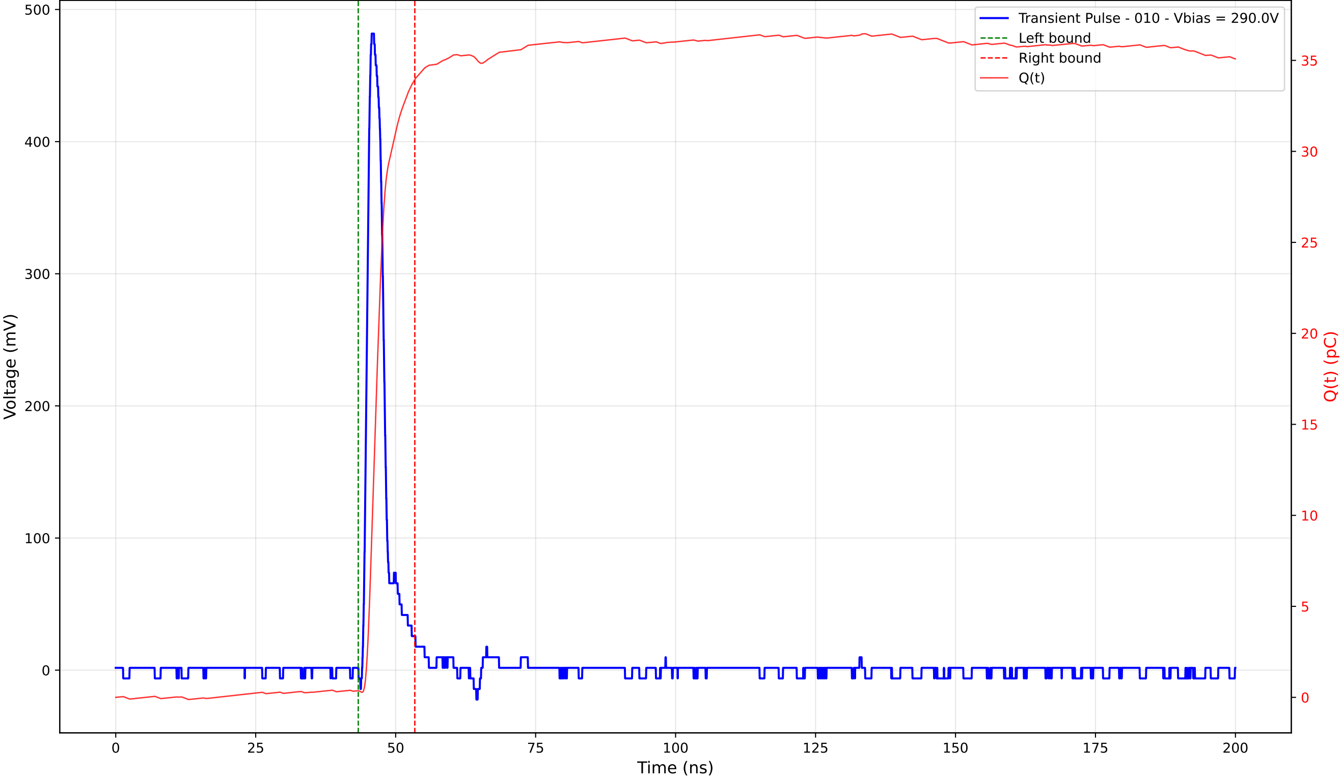
Transient Pulse - Sample: 4003 - Position: 280.0 \mu\text{m} - Charge: 33.58 pC - Rise Time: 1.08 ns
