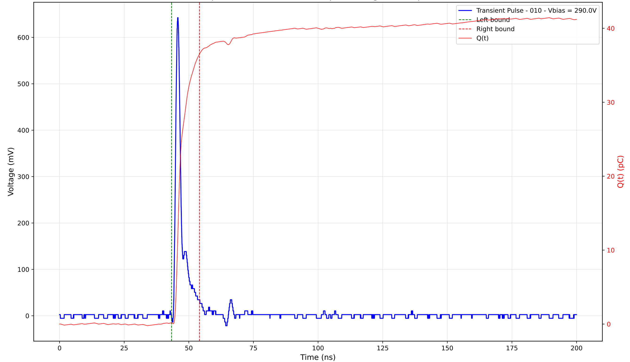
Transient Pulse - Sample: 4003 - Position: 205.0 \mu\text{m} - Charge: 36.35 pC - Rise Time: 1.05 ns
