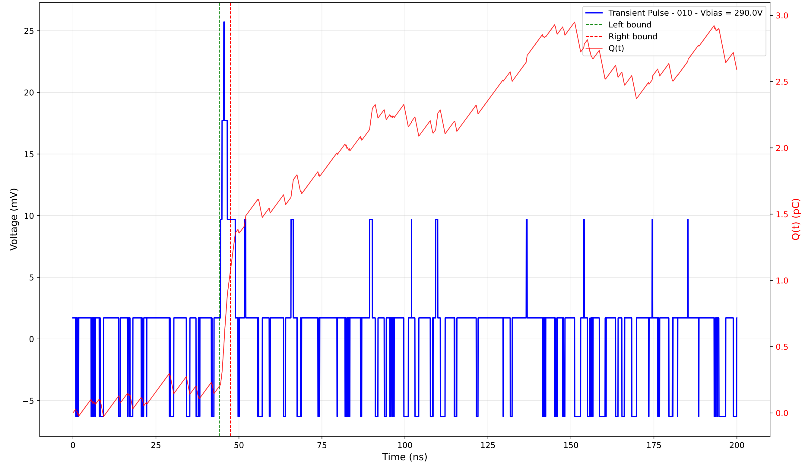
Transient Pulse - Sample: 4003 - Position: 10.0 \mu\text{m} - Charge: 0.87 pC - Rise Time: 1.00 ns
