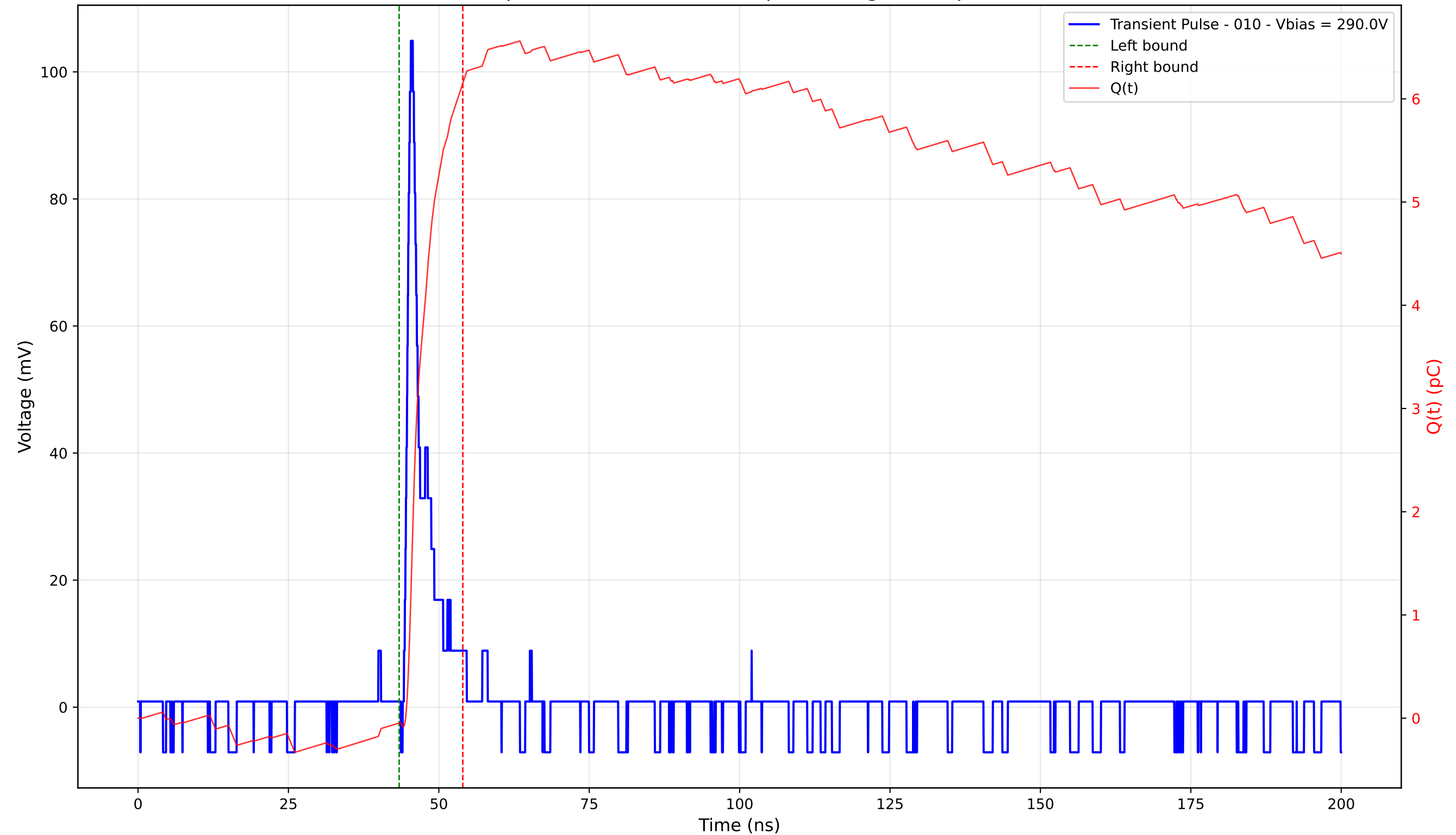
Transient Pulse - Sample: 4003 - Position: 85.0 \mu\text{m} - Charge: 6.20 pC - Rise Time: 0.86 ns
