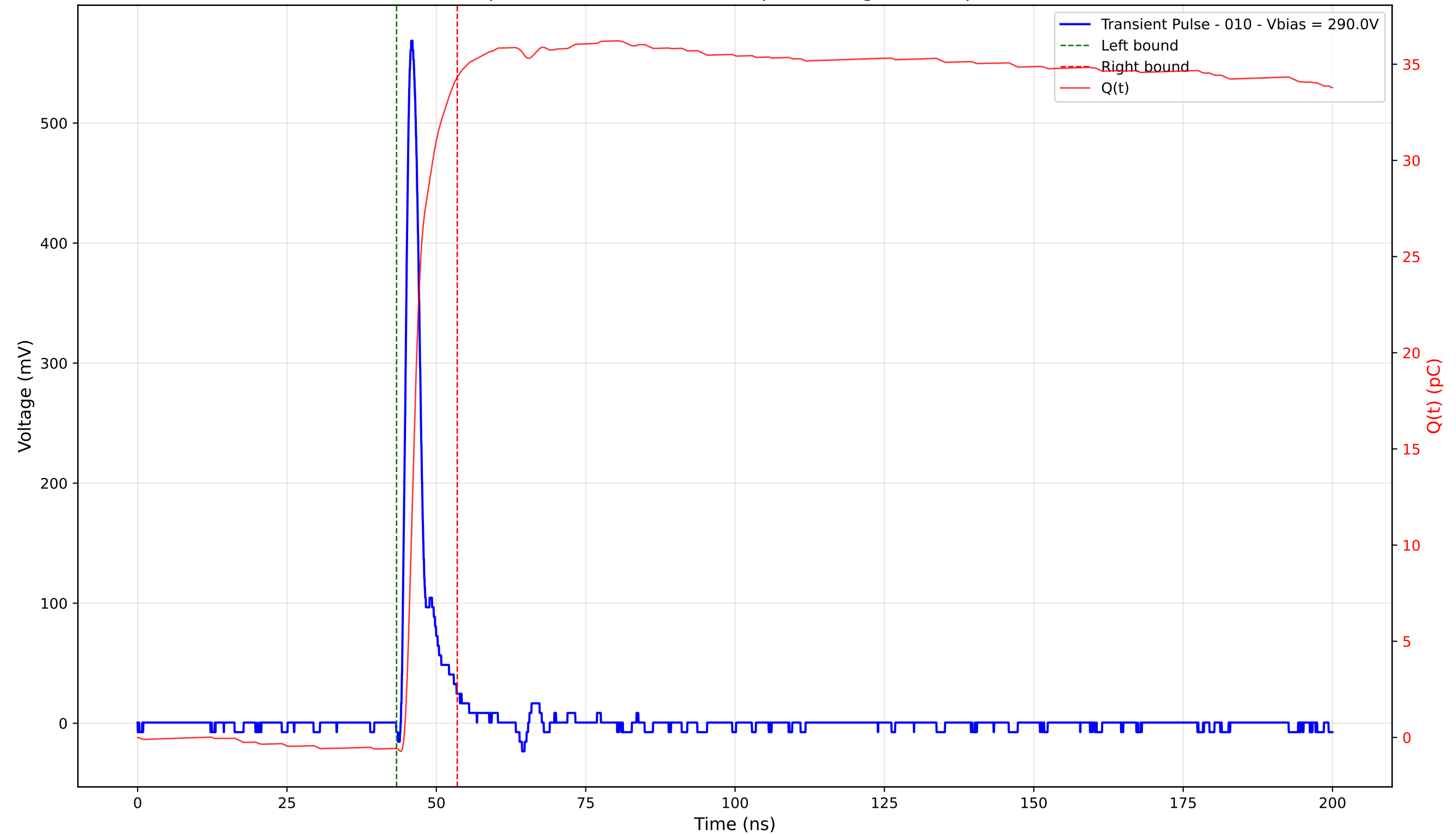
Transient Pulse - Sample: 4003 - Position: 245.0 \mu\text{m} - Charge: 34.90 pC - Rise Time: 1.10 ns
