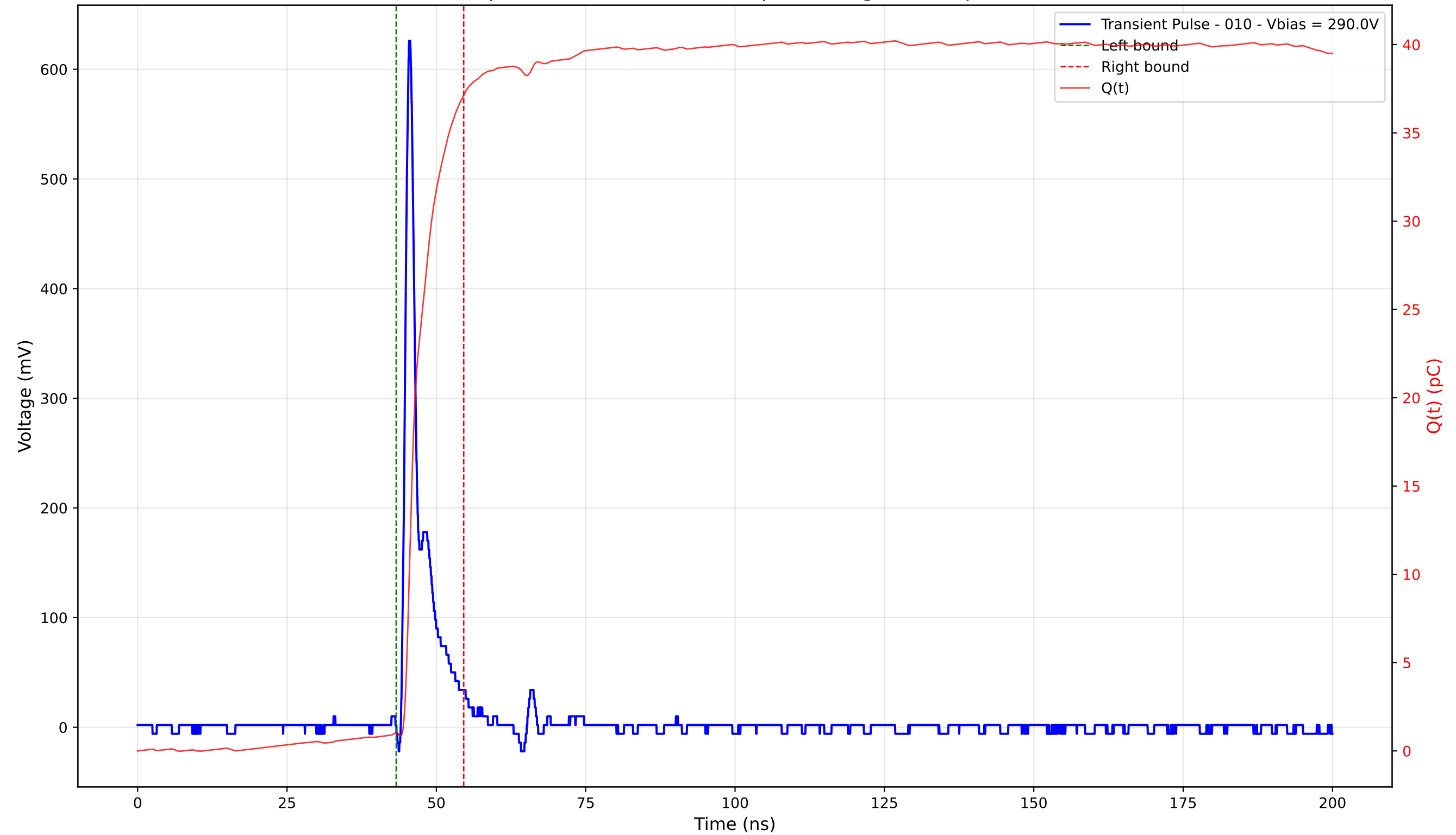
Transient Pulse - Sample: 4003 - Position: 155.0 \mu\text{m} - Charge: 36.11 pC - Rise Time: 0.93 ns
