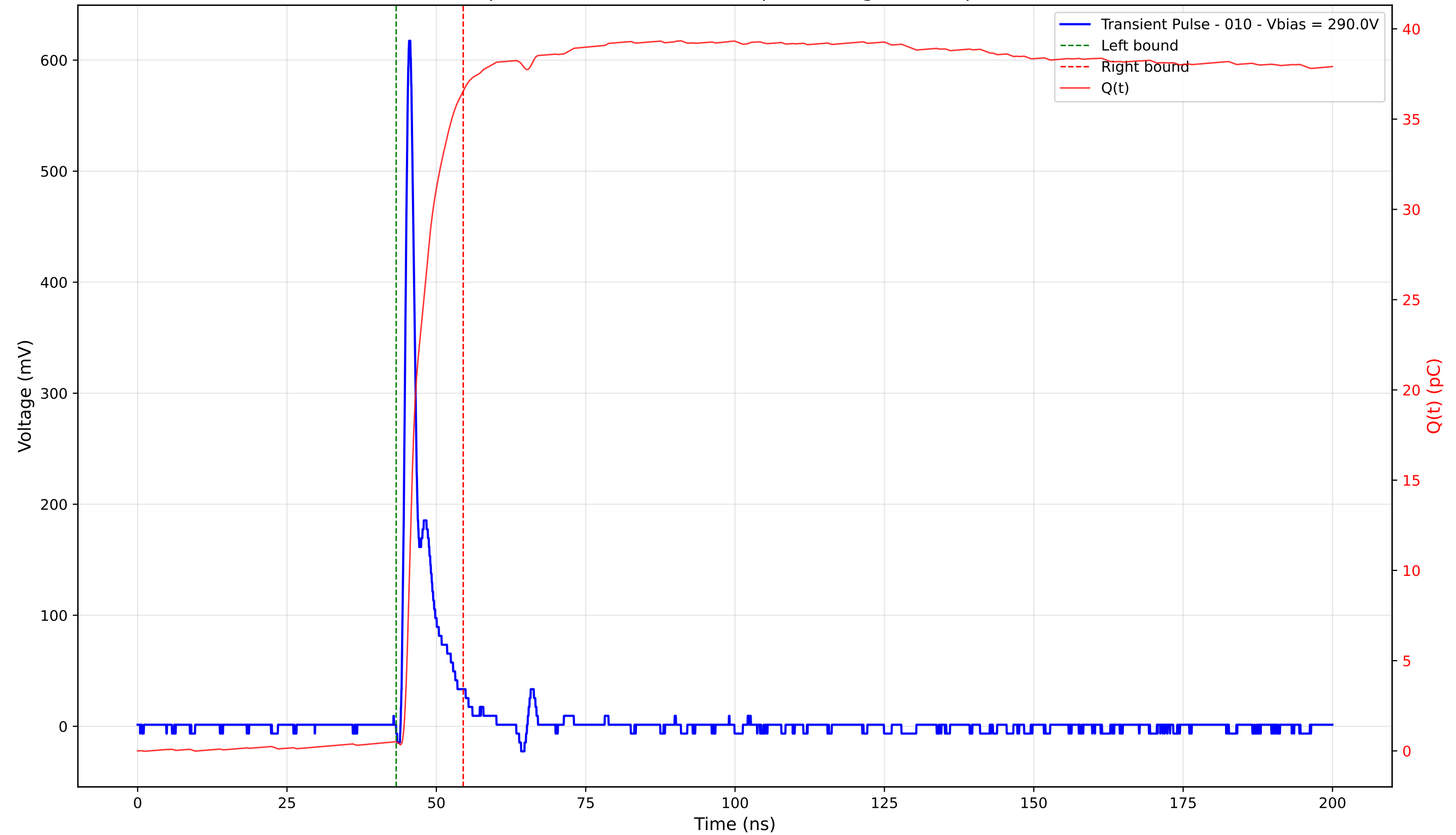
Transient Pulse - Sample: 4003 - Position: 150.0 \mu\text{m} - Charge: 36.05 pC - Rise Time: 0.91 ns
