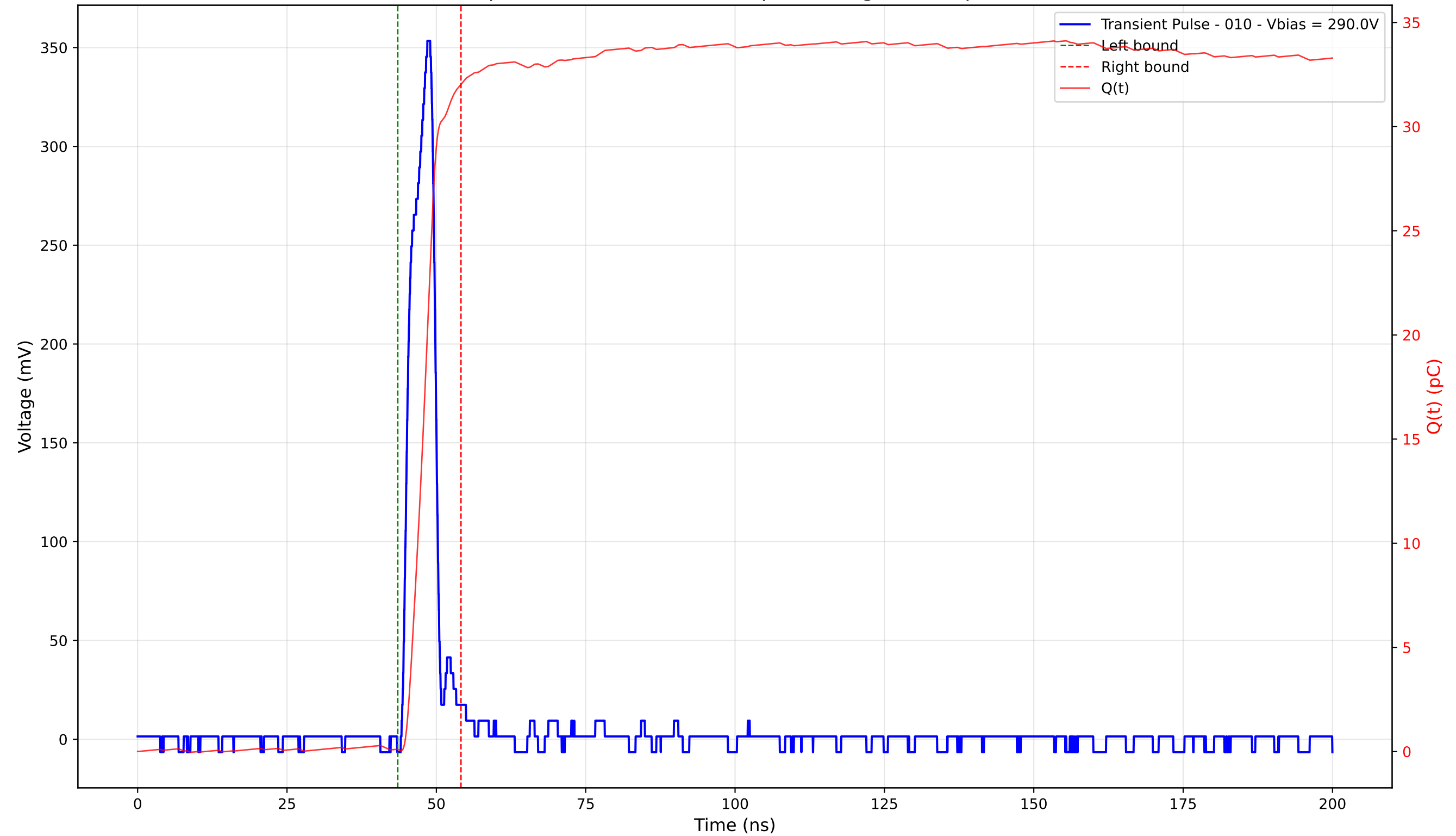
Transient Pulse - Sample: 4003 - Position: 370.0 \mu\text{m} - Charge: 31.93 pC - Rise Time: 3.32 ns
