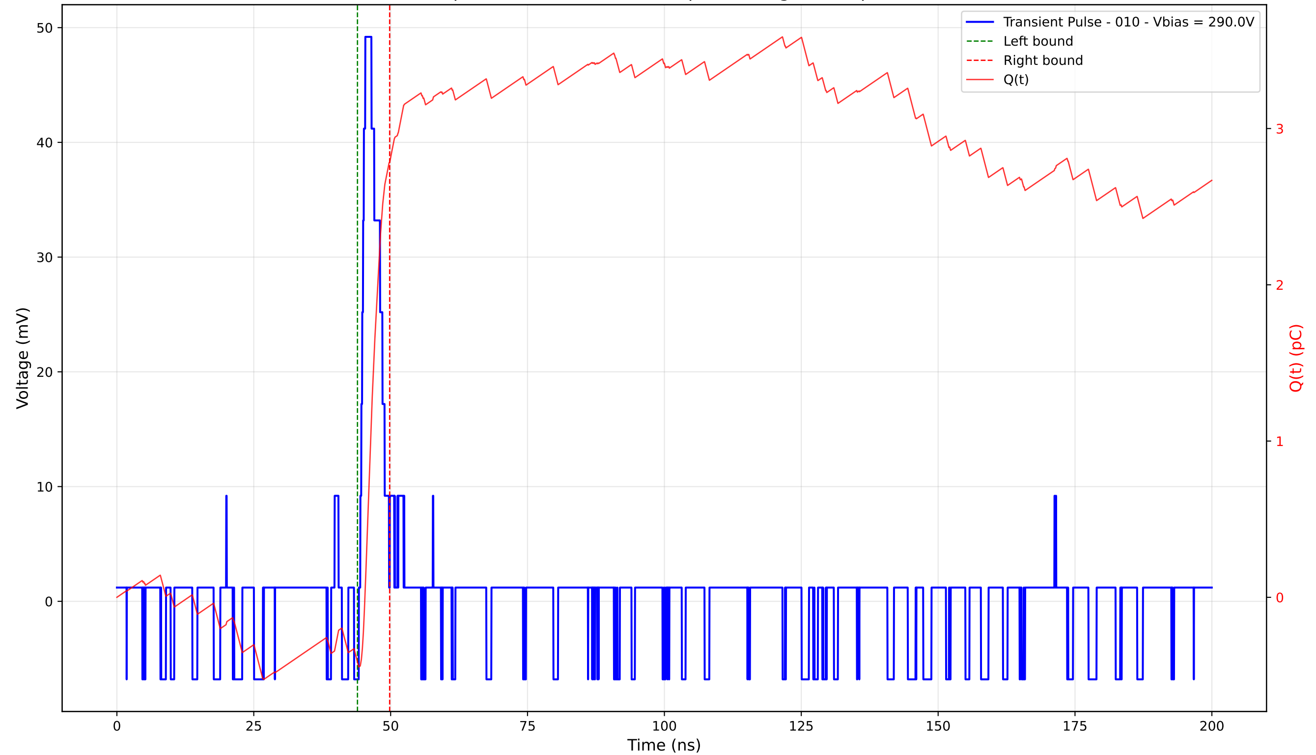
Transient Pulse - Sample: 4003 - Position: 55.0 \mu\text{m} - Charge: 3.20 pC - Rise Time: 0.91 ns
