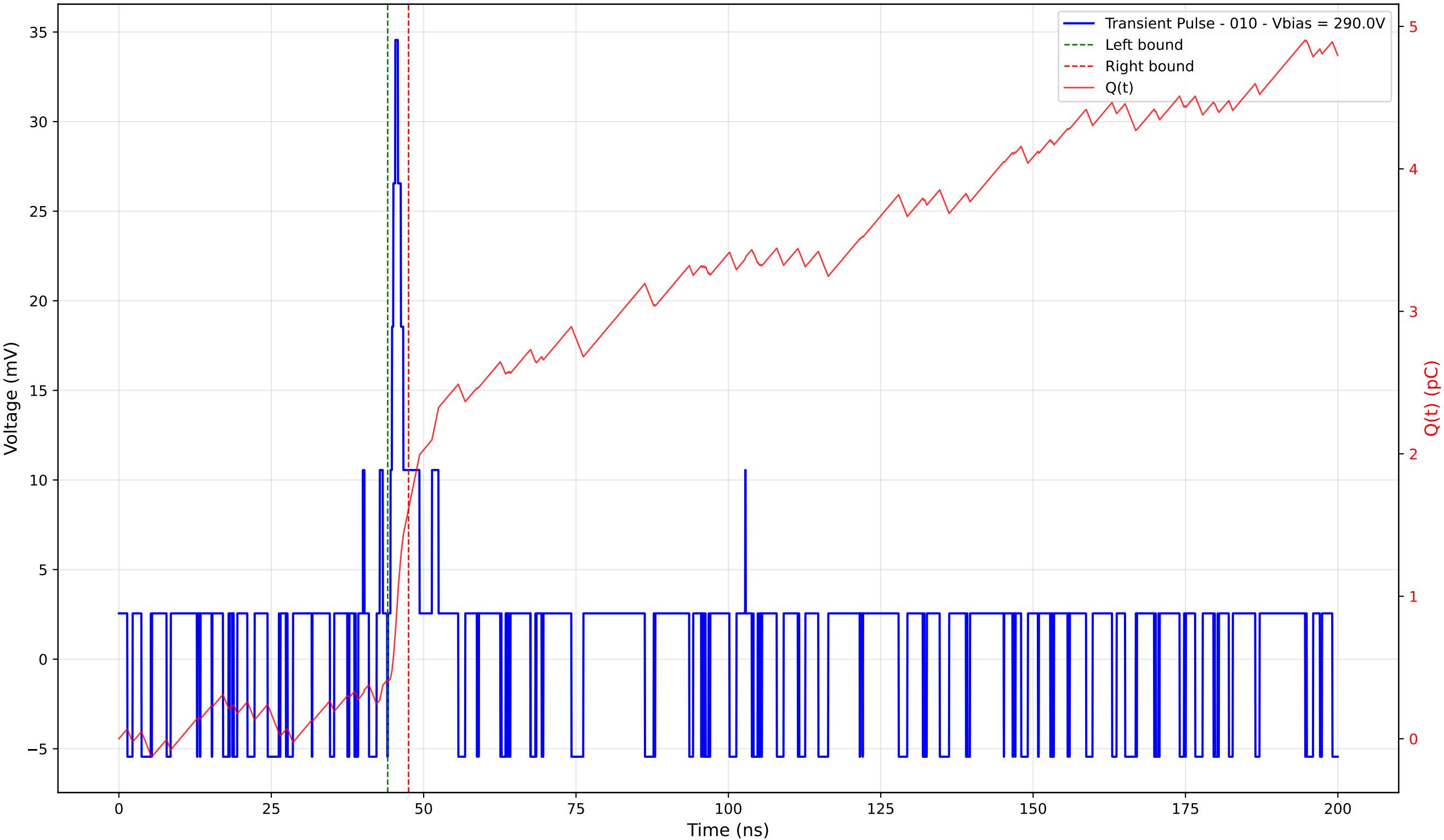
Transient Pulse - Sample: 4003 - Position: 75.0 \mu\text{m} - Charge: 1.21 pC - Rise Time: 0.80 ns
