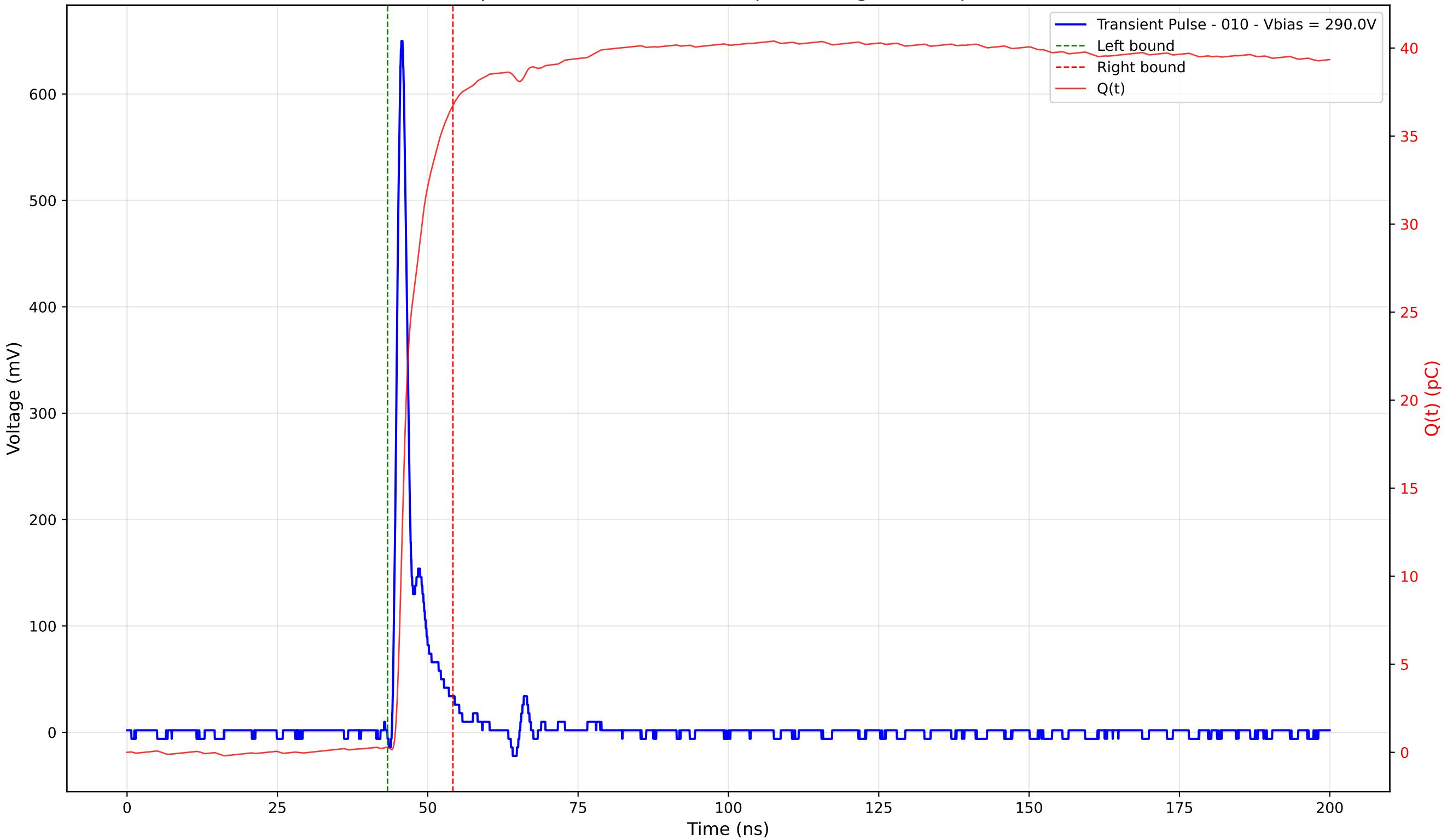
Transient Pulse - Sample: 4003 - Position: 195.0 \mu\text{m} - Charge: 36.45 pC - Rise Time: 1.02 ns
