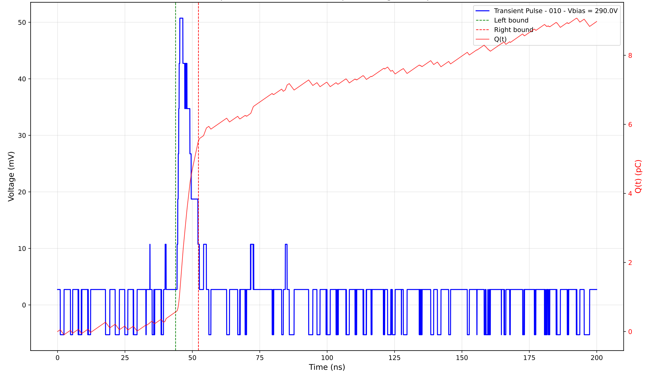
Transient Pulse - Sample: 4003 - Position: 410.0 \mu\text{m} - Charge: 4.95 pC - Rise Time: 1.01 ns
