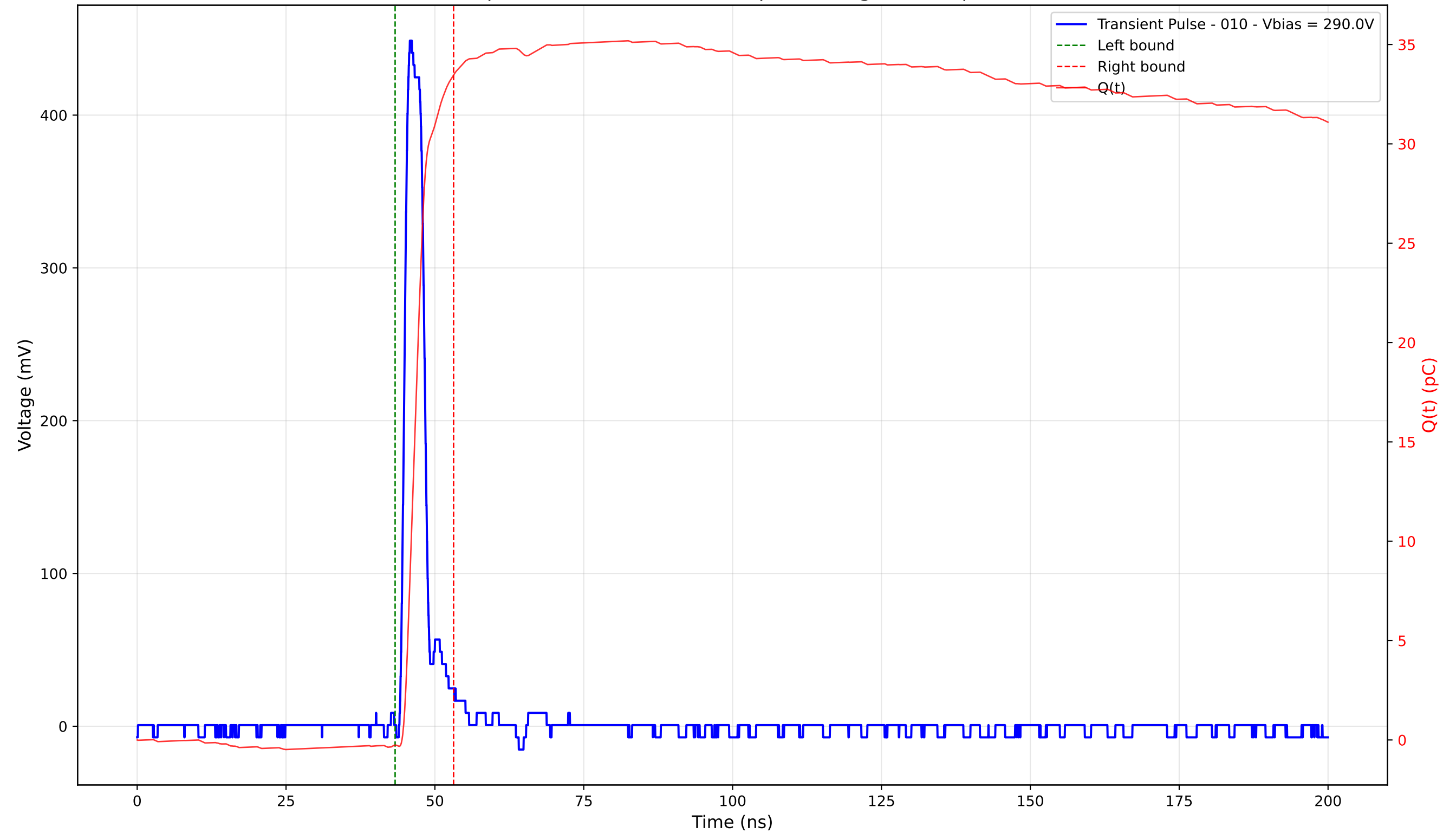
Transient Pulse - Sample: 4003 - Position: 305.0 \mu\text{m} - Charge: 33.73 pC - Rise Time: 1.13 ns
