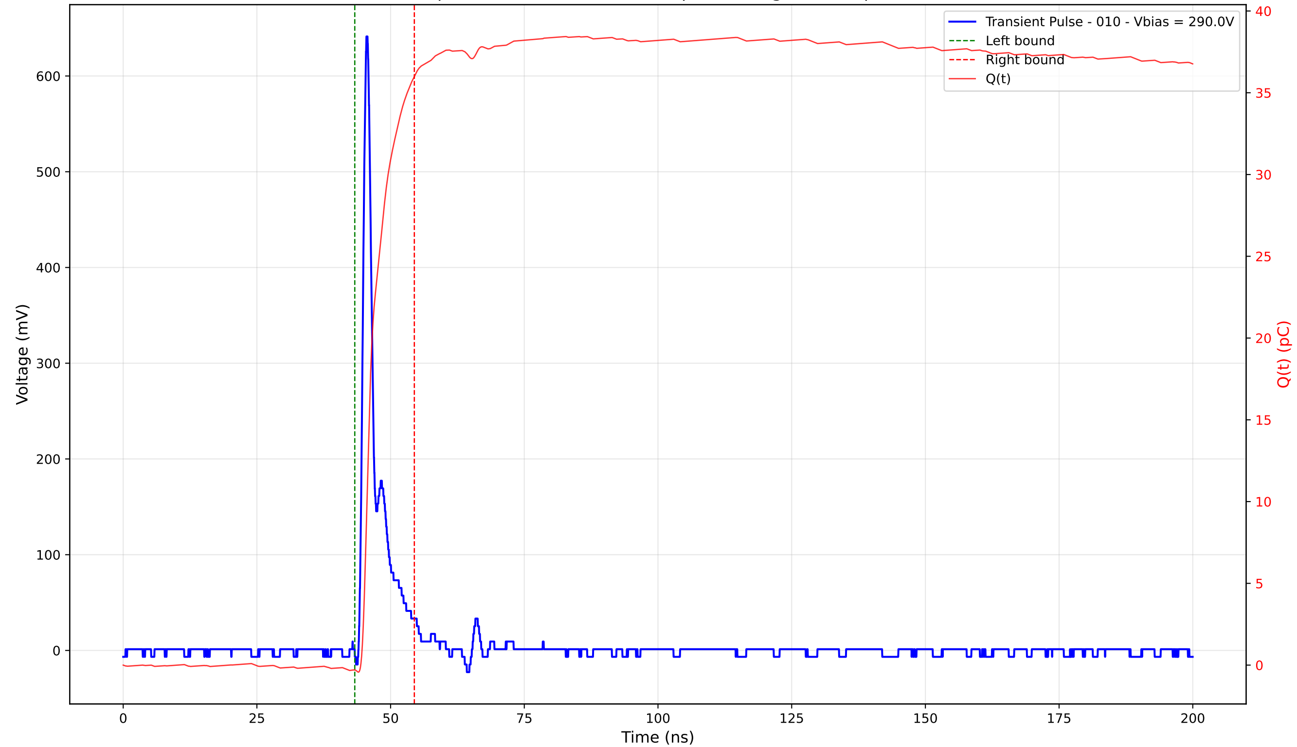
Transient Pulse - Sample: 4003 - Position: 170.0 \mu\text{m} - Charge: 36.29 pC - Rise Time: 0.98 ns
