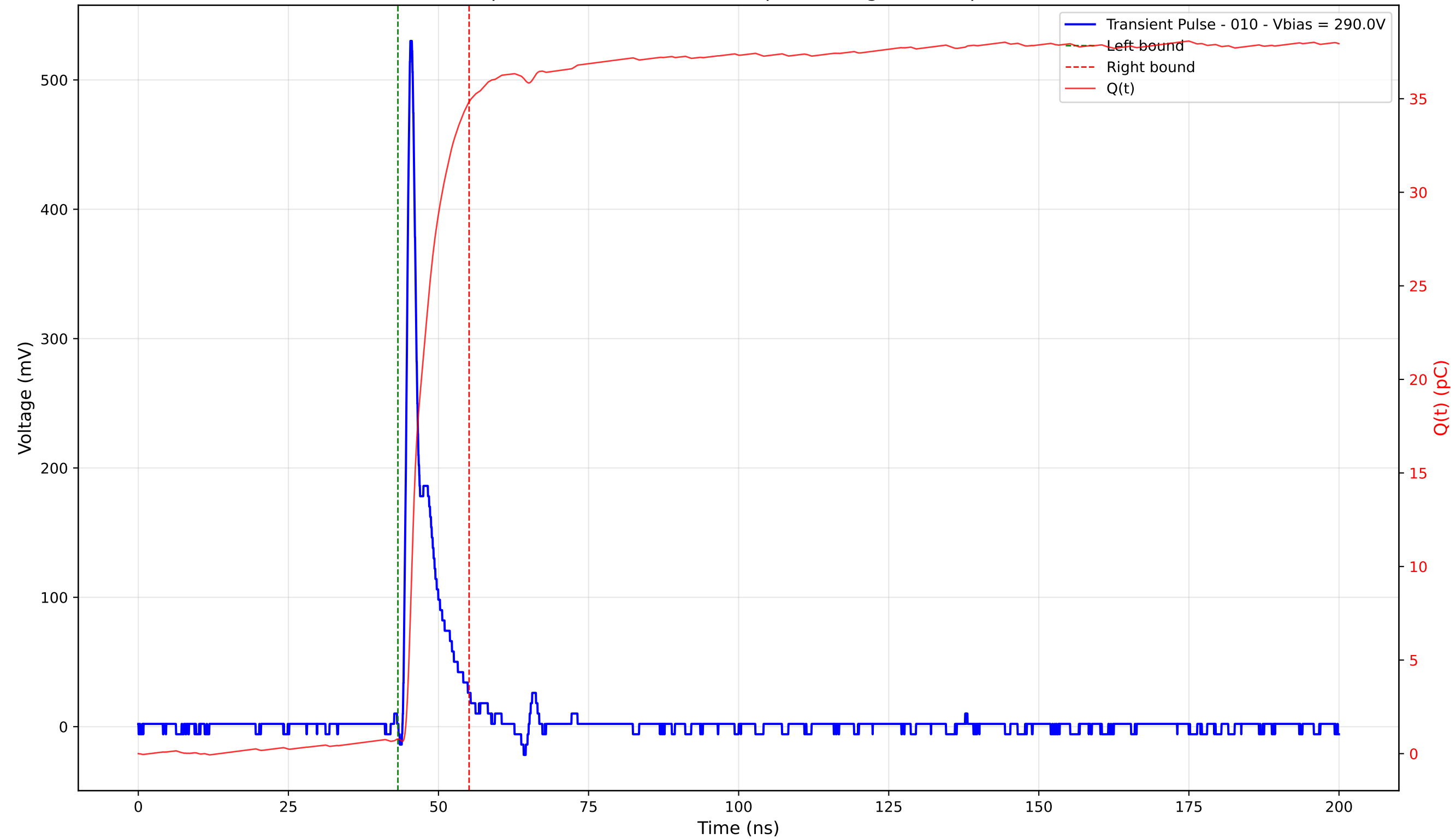
Transient Pulse - Sample: 4003 - Position: 115.0 \mu\text{m} - Charge: 34.05 pC - Rise Time: 0.88 ns
