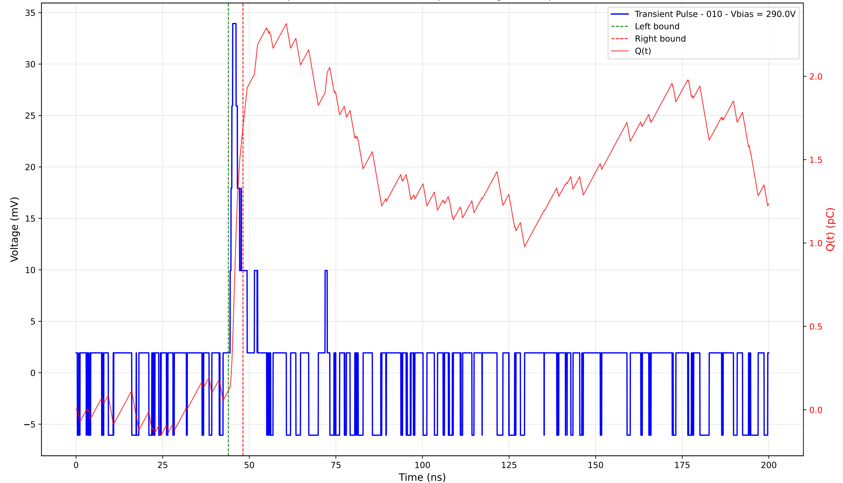
Transient Pulse - Sample: 4003 - Position: 30.0 \mu\text{m} - Charge: 1.58 pC - Rise Time: 0.76 ns
