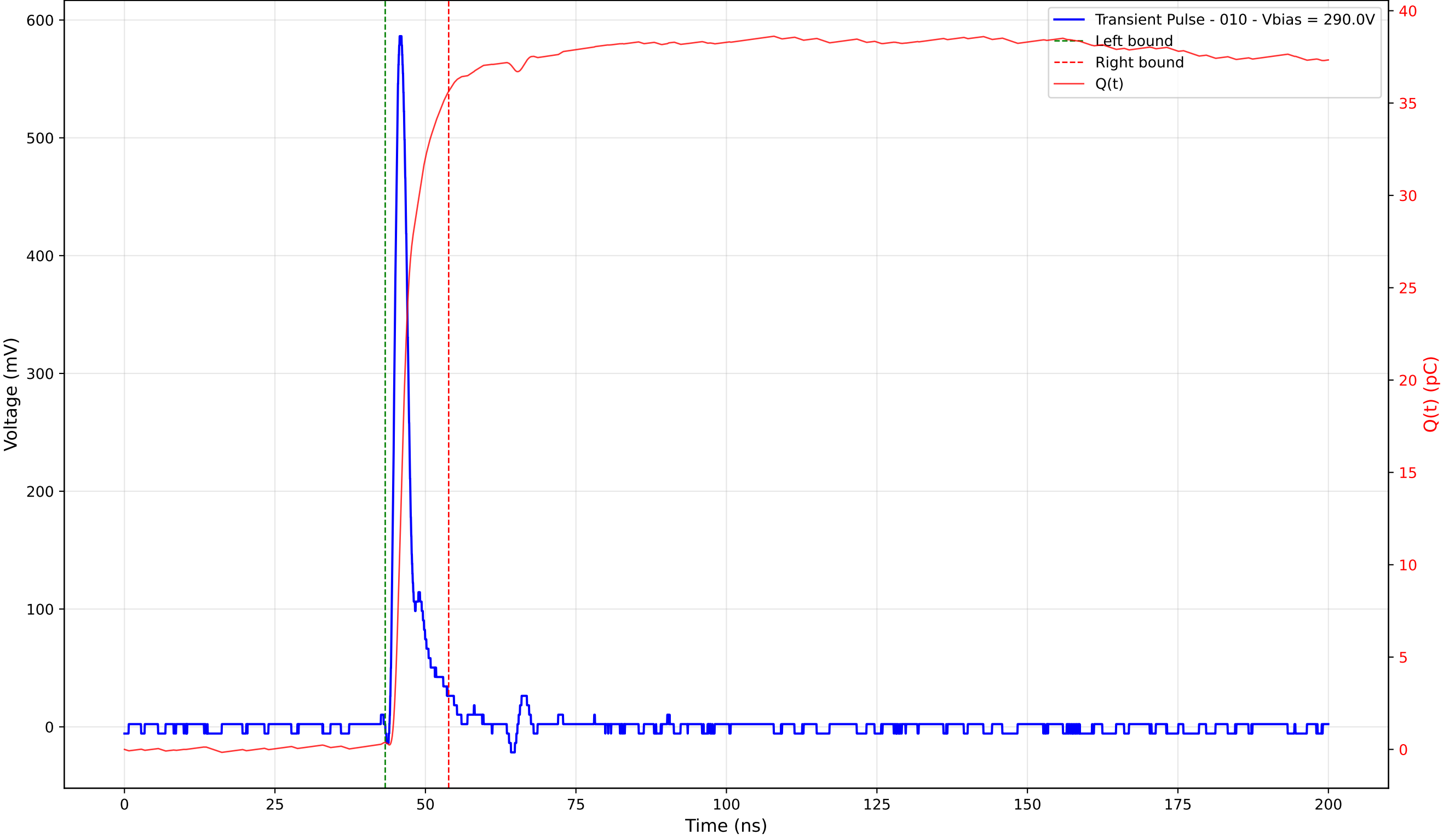
Transient Pulse - Sample: 4003 - Position: 235.0 \mu\text{m} - Charge: 35.26 pC - Rise Time: 1.08 ns
