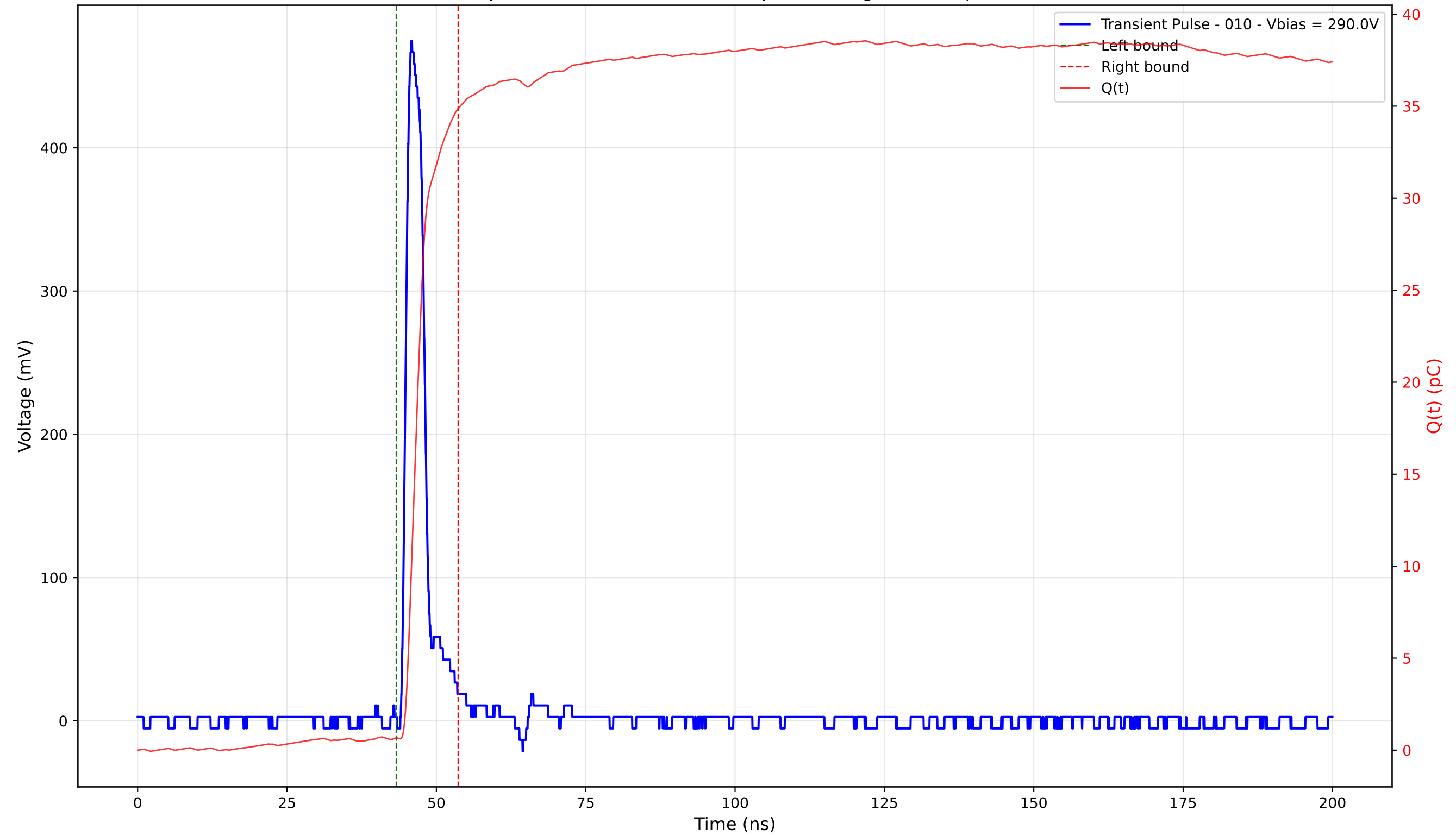
Transient Pulse - Sample: 4003 - Position: 290.0 \mu\text{m} - Charge: 34.21 pC - Rise Time: 1.15 ns
