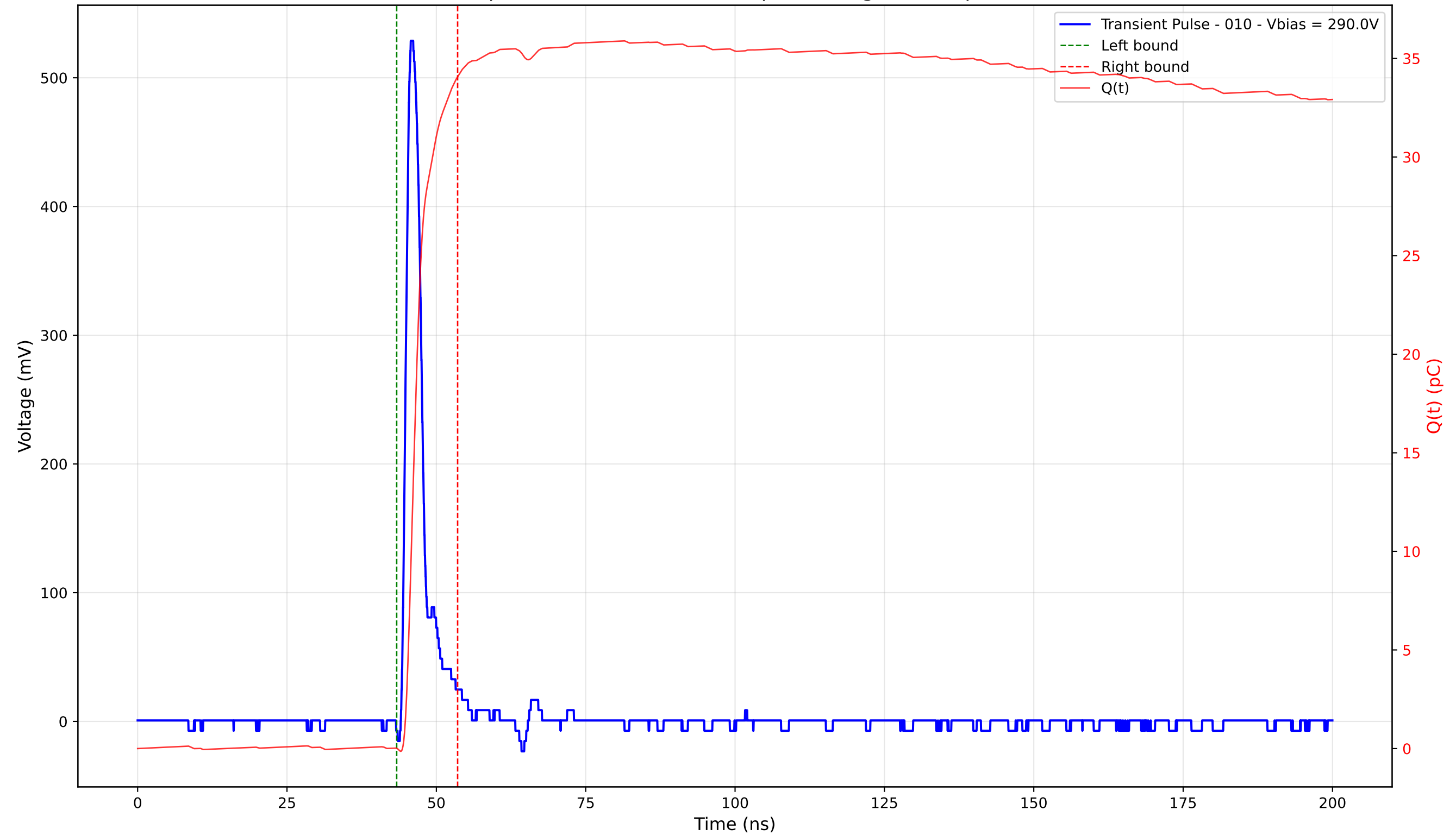
Transient Pulse - Sample: 4003 - Position: 260.0 \mu\text{m} - Charge: 34.06 pC - Rise Time: 1.09 ns
