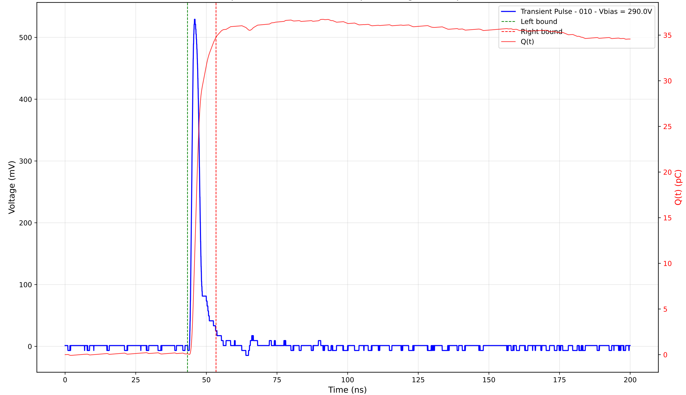
Transient Pulse - Sample: 4003 - Position: 265.0 \mu\text{m} - Charge: 34.67 pC - Rise Time: 1.10 ns
