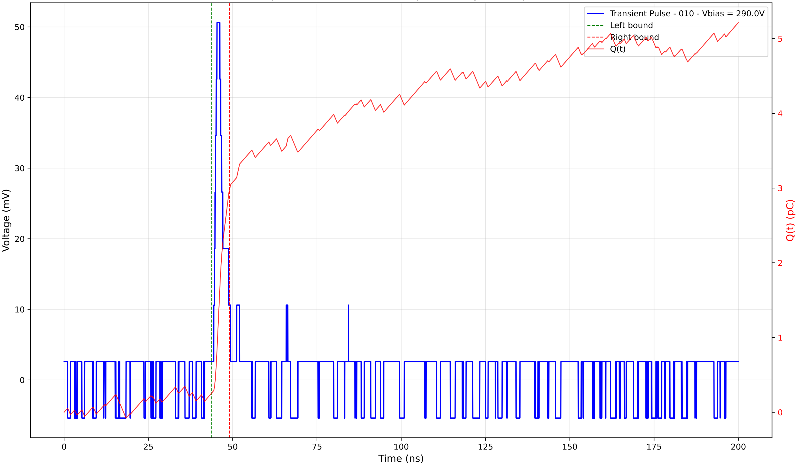
Transient Pulse - Sample: 4003 - Position: 45.0 \mu\text{m} - Charge: 2.72 pC - Rise Time: 0.95 ns
