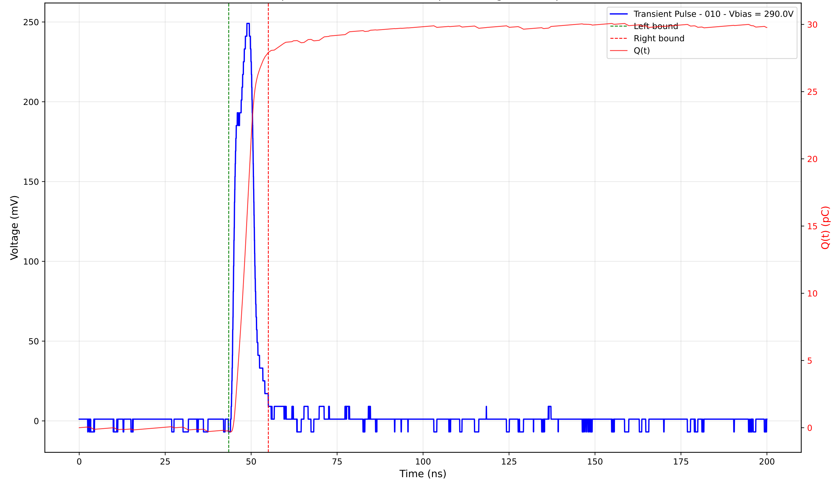
Transient Pulse - Sample: 4003 - Position: 385.0 \mu\text{m} - Charge: 28.16 pC - Rise Time: 3.36 ns
