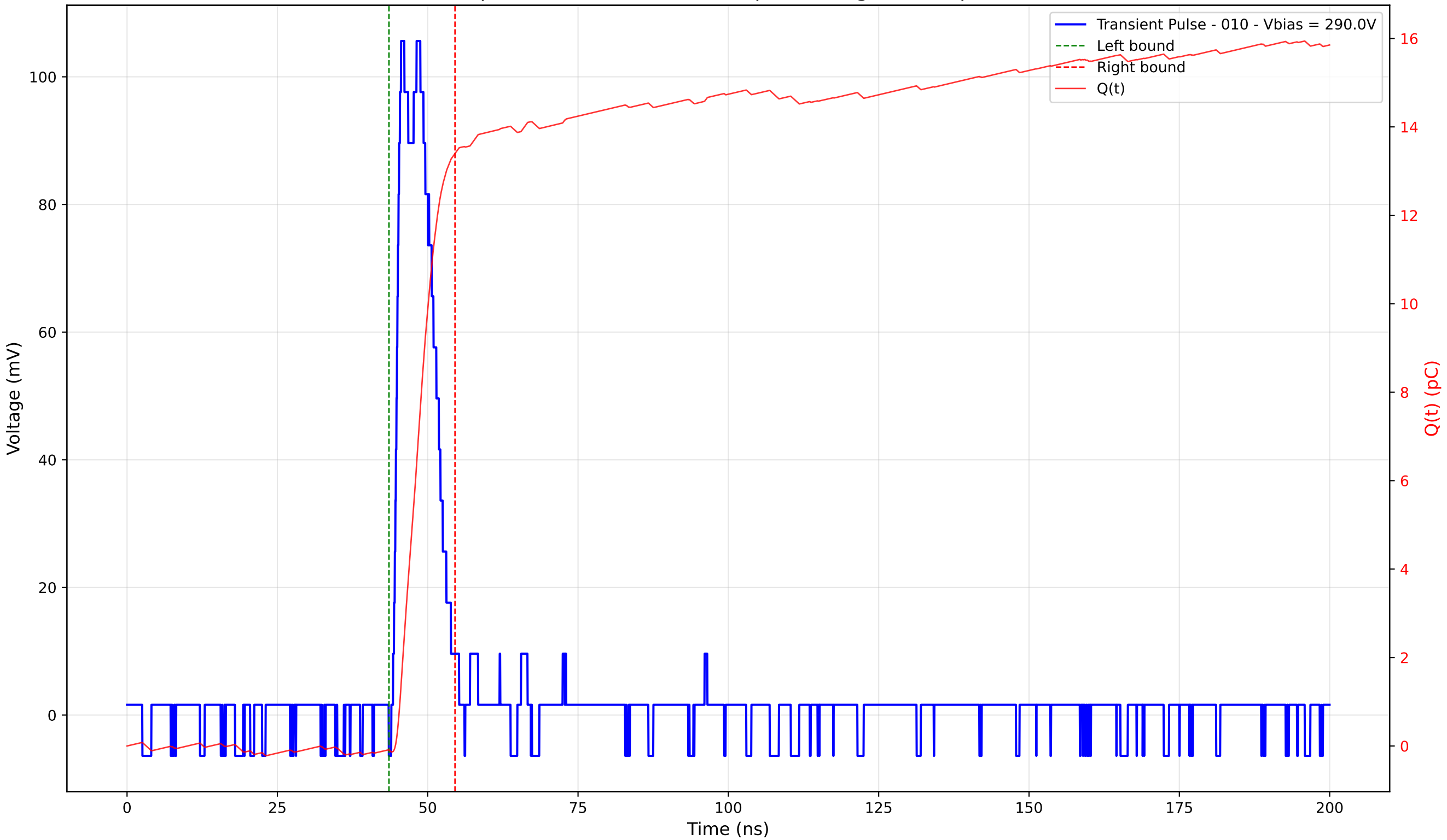
Transient Pulse - Sample: 4003 - Position: 400.0 \mu\text{m} - Charge: 13.49 pC - Rise Time: 1.00 ns
