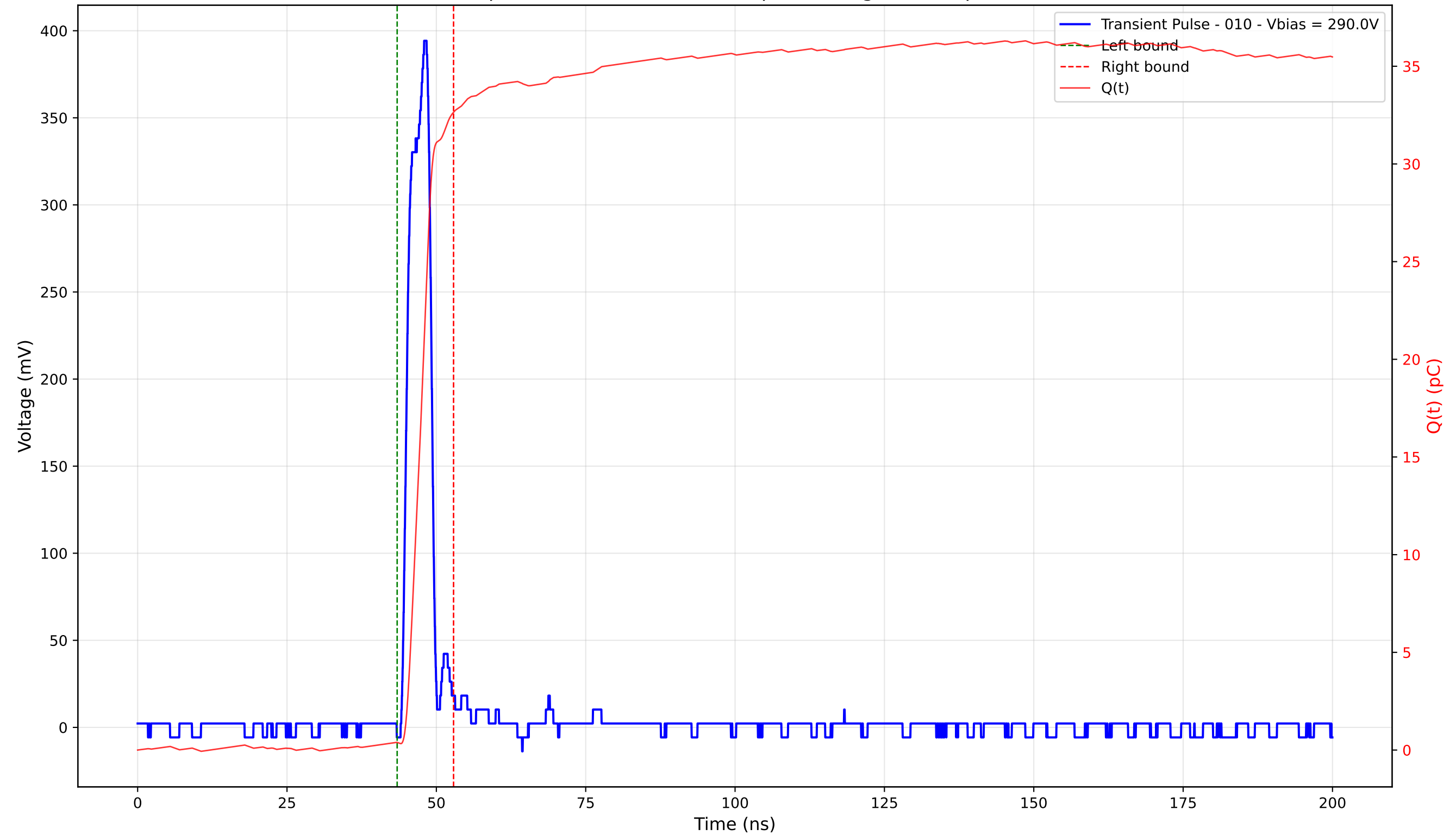
Transient Pulse - Sample: 4003 - Position: 350.0 \mu\text{m} - Charge: 32.26 pC - Rise Time: 3.03 ns
