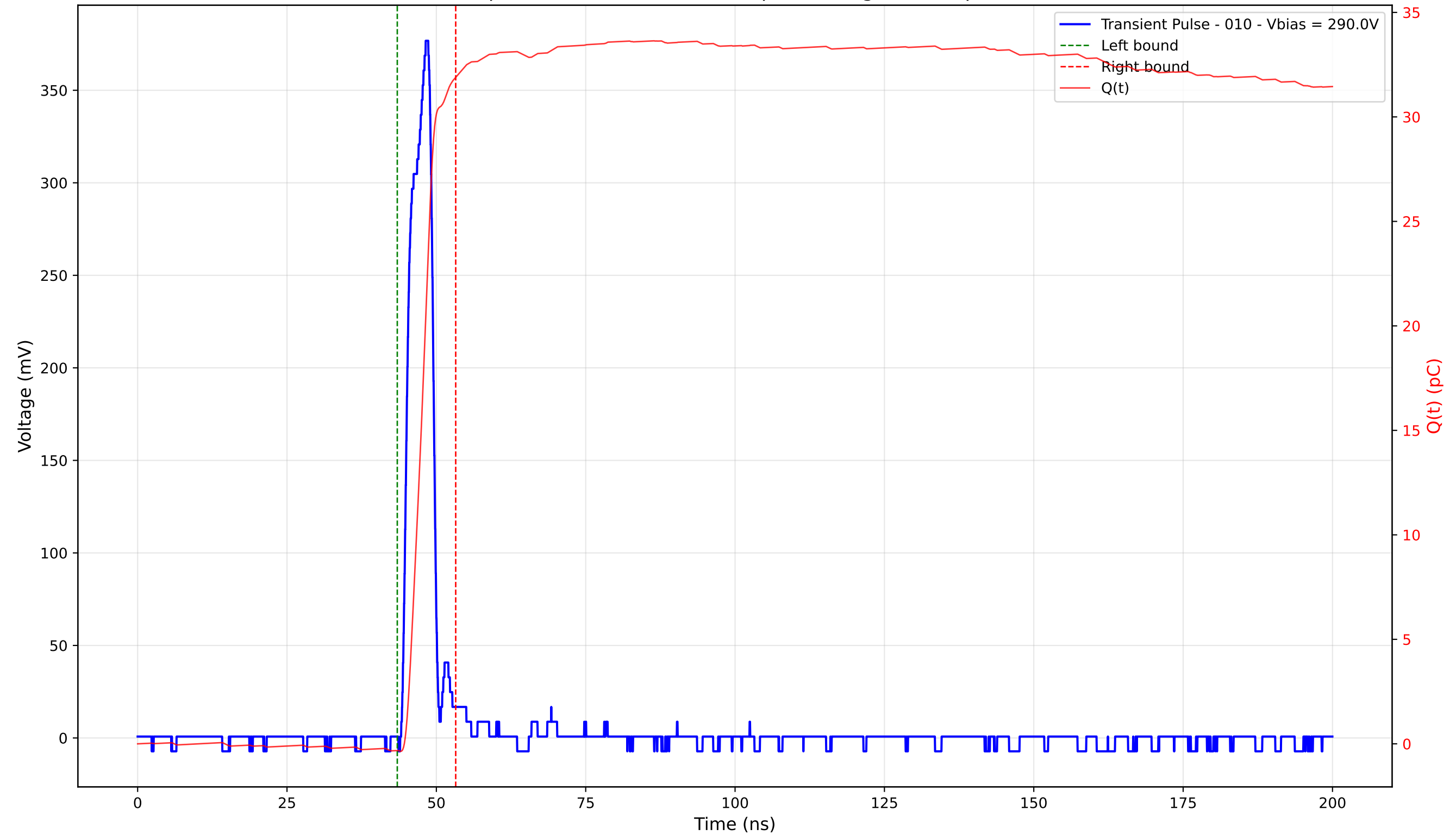
Transient Pulse - Sample: 4003 - Position: 360.0 \mu\text{m} - Charge: 32.21 pC - Rise Time: 3.13 ns
