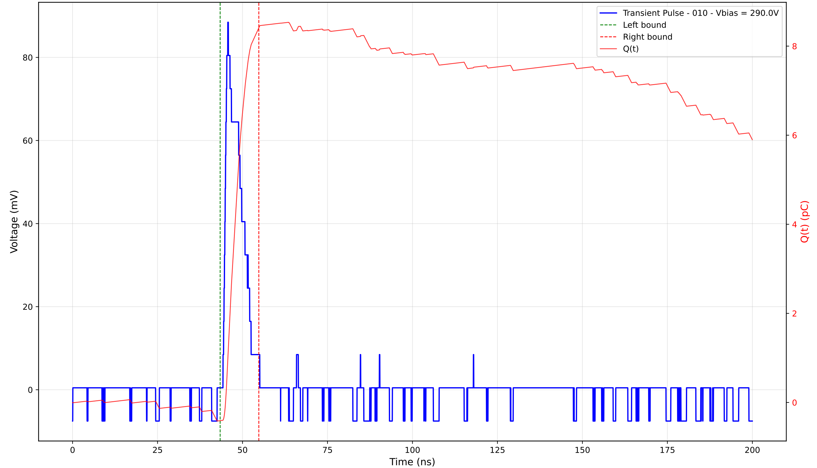
Transient Pulse - Sample: 4003 - Position: 405.0 \mu\text{m} - Charge: 8.82 pC - Rise Time: 0.94 ns
