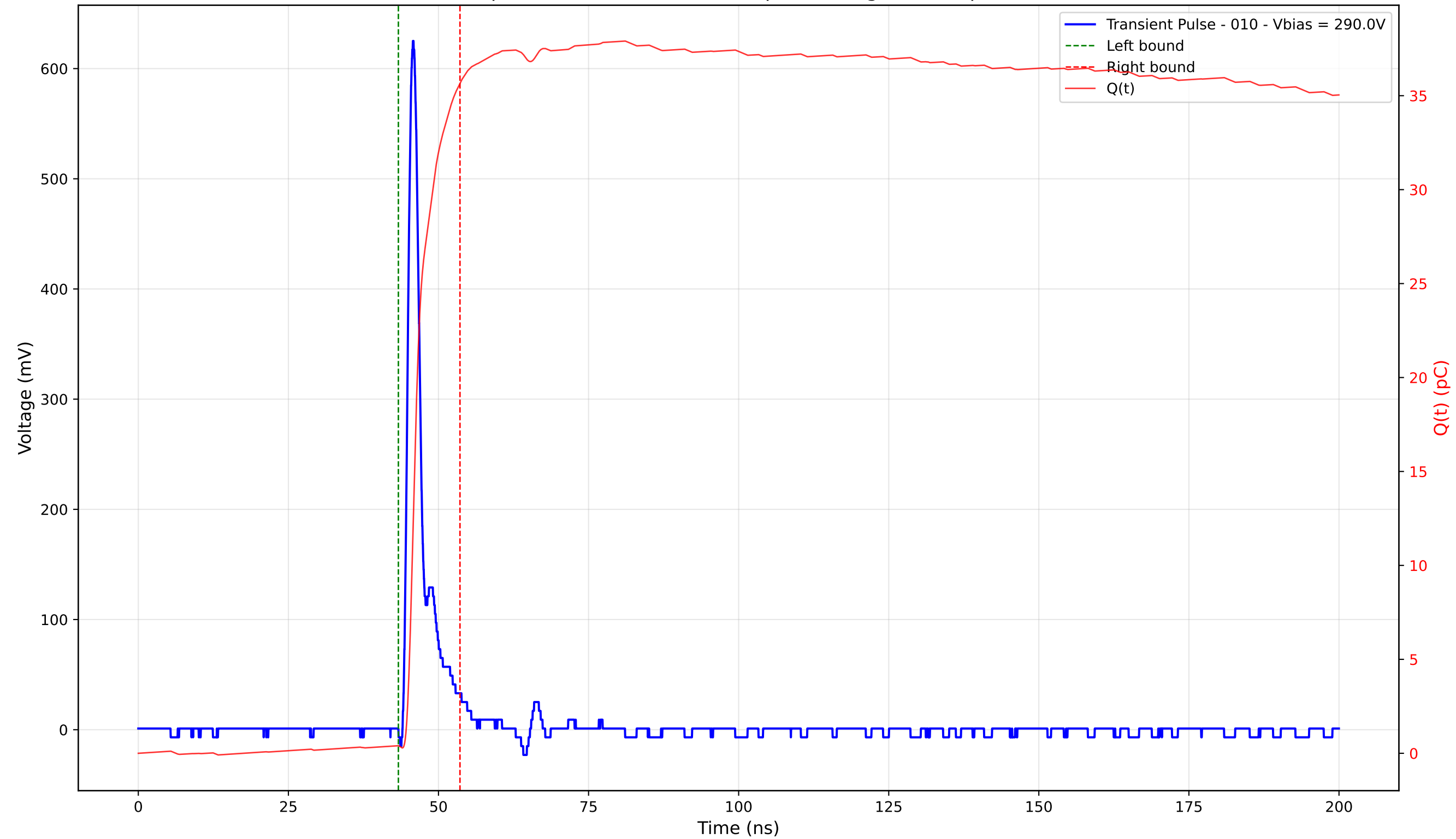
Transient Pulse - Sample: 4003 - Position: 215.0 \mu\text{m} - Charge: 35.25 pC - Rise Time: 1.09 ns
