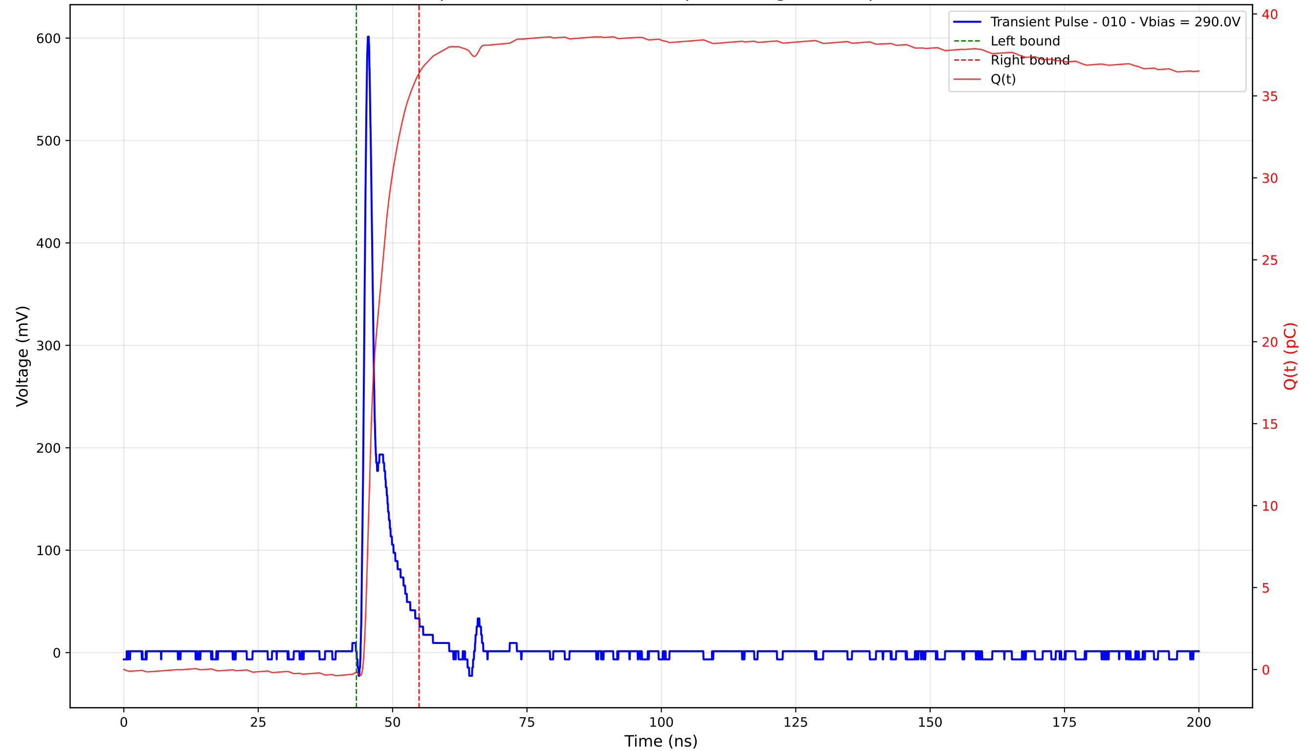
Transient Pulse - Sample: 4003 - Position: 130.0 \mu\text{m} - Charge: 36.57 pC - Rise Time: 0.88 ns
