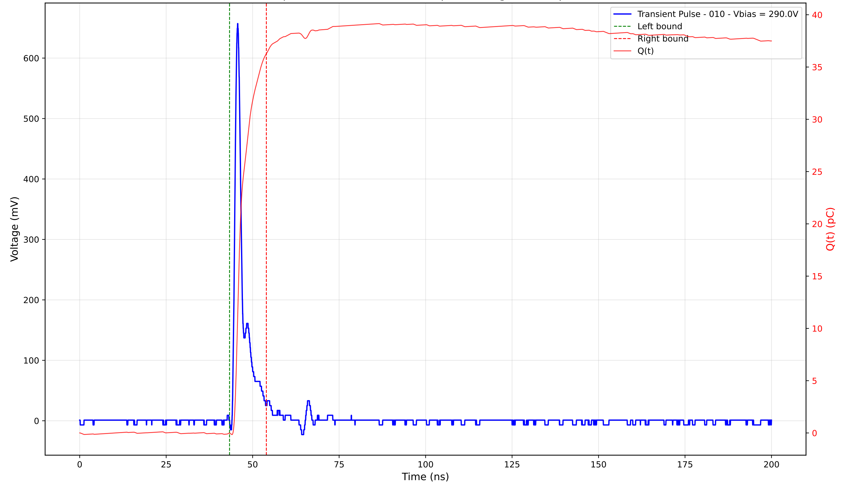
Transient Pulse - Sample: 4003 - Position: 190.0 \mu\text{m} - Charge: 36.28 pC - Rise Time: 1.01 ns
