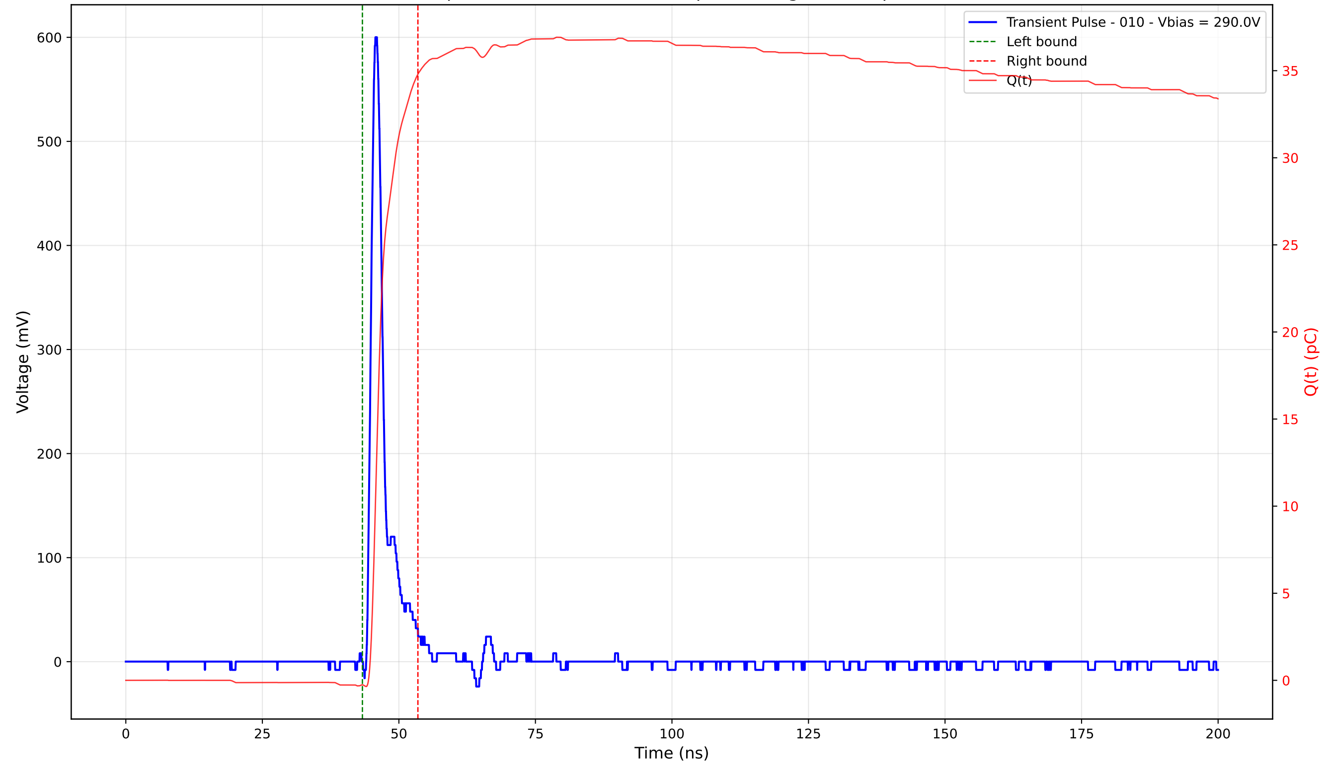
Transient Pulse - Sample: 4003 - Position: 225.0 \mu\text{m} - Charge: 35.07 pC - Rise Time: 1.06 ns
