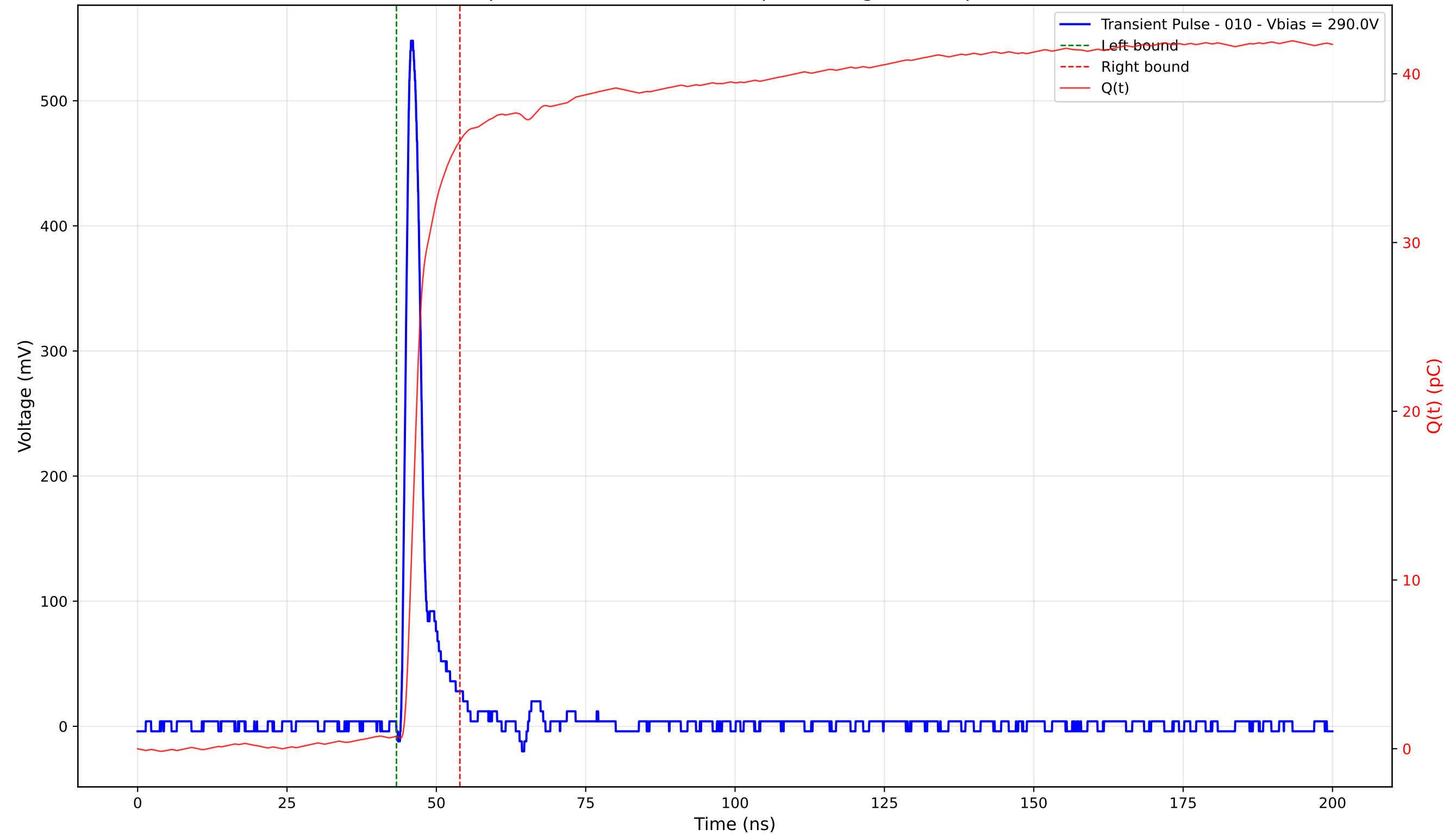
Transient Pulse - Sample: 4003 - Position: 255.0 \mu\text{m} - Charge: 35.29 pC - Rise Time: 1.11 ns
