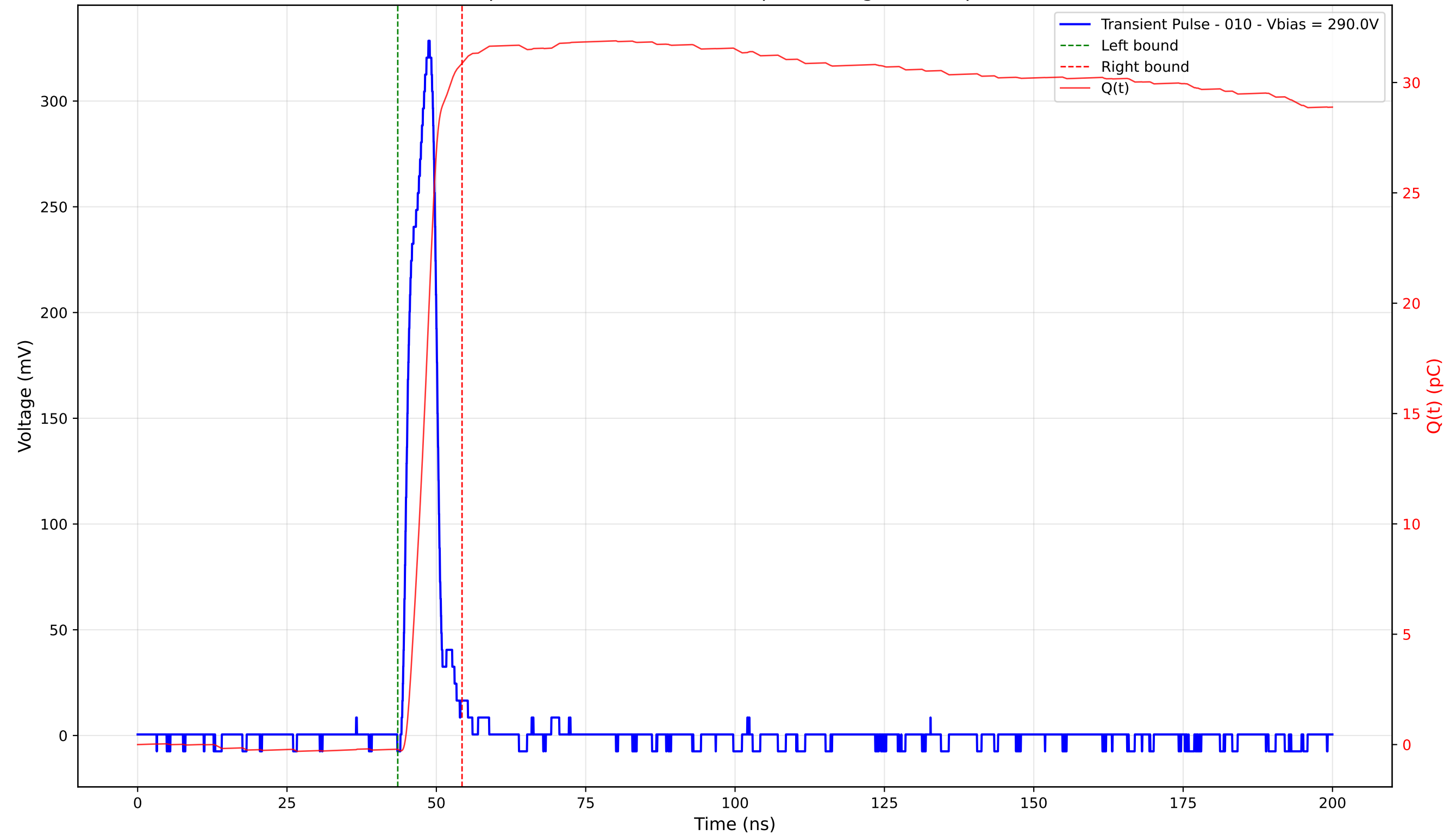
Transient Pulse - Sample: 4003 - Position: 375.0 \mu\text{m} - Charge: 31.09 pC - Rise Time: 3.26 ns
